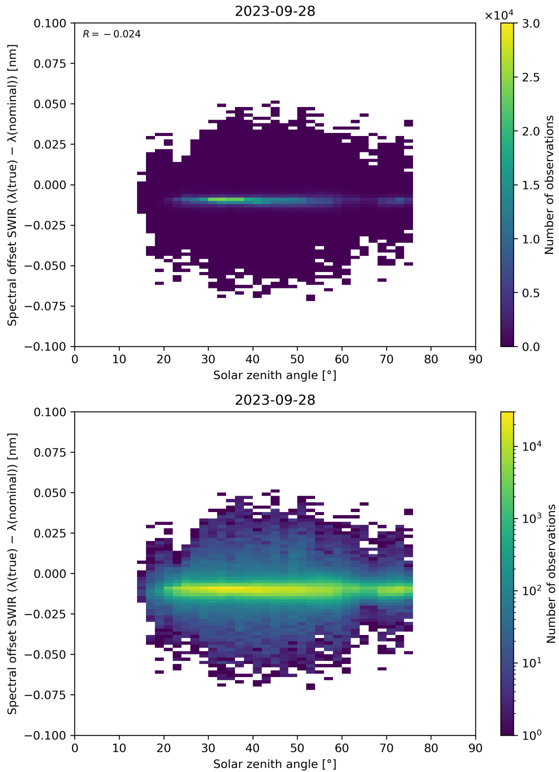
Figure 104: Scatter density plot of “Solar zenith angle” against “Spectral offset SWIR ( \lambda(\text{true}) - \lambda(\text{nominal}) )” for 2023-09-27 to 2023-09-29.
