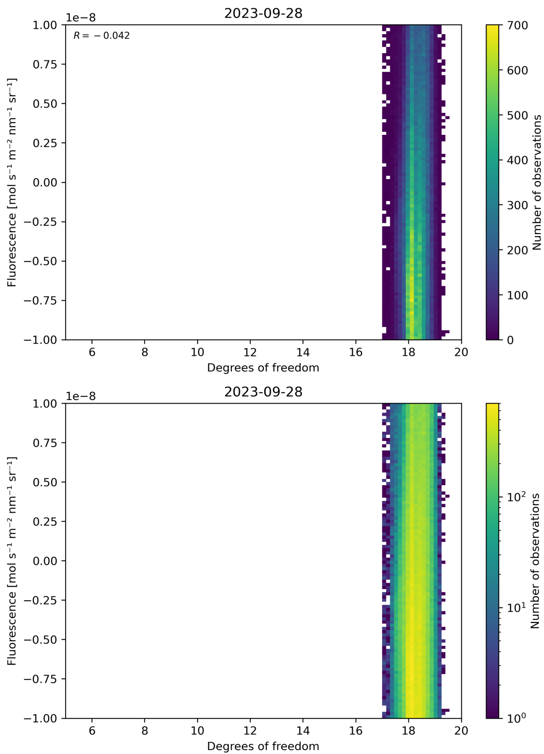
Figure 51: Scatter density plot of “Degrees of freedom” against “Fluorescence” for 2023-09-27 to 2023-09-29.
