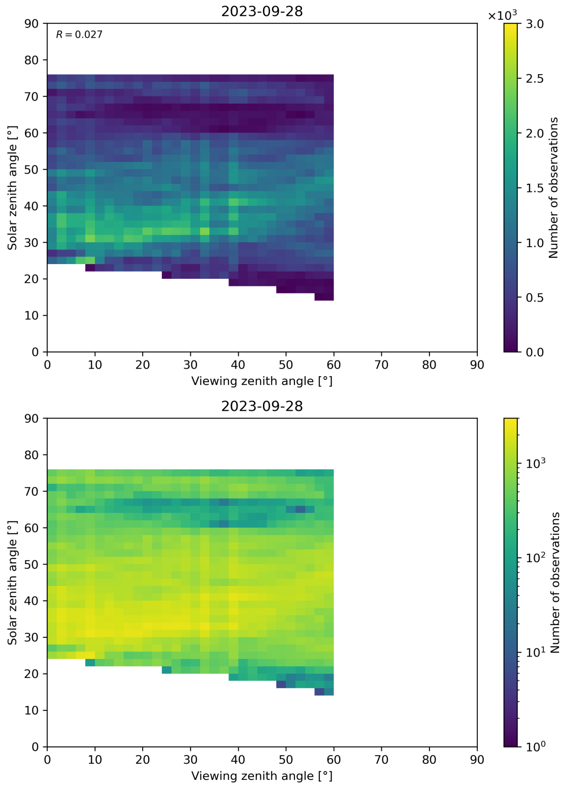
Figure 115: Scatter density plot of “Viewing zenith angle” against “Solar zenith angle” for 2023-09-27 to 2023-09-29.
