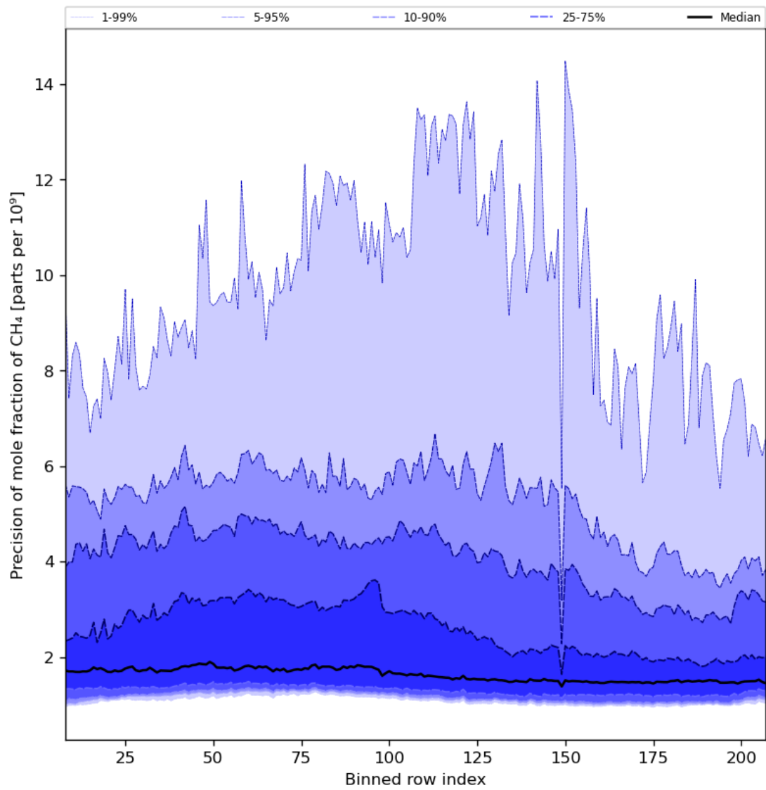
Figure 35: Along track statistics of “Precision of mole fraction of CH 4 ” for 2023-09-27 to 2023-09-29
