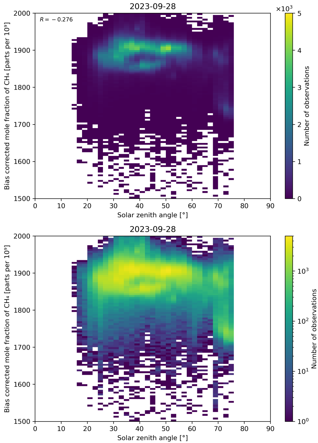
Figure 100: Scatter density plot of “Solar zenith angle” against “Bias corrected mole fraction of \text{CH}_4 ” for 2023-09-27 to 2023-09-29.
