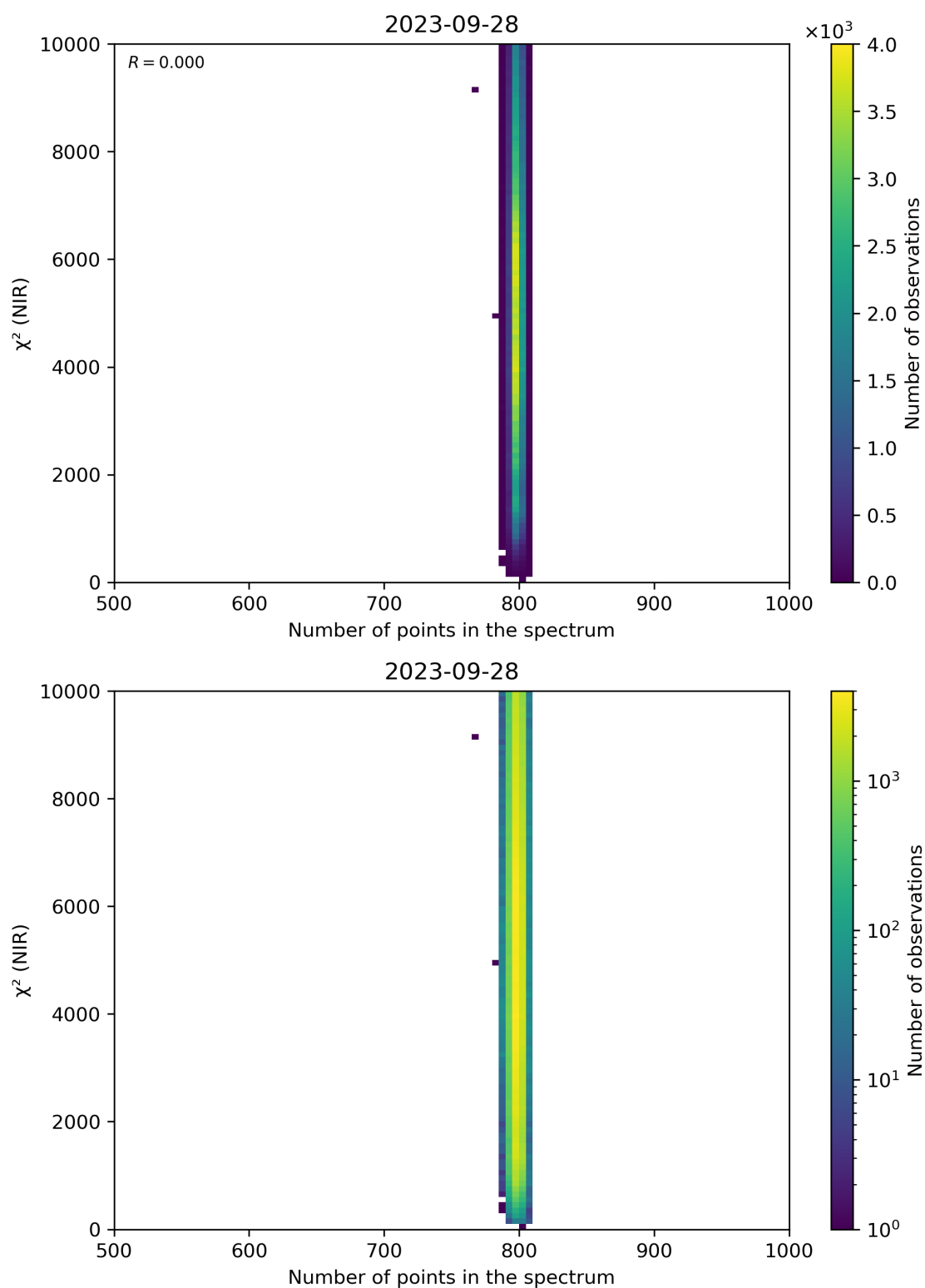
Figure 88: Scatter density plot of “Number of points in the spectrum” against “ \chi^2 (NIR)” for 2023-09-27 to 2023-09-29.
