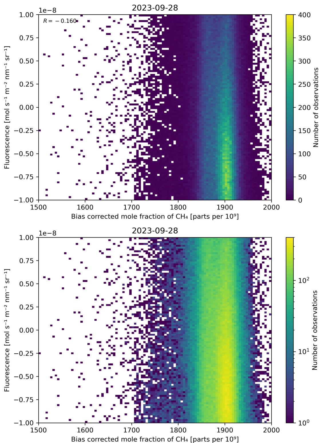
Figure 66: Scatter density plot of “Bias corrected mole fraction of \text{CH}_4 ” against “Fluorescence” for 2023-09-27 to 2023-09-29.
