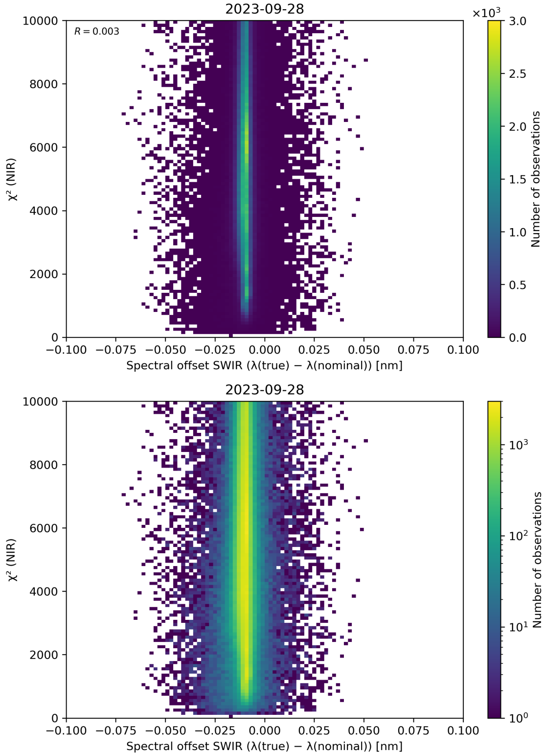
Figure 117: Scatter density plot of “Spectral offset SWIR ( \lambda(\text{true}) - \lambda(\text{nominal}) )” against “ \chi^2 (NIR)” for 2023-09-27 to 2023-09-29.
