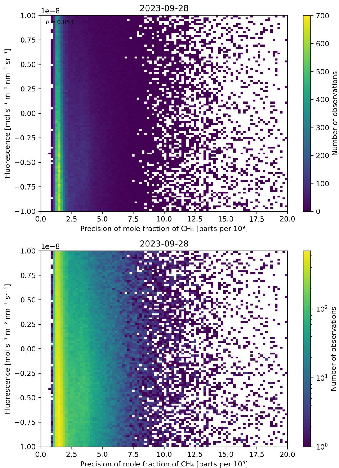
Figure 81: Scatter density plot of “Precision of mole fraction of \text{CH}_4 ” against “Fluorescence” for 2023-09-27 to 2023-09-29.
