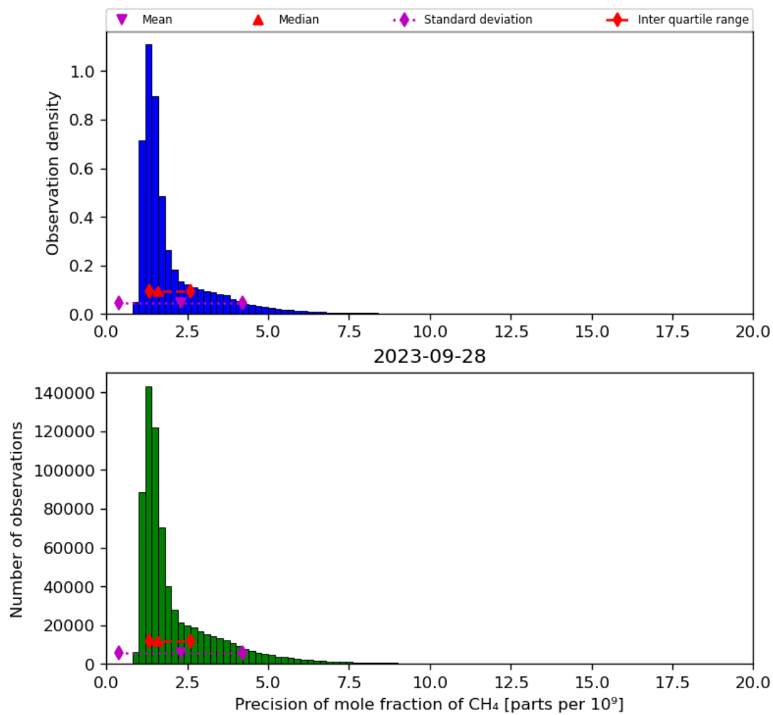
Figure 24: Histogram of “Precision of mole fraction of CH 4 ” for 2023-09-27 to 2023-09-29
