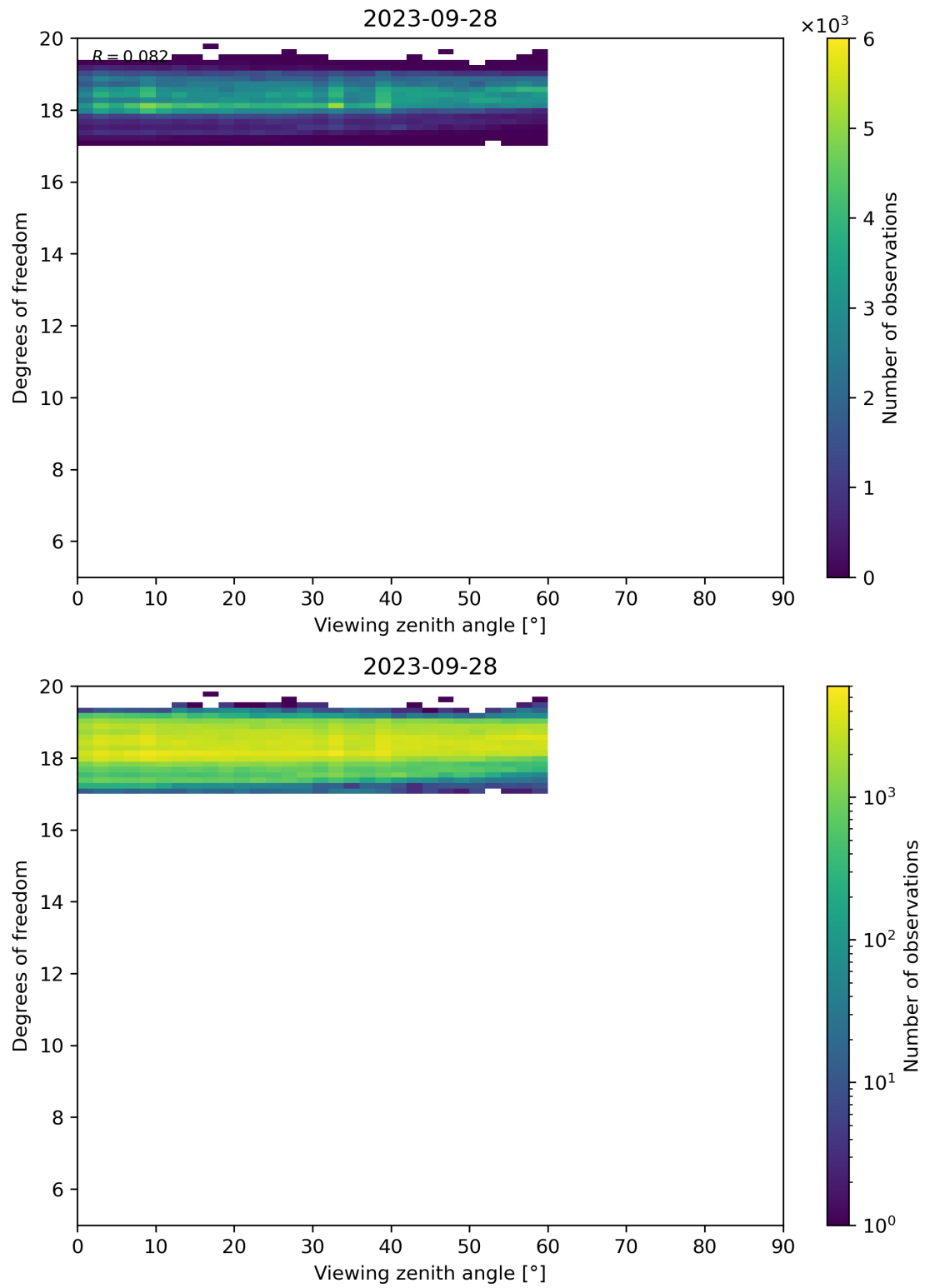
Figure 107: Scatter density plot of “Viewing zenith angle” against “Degrees of freedom” for 2023-09-27 to 2023-09-29.
