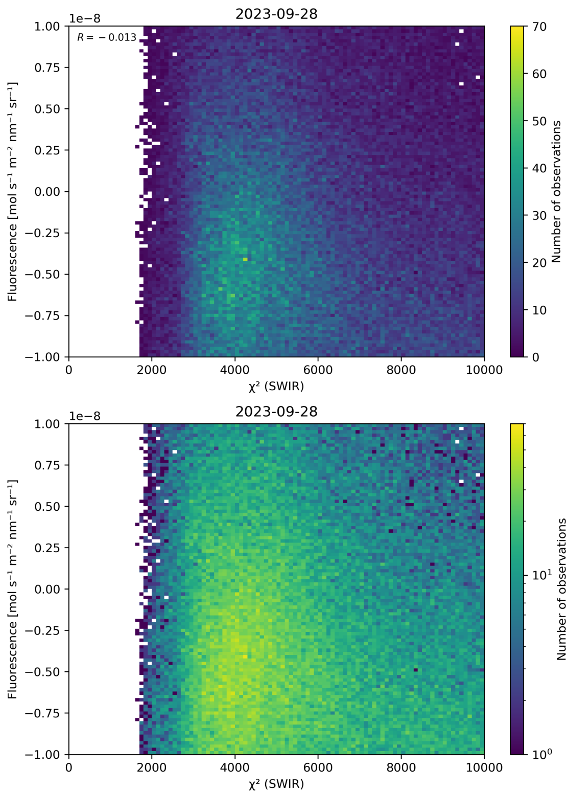
Figure 49: Scatter density plot of “ \chi^2 (SWIR)” against “Fluorescence” for 2023-09-27 to 2023-09-29.
