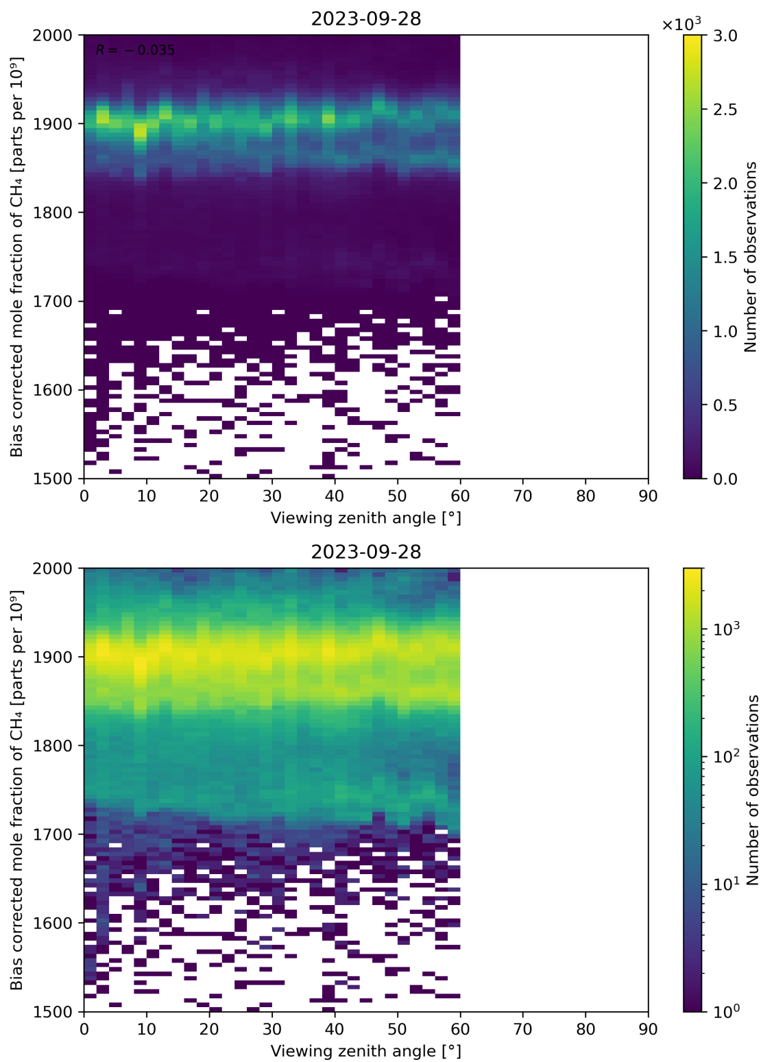
Figure 111: Scatter density plot of “Viewing zenith angle” against “Bias corrected mole fraction of CH 4 ” for 2023-09-27 to 2023-09-29.
