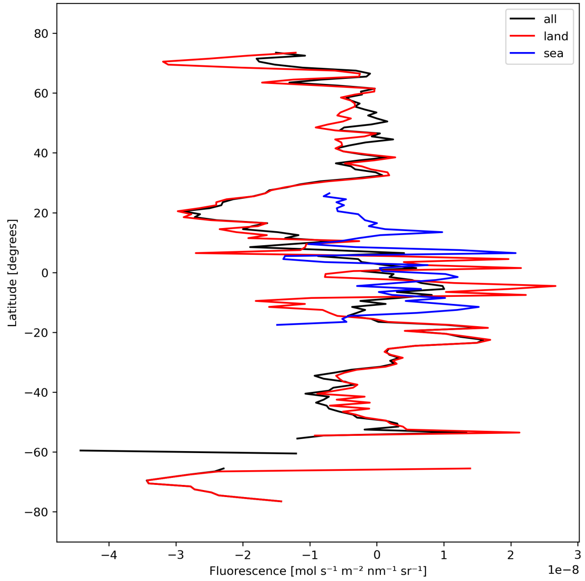
Figure 21: Zonal average of “Fluorescence” for 2023-09-27 to 2023-09-29.
