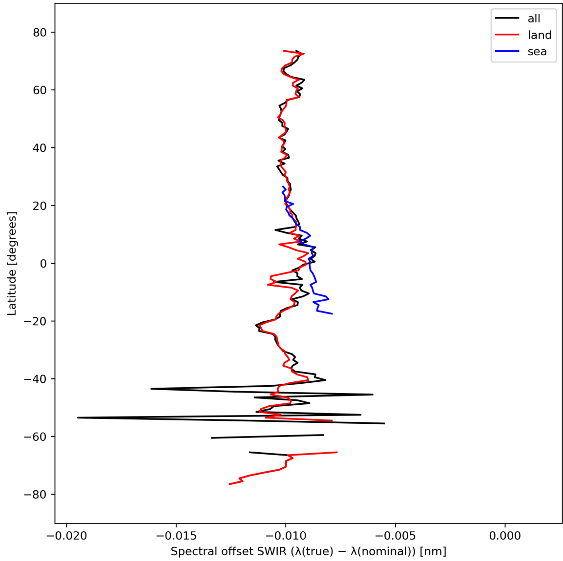
Figure 16: Zonal average of “Spectral offset SWIR ( \lambda(\text{true}) - \lambda(\text{nominal}) )” for 2023-09-27 to 2023-09-29.
