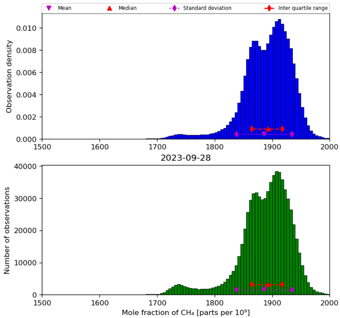
Figure 23: Histogram of “Mole fraction of CH 4 ” for 2023-09-27 to 2023-09-29
