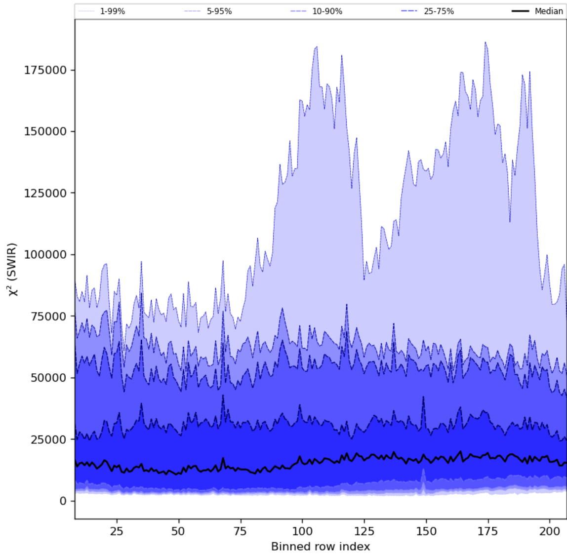
Figure 39: Along track statistics of “ \chi^2 (SWIR)” for 2023-09-27 to 2023-09-29
