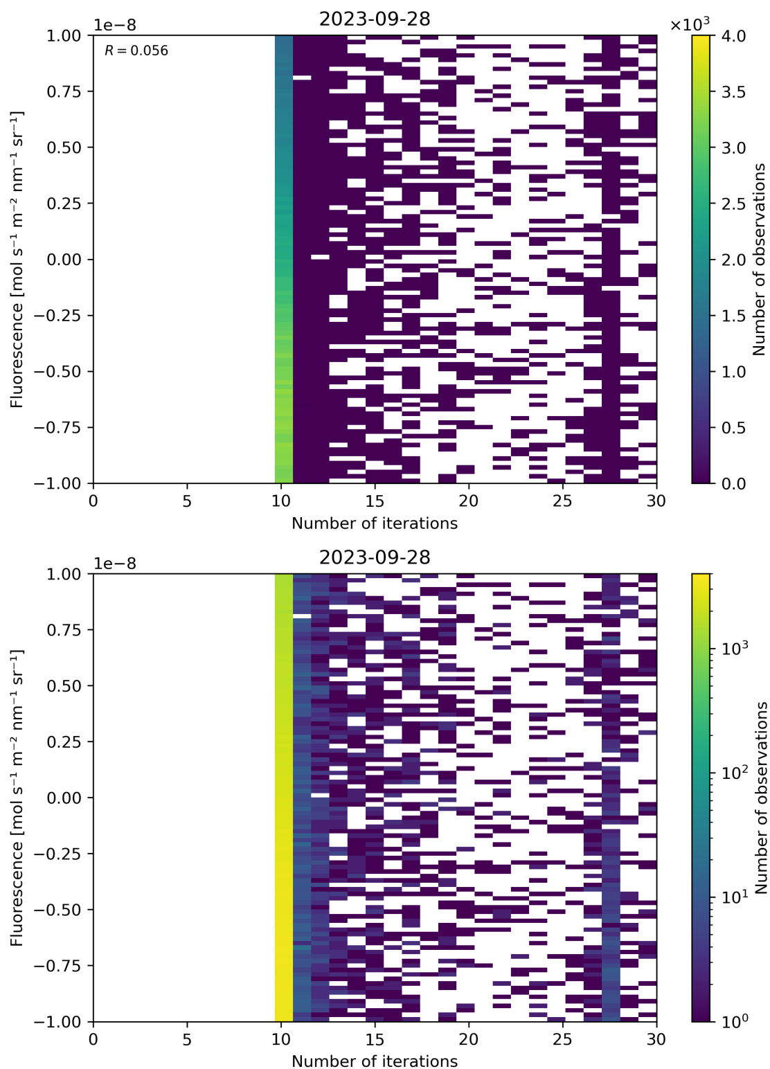
Figure 87: Scatter density plot of “Number of iterations” against “Fluorescence” for 2023-09-27 to 2023-09-29.
