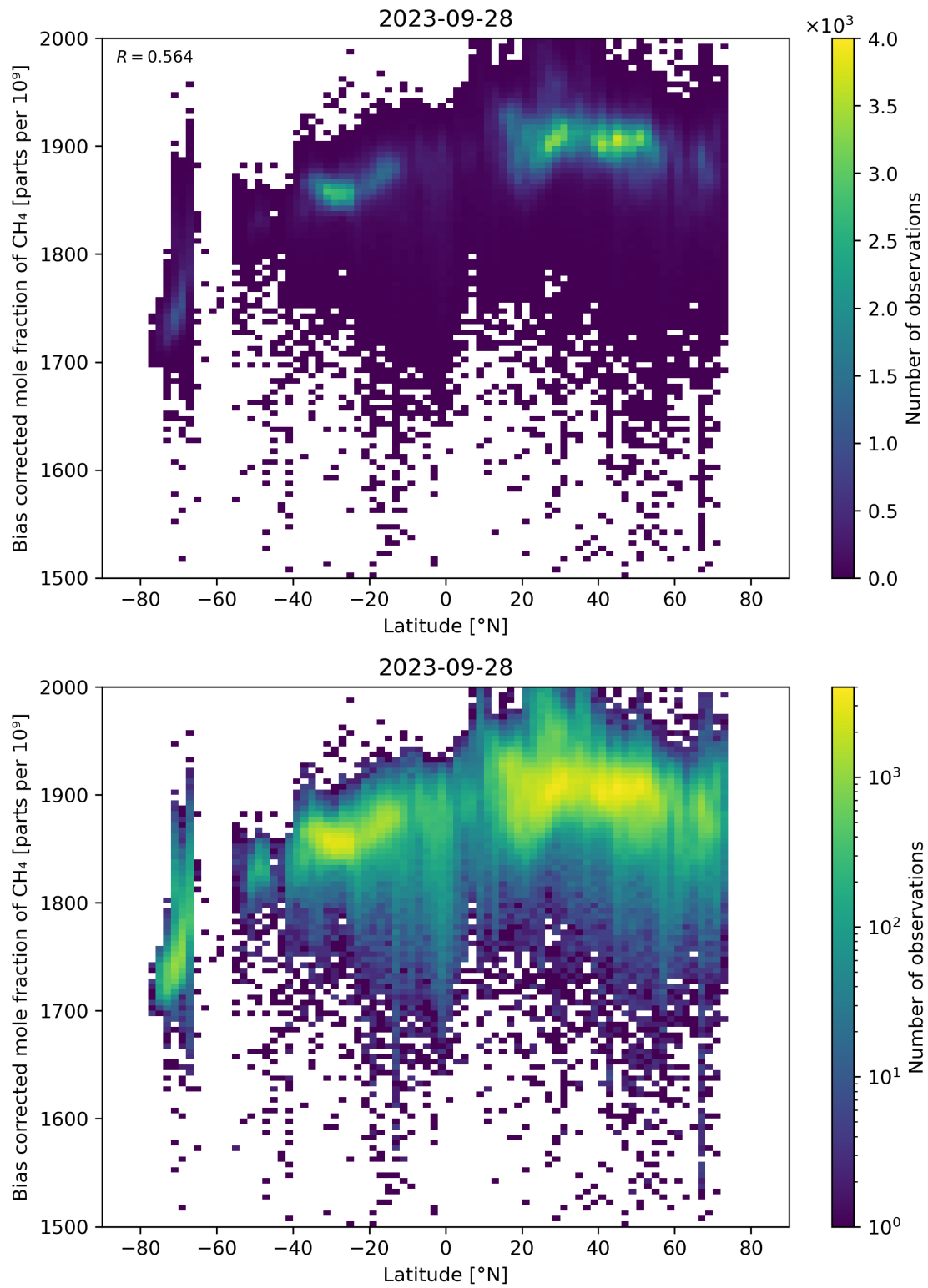
Figure 58: Scatter density plot of “Latitude” against “Bias corrected mole fraction of \text{CH}_4 ” for 2023-09-27 to 2023-09-29.
