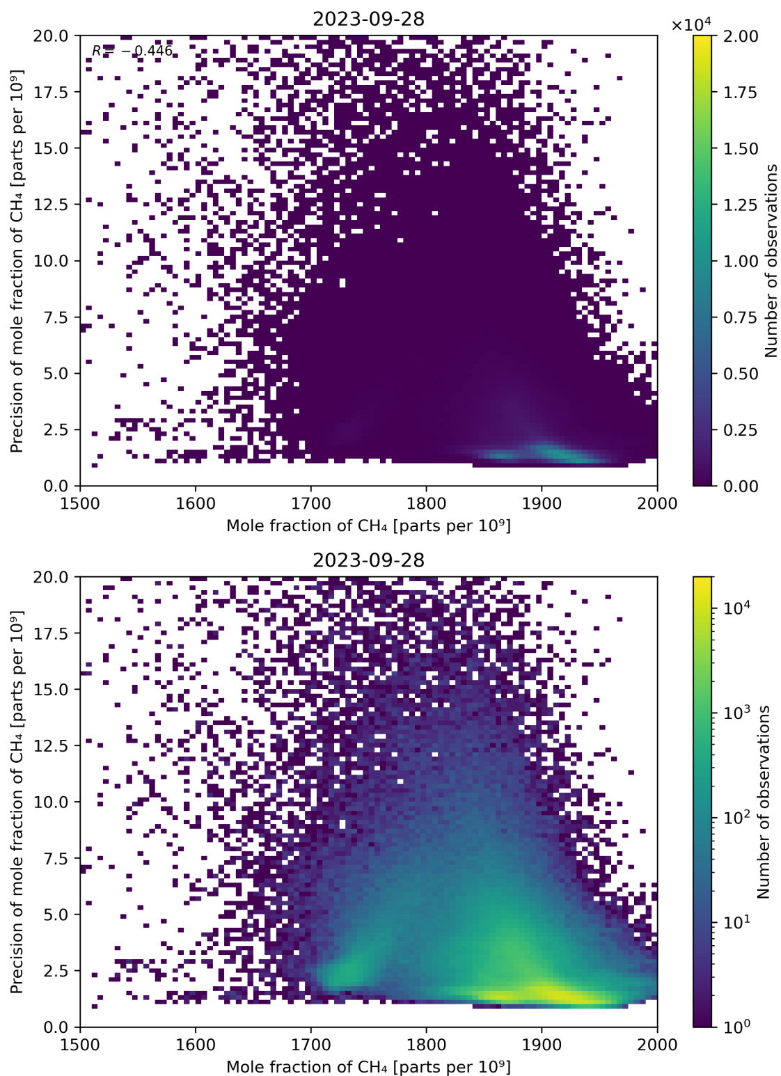
Figure 75: Scatter density plot of “Mole fraction of CH 4 ” against “Precision of mole fraction of CH 4 ” for 2023-09-27 to 2023-09-29.
