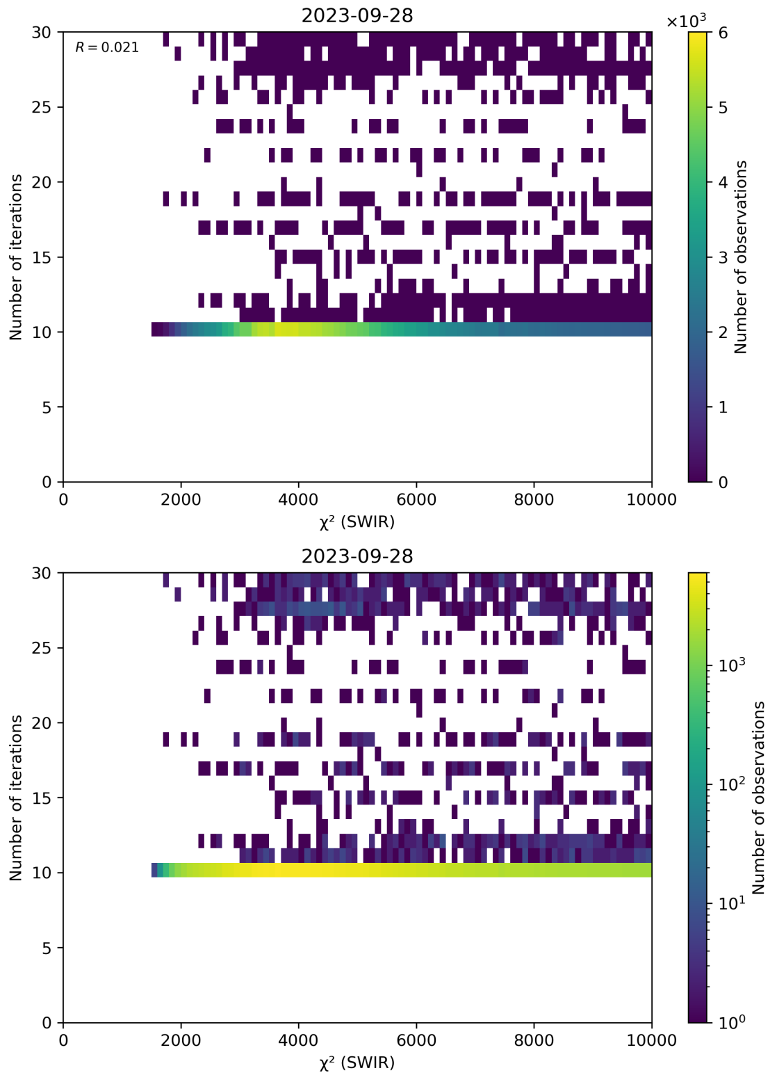
Figure 50: Scatter density plot of “ \chi^2 (SWIR)” against “Number of iterations” for 2023-09-27 to 2023-09-29.
