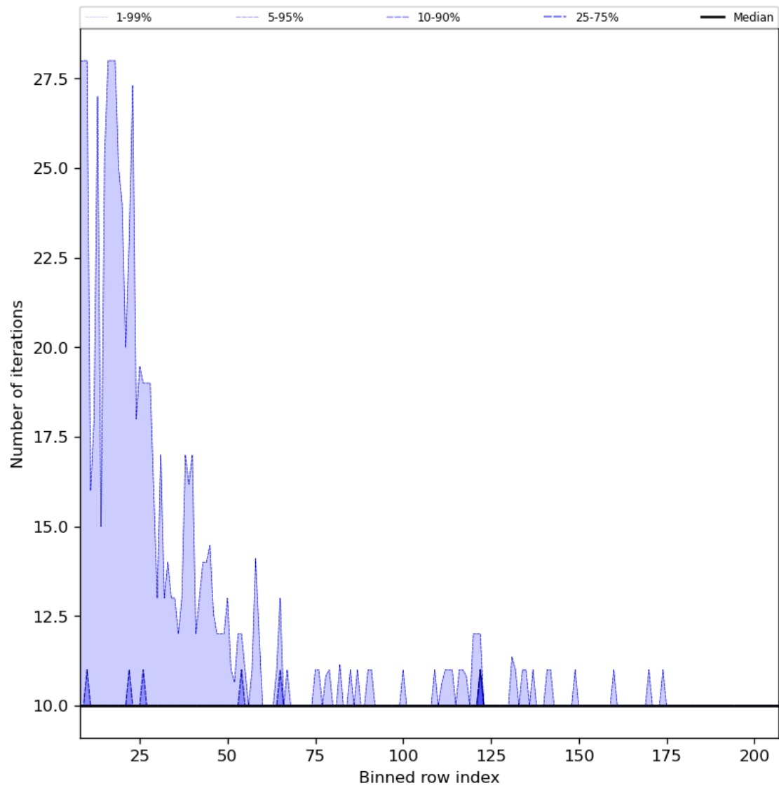
Figure 42: Along track statistics of “Number of iterations” for 2023-09-27 to 2023-09-29
