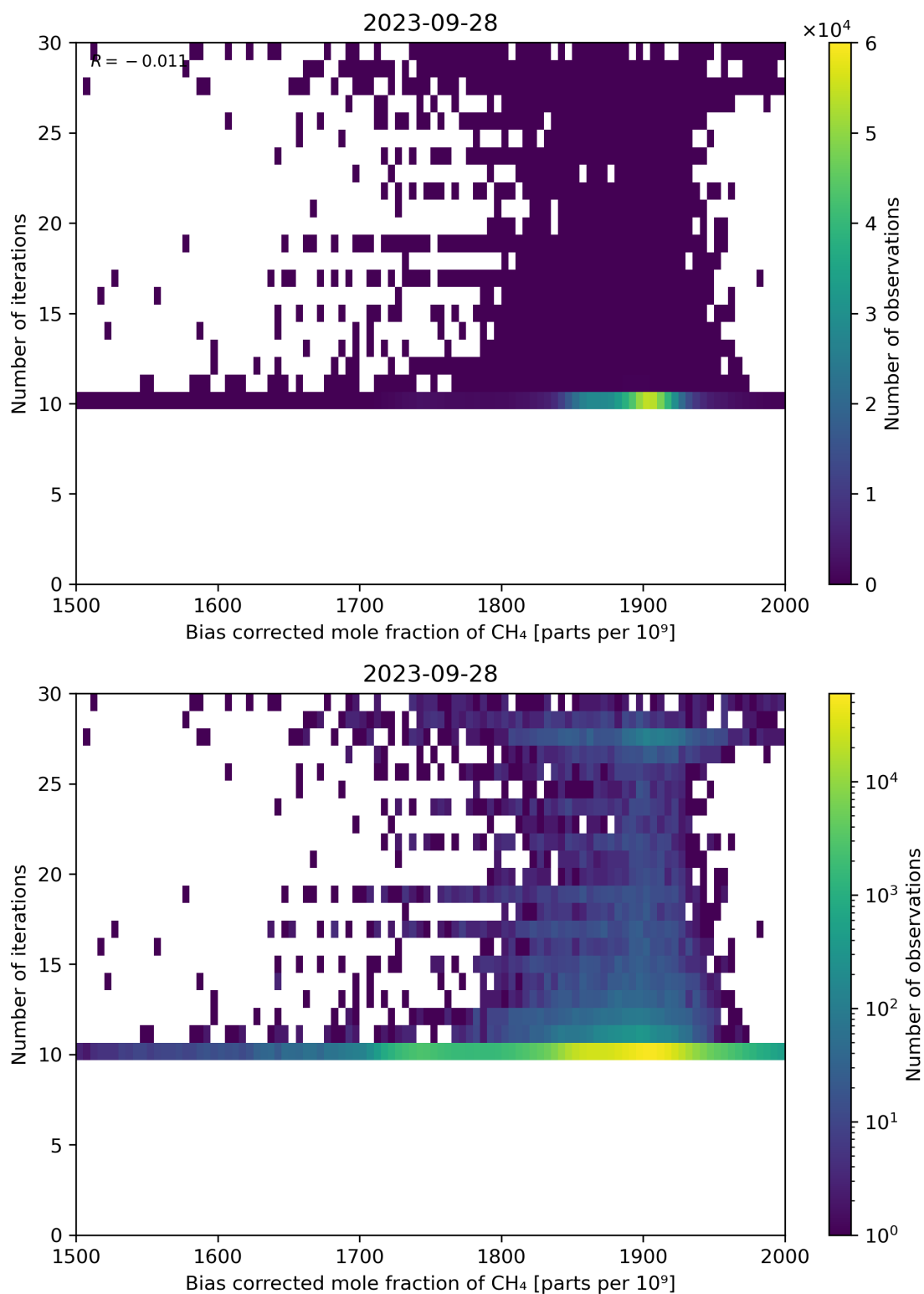
Figure 67: Scatter density plot of “Bias corrected mole fraction of CH 4 ” against “Number of iterations” for 2023-09-27 to 2023-09-29.
