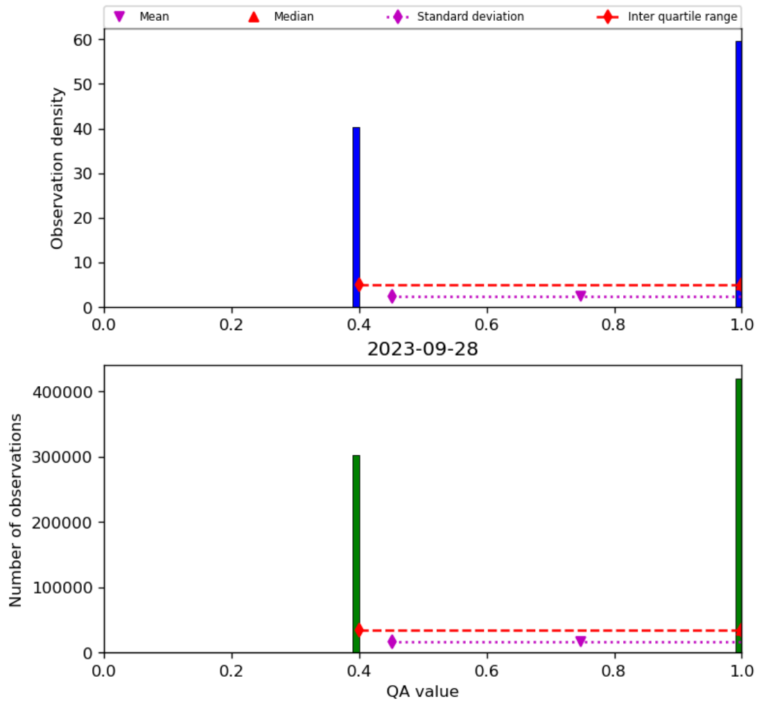
Figure 22: Histogram of “QA value” for 2023-09-27 to 2023-09-29
