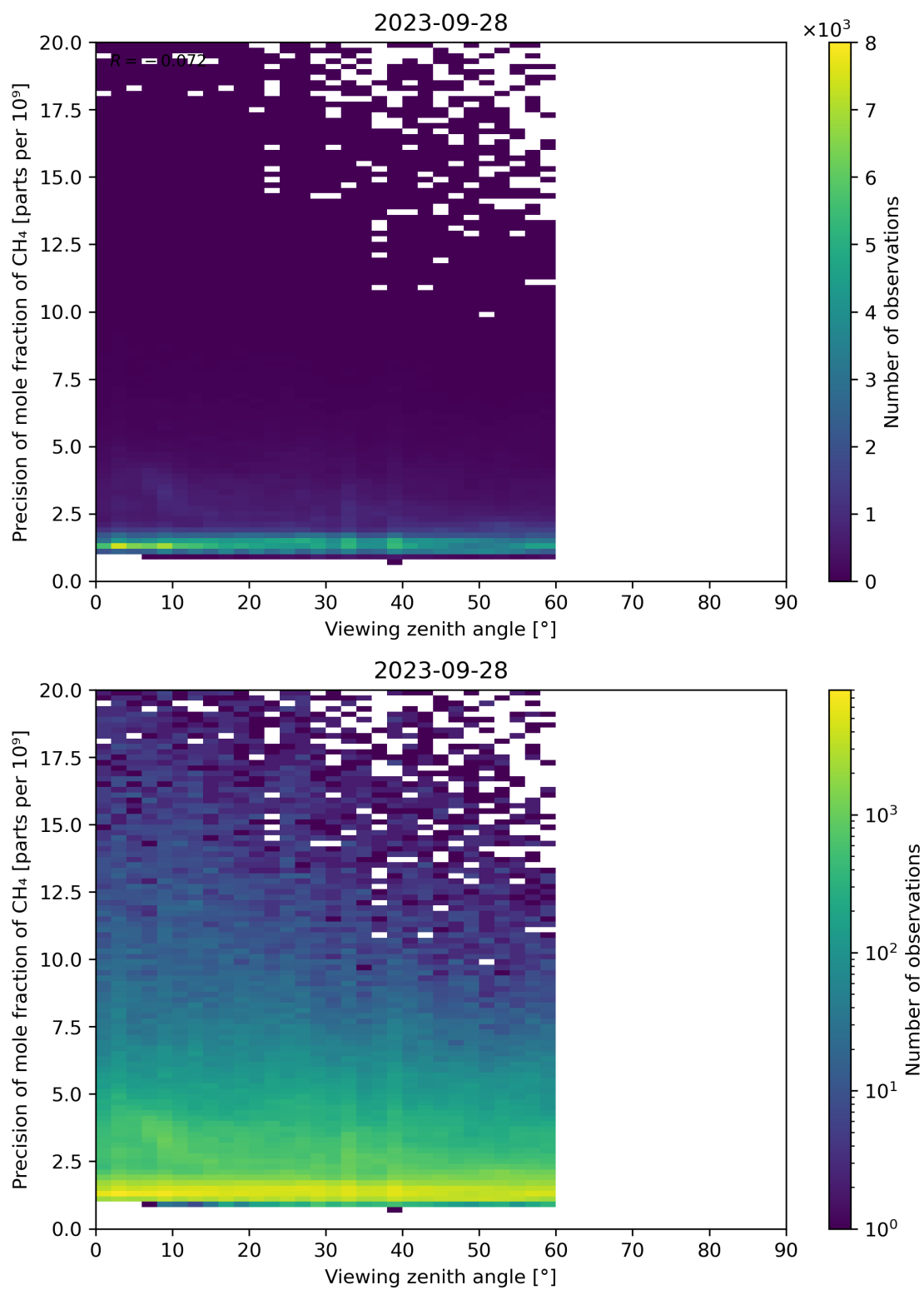
Figure 112: Scatter density plot of “Viewing zenith angle” against “Precision of mole fraction of \text{CH}_4 ” for 2023-09-27 to 2023-09-29.
