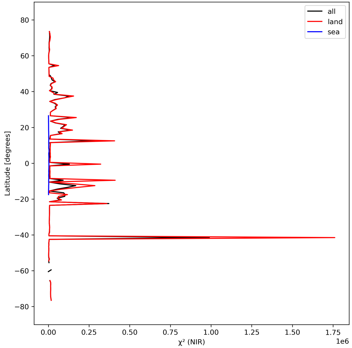
Figure 18: Zonal average of “ \chi^2 (NIR)” for 2023-09-27 to 2023-09-29.
