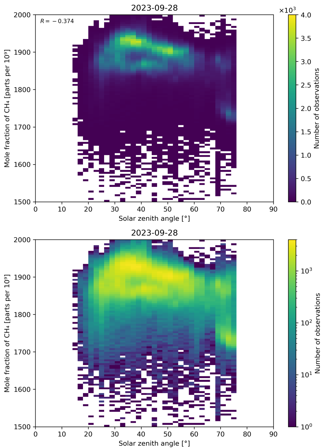
Figure 99: Scatter density plot of “Solar zenith angle” against “Mole fraction of CH 4 ” for 2023-09-27 to 2023-09-29.
