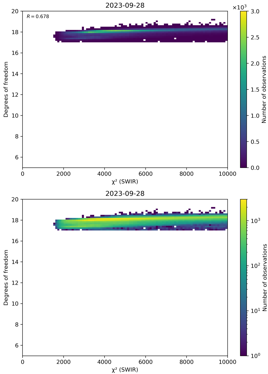
Figure 48: Scatter density plot of “ \chi^2 (SWIR)” against “Degrees of freedom” for 2023-09-27 to 2023-09-29.
