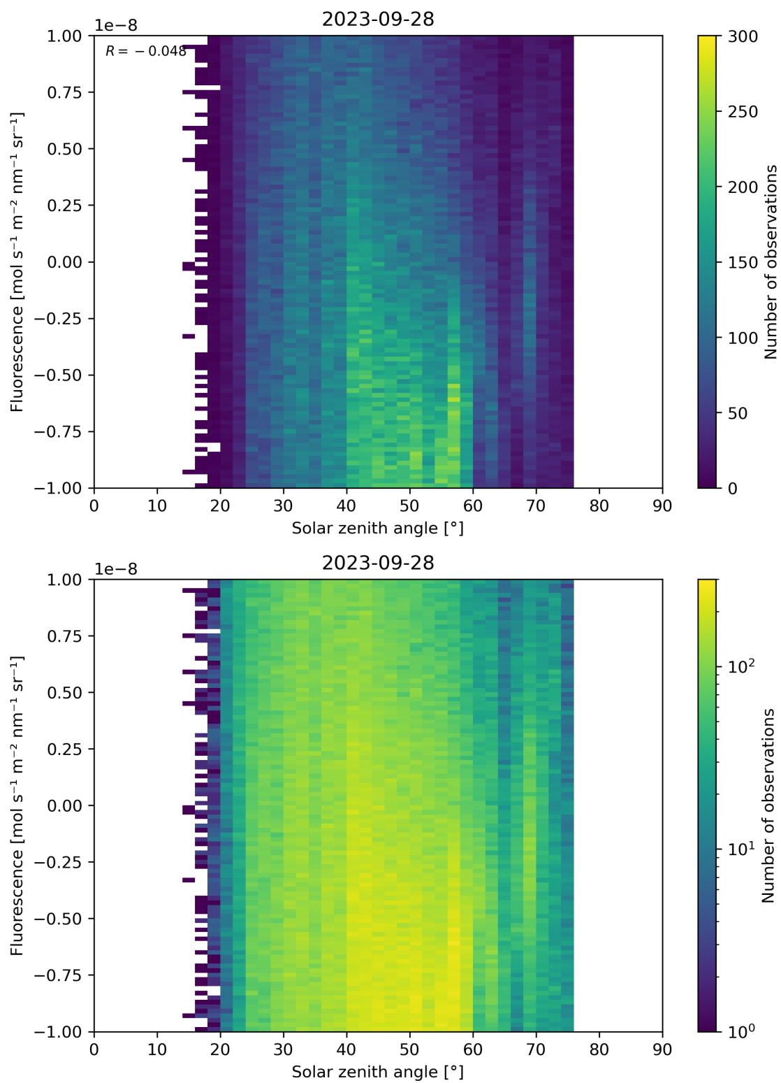
Figure 97: Scatter density plot of “Solar zenith angle” against “Fluorescence” for 2023-09-27 to 2023-09-29.
