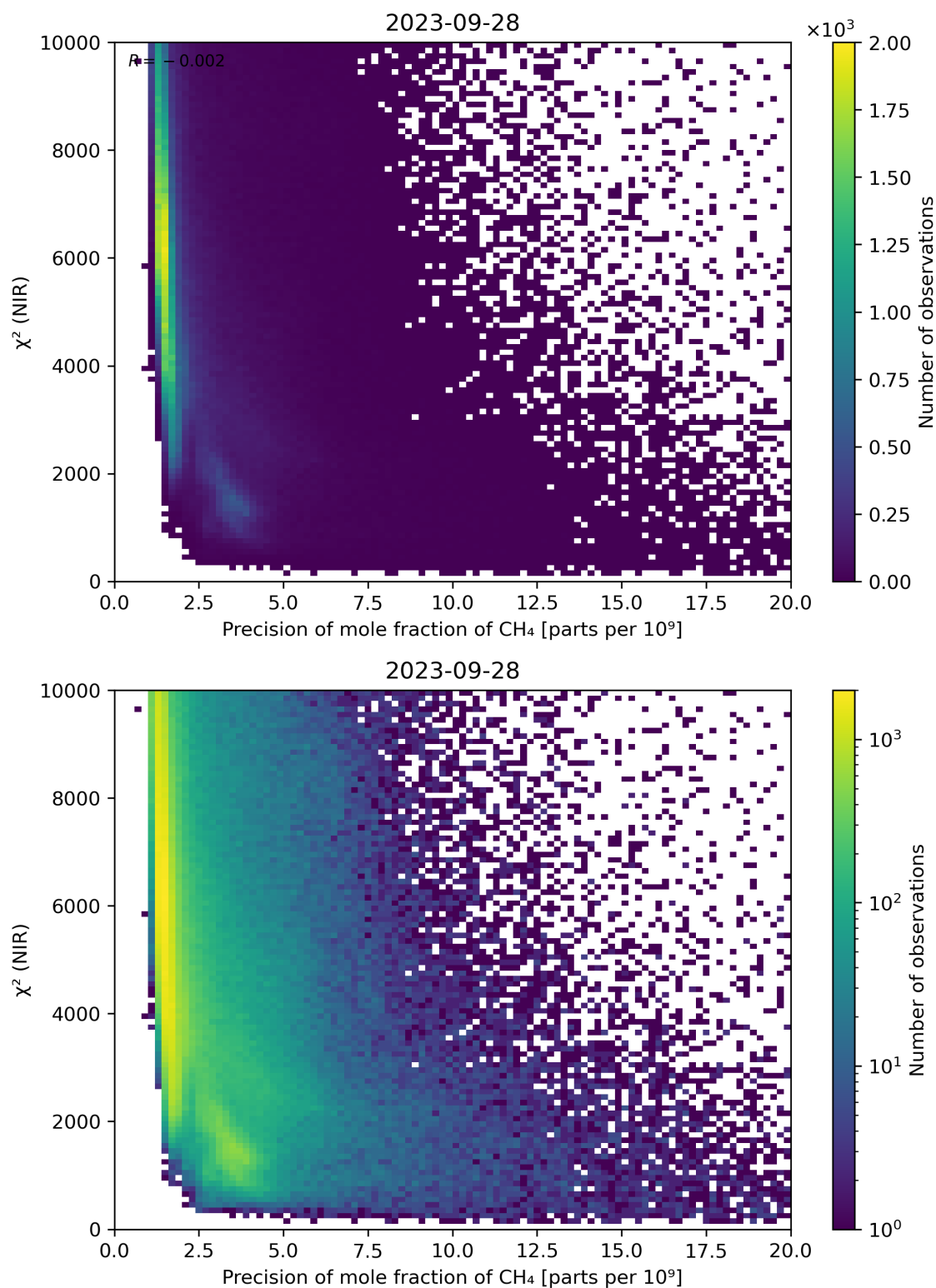
Figure 78: Scatter density plot of “Precision of mole fraction of CH 4 ” against “ \chi^2 (NIR)” for 2023-09-27 to 2023-09-29.
