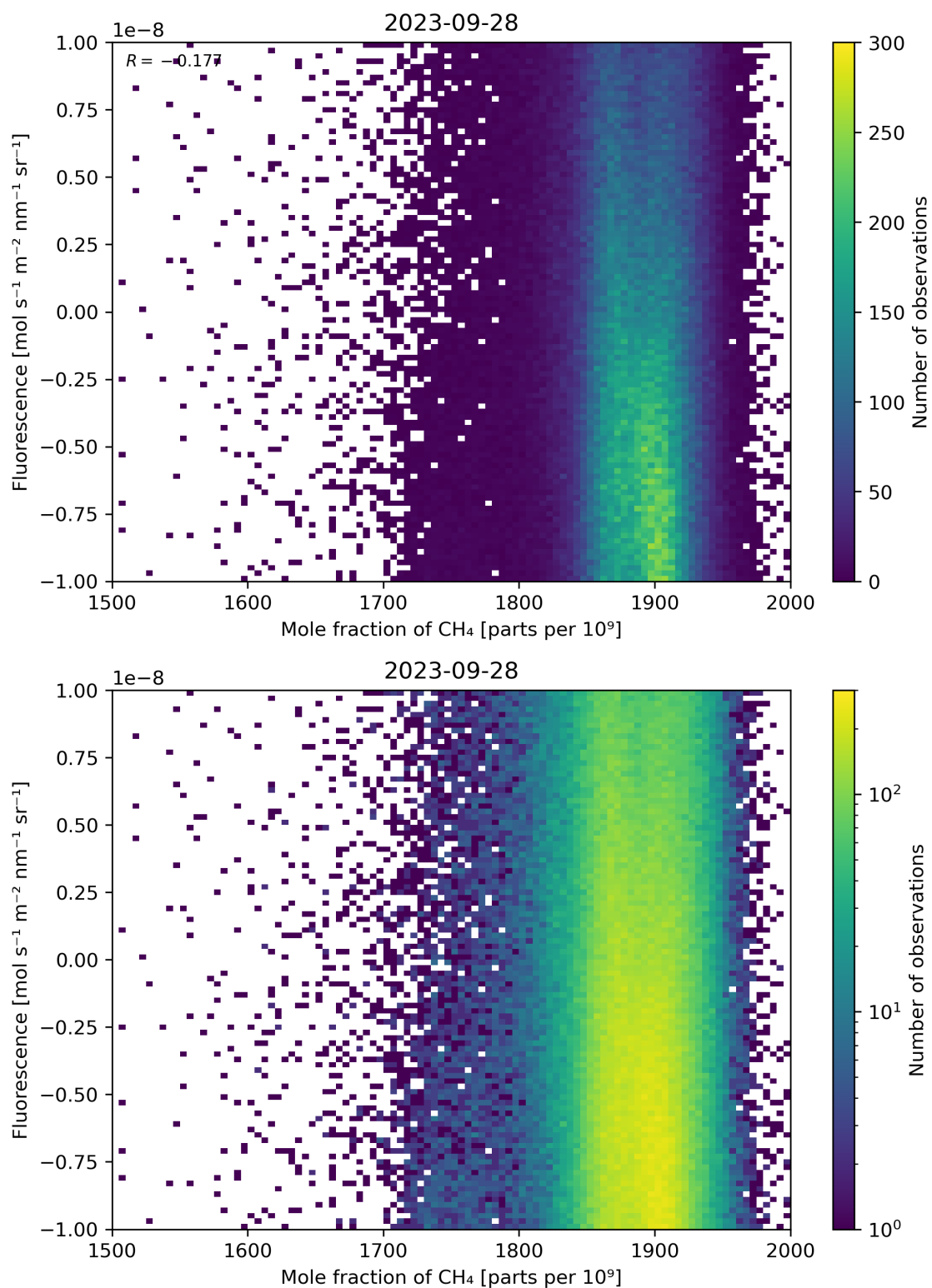
Figure 73: Scatter density plot of “Mole fraction of \text{CH}_4 ” against “Fluorescence” for 2023-09-27 to 2023-09-29.
