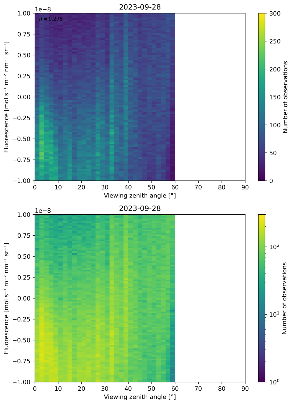
Figure 108: Scatter density plot of “Viewing zenith angle” against “Fluorescence” for 2023-09-27 to 2023-09-29.
