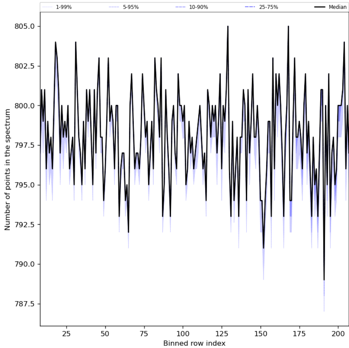
Figure 37: Along track statistics of “Number of points in the spectrum” for 2023-09-27 to 2023-09-29
