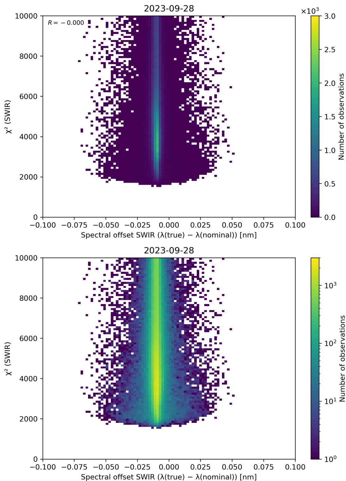
Figure 118: Scatter density plot of “Spectral offset SWIR ( \lambda(\text{true}) - \lambda(\text{nominal}) )” against “ \chi^2 (SWIR)” for 2023-09-27 to 2023-09-29.
