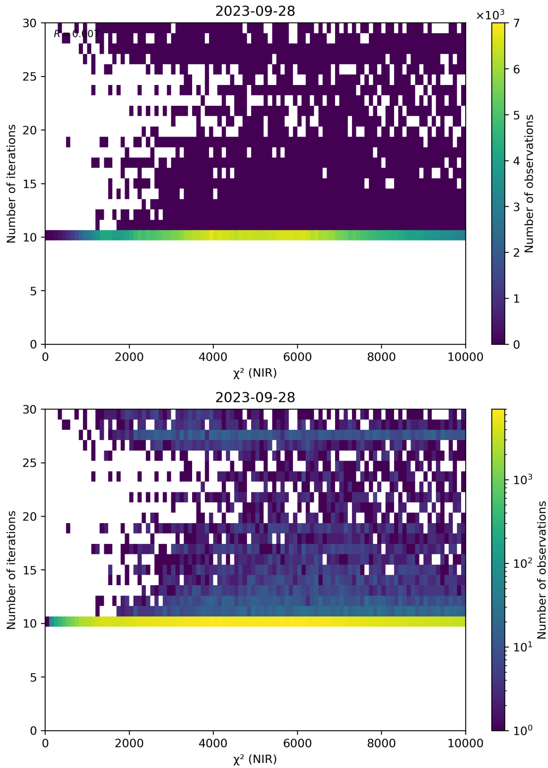
Figure 46: Scatter density plot of “ \chi^2 (NIR)” against “Number of iterations” for 2023-09-27 to 2023-09-29.
