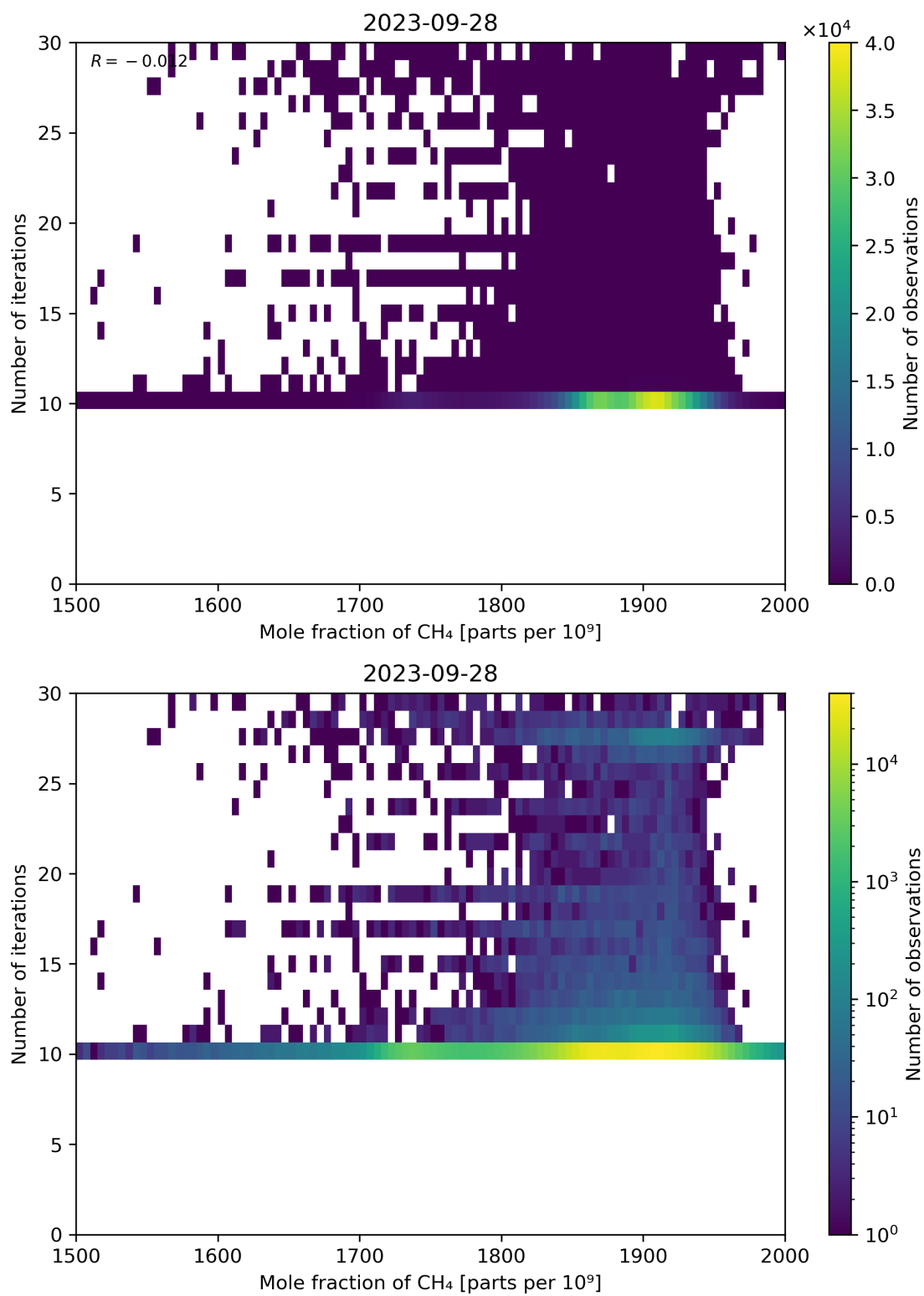
Figure 76: Scatter density plot of “Mole fraction of CH 4 ” against “Number of iterations” for 2023-09-27 to 2023-09-29.
