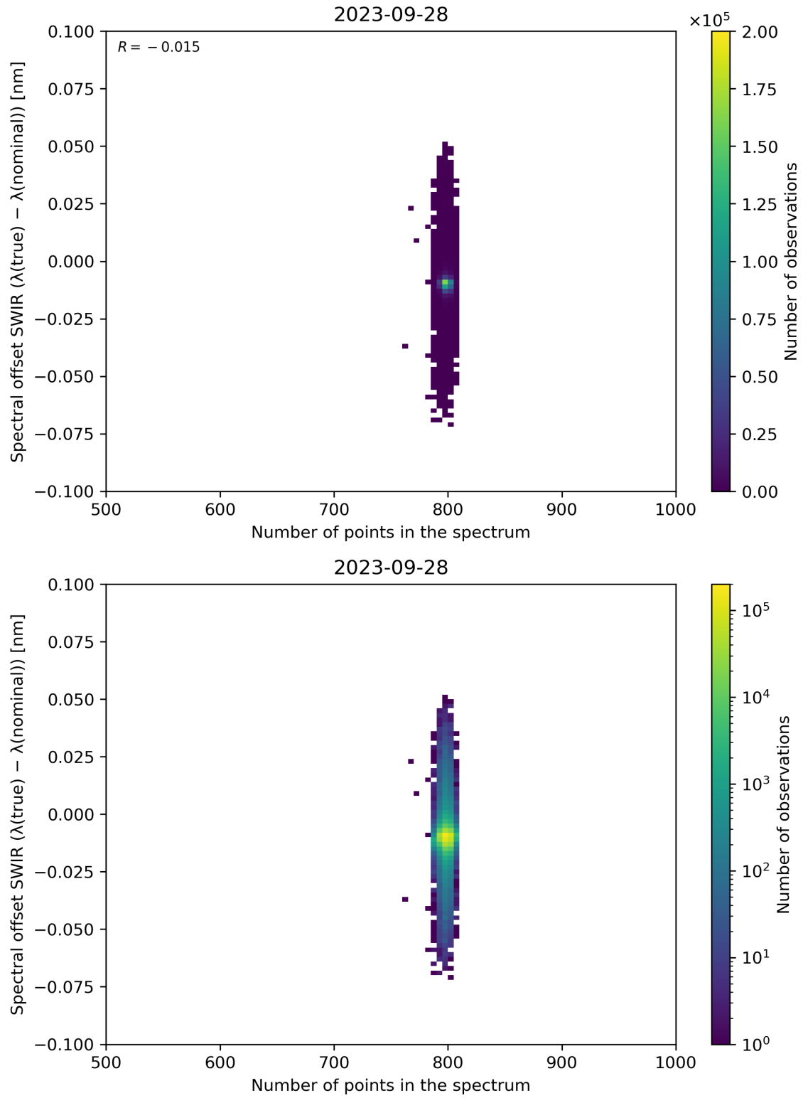
Figure 93: Scatter density plot of “Number of points in the spectrum” against “Spectral offset SWIR ( \lambda(\text{true}) - \lambda(\text{nominal}) )” for 2023-09-27 to 2023-09-29.
