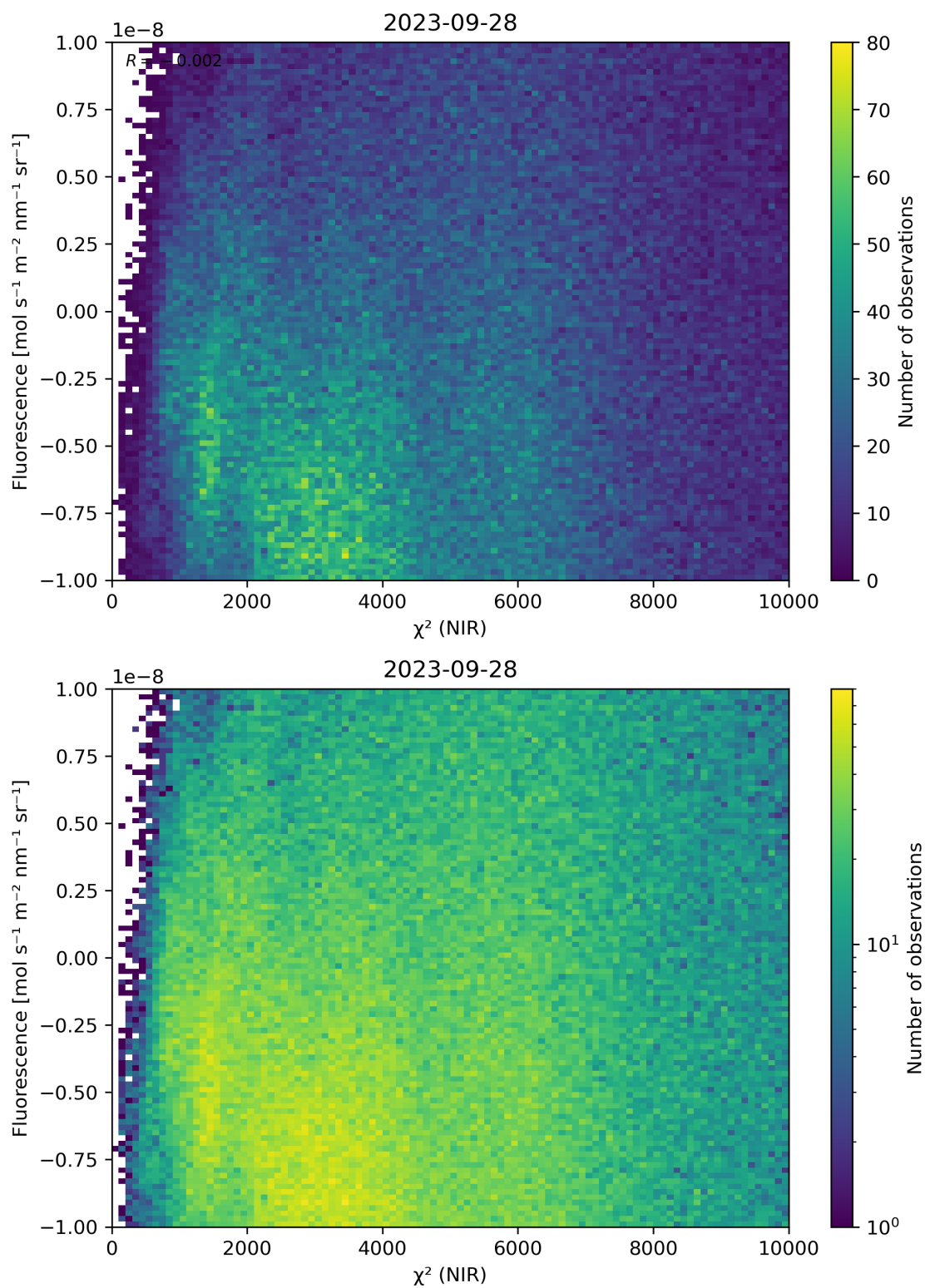
Figure 45: Scatter density plot of “ \chi^2 (NIR)” against “Fluorescence” for 2023-09-27 to 2023-09-29.
