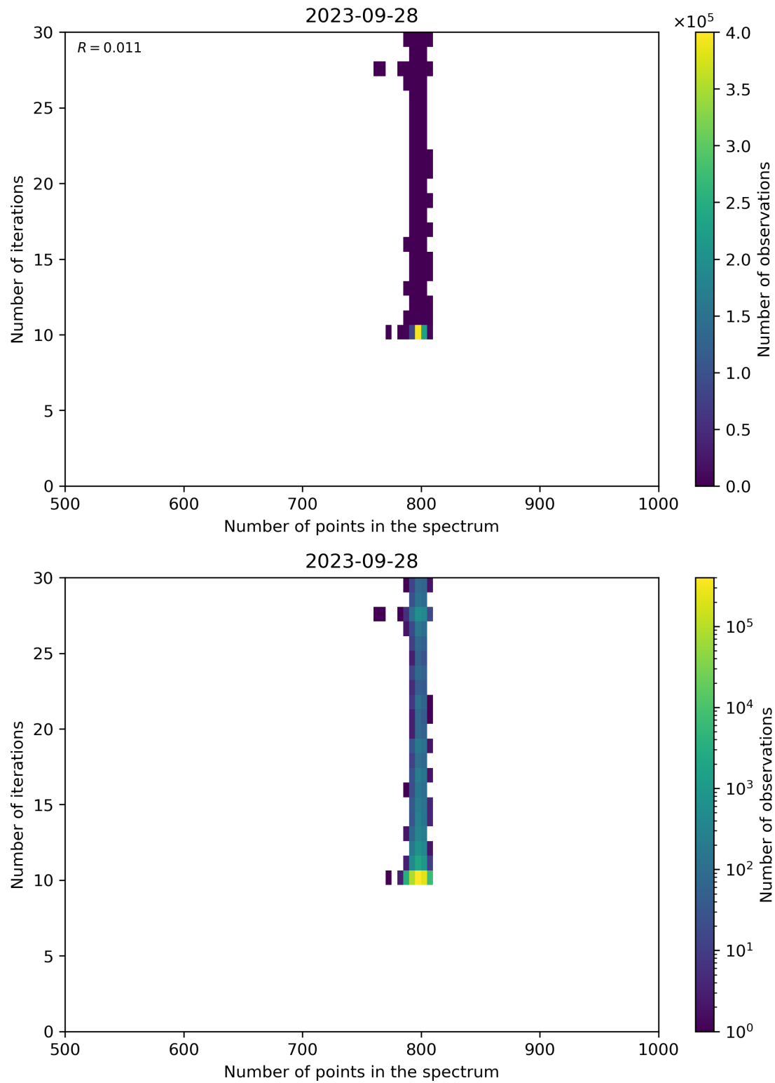
Figure 92: Scatter density plot of “Number of points in the spectrum” against “Number of iterations” for 2023-09-27 to 2023-09-29.
