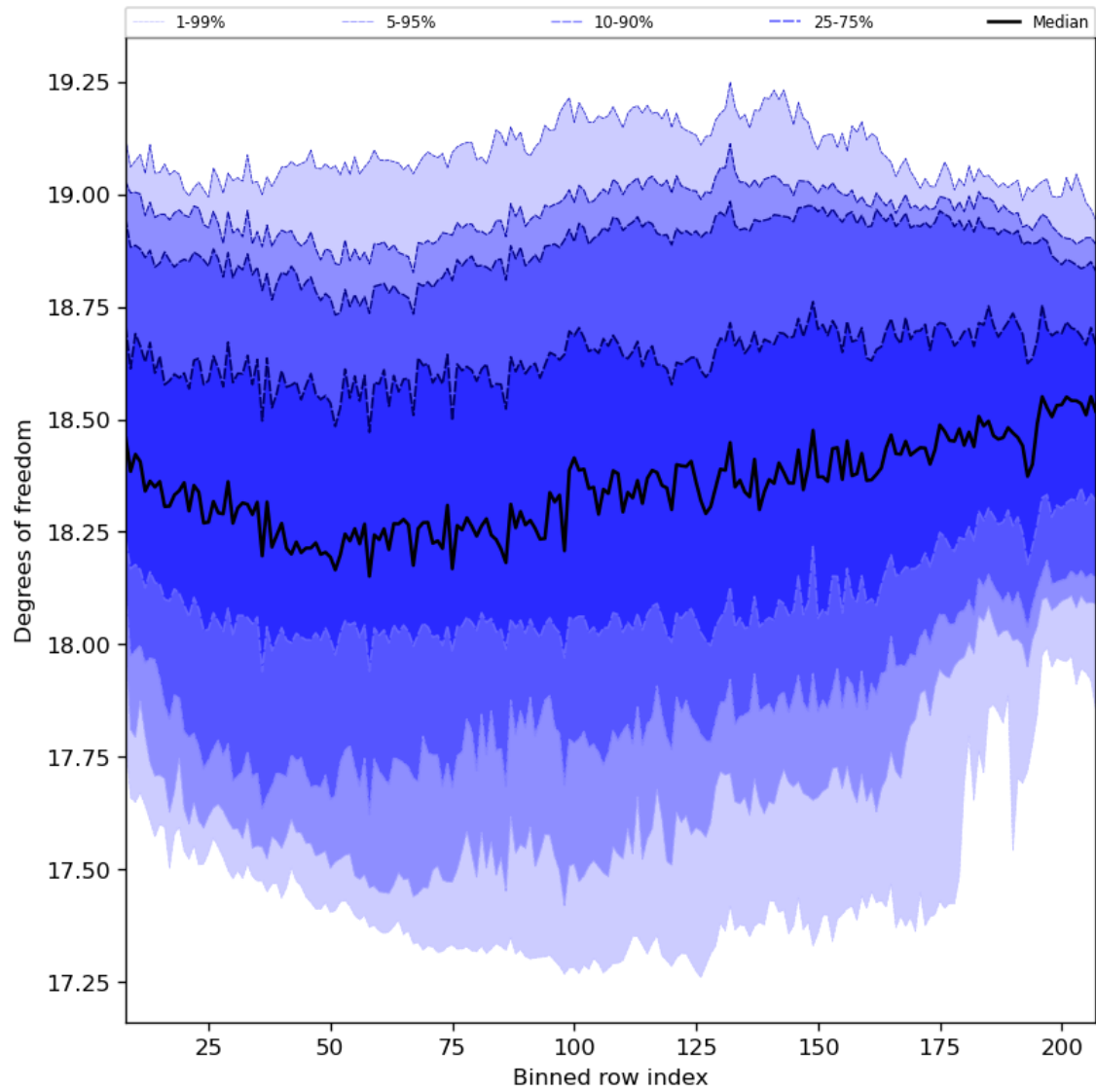
Figure 41: Along track statistics of “Degrees of freedom” for 2023-09-27 to 2023-09-29
