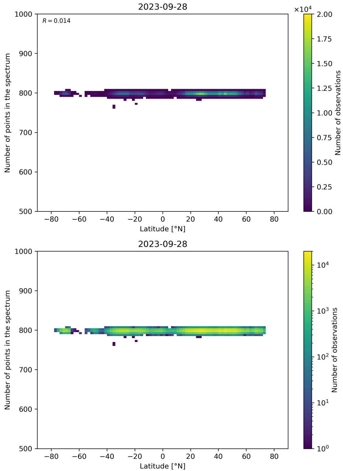
Figure 61: Scatter density plot of “Latitude” against “Number of points in the spectrum” for 2023-09-27 to 2023-09-29.
