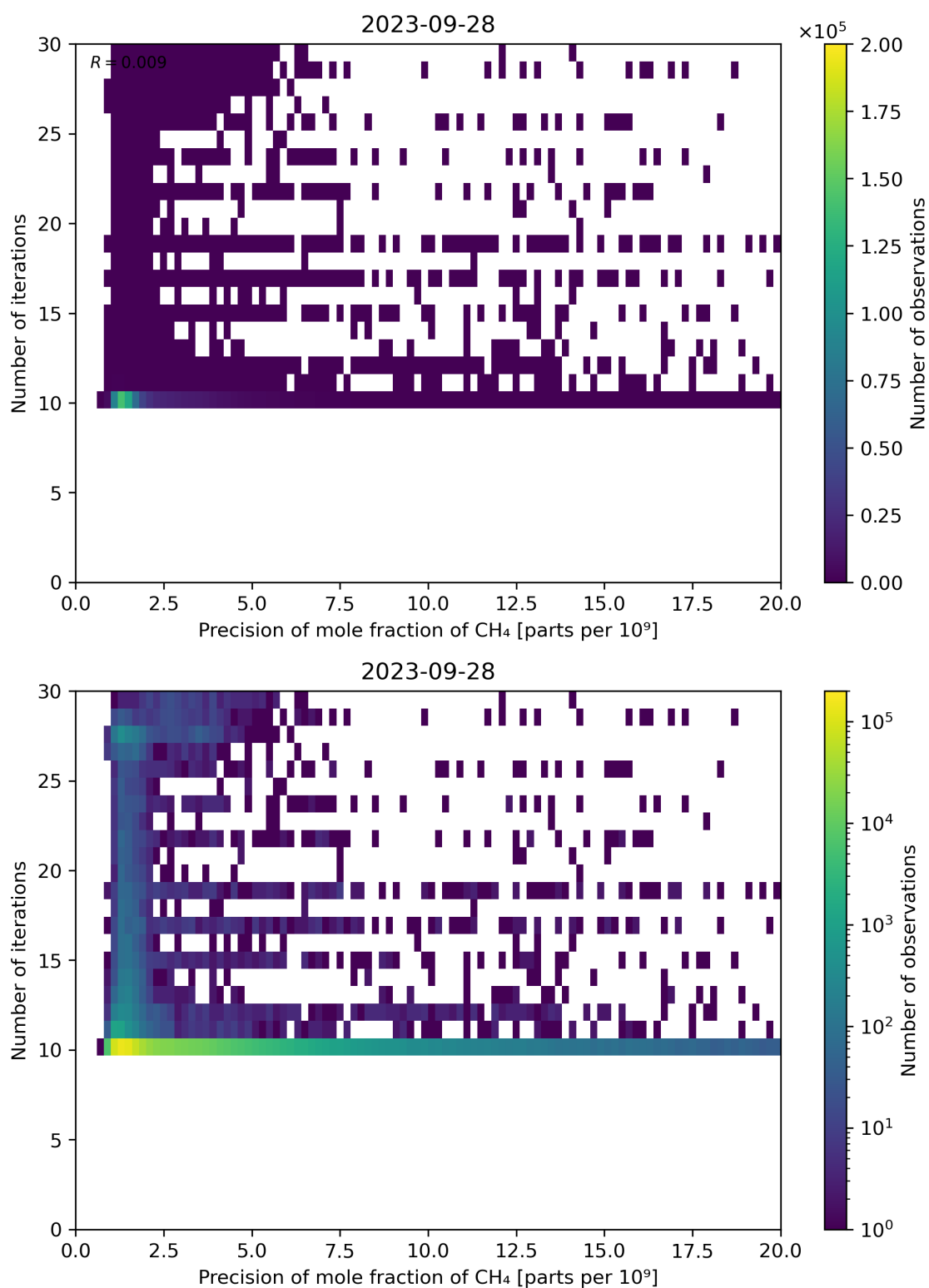
Figure 83: Scatter density plot of “Precision of mole fraction of CH 4 ” against “Number of iterations” for 2023-09-27 to 2023-09-29.
