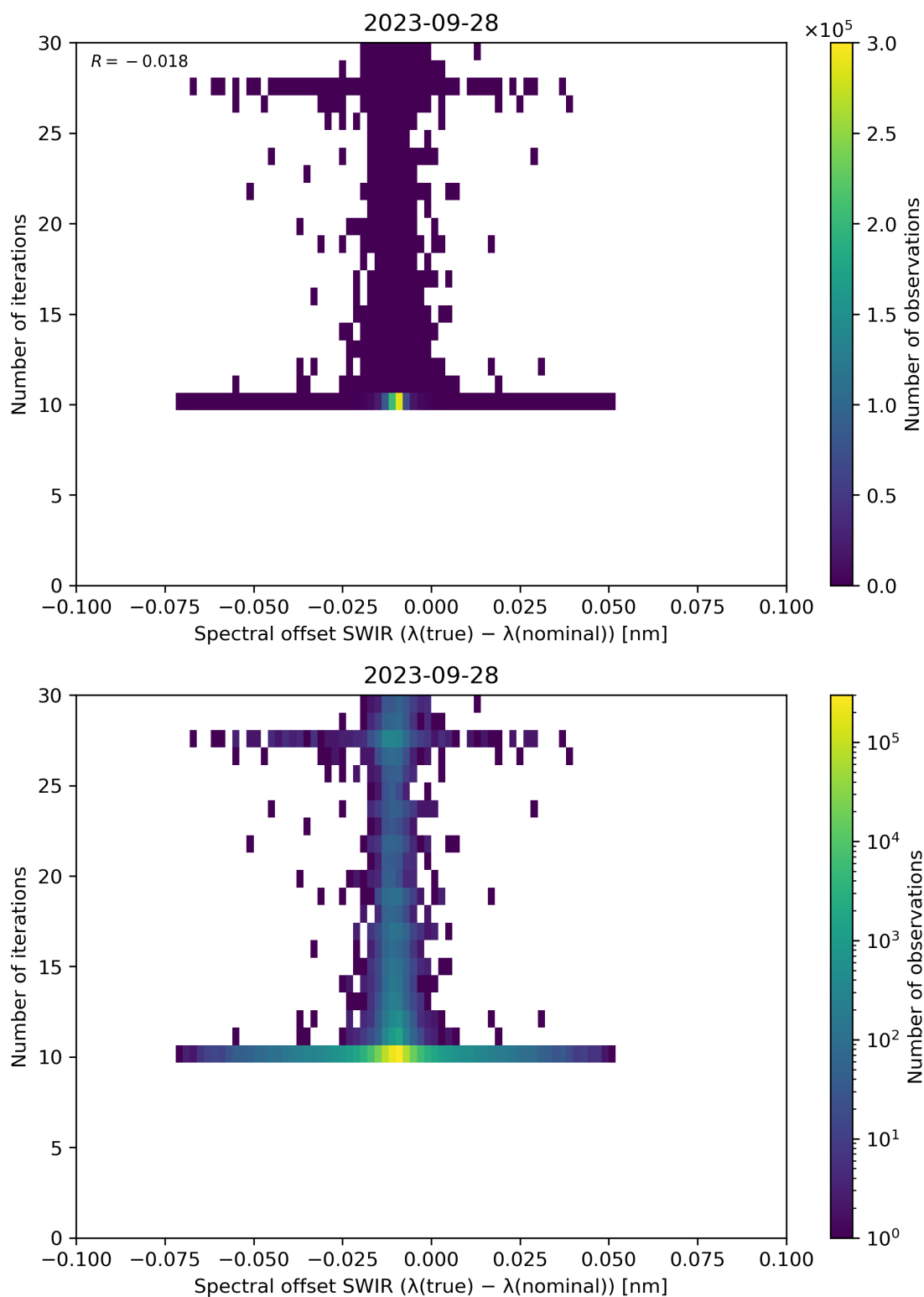
Figure 121: Scatter density plot of “Spectral offset SWIR ( \lambda(\text{true}) - \lambda(\text{nominal}) )” against “Number of iterations” for 2023-09-27 to 2023-09-29.
