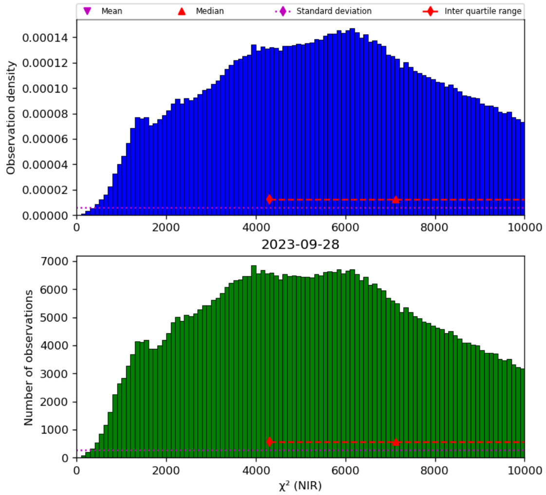
Figure 29: Histogram of “ \chi^2 (NIR)” for 2023-09-27 to 2023-09-29
