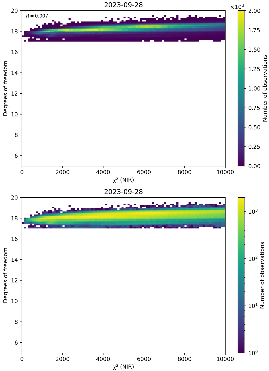
Figure 44: Scatter density plot of “ \chi^2 (NIR)” against “Degrees of freedom” for 2023-09-27 to 2023-09-29.
