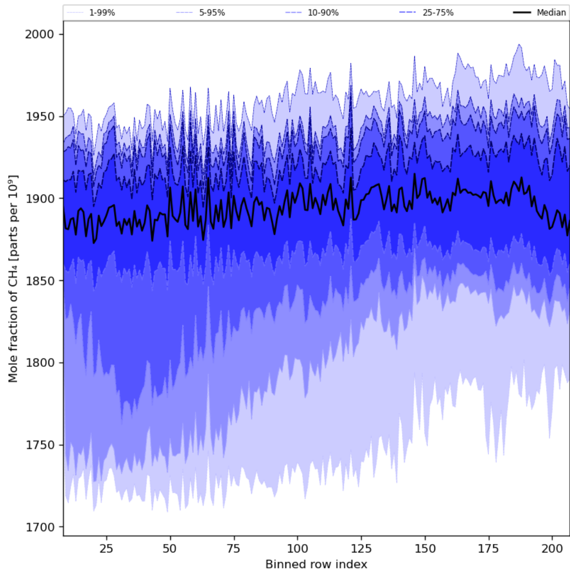
Figure 34: Along track statistics of “Mole fraction of CH 4 ” for 2023-09-27 to 2023-09-29
