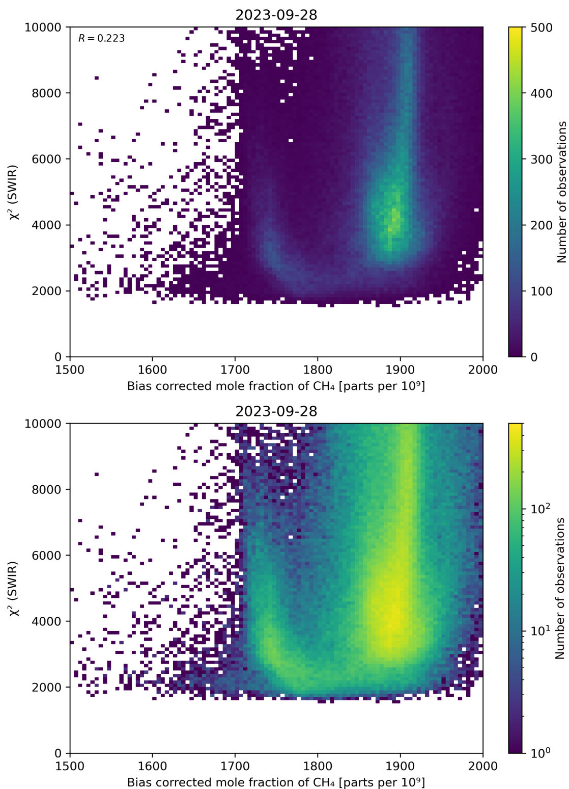
Figure 64: Scatter density plot of “Bias corrected mole fraction of \text{CH}_4 ” against “ \chi^2 (SWIR)” for 2023-09-27 to 2023-09-29.
