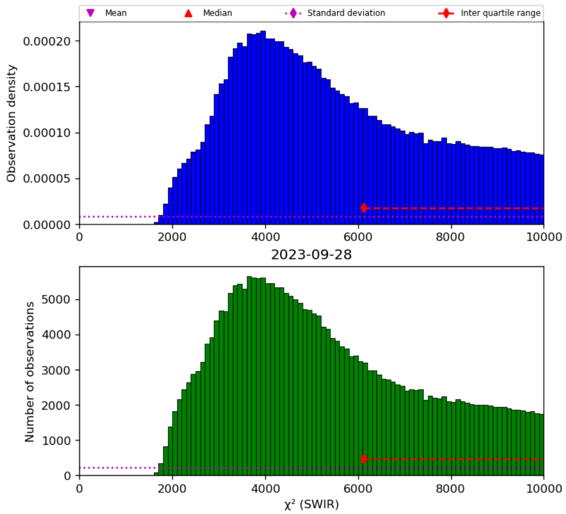
Figure 28: Histogram of “ \chi^2 (SWIR)” for 2023-09-27 to 2023-09-29
