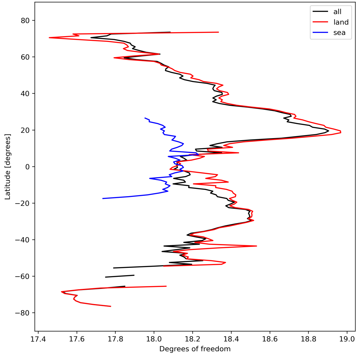
Figure 19: Zonal average of “Degrees of freedom” for 2023-09-27 to 2023-09-29.
