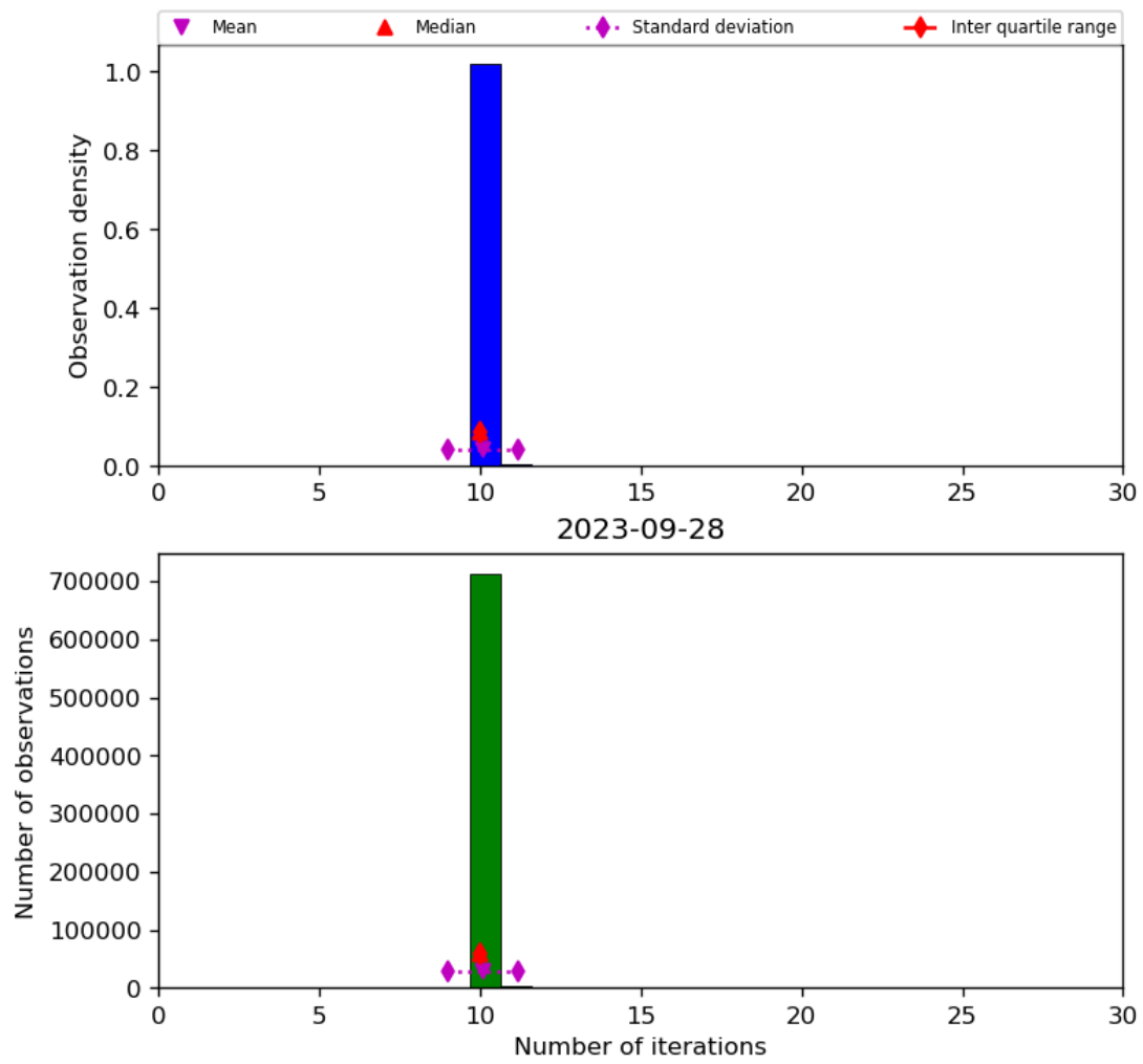
Figure 31: Histogram of “Number of iterations” for 2023-09-27 to 2023-09-29
