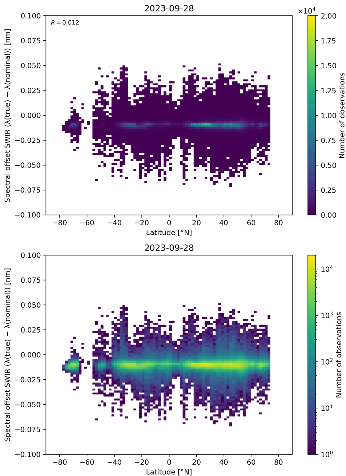
Figure 62: Scatter density plot of “Latitude” against “Spectral offset SWIR ( \lambda(\text{true}) - \lambda(\text{nominal}) )” for 2023-09-27 to 2023-09-29.
