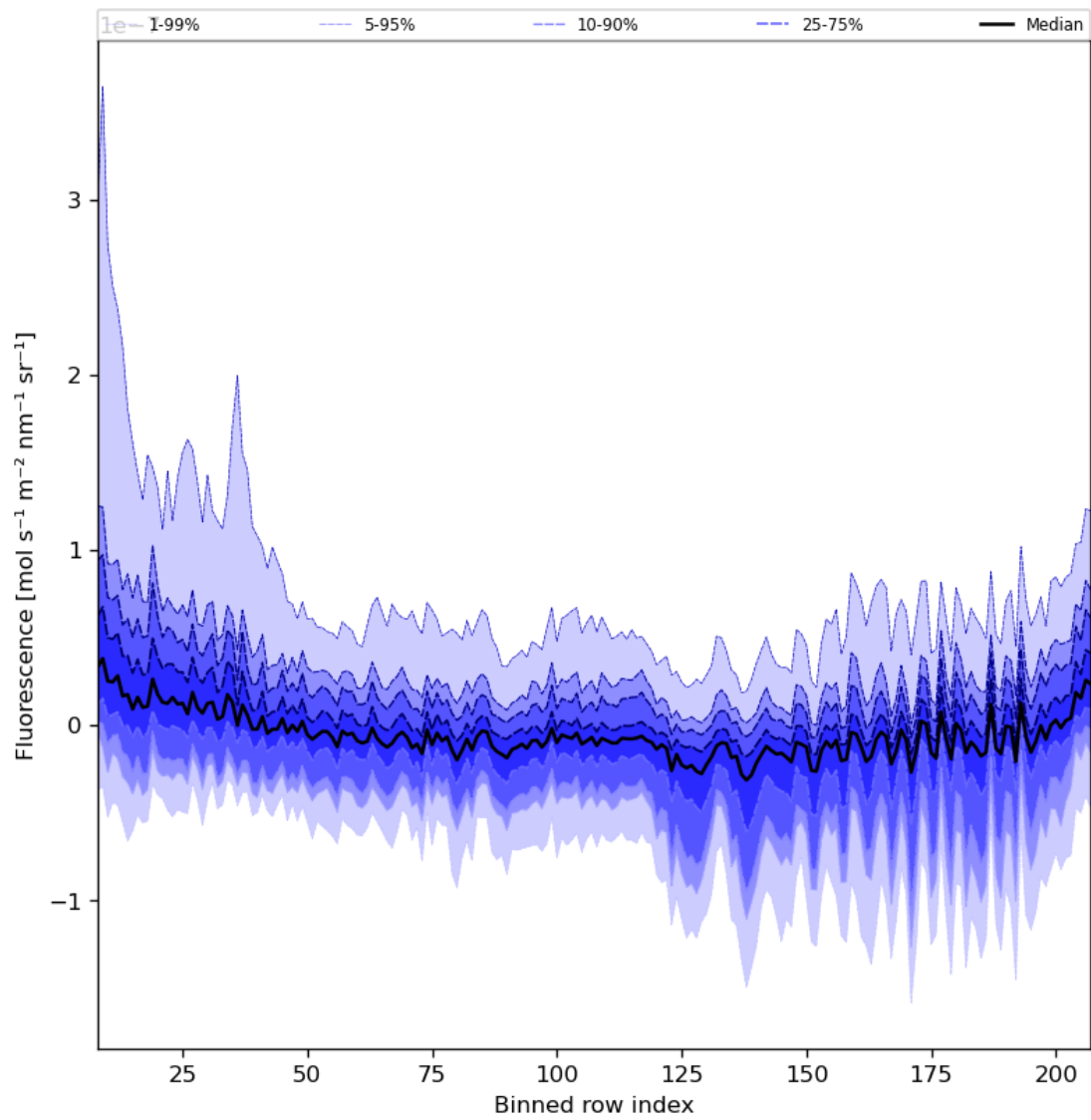
Figure 43: Along track statistics of "Fluorescence" for 2023-09-27 to 2023-09-29
