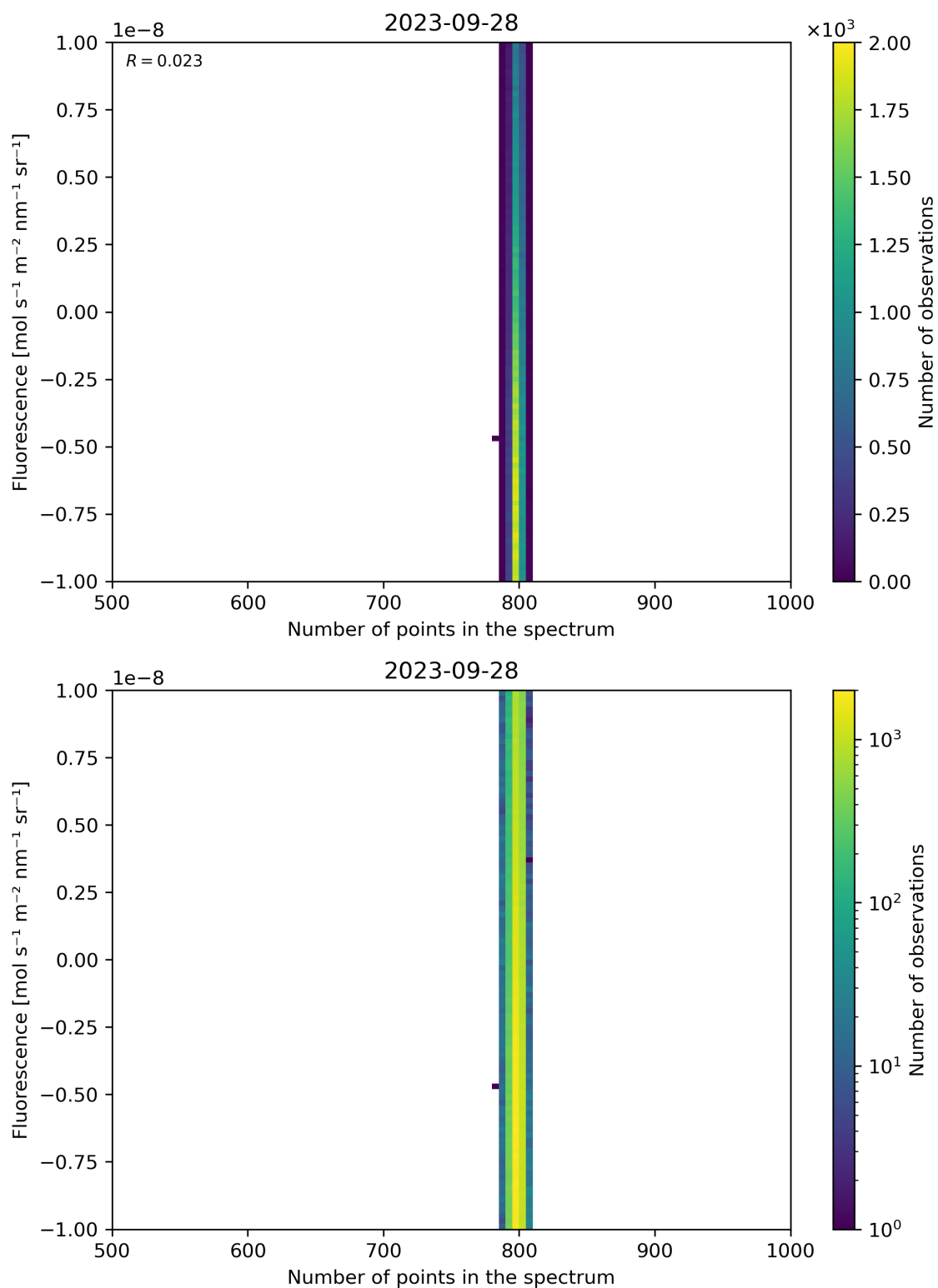
Figure 91: Scatter density plot of “Number of points in the spectrum” against “Fluorescence” for 2023-09-27 to 2023-09-29.
