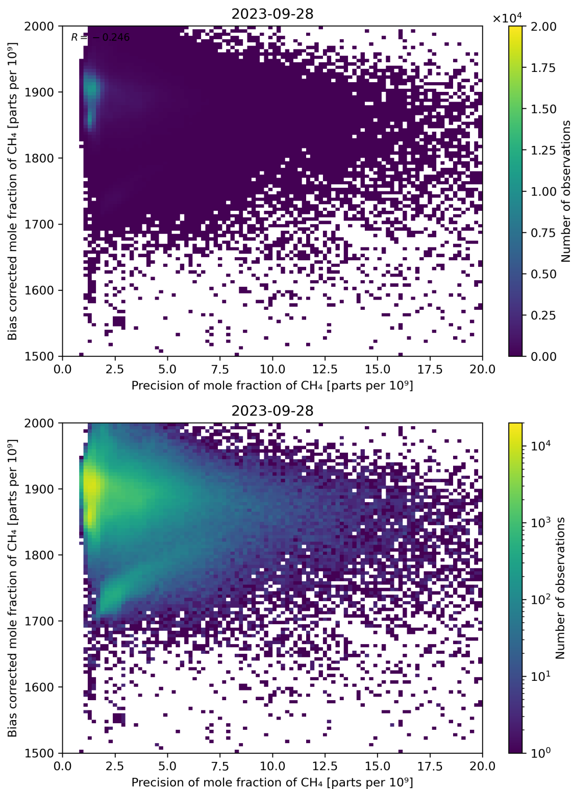
Figure 82: Scatter density plot of “Precision of mole fraction of CH 4 ” against “Bias corrected mole fraction of CH 4 ” for 2023-09-27 to 2023-09-29.
