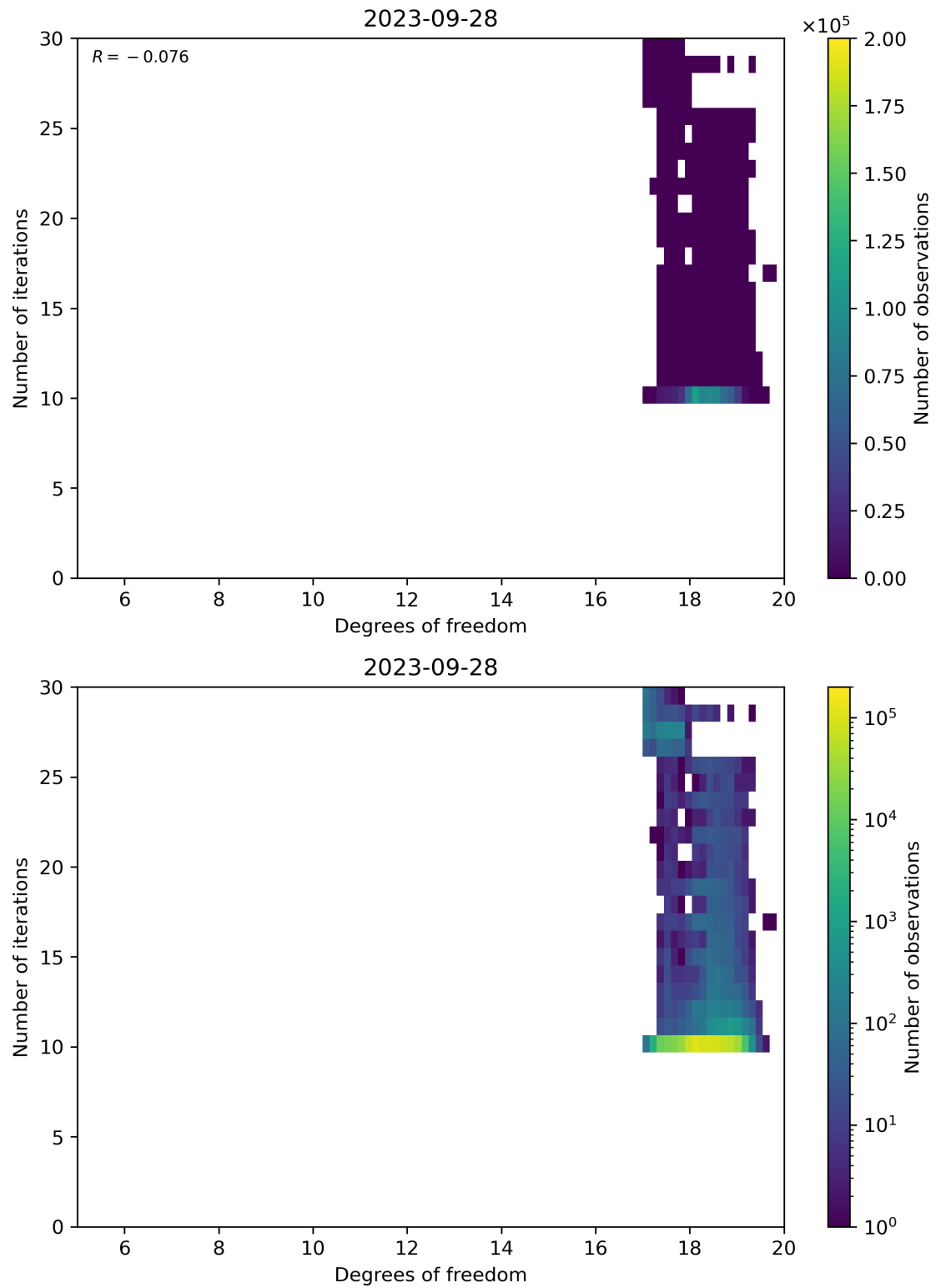
Figure 52: Scatter density plot of “Degrees of freedom” against “Number of iterations” for 2023-09-27 to 2023-09-29.
