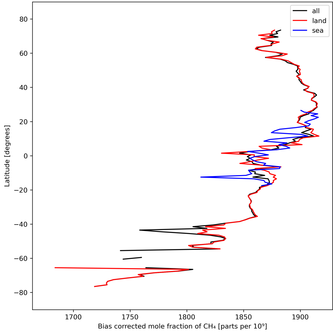
Figure 14: Zonal average of “Bias corrected mole fraction of CH 4 ” for 2023-09-27 to 2023-09-29.
