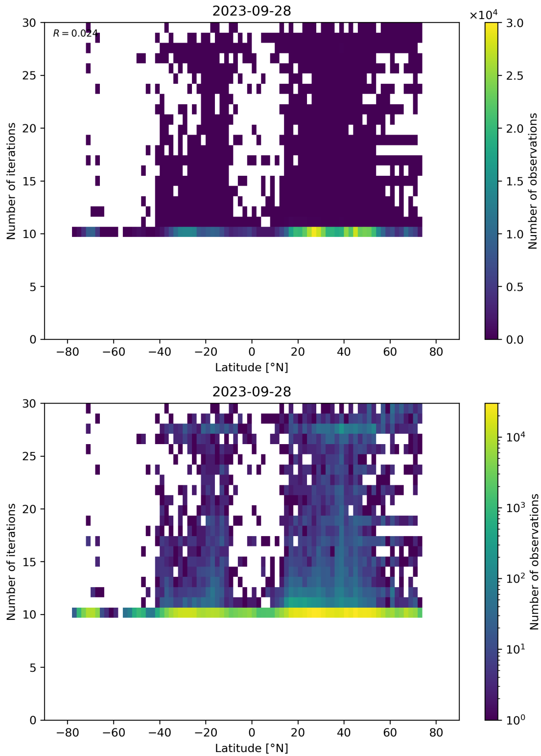
Figure 60: Scatter density plot of “Latitude” against “Number of iterations” for 2023-09-27 to 2023-09-29.
