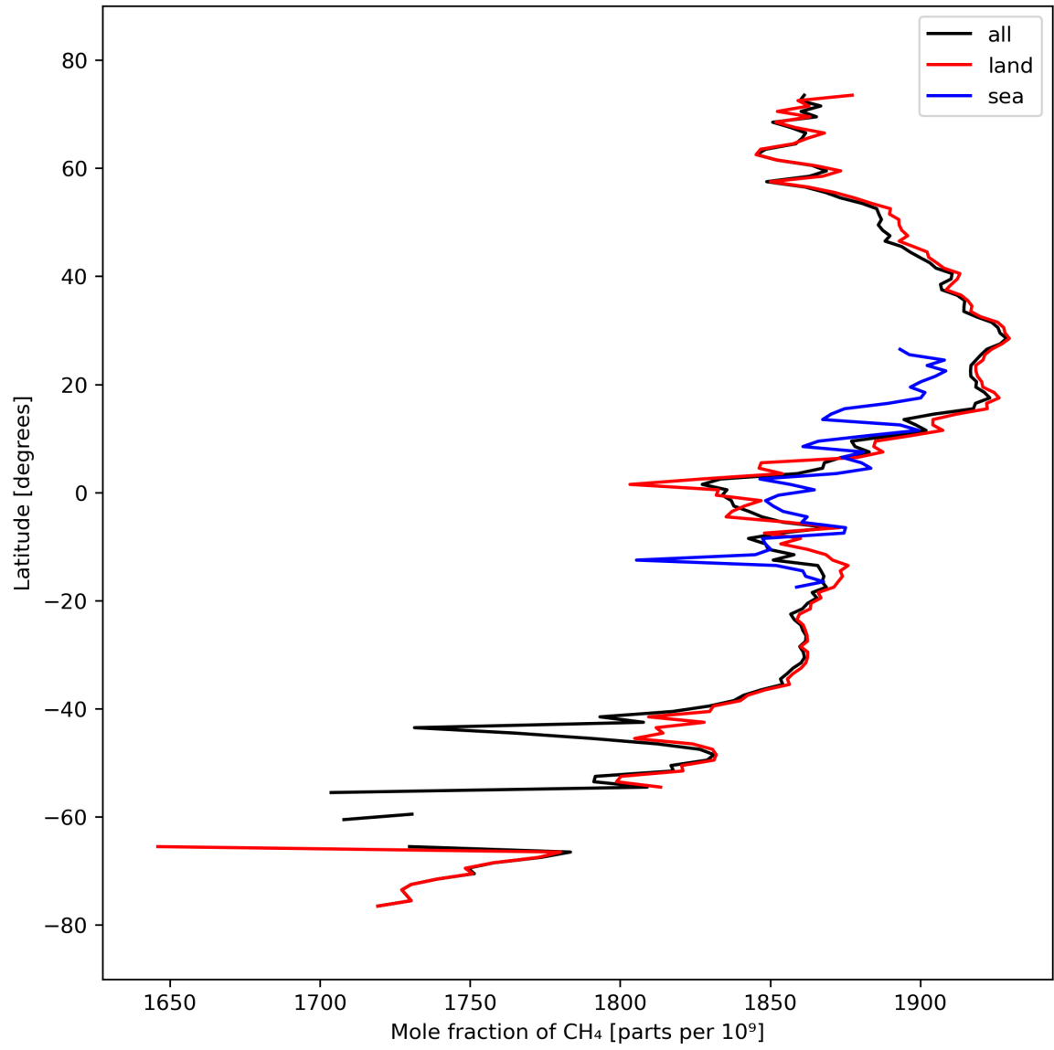
Figure 12: Zonal average of “Mole fraction of \text{CH}_4 ” for 2023-09-27 to 2023-09-29.
