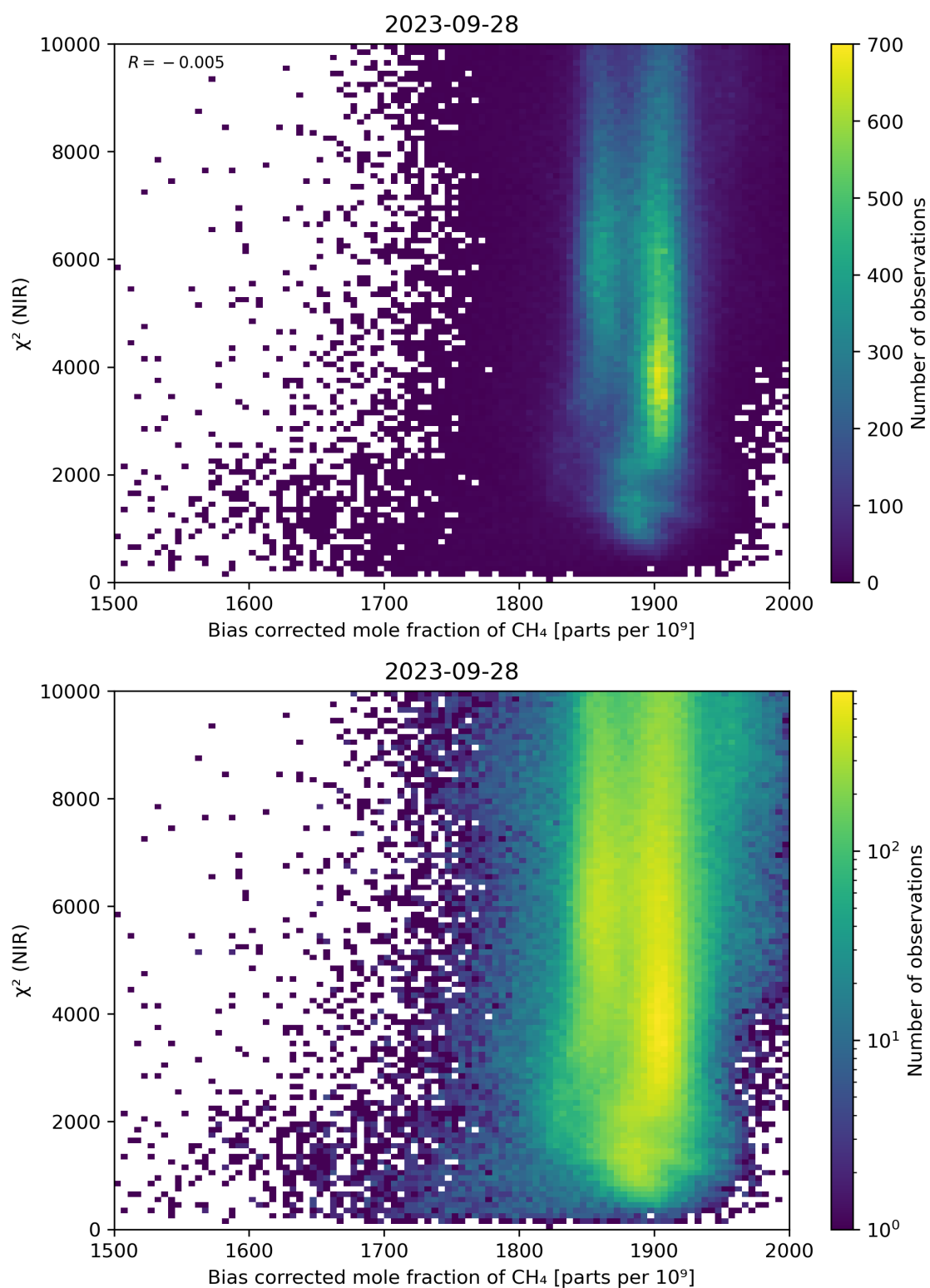
Figure 63: Scatter density plot of “Bias corrected mole fraction of CH 4 ” against “ \chi^2 (NIR)” for 2023-09-27 to 2023-09-29.
