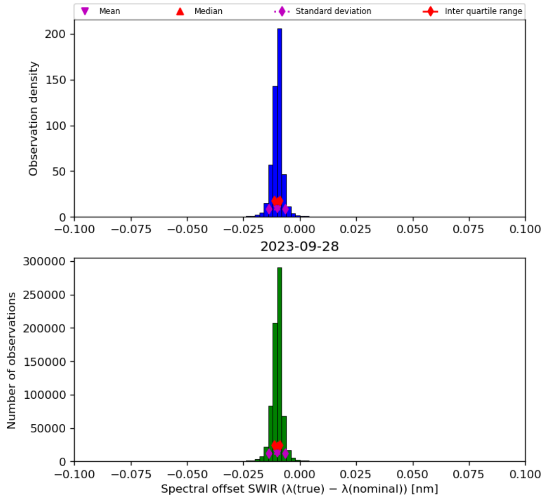
Figure 27: Histogram of “Spectral offset SWIR ( \lambda(\text{true}) - \lambda(\text{nominal}) )” for 2023-09-27 to 2023-09-29
