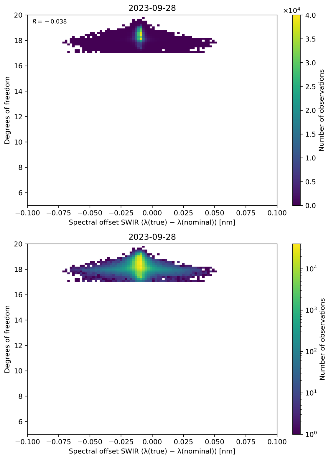
Figure 119: Scatter density plot of “Spectral offset SWIR ( \lambda(\text{true}) - \lambda(\text{nominal}) )” against “Degrees of freedom” for 2023-09-27 to 2023-09-29.
