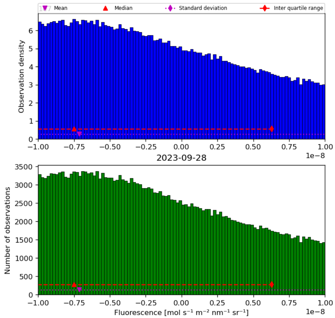
Figure 32: Histogram of “Fluorescence” for 2023-09-27 to 2023-09-29
