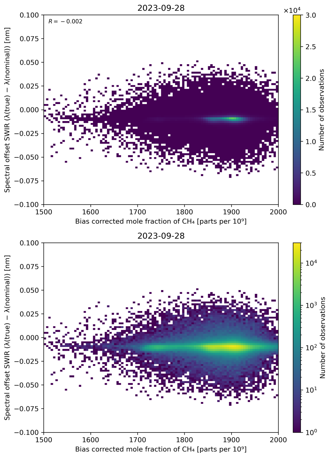
Figure 69: Scatter density plot of “Bias corrected mole fraction of \text{CH}_4 ” against “Spectral offset SWIR ( \lambda(\text{true}) - \lambda(\text{nominal}) )” for 2023-09-27 to 2023-09-29.
