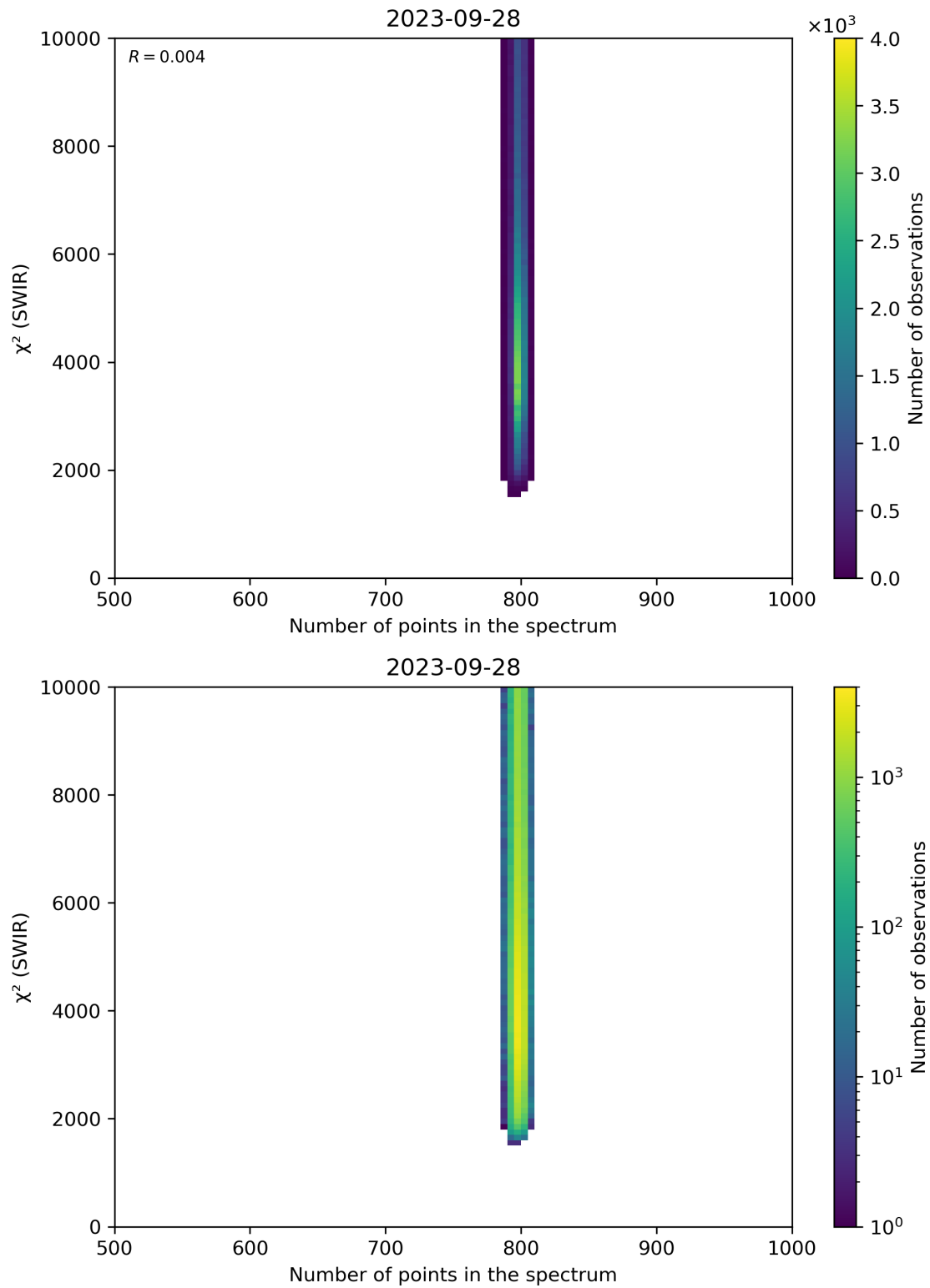
Figure 89: Scatter density plot of “Number of points in the spectrum” against “ \chi^2 (SWIR)” for 2023-09-27 to 2023-09-29.
