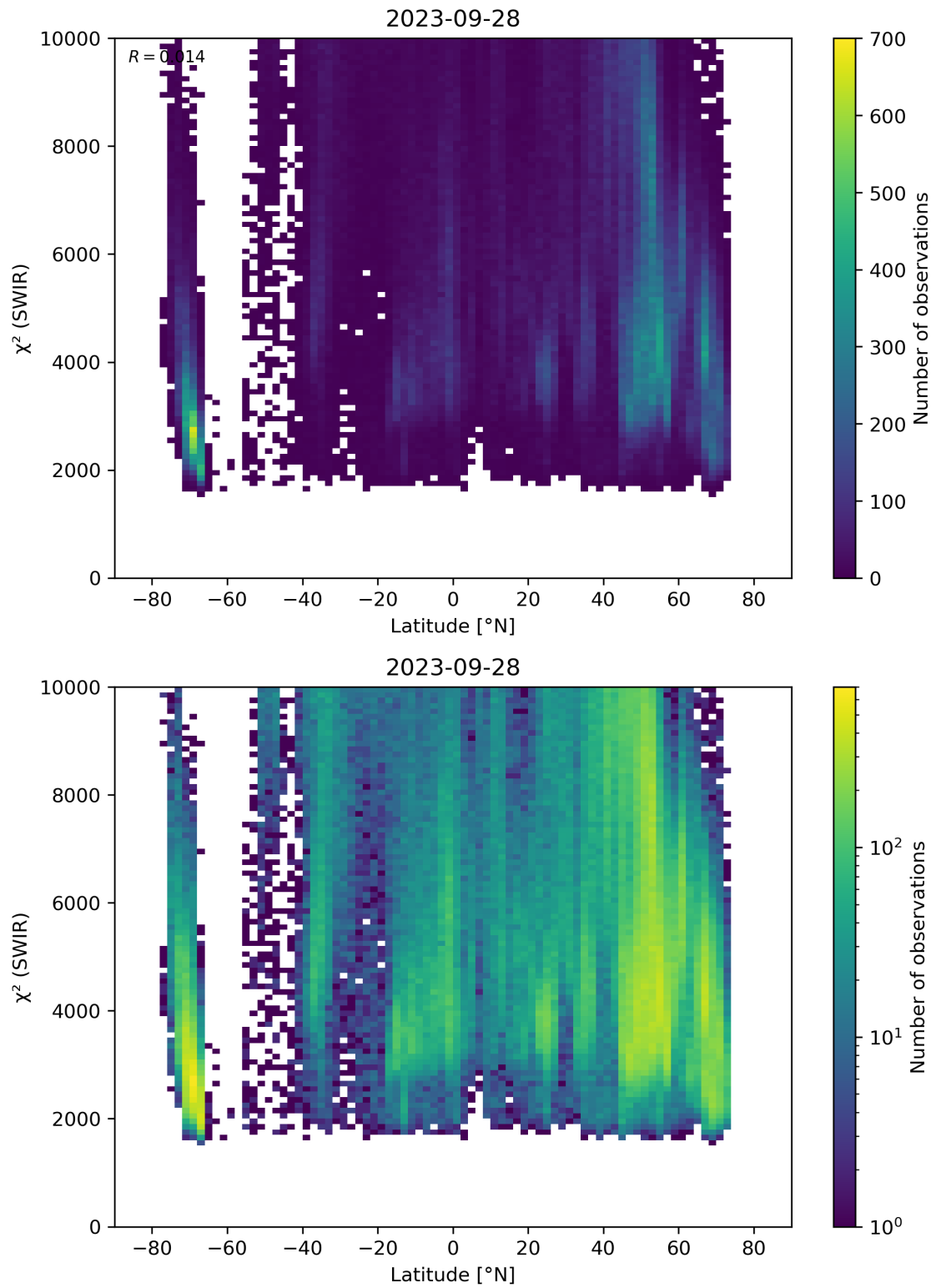
Figure 54: Scatter density plot of “Latitude” against “ \chi^2 (SWIR)” for 2023-09-27 to 2023-09-29.
