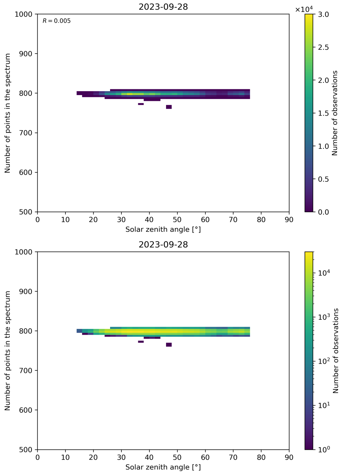
Figure 103: Scatter density plot of “Solar zenith angle” against “Number of points in the spectrum” for 2023-09-27 to 2023-09-29.
