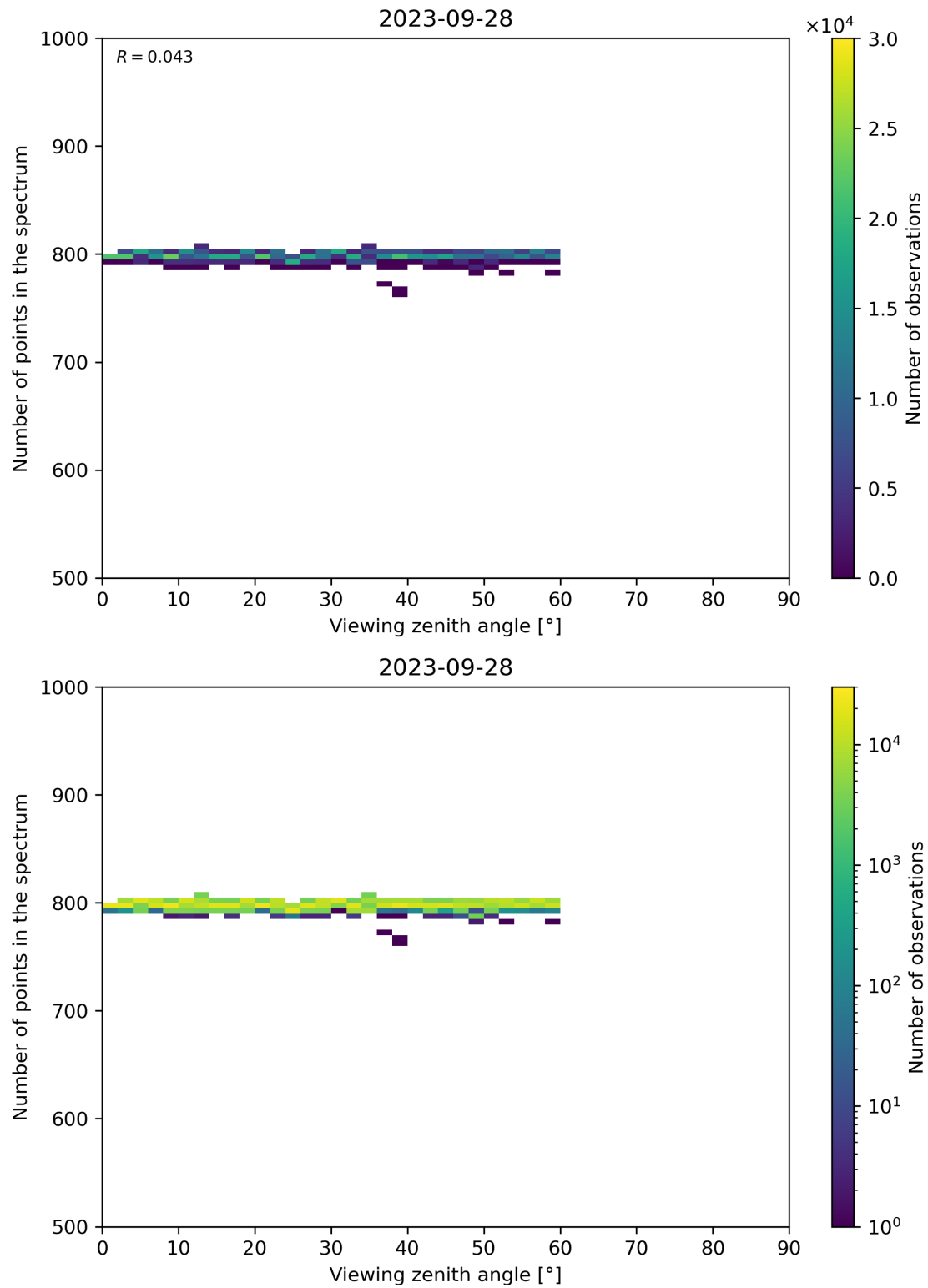
Figure 114: Scatter density plot of “Viewing zenith angle” against “Number of points in the spectrum” for 2023-09-27 to 2023-09-29.
