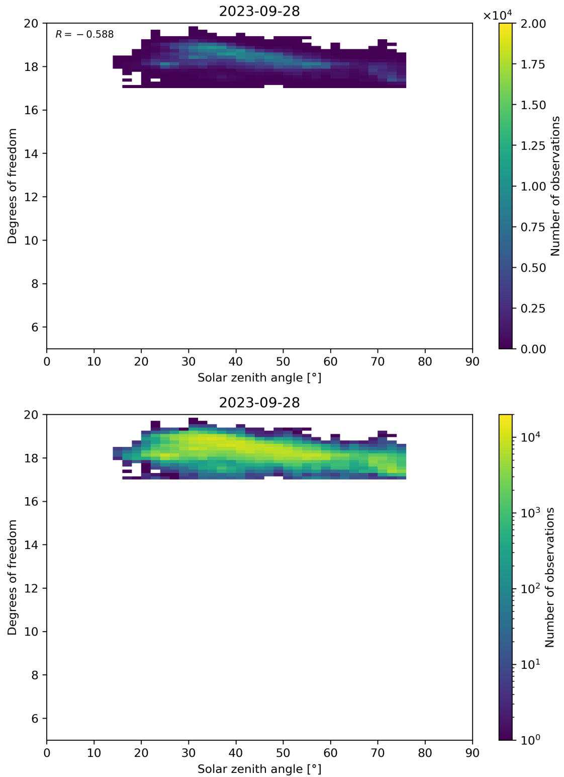
Figure 96: Scatter density plot of “Solar zenith angle” against “Degrees of freedom” for 2023-09-27 to 2023-09-29.
