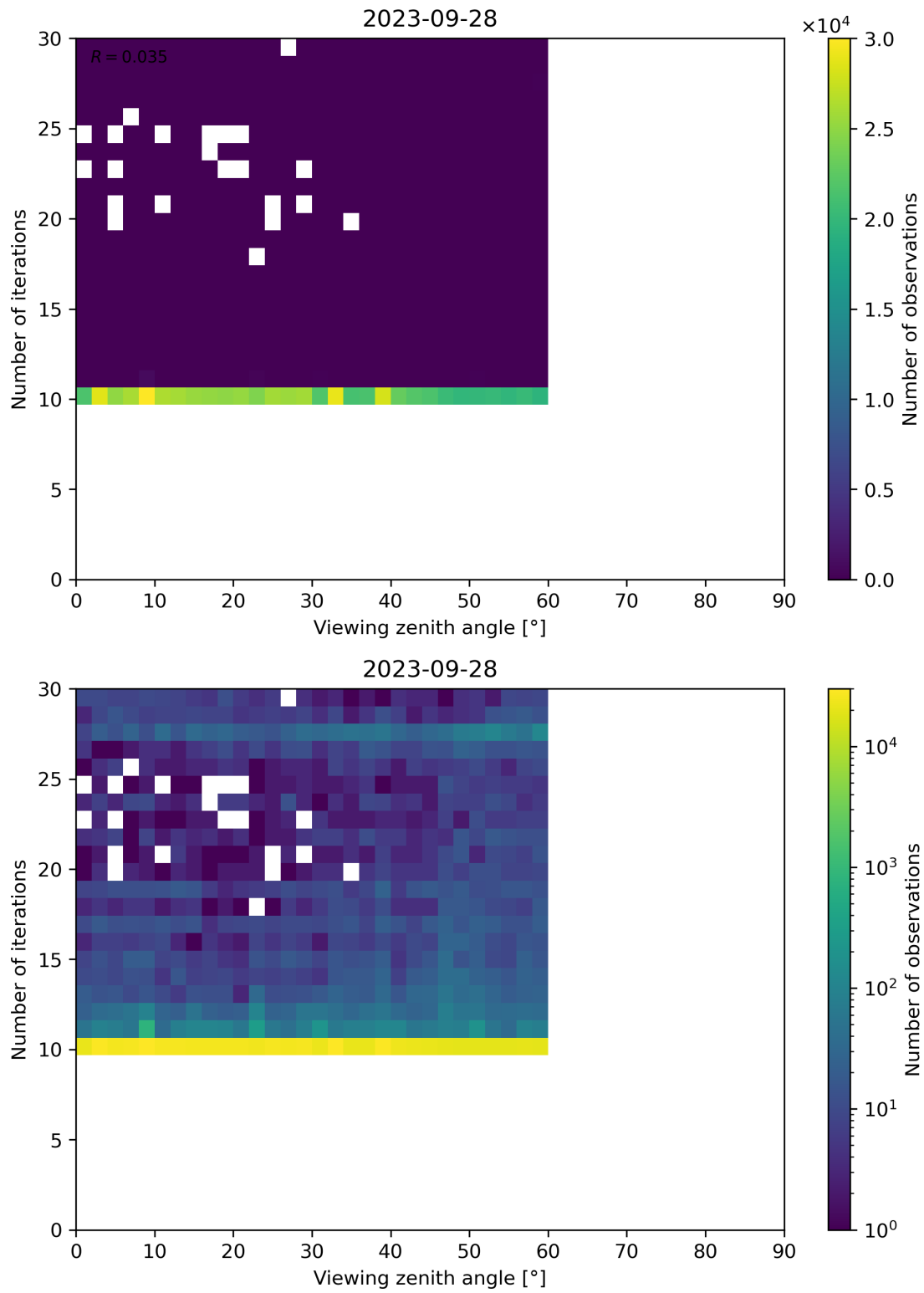
Figure 113: Scatter density plot of “Viewing zenith angle” against “Number of iterations” for 2023-09-27 to 2023-09-29.
