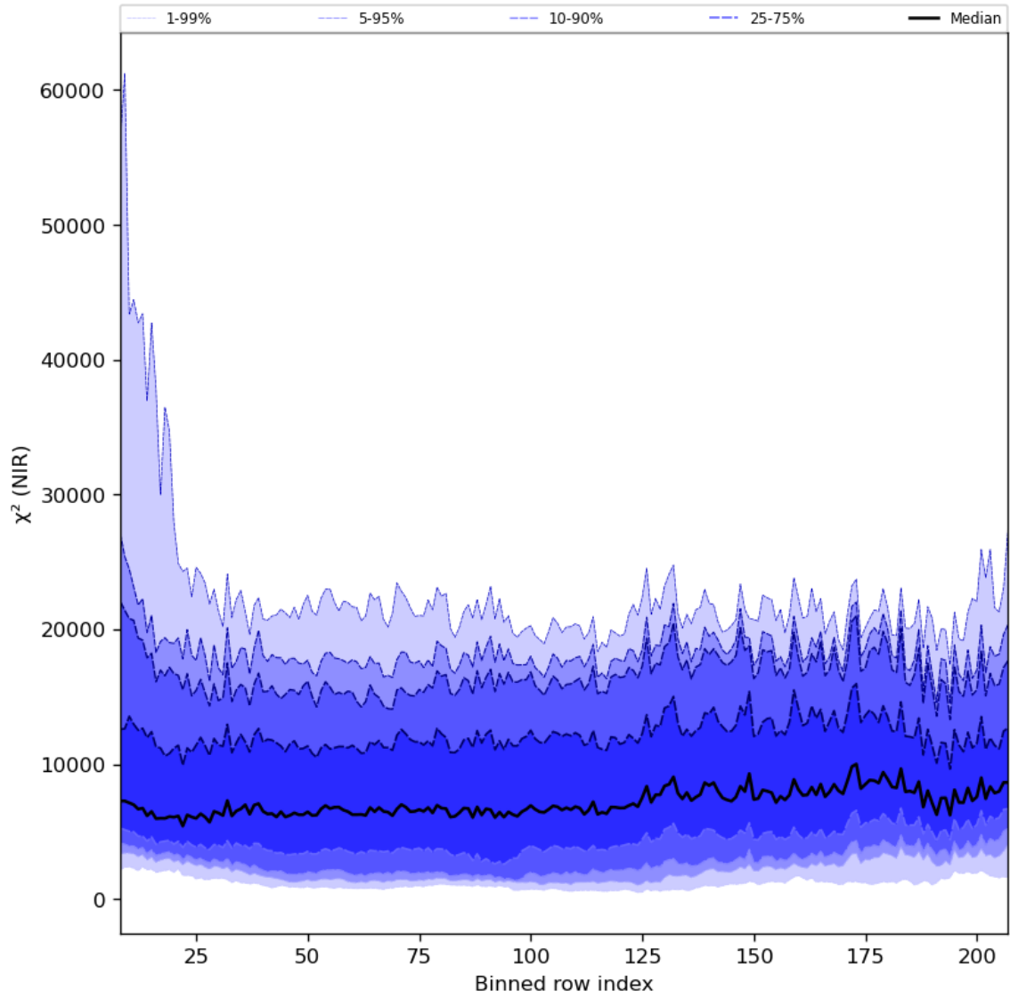
Figure 40: Along track statistics of “ \chi^2 (NIR)” for 2023-09-27 to 2023-09-29
