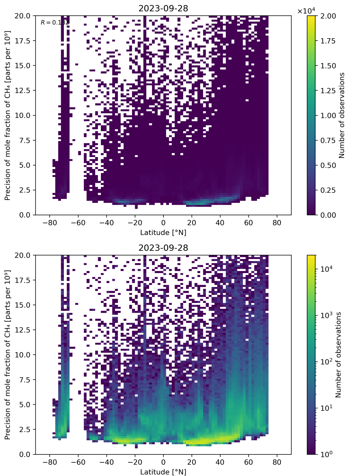
Figure 59: Scatter density plot of “Latitude” against “Precision of mole fraction of CH 4 ” for 2023-09-27 to 2023-09-29.
