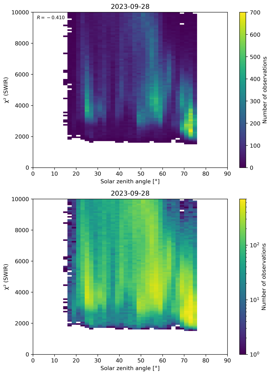
Figure 95: Scatter density plot of “Solar zenith angle” against “ \chi^2 (SWIR)” for 2023-09-27 to 2023-09-29.
