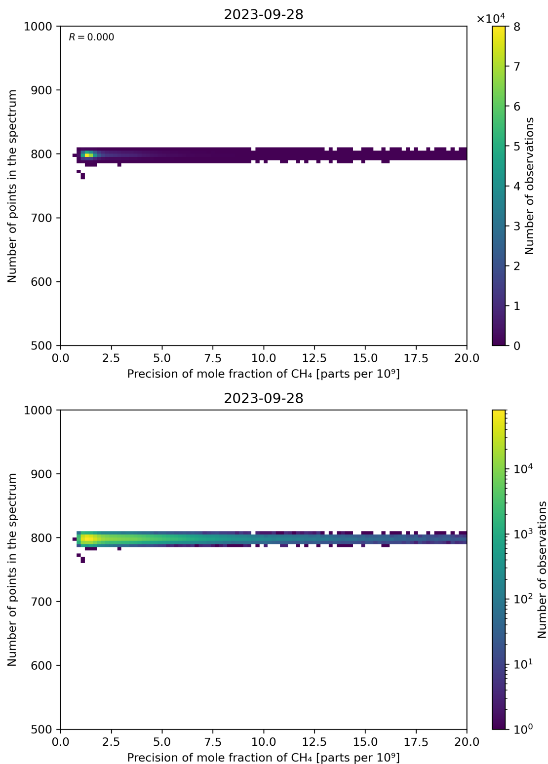
Figure 84: Scatter density plot of “Precision of mole fraction of \text{CH}_4 ” against “Number of points in the spectrum” for 2023-09-27 to 2023-09-29.
