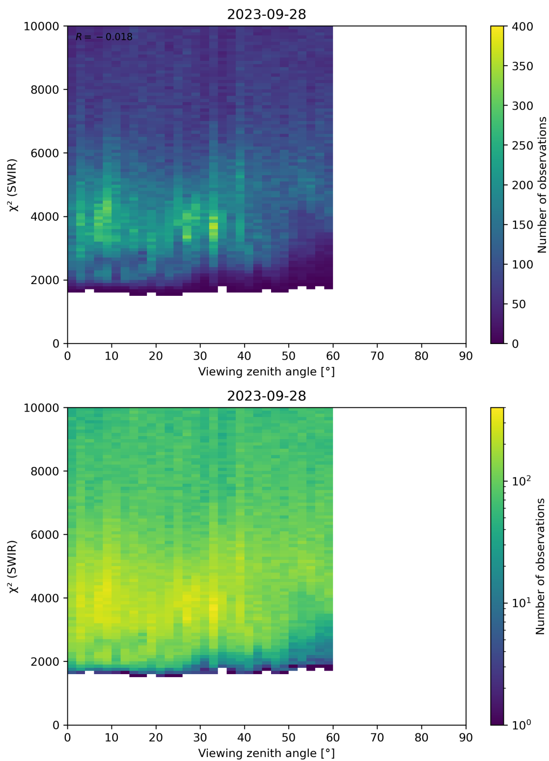
Figure 106: Scatter density plot of “Viewing zenith angle” against “ \chi^2 (SWIR)” for 2023-09-27 to 2023-09-29.
