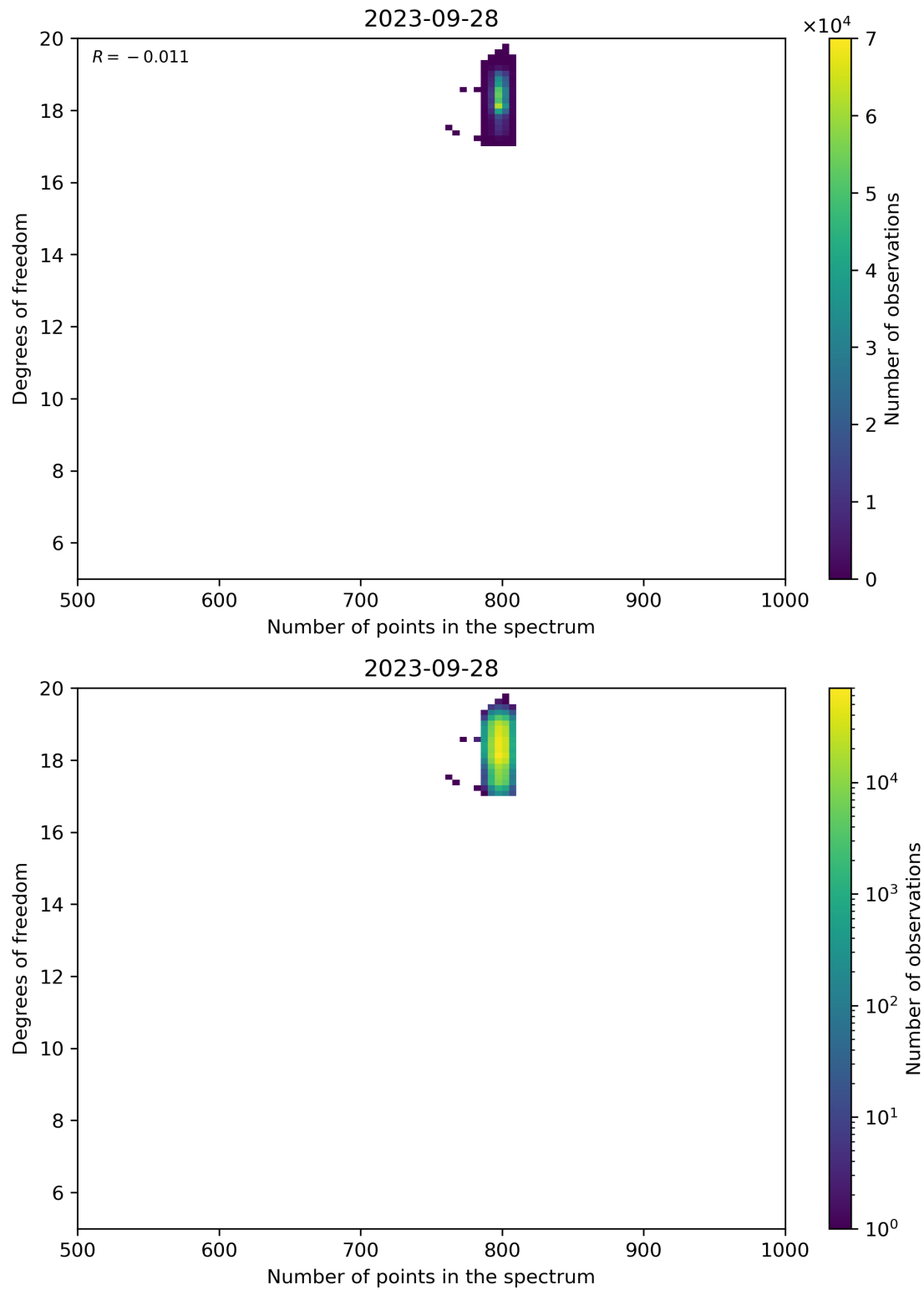
Figure 90: Scatter density plot of “Number of points in the spectrum” against “Degrees of freedom” for 2023-09-27 to 2023-09-29.
