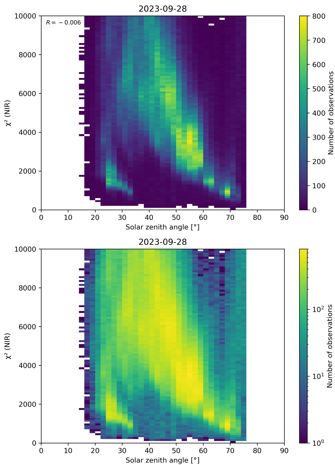
Figure 94: Scatter density plot of “Solar zenith angle” against “ \chi^2 (NIR)” for 2023-09-27 to 2023-09-29.
