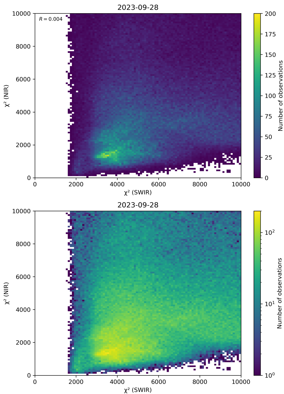
Figure 47: Scatter density plot of “ \chi^2 (SWIR)” against “ \chi^2 (NIR)” for 2023-09-27 to 2023-09-29.
