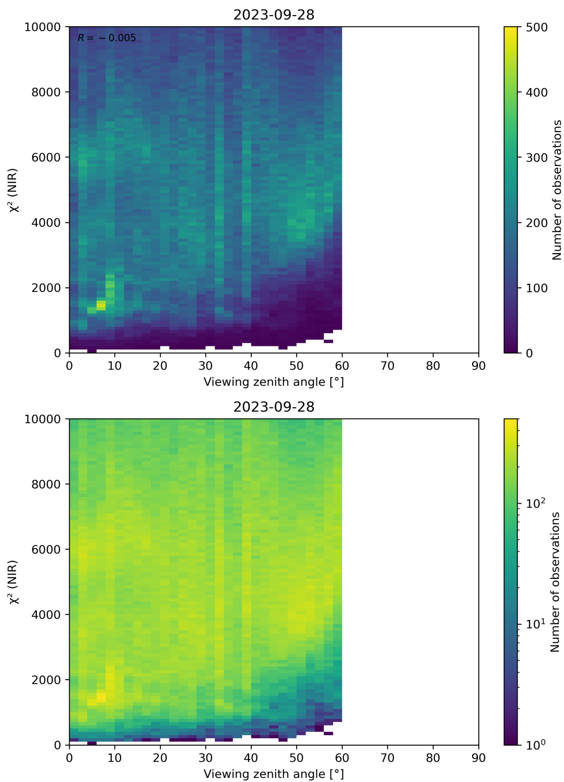
Figure 105: Scatter density plot of “Viewing zenith angle” against “ \chi^2 (NIR)” for 2023-09-27 to 2023-09-29.
