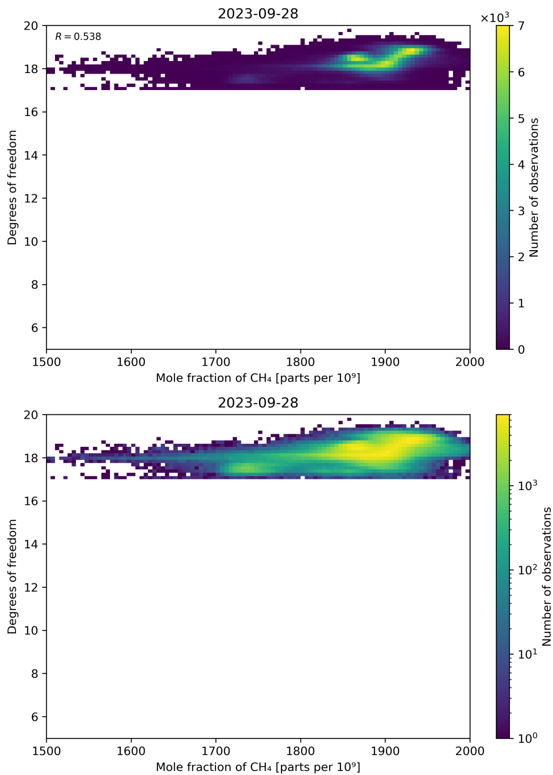
Figure 72: Scatter density plot of “Mole fraction of CH 4 ” against “Degrees of freedom” for 2023-09-27 to 2023-09-29.
