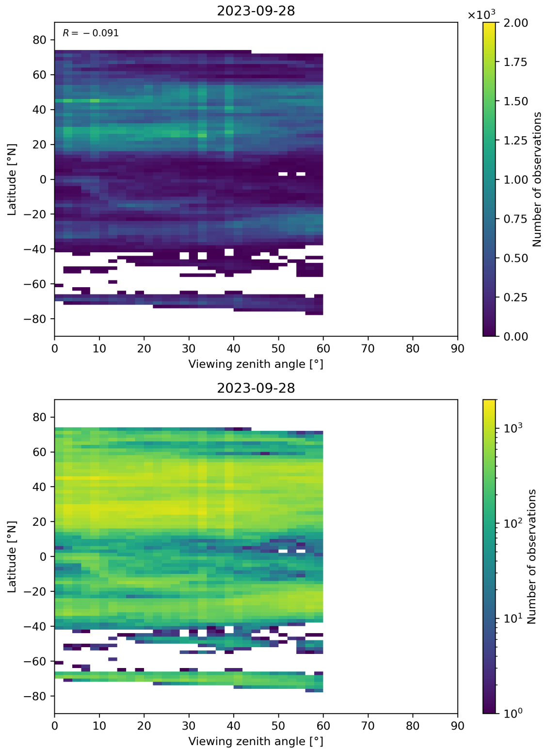
Figure 109: Scatter density plot of “Viewing zenith angle” against “Latitude” for 2023-09-27 to 2023-09-29.
