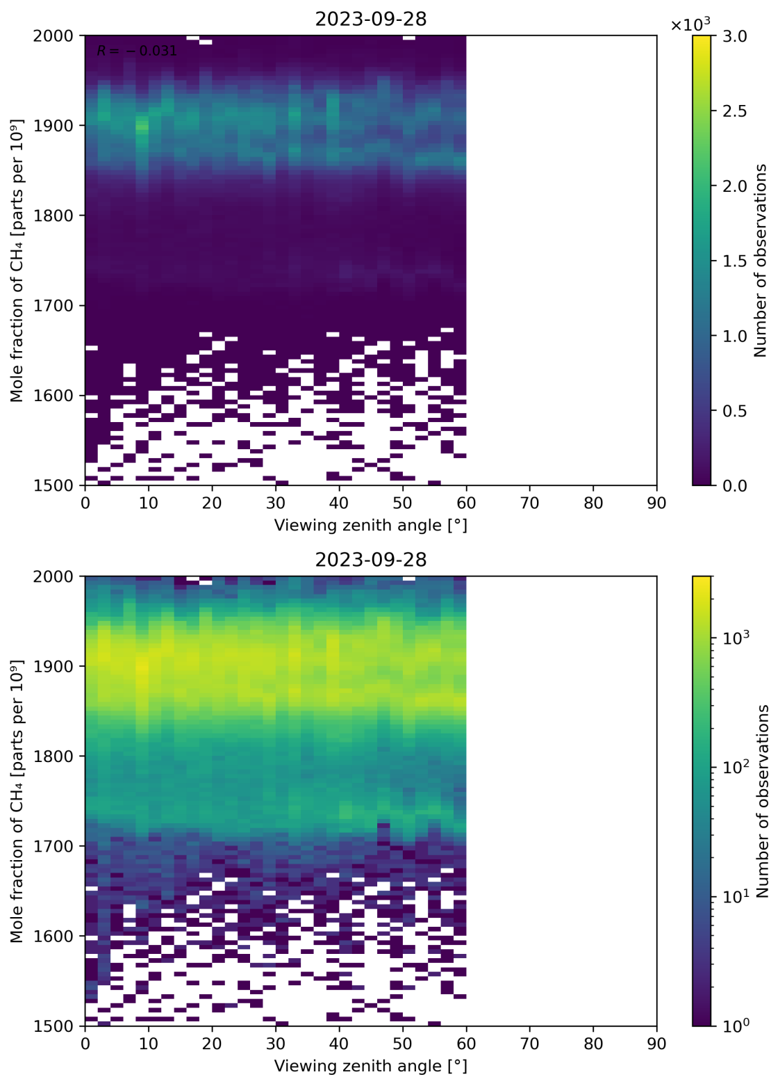
Figure 110: Scatter density plot of “Viewing zenith angle” against “Mole fraction of CH 4 ” for 2023-09-27 to 2023-09-29.
