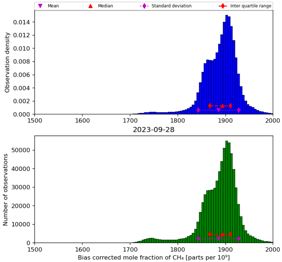
Figure 25: Histogram of “Bias corrected mole fraction of CH 4 ” for 2023-09-27 to 2023-09-29
