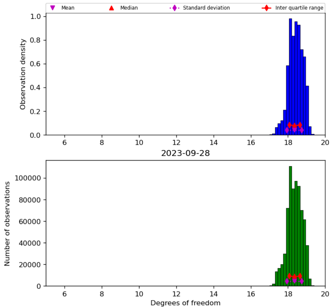
Figure 30: Histogram of “Degrees of freedom” for 2023-09-27 to 2023-09-29
