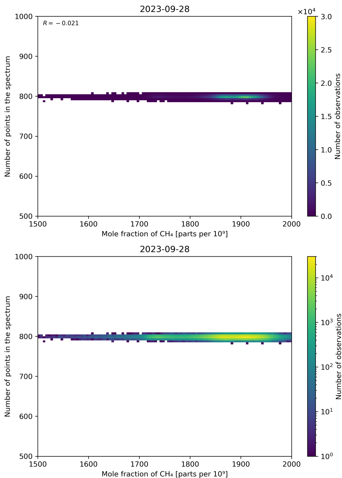
Figure 77: Scatter density plot of “Mole fraction of CH 4 ” against “Number of points in the spectrum” for 2023-09-27 to 2023-09-29.
