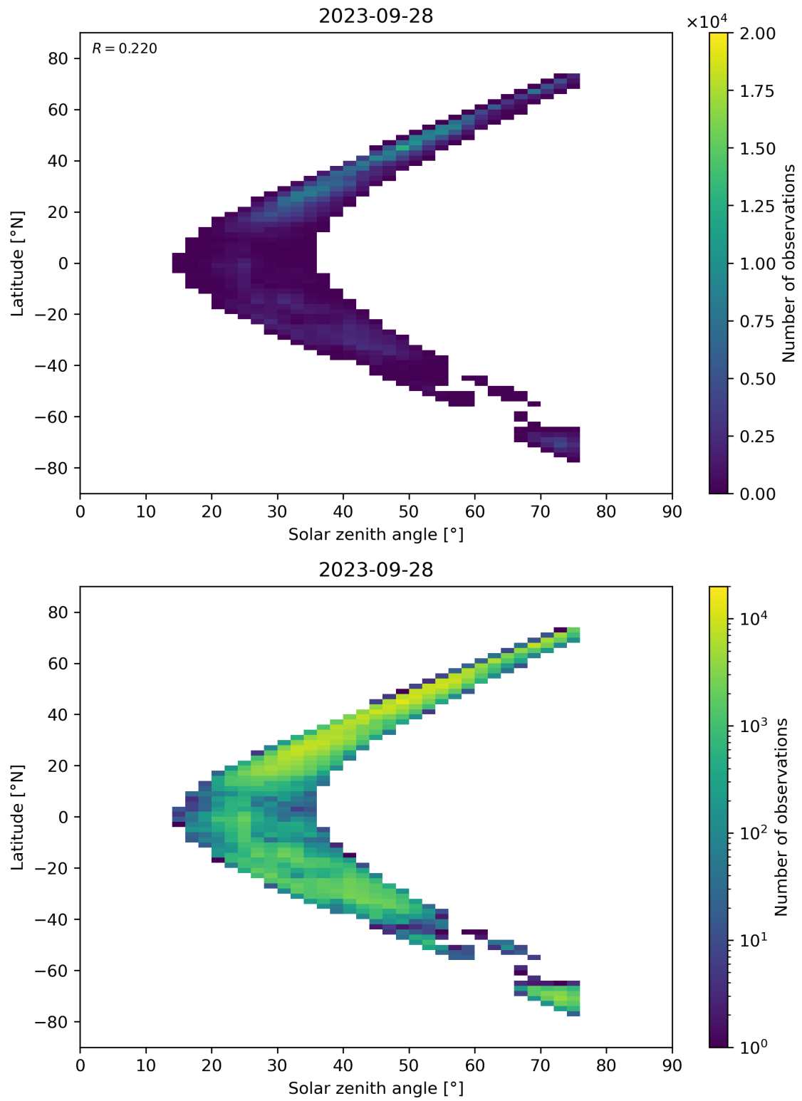
Figure 98: Scatter density plot of “Solar zenith angle” against “Latitude” for 2023-09-27 to 2023-09-29.
