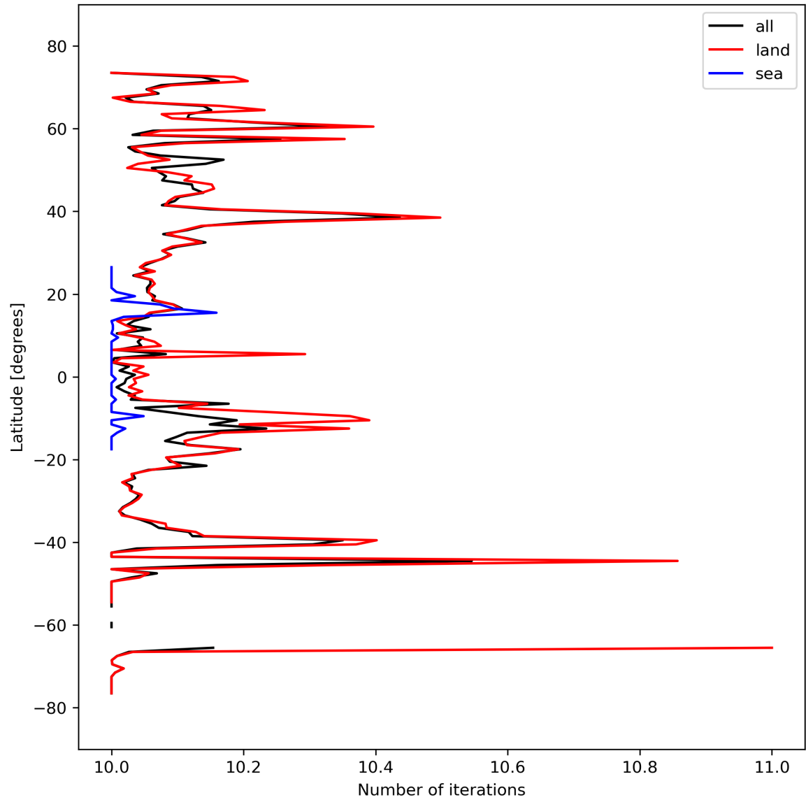
Figure 20: Zonal average of “Number of iterations” for 2023-09-27 to 2023-09-29.
