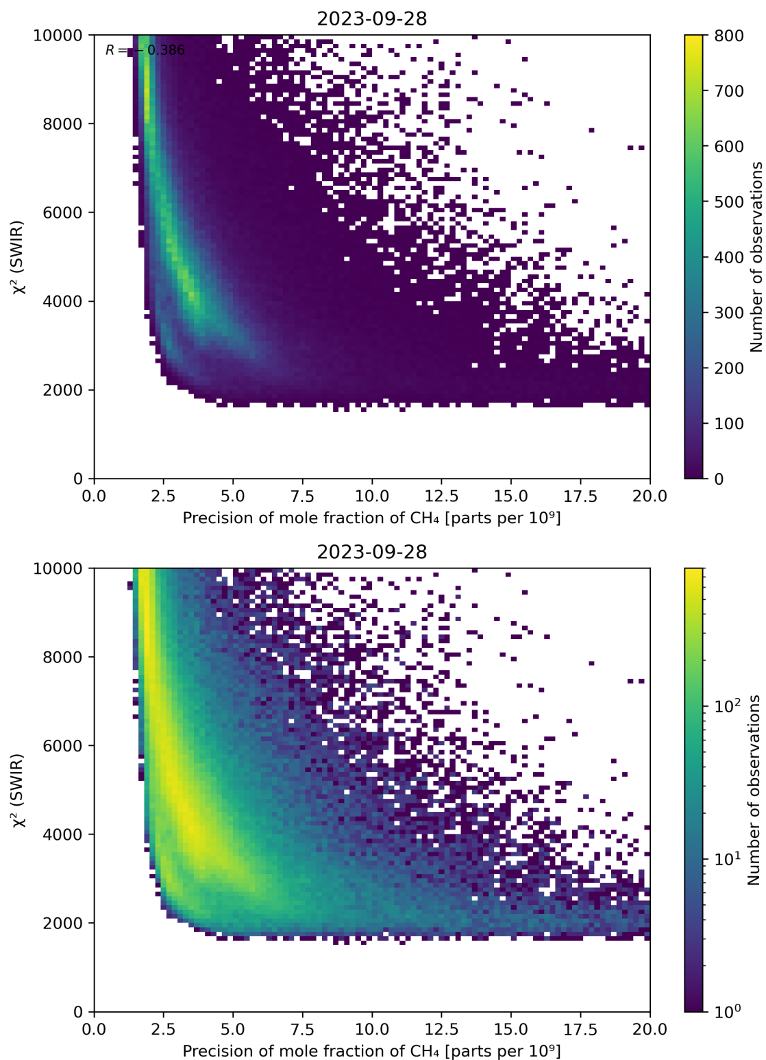
Figure 79: Scatter density plot of “Precision of mole fraction of \text{CH}_4 ” against “ \chi^2 (SWIR)” for 2023-09-27 to 2023-09-29.
