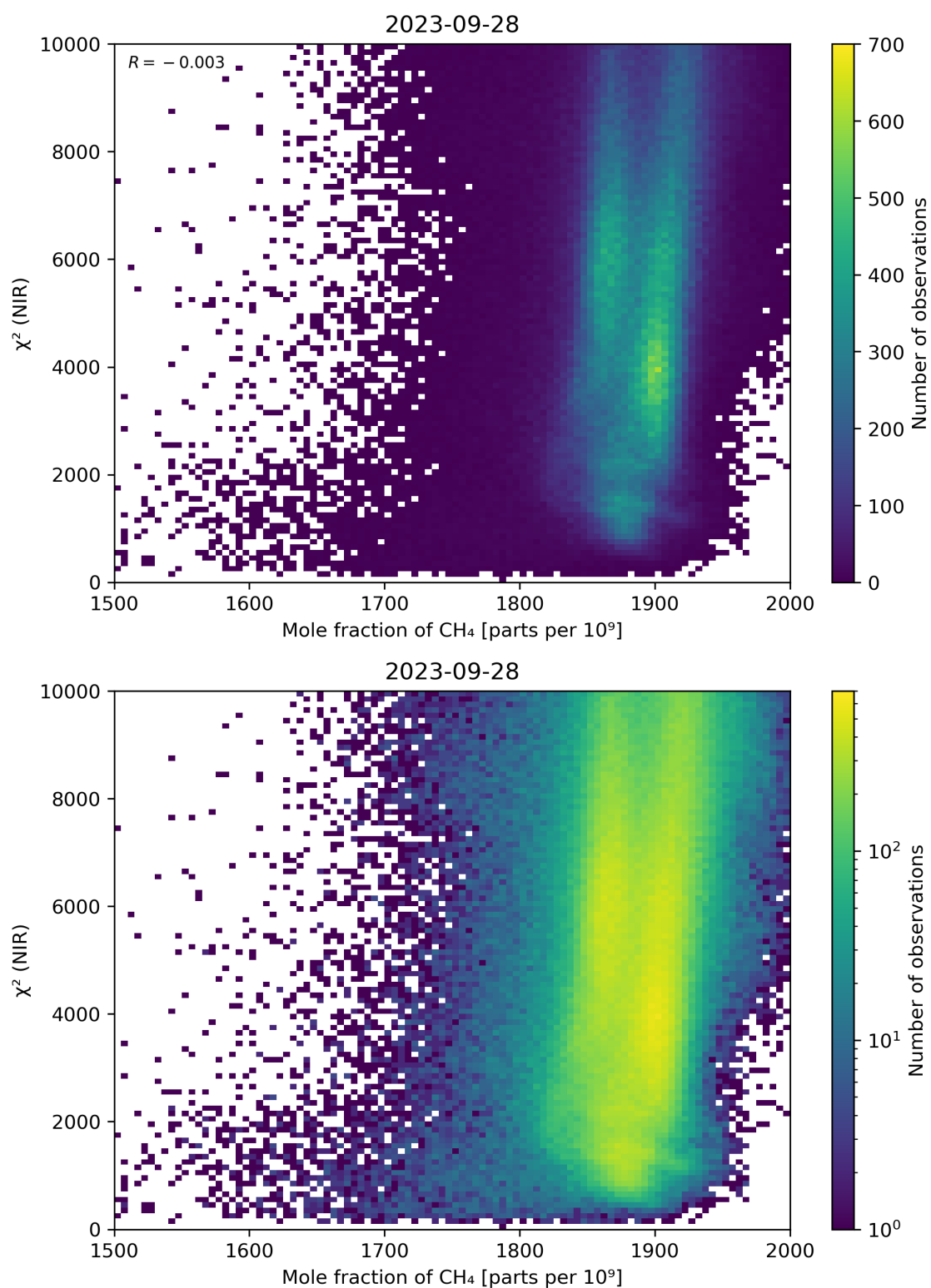
Figure 70: Scatter density plot of “Mole fraction of CH 4 ” against “ \chi^2 (NIR)” for 2023-09-27 to 2023-09-29.
