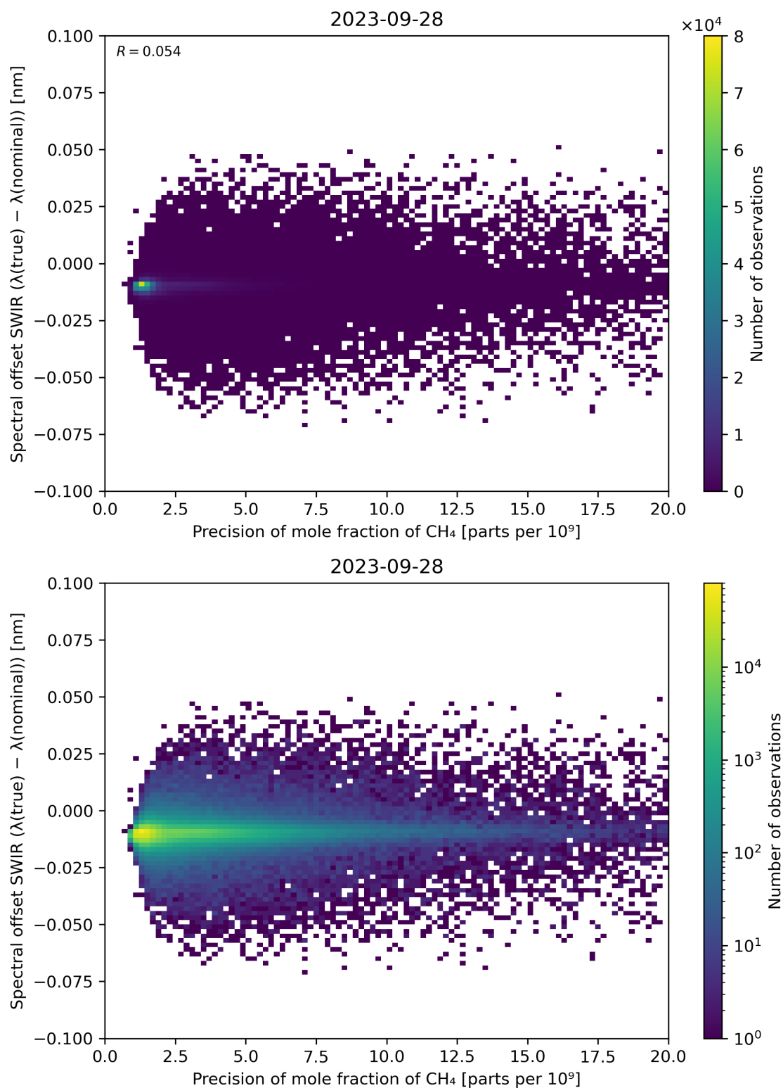
Figure 85: Scatter density plot of “Precision of mole fraction of CH 4 ” against “Spectral offset SWIR ( \lambda(\text{true}) - \lambda(\text{nominal}) )” for 2023-09-27 to 2023-09-29.
