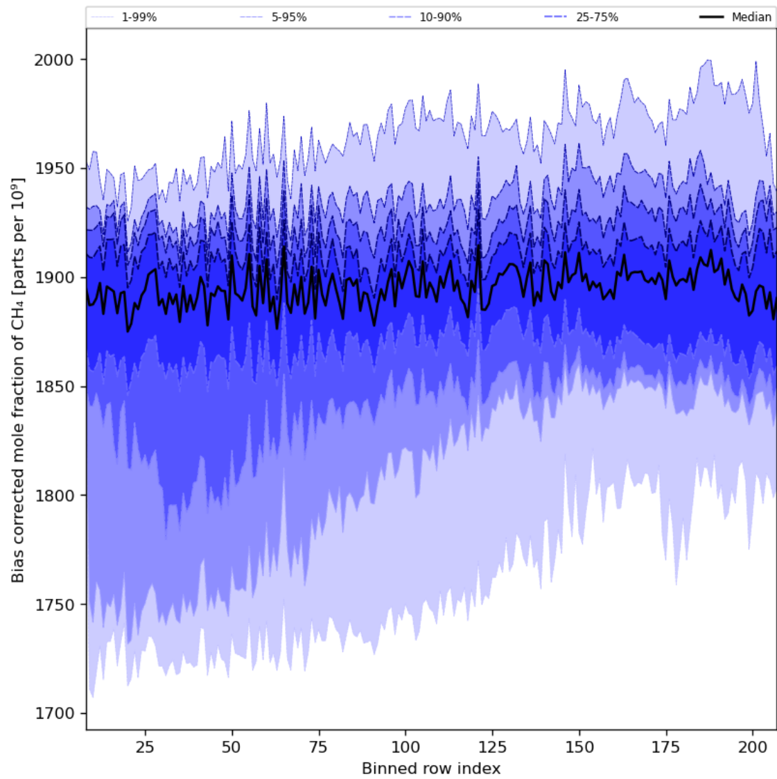
Figure 36: Along track statistics of “Bias corrected mole fraction of CH 4 ” for 2023-09-27 to 2023-09-29
