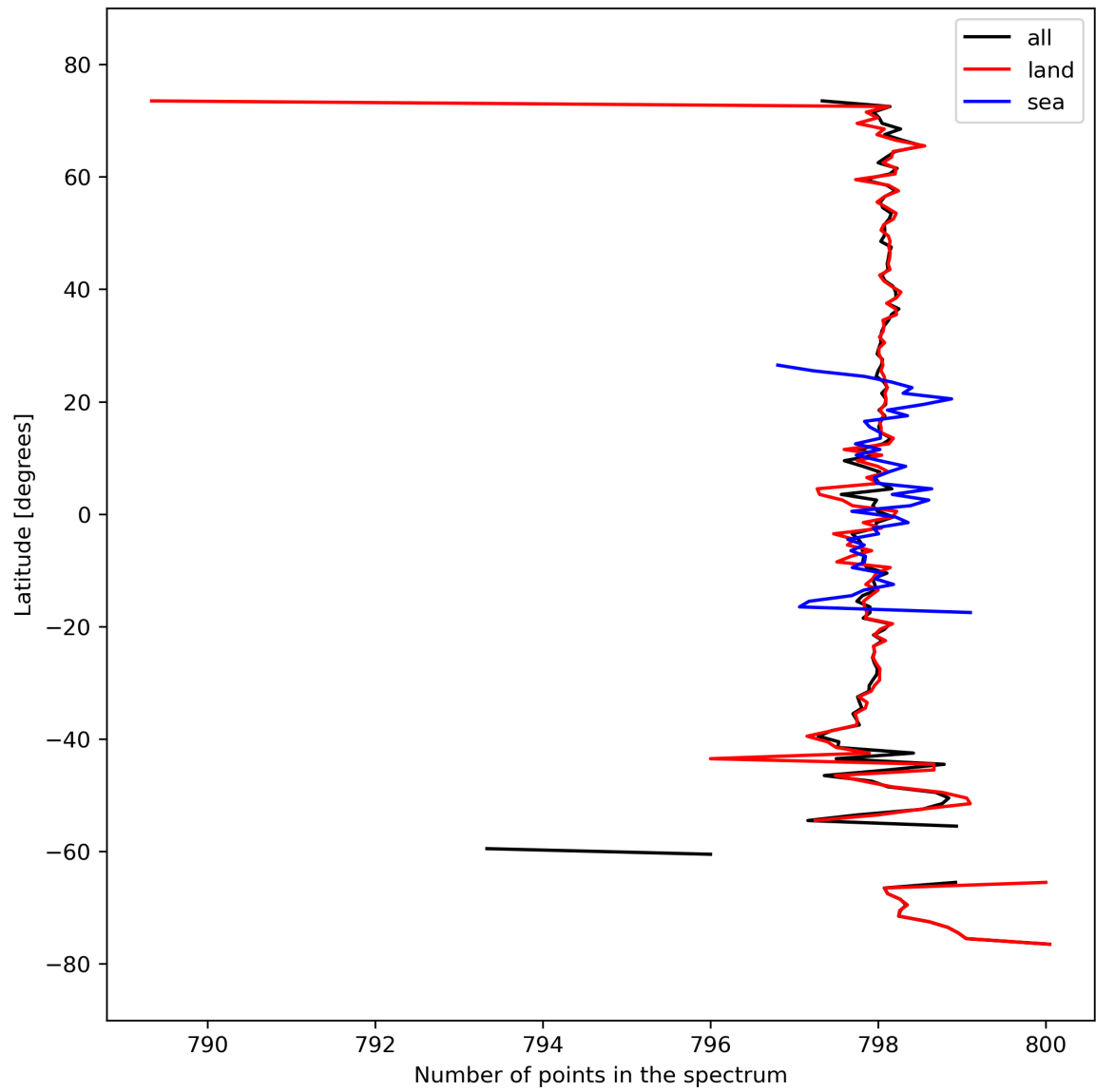
Figure 15: Zonal average of “Number of points in the spectrum” for 2023-09-27 to 2023-09-29.
