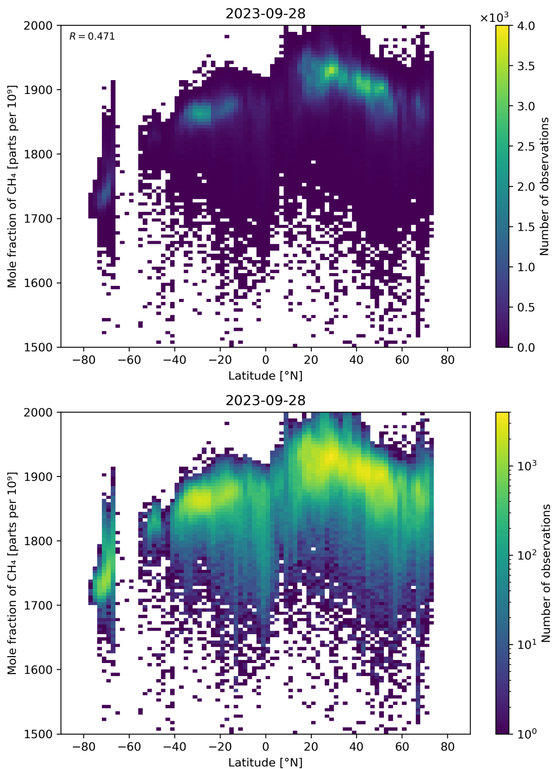
Figure 57: Scatter density plot of “Latitude” against “Mole fraction of \text{CH}_4 ” for 2023-09-27 to 2023-09-29.
