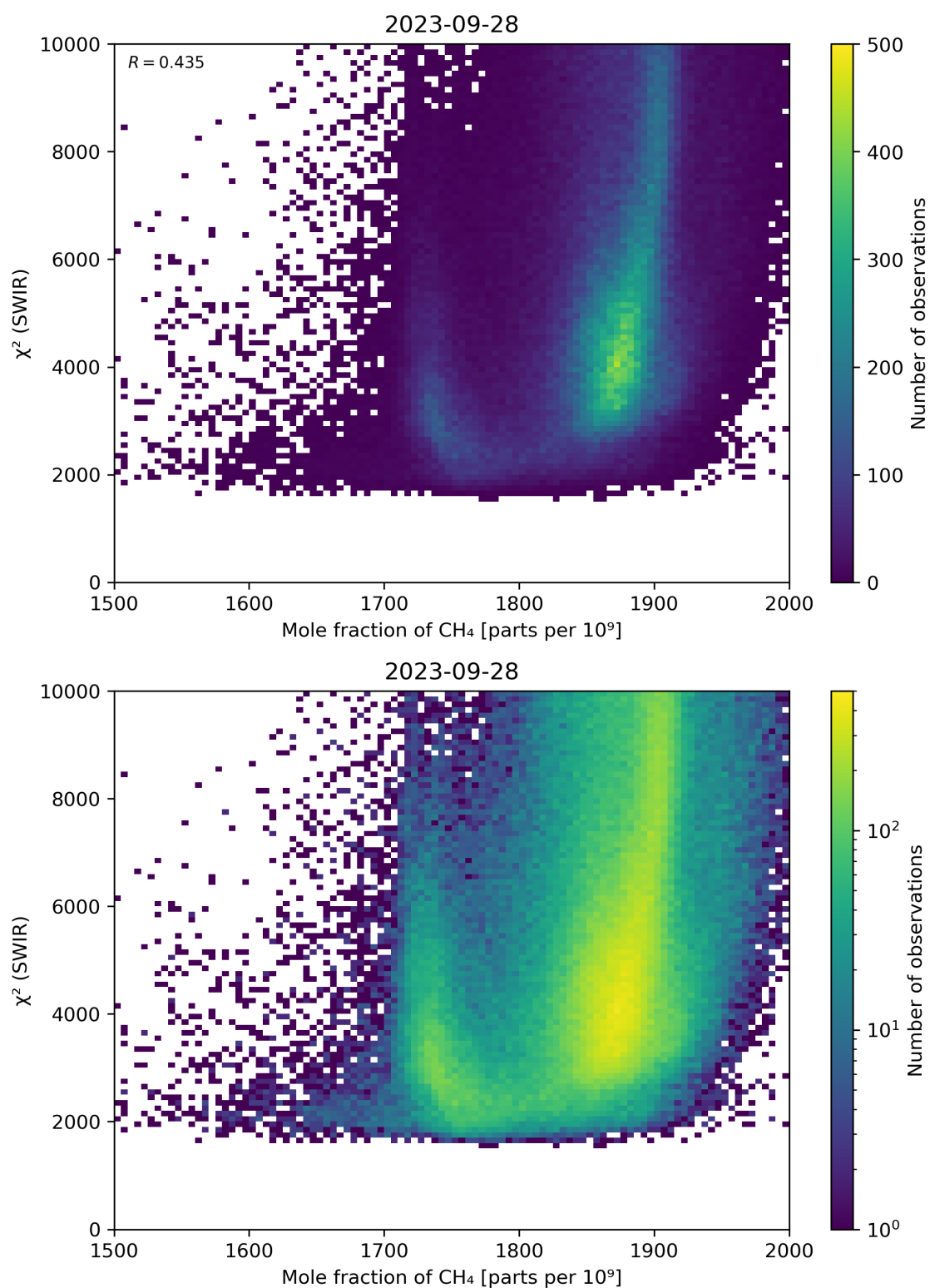
Figure 71: Scatter density plot of “Mole fraction of \text{CH}_4 ” against “ \chi^2 (SWIR)” for 2023-09-27 to 2023-09-29.
