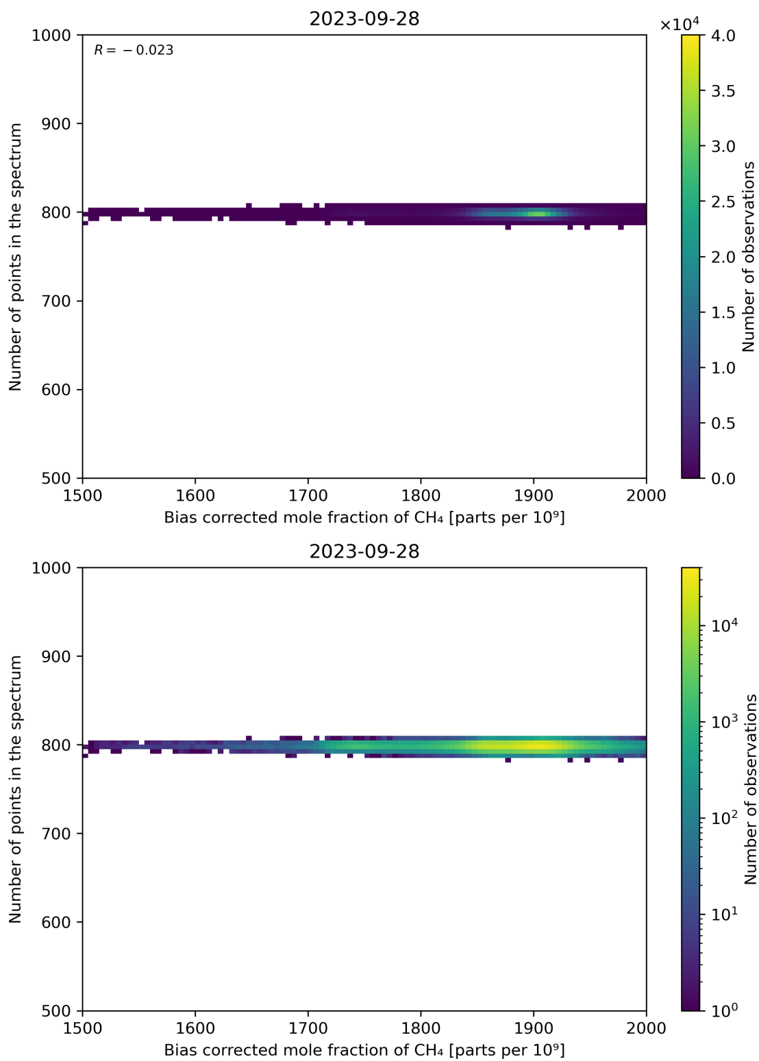
Figure 68: Scatter density plot of “Bias corrected mole fraction of CH 4 ” against “Number of points in the spectrum” for 2023-09-27 to 2023-09-29.
