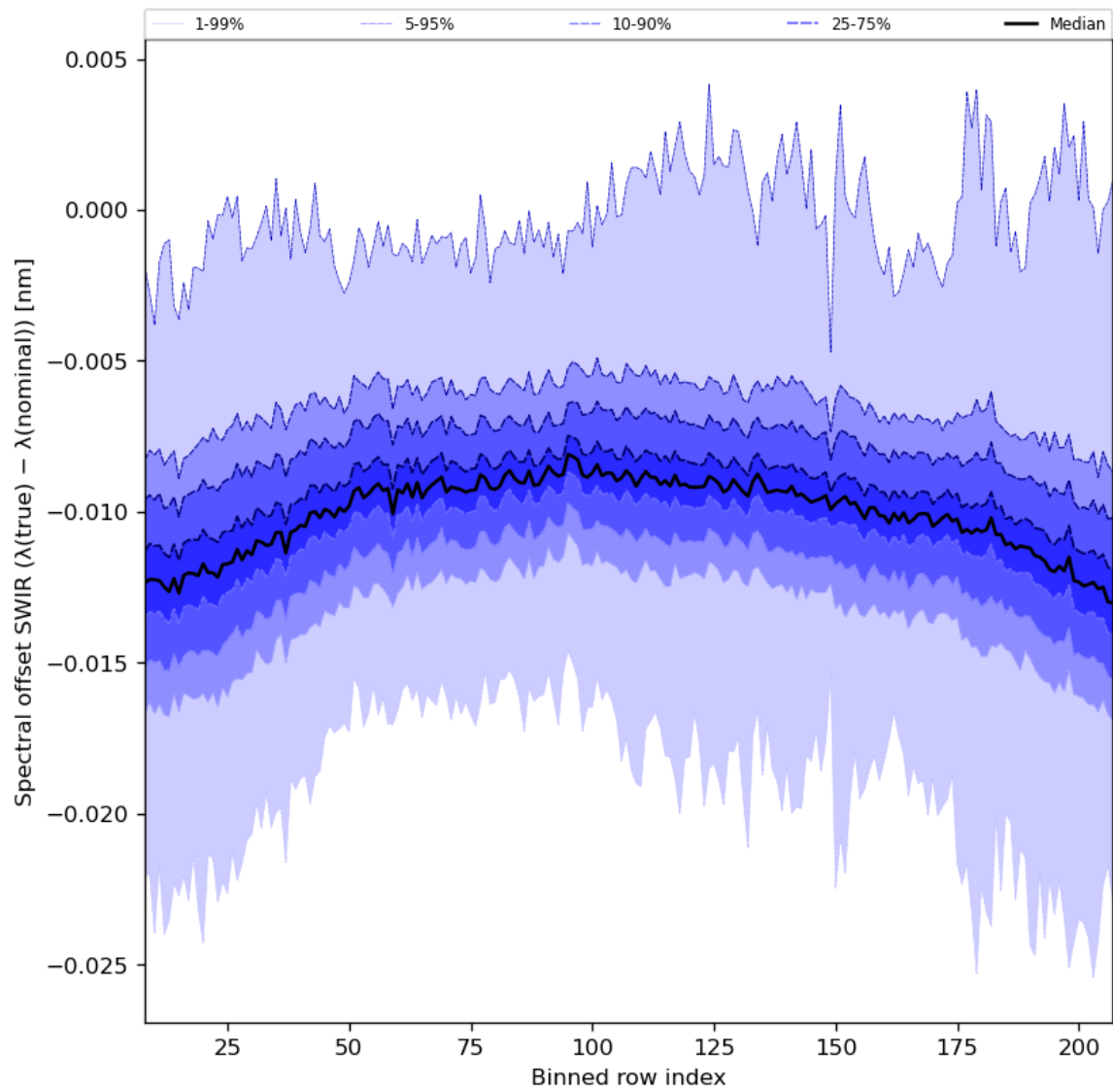
Figure 38: Along track statistics of “Spectral offset SWIR ( \lambda(\text{true}) - \lambda(\text{nominal}) )” for 2023-09-27 to 2023-09-29
