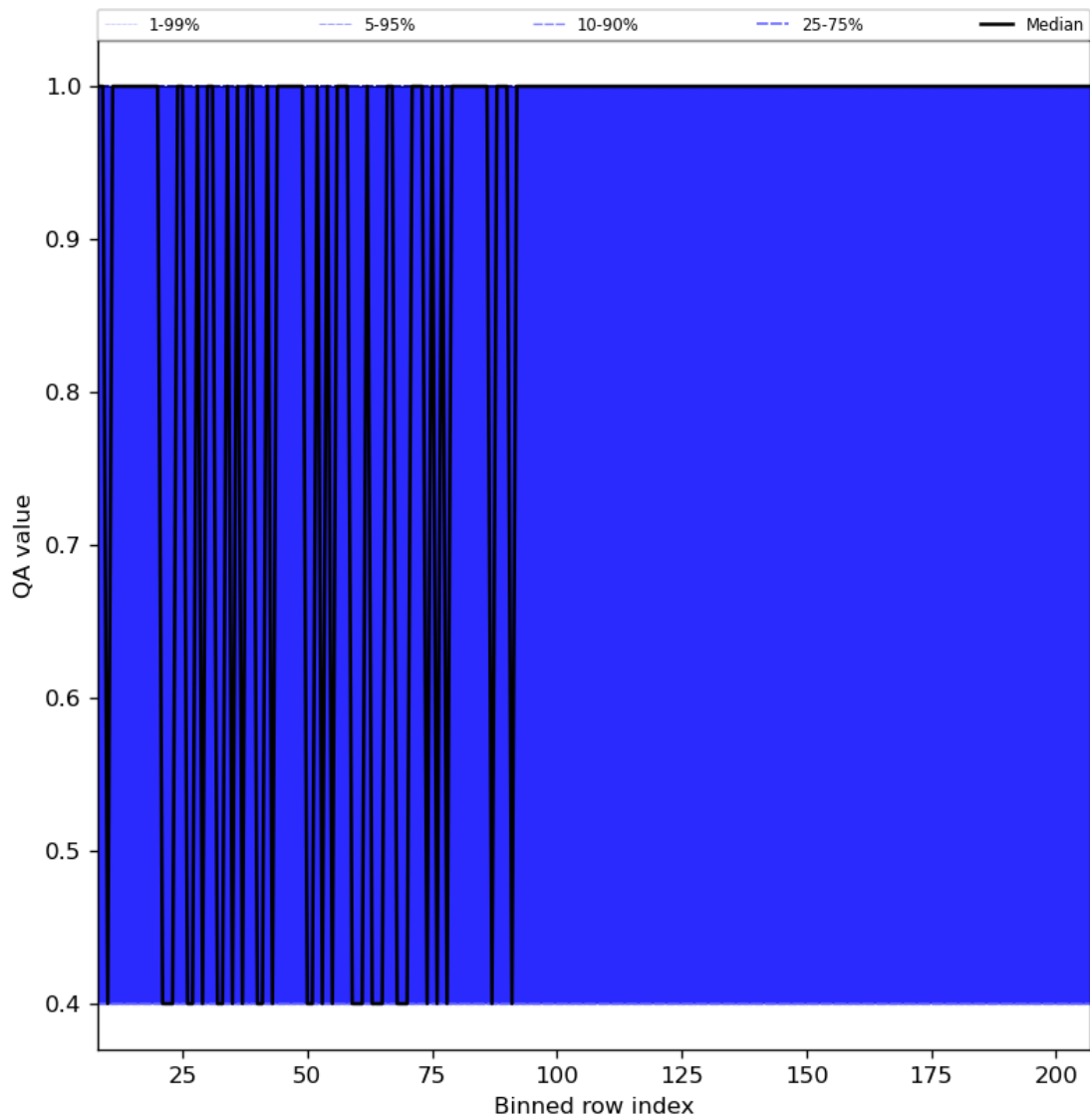
Figure 33: Along track statistics of “QA value” for 2023-09-27 to 2023-09-29
