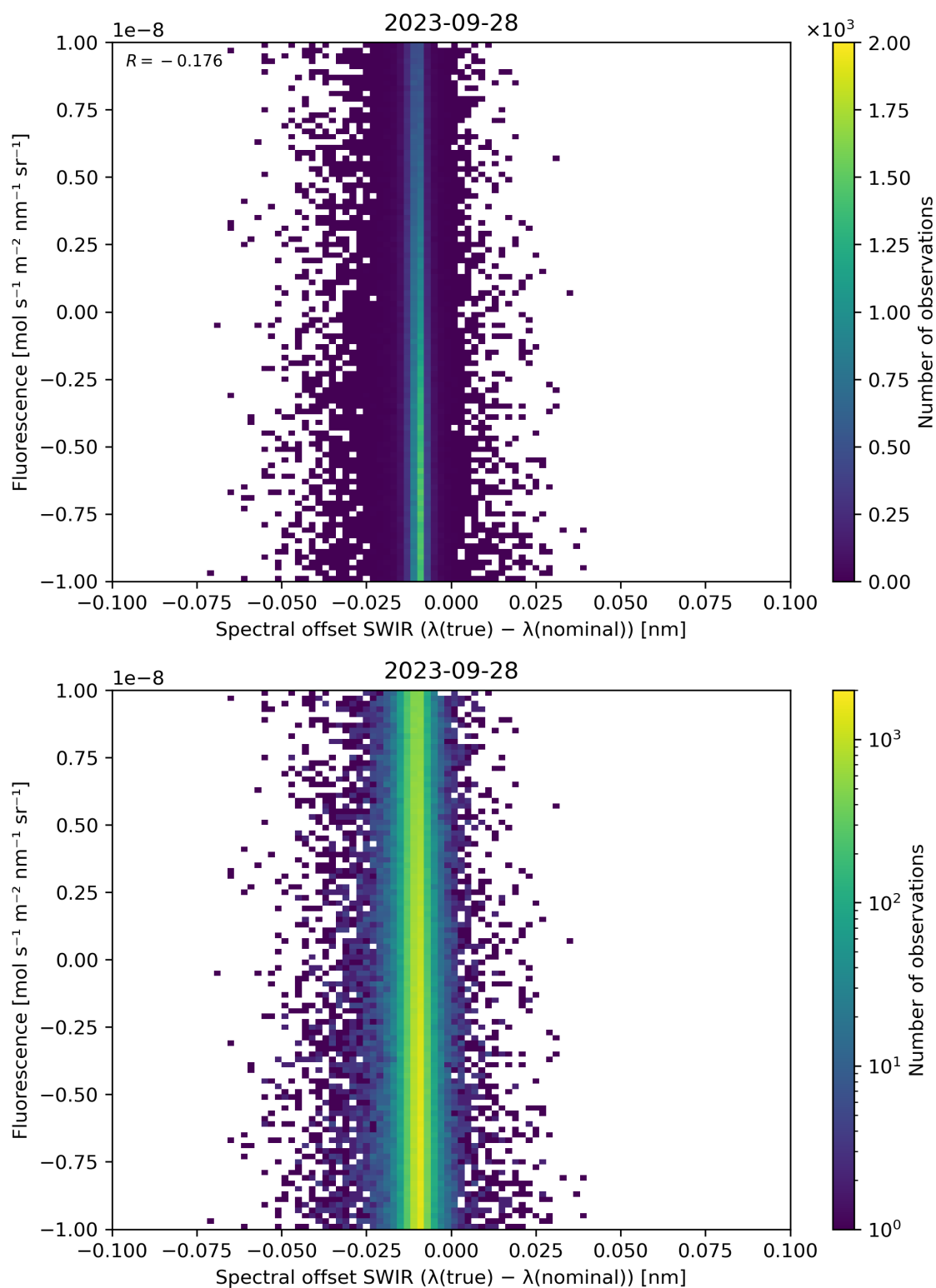
Figure 120: Scatter density plot of “Spectral offset SWIR ( \lambda(\text{true}) - \lambda(\text{nominal}) )” against “Fluorescence” for 2023-09-27 to 2023-09-29.
