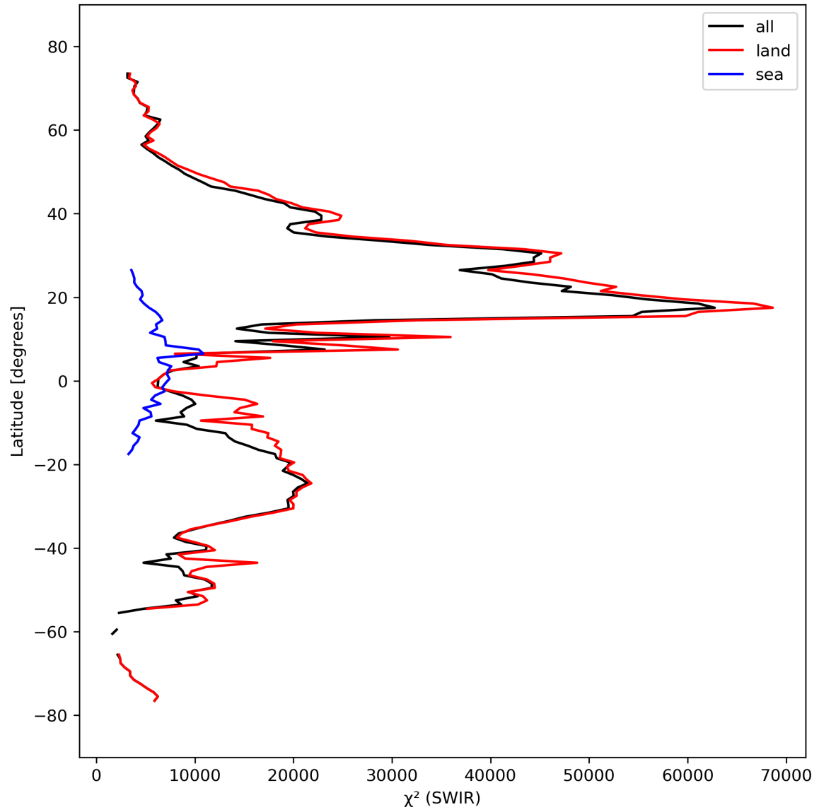
Figure 17: Zonal average of “ \chi^2 (SWIR)” for 2023-09-27 to 2023-09-29.
