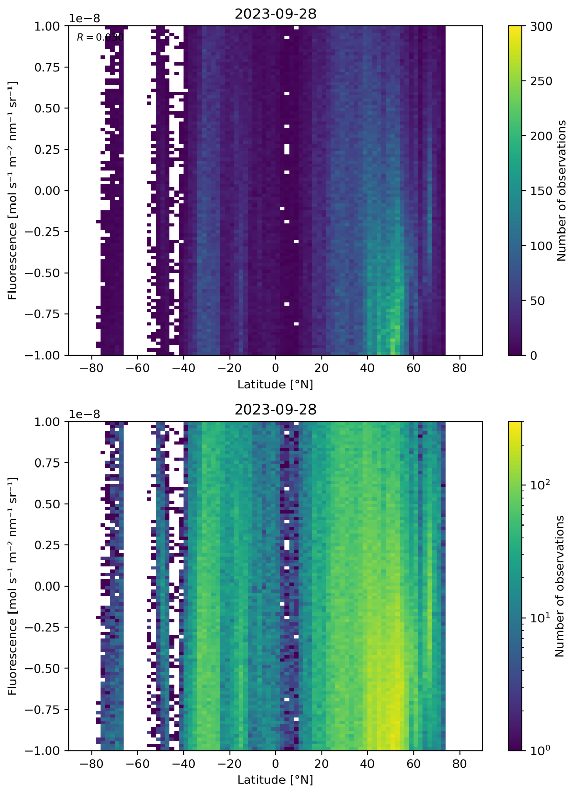
Figure 56: Scatter density plot of “Latitude” against “Fluorescence” for 2023-09-27 to 2023-09-29.
