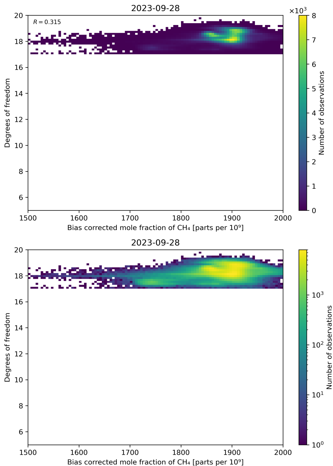
Figure 65: Scatter density plot of “Bias corrected mole fraction of CH 4 ” against “Degrees of freedom” for 2023-09-27 to 2023-09-29.
