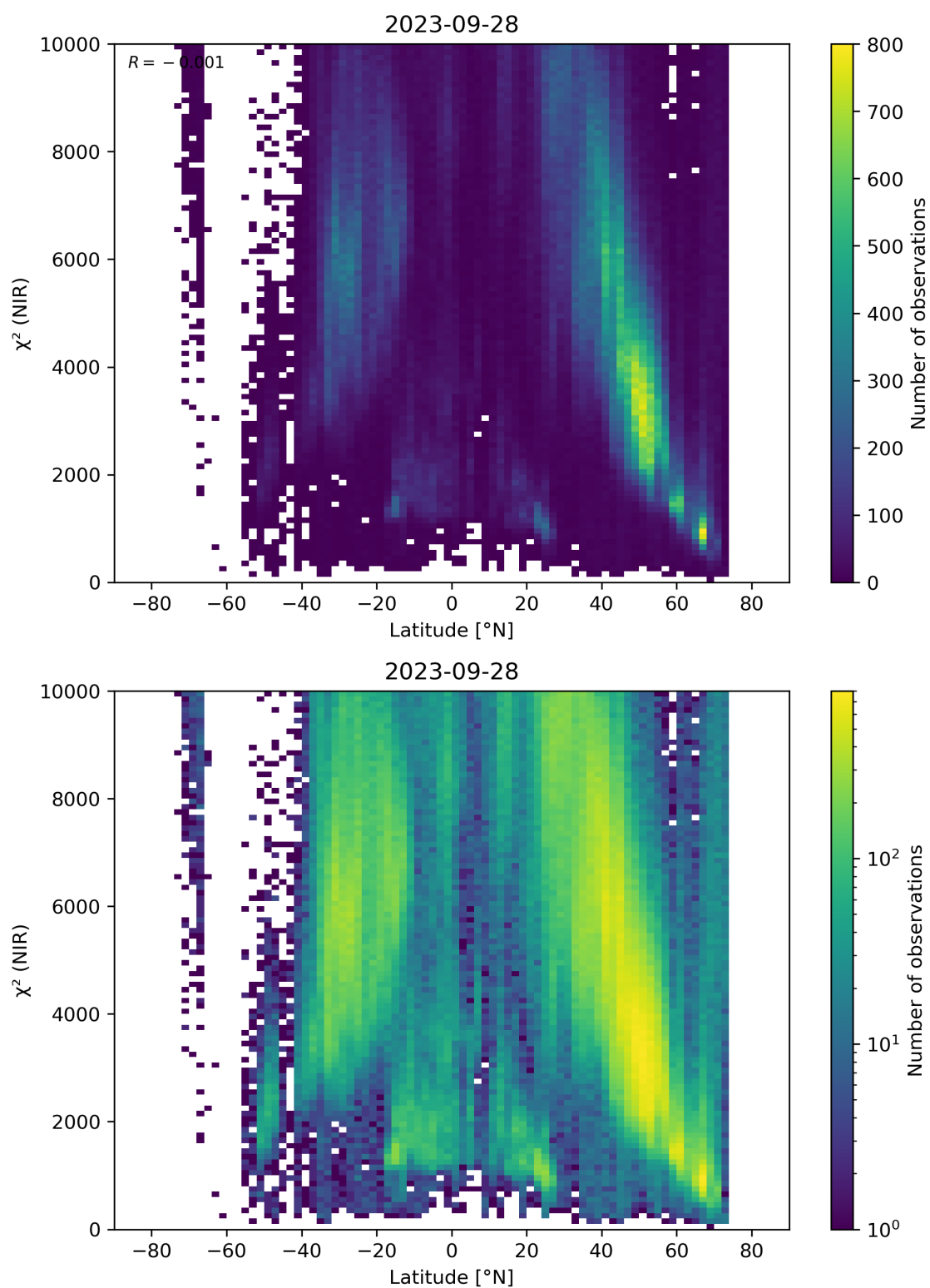
Figure 53: Scatter density plot of “Latitude” against “ \chi^2 (NIR)” for 2023-09-27 to 2023-09-29.
