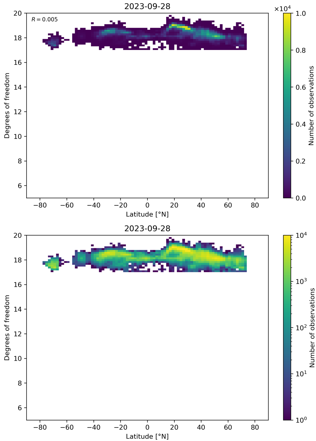
Figure 55: Scatter density plot of “Latitude” against “Degrees of freedom” for 2023-09-27 to 2023-09-29.
