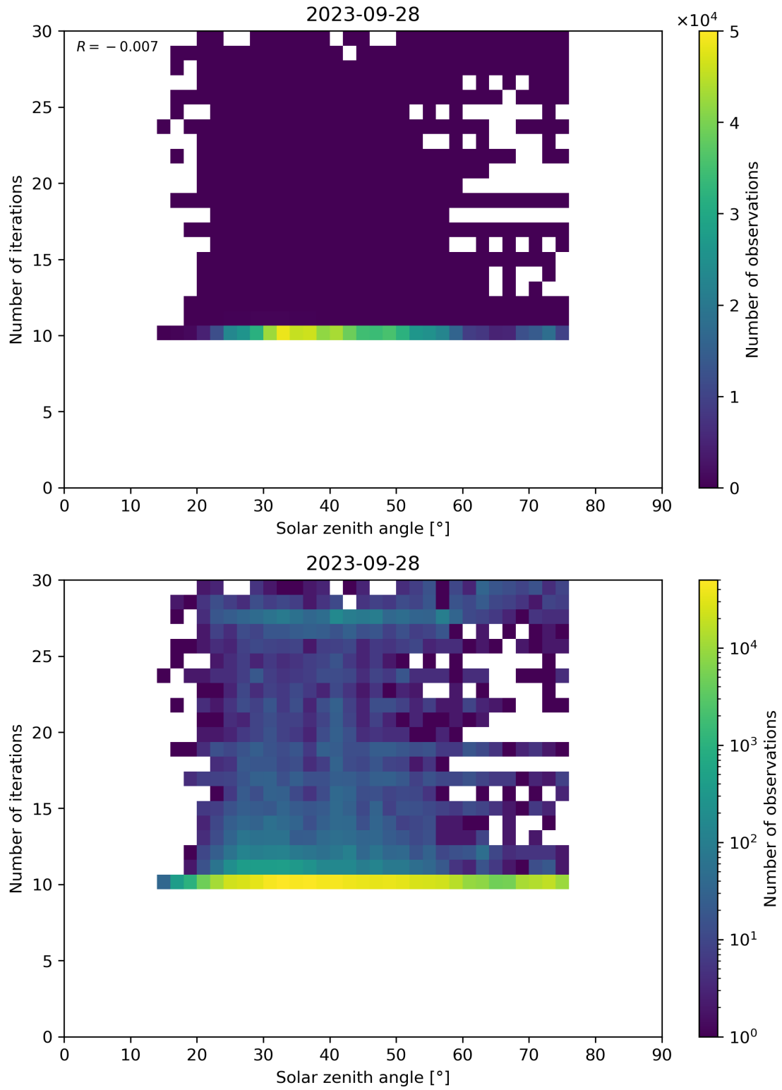
Figure 102: Scatter density plot of “Solar zenith angle” against “Number of iterations” for 2023-09-27 to 2023-09-29.
