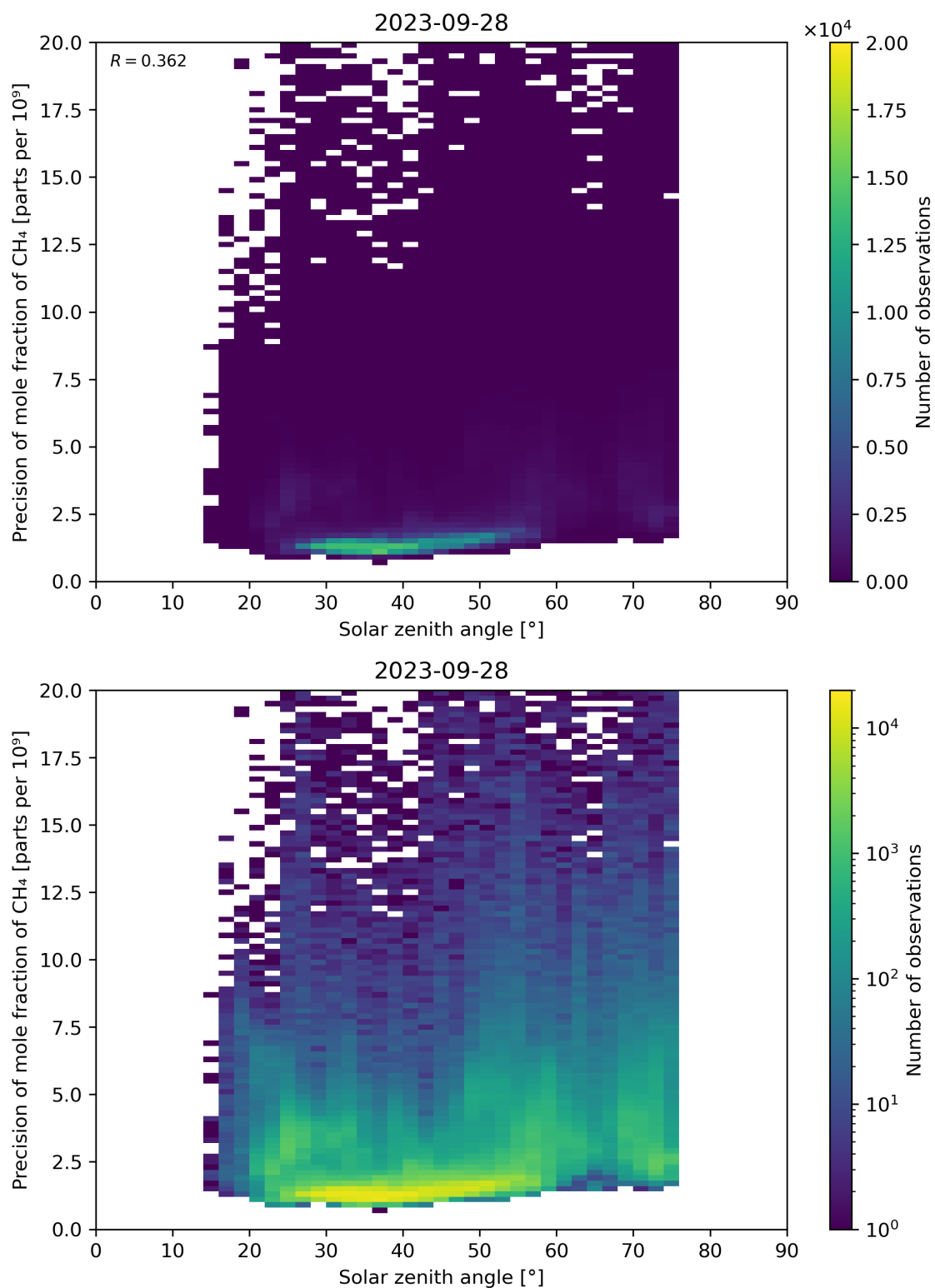
Figure 101: Scatter density plot of “Solar zenith angle” against “Precision of mole fraction of CH 4 ” for 2023-09-27 to 2023-09-29.
