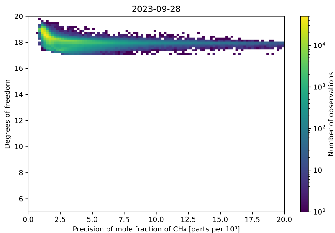
Figure 80: Scatter density plot of “Precision of mole fraction of CH 4 ” against “Degrees of freedom” for 2023-09-27 to 2023-09-29.
