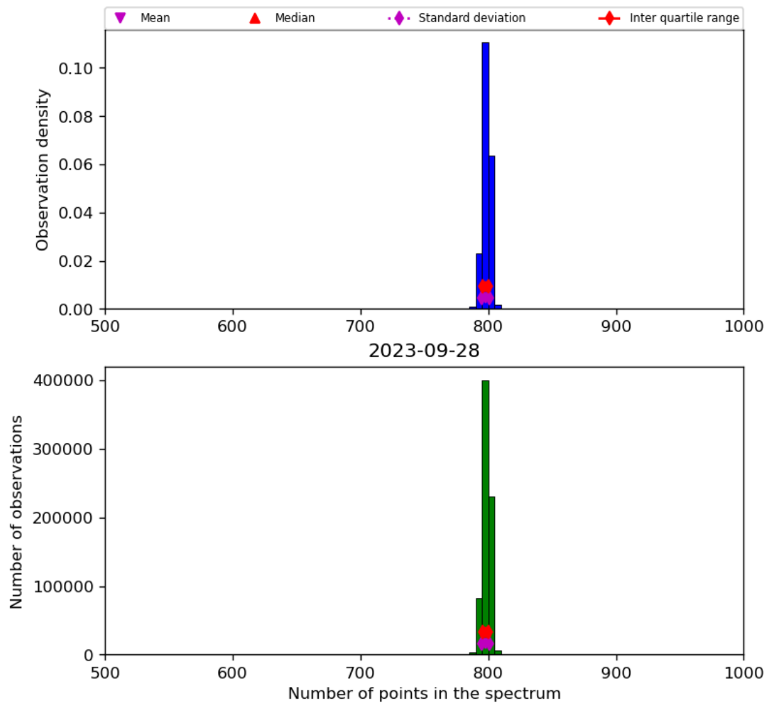
Figure 26: Histogram of “Number of points in the spectrum” for 2023-09-27 to 2023-09-29
