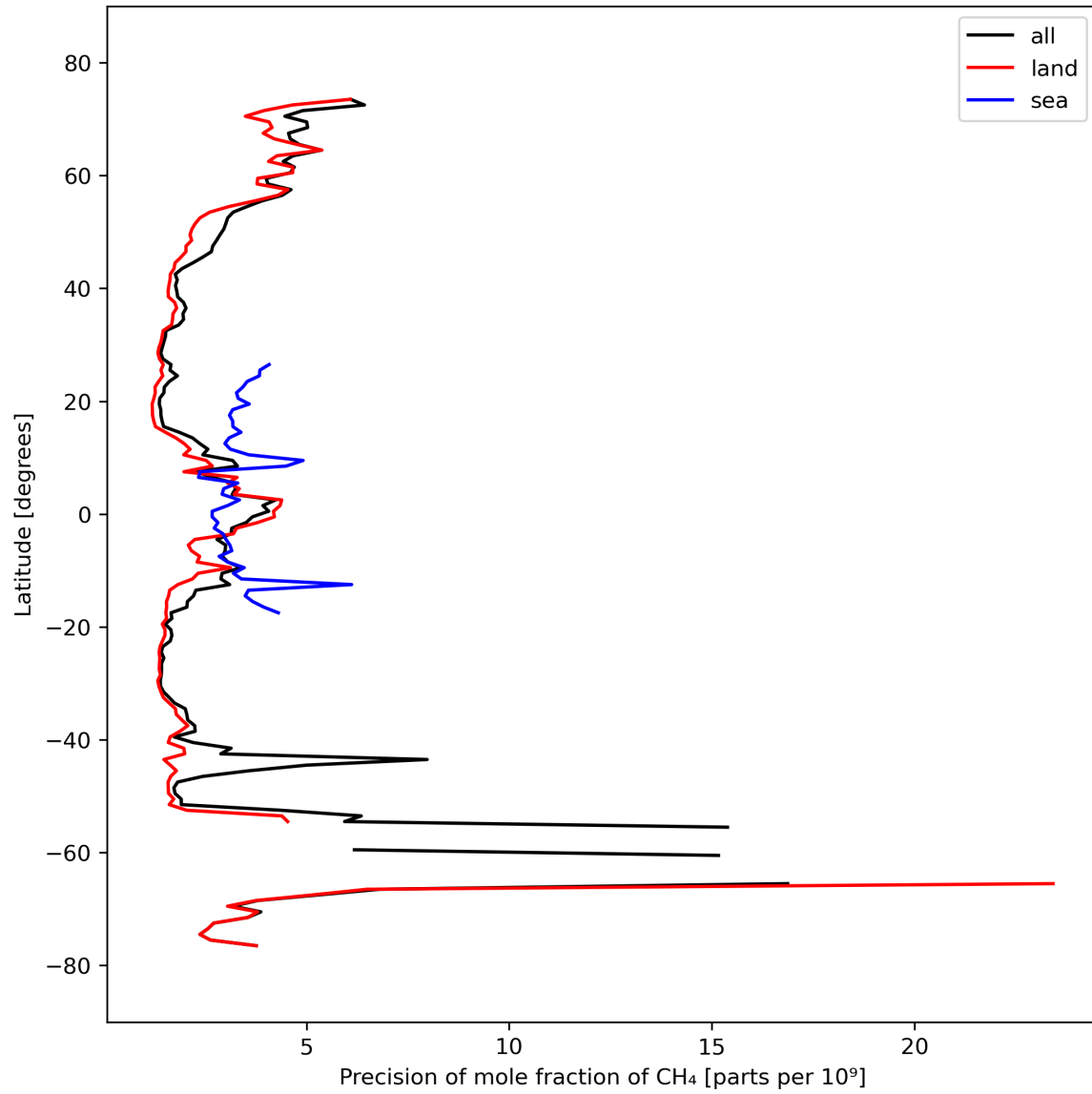
Figure 13: Zonal average of “Precision of mole fraction of CH 4 ” for 2023-09-27 to 2023-09-29.
