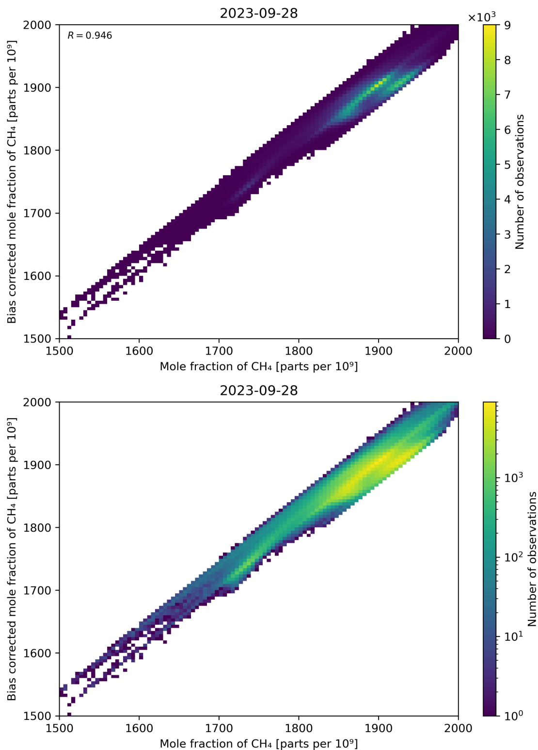
Figure 74: Scatter density plot of “Mole fraction of CH 4 ” against “Bias corrected mole fraction of CH 4 ” for 2023-09-27 to 2023-09-29.
