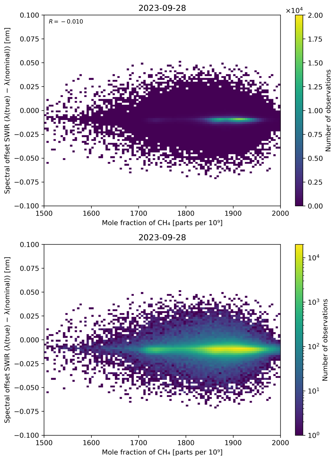
Figure 86: Scatter density plot of “Mole fraction of CH 4 ” against “Spectral offset SWIR ( \lambda(\text{true}) - \lambda(\text{nominal}) )” for 2023-09-27 to 2023-09-29.
