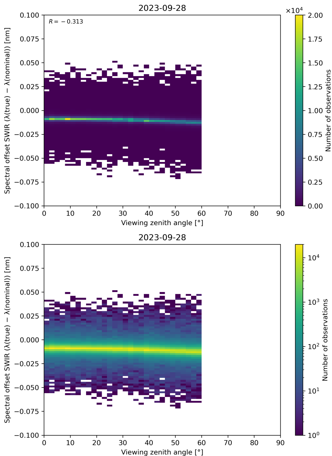
Figure 116: Scatter density plot of “Viewing zenith angle” against “Spectral offset SWIR ( \lambda(\text{true}) - \lambda(\text{nominal}) )” for 2023-09-27 to 2023-09-29.
