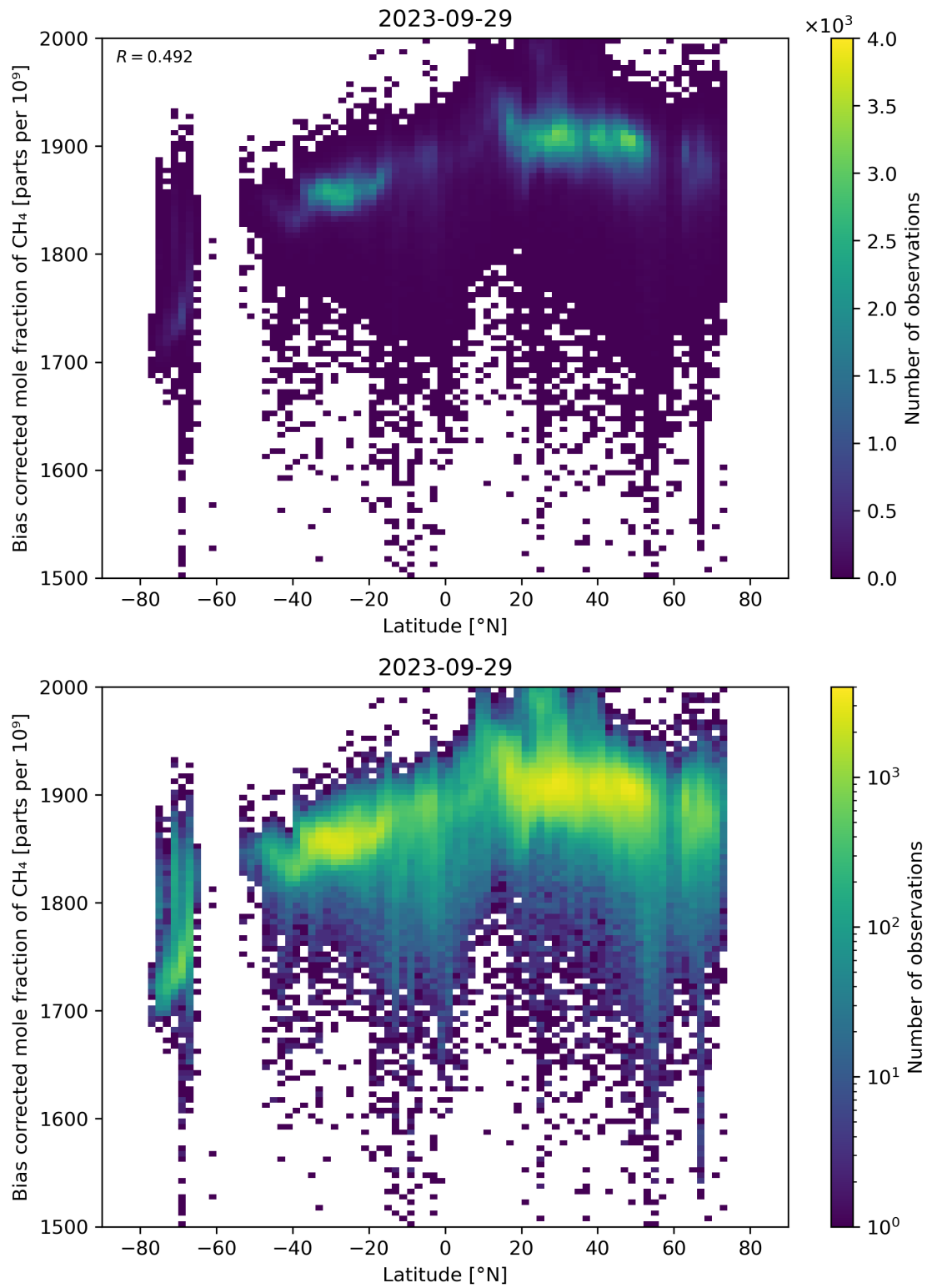
Figure 58: Scatter density plot of “Latitude” against “Bias corrected mole fraction of \text{CH}_4 ” for 2023-09-28 to 2023-09-30.
