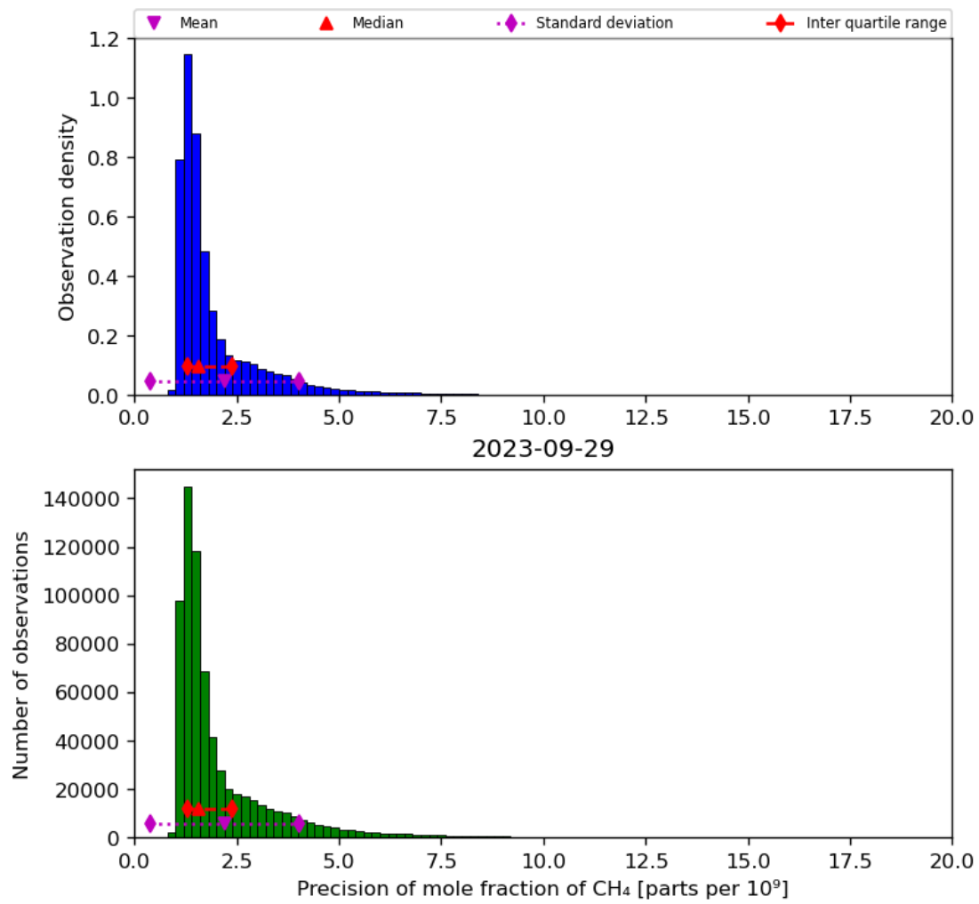
Figure 24: Histogram of “Precision of mole fraction of CH 4 ” for 2023-09-28 to 2023-09-30
