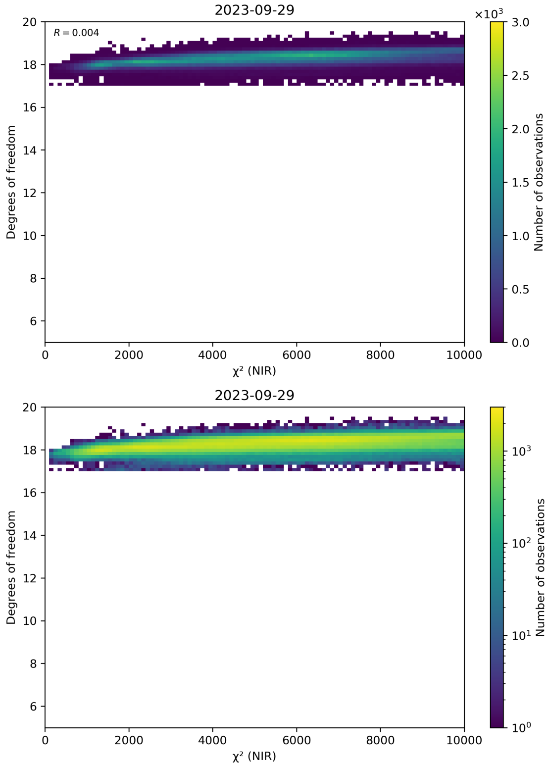
Figure 44: Scatter density plot of “ \chi^2 (NIR)” against “Degrees of freedom” for 2023-09-28 to 2023-09-30.
