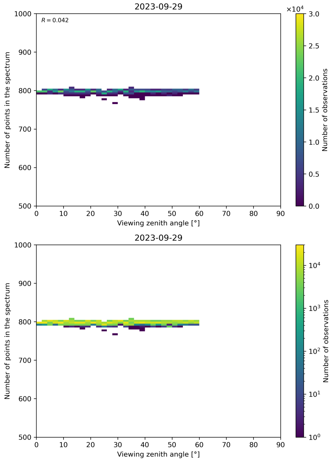
Figure 114: Scatter density plot of “Viewing zenith angle” against “Number of points in the spectrum” for 2023-09-28 to 2023-09-30.
