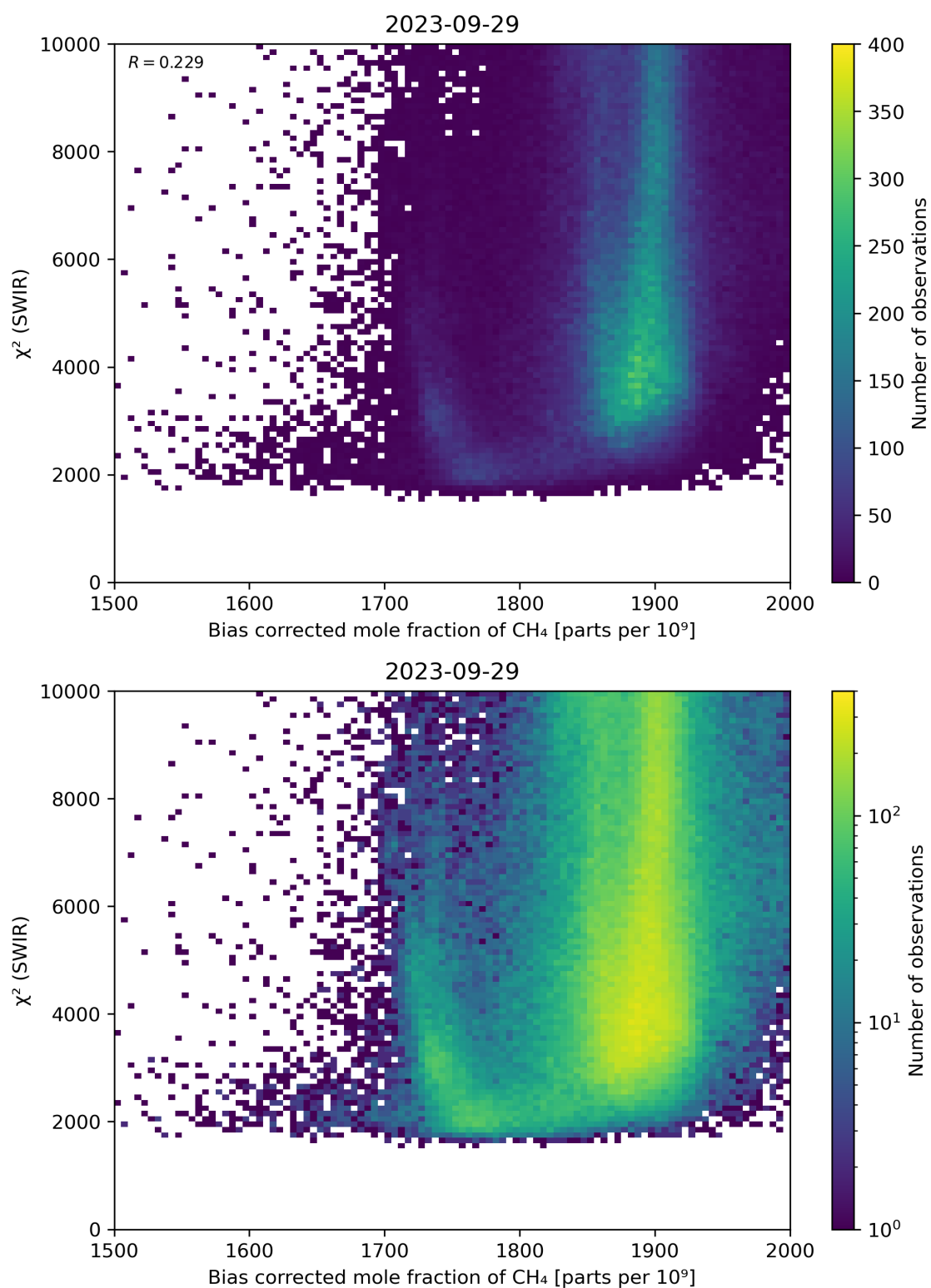
Figure 64: Scatter density plot of “Bias corrected mole fraction of \text{CH}_4 ” against “ \chi^2 (SWIR)” for 2023-09-28 to 2023-09-30.
