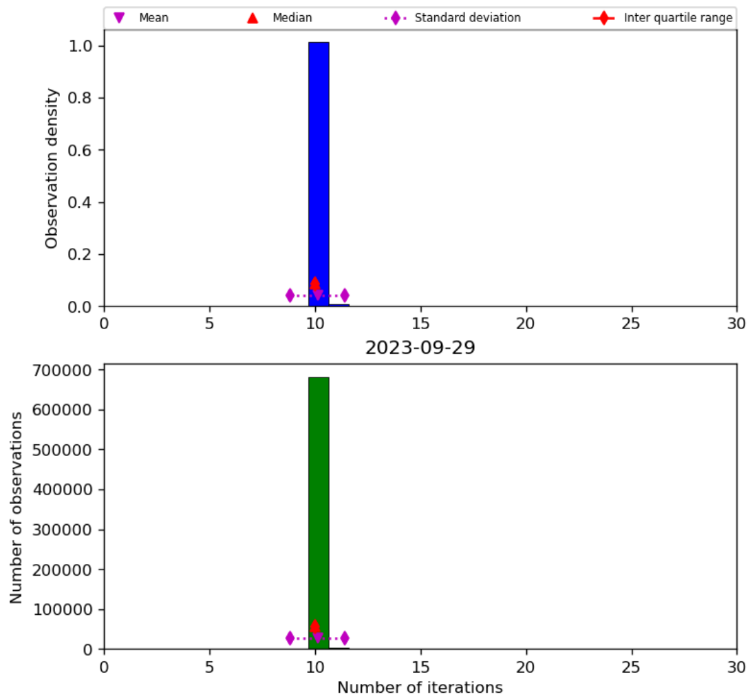
Figure 31: Histogram of “Number of iterations” for 2023-09-28 to 2023-09-30
