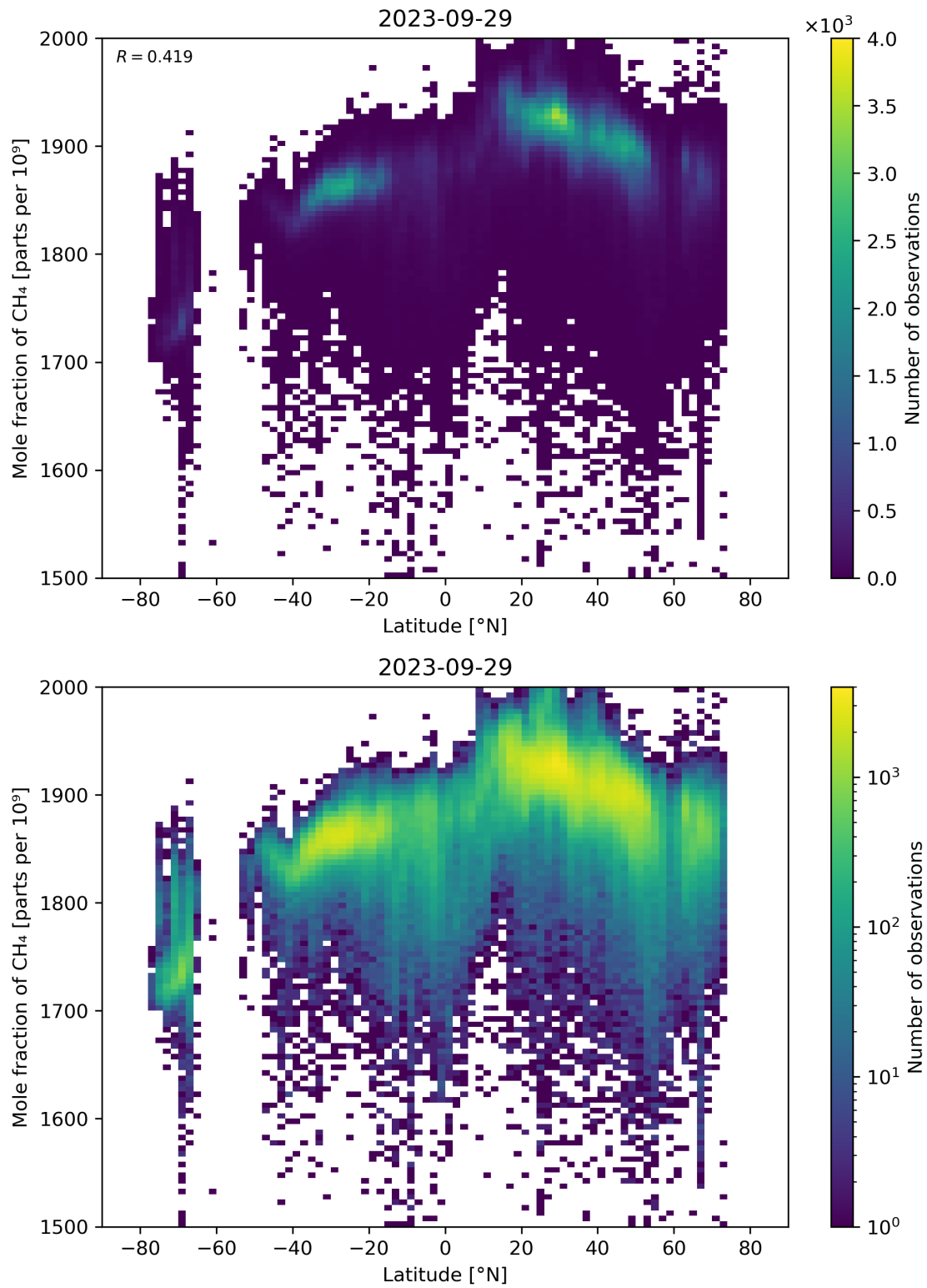
Figure 57: Scatter density plot of “Latitude” against “Mole fraction of CH 4 ” for 2023-09-28 to 2023-09-30.
