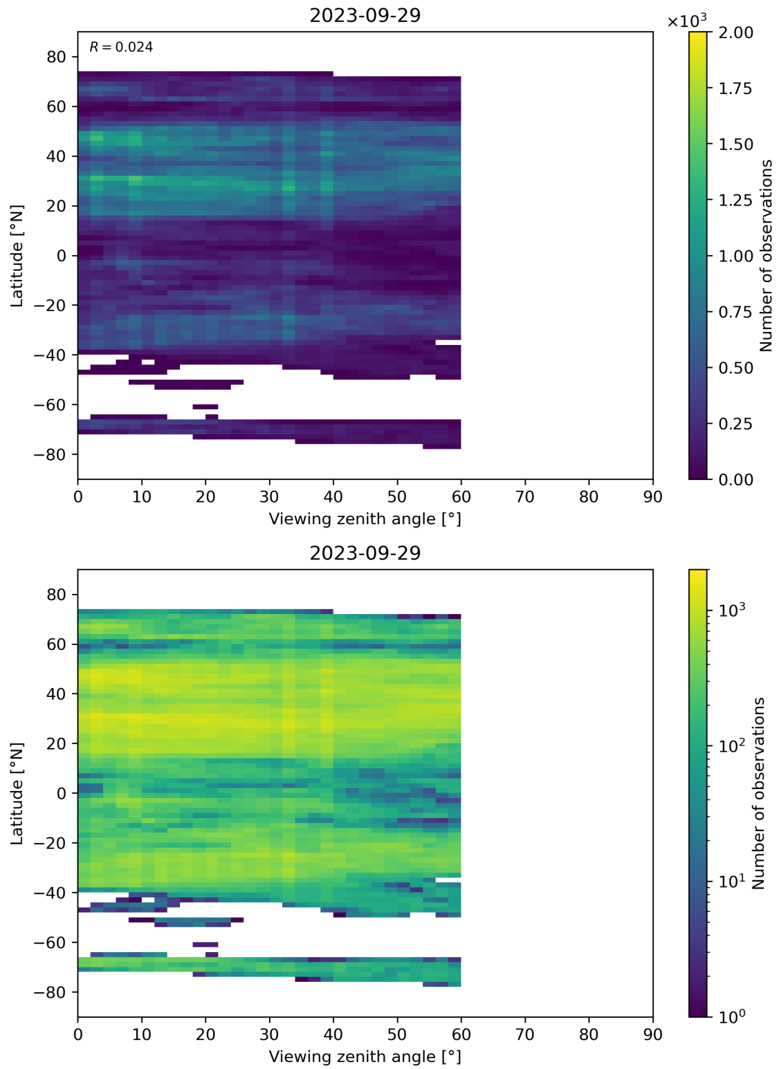
Figure 109: Scatter density plot of “Viewing zenith angle” against “Latitude” for 2023-09-28 to 2023-09-30.
