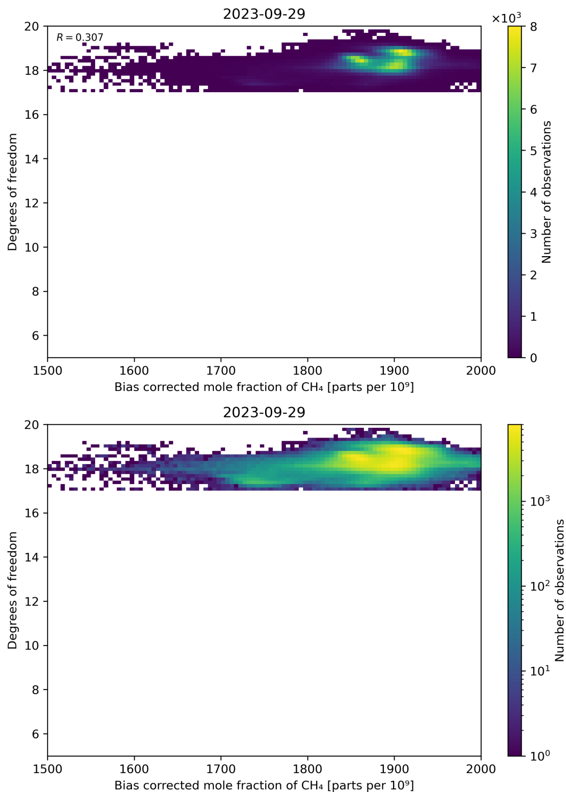
Figure 65: Scatter density plot of “Bias corrected mole fraction of CH 4 ” against “Degrees of freedom” for 2023-09-28 to 2023-09-30.
