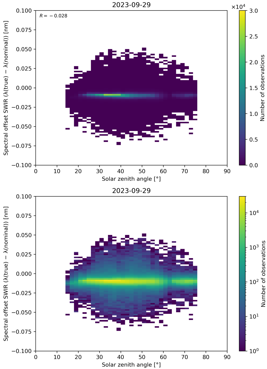
Figure 104: Scatter density plot of “Solar zenith angle” against “Spectral offset SWIR ( \lambda(\text{true}) - \lambda(\text{nominal}) )” for 2023-09-28 to 2023-09-30.
