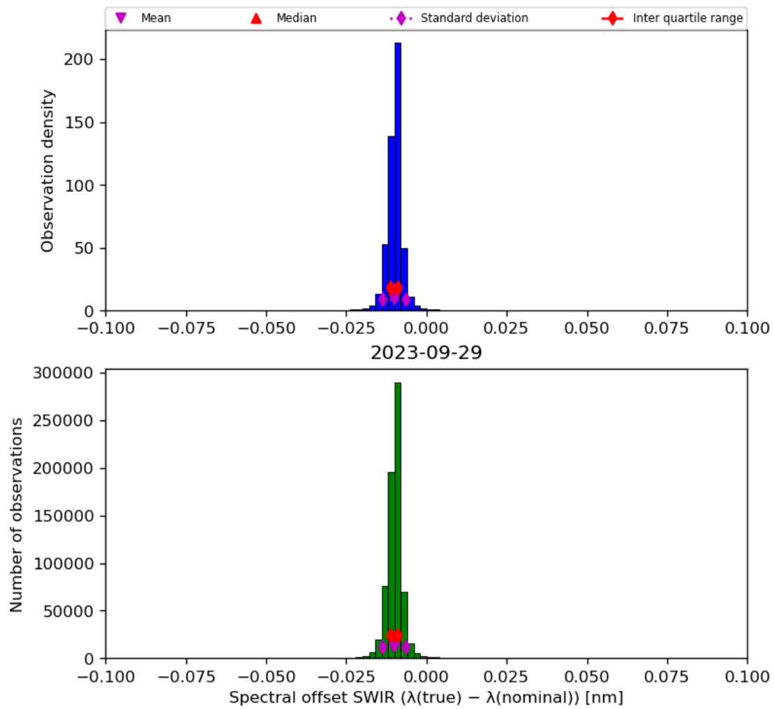
Figure 27: Histogram of “Spectral offset SWIR ( \lambda(\text{true}) - \lambda(\text{nominal}) )” for 2023-09-28 to 2023-09-30
