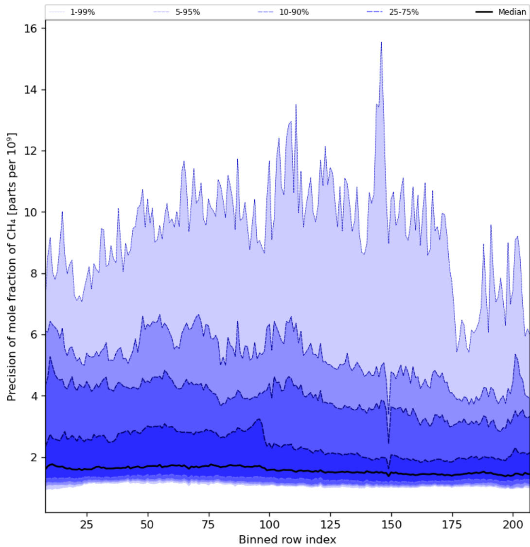
Figure 35: Along track statistics of “Precision of mole fraction of CH 4 ” for 2023-09-28 to 2023-09-30
