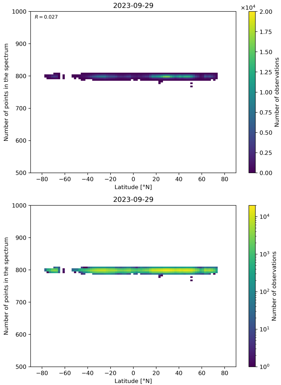
Figure 61: Scatter density plot of “Latitude” against “Number of points in the spectrum” for 2023-09-28 to 2023-09-30.
