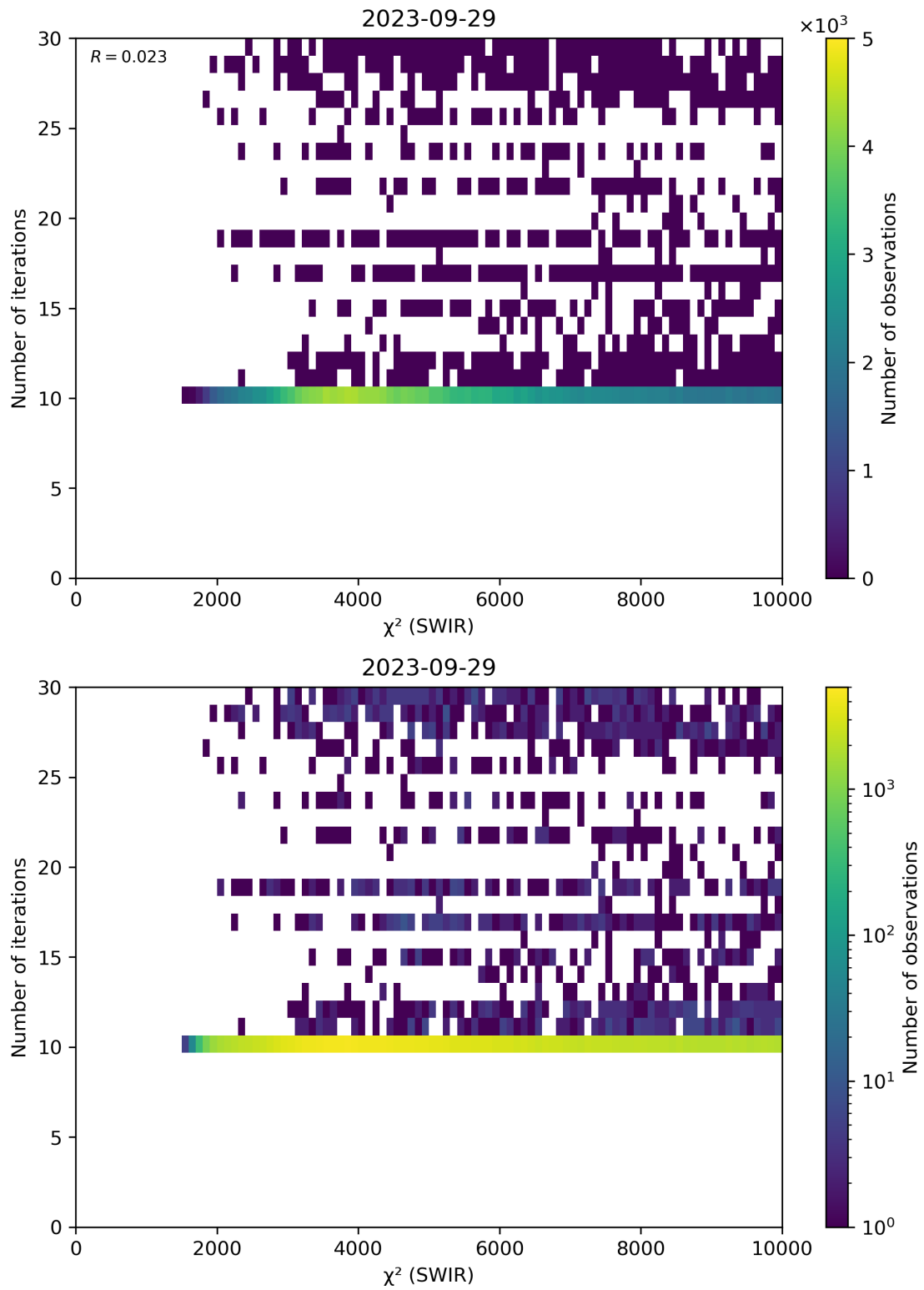
Figure 50: Scatter density plot of “ \chi^2 (SWIR)” against “Number of iterations” for 2023-09-28 to 2023-09-30.
