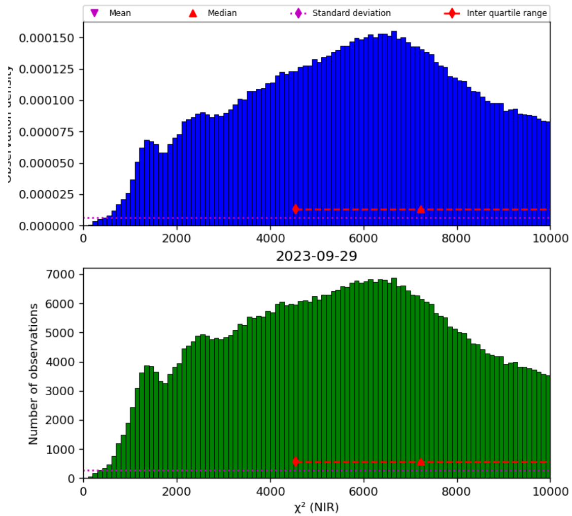
Figure 29: Histogram of “ \chi^2 (NIR)” for 2023-09-28 to 2023-09-30
