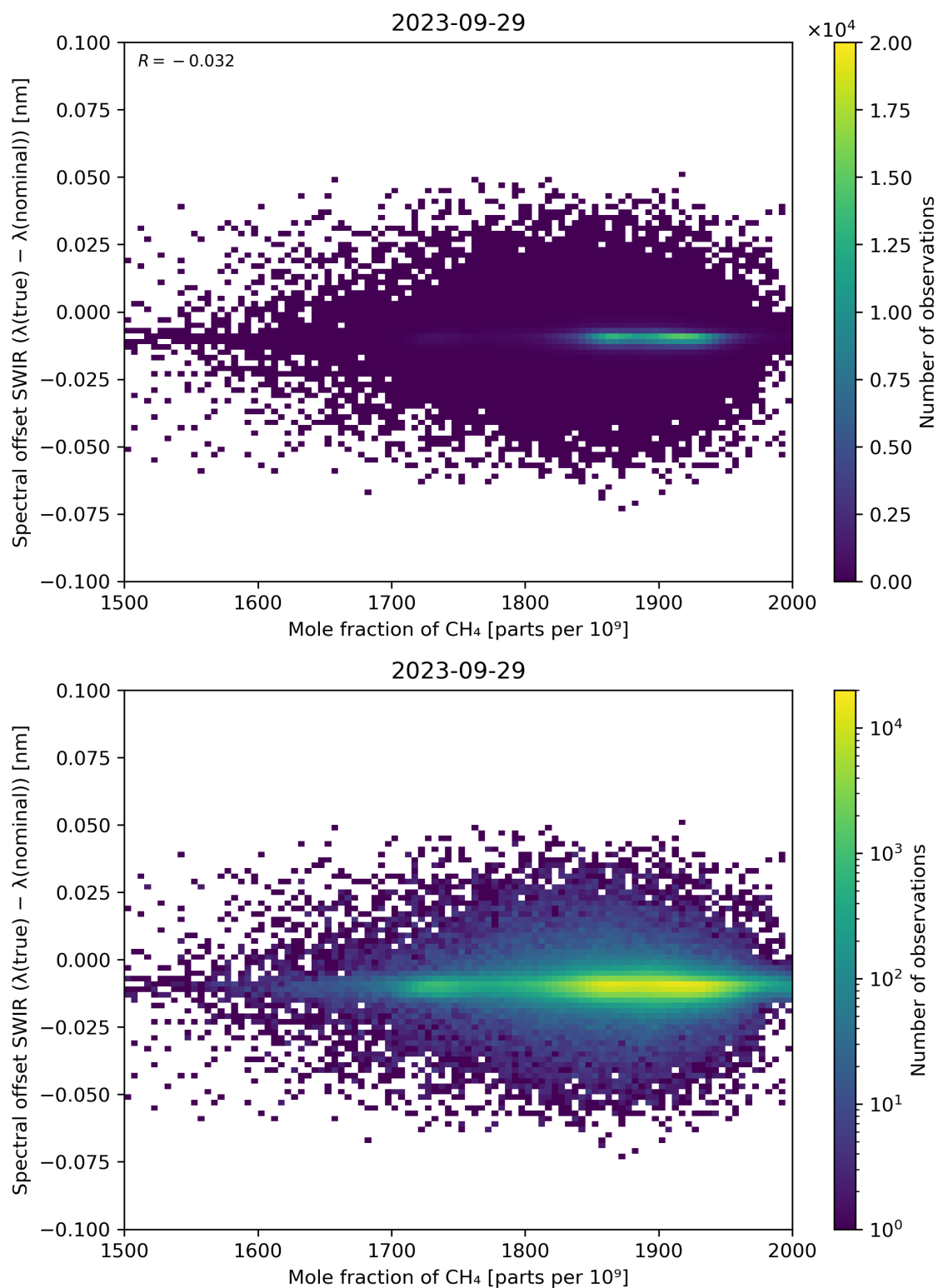
Figure 86: Scatter density plot of “Mole fraction of CH 4 ” against “Spectral offset SWIR ( \lambda(\text{true}) - \lambda(\text{nominal}) )” for 2023-09-28 to 2023-09-30.
