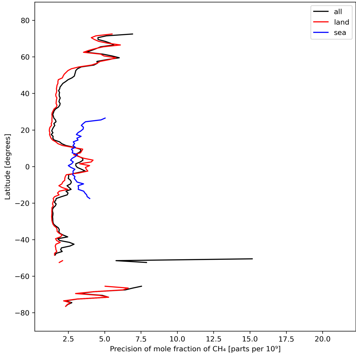
Figure 13: Zonal average of “Precision of mole fraction of \text{CH}_4 ” for 2023-09-28 to 2023-09-30.
