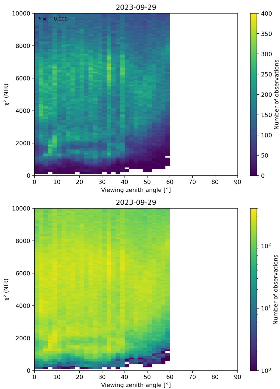
Figure 105: Scatter density plot of “Viewing zenith angle” against “ \chi^2 (NIR)” for 2023-09-28 to 2023-09-30.
