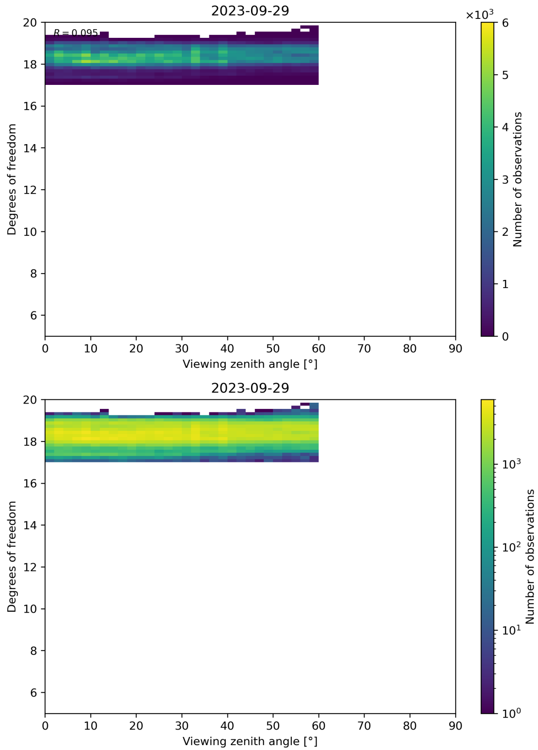
Figure 107: Scatter density plot of “Viewing zenith angle” against “Degrees of freedom” for 2023-09-28 to 2023-09-30.
