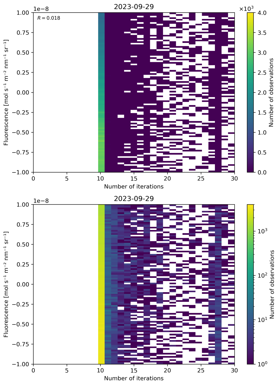
Figure 87: Scatter density plot of “Number of iterations” against “Fluorescence” for 2023-09-28 to 2023-09-30.
