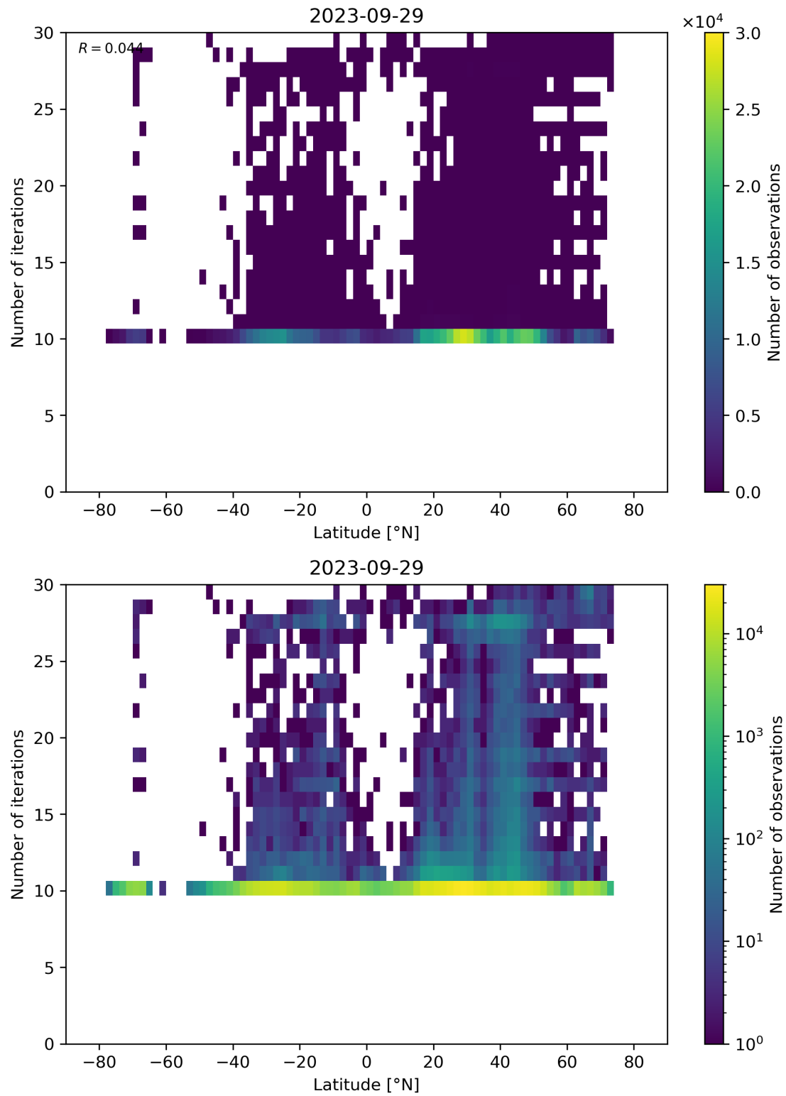
Figure 60: Scatter density plot of “Latitude” against “Number of iterations” for 2023-09-28 to 2023-09-30.
