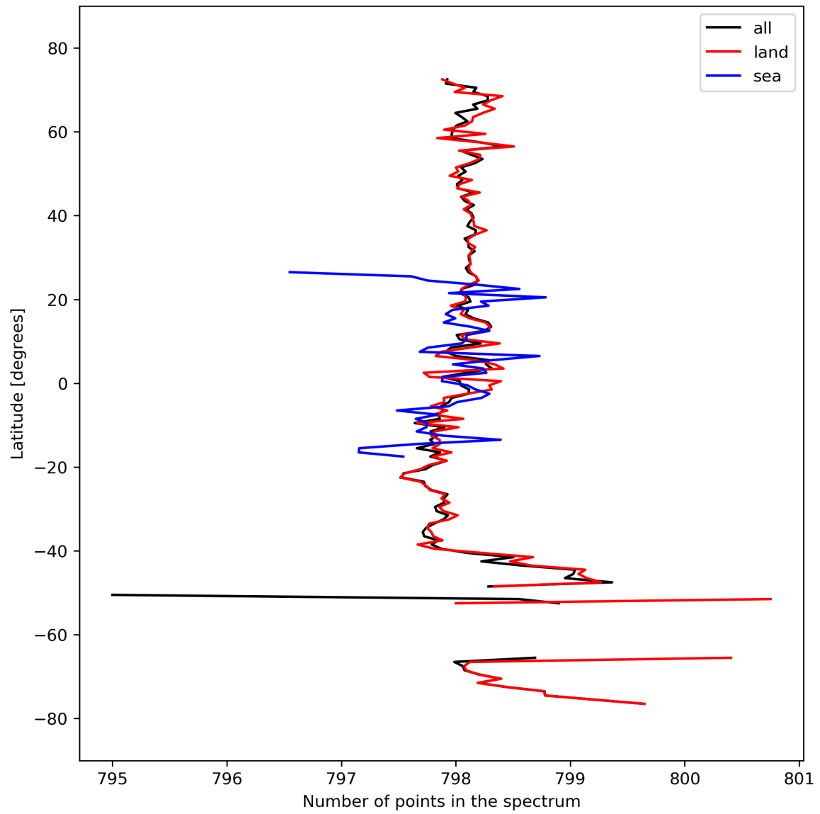
Figure 15: Zonal average of “Number of points in the spectrum” for 2023-09-28 to 2023-09-30.
