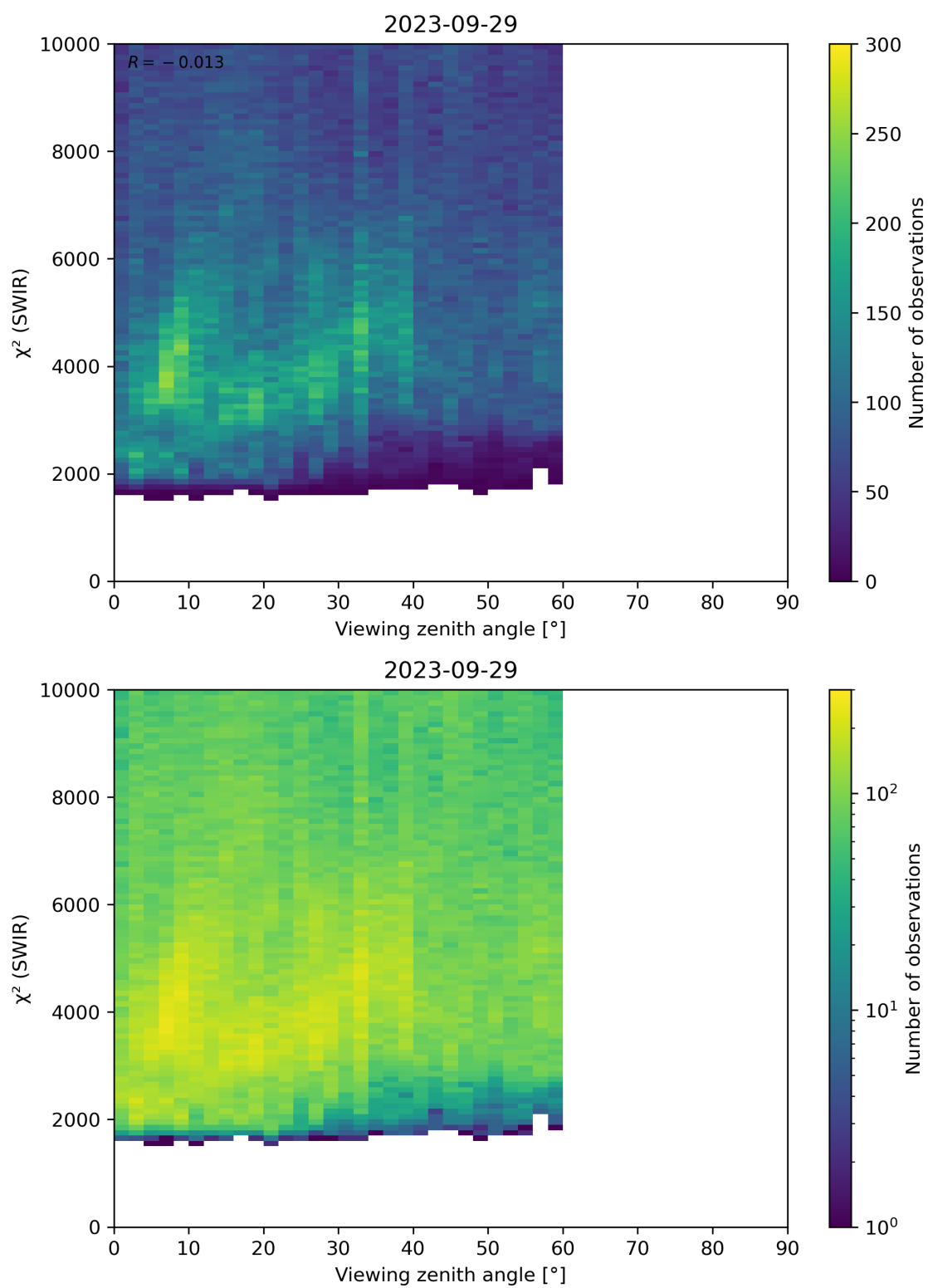
Figure 106: Scatter density plot of “Viewing zenith angle” against “ \chi^2 (SWIR)” for 2023-09-28 to 2023-09-30.
