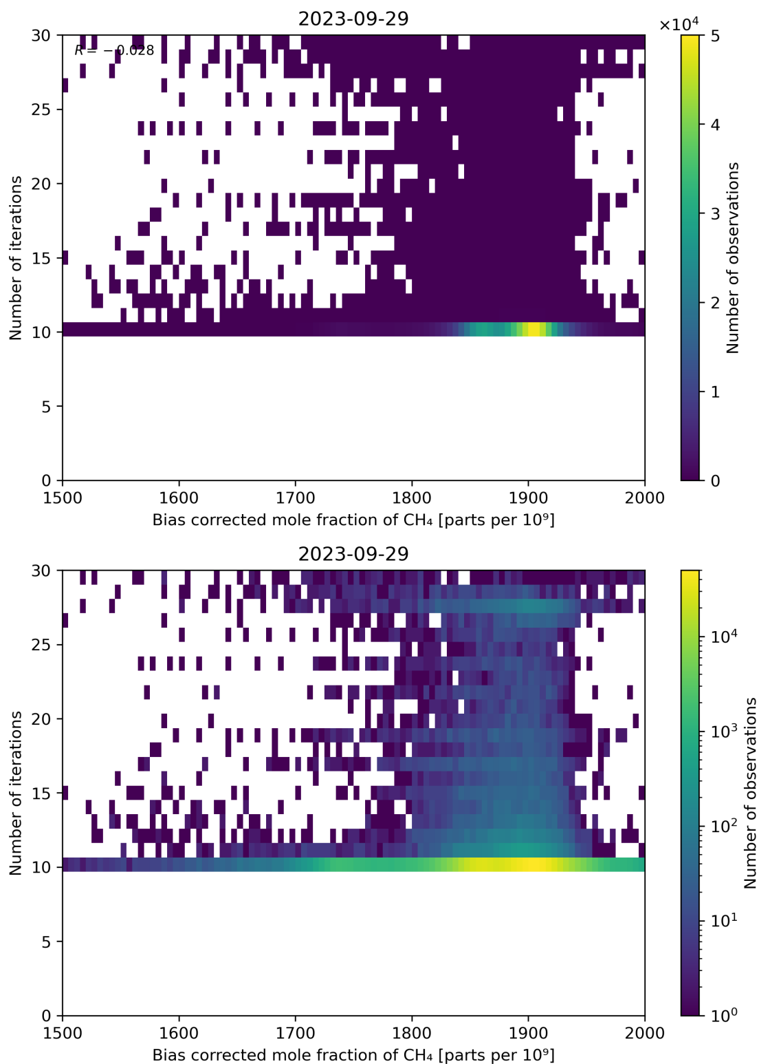
Figure 67: Scatter density plot of “Bias corrected mole fraction of CH 4 ” against “Number of iterations” for 2023-09-28 to 2023-09-30.
