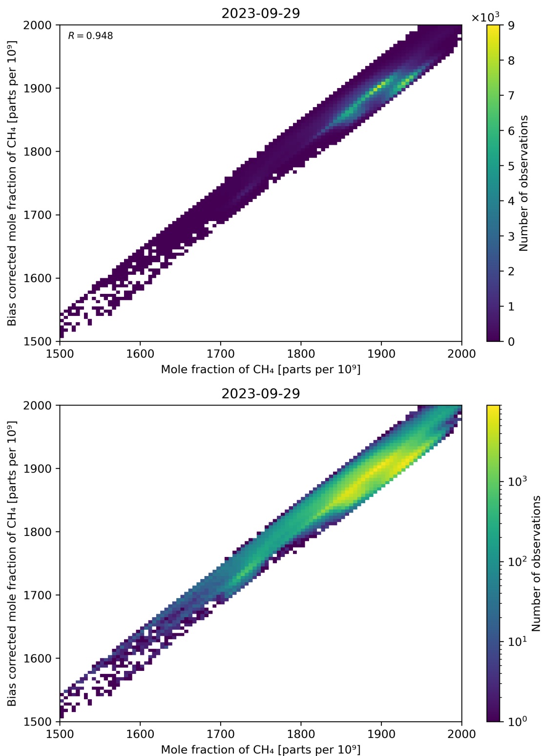
Figure 74: Scatter density plot of “Mole fraction of CH 4 ” against “Bias corrected mole fraction of CH 4 ” for 2023-09-28 to 2023-09-30.
