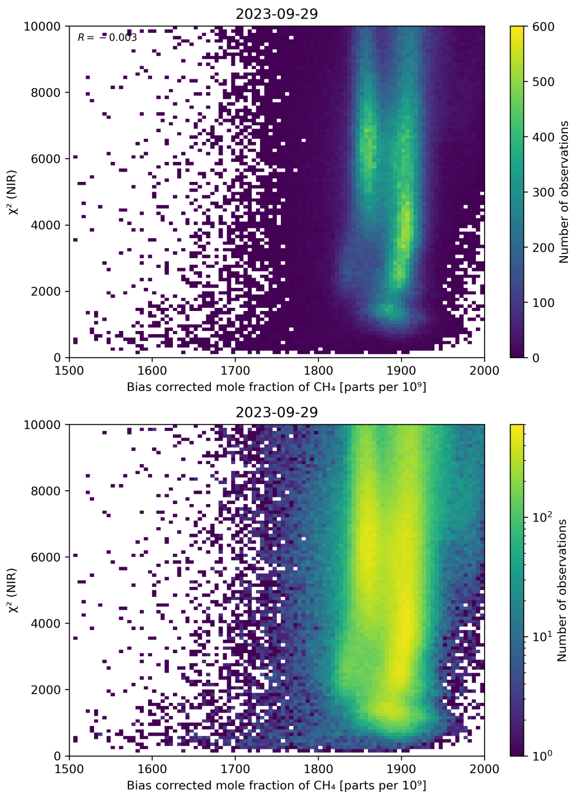
Figure 63: Scatter density plot of “Bias corrected mole fraction of CH 4 ” against “ \chi^2 (NIR)” for 2023-09-28 to 2023-09-30.
