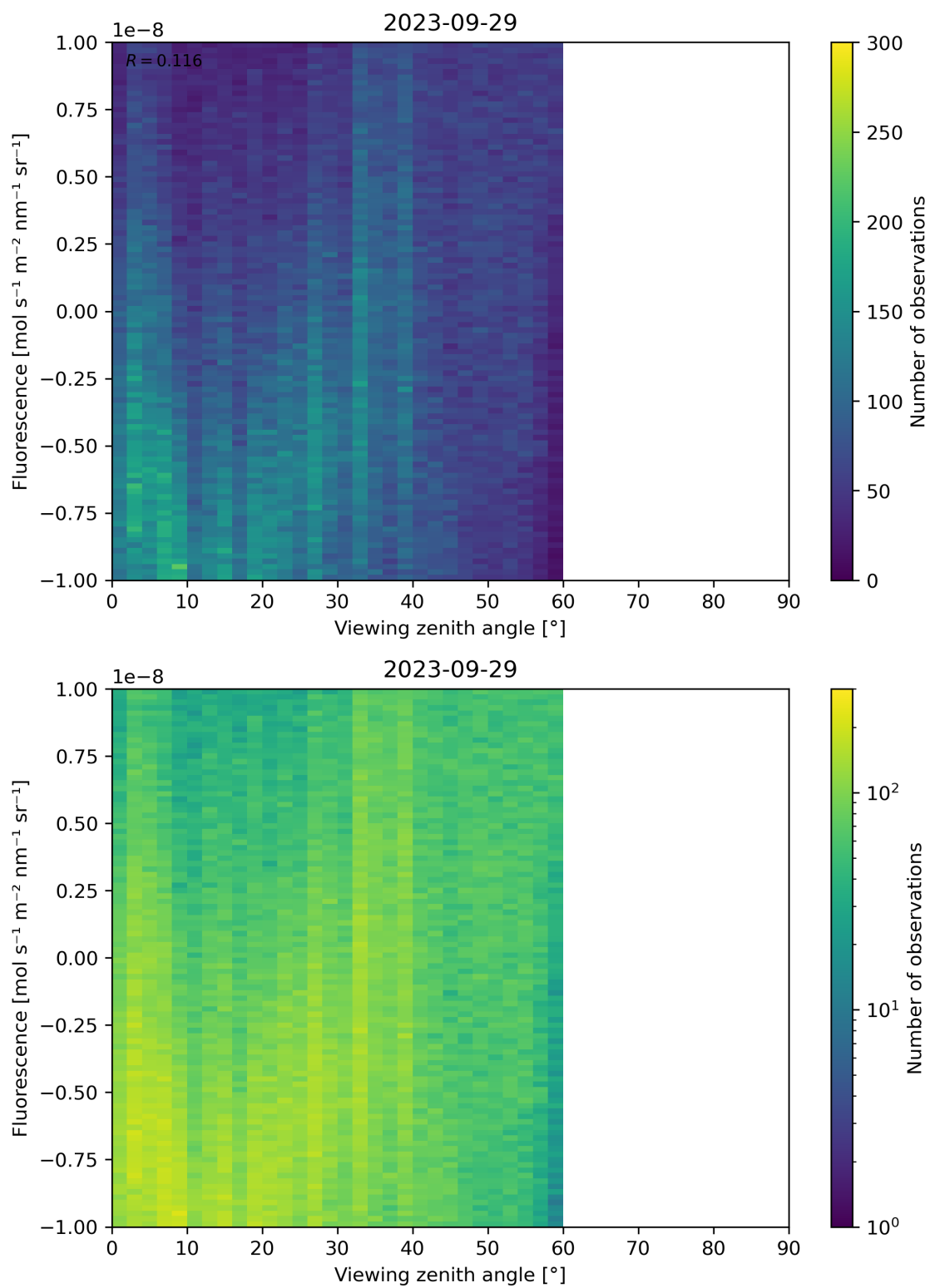
Figure 108: Scatter density plot of “Viewing zenith angle” against “Fluorescence” for 2023-09-28 to 2023-09-30.
