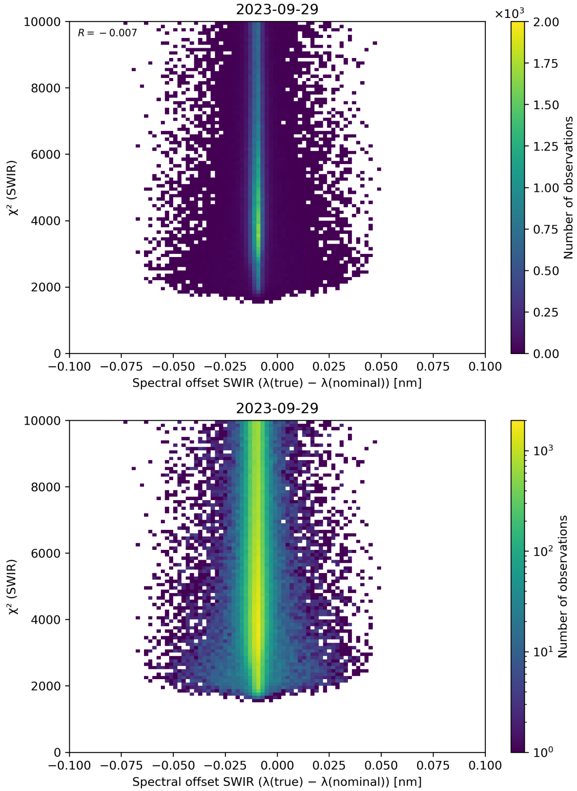
Figure 118: Scatter density plot of “Spectral offset SWIR ( \lambda(\text{true}) - \lambda(\text{nominal}) )” against “ \chi^2 (SWIR)” for 2023-09-28 to 2023-09-30.
