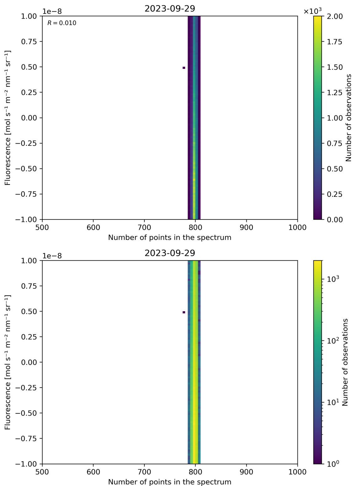
Figure 91: Scatter density plot of “Number of points in the spectrum” against “Fluorescence” for 2023-09-28 to 2023-09-30.
