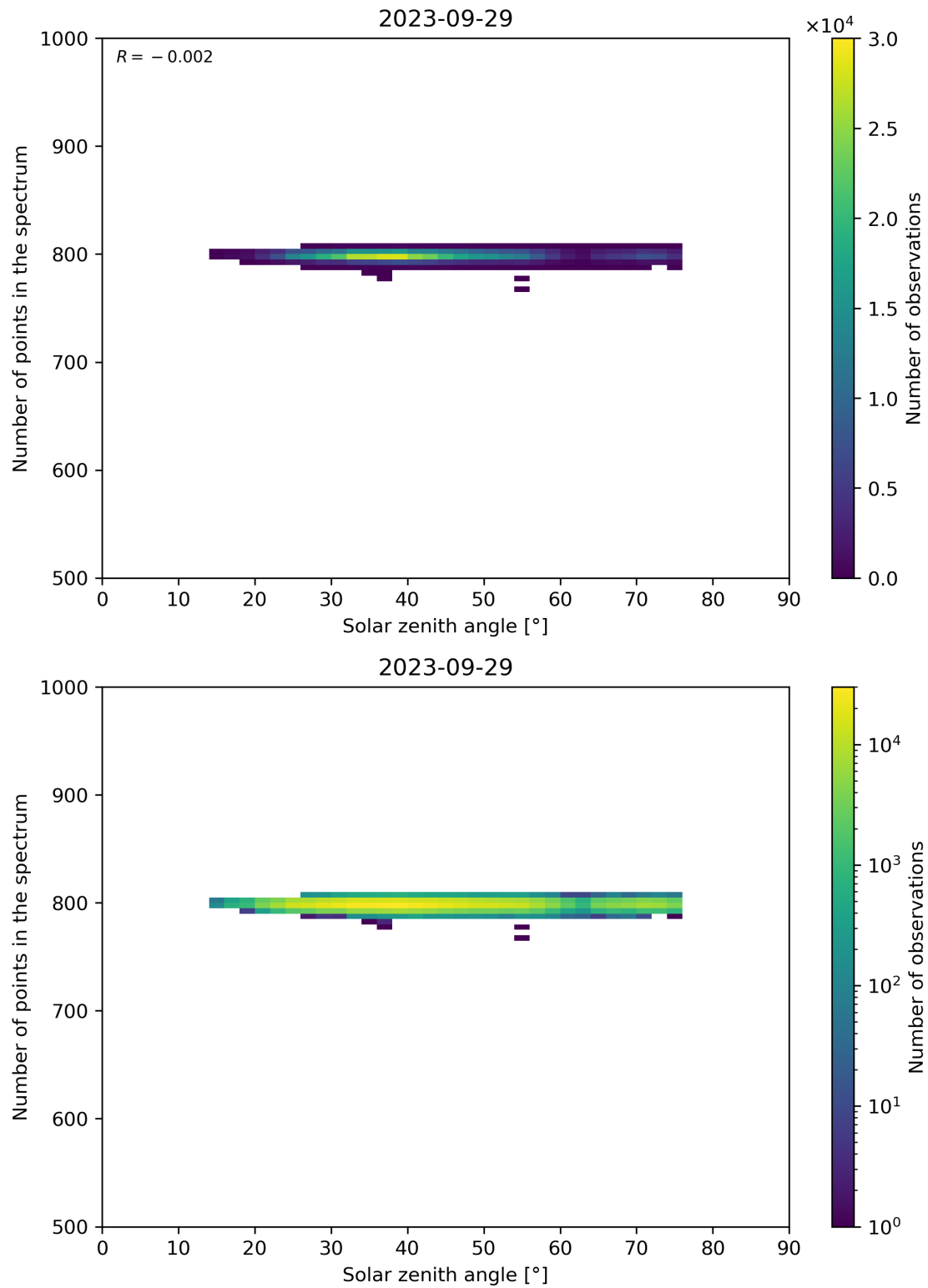
Figure 103: Scatter density plot of “Solar zenith angle” against “Number of points in the spectrum” for 2023-09-28 to 2023-09-30.
