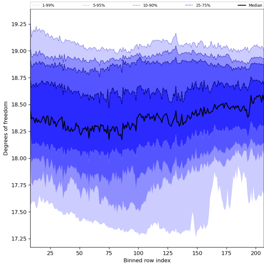
Figure 41: Along track statistics of “Degrees of freedom” for 2023-09-28 to 2023-09-30
