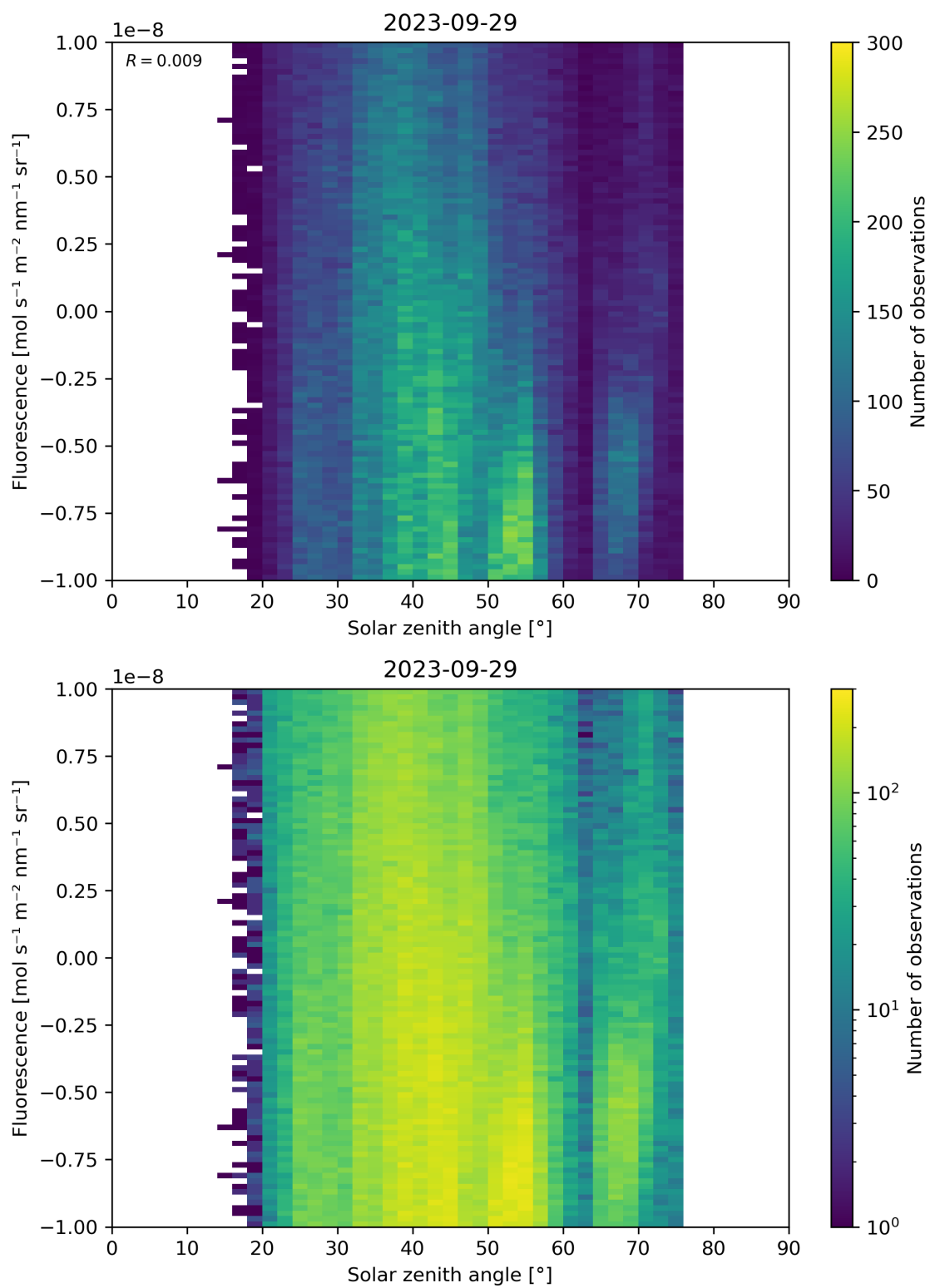
Figure 97: Scatter density plot of “Solar zenith angle” against “Fluorescence” for 2023-09-28 to 2023-09-30.
