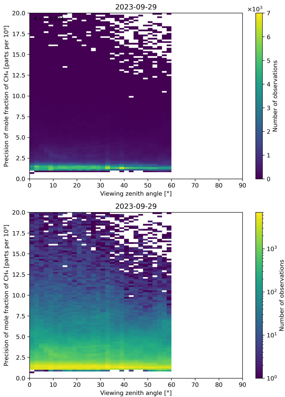
Figure 112: Scatter density plot of “Viewing zenith angle” against “Precision of mole fraction of CH 4 ” for 2023-09-28 to 2023-09-30.
