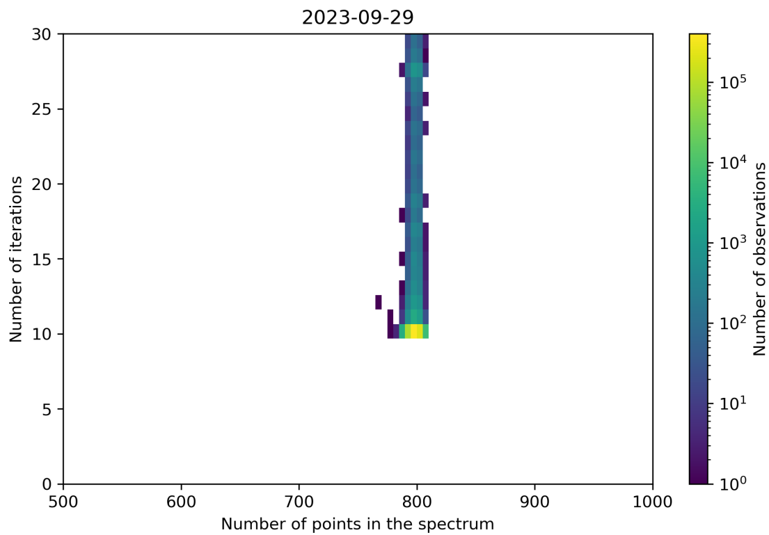
Figure 92: Scatter density plot of “Number of points in the spectrum” against “Number of iterations” for 2023-09-28 to 2023-09-30.
