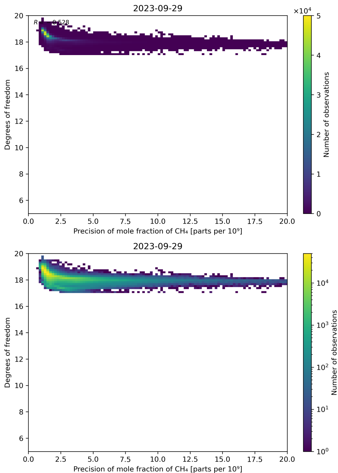
Figure 80: Scatter density plot of “Precision of mole fraction of CH 4 ” against “Degrees of freedom” for 2023-09-28 to 2023-09-30.
