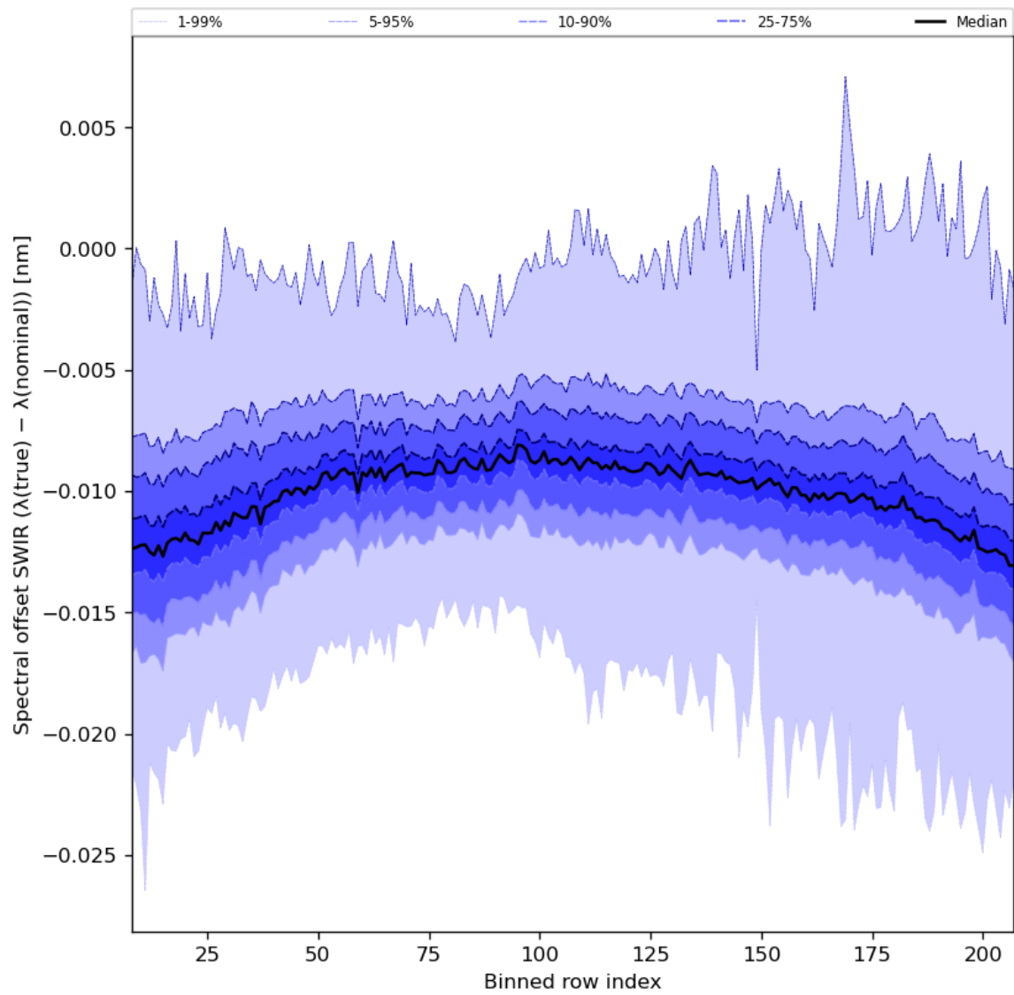
Figure 38: Along track statistics of “Spectral offset SWIR ( \lambda(\text{true}) - \lambda(\text{nominal}) )” for 2023-09-28 to 2023-09-30
