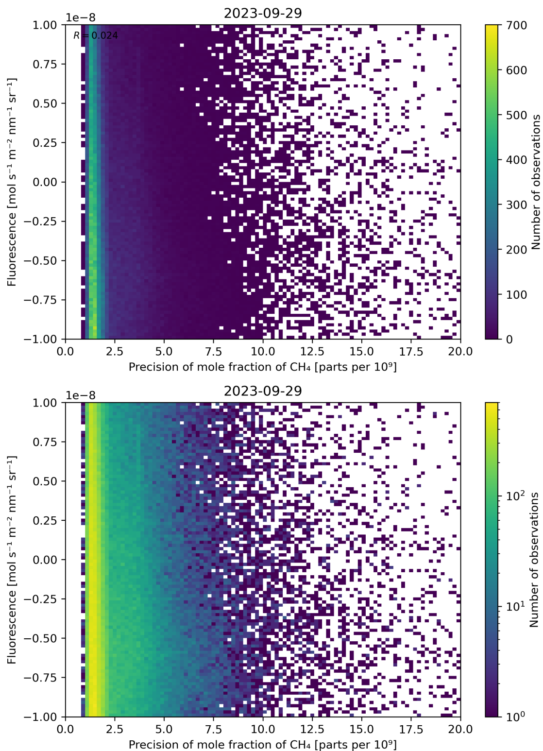
Figure 81: Scatter density plot of “Precision of mole fraction of \text{CH}_4 ” against “Fluorescence” for 2023-09-28 to 2023-09-30.
