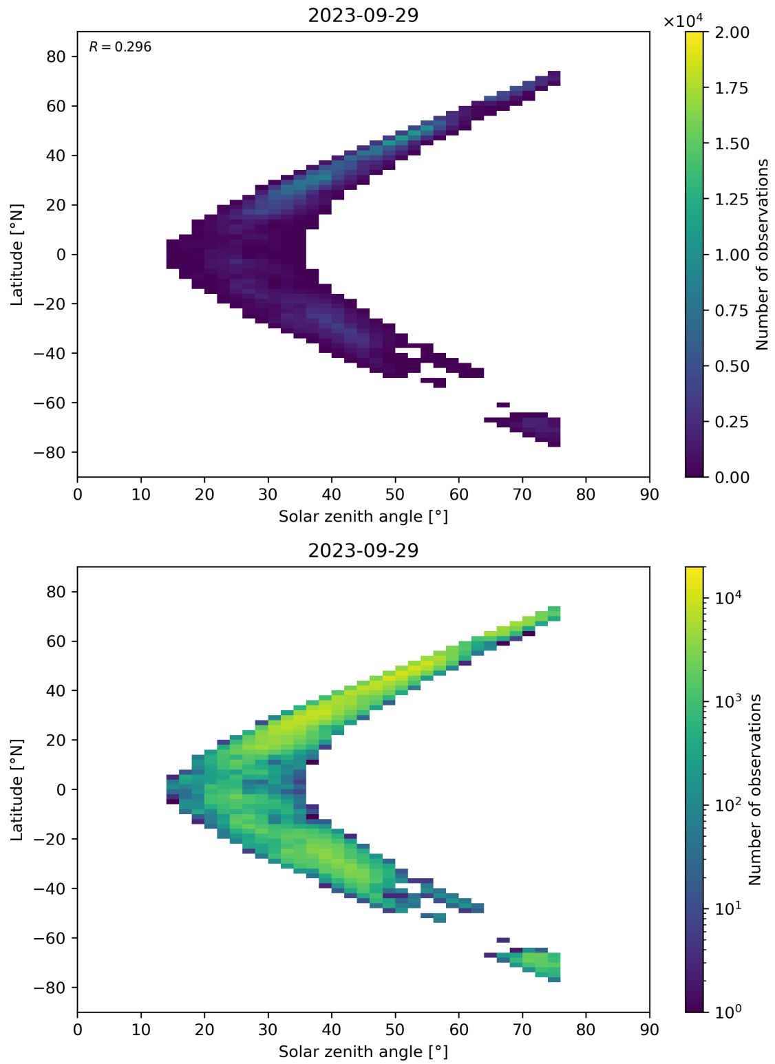
Figure 98: Scatter density plot of “Solar zenith angle” against “Latitude” for 2023-09-28 to 2023-09-30.
