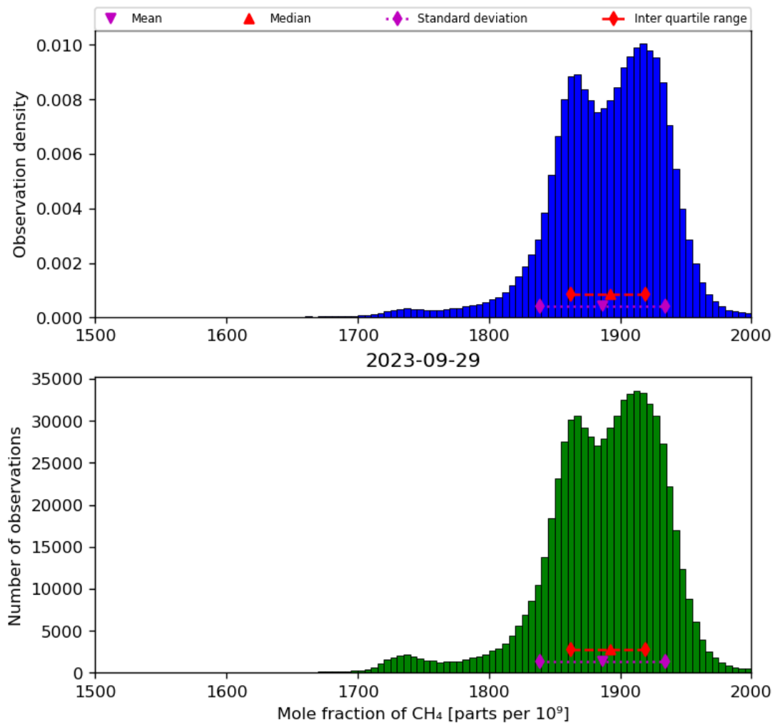
Figure 23: Histogram of “Mole fraction of CH 4 ” for 2023-09-28 to 2023-09-30
