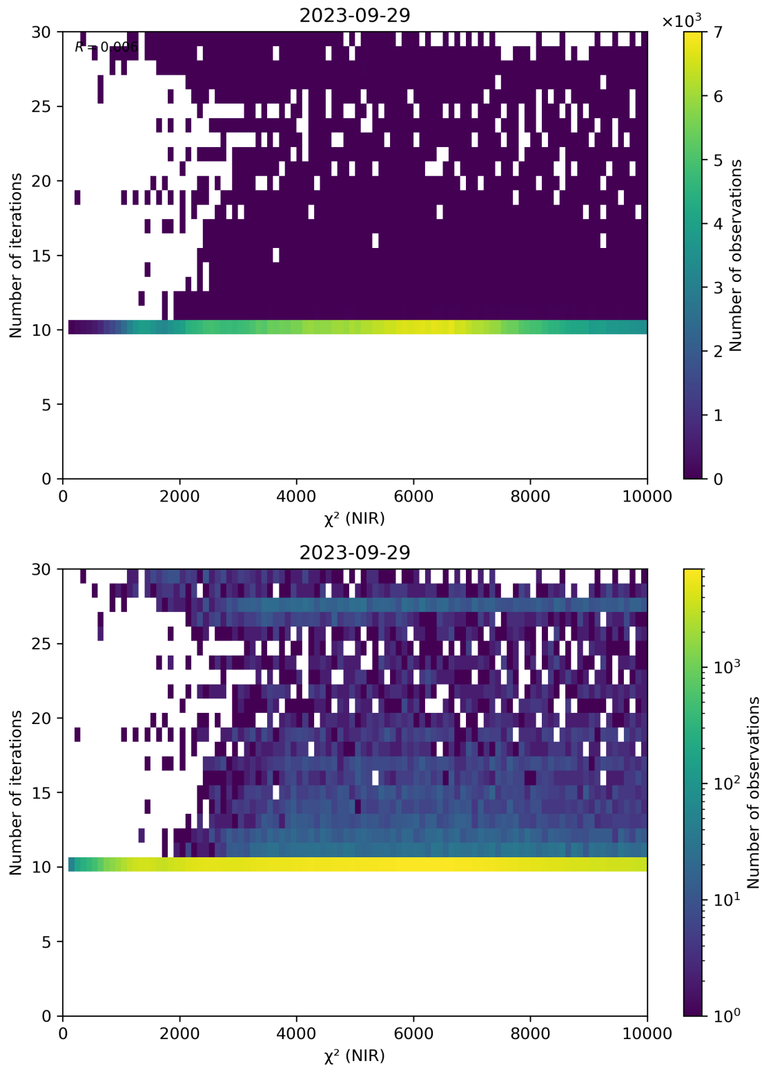
Figure 46: Scatter density plot of “ \chi^2 (NIR)” against “Number of iterations” for 2023-09-28 to 2023-09-30.
