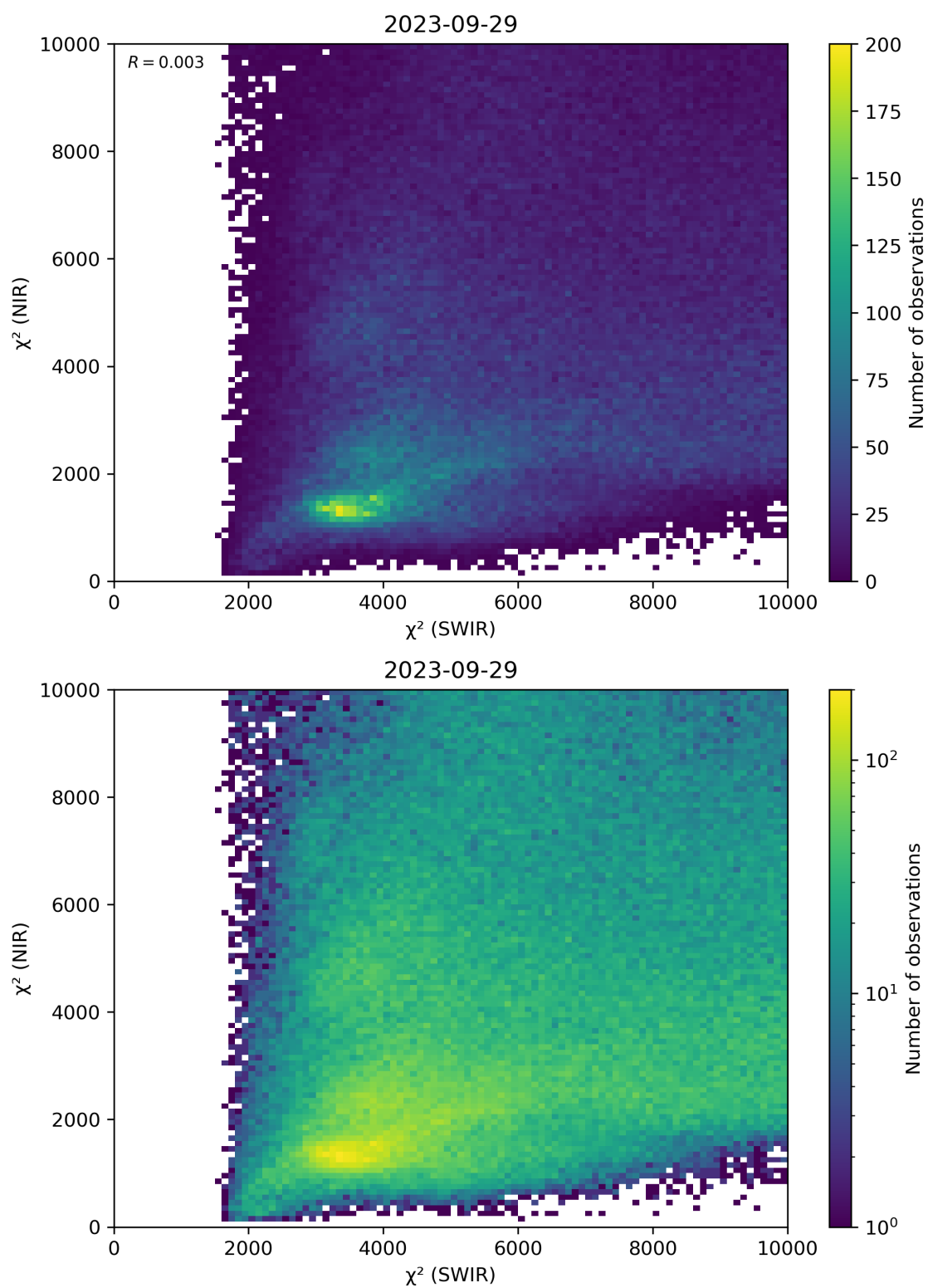
Figure 47: Scatter density plot of “ \chi^2 (SWIR)” against “ \chi^2 (NIR)” for 2023-09-28 to 2023-09-30.
