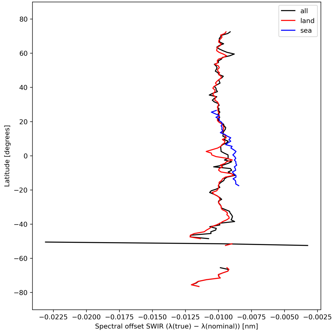
Figure 16: Zonal average of “Spectral offset SWIR ( \lambda(\text{true}) - \lambda(\text{nominal}) )” for 2023-09-28 to 2023-09-30.
