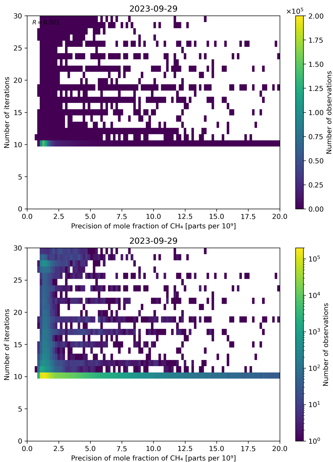
Figure 83: Scatter density plot of “Precision of mole fraction of CH 4 ” against “Number of iterations” for 2023-09-28 to 2023-09-30.
