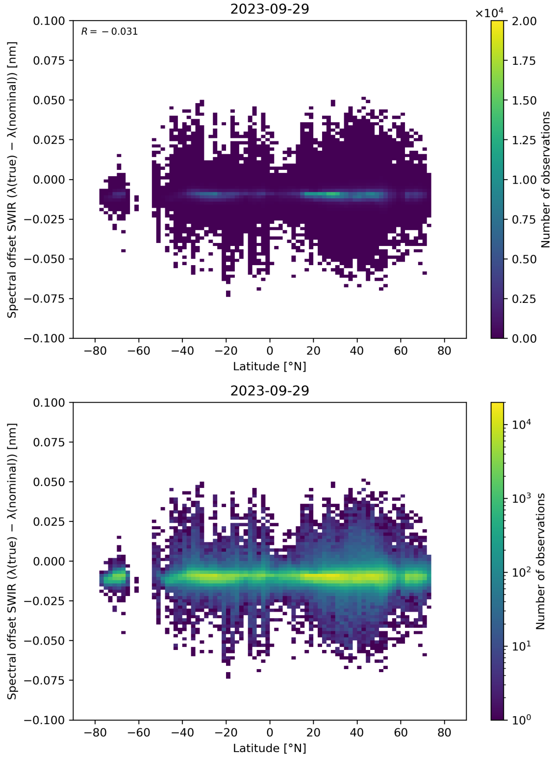
Figure 62: Scatter density plot of “Latitude” against “Spectral offset SWIR ( \lambda(\text{true}) - \lambda(\text{nominal}) )” for 2023-09-28 to 2023-09-30.
