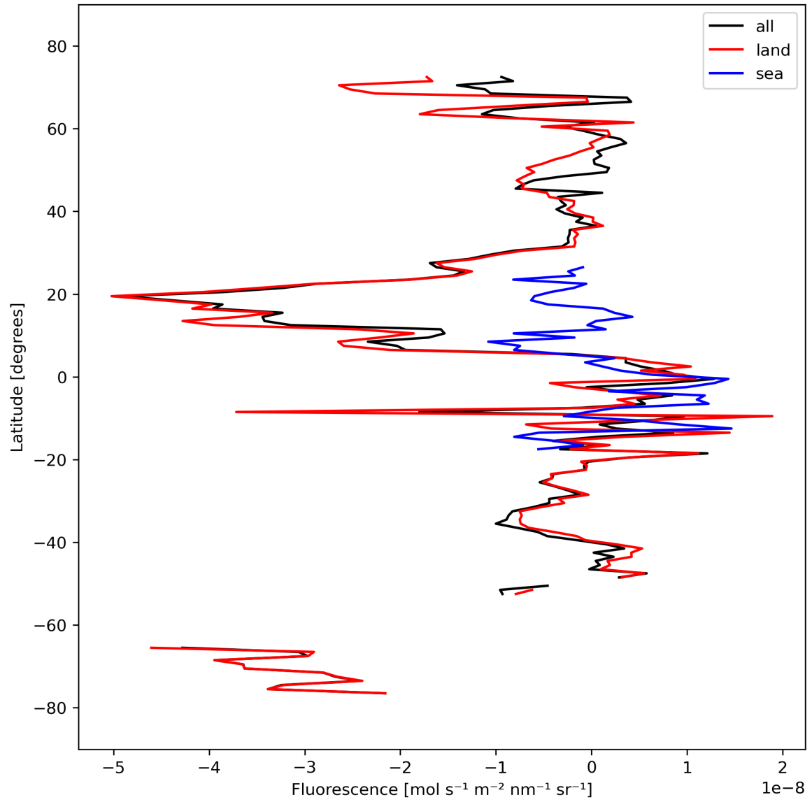
Figure 21: Zonal average of “Fluorescence” for 2023-09-28 to 2023-09-30.
