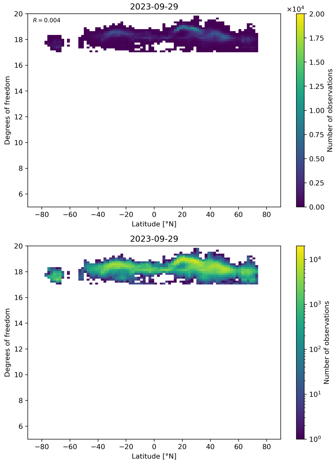
Figure 55: Scatter density plot of “Latitude” against “Degrees of freedom” for 2023-09-28 to 2023-09-30.
