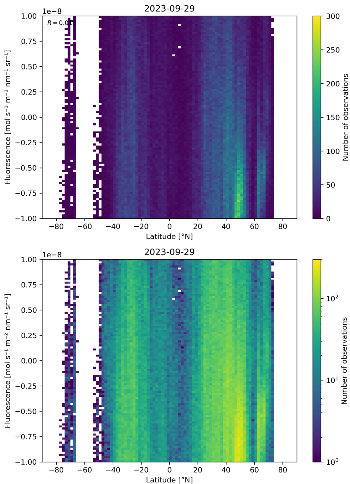
Figure 56: Scatter density plot of “Latitude” against “Fluorescence” for 2023-09-28 to 2023-09-30.
