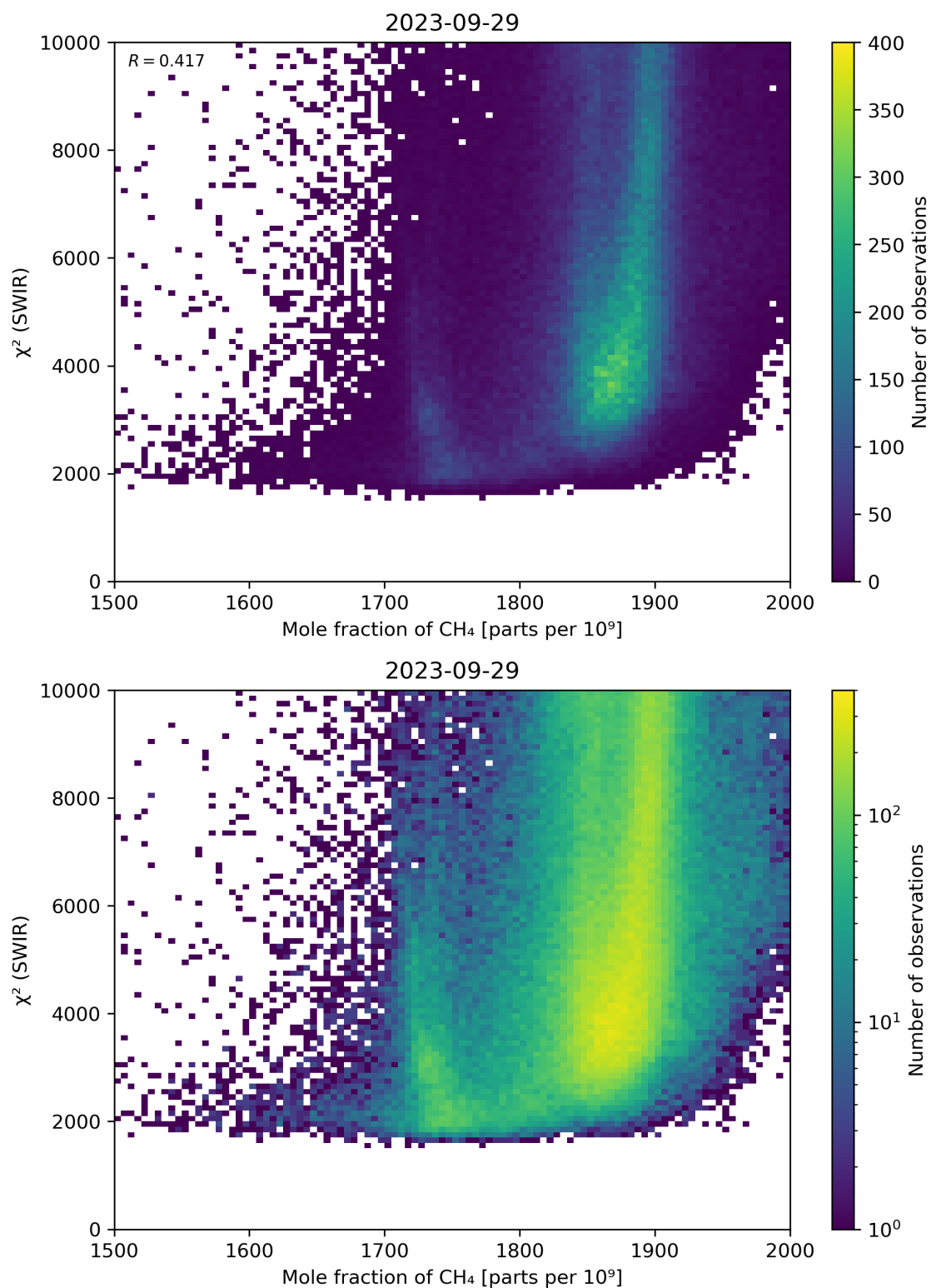
Figure 71: Scatter density plot of “Mole fraction of \text{CH}_4 ” against “ \chi^2 (SWIR)” for 2023-09-28 to 2023-09-30.
