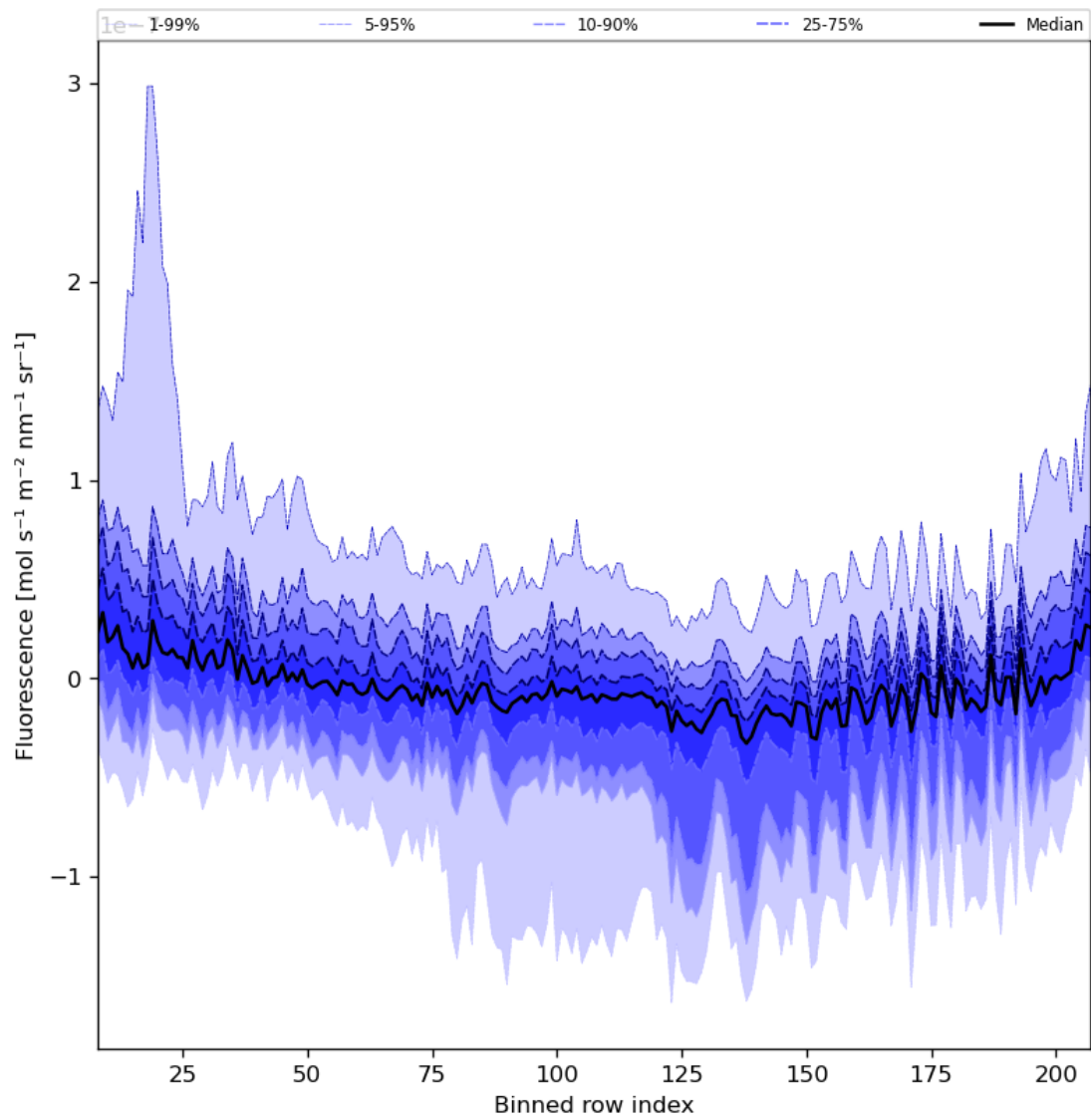
Figure 43: Along track statistics of “Fluorescence” for 2023-09-28 to 2023-09-30
