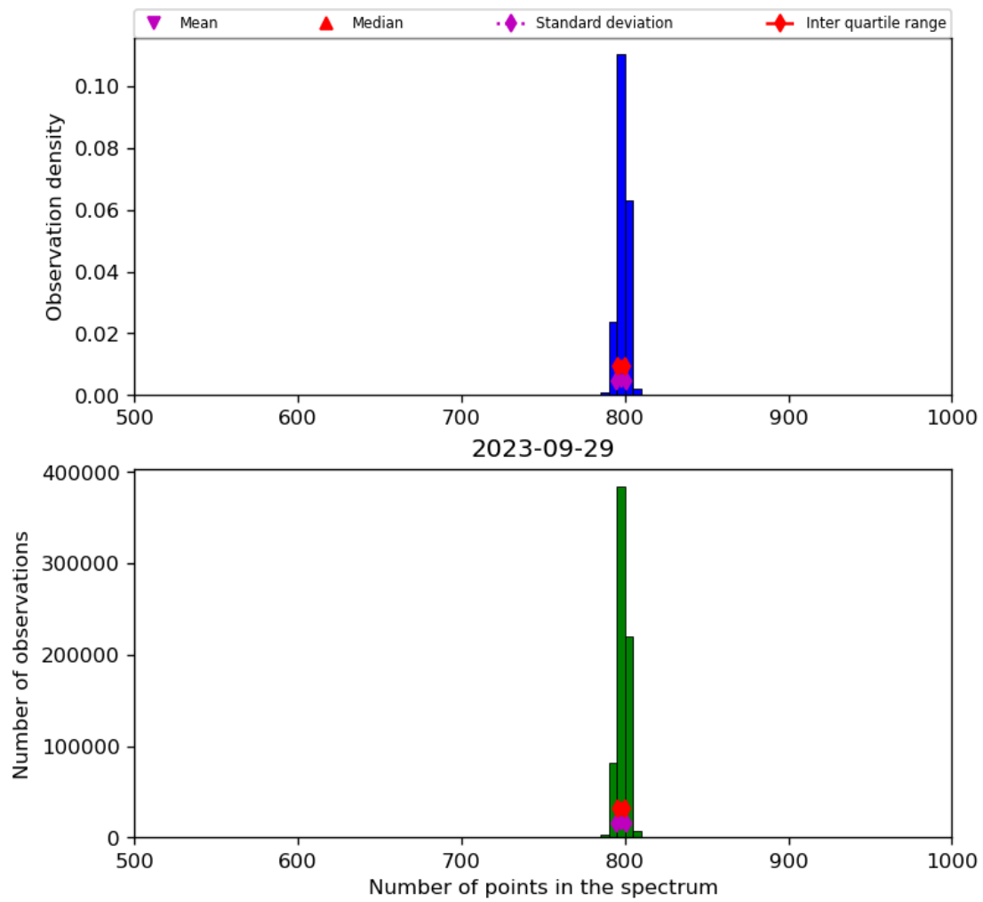
Figure 26: Histogram of “Number of points in the spectrum” for 2023-09-28 to 2023-09-30
