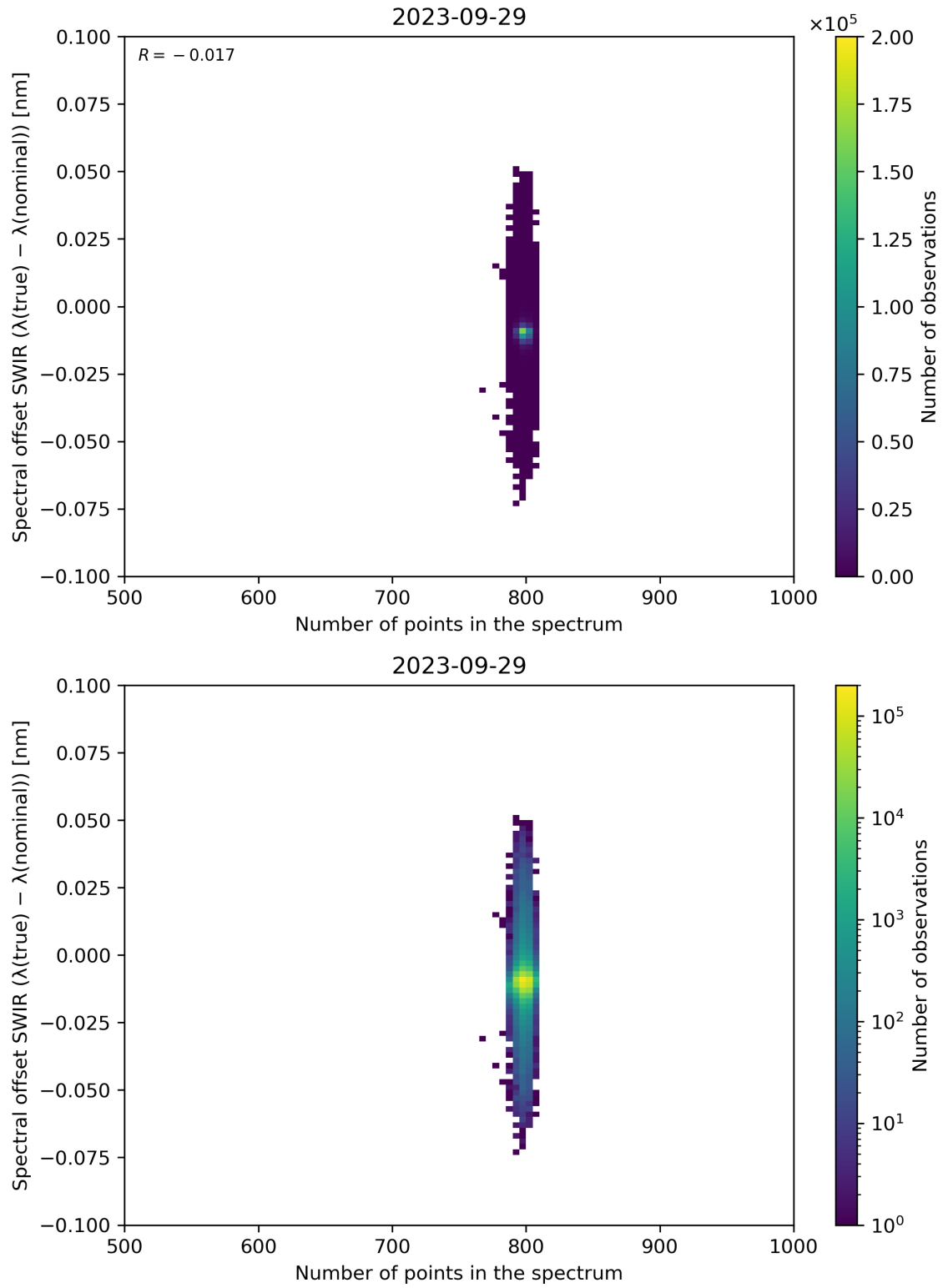
Figure 93: Scatter density plot of “Number of points in the spectrum” against “Spectral offset SWIR ( \lambda(\text{true}) - \lambda(\text{nominal}) )” for 2023-09-28 to 2023-09-30.
