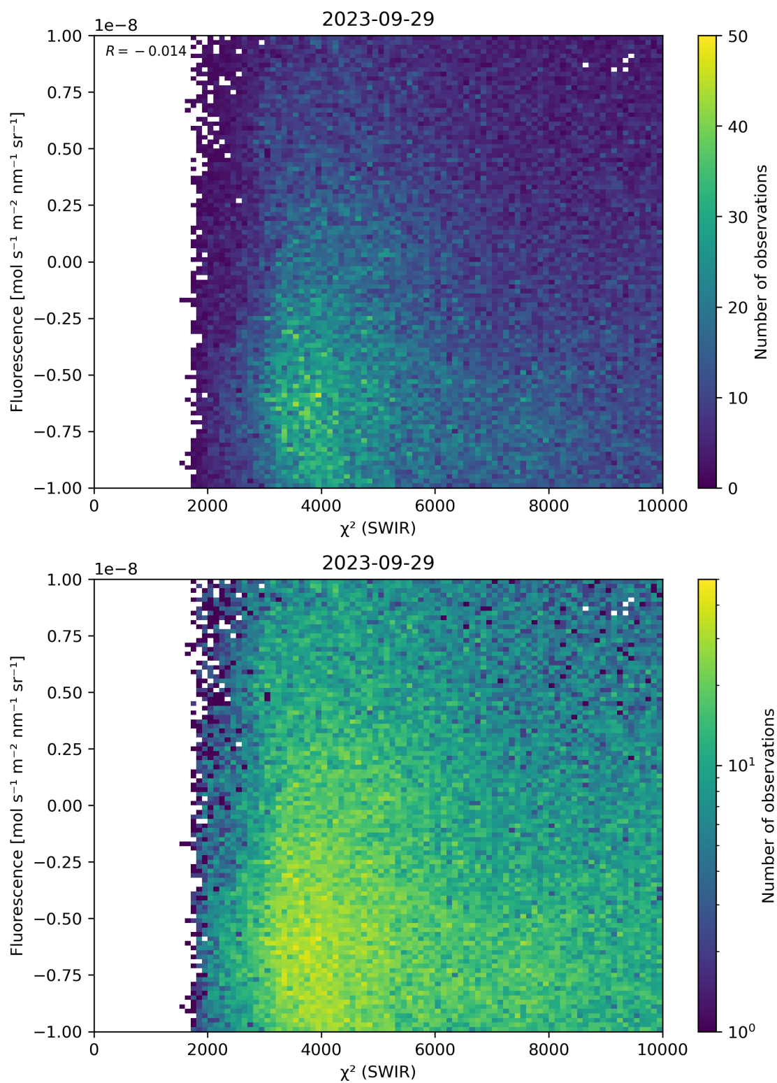
Figure 49: Scatter density plot of “ \chi^2 (SWIR)” against “Fluorescence” for 2023-09-28 to 2023-09-30.
