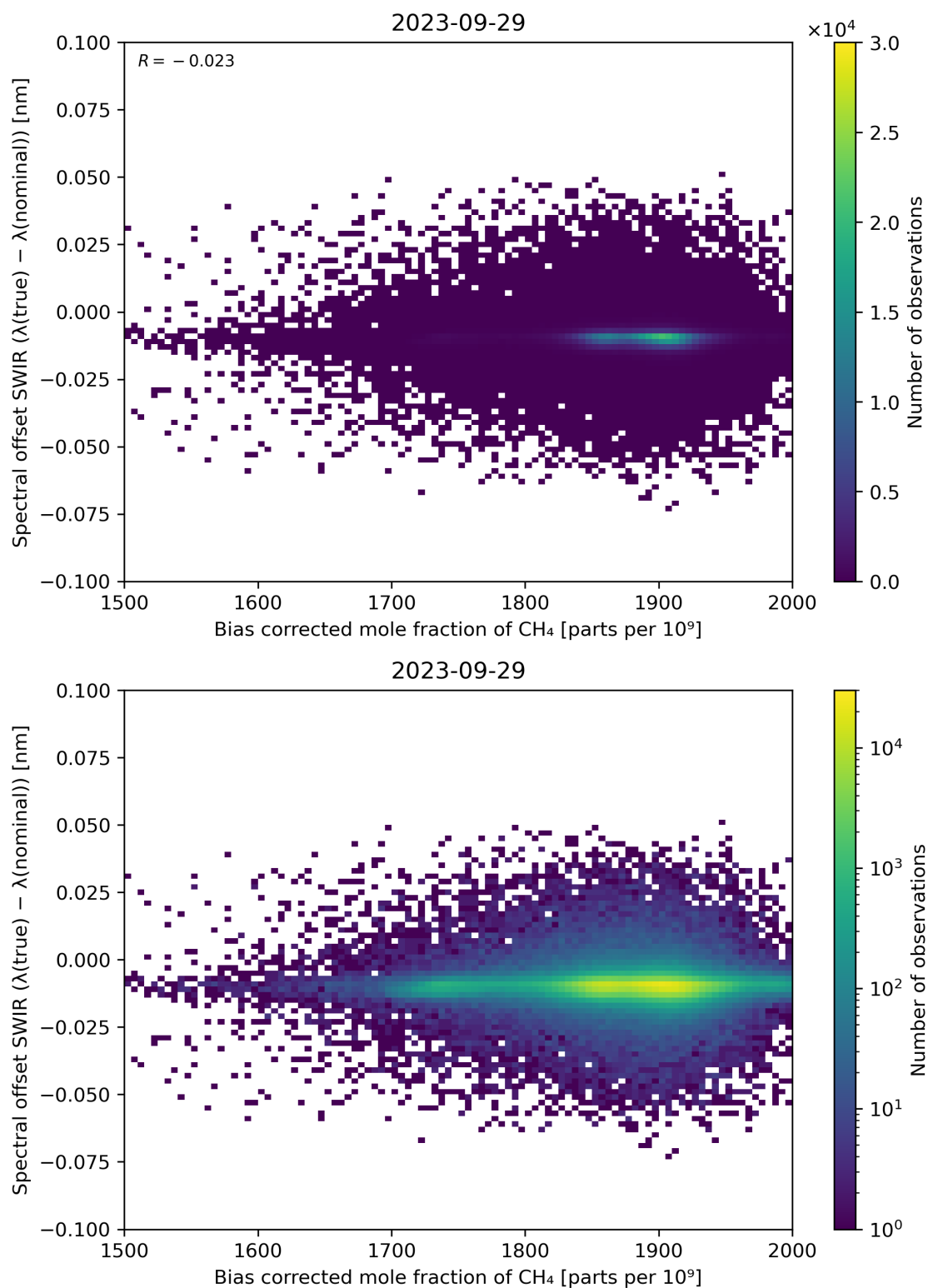
Figure 69: Scatter density plot of “Bias corrected mole fraction of \text{CH}_4 ” against “Spectral offset SWIR ( \lambda(\text{true}) - \lambda(\text{nominal}) )” for 2023-09-28 to 2023-09-30.
