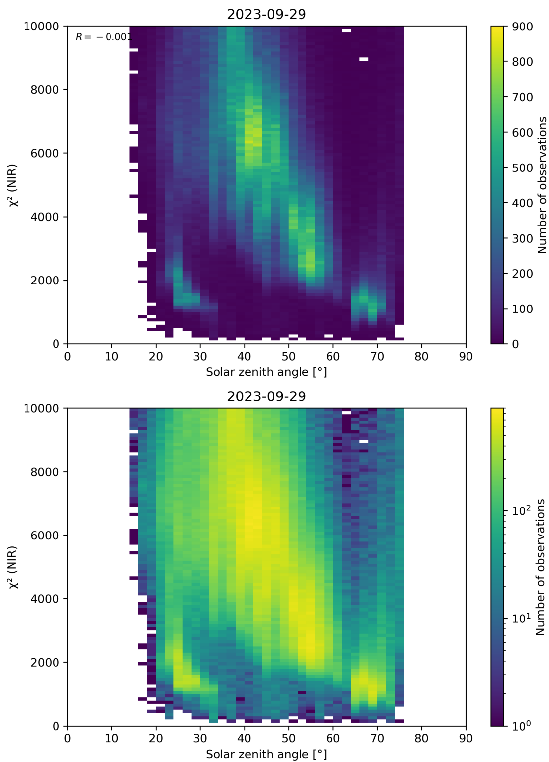
Figure 94: Scatter density plot of “Solar zenith angle” against “ \chi^2 (NIR)” for 2023-09-28 to 2023-09-30.
