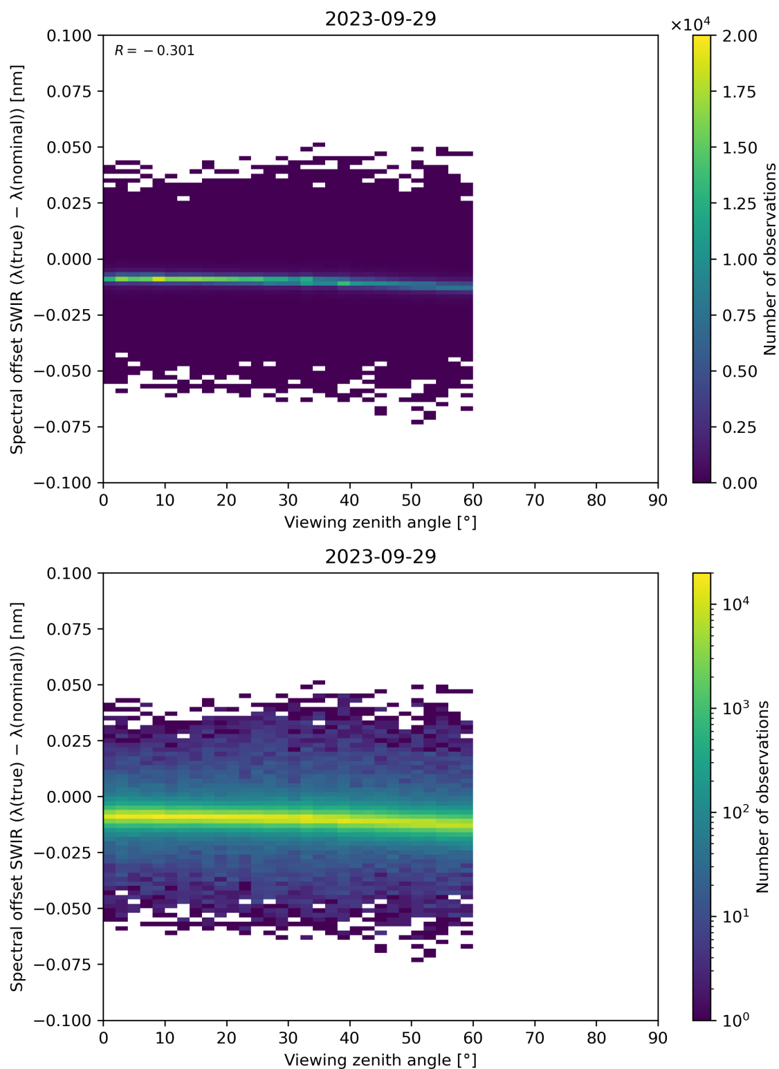
Figure 116: Scatter density plot of “Viewing zenith angle” against “Spectral offset SWIR ( \lambda(\text{true}) - \lambda(\text{nominal}) )” for 2023-09-28 to 2023-09-30.
