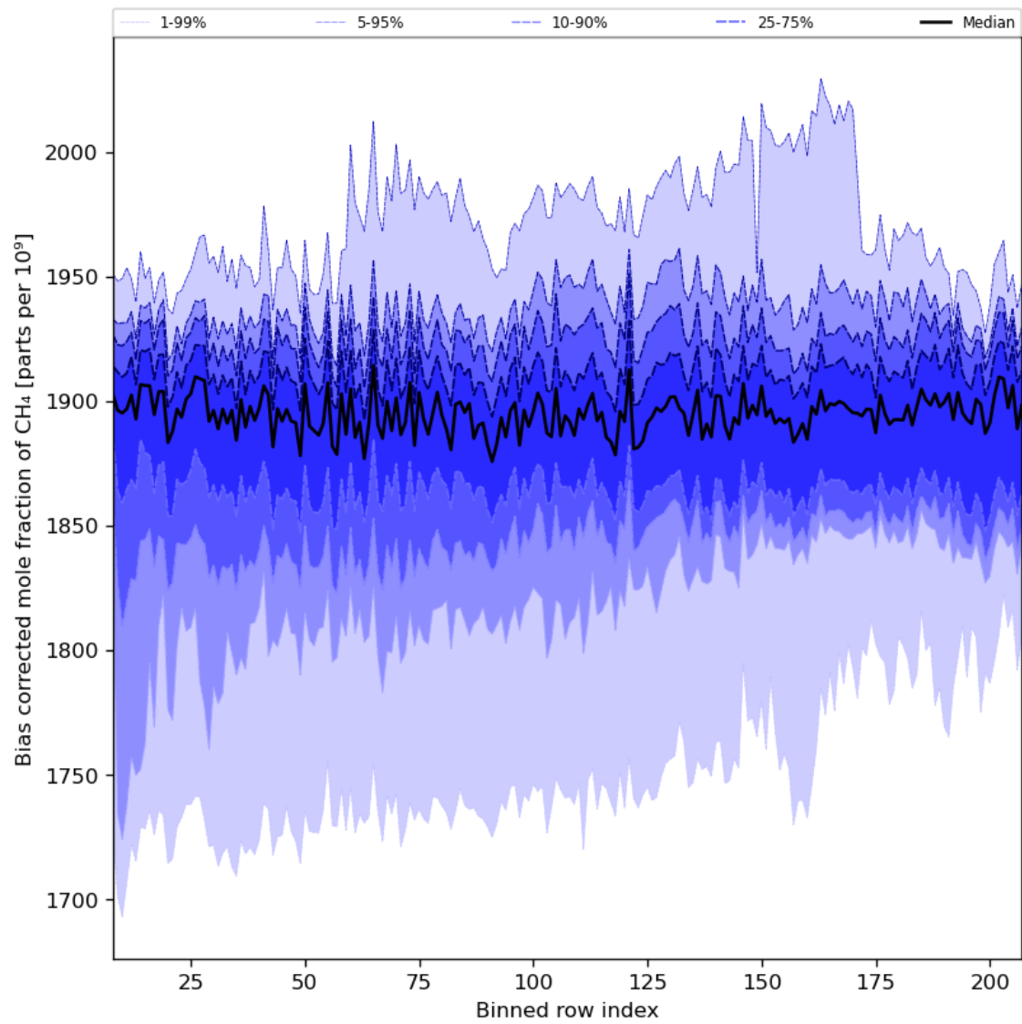
Figure 36: Along track statistics of “Bias corrected mole fraction of CH 4 ” for 2023-09-28 to 2023-09-30
