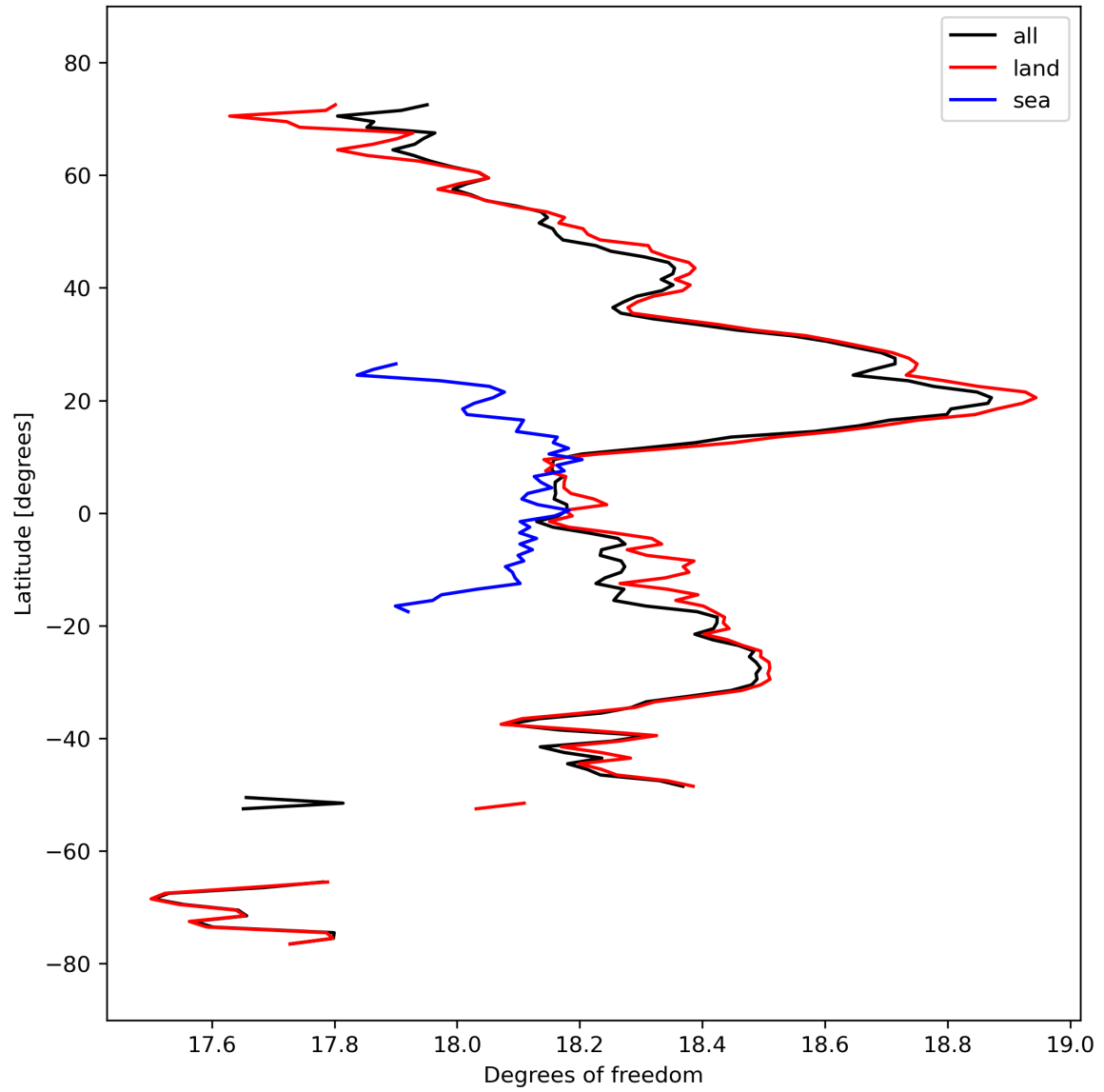
Figure 19: Zonal average of “Degrees of freedom” for 2023-09-28 to 2023-09-30.
