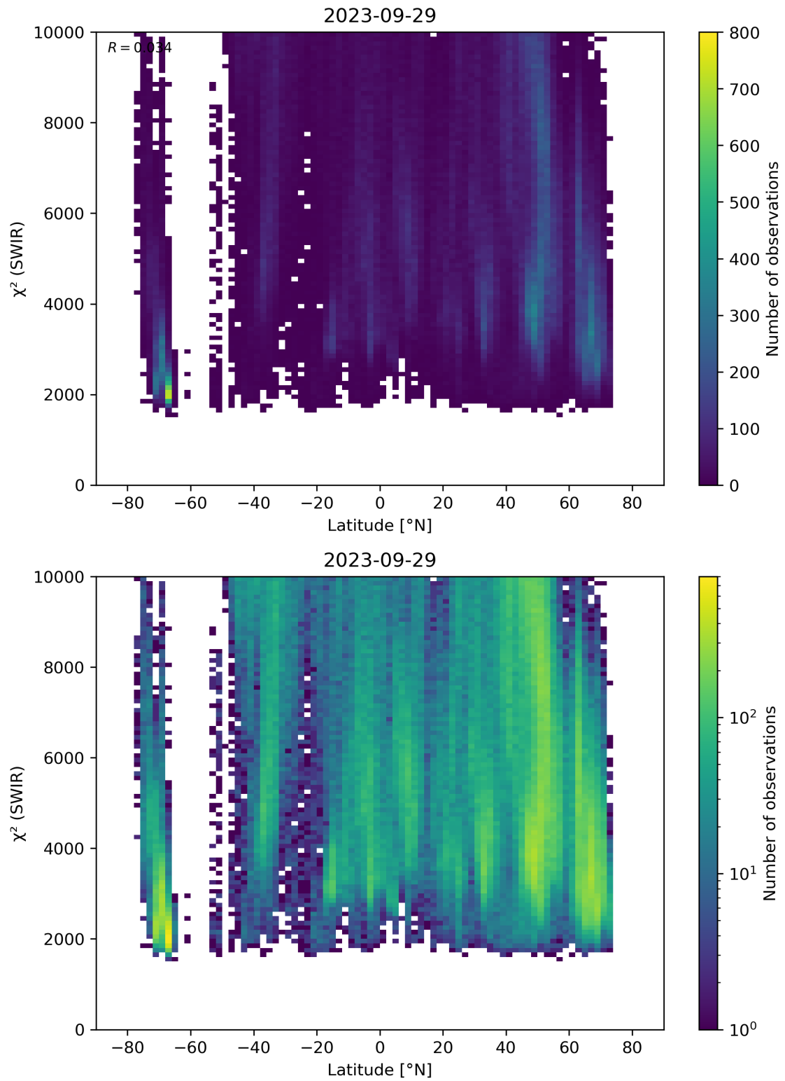
Figure 54: Scatter density plot of “Latitude” against “ \chi^2 (SWIR)” for 2023-09-28 to 2023-09-30.
