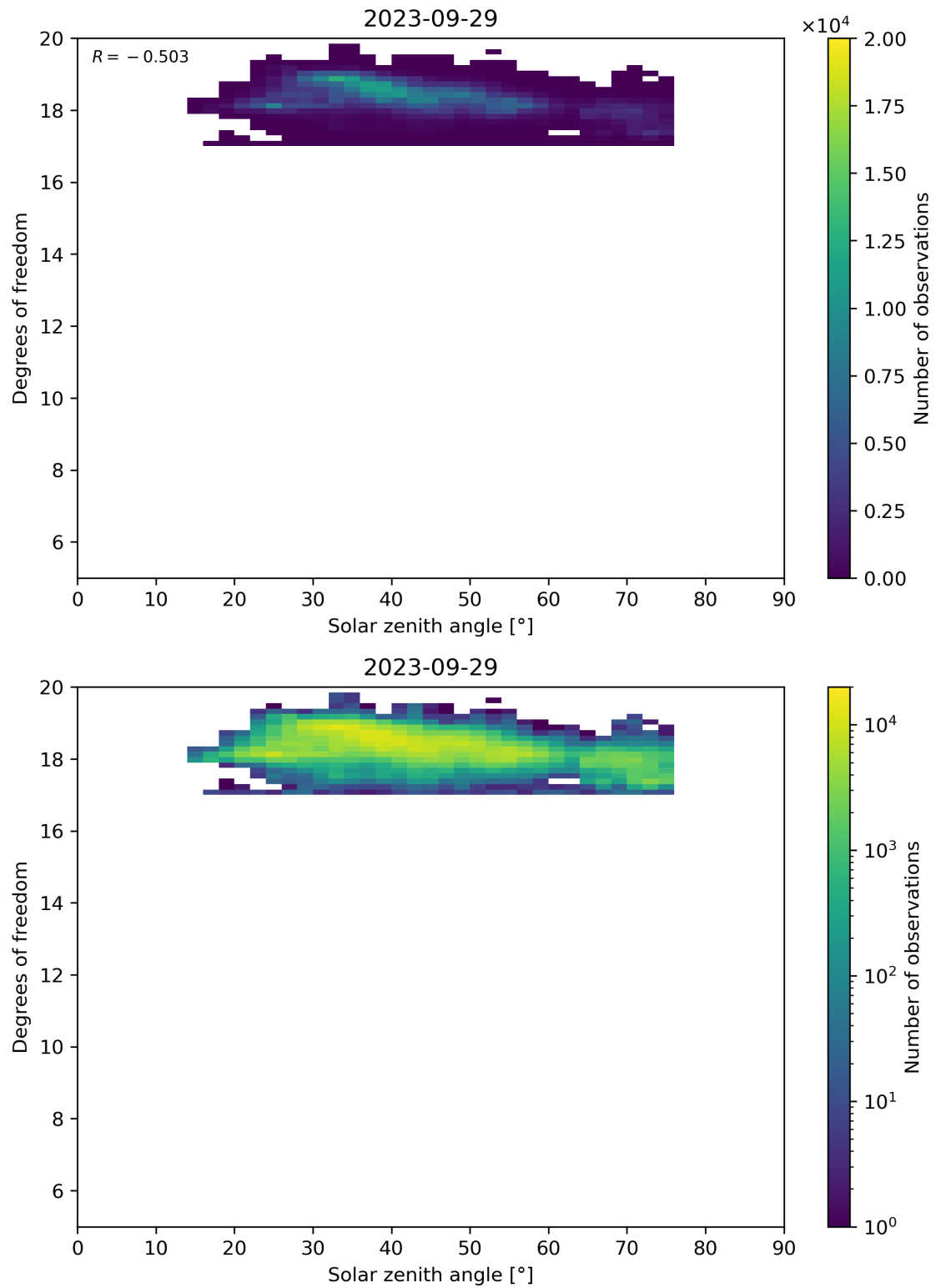
Figure 96: Scatter density plot of “Solar zenith angle” against “Degrees of freedom” for 2023-09-28 to 2023-09-30.
