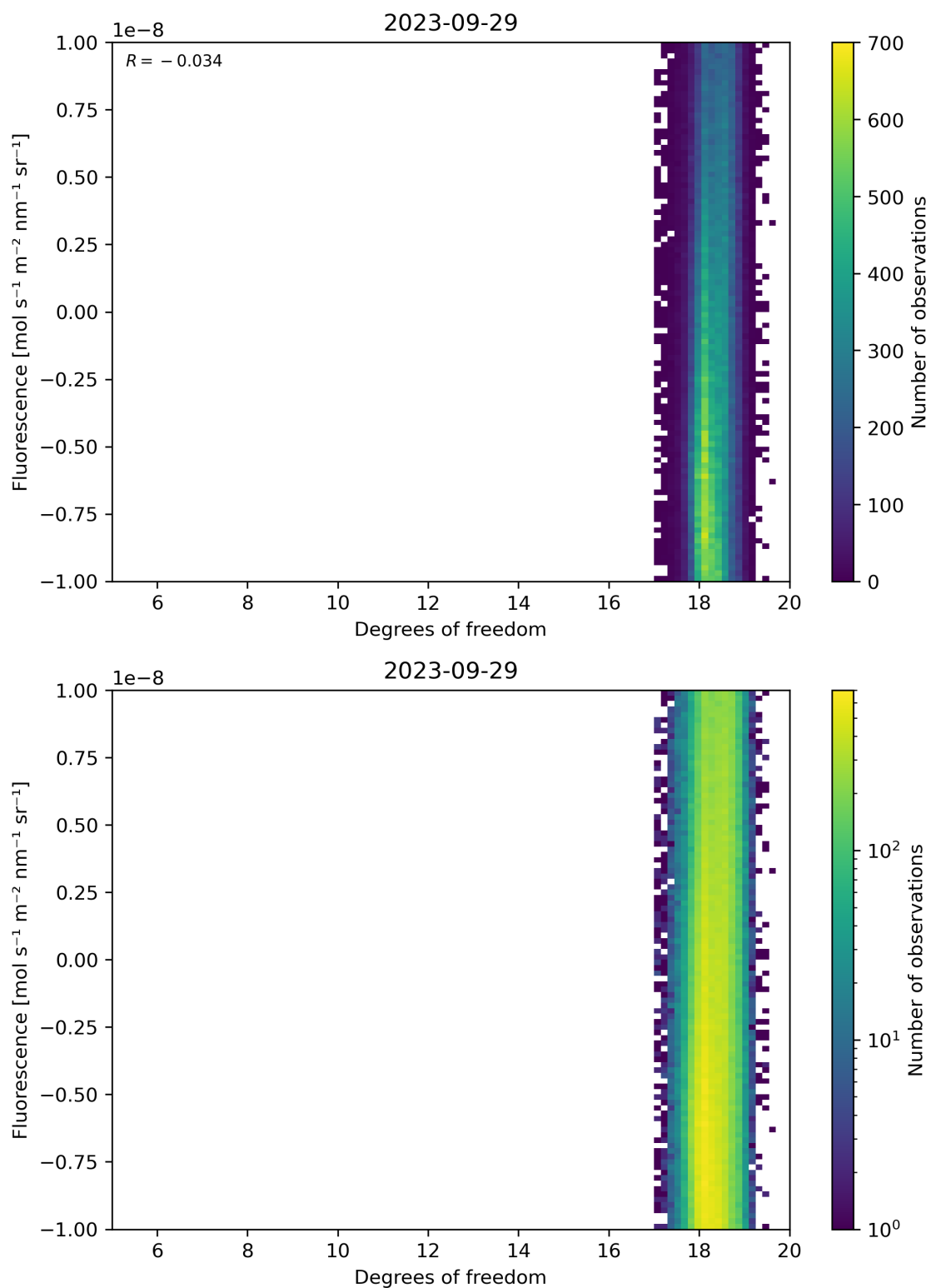
Figure 51: Scatter density plot of “Degrees of freedom” against “Fluorescence” for 2023-09-28 to 2023-09-30.
