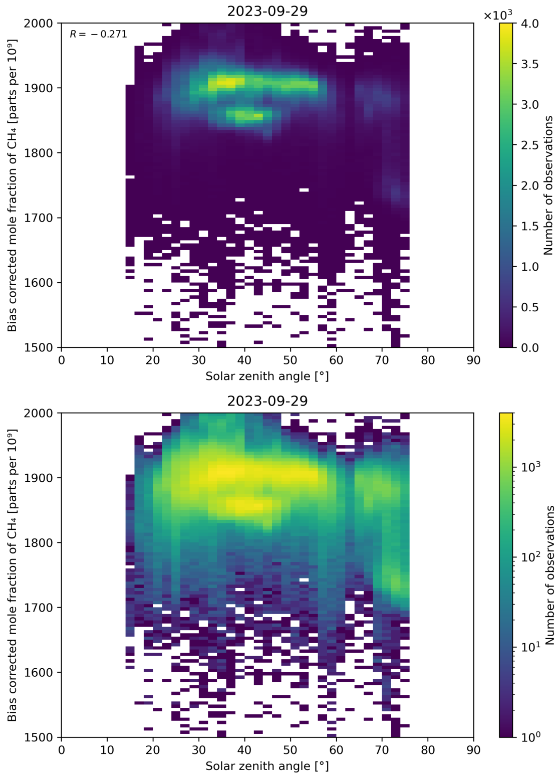
Figure 100: Scatter density plot of “Solar zenith angle” against “Bias corrected mole fraction of \text{CH}_4 ” for 2023-09-28 to 2023-09-30.
