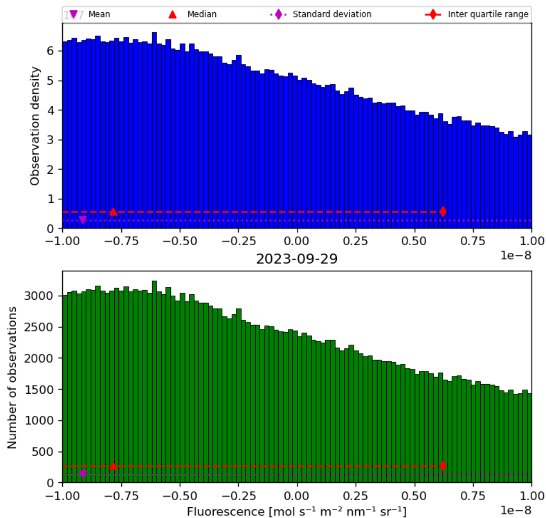
Figure 32: Histogram of “Fluorescence” for 2023-09-28 to 2023-09-30
