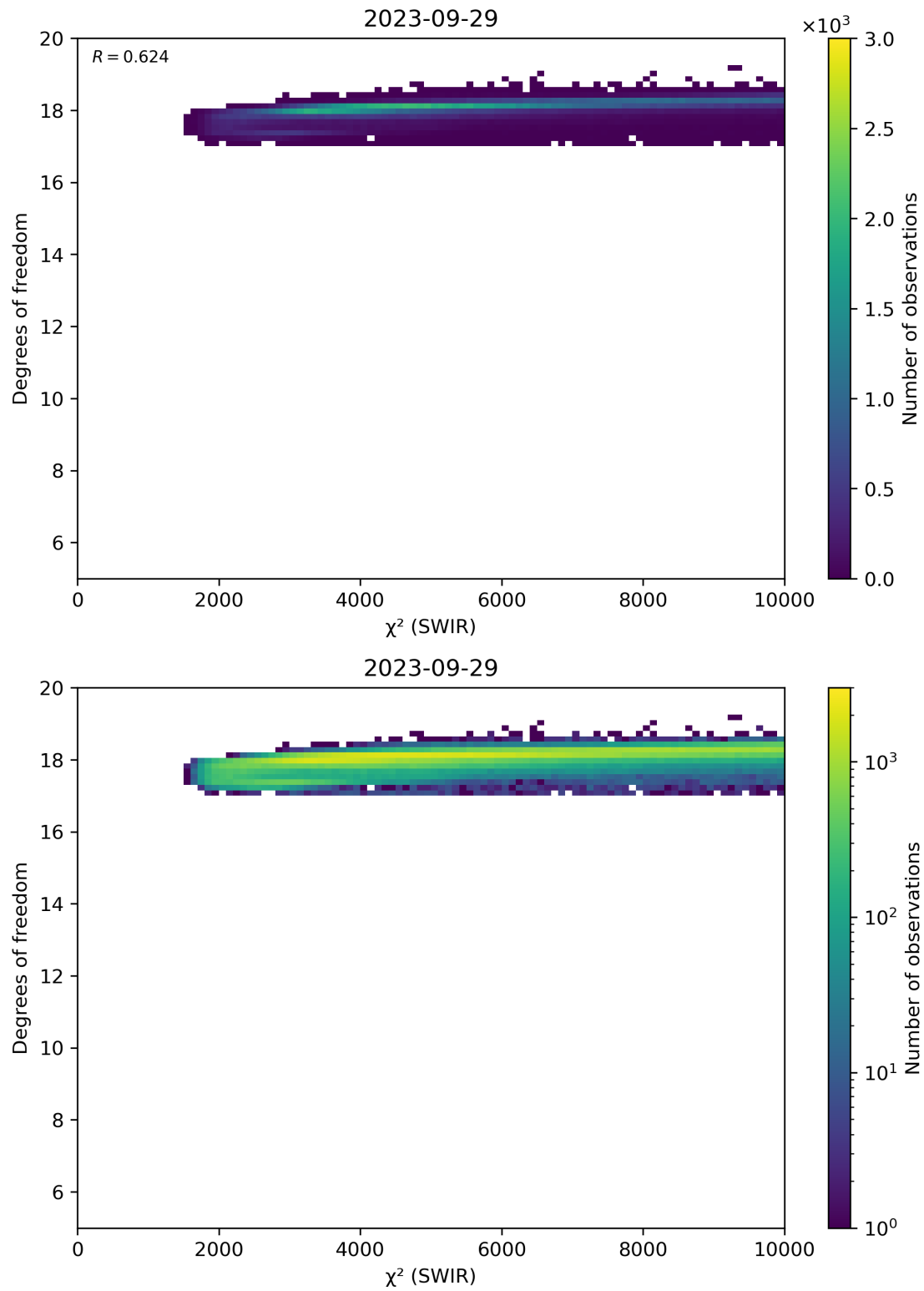
Figure 48: Scatter density plot of “ \chi^2 (SWIR)” against “Degrees of freedom” for 2023-09-28 to 2023-09-30.
