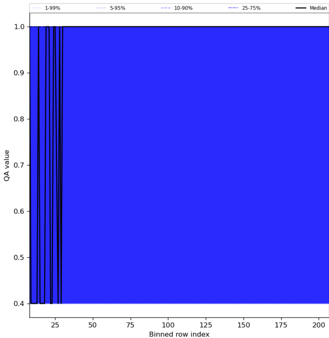
Figure 33: Along track statistics of “QA value” for 2023-09-28 to 2023-09-30
