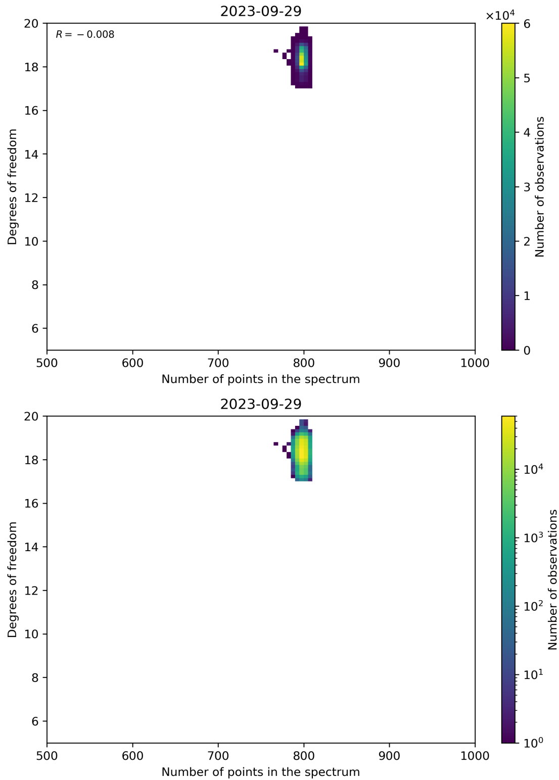
Figure 90: Scatter density plot of “Number of points in the spectrum” against “Degrees of freedom” for 2023-09-28 to 2023-09-30.
