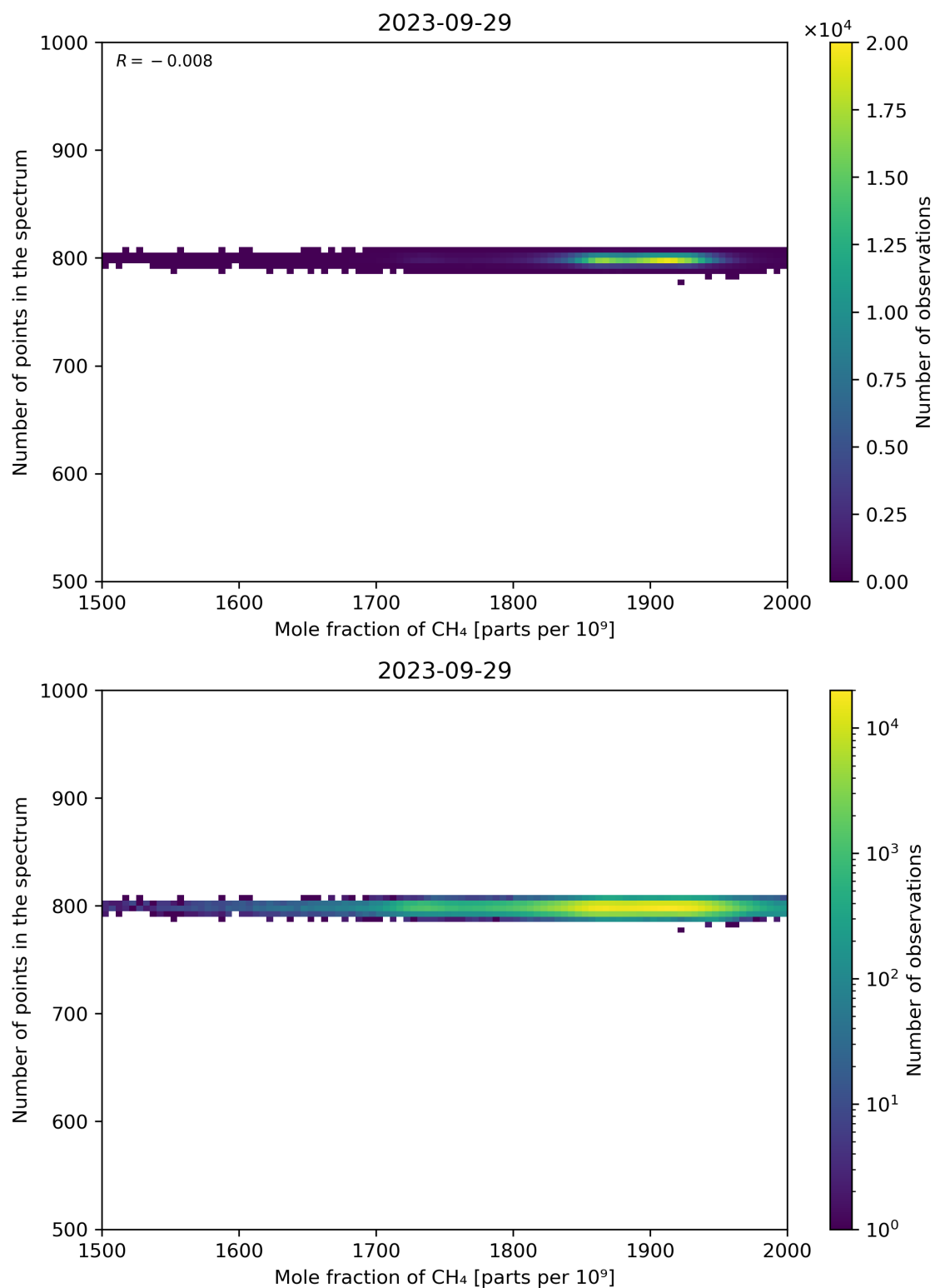
Figure 77: Scatter density plot of “Mole fraction of CH 4 ” against “Number of points in the spectrum” for 2023-09-28 to 2023-09-30.
