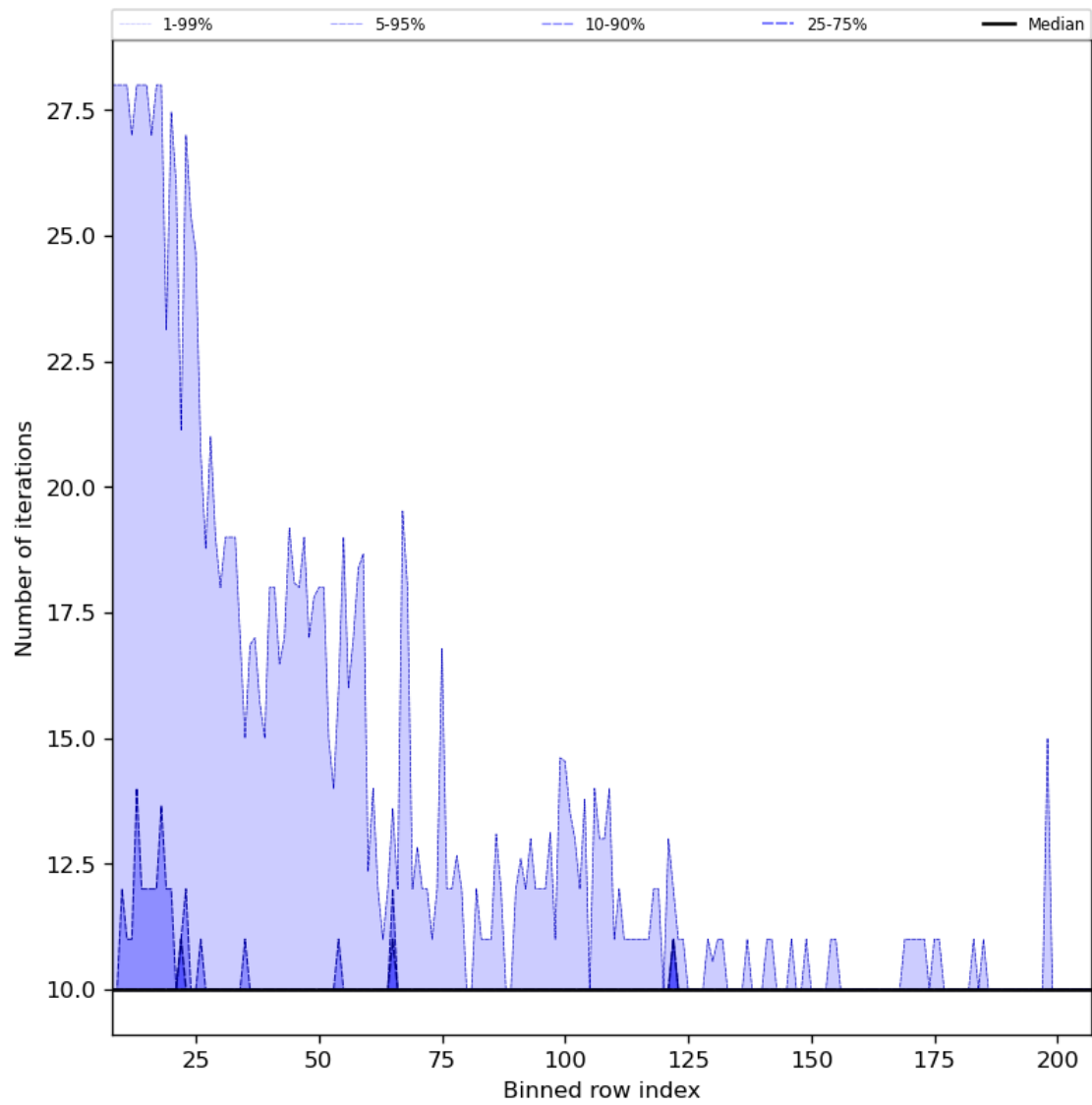
Figure 42: Along track statistics of “Number of iterations” for 2023-09-28 to 2023-09-30
