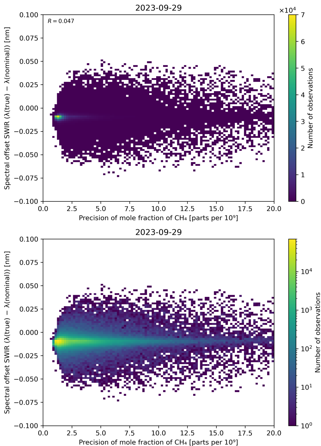
Figure 85: Scatter density plot of “Precision of mole fraction of CH 4 ” against “Spectral offset SWIR ( \lambda(\text{true}) - \lambda(\text{nominal}) )” for 2023-09-28 to 2023-09-30.
