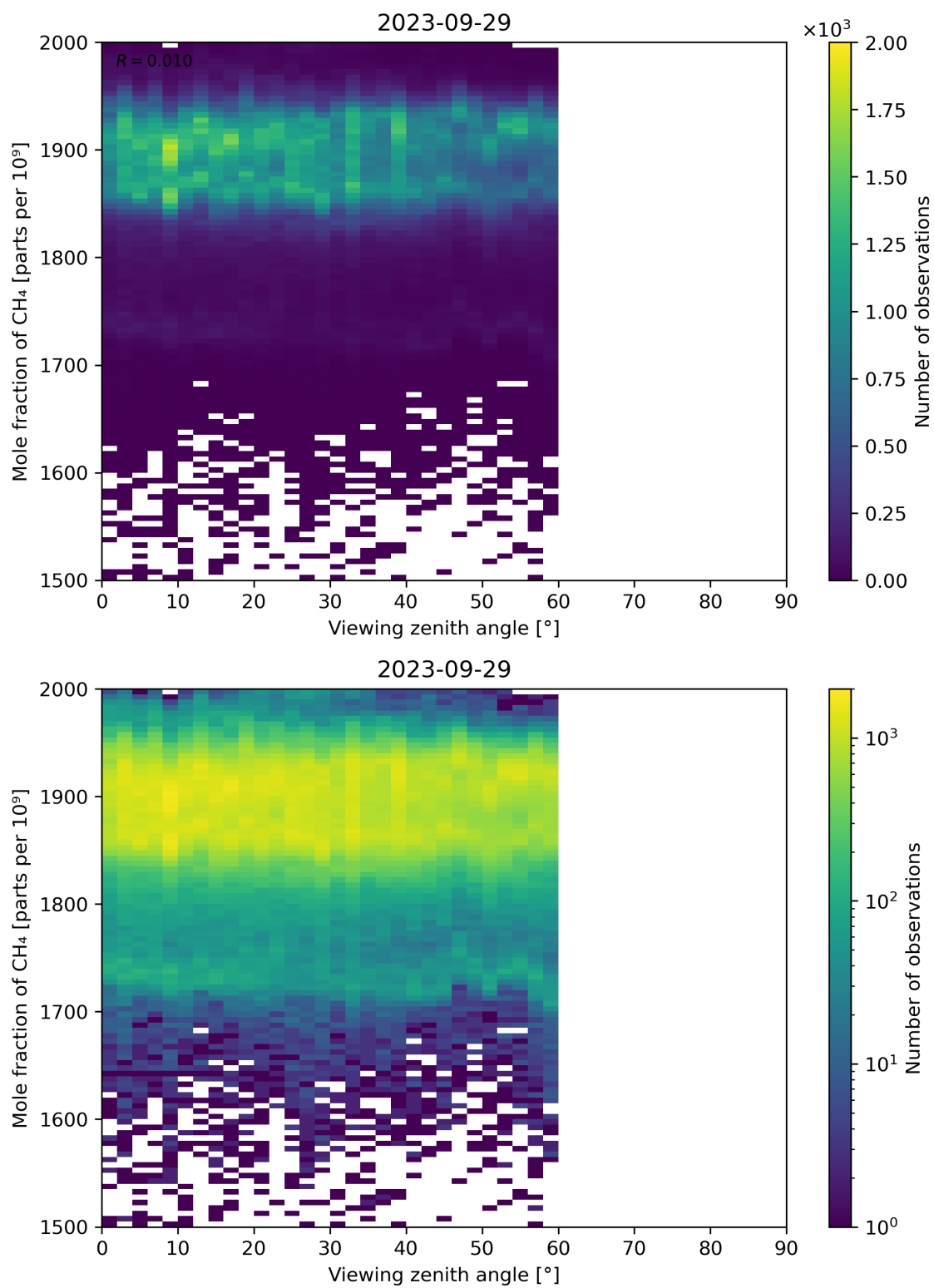
Figure 110: Scatter density plot of “Viewing zenith angle” against “Mole fraction of CH 4 ” for 2023-09-28 to 2023-09-30.
