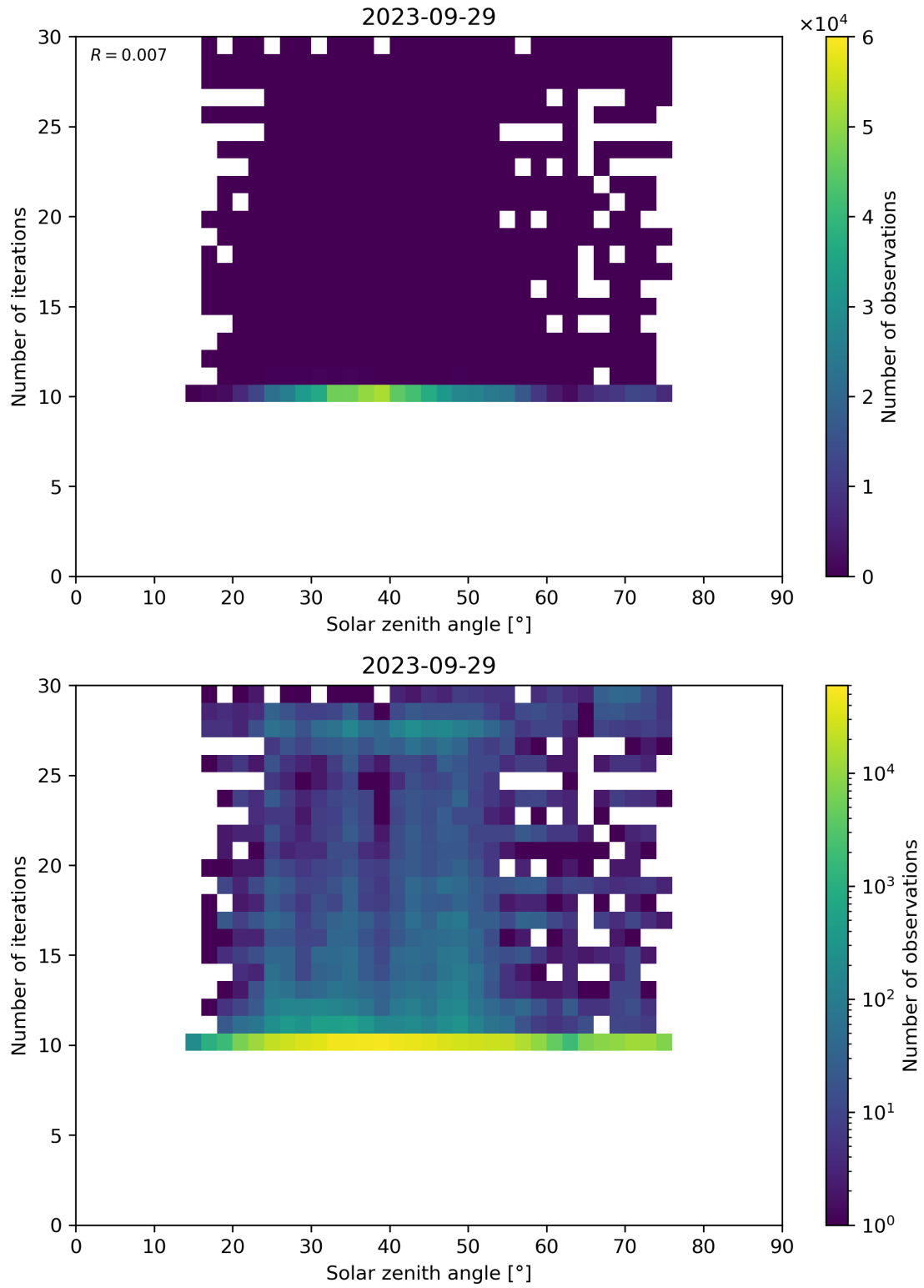
Figure 102: Scatter density plot of “Solar zenith angle” against “Number of iterations” for 2023-09-28 to 2023-09-30.
