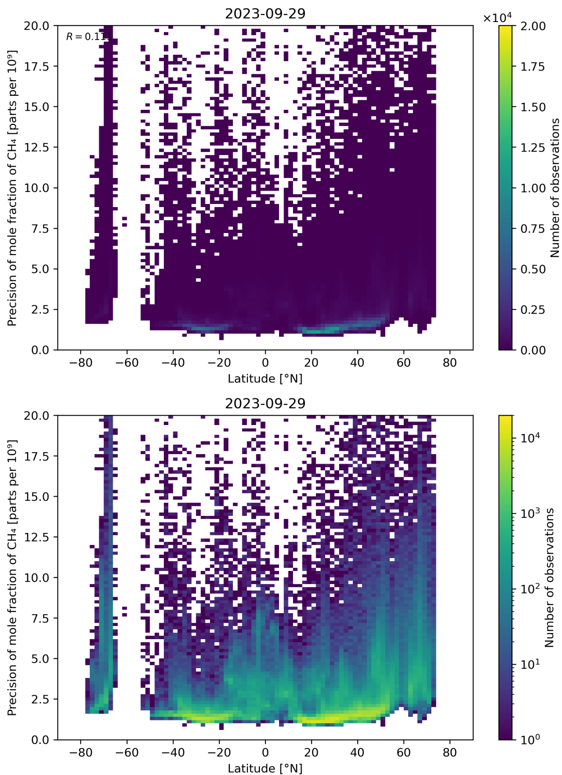
Figure 59: Scatter density plot of “Latitude” against “Precision of mole fraction of CH 4 ” for 2023-09-28 to 2023-09-30.
