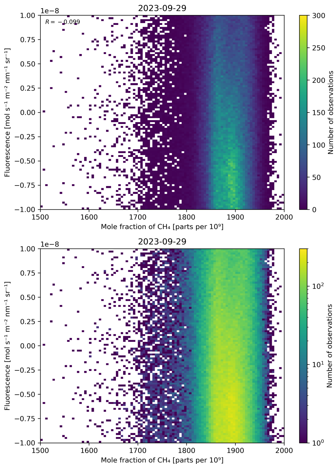
Figure 73: Scatter density plot of “Mole fraction of \text{CH}_4 ” against “Fluorescence” for 2023-09-28 to 2023-09-30.
