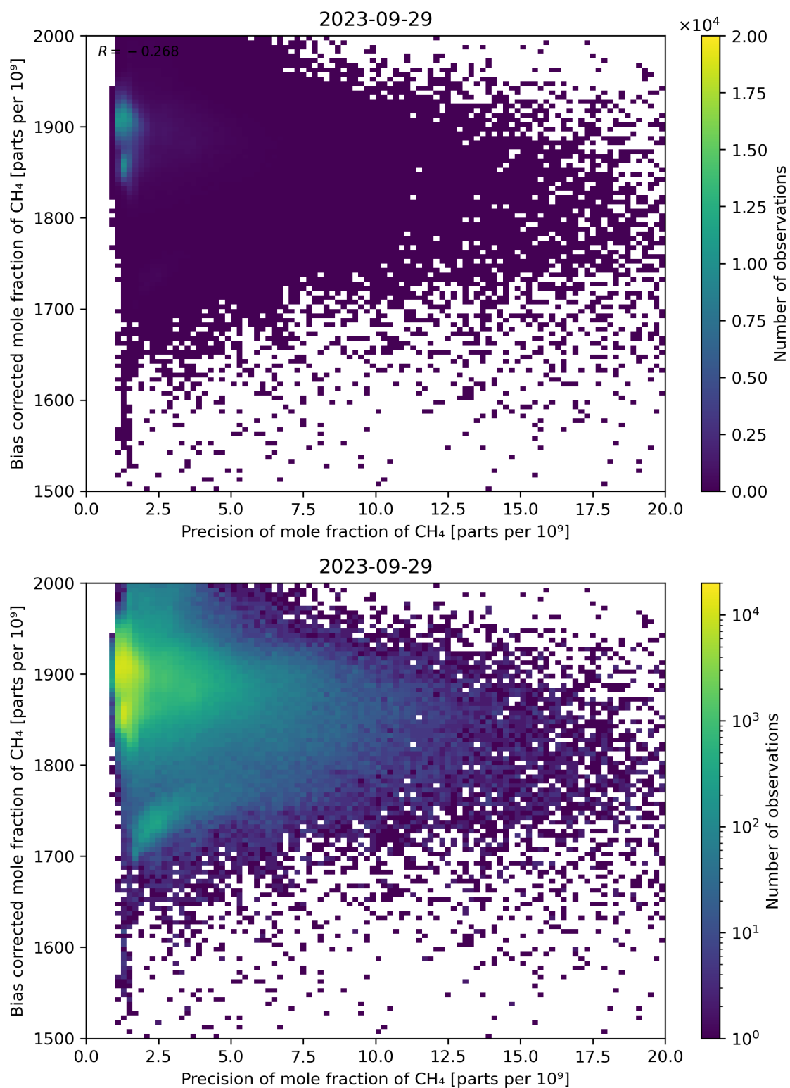
Figure 82: Scatter density plot of “Precision of mole fraction of CH 4 ” against “Bias corrected mole fraction of CH 4 ” for 2023-09-28 to 2023-09-30.
