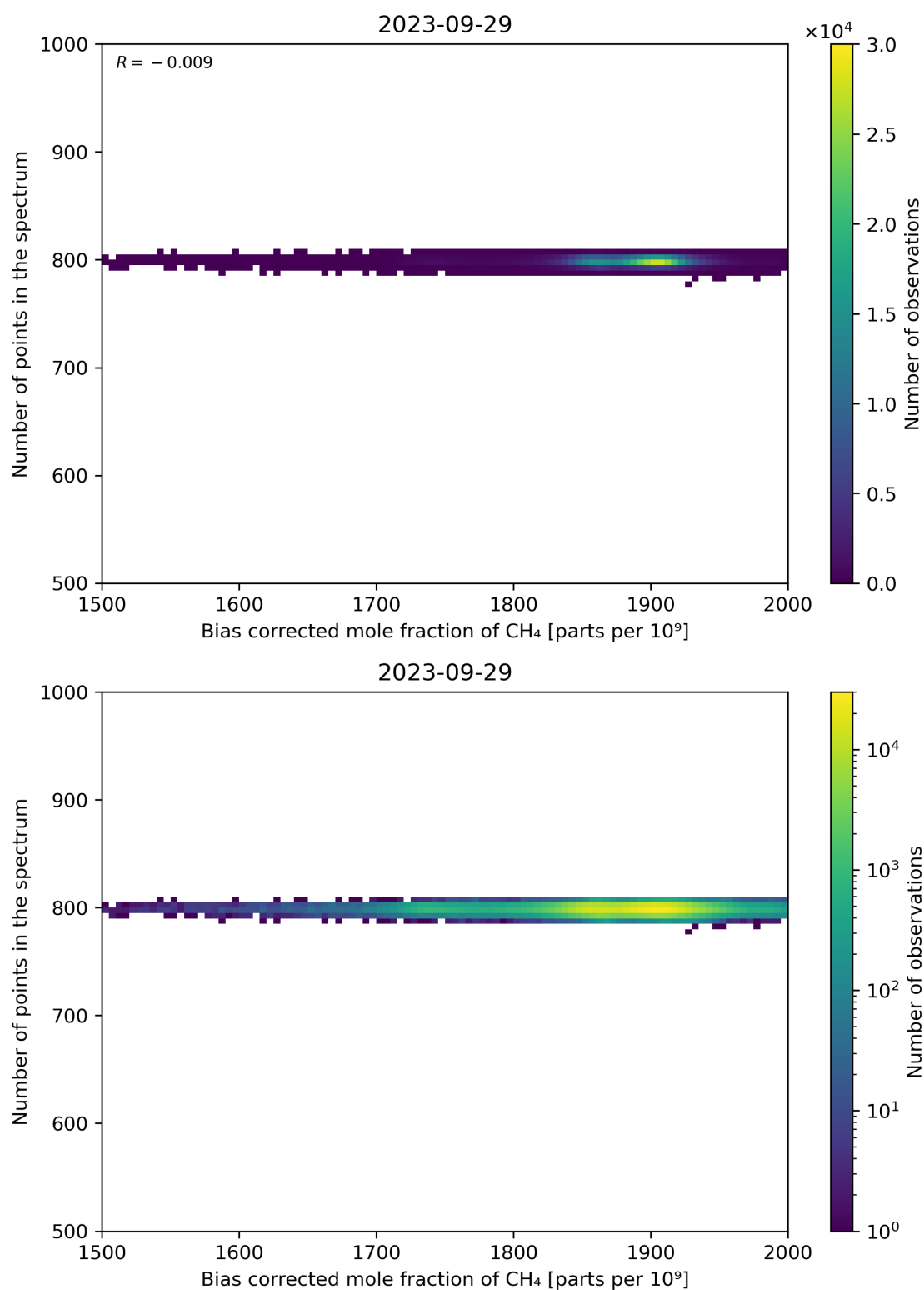
Figure 68: Scatter density plot of “Bias corrected mole fraction of CH 4 ” against “Number of points in the spectrum” for 2023-09-28 to 2023-09-30.
