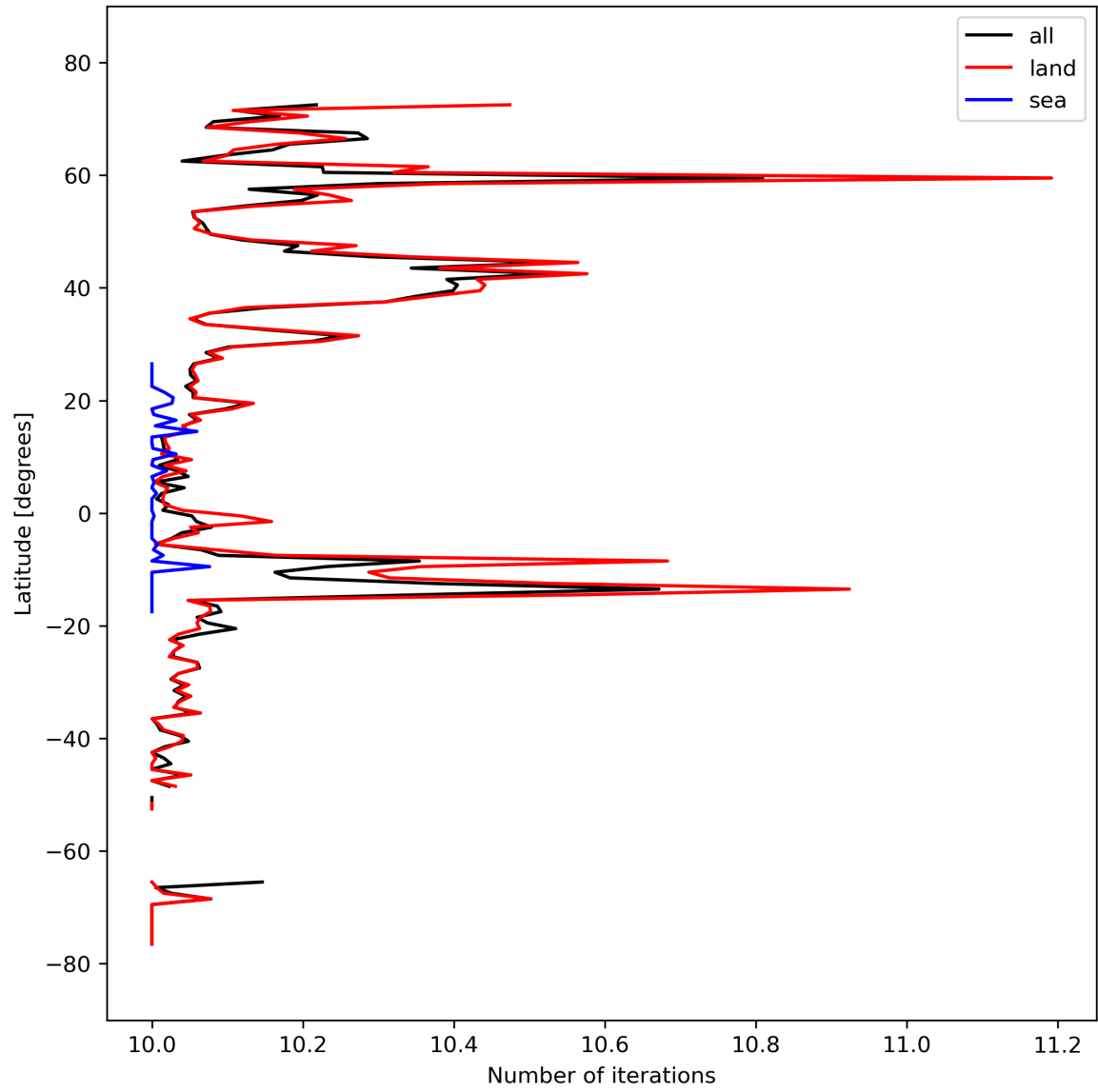
Figure 20: Zonal average of “Number of iterations” for 2023-09-28 to 2023-09-30.
