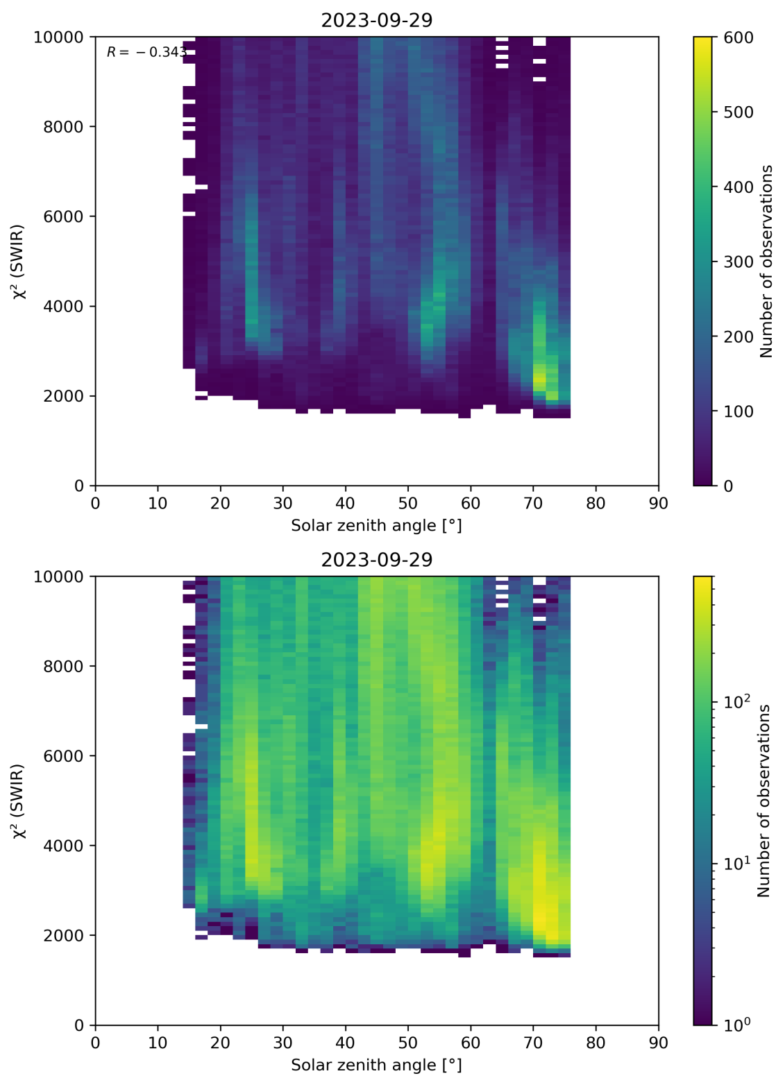
Figure 95: Scatter density plot of “Solar zenith angle” against “ \chi^2 (SWIR)” for 2023-09-28 to 2023-09-30.
