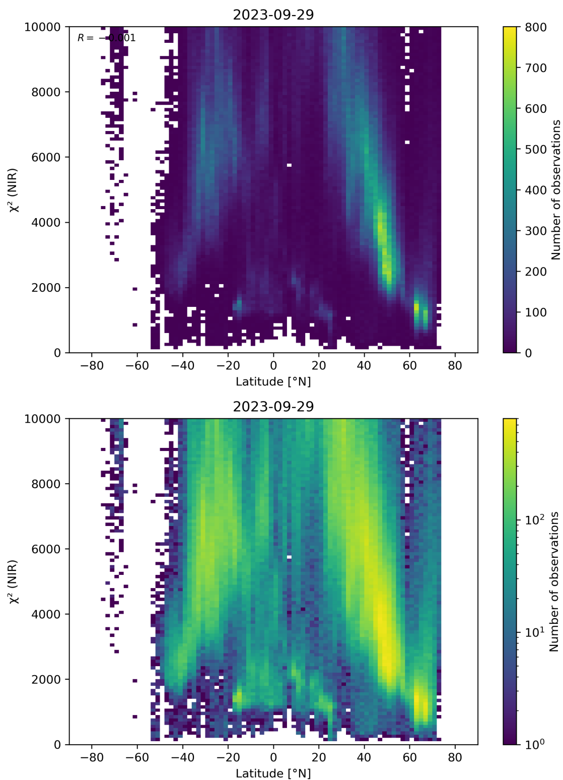
Figure 53: Scatter density plot of “Latitude” against “ \chi^2 (NIR)” for 2023-09-28 to 2023-09-30.
