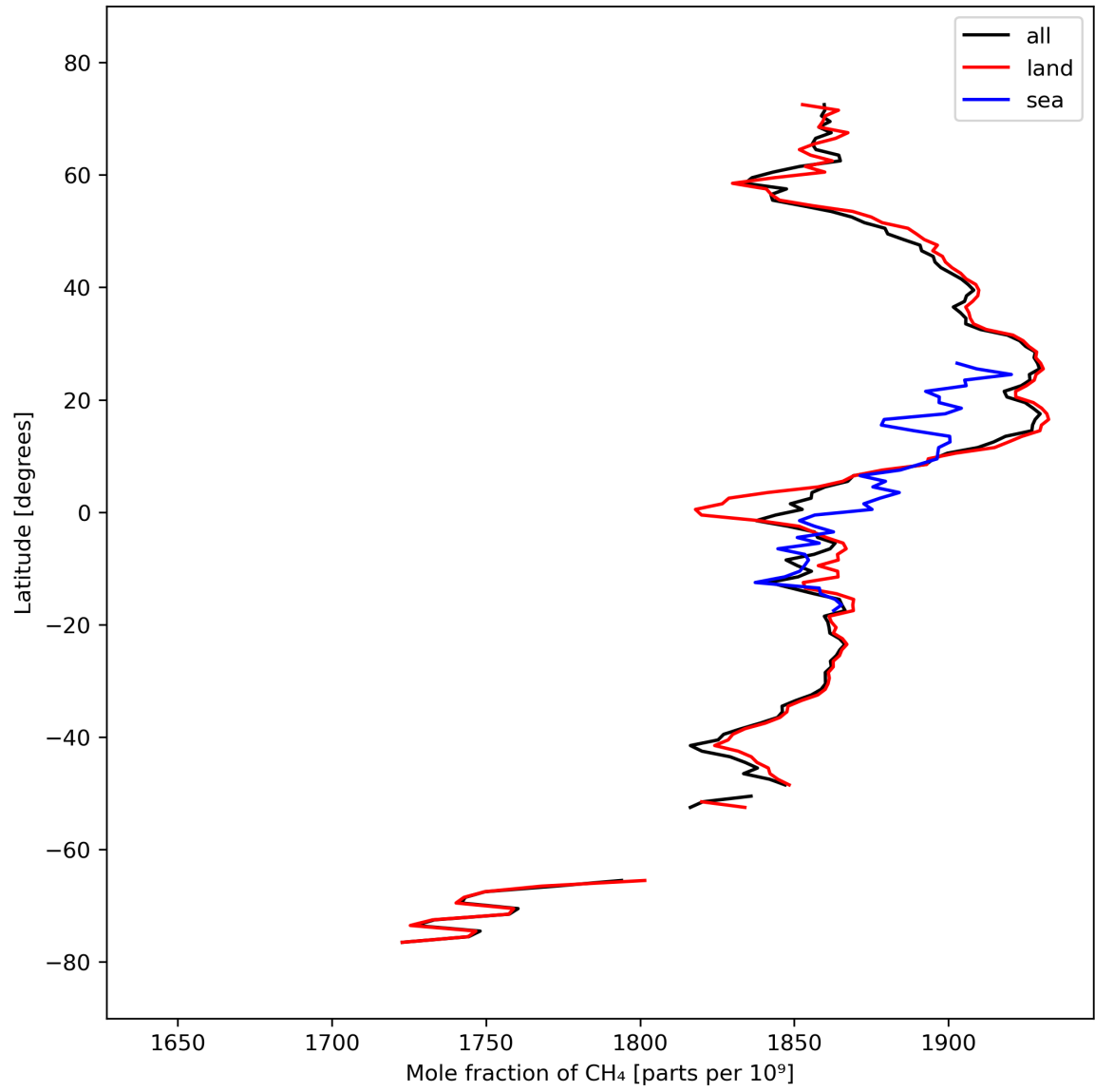
Figure 12: Zonal average of “Mole fraction of \text{CH}_4 ” for 2023-09-28 to 2023-09-30.
