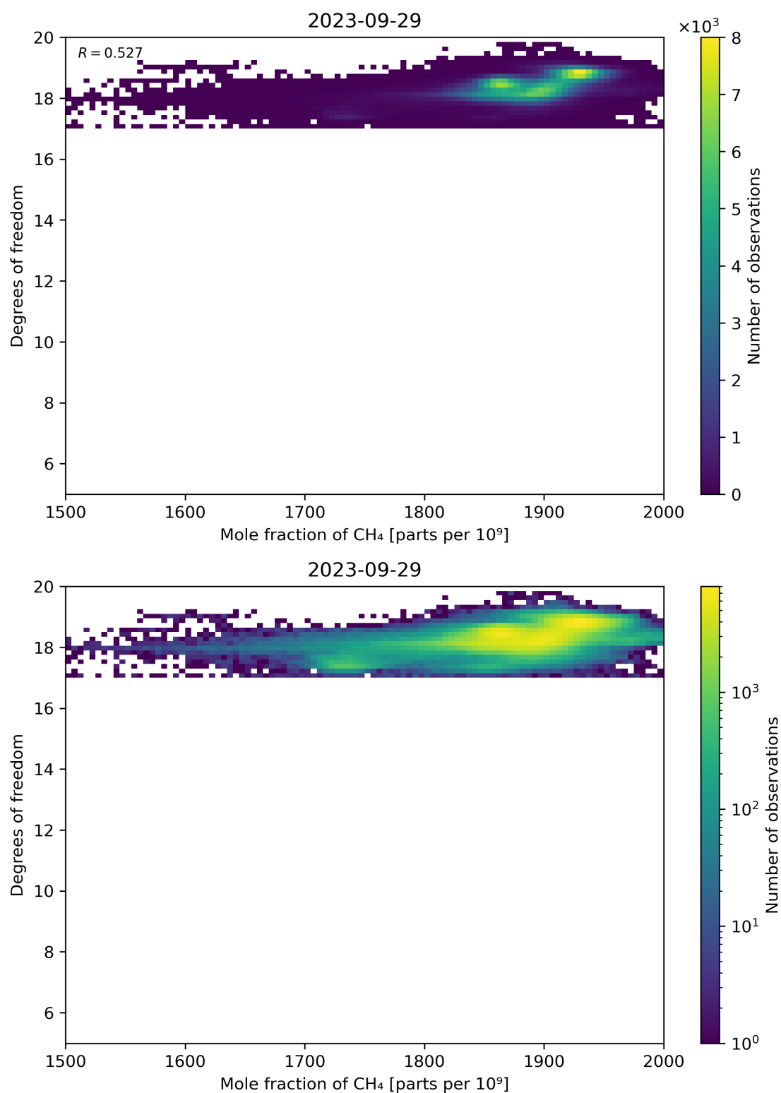
Figure 72: Scatter density plot of “Mole fraction of CH 4 ” against “Degrees of freedom” for 2023-09-28 to 2023-09-30.
