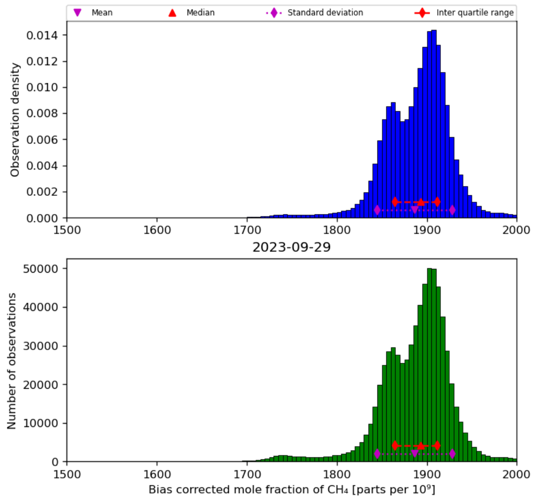
Figure 25: Histogram of “Bias corrected mole fraction of CH 4 ” for 2023-09-28 to 2023-09-30
