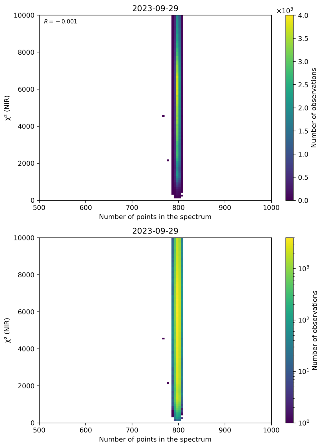
Figure 88: Scatter density plot of “Number of points in the spectrum” against “ \chi^2 (NIR)” for 2023-09-28 to 2023-09-30.
