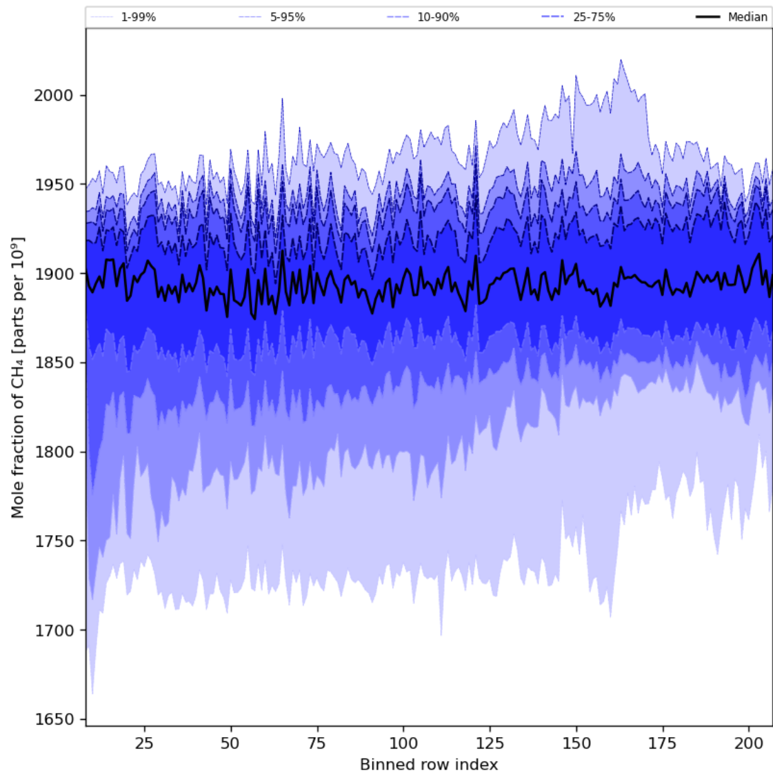
Figure 34: Along track statistics of “Mole fraction of CH 4 ” for 2023-09-28 to 2023-09-30
