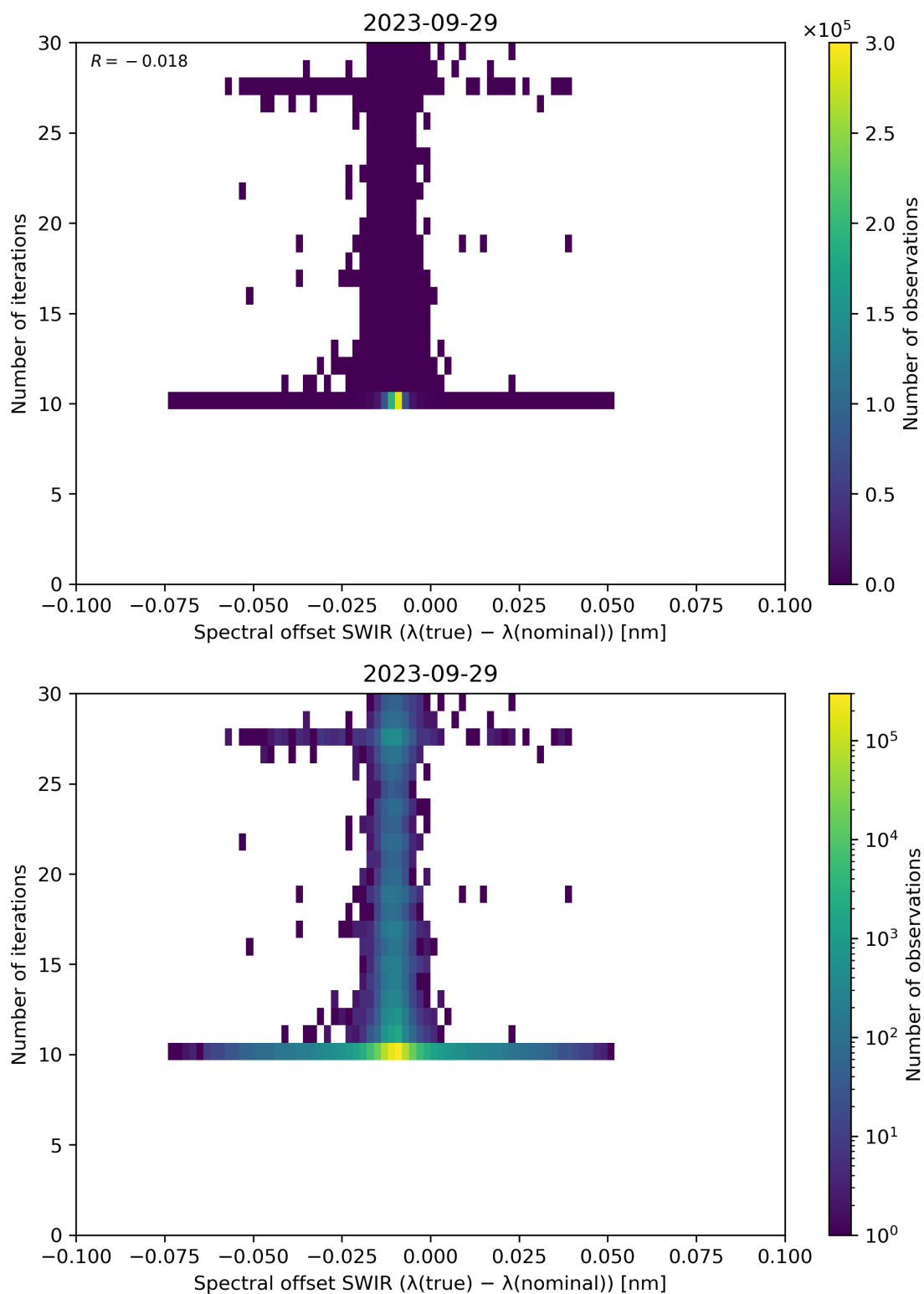
Figure 121: Scatter density plot of “Spectral offset SWIR ( \lambda(\text{true}) - \lambda(\text{nominal}) )” against “Number of iterations” for 2023-09-28 to 2023-09-30.
