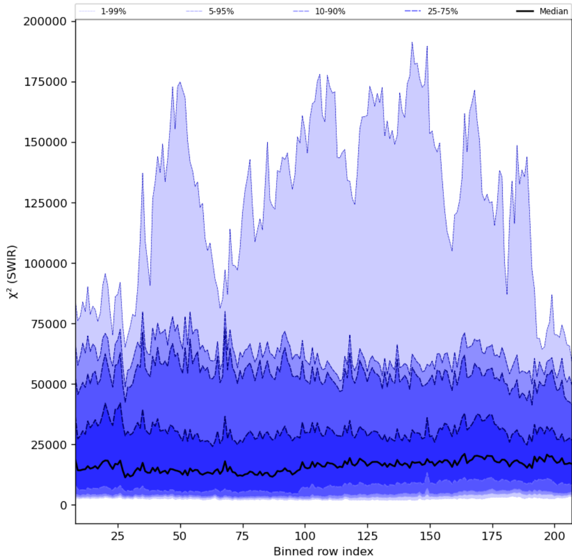
Figure 39: Along track statistics of “ \chi^2 (SWIR)” for 2023-09-28 to 2023-09-30
