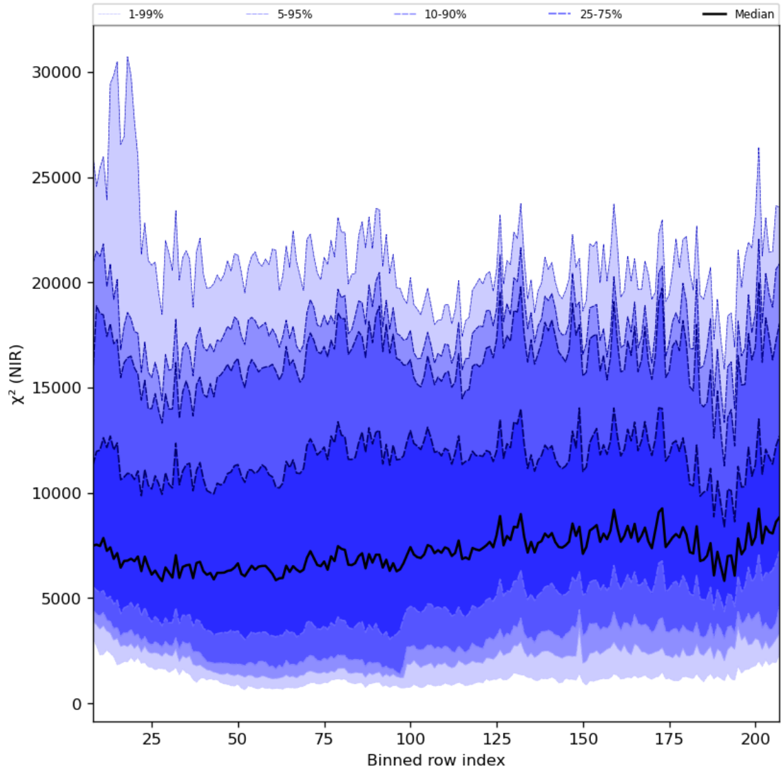
Figure 40: Along track statistics of “ \chi^2 (NIR)” for 2023-09-28 to 2023-09-30
