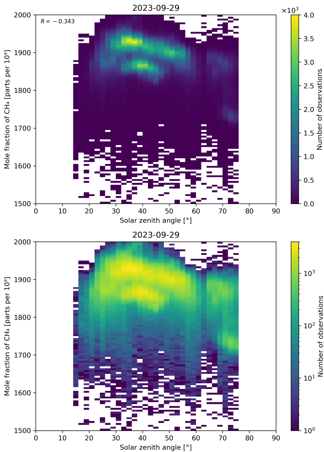
Figure 99: Scatter density plot of “Solar zenith angle” against “Mole fraction of CH 4 ” for 2023-09-28 to 2023-09-30.
