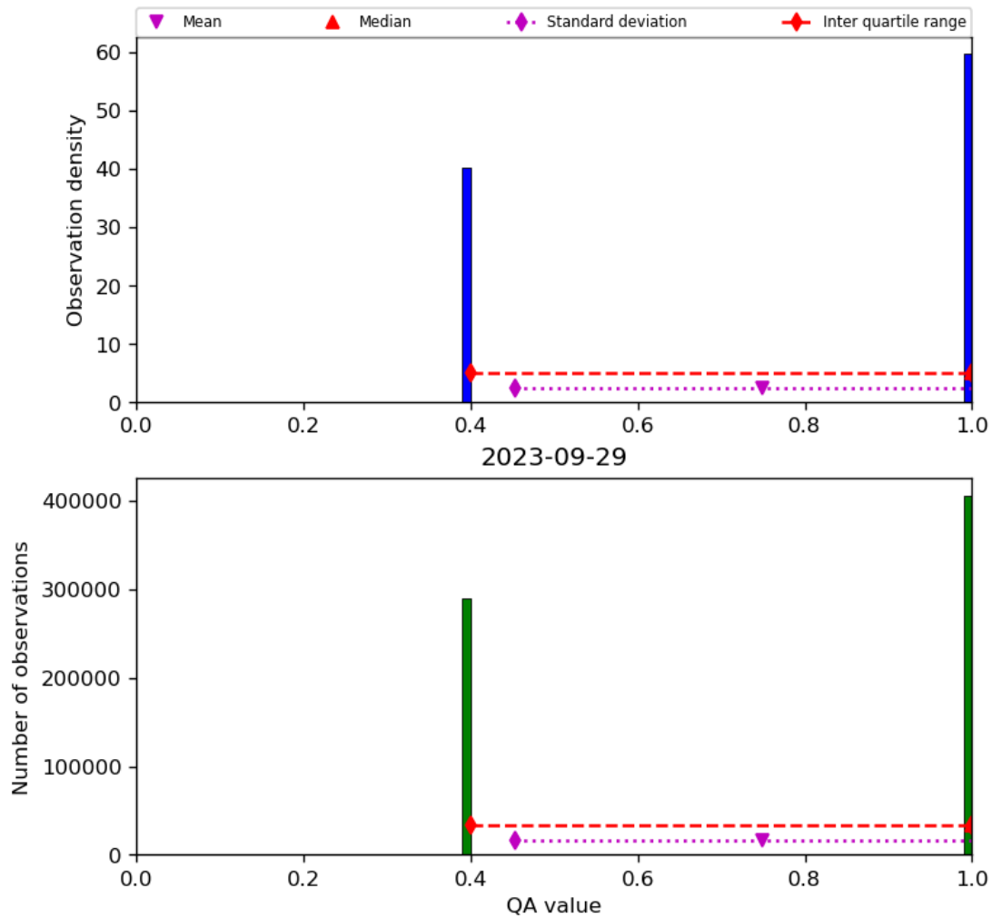
Figure 22: Histogram of “QA value” for 2023-09-28 to 2023-09-30
