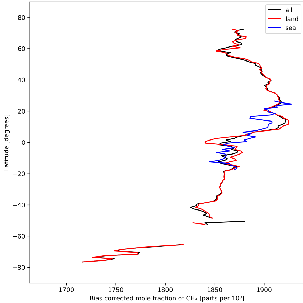
Figure 14: Zonal average of “Bias corrected mole fraction of CH 4 ” for 2023-09-28 to 2023-09-30.
