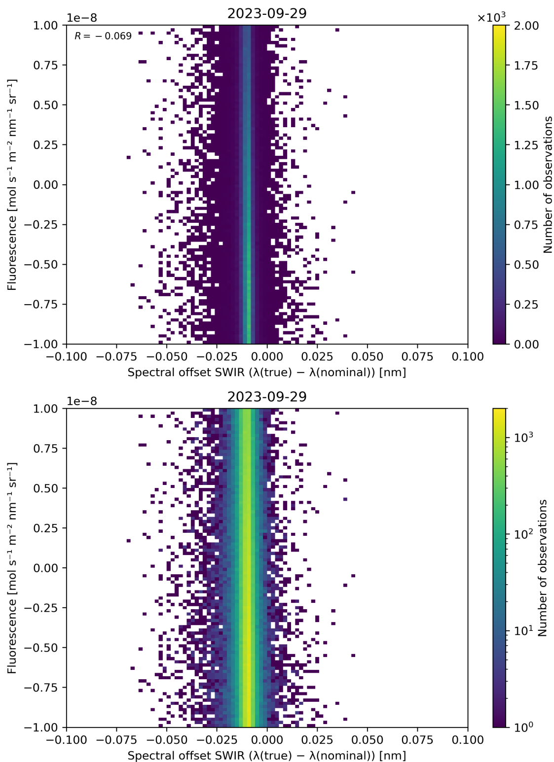
Figure 120: Scatter density plot of “Spectral offset SWIR ( \lambda(\text{true}) - \lambda(\text{nominal}) )” against “Fluorescence” for 2023-09-28 to 2023-09-30.
