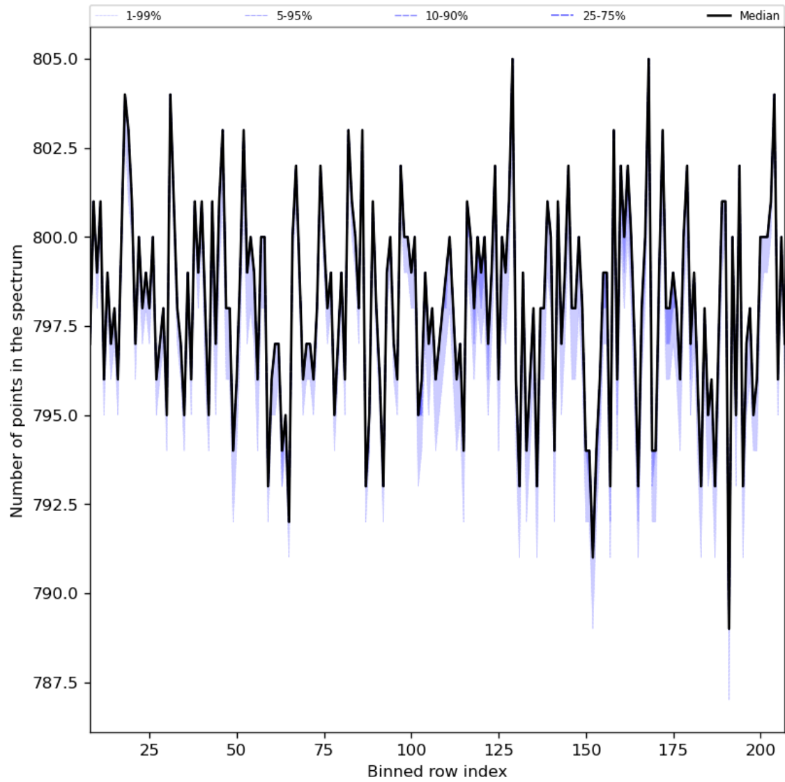
Figure 37: Along track statistics of “Number of points in the spectrum” for 2023-09-28 to 2023-09-30
