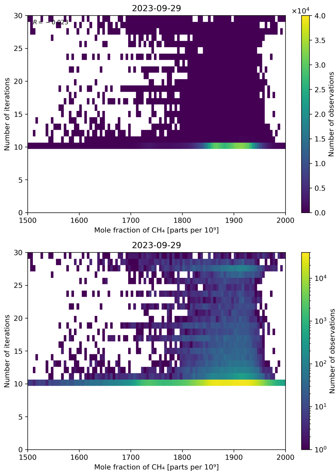
Figure 76: Scatter density plot of “Mole fraction of CH 4 ” against “Number of iterations” for 2023-09-28 to 2023-09-30.
