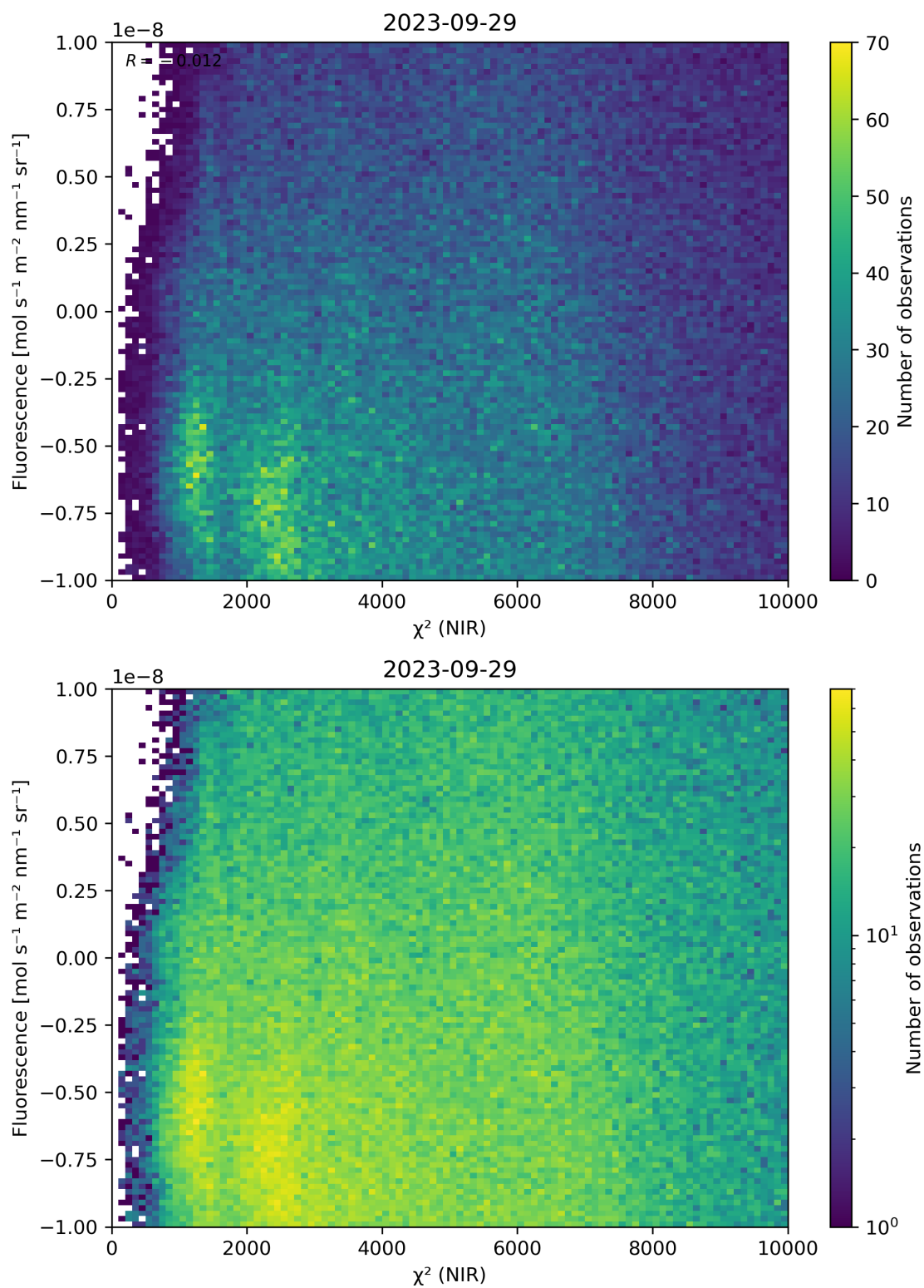
Figure 45: Scatter density plot of “ \chi^2 (NIR)” against “Fluorescence” for 2023-09-28 to 2023-09-30.
