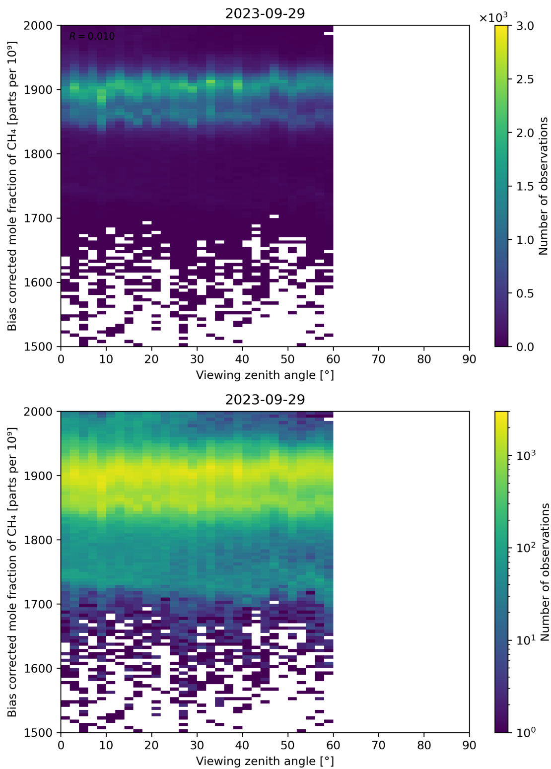
Figure 111: Scatter density plot of “Viewing zenith angle” against “Bias corrected mole fraction of CH 4 ” for 2023-09-28 to 2023-09-30.
