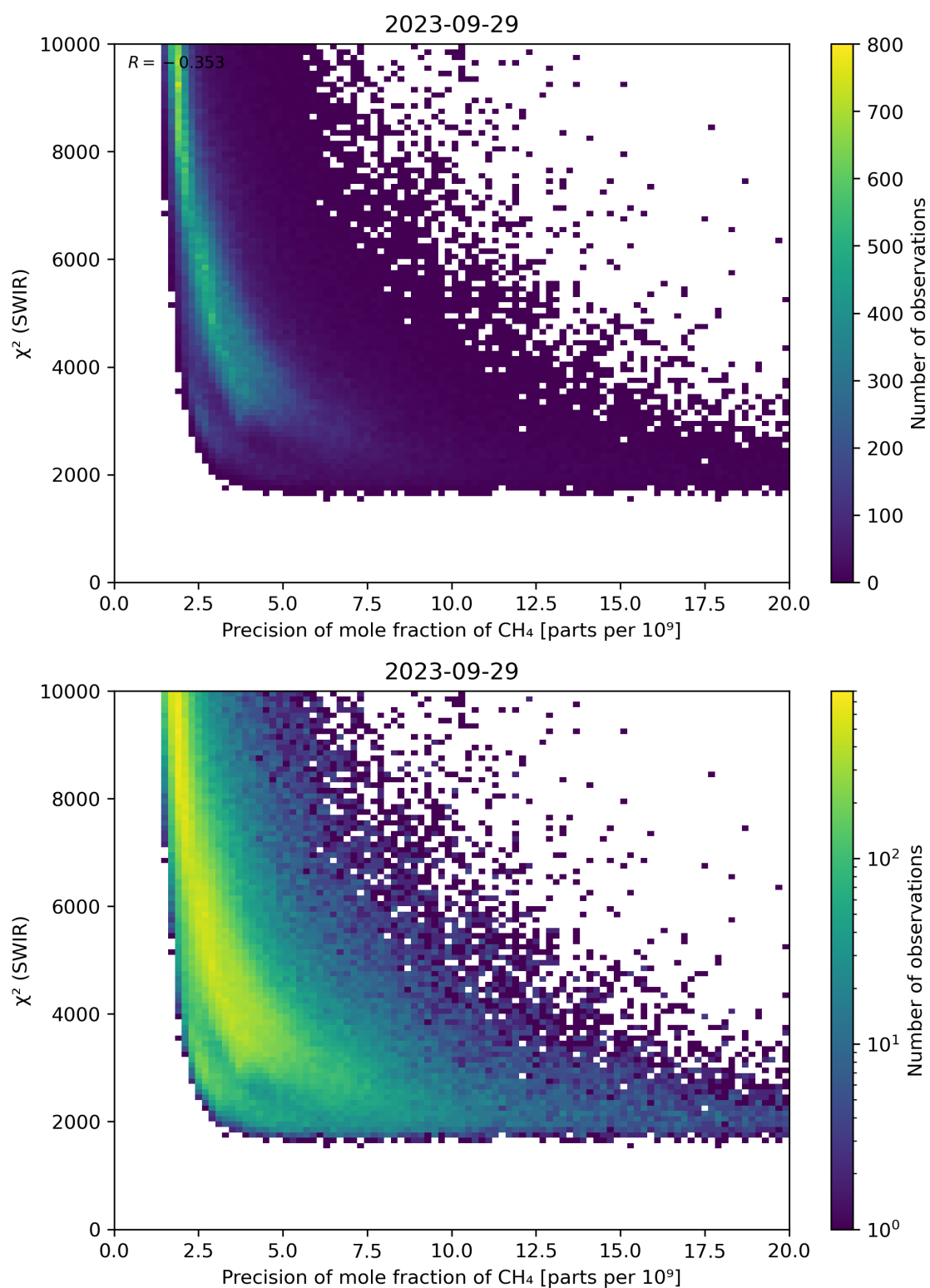
Figure 79: Scatter density plot of “Precision of mole fraction of CH 4 ” against “ \chi^2 (SWIR)” for 2023-09-28 to 2023-09-30.
