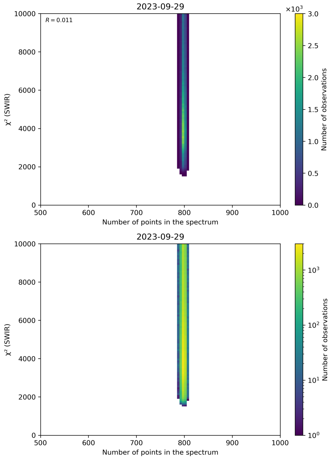
Figure 89: Scatter density plot of “Number of points in the spectrum” against “ \chi^2 (SWIR)” for 2023-09-28 to 2023-09-30.
