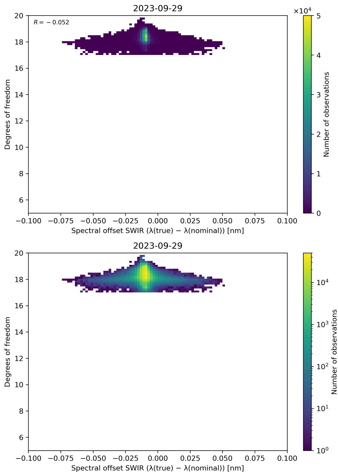
Figure 119: Scatter density plot of “Spectral offset SWIR ( \lambda(\text{true}) - \lambda(\text{nominal}) )” against “Degrees of freedom” for 2023-09-28 to 2023-09-30.
