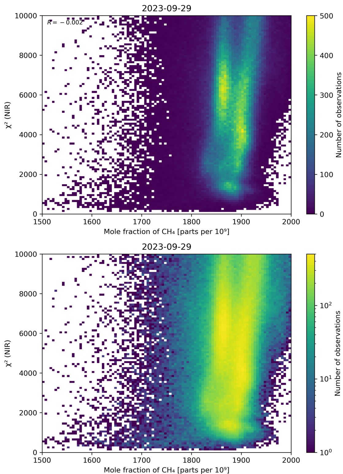
Figure 70: Scatter density plot of “Mole fraction of CH 4 ” against “ \chi^2 (NIR)” for 2023-09-28 to 2023-09-30.
