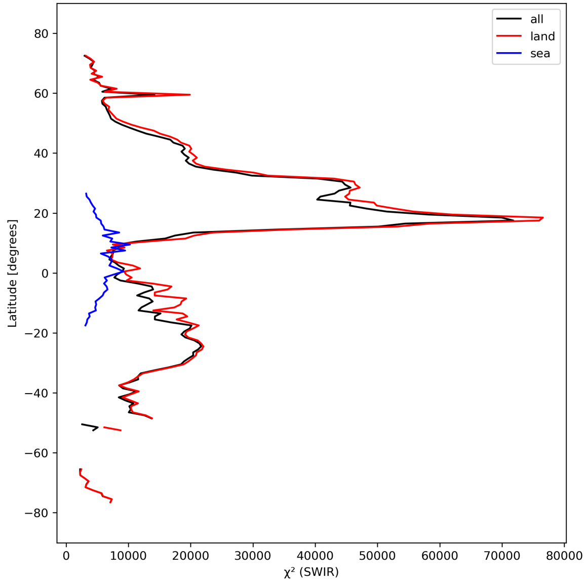
Figure 17: Zonal average of “ \chi^2 (SWIR)” for 2023-09-28 to 2023-09-30.
