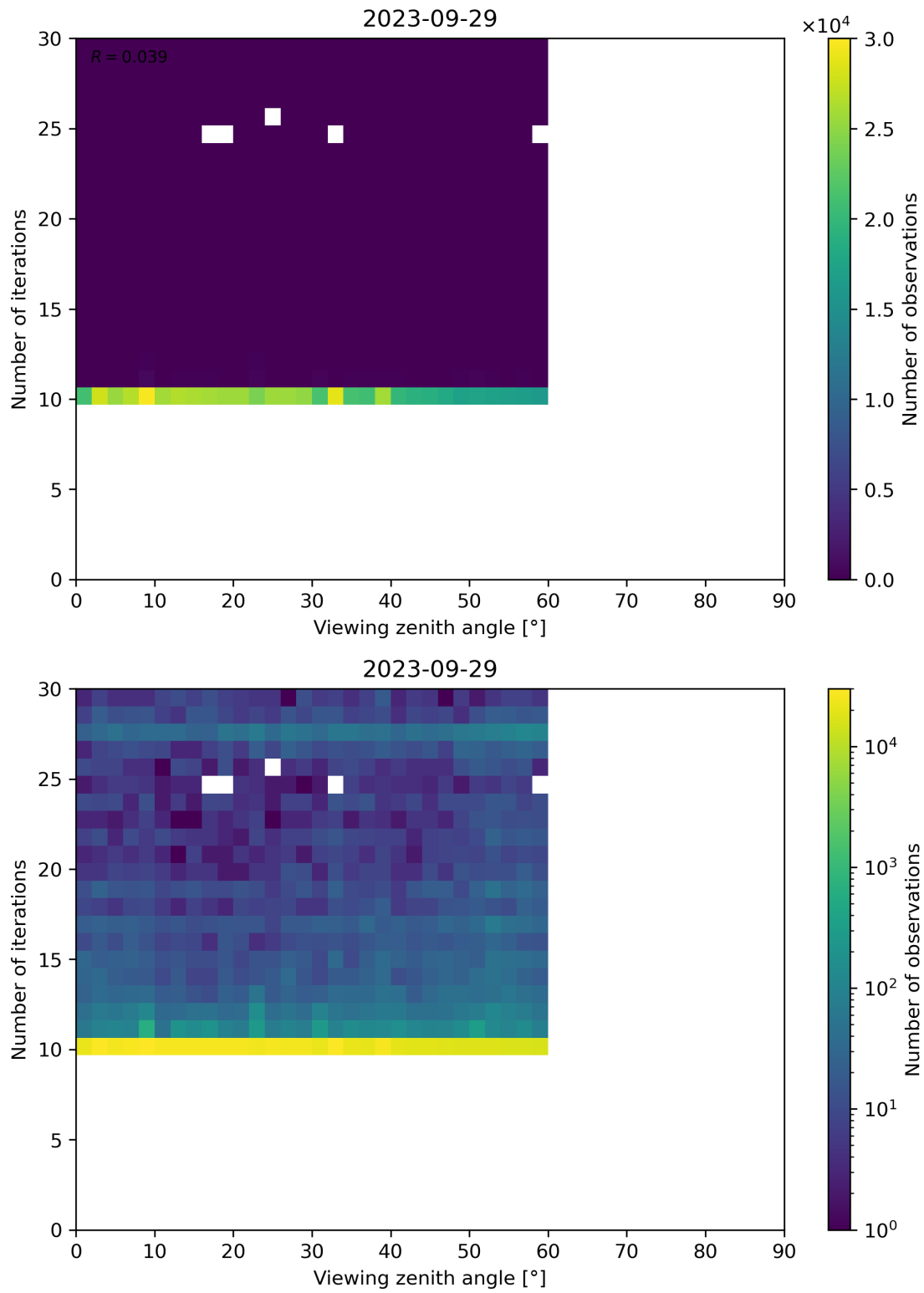
Figure 113: Scatter density plot of “Viewing zenith angle” against “Number of iterations” for 2023-09-28 to 2023-09-30.
