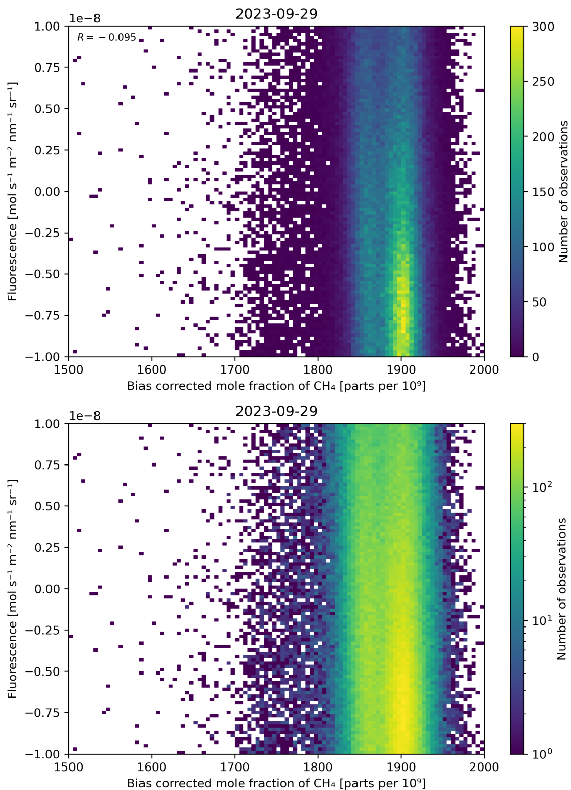
Figure 66: Scatter density plot of “Bias corrected mole fraction of \text{CH}_4 ” against “Fluorescence” for 2023-09-28 to 2023-09-30.
