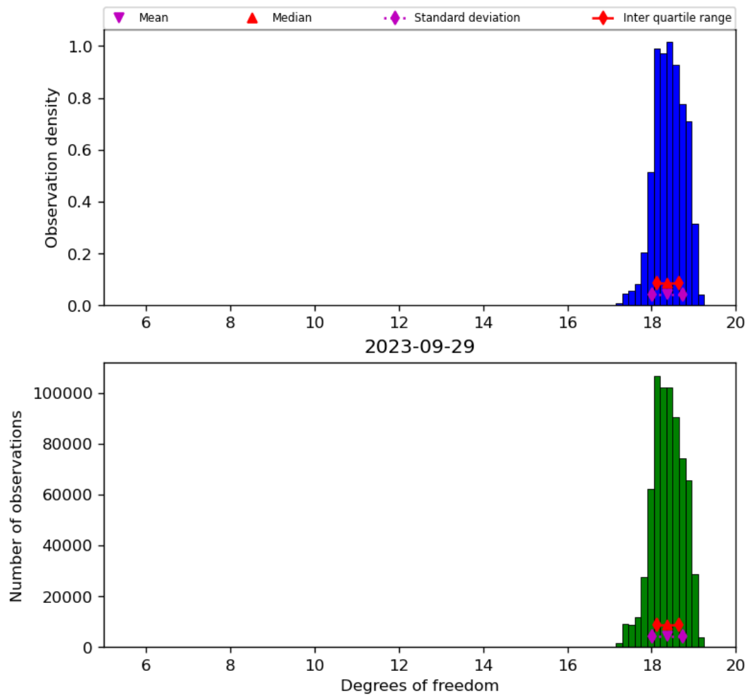
Figure 30: Histogram of “Degrees of freedom” for 2023-09-28 to 2023-09-30
