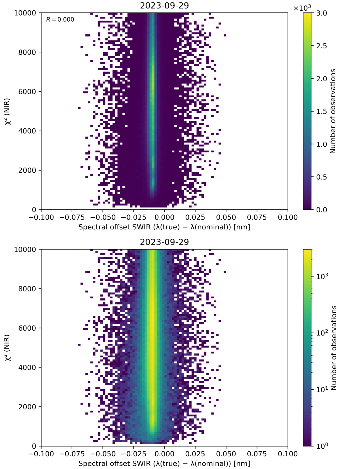
Figure 117: Scatter density plot of “Spectral offset SWIR ( \lambda(\text{true}) - \lambda(\text{nominal}) )” against “ \chi^2 (NIR)” for 2023-09-28 to 2023-09-30.
