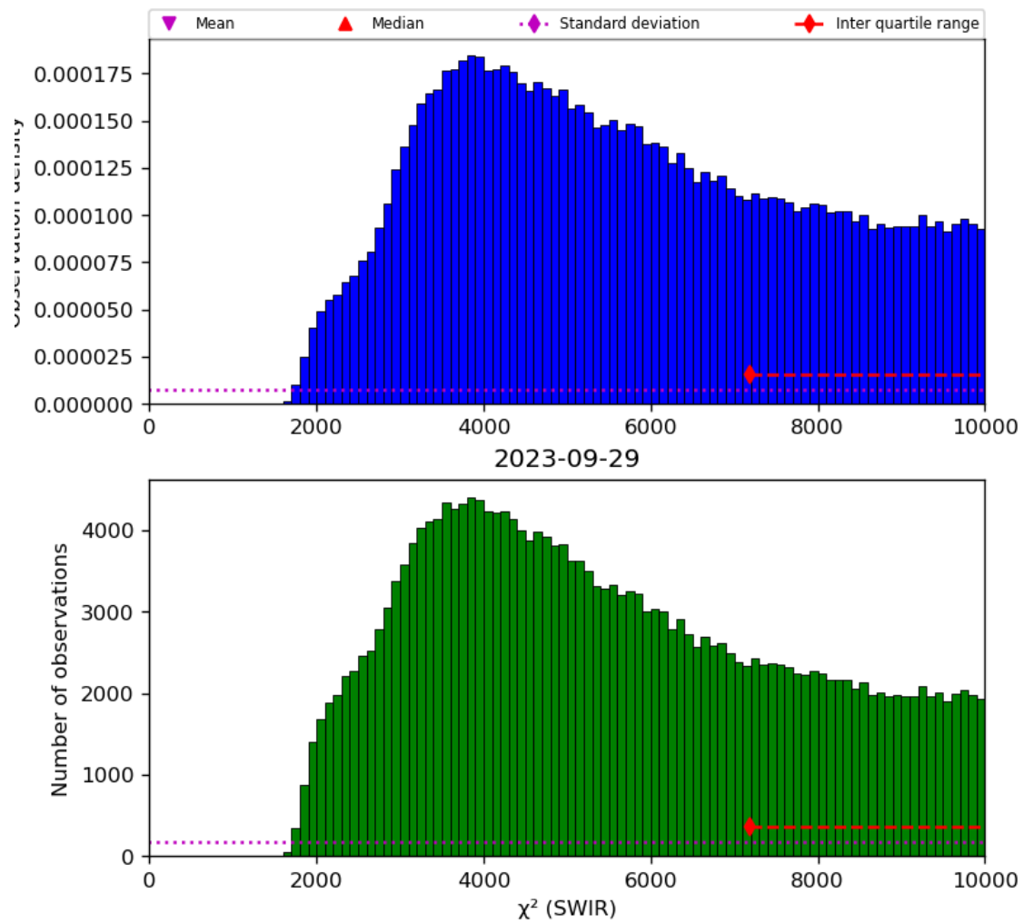
Figure 28: Histogram of “ \chi^2 (SWIR)” for 2023-09-28 to 2023-09-30
