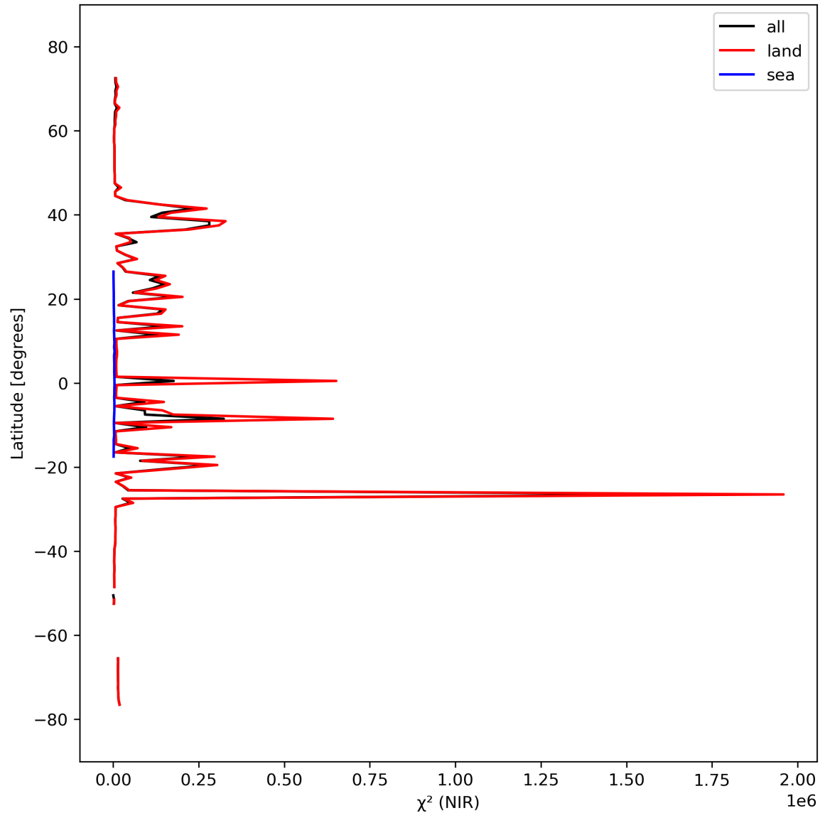
Figure 18: Zonal average of “ \chi^2 (NIR)” for 2023-09-28 to 2023-09-30.
