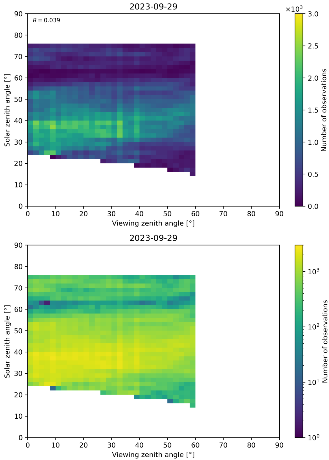
Figure 115: Scatter density plot of “Viewing zenith angle” against “Solar zenith angle” for 2023-09-28 to 2023-09-30.
