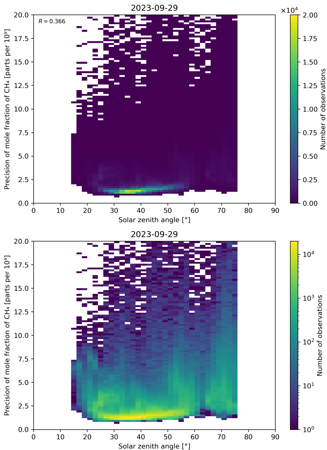
Figure 101: Scatter density plot of “Solar zenith angle” against “Precision of mole fraction of CH 4 ” for 2023-09-28 to 2023-09-30.
