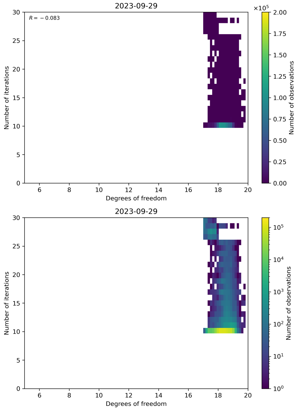
Figure 52: Scatter density plot of “Degrees of freedom” against “Number of iterations” for 2023-09-28 to 2023-09-30.
