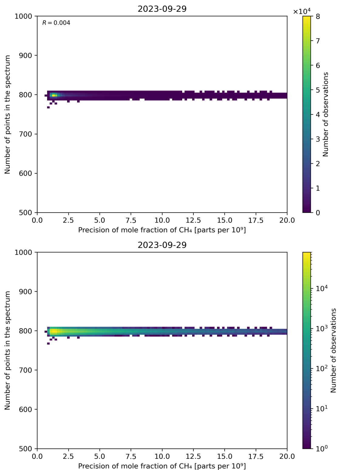
Figure 84: Scatter density plot of “Precision of mole fraction of CH 4 ” against “Number of points in the spectrum” for 2023-09-28 to 2023-09-30.
