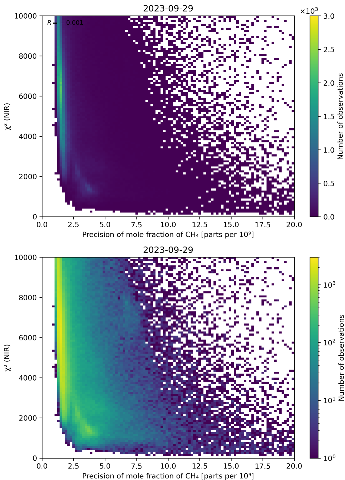
Figure 78: Scatter density plot of “Precision of mole fraction of CH 4 ” against “ \chi^2 (NIR)” for 2023-09-28 to 2023-09-30.
