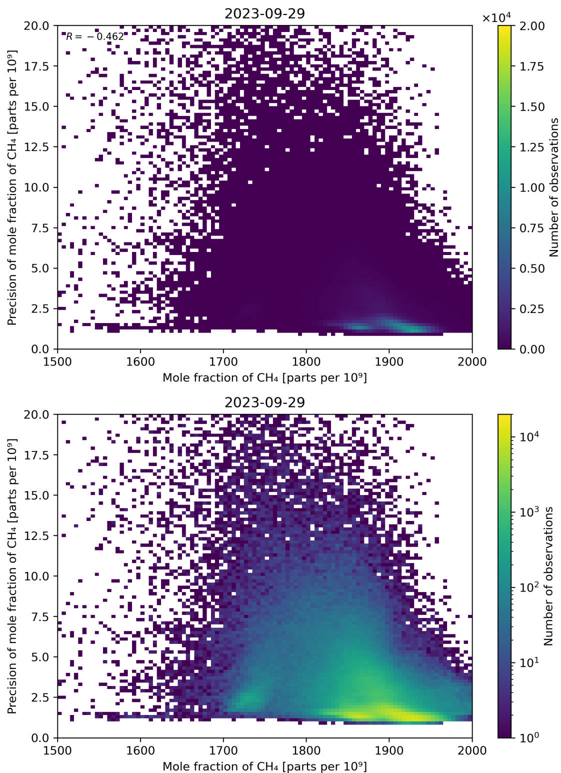
Figure 75: Scatter density plot of “Mole fraction of CH 4 ” against “Precision of mole fraction of CH 4 ” for 2023-09-28 to 2023-09-30.
