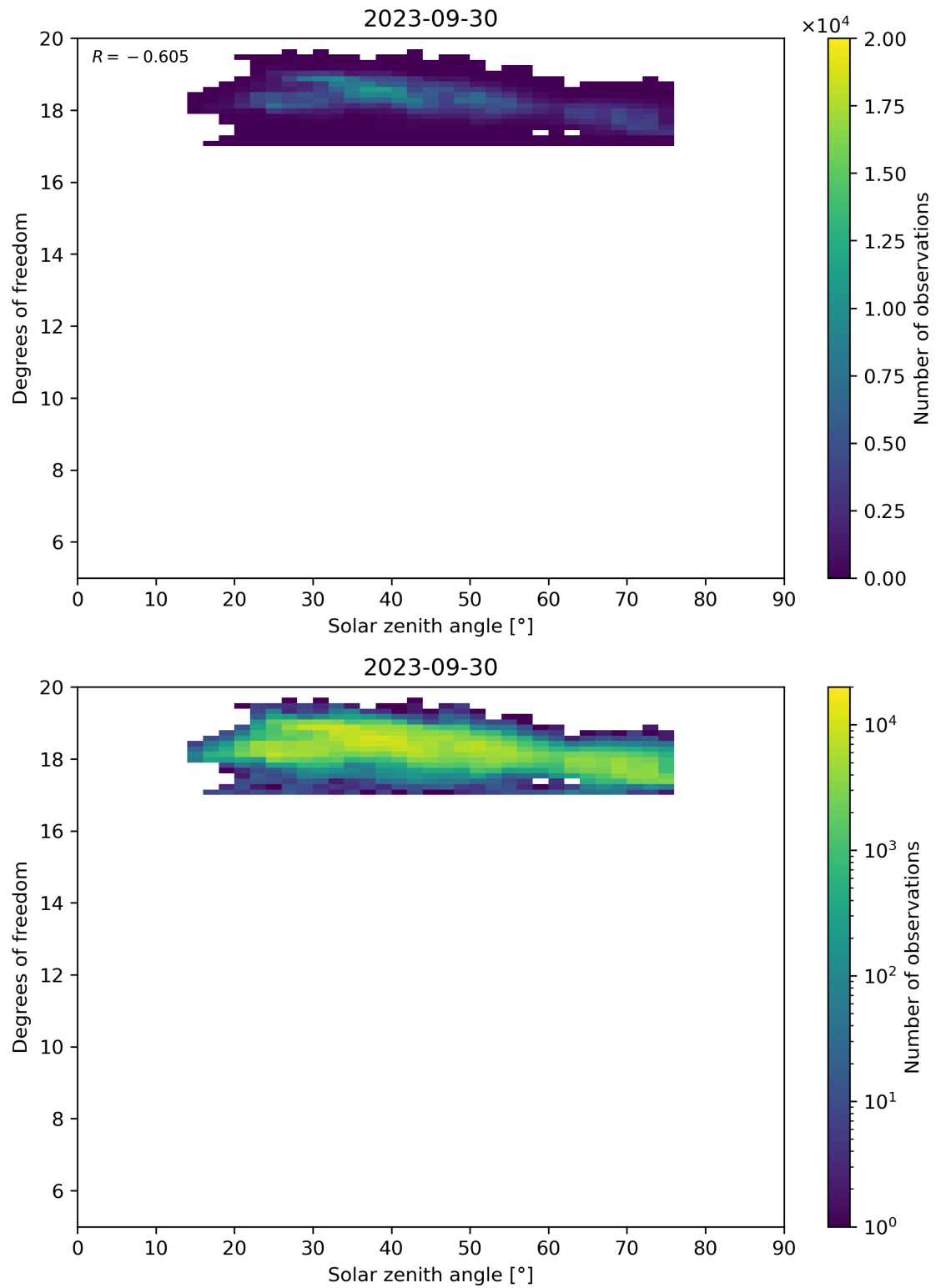
Figure 96: Scatter density plot of “Solar zenith angle” against “Degrees of freedom” for 2023-09-29 to 2023-10-01.
