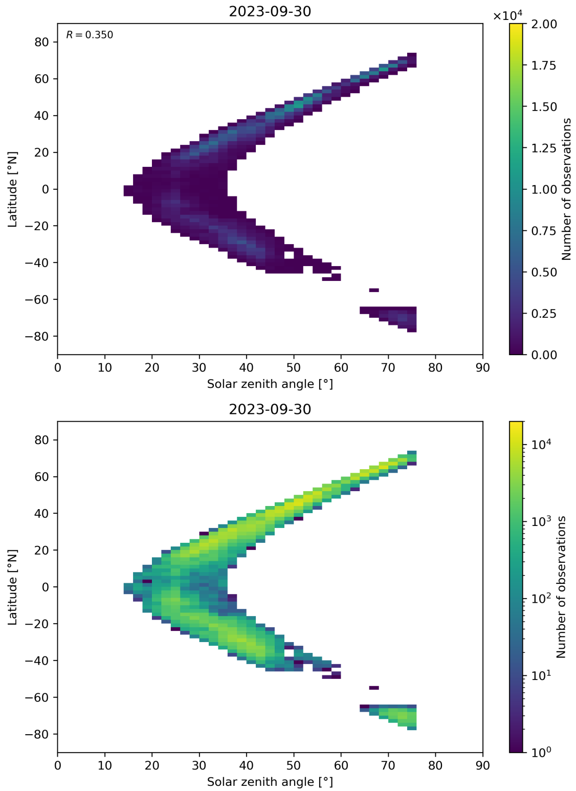
Figure 98: Scatter density plot of “Solar zenith angle” against “Latitude” for 2023-09-29 to 2023-10-01.
