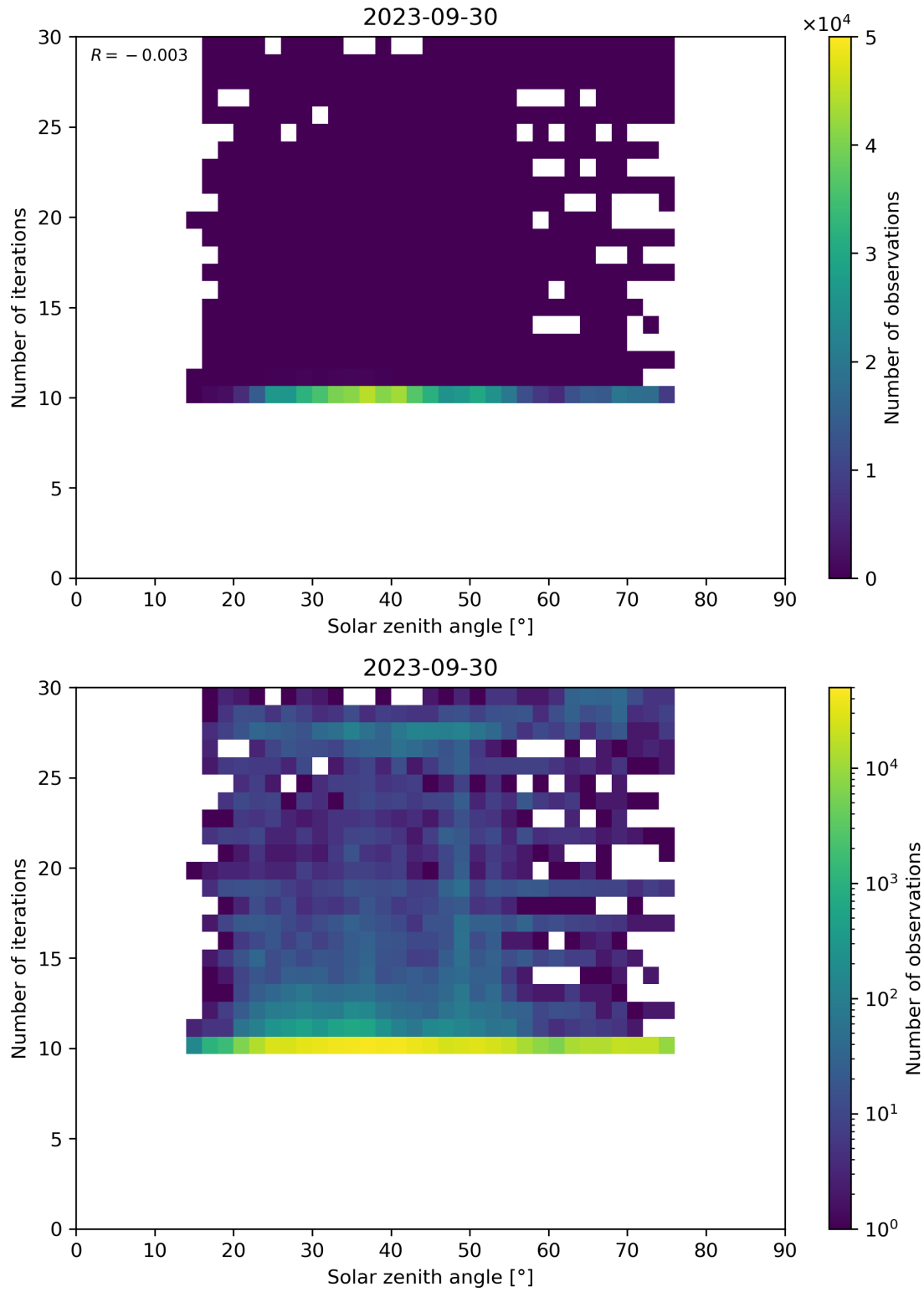
Figure 102: Scatter density plot of “Solar zenith angle” against “Number of iterations” for 2023-09-29 to 2023-10-01.
