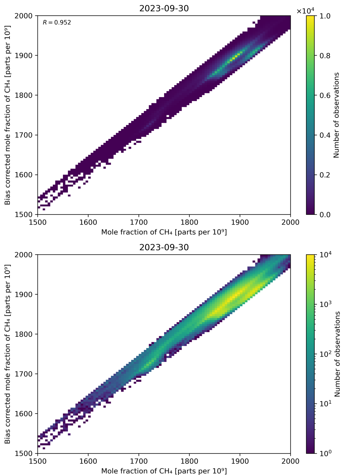
Figure 74: Scatter density plot of “Mole fraction of CH 4 ” against “Bias corrected mole fraction of CH 4 ” for 2023-09-29 to 2023-10-01.
