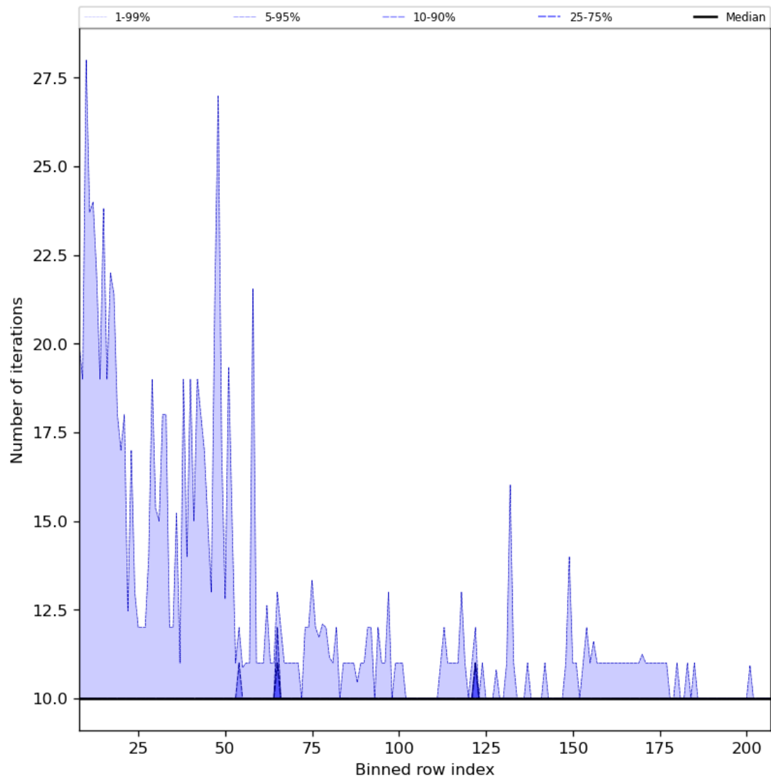
Figure 42: Along track statistics of “Number of iterations” for 2023-09-29 to 2023-10-01
