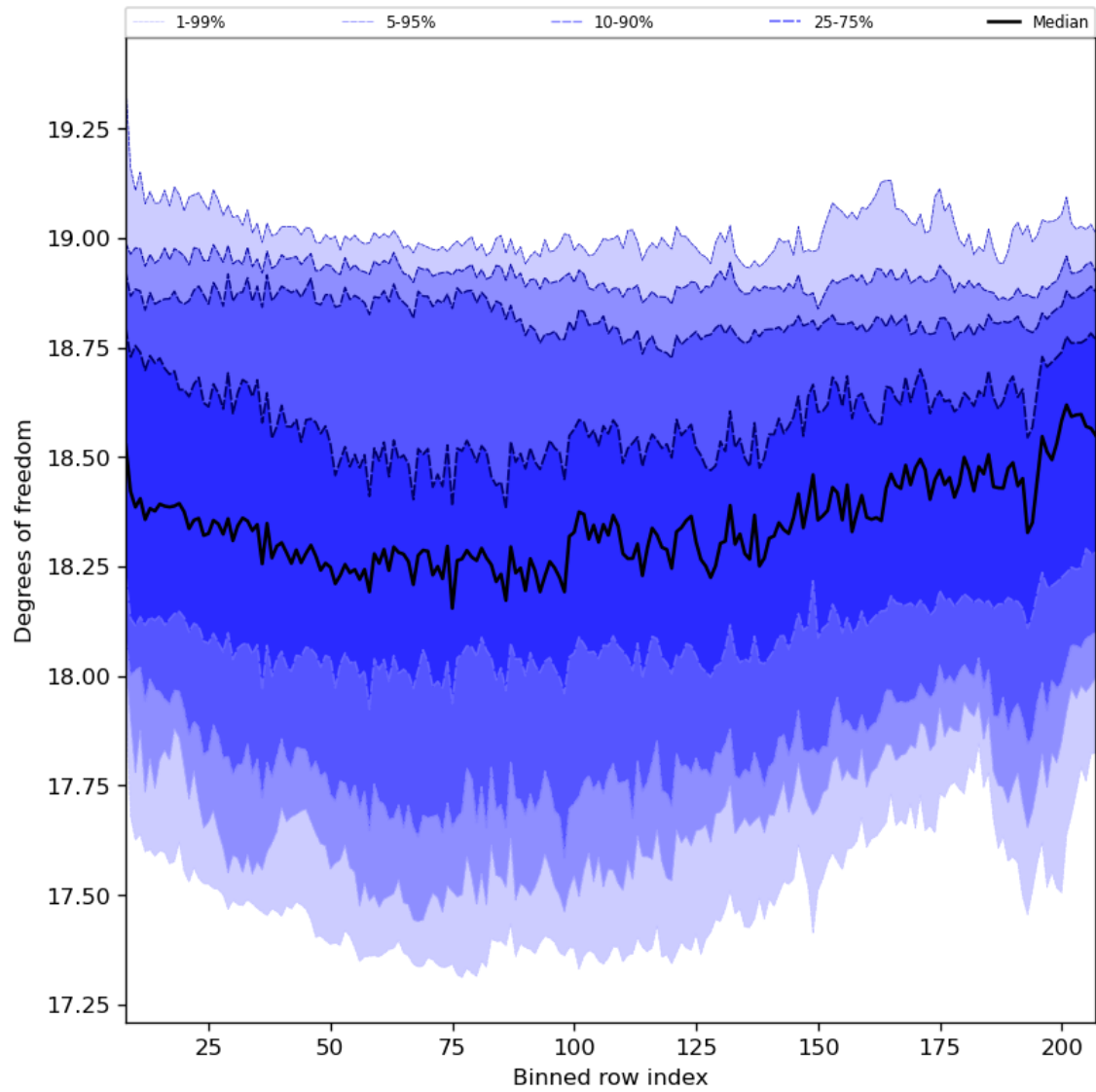
Figure 41: Along track statistics of “Degrees of freedom” for 2023-09-29 to 2023-10-01
