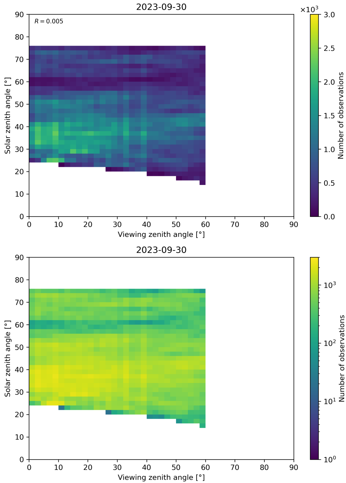
Figure 115: Scatter density plot of “Viewing zenith angle” against “Solar zenith angle” for 2023-09-29 to 2023-10-01.
