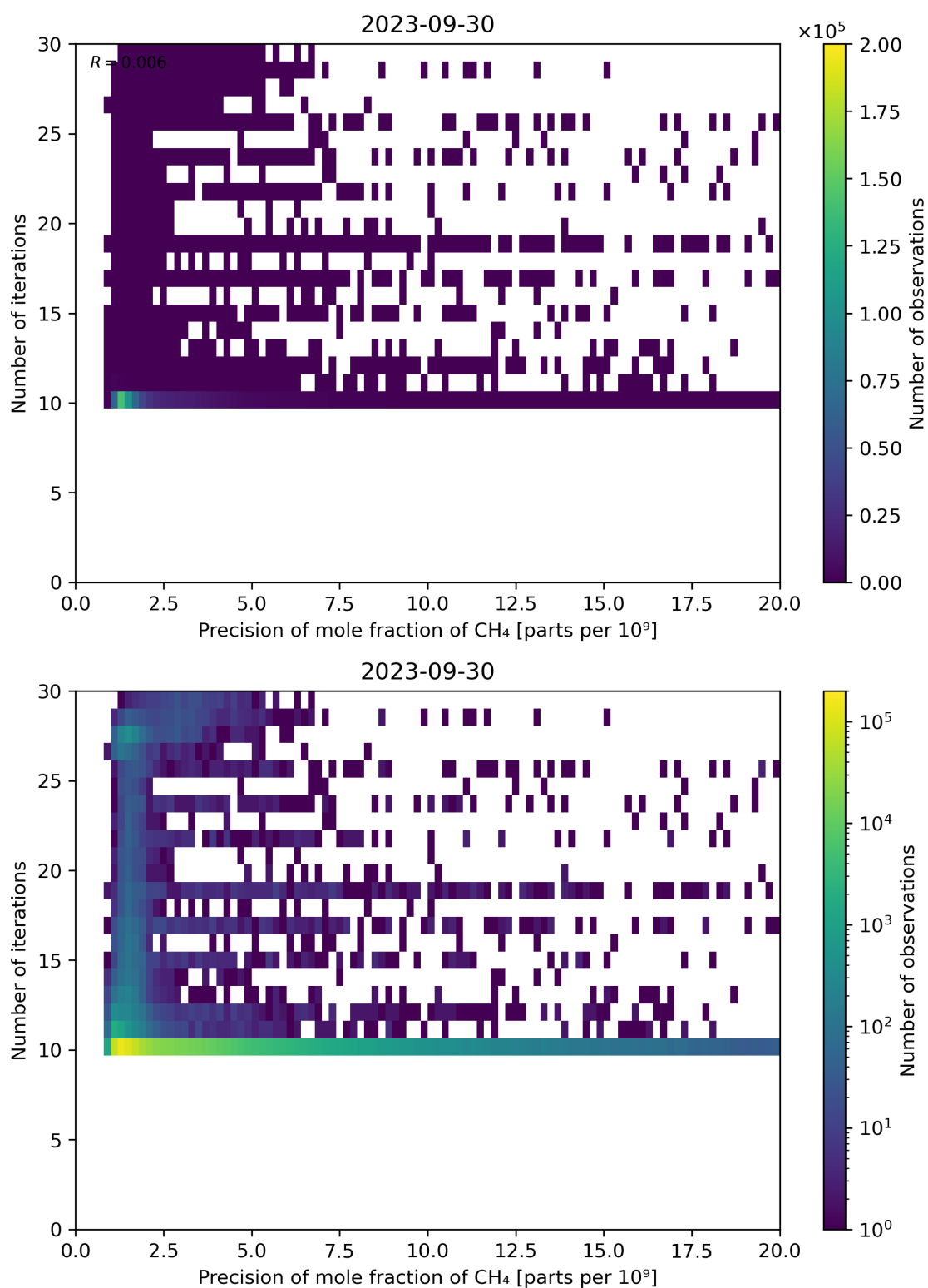
Figure 83: Scatter density plot of “Precision of mole fraction of CH 4 ” against “Number of iterations” for 2023-09-29 to 2023-10-01.
