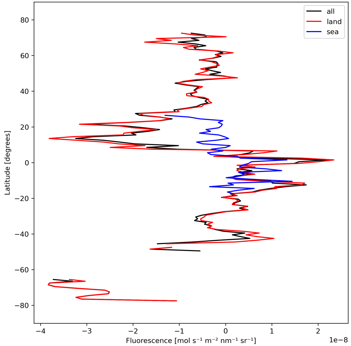
Figure 21: Zonal average of “Fluorescence” for 2023-09-29 to 2023-10-01.
