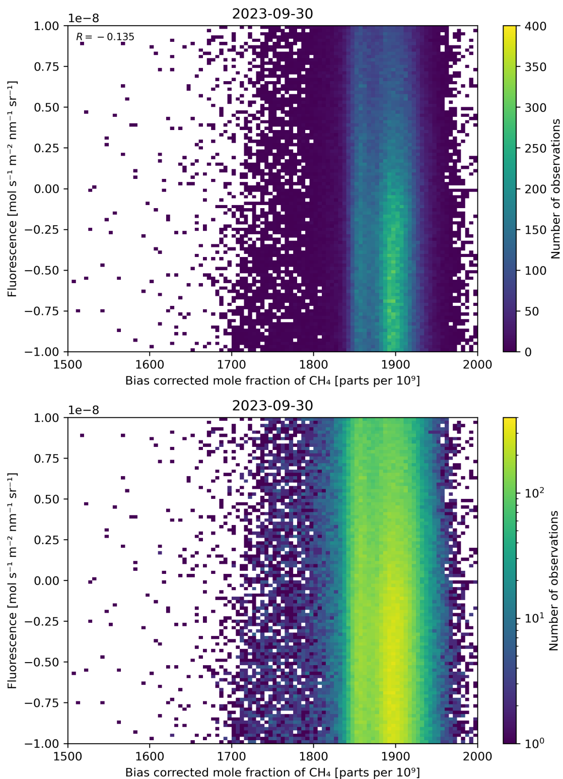
Figure 66: Scatter density plot of “Bias corrected mole fraction of \text{CH}_4 ” against “Fluorescence” for 2023-09-29 to 2023-10-01.
