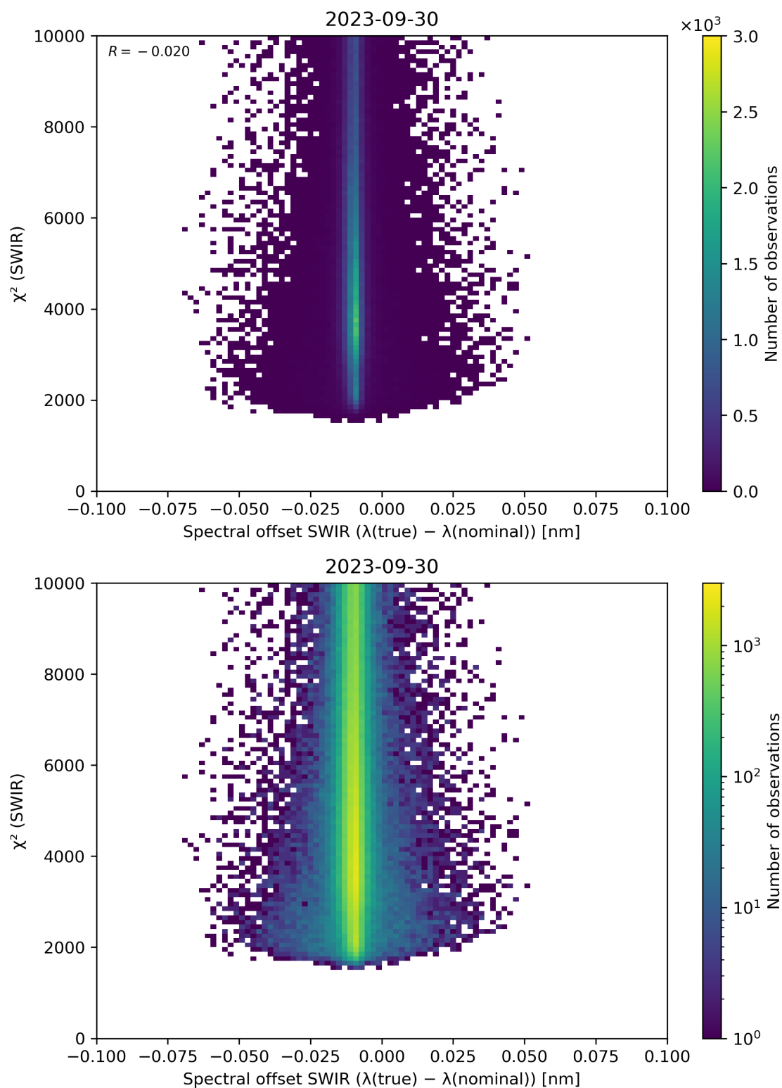
Figure 118: Scatter density plot of “Spectral offset SWIR ( \lambda(\text{true}) - \lambda(\text{nominal}) )” against “ \chi^2 (SWIR)” for 2023-09-29 to 2023-10-01.
