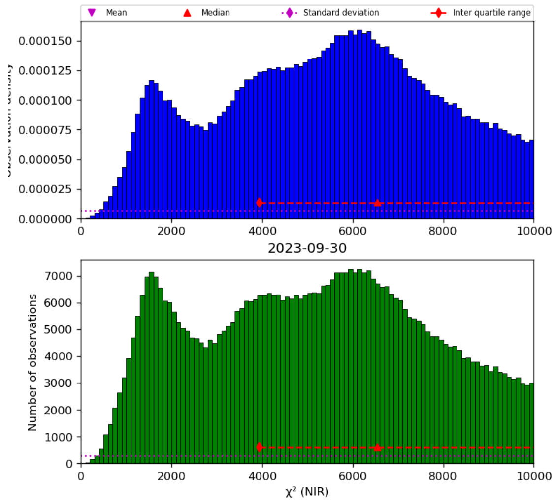
Figure 29: Histogram of “ \chi^2 (NIR)” for 2023-09-29 to 2023-10-01
