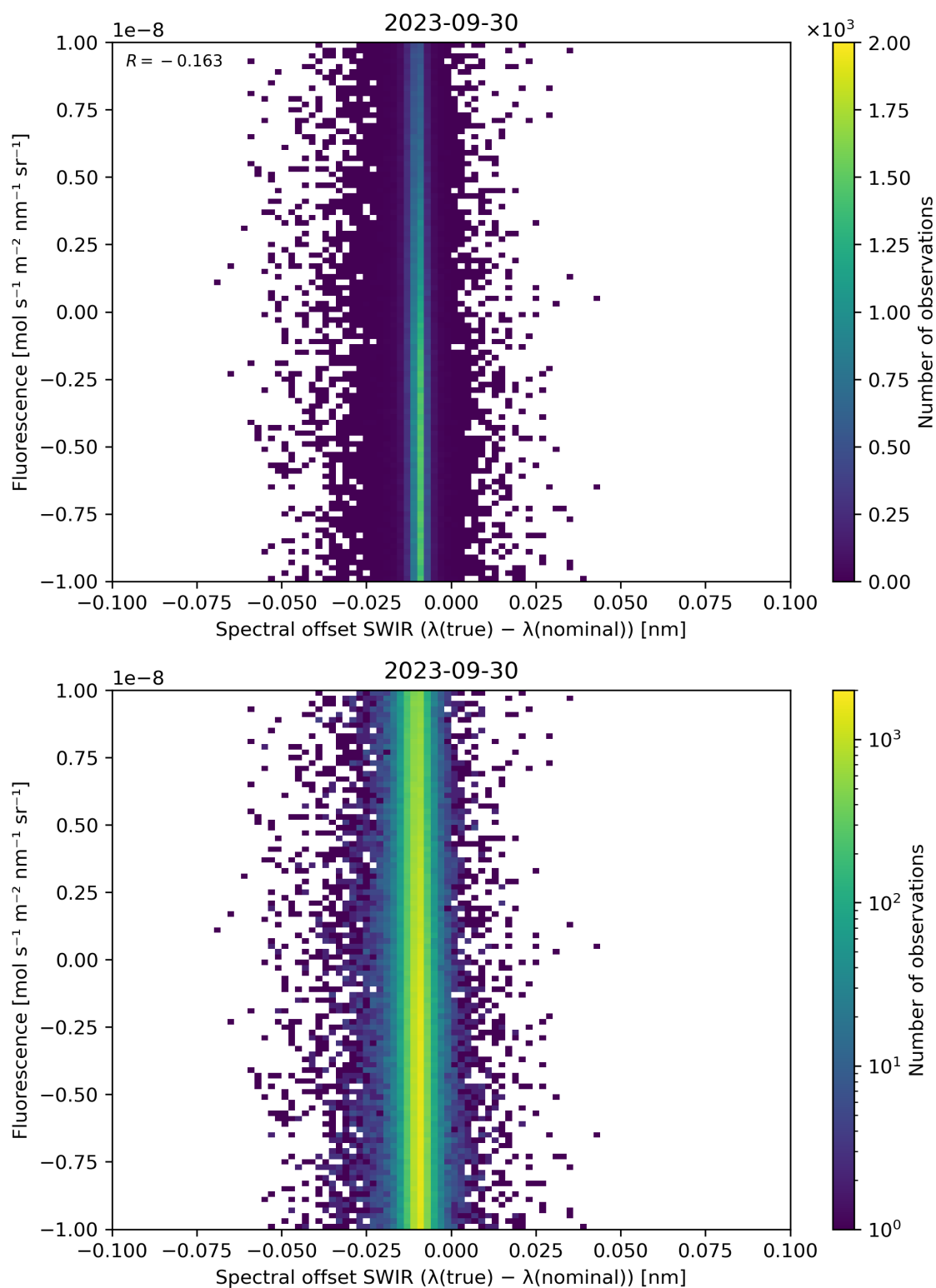
Figure 120: Scatter density plot of “Spectral offset SWIR ( \lambda(\text{true}) - \lambda(\text{nominal}) )” against “Fluorescence” for 2023-09-29 to 2023-10-01.
