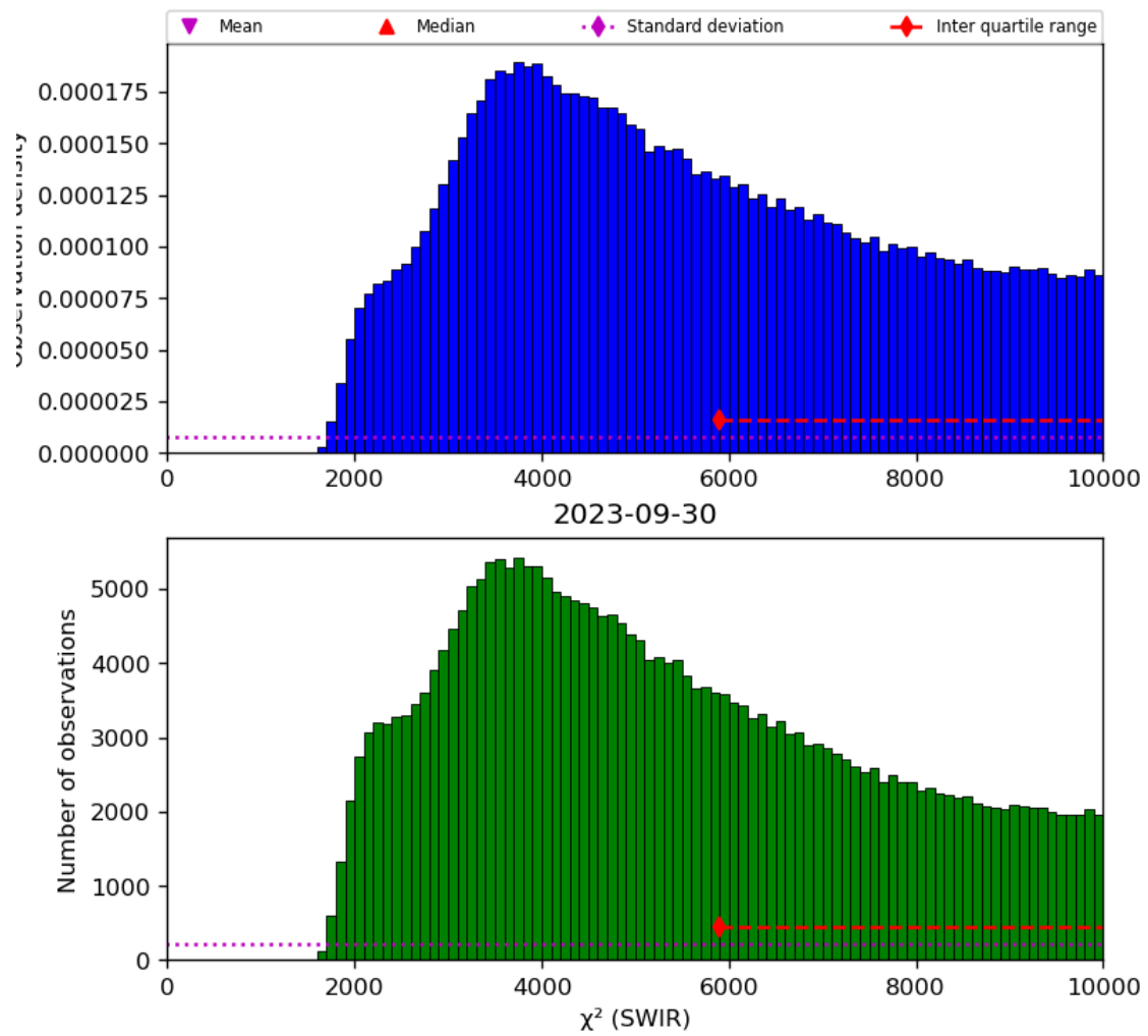
Figure 28: Histogram of “ \chi^2 (SWIR)” for 2023-09-29 to 2023-10-01
