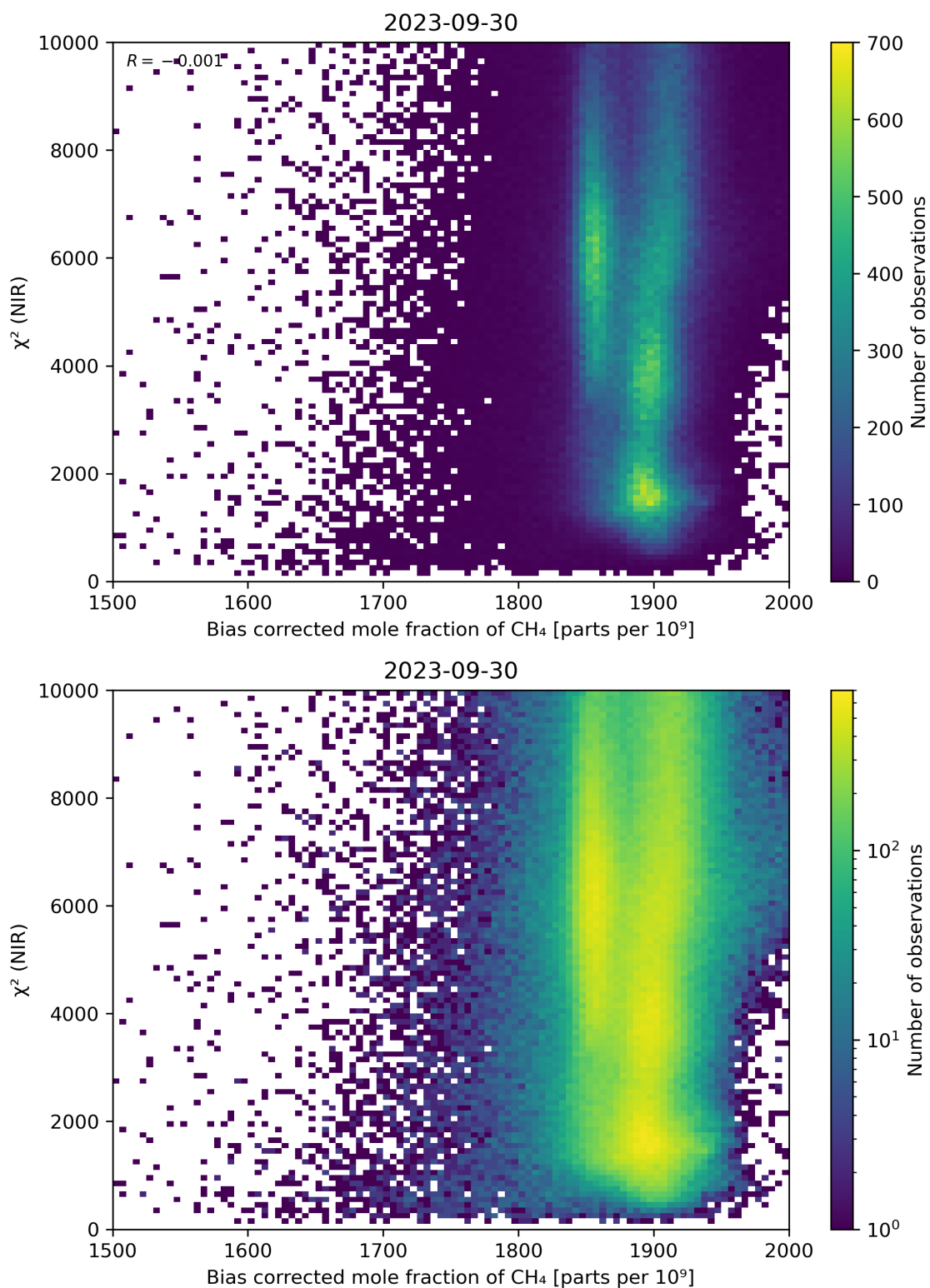
Figure 63: Scatter density plot of “Bias corrected mole fraction of CH 4 ” against “ \chi^2 (NIR)” for 2023-09-29 to 2023-10-01.
