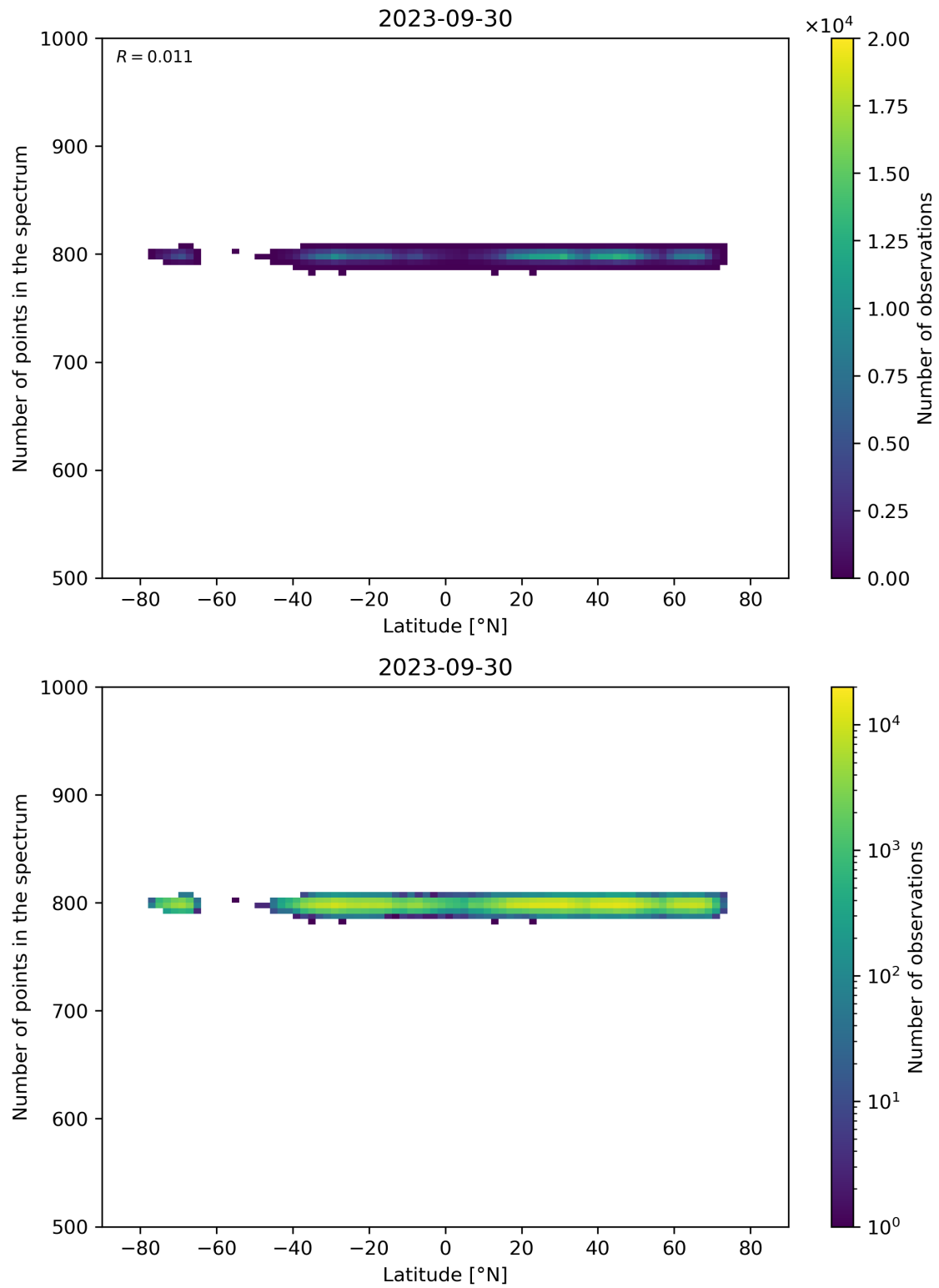
Figure 61: Scatter density plot of “Latitude” against “Number of points in the spectrum” for 2023-09-29 to 2023-10-01.
