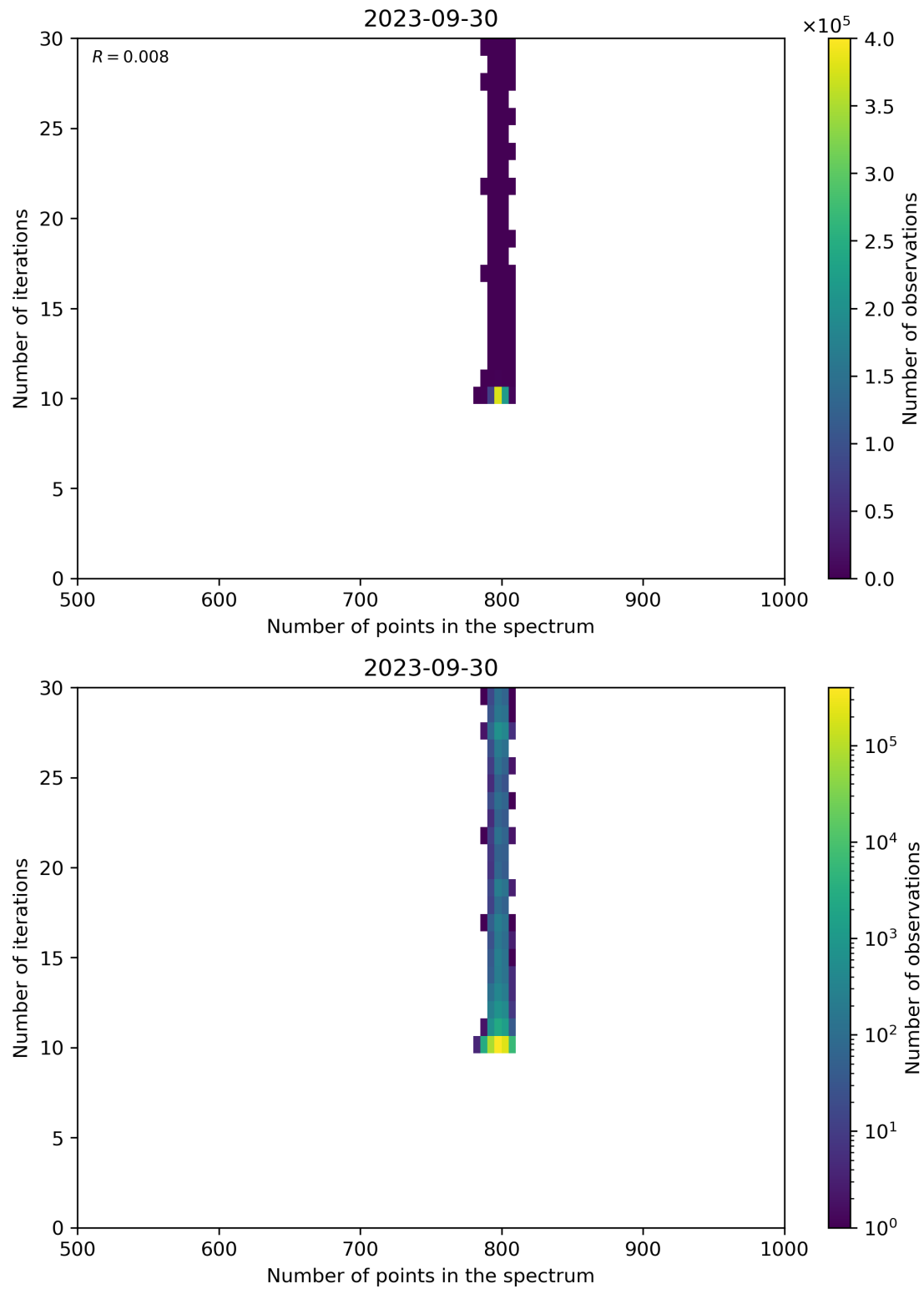
Figure 92: Scatter density plot of “Number of points in the spectrum” against “Number of iterations” for 2023-09-29 to 2023-10-01.
