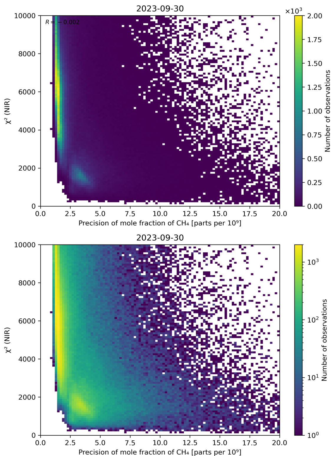
Figure 78: Scatter density plot of “Precision of mole fraction of CH 4 ” against “ \chi^2 (NIR)” for 2023-09-29 to 2023-10-01.
