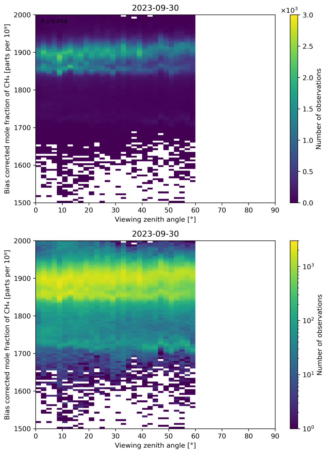
Figure 111: Scatter density plot of “Viewing zenith angle” against “Bias corrected mole fraction of CH 4 ” for 2023-09-29 to 2023-10-01.
