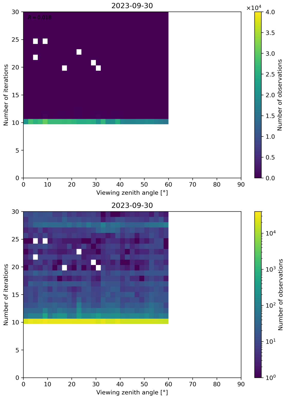
Figure 113: Scatter density plot of “Viewing zenith angle” against “Number of iterations” for 2023-09-29 to 2023-10-01.
