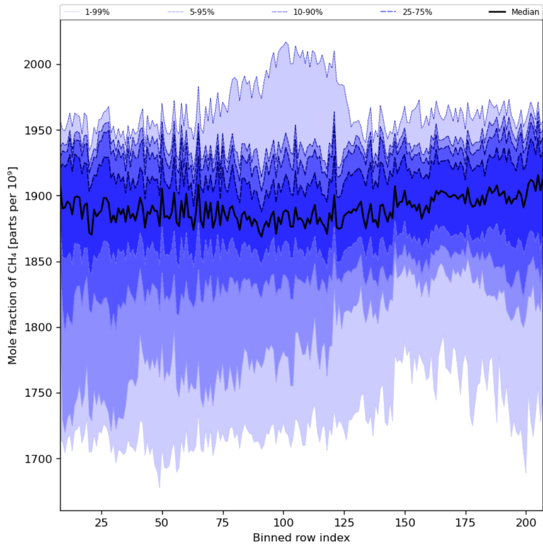
Figure 34: Along track statistics of “Mole fraction of CH 4 ” for 2023-09-29 to 2023-10-01
