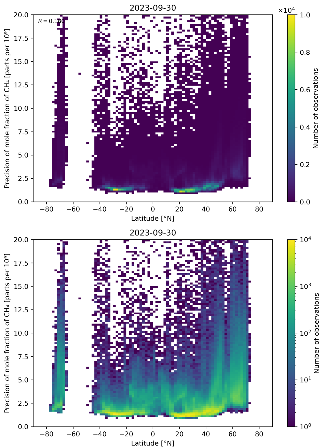
Figure 59: Scatter density plot of “Latitude” against “Precision of mole fraction of \text{CH}_4 ” for 2023-09-29 to 2023-10-01.
