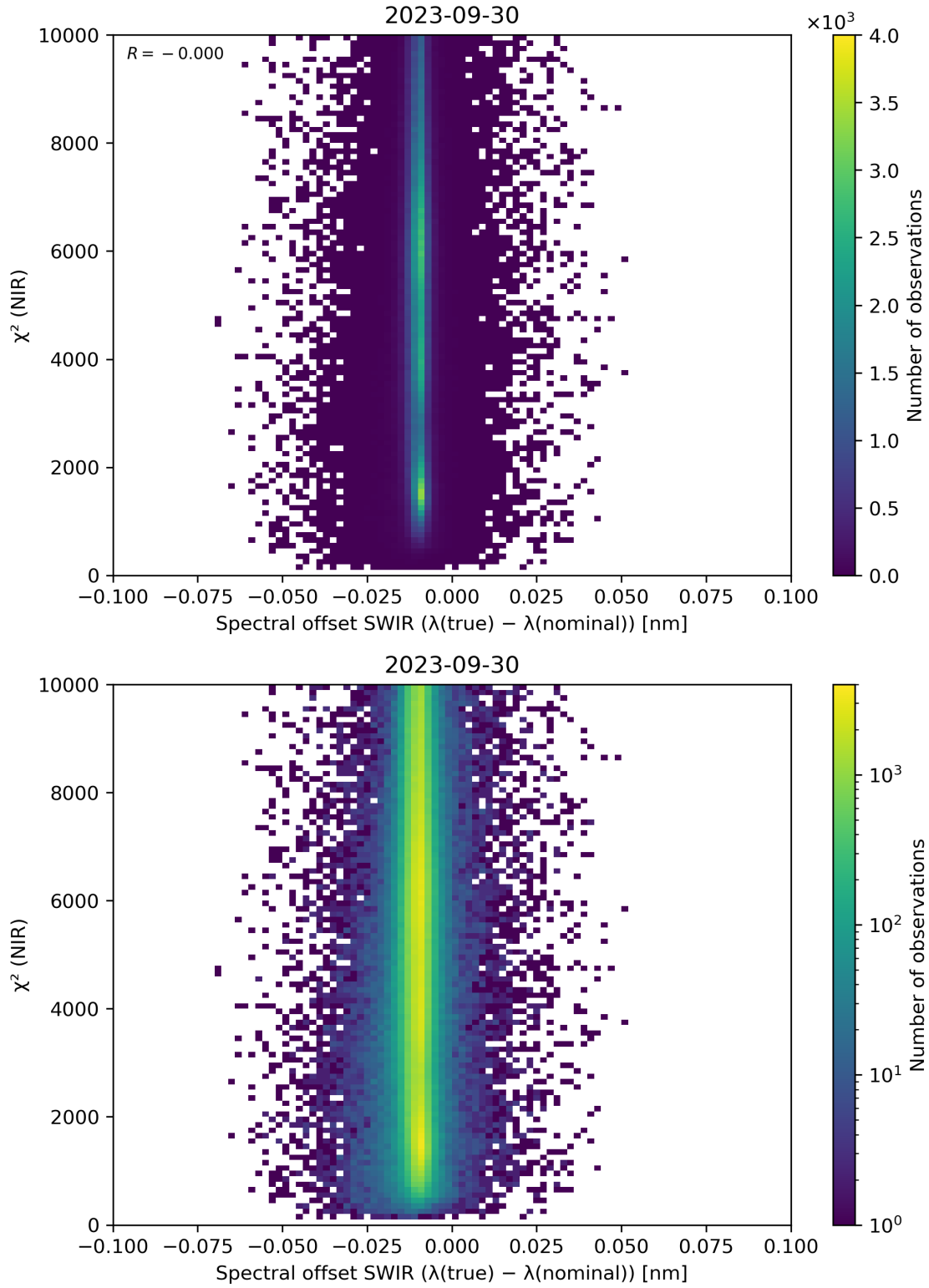
Figure 117: Scatter density plot of “Spectral offset SWIR ( \lambda(\text{true}) - \lambda(\text{nominal}) )” against “ \chi^2 (NIR)” for 2023-09-29 to 2023-10-01.
