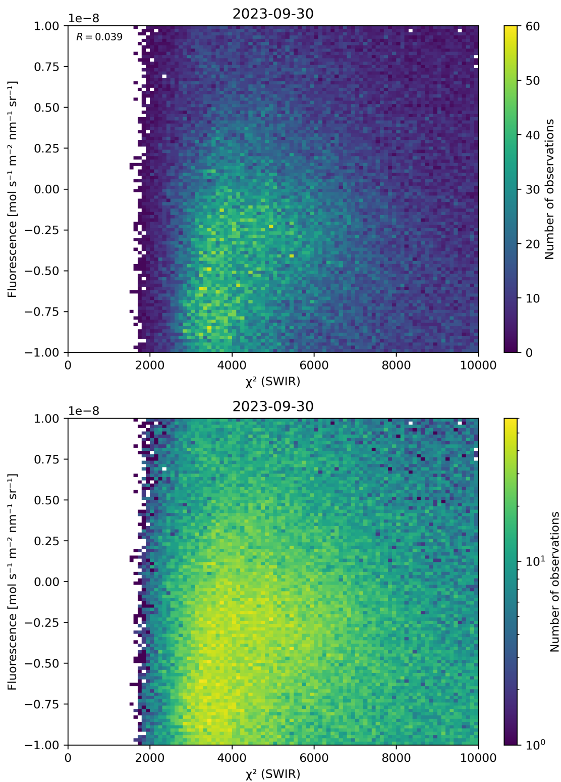
Figure 49: Scatter density plot of “ \chi^2 (SWIR)” against “Fluorescence” for 2023-09-29 to 2023-10-01.
