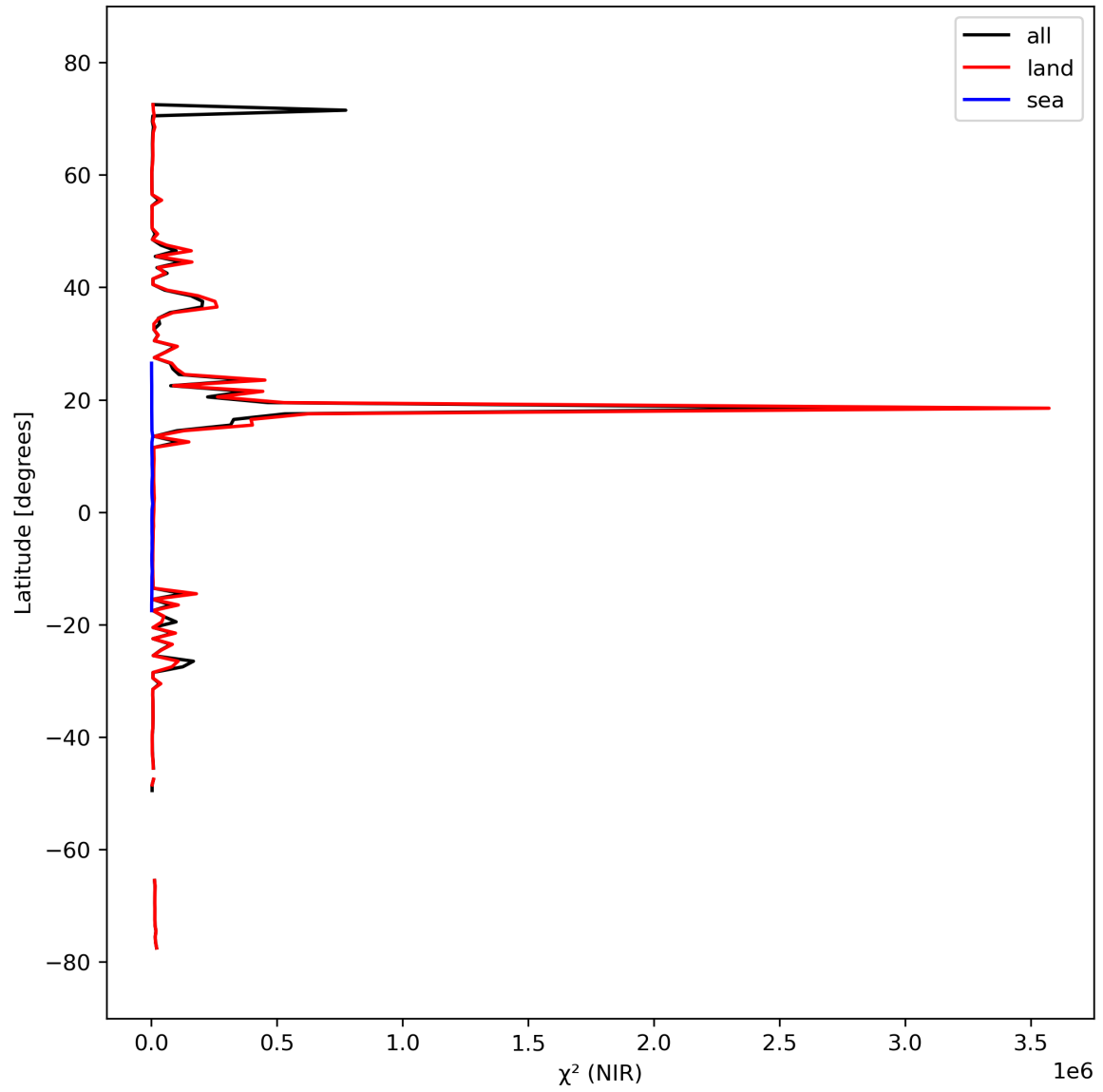
Figure 18: Zonal average of “ \chi^2 (NIR)” for 2023-09-29 to 2023-10-01.
