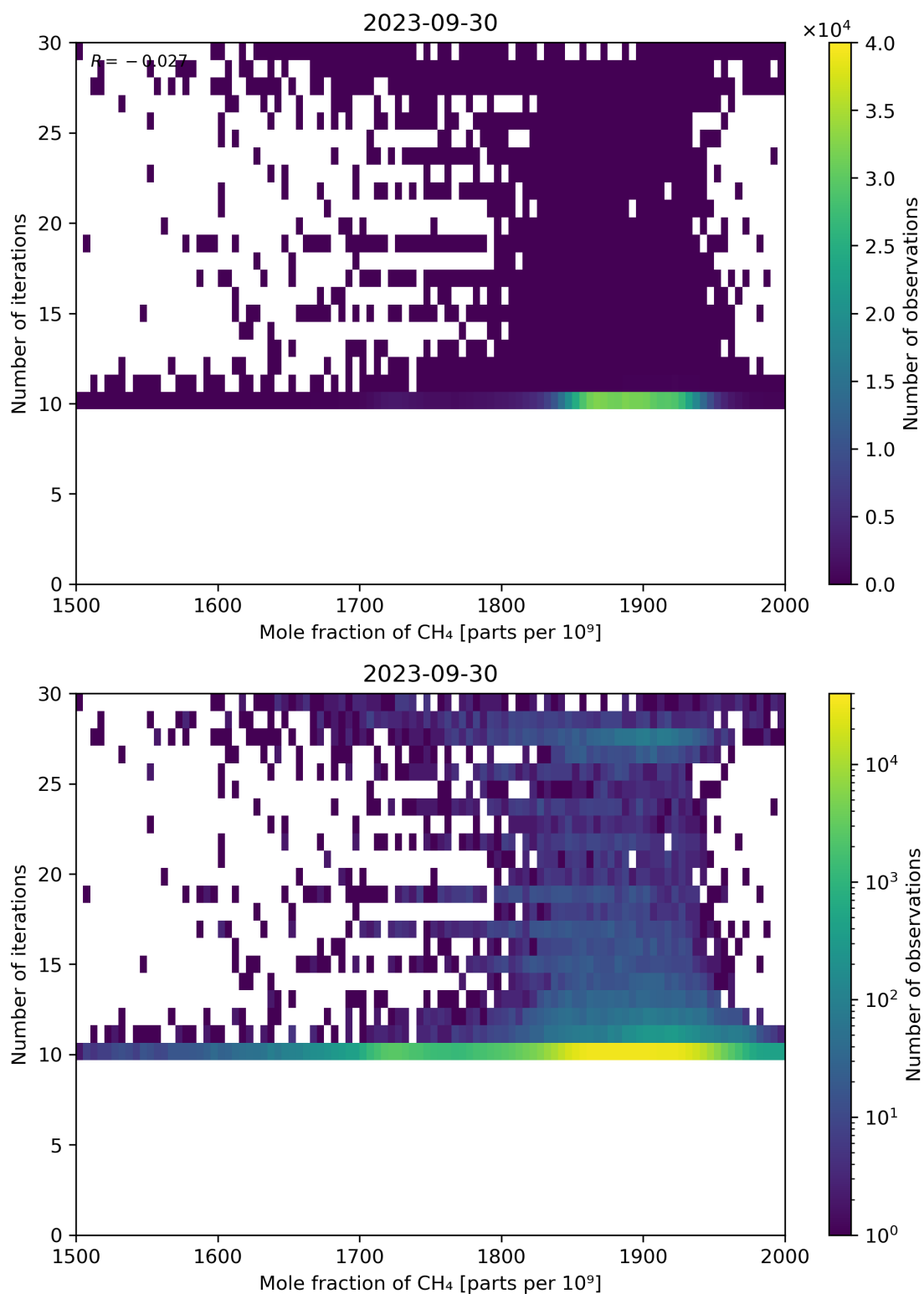
Figure 76: Scatter density plot of “Mole fraction of CH 4 ” against “Number of iterations” for 2023-09-29 to 2023-10-01.
