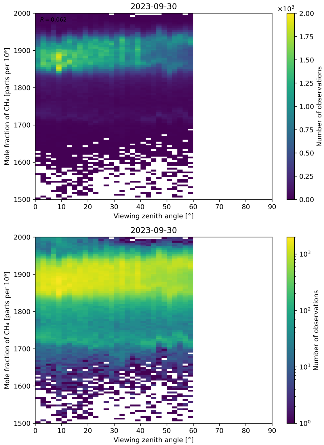
Figure 110: Scatter density plot of “Viewing zenith angle” against “Mole fraction of CH 4 ” for 2023-09-29 to 2023-10-01.
