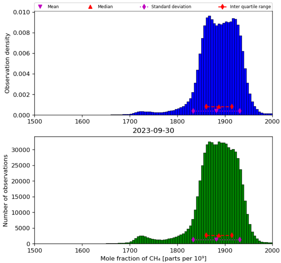
Figure 23: Histogram of “Mole fraction of CH 4 ” for 2023-09-29 to 2023-10-01
