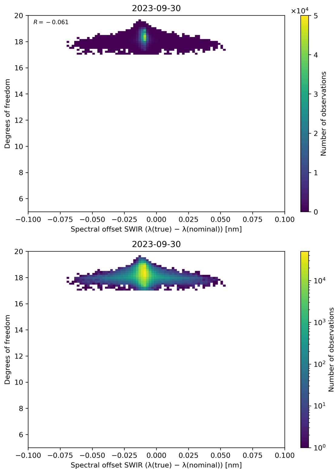
Figure 119: Scatter density plot of “Spectral offset SWIR ( \lambda(\text{true}) - \lambda(\text{nominal}) )” against “Degrees of freedom” for 2023-09-29 to 2023-10-01.
