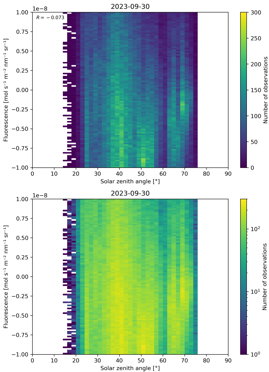
Figure 97: Scatter density plot of “Solar zenith angle” against “Fluorescence” for 2023-09-29 to 2023-10-01.
