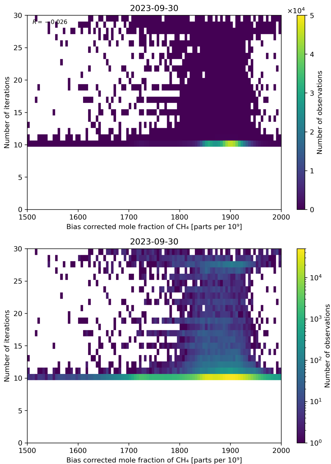
Figure 67: Scatter density plot of “Bias corrected mole fraction of CH 4 ” against “Number of iterations” for 2023-09-29 to 2023-10-01.
