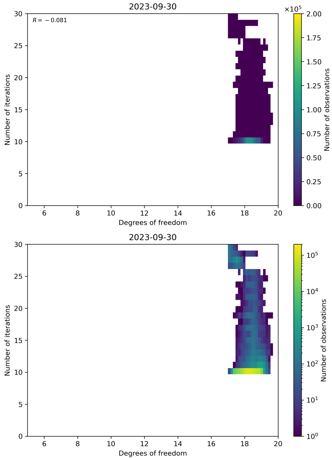
Figure 52: Scatter density plot of “Degrees of freedom” against “Number of iterations” for 2023-09-29 to 2023-10-01.
