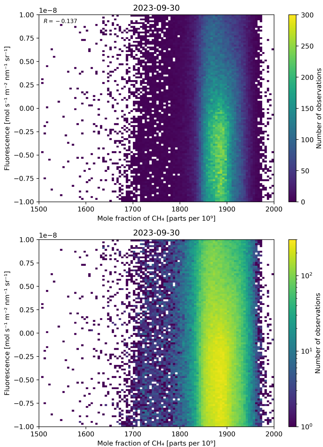
Figure 73: Scatter density plot of “Mole fraction of \text{CH}_4 ” against “Fluorescence” for 2023-09-29 to 2023-10-01.
