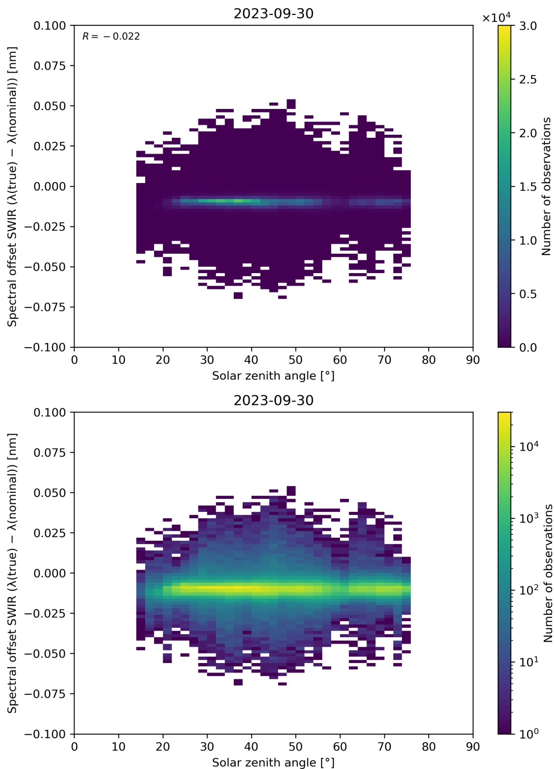
Figure 104: Scatter density plot of “Solar zenith angle” against “Spectral offset SWIR ( \lambda(\text{true}) - \lambda(\text{nominal}) )” for 2023-09-29 to 2023-10-01.
