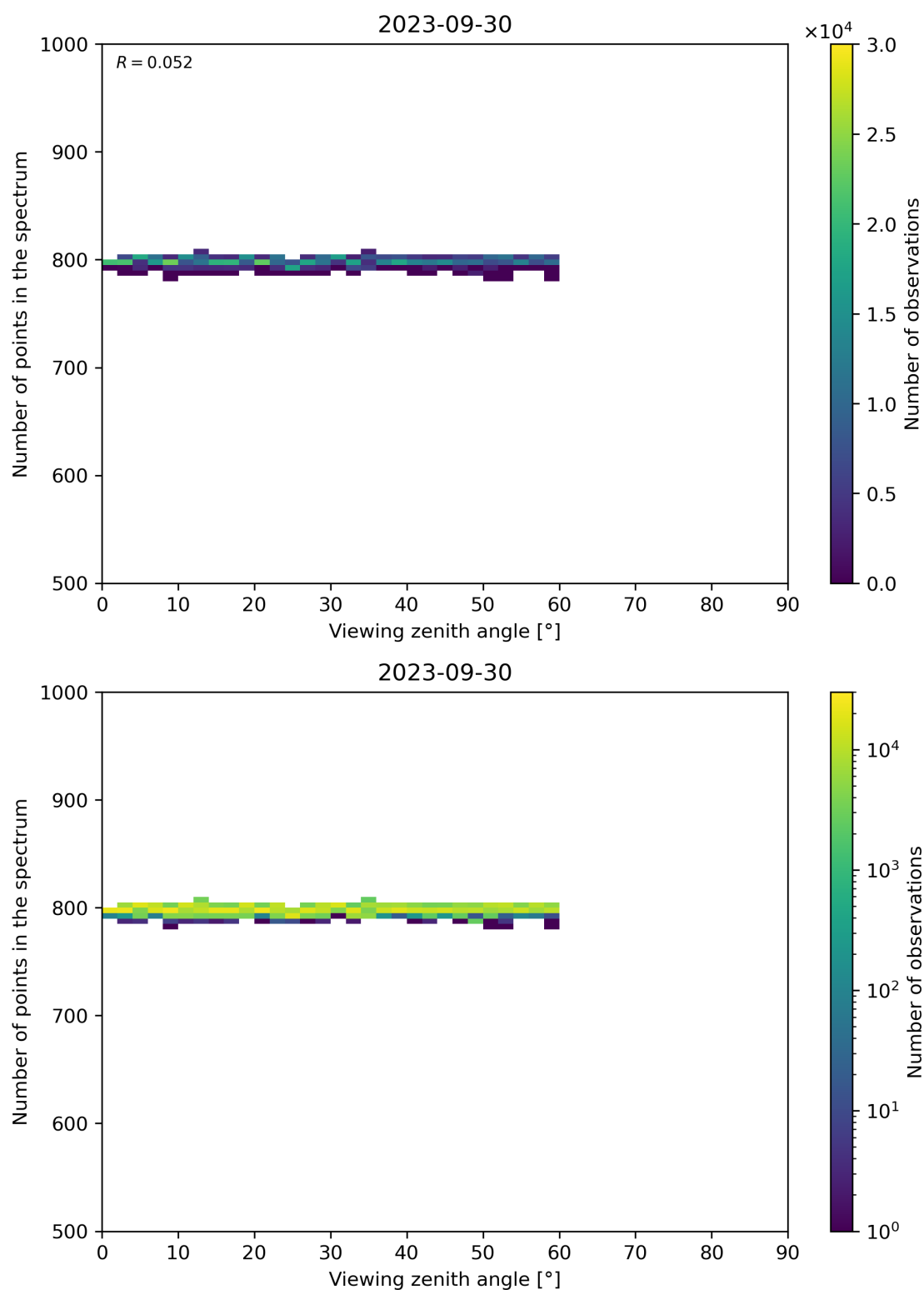
Figure 114: Scatter density plot of “Viewing zenith angle” against “Number of points in the spectrum” for 2023-09-29 to 2023-10-01.
