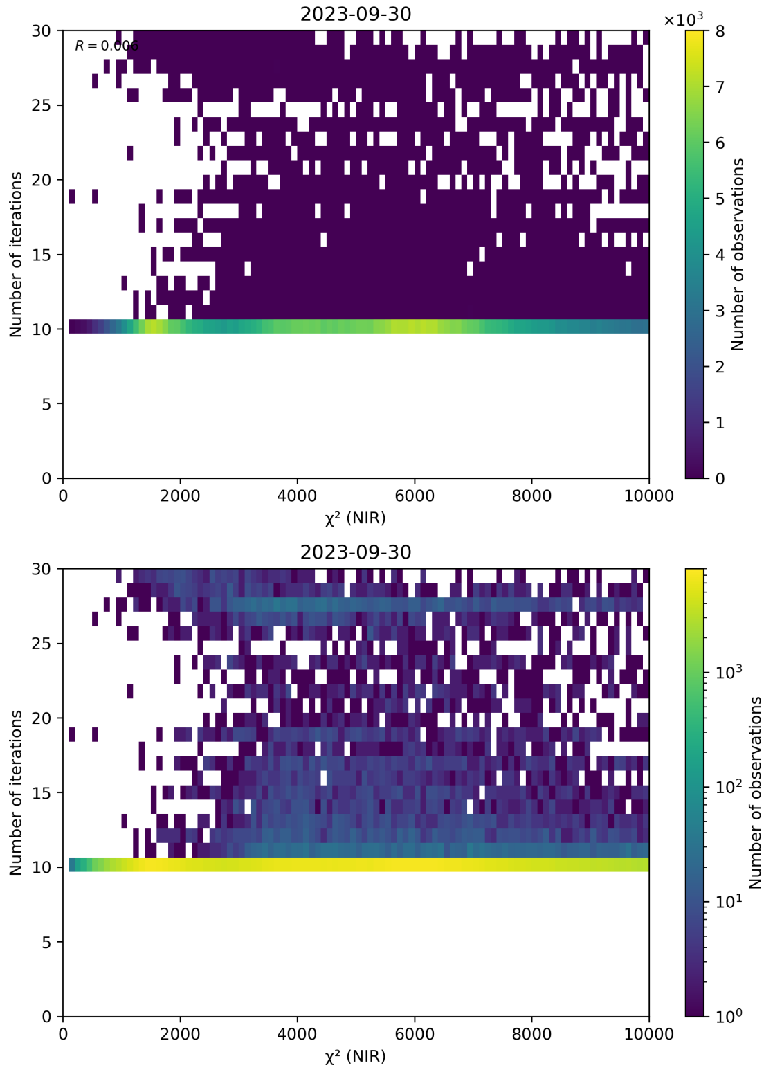
Figure 46: Scatter density plot of “ \chi^2 (NIR)” against “Number of iterations” for 2023-09-29 to 2023-10-01.
