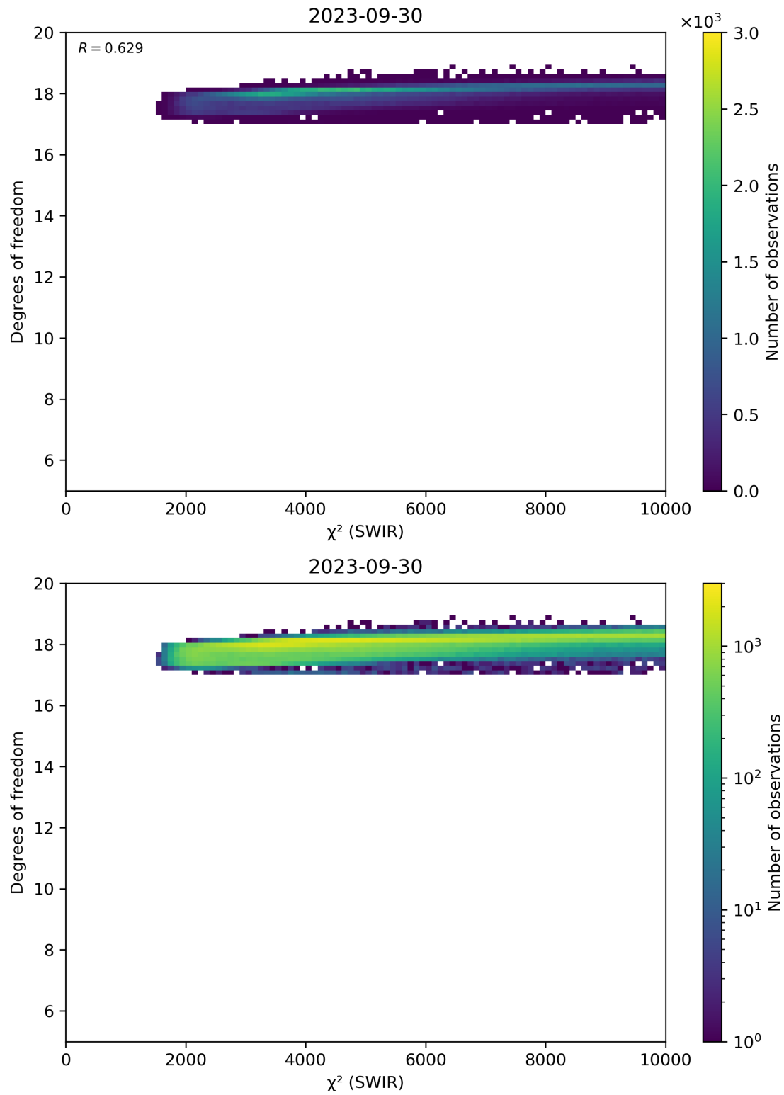
Figure 48: Scatter density plot of “ \chi^2 (SWIR)” against “Degrees of freedom” for 2023-09-29 to 2023-10-01.
