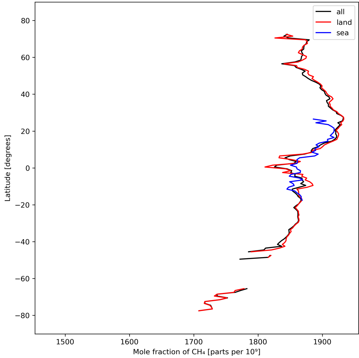
Figure 12: Zonal average of “Mole fraction of CH 4 ” for 2023-09-29 to 2023-10-01.
