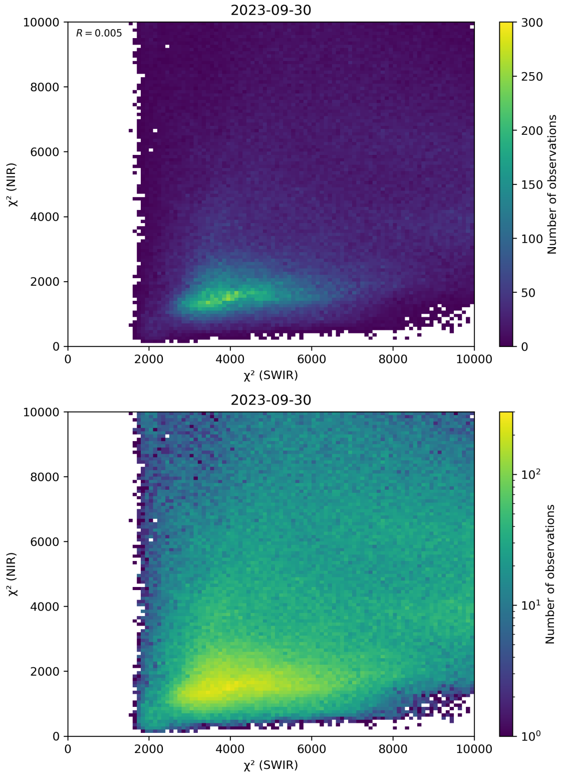
Figure 47: Scatter density plot of “ \chi^2 (SWIR)” against “ \chi^2 (NIR)” for 2023-09-29 to 2023-10-01.
