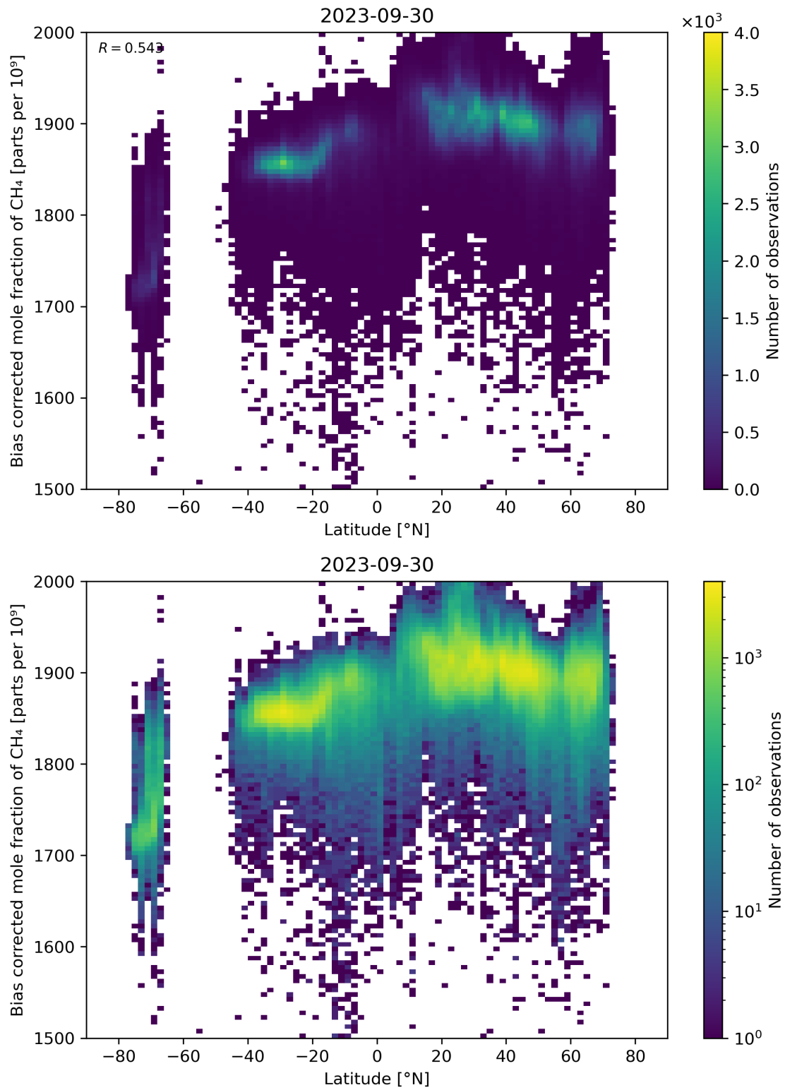
Figure 58: Scatter density plot of “Latitude” against “Bias corrected mole fraction of CH 4 ” for 2023-09-29 to 2023-10-01.
