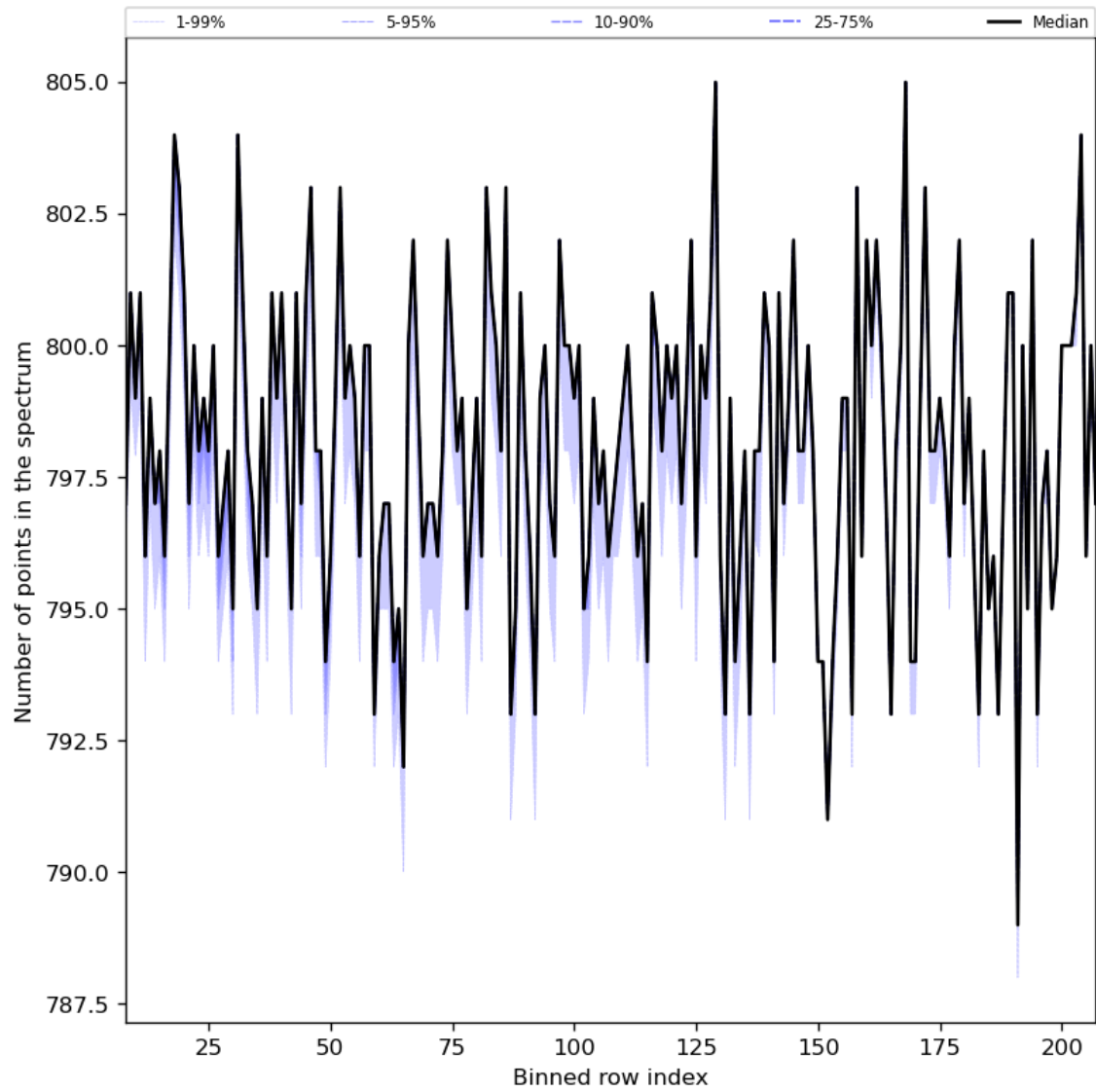
Figure 37: Along track statistics of “Number of points in the spectrum” for 2023-09-29 to 2023-10-01
