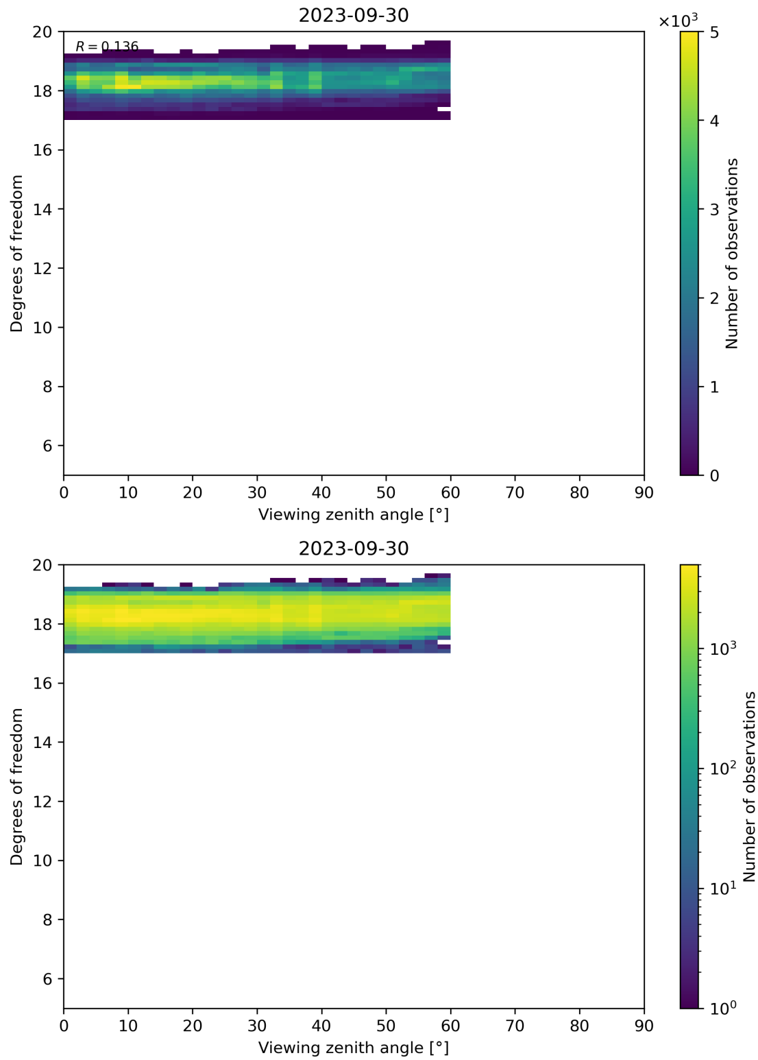
Figure 107: Scatter density plot of “Viewing zenith angle” against “Degrees of freedom” for 2023-09-29 to 2023-10-01.
