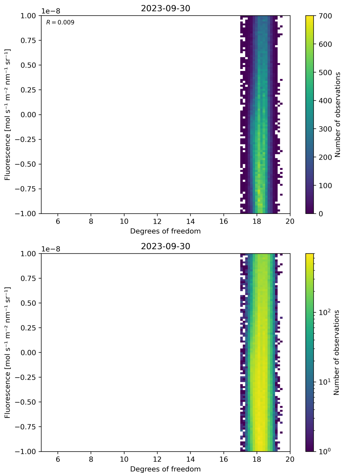
Figure 51: Scatter density plot of “Degrees of freedom” against “Fluorescence” for 2023-09-29 to 2023-10-01.
