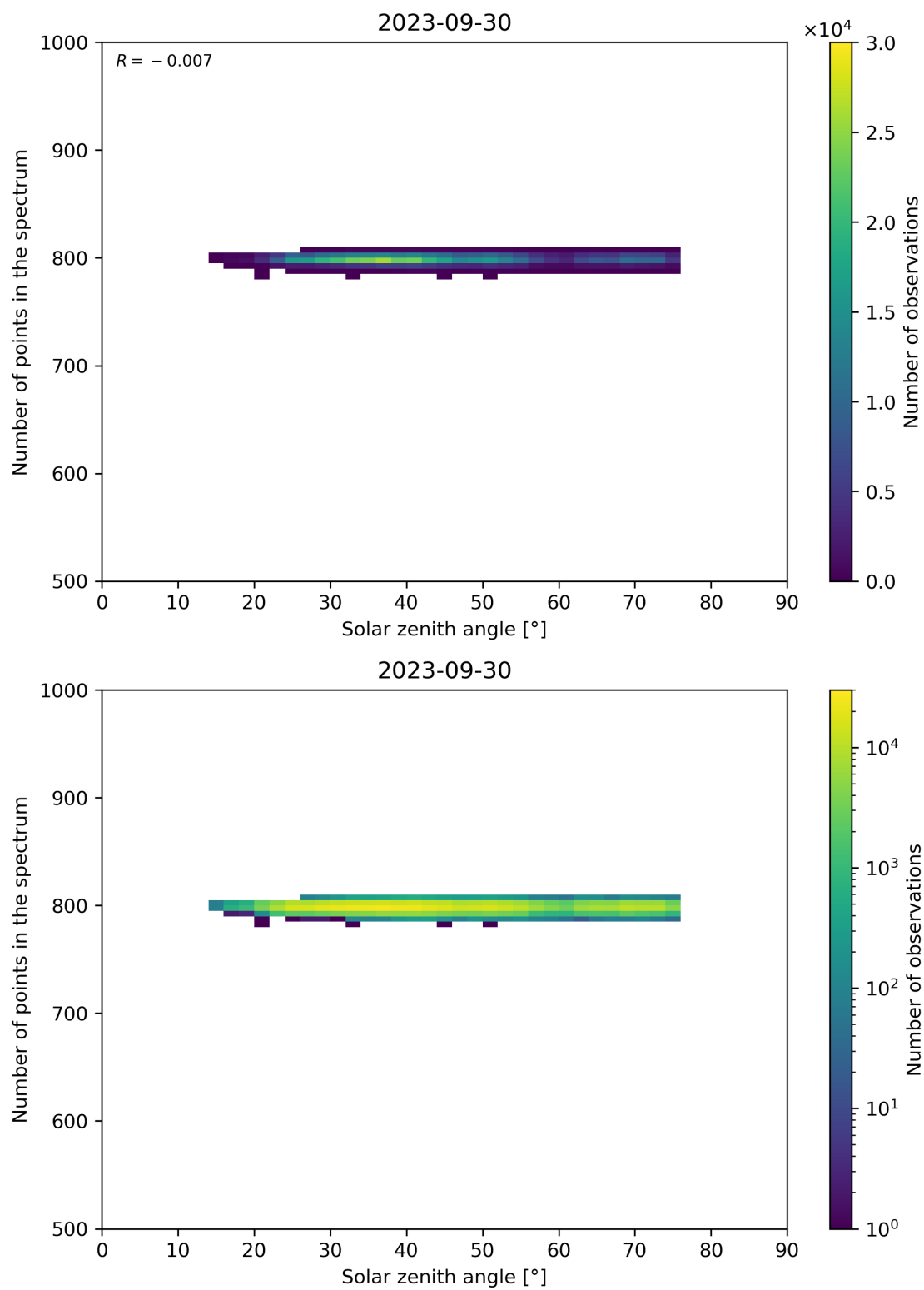
Figure 103: Scatter density plot of “Solar zenith angle” against “Number of points in the spectrum” for 2023-09-29 to 2023-10-01.
