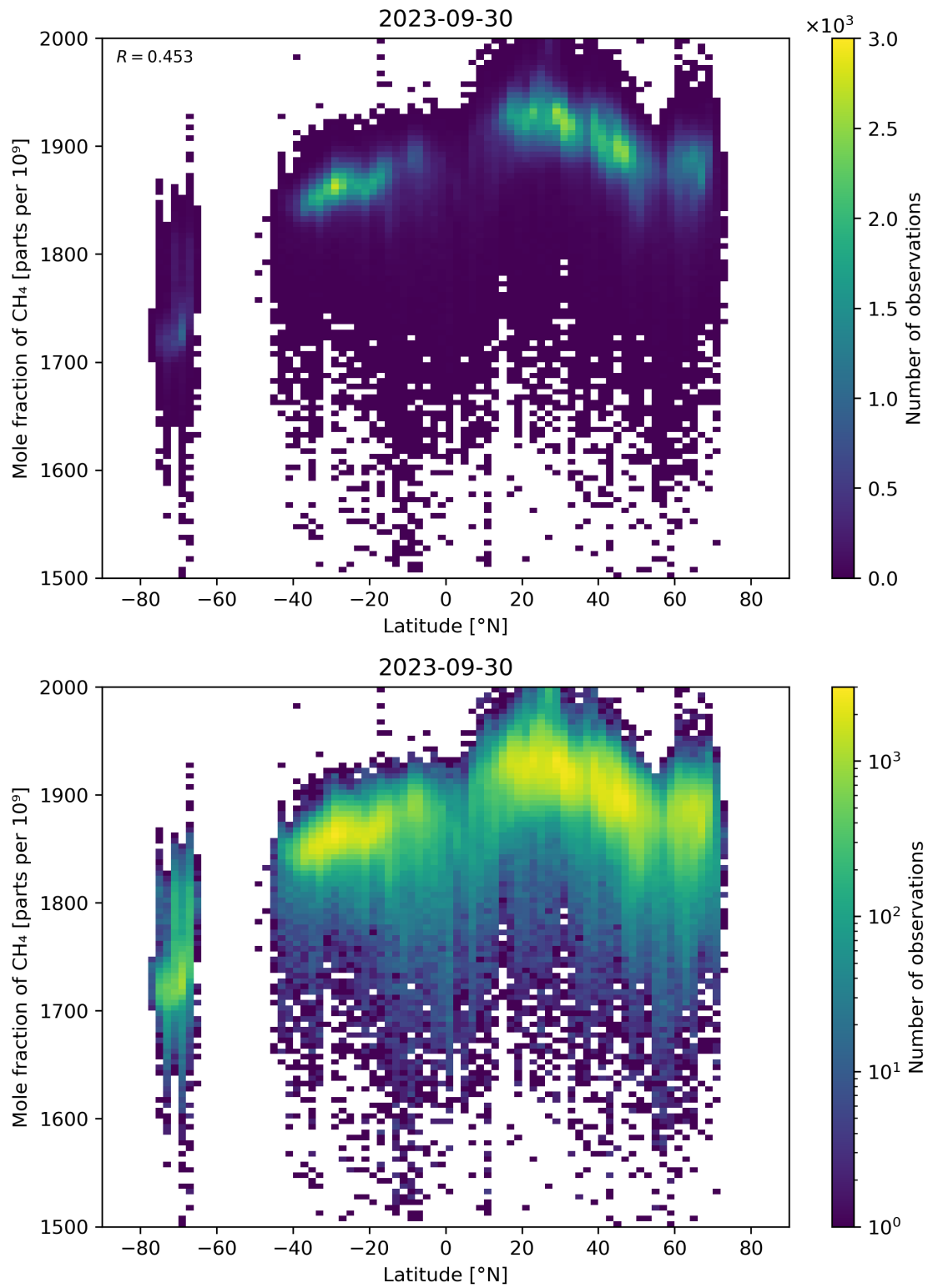
Figure 57: Scatter density plot of “Latitude” against “Mole fraction of CH 4 ” for 2023-09-29 to 2023-10-01.
