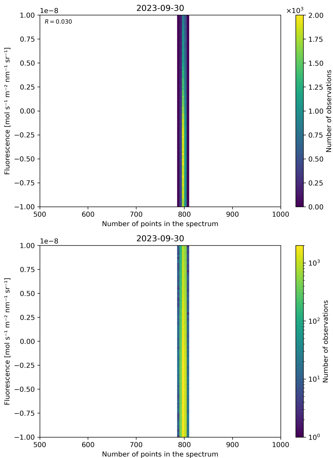
Figure 91: Scatter density plot of “Number of points in the spectrum” against “Fluorescence” for 2023-09-29 to 2023-10-01.
