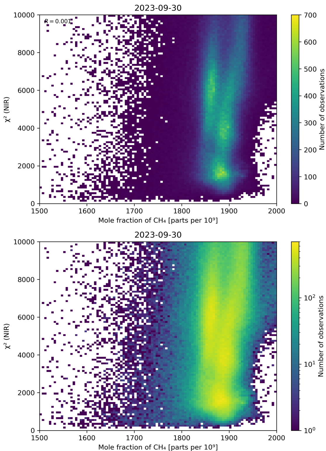
Figure 70: Scatter density plot of “Mole fraction of \text{CH}_4 ” against “ \chi^2 (NIR)” for 2023-09-29 to 2023-10-01.
