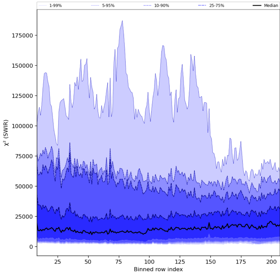
Figure 39: Along track statistics of “ \chi^2 (SWIR)” for 2023-09-29 to 2023-10-01
