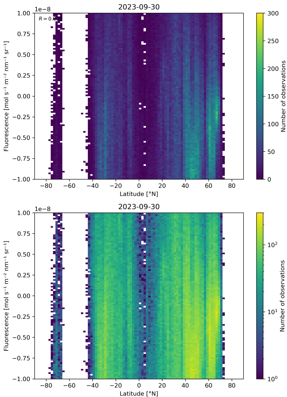
Figure 56: Scatter density plot of “Latitude” against “Fluorescence” for 2023-09-29 to 2023-10-01.
