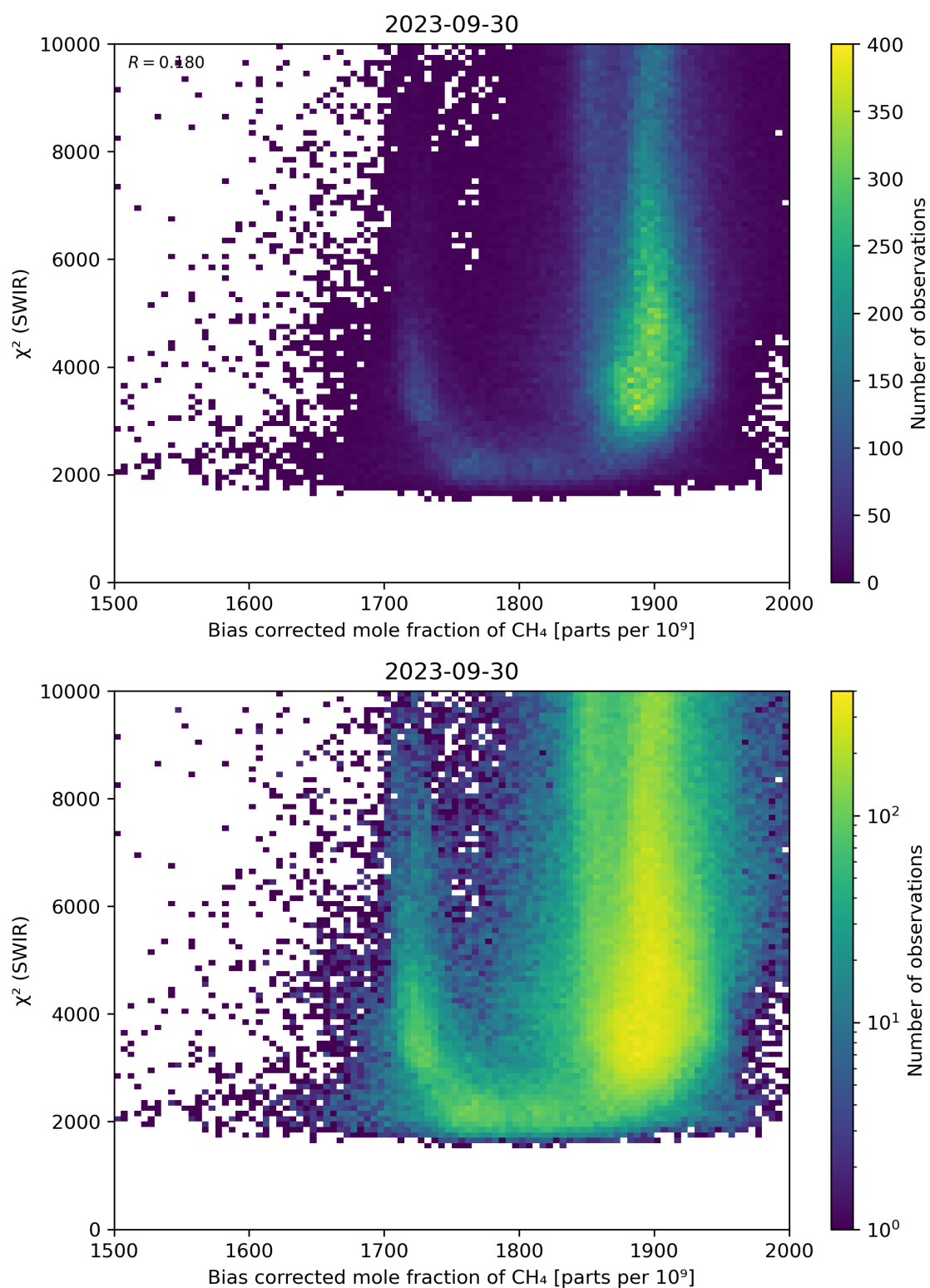
Figure 64: Scatter density plot of “Bias corrected mole fraction of \text{CH}_4 ” against “ \chi^2 (SWIR)” for 2023-09-29 to 2023-10-01.
