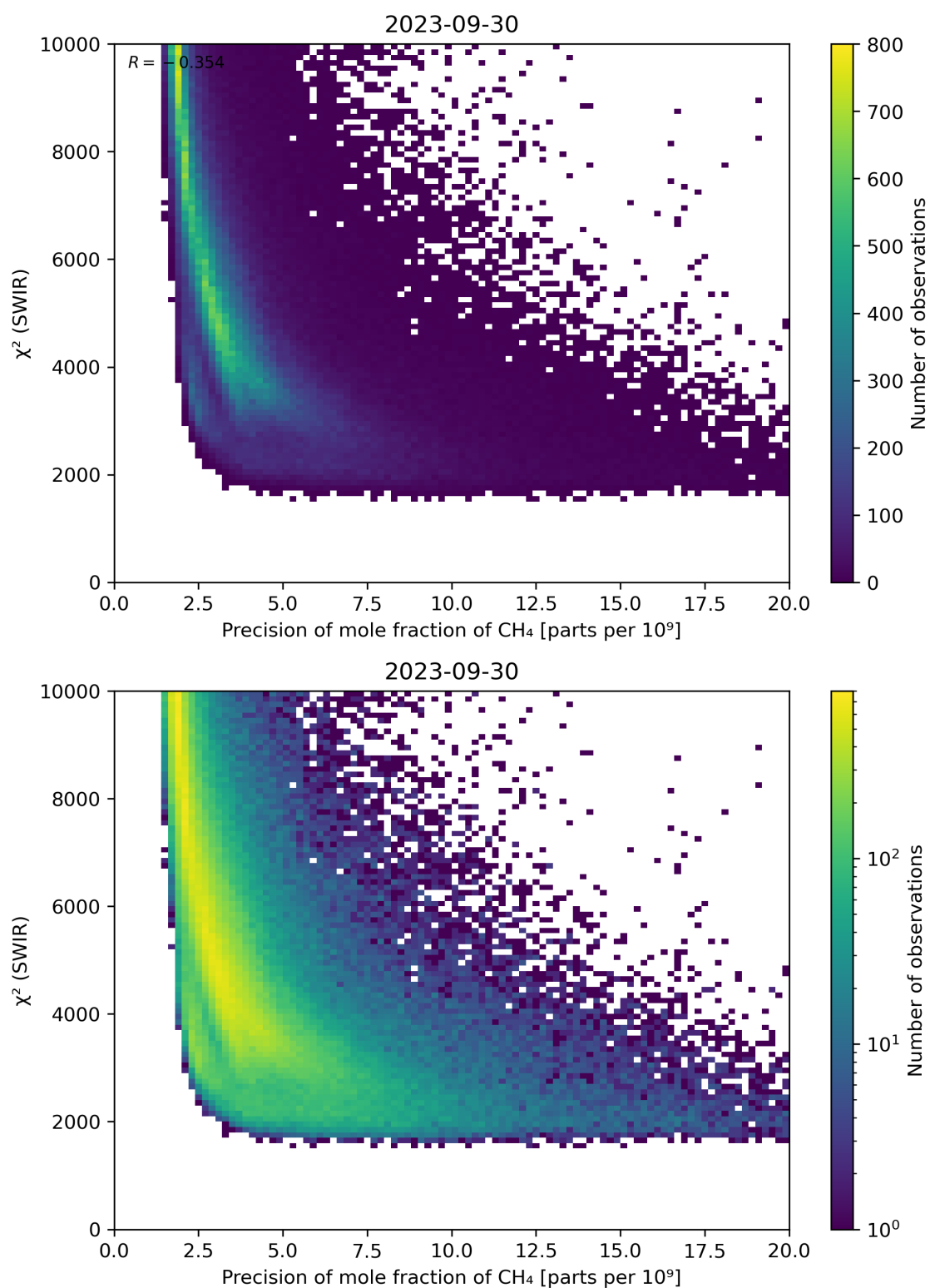
Figure 79: Scatter density plot of “Precision of mole fraction of CH 4 ” against “ \chi^2 (SWIR)” for 2023-09-29 to 2023-10-01.
