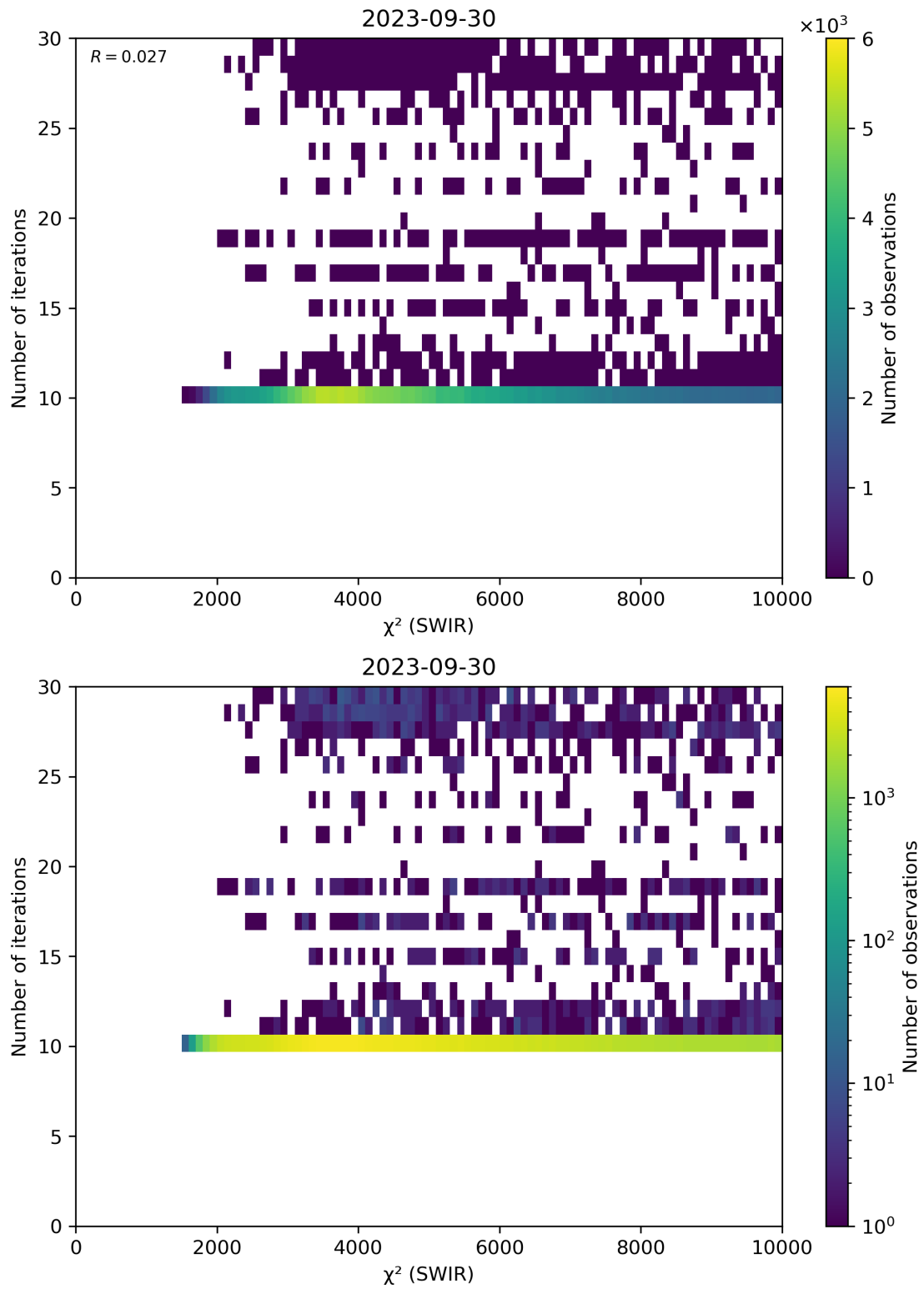
Figure 50: Scatter density plot of “ \chi^2 (SWIR)” against “Number of iterations” for 2023-09-29 to 2023-10-01.
