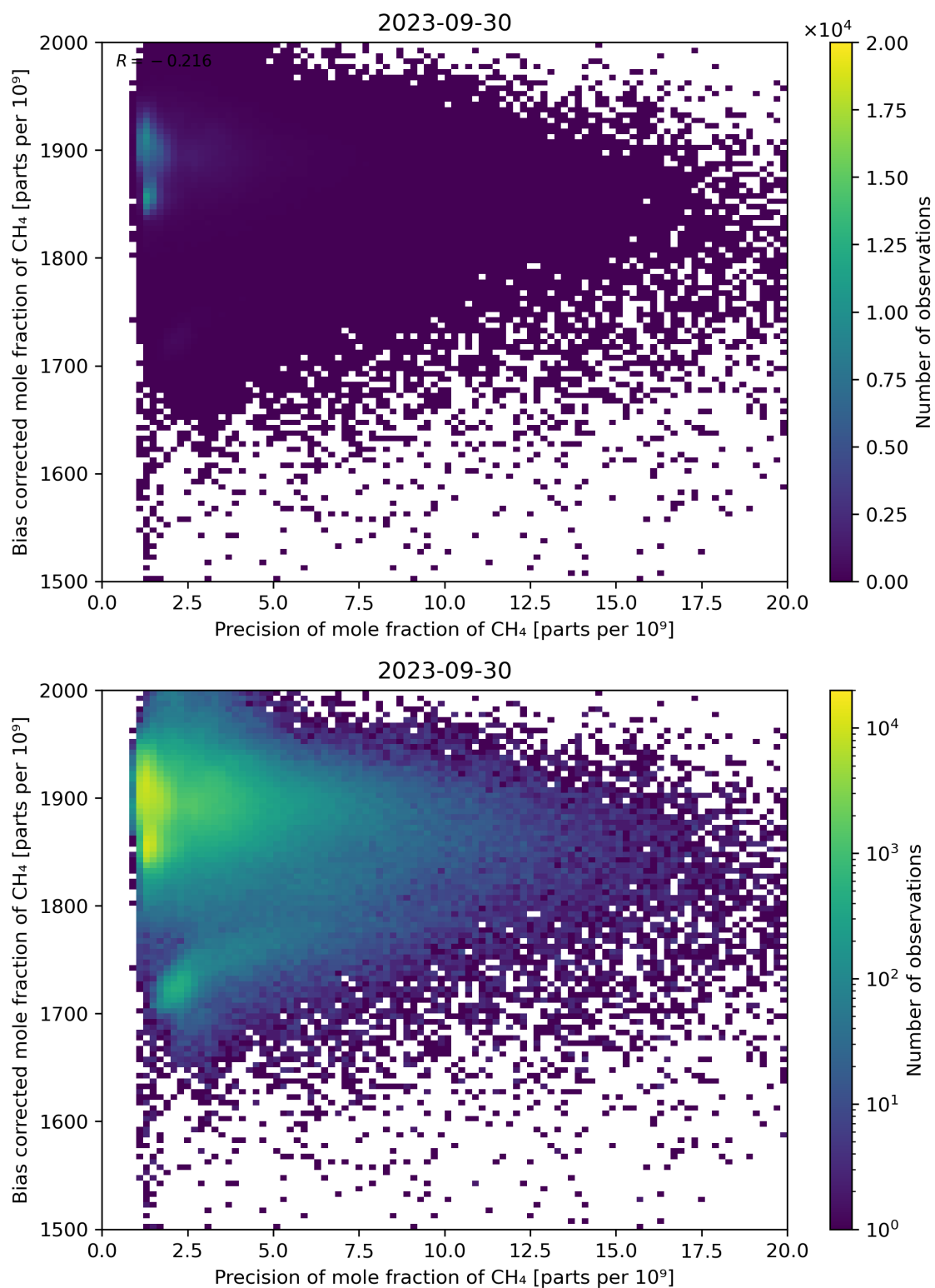
Figure 82: Scatter density plot of “Precision of mole fraction of CH 4 ” against “Bias corrected mole fraction of CH 4 ” for 2023-09-29 to 2023-10-01.
