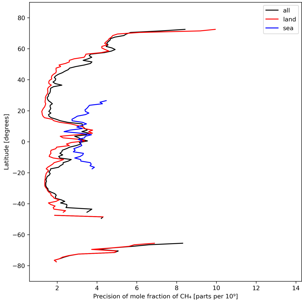
Figure 13: Zonal average of “Precision of mole fraction of CH 4 ” for 2023-09-29 to 2023-10-01.
