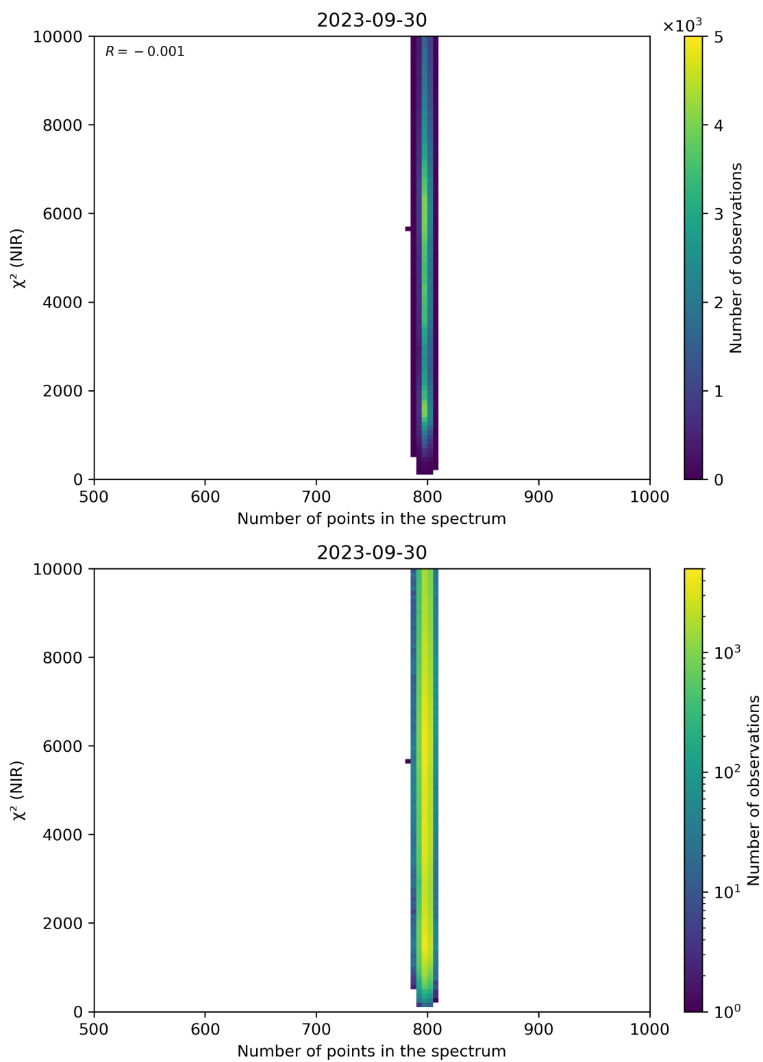
Figure 88: Scatter density plot of “Number of points in the spectrum” against “ \chi^2 (NIR)” for 2023-09-29 to 2023-10-01.
