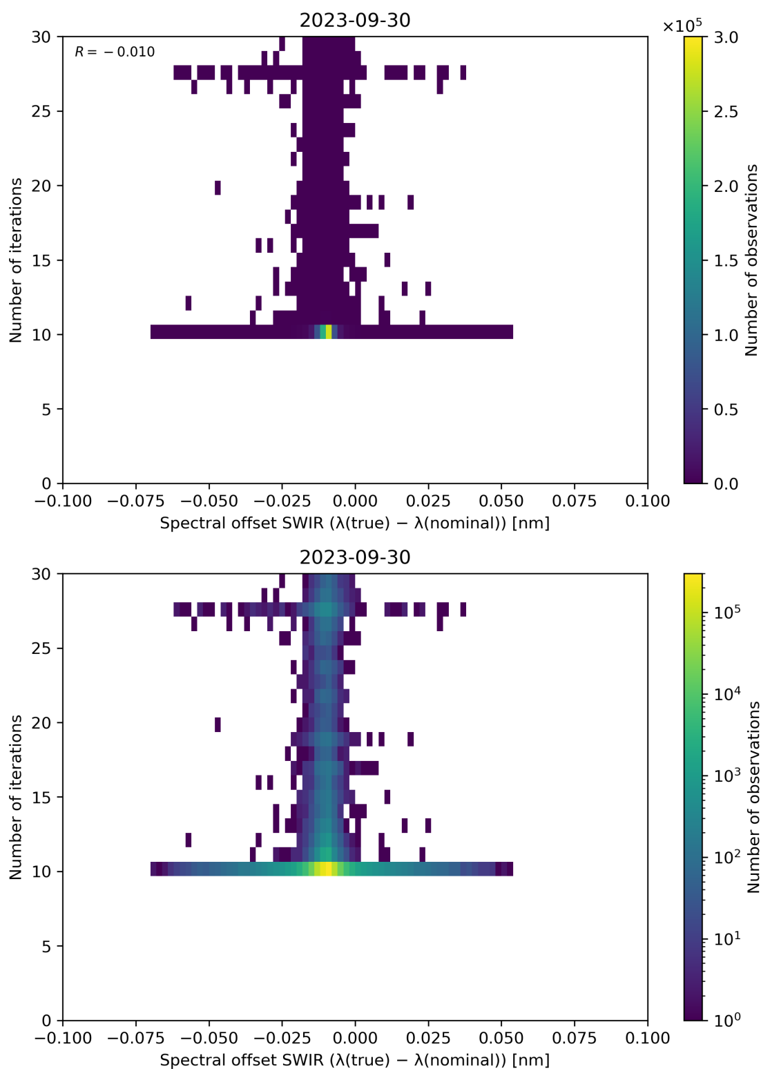
Figure 121: Scatter density plot of “Spectral offset SWIR ( \lambda(\text{true}) - \lambda(\text{nominal}) )” against “Number of iterations” for 2023-09-29 to 2023-10-01.
