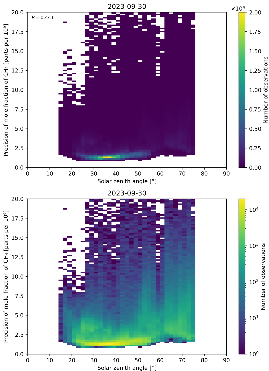
Figure 101: Scatter density plot of “Solar zenith angle” against “Precision of mole fraction of \text{CH}_4 ” for 2023-09-29 to 2023-10-01.
