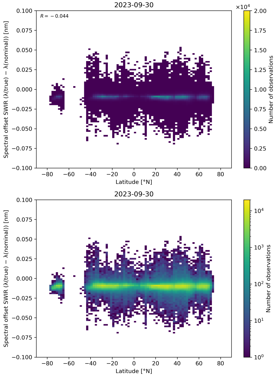
Figure 62: Scatter density plot of “Latitude” against “Spectral offset SWIR ( \lambda(\text{true}) - \lambda(\text{nominal}) )” for 2023-09-29 to 2023-10-01.
