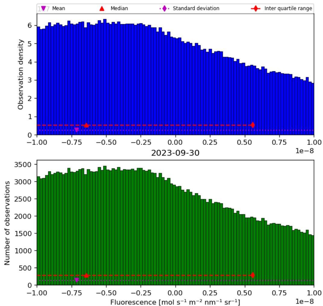
Figure 32: Histogram of “Fluorescence” for 2023-09-29 to 2023-10-01
