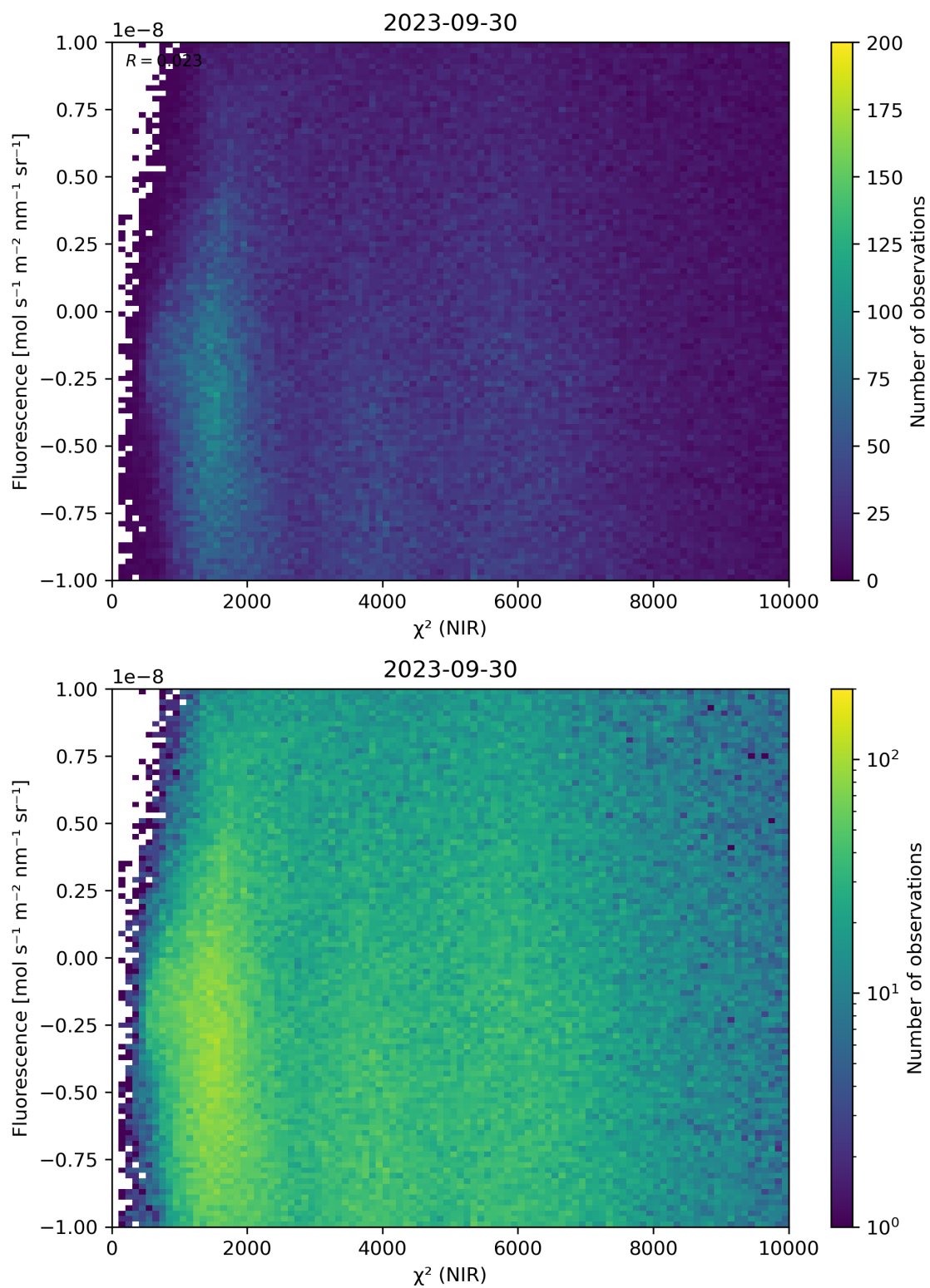
Figure 45: Scatter density plot of “ \chi^2 (NIR)” against “Fluorescence” for 2023-09-29 to 2023-10-01.
