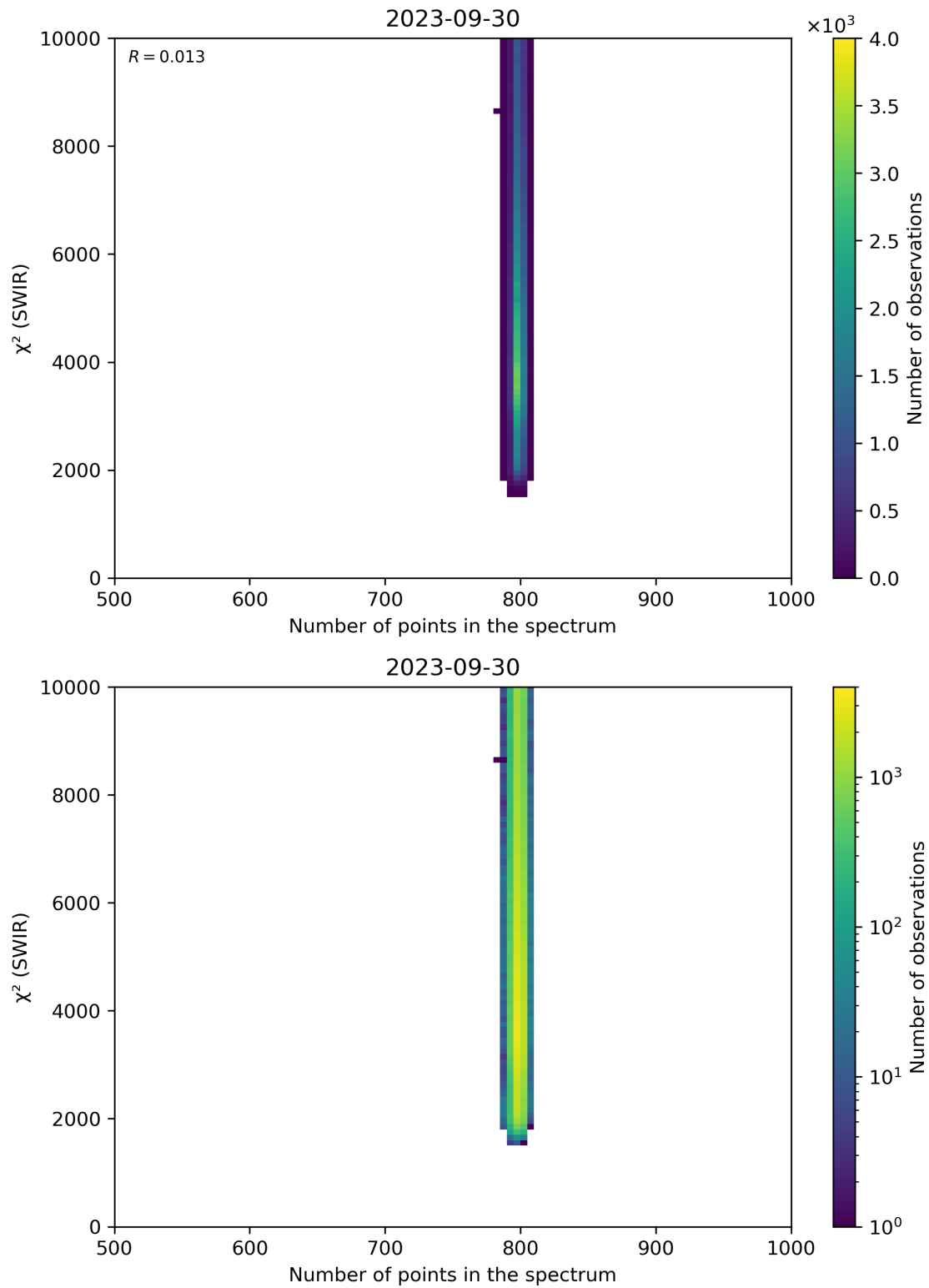
Figure 89: Scatter density plot of “Number of points in the spectrum” against “ \chi^2 (SWIR)” for 2023-09-29 to 2023-10-01.
