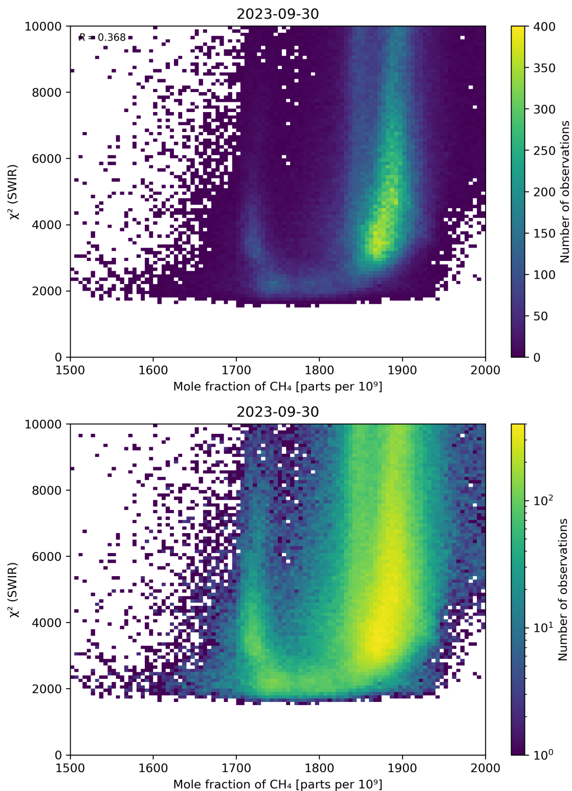
Figure 71: Scatter density plot of “Mole fraction of \text{CH}_4 ” against “ \chi^2 (SWIR)” for 2023-09-29 to 2023-10-01.
