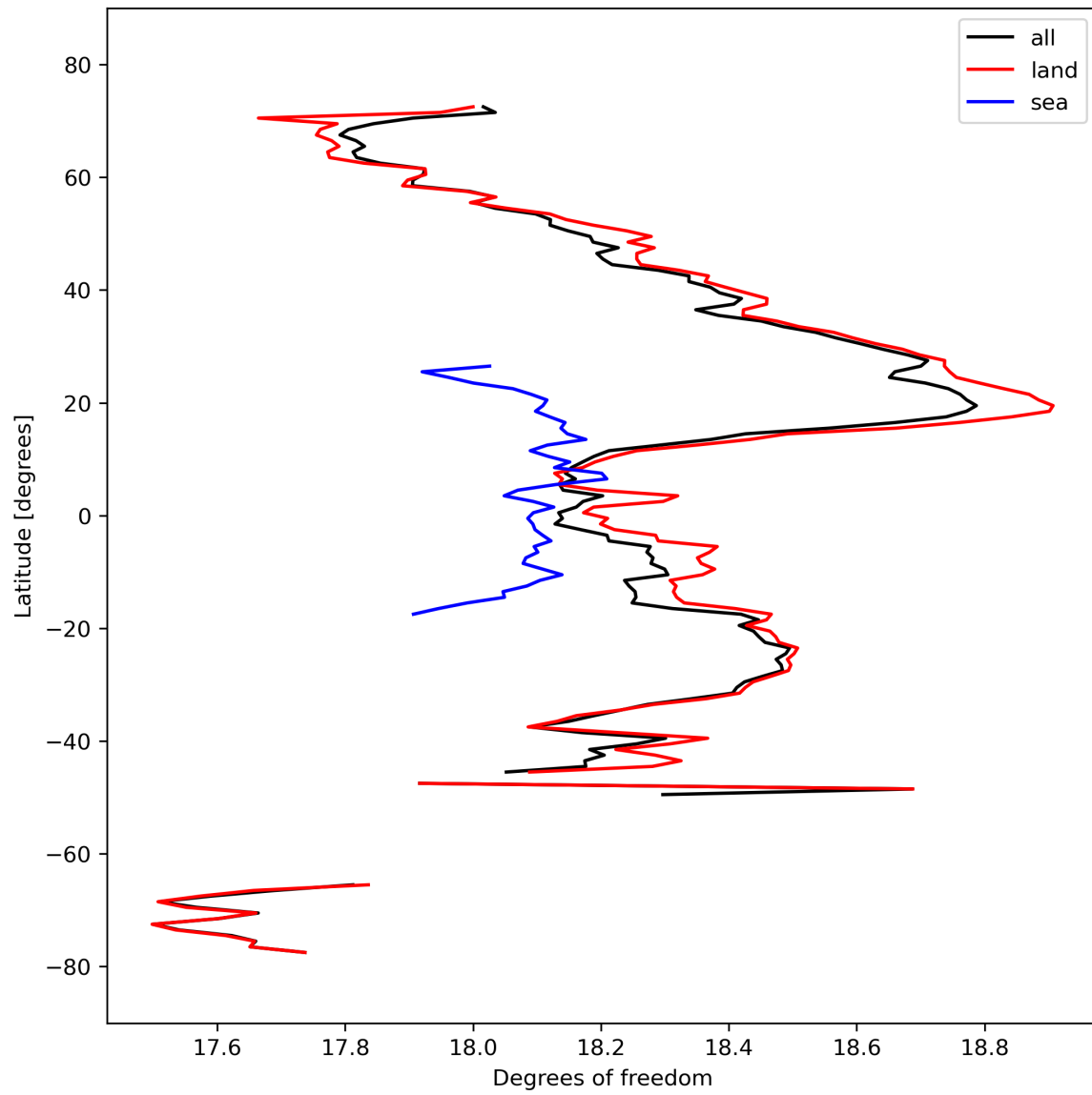
Figure 19: Zonal average of “Degrees of freedom” for 2023-09-29 to 2023-10-01.
