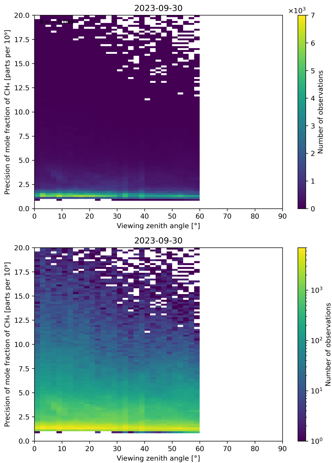
Figure 112: Scatter density plot of “Viewing zenith angle” against “Precision of mole fraction of CH 4 ” for 2023-09-29 to 2023-10-01.
