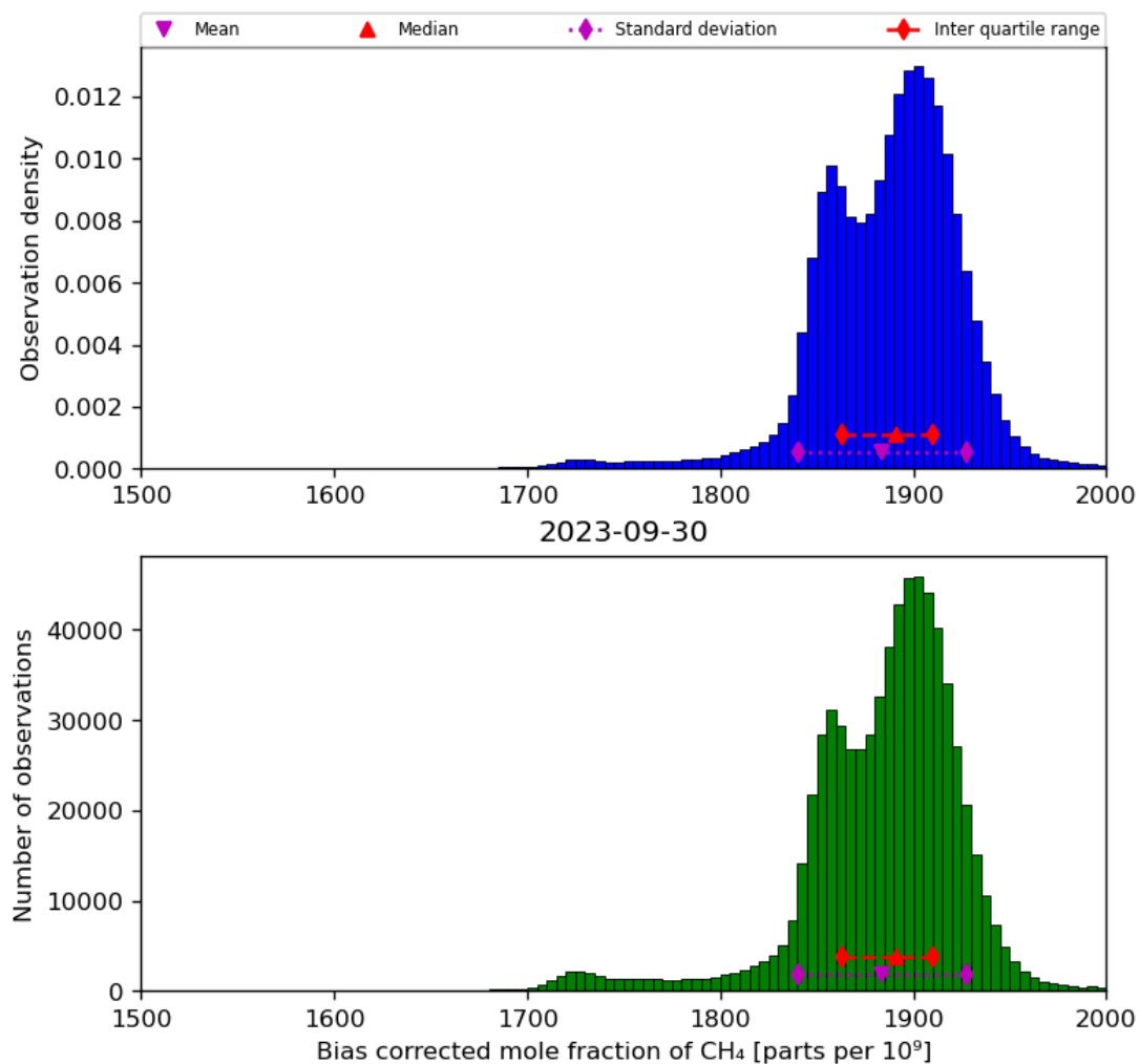
Figure 25: Histogram of “Bias corrected mole fraction of CH 4 ” for 2023-09-29 to 2023-10-01
