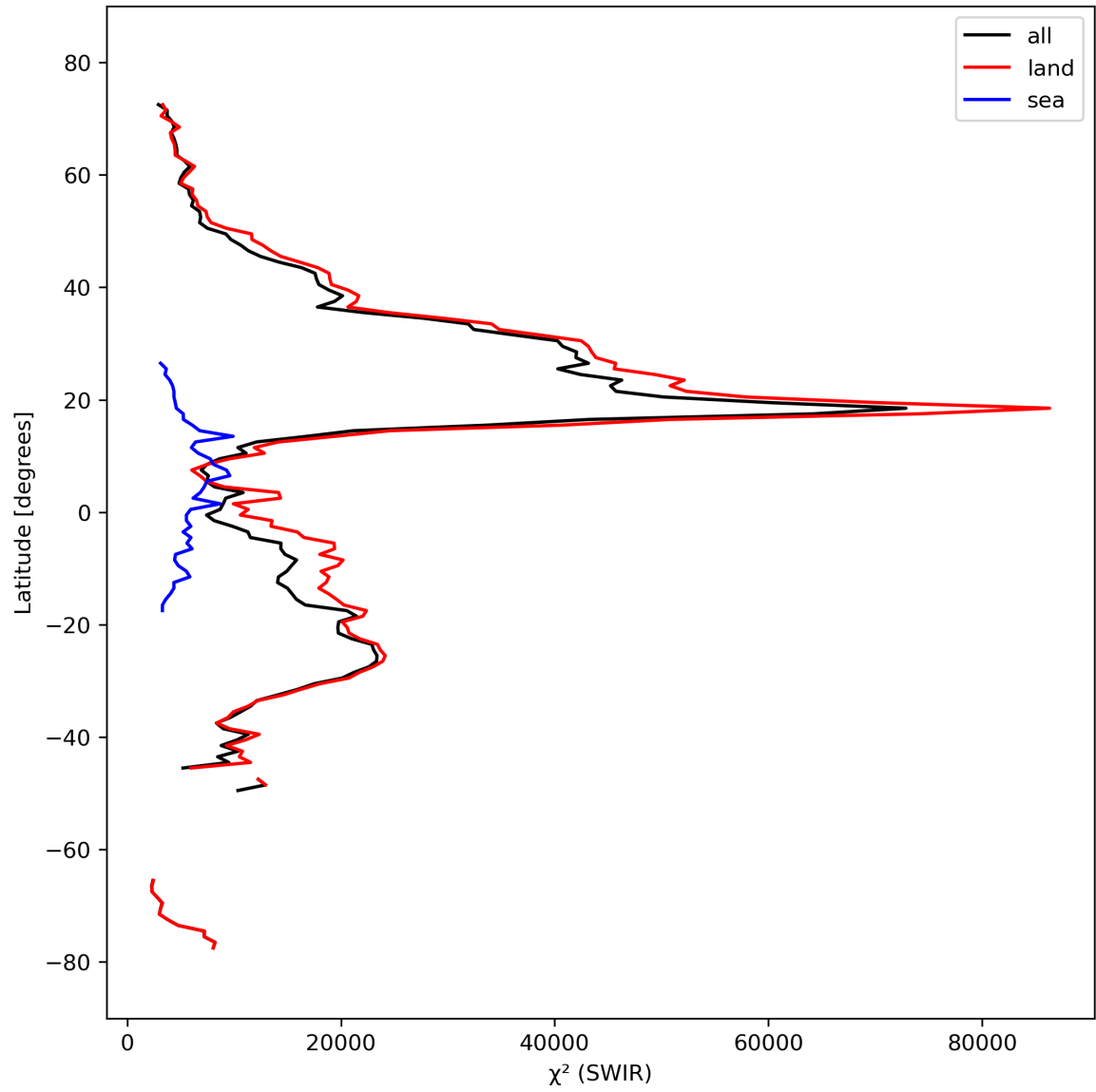
Figure 17: Zonal average of “ \chi^2 (SWIR)” for 2023-09-29 to 2023-10-01.
