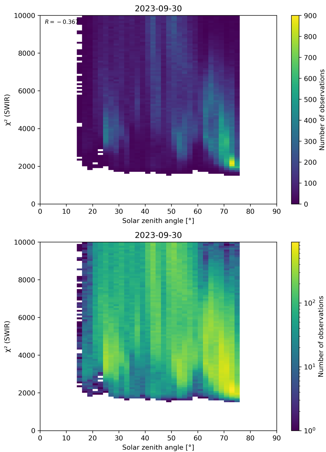
Figure 95: Scatter density plot of “Solar zenith angle” against “ \chi^2 (SWIR)” for 2023-09-29 to 2023-10-01.
