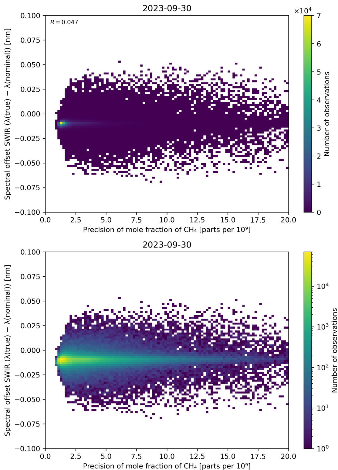
Figure 85: Scatter density plot of “Precision of mole fraction of \text{CH}_4 ” against “Spectral offset SWIR ( \lambda(\text{true}) - \lambda(\text{nominal}) )” for 2023-09-29 to 2023-10-01.
