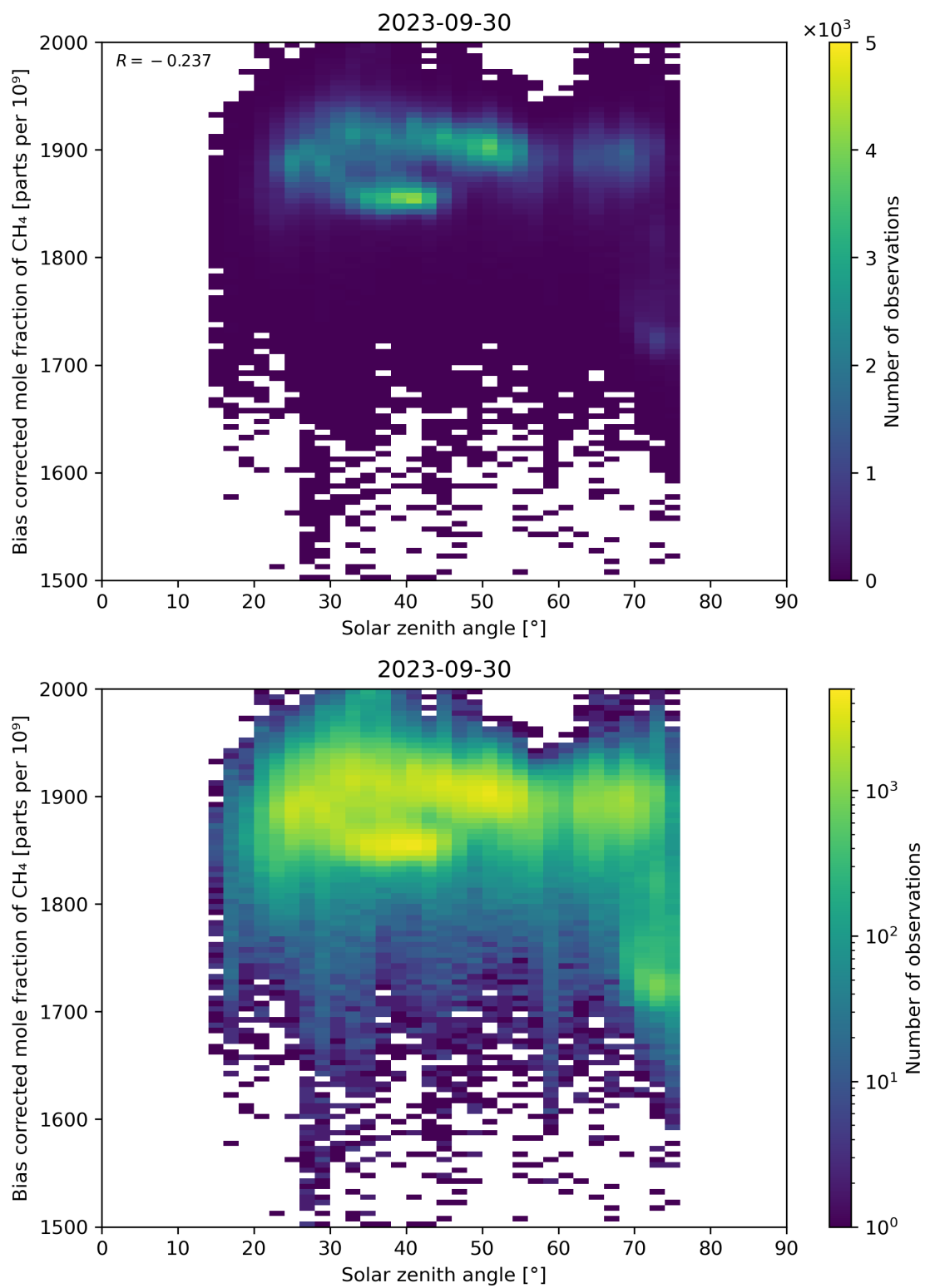
Figure 100: Scatter density plot of “Solar zenith angle” against “Bias corrected mole fraction of \text{CH}_4 ” for 2023-09-29 to 2023-10-01.
