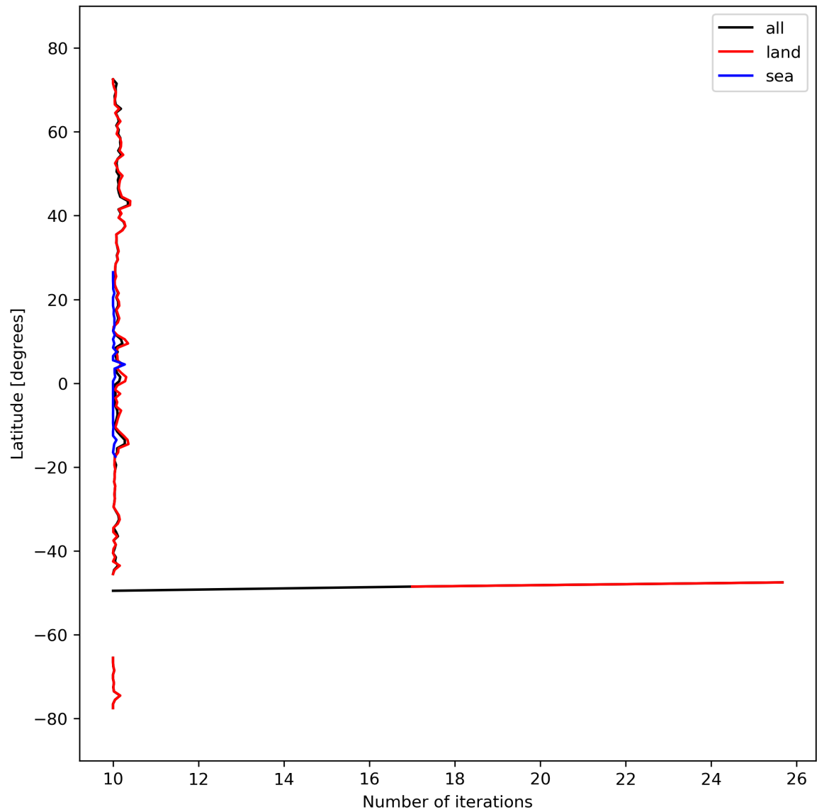
Figure 20: Zonal average of “Number of iterations” for 2023-09-29 to 2023-10-01.
