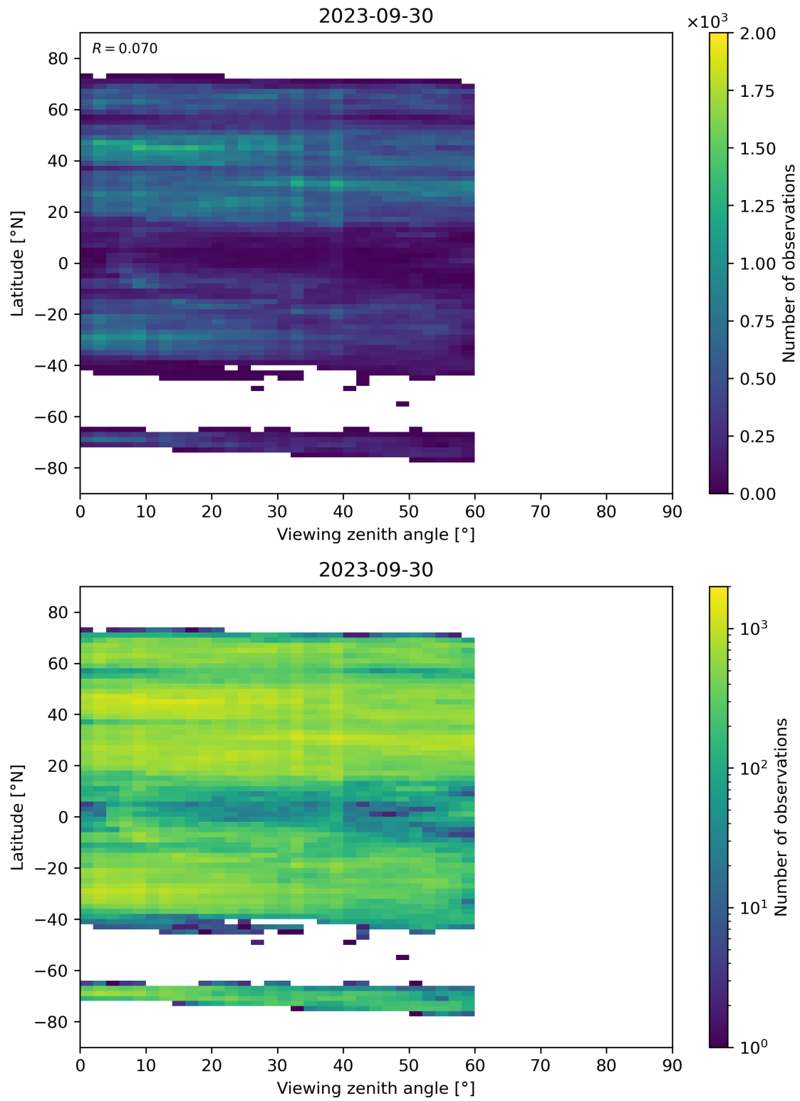
Figure 109: Scatter density plot of “Viewing zenith angle” against “Latitude” for 2023-09-29 to 2023-10-01.
