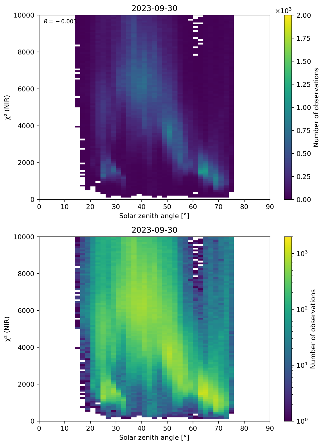
Figure 94: Scatter density plot of “Solar zenith angle” against “ \chi^2 (NIR)” for 2023-09-29 to 2023-10-01.
