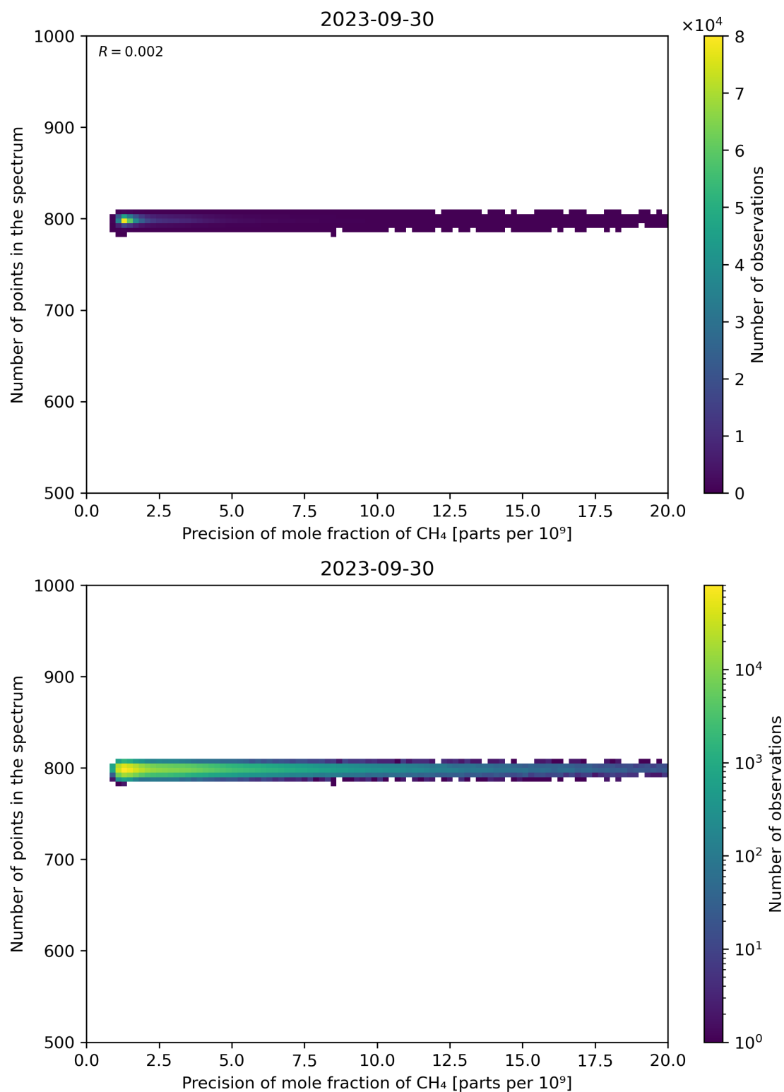
Figure 84: Scatter density plot of “Precision of mole fraction of \text{CH}_4 ” against “Number of points in the spectrum” for 2023-09-29 to 2023-10-01.
