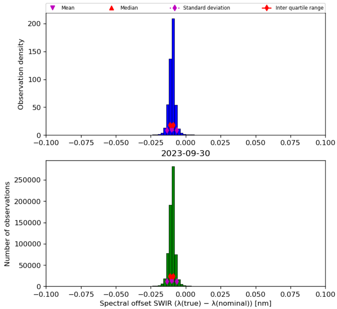
Figure 27: Histogram of “Spectral offset SWIR ( \lambda(\text{true}) - \lambda(\text{nominal}) )” for 2023-09-29 to 2023-10-01
