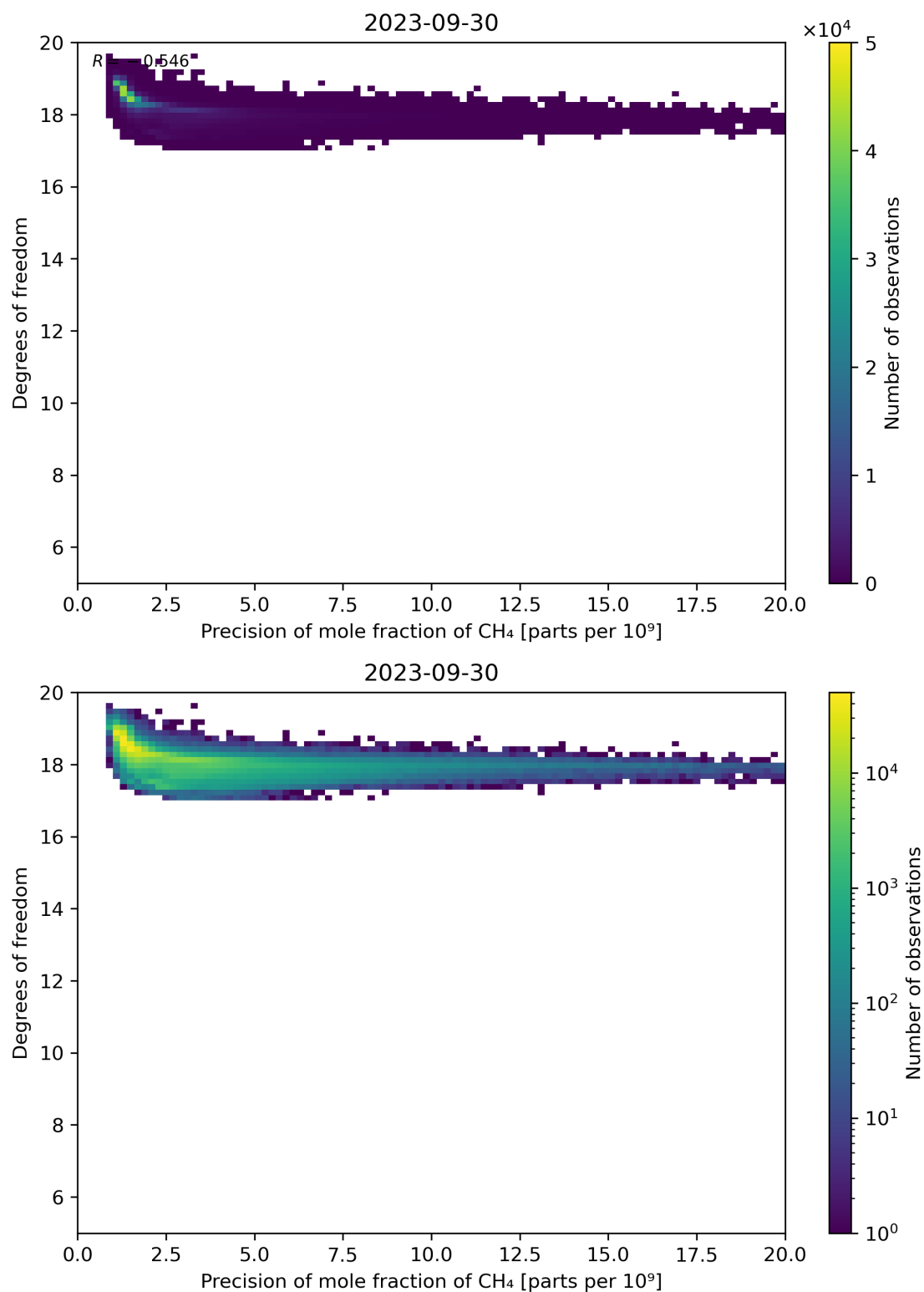
Figure 80: Scatter density plot of “Precision of mole fraction of CH 4 ” against “Degrees of freedom” for 2023-09-29 to 2023-10-01.
