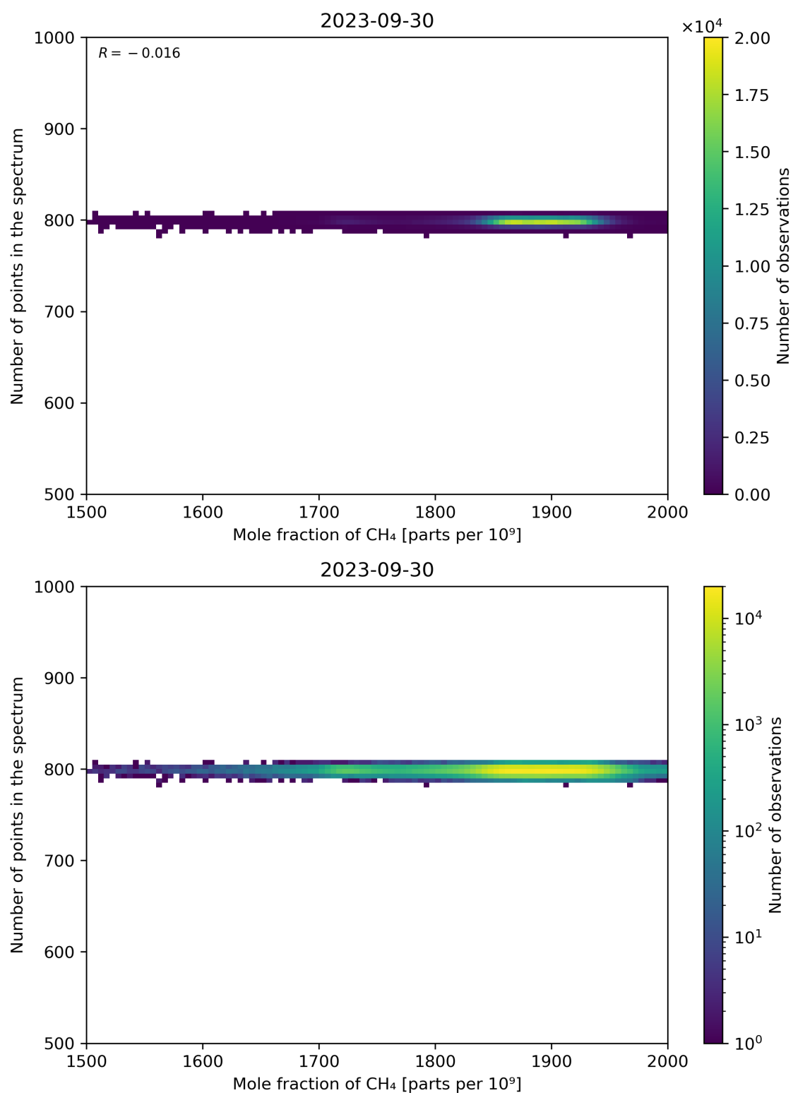
Figure 77: Scatter density plot of “Mole fraction of CH 4 ” against “Number of points in the spectrum” for 2023-09-29 to 2023-10-01.
