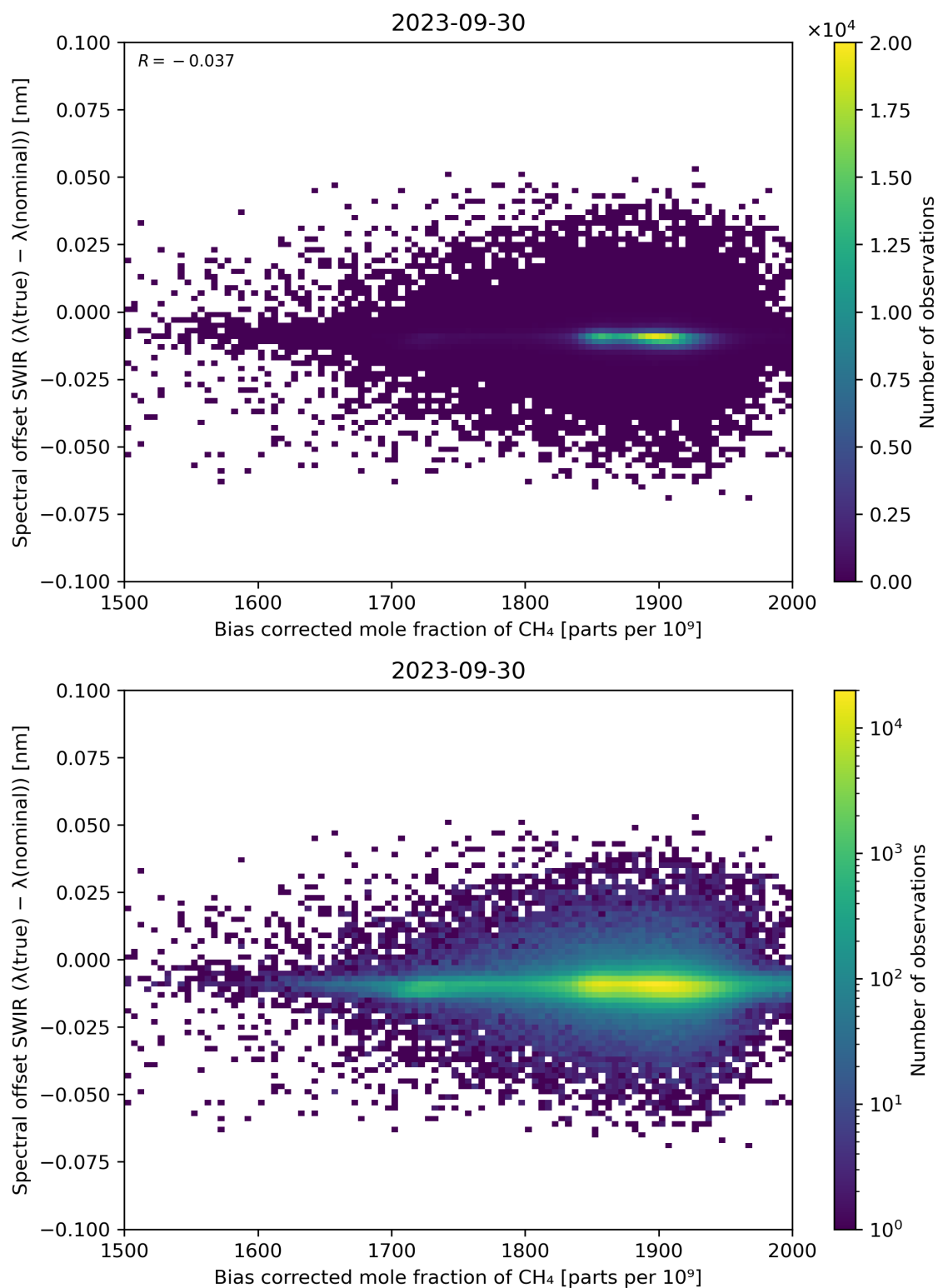
Figure 69: Scatter density plot of “Bias corrected mole fraction of \text{CH}_4 ” against “Spectral offset SWIR ( \lambda(\text{true}) - \lambda(\text{nominal}) )” for 2023-09-29 to 2023-10-01.
