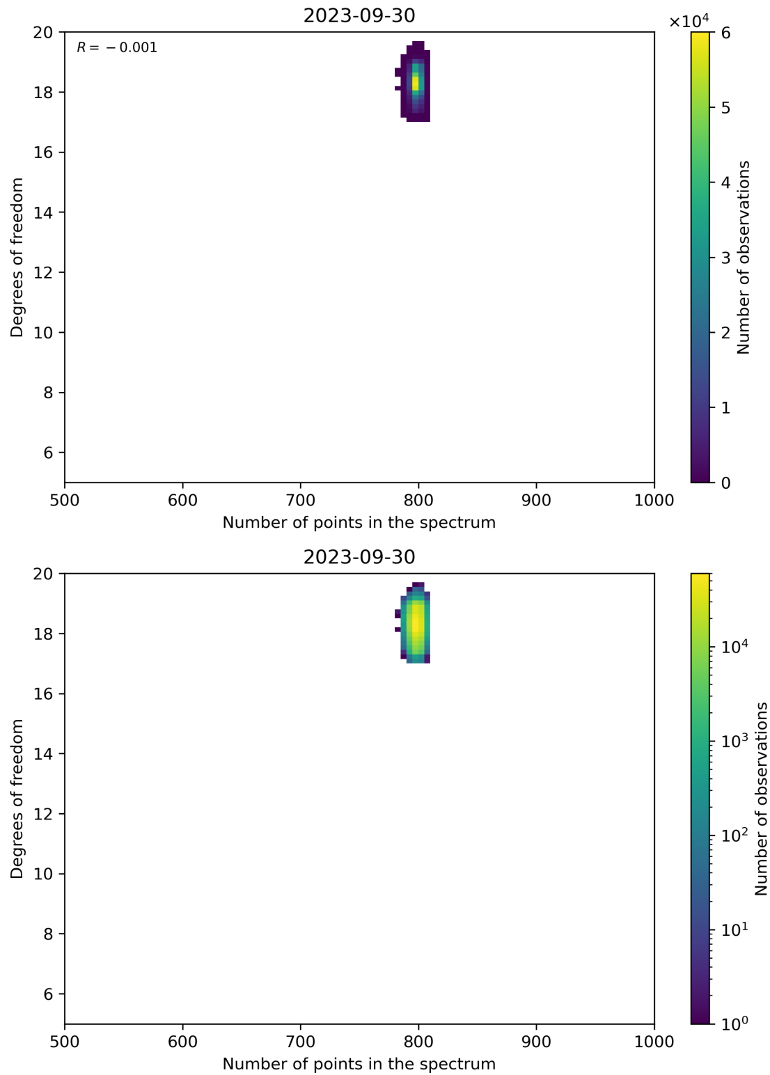
Figure 90: Scatter density plot of “Number of points in the spectrum” against “Degrees of freedom” for 2023-09-29 to 2023-10-01.
