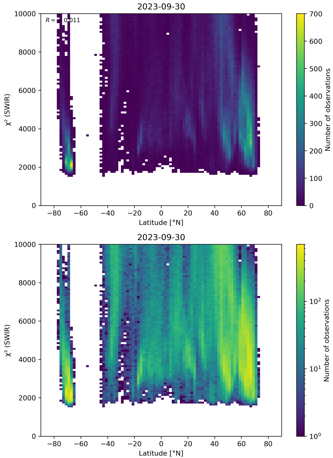
Figure 54: Scatter density plot of “Latitude” against “ \chi^2 (SWIR)” for 2023-09-29 to 2023-10-01.
