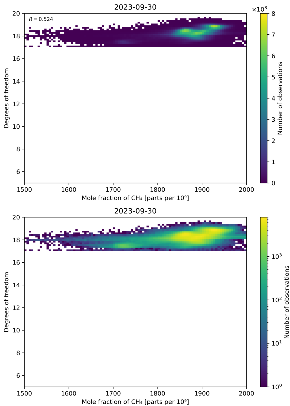
Figure 72: Scatter density plot of “Mole fraction of CH 4 ” against “Degrees of freedom” for 2023-09-29 to 2023-10-01.
