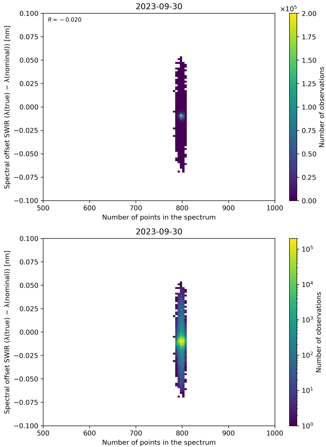
Figure 93: Scatter density plot of “Number of points in the spectrum” against “Spectral offset SWIR ( \lambda(\text{true}) - \lambda(\text{nominal}) )” for 2023-09-29 to 2023-10-01.
