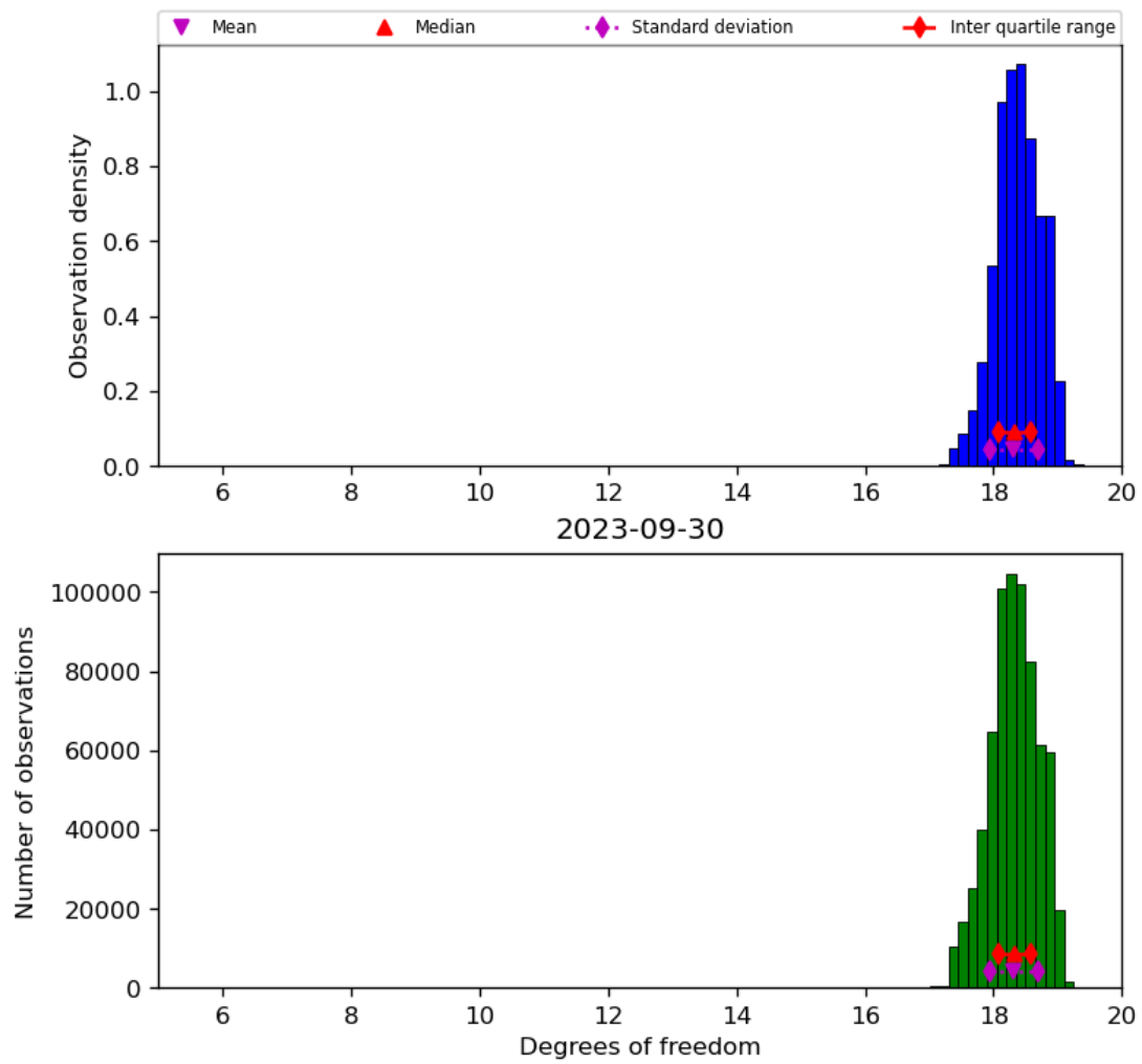
Figure 30: Histogram of “Degrees of freedom” for 2023-09-29 to 2023-10-01
