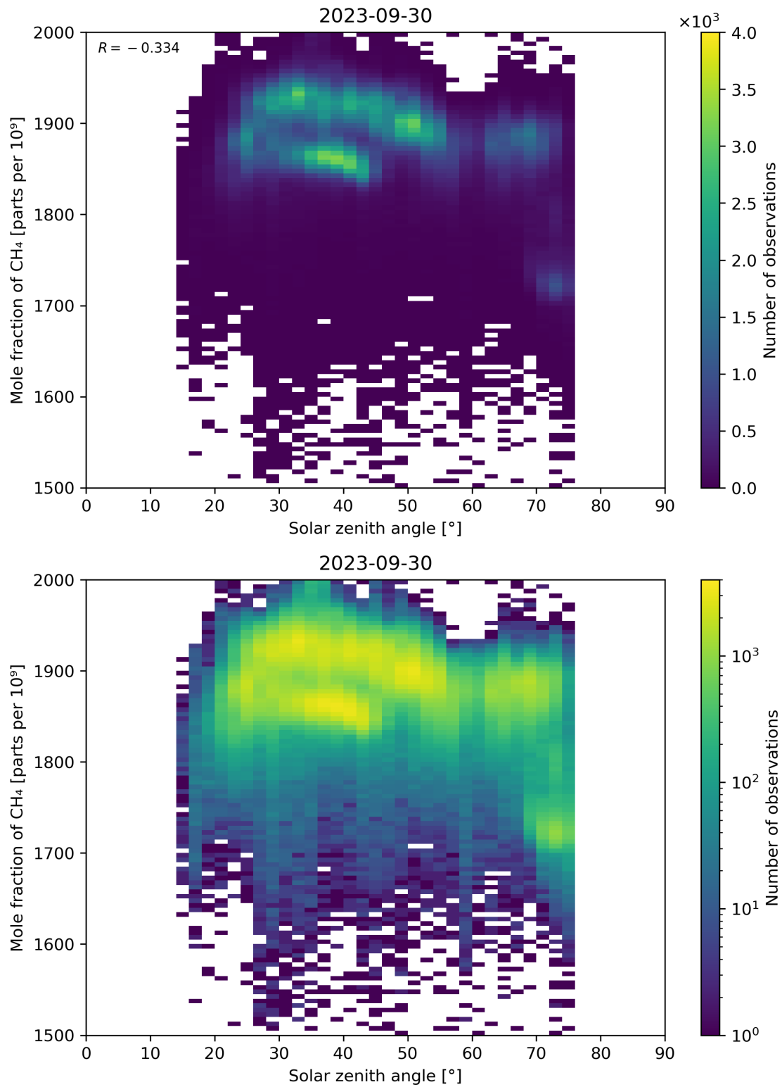
Figure 99: Scatter density plot of “Solar zenith angle” against “Mole fraction of CH 4 ” for 2023-09-29 to 2023-10-01.
