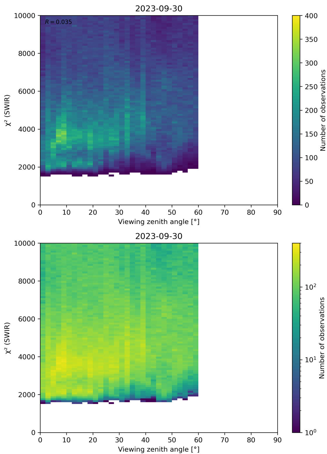
Figure 106: Scatter density plot of “Viewing zenith angle” against “ \chi^2 (SWIR)” for 2023-09-29 to 2023-10-01.
