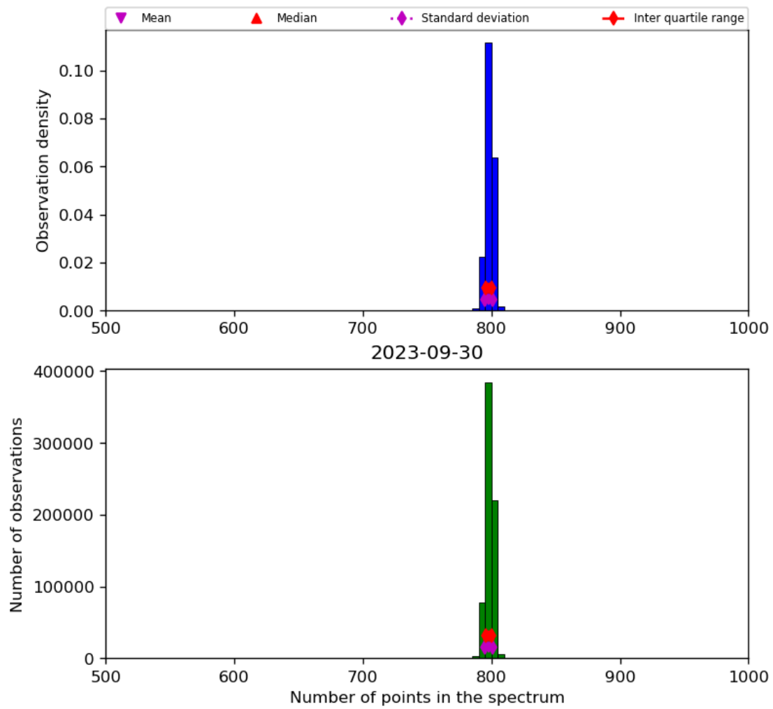
Figure 26: Histogram of “Number of points in the spectrum” for 2023-09-29 to 2023-10-01
