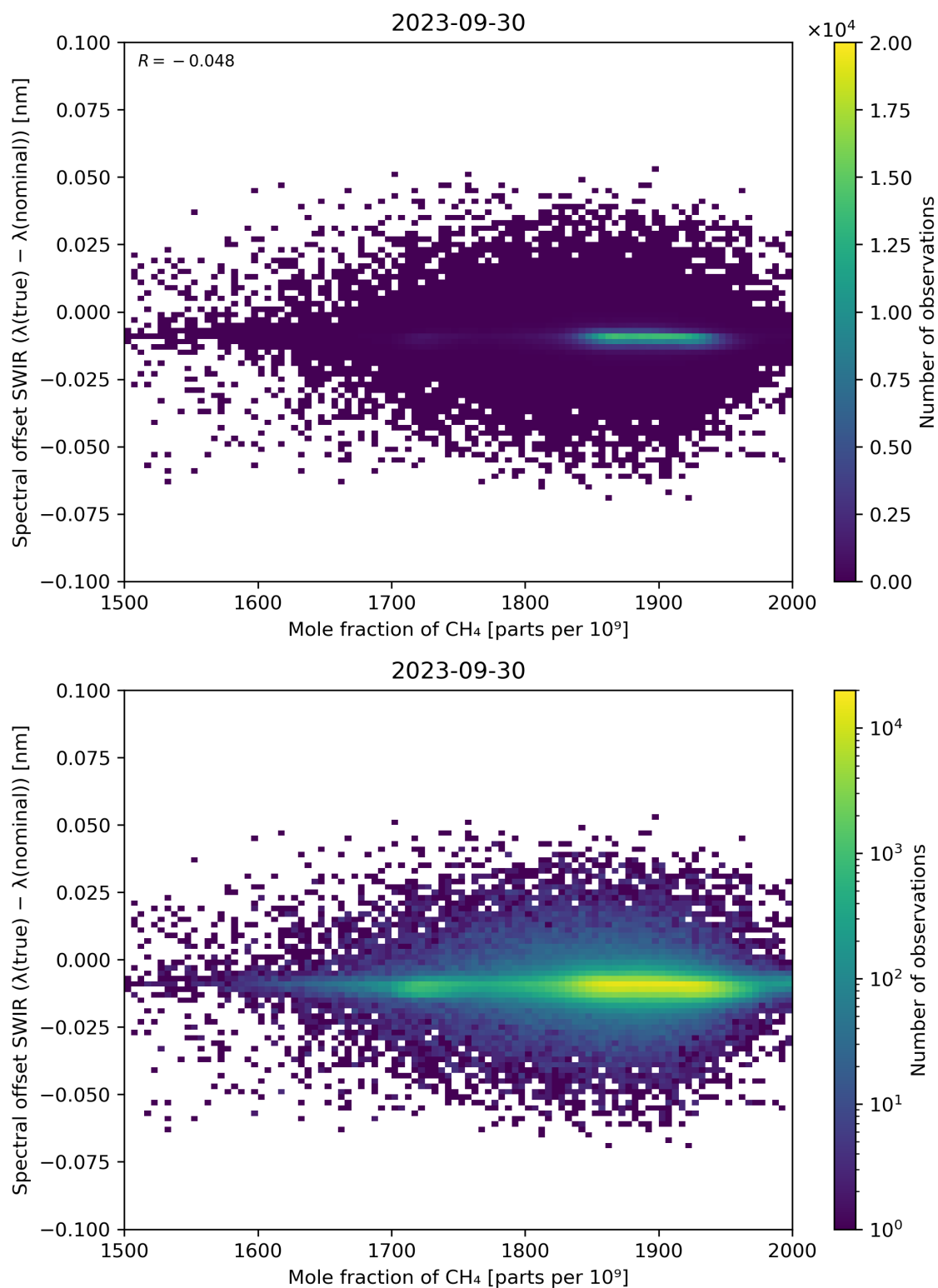
Figure 86: Scatter density plot of “Mole fraction of CH 4 ” against “Spectral offset SWIR ( \lambda(\text{true}) - \lambda(\text{nominal}) )” for 2023-09-29 to 2023-10-01.
