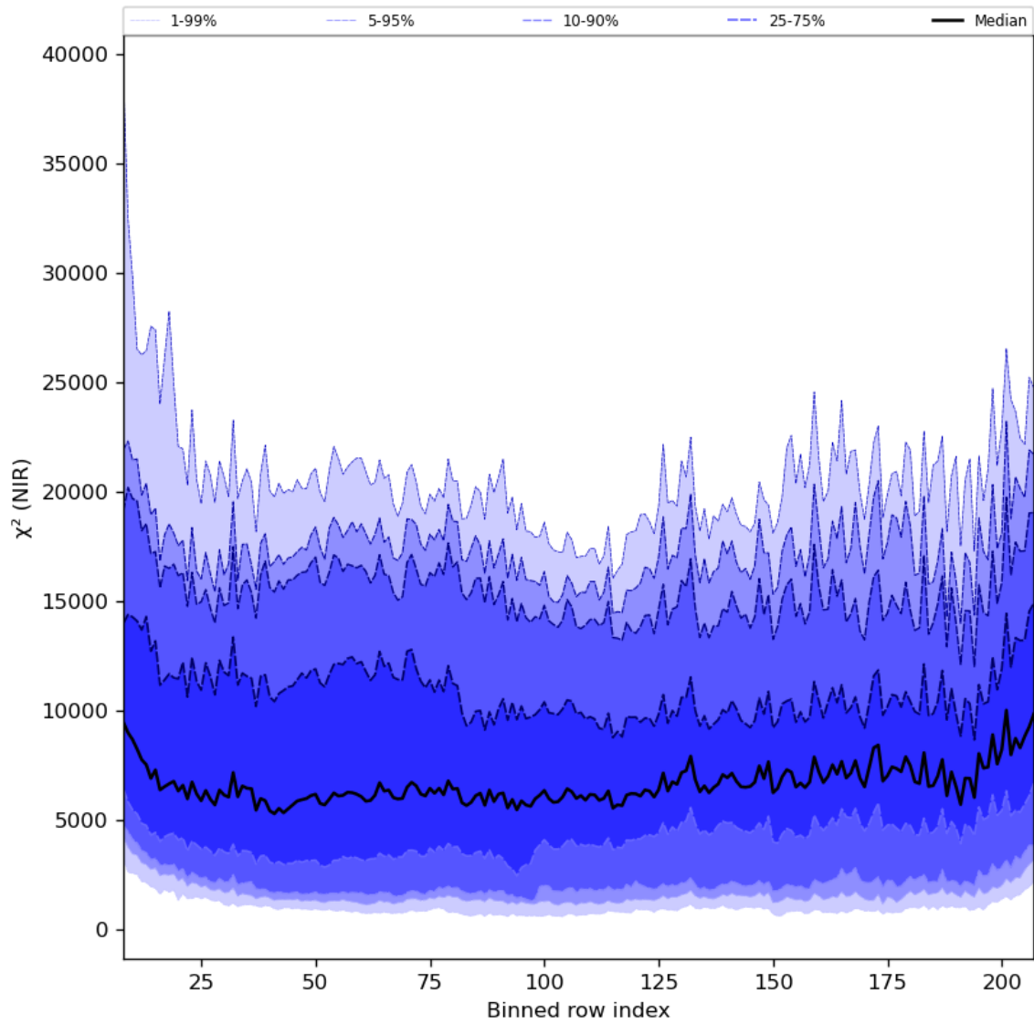
Figure 40: Along track statistics of “ \chi^2 (NIR)” for 2023-09-29 to 2023-10-01
