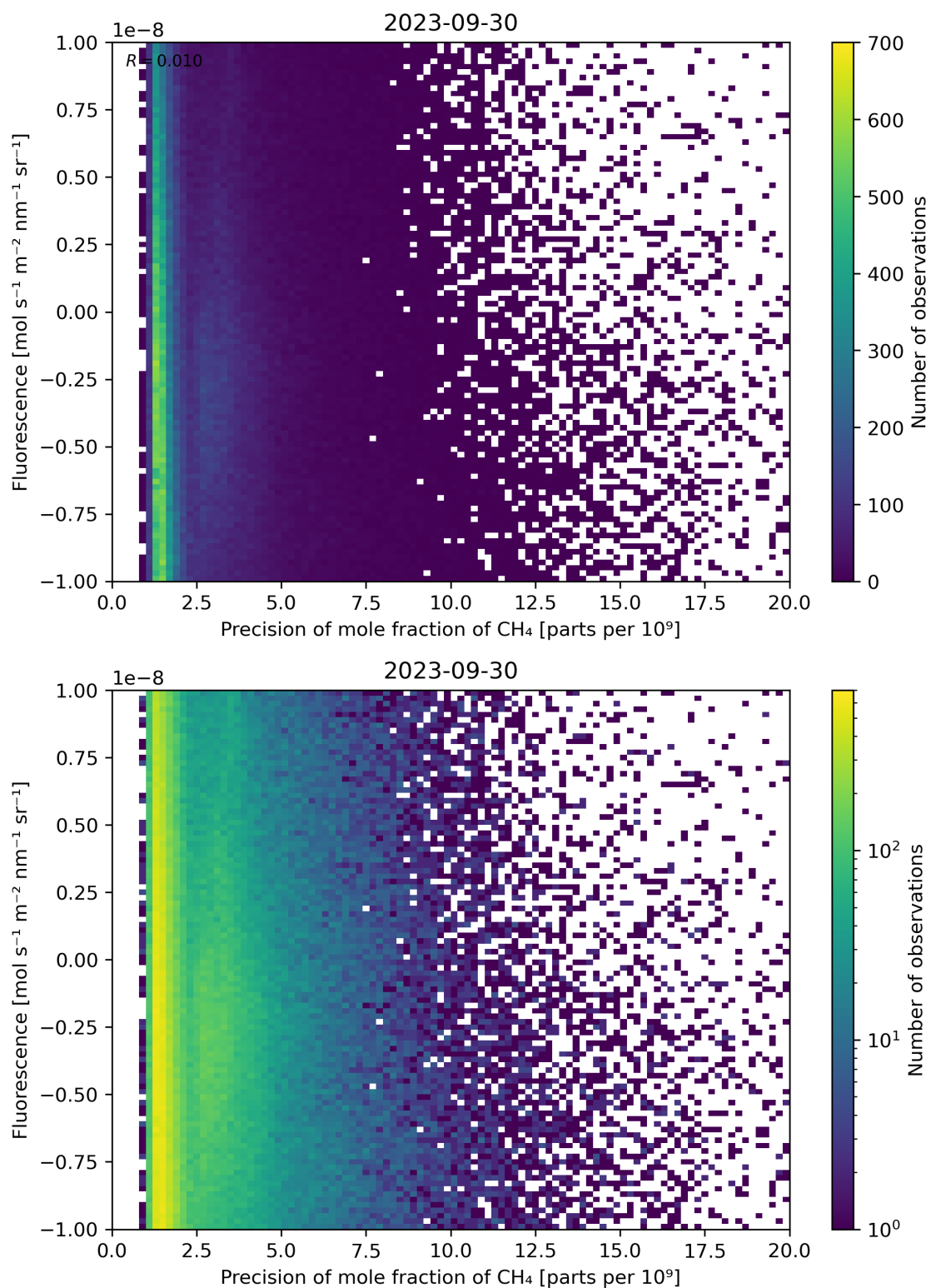
Figure 81: Scatter density plot of “Precision of mole fraction of \text{CH}_4 ” against “Fluorescence” for 2023-09-29 to 2023-10-01.
