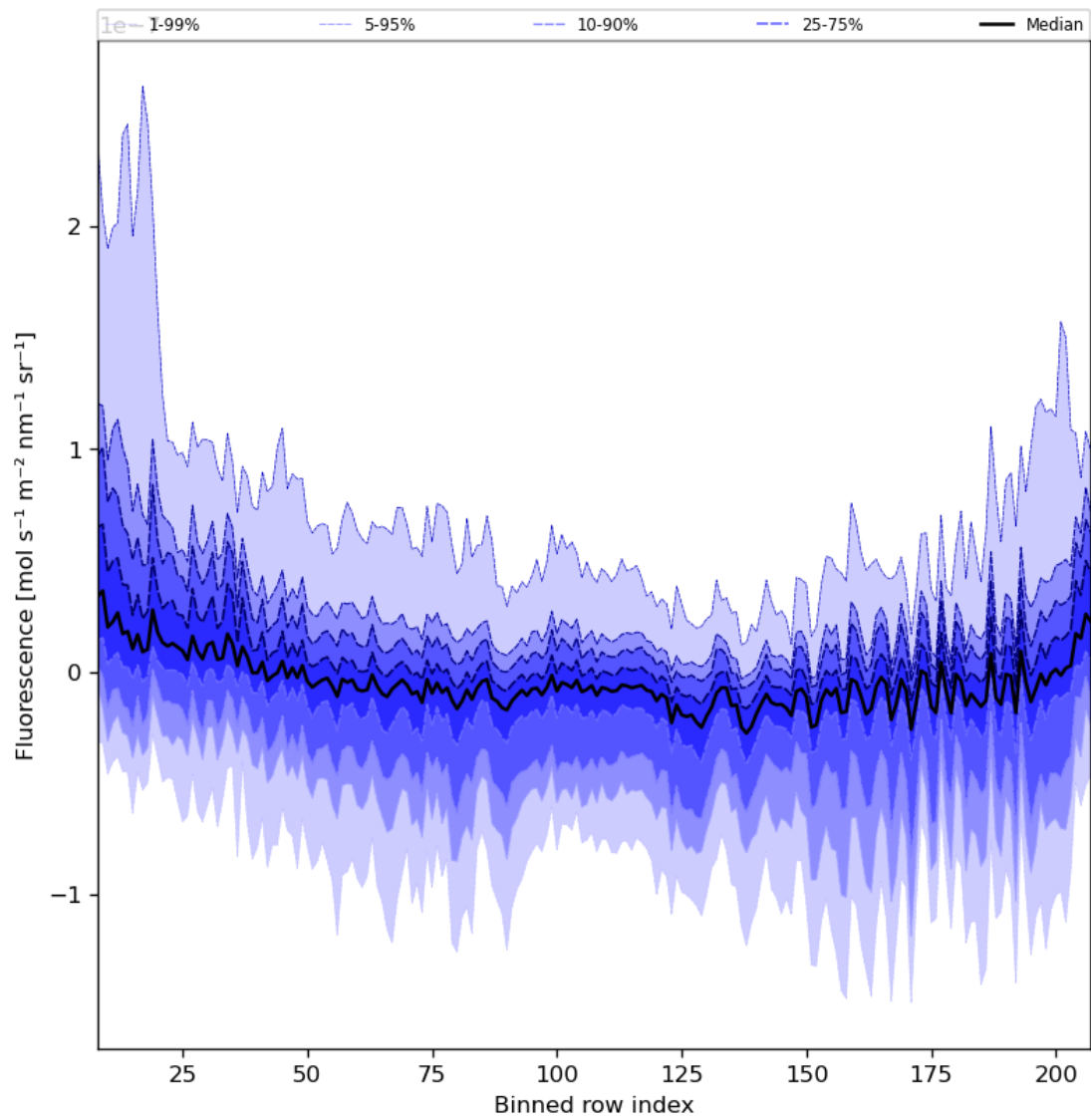
Figure 43: Along track statistics of "Fluorescence" for 2023-09-29 to 2023-10-01
