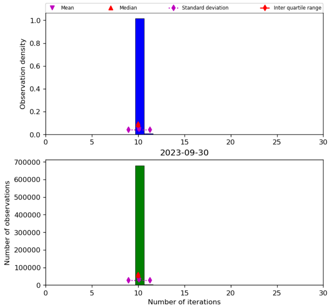
Figure 31: Histogram of “Number of iterations” for 2023-09-29 to 2023-10-01
