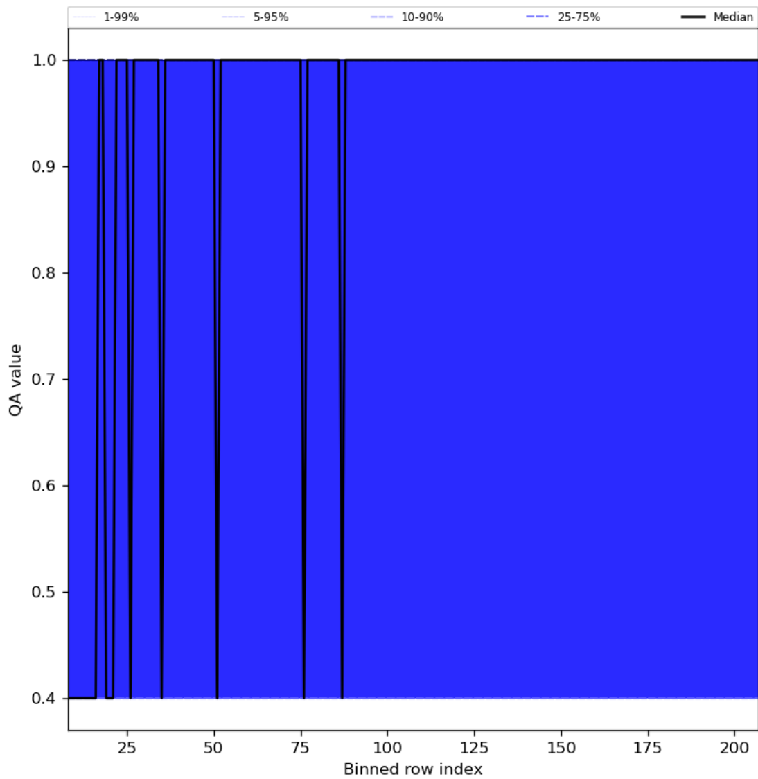
Figure 33: Along track statistics of “QA value” for 2023-09-29 to 2023-10-01
