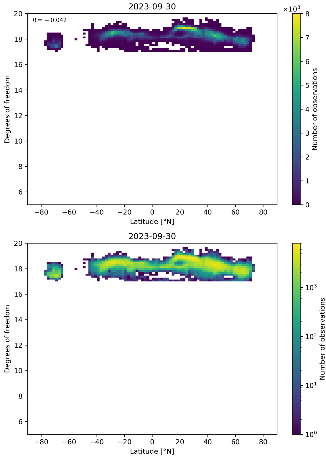
Figure 55: Scatter density plot of “Latitude” against “Degrees of freedom” for 2023-09-29 to 2023-10-01.
