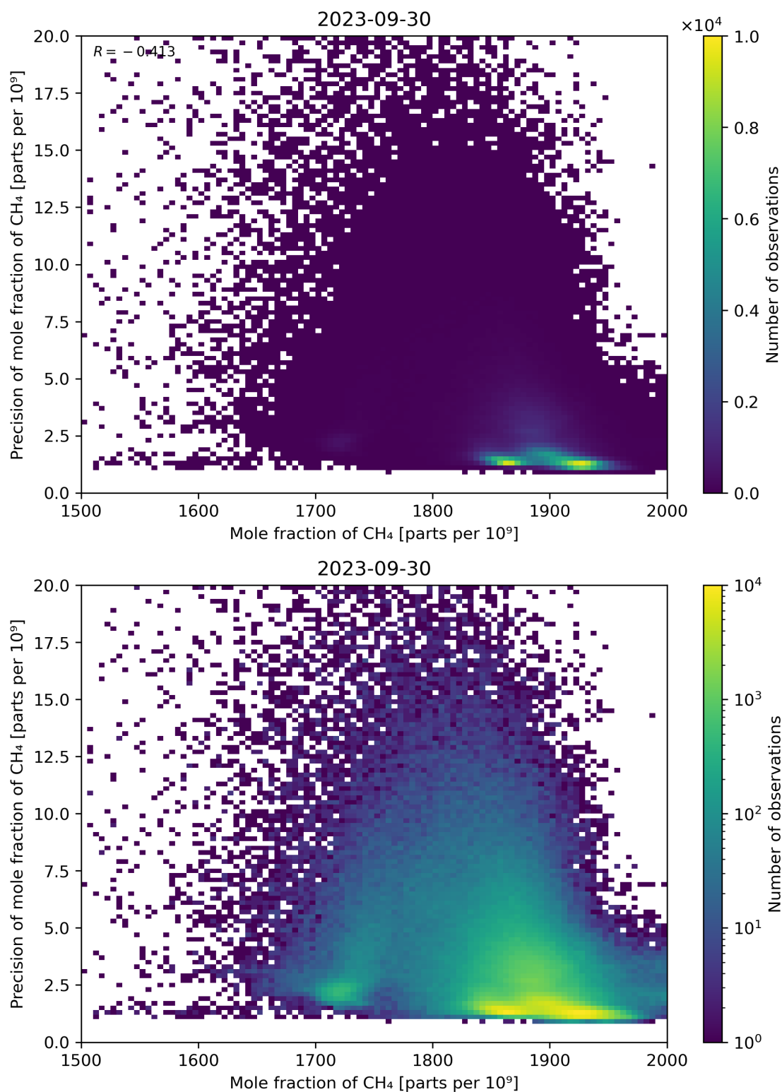
Figure 75: Scatter density plot of “Mole fraction of CH 4 ” against “Precision of mole fraction of CH 4 ” for 2023-09-29 to 2023-10-01.
