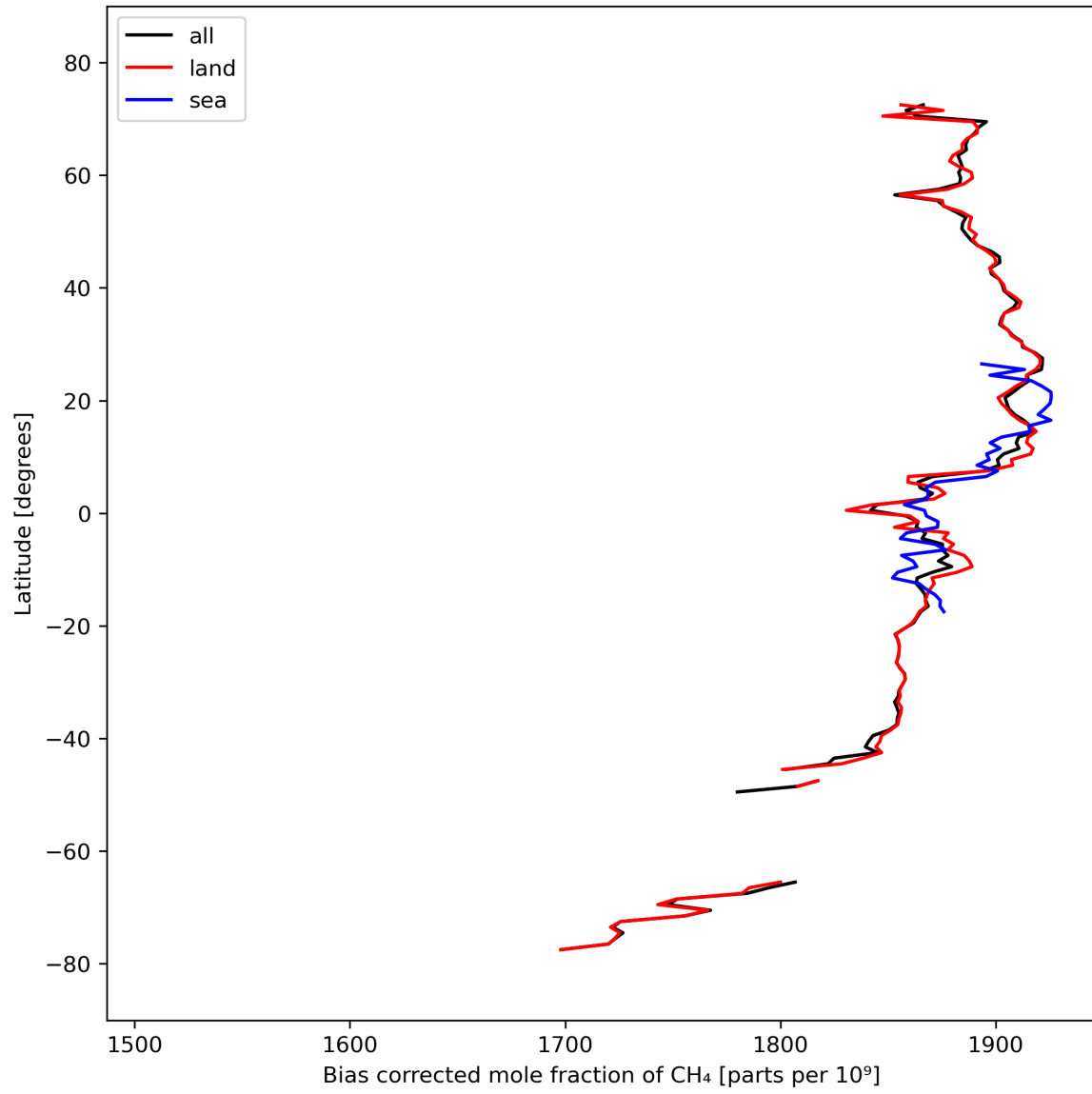
Figure 14: Zonal average of “Bias corrected mole fraction of \text{CH}_4 ” for 2023-09-29 to 2023-10-01.
