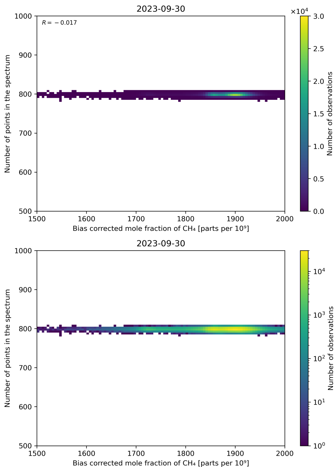
Figure 68: Scatter density plot of “Bias corrected mole fraction of CH 4 ” against “Number of points in the spectrum” for 2023-09-29 to 2023-10-01.
