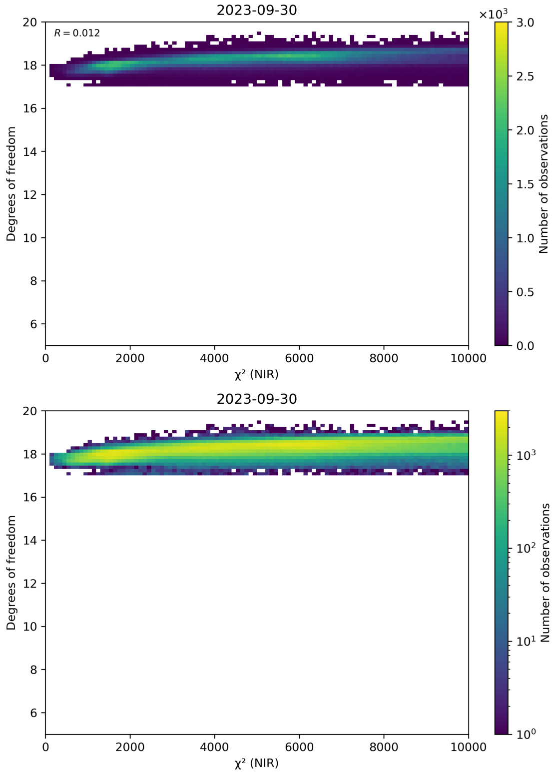
Figure 44: Scatter density plot of “ \chi^2 (NIR)” against “Degrees of freedom” for 2023-09-29 to 2023-10-01.
