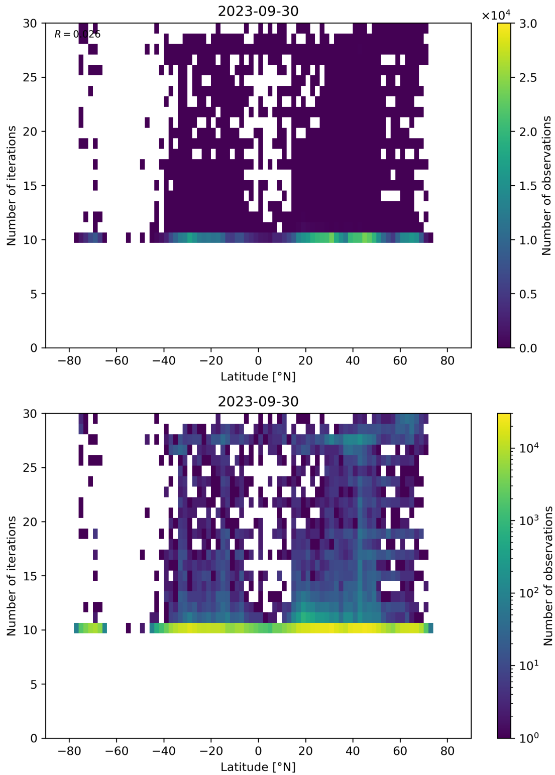
Figure 60: Scatter density plot of “Latitude” against “Number of iterations” for 2023-09-29 to 2023-10-01.
