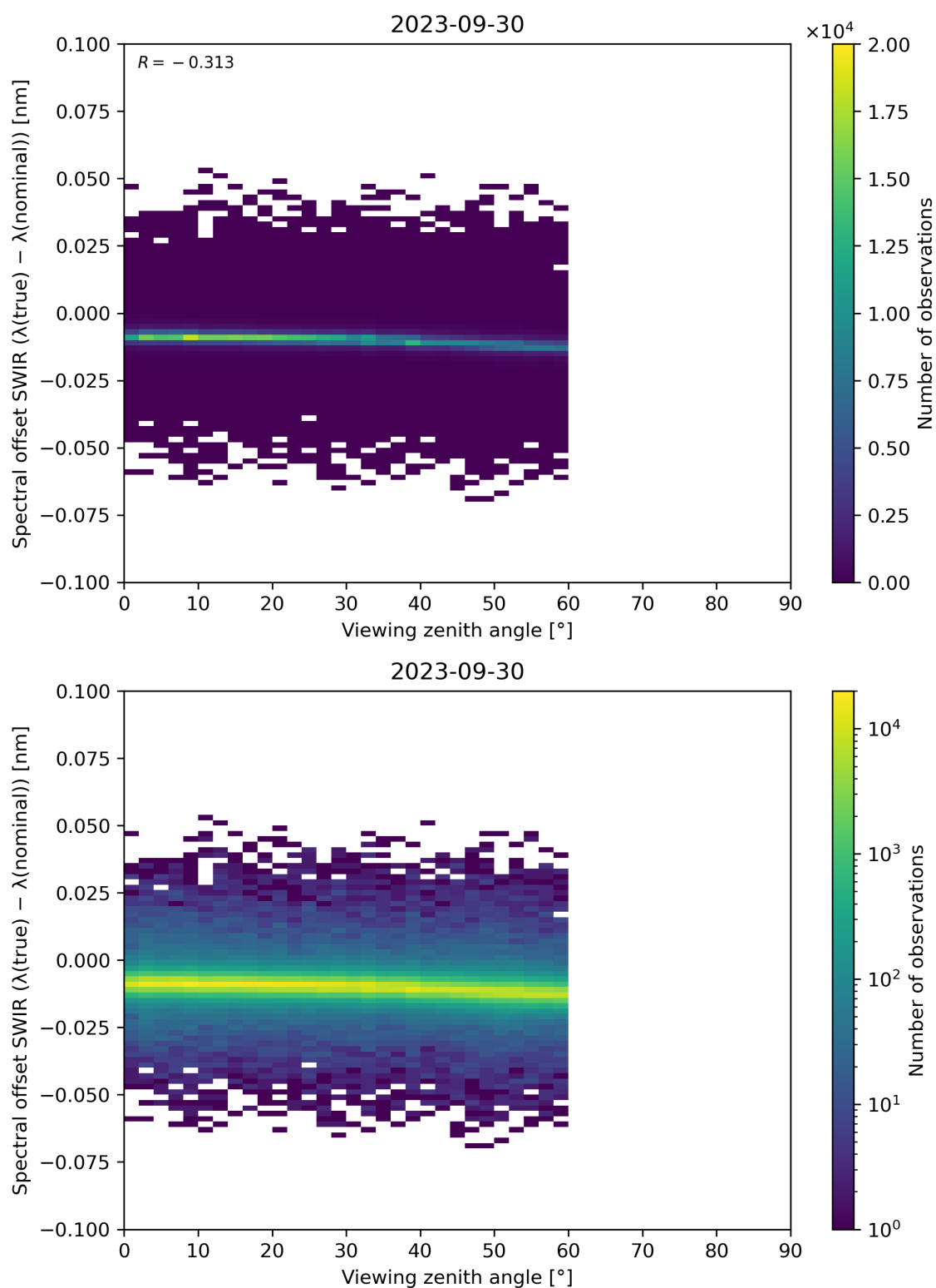
Figure 116: Scatter density plot of “Viewing zenith angle” against “Spectral offset SWIR ( \lambda(\text{true}) - \lambda(\text{nominal}) )” for 2023-09-29 to 2023-10-01.
