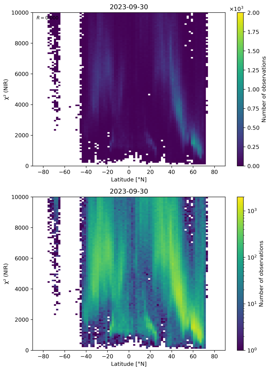
Figure 53: Scatter density plot of “Latitude” against “ \chi^2 (NIR)” for 2023-09-29 to 2023-10-01.
