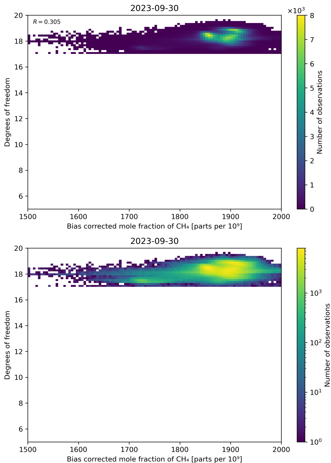
Figure 65: Scatter density plot of “Bias corrected mole fraction of CH 4 ” against “Degrees of freedom” for 2023-09-29 to 2023-10-01.
