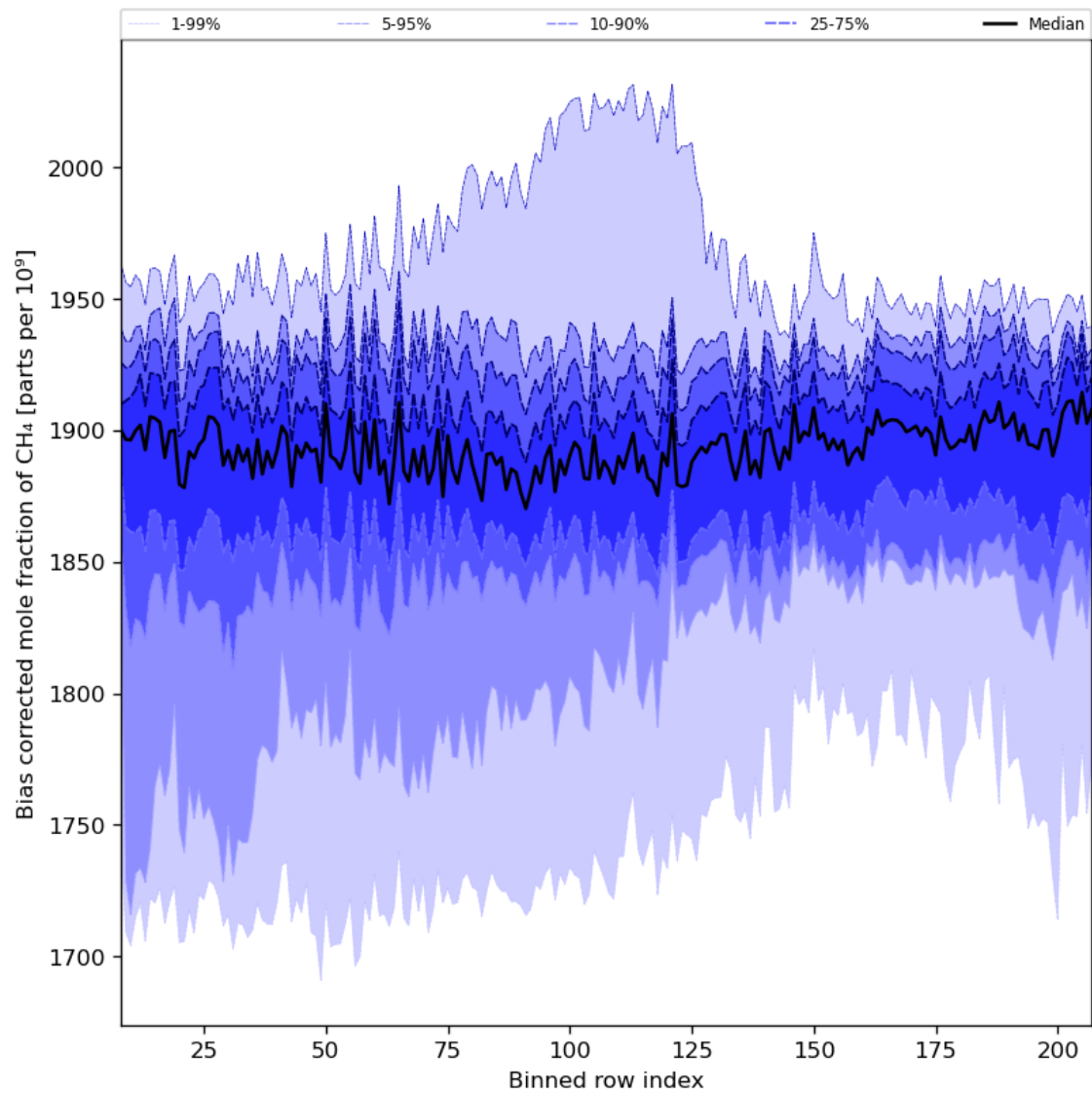
Figure 36: Along track statistics of “Bias corrected mole fraction of CH 4 ” for 2023-09-29 to 2023-10-01
