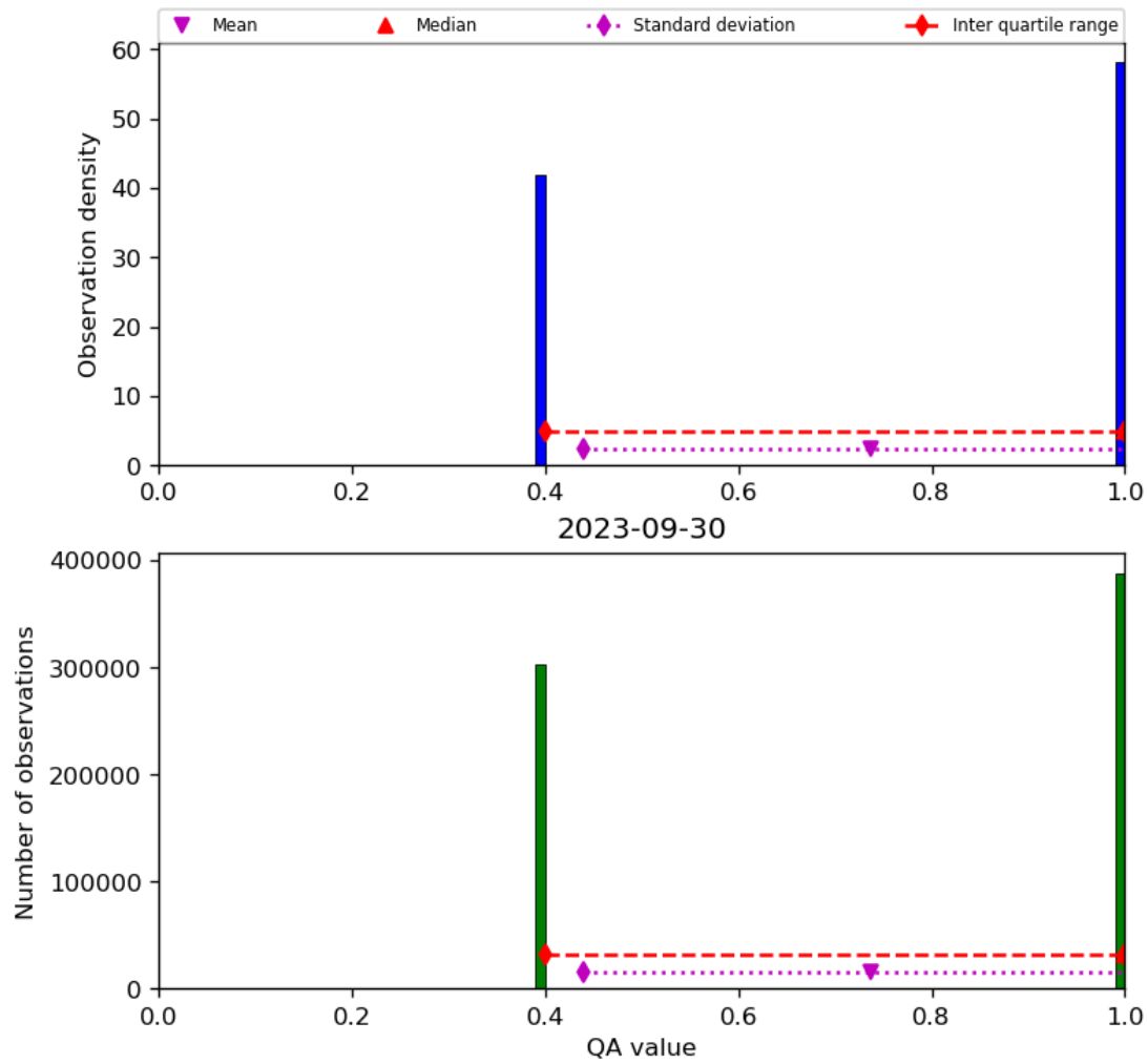
Figure 22: Histogram of “QA value” for 2023-09-29 to 2023-10-01
