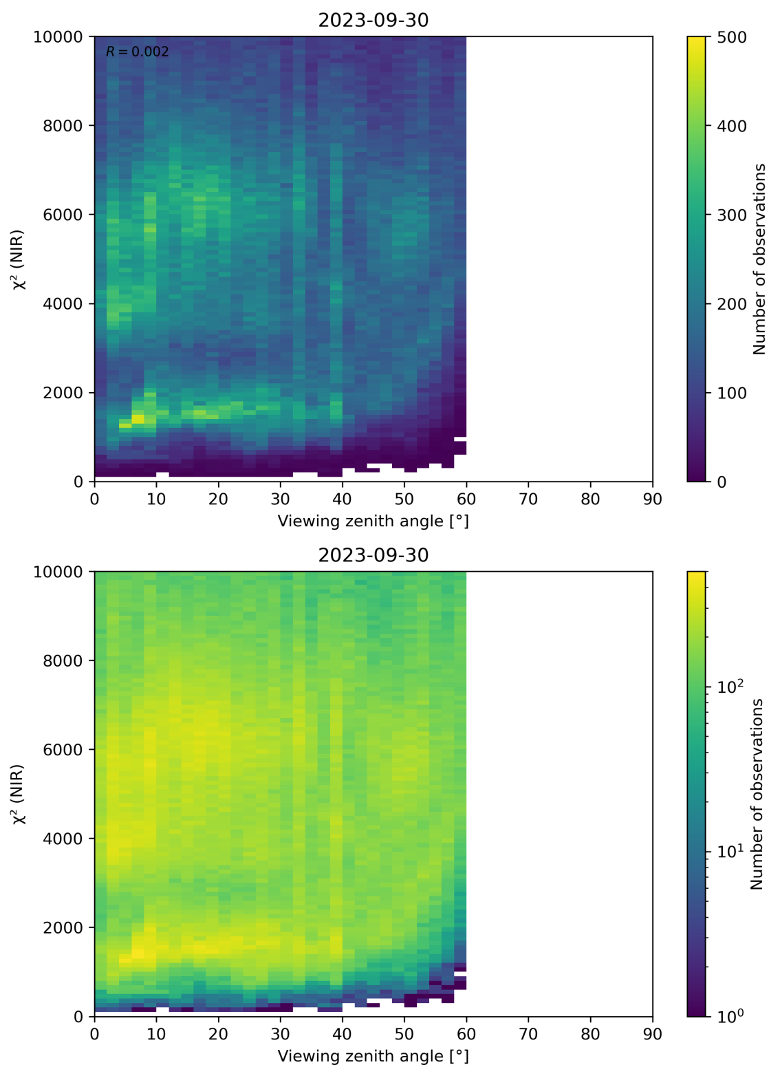
Figure 105: Scatter density plot of “Viewing zenith angle” against “ \chi^2 (NIR)” for 2023-09-29 to 2023-10-01.
