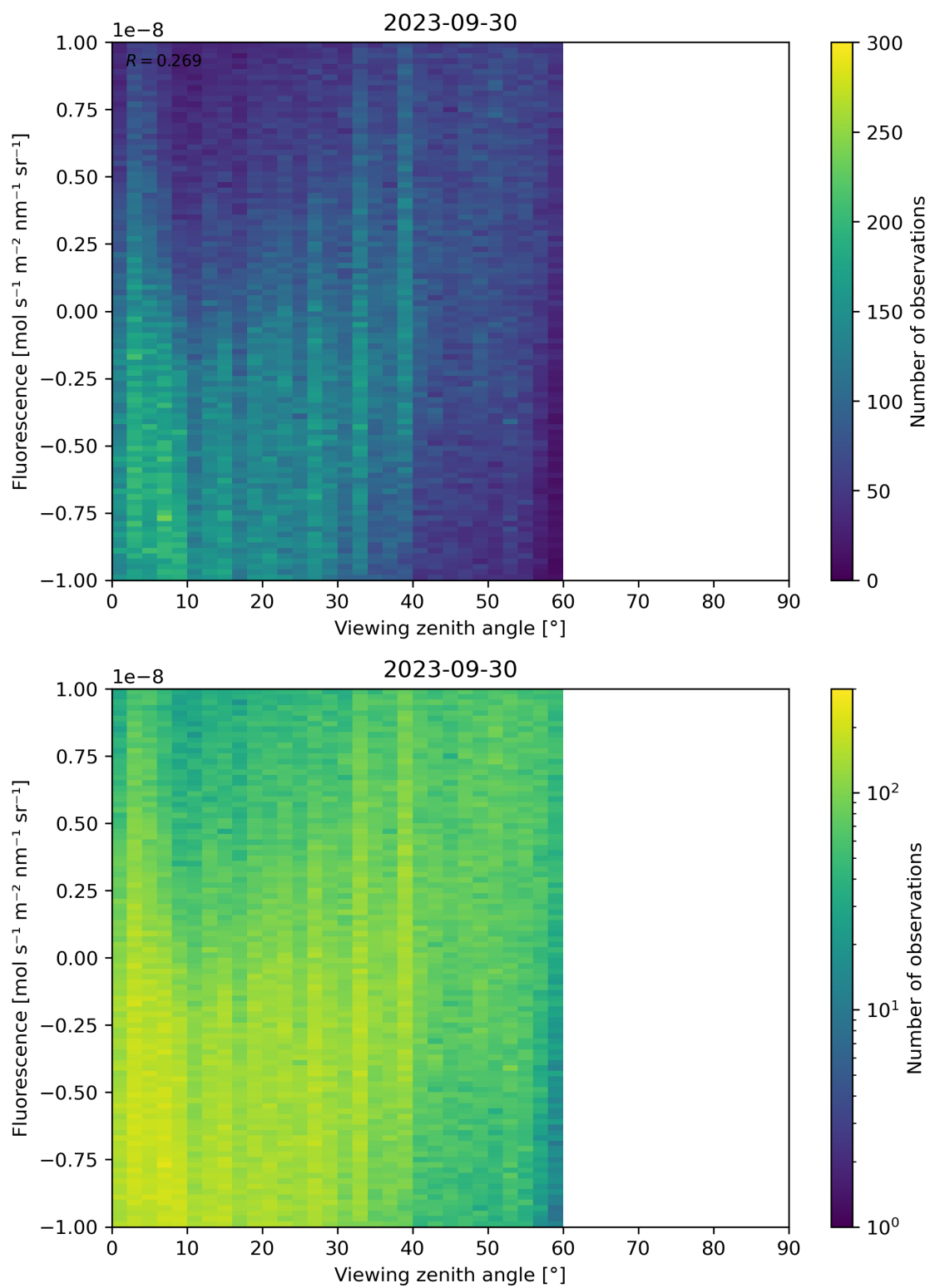
Figure 108: Scatter density plot of “Viewing zenith angle” against “Fluorescence” for 2023-09-29 to 2023-10-01.
