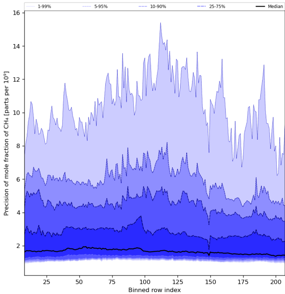
Figure 35: Along track statistics of “Precision of mole fraction of CH 4 ” for 2023-09-29 to 2023-10-01
