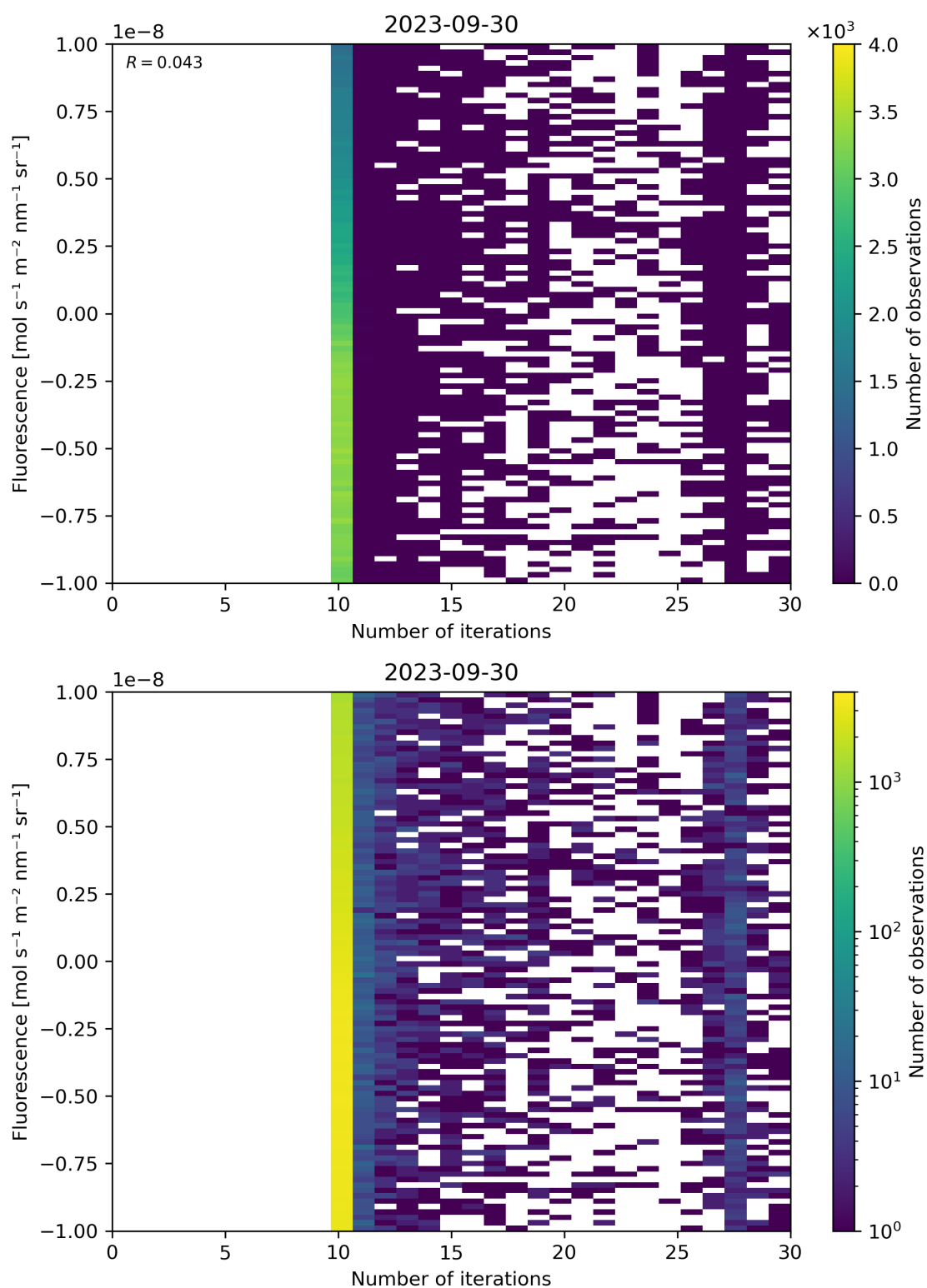
Figure 87: Scatter density plot of “Number of iterations” against “Fluorescence” for 2023-09-29 to 2023-10-01.
