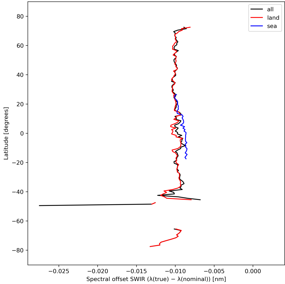
Figure 16: Zonal average of “Spectral offset SWIR ( \lambda(\text{true}) - \lambda(\text{nominal}) )” for 2023-09-29 to 2023-10-01.
