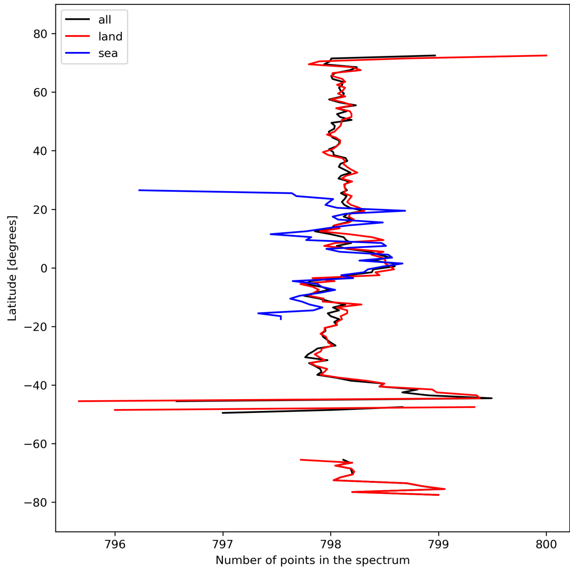
Figure 15: Zonal average of “Number of points in the spectrum” for 2023-09-29 to 2023-10-01.
