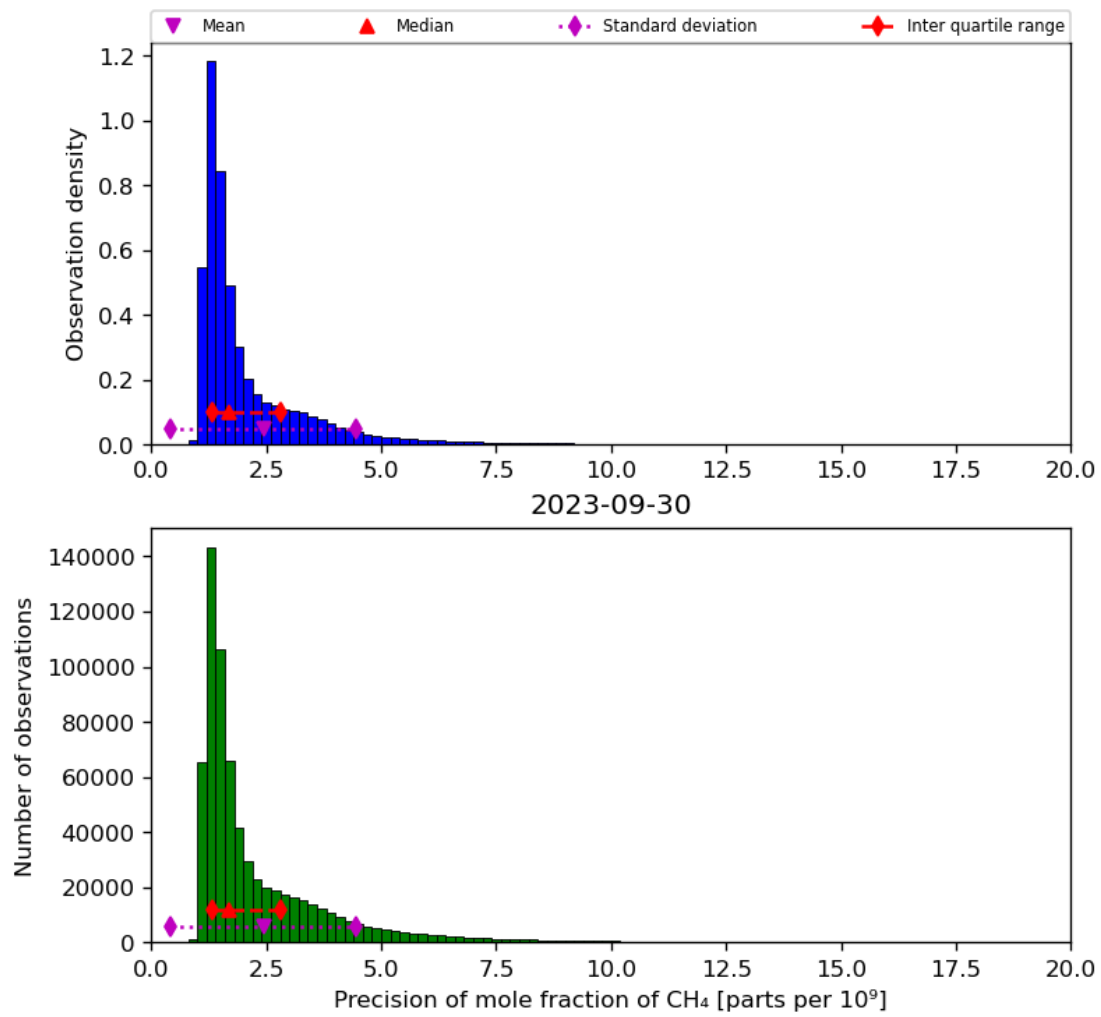
Figure 24: Histogram of “Precision of mole fraction of CH 4 ” for 2023-09-29 to 2023-10-01
