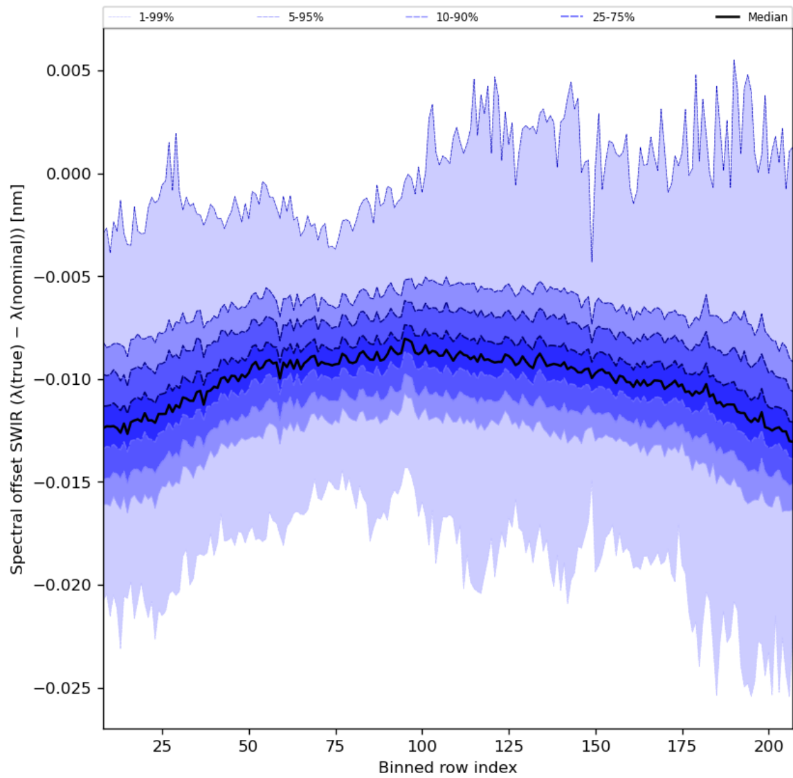
Figure 38: Along track statistics of “Spectral offset SWIR ( \lambda(\text{true}) - \lambda(\text{nominal}) )” for 2023-09-29 to 2023-10-01
