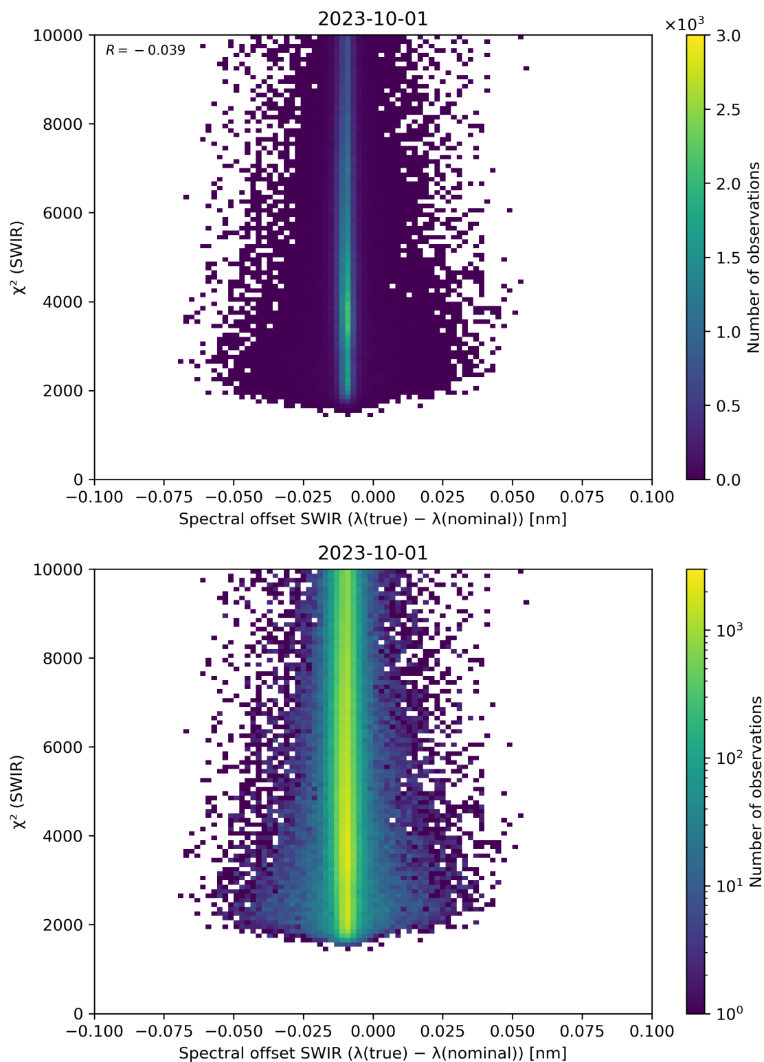
Figure 118: Scatter density plot of “Spectral offset SWIR ( \lambda(\text{true}) - \lambda(\text{nominal}) )” against “ \chi^2 (SWIR)” for 2023-10-01 to 2023-10-02.
