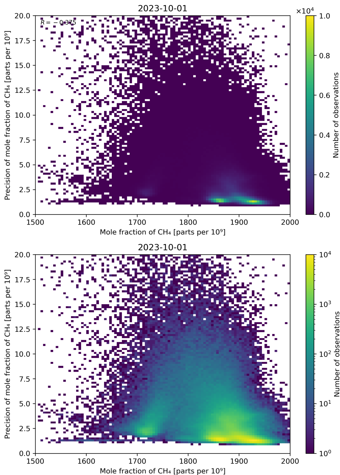
Figure 75: Scatter density plot of “Mole fraction of CH 4 ” against “Precision of mole fraction of CH 4 ” for 2023-10-01 to 2023-10-02.
