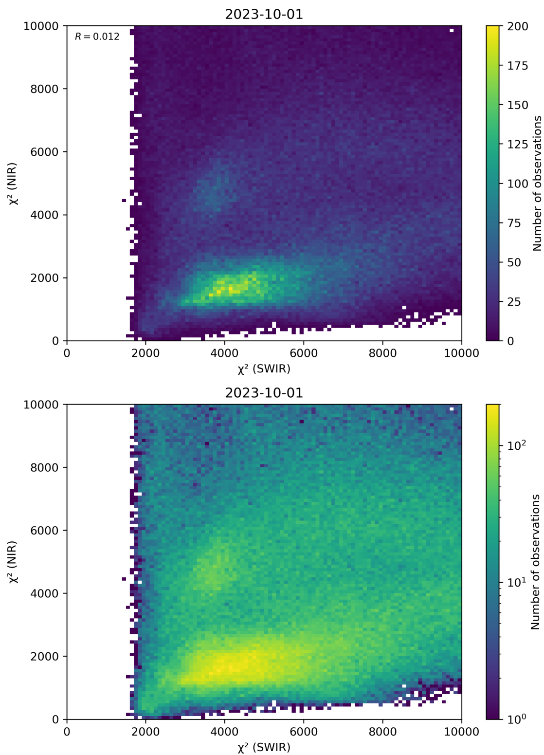
Figure 47: Scatter density plot of “ \chi^2 (SWIR)” against “ \chi^2 (NIR)” for 2023-10-01 to 2023-10-02.
