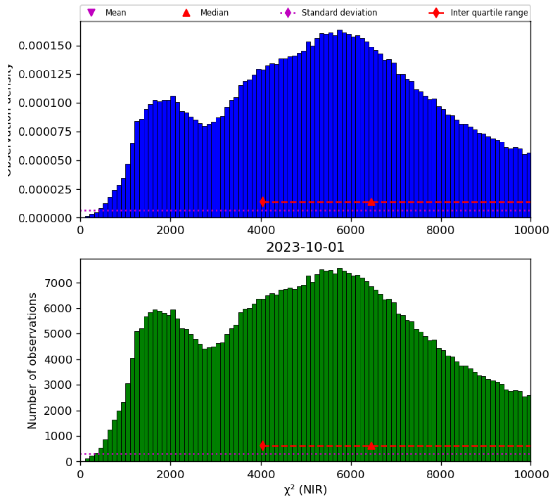
Figure 29: Histogram of “ \chi^2 (NIR)” for 2023-10-01 to 2023-10-02
