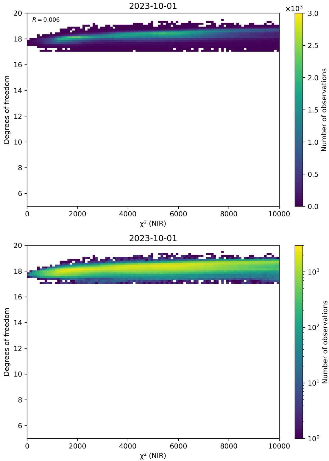
Figure 44: Scatter density plot of “ \chi^2 (NIR)” against “Degrees of freedom” for 2023-10-01 to 2023-10-02.
