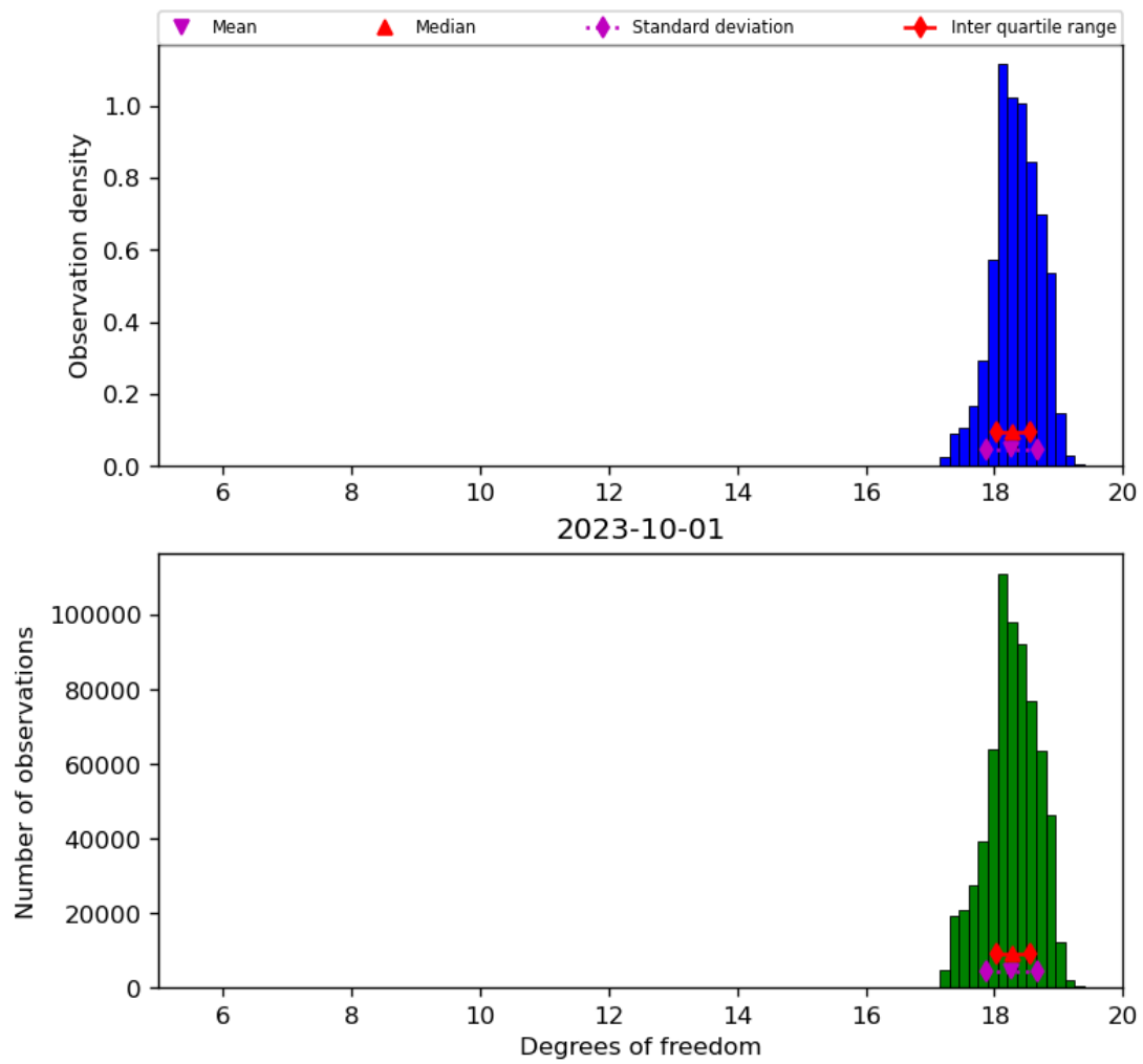
Figure 30: Histogram of “Degrees of freedom” for 2023-10-01 to 2023-10-02
