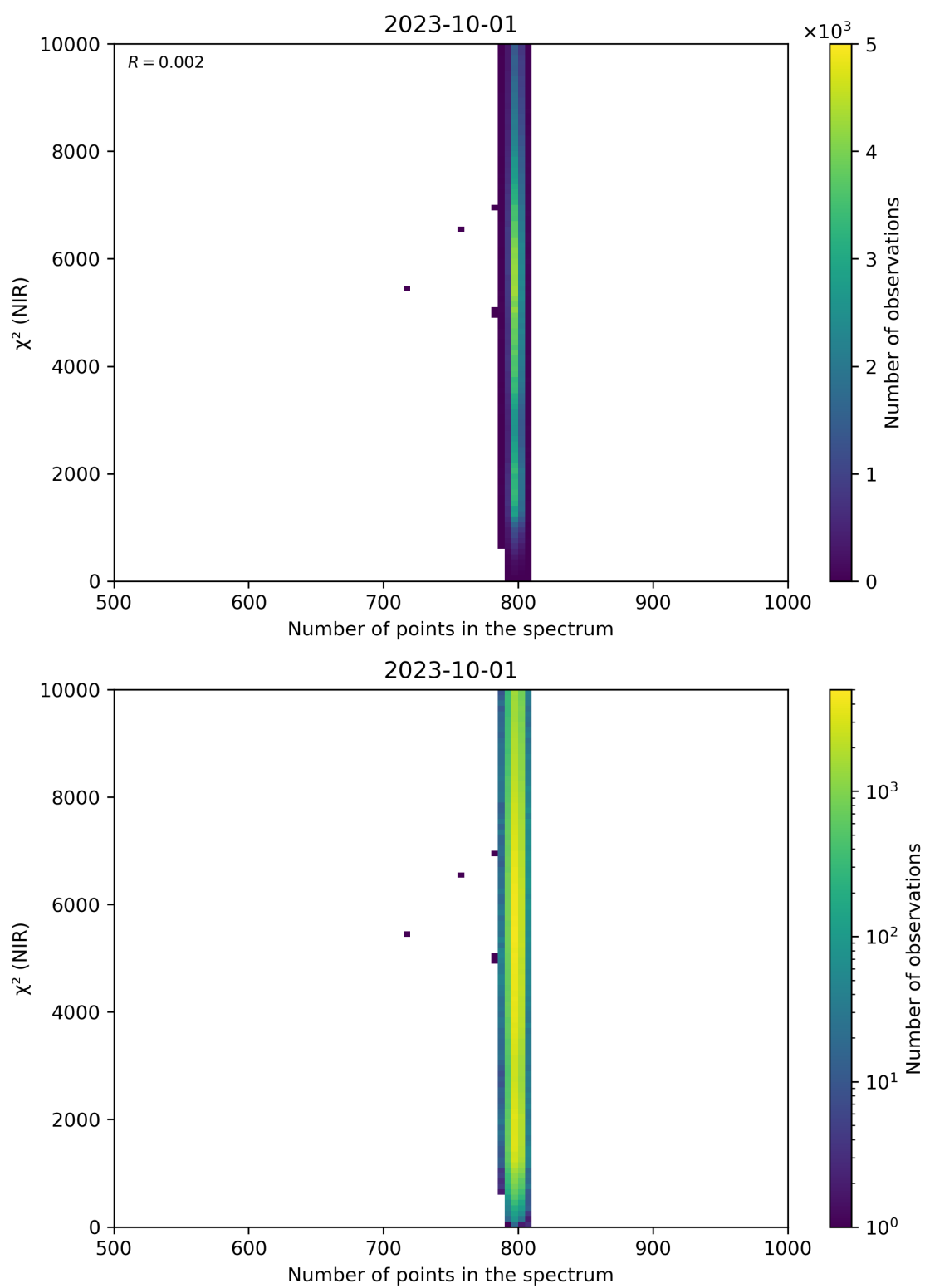
Figure 88: Scatter density plot of “Number of points in the spectrum” against “ \chi^2 (NIR)” for 2023-10-01 to 2023-10-02.
