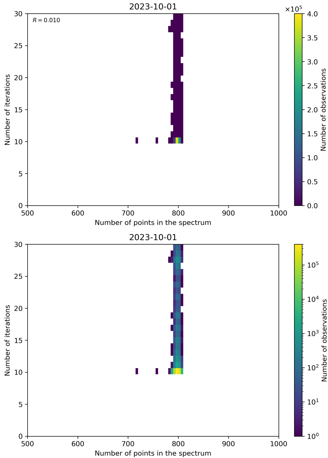
Figure 92: Scatter density plot of “Number of points in the spectrum” against “Number of iterations” for 2023-10-01 to 2023-10-02.
