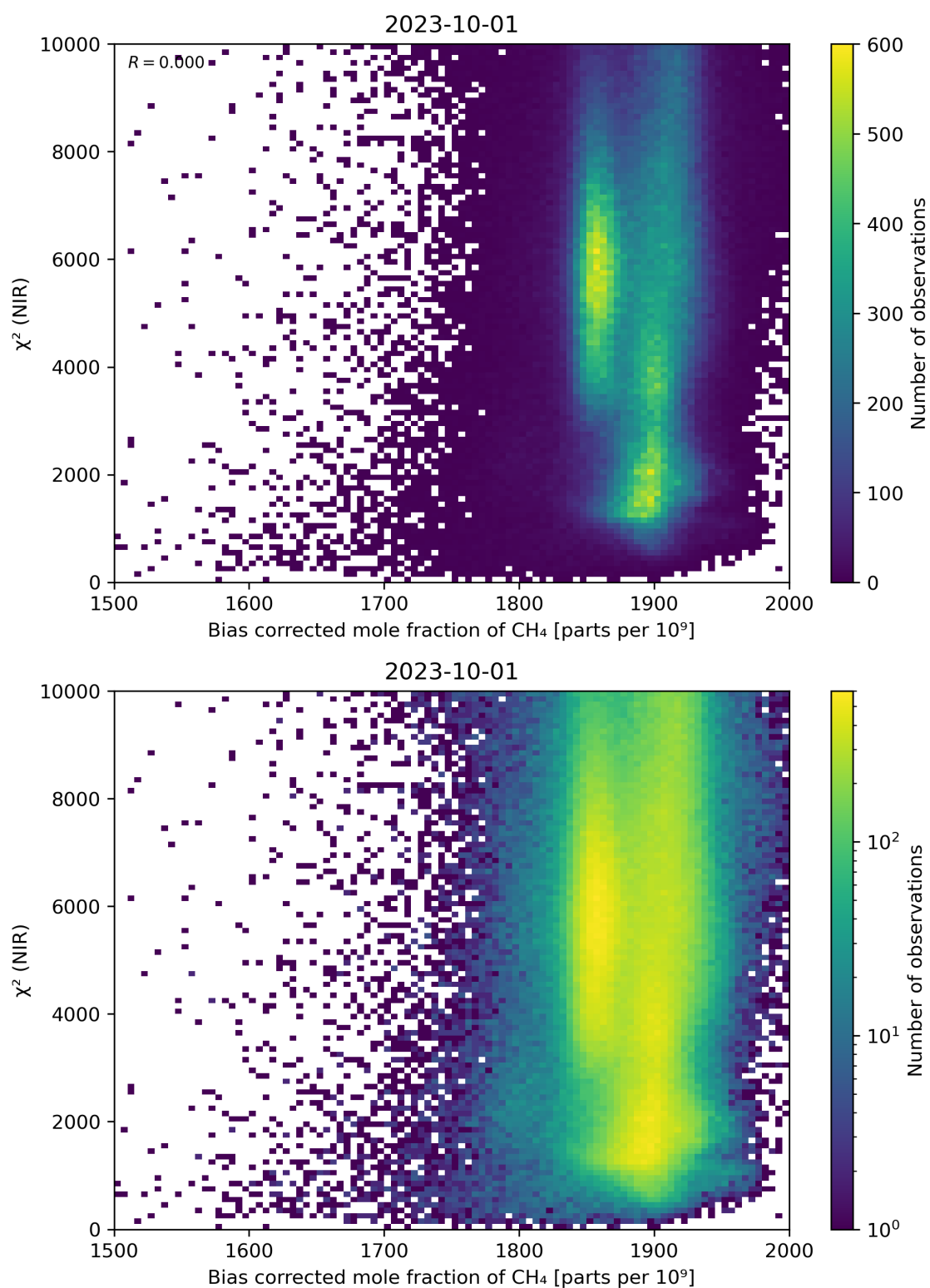
Figure 63: Scatter density plot of “Bias corrected mole fraction of CH 4 ” against “ \chi^2 (NIR)” for 2023-10-01 to 2023-10-02.
