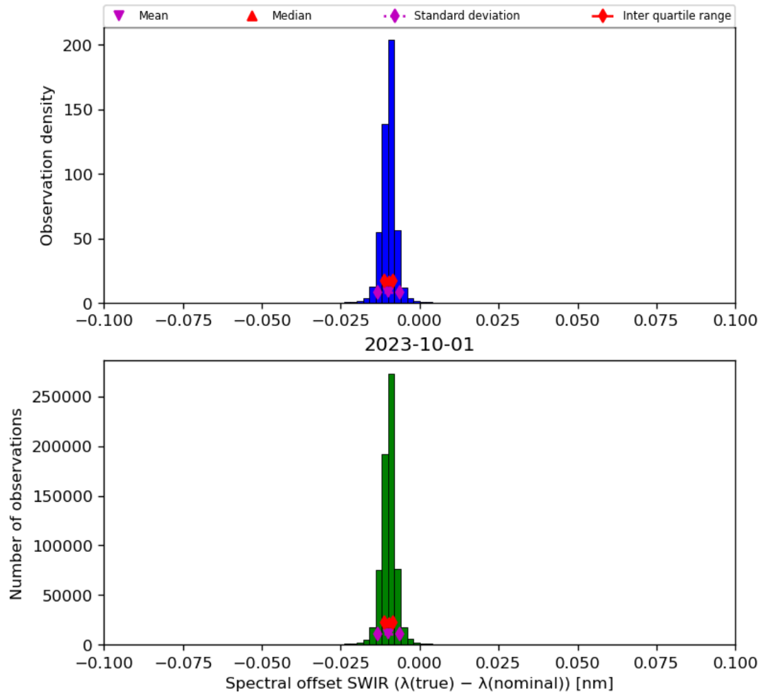
Figure 27: Histogram of “Spectral offset SWIR ( \lambda(\text{true}) - \lambda(\text{nominal}) )” for 2023-10-01 to 2023-10-02
