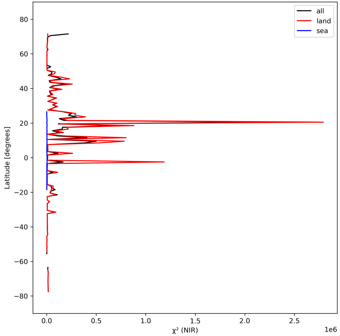
Figure 18: Zonal average of “ \chi^2 (NIR)” for 2023-10-01 to 2023-10-02.
