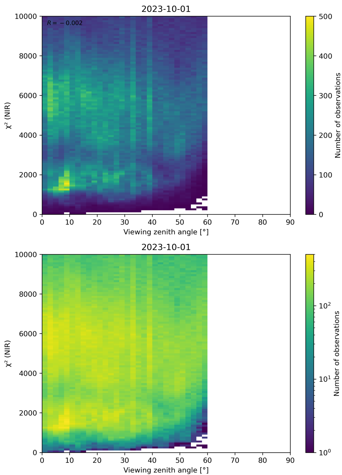
Figure 105: Scatter density plot of “Viewing zenith angle” against “ \chi^2 (NIR)” for 2023-10-01 to 2023-10-02.
