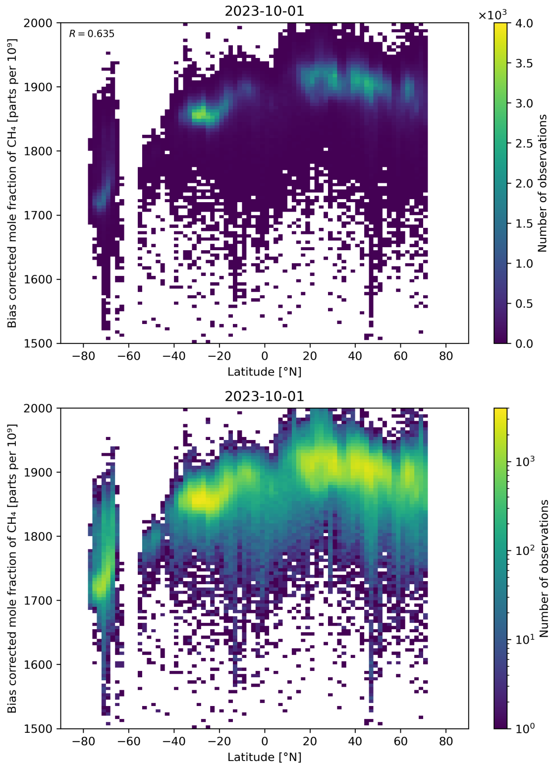
Figure 58: Scatter density plot of “Latitude” against “Bias corrected mole fraction of CH 4 ” for 2023-10-01 to 2023-10-02.
