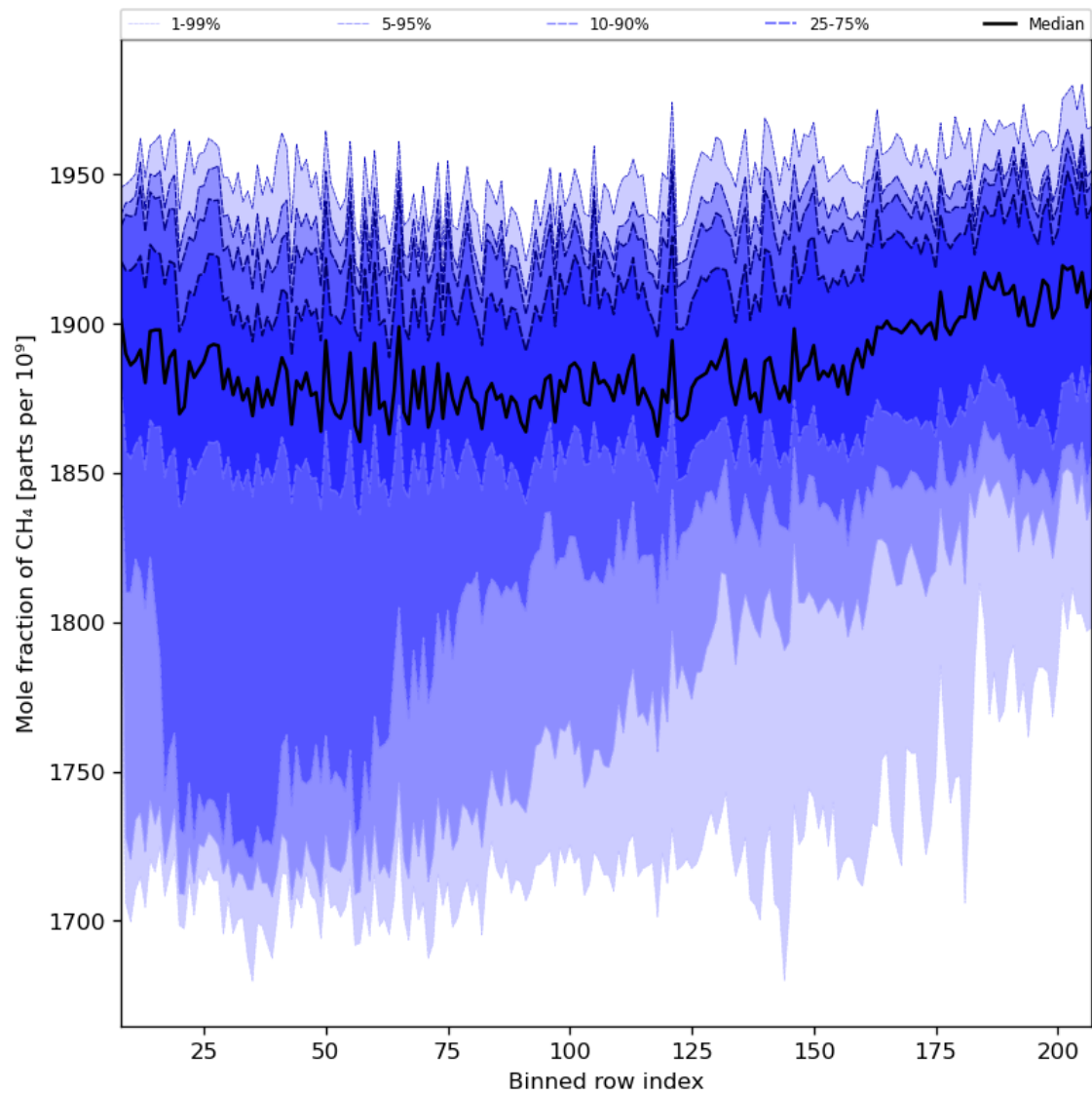
Figure 34: Along track statistics of “Mole fraction of CH 4 ” for 2023-10-01 to 2023-10-02
