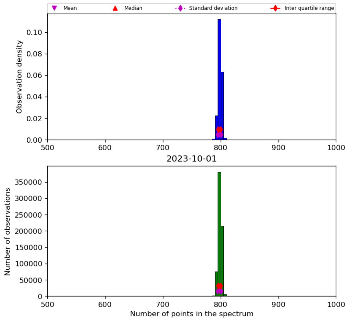
Figure 26: Histogram of “Number of points in the spectrum” for 2023-10-01 to 2023-10-02
