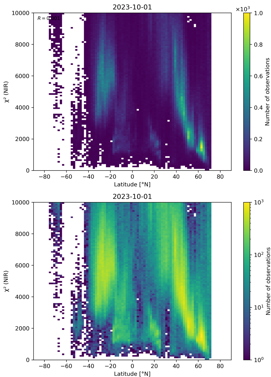
Figure 53: Scatter density plot of “Latitude” against “ \chi^2 (NIR)” for 2023-10-01 to 2023-10-02.
