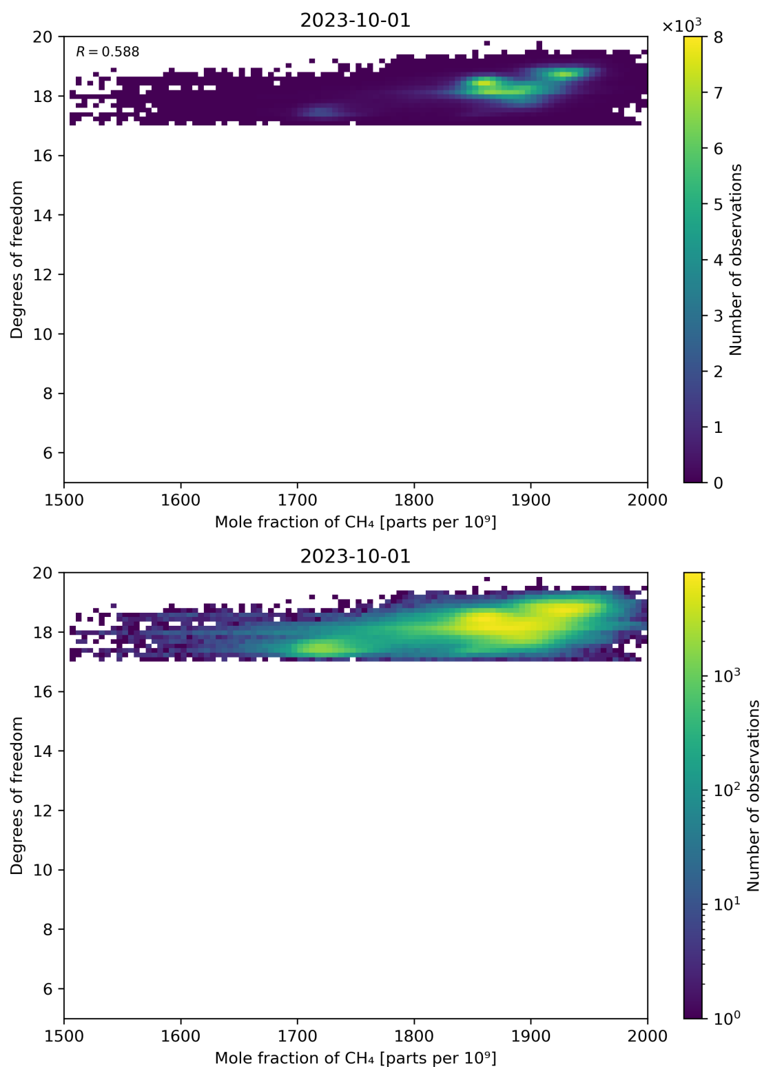
Figure 72: Scatter density plot of “Mole fraction of CH 4 ” against “Degrees of freedom” for 2023-10-01 to 2023-10-02.
