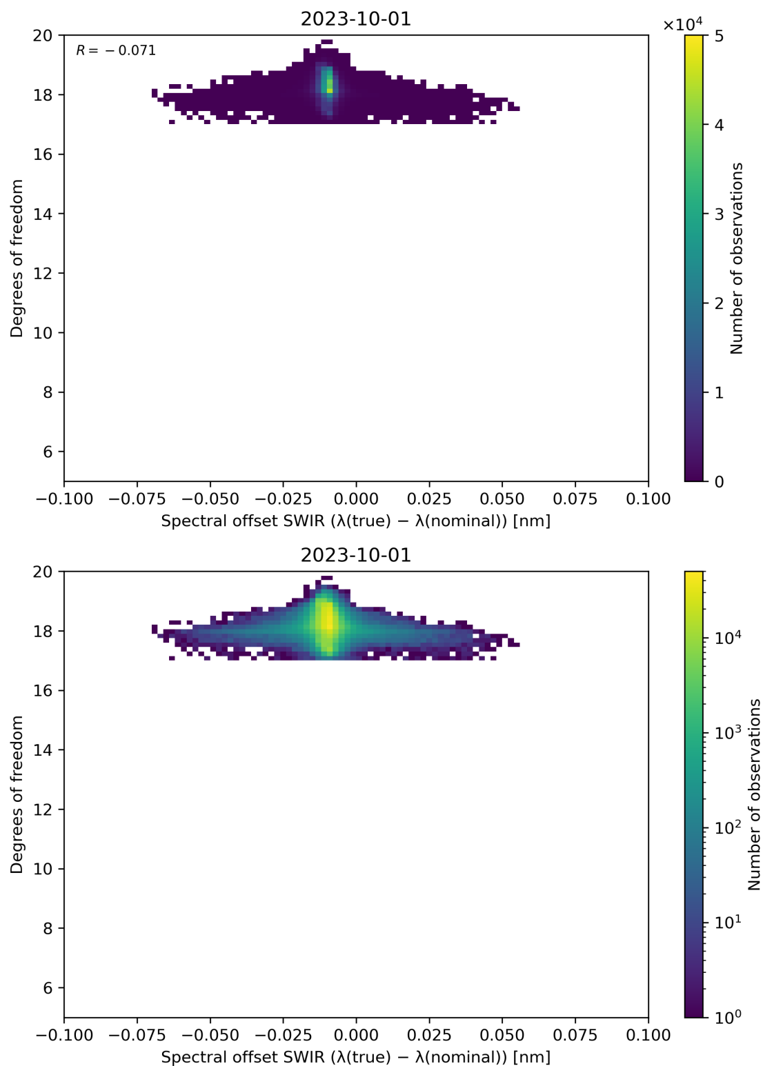
Figure 119: Scatter density plot of “Spectral offset SWIR ( \lambda(\text{true}) - \lambda(\text{nominal}) )” against “Degrees of freedom” for 2023-10-01 to 2023-10-02.
