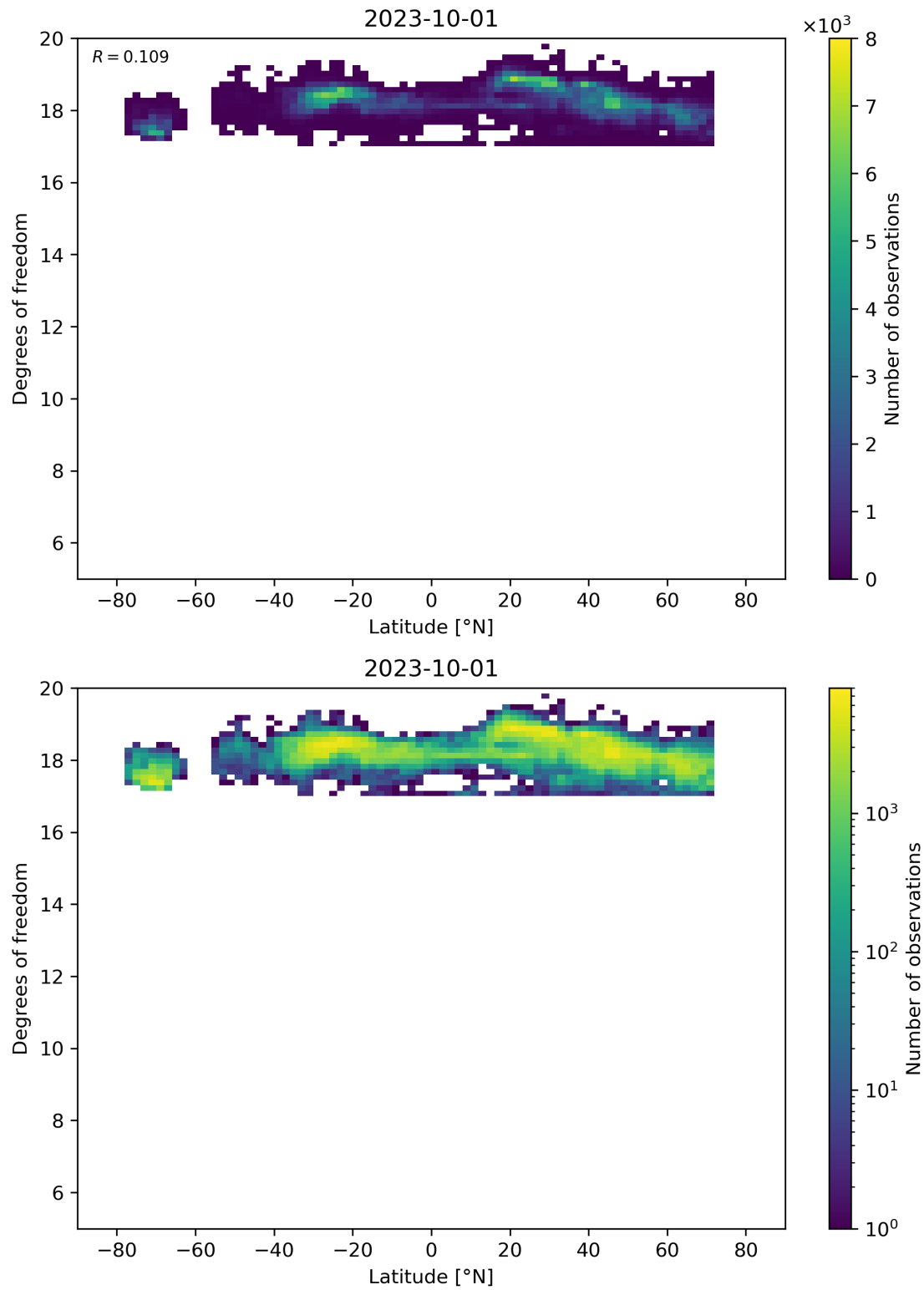
Figure 55: Scatter density plot of “Latitude” against “Degrees of freedom” for 2023-10-01 to 2023-10-02.
