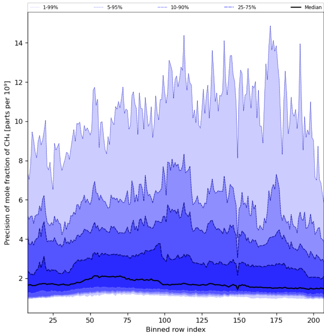
Figure 35: Along track statistics of “Precision of mole fraction of CH 4 ” for 2023-10-01 to 2023-10-02
