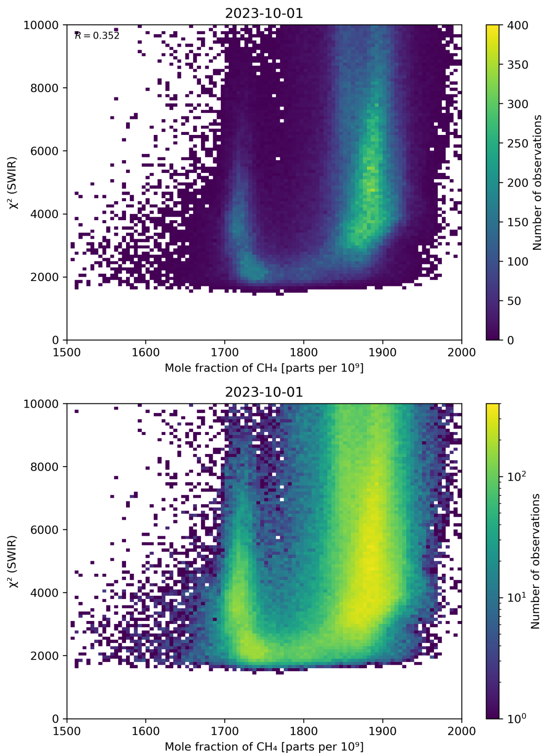
Figure 71: Scatter density plot of “Mole fraction of \text{CH}_4 ” against “ \chi^2 (SWIR)” for 2023-10-01 to 2023-10-02.
