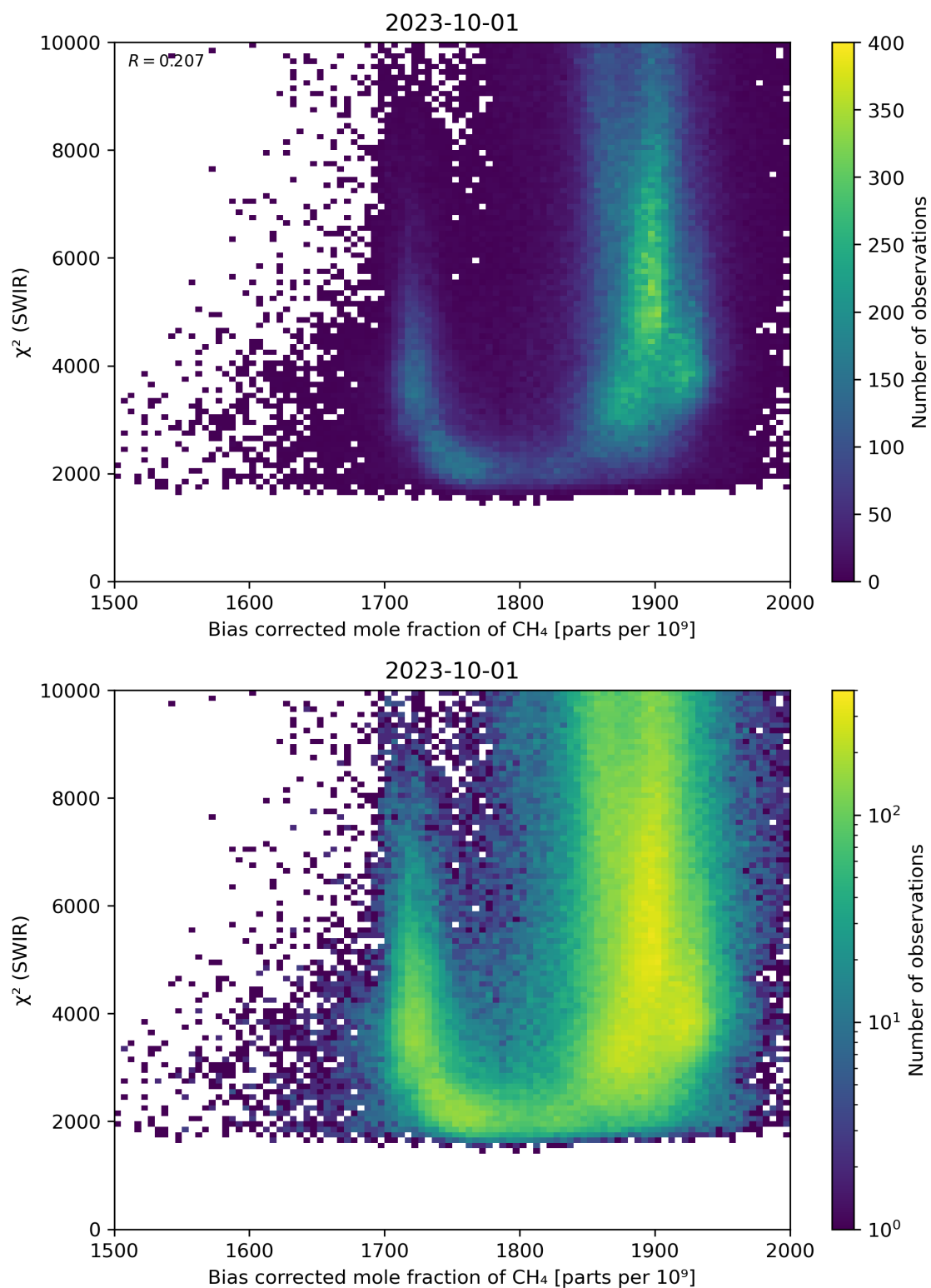
Figure 64: Scatter density plot of “Bias corrected mole fraction of CH 4 ” against “ \chi^2 (SWIR)” for 2023-10-01 to 2023-10-02.
