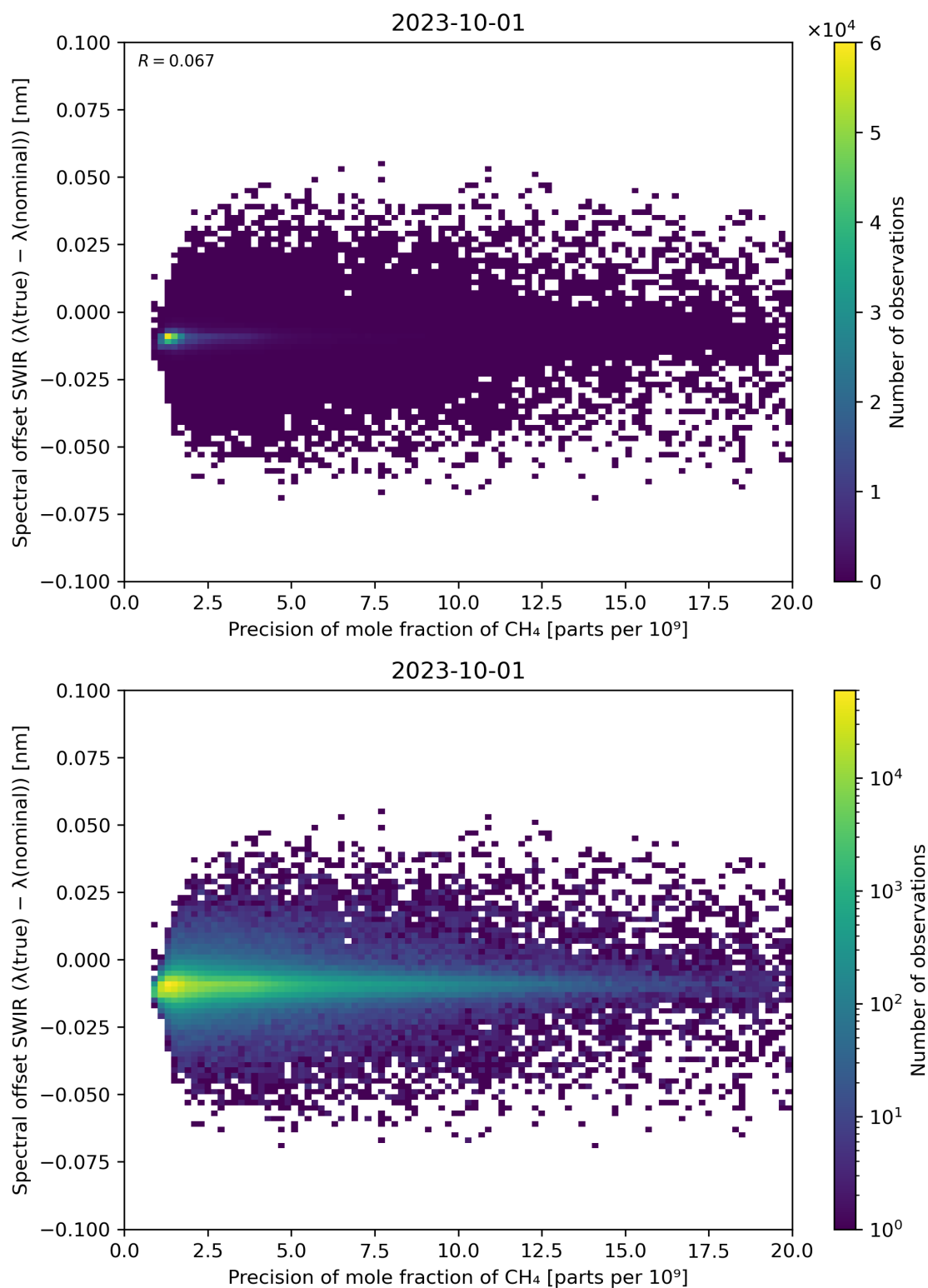
Figure 85: Scatter density plot of “Precision of mole fraction of \text{CH}_4 ” against “Spectral offset SWIR ( \lambda(\text{true}) - \lambda(\text{nominal}) )” for 2023-10-01 to 2023-10-02.
