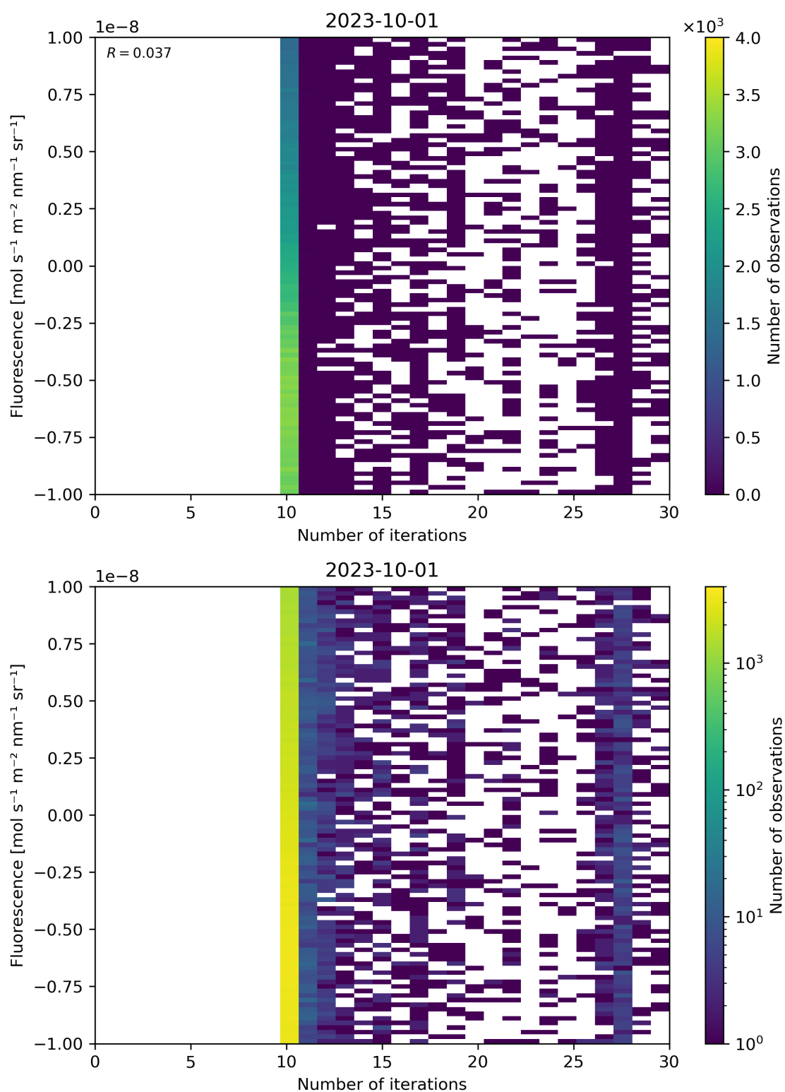
Figure 87: Scatter density plot of “Number of iterations” against “Fluorescence” for 2023-10-01 to 2023-10-02.
