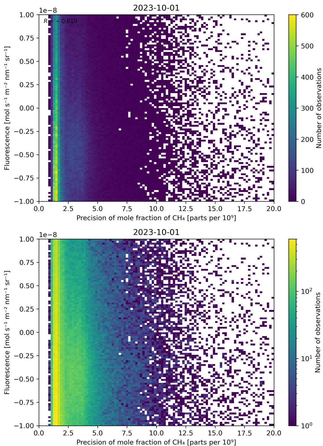
Figure 81: Scatter density plot of “Precision of mole fraction of \text{CH}_4 ” against “Fluorescence” for 2023-10-01 to 2023-10-02.
