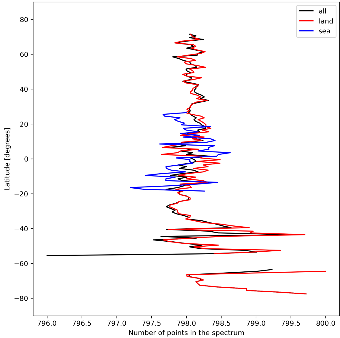
Figure 15: Zonal average of “Number of points in the spectrum” for 2023-10-01 to 2023-10-02.
