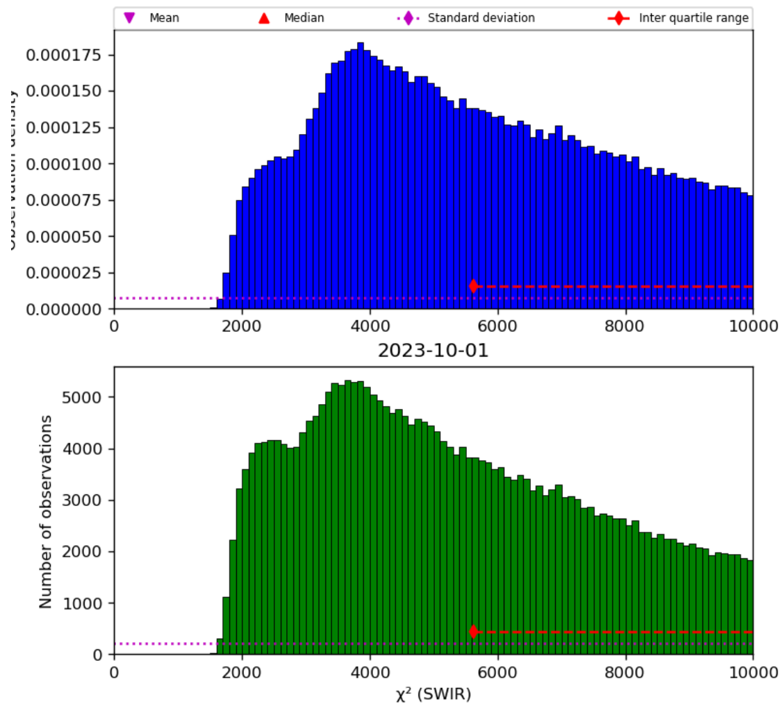
Figure 28: Histogram of “ \chi^2 (SWIR)” for 2023-10-01 to 2023-10-02
