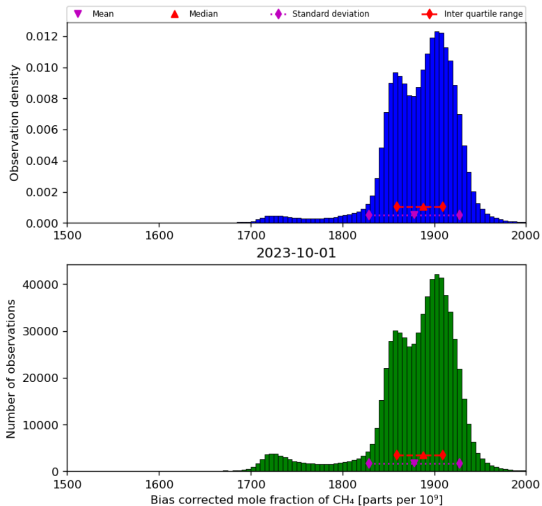
Figure 25: Histogram of “Bias corrected mole fraction of CH 4 ” for 2023-10-01 to 2023-10-02
