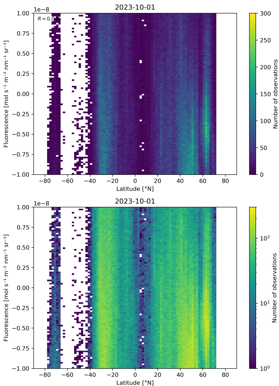
Figure 56: Scatter density plot of “Latitude” against “Fluorescence” for 2023-10-01 to 2023-10-02.
