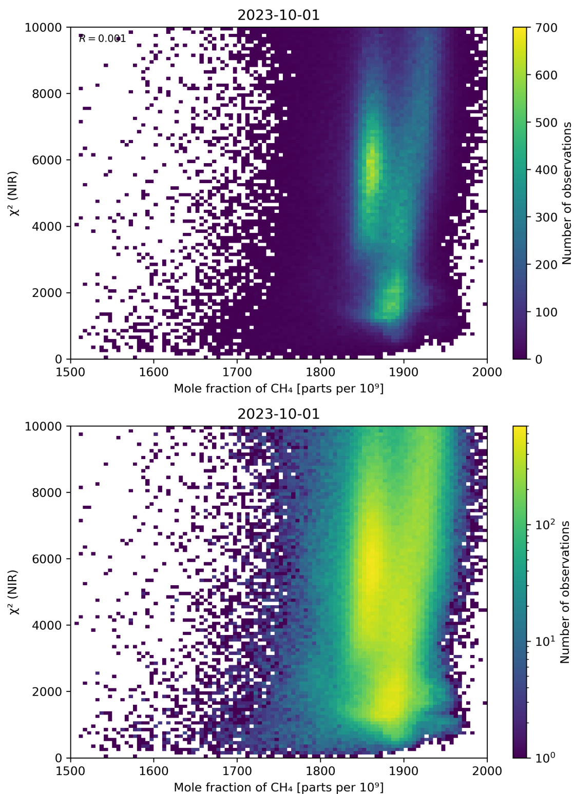
Figure 70: Scatter density plot of “Mole fraction of CH 4 ” against “ \chi^2 (NIR)” for 2023-10-01 to 2023-10-02.
