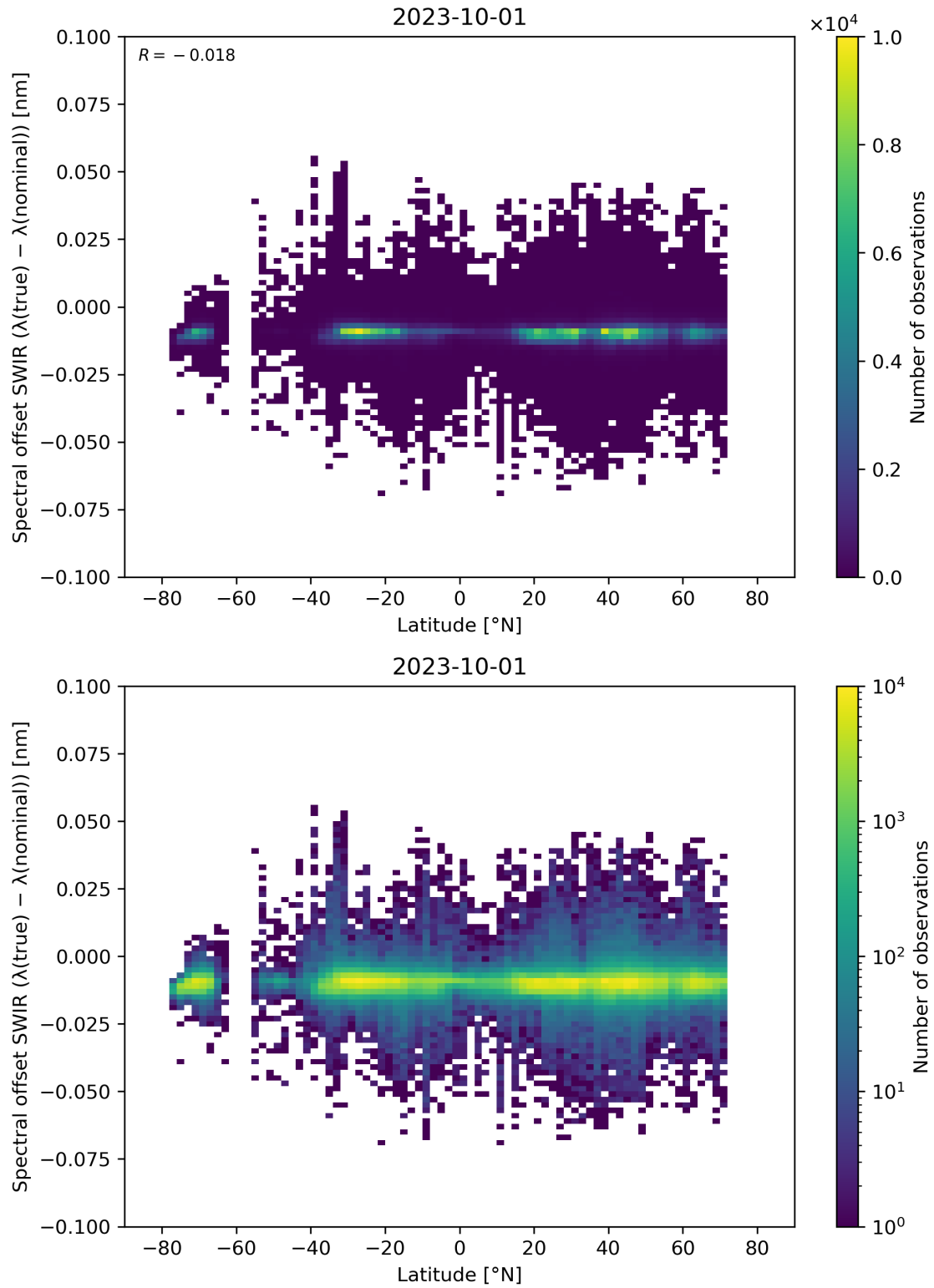
Figure 62: Scatter density plot of “Latitude” against “Spectral offset SWIR ( \lambda(\text{true}) - \lambda(\text{nominal}) )” for 2023-10-01 to 2023-10-02.
