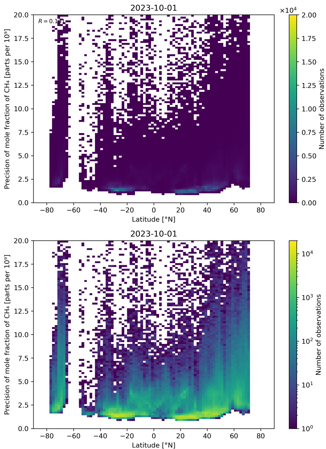
Figure 59: Scatter density plot of “Latitude” against “Precision of mole fraction of CH 4 ” for 2023-10-01 to 2023-10-02.
