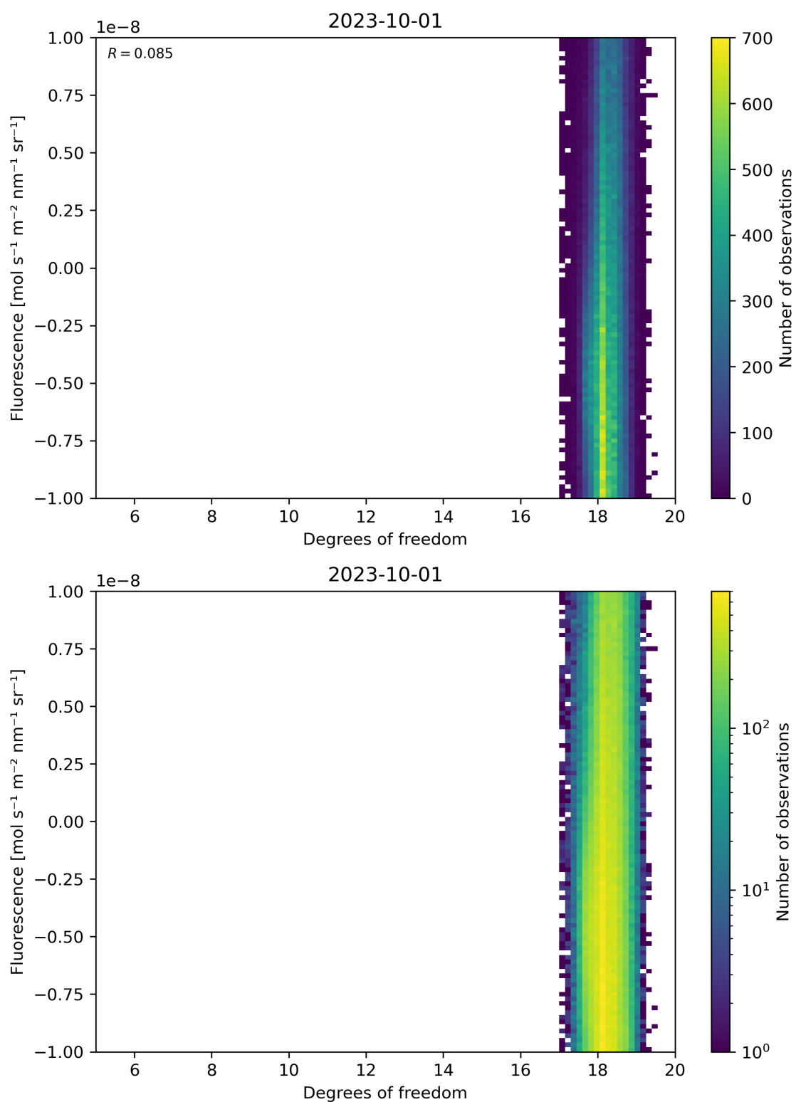
Figure 51: Scatter density plot of “Degrees of freedom” against “Fluorescence” for 2023-10-01 to 2023-10-02.
