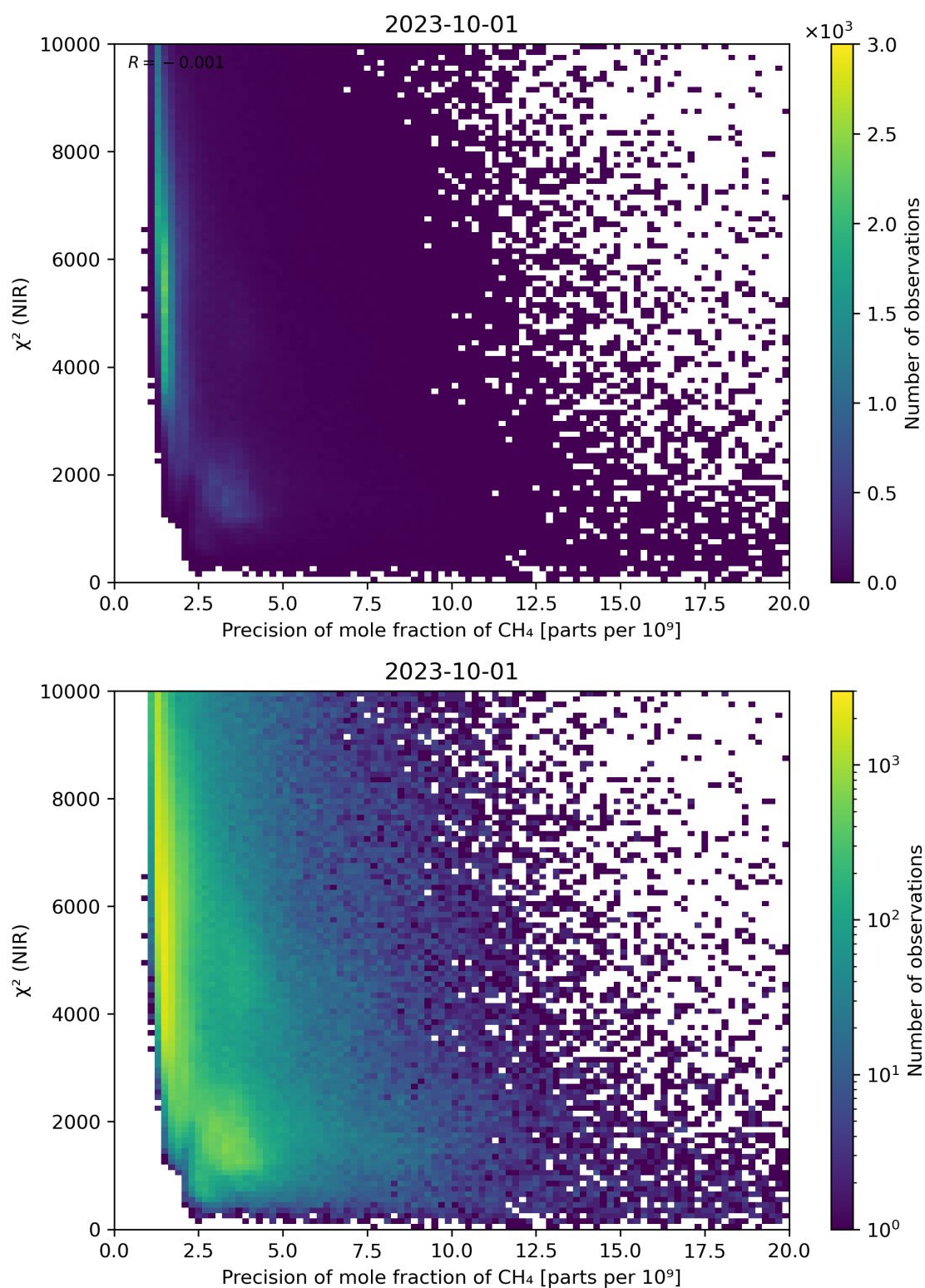
Figure 78: Scatter density plot of “Precision of mole fraction of CH 4 ” against “ \chi^2 (NIR)” for 2023-10-01 to 2023-10-02.
