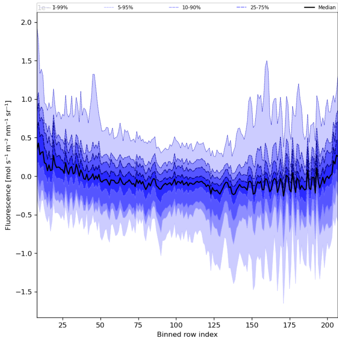
Figure 43: Along track statistics of “Fluorescence” for 2023-10-01 to 2023-10-02
