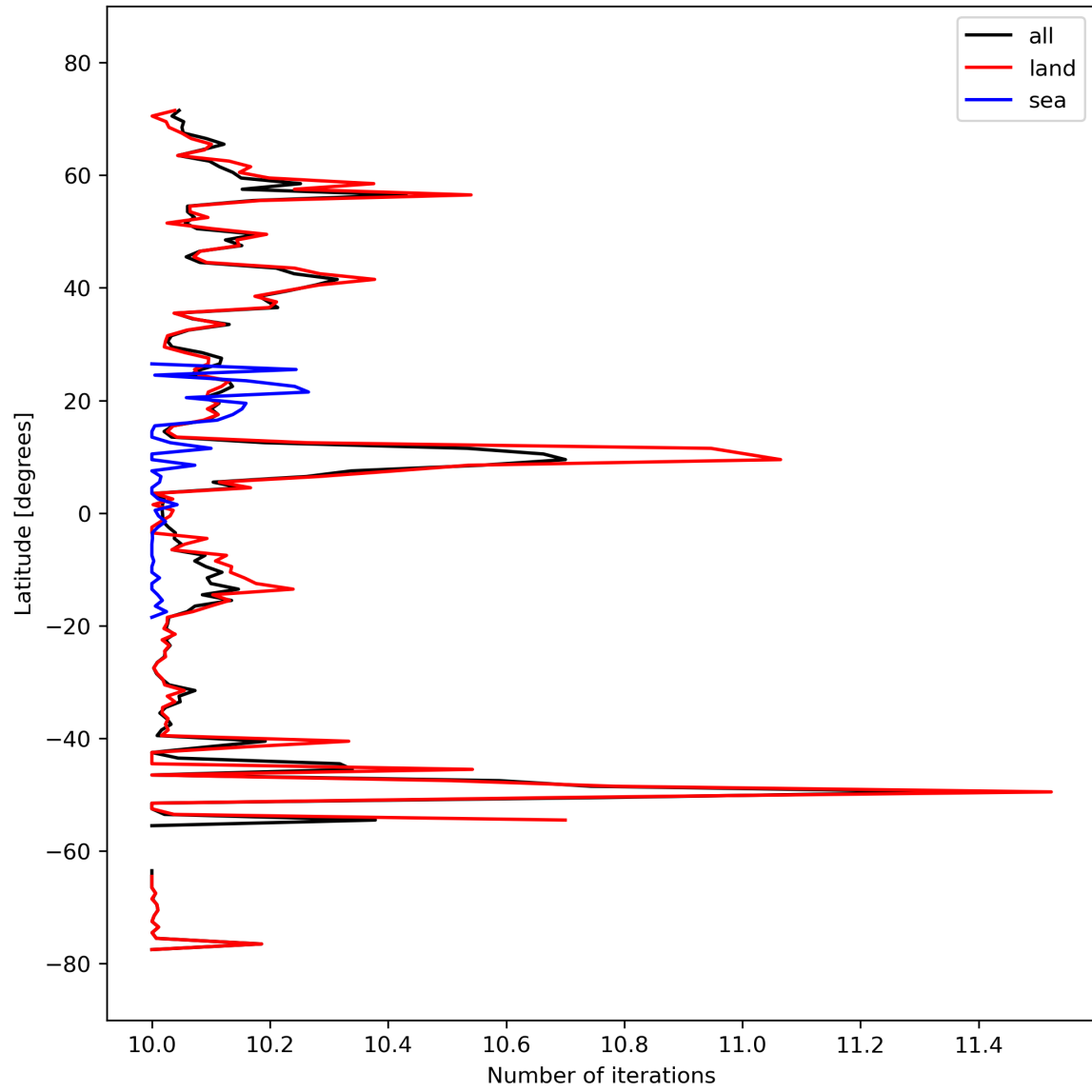
Figure 20: Zonal average of “Number of iterations” for 2023-10-01 to 2023-10-02.
