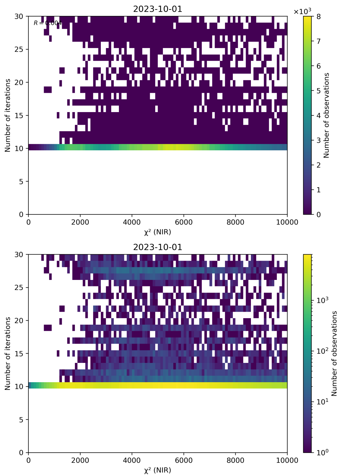
Figure 46: Scatter density plot of “ \chi^2 (NIR)” against “Number of iterations” for 2023-10-01 to 2023-10-02.
