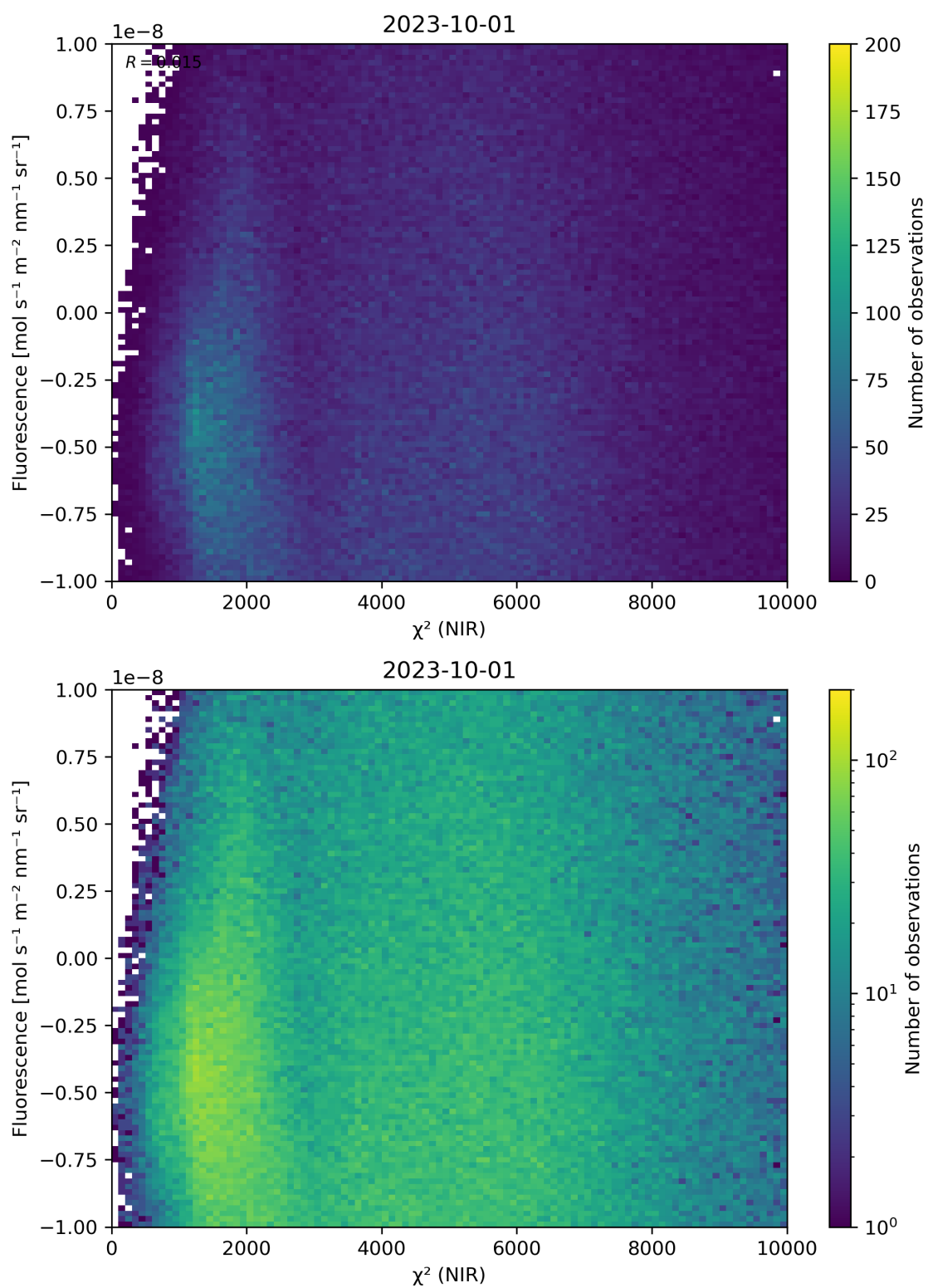
Figure 45: Scatter density plot of “ \chi^2 (NIR)” against “Fluorescence” for 2023-10-01 to 2023-10-02.
