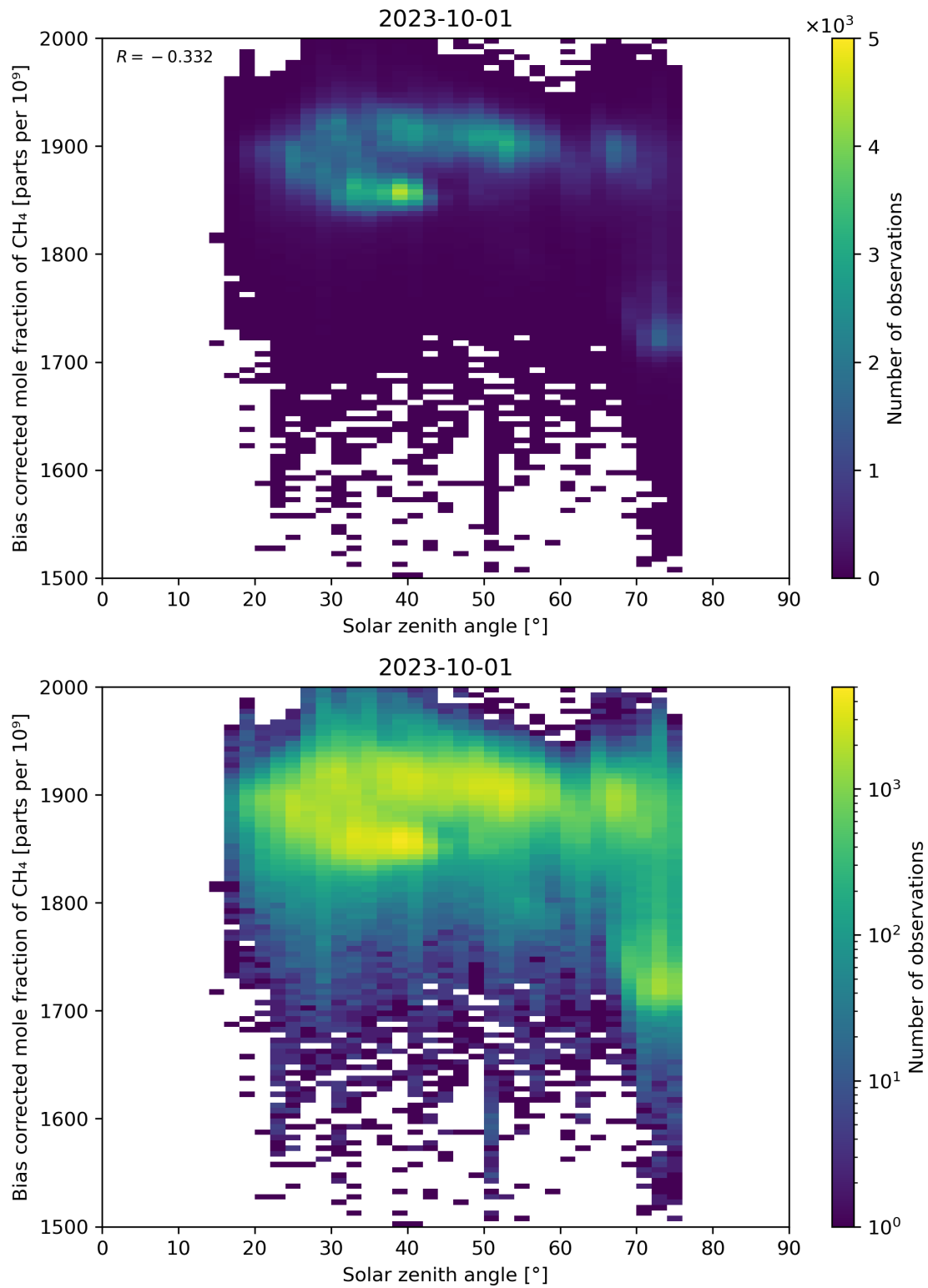
Figure 100: Scatter density plot of “Solar zenith angle” against “Bias corrected mole fraction of CH 4 ” for 2023-10-01 to 2023-10-02.
