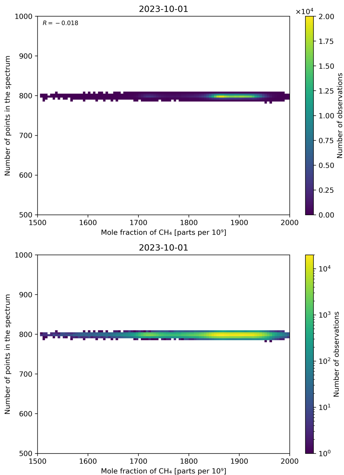
Figure 77: Scatter density plot of “Mole fraction of CH 4 ” against “Number of points in the spectrum” for 2023-10-01 to 2023-10-02.
