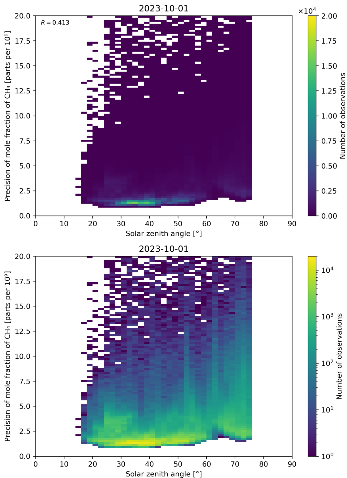
Figure 101: Scatter density plot of “Solar zenith angle” against “Precision of mole fraction of CH 4 ” for 2023-10-01 to 2023-10-02.
