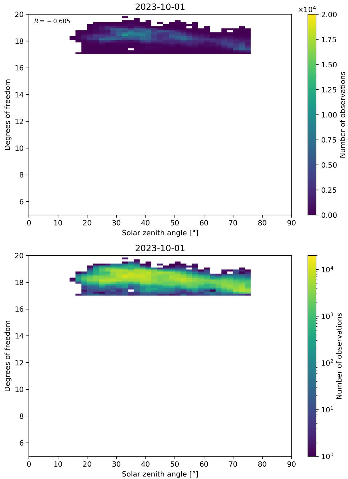
Figure 96: Scatter density plot of “Solar zenith angle” against “Degrees of freedom” for 2023-10-01 to 2023-10-02.
