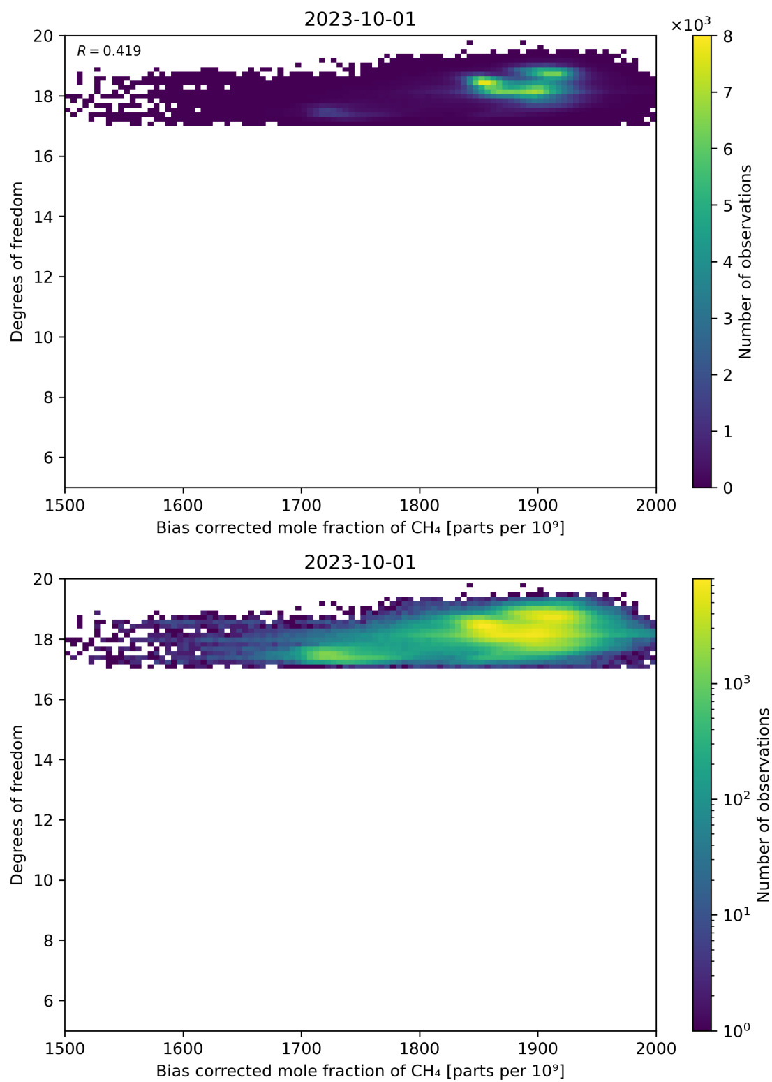
Figure 65: Scatter density plot of “Bias corrected mole fraction of CH 4 ” against “Degrees of freedom” for 2023-10-01 to 2023-10-02.
