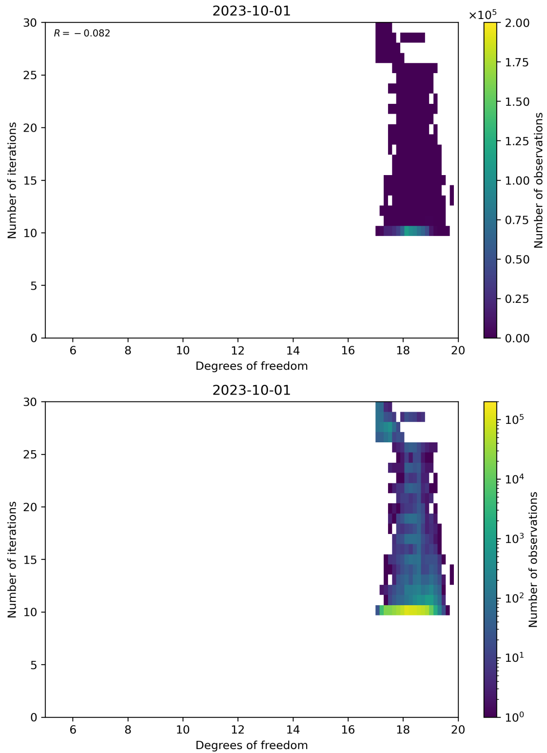
Figure 52: Scatter density plot of “Degrees of freedom” against “Number of iterations” for 2023-10-01 to 2023-10-02.
