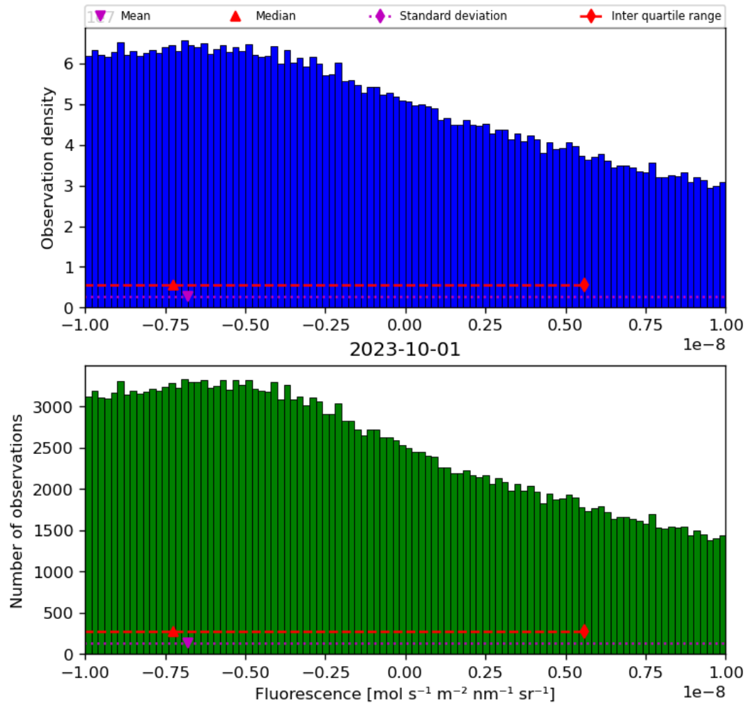
Figure 32: Histogram of “Fluorescence” for 2023-10-01 to 2023-10-02
