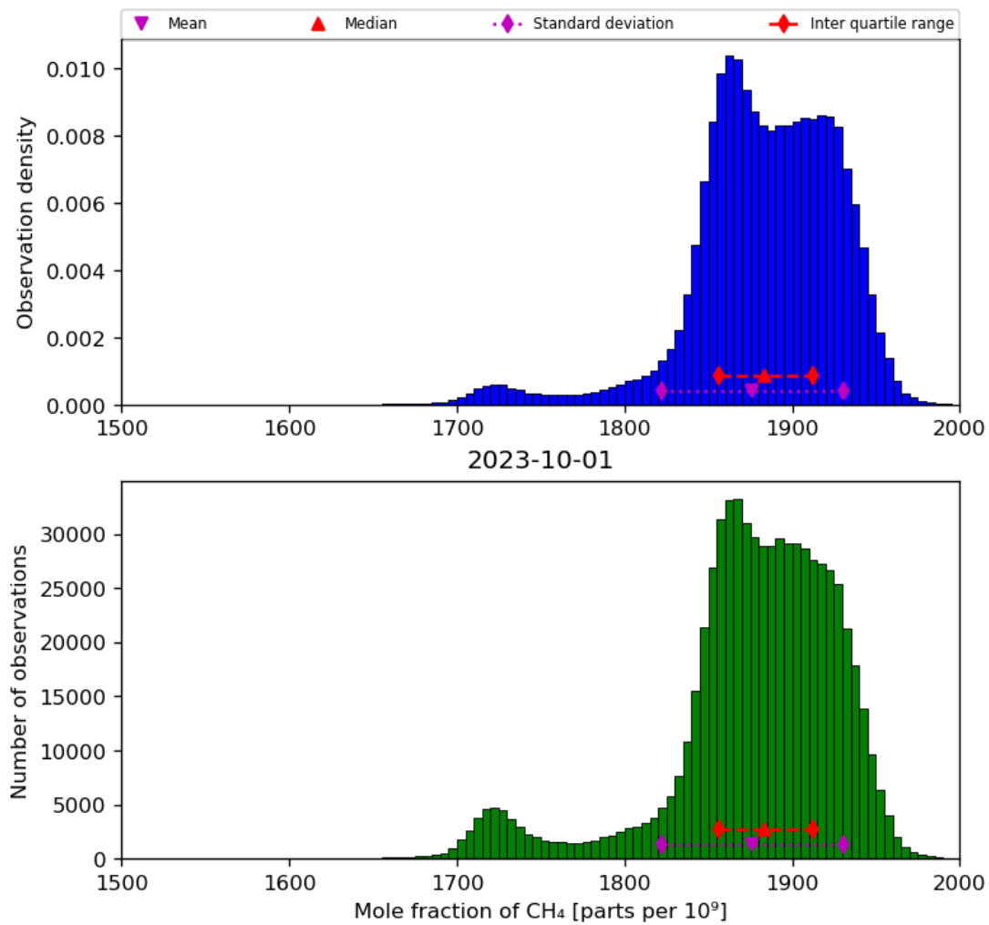
Figure 23: Histogram of “Mole fraction of CH 4 ” for 2023-10-01 to 2023-10-02
