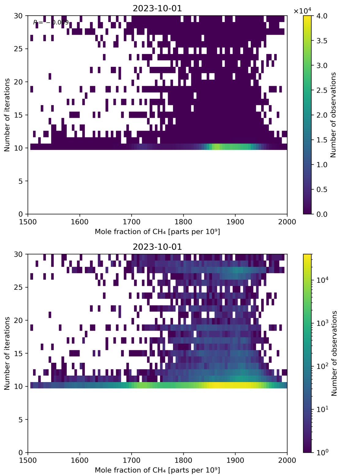
Figure 76: Scatter density plot of “Mole fraction of CH 4 ” against “Number of iterations” for 2023-10-01 to 2023-10-02.
