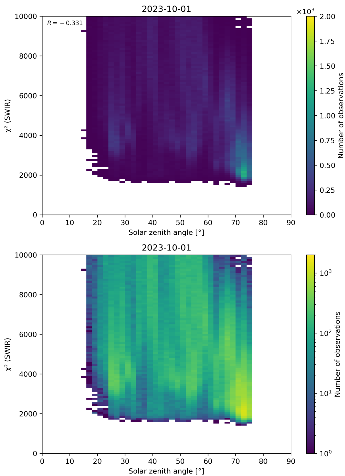
Figure 95: Scatter density plot of “Solar zenith angle” against “ \chi^2 (SWIR)” for 2023-10-01 to 2023-10-02.
