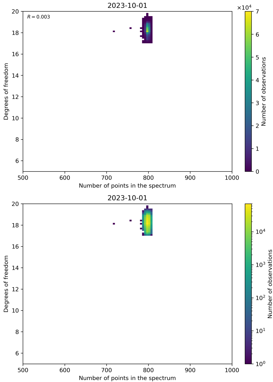
Figure 90: Scatter density plot of “Number of points in the spectrum” against “Degrees of freedom” for 2023-10-01 to 2023-10-02.
