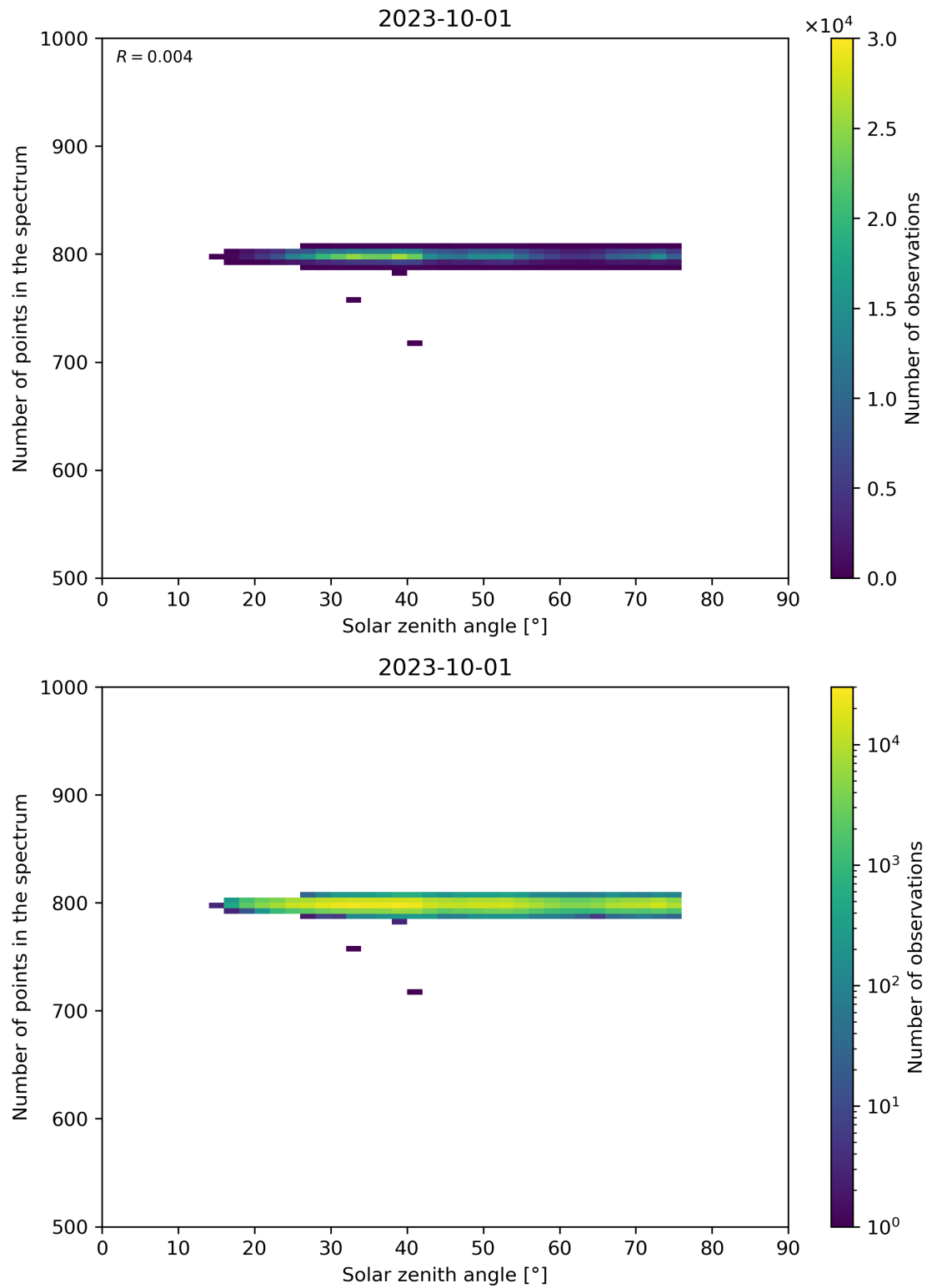
Figure 103: Scatter density plot of “Solar zenith angle” against “Number of points in the spectrum” for 2023-10-01 to 2023-10-02.
