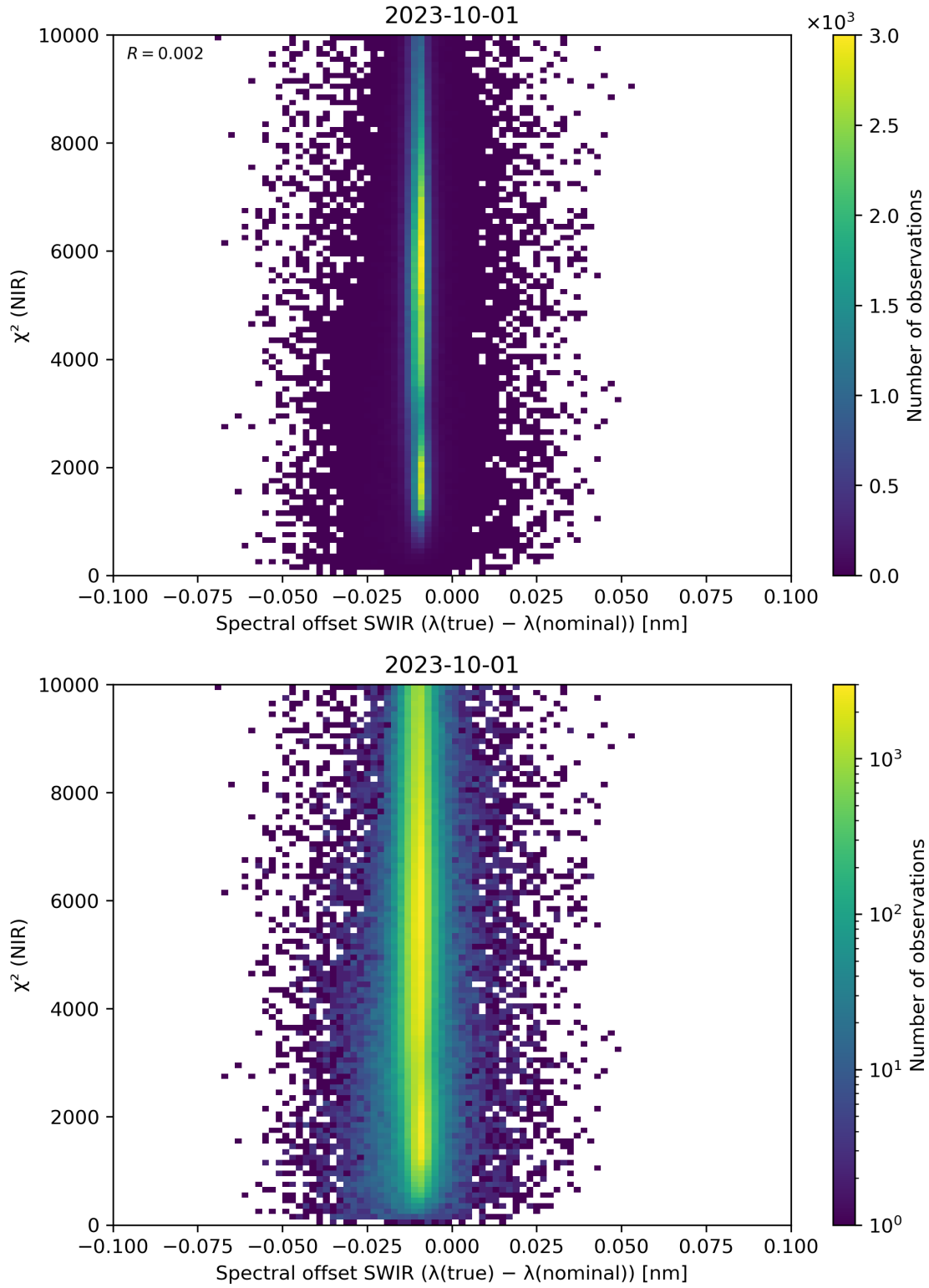
Figure 117: Scatter density plot of “Spectral offset SWIR ( \lambda(\text{true}) - \lambda(\text{nominal}) )” against “ \chi^2 (NIR)” for 2023-10-01 to 2023-10-02.
