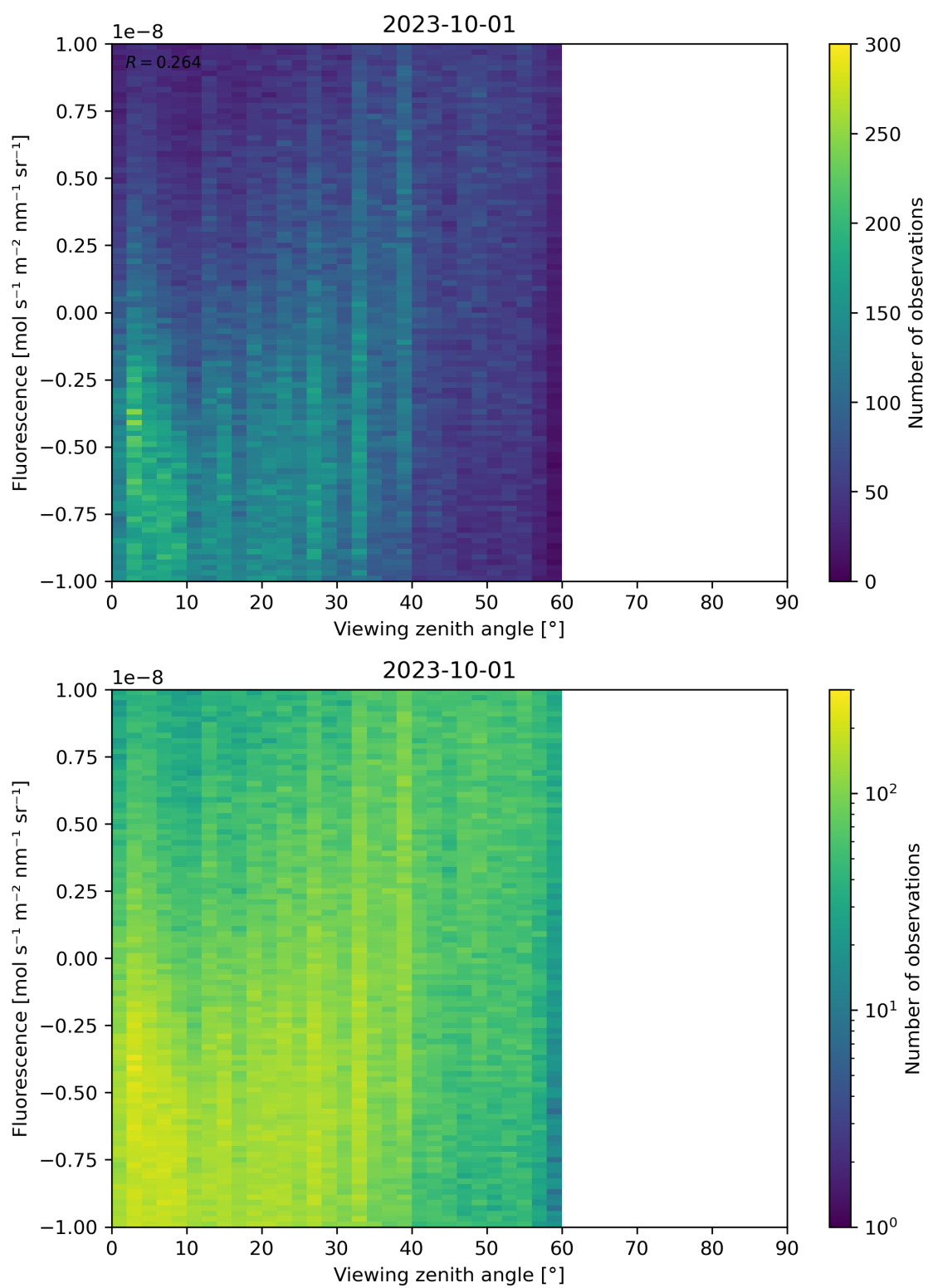
Figure 108: Scatter density plot of “Viewing zenith angle” against “Fluorescence” for 2023-10-01 to 2023-10-02.
