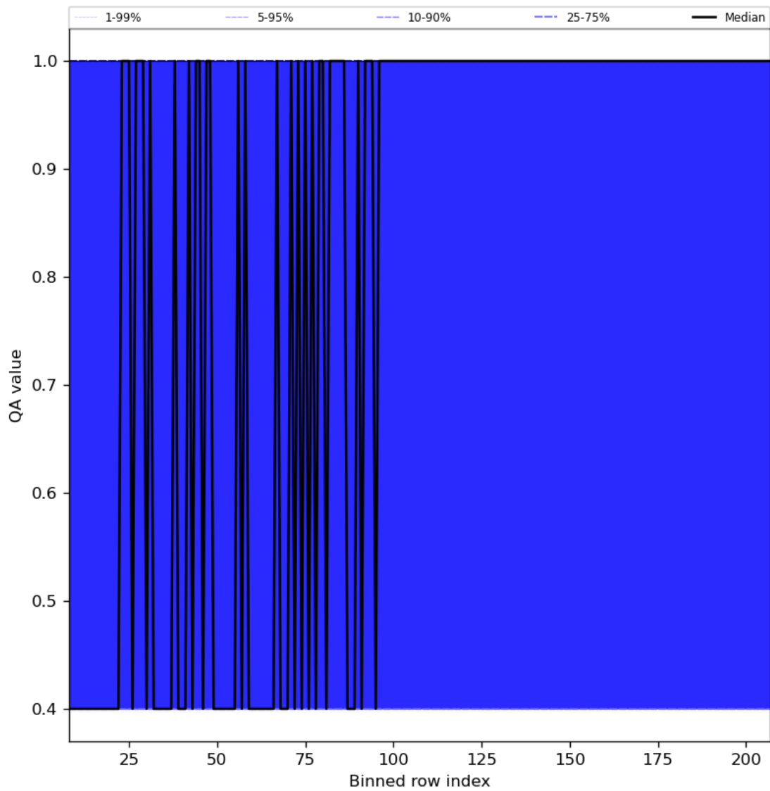
Figure 33: Along track statistics of “QA value” for 2023-10-01 to 2023-10-02
