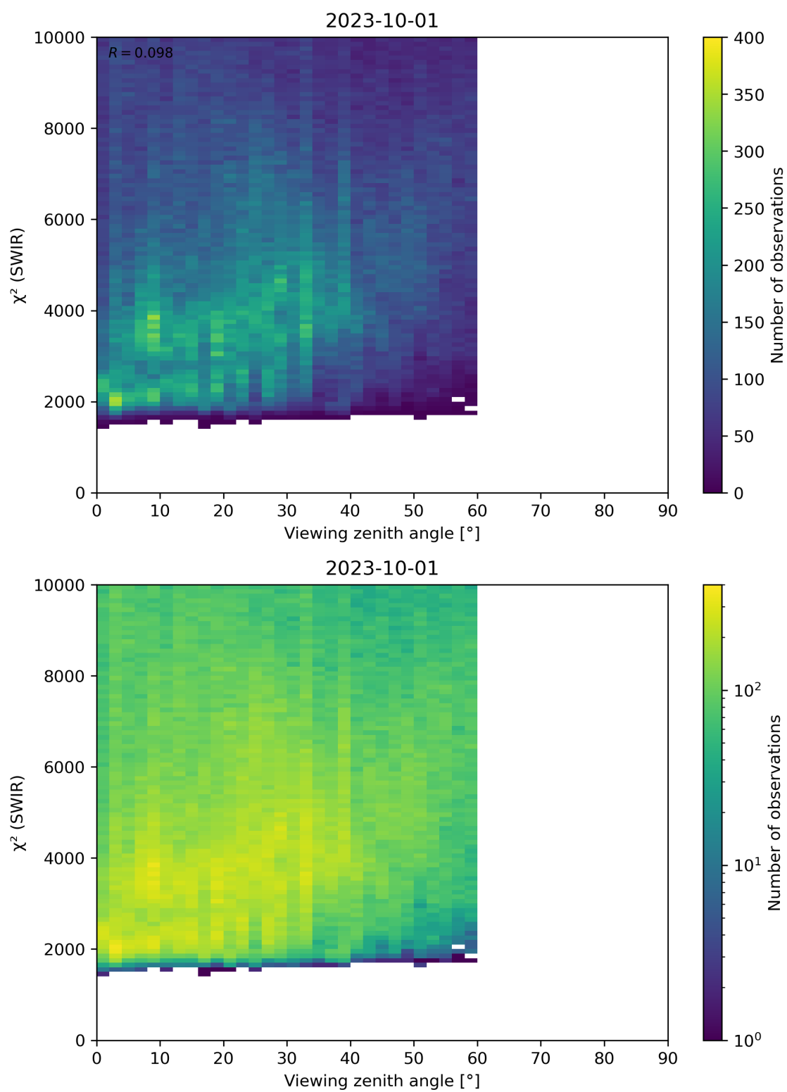
Figure 106: Scatter density plot of “Viewing zenith angle” against “ \chi^2 (SWIR)” for 2023-10-01 to 2023-10-02.
