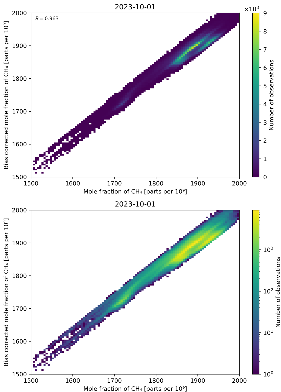
Figure 74: Scatter density plot of “Mole fraction of CH 4 ” against “Bias corrected mole fraction of CH 4 ” for 2023-10-01 to 2023-10-02.
