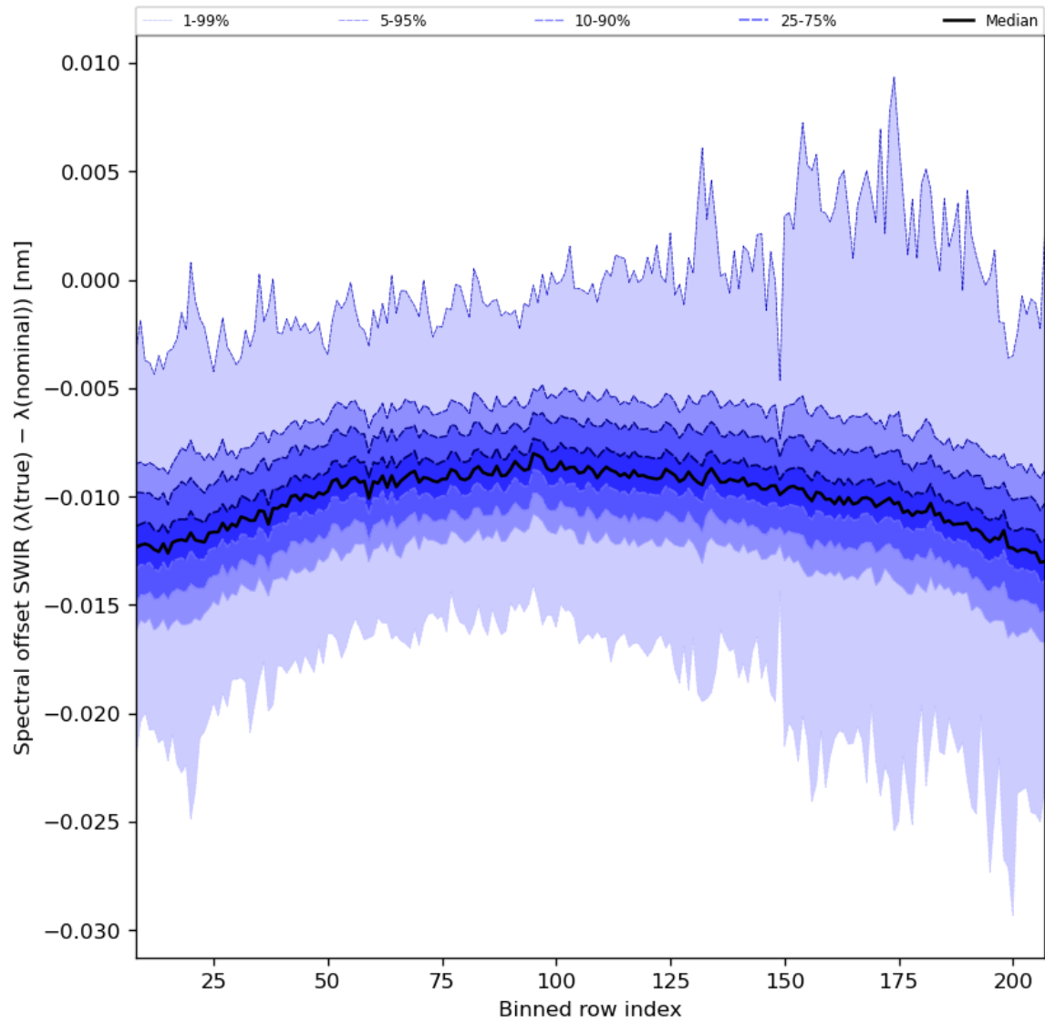
Figure 38: Along track statistics of “Spectral offset SWIR ( \lambda(\text{true}) - \lambda(\text{nominal}) )” for 2023-10-01 to 2023-10-02
