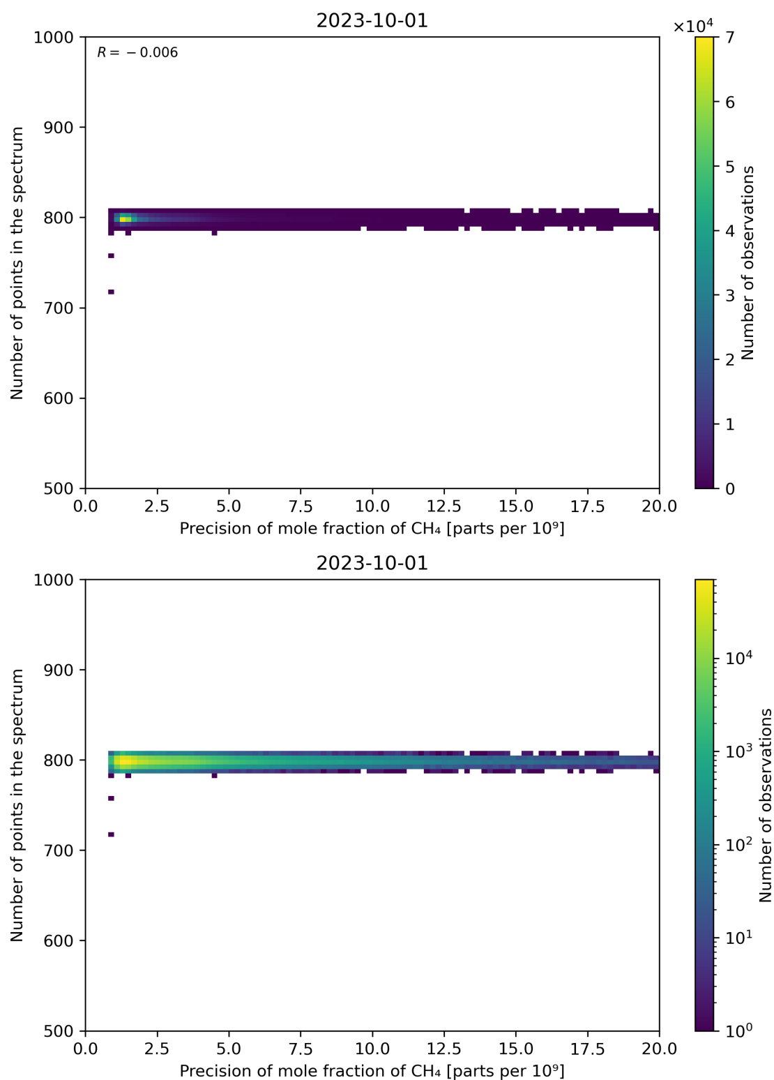
Figure 84: Scatter density plot of “Precision of mole fraction of CH 4 ” against “Number of points in the spectrum” for 2023-10-01 to 2023-10-02.
