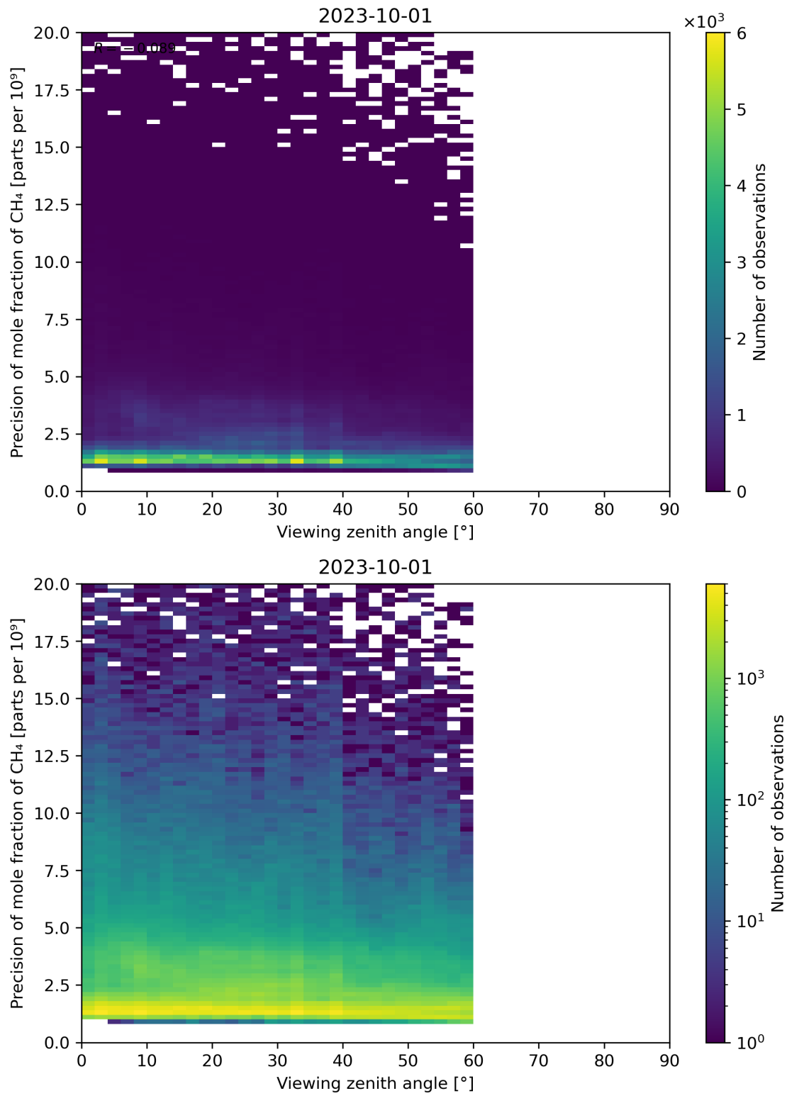
Figure 112: Scatter density plot of “Viewing zenith angle” against “Precision of mole fraction of CH 4 ” for 2023-10-01 to 2023-10-02.
