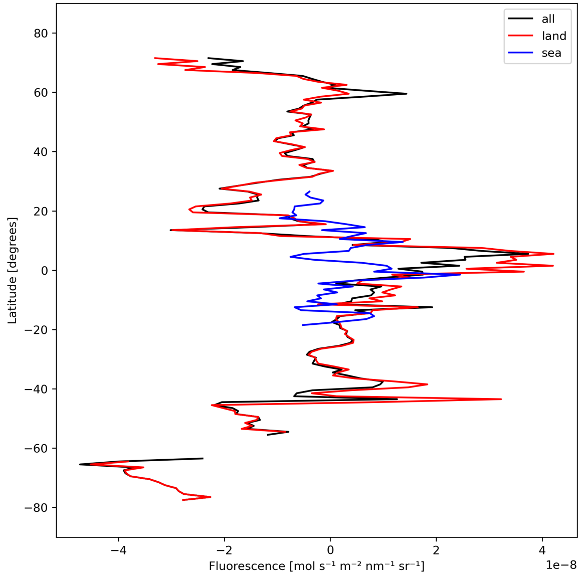
Figure 21: Zonal average of “Fluorescence” for 2023-10-01 to 2023-10-02.
