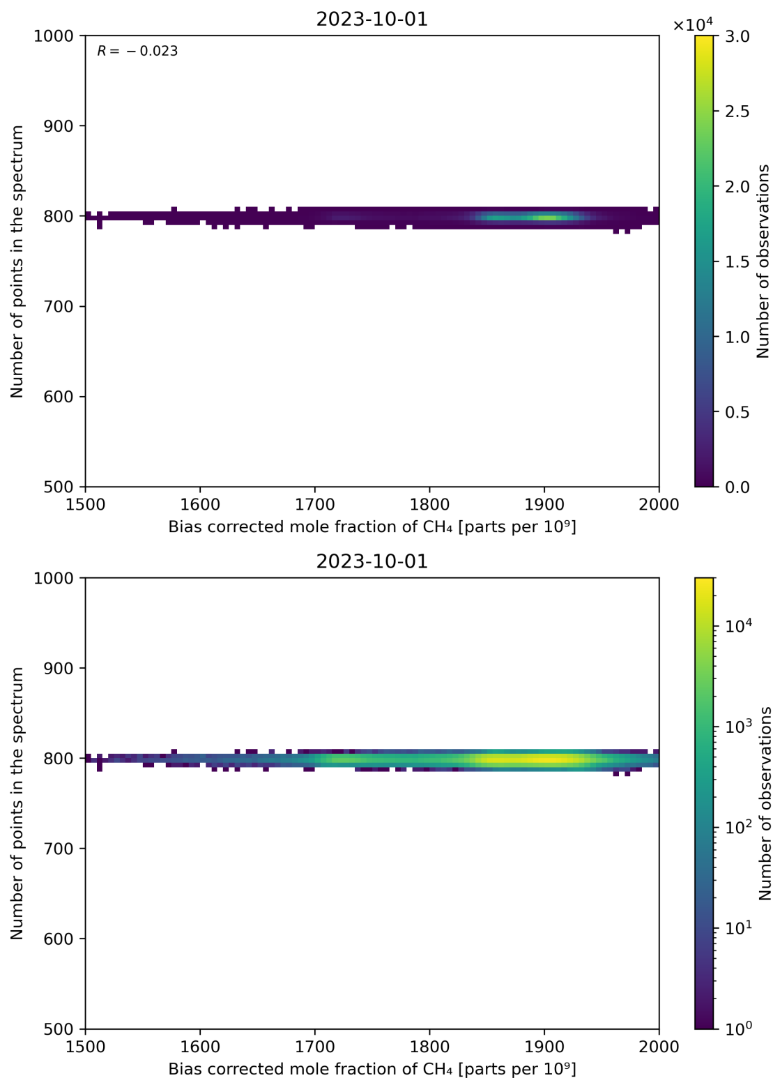
Figure 68: Scatter density plot of “Bias corrected mole fraction of CH 4 ” against “Number of points in the spectrum” for 2023-10-01 to 2023-10-02.
