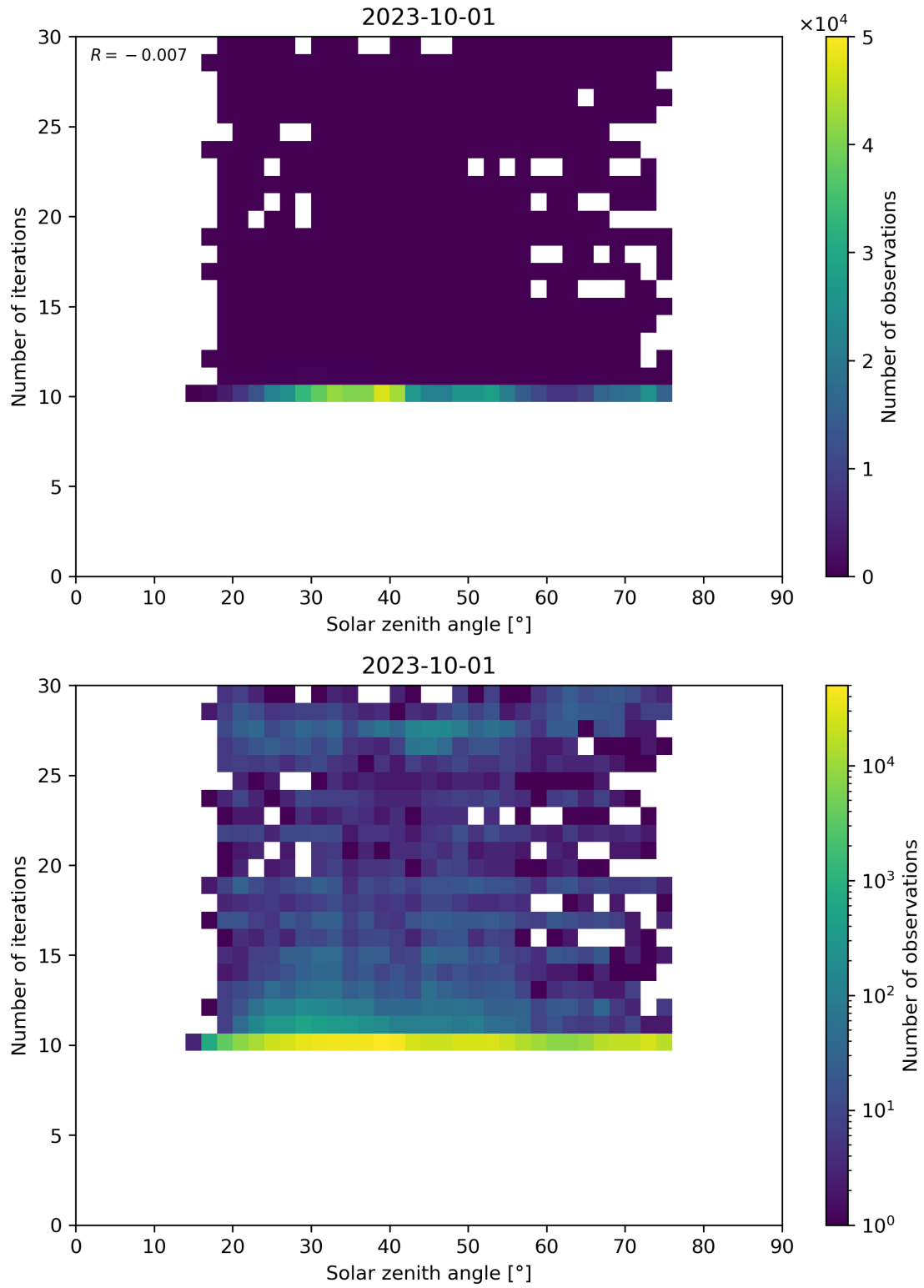
Figure 102: Scatter density plot of “Solar zenith angle” against “Number of iterations” for 2023-10-01 to 2023-10-02.
