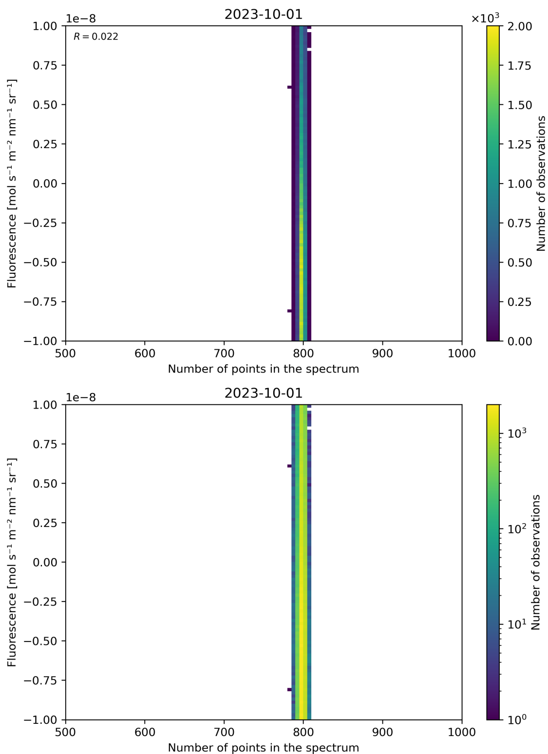
Figure 91: Scatter density plot of “Number of points in the spectrum” against “Fluorescence” for 2023-10-01 to 2023-10-02.
