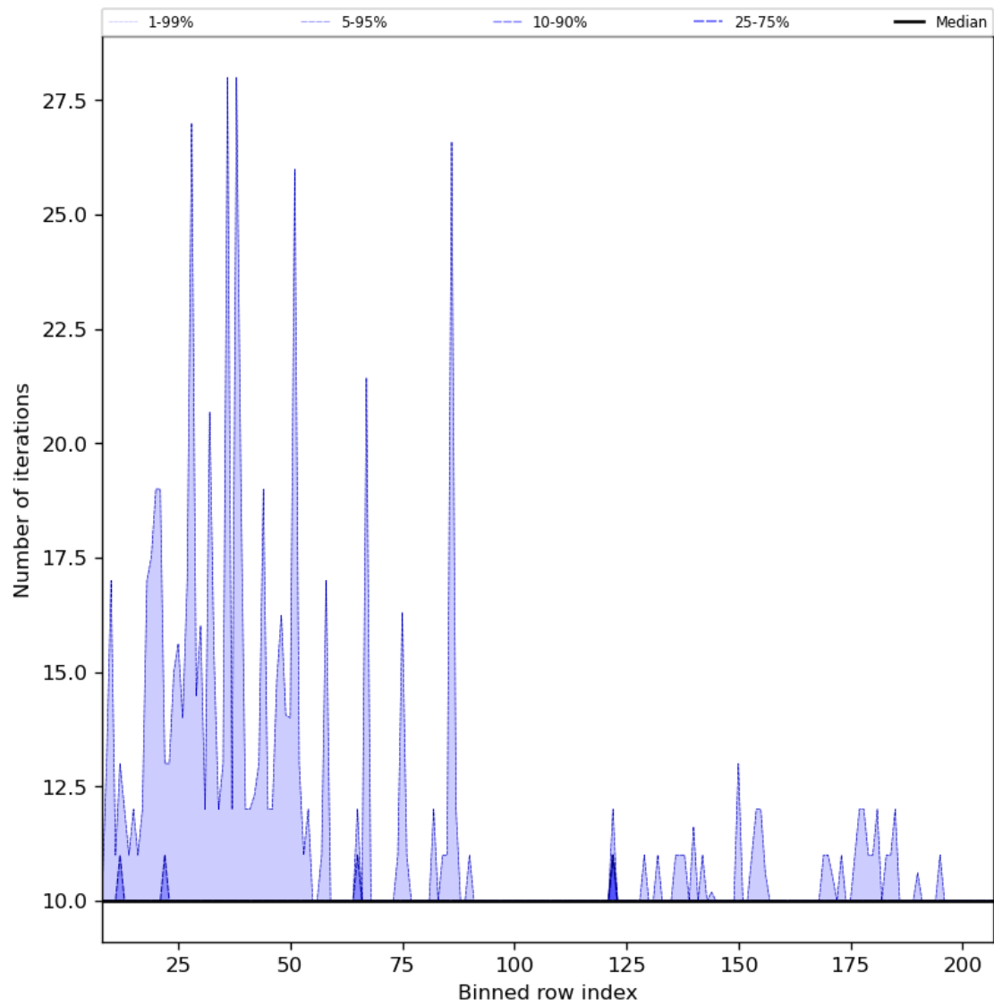
Figure 42: Along track statistics of “Number of iterations” for 2023-10-01 to 2023-10-02
