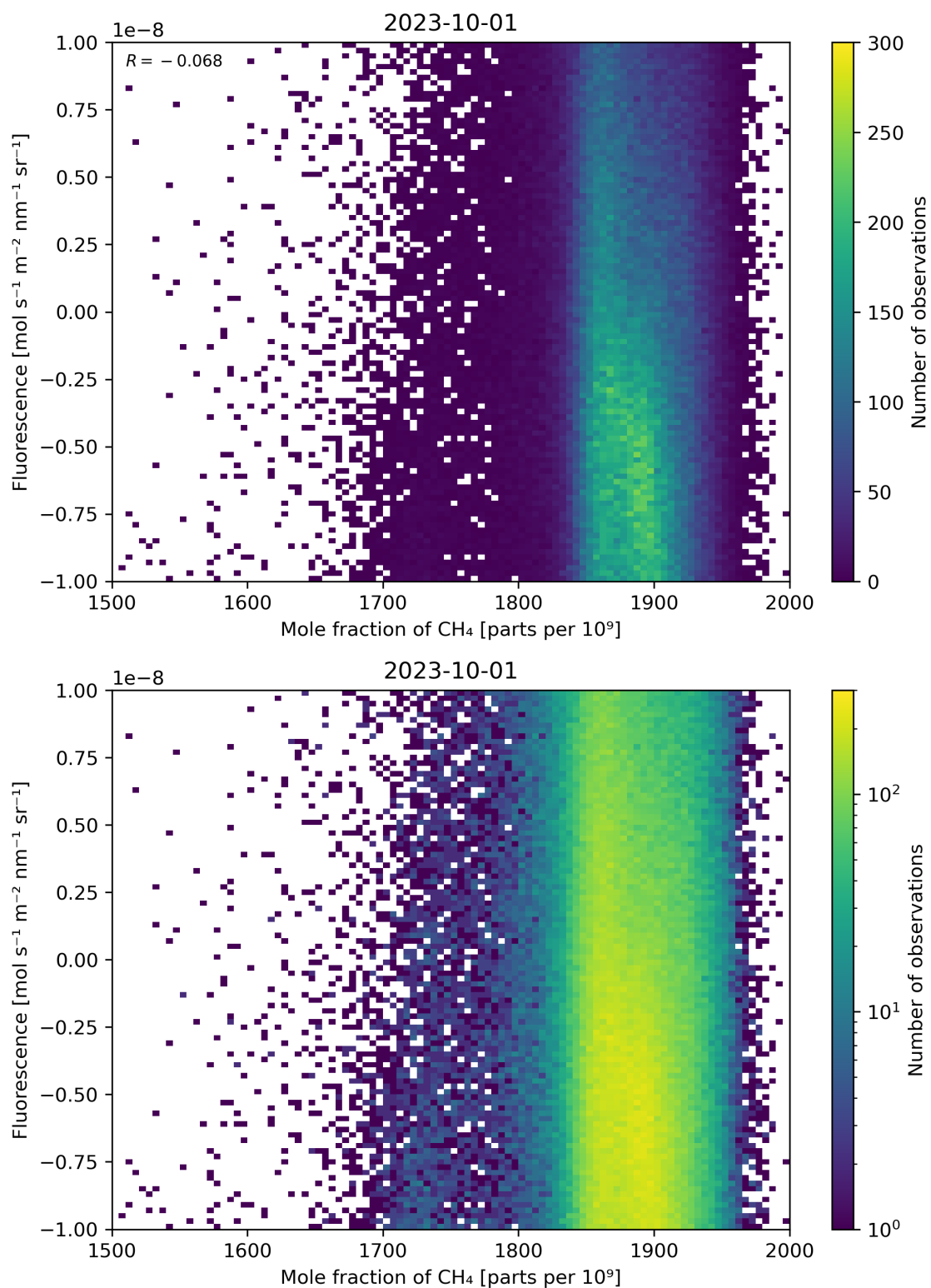
Figure 73: Scatter density plot of “Mole fraction of \text{CH}_4 ” against “Fluorescence” for 2023-10-01 to 2023-10-02.
