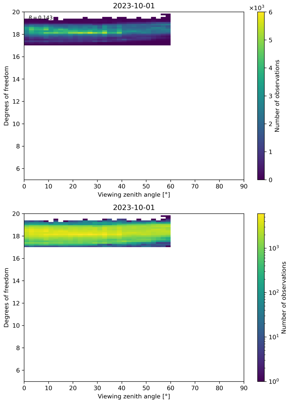
Figure 107: Scatter density plot of “Viewing zenith angle” against “Degrees of freedom” for 2023-10-01 to 2023-10-02.
