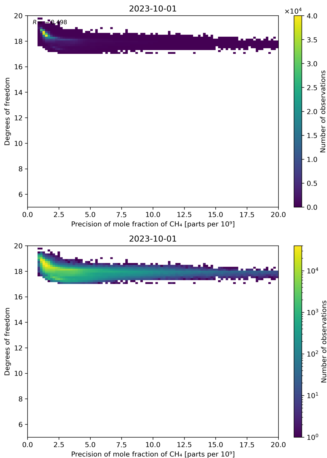
Figure 80: Scatter density plot of “Precision of mole fraction of CH 4 ” against “Degrees of freedom” for 2023-10-01 to 2023-10-02.
