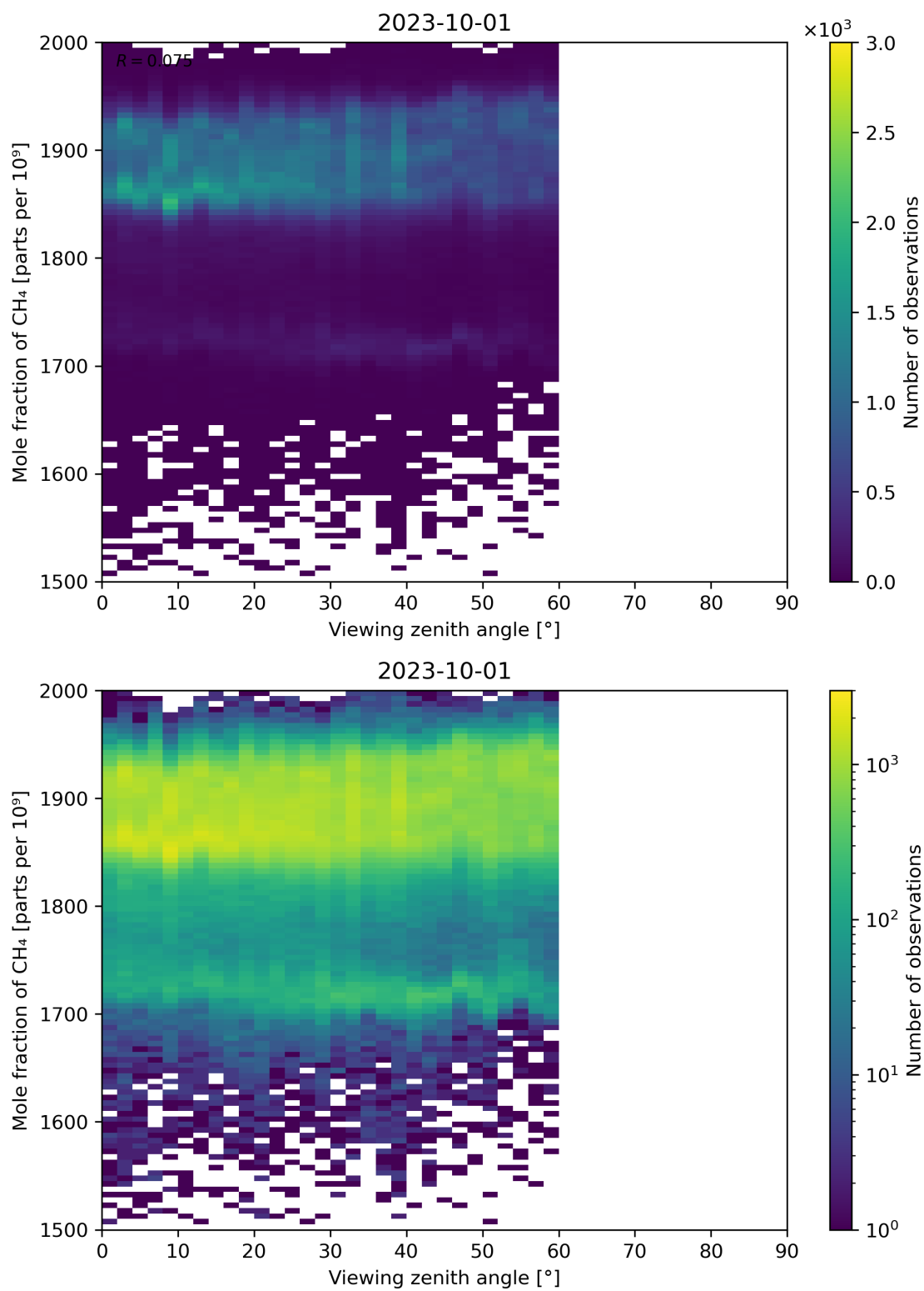
Figure 110: Scatter density plot of “Viewing zenith angle” against “Mole fraction of CH 4 ” for 2023-10-01 to 2023-10-02.
