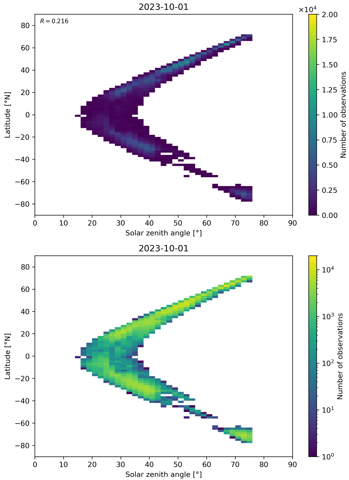
Figure 98: Scatter density plot of “Solar zenith angle” against “Latitude” for 2023-10-01 to 2023-10-02.
