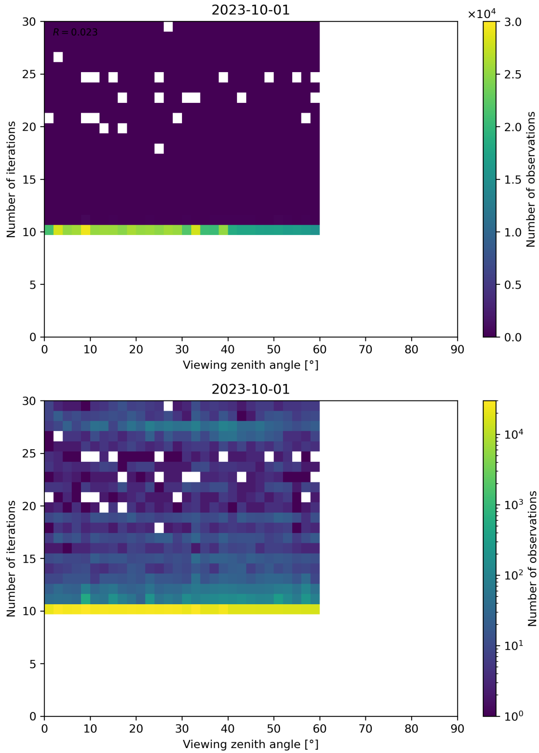
Figure 113: Scatter density plot of “Viewing zenith angle” against “Number of iterations” for 2023-10-01 to 2023-10-02.
