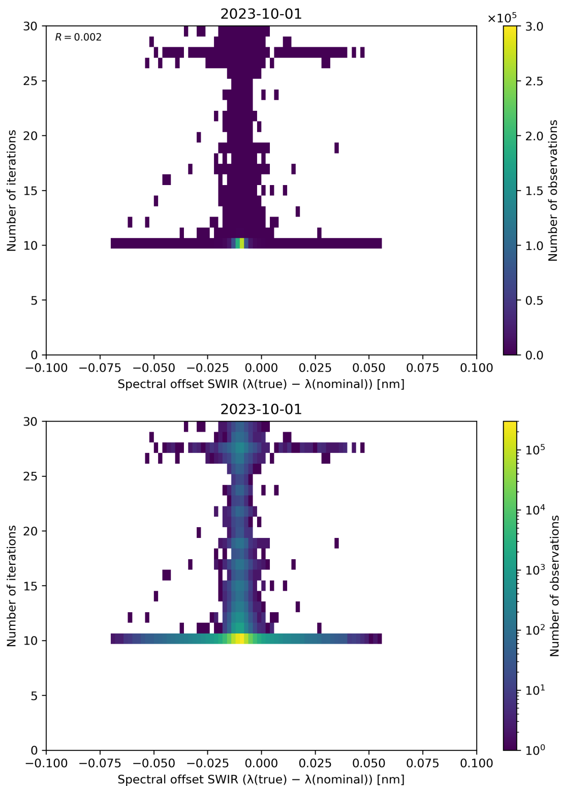
Figure 121: Scatter density plot of “Spectral offset SWIR ( \lambda(\text{true}) - \lambda(\text{nominal}) )” against “Number of iterations” for 2023-10-01 to 2023-10-02.
