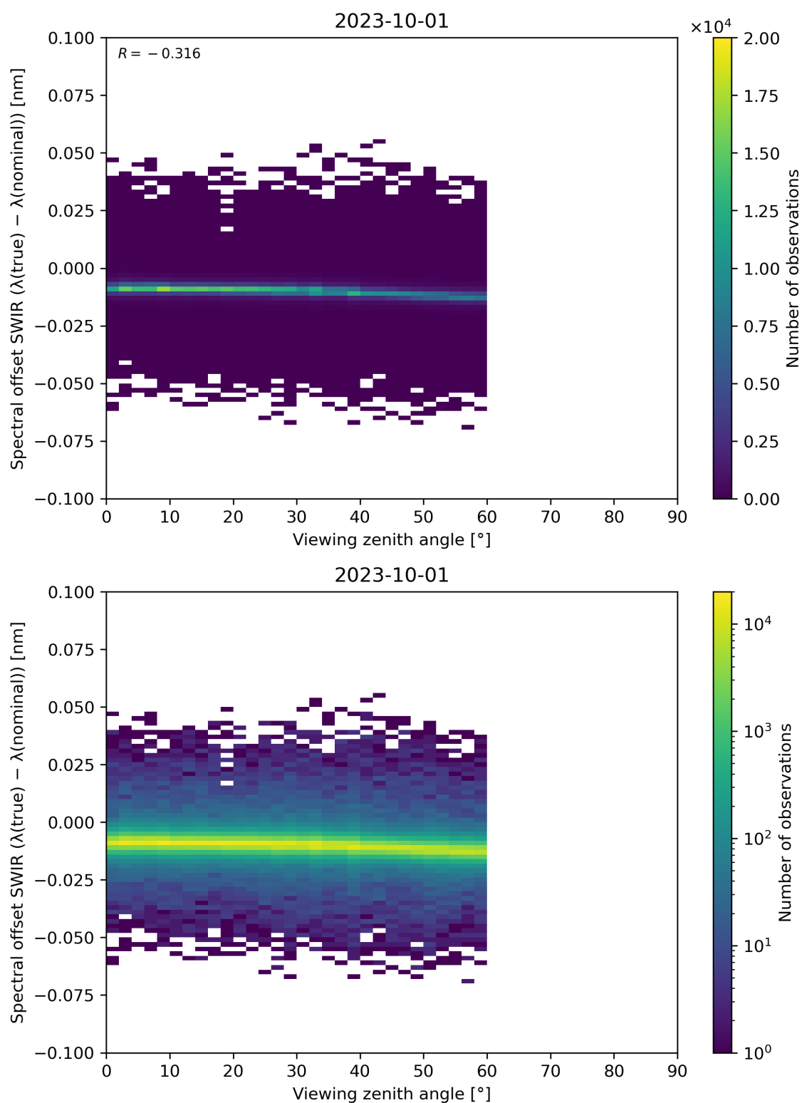
Figure 116: Scatter density plot of “Viewing zenith angle” against “Spectral offset SWIR ( \lambda(\text{true}) - \lambda(\text{nominal}) )” for 2023-10-01 to 2023-10-02.
