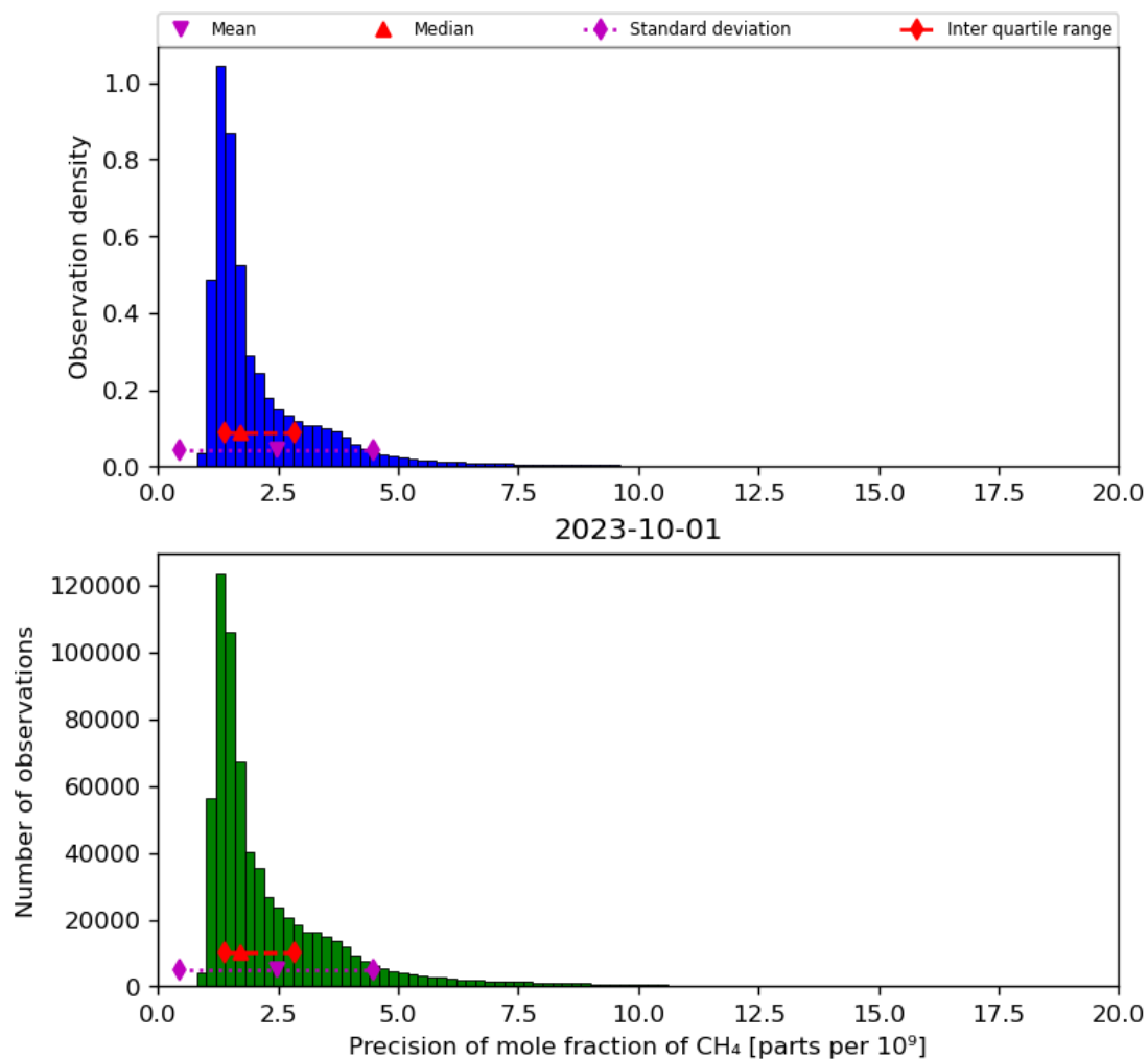
Figure 24: Histogram of “Precision of mole fraction of CH 4 ” for 2023-10-01 to 2023-10-02
