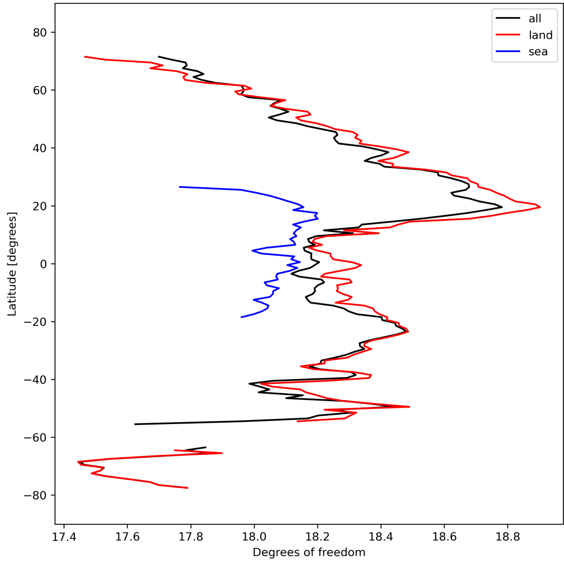
Figure 19: Zonal average of “Degrees of freedom” for 2023-10-01 to 2023-10-02.
