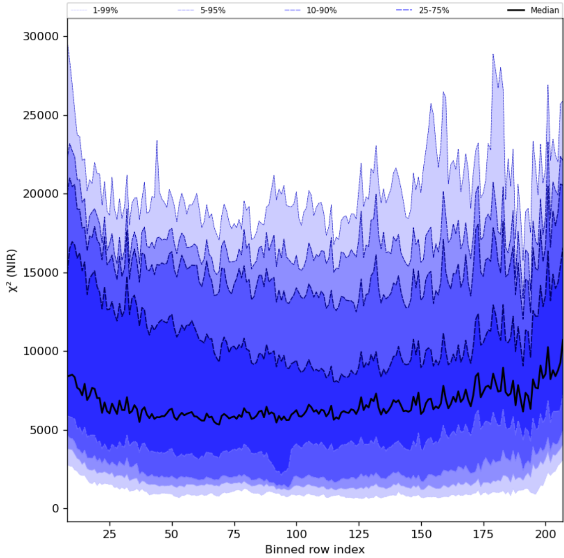
Figure 40: Along track statistics of “ \chi^2 (NIR)” for 2023-10-01 to 2023-10-02
