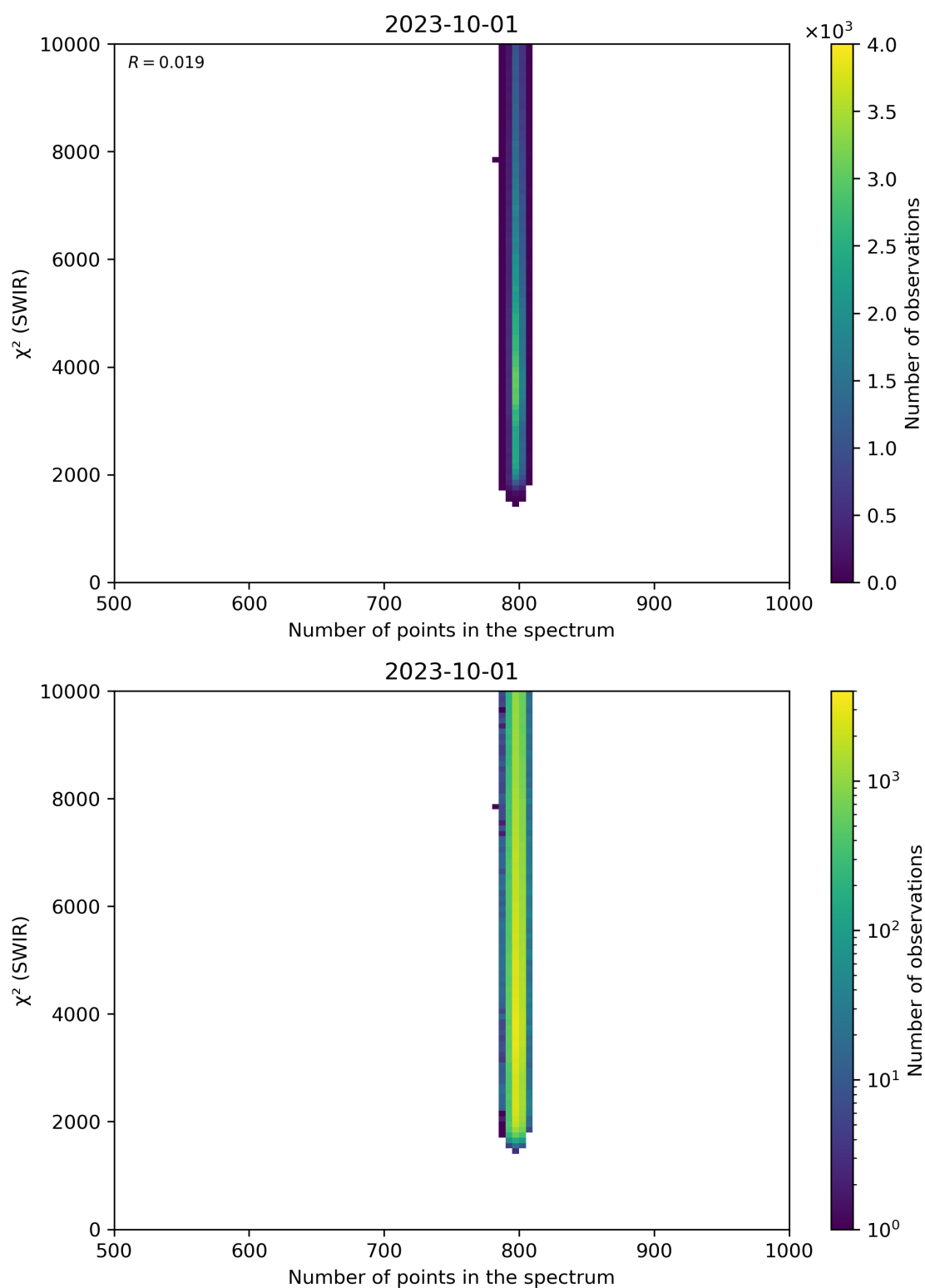
Figure 89: Scatter density plot of “Number of points in the spectrum” against “ \chi^2 (SWIR)” for 2023-10-01 to 2023-10-02.
