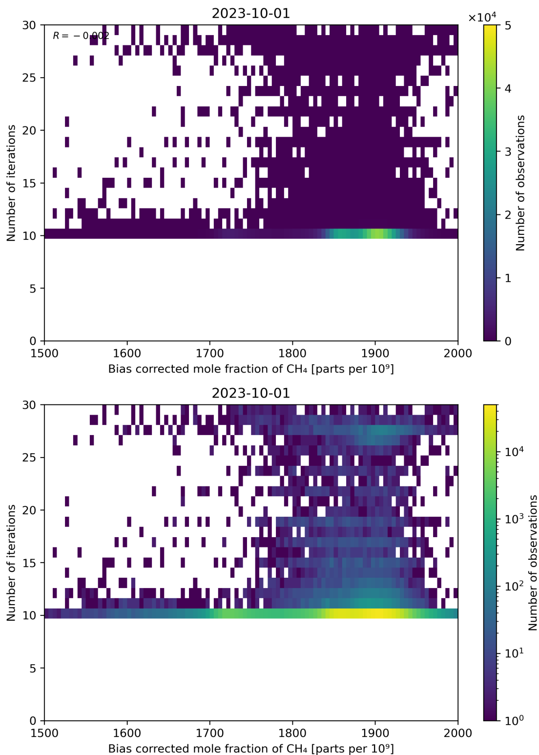
Figure 67: Scatter density plot of “Bias corrected mole fraction of CH 4 ” against “Number of iterations” for 2023-10-01 to 2023-10-02.
