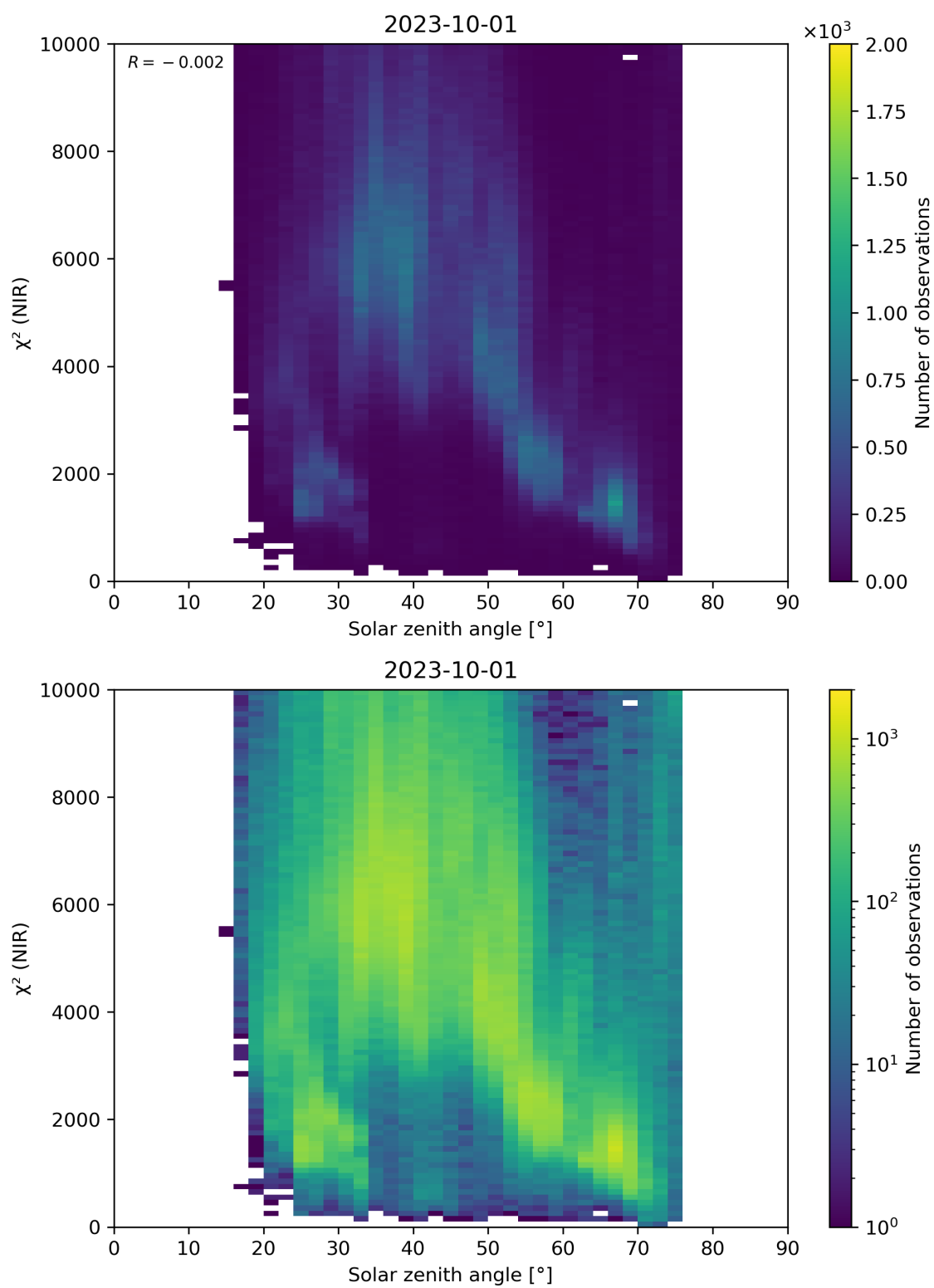
Figure 94: Scatter density plot of “Solar zenith angle” against “ \chi^2 (NIR)” for 2023-10-01 to 2023-10-02.
