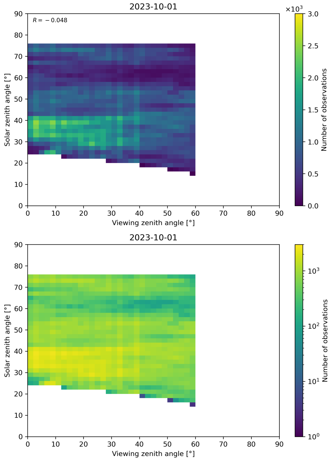
Figure 115: Scatter density plot of “Viewing zenith angle” against “Solar zenith angle” for 2023-10-01 to 2023-10-02.
