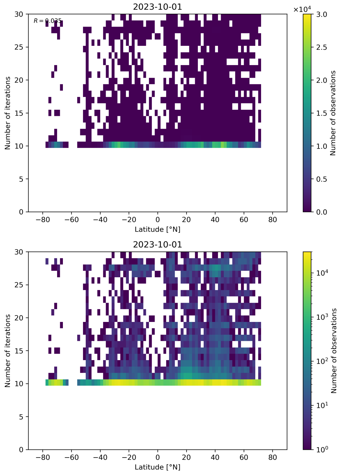
Figure 60: Scatter density plot of “Latitude” against “Number of iterations” for 2023-10-01 to 2023-10-02.
