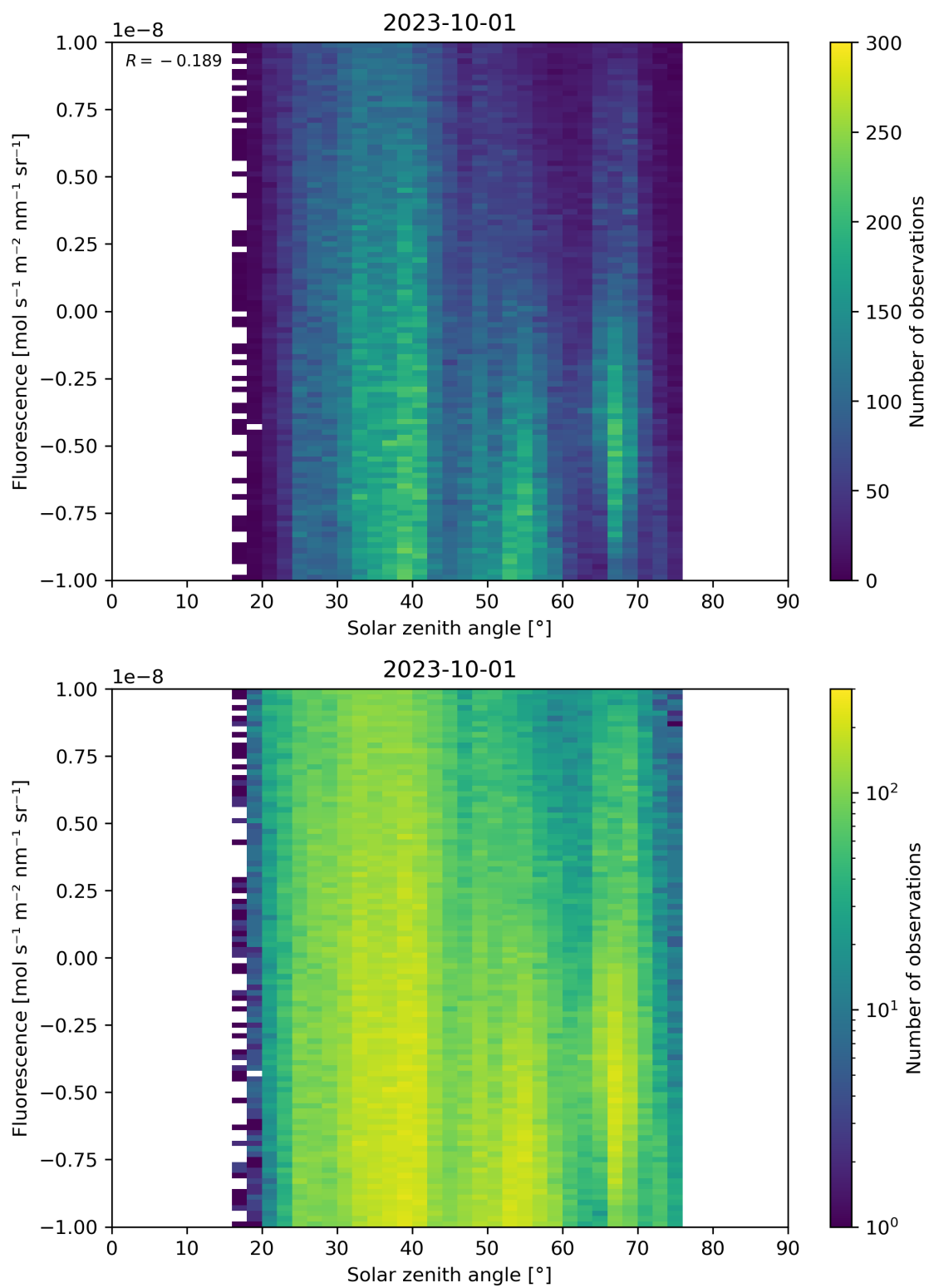
Figure 97: Scatter density plot of “Solar zenith angle” against “Fluorescence” for 2023-10-01 to 2023-10-02.
