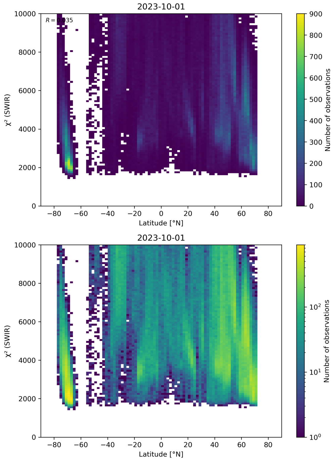
Figure 54: Scatter density plot of “Latitude” against “ \chi^2 (SWIR)” for 2023-10-01 to 2023-10-02.
