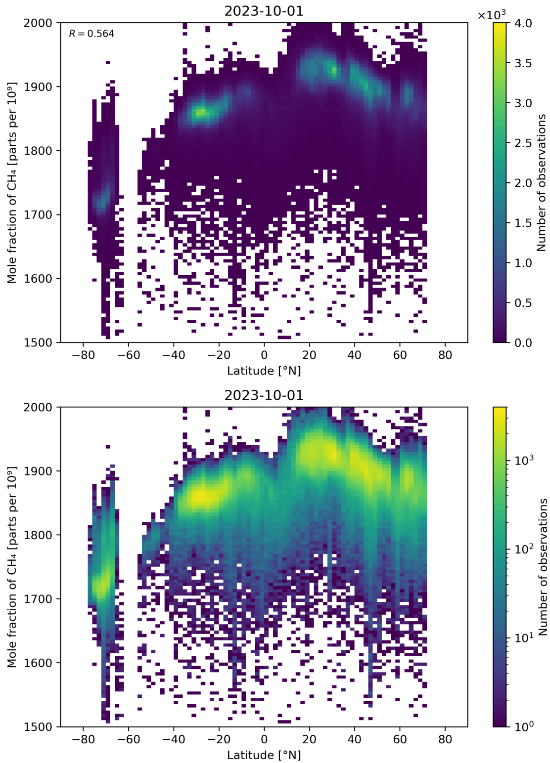
Figure 57: Scatter density plot of “Latitude” against “Mole fraction of CH 4 ” for 2023-10-01 to 2023-10-02.
