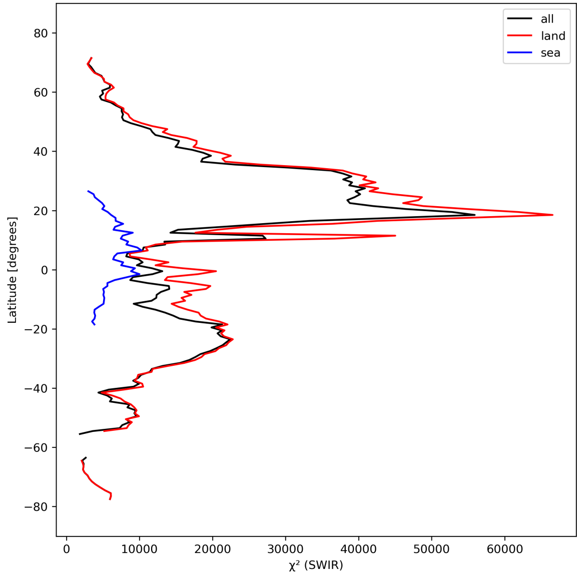
Figure 17: Zonal average of “ \chi^2 (SWIR)” for 2023-10-01 to 2023-10-02.
