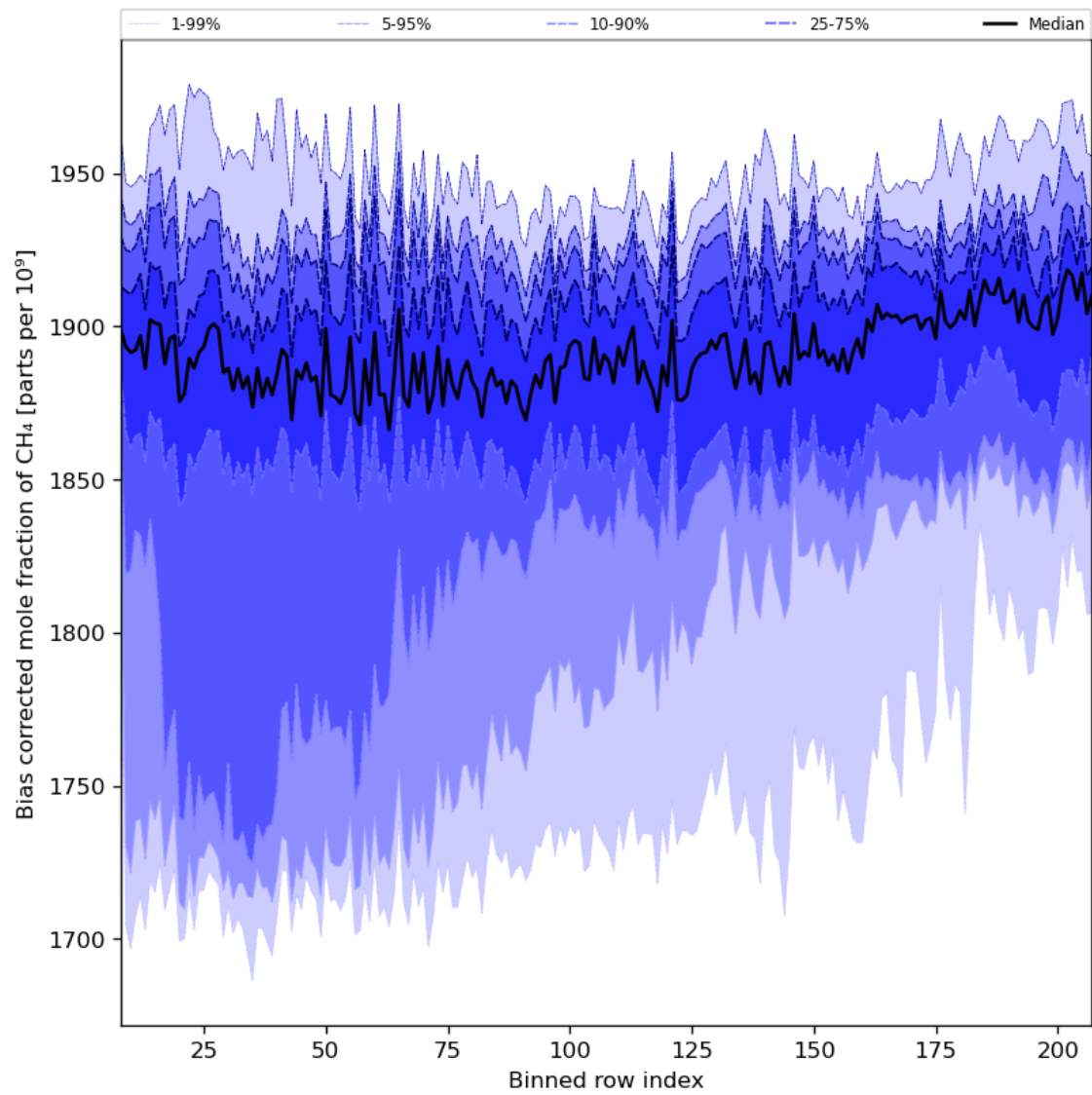
Figure 36: Along track statistics of “Bias corrected mole fraction of CH 4 ” for 2023-10-01 to 2023-10-02
