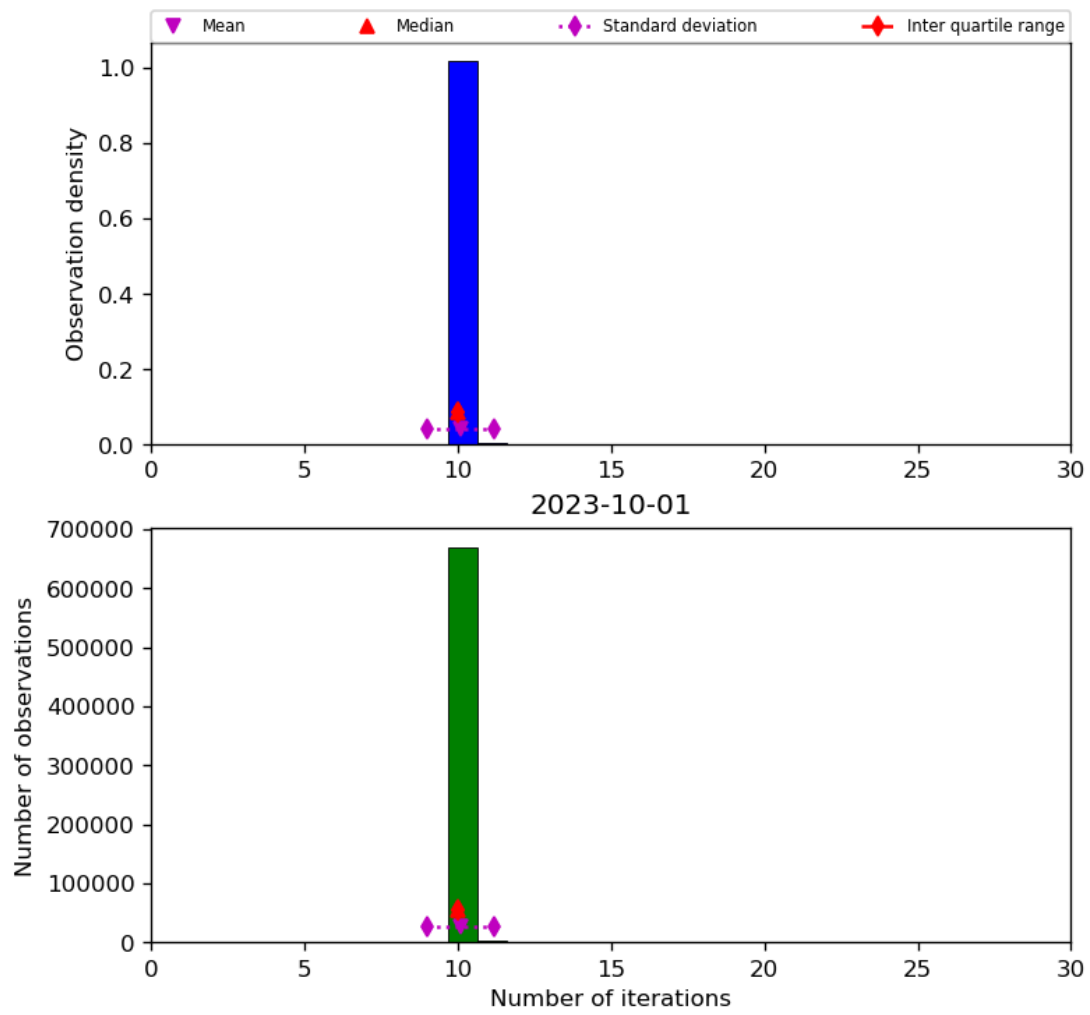
Figure 31: Histogram of “Number of iterations” for 2023-10-01 to 2023-10-02
