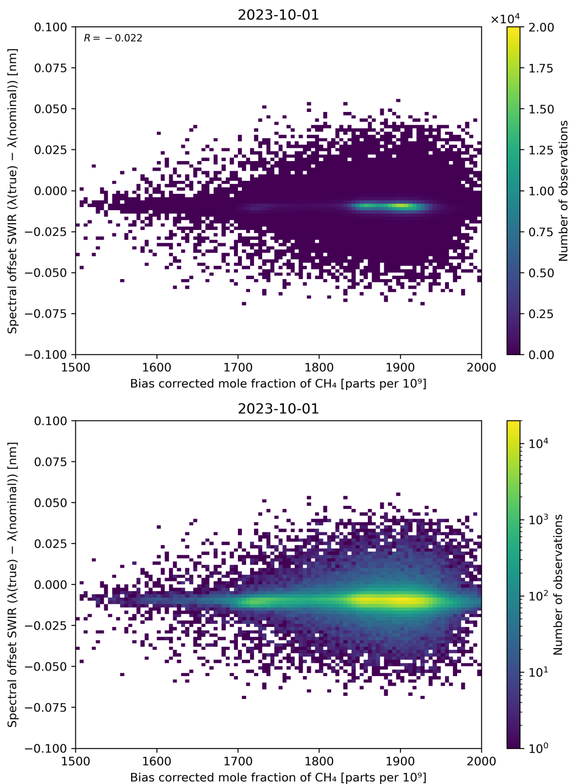
Figure 69: Scatter density plot of “Bias corrected mole fraction of CH 4 ” against “Spectral offset SWIR ( \lambda(\text{true}) - \lambda(\text{nominal}) )” for 2023-10-01 to 2023-10-02.
