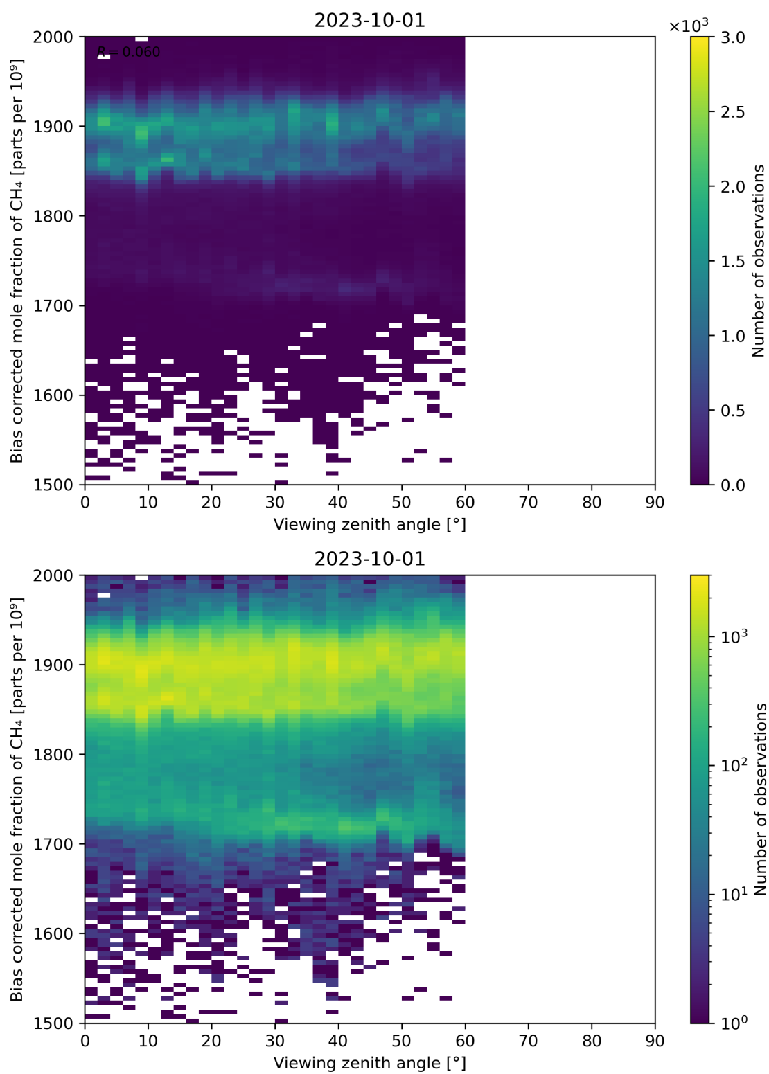
Figure 111: Scatter density plot of “Viewing zenith angle” against “Bias corrected mole fraction of CH 4 ” for 2023-10-01 to 2023-10-02.
