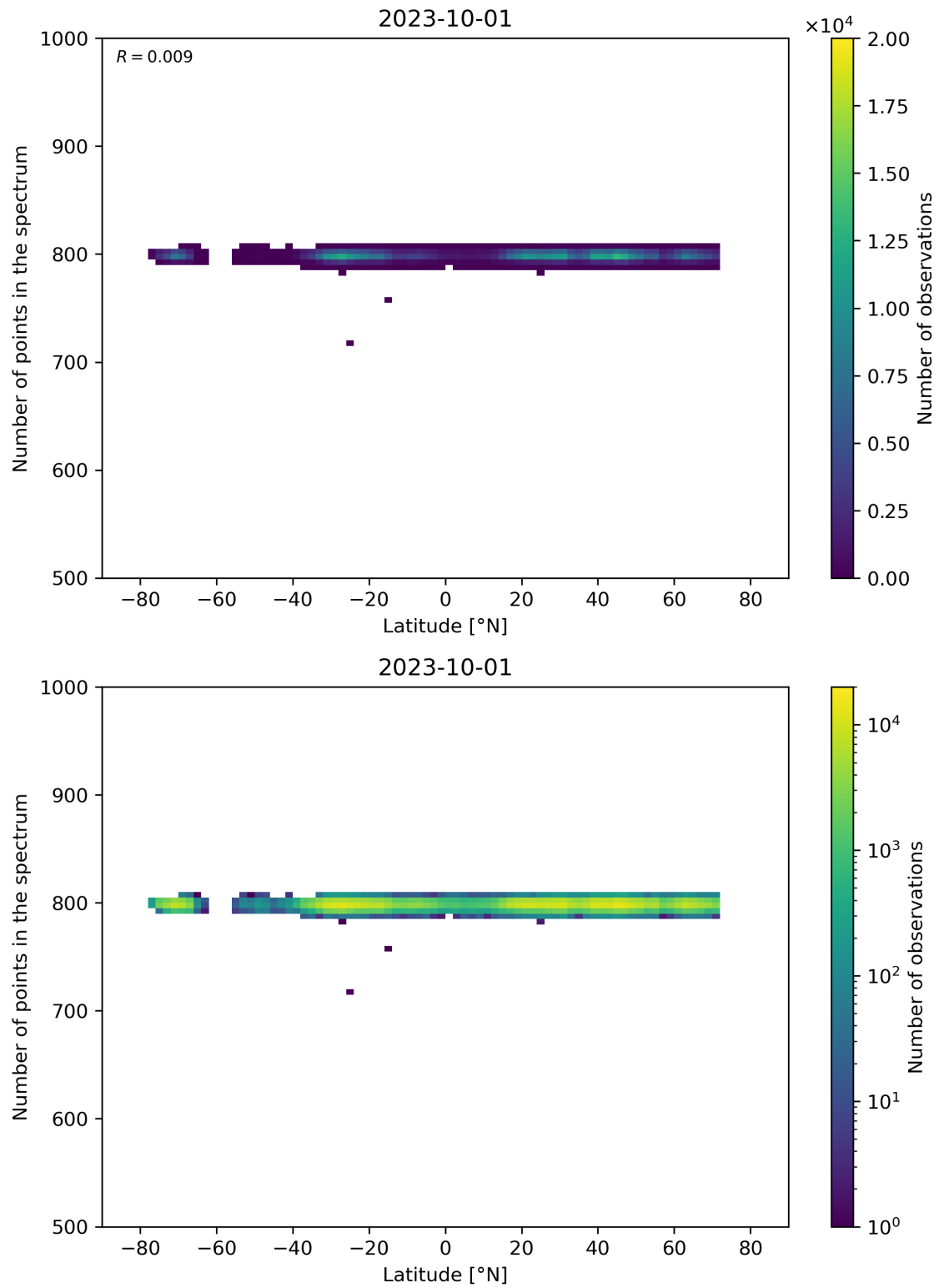
Figure 61: Scatter density plot of “Latitude” against “Number of points in the spectrum” for 2023-10-01 to 2023-10-02.
