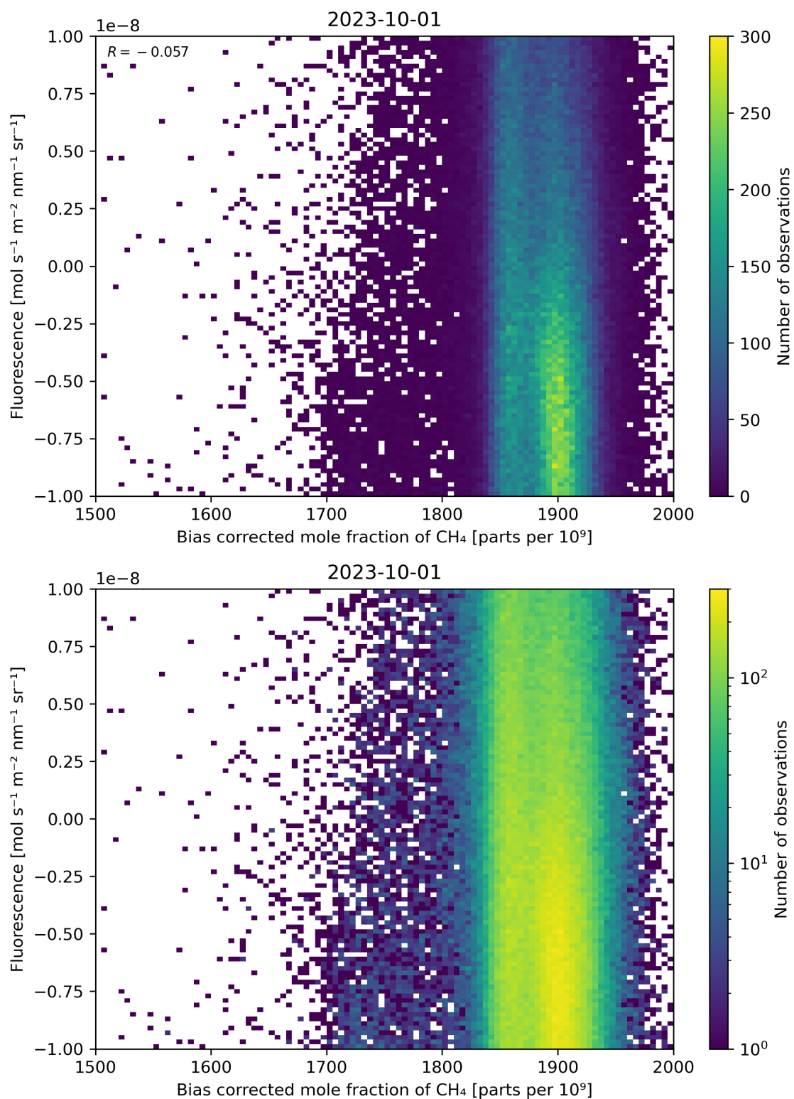
Figure 66: Scatter density plot of “Bias corrected mole fraction of \text{CH}_4 ” against “Fluorescence” for 2023-10-01 to 2023-10-02.
