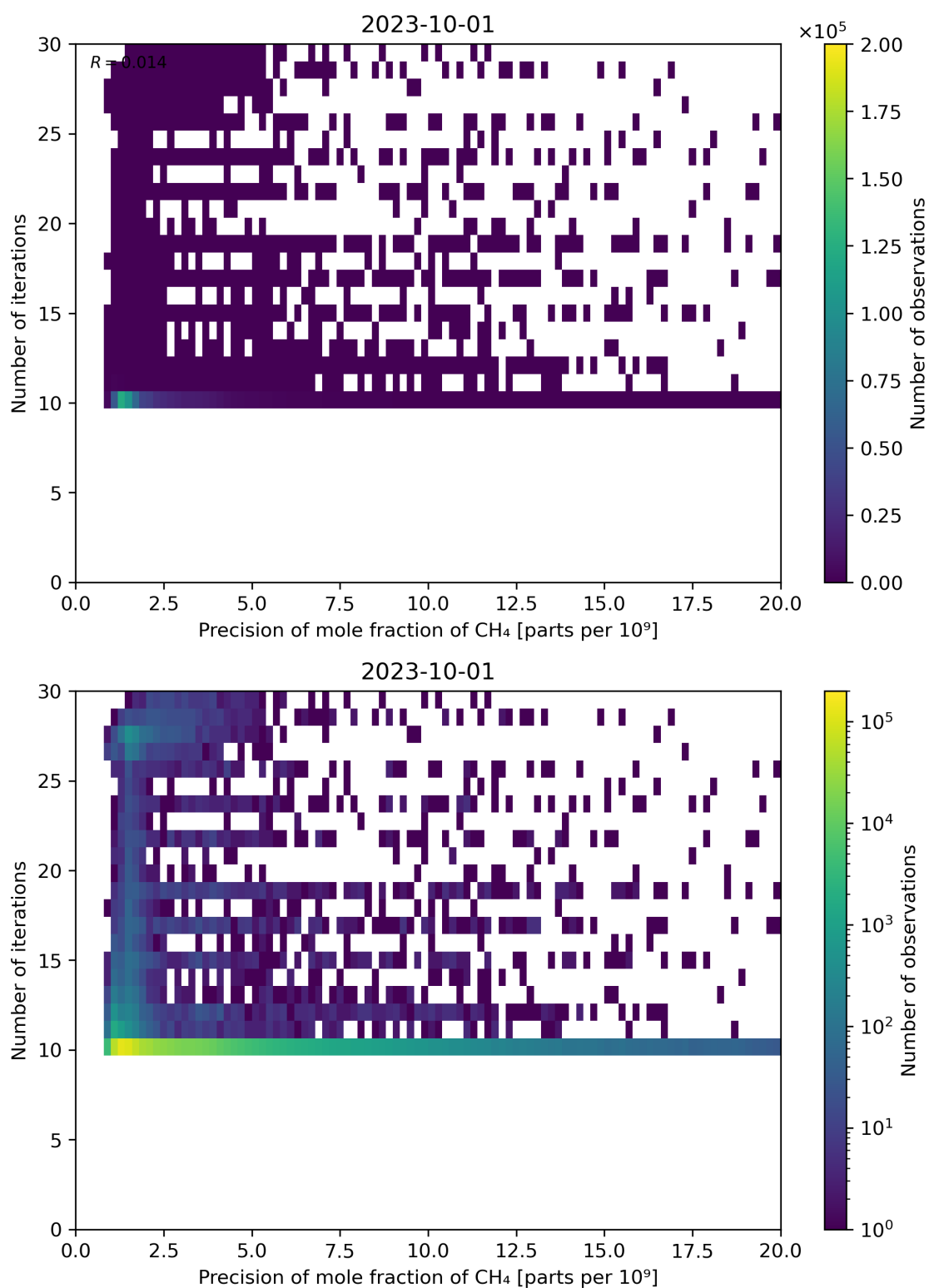
Figure 83: Scatter density plot of “Precision of mole fraction of CH 4 ” against “Number of iterations” for 2023-10-01 to 2023-10-02.
