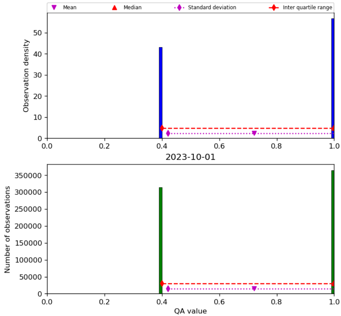
Figure 22: Histogram of “QA value” for 2023-10-01 to 2023-10-02
