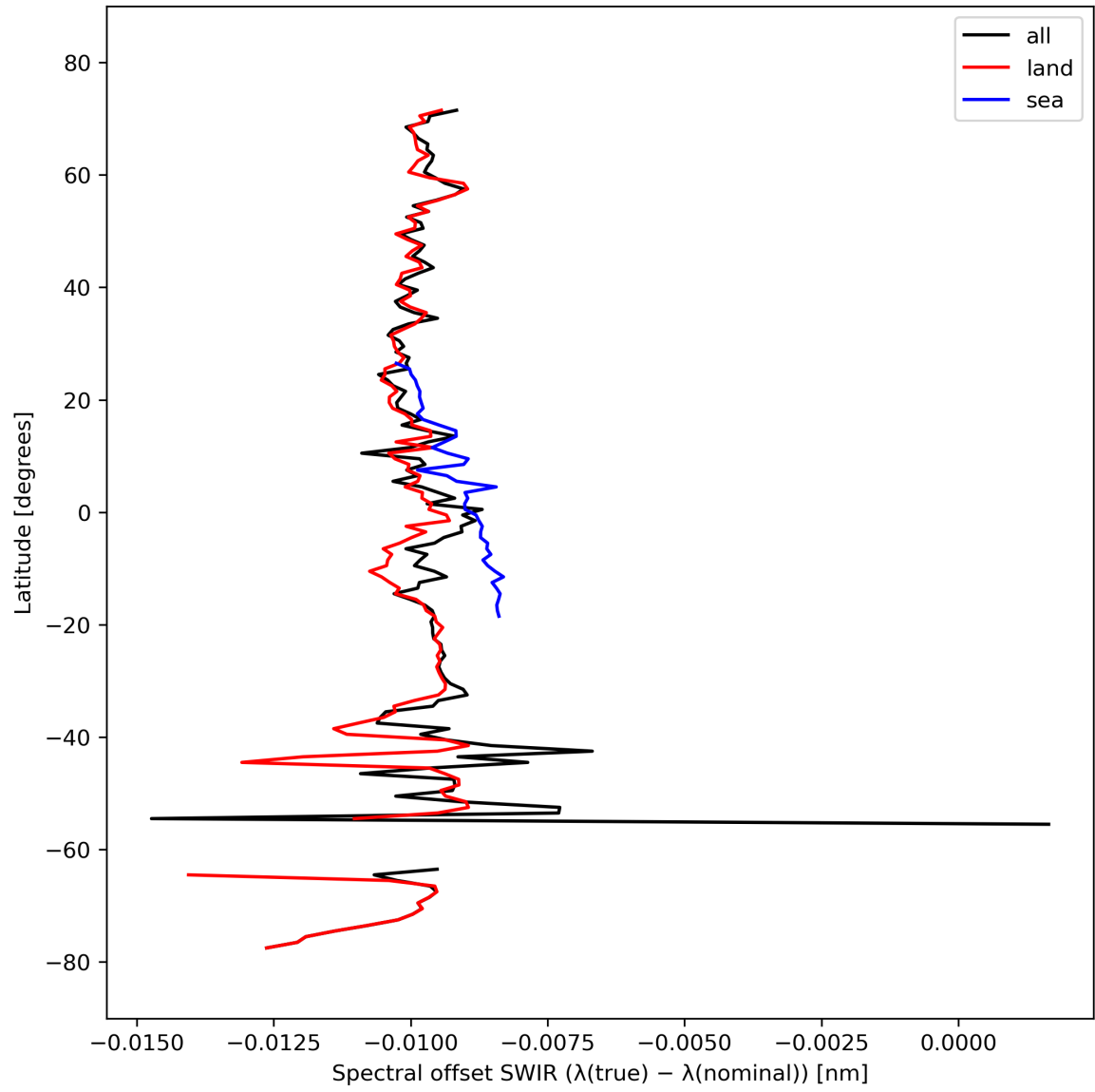
Figure 16: Zonal average of “Spectral offset SWIR ( \lambda(\text{true}) - \lambda(\text{nominal}) )” for 2023-10-01 to 2023-10-02.
