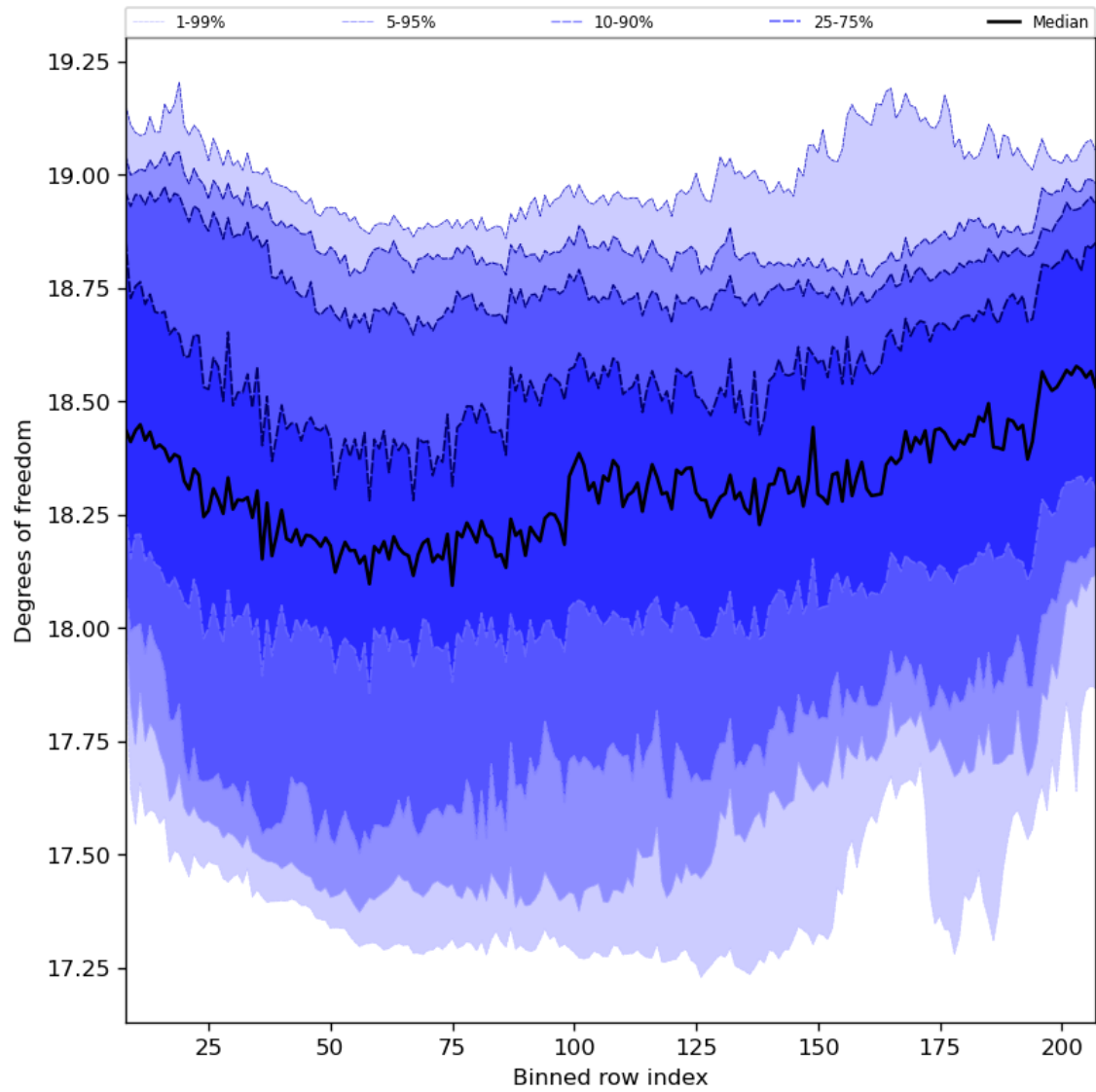
Figure 41: Along track statistics of “Degrees of freedom” for 2023-10-01 to 2023-10-02
