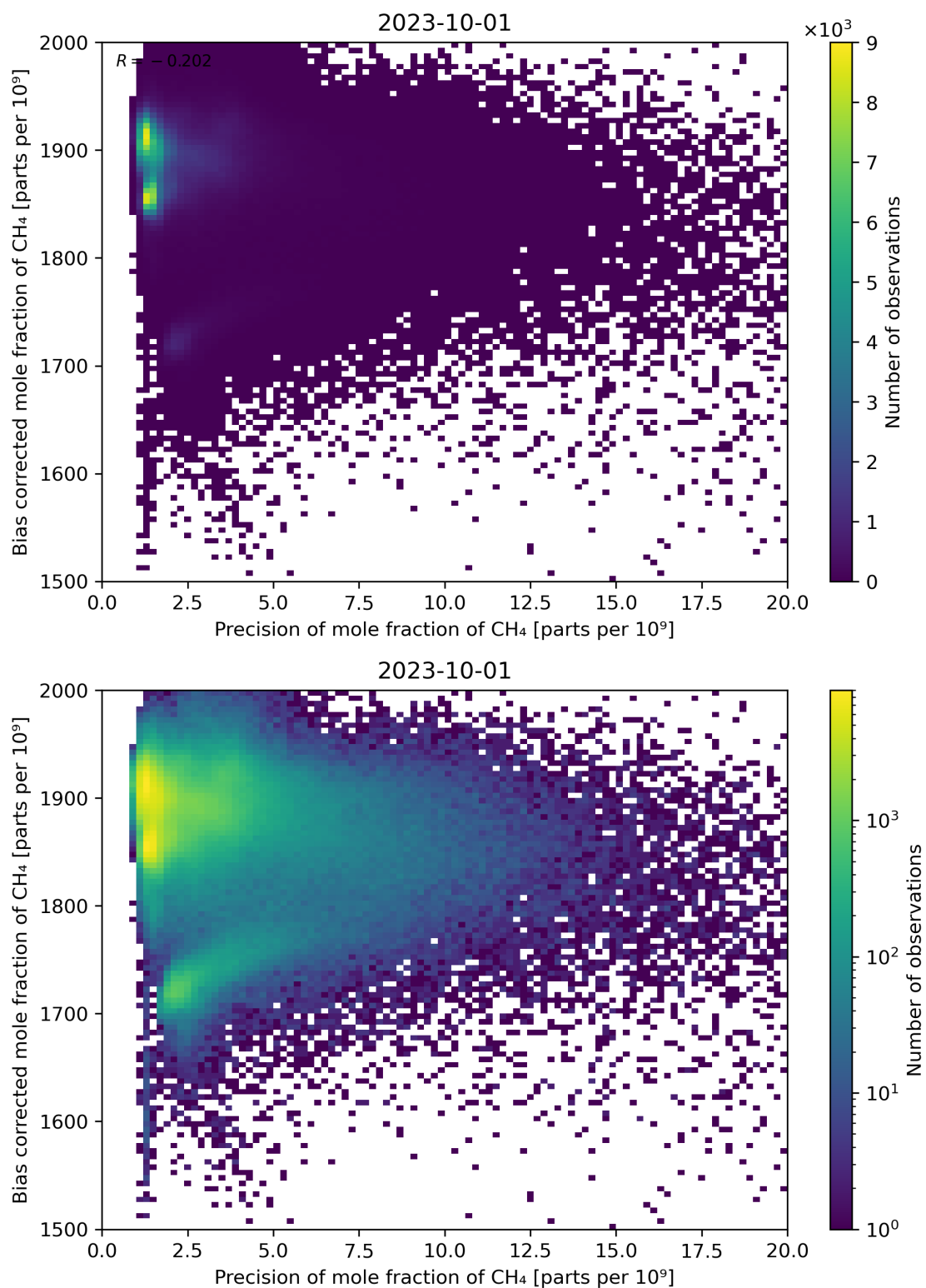
Figure 82: Scatter density plot of “Precision of mole fraction of CH 4 ” against “Bias corrected mole fraction of CH 4 ” for 2023-10-01 to 2023-10-02.
