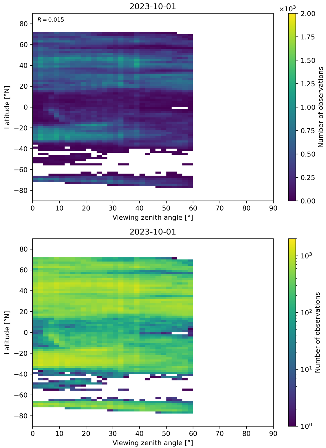
Figure 109: Scatter density plot of “Viewing zenith angle” against “Latitude” for 2023-10-01 to 2023-10-02.
