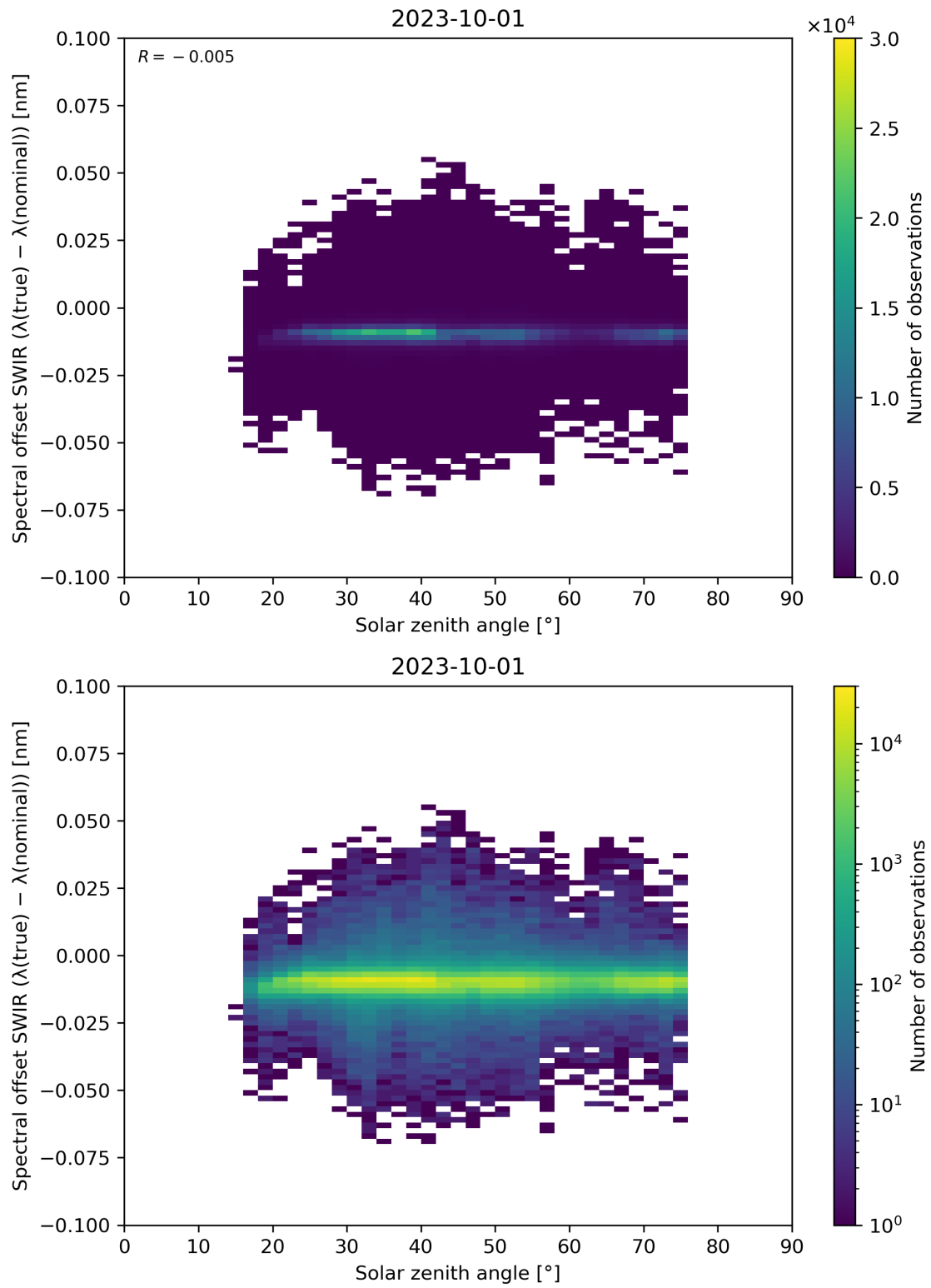
Figure 104: Scatter density plot of “Solar zenith angle” against “Spectral offset SWIR ( \lambda(\text{true}) - \lambda(\text{nominal}) )” for 2023-10-01 to 2023-10-02.
