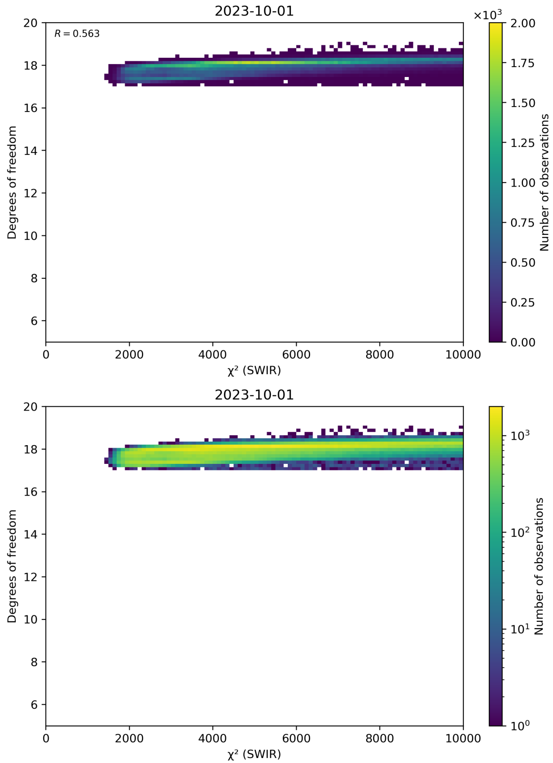
Figure 48: Scatter density plot of " \chi^2 (SWIR)" against "Degrees of freedom" for 2023-10-01 to 2023-10-02.
