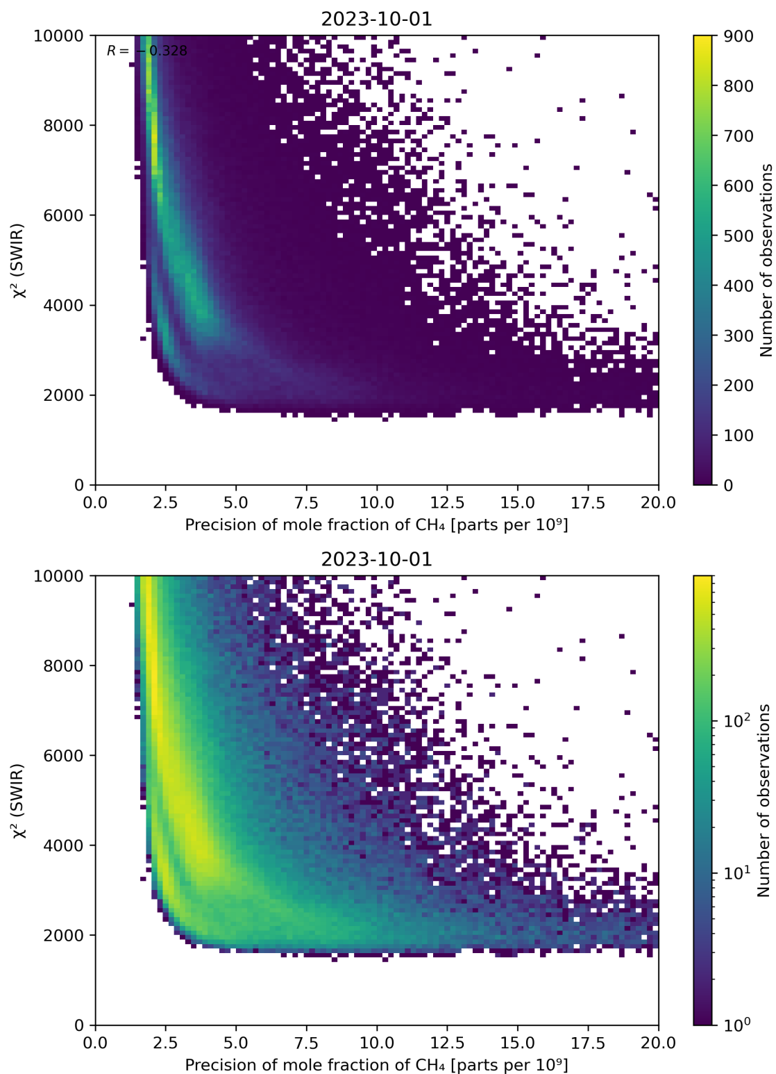
Figure 79: Scatter density plot of “Precision of mole fraction of \text{CH}_4 ” against “ \chi^2 (SWIR)” for 2023-10-01 to 2023-10-02.
