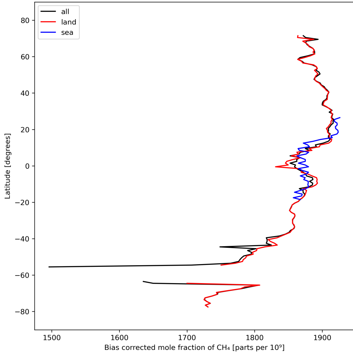
Figure 14: Zonal average of “Bias corrected mole fraction of CH 4 ” for 2023-10-01 to 2023-10-02.
