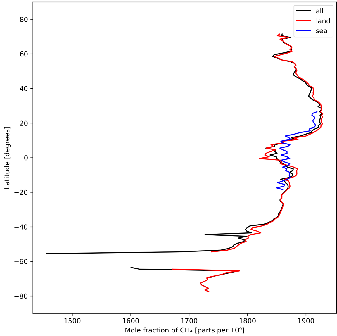
Figure 12: Zonal average of “Mole fraction of \text{CH}_4 ” for 2023-10-01 to 2023-10-02.
