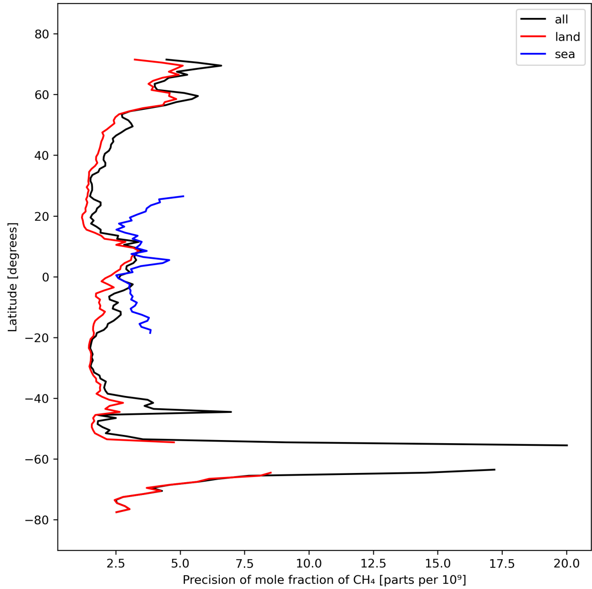
Figure 13: Zonal average of “Precision of mole fraction of CH 4 ” for 2023-10-01 to 2023-10-02.
