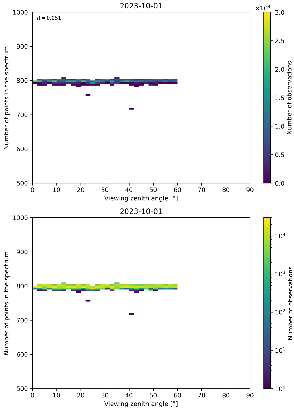
Figure 114: Scatter density plot of “Viewing zenith angle” against “Number of points in the spectrum” for 2023-10-01 to 2023-10-02.
