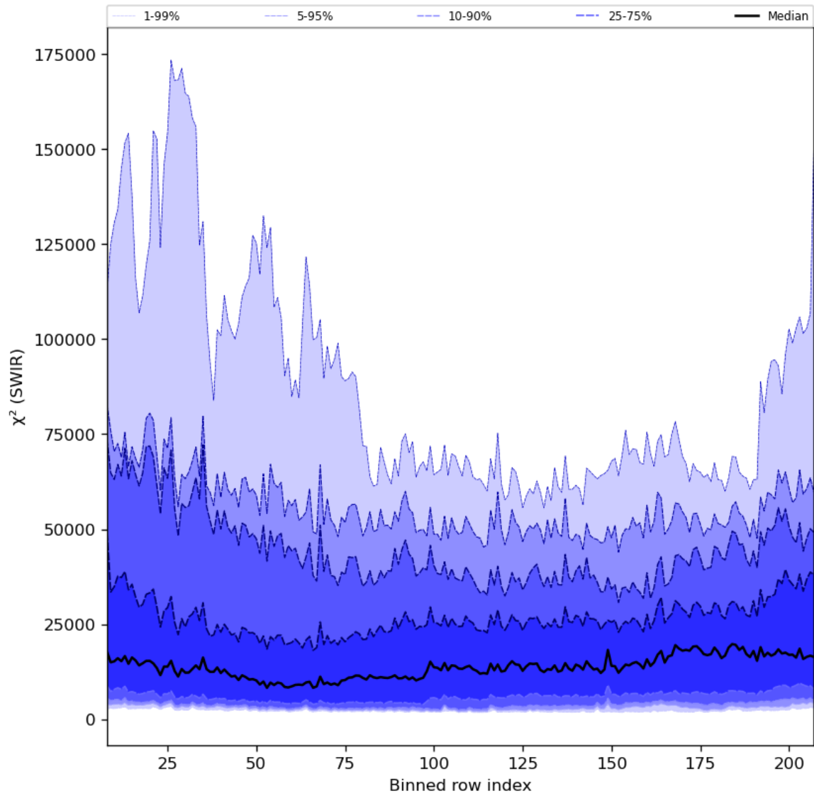
Figure 39: Along track statistics of " \chi^2 (SWIR)" for 2023-10-01 to 2023-10-02
