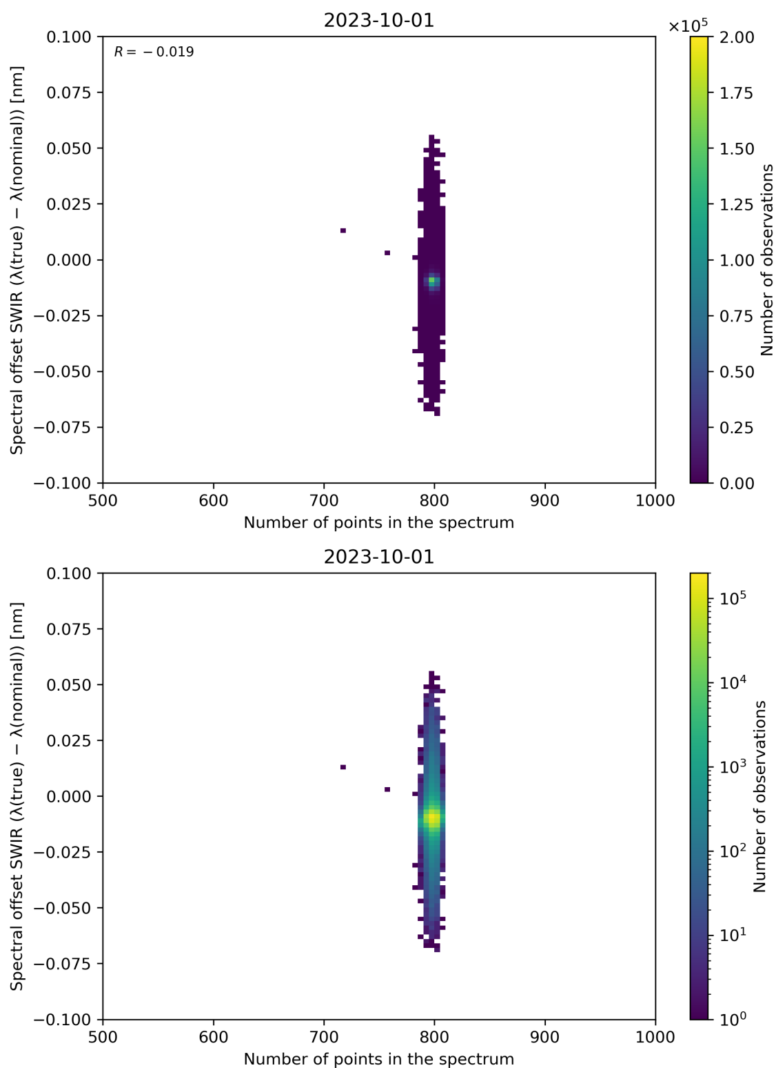
Figure 93: Scatter density plot of “Number of points in the spectrum” against “Spectral offset SWIR ( \lambda(\text{true}) - \lambda(\text{nominal}) )” for 2023-10-01 to 2023-10-02.
