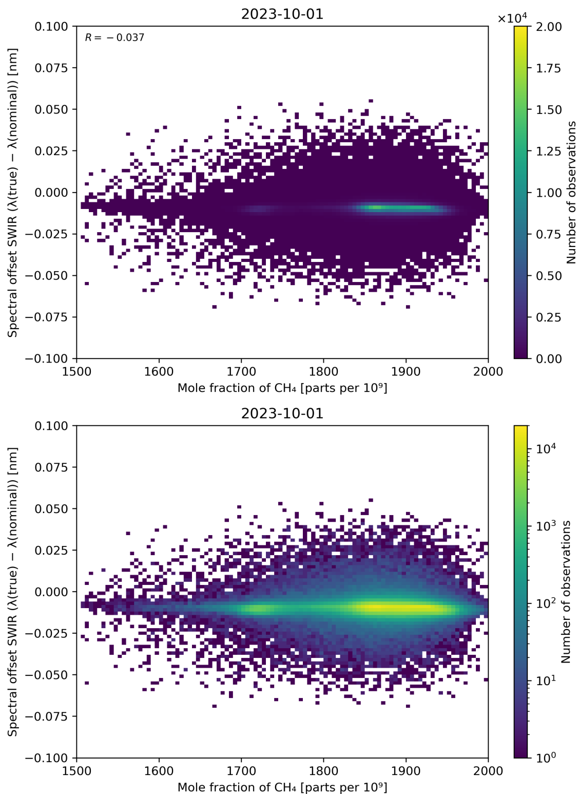
Figure 86: Scatter density plot of “Mole fraction of CH 4 ” against “Spectral offset SWIR ( \lambda(\text{true}) - \lambda(\text{nominal}) )” for 2023-10-01 to 2023-10-02.
