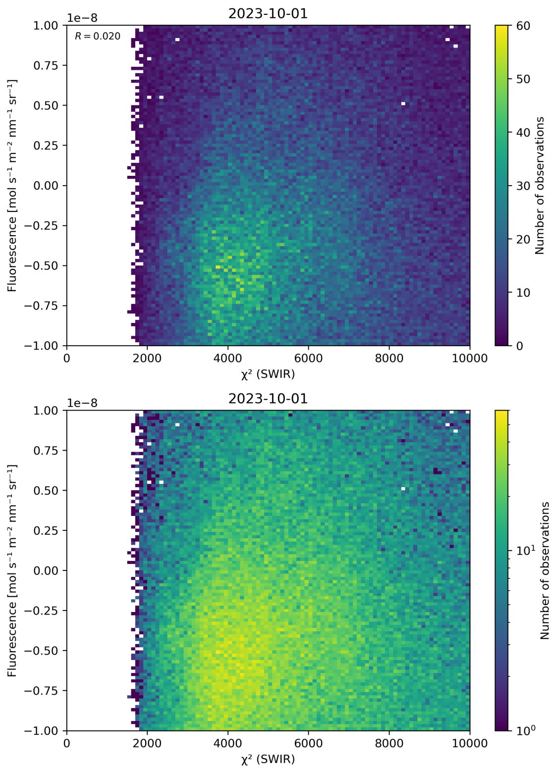
Figure 49: Scatter density plot of “ \chi^2 (SWIR)” against “Fluorescence” for 2023-10-01 to 2023-10-02.
