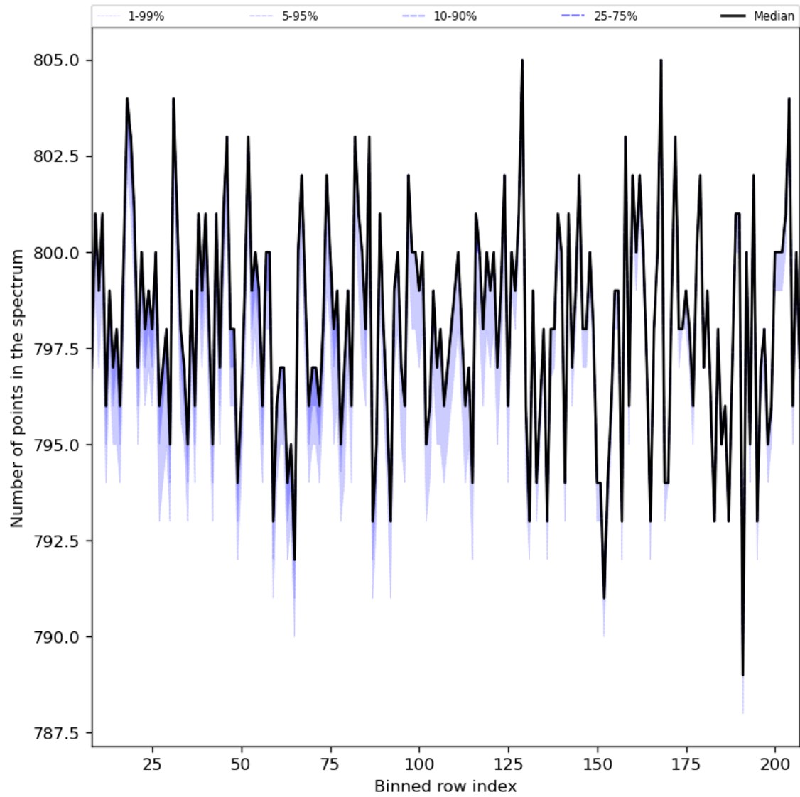
Figure 37: Along track statistics of “Number of points in the spectrum” for 2023-10-01 to 2023-10-02
