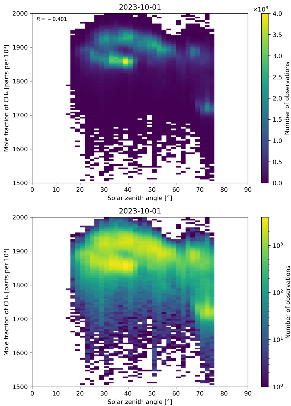
Figure 99: Scatter density plot of “Solar zenith angle” against “Mole fraction of \text{CH}_4 ” for 2023-10-01 to 2023-10-02.
