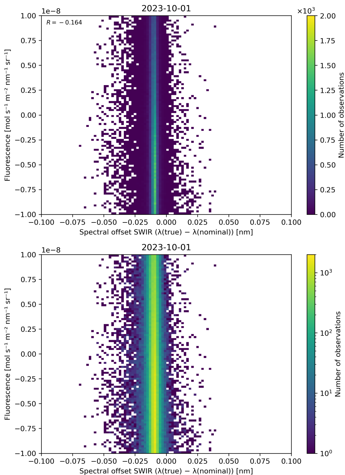
Figure 120: Scatter density plot of “Spectral offset SWIR ( \lambda(\text{true}) - \lambda(\text{nominal}) )” against “Fluorescence” for 2023-10-01 to 2023-10-02.
