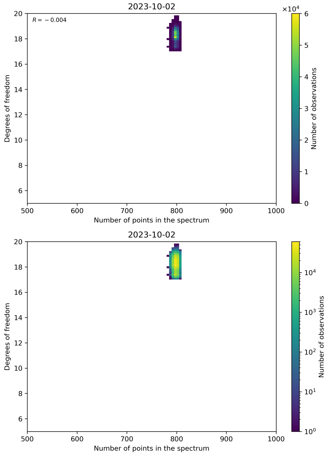
Figure 90: Scatter density plot of “Number of points in the spectrum” against “Degrees of freedom” for 2023-10-01 to 2023-10-03.
