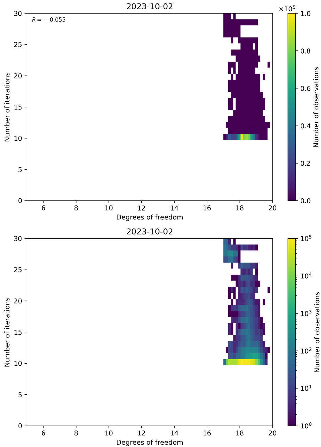
Figure 52: Scatter density plot of “Degrees of freedom” against “Number of iterations” for 2023-10-01 to 2023-10-03.
