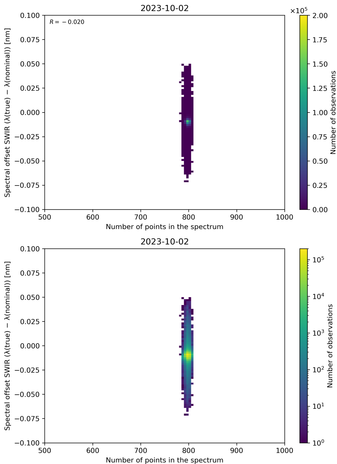
Figure 93: Scatter density plot of “Number of points in the spectrum” against “Spectral offset SWIR ( \lambda(\text{true}) - \lambda(\text{nominal})) ” for 2023-10-01 to 2023-10-03.
