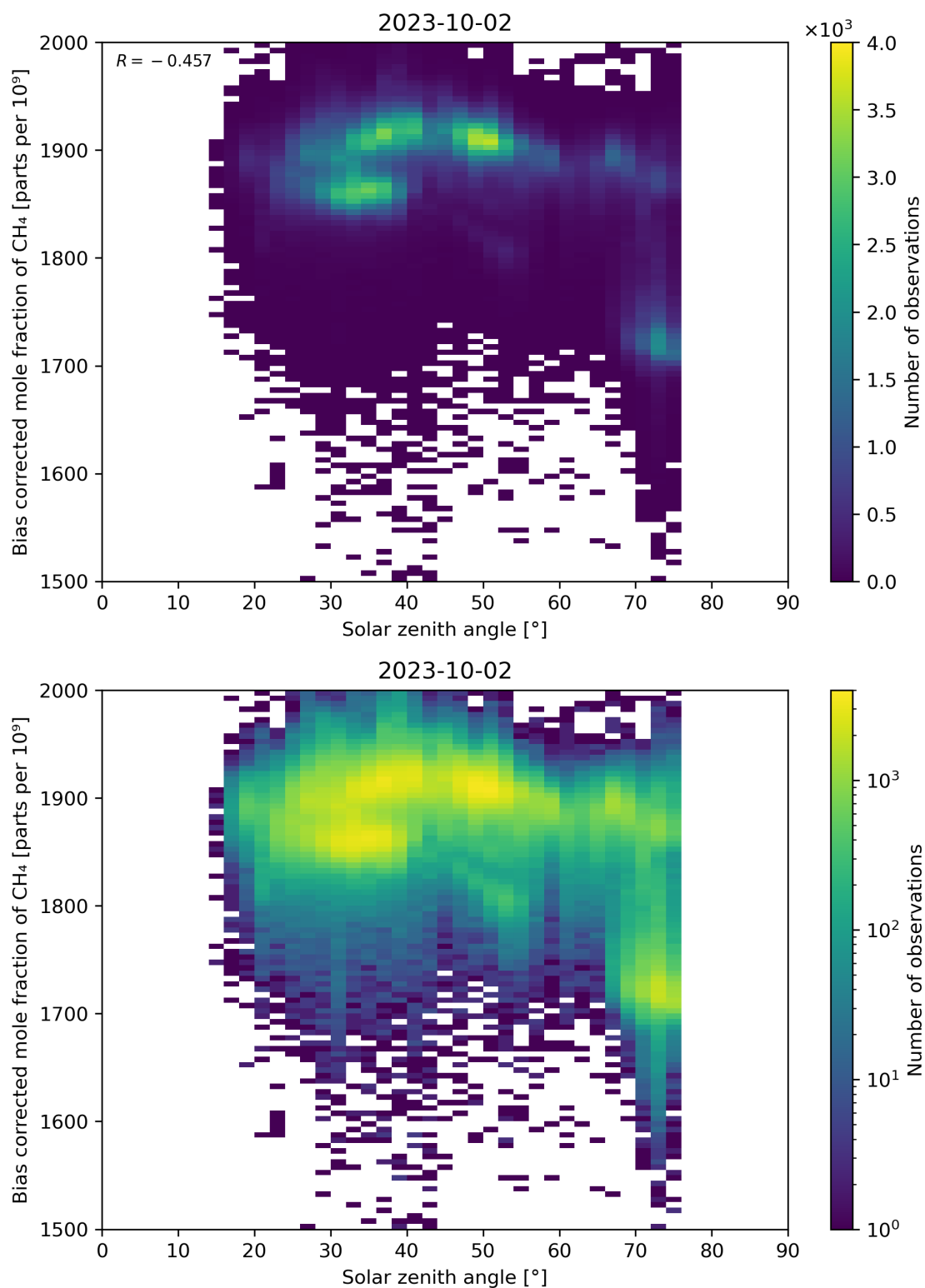
Figure 100: Scatter density plot of “Solar zenith angle” against “Bias corrected mole fraction of \text{CH}_4 ” for 2023-10-01 to 2023-10-03.
