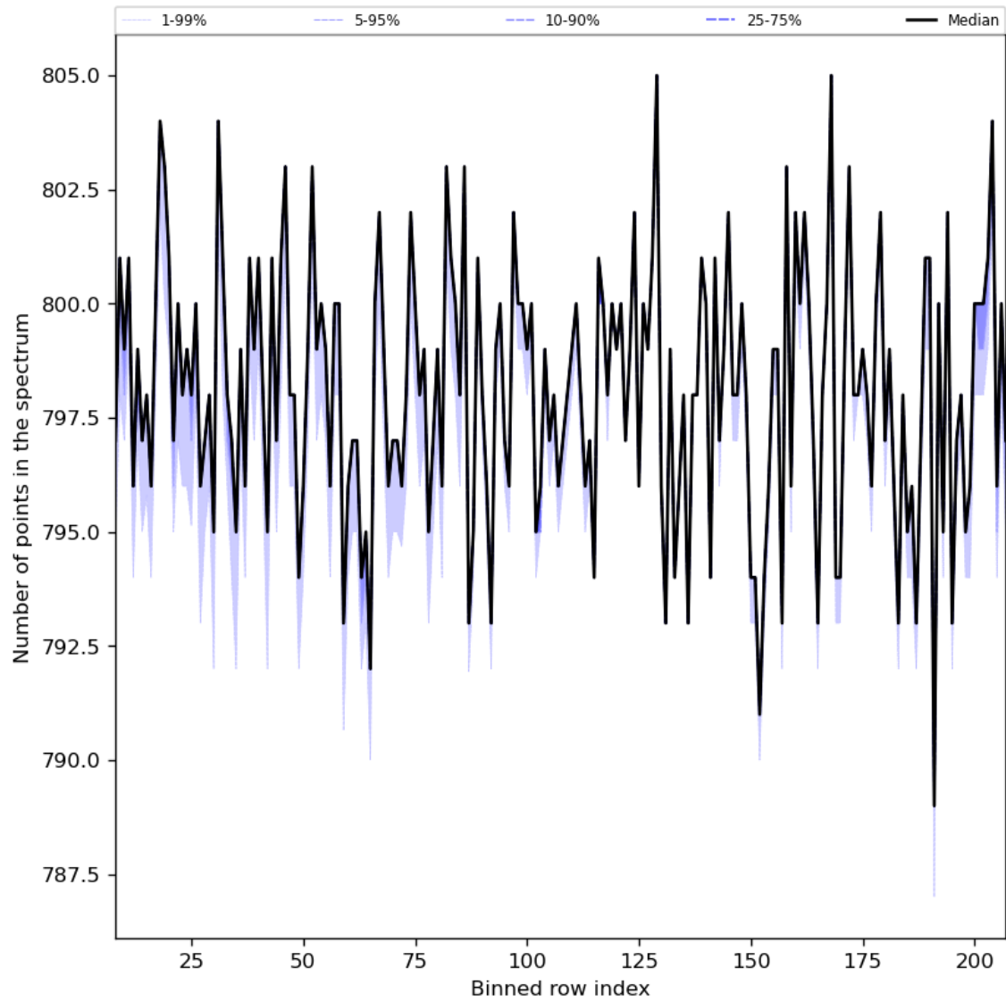
Figure 37: Along track statistics of “Number of points in the spectrum” for 2023-10-01 to 2023-10-03
