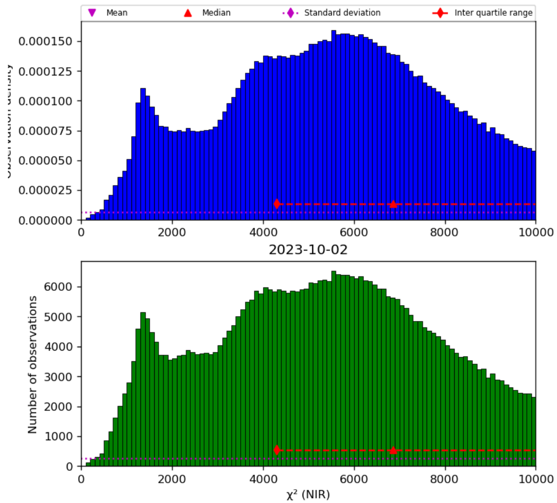
Figure 29: Histogram of “ \chi^2 (NIR)” for 2023-10-01 to 2023-10-03
