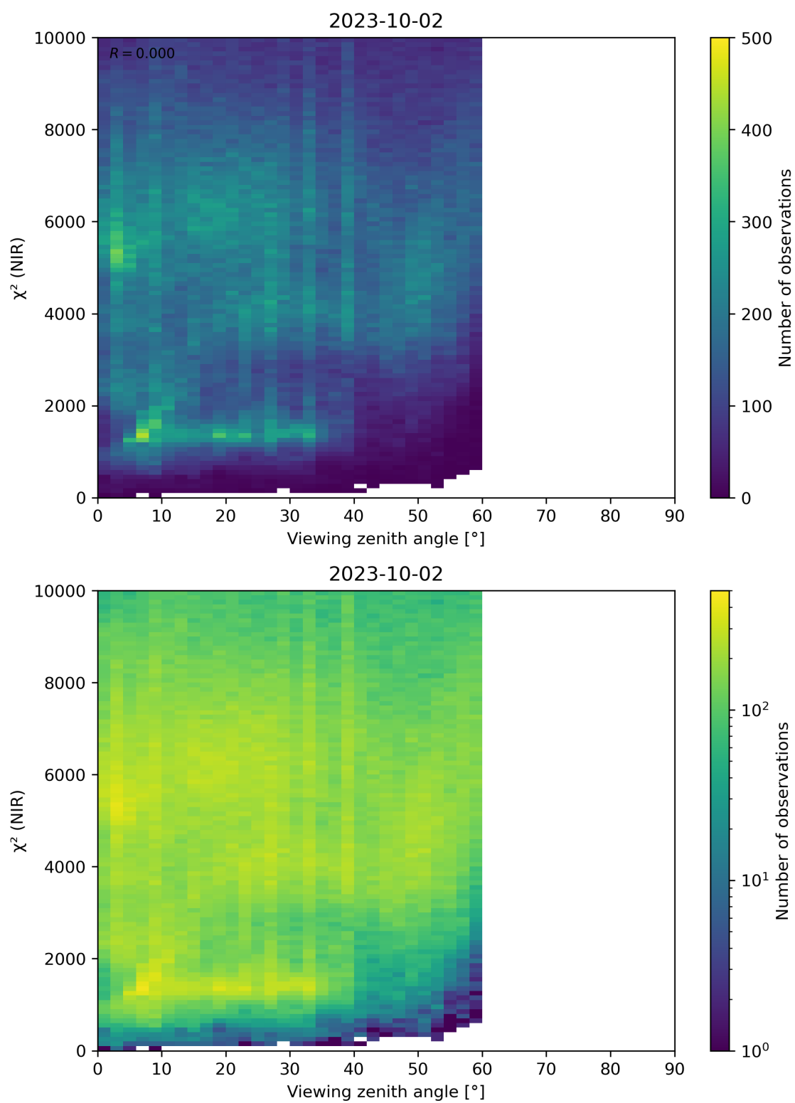
Figure 105: Scatter density plot of “Viewing zenith angle” against “ \chi^2 (NIR)” for 2023-10-01 to 2023-10-03.
