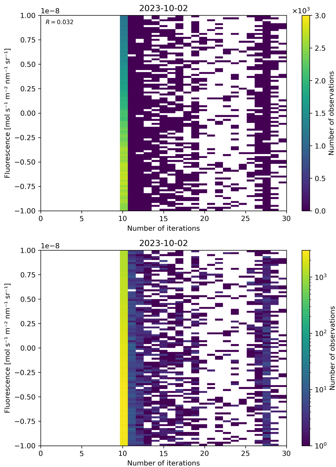
Figure 87: Scatter density plot of “Number of iterations” against “Fluorescence” for 2023-10-01 to 2023-10-03.
