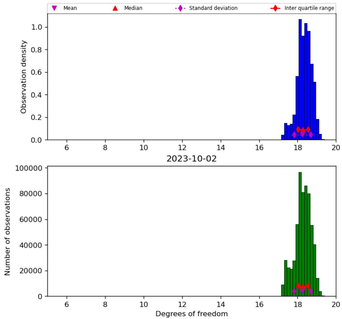
Figure 30: Histogram of “Degrees of freedom” for 2023-10-01 to 2023-10-03
