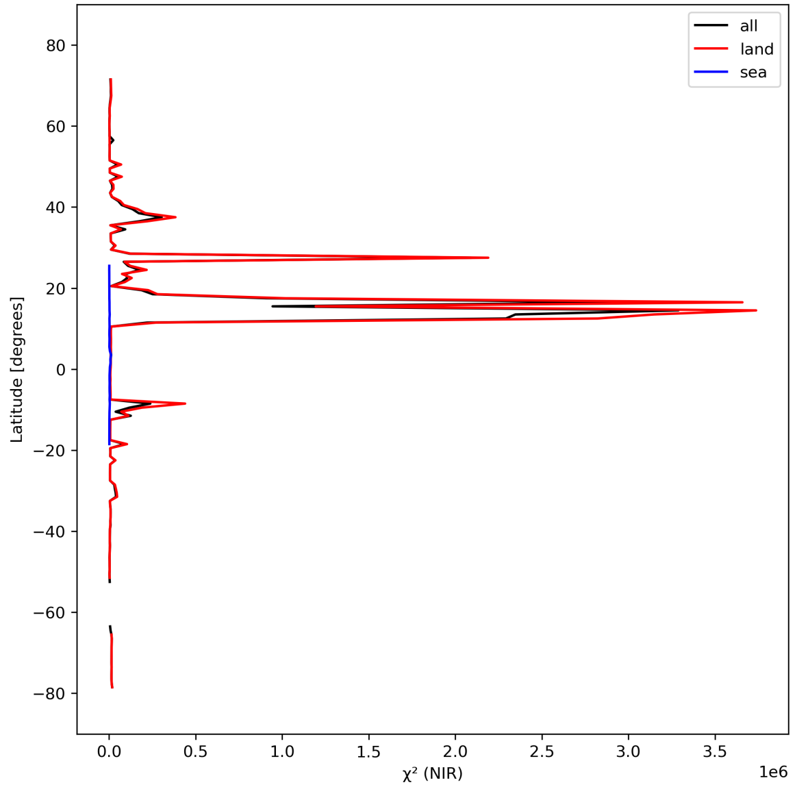
Figure 18: Zonal average of “ \chi^2 (NIR)” for 2023-10-01 to 2023-10-03.
