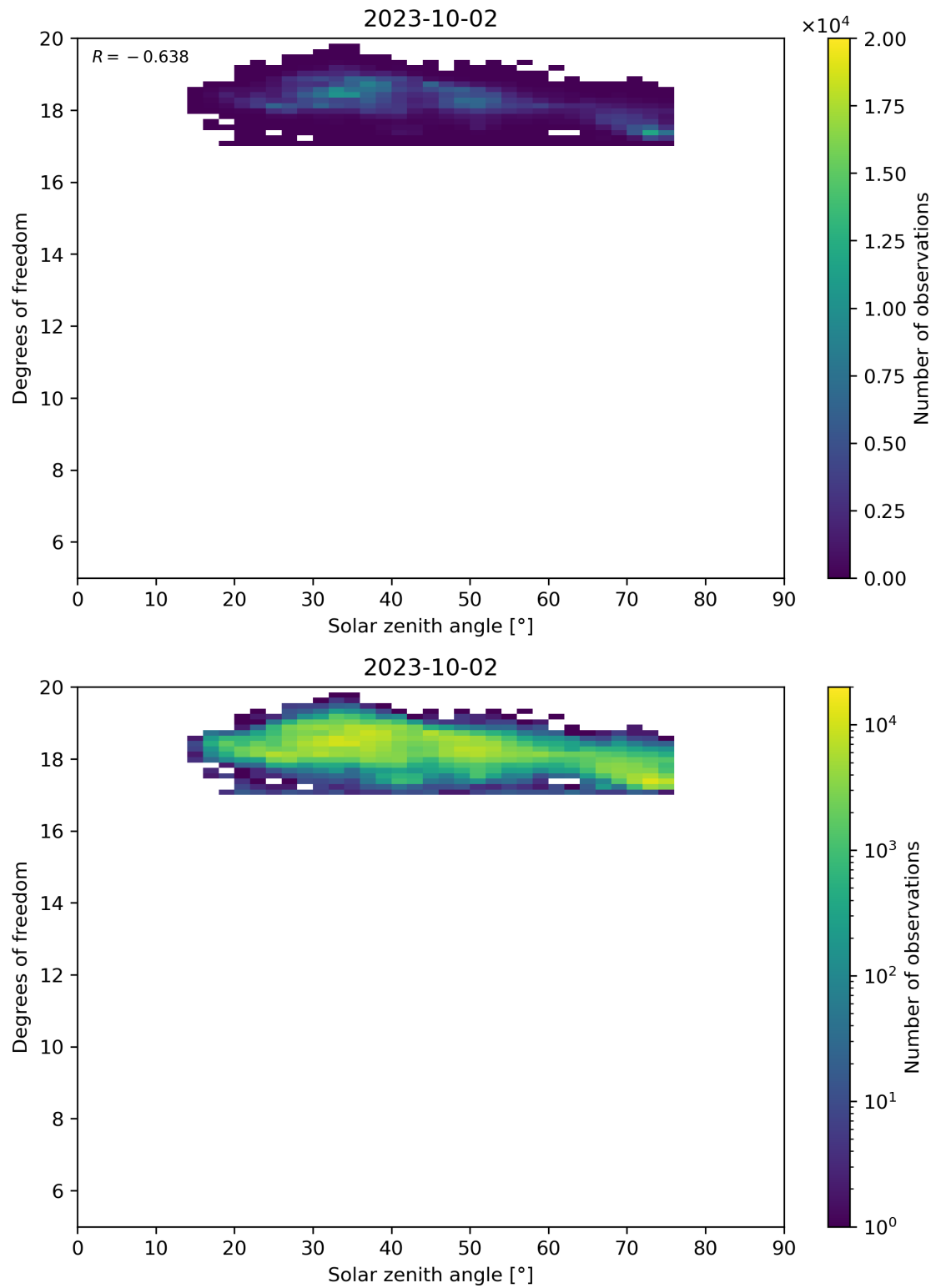
Figure 96: Scatter density plot of “Solar zenith angle” against “Degrees of freedom” for 2023-10-01 to 2023-10-03.
