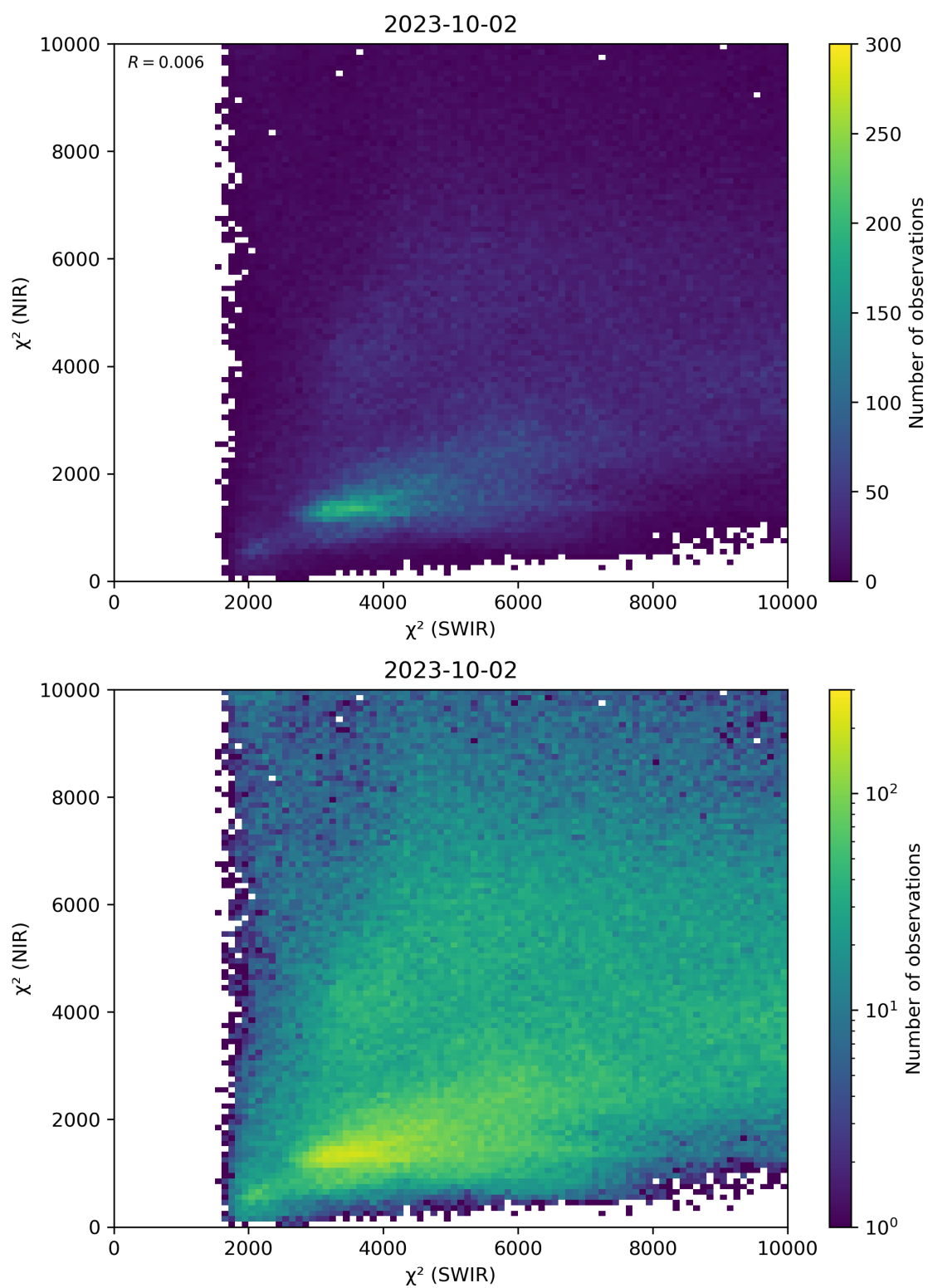
Figure 47: Scatter density plot of “ \chi^2 (SWIR)” against “ \chi^2 (NIR)” for 2023-10-01 to 2023-10-03.
