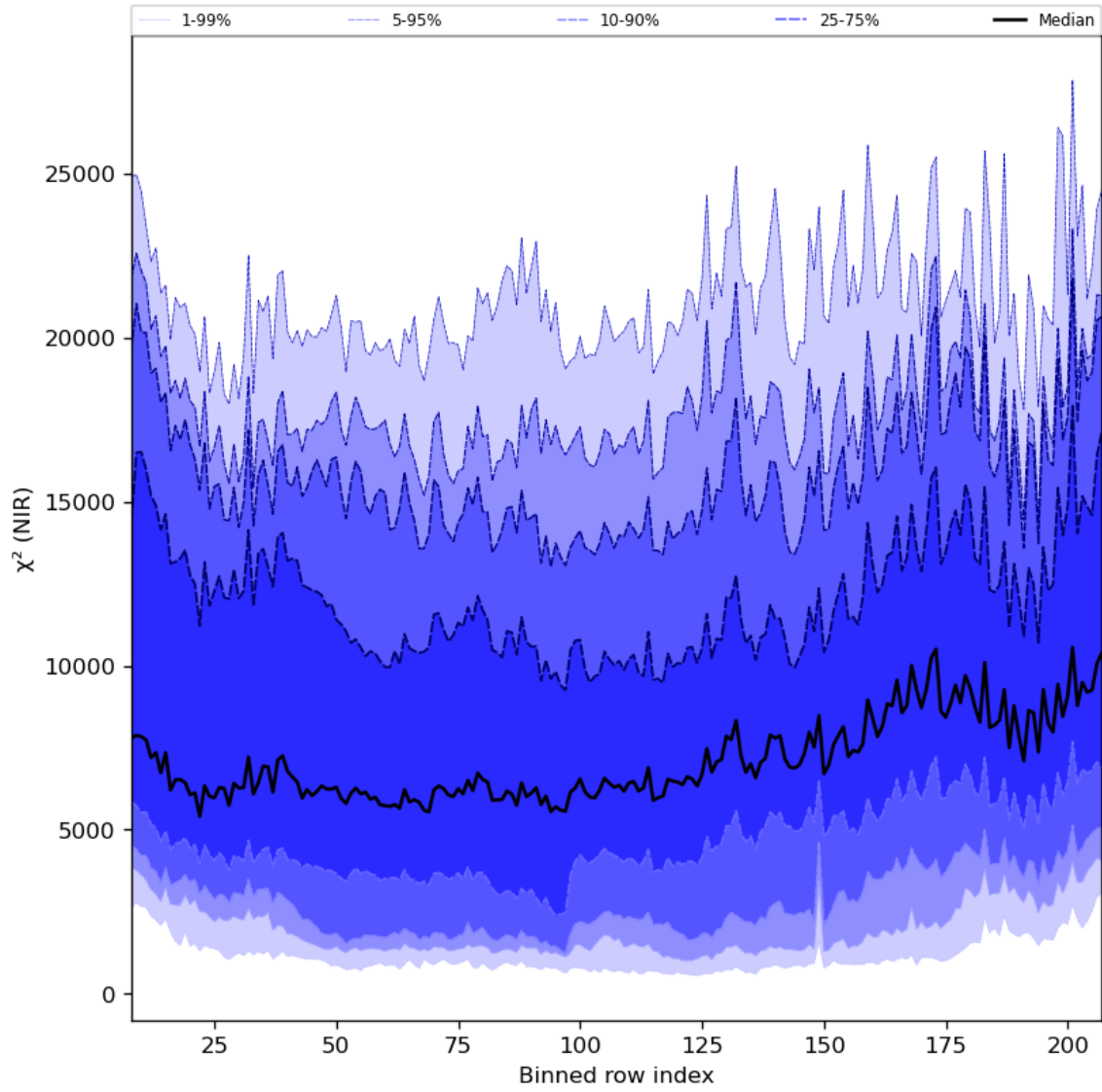
Figure 40: Along track statistics of “ \chi^2 (NIR)” for 2023-10-01 to 2023-10-03
