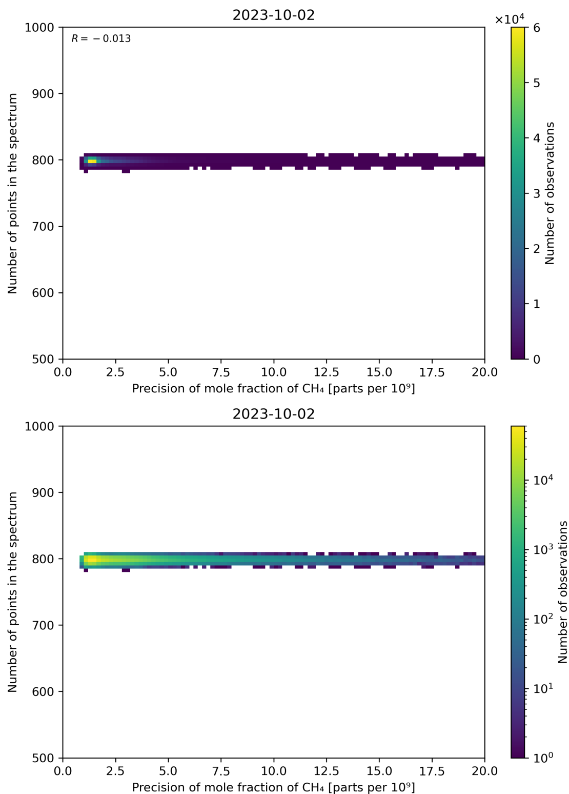
Figure 84: Scatter density plot of “Precision of mole fraction of CH 4 ” against “Number of points in the spectrum” for 2023-10-01 to 2023-10-03.
