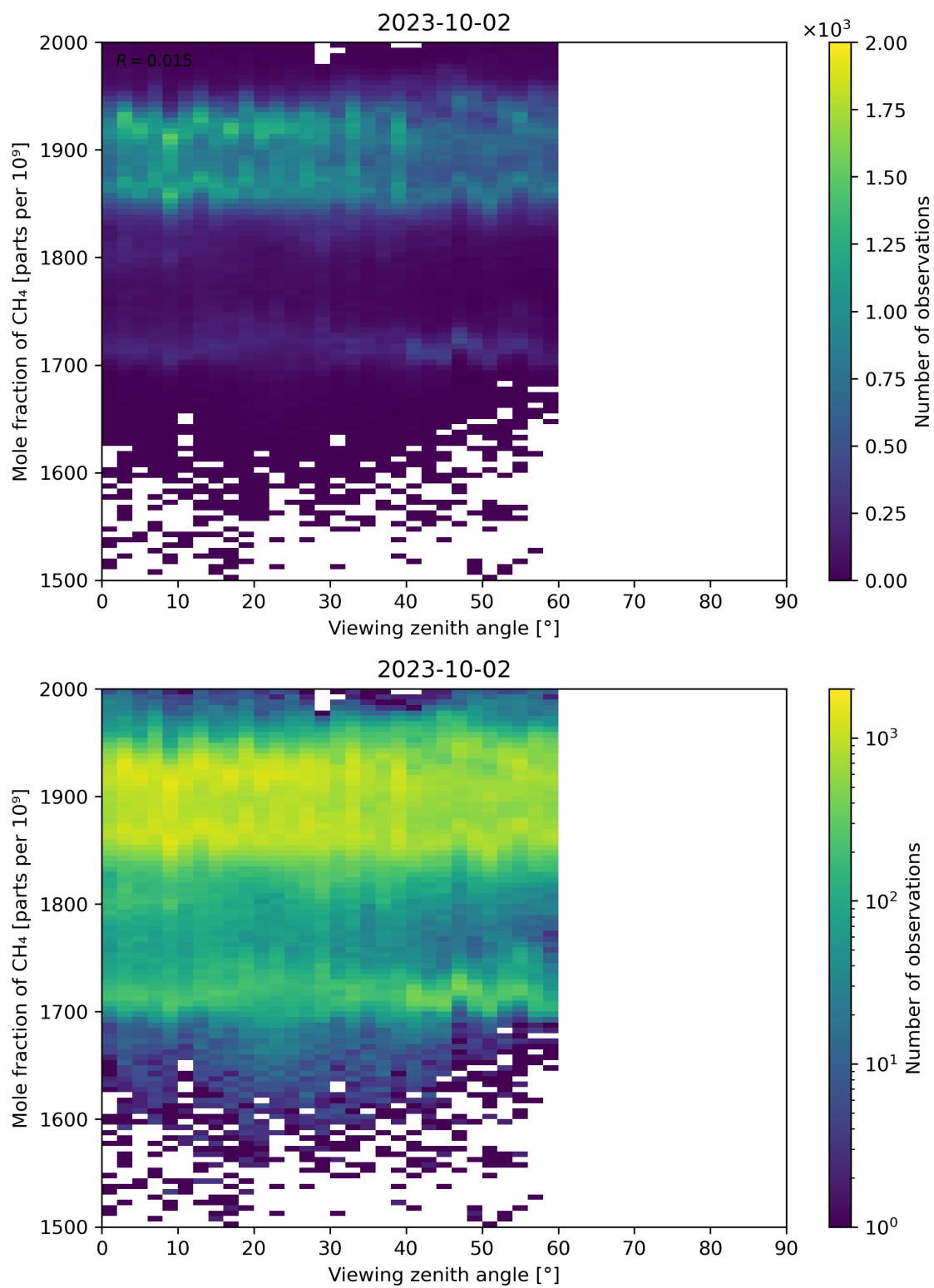
Figure 110: Scatter density plot of “Viewing zenith angle” against “Mole fraction of CH 4 ” for 2023-10-01 to 2023-10-03.
