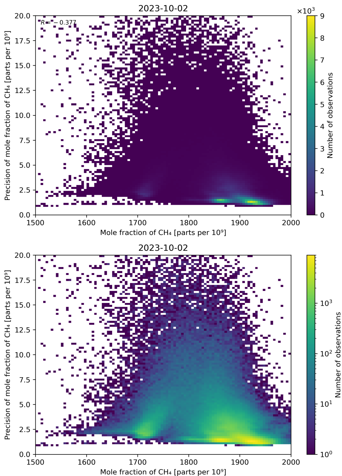
Figure 75: Scatter density plot of “Mole fraction of CH 4 ” against “Precision of mole fraction of CH 4 ” for 2023-10-01 to 2023-10-03.
