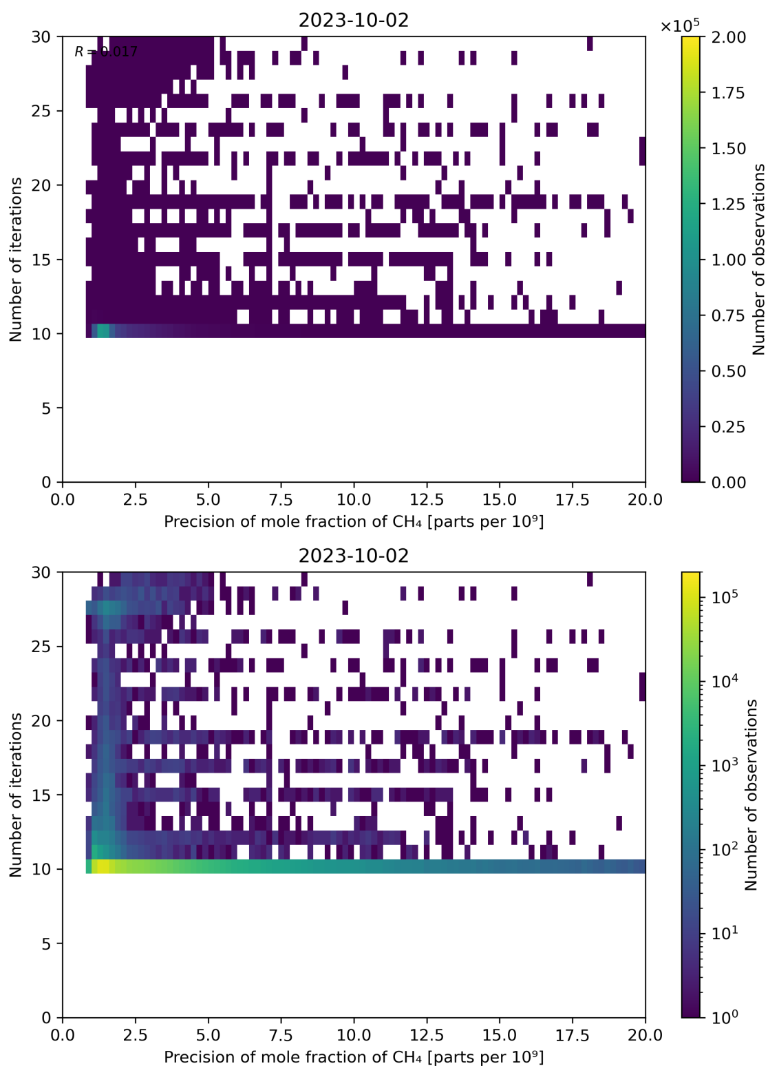
Figure 83: Scatter density plot of “Precision of mole fraction of CH 4 ” against “Number of iterations” for 2023-10-01 to 2023-10-03.
