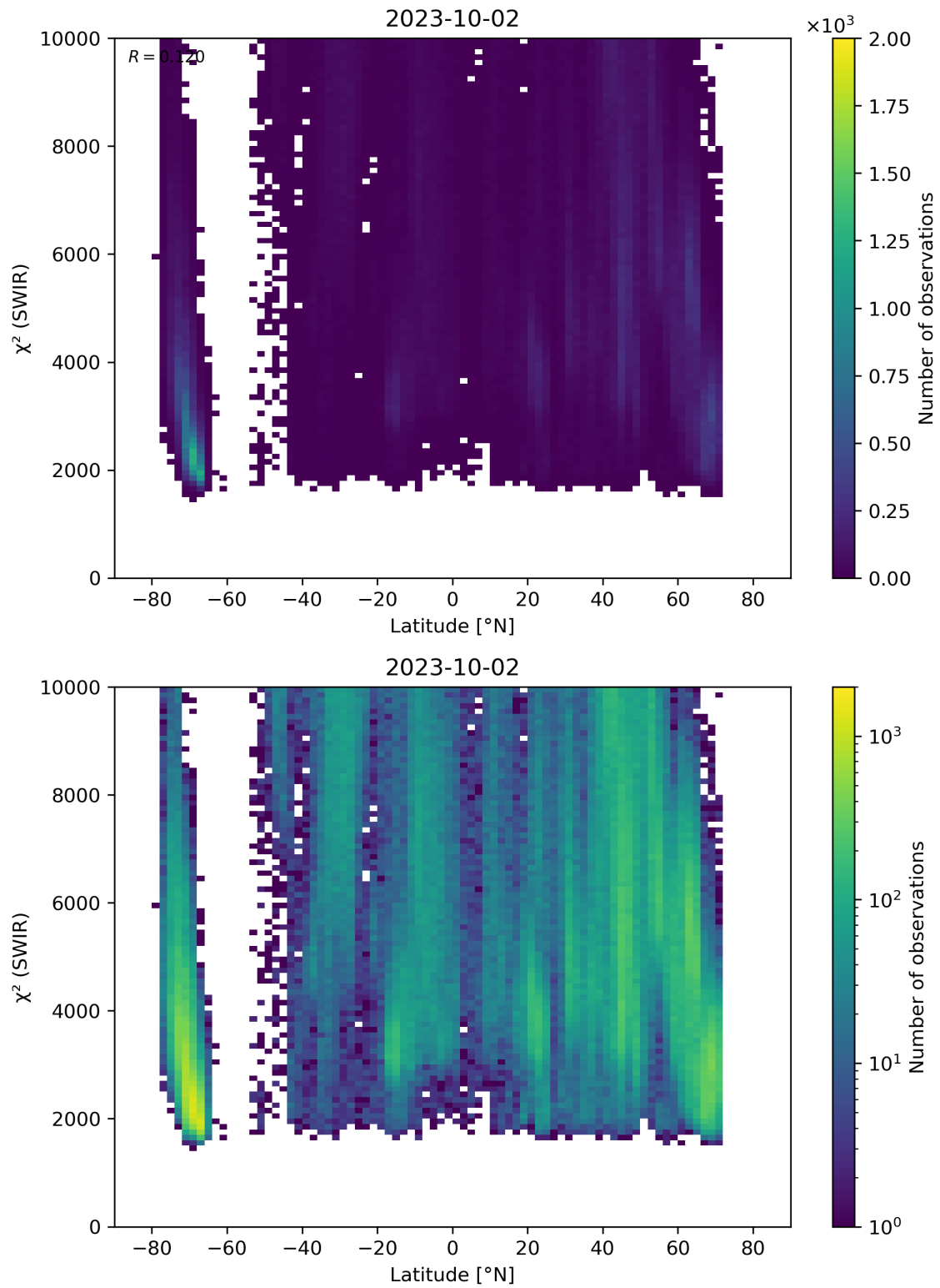
Figure 54: Scatter density plot of “Latitude” against “ \chi^2 (SWIR)” for 2023-10-01 to 2023-10-03.
