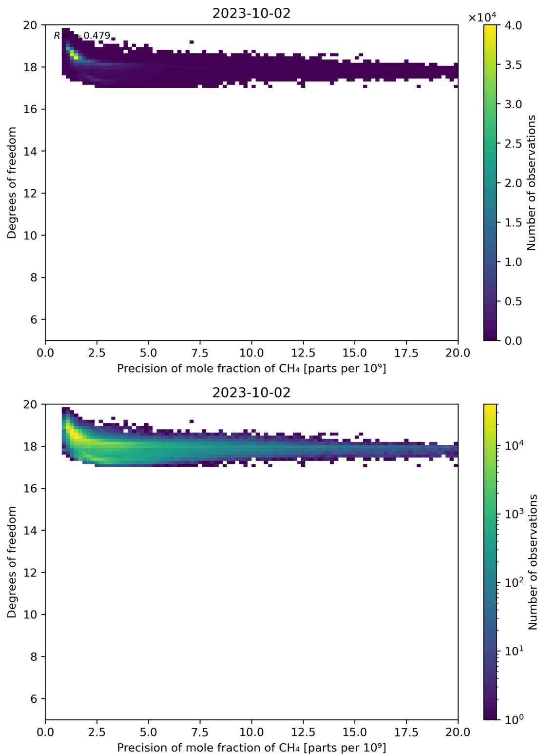
Figure 80: Scatter density plot of “Precision of mole fraction of CH 4 ” against “Degrees of freedom” for 2023-10-01 to 2023-10-03.
