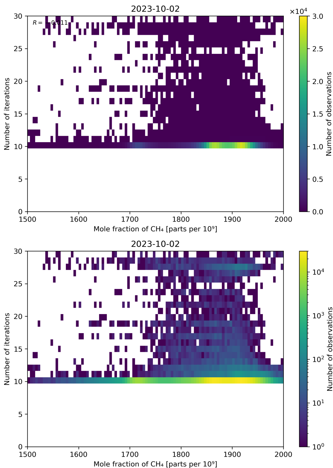
Figure 76: Scatter density plot of “Mole fraction of CH 4 ” against “Number of iterations” for 2023-10-01 to 2023-10-03.
