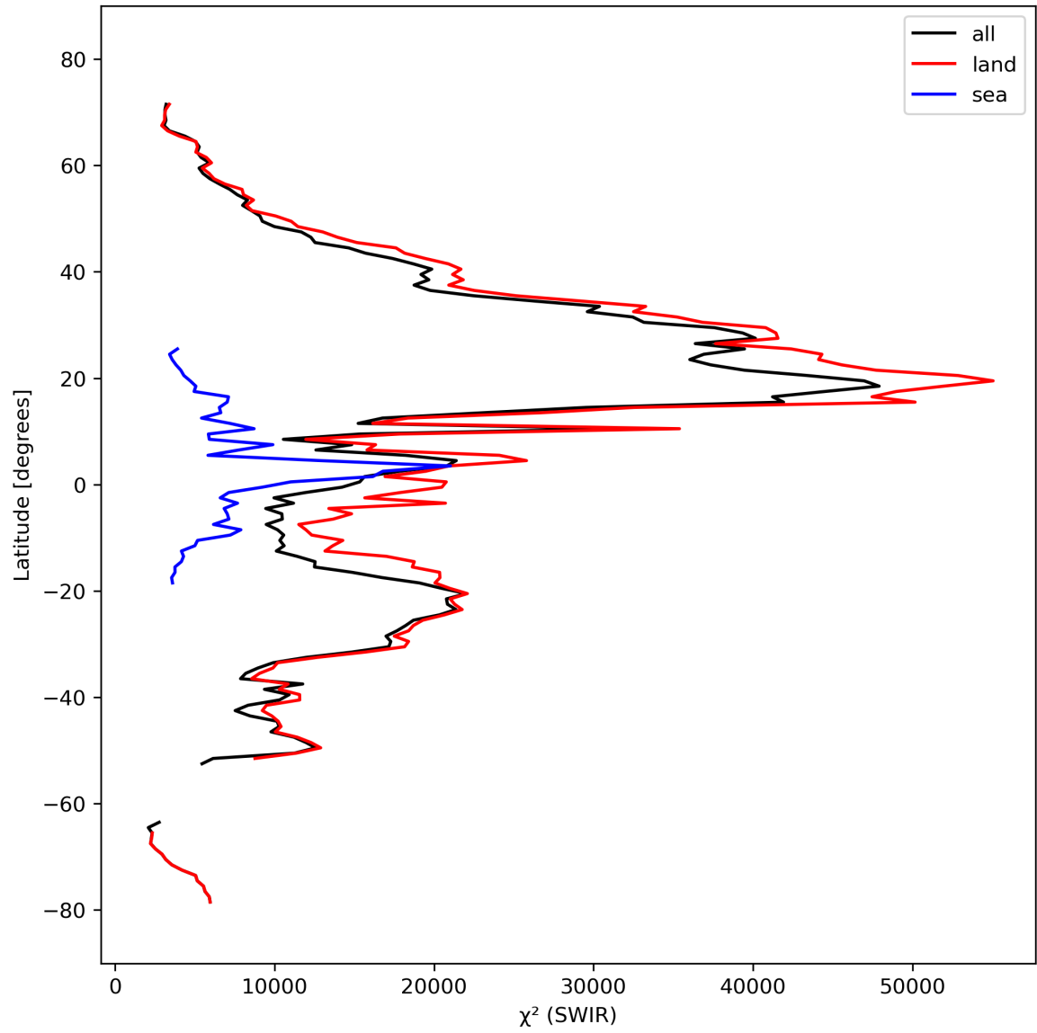
Figure 17: Zonal average of “ \chi^2 (SWIR)” for 2023-10-01 to 2023-10-03.
