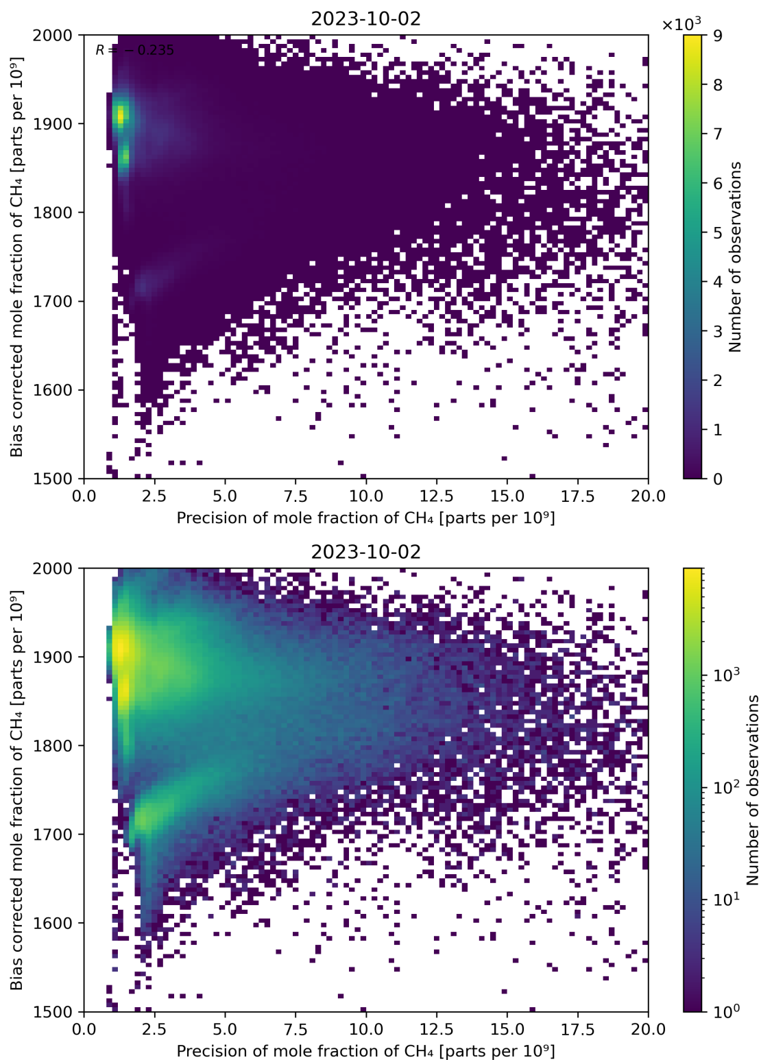
Figure 82: Scatter density plot of “Precision of mole fraction of CH 4 ” against “Bias corrected mole fraction of CH 4 ” for 2023-10-01 to 2023-10-03.
