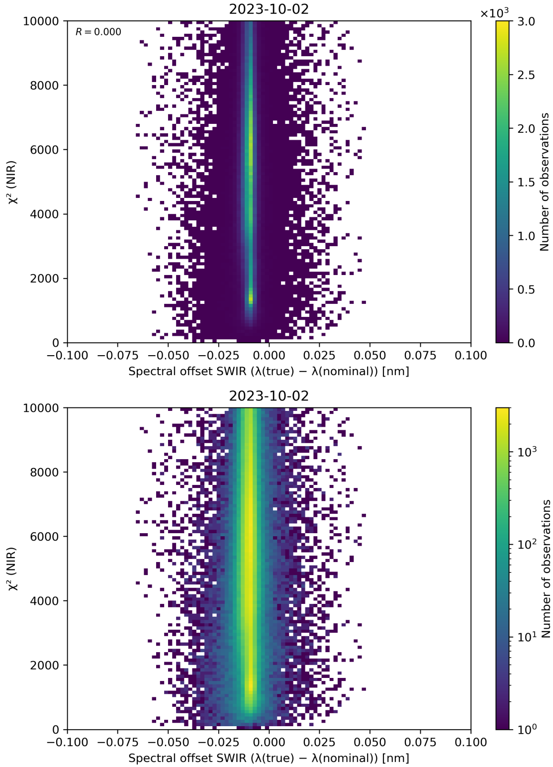
Figure 117: Scatter density plot of “Spectral offset SWIR ( \lambda(\text{true}) - \lambda(\text{nominal}) )” against “ \chi^2 (NIR)” for 2023-10-01 to 2023-10-03.
