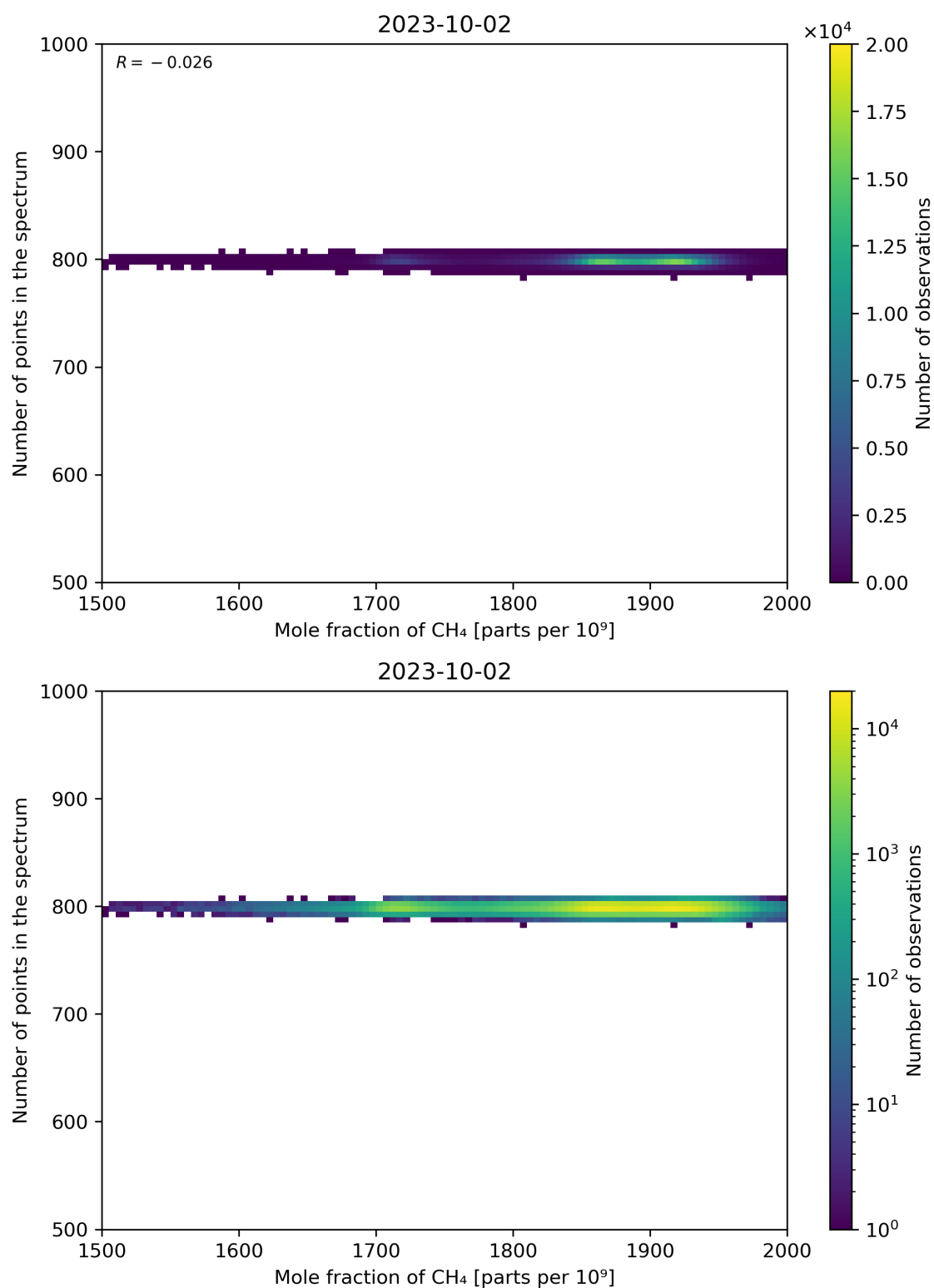
Figure 77: Scatter density plot of “Mole fraction of CH 4 ” against “Number of points in the spectrum” for 2023-10-01 to 2023-10-03.
