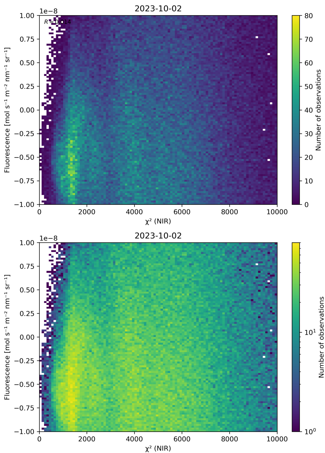
Figure 45: Scatter density plot of “ \chi^2 (NIR)” against “Fluorescence” for 2023-10-01 to 2023-10-03.
