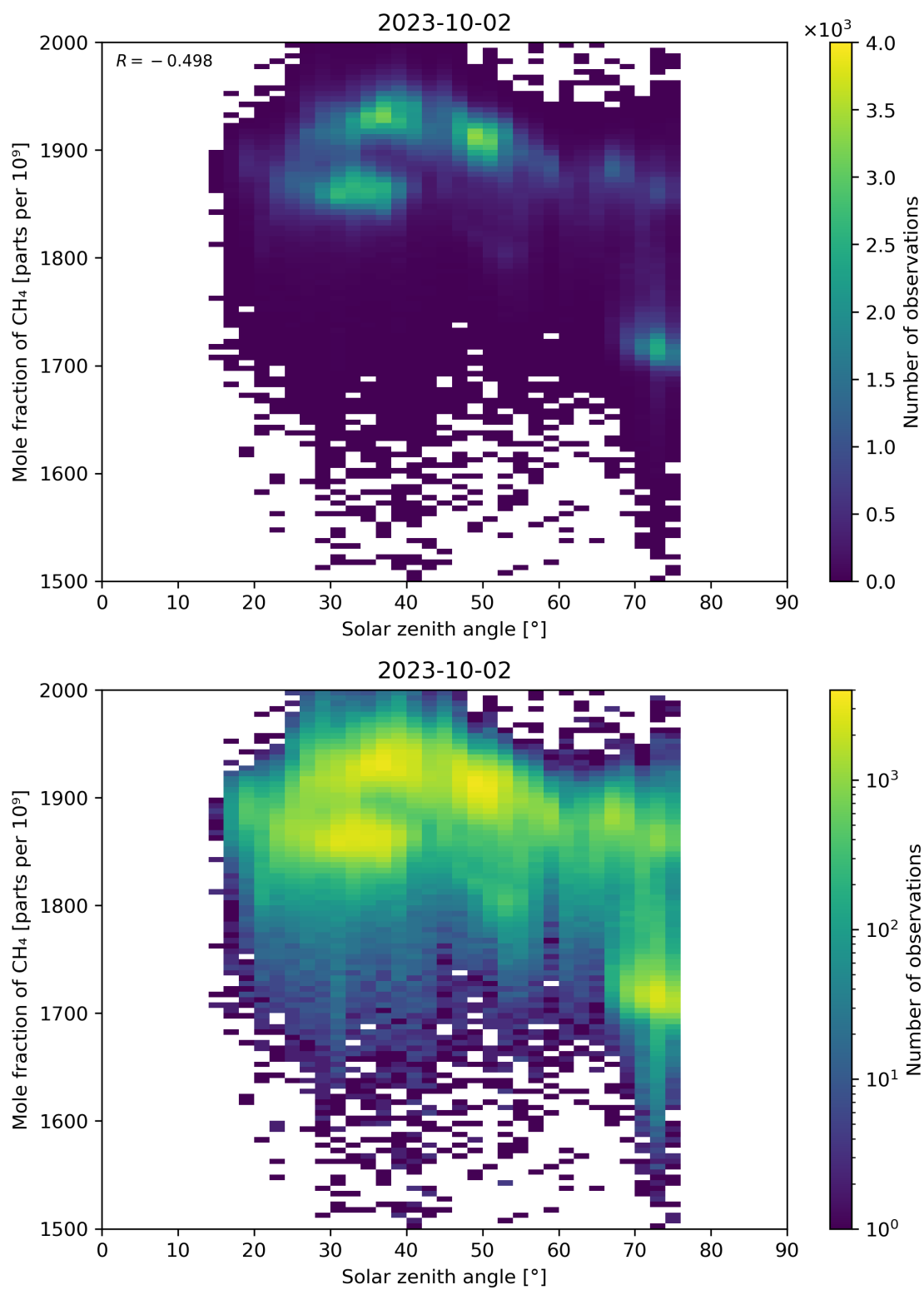
Figure 99: Scatter density plot of “Solar zenith angle” against “Mole fraction of CH 4 ” for 2023-10-01 to 2023-10-03.
