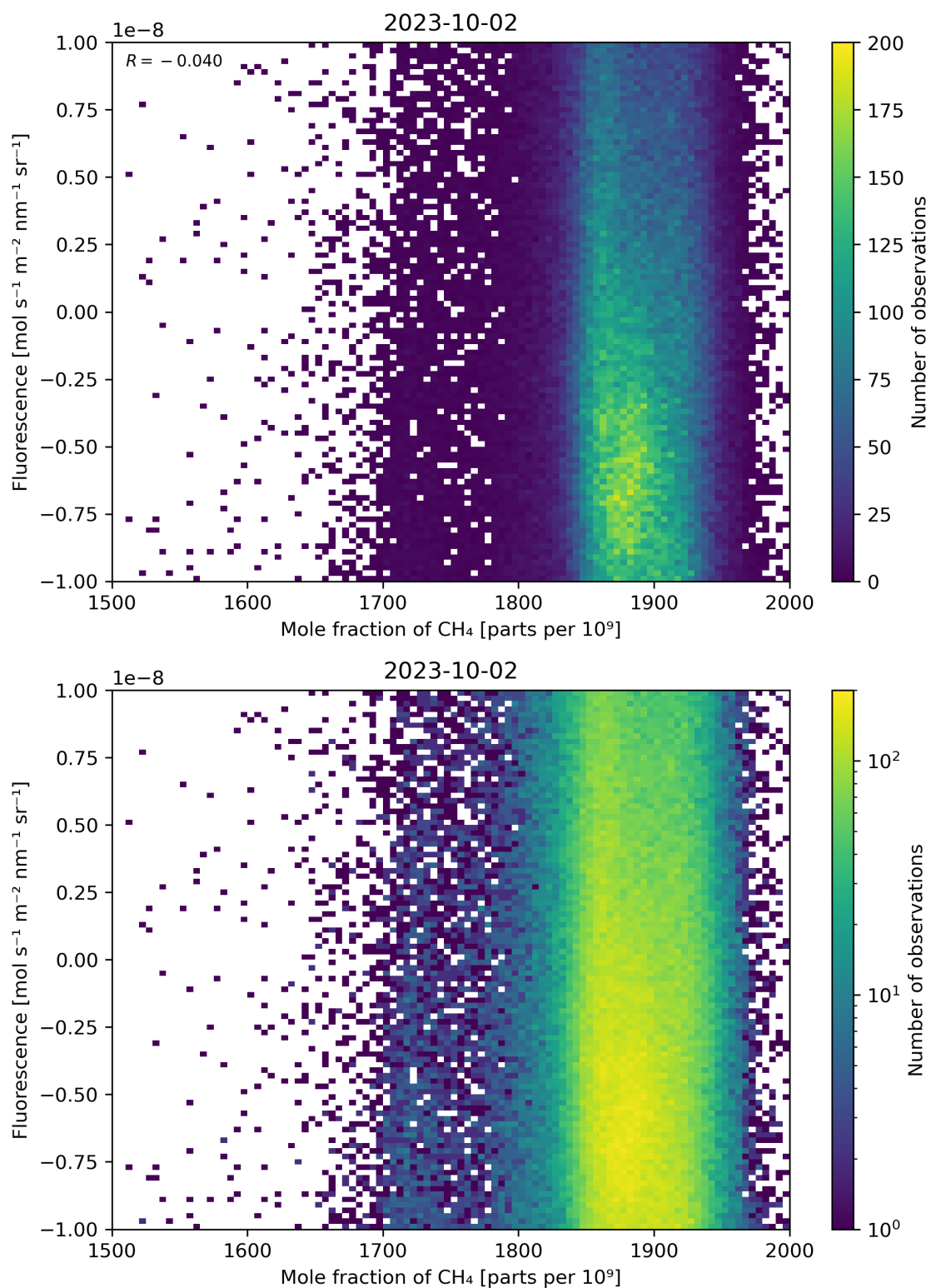
Figure 73: Scatter density plot of “Mole fraction of \text{CH}_4 ” against “Fluorescence” for 2023-10-01 to 2023-10-03.
