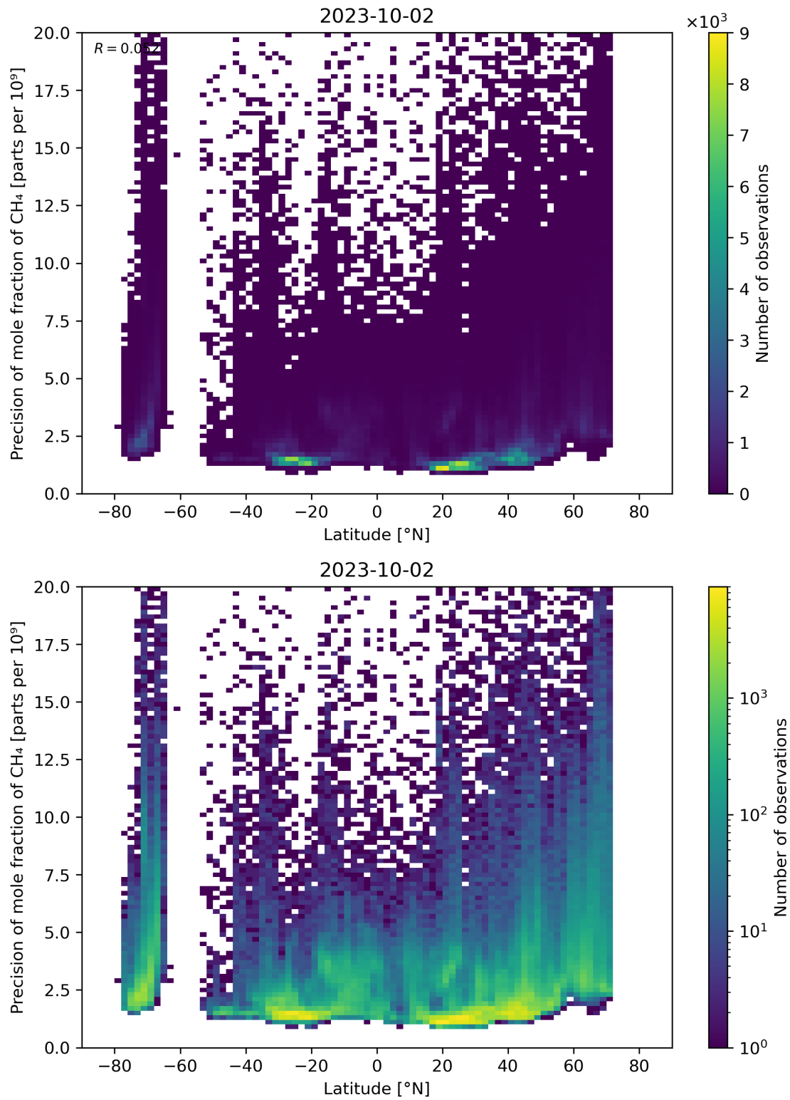
Figure 59: Scatter density plot of “Latitude” against “Precision of mole fraction of CH 4 ” for 2023-10-01 to 2023-10-03.
