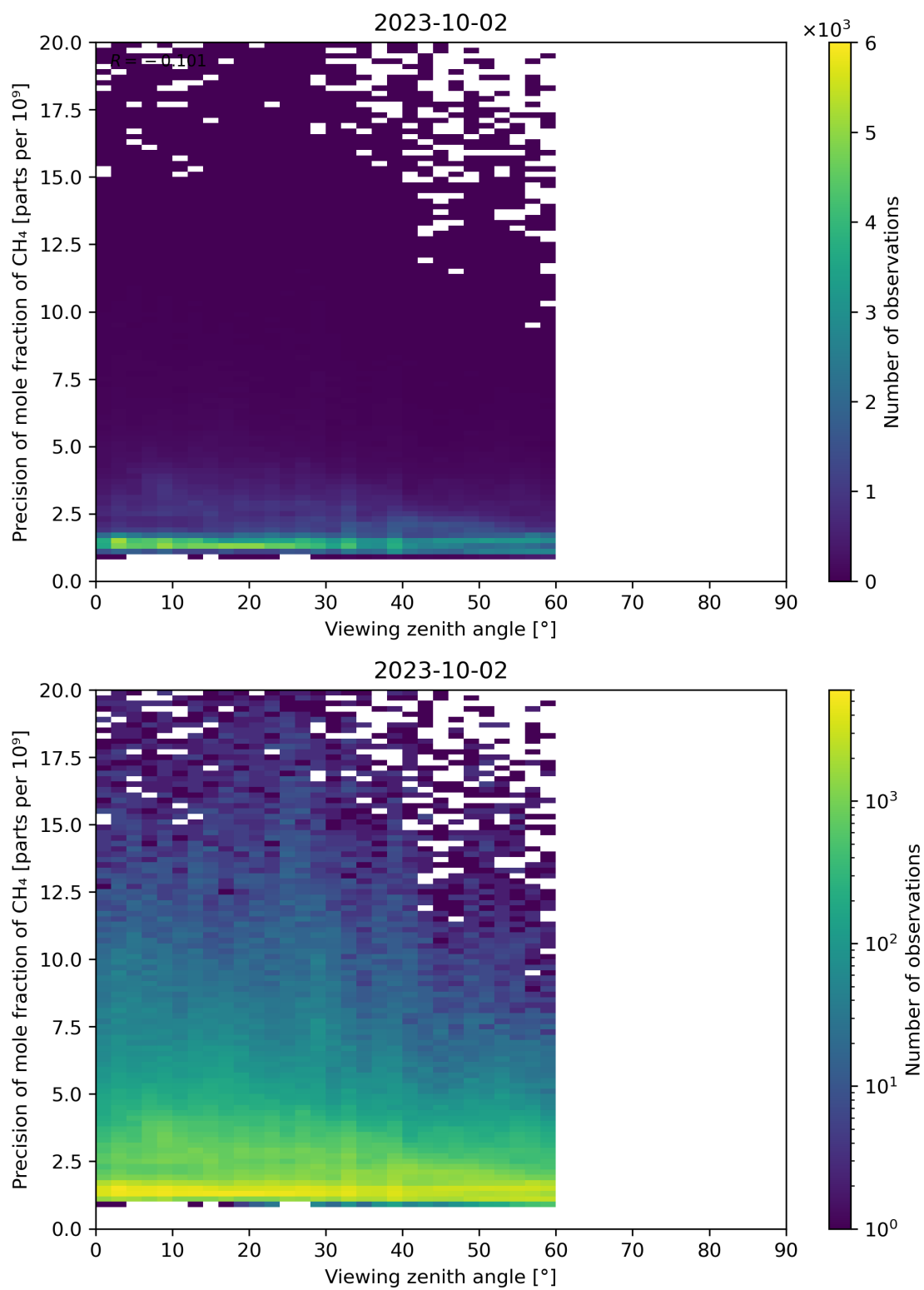
Figure 112: Scatter density plot of “Viewing zenith angle” against “Precision of mole fraction of CH 4 ” for 2023-10-01 to 2023-10-03.
