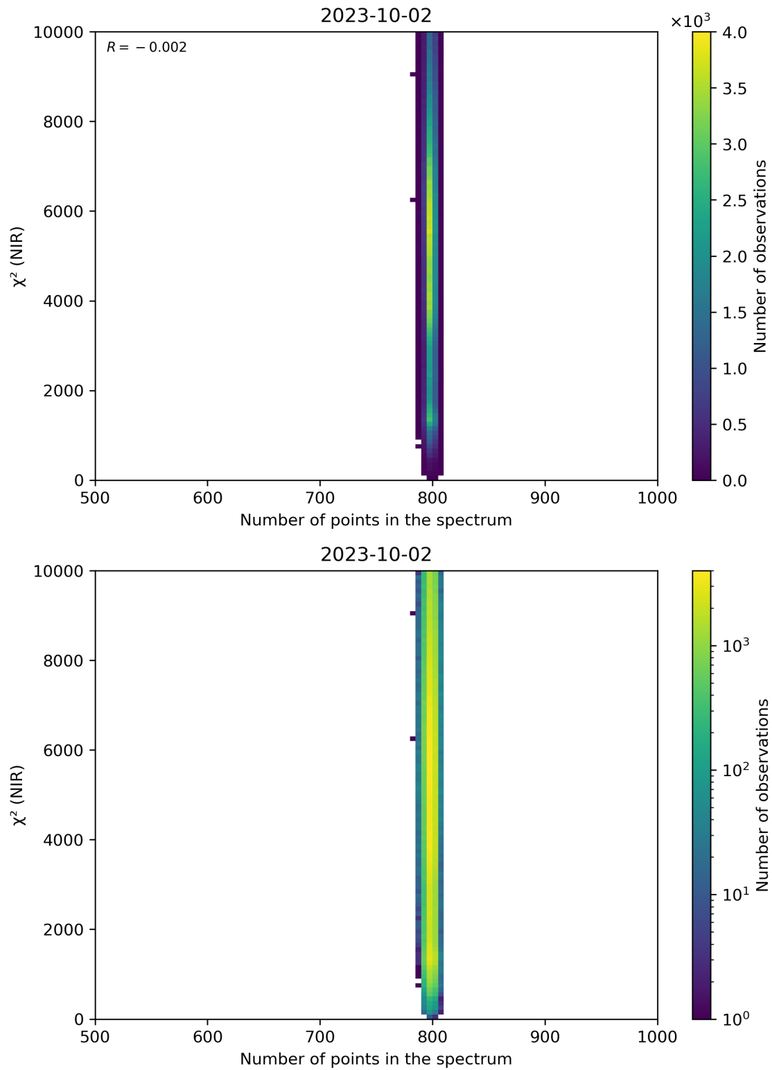
Figure 88: Scatter density plot of “Number of points in the spectrum” against “ \chi^2 (NIR)” for 2023-10-01 to 2023-10-03.
