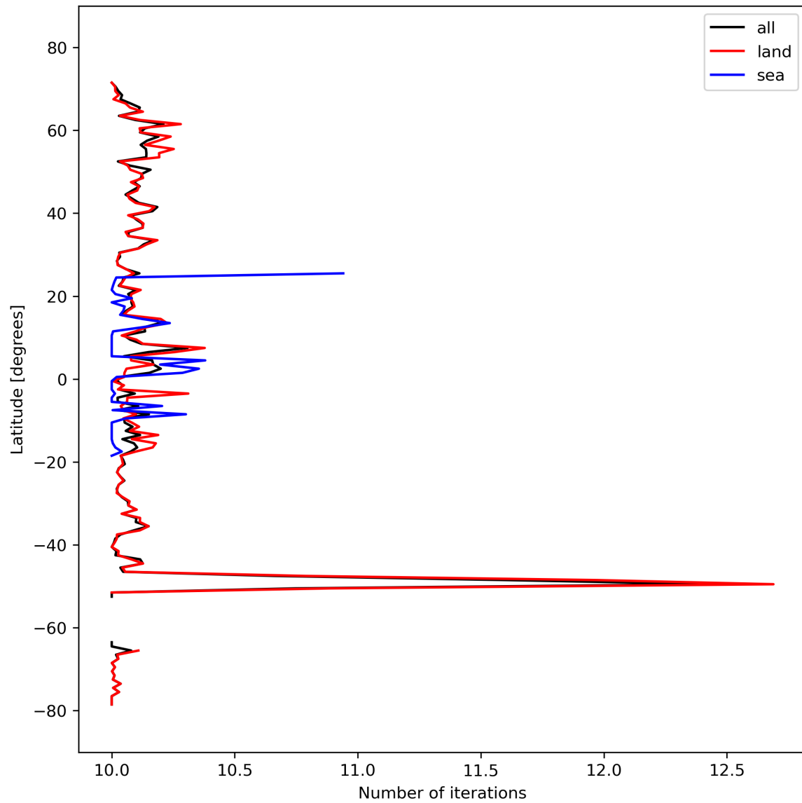
Figure 20: Zonal average of “Number of iterations” for 2023-10-01 to 2023-10-03.
