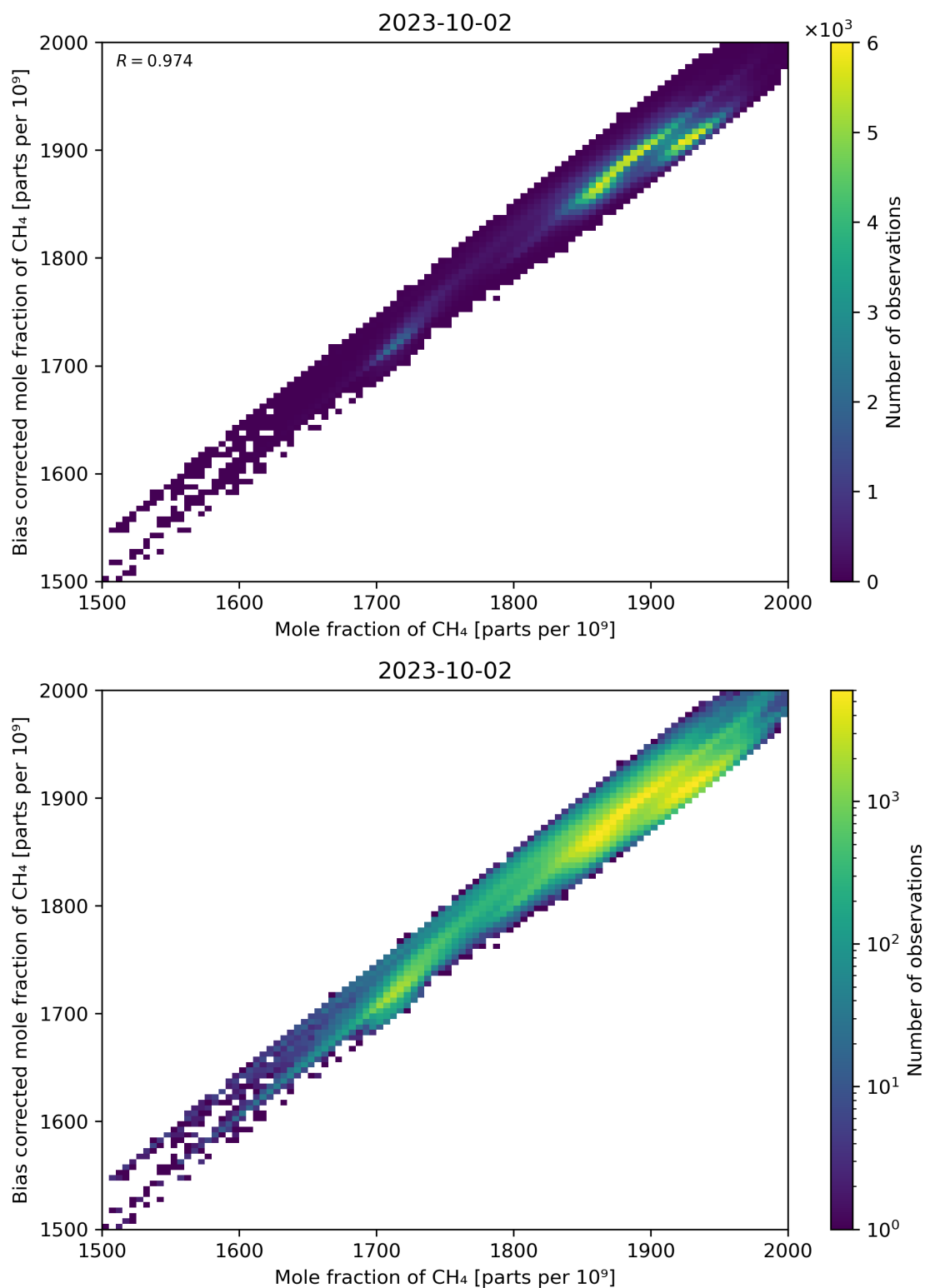
Figure 74: Scatter density plot of “Mole fraction of CH 4 ” against “Bias corrected mole fraction of CH 4 ” for 2023-10-01 to 2023-10-03.
