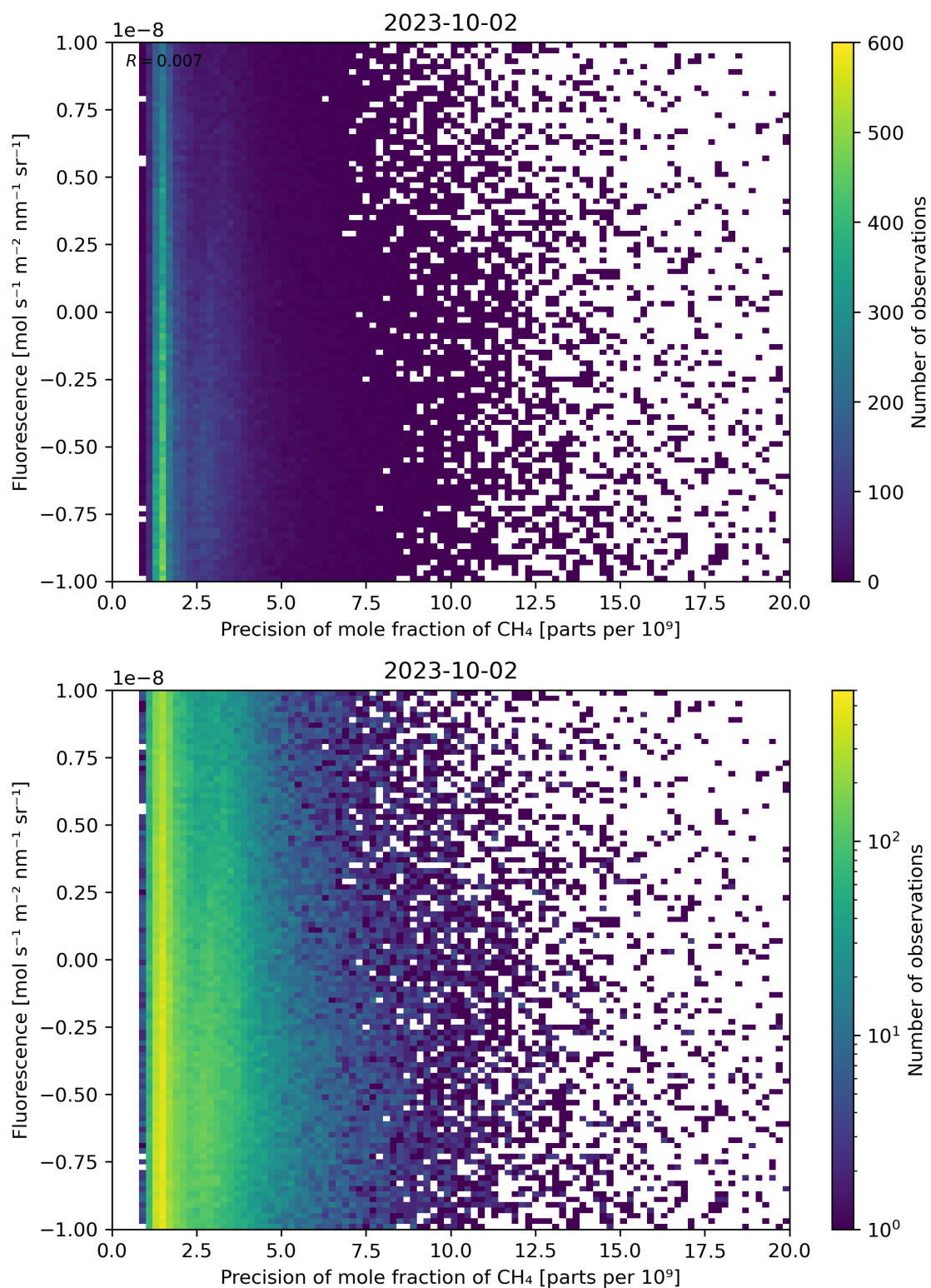
Figure 81: Scatter density plot of “Precision of mole fraction of \text{CH}_4 ” against “Fluorescence” for 2023-10-01 to 2023-10-03.
