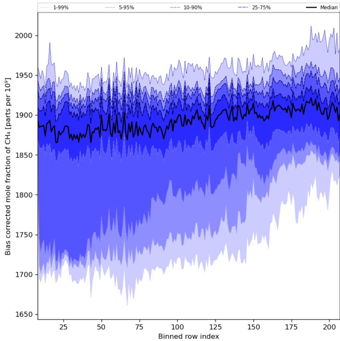
Figure 36: Along track statistics of “Bias corrected mole fraction of CH 4 ” for 2023-10-01 to 2023-10-03
