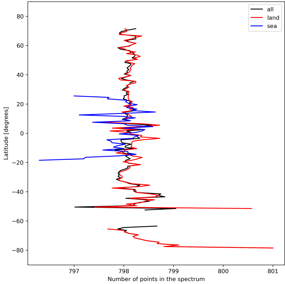
Figure 15: Zonal average of “Number of points in the spectrum” for 2023-10-01 to 2023-10-03.
