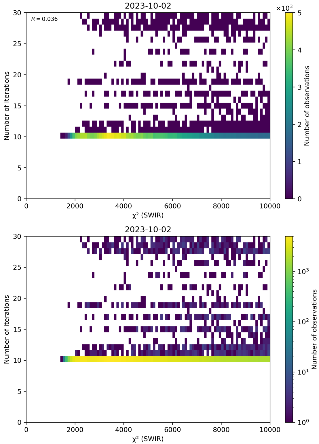
Figure 50: Scatter density plot of “ \chi^2 (SWIR)” against “Number of iterations” for 2023-10-01 to 2023-10-03.
