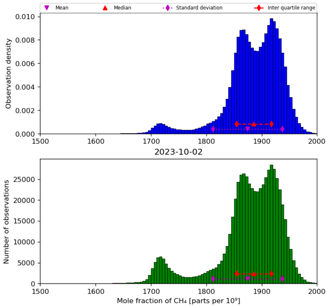
Figure 23: Histogram of “Mole fraction of CH 4 ” for 2023-10-01 to 2023-10-03
