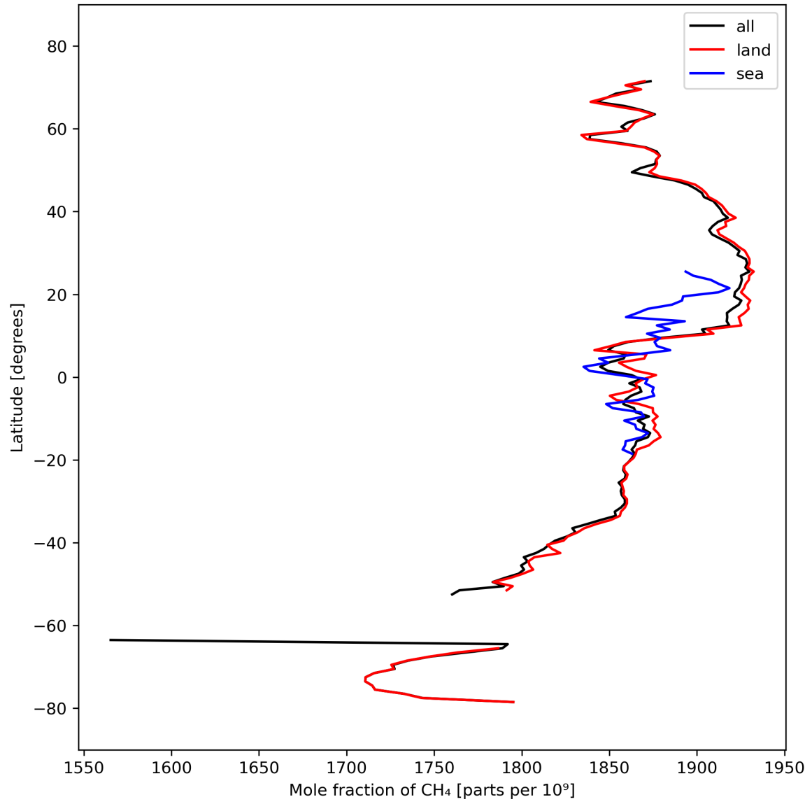
Figure 12: Zonal average of “Mole fraction of \text{CH}_4 ” for 2023-10-01 to 2023-10-03.
