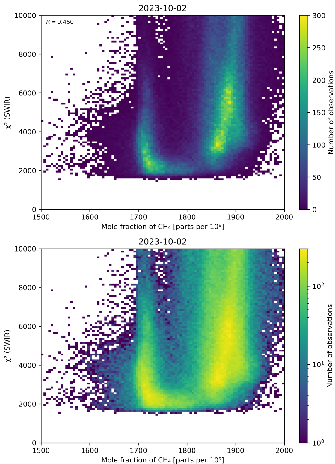
Figure 71: Scatter density plot of “Mole fraction of CH 4 ” against “ \chi^2 (SWIR)” for 2023-10-01 to 2023-10-03.
