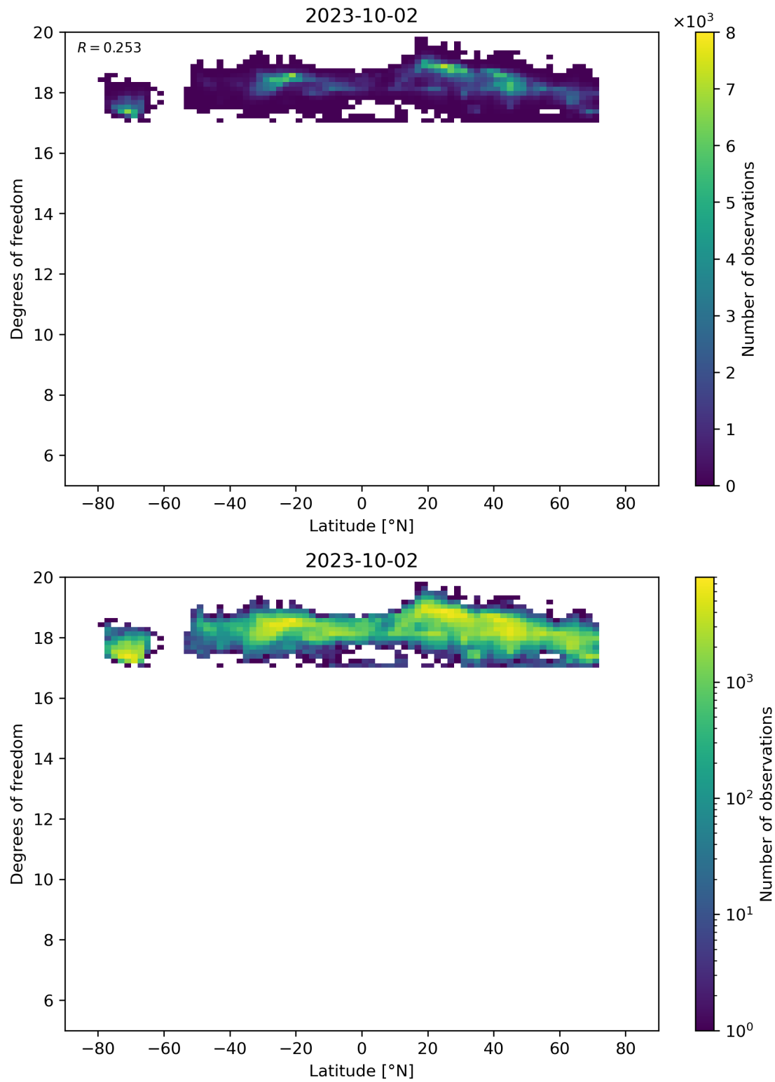
Figure 55: Scatter density plot of “Latitude” against “Degrees of freedom” for 2023-10-01 to 2023-10-03.
