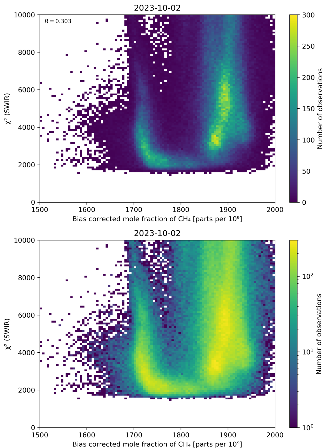
Figure 64: Scatter density plot of “Bias corrected mole fraction of \text{CH}_4 ” against “ \chi^2 (SWIR)” for 2023-10-01 to 2023-10-03.
