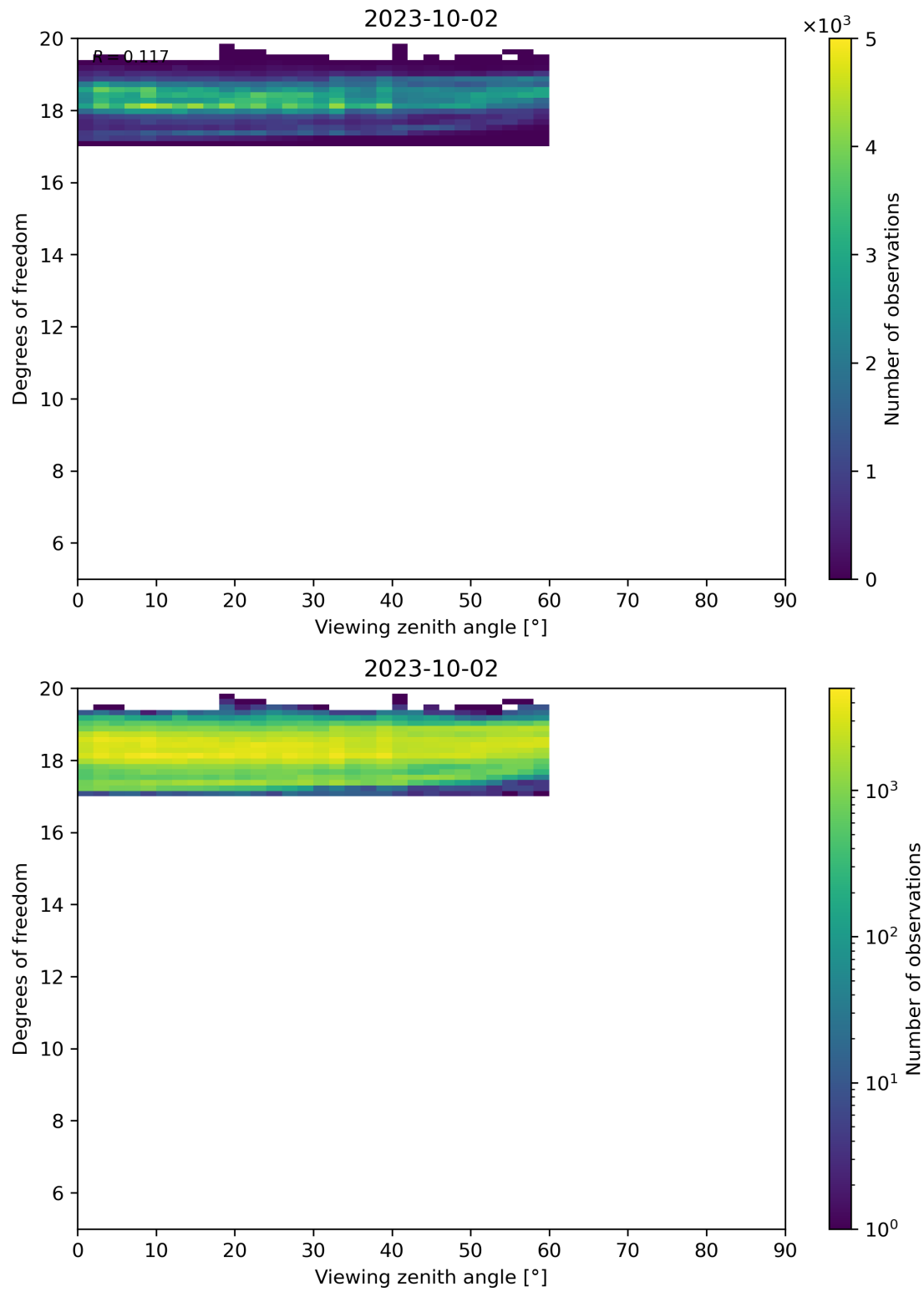
Figure 107: Scatter density plot of “Viewing zenith angle” against “Degrees of freedom” for 2023-10-01 to 2023-10-03.
