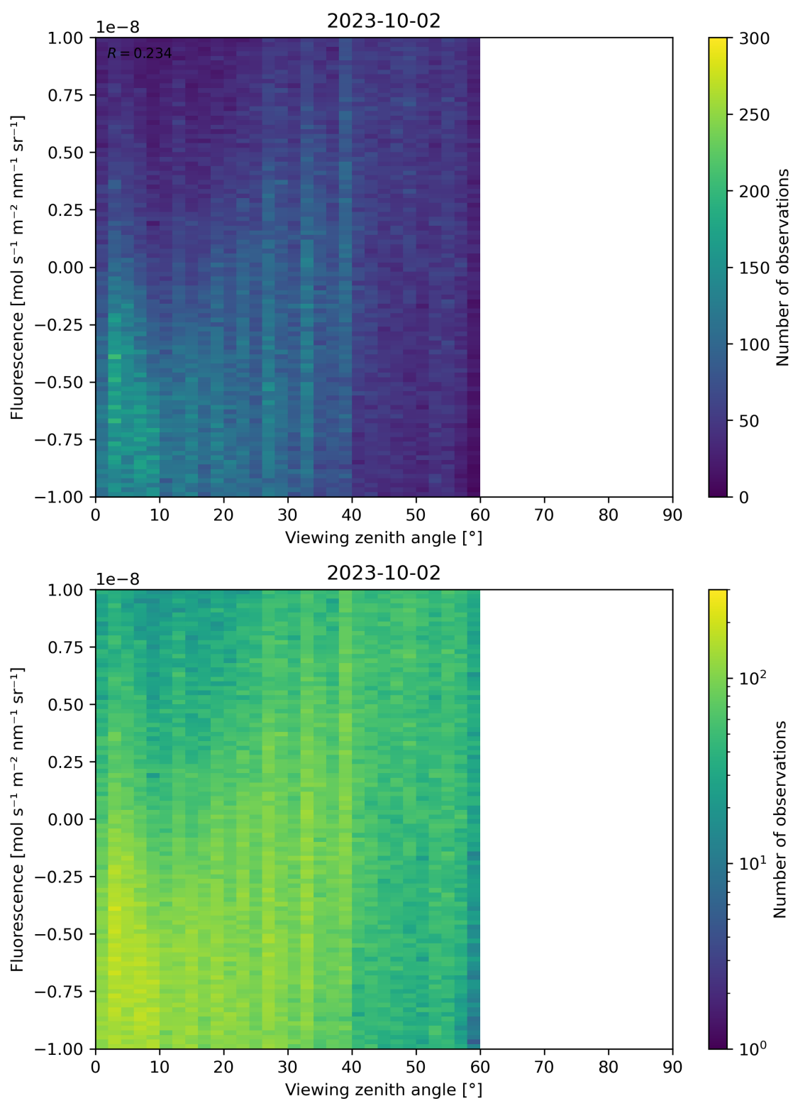
Figure 108: Scatter density plot of “Viewing zenith angle” against “Fluorescence” for 2023-10-01 to 2023-10-03.
