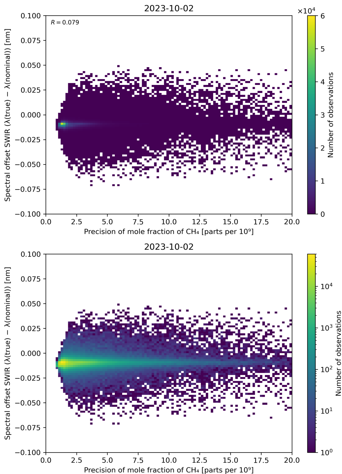
Figure 85: Scatter density plot of “Precision of mole fraction of \text{CH}_4 ” against “Spectral offset SWIR ( \lambda(\text{true}) - \lambda(\text{nominal}) )” for 2023-10-01 to 2023-10-03.
