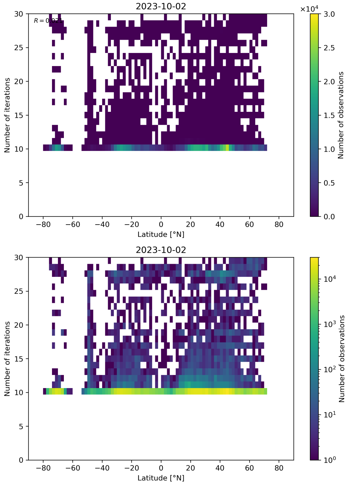
Figure 60: Scatter density plot of “Latitude” against “Number of iterations” for 2023-10-01 to 2023-10-03.
