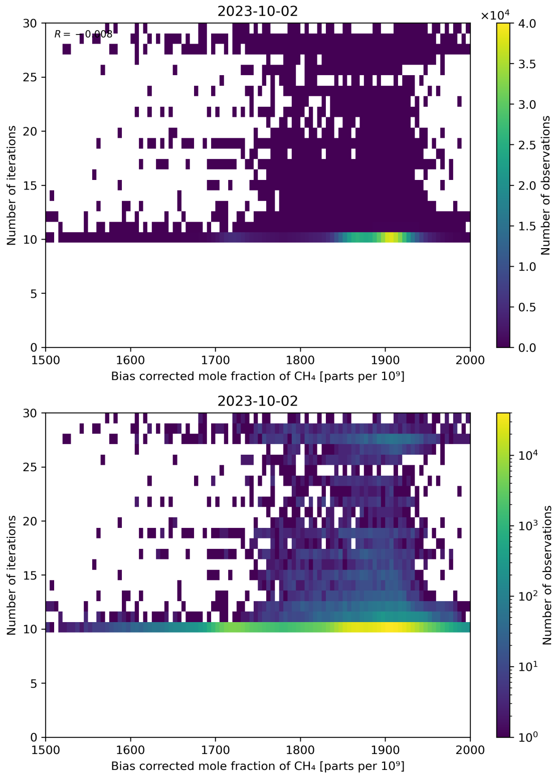
Figure 67: Scatter density plot of “Bias corrected mole fraction of CH 4 ” against “Number of iterations” for 2023-10-01 to 2023-10-03.
