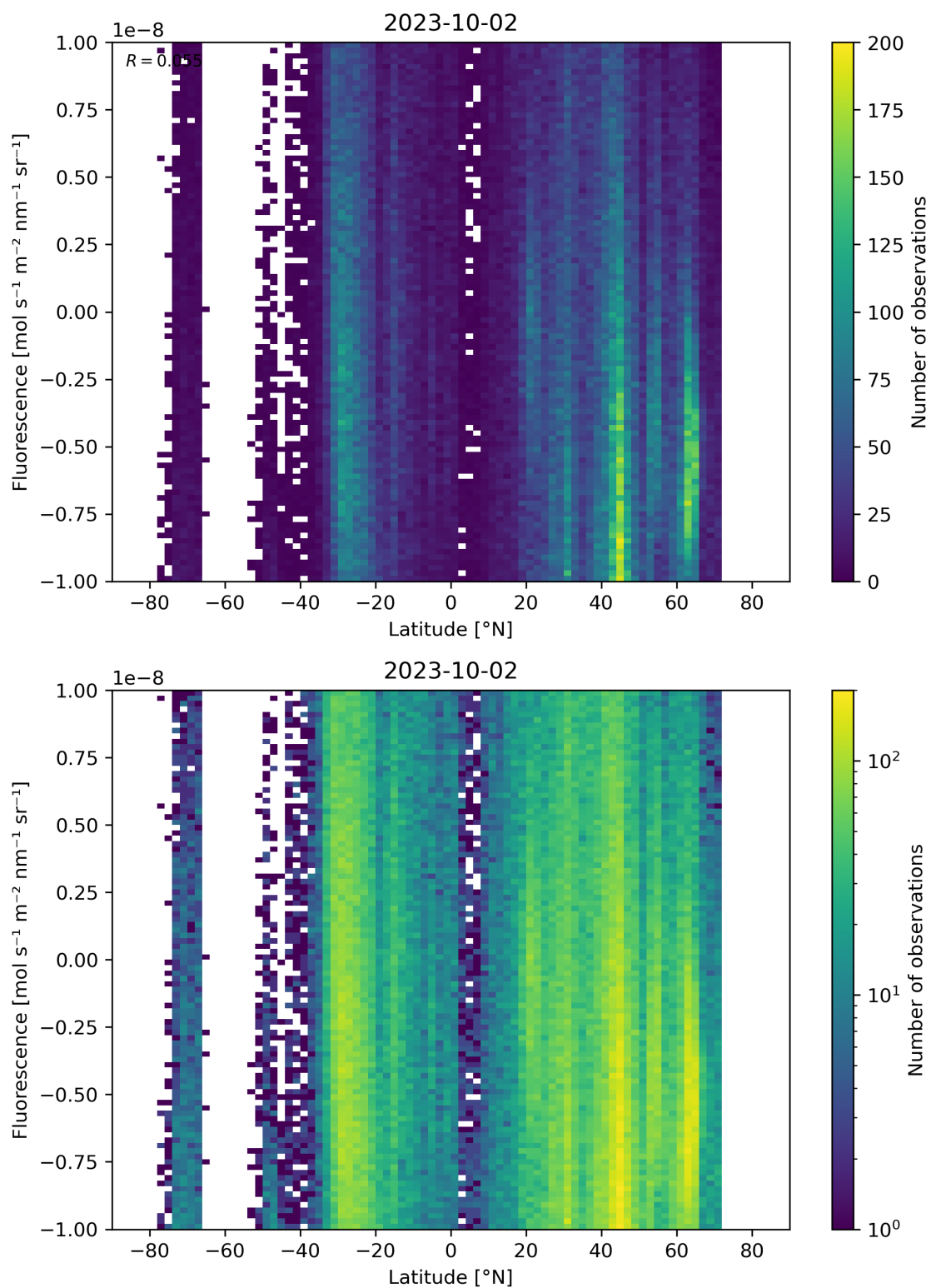
Figure 56: Scatter density plot of “Latitude” against “Fluorescence” for 2023-10-01 to 2023-10-03.
