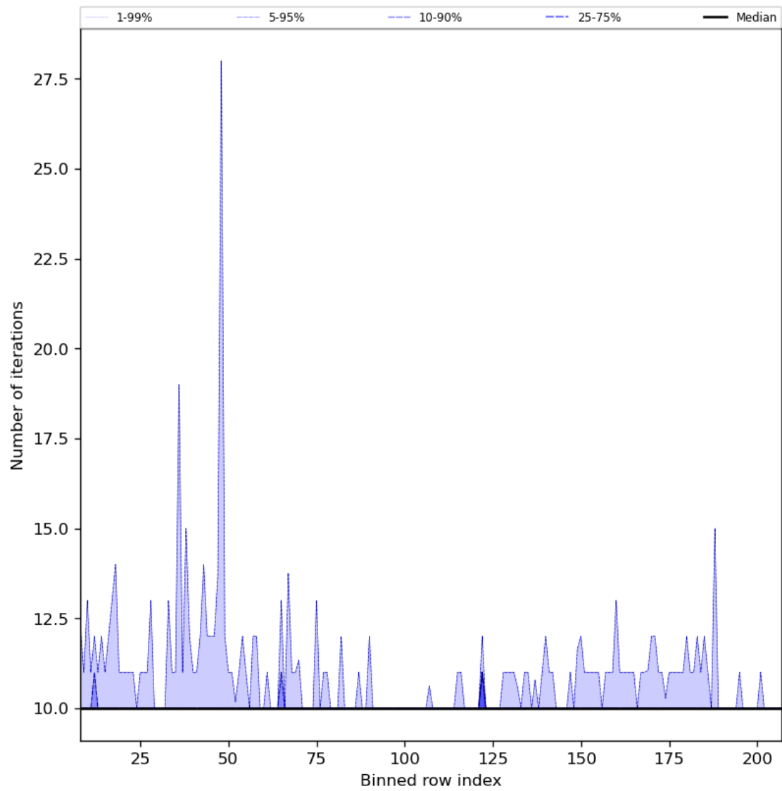
Figure 42: Along track statistics of “Number of iterations” for 2023-10-01 to 2023-10-03
