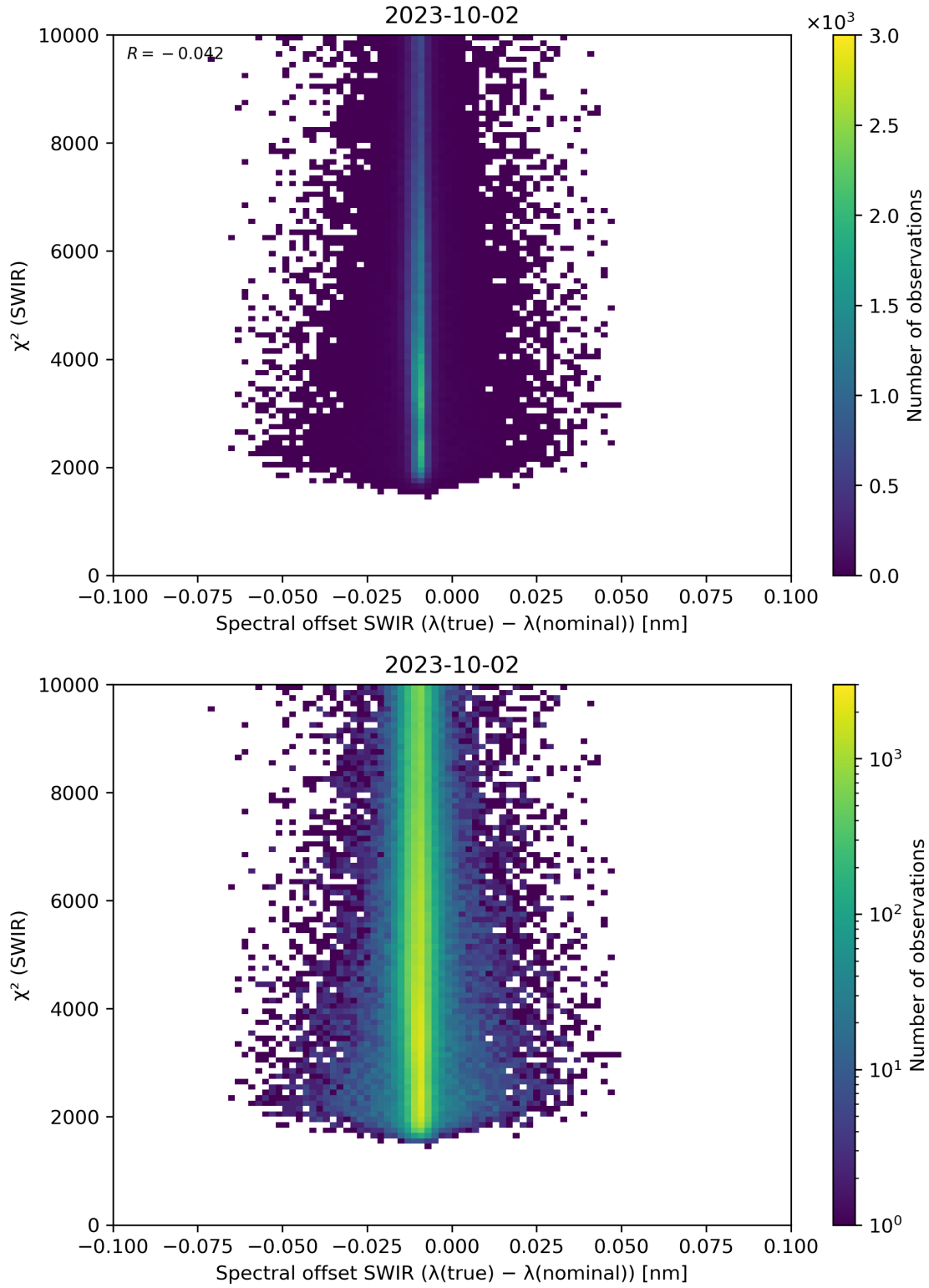
Figure 118: Scatter density plot of “Spectral offset SWIR ( \lambda(\text{true}) - \lambda(\text{nominal}) )” against “ \chi^2 (SWIR)” for 2023-10-01 to 2023-10-03.
