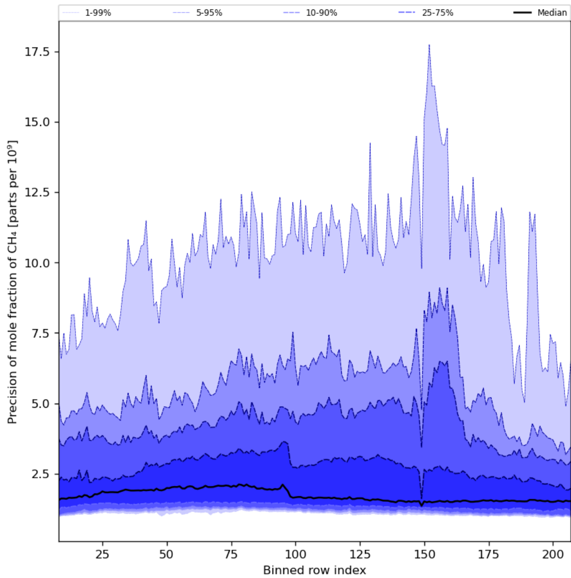
Figure 35: Along track statistics of “Precision of mole fraction of CH 4 ” for 2023-10-01 to 2023-10-03
