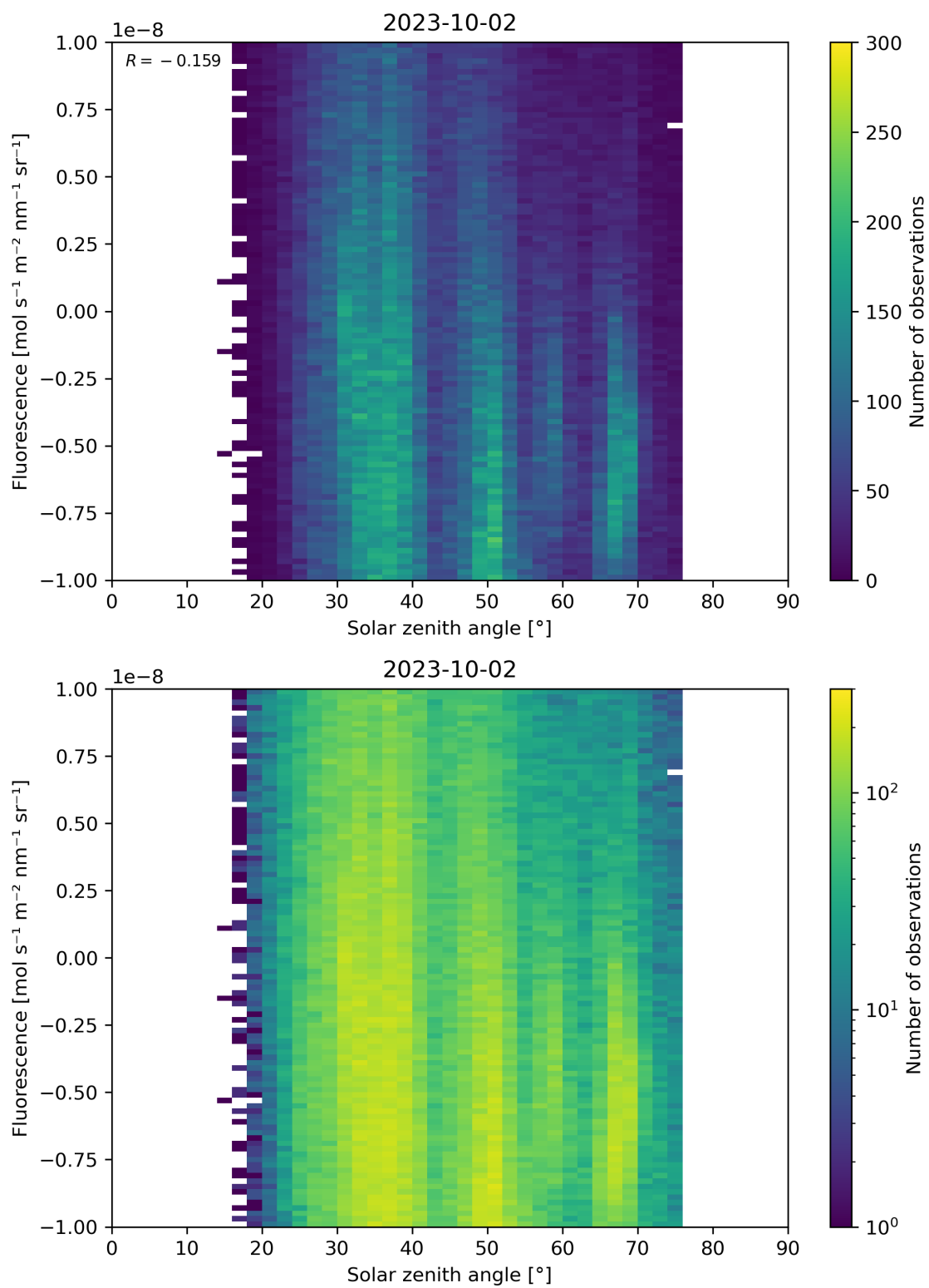
Figure 97: Scatter density plot of “Solar zenith angle” against “Fluorescence” for 2023-10-01 to 2023-10-03.
