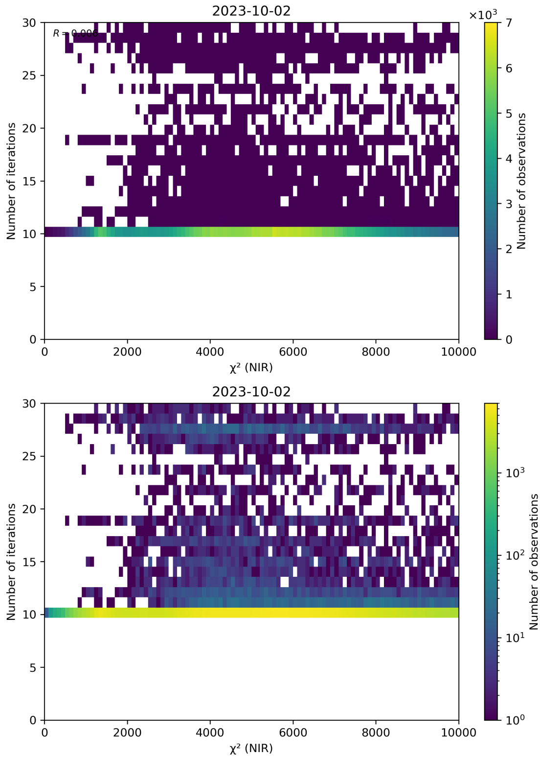
Figure 46: Scatter density plot of “ \chi^2 (NIR)” against “Number of iterations” for 2023-10-01 to 2023-10-03.
