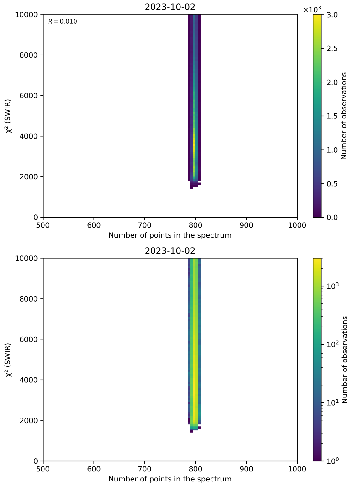
Figure 89: Scatter density plot of “Number of points in the spectrum” against “ \chi^2 (SWIR)” for 2023-10-01 to 2023-10-03.
