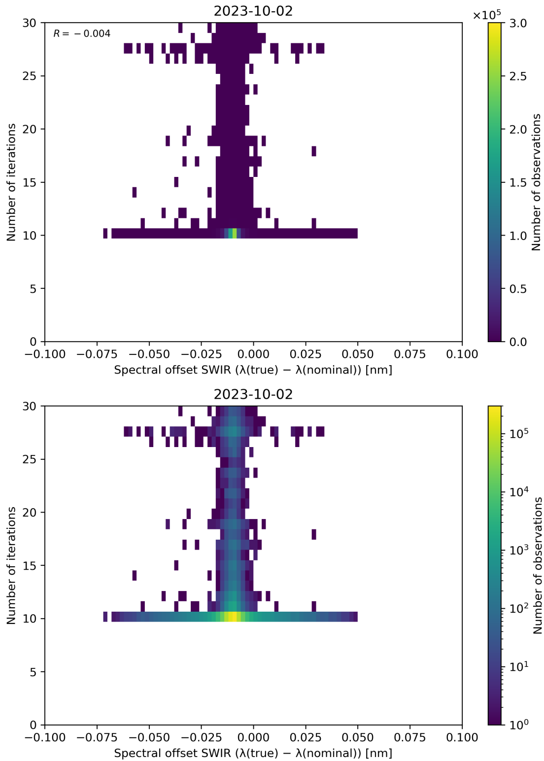
Figure 121: Scatter density plot of “Spectral offset SWIR ( \lambda(\text{true}) - \lambda(\text{nominal}) )” against “Number of iterations” for 2023-10-01 to 2023-10-03.
