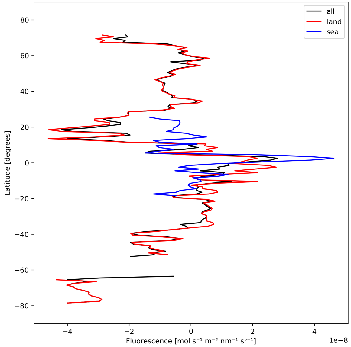
Figure 21: Zonal average of “Fluorescence” for 2023-10-01 to 2023-10-03.
