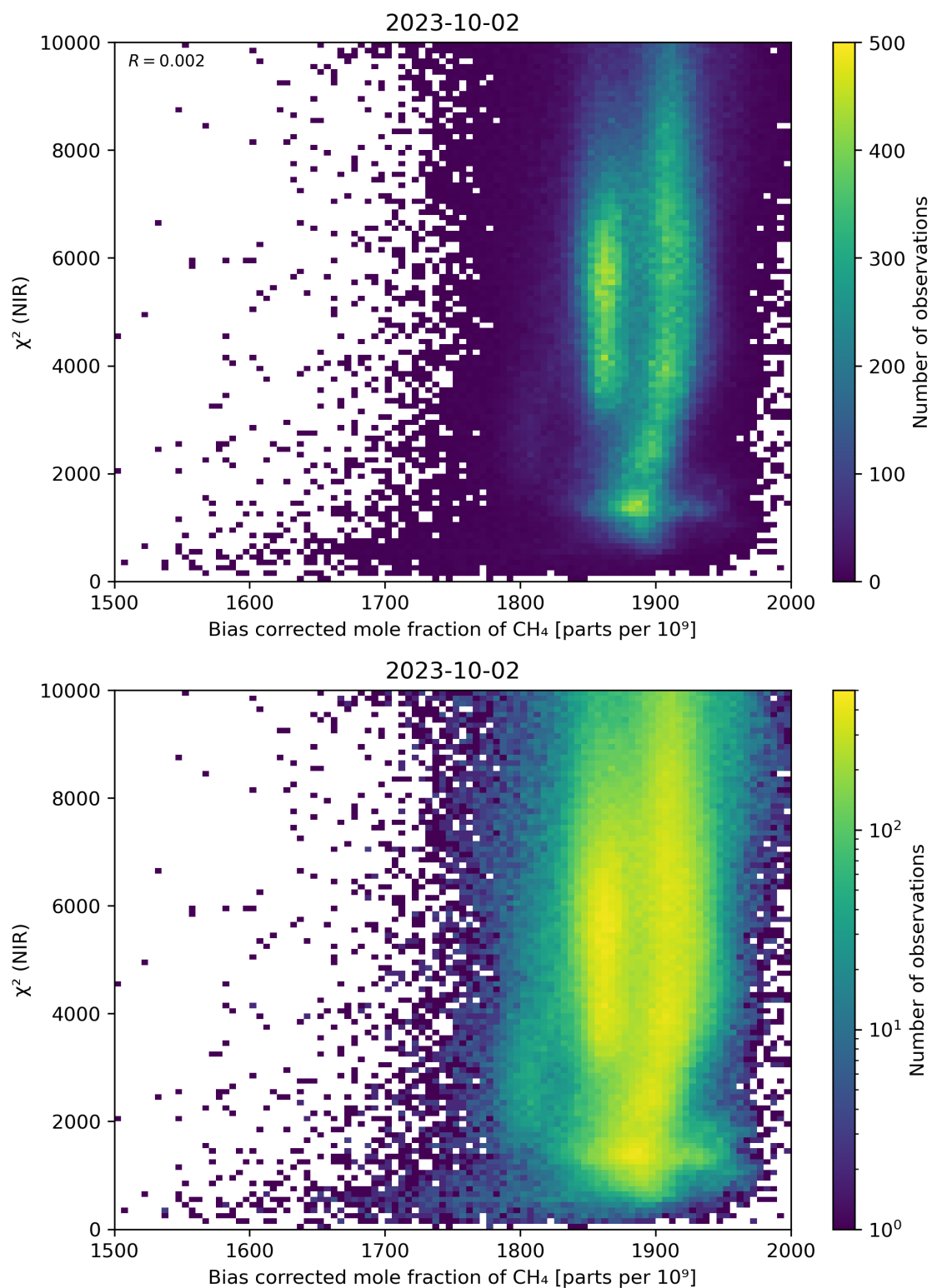
Figure 63: Scatter density plot of “Bias corrected mole fraction of CH 4 ” against “ \chi^2 (NIR)” for 2023-10-01 to 2023-10-03.
