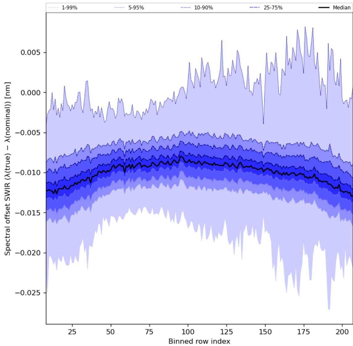
Figure 38: Along track statistics of “Spectral offset SWIR ( \lambda(\text{true}) - \lambda(\text{nominal}) )” for 2023-10-01 to 2023-10-03
