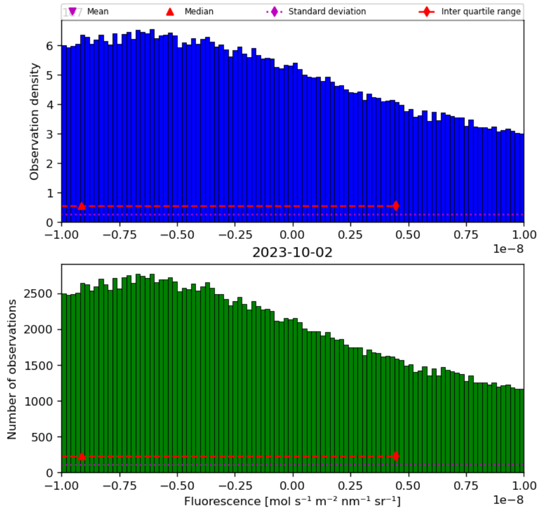
Figure 32: Histogram of “Fluorescence” for 2023-10-01 to 2023-10-03
