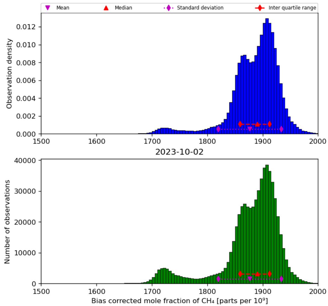
Figure 25: Histogram of “Bias corrected mole fraction of CH 4 ” for 2023-10-01 to 2023-10-03
