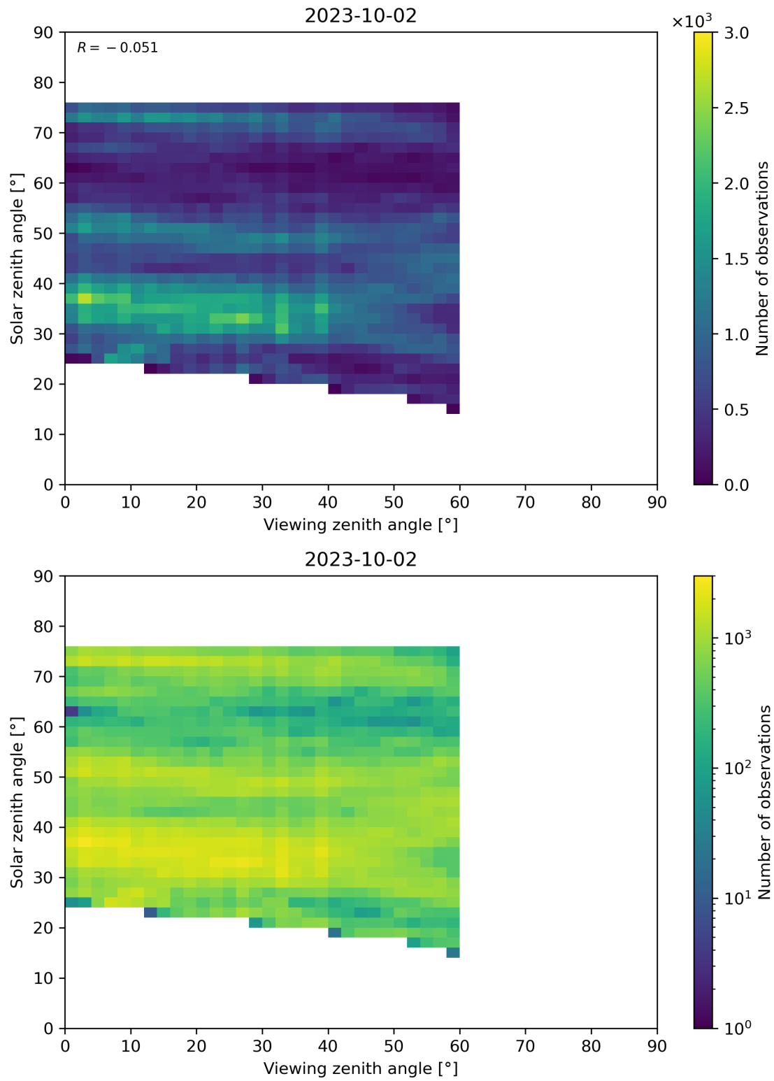
Figure 115: Scatter density plot of “Viewing zenith angle” against “Solar zenith angle” for 2023-10-01 to 2023-10-03.
