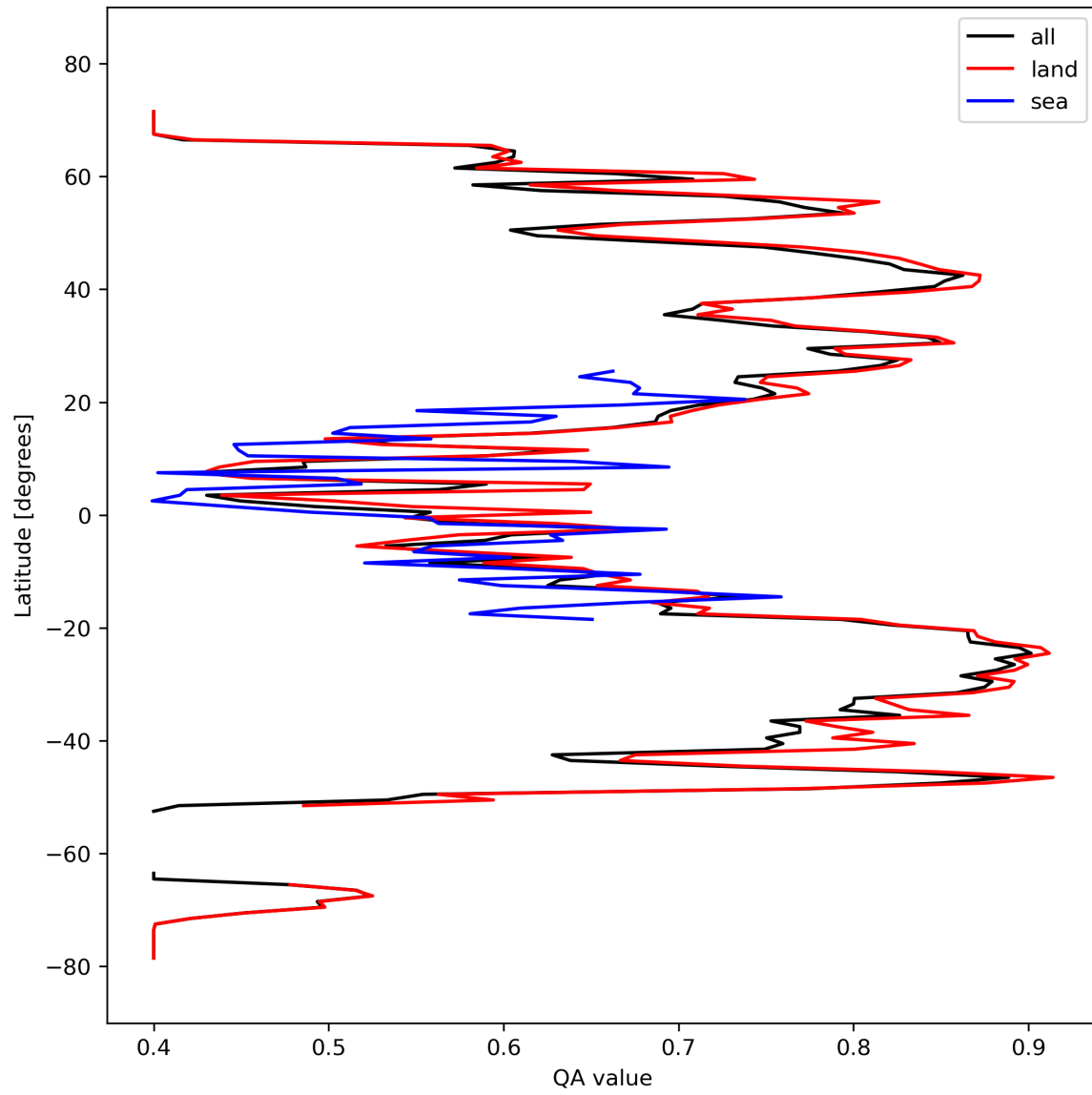
Figure 11: Zonal average of “QA value” for 2023-10-01 to 2023-10-03.
