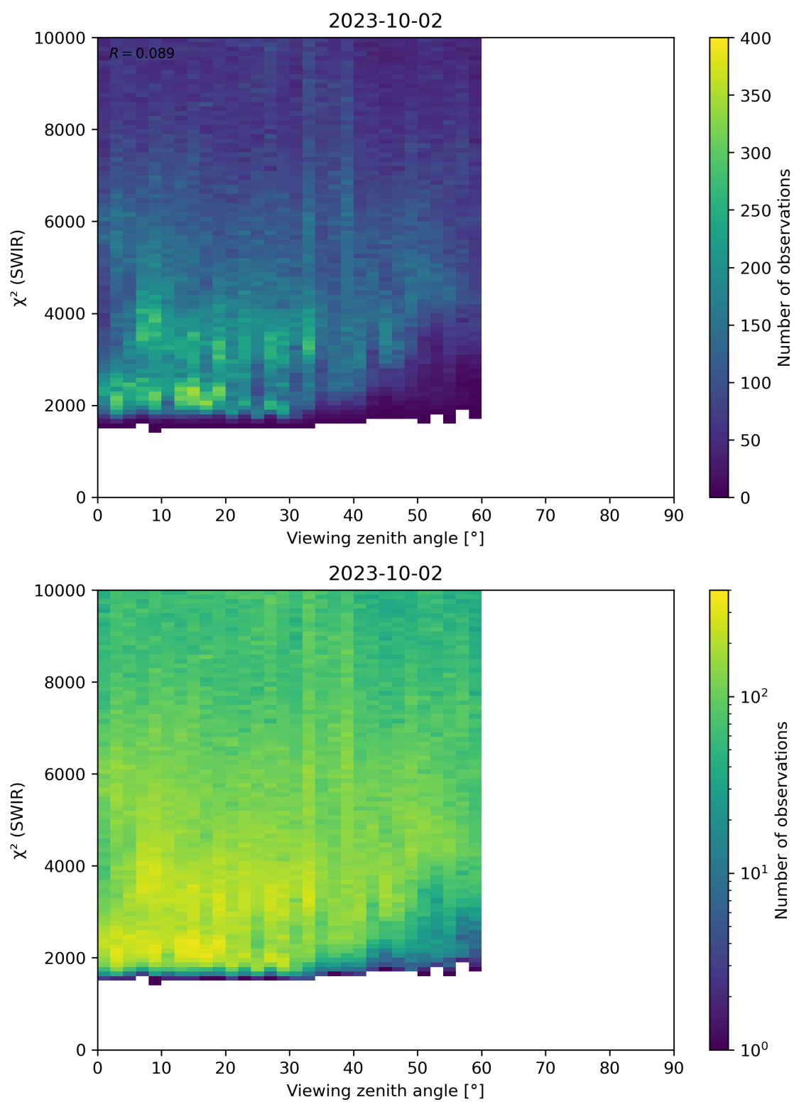
Figure 106: Scatter density plot of “Viewing zenith angle” against “ \chi^2 (SWIR)” for 2023-10-01 to 2023-10-03.
