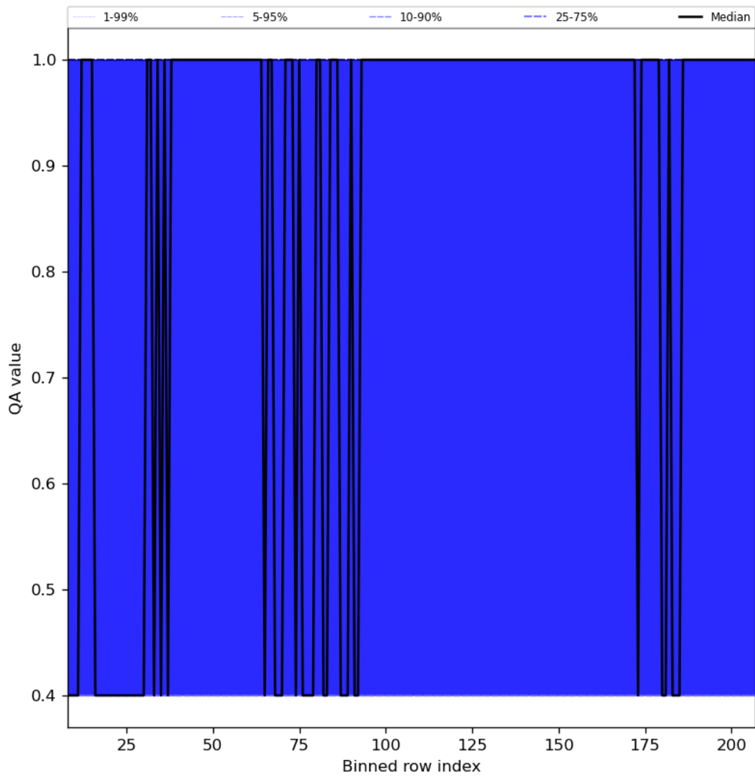
Figure 33: Along track statistics of “QA value” for 2023-10-01 to 2023-10-03
