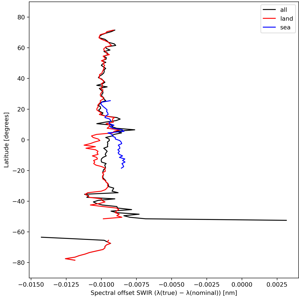
Figure 16: Zonal average of “Spectral offset SWIR ( \lambda(\text{true}) - \lambda(\text{nominal}) )” for 2023-10-01 to 2023-10-03.
