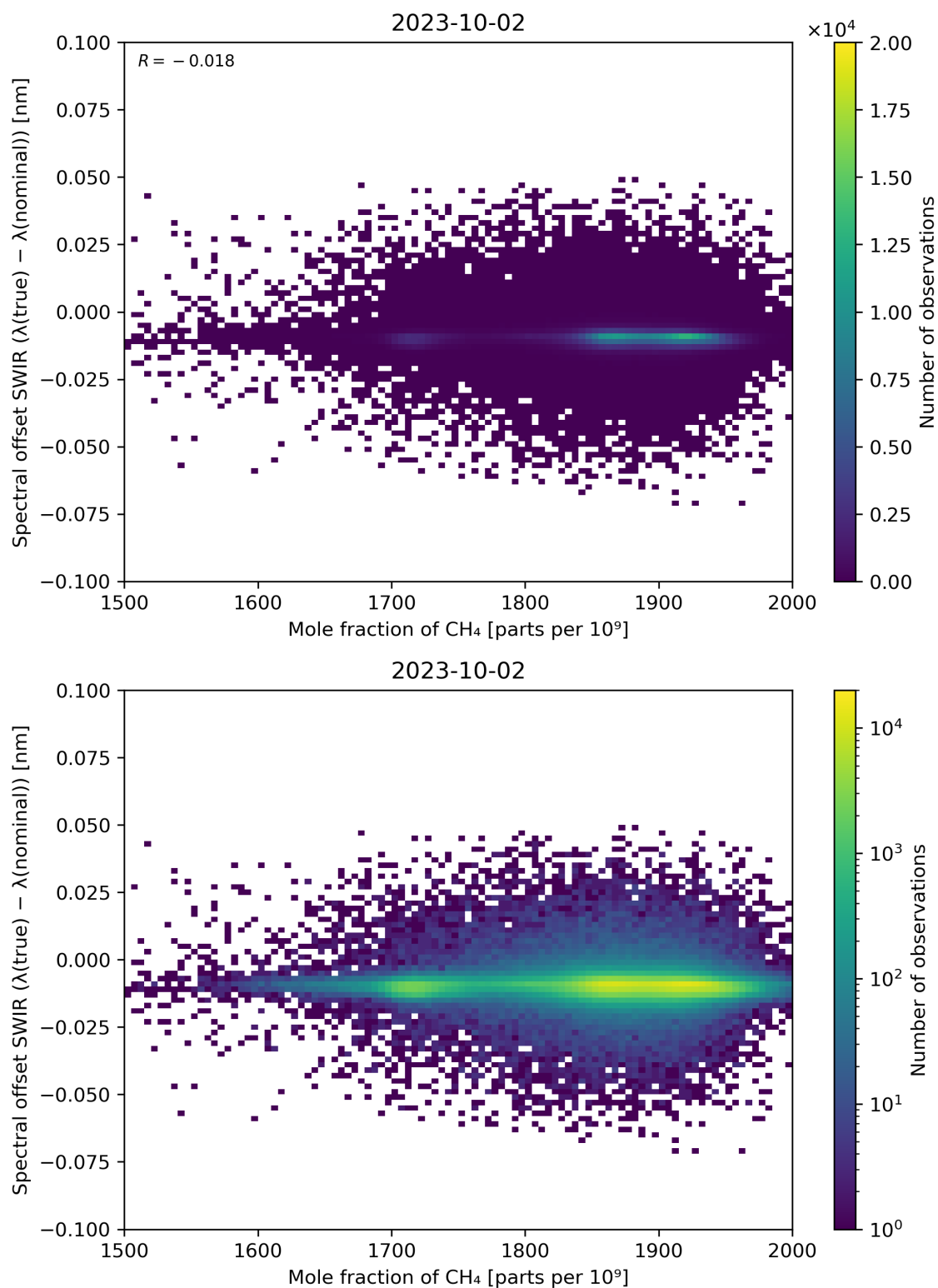
Figure 86: Scatter density plot of “Mole fraction of CH 4 ” against “Spectral offset SWIR ( \lambda(\text{true}) - \lambda(\text{nominal}) )” for 2023-10-01 to 2023-10-03.
