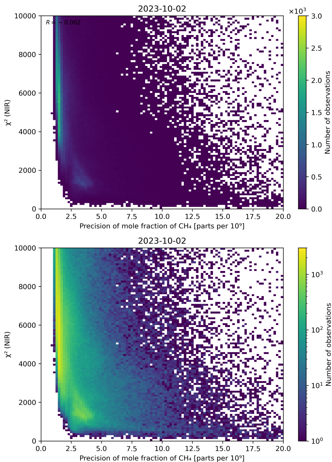
Figure 78: Scatter density plot of “Precision of mole fraction of CH 4 ” against “ \chi^2 (NIR)” for 2023-10-01 to 2023-10-03.
