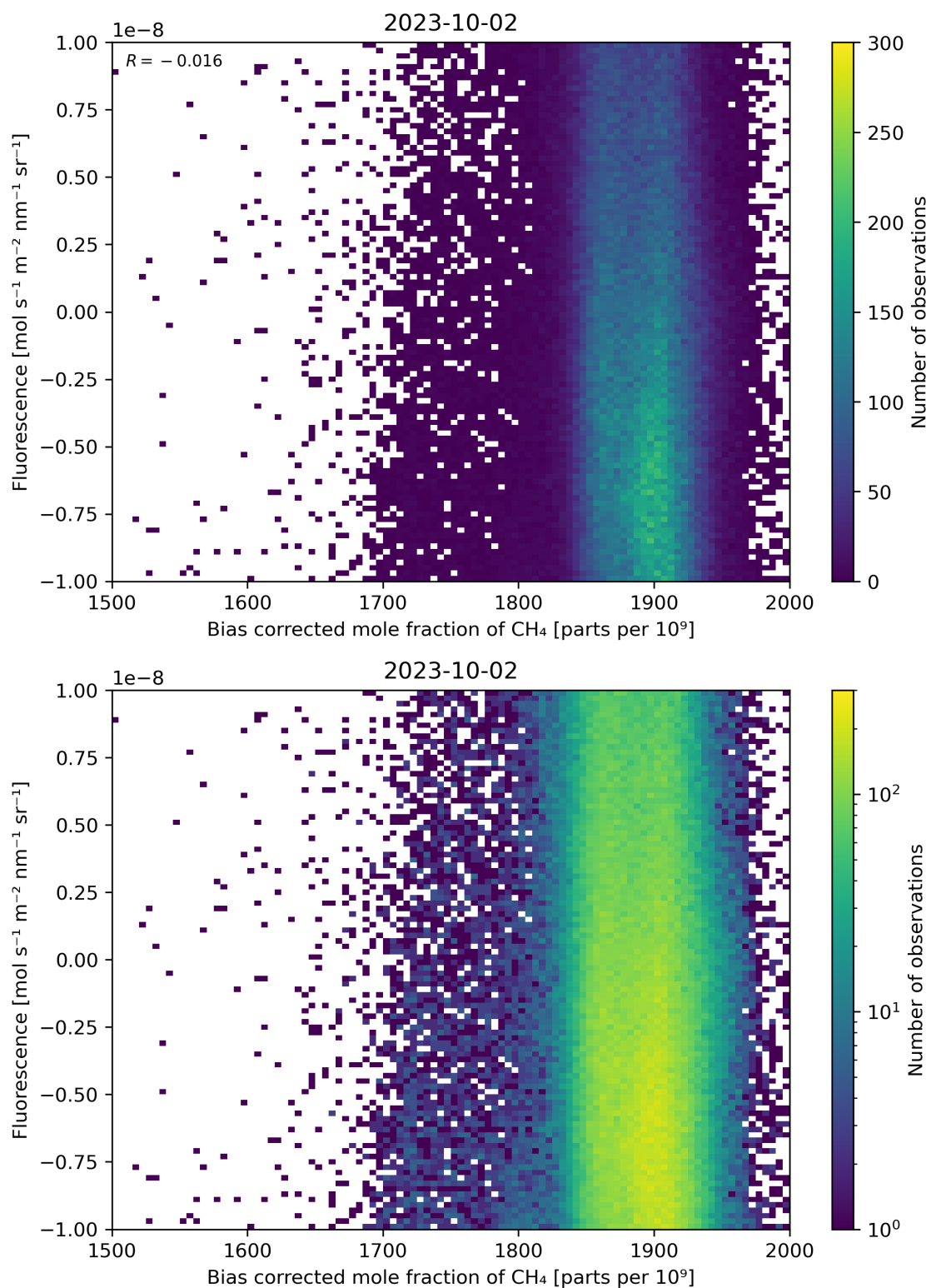
Figure 66: Scatter density plot of “Bias corrected mole fraction of \text{CH}_4 ” against “Fluorescence” for 2023-10-01 to 2023-10-03.
