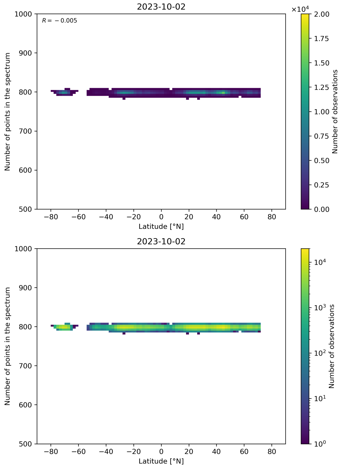
Figure 61: Scatter density plot of “Latitude” against “Number of points in the spectrum” for 2023-10-01 to 2023-10-03.
