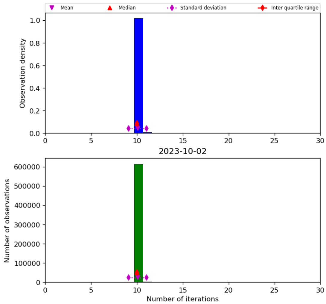
Figure 31: Histogram of “Number of iterations” for 2023-10-01 to 2023-10-03
