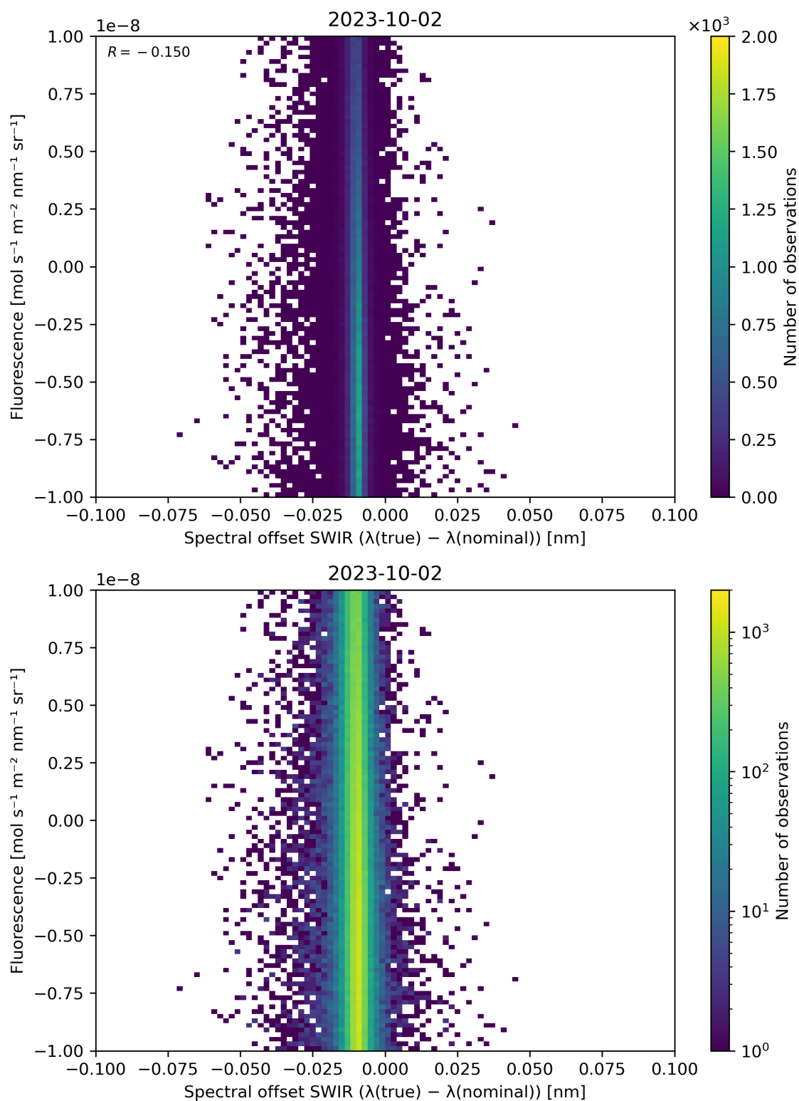
Figure 120: Scatter density plot of “Spectral offset SWIR ( \lambda(\text{true}) - \lambda(\text{nominal}) )” against “Fluorescence” for 2023-10-01 to 2023-10-03.
