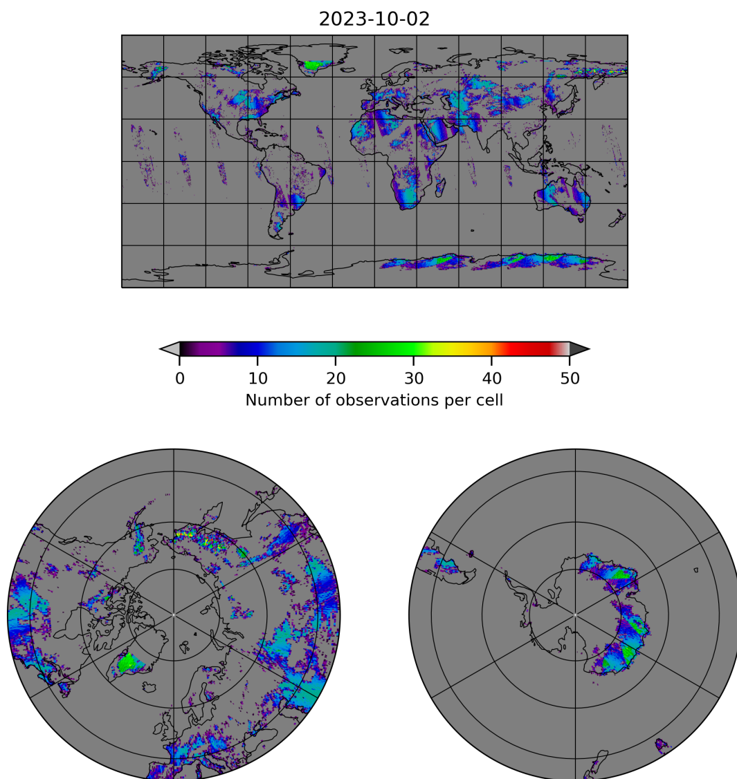
Figure 10: Map of the number of observations for 2023-10-01 to 2023-10-03
