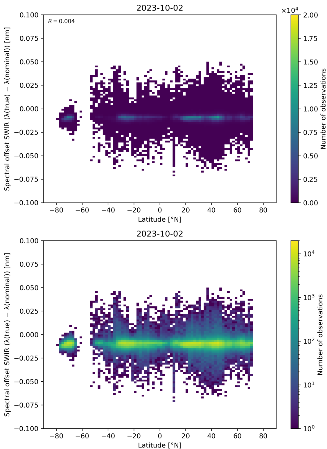
Figure 62: Scatter density plot of “Latitude” against “Spectral offset SWIR ( \lambda(\text{true}) - \lambda(\text{nominal}) )” for 2023-10-01 to 2023-10-03.
