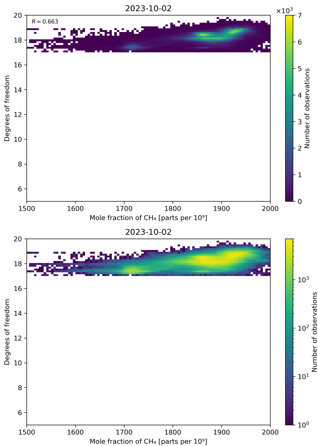
Figure 72: Scatter density plot of “Mole fraction of CH 4 ” against “Degrees of freedom” for 2023-10-01 to 2023-10-03.
