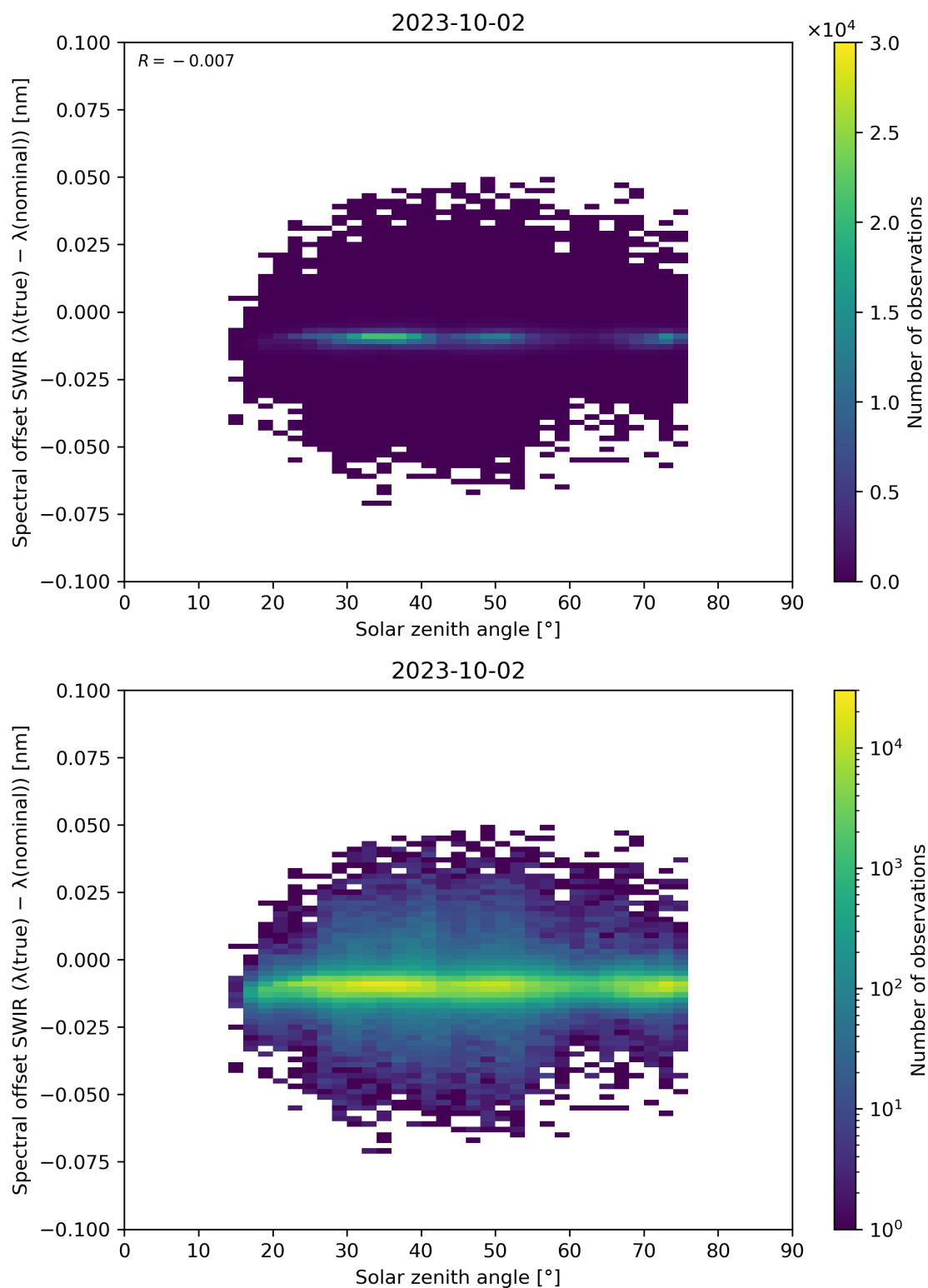
Figure 104: Scatter density plot of “Solar zenith angle” against “Spectral offset SWIR ( \lambda(\text{true}) - \lambda(\text{nominal}) )” for 2023-10-01 to 2023-10-03.
