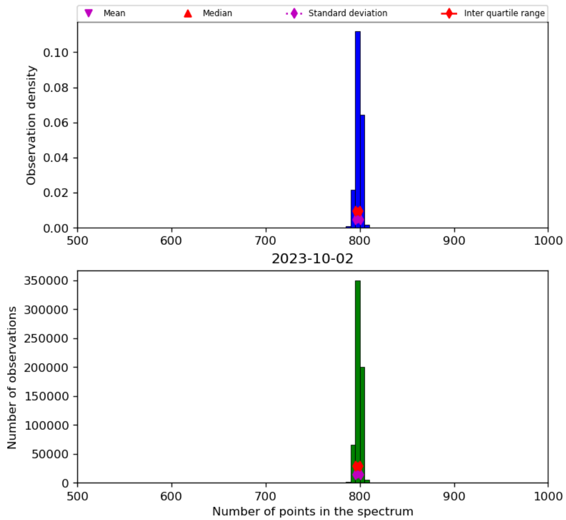
Figure 26: Histogram of “Number of points in the spectrum” for 2023-10-01 to 2023-10-03
