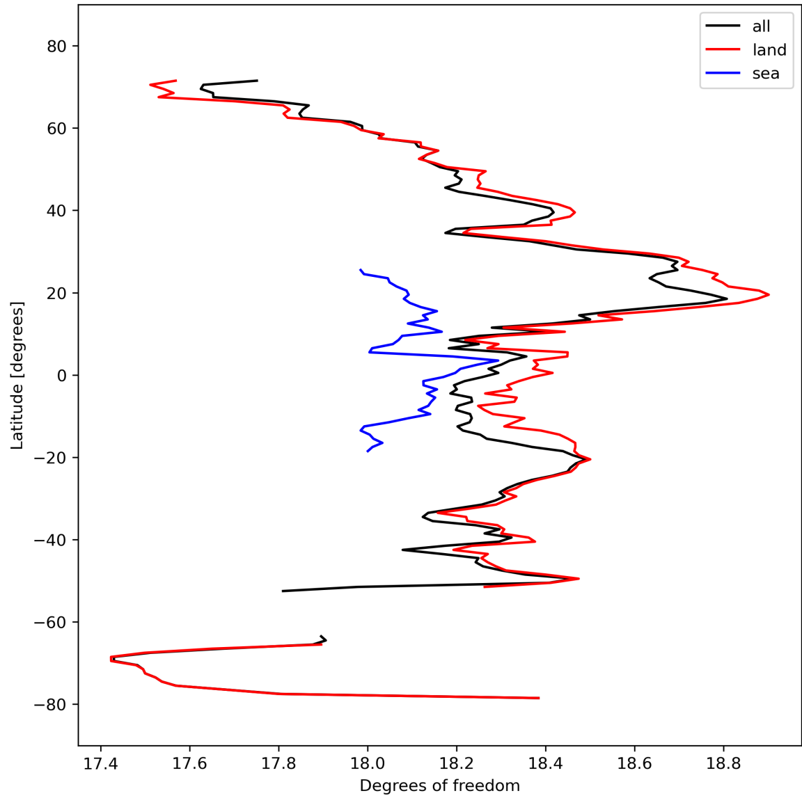
Figure 19: Zonal average of “Degrees of freedom” for 2023-10-01 to 2023-10-03.
