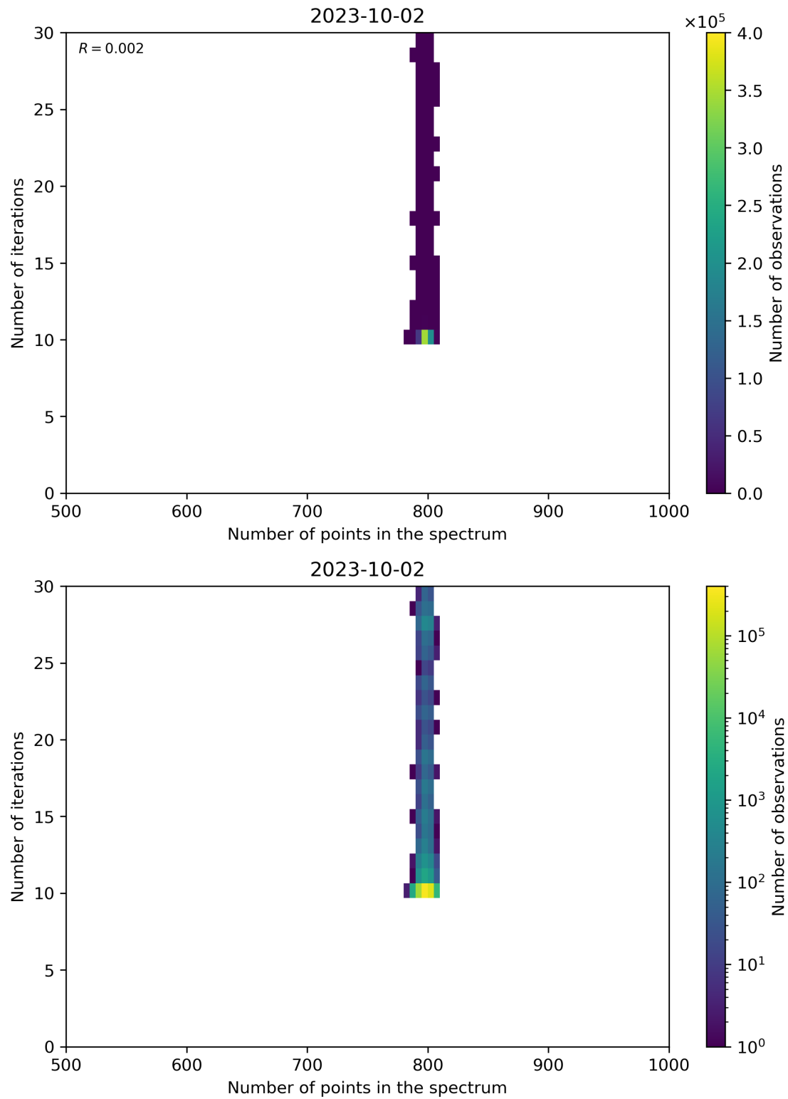
Figure 92: Scatter density plot of “Number of points in the spectrum” against “Number of iterations” for 2023-10-01 to 2023-10-03.
