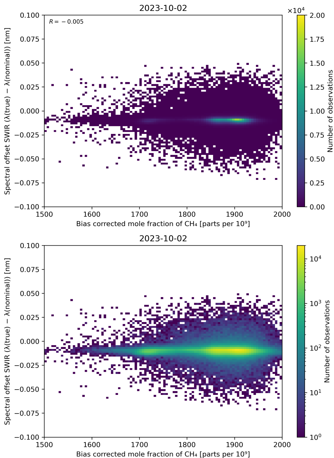
Figure 69: Scatter density plot of “Bias corrected mole fraction of \text{CH}_4 ” against “Spectral offset SWIR ( \lambda(\text{true}) - \lambda(\text{nominal}) )” for 2023-10-01 to 2023-10-03.
