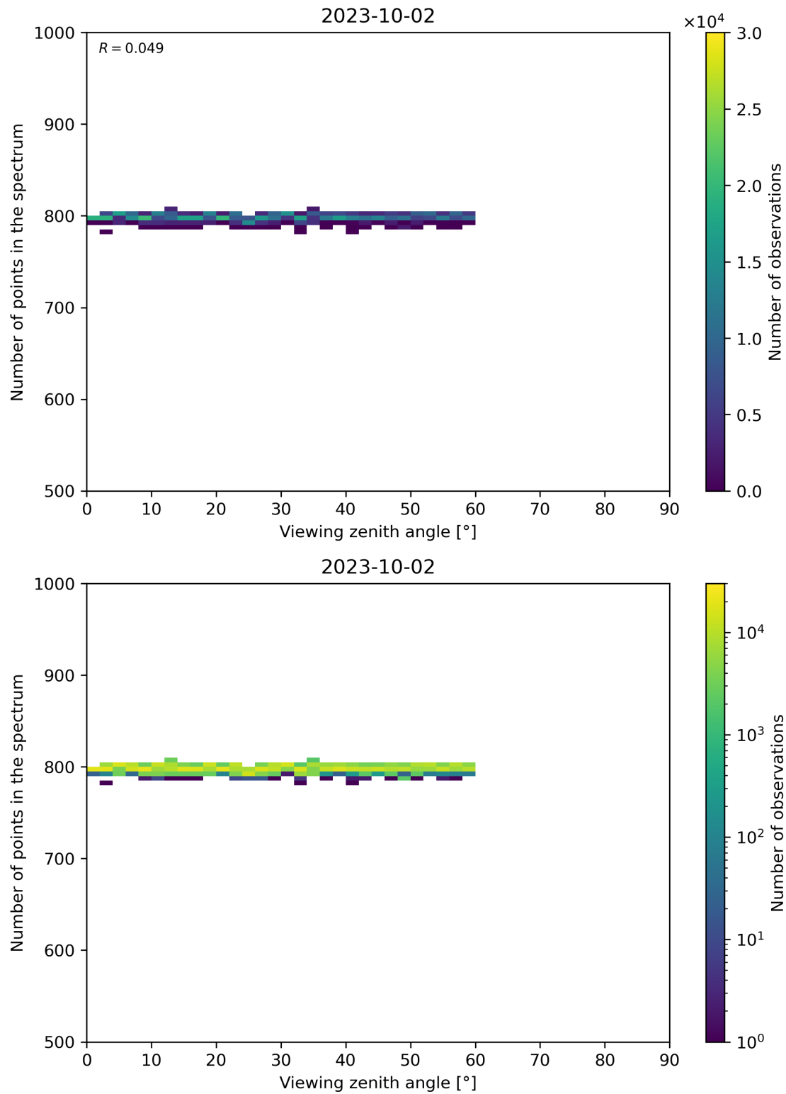
Figure 114: Scatter density plot of “Viewing zenith angle” against “Number of points in the spectrum” for 2023-10-01 to 2023-10-03.
