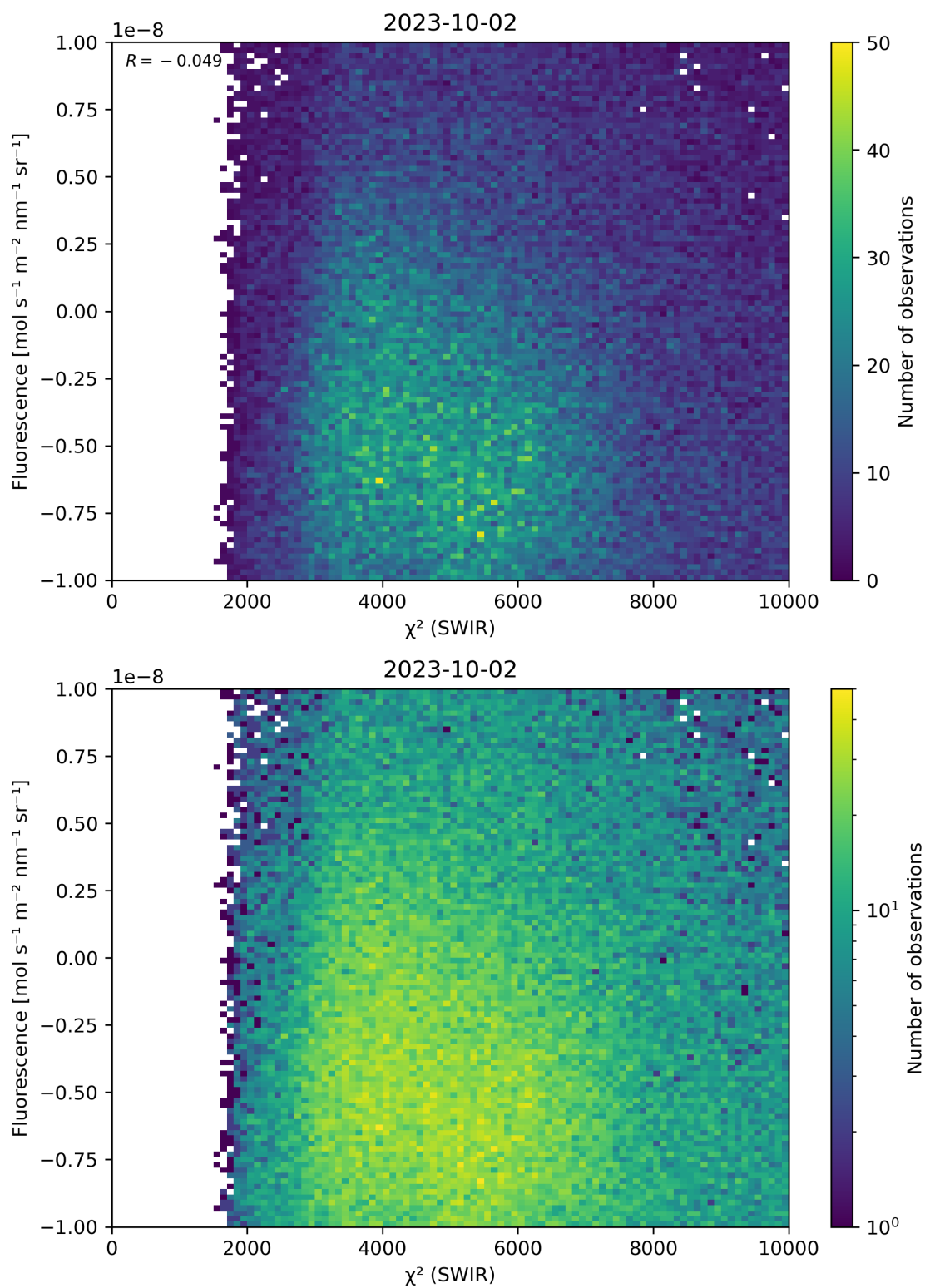
Figure 49: Scatter density plot of “ \chi^2 (SWIR)” against “Fluorescence” for 2023-10-01 to 2023-10-03.
