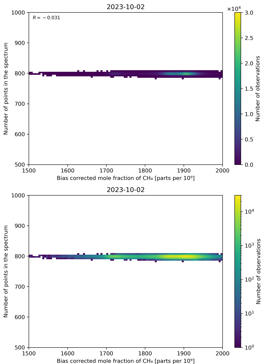
Figure 68: Scatter density plot of “Bias corrected mole fraction of CH 4 ” against “Number of points in the spectrum” for 2023-10-01 to 2023-10-03.
