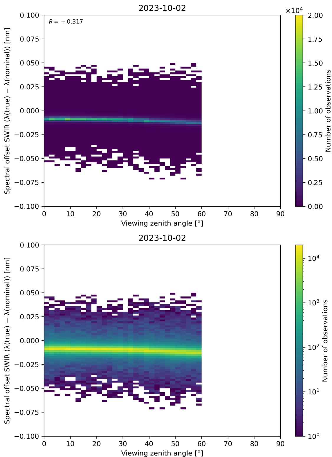
Figure 116: Scatter density plot of “Viewing zenith angle” against “Spectral offset SWIR ( \lambda(\text{true}) - \lambda(\text{nominal}) )” for 2023-10-01 to 2023-10-03.
