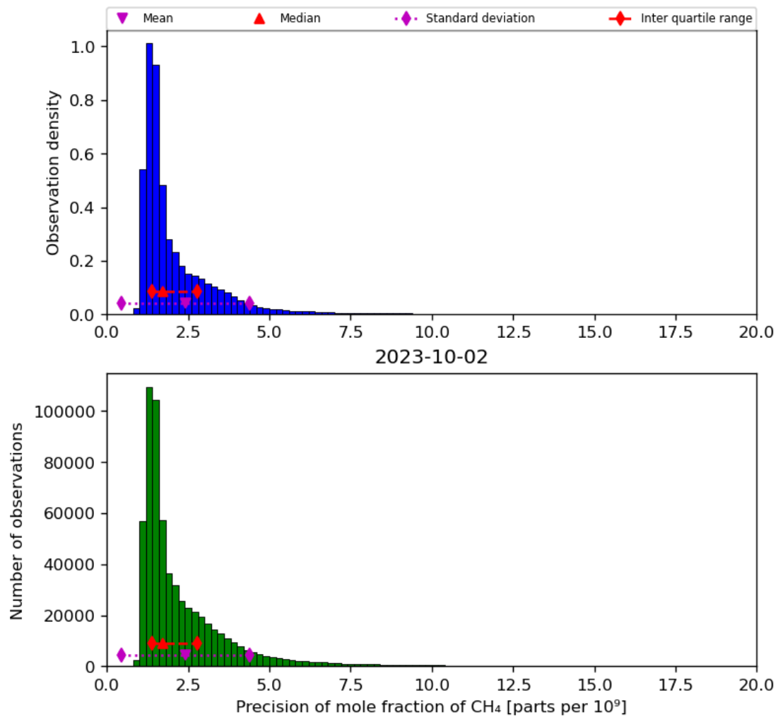
Figure 24: Histogram of “Precision of mole fraction of CH 4 ” for 2023-10-01 to 2023-10-03
