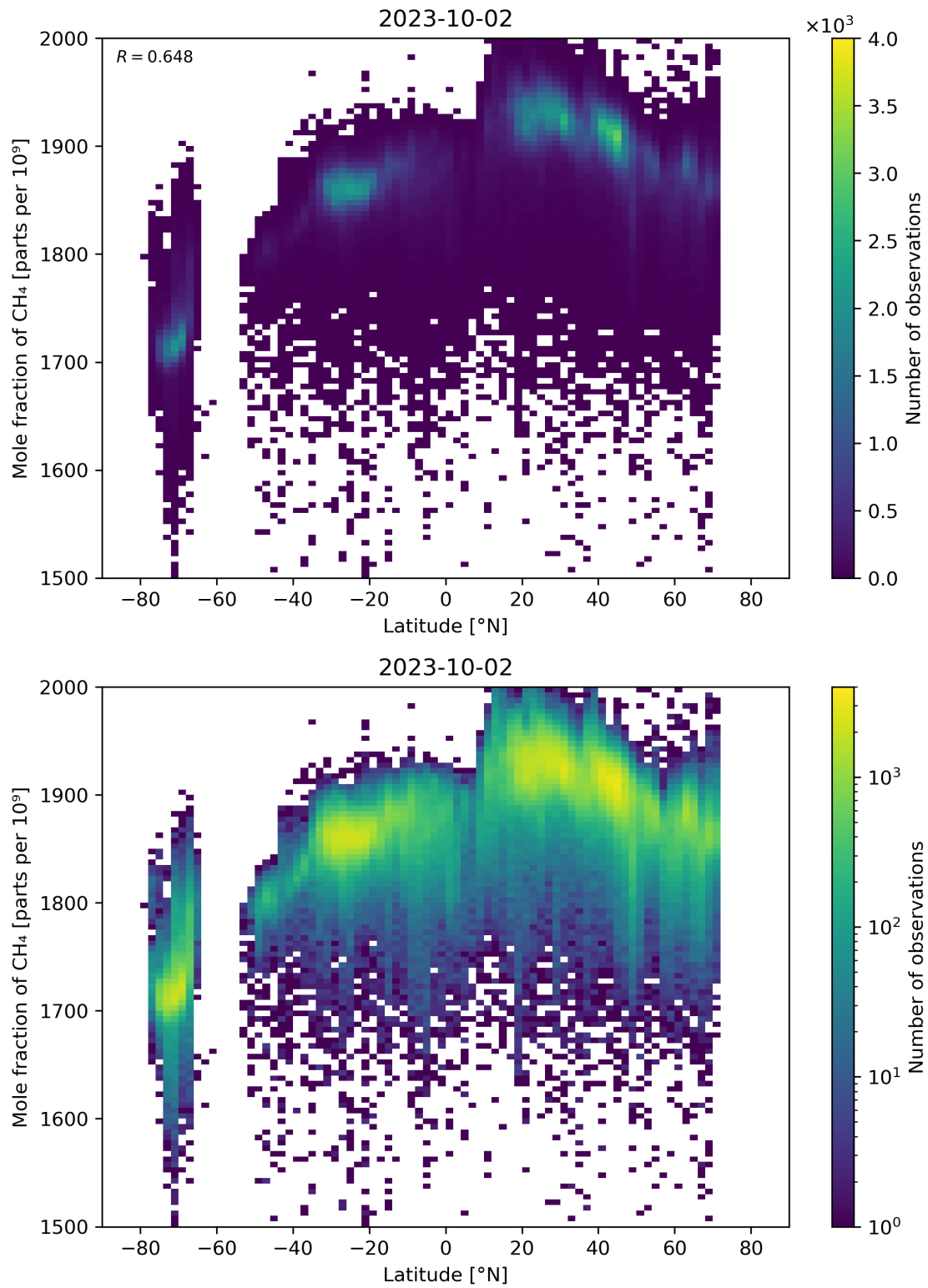
Figure 57: Scatter density plot of “Latitude” against “Mole fraction of CH 4 ” for 2023-10-01 to 2023-10-03.
