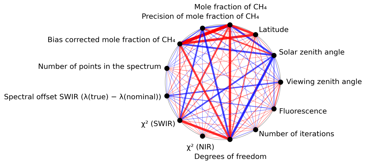
Figure 1: Map of correlation graph for 2023-10-01 to 2023-10-03.
