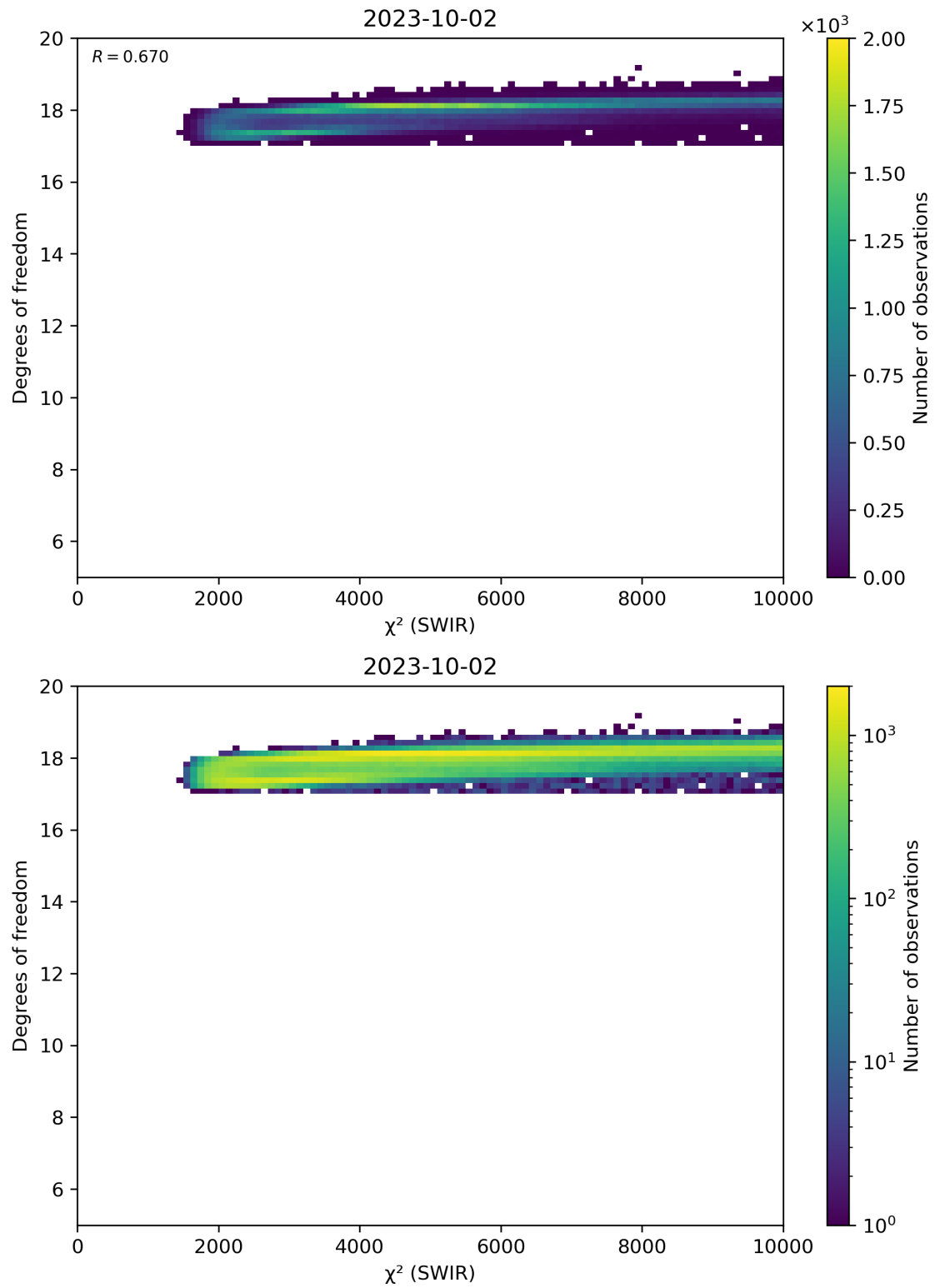
Figure 48: Scatter density plot of “ \chi^2 (SWIR)” against “Degrees of freedom” for 2023-10-01 to 2023-10-03.
