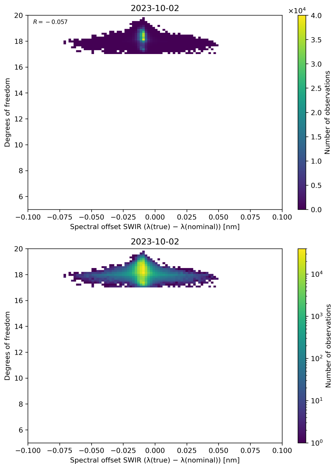
Figure 119: Scatter density plot of “Spectral offset SWIR ( \lambda(\text{true}) - \lambda(\text{nominal}) )” against “Degrees of freedom” for 2023-10-01 to 2023-10-03.
