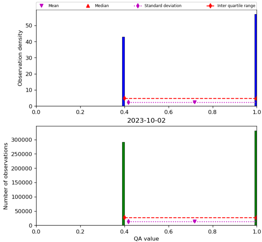
Figure 22: Histogram of “QA value” for 2023-10-01 to 2023-10-03
