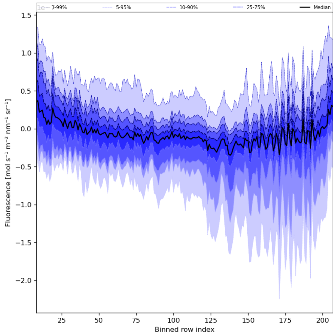
Figure 43: Along track statistics of “Fluorescence” for 2023-10-01 to 2023-10-03
