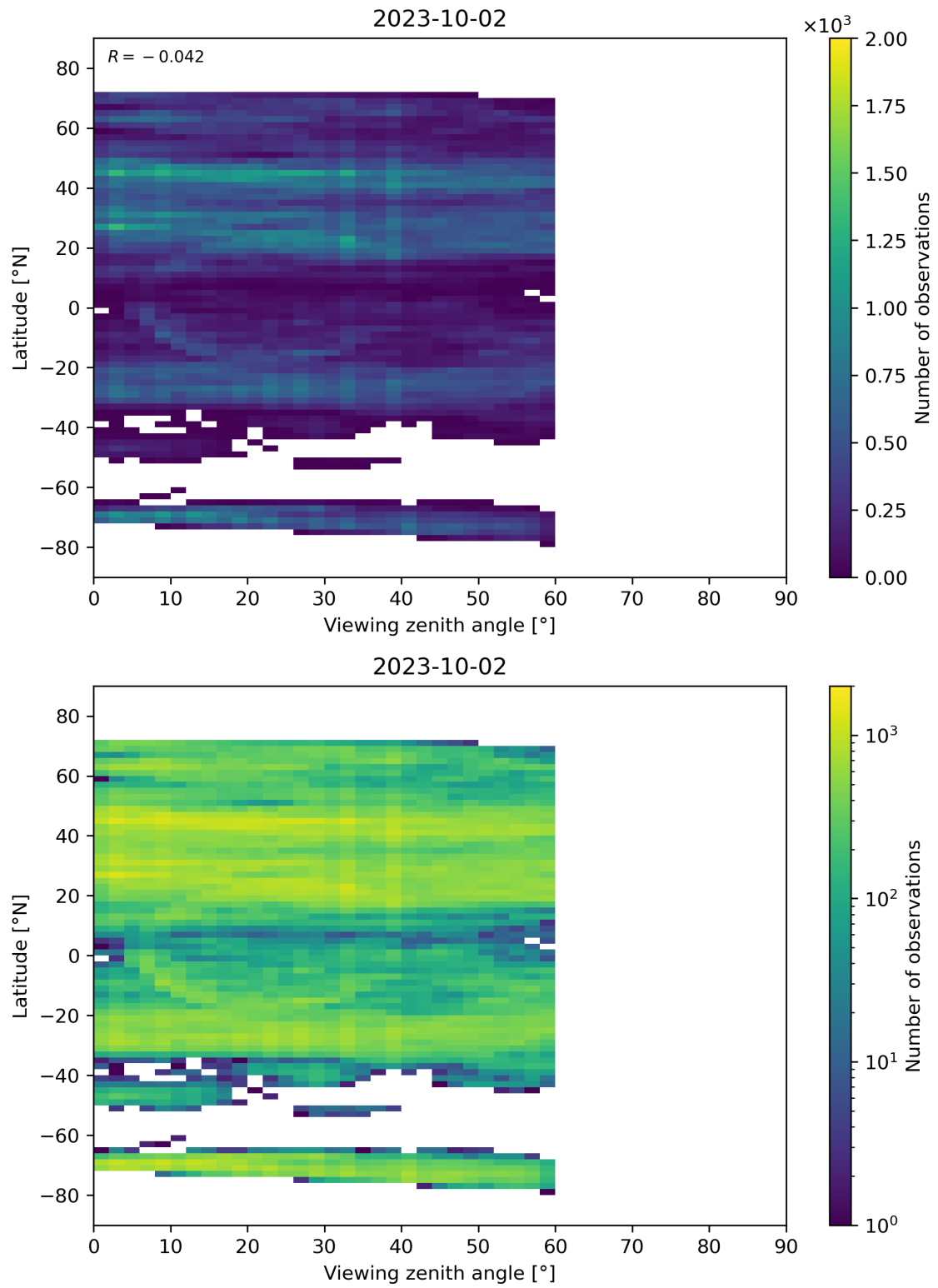
Figure 109: Scatter density plot of “Viewing zenith angle” against “Latitude” for 2023-10-01 to 2023-10-03.
