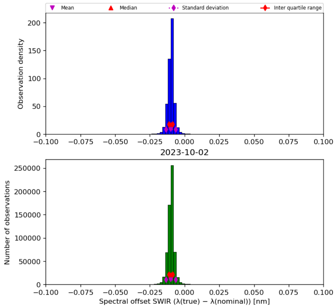
Figure 27: Histogram of “Spectral offset SWIR ( \lambda(\text{true}) - \lambda(\text{nominal}) )” for 2023-10-01 to 2023-10-03
