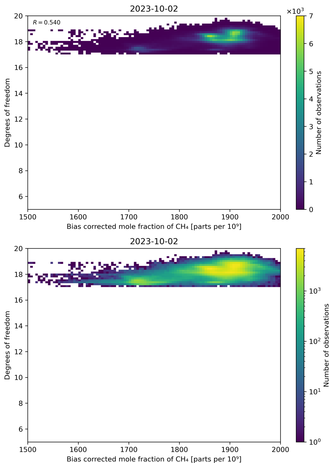
Figure 65: Scatter density plot of “Bias corrected mole fraction of CH 4 ” against “Degrees of freedom” for 2023-10-01 to 2023-10-03.
