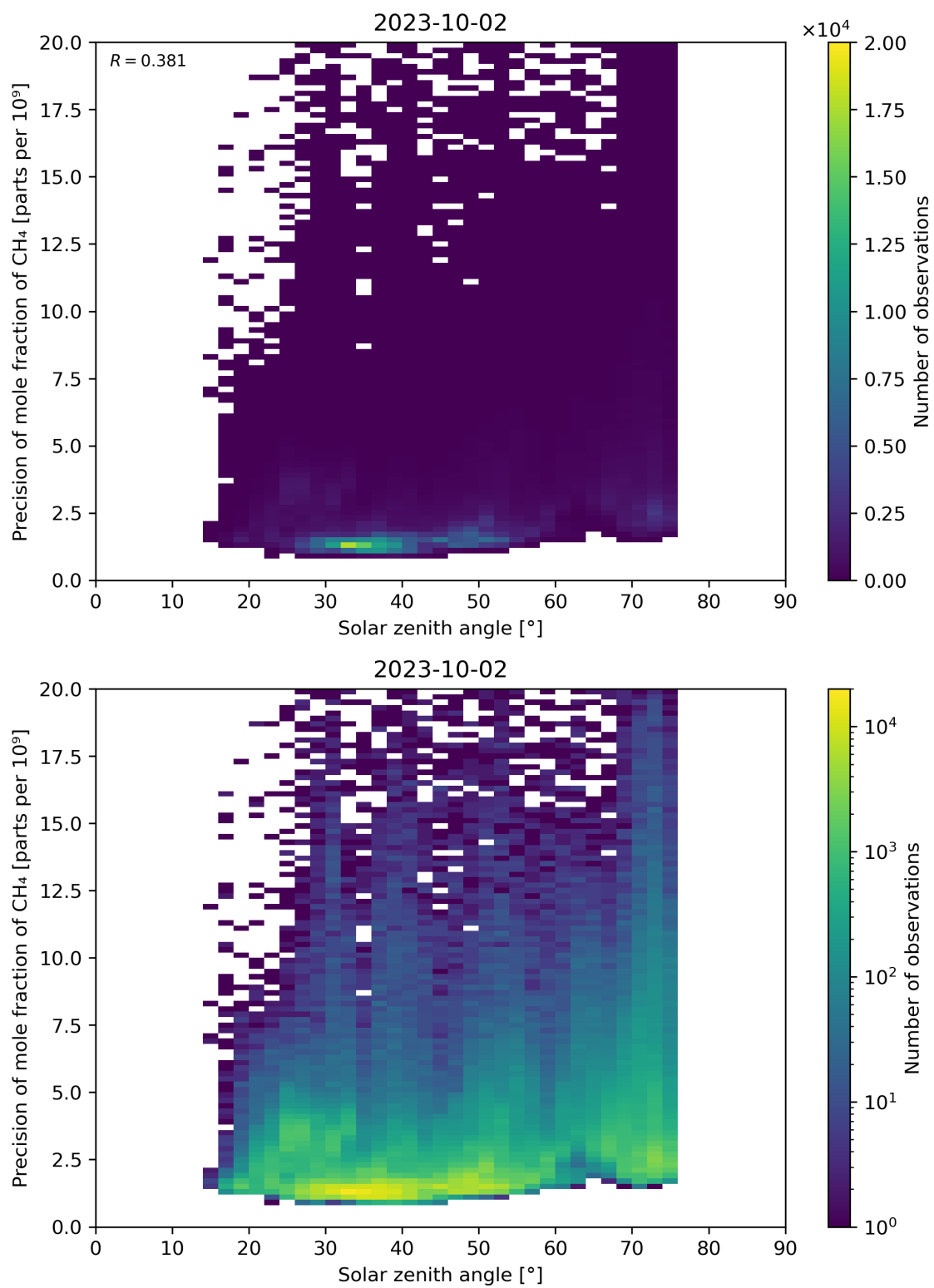
Figure 101: Scatter density plot of “Solar zenith angle” against “Precision of mole fraction of CH 4 ” for 2023-10-01 to 2023-10-03.
