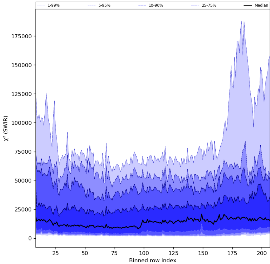
Figure 39: Along track statistics of " \chi^2 (SWIR)" for 2023-10-01 to 2023-10-03
