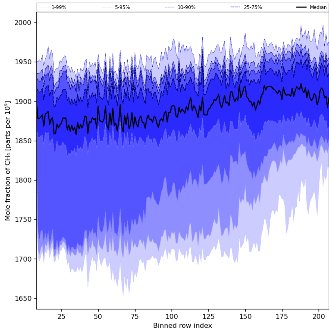
Figure 34: Along track statistics of “Mole fraction of CH 4 ” for 2023-10-01 to 2023-10-03
