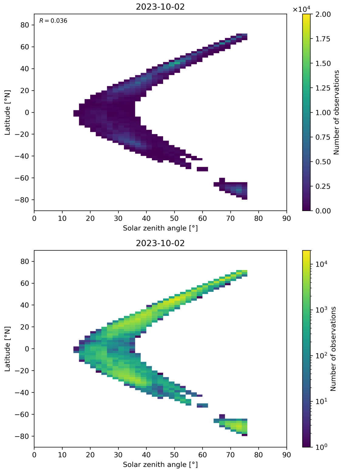
Figure 98: Scatter density plot of “Solar zenith angle” against “Latitude” for 2023-10-01 to 2023-10-03.
