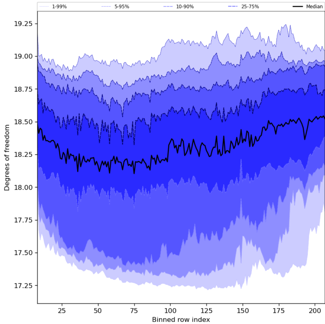
Figure 41: Along track statistics of “Degrees of freedom” for 2023-10-01 to 2023-10-03
