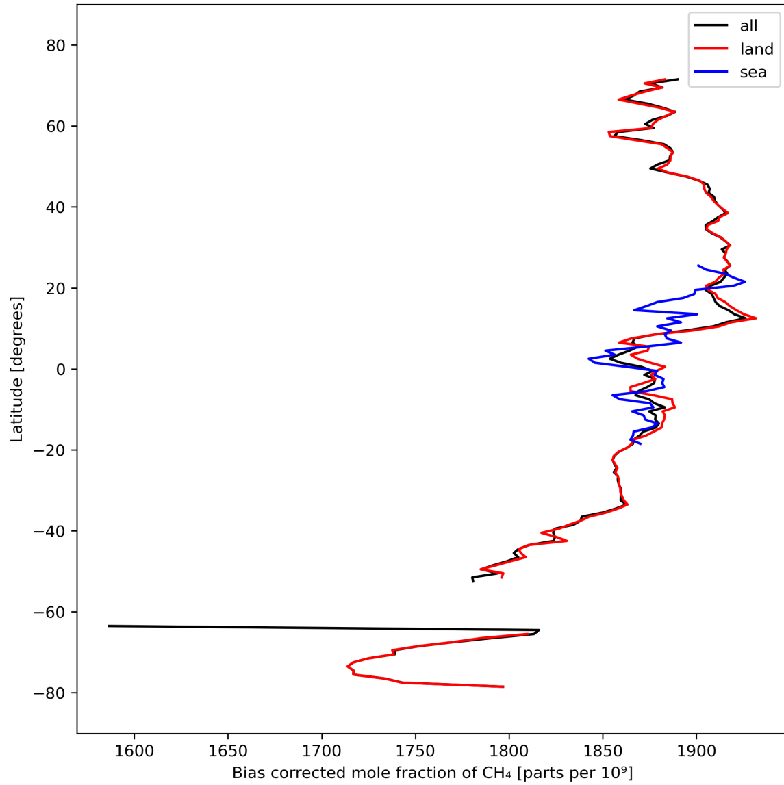
Figure 14: Zonal average of “Bias corrected mole fraction of CH 4 ” for 2023-10-01 to 2023-10-03.
