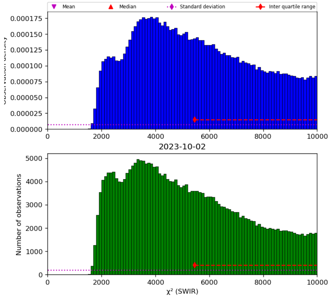
Figure 28: Histogram of “ \chi^2 (SWIR)” for 2023-10-01 to 2023-10-03
