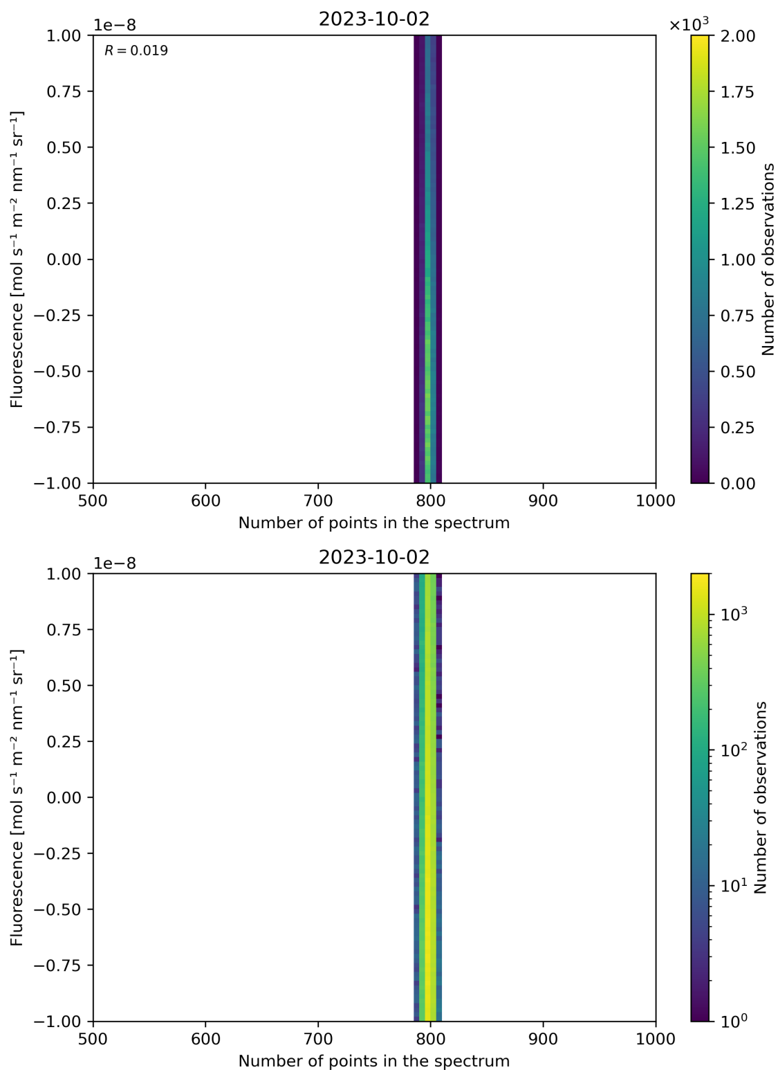
Figure 91: Scatter density plot of “Number of points in the spectrum” against “Fluorescence” for 2023-10-01 to 2023-10-03.
