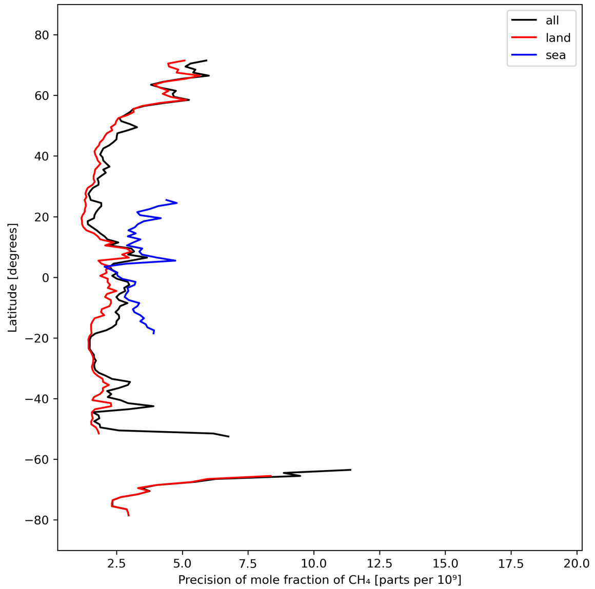
Figure 13: Zonal average of “Precision of mole fraction of CH 4 ” for 2023-10-01 to 2023-10-03.
