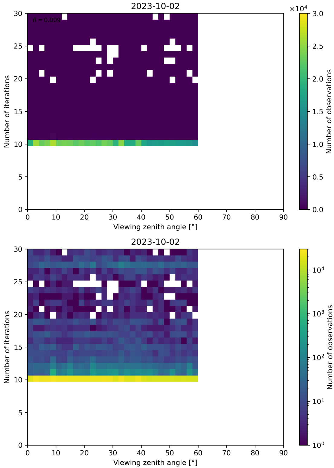
Figure 113: Scatter density plot of “Viewing zenith angle” against “Number of iterations” for 2023-10-01 to 2023-10-03.
