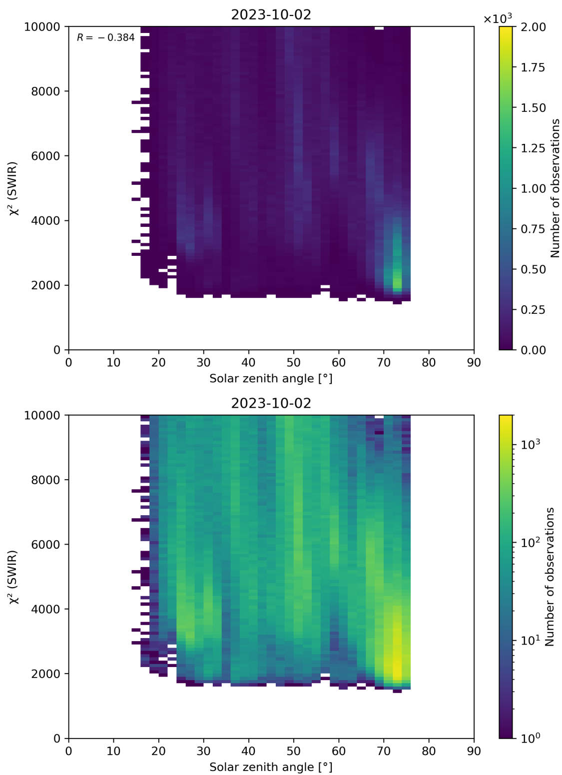
Figure 95: Scatter density plot of “Solar zenith angle” against “ \chi^2 (SWIR)” for 2023-10-01 to 2023-10-03.
