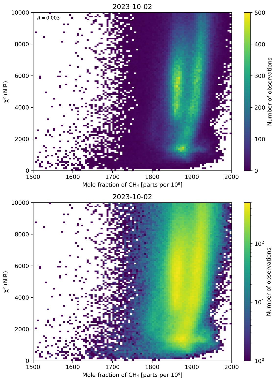
Figure 70: Scatter density plot of “Mole fraction of CH 4 ” against “ \chi^2 (NIR)” for 2023-10-01 to 2023-10-03.
