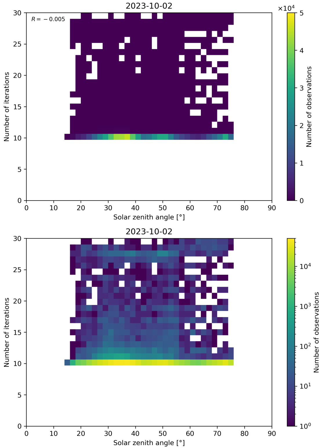
Figure 102: Scatter density plot of “Solar zenith angle” against “Number of iterations” for 2023-10-01 to 2023-10-03.
