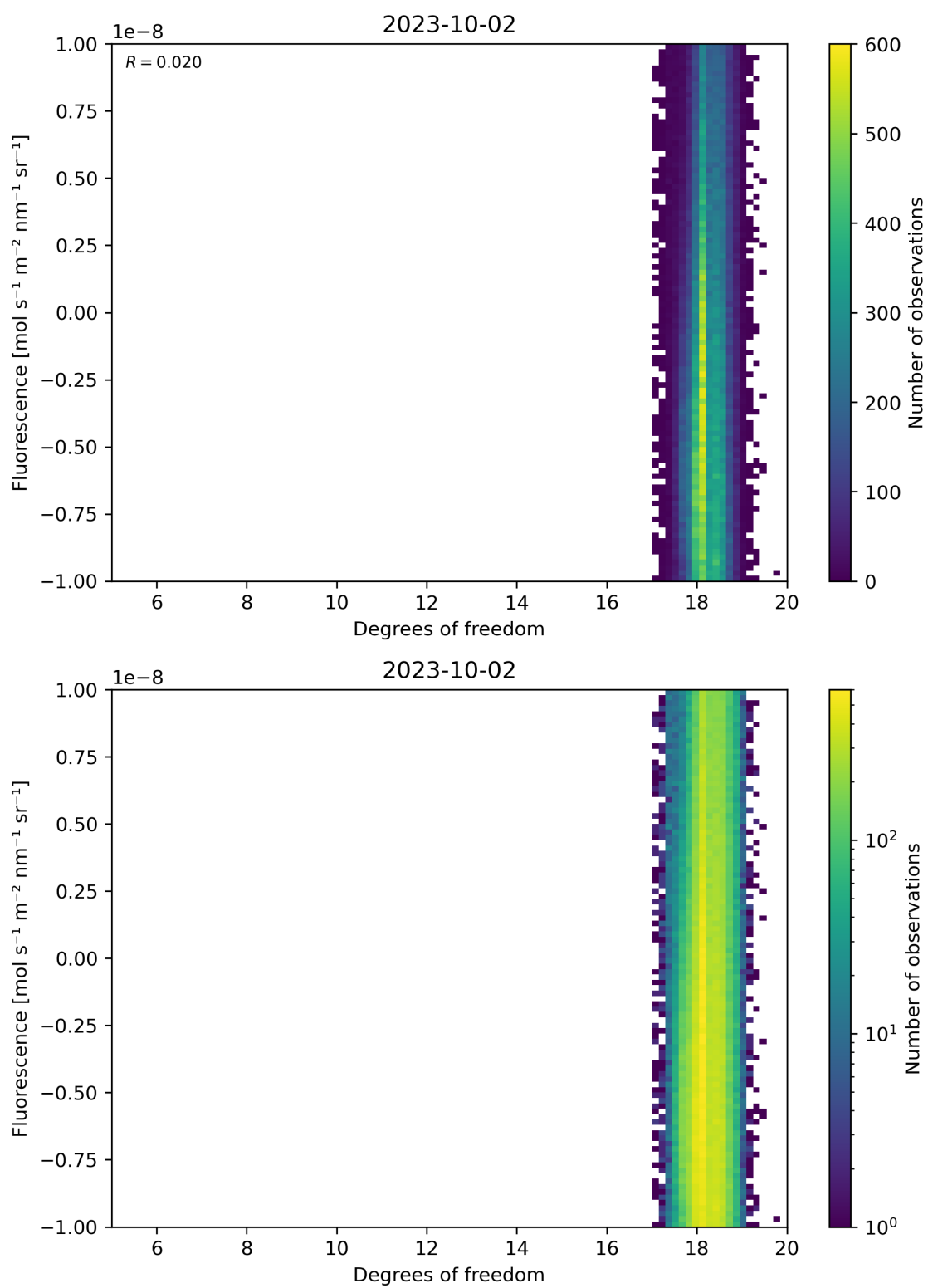
Figure 51: Scatter density plot of “Degrees of freedom” against “Fluorescence” for 2023-10-01 to 2023-10-03.
