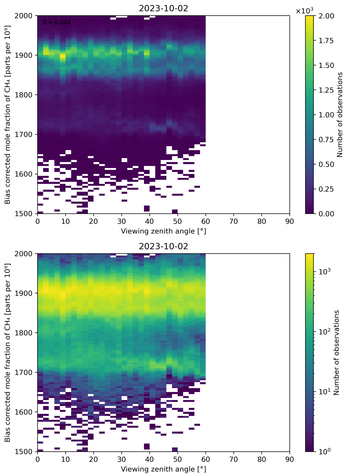
Figure 111: Scatter density plot of “Viewing zenith angle” against “Bias corrected mole fraction of CH 4 ” for 2023-10-01 to 2023-10-03.
