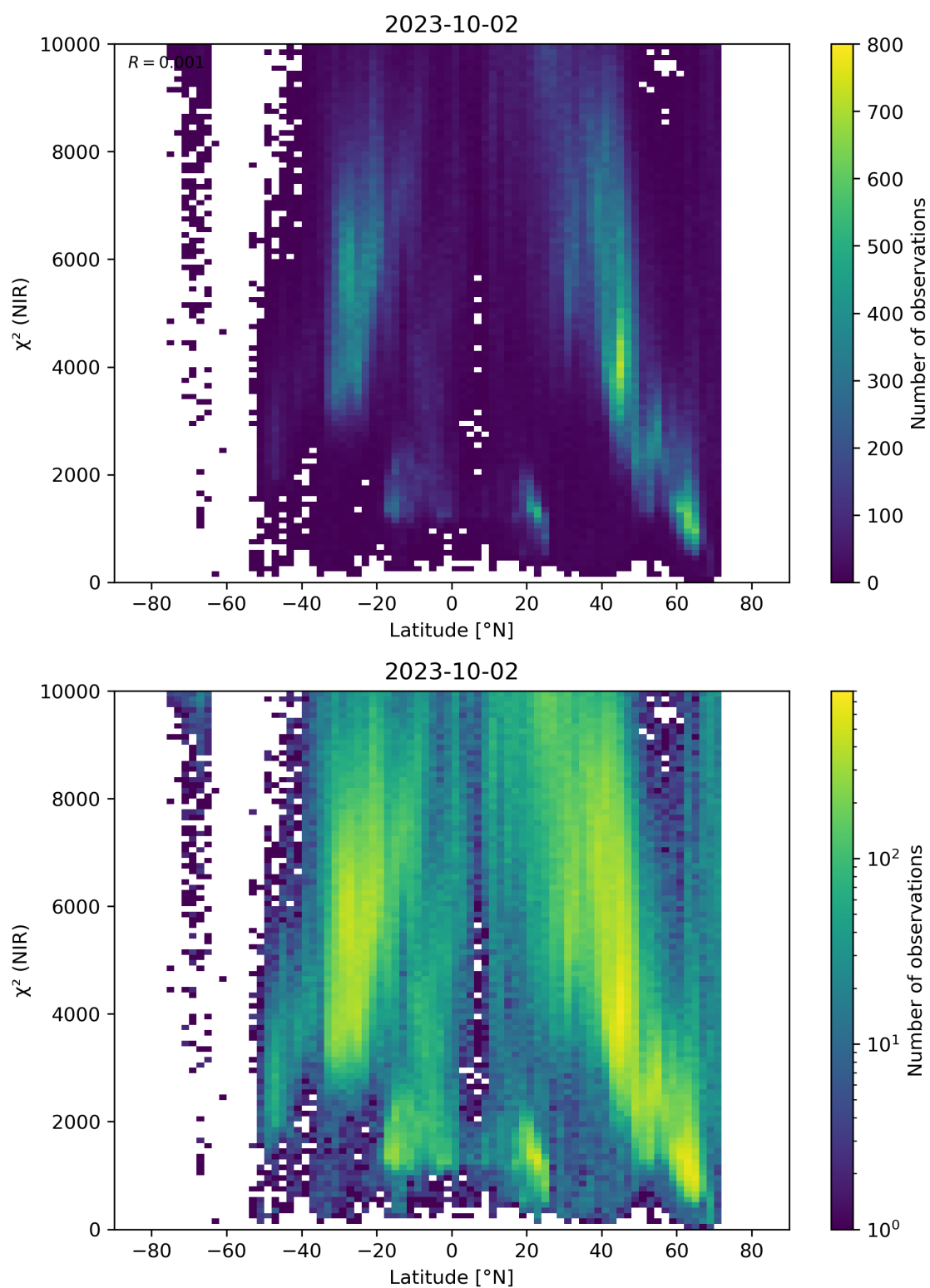
Figure 53: Scatter density plot of “Latitude” against “ \chi^2 (NIR)” for 2023-10-01 to 2023-10-03.
