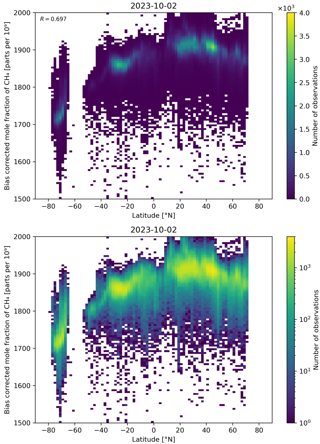
Figure 58: Scatter density plot of “Latitude” against “Bias corrected mole fraction of CH 4 ” for 2023-10-01 to 2023-10-03.
