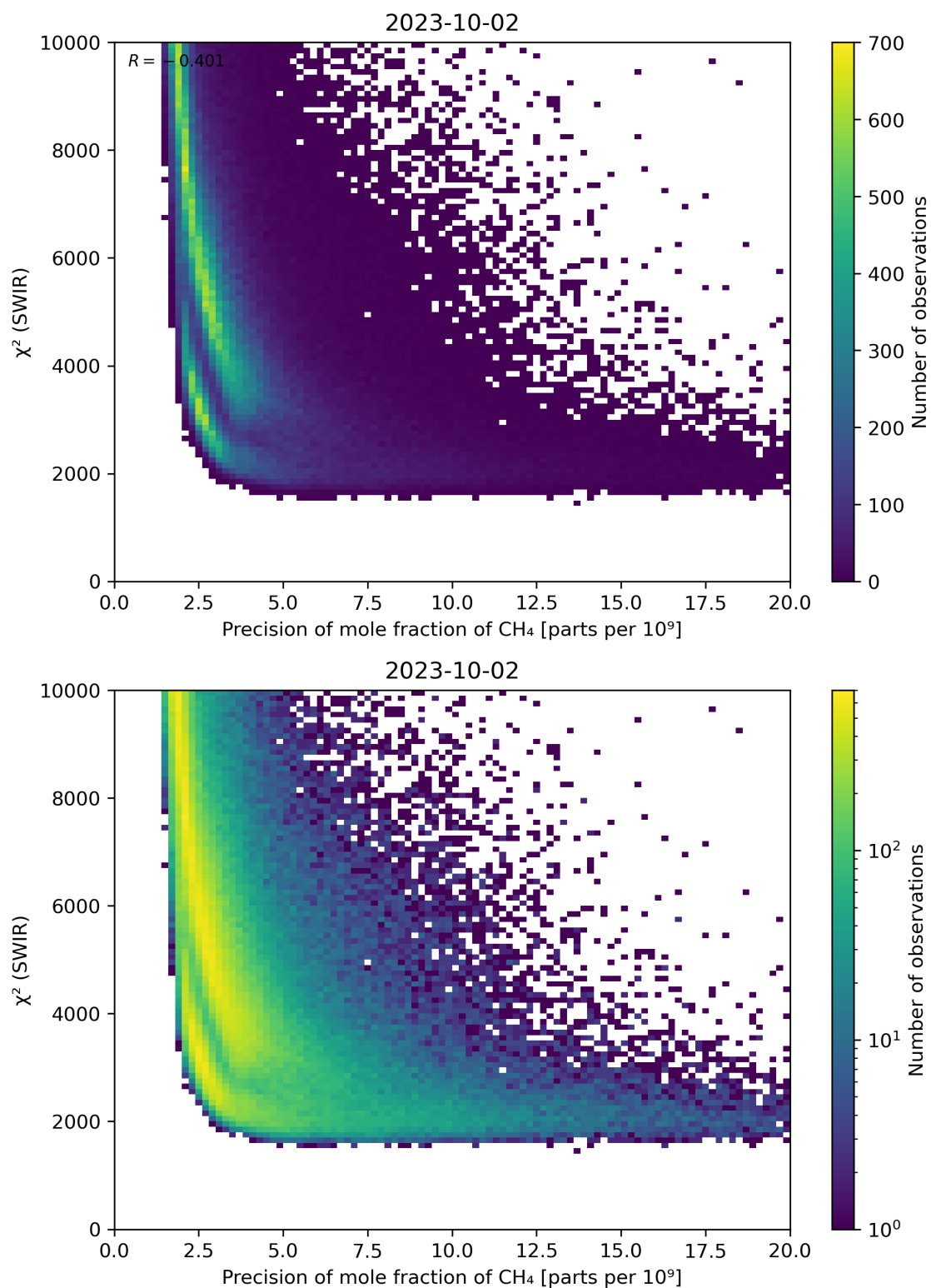
Figure 79: Scatter density plot of “Precision of mole fraction of \text{CH}_4 ” against “ \chi^2 (SWIR)” for 2023-10-01 to 2023-10-03.
