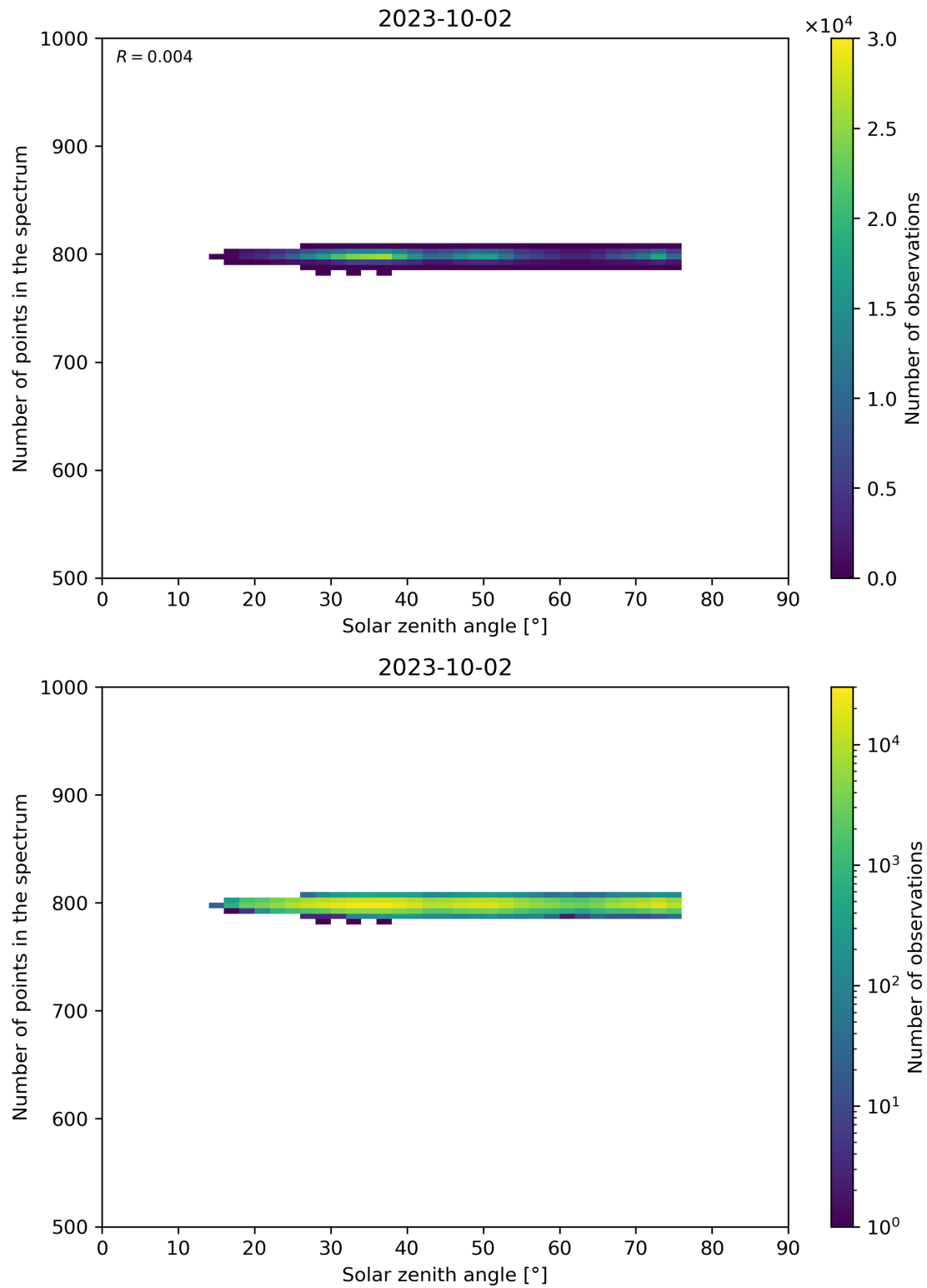
Figure 103: Scatter density plot of “Solar zenith angle” against “Number of points in the spectrum” for 2023-10-01 to 2023-10-03.
