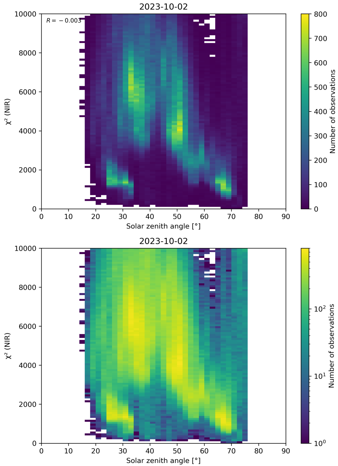
Figure 94: Scatter density plot of “Solar zenith angle” against “ \chi^2 (NIR)” for 2023-10-01 to 2023-10-03.
