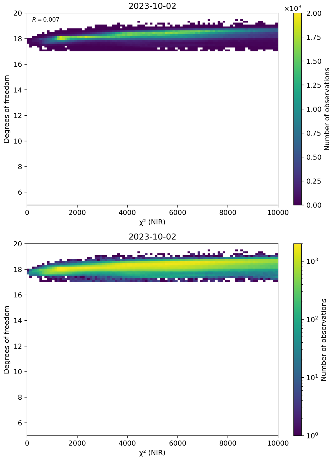
Figure 44: Scatter density plot of “ \chi^2 (NIR)” against “Degrees of freedom” for 2023-10-01 to 2023-10-03.
