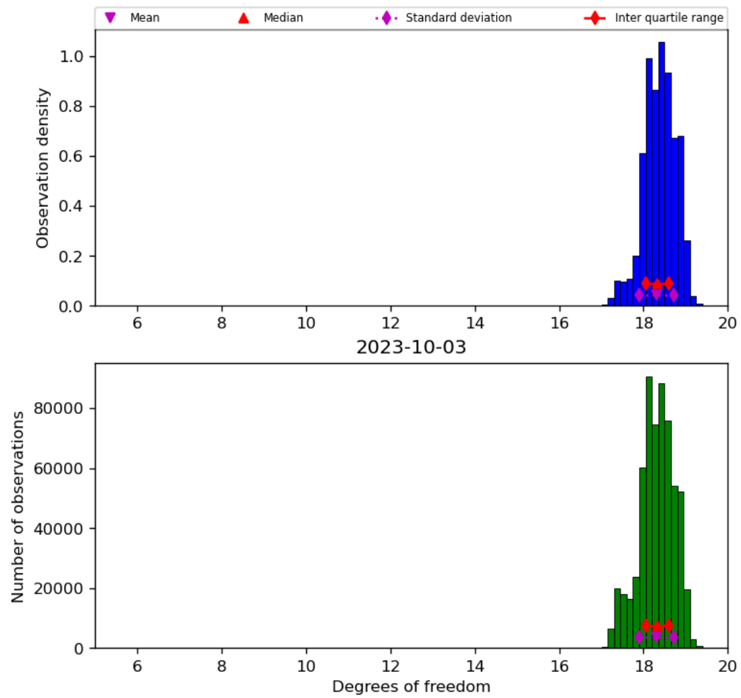
Figure 30: Histogram of “Degrees of freedom” for 2023-10-02 to 2023-10-04
