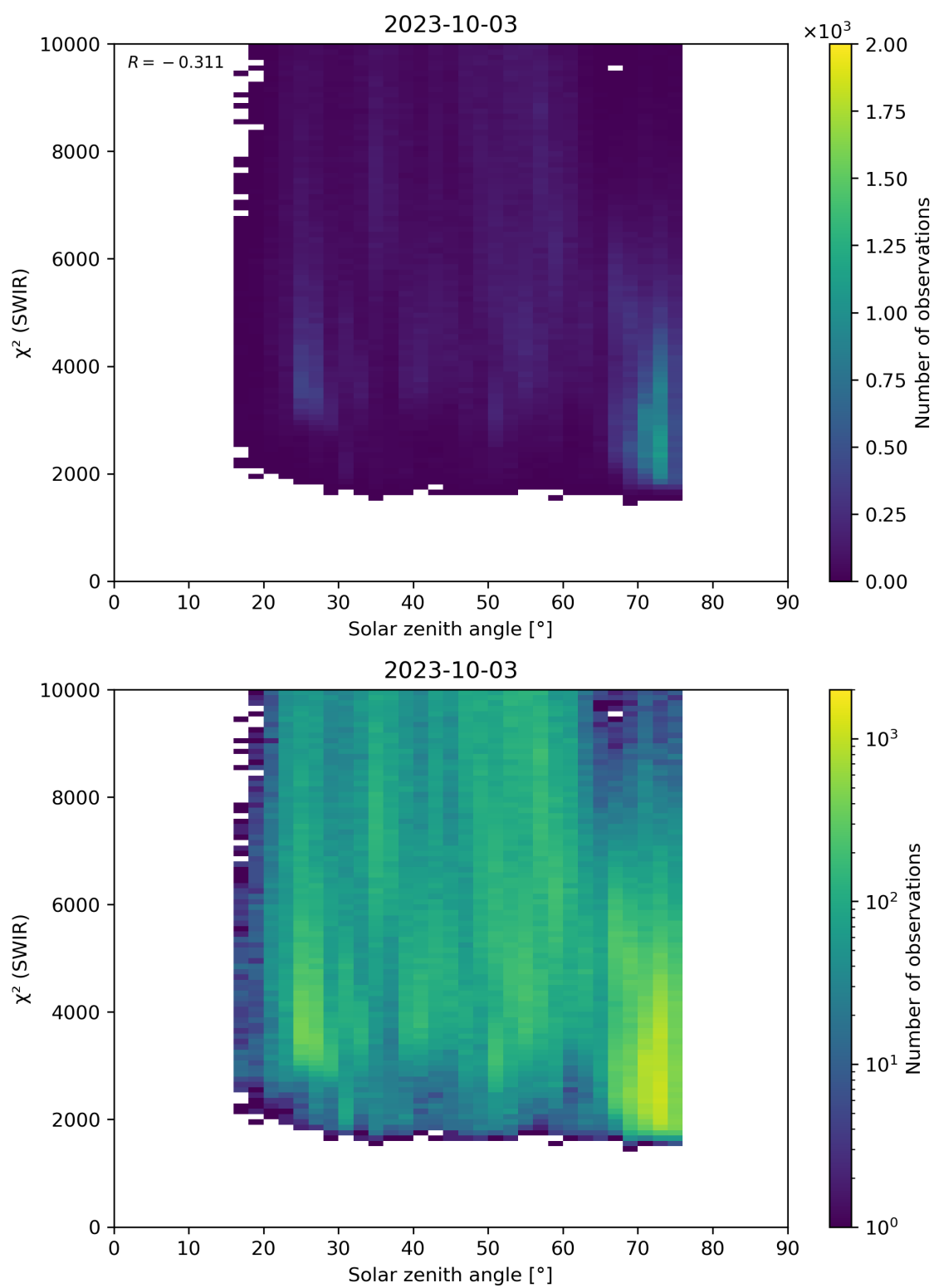
Figure 95: Scatter density plot of “Solar zenith angle” against “ \chi^2 (SWIR)” for 2023-10-02 to 2023-10-04.
