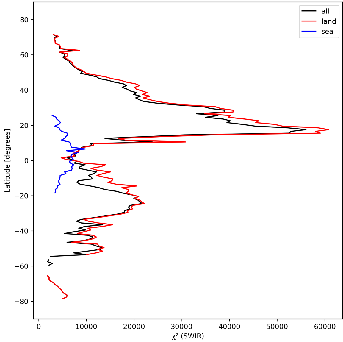
Figure 17: Zonal average of “ \chi^2 (SWIR)” for 2023-10-02 to 2023-10-04.
