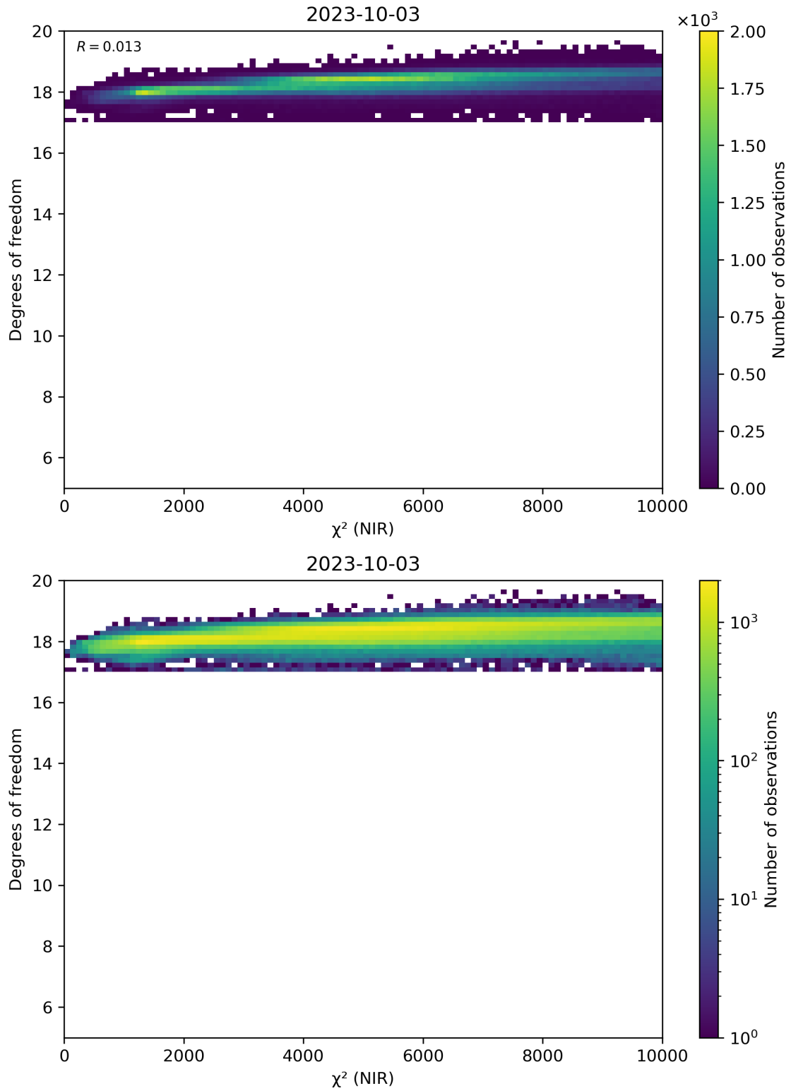
Figure 44: Scatter density plot of “ \chi^2 (NIR)” against “Degrees of freedom” for 2023-10-02 to 2023-10-04.
