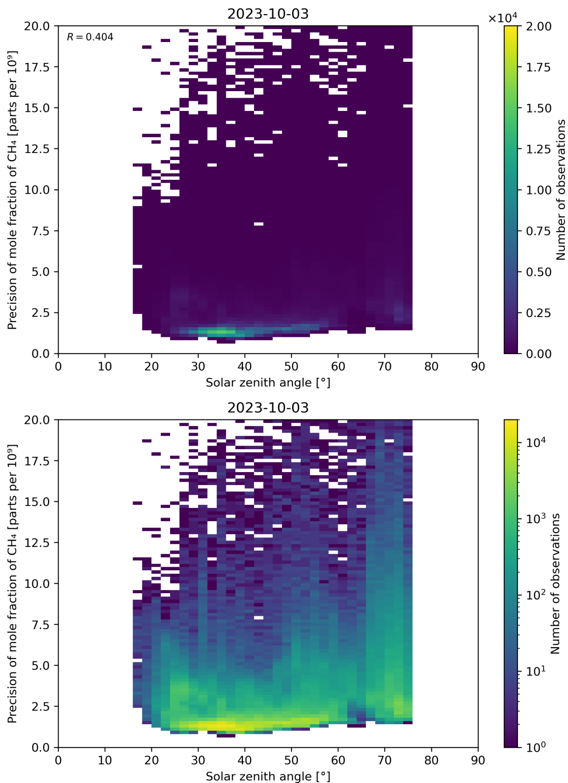
Figure 101: Scatter density plot of “Solar zenith angle” against “Precision of mole fraction of CH 4 ” for 2023-10-02 to 2023-10-04.
