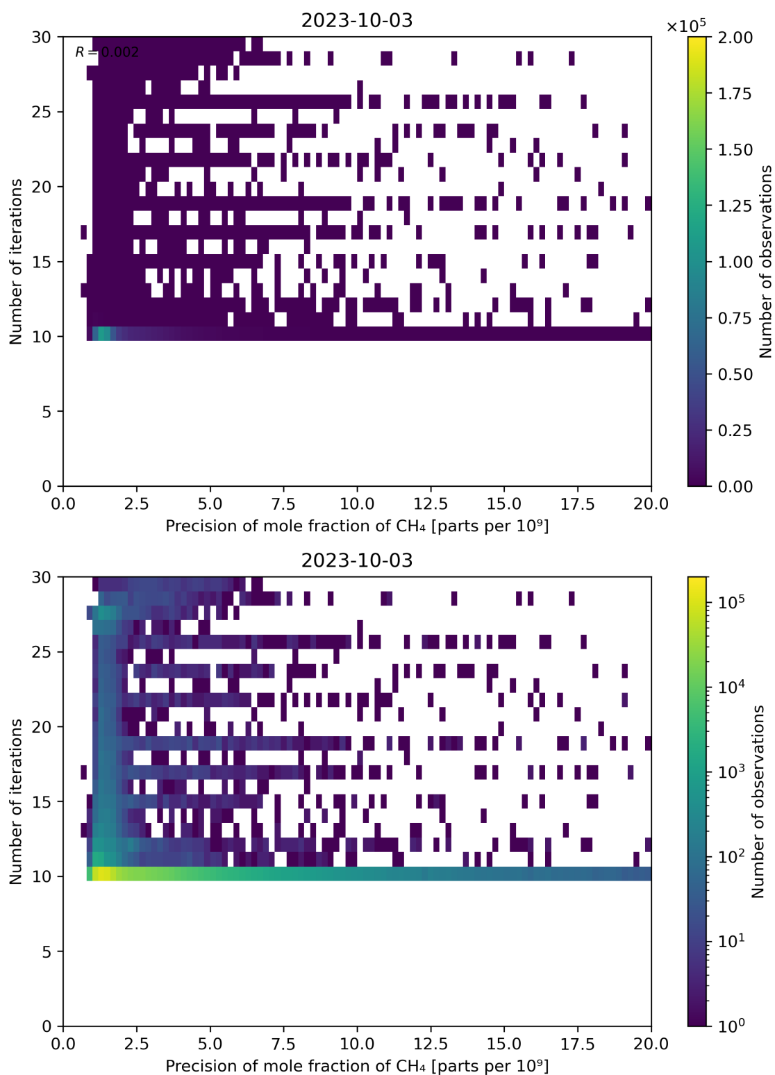
Figure 83: Scatter density plot of “Precision of mole fraction of CH 4 ” against “Number of iterations” for 2023-10-02 to 2023-10-04.
