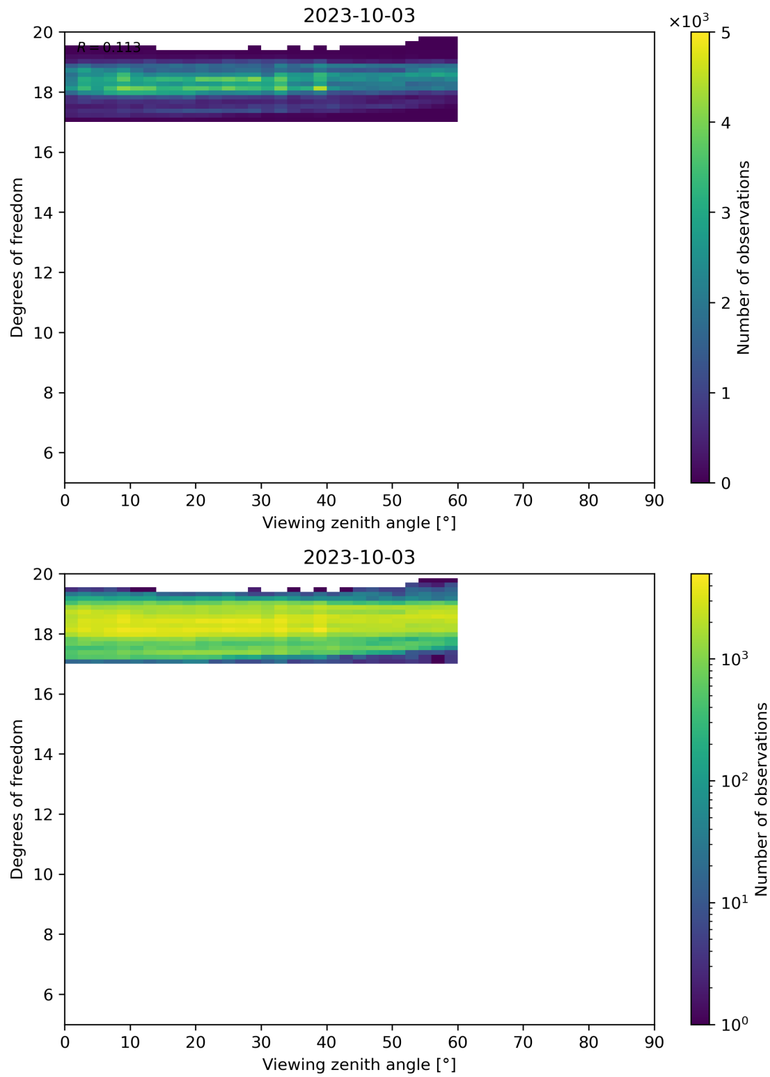
Figure 107: Scatter density plot of “Viewing zenith angle” against “Degrees of freedom” for 2023-10-02 to 2023-10-04.
