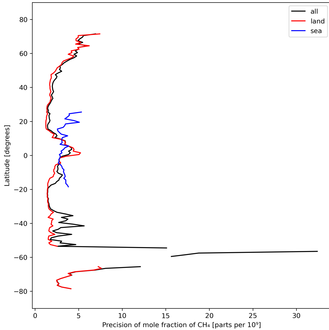
Figure 13: Zonal average of “Precision of mole fraction of CH 4 ” for 2023-10-02 to 2023-10-04.
