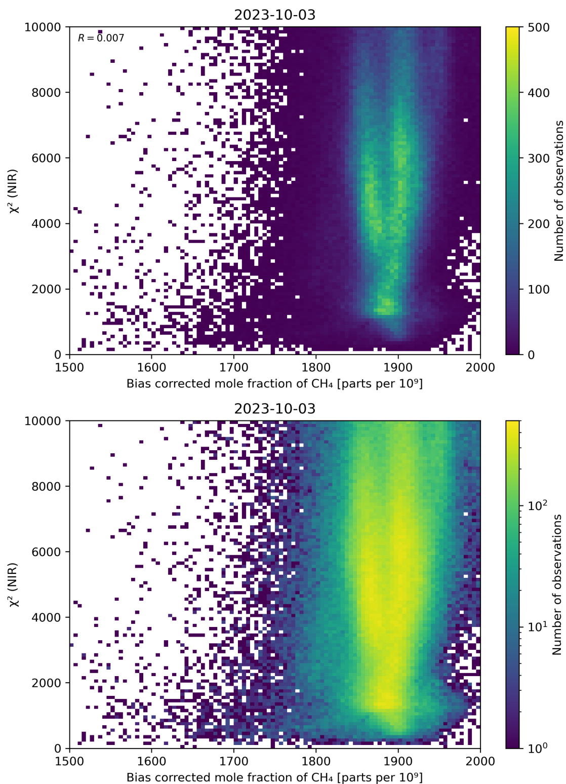
Figure 63: Scatter density plot of “Bias corrected mole fraction of CH 4 ” against “ \chi^2 (NIR)” for 2023-10-02 to 2023-10-04.
