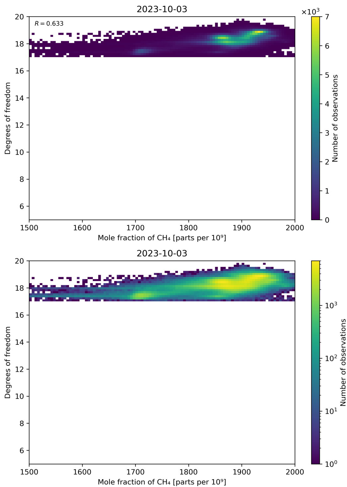
Figure 72: Scatter density plot of “Mole fraction of CH 4 ” against “Degrees of freedom” for 2023-10-02 to 2023-10-04.
