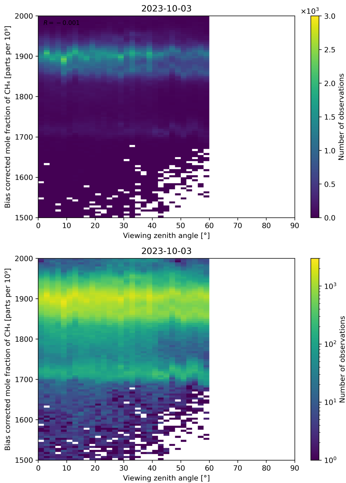
Figure 111: Scatter density plot of “Viewing zenith angle” against “Bias corrected mole fraction of CH 4 ” for 2023-10-02 to 2023-10-04.
