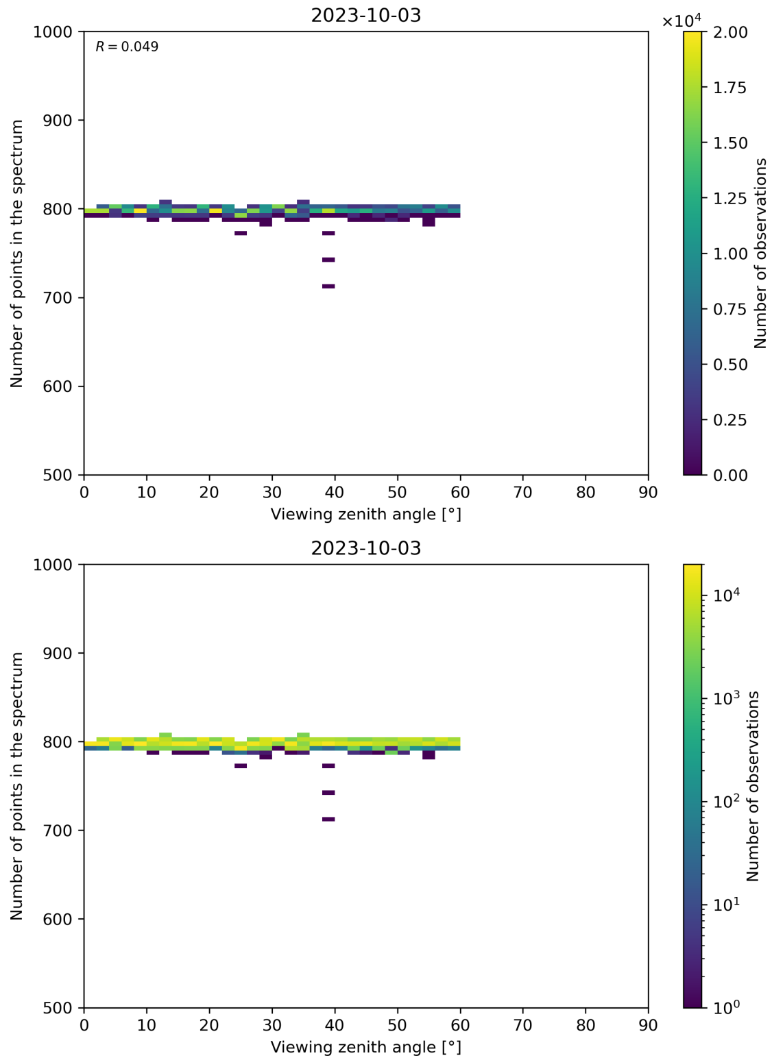
Figure 114: Scatter density plot of “Viewing zenith angle” against “Number of points in the spectrum” for 2023-10-02 to 2023-10-04.
