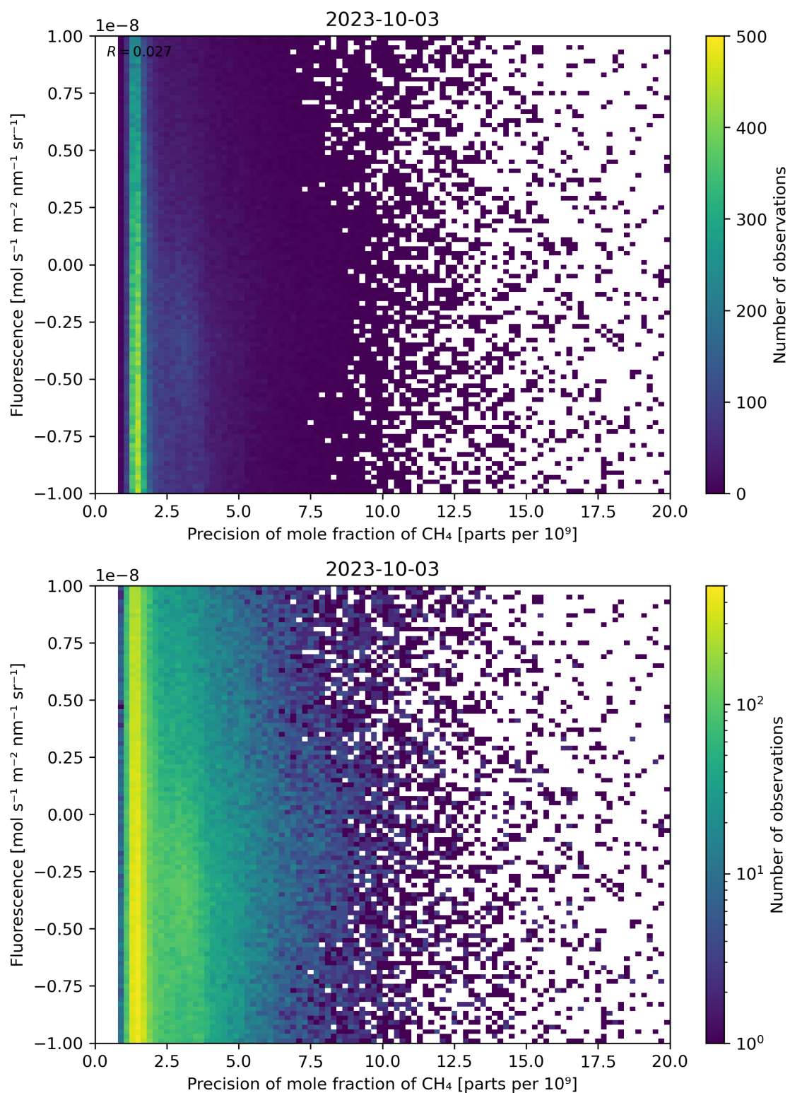
Figure 81: Scatter density plot of “Precision of mole fraction of \text{CH}_4 ” against “Fluorescence” for 2023-10-02 to 2023-10-04.
