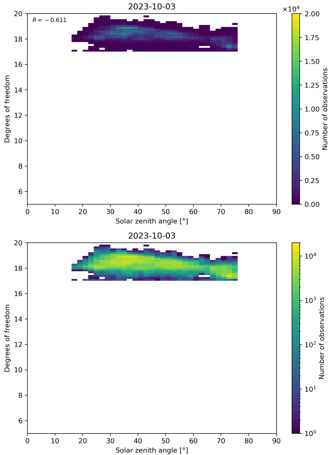
Figure 96: Scatter density plot of “Solar zenith angle” against “Degrees of freedom” for 2023-10-02 to 2023-10-04.
