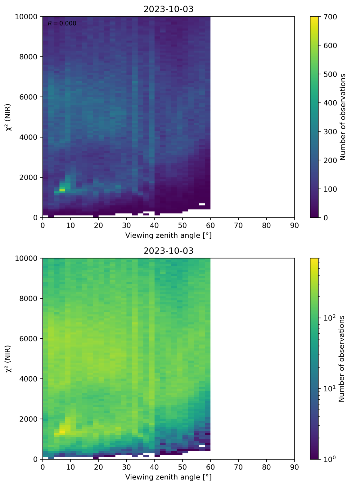
Figure 105: Scatter density plot of “Viewing zenith angle” against “ \chi^2 (NIR)” for 2023-10-02 to 2023-10-04.
