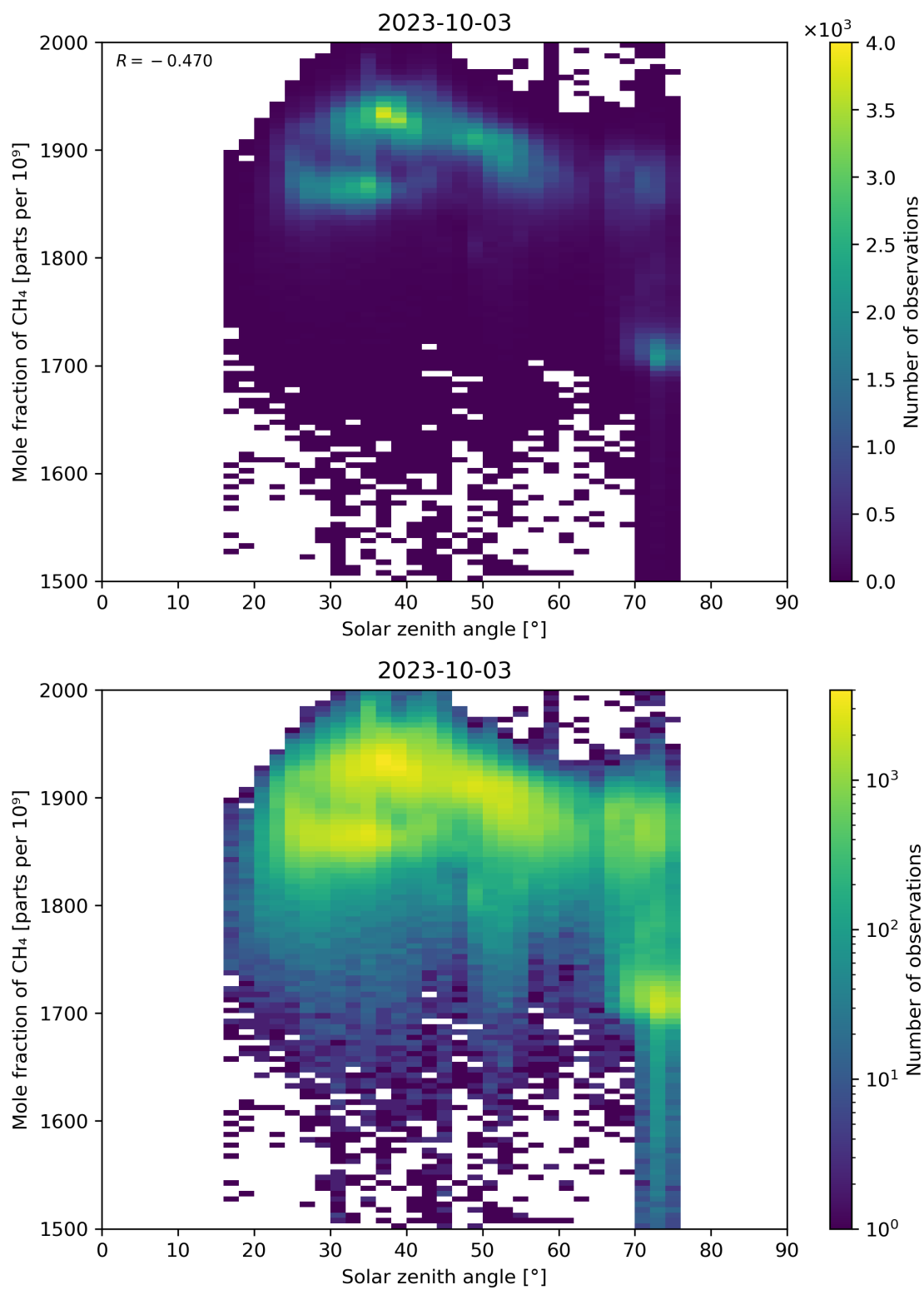
Figure 99: Scatter density plot of “Solar zenith angle” against “Mole fraction of \text{CH}_4 ” for 2023-10-02 to 2023-10-04.
