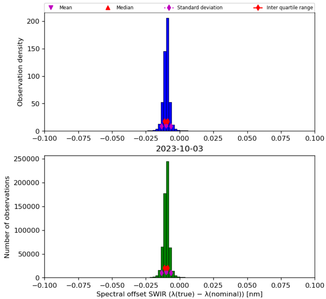
Figure 27: Histogram of “Spectral offset SWIR ( \lambda(\text{true}) - \lambda(\text{nominal}) )” for 2023-10-02 to 2023-10-04
