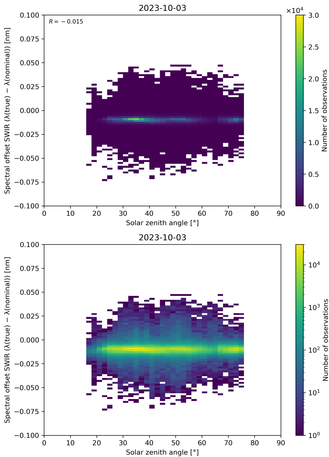
Figure 104: Scatter density plot of “Solar zenith angle” against “Spectral offset SWIR ( \lambda(\text{true}) - \lambda(\text{nominal}) )” for 2023-10-02 to 2023-10-04.
