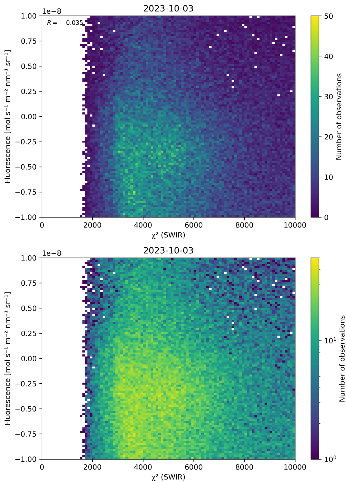
Figure 49: Scatter density plot of “ \chi^2 (SWIR)” against “Fluorescence” for 2023-10-02 to 2023-10-04.
