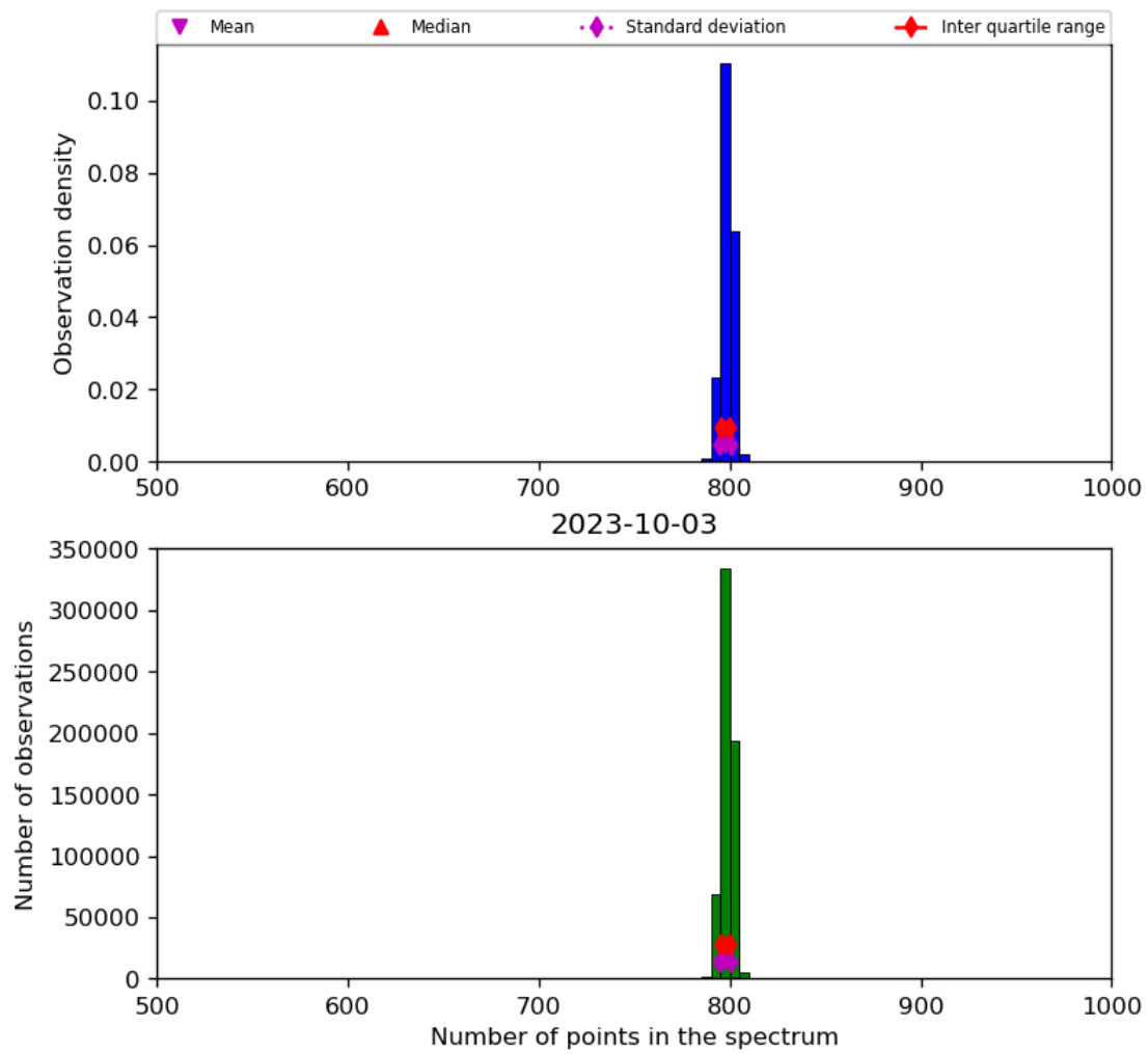
Figure 26: Histogram of “Number of points in the spectrum” for 2023-10-02 to 2023-10-04
