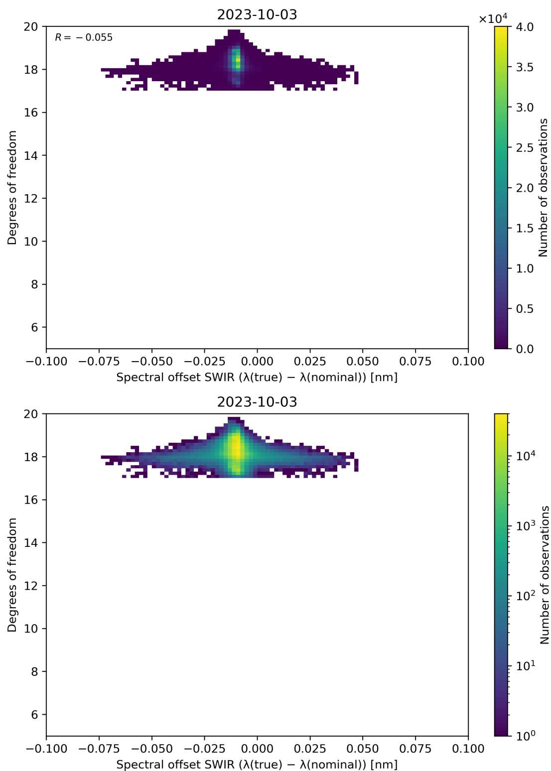
Figure 119: Scatter density plot of “Spectral offset SWIR ( \lambda(\text{true}) - \lambda(\text{nominal}) )” against “Degrees of freedom” for 2023-10-02 to 2023-10-04.
