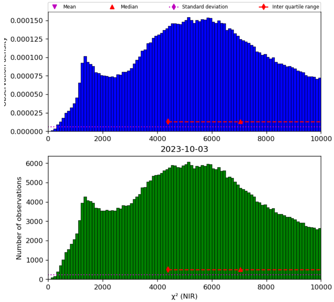
Figure 29: Histogram of “ \chi^2 (NIR)” for 2023-10-02 to 2023-10-04
