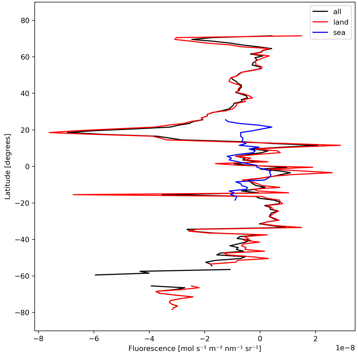
Figure 21: Zonal average of “Fluorescence” for 2023-10-02 to 2023-10-04.
