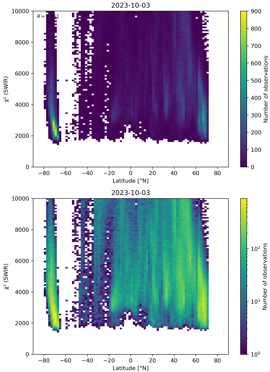
Figure 54: Scatter density plot of “Latitude” against “ \chi^2 (SWIR)” for 2023-10-02 to 2023-10-04.
