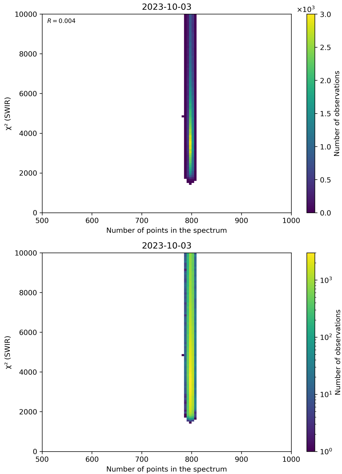
Figure 89: Scatter density plot of “Number of points in the spectrum” against “ \chi^2 (SWIR)” for 2023-10-02 to 2023-10-04.
