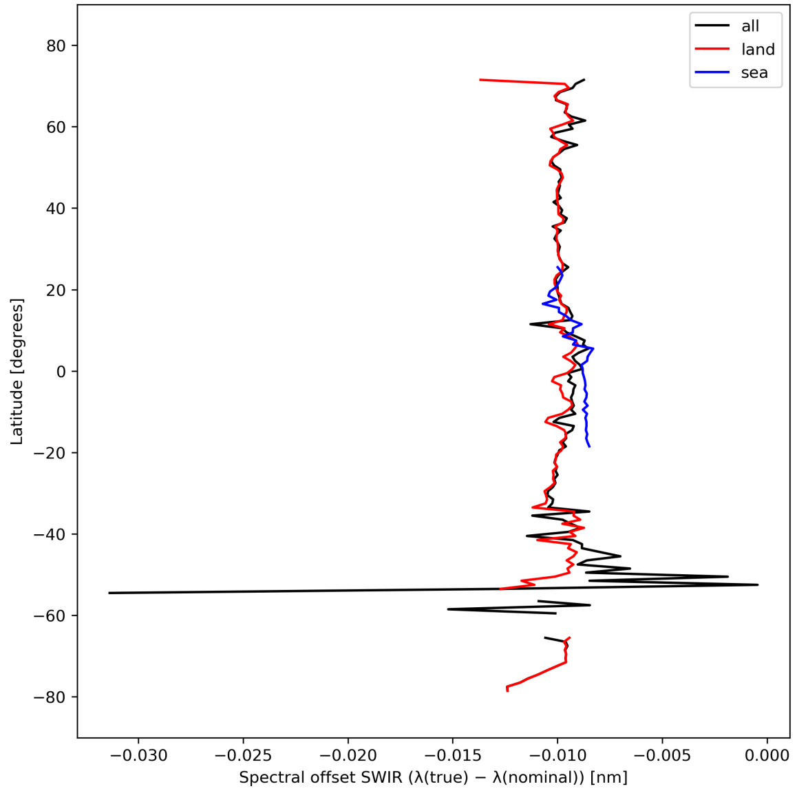
Figure 16: Zonal average of “Spectral offset SWIR ( \lambda(\text{true}) - \lambda(\text{nominal}) )” for 2023-10-02 to 2023-10-04.
