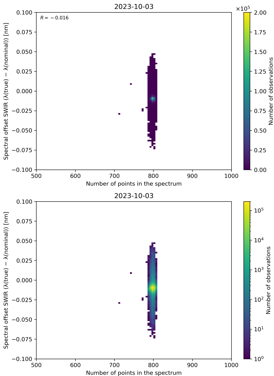
Figure 93: Scatter density plot of “Number of points in the spectrum” against “Spectral offset SWIR ( \lambda(\text{true}) - \lambda(\text{nominal}) )” for 2023-10-02 to 2023-10-04.
