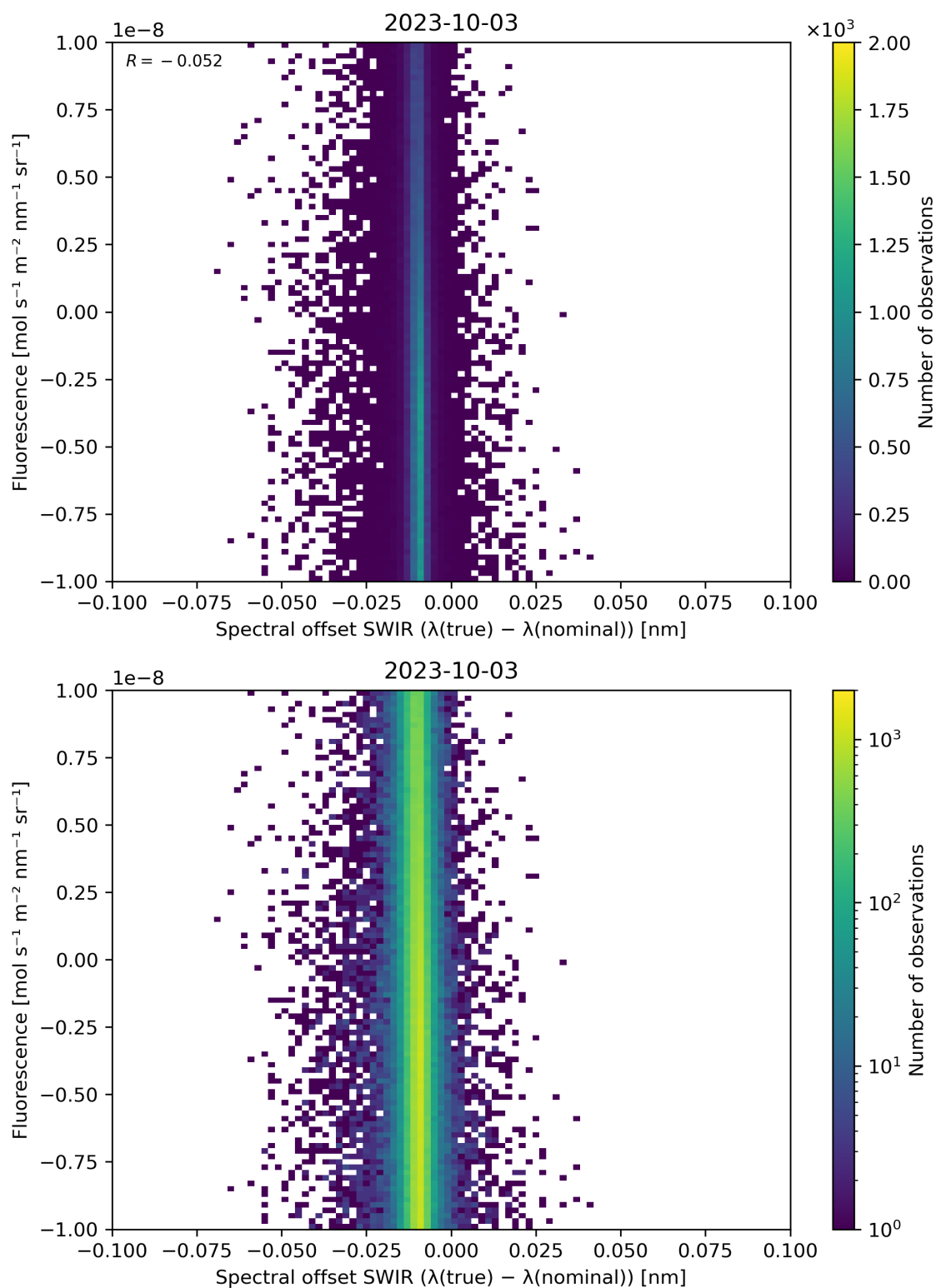
Figure 120: Scatter density plot of “Spectral offset SWIR ( \lambda(\text{true}) - \lambda(\text{nominal}) )” against “Fluorescence” for 2023-10-02 to 2023-10-04.
