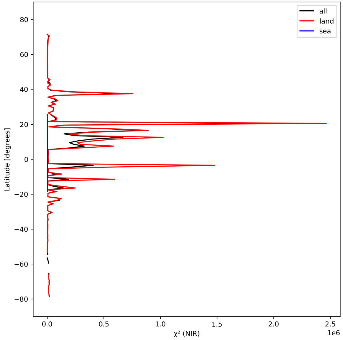
Figure 18: Zonal average of “ \chi^2 (NIR)” for 2023-10-02 to 2023-10-04.
