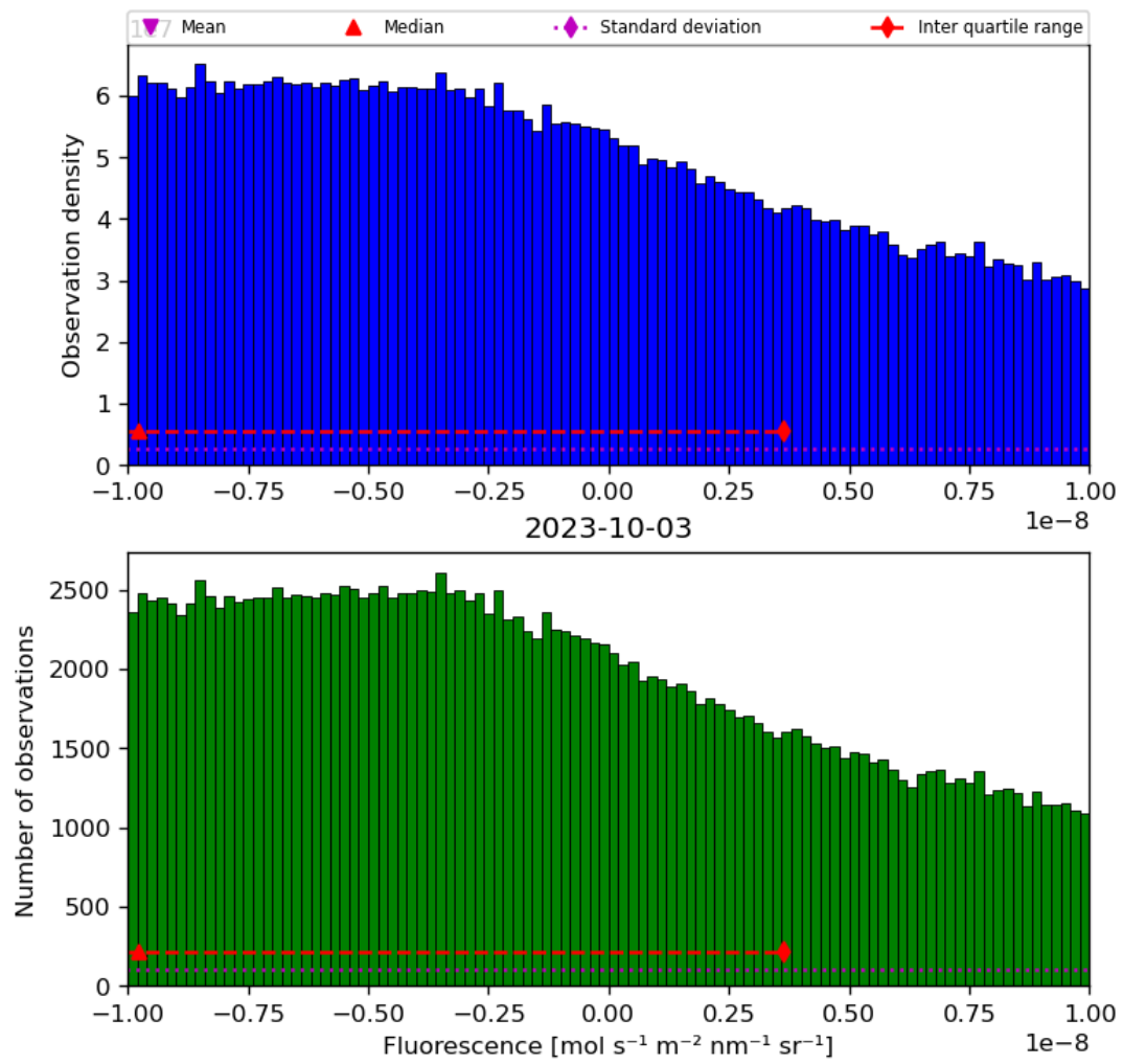
Figure 32: Histogram of “Fluorescence” for 2023-10-02 to 2023-10-04
