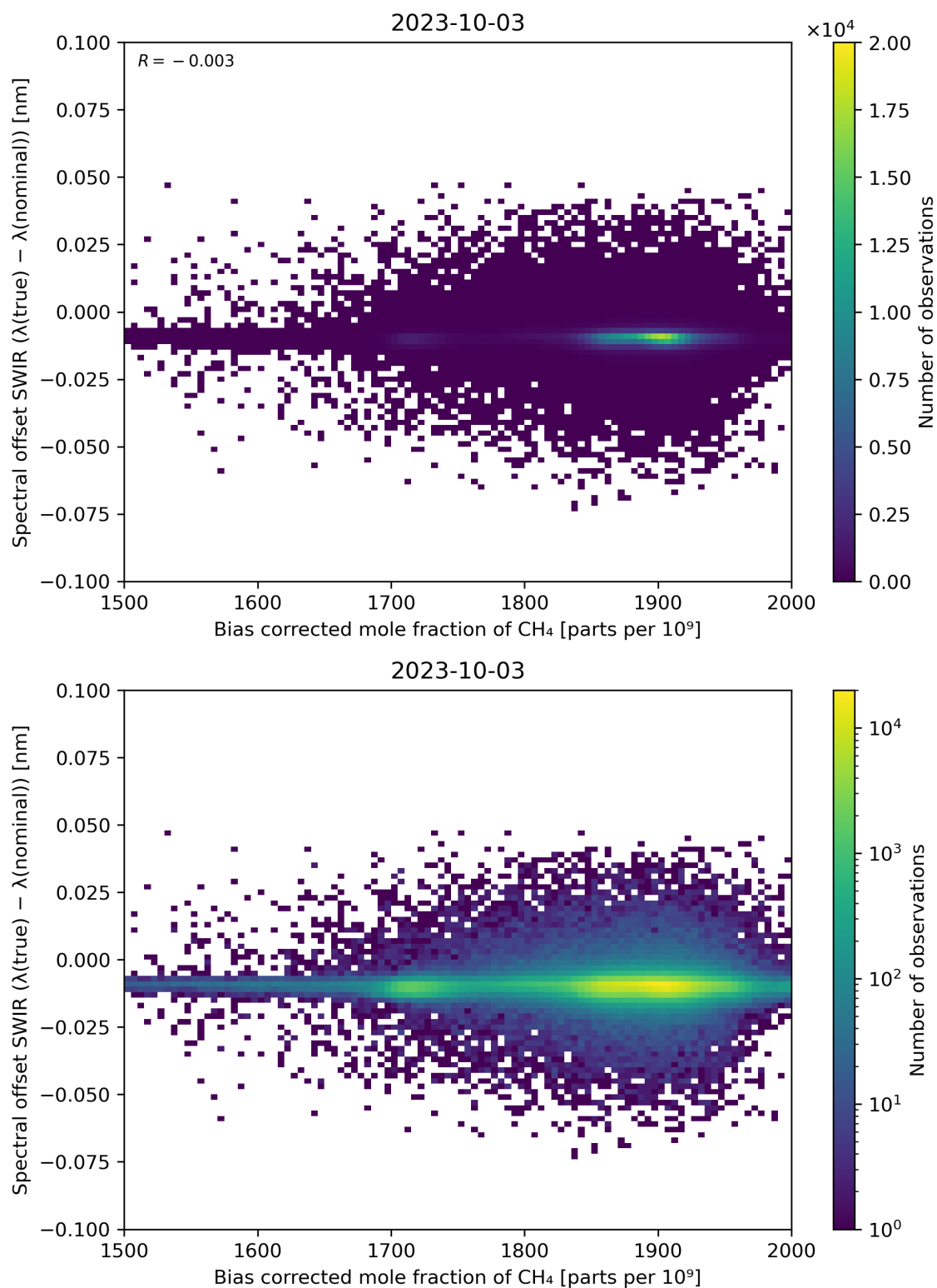
Figure 69: Scatter density plot of “Bias corrected mole fraction of \text{CH}_4 ” against “Spectral offset SWIR ( \lambda(\text{true}) - \lambda(\text{nominal}) )” for 2023-10-02 to 2023-10-04.
