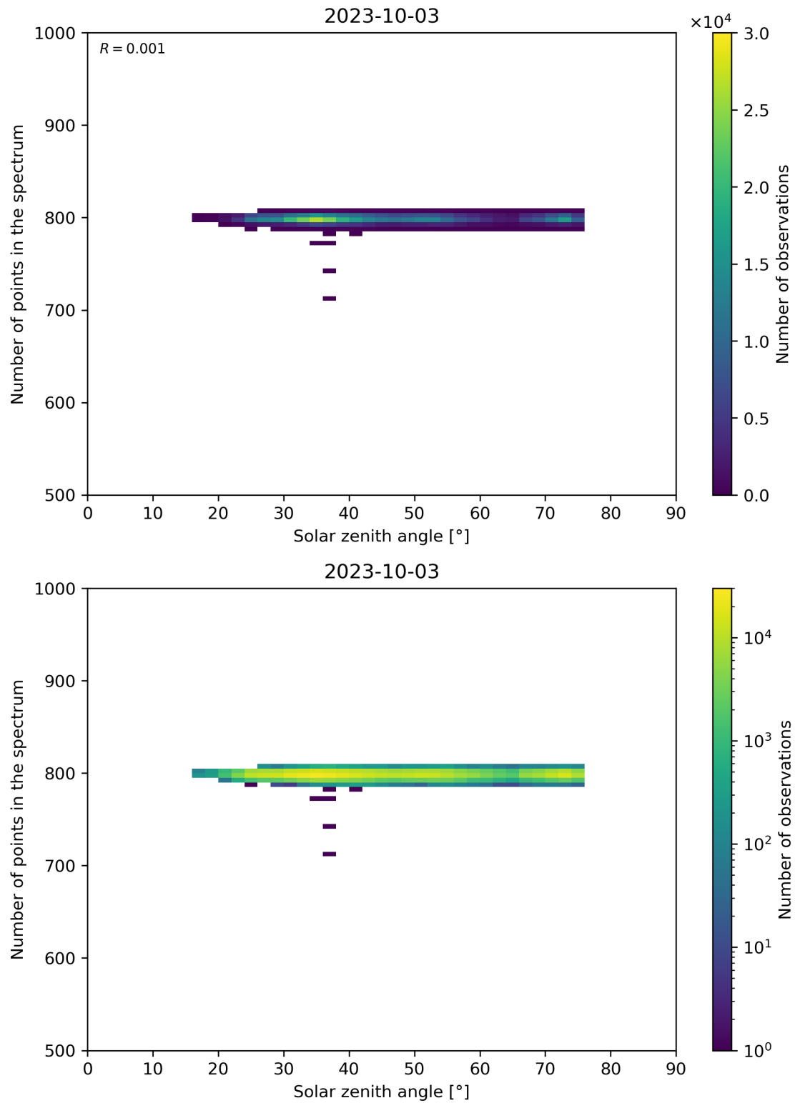
Figure 103: Scatter density plot of “Solar zenith angle” against “Number of points in the spectrum” for 2023-10-02 to 2023-10-04.
