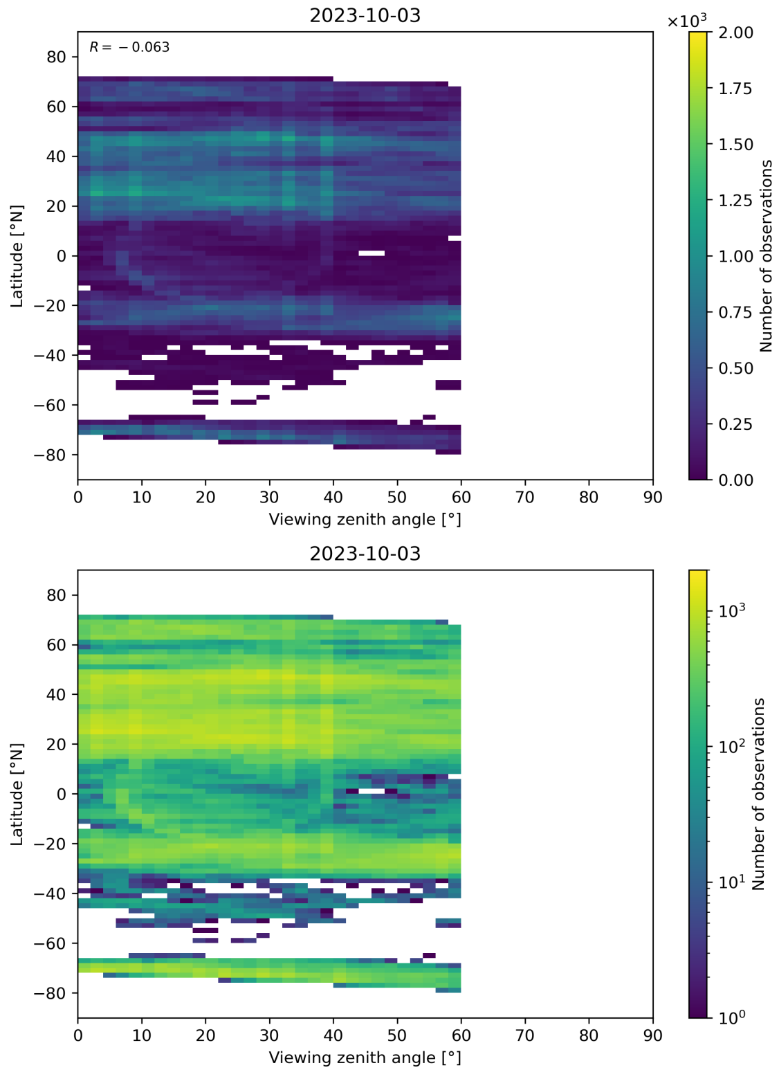
Figure 109: Scatter density plot of “Viewing zenith angle” against “Latitude” for 2023-10-02 to 2023-10-04.
