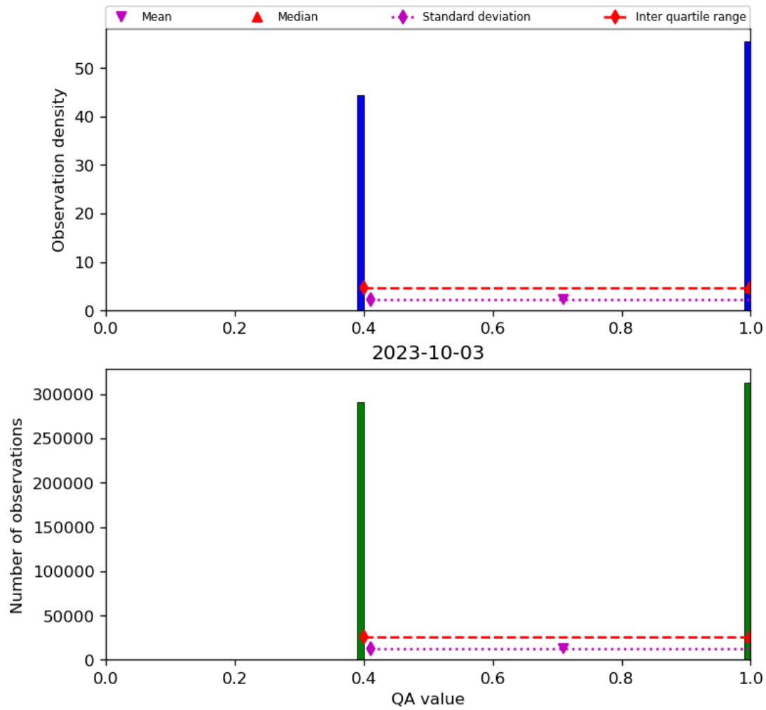
Figure 22: Histogram of “QA value” for 2023-10-02 to 2023-10-04
