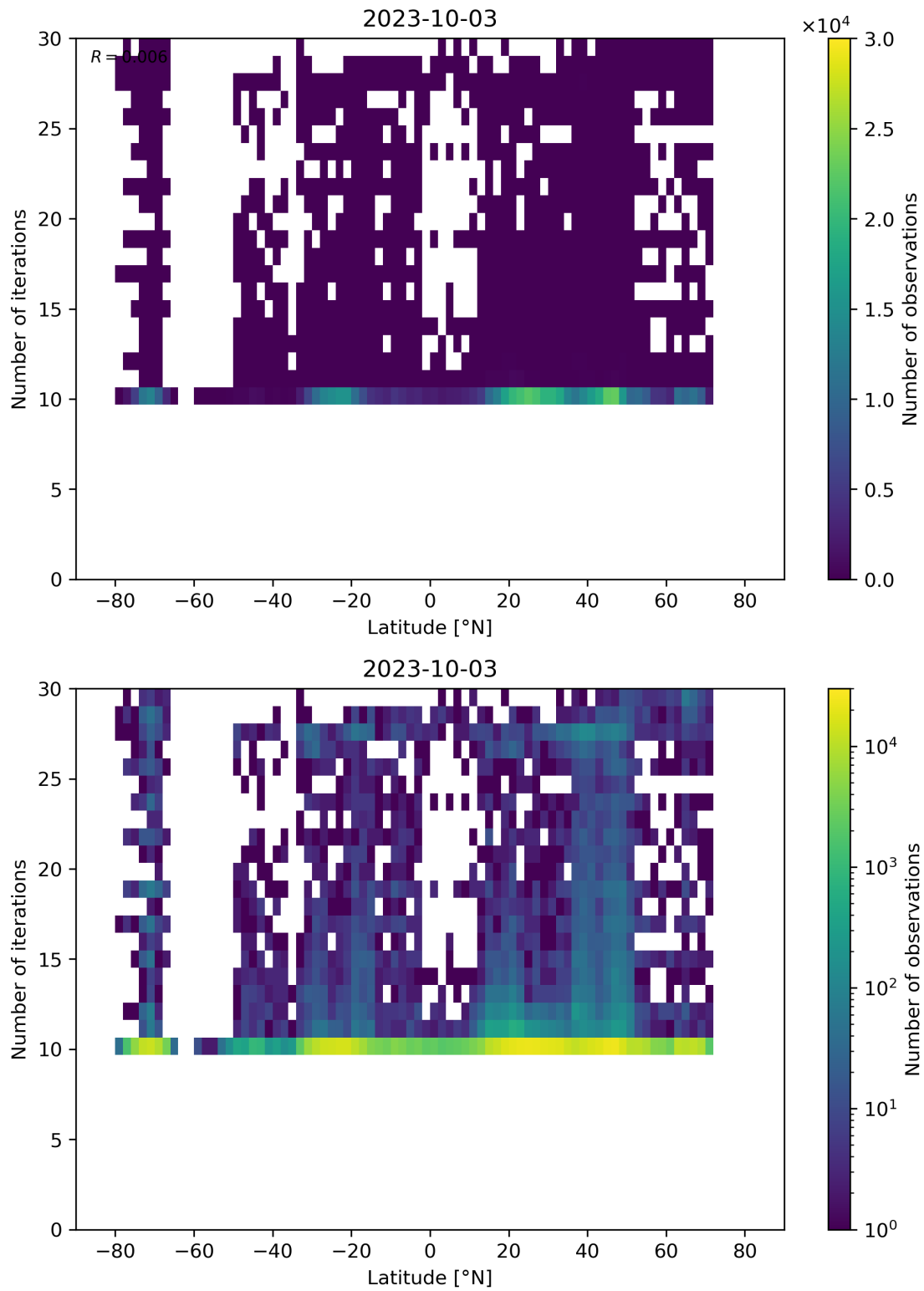
Figure 60: Scatter density plot of “Latitude” against “Number of iterations” for 2023-10-02 to 2023-10-04.
