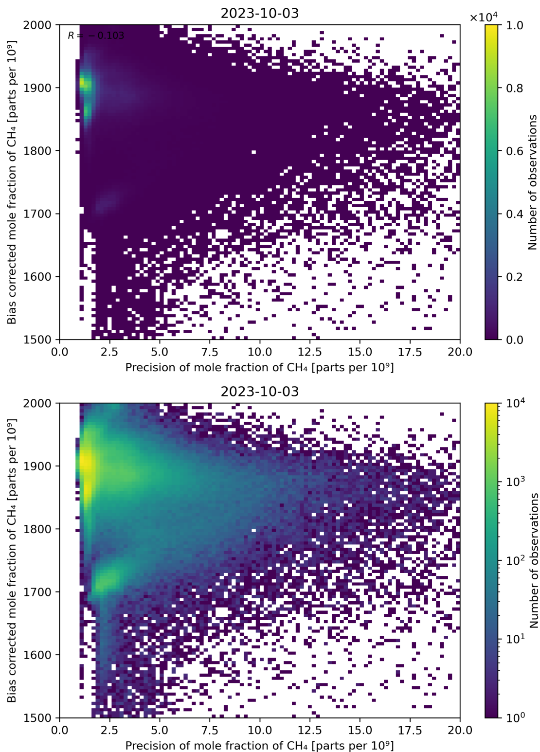
Figure 82: Scatter density plot of “Precision of mole fraction of \text{CH}_4 ” against “Bias corrected mole fraction of \text{CH}_4 ” for 2023-10-02 to 2023-10-04.
