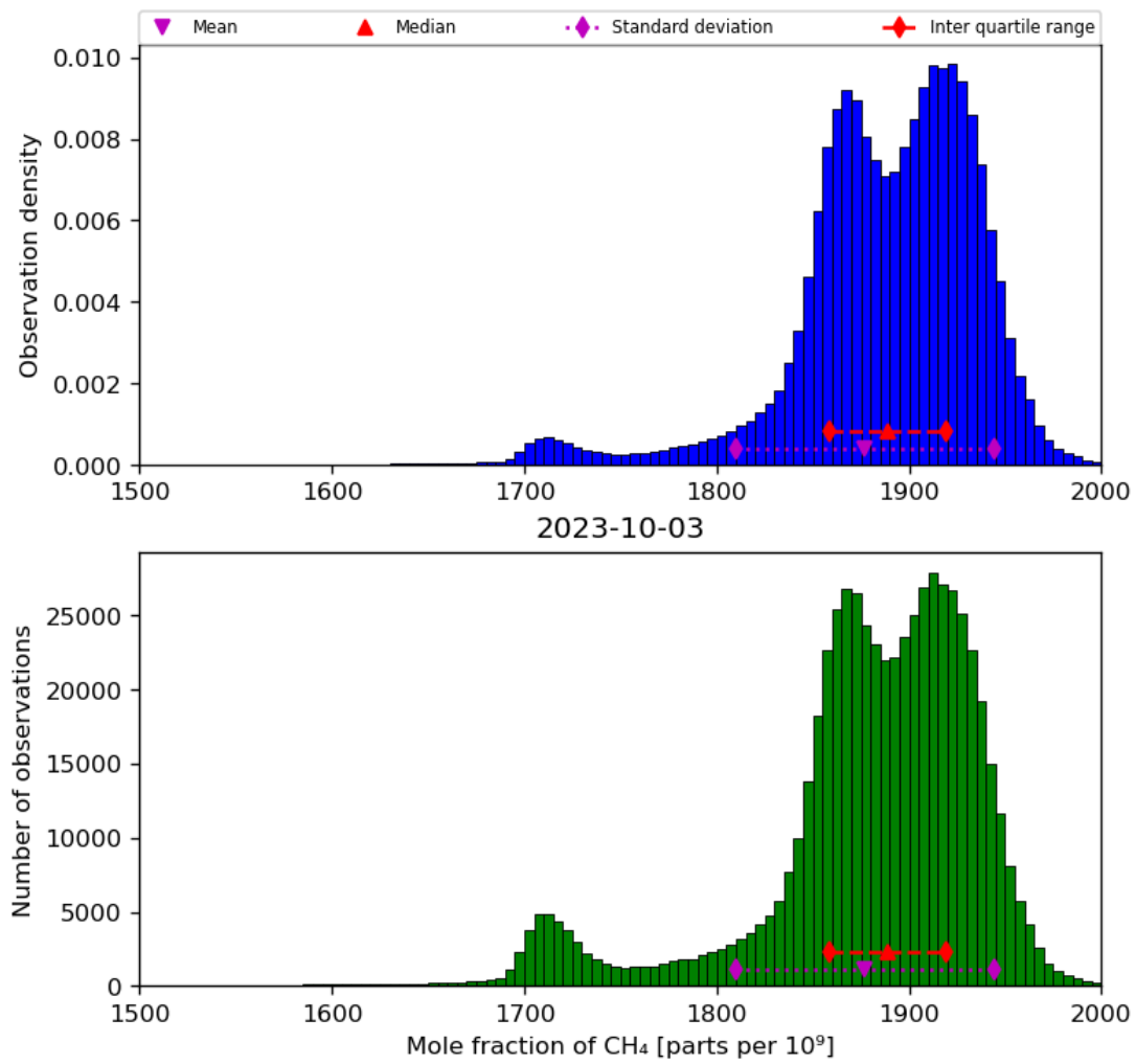
Figure 23: Histogram of “Mole fraction of CH 4 ” for 2023-10-02 to 2023-10-04
