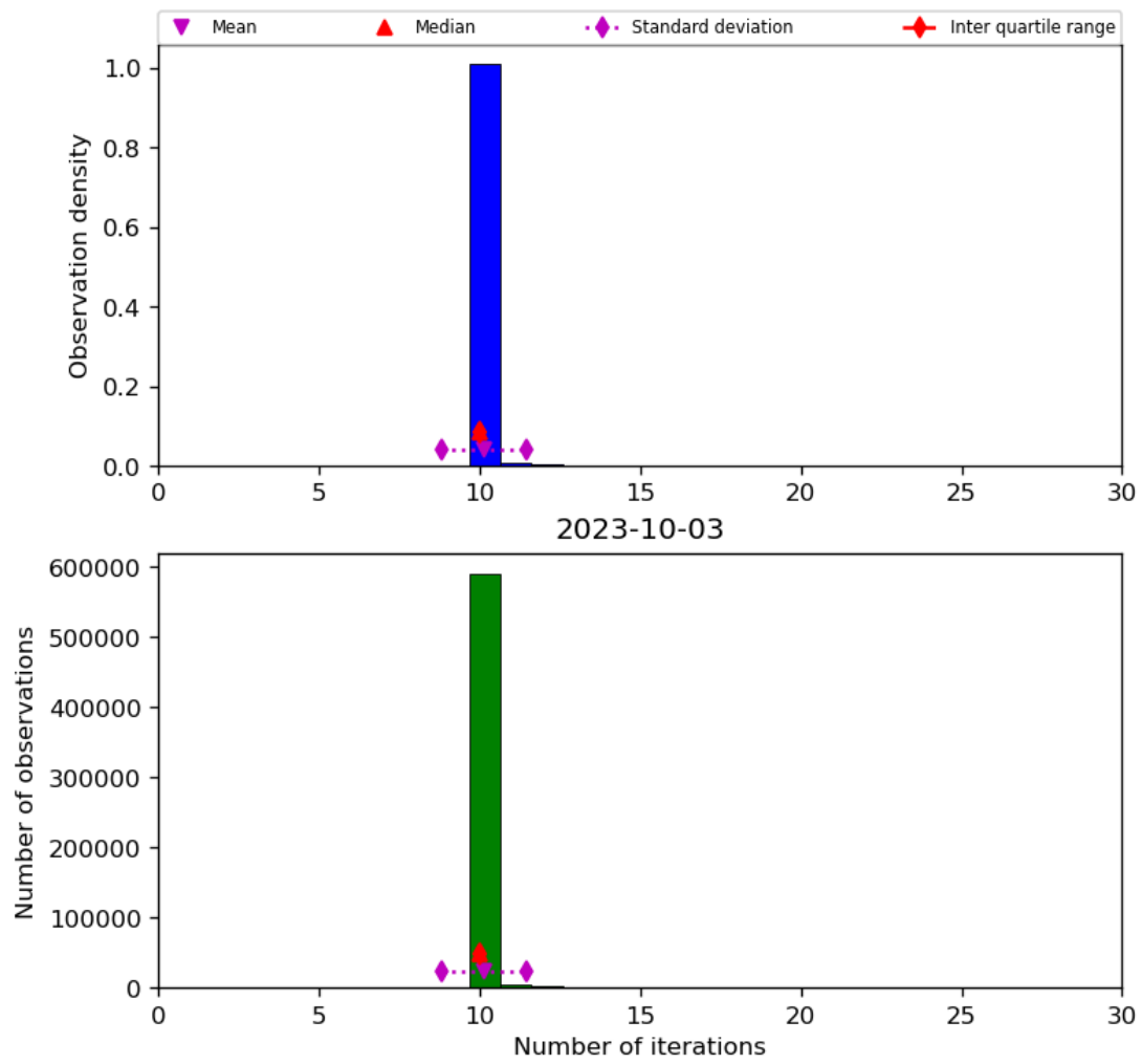
Figure 31: Histogram of “Number of iterations” for 2023-10-02 to 2023-10-04
