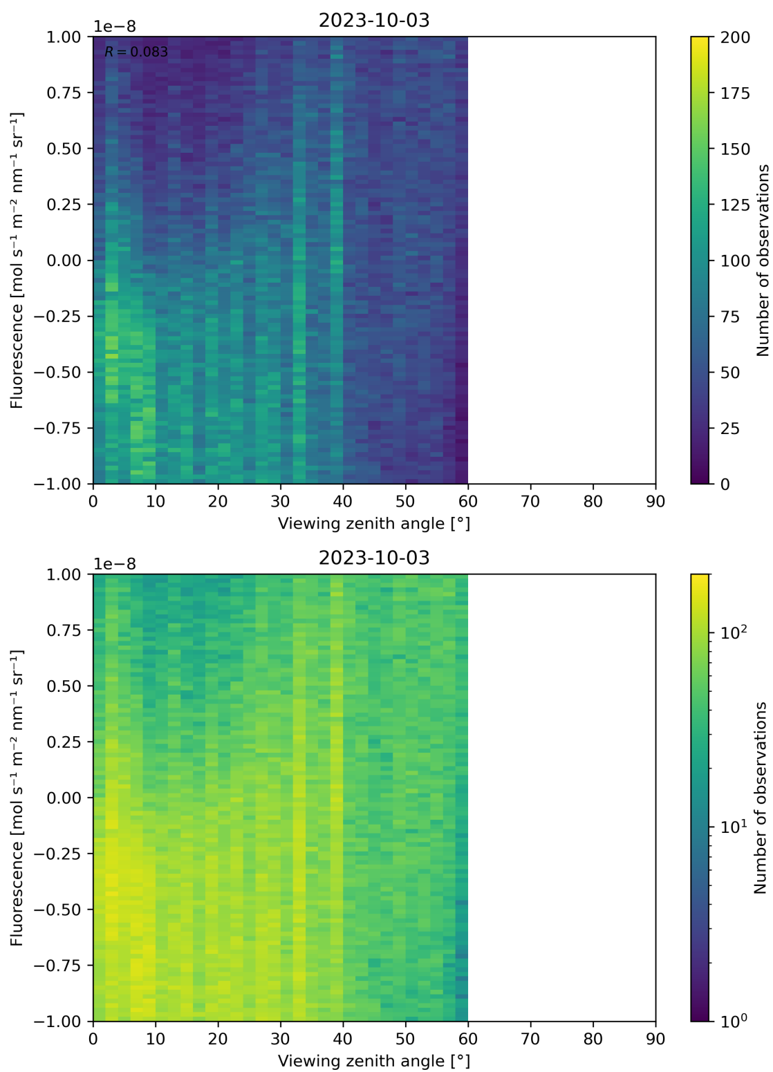
Figure 108: Scatter density plot of “Viewing zenith angle” against “Fluorescence” for 2023-10-02 to 2023-10-04.
