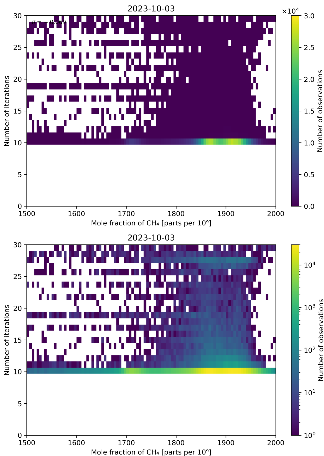
Figure 76: Scatter density plot of “Mole fraction of CH 4 ” against “Number of iterations” for 2023-10-02 to 2023-10-04.
