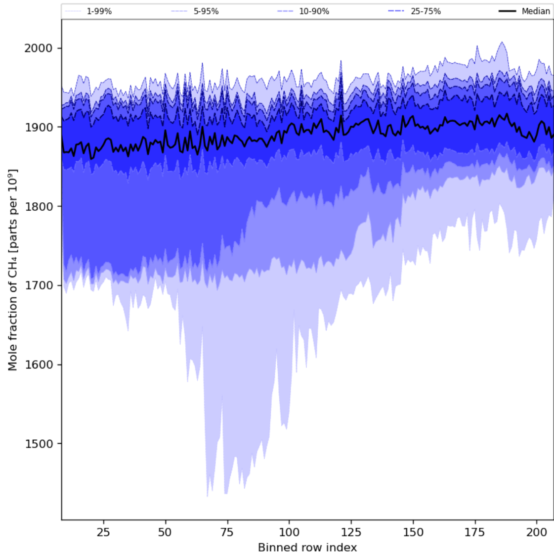
Figure 34: Along track statistics of “Mole fraction of CH 4 ” for 2023-10-02 to 2023-10-04
