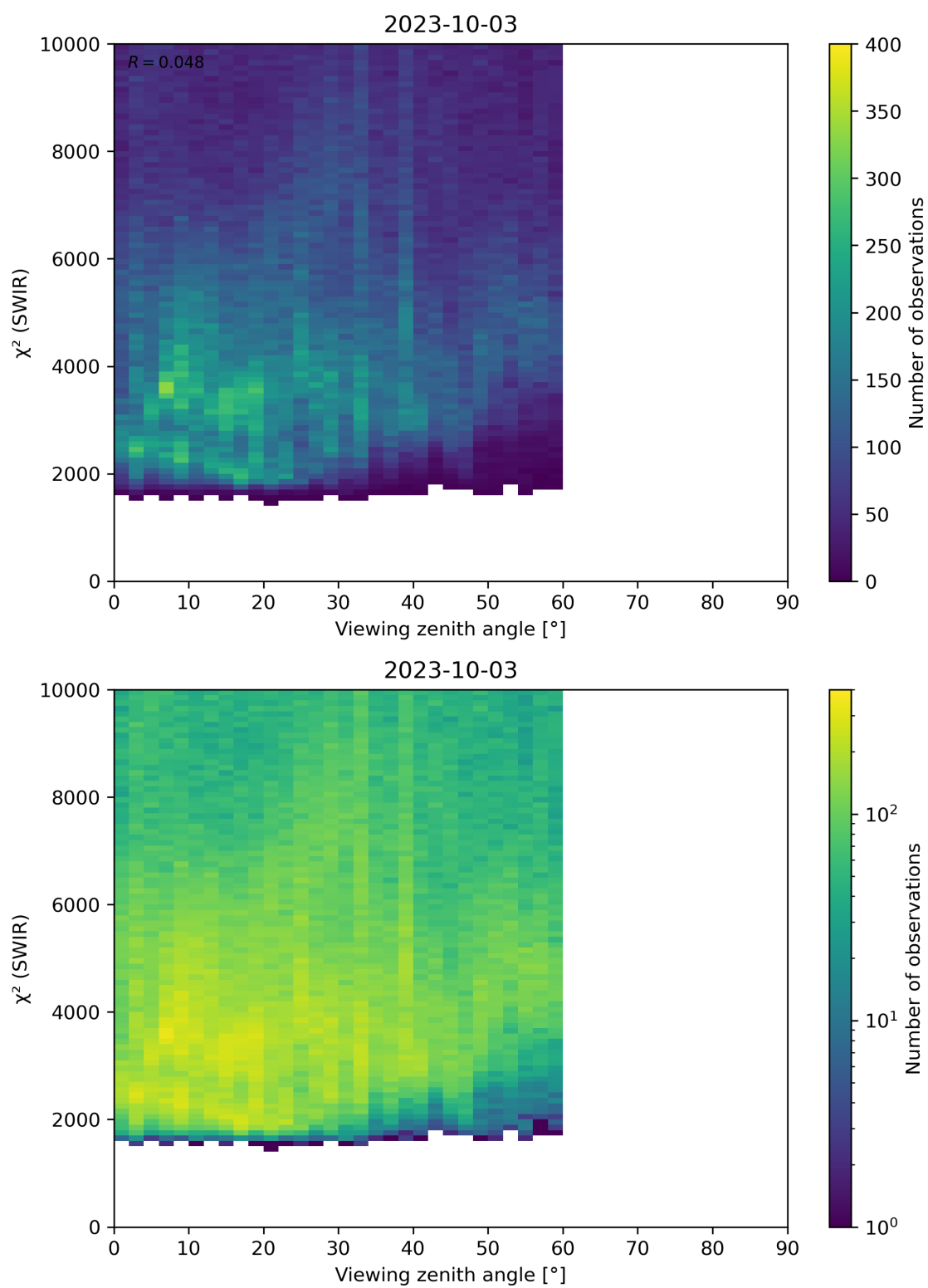
Figure 106: Scatter density plot of “Viewing zenith angle” against “ \chi^2 (SWIR)” for 2023-10-02 to 2023-10-04.
