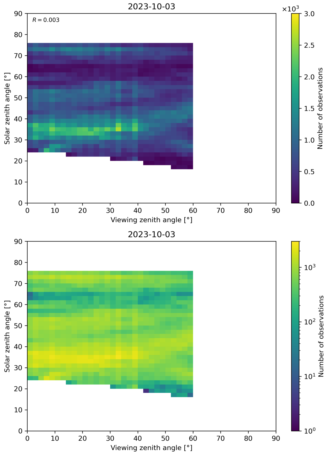
Figure 115: Scatter density plot of “Viewing zenith angle” against “Solar zenith angle” for 2023-10-02 to 2023-10-04.
