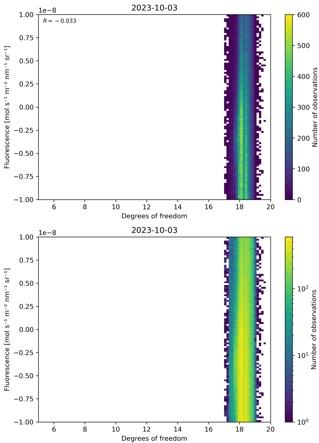
Figure 51: Scatter density plot of “Degrees of freedom” against “Fluorescence” for 2023-10-02 to 2023-10-04.
