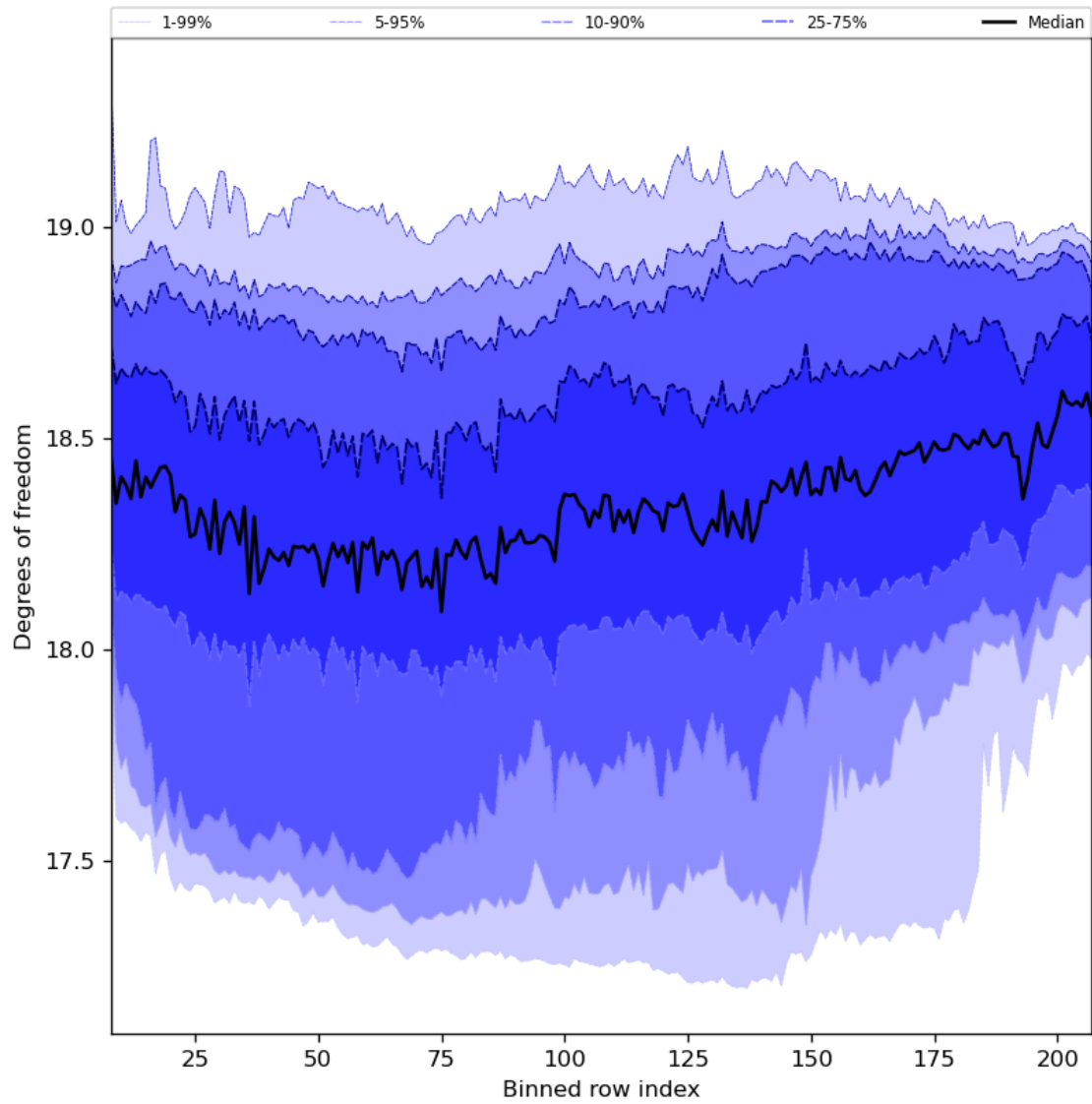
Figure 41: Along track statistics of “Degrees of freedom” for 2023-10-02 to 2023-10-04
