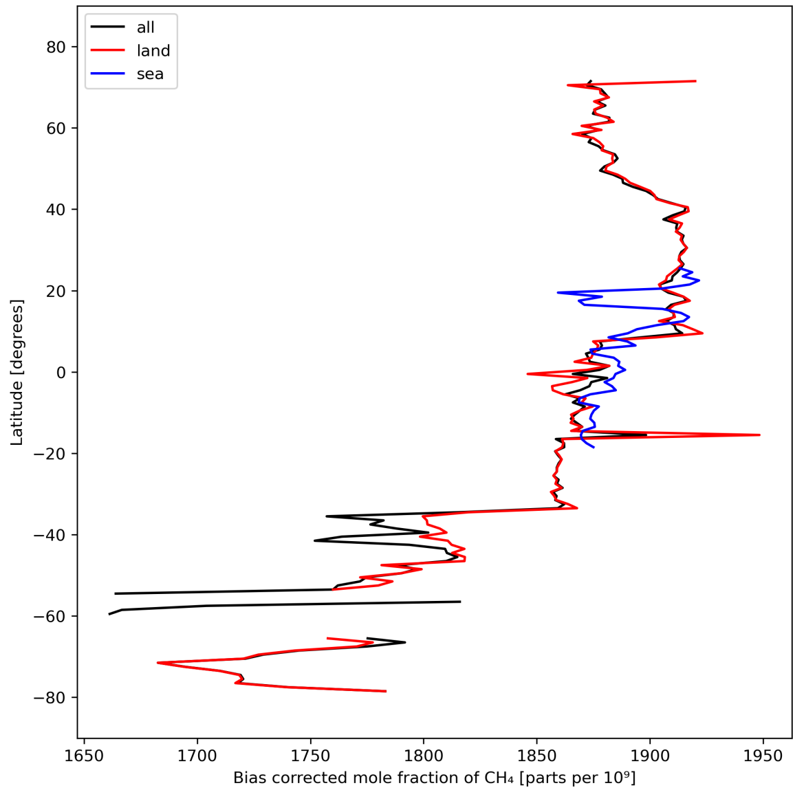
Figure 14: Zonal average of “Bias corrected mole fraction of CH 4 ” for 2023-10-02 to 2023-10-04.
