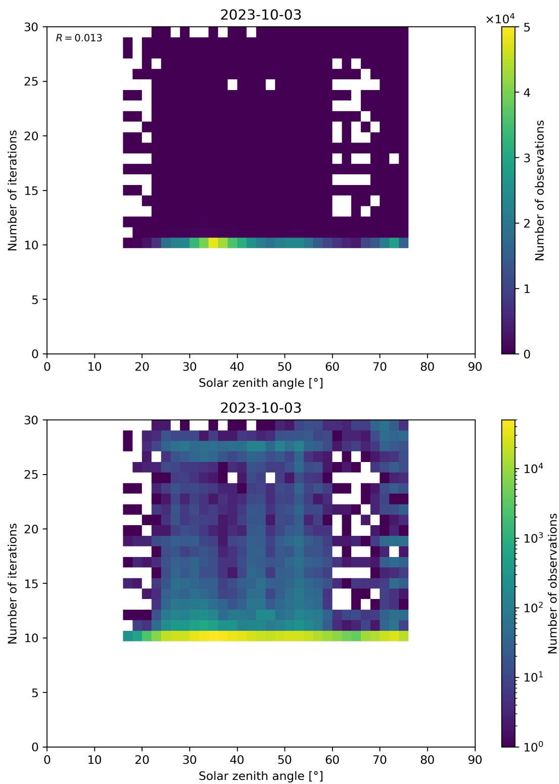
Figure 102: Scatter density plot of “Solar zenith angle” against “Number of iterations” for 2023-10-02 to 2023-10-04.
