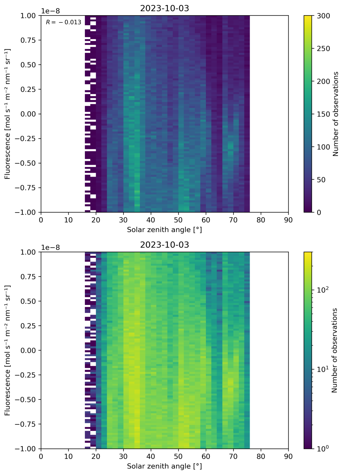
Figure 97: Scatter density plot of “Solar zenith angle” against “Fluorescence” for 2023-10-02 to 2023-10-04.
