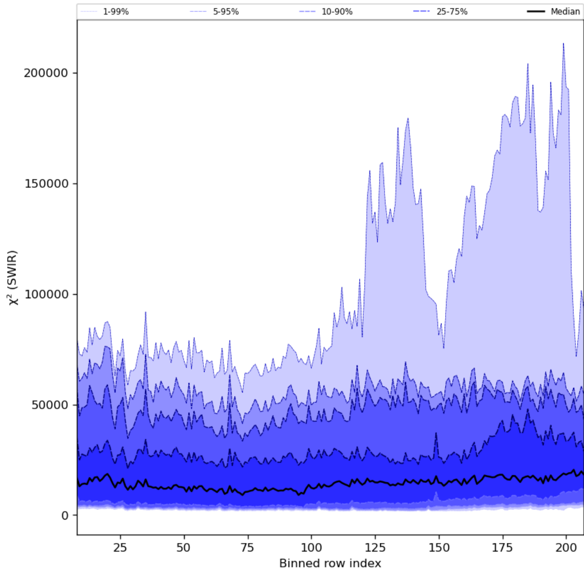
Figure 39: Along track statistics of “ \chi^2 (SWIR)” for 2023-10-02 to 2023-10-04
