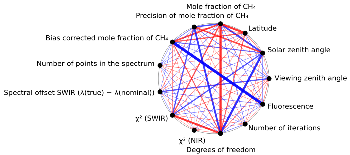
Figure 1: Map of correlation graph for 2023-10-02 to 2023-10-04.
