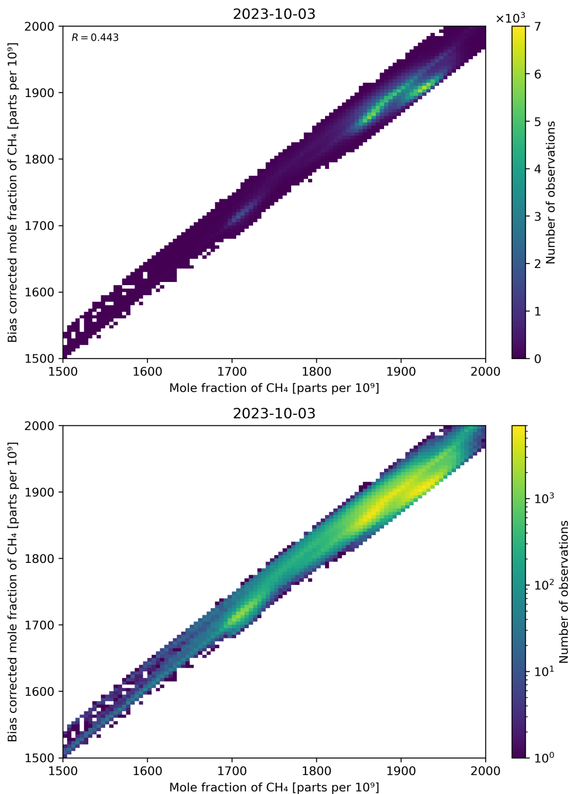
Figure 74: Scatter density plot of “Mole fraction of CH 4 ” against “Bias corrected mole fraction of CH 4 ” for 2023-10-02 to 2023-10-04.
