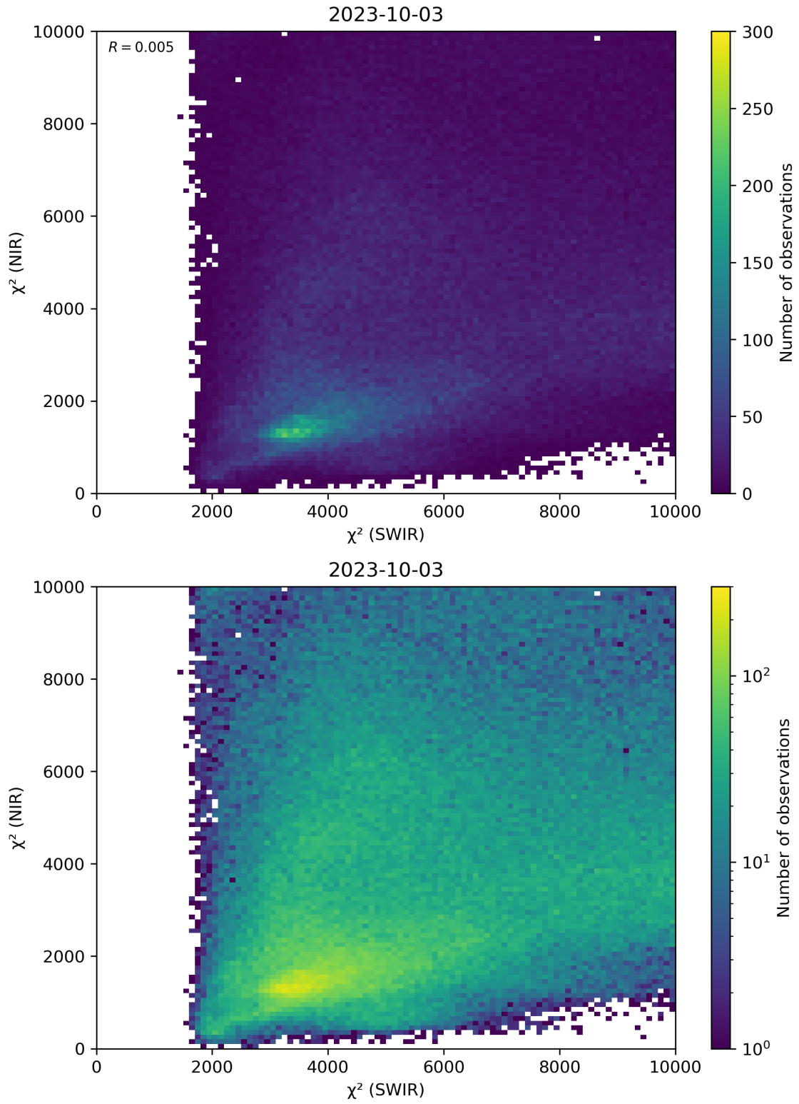
Figure 47: Scatter density plot of “ \chi^2 (SWIR)” against “ \chi^2 (NIR)” for 2023-10-02 to 2023-10-04.
