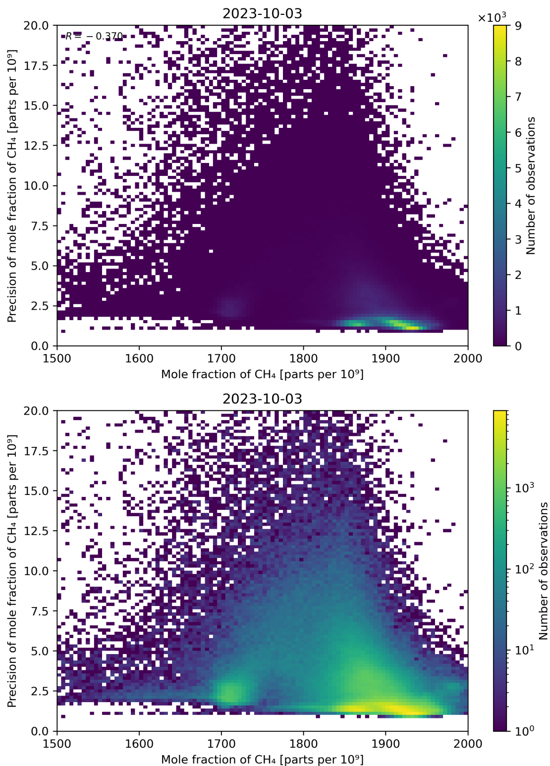
Figure 75: Scatter density plot of “Mole fraction of CH 4 ” against “Precision of mole fraction of CH 4 ” for 2023-10-02 to 2023-10-04.
