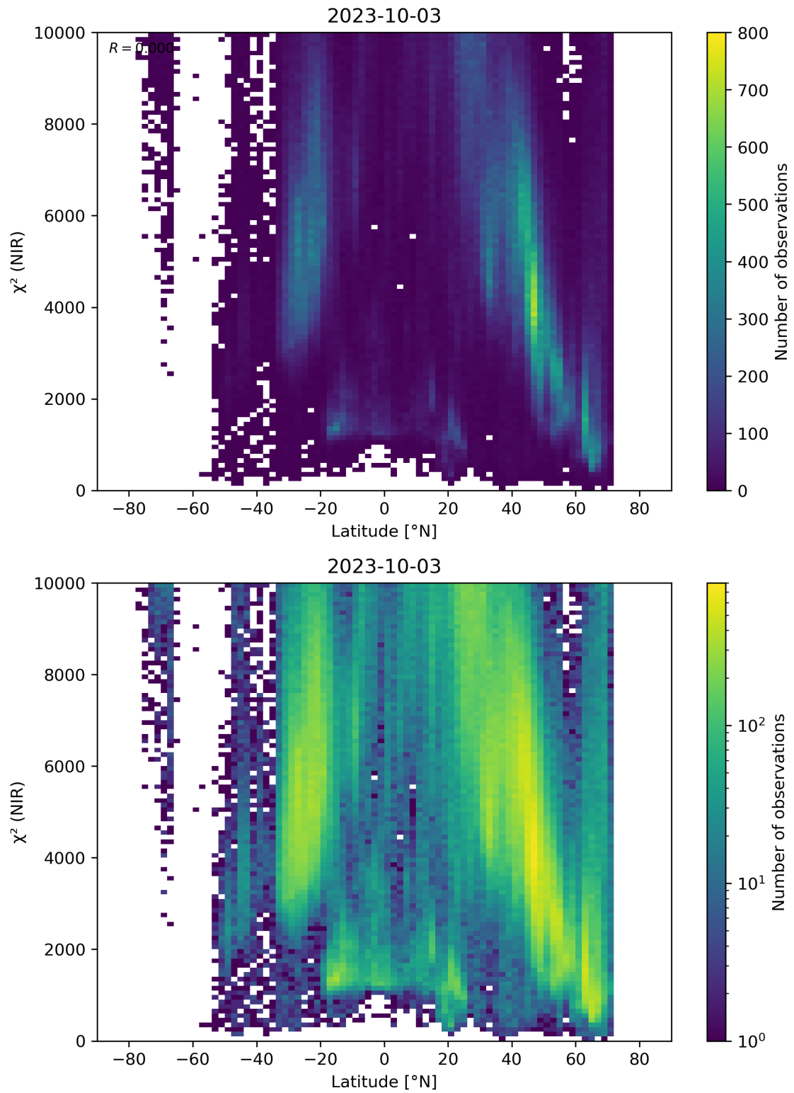
Figure 53: Scatter density plot of “Latitude” against “ \chi^2 (NIR)” for 2023-10-02 to 2023-10-04.
