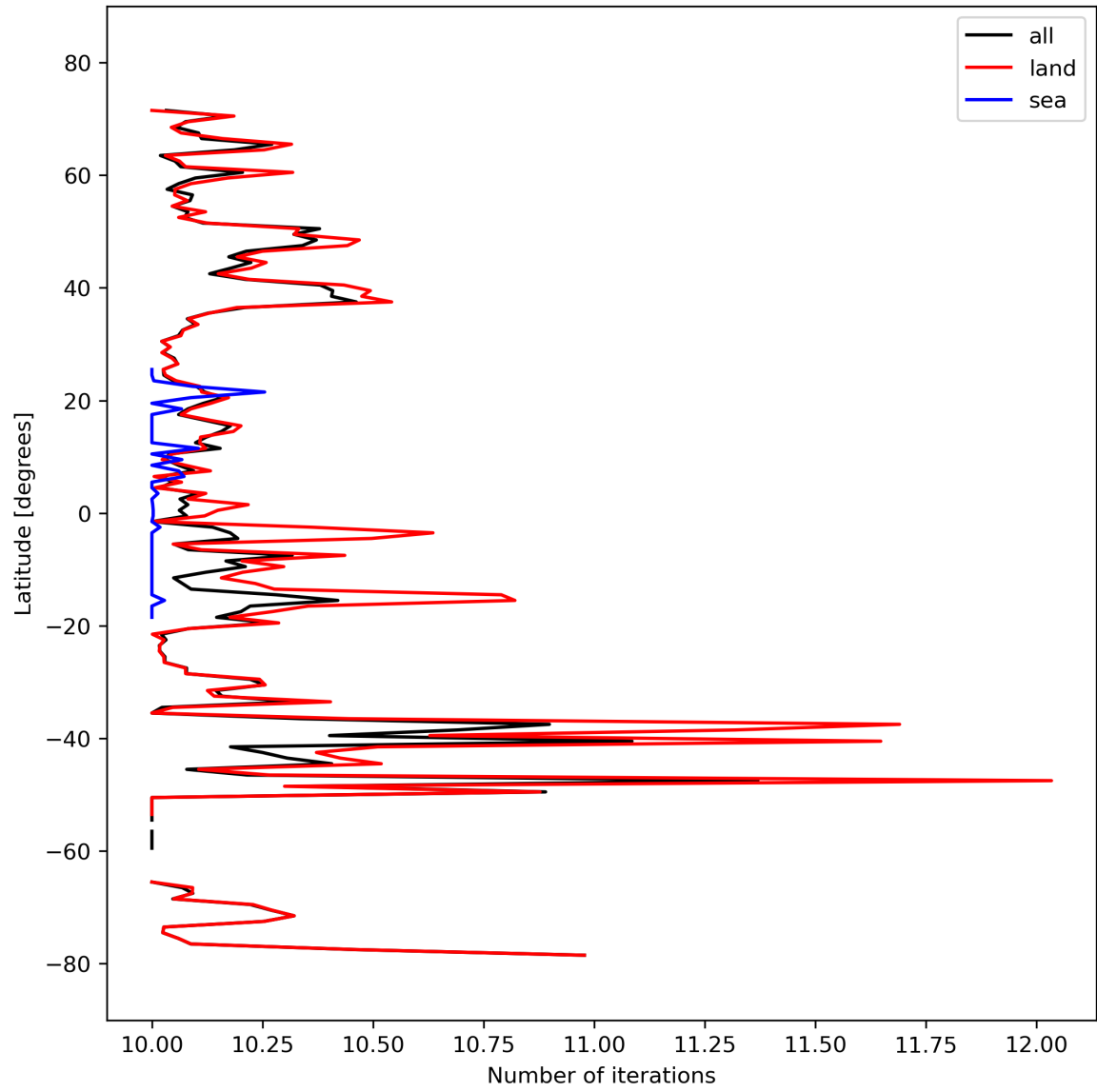
Figure 20: Zonal average of “Number of iterations” for 2023-10-02 to 2023-10-04.
