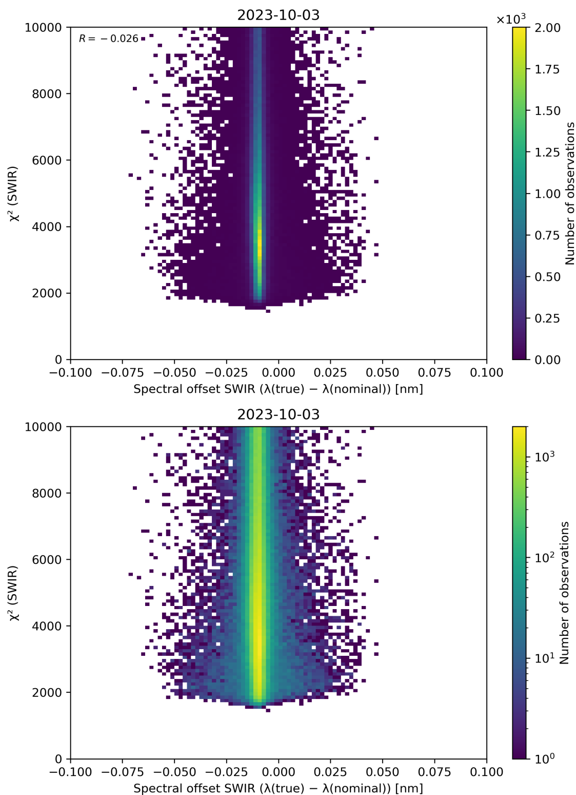
Figure 118: Scatter density plot of “Spectral offset SWIR ( \lambda(\text{true}) - \lambda(\text{nominal}) )” against “ \chi^2 (SWIR)” for 2023-10-02 to 2023-10-04.
