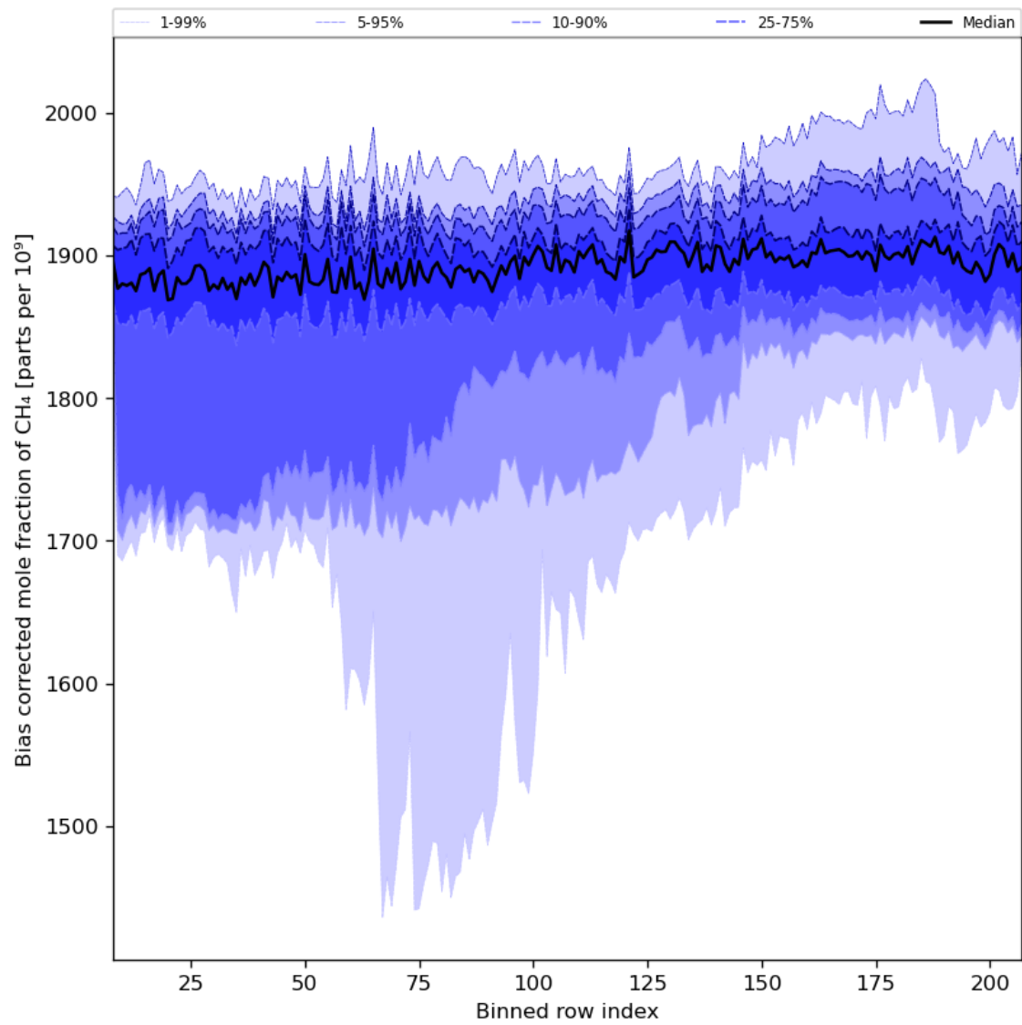
Figure 36: Along track statistics of “Bias corrected mole fraction of CH 4 ” for 2023-10-02 to 2023-10-04
