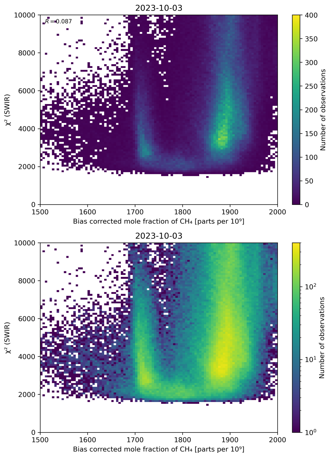
Figure 64: Scatter density plot of “Bias corrected mole fraction of CH 4 ” against “ \chi^2 (SWIR)” for 2023-10-02 to 2023-10-04.
