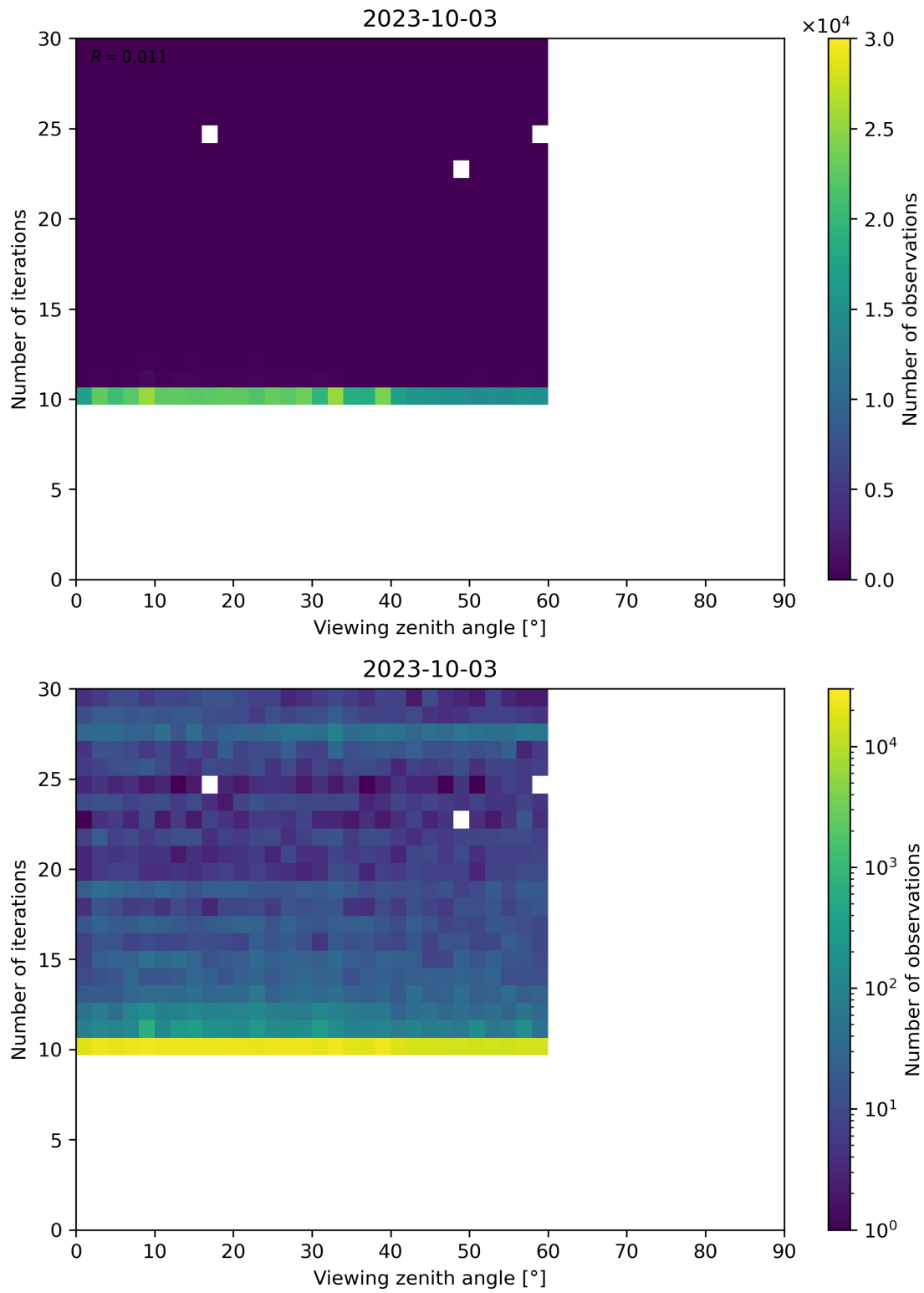
Figure 113: Scatter density plot of “Viewing zenith angle” against “Number of iterations” for 2023-10-02 to 2023-10-04.
