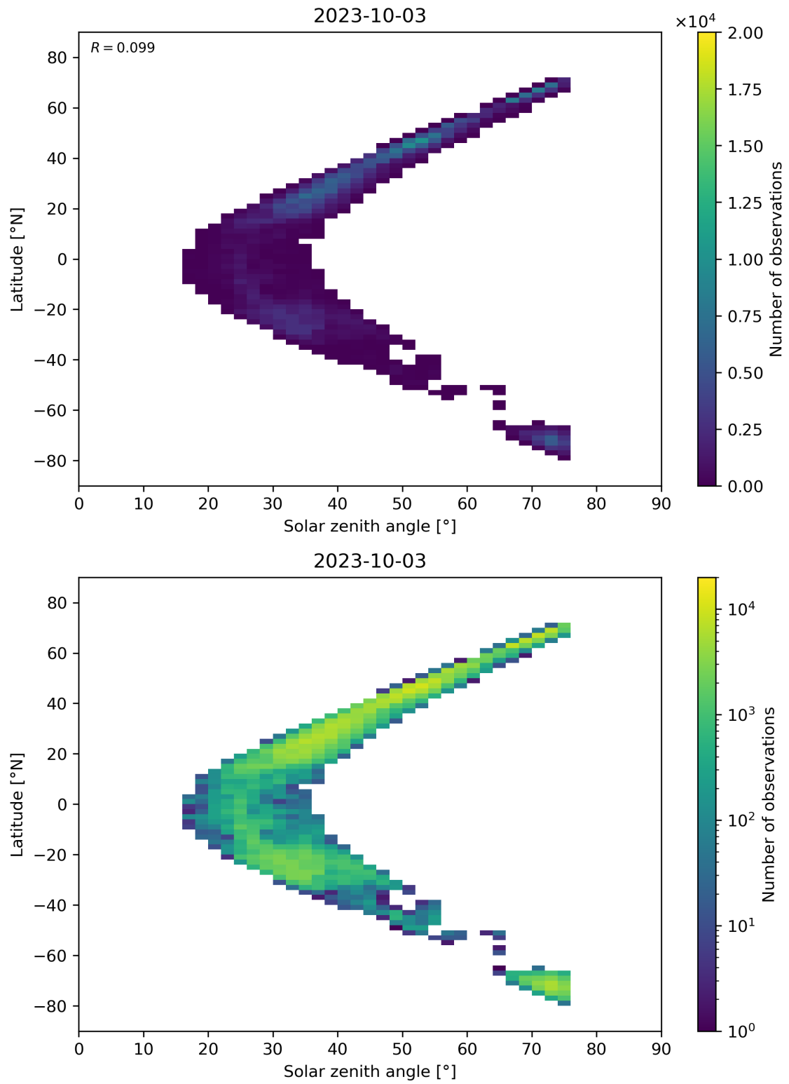
Figure 98: Scatter density plot of “Solar zenith angle” against “Latitude” for 2023-10-02 to 2023-10-04.
