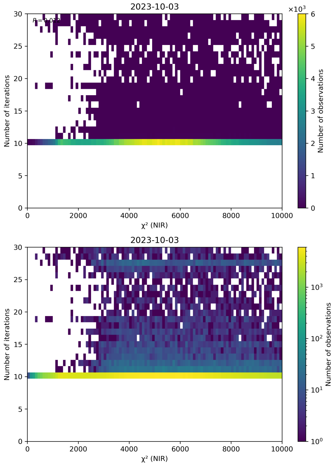
Figure 46: Scatter density plot of “ \chi^2 (NIR)” against “Number of iterations” for 2023-10-02 to 2023-10-04.
