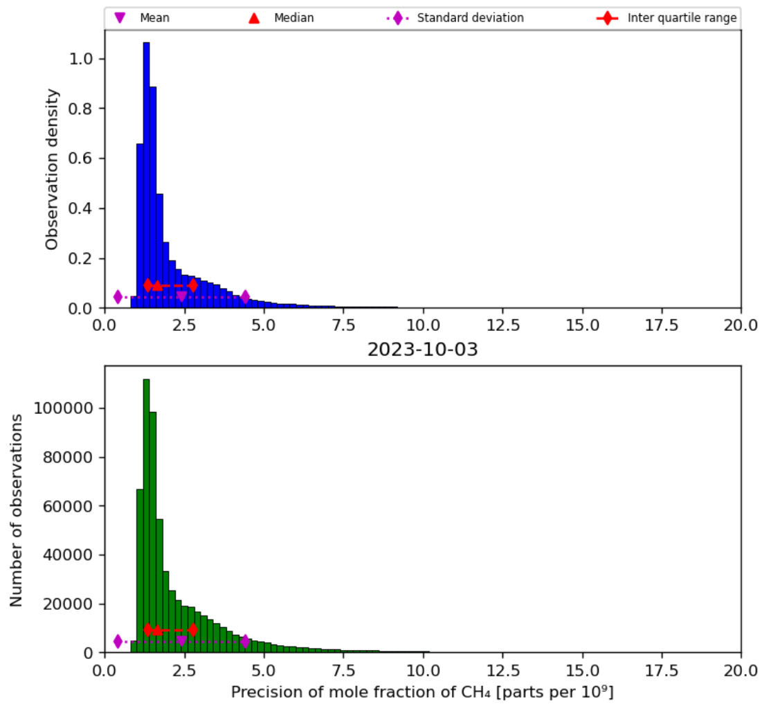
Figure 24: Histogram of “Precision of mole fraction of CH 4 ” for 2023-10-02 to 2023-10-04
