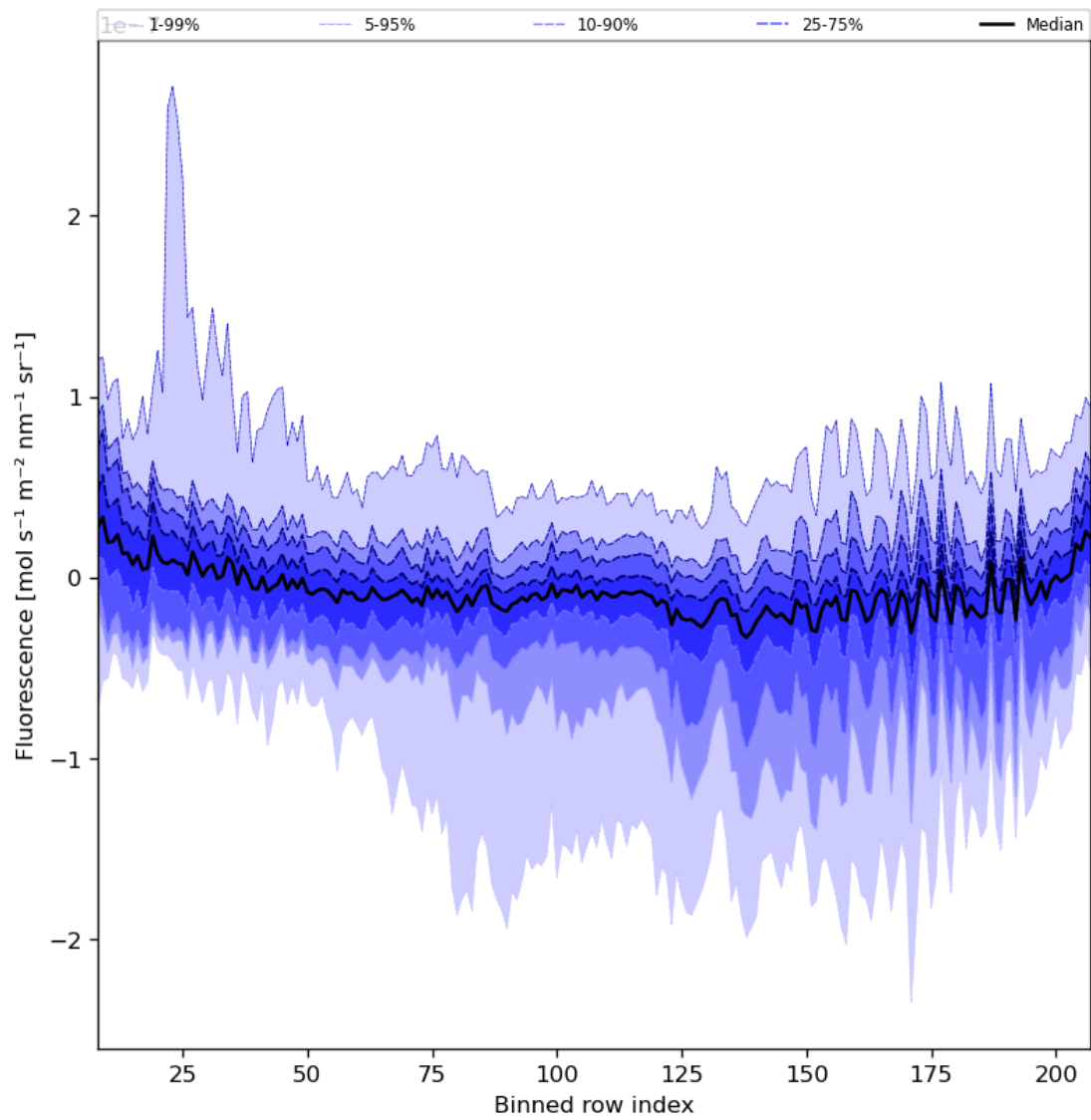
Figure 43: Along track statistics of “Fluorescence” for 2023-10-02 to 2023-10-04
