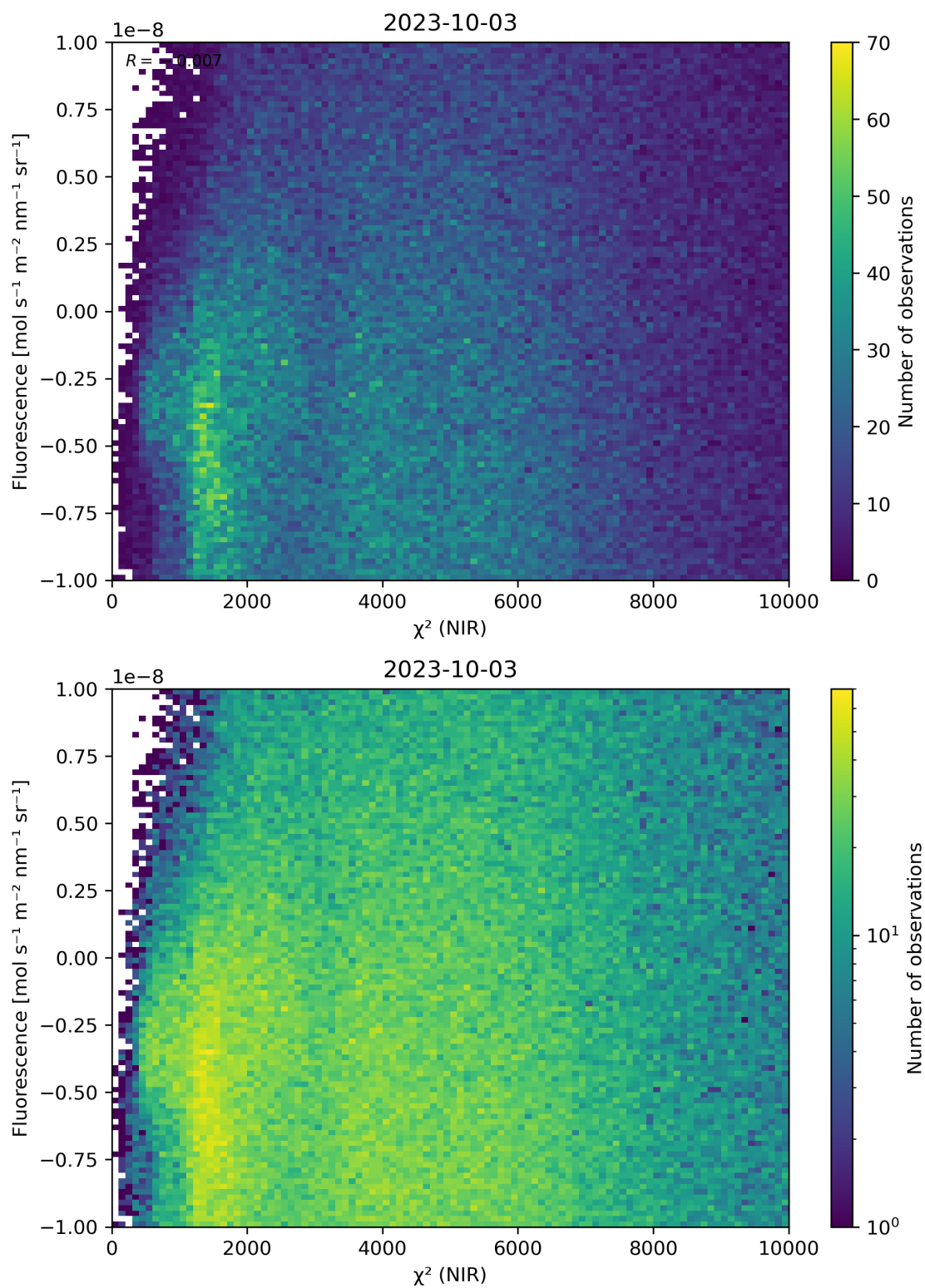
Figure 45: Scatter density plot of “ \chi^2 (NIR)” against “Fluorescence” for 2023-10-02 to 2023-10-04.
