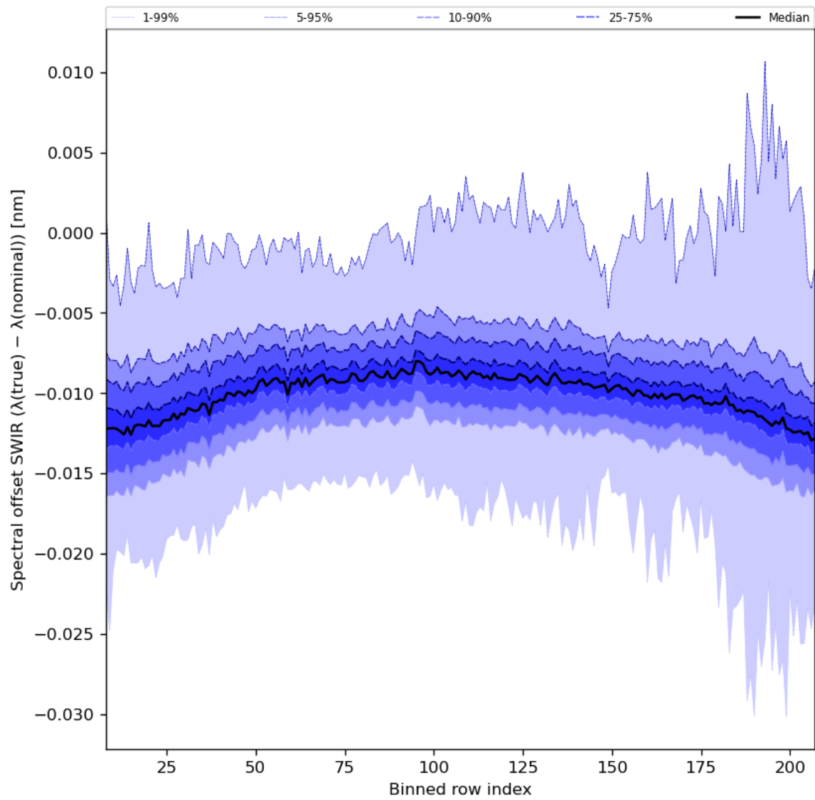
Figure 38: Along track statistics of “Spectral offset SWIR ( \lambda(\text{true}) - \lambda(\text{nominal}) )” for 2023-10-02 to 2023-10-04
