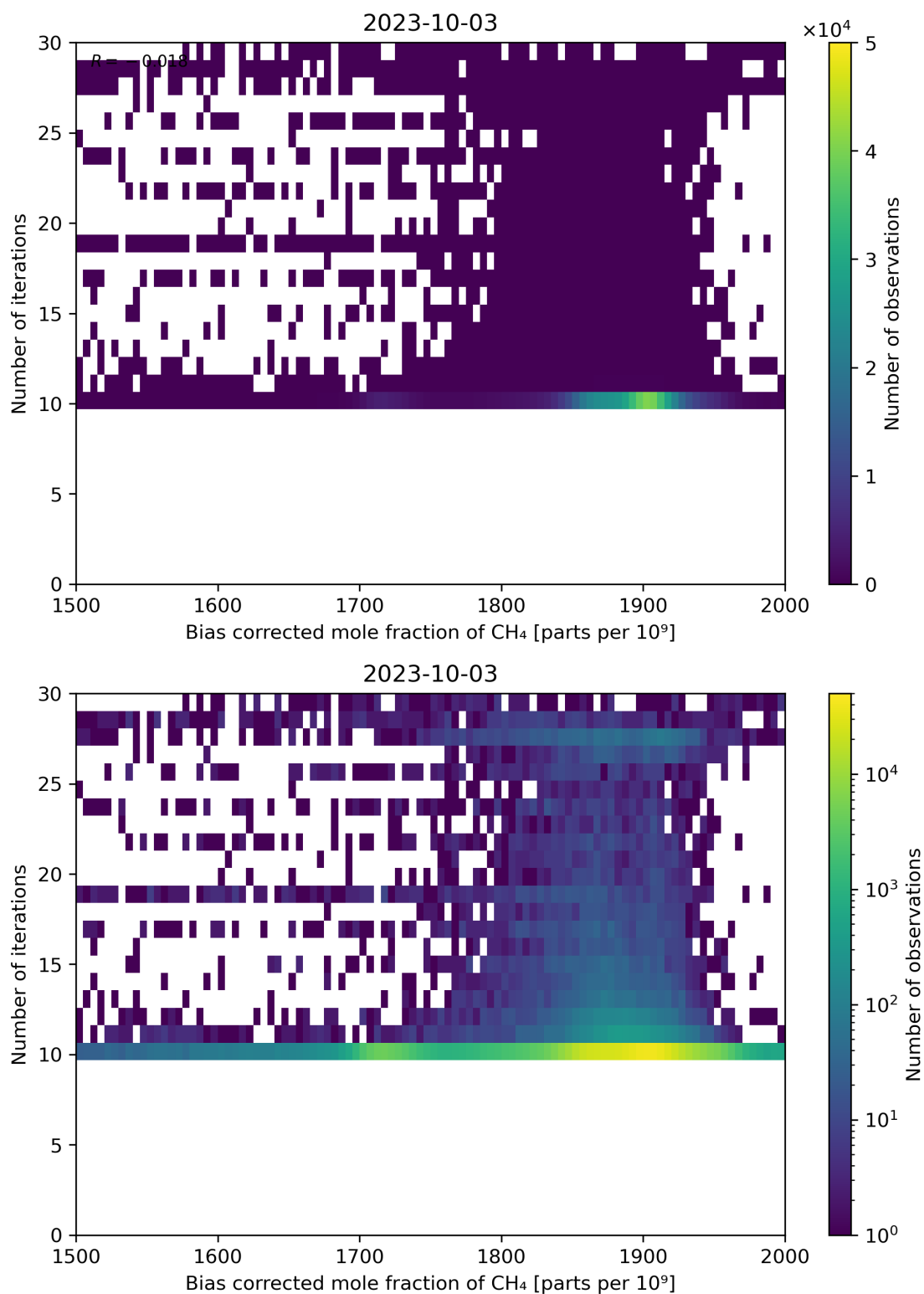
Figure 67: Scatter density plot of “Bias corrected mole fraction of CH 4 ” against “Number of iterations” for 2023-10-02 to 2023-10-04.
