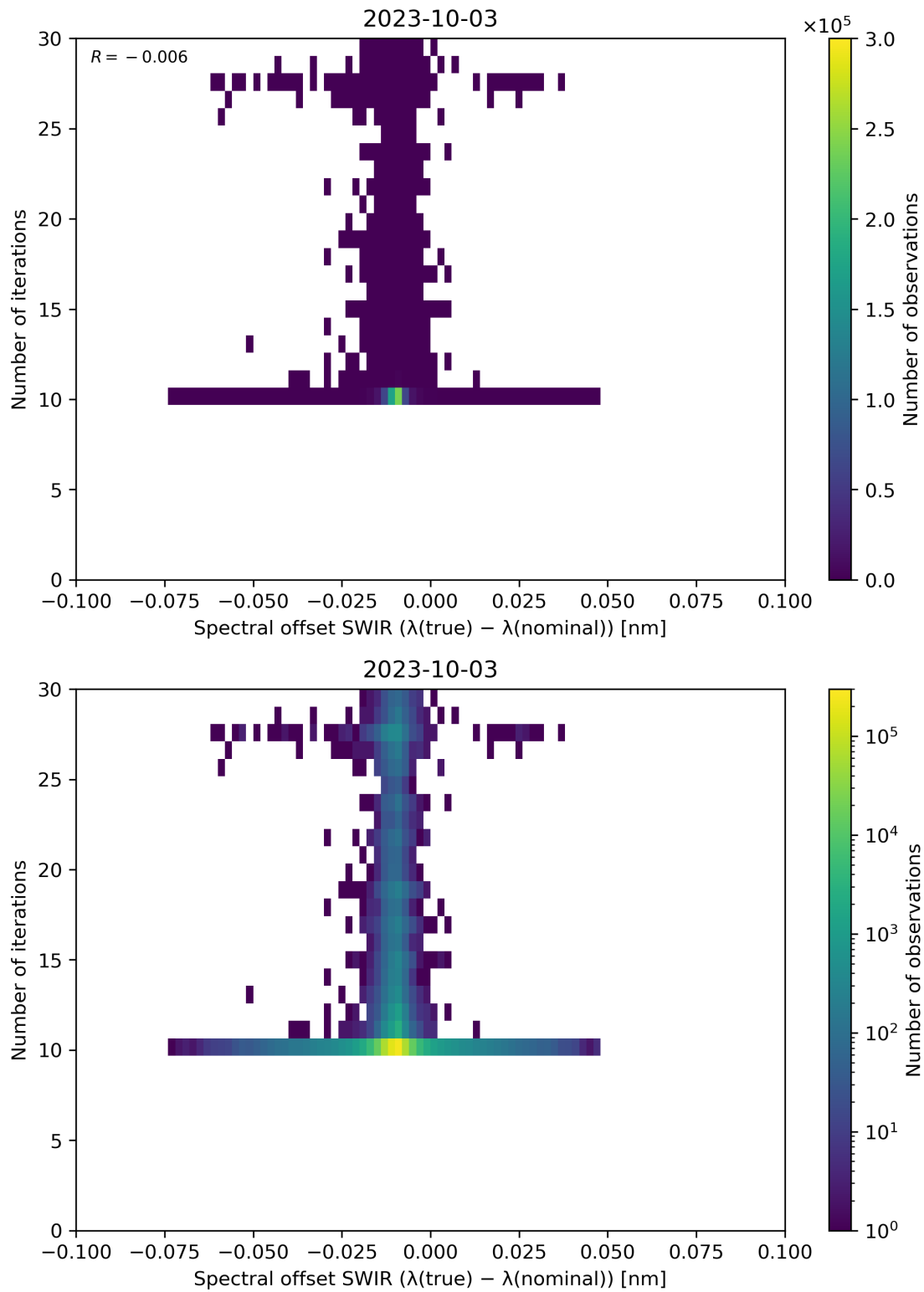
Figure 121: Scatter density plot of “Spectral offset SWIR ( \lambda(\text{true}) - \lambda(\text{nominal}) )” against “Number of iterations” for 2023-10-02 to 2023-10-04.
