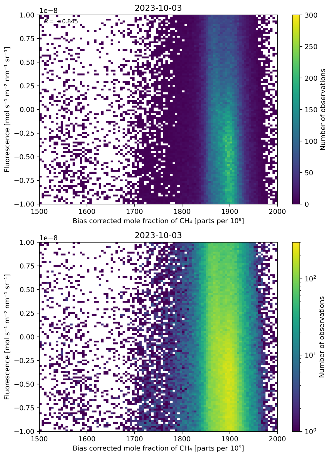
Figure 66: Scatter density plot of “Bias corrected mole fraction of \text{CH}_4 ” against “Fluorescence” for 2023-10-02 to 2023-10-04.
