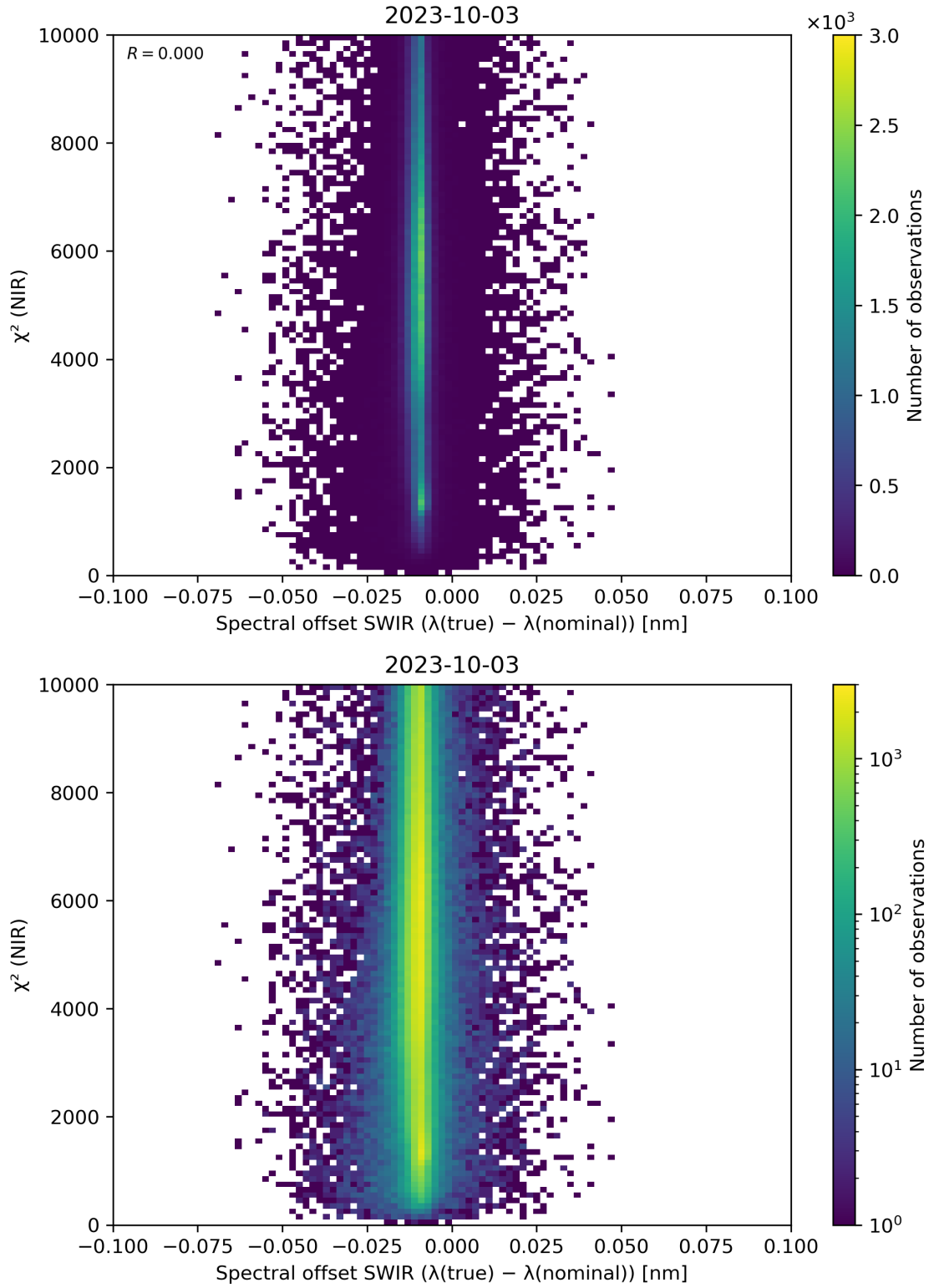
Figure 117: Scatter density plot of “Spectral offset SWIR ( \lambda(\text{true}) - \lambda(\text{nominal}) )” against “ \chi^2 (NIR)” for 2023-10-02 to 2023-10-04.
