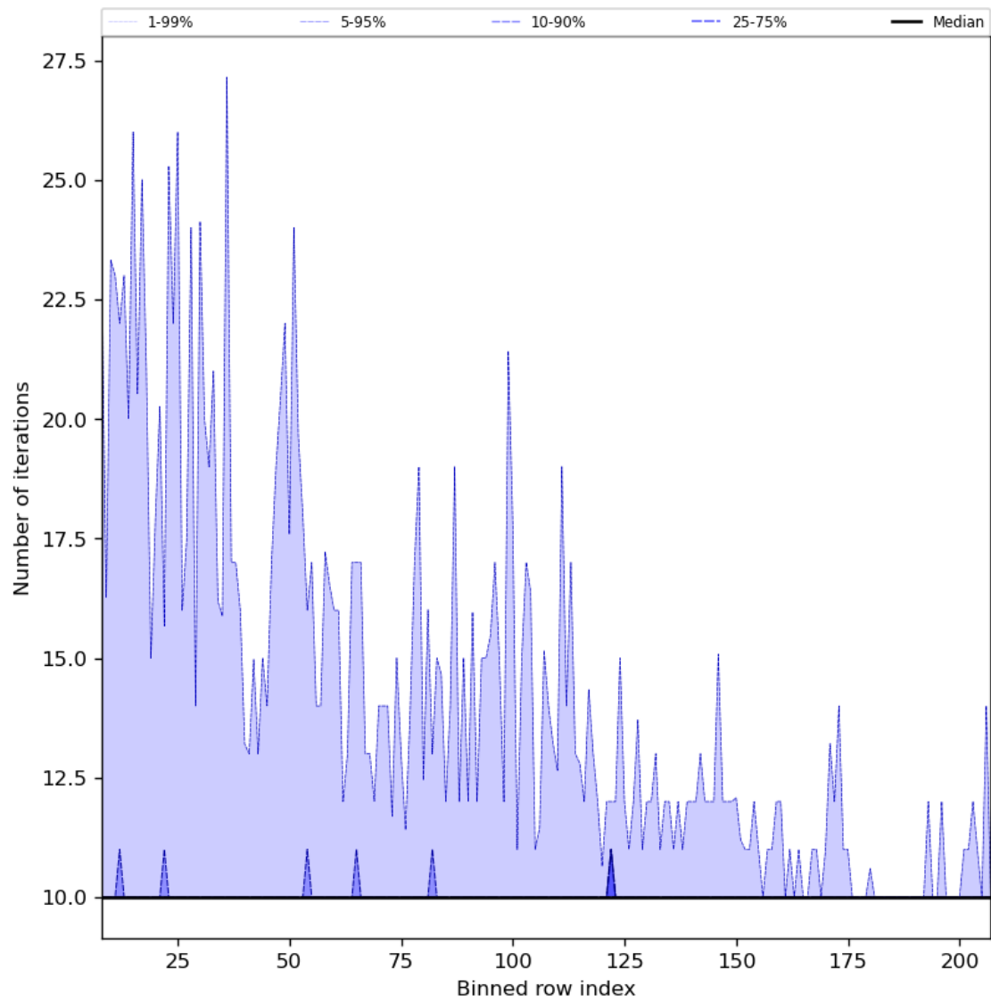
Figure 42: Along track statistics of “Number of iterations” for 2023-10-02 to 2023-10-04
