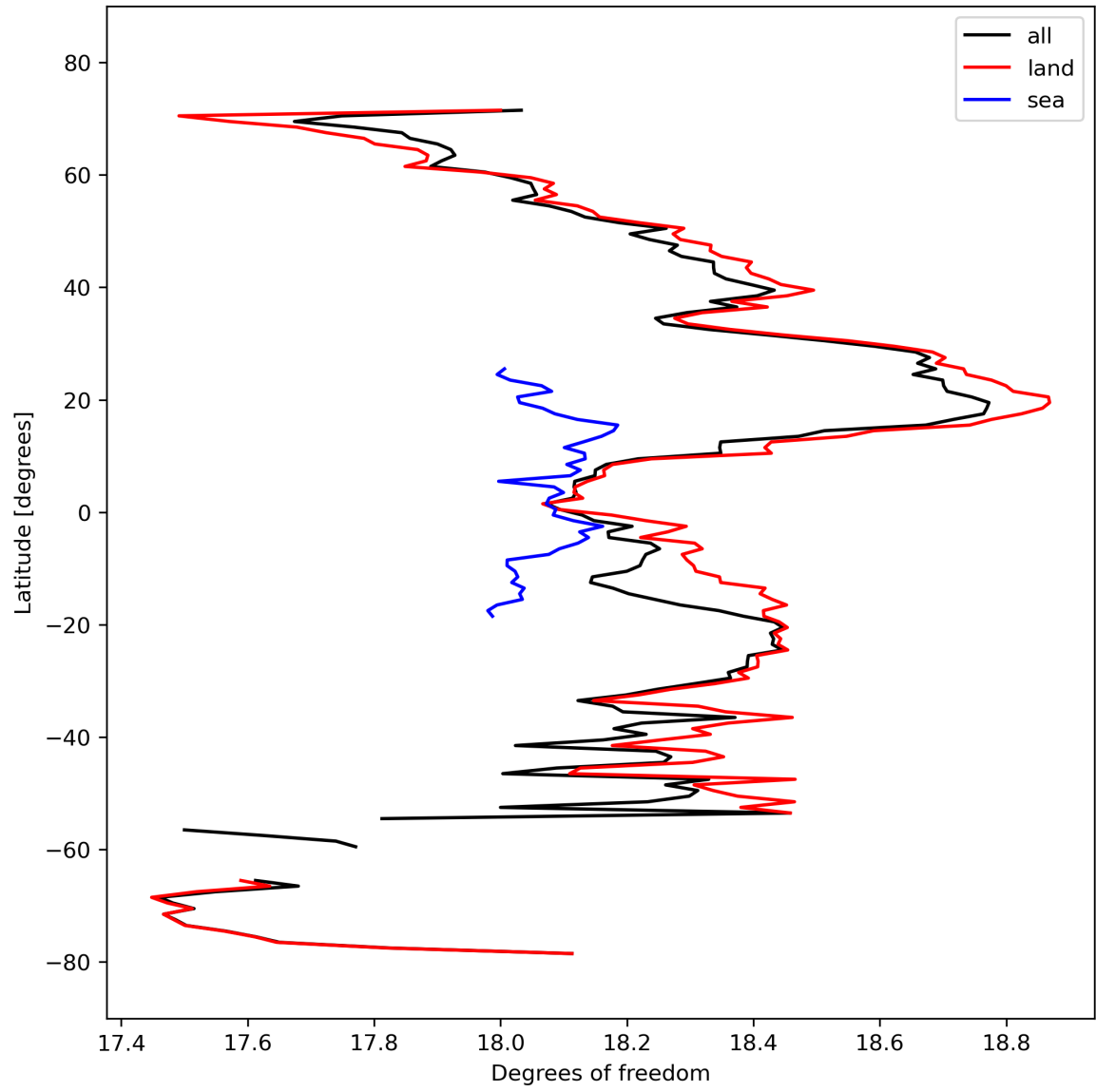
Figure 19: Zonal average of “Degrees of freedom” for 2023-10-02 to 2023-10-04.
