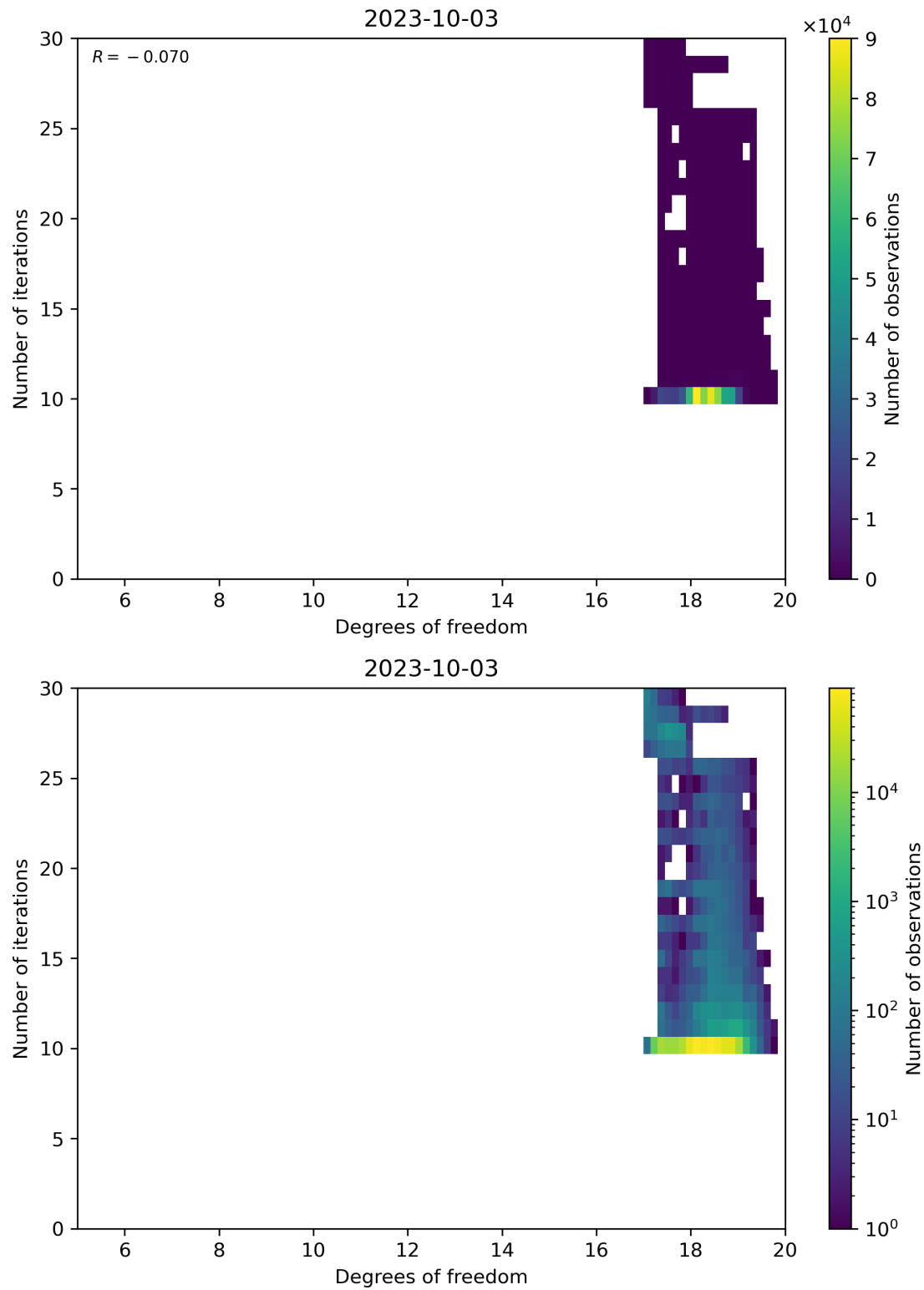
Figure 52: Scatter density plot of “Degrees of freedom” against “Number of iterations” for 2023-10-02 to 2023-10-04.
