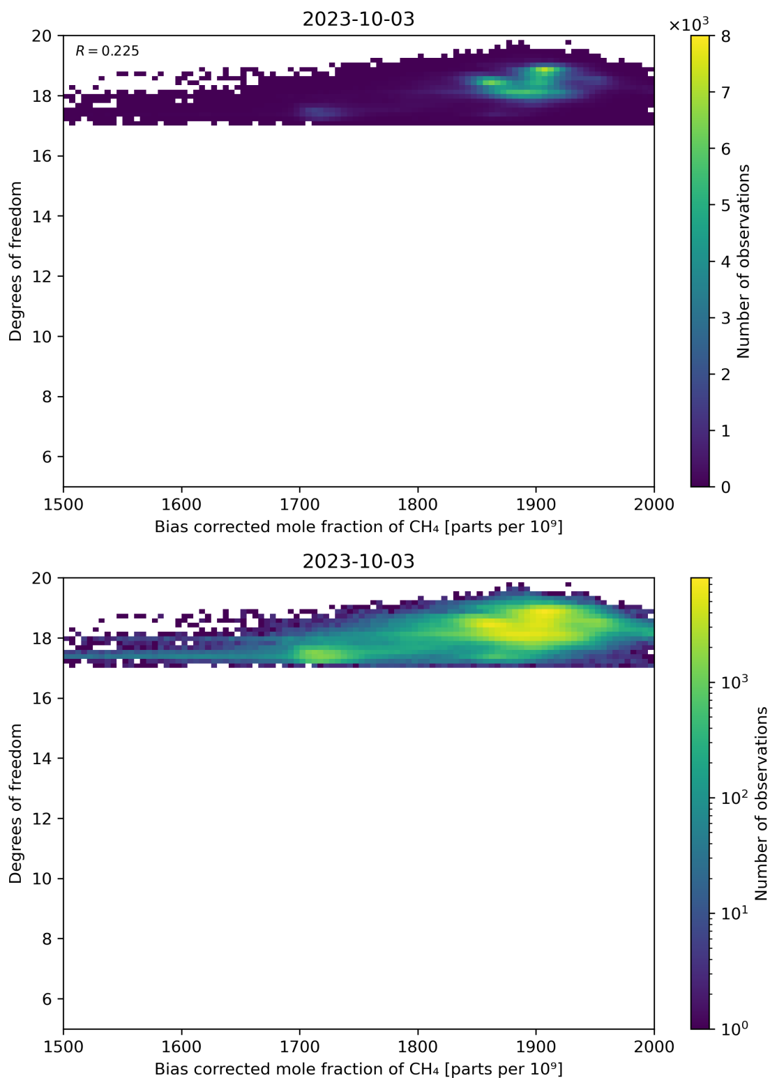
Figure 65: Scatter density plot of “Bias corrected mole fraction of CH 4 ” against “Degrees of freedom” for 2023-10-02 to 2023-10-04.
