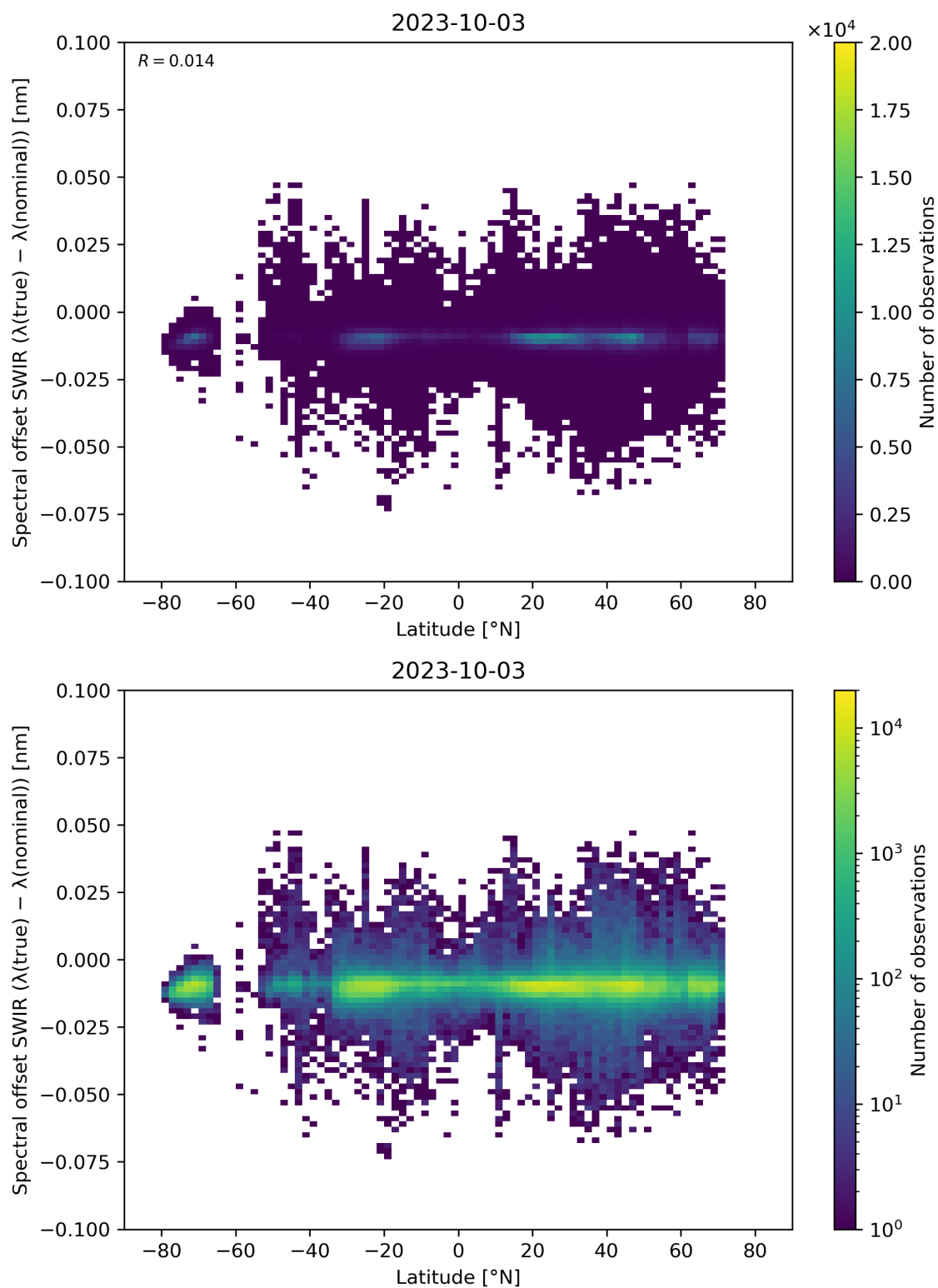
Figure 62: Scatter density plot of “Latitude” against “Spectral offset SWIR ( \lambda(\text{true}) - \lambda(\text{nominal}) )” for 2023-10-02 to 2023-10-04.
