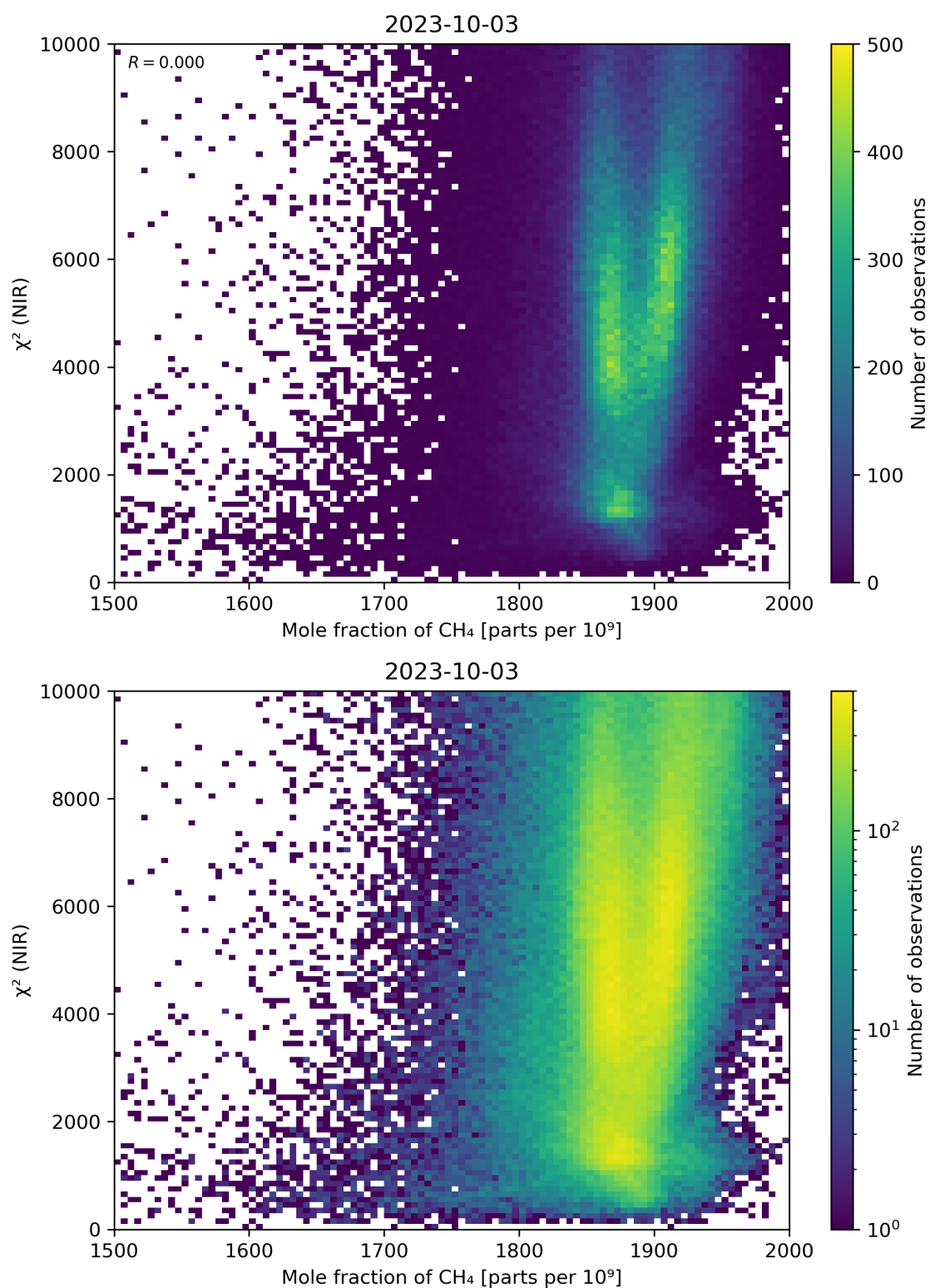
Figure 70: Scatter density plot of “Mole fraction of CH 4 ” against “ \chi^2 (NIR)” for 2023-10-02 to 2023-10-04.
