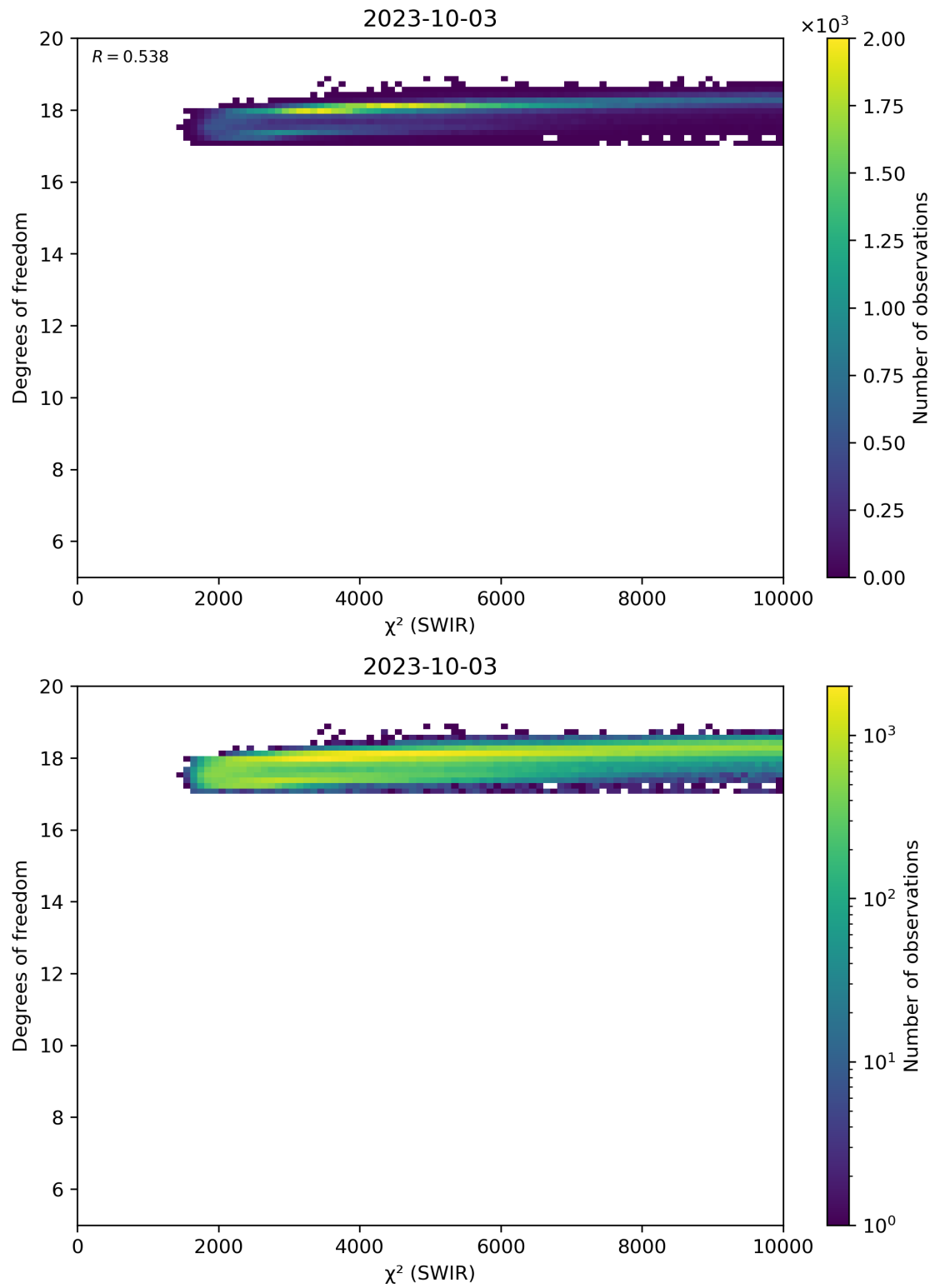
Figure 48: Scatter density plot of “ \chi^2 (SWIR)” against “Degrees of freedom” for 2023-10-02 to 2023-10-04.
