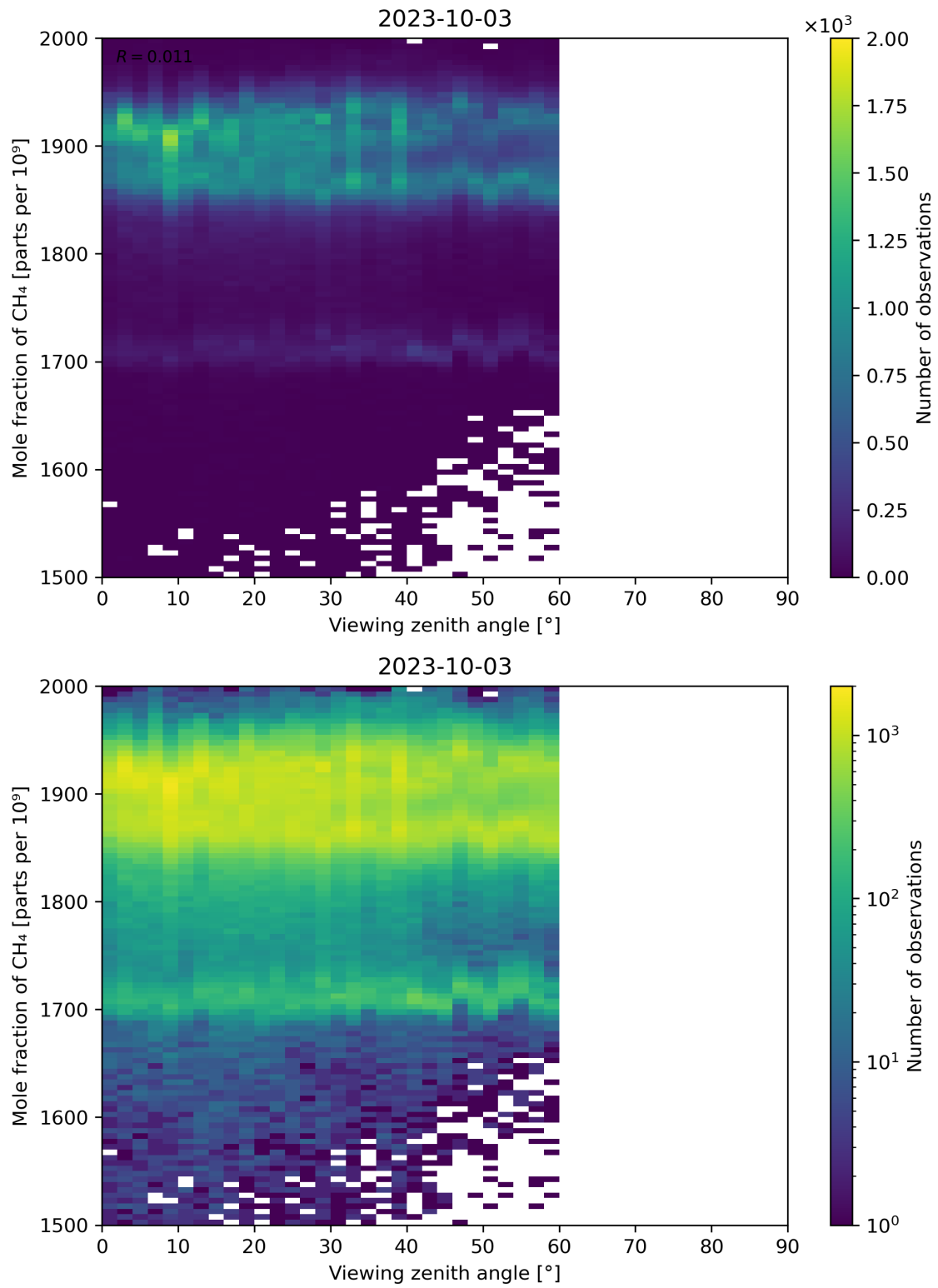
Figure 110: Scatter density plot of “Viewing zenith angle” against “Mole fraction of CH 4 ” for 2023-10-02 to 2023-10-04.
