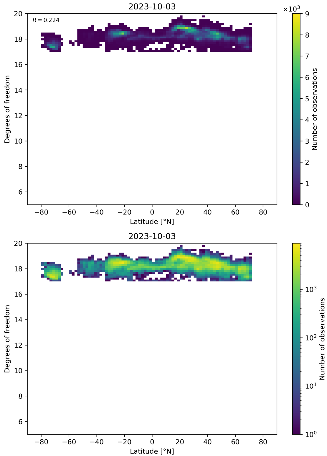
Figure 55: Scatter density plot of “Latitude” against “Degrees of freedom” for 2023-10-02 to 2023-10-04.
