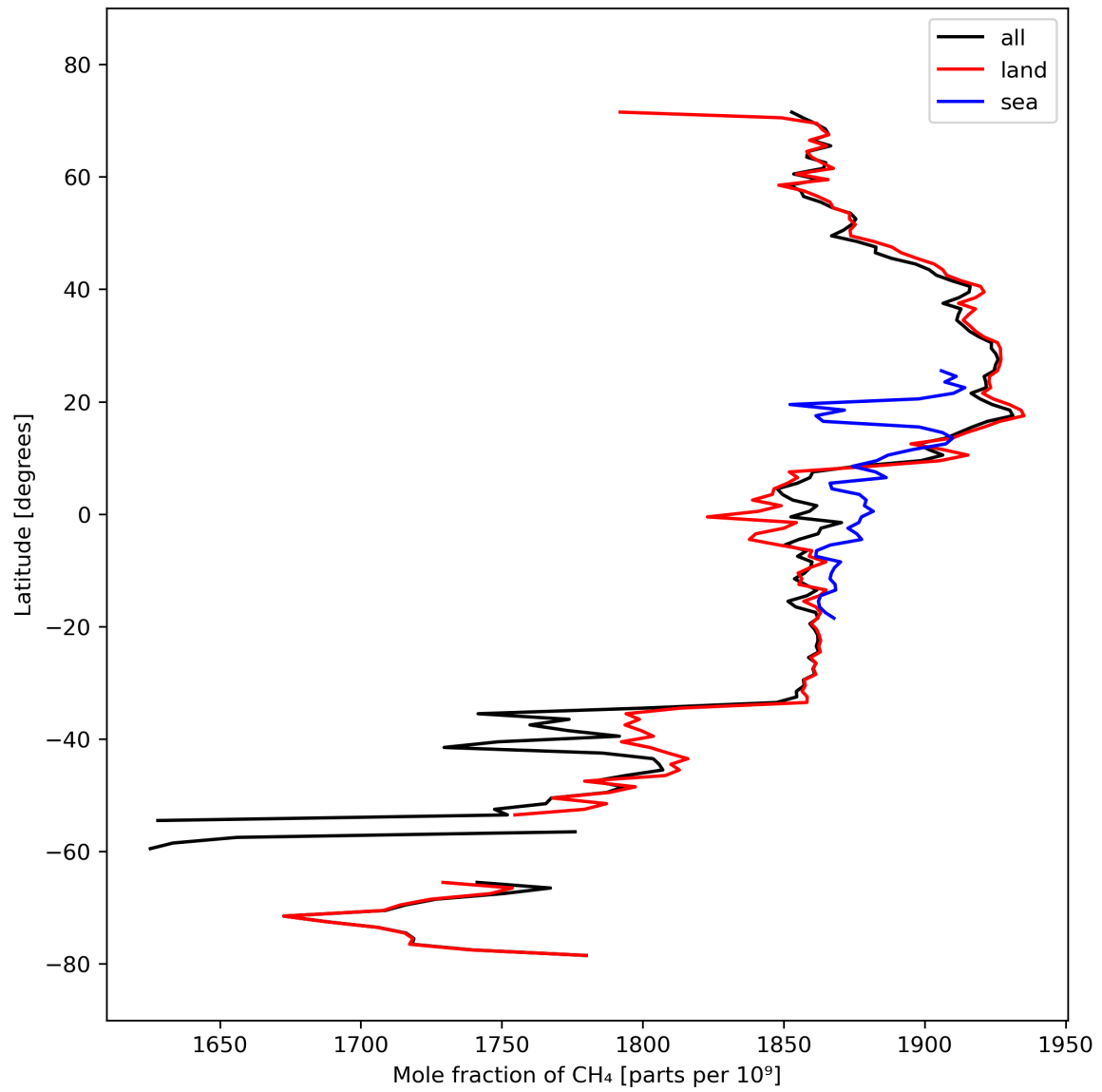
Figure 12: Zonal average of “Mole fraction of \text{CH}_4 ” for 2023-10-02 to 2023-10-04.
