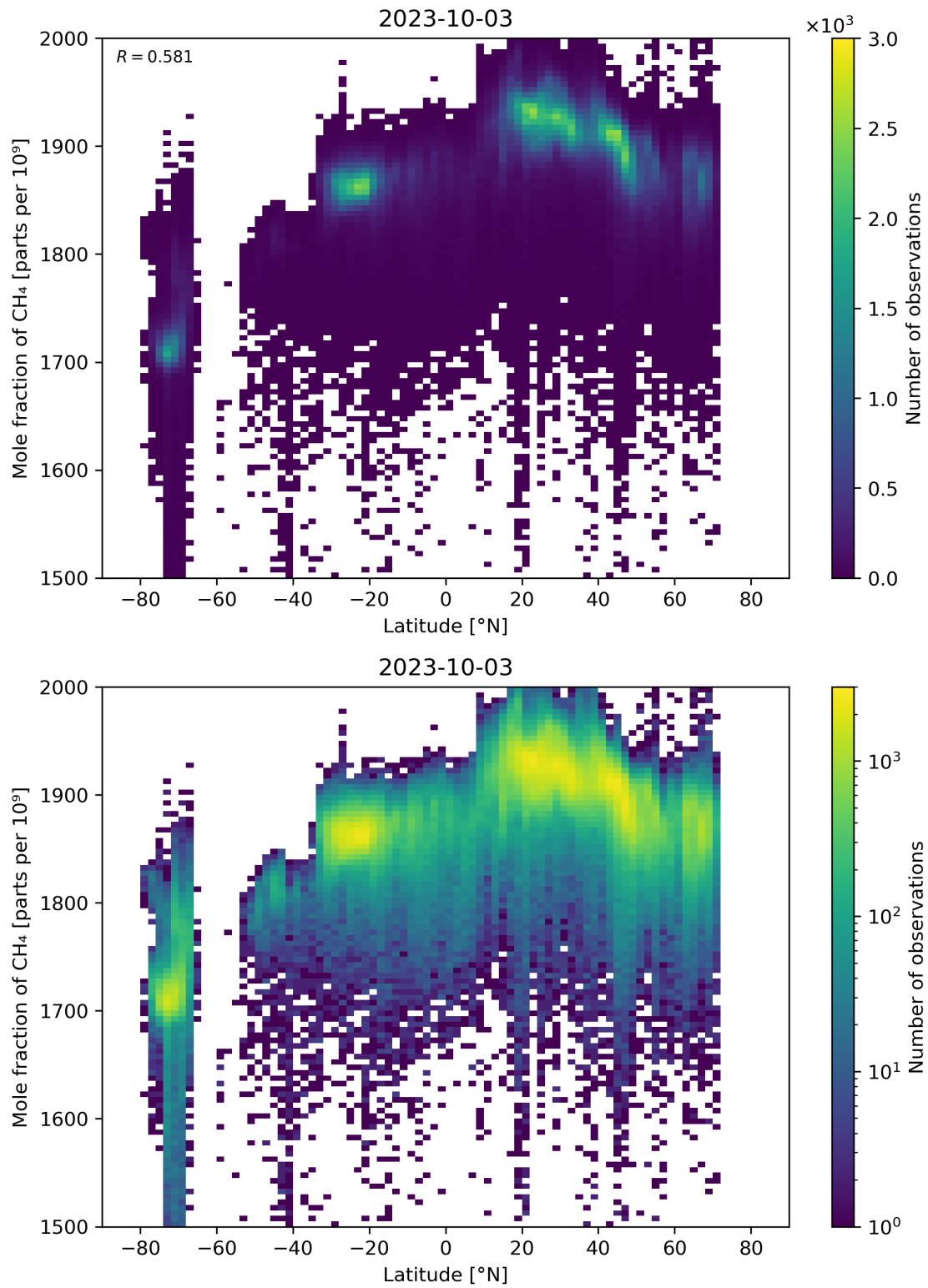
Figure 57: Scatter density plot of “Latitude” against “Mole fraction of CH 4 ” for 2023-10-02 to 2023-10-04.
