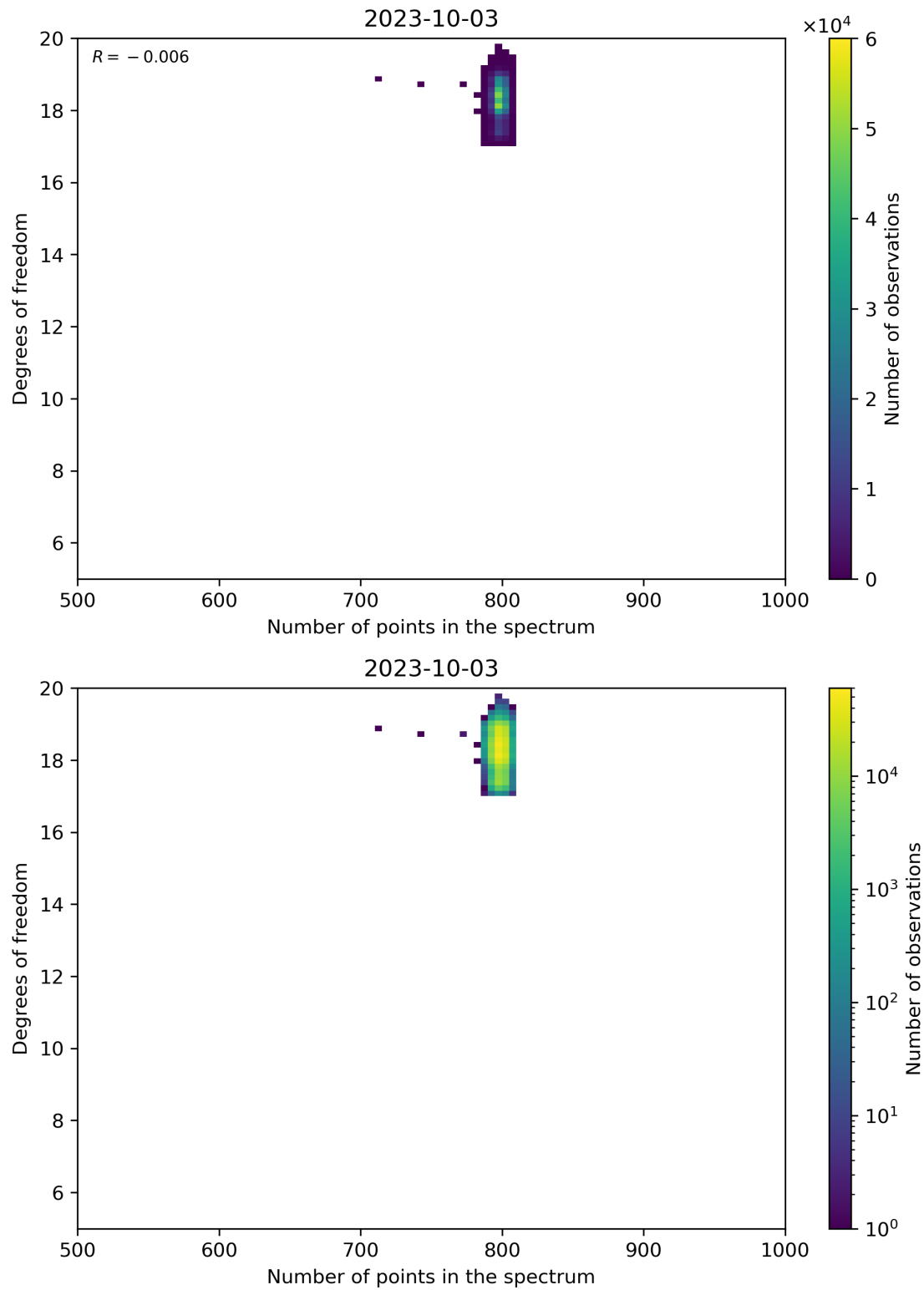
Figure 90: Scatter density plot of “Number of points in the spectrum” against “Degrees of freedom” for 2023-10-02 to 2023-10-04.
