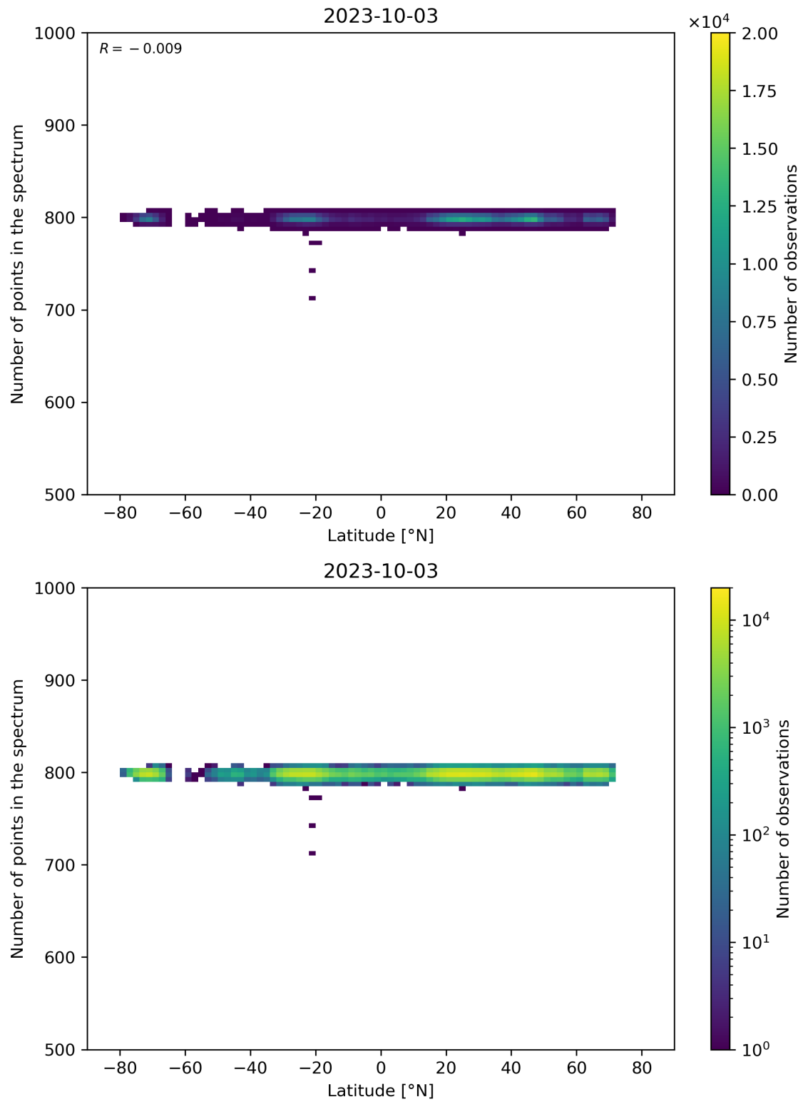
Figure 61: Scatter density plot of “Latitude” against “Number of points in the spectrum” for 2023-10-02 to 2023-10-04.
