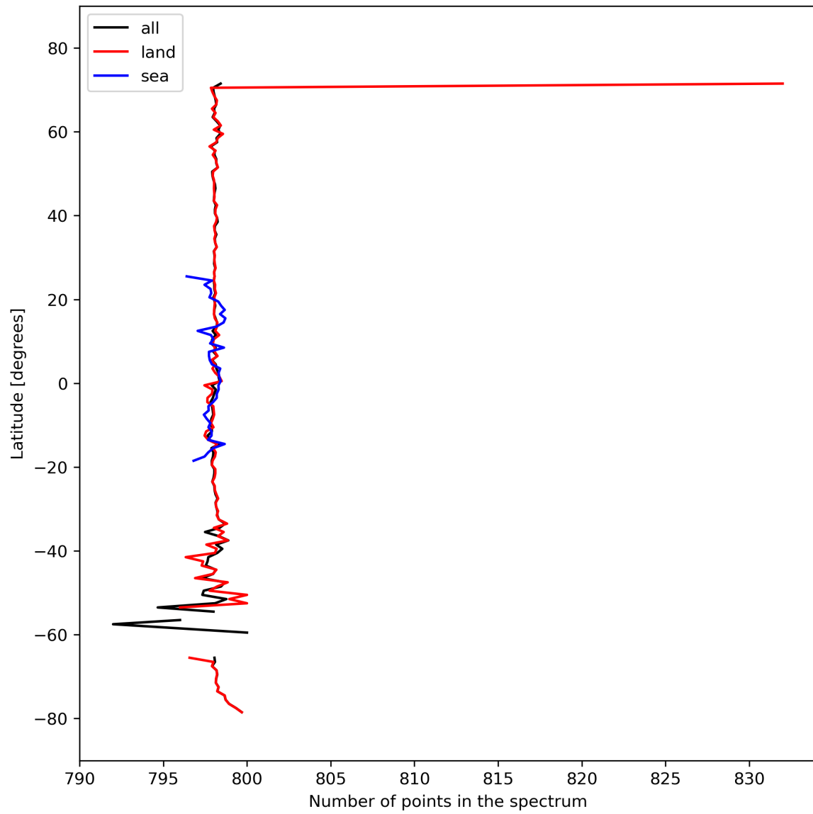
Figure 15: Zonal average of “Number of points in the spectrum” for 2023-10-02 to 2023-10-04.
