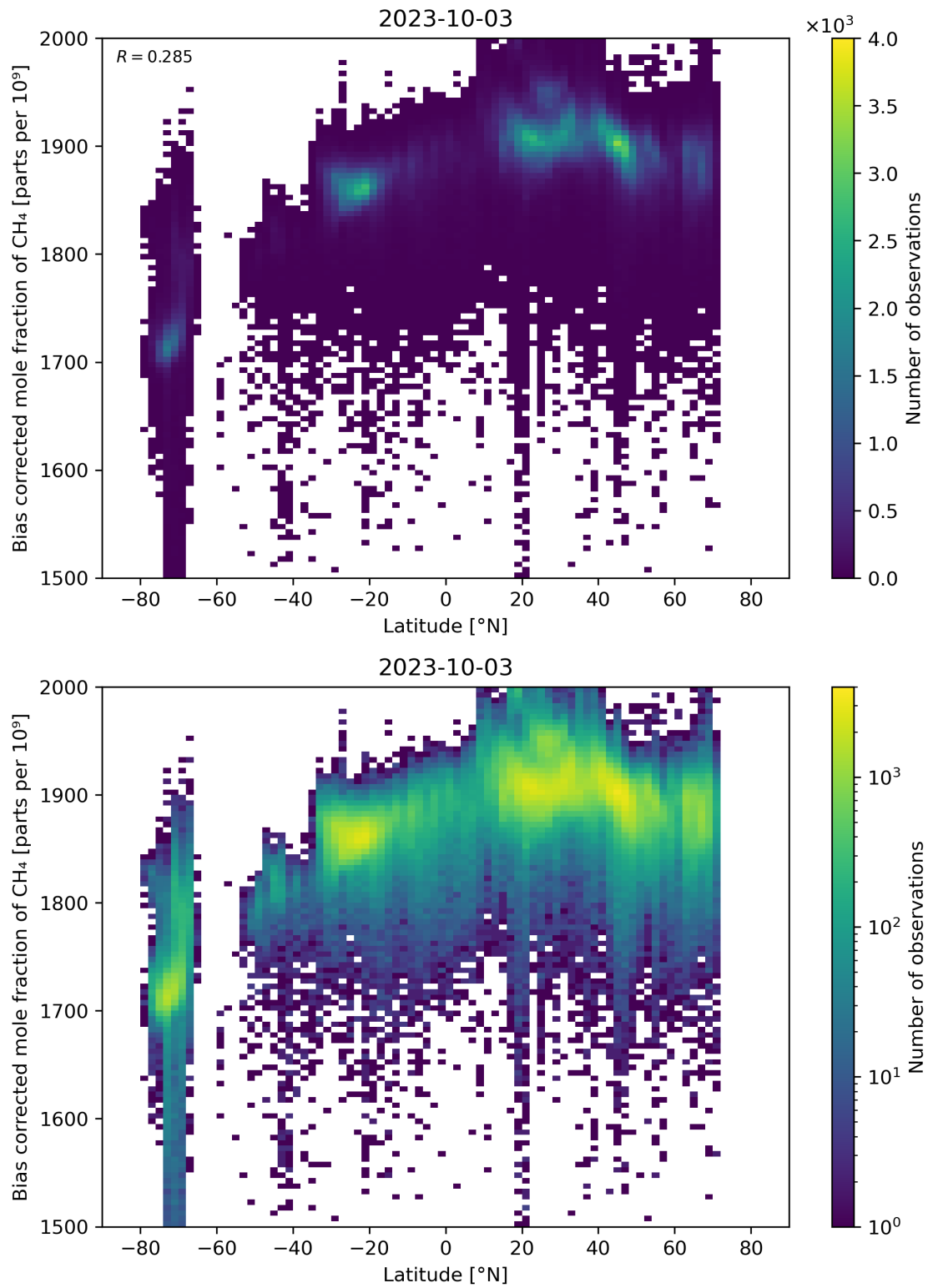
Figure 58: Scatter density plot of “Latitude” against “Bias corrected mole fraction of CH 4 ” for 2023-10-02 to 2023-10-04.
