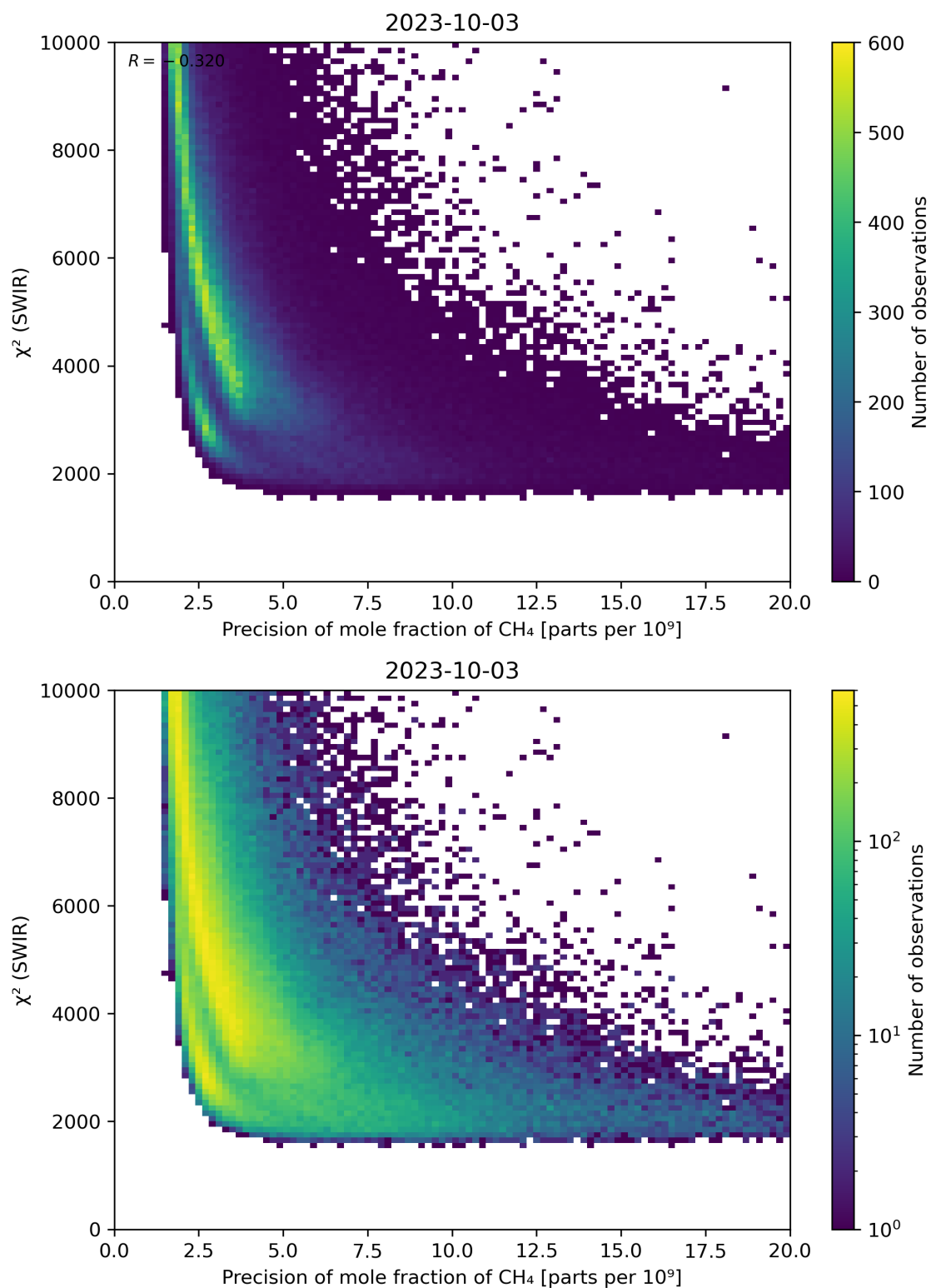
Figure 79: Scatter density plot of “Precision of mole fraction of CH 4 ” against “ \chi^2 (SWIR)” for 2023-10-02 to 2023-10-04.
