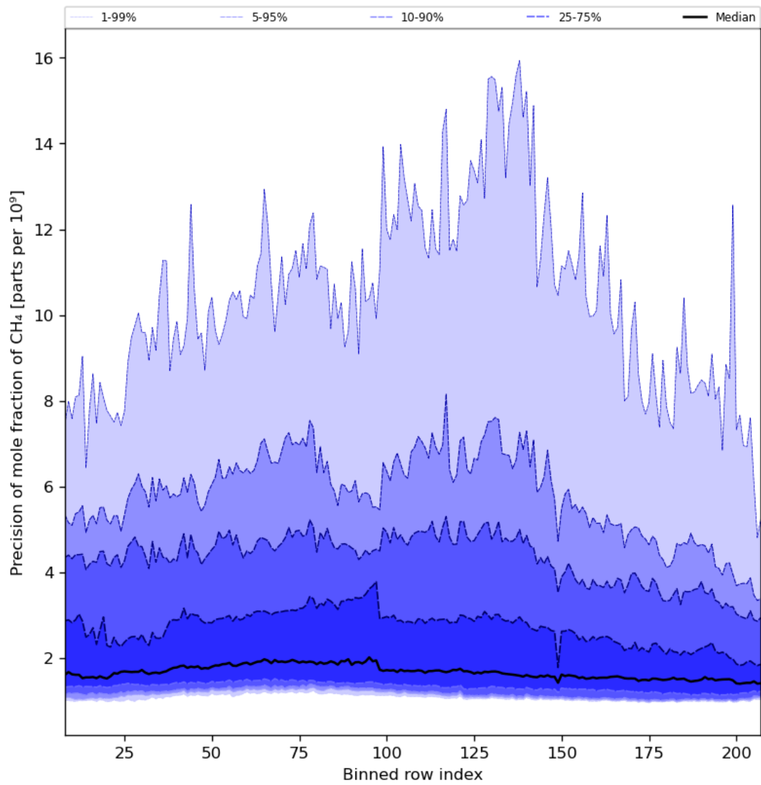
Figure 35: Along track statistics of “Precision of mole fraction of CH 4 ” for 2023-10-02 to 2023-10-04
