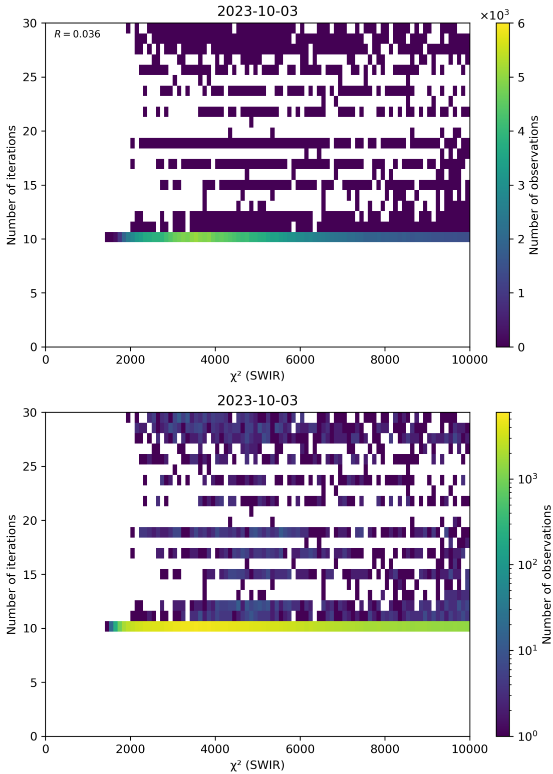
Figure 50: Scatter density plot of “ \chi^2 (SWIR)” against “Number of iterations” for 2023-10-02 to 2023-10-04.
