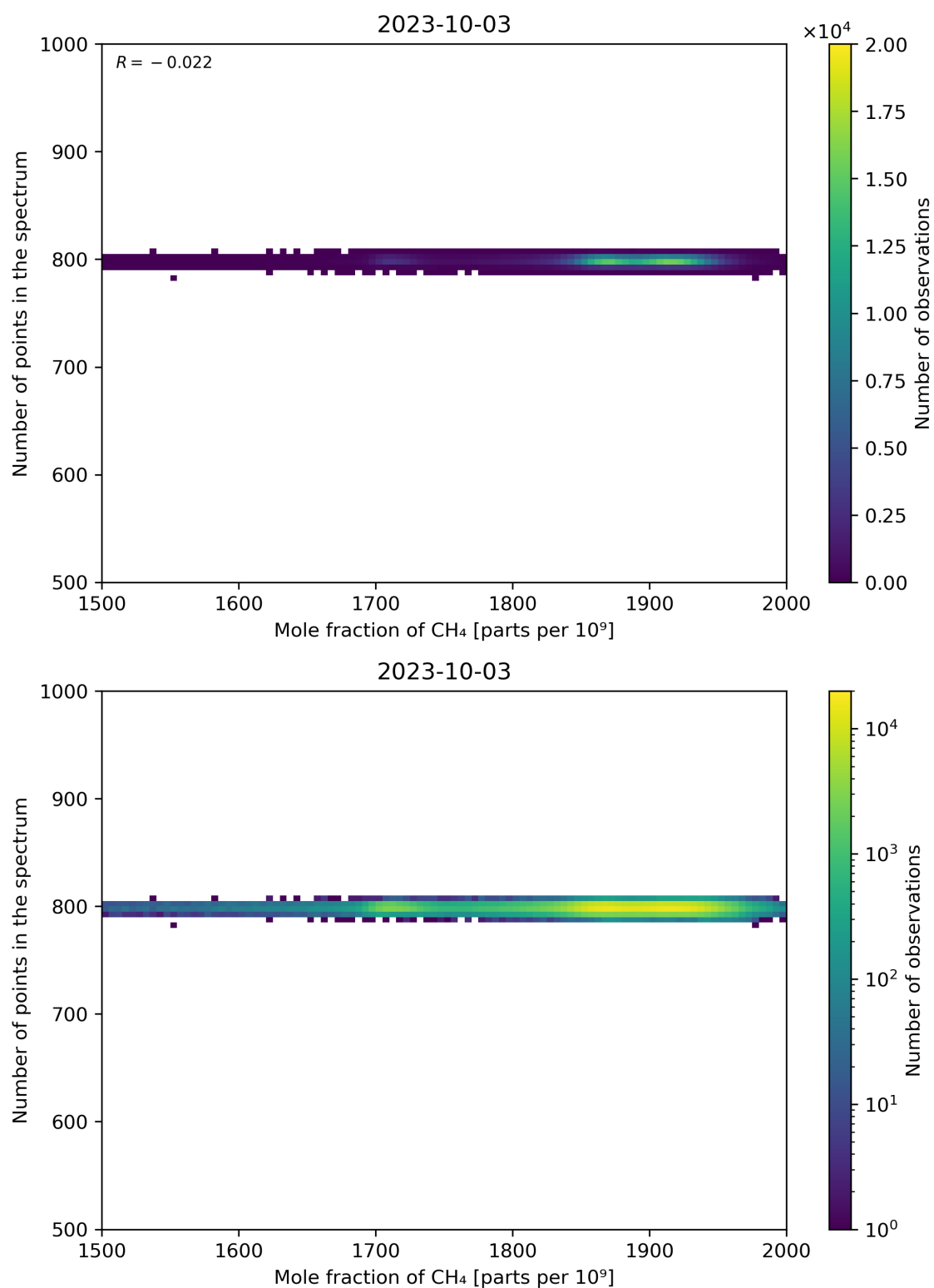
Figure 77: Scatter density plot of “Mole fraction of CH 4 ” against “Number of points in the spectrum” for 2023-10-02 to 2023-10-04.
