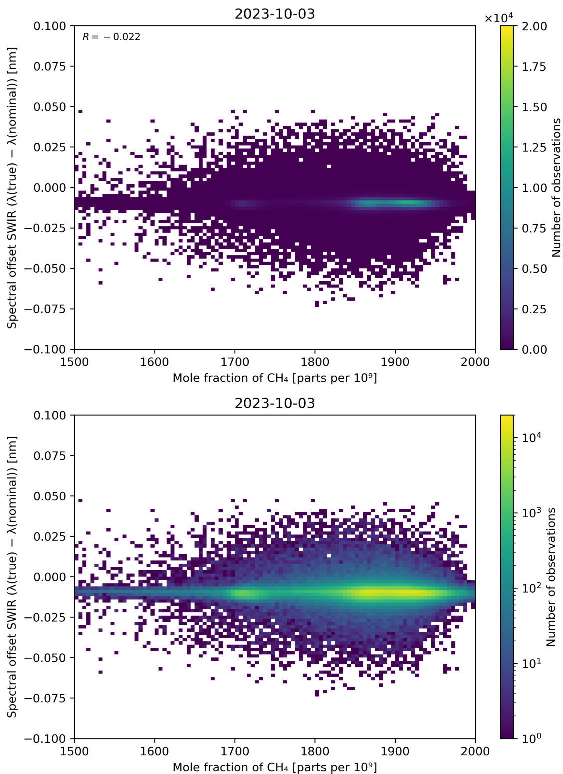
Figure 86: Scatter density plot of “Mole fraction of CH 4 ” against “Spectral offset SWIR ( \lambda(\text{true}) - \lambda(\text{nominal}) )” for 2023-10-02 to 2023-10-04.
