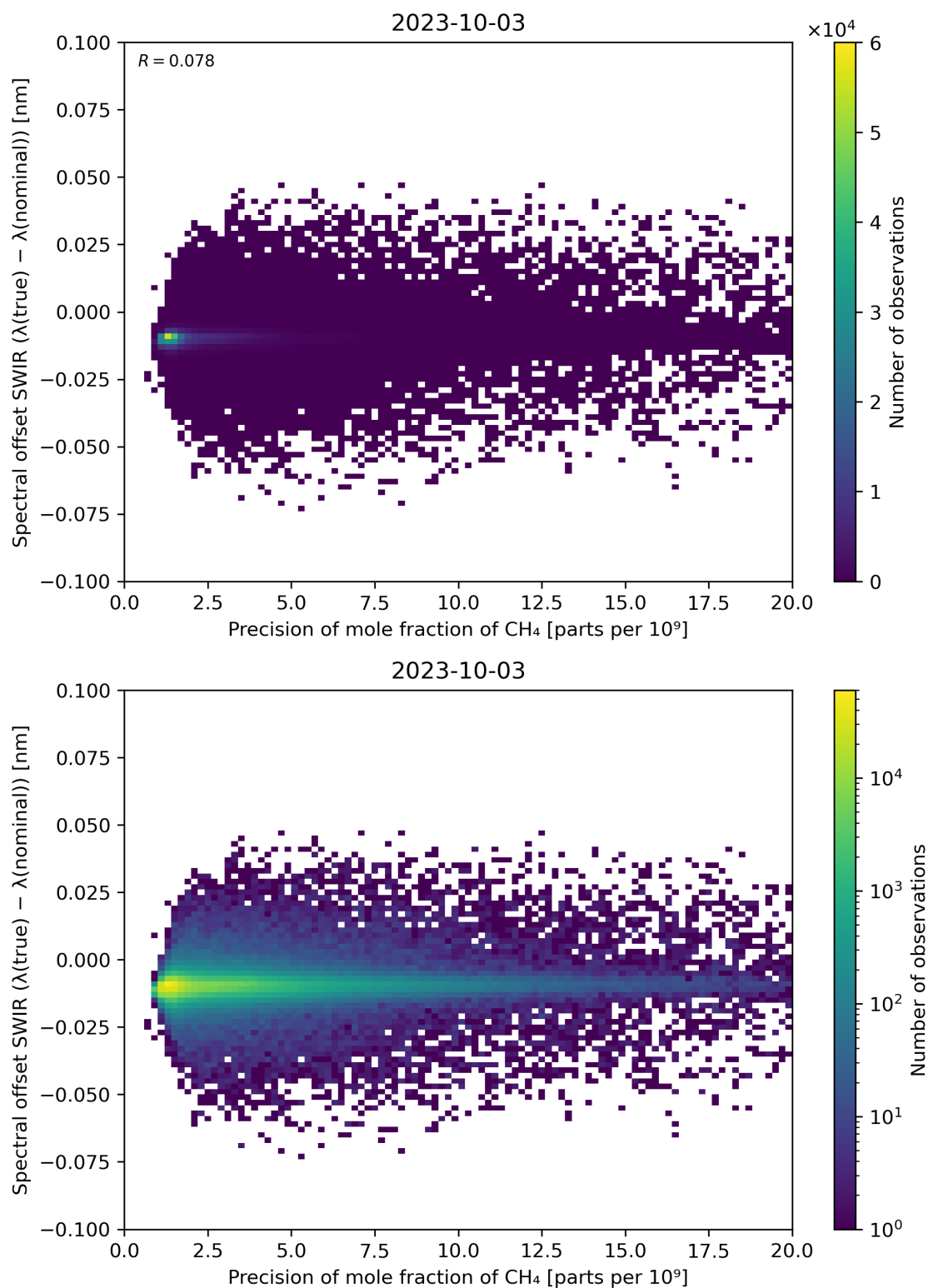
Figure 85: Scatter density plot of “Precision of mole fraction of CH 4 ” against “Spectral offset SWIR ( \lambda(\text{true}) - \lambda(\text{nominal}) )” for 2023-10-02 to 2023-10-04.
