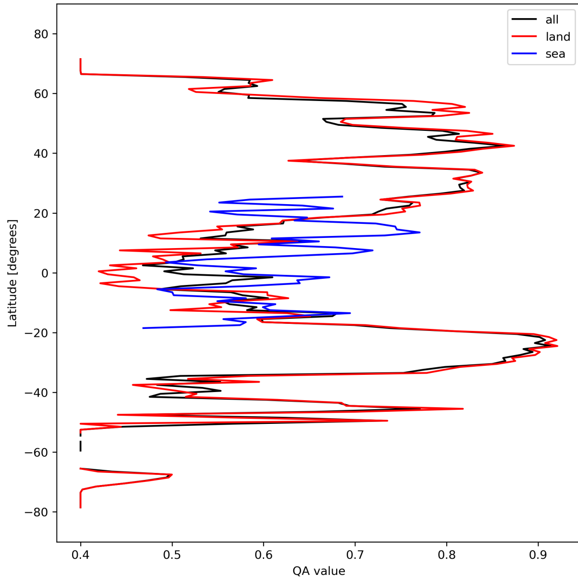
Figure 11: Zonal average of “QA value” for 2023-10-02 to 2023-10-04.
