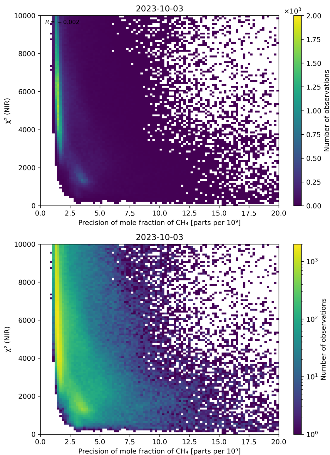
Figure 78: Scatter density plot of “Precision of mole fraction of CH 4 ” against “ \chi^2 (NIR)” for 2023-10-02 to 2023-10-04.
