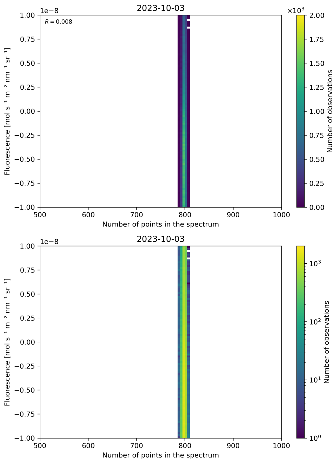
Figure 91: Scatter density plot of “Number of points in the spectrum” against “Fluorescence” for 2023-10-02 to 2023-10-04.
