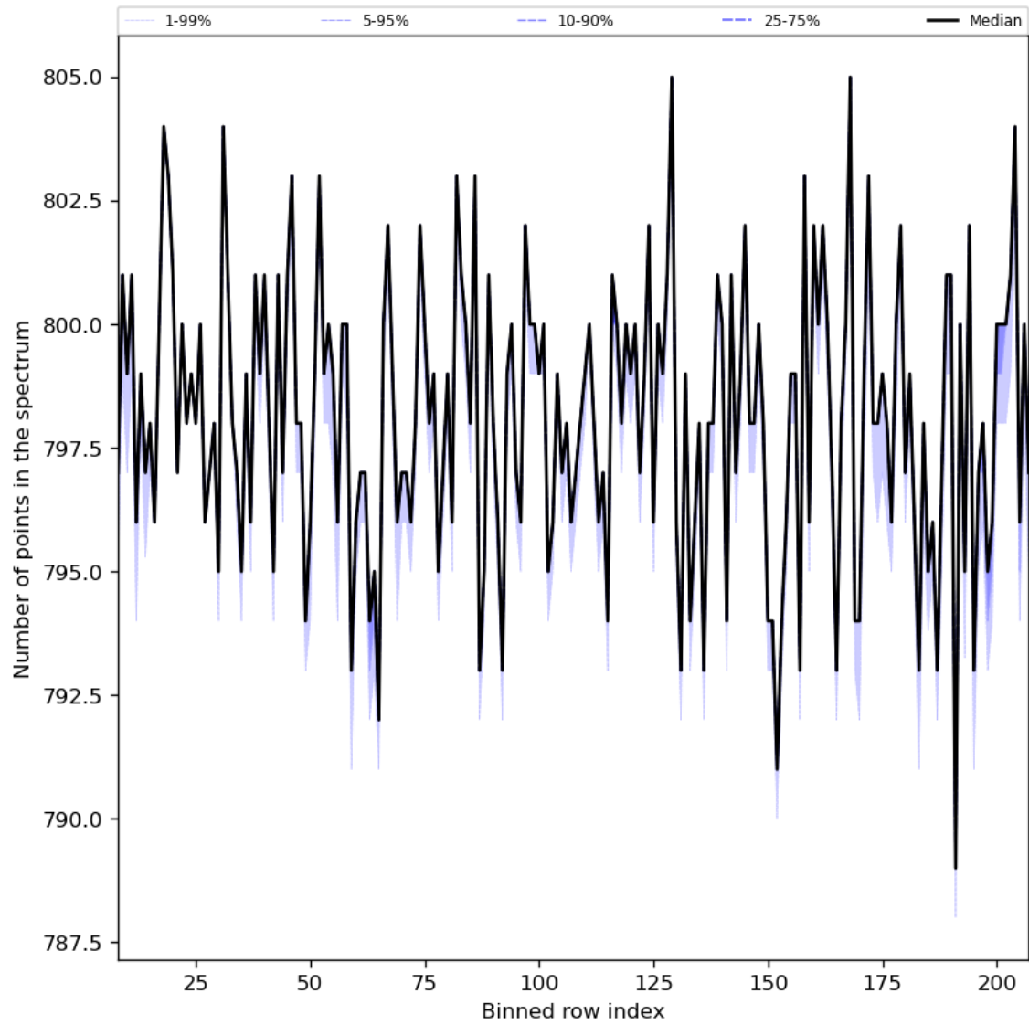
Figure 37: Along track statistics of “Number of points in the spectrum” for 2023-10-02 to 2023-10-04
