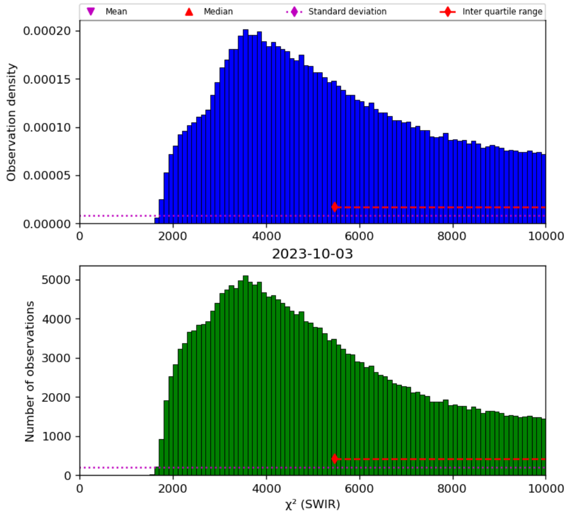
Figure 28: Histogram of “ \chi^2 (SWIR)” for 2023-10-02 to 2023-10-04
