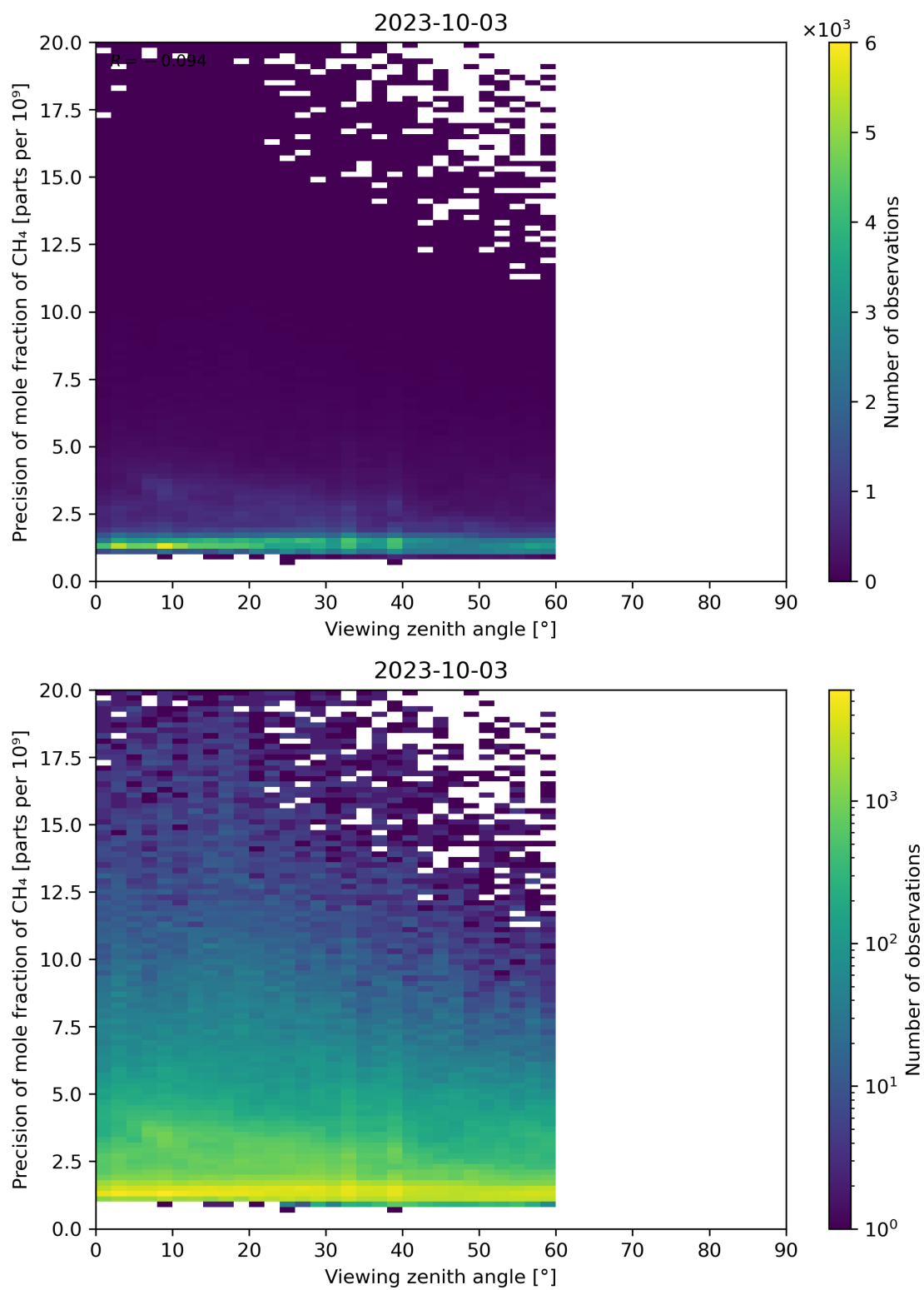
Figure 112: Scatter density plot of “Viewing zenith angle” against “Precision of mole fraction of CH 4 ” for 2023-10-02 to 2023-10-04.
