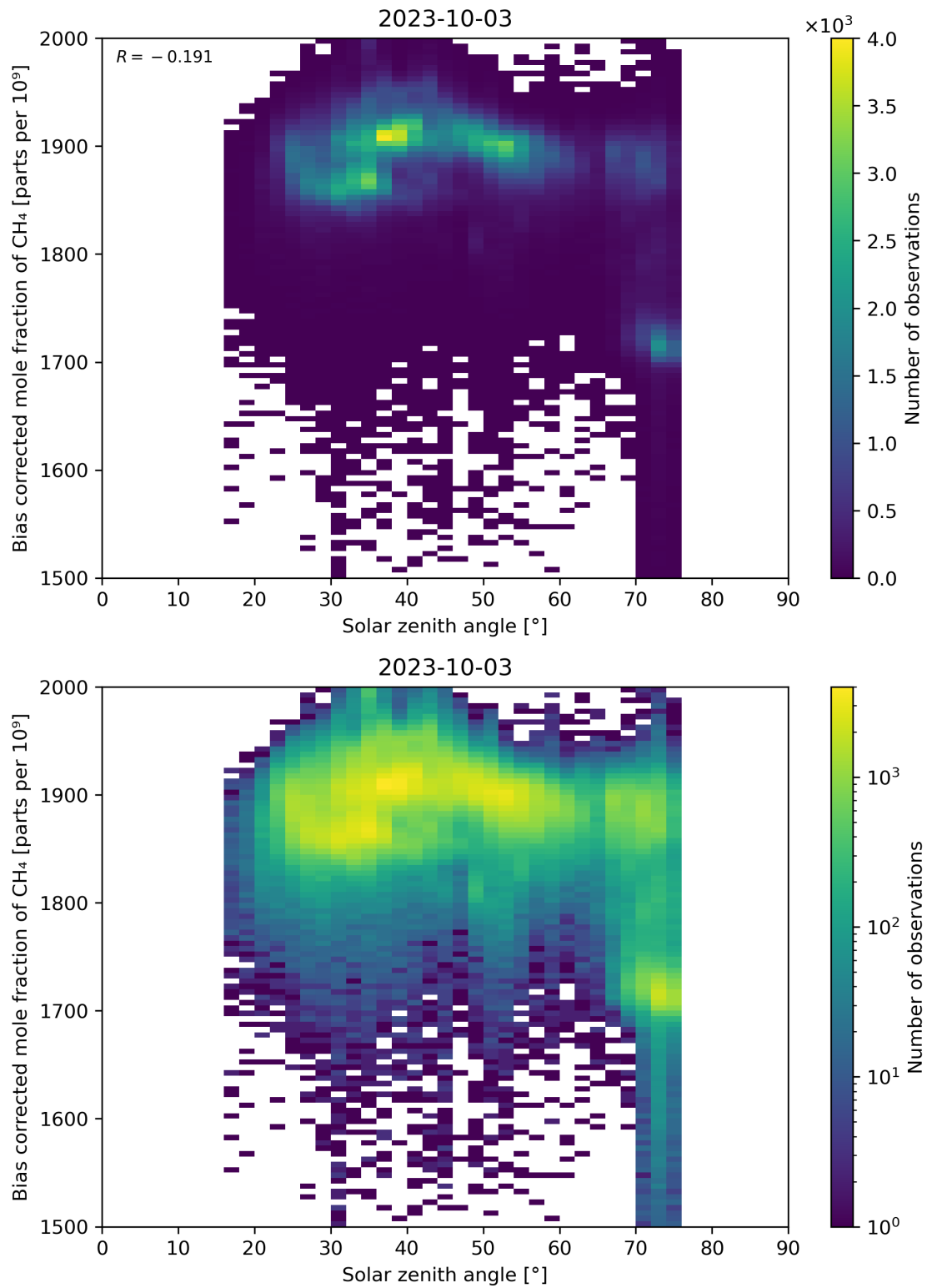
Figure 100: Scatter density plot of “Solar zenith angle” against “Bias corrected mole fraction of CH 4 ” for 2023-10-02 to 2023-10-04.
