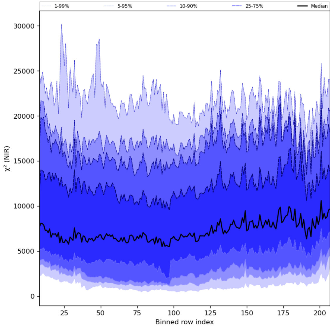
Figure 40: Along track statistics of " \chi^2 (NIR)" for 2023-10-02 to 2023-10-04
