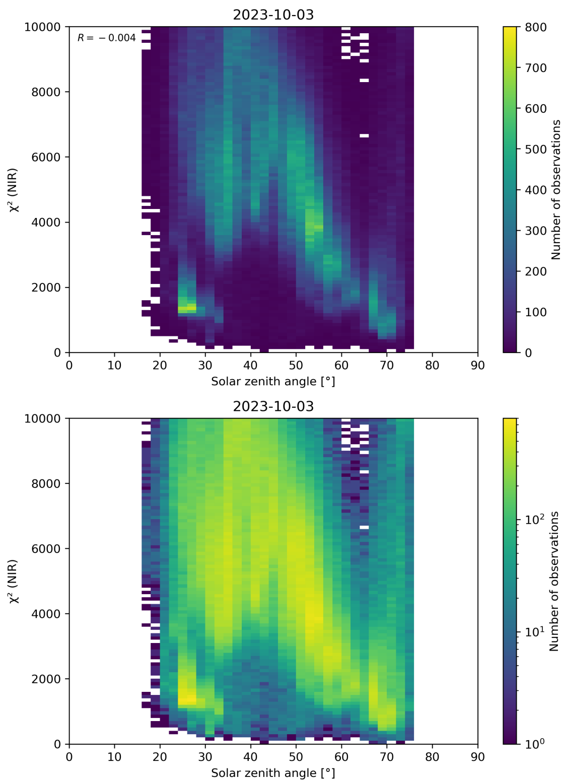
Figure 94: Scatter density plot of “Solar zenith angle” against “ \chi^2 (NIR)” for 2023-10-02 to 2023-10-04.
