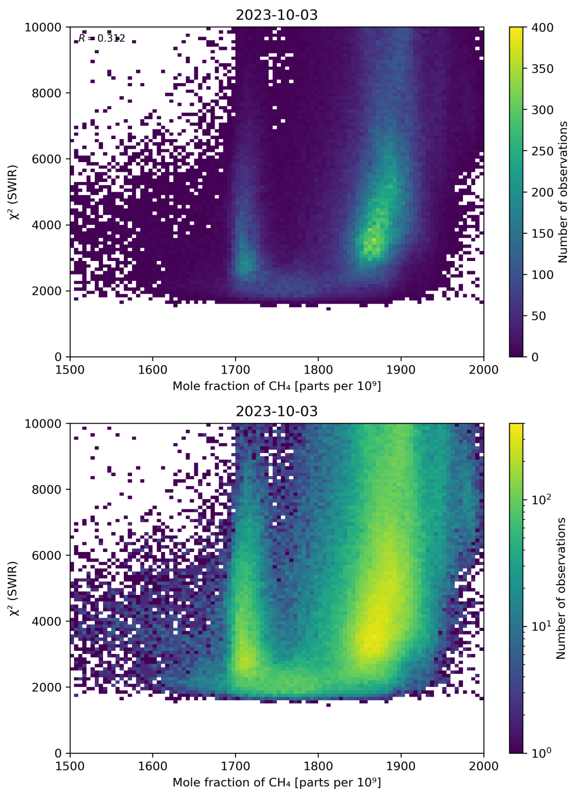
Figure 71: Scatter density plot of “Mole fraction of \text{CH}_4 ” against “ \chi^2 (SWIR)” for 2023-10-02 to 2023-10-04.
