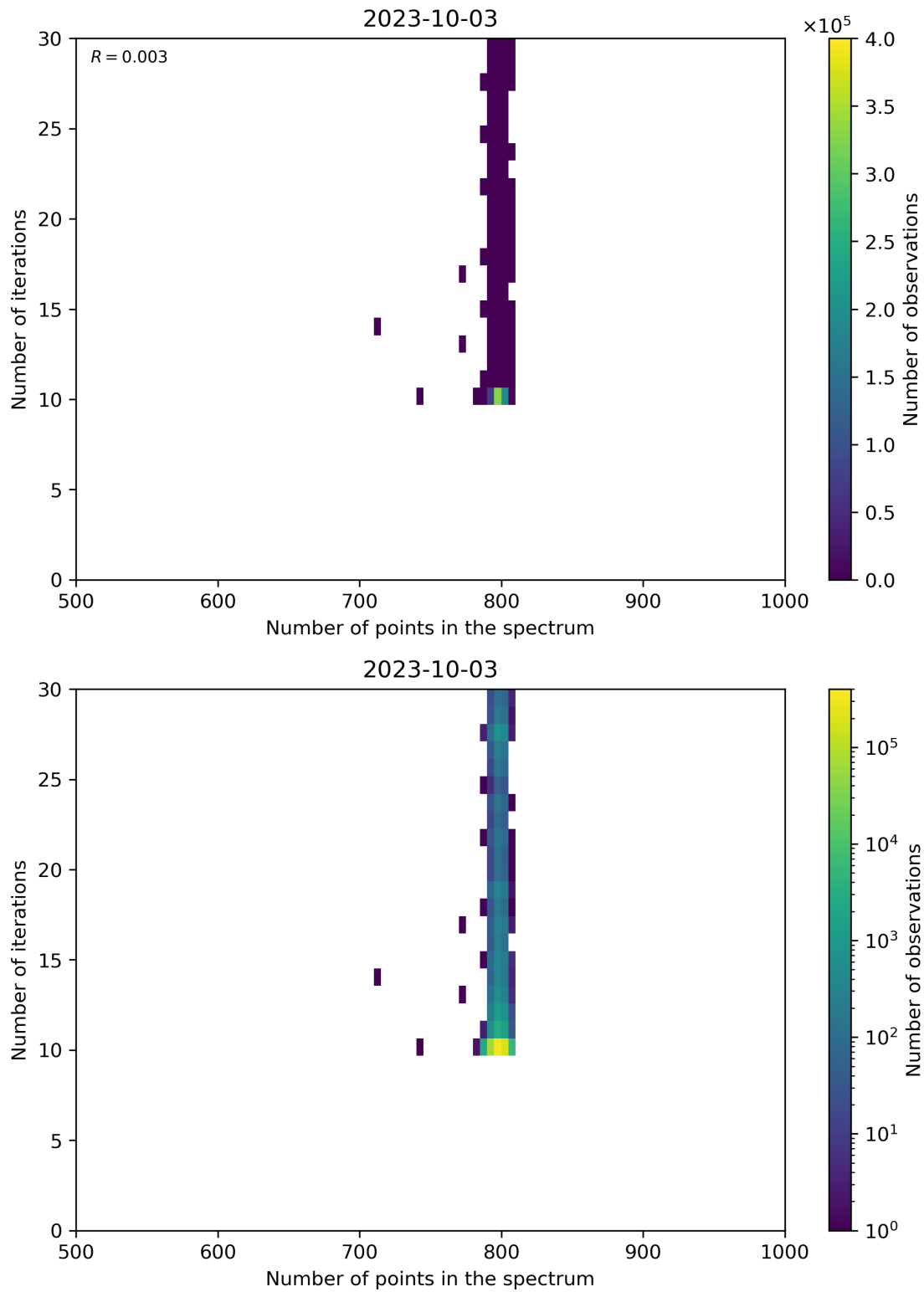
Figure 92: Scatter density plot of “Number of points in the spectrum” against “Number of iterations” for 2023-10-02 to 2023-10-04.
