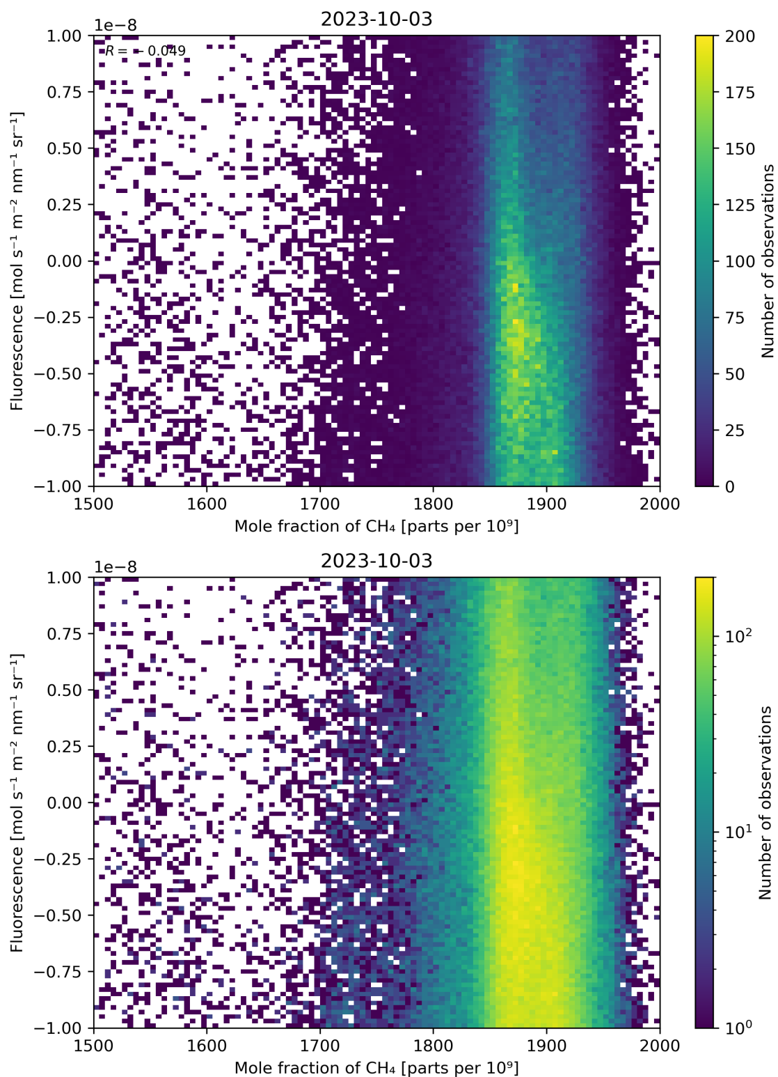
Figure 73: Scatter density plot of “Mole fraction of \text{CH}_4 ” against “Fluorescence” for 2023-10-02 to 2023-10-04.
