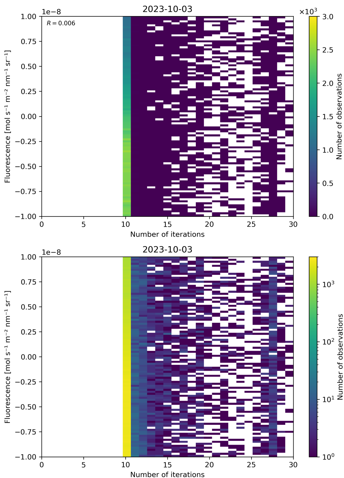
Figure 87: Scatter density plot of “Number of iterations” against “Fluorescence” for 2023-10-02 to 2023-10-04.
