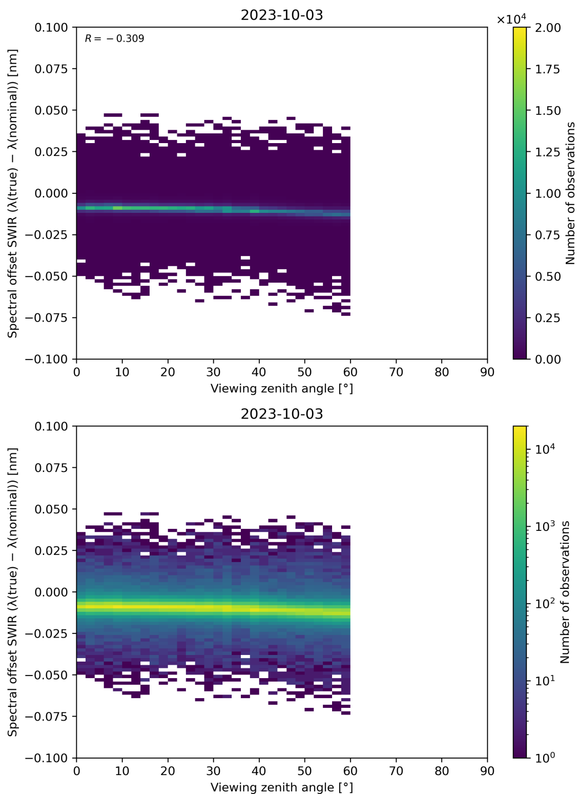
Figure 116: Scatter density plot of “Viewing zenith angle” against “Spectral offset SWIR ( \lambda(\text{true}) - \lambda(\text{nominal}) )” for 2023-10-02 to 2023-10-04.
