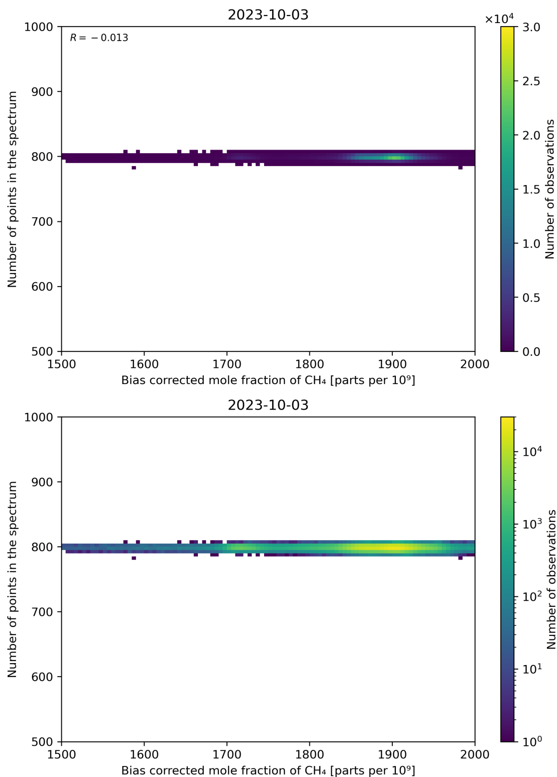
Figure 68: Scatter density plot of “Bias corrected mole fraction of CH 4 ” against “Number of points in the spectrum” for 2023-10-02 to 2023-10-04.
