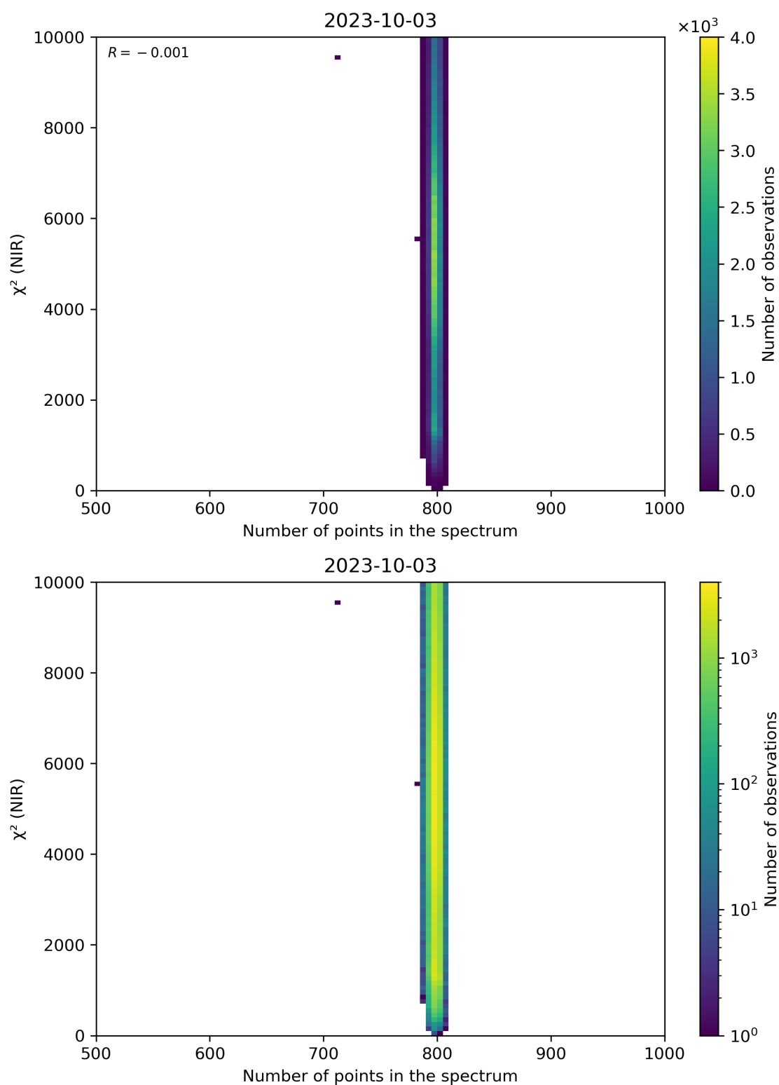
Figure 88: Scatter density plot of “Number of points in the spectrum” against “ \chi^2 (NIR)” for 2023-10-02 to 2023-10-04.
