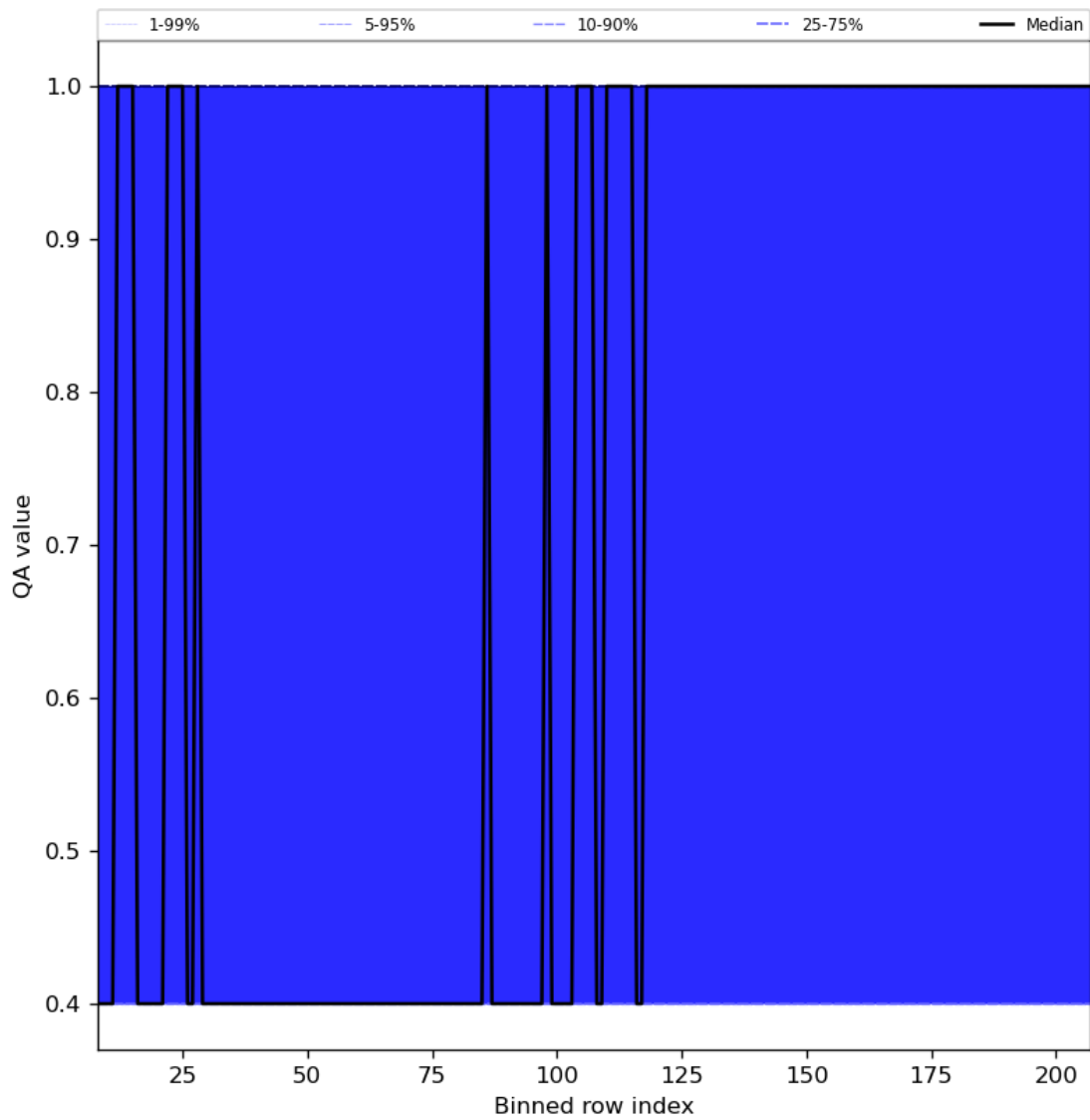
Figure 33: Along track statistics of “QA value” for 2023-10-02 to 2023-10-04
