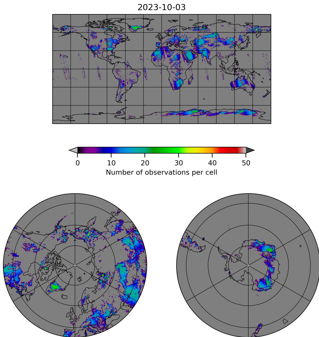
Figure 10: Map of the number of observations for 2023-10-02 to 2023-10-04
