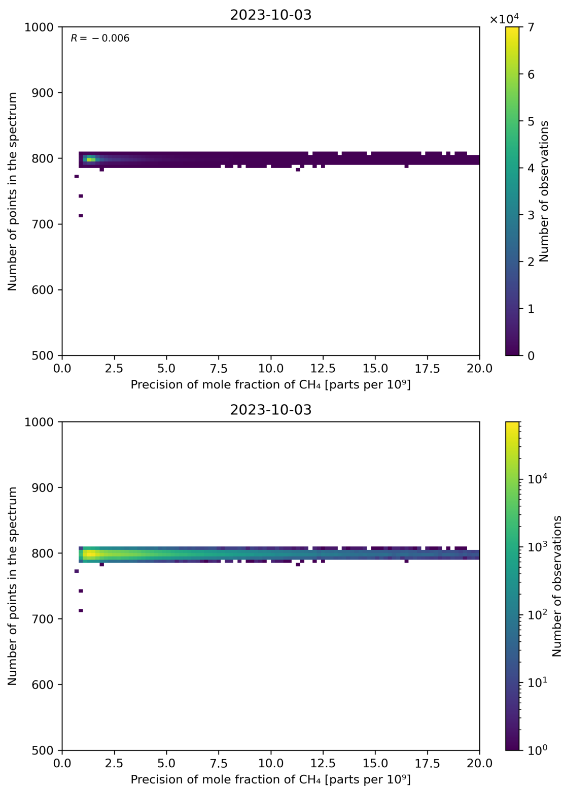
Figure 84: Scatter density plot of “Precision of mole fraction of CH 4 ” against “Number of points in the spectrum” for 2023-10-02 to 2023-10-04.
