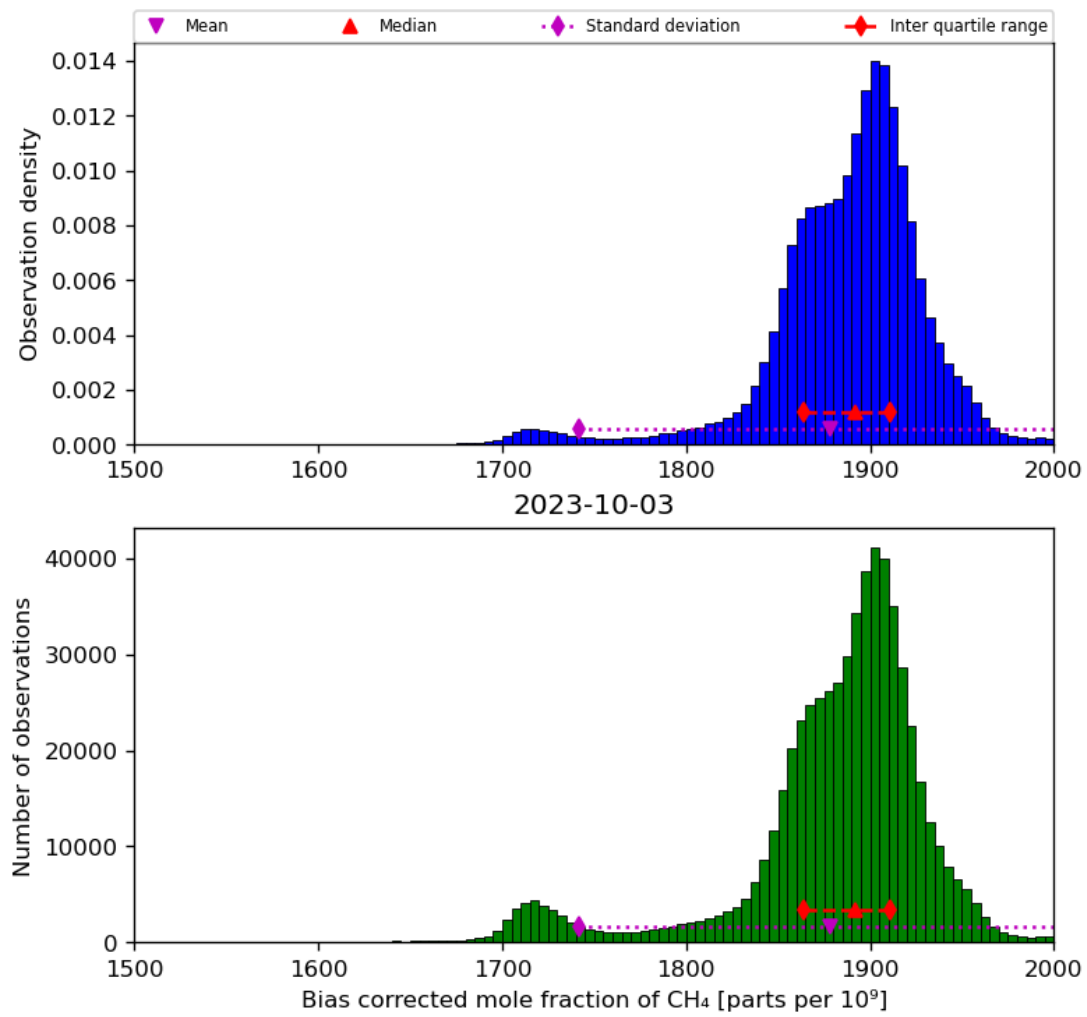
Figure 25: Histogram of “Bias corrected mole fraction of CH 4 ” for 2023-10-02 to 2023-10-04
