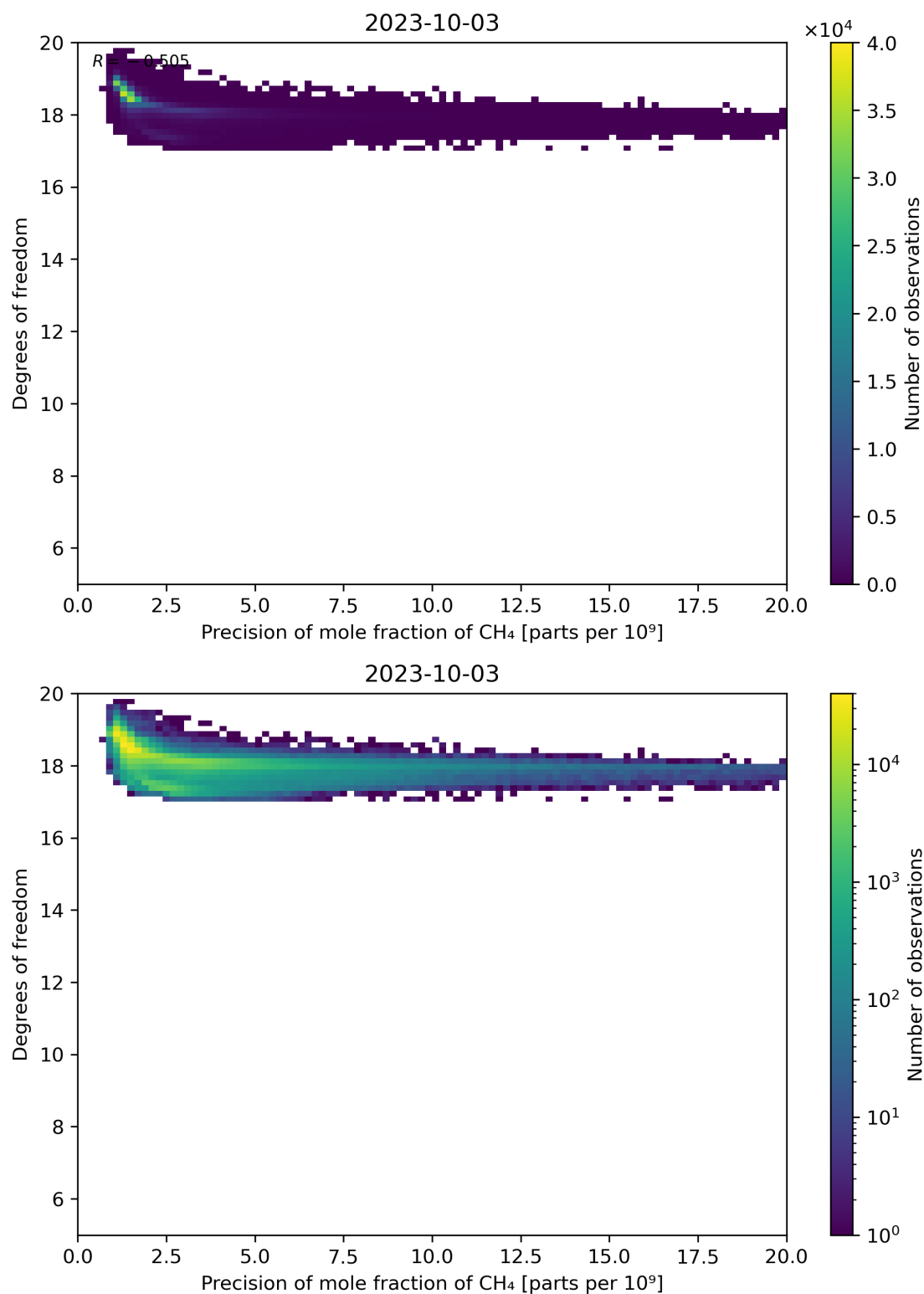
Figure 80: Scatter density plot of “Precision of mole fraction of CH 4 ” against “Degrees of freedom” for 2023-10-02 to 2023-10-04.
