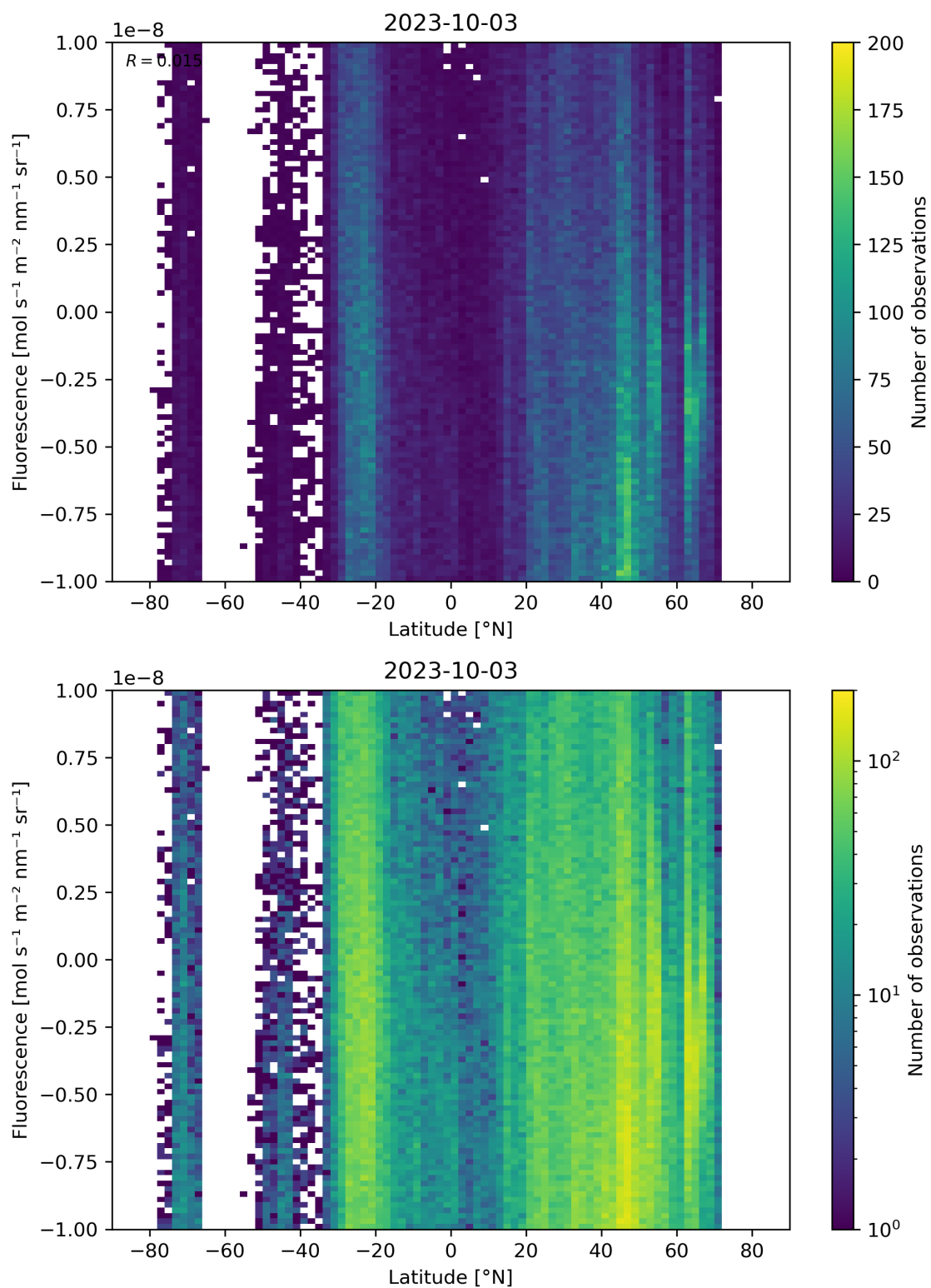
Figure 56: Scatter density plot of “Latitude” against “Fluorescence” for 2023-10-02 to 2023-10-04.
