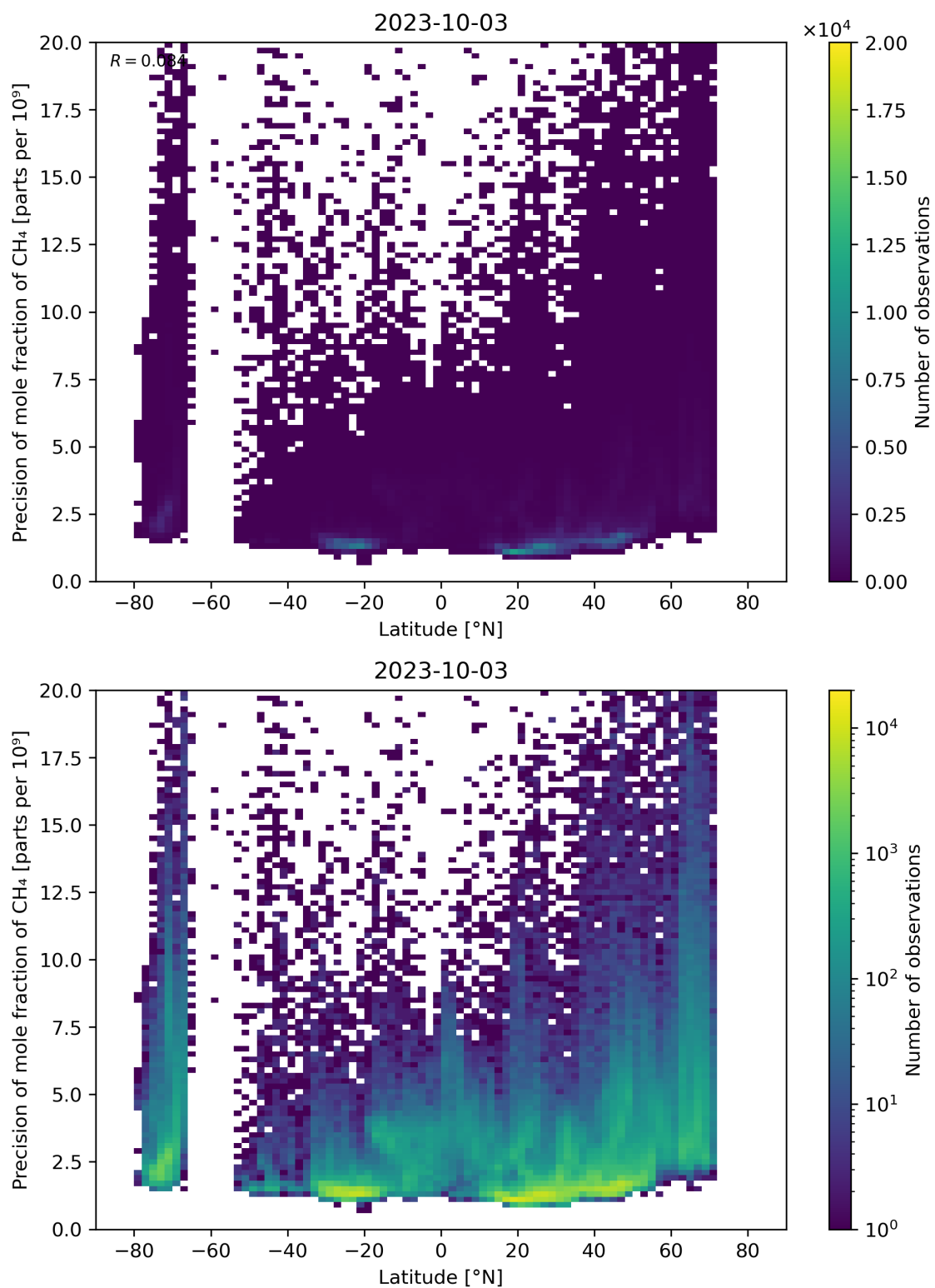
Figure 59: Scatter density plot of “Latitude” against “Precision of mole fraction of \text{CH}_4 ” for 2023-10-02 to 2023-10-04.
