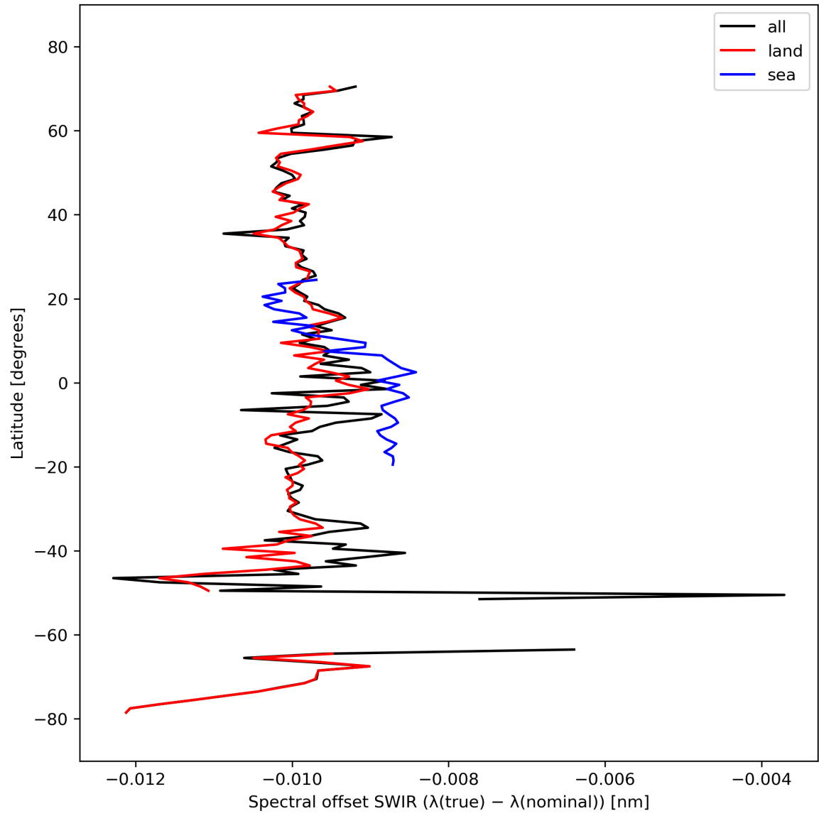
Figure 16: Zonal average of “Spectral offset SWIR ( \lambda(\text{true}) - \lambda(\text{nominal}) )” for 2023-10-03 to 2023-10-05.
