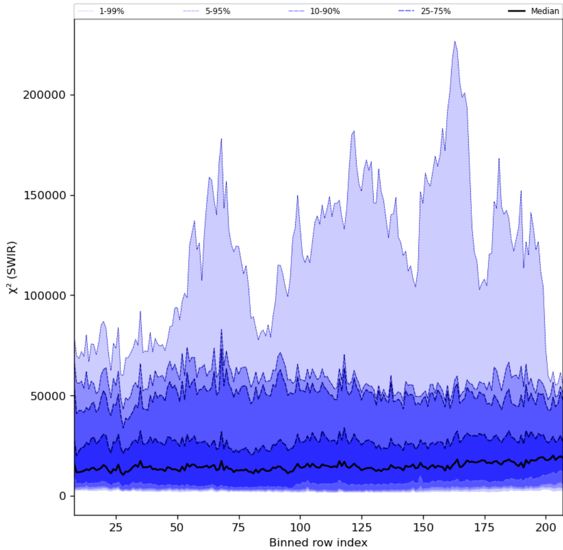
Figure 39: Along track statistics of " \chi^2 (SWIR)" for 2023-10-03 to 2023-10-05
