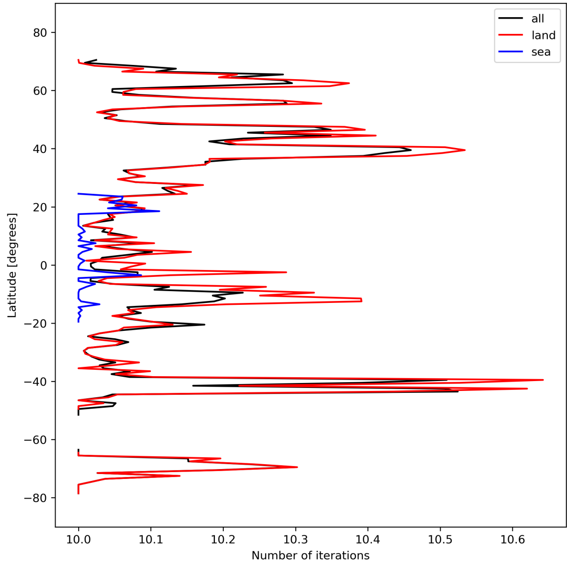
Figure 20: Zonal average of “Number of iterations” for 2023-10-03 to 2023-10-05.
