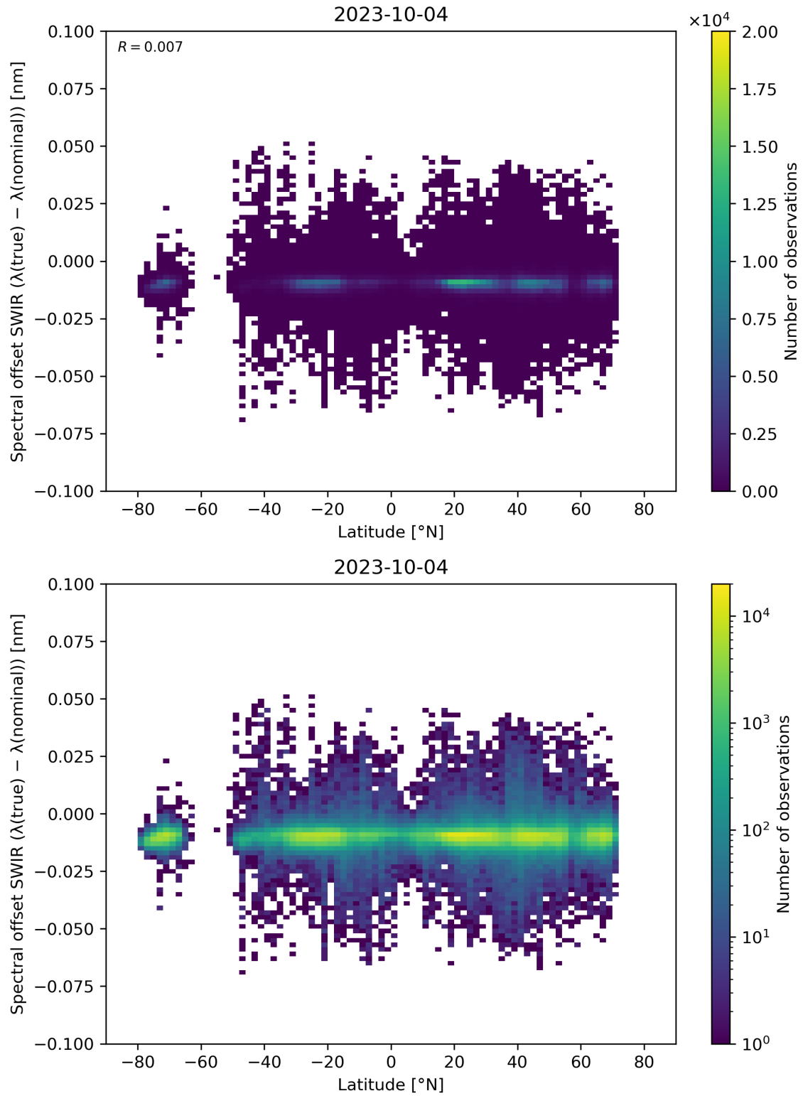
Figure 62: Scatter density plot of “Latitude” against “Spectral offset SWIR ( \lambda(\text{true}) - \lambda(\text{nominal}) )” for 2023-10-03 to 2023-10-05.
