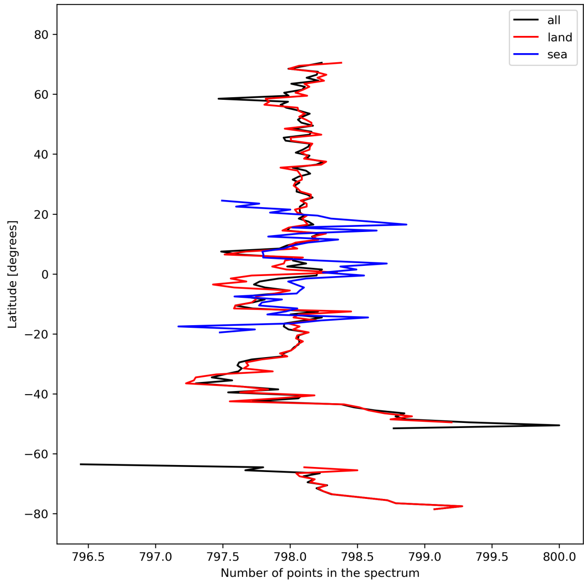
Figure 15: Zonal average of “Number of points in the spectrum” for 2023-10-03 to 2023-10-05.
