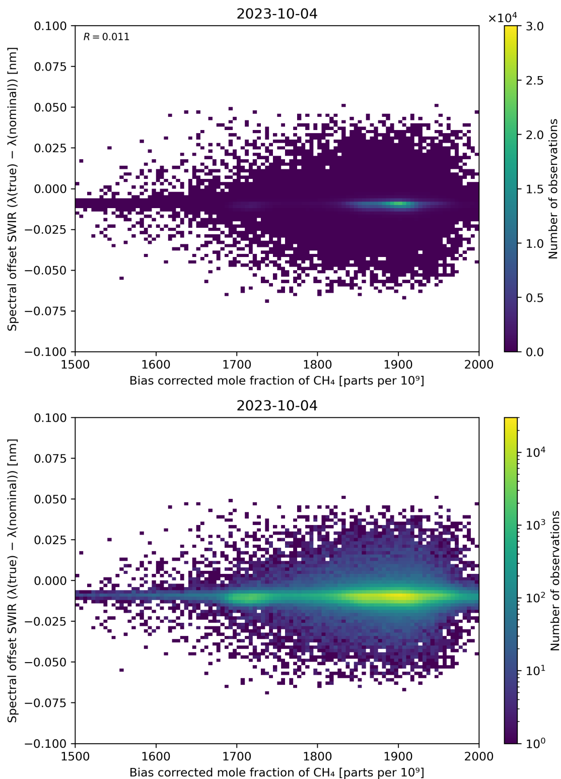
Figure 69: Scatter density plot of “Bias corrected mole fraction of \text{CH}_4 ” against “Spectral offset SWIR ( \lambda(\text{true}) - \lambda(\text{nominal}) )” for 2023-10-03 to 2023-10-05.
