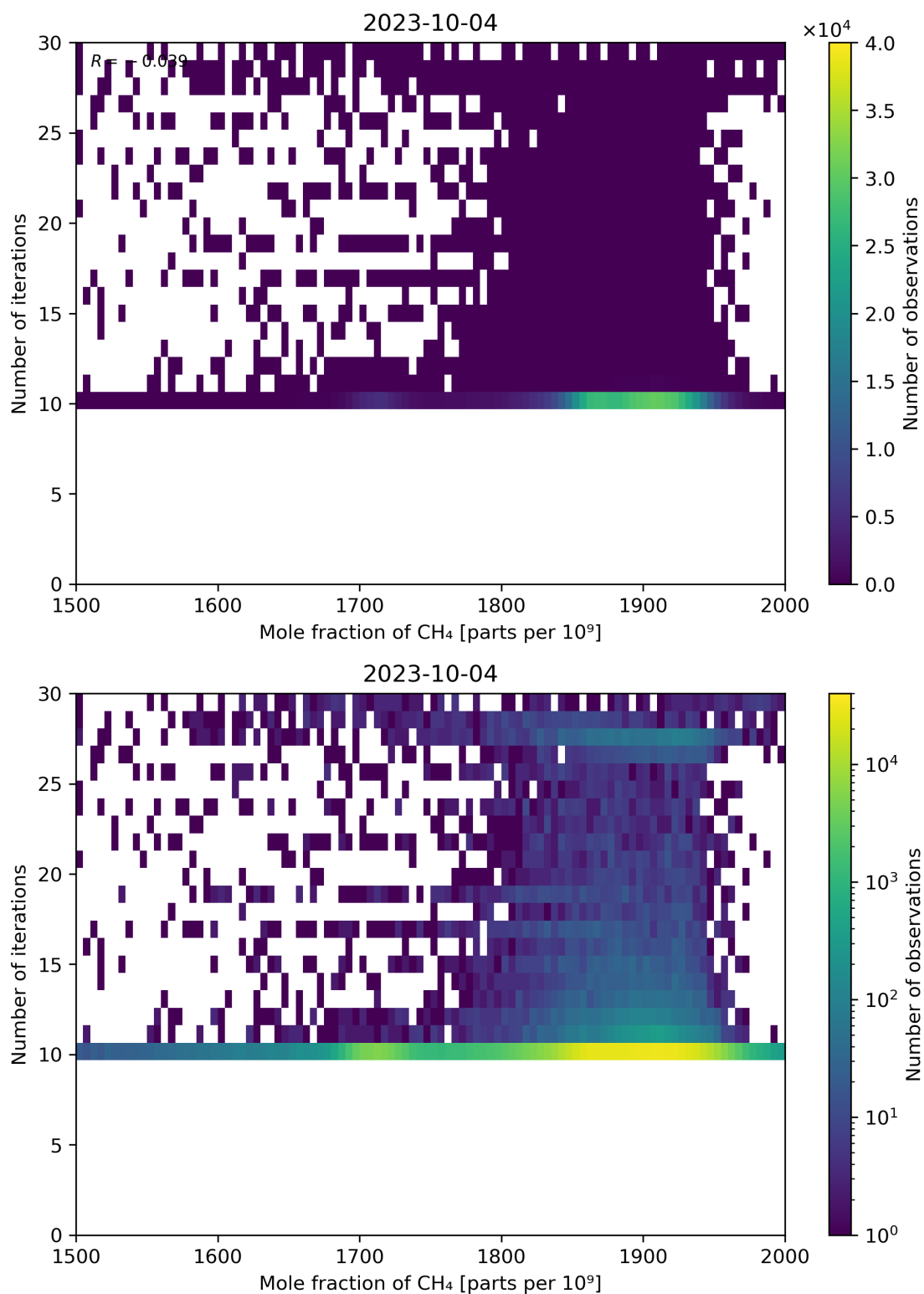
Figure 76: Scatter density plot of “Mole fraction of CH 4 ” against “Number of iterations” for 2023-10-03 to 2023-10-05.
