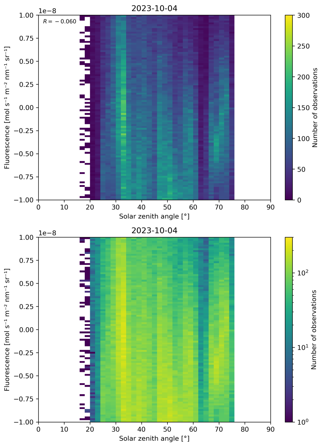
Figure 97: Scatter density plot of “Solar zenith angle” against “Fluorescence” for 2023-10-03 to 2023-10-05.
