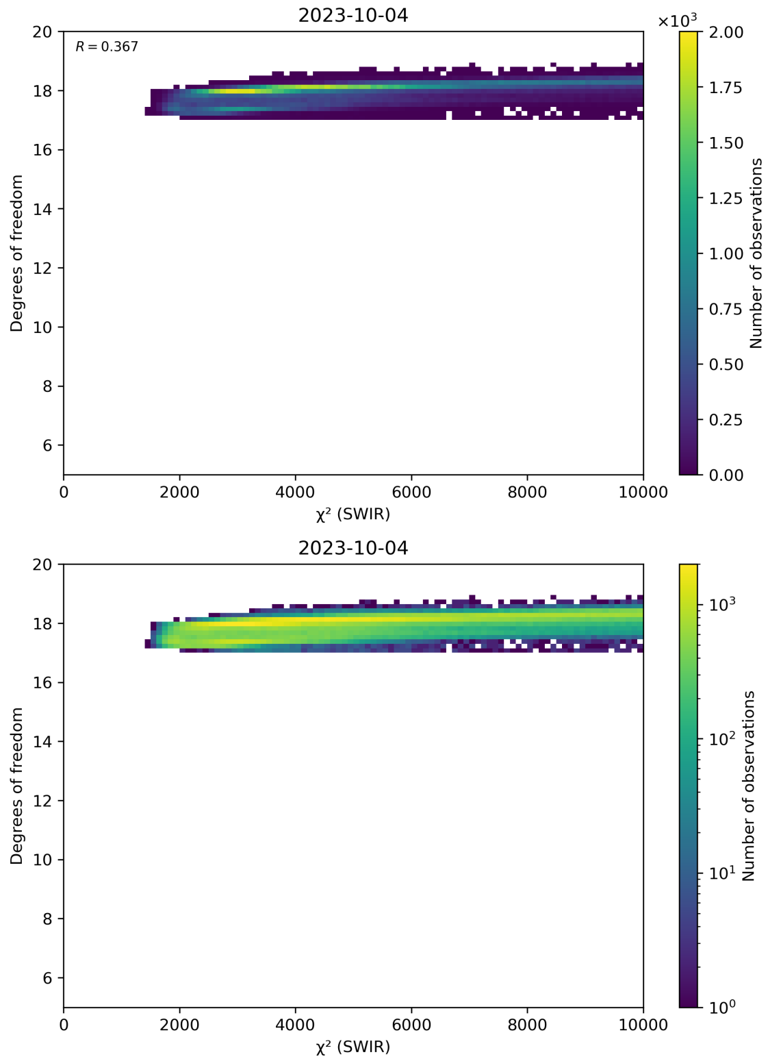
Figure 48: Scatter density plot of “ \chi^2 (SWIR)” against “Degrees of freedom” for 2023-10-03 to 2023-10-05.
