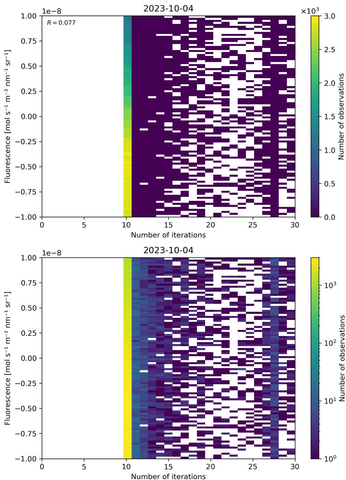
Figure 87: Scatter density plot of “Number of iterations” against “Fluorescence” for 2023-10-03 to 2023-10-05.
