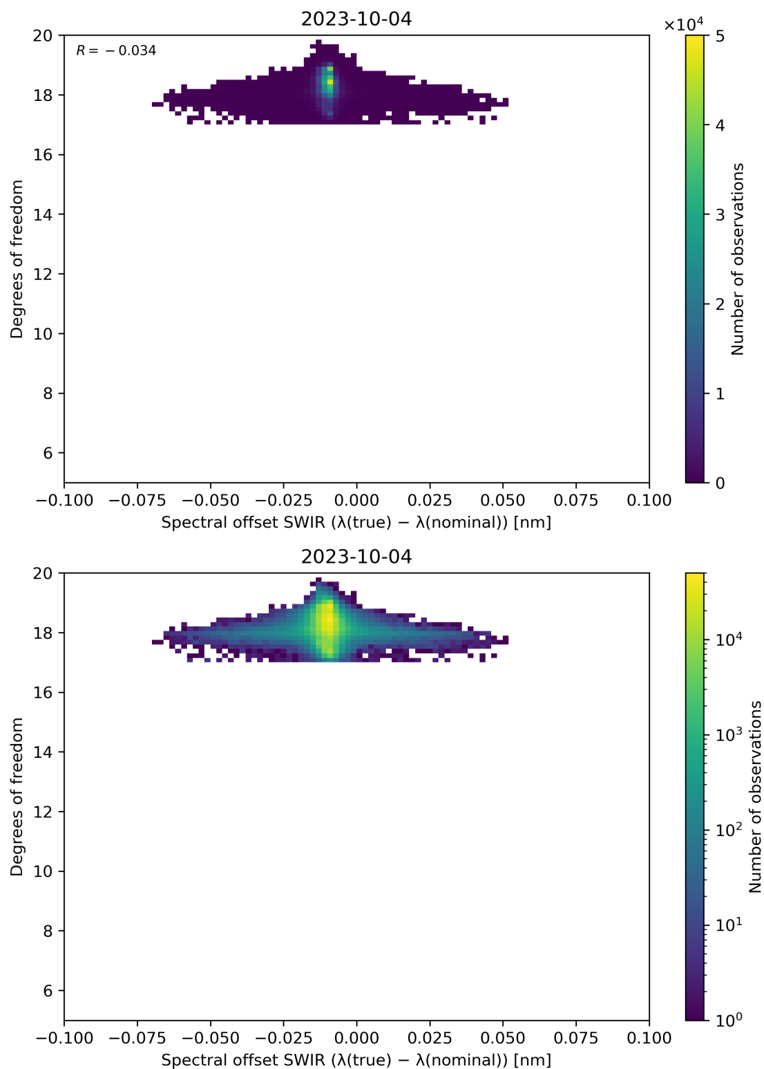
Figure 119: Scatter density plot of “Spectral offset SWIR ( \lambda(\text{true}) - \lambda(\text{nominal}) )” against “Degrees of freedom” for 2023-10-03 to 2023-10-05.
