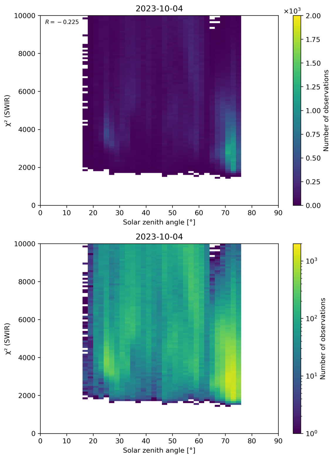
Figure 95: Scatter density plot of “Solar zenith angle” against “ \chi^2 (SWIR)” for 2023-10-03 to 2023-10-05.
