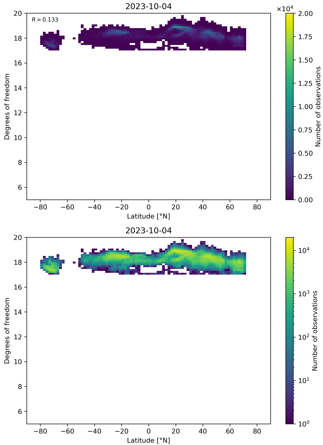
Figure 55: Scatter density plot of “Latitude” against “Degrees of freedom” for 2023-10-03 to 2023-10-05.
