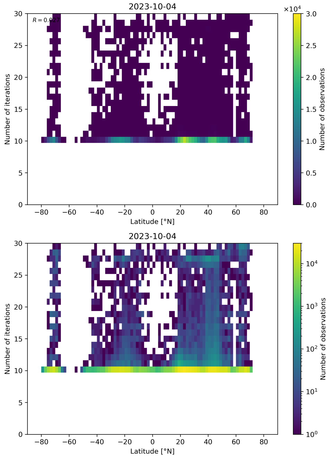
Figure 60: Scatter density plot of “Latitude” against “Number of iterations” for 2023-10-03 to 2023-10-05.
