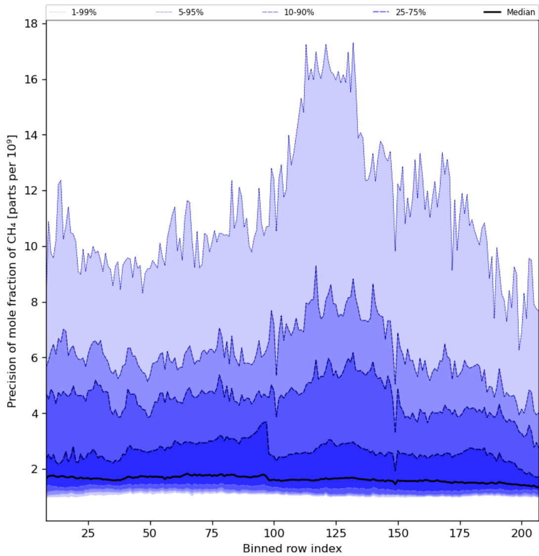
Figure 35: Along track statistics of “Precision of mole fraction of CH 4 ” for 2023-10-03 to 2023-10-05
