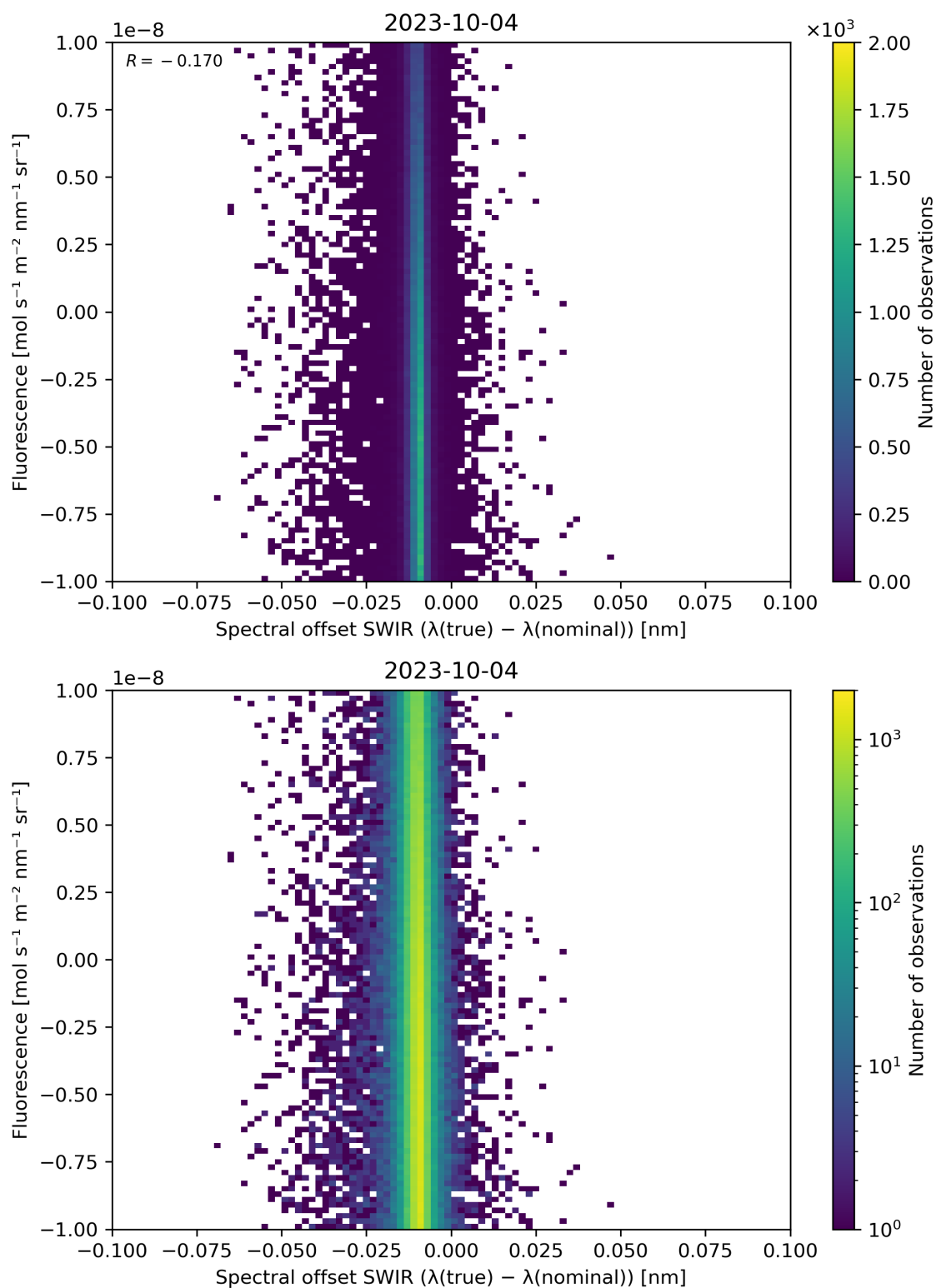
Figure 120: Scatter density plot of “Spectral offset SWIR ( \lambda(\text{true}) - \lambda(\text{nominal}) )” against “Fluorescence” for 2023-10-03 to 2023-10-05.
