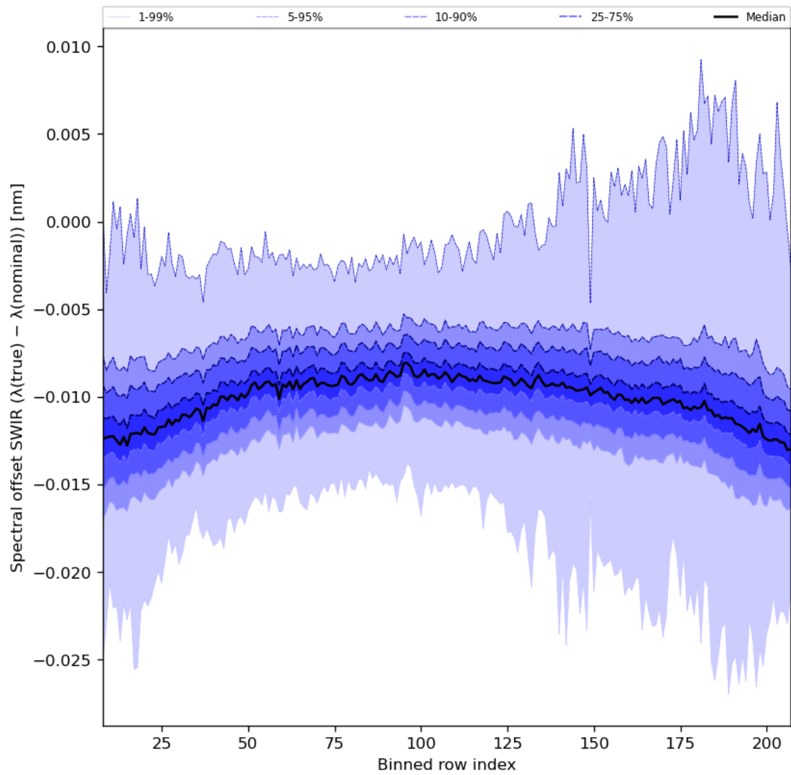
Figure 38: Along track statistics of “Spectral offset SWIR ( \lambda(\text{true}) - \lambda(\text{nominal}) )” for 2023-10-03 to 2023-10-05
