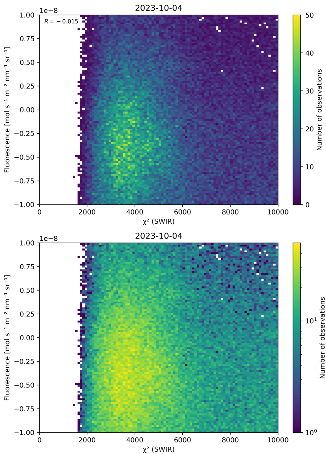
Figure 49: Scatter density plot of “ \chi^2 (SWIR)” against “Fluorescence” for 2023-10-03 to 2023-10-05.
