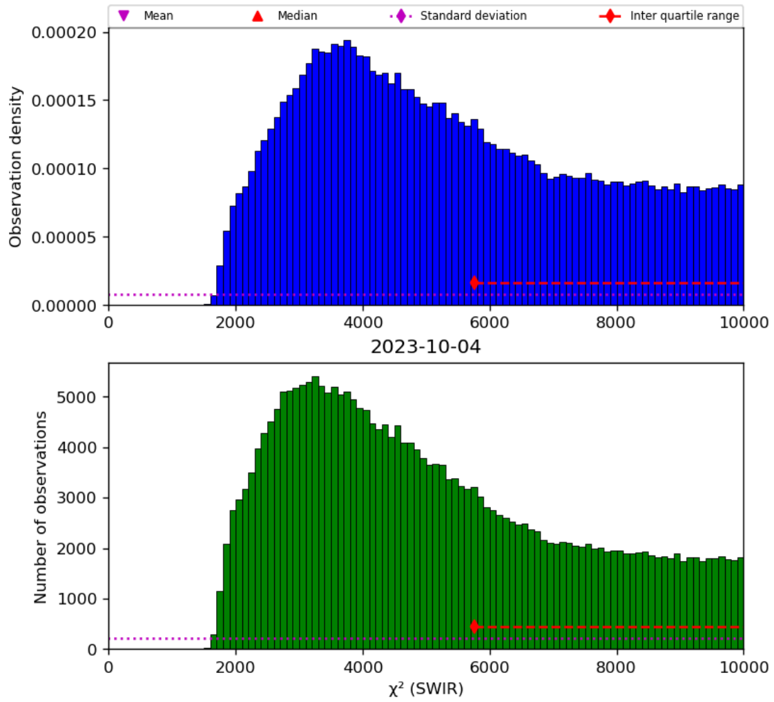
Figure 28: Histogram of “ \chi^2 (SWIR)” for 2023-10-03 to 2023-10-05
