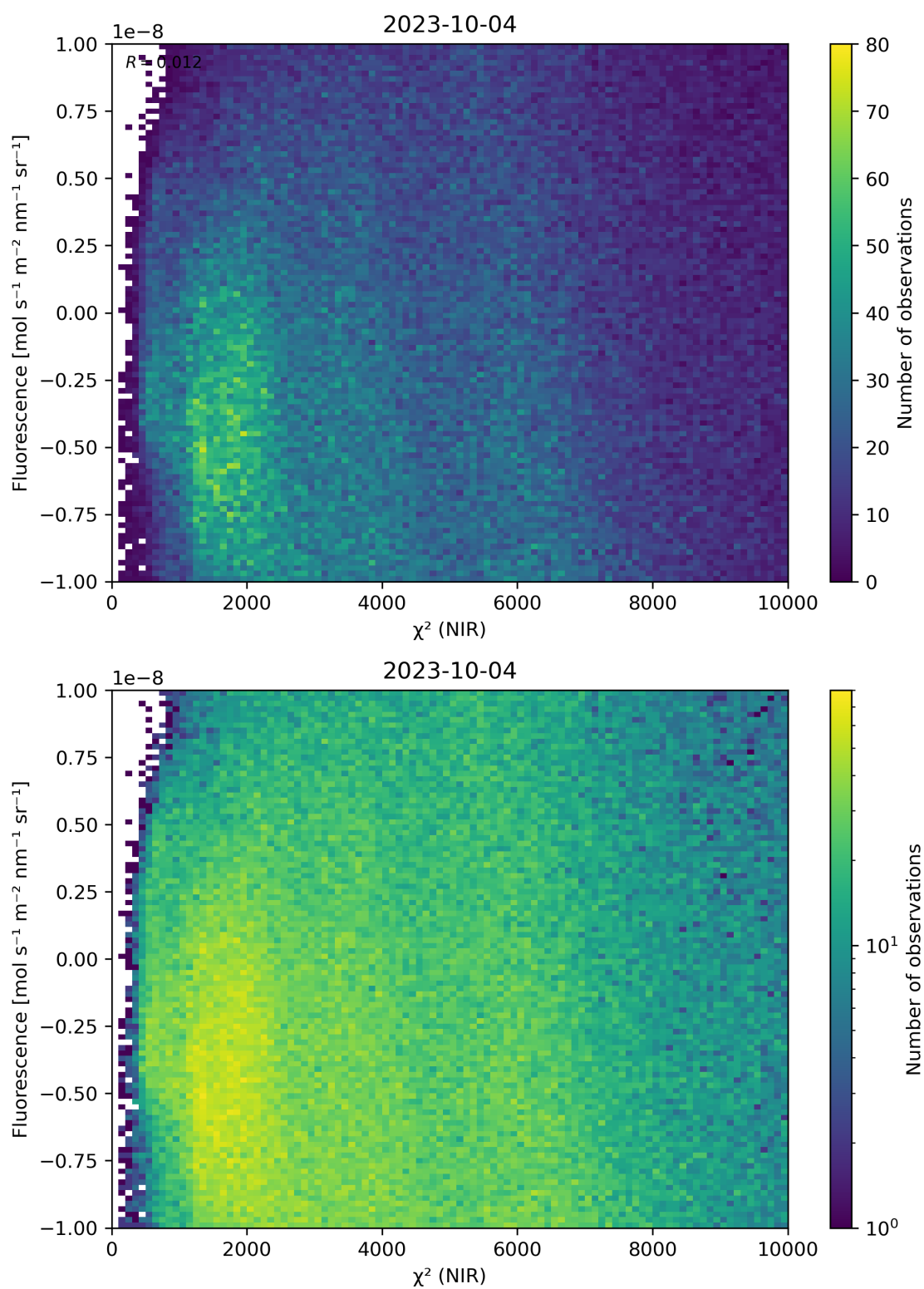
Figure 45: Scatter density plot of “ \chi^2 (NIR)” against “Fluorescence” for 2023-10-03 to 2023-10-05.
