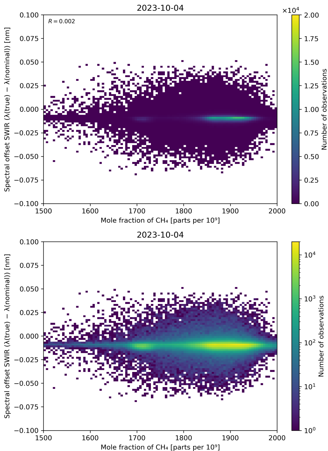
Figure 86: Scatter density plot of “Mole fraction of CH 4 ” against “Spectral offset SWIR ( \lambda(\text{true}) - \lambda(\text{nominal}) )” for 2023-10-03 to 2023-10-05.
