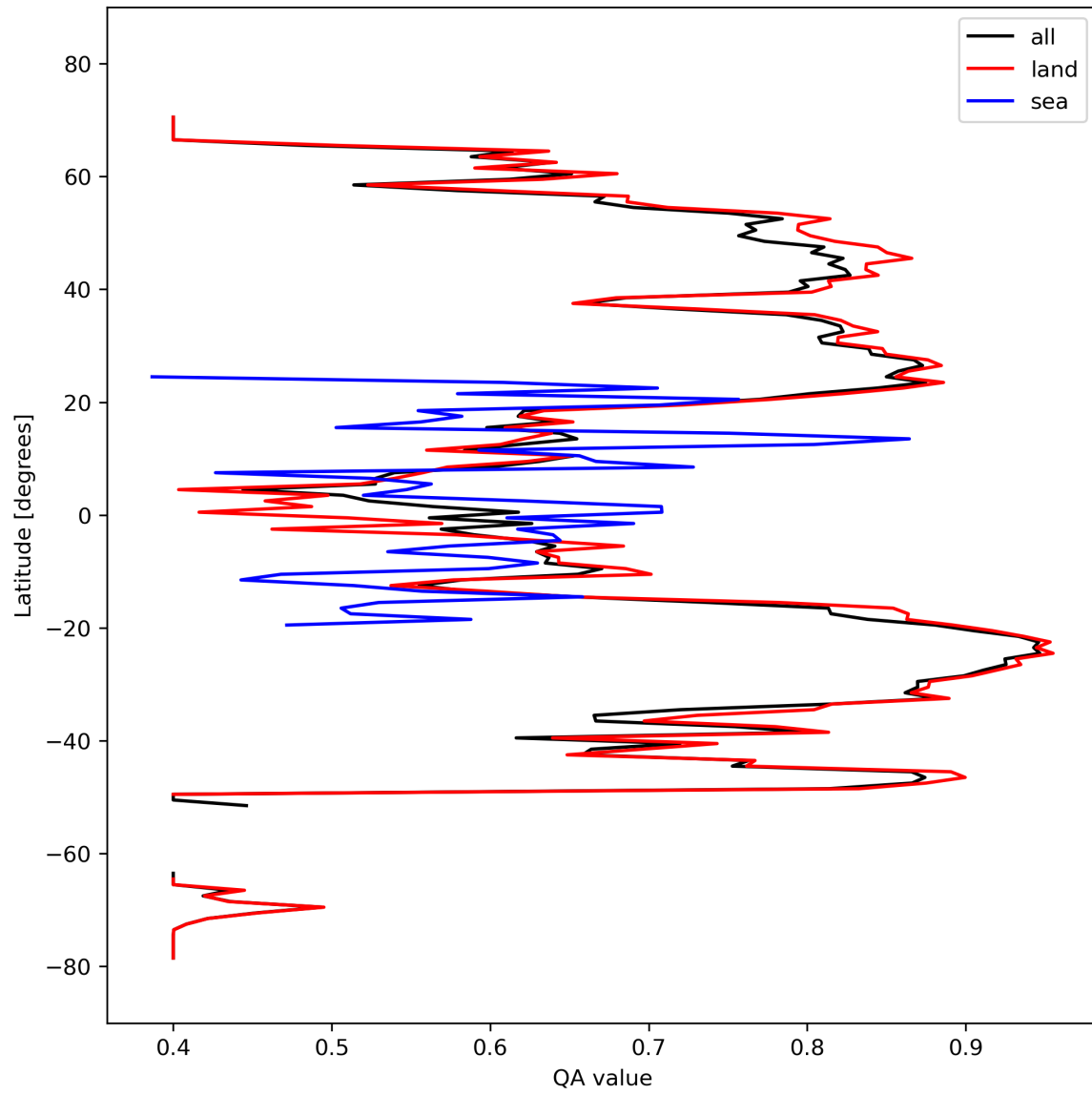
Figure 11: Zonal average of “QA value” for 2023-10-03 to 2023-10-05.
