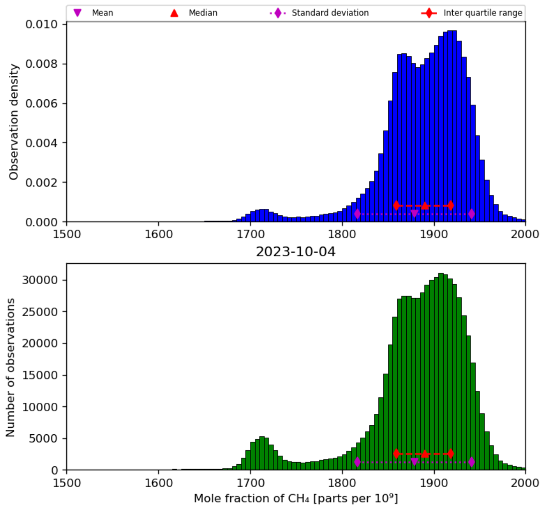
Figure 23: Histogram of “Mole fraction of CH 4 ” for 2023-10-03 to 2023-10-05
