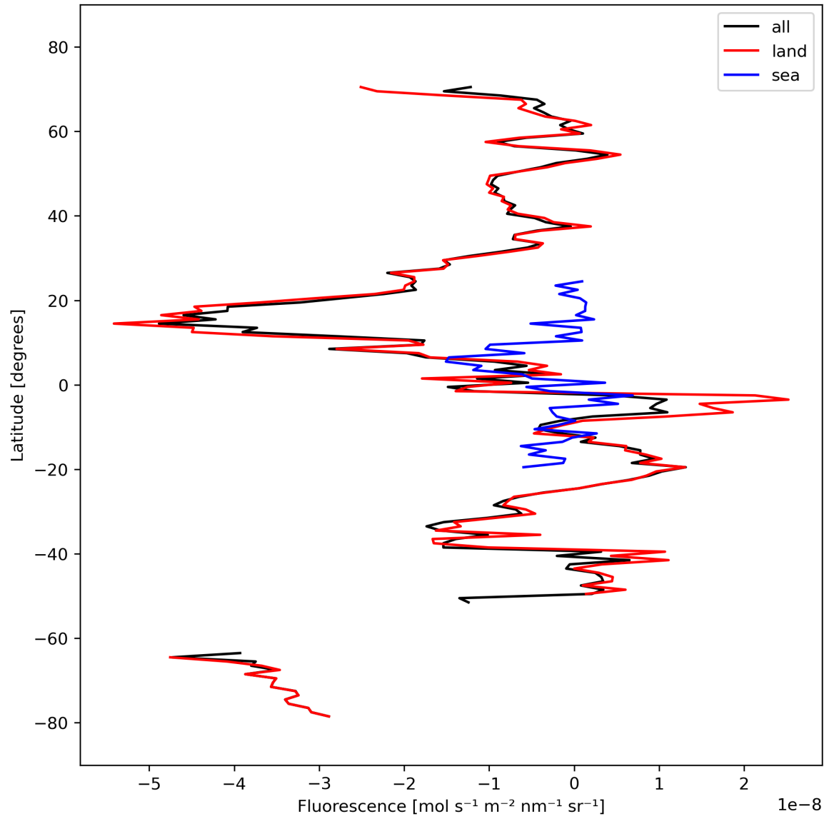
Figure 21: Zonal average of “Fluorescence” for 2023-10-03 to 2023-10-05.
