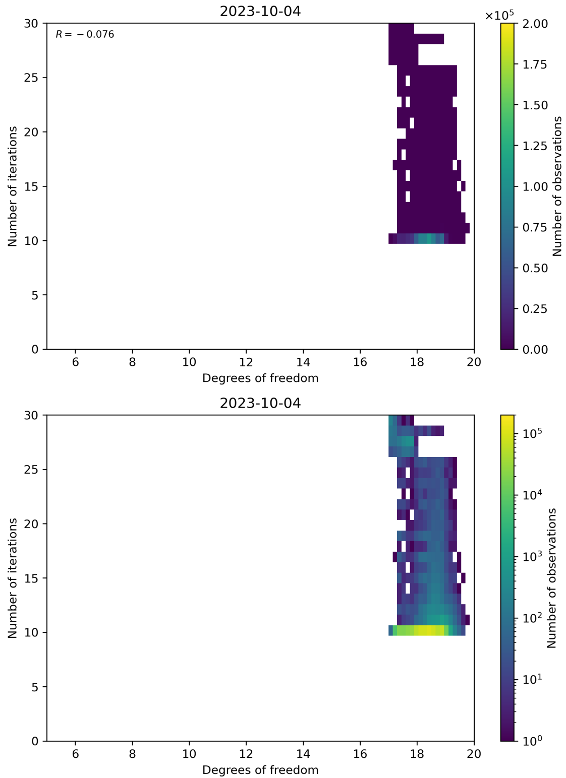
Figure 52: Scatter density plot of “Degrees of freedom” against “Number of iterations” for 2023-10-03 to 2023-10-05.
