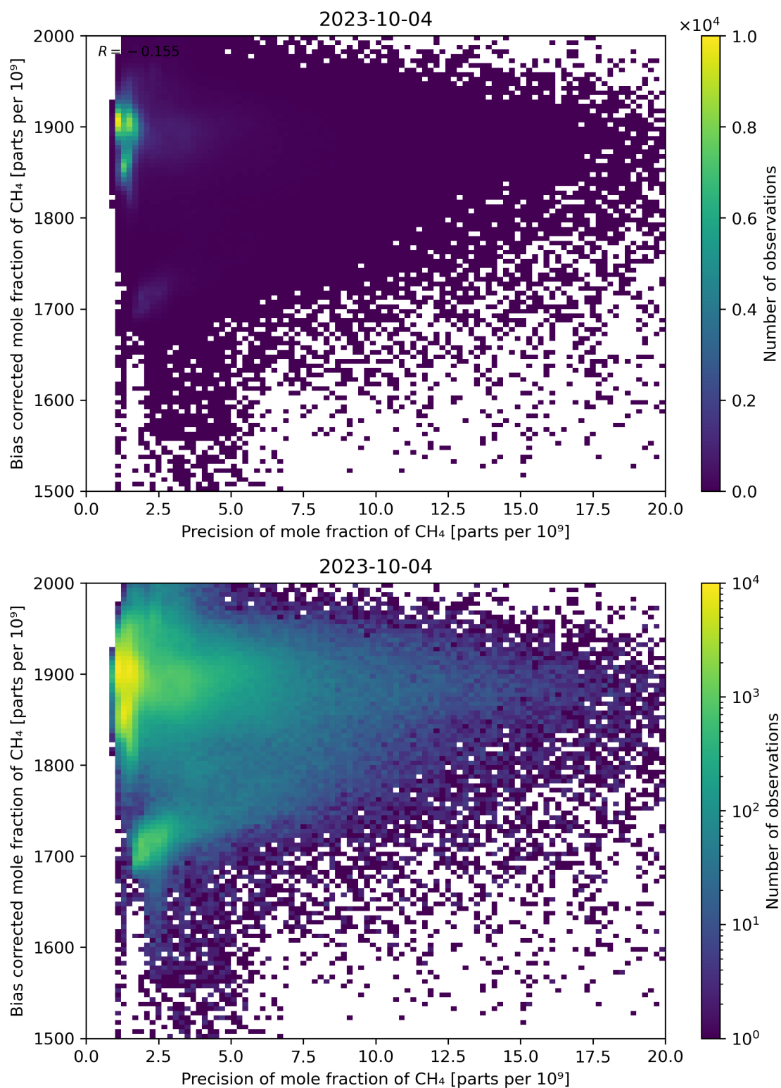
Figure 82: Scatter density plot of “Precision of mole fraction of CH 4 ” against “Bias corrected mole fraction of CH 4 ” for 2023-10-03 to 2023-10-05.
