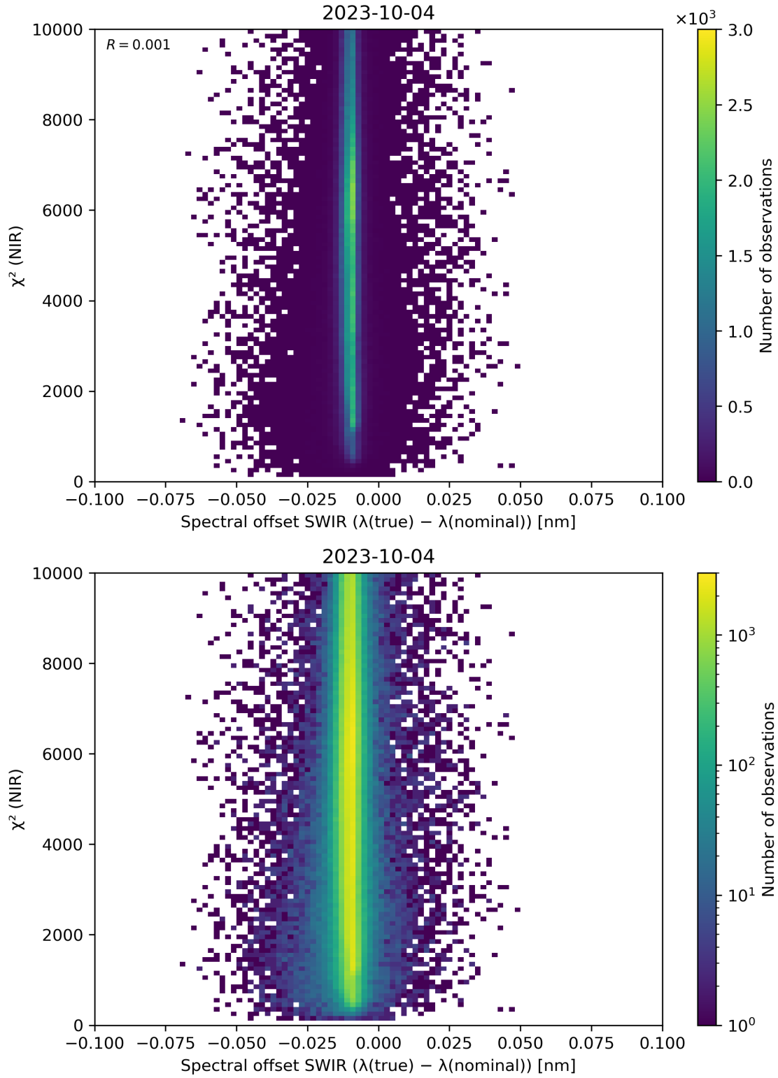
Figure 117: Scatter density plot of “Spectral offset SWIR ( \lambda(\text{true}) - \lambda(\text{nominal}) )” against “ \chi^2 (NIR)” for 2023-10-03 to 2023-10-05.
