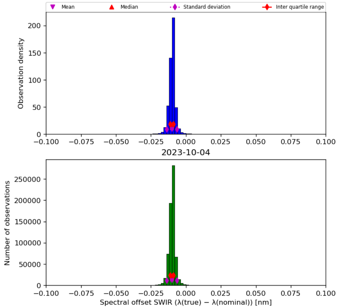
Figure 27: Histogram of “Spectral offset SWIR ( \lambda(\text{true}) - \lambda(\text{nominal}) )” for 2023-10-03 to 2023-10-05
