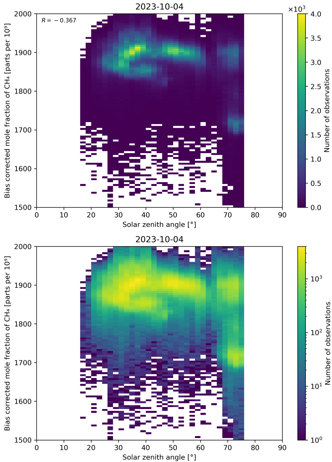
Figure 100: Scatter density plot of “Solar zenith angle” against “Bias corrected mole fraction of \text{CH}_4 ” for 2023-10-03 to 2023-10-05.
