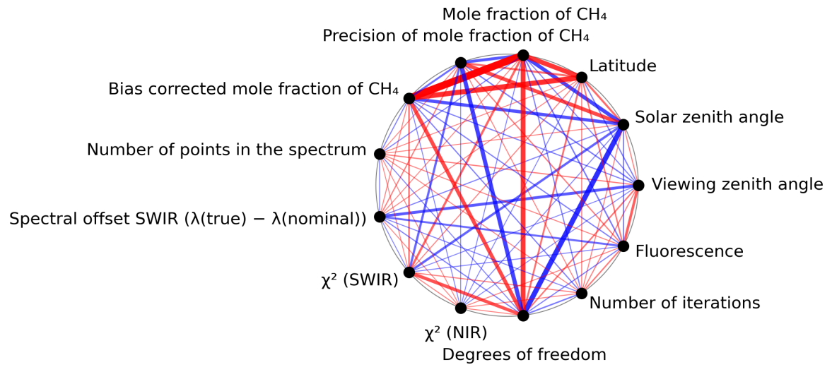
Figure 1: Map of correlation graph for 2023-10-03 to 2023-10-05.
