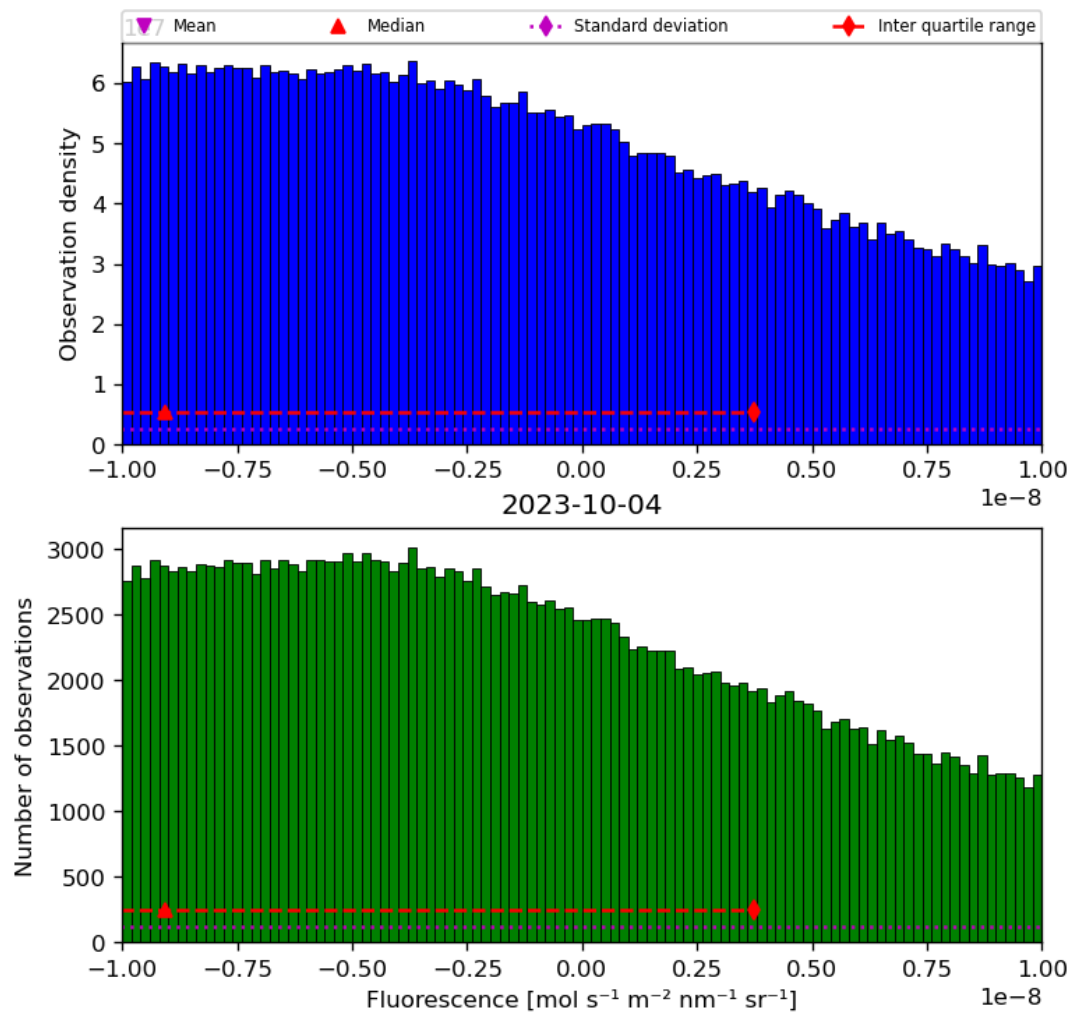
Figure 32: Histogram of “Fluorescence” for 2023-10-03 to 2023-10-05
