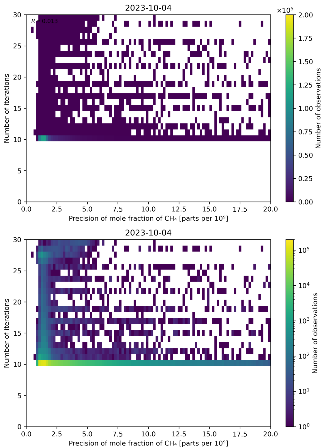
Figure 83: Scatter density plot of “Precision of mole fraction of CH 4 ” against “Number of iterations” for 2023-10-03 to 2023-10-05.
