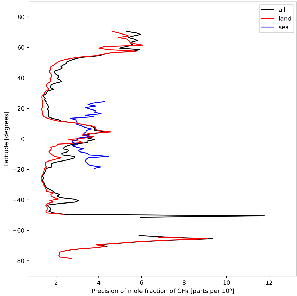
Figure 13: Zonal average of “Precision of mole fraction of CH 4 ” for 2023-10-03 to 2023-10-05.
