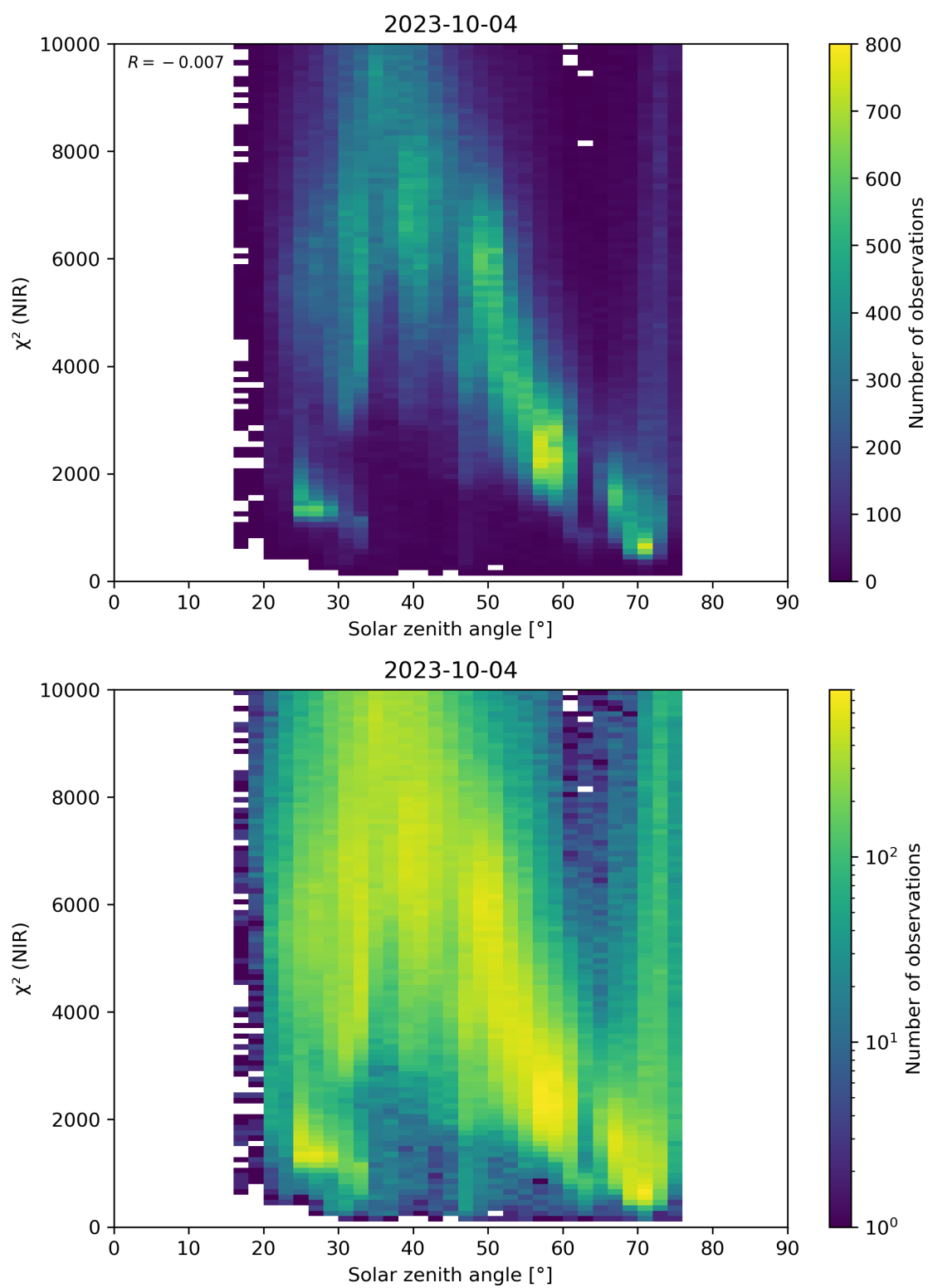
Figure 94: Scatter density plot of “Solar zenith angle” against “ \chi^2 (NIR)” for 2023-10-03 to 2023-10-05.
