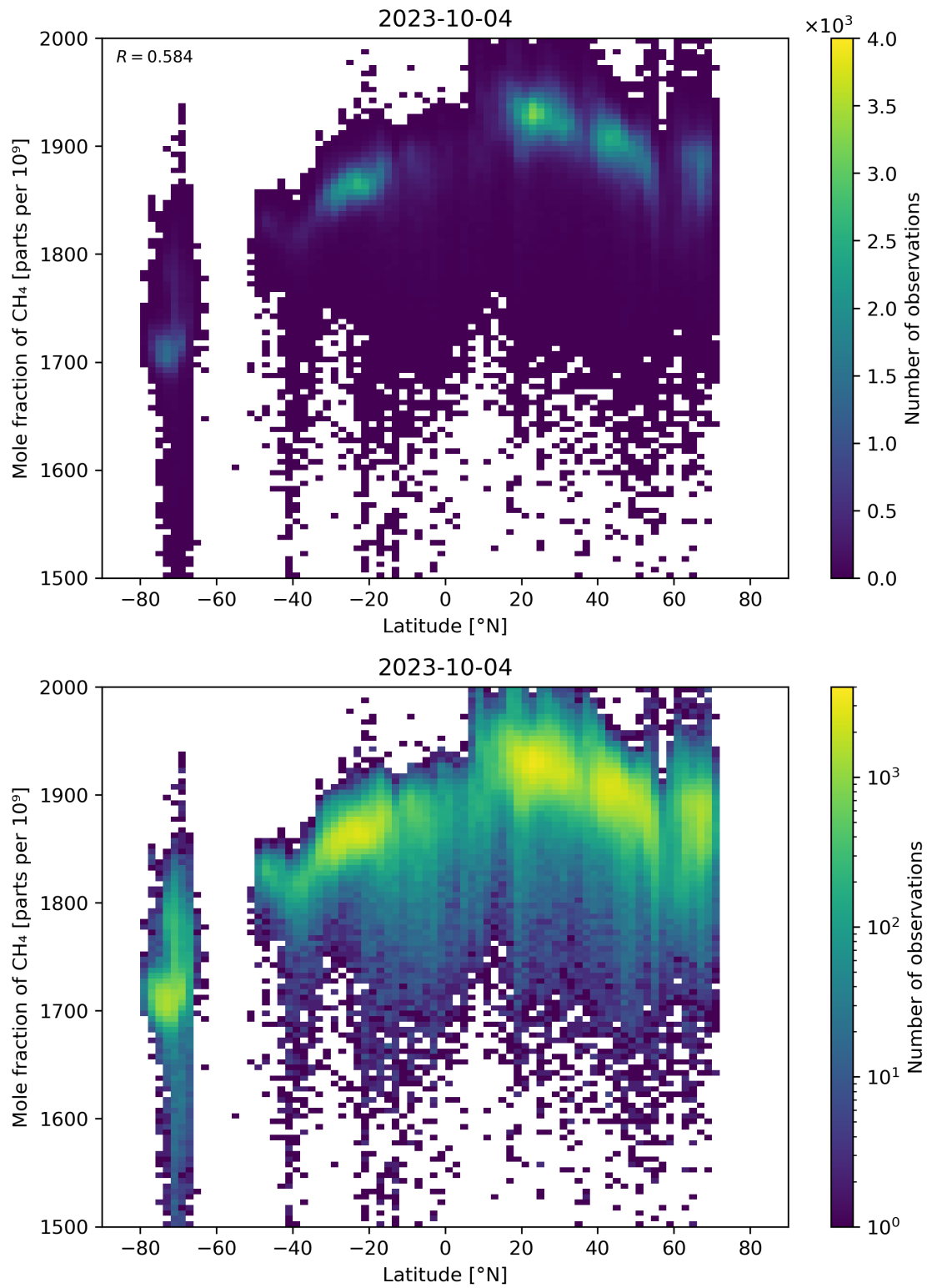
Figure 57: Scatter density plot of “Latitude” against “Mole fraction of CH 4 ” for 2023-10-03 to 2023-10-05.
