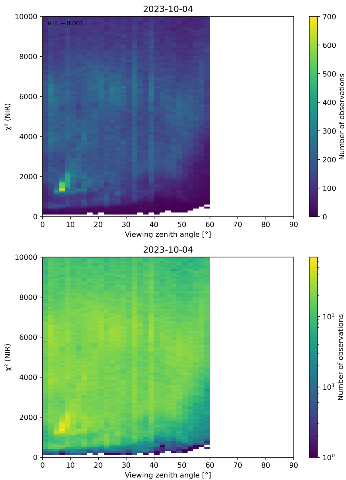
Figure 105: Scatter density plot of “Viewing zenith angle” against “ \chi^2 (NIR)” for 2023-10-03 to 2023-10-05.
