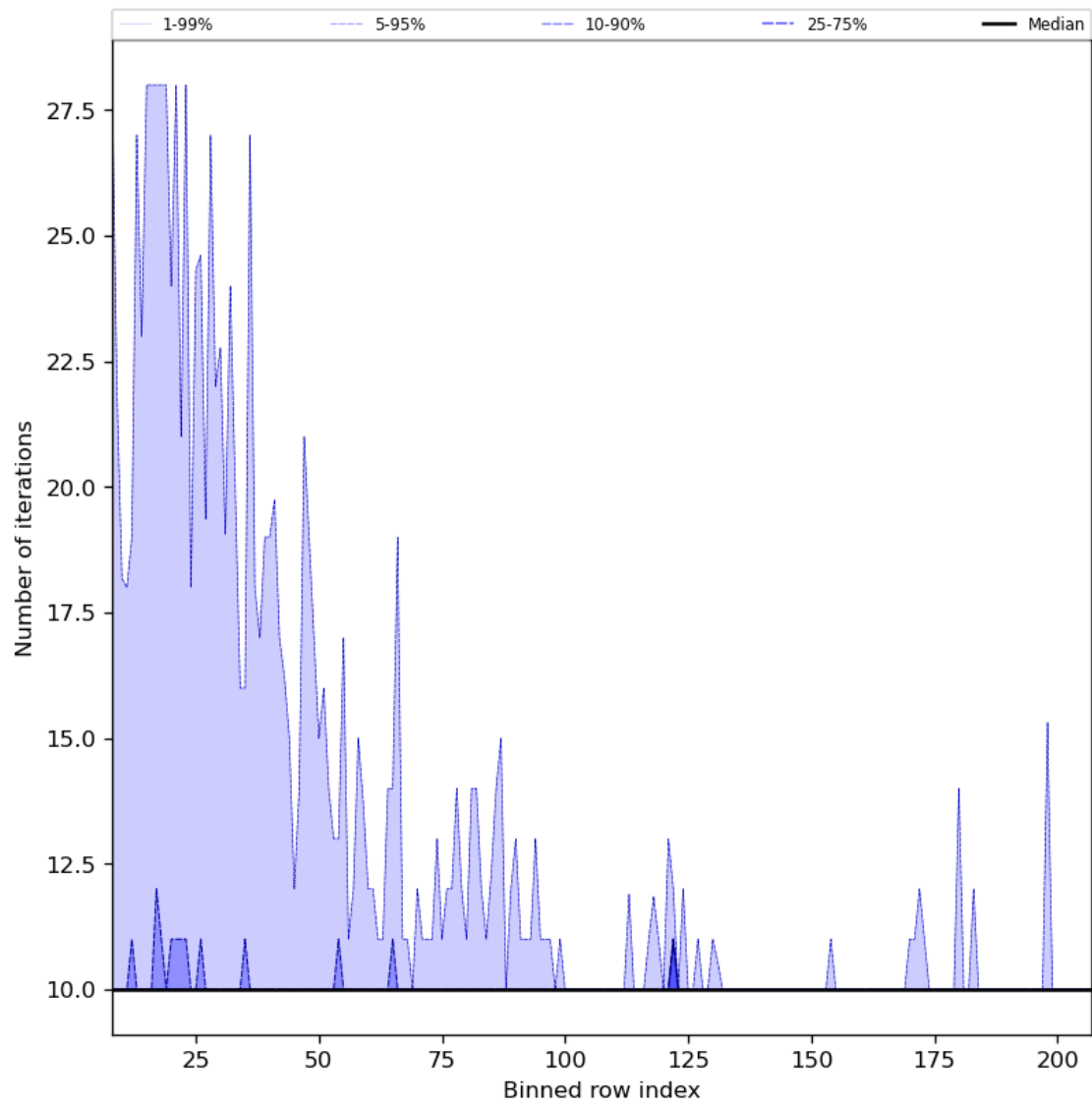
Figure 42: Along track statistics of “Number of iterations” for 2023-10-03 to 2023-10-05
