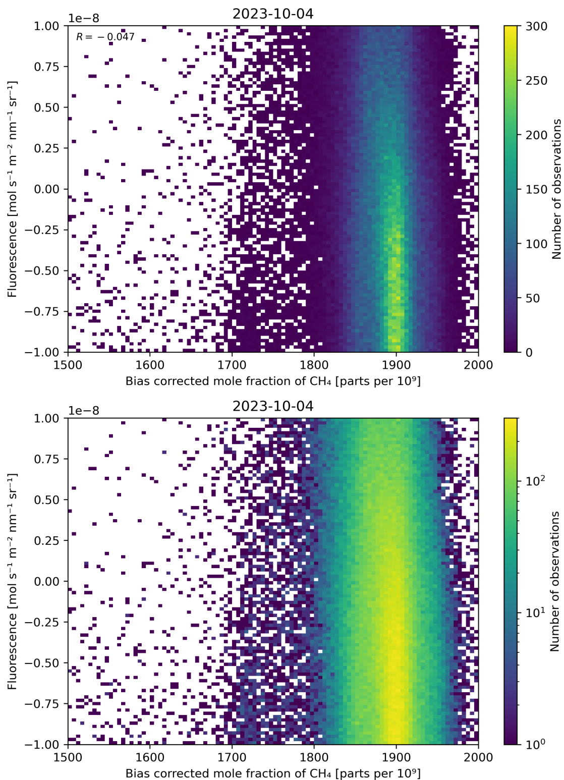
Figure 66: Scatter density plot of “Bias corrected mole fraction of \text{CH}_4 ” against “Fluorescence” for 2023-10-03 to 2023-10-05.
