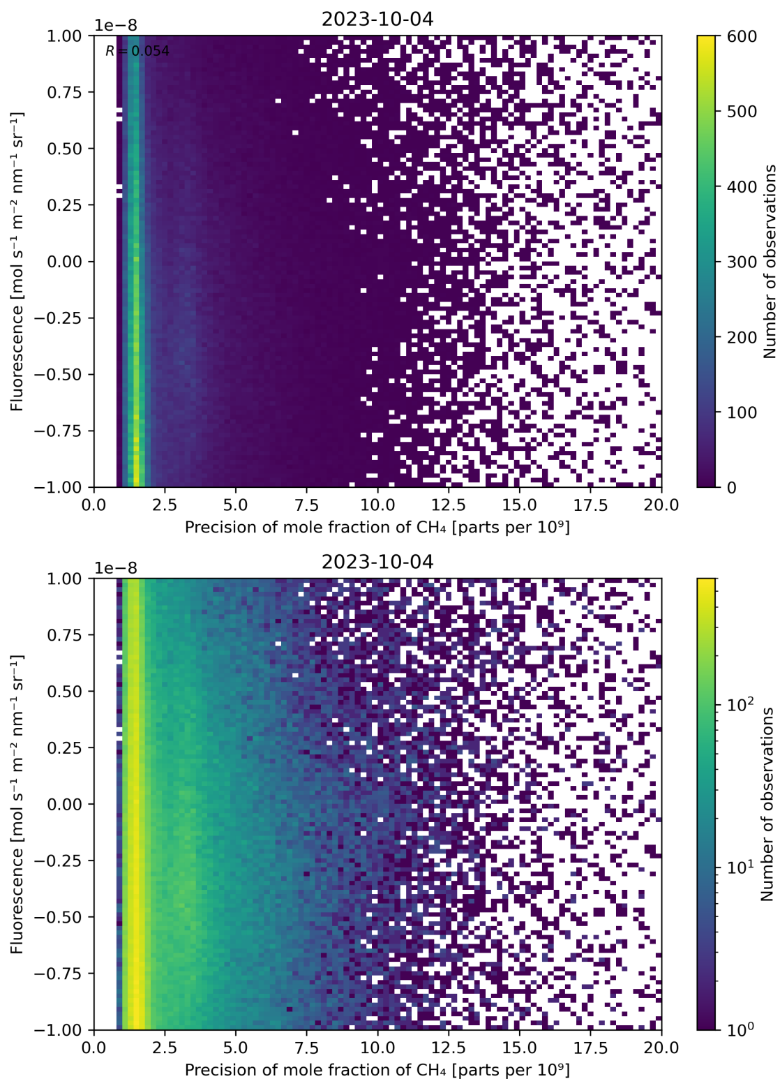
Figure 81: Scatter density plot of “Precision of mole fraction of \text{CH}_4 ” against “Fluorescence” for 2023-10-03 to 2023-10-05.
