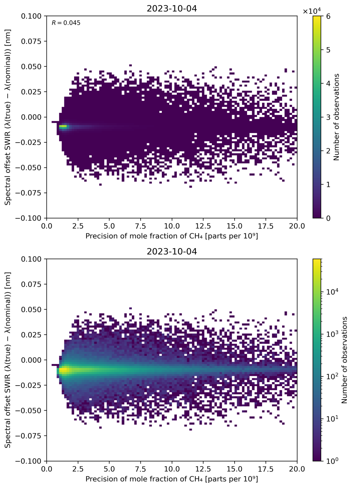
Figure 85: Scatter density plot of “Precision of mole fraction of CH 4 ” against “Spectral offset SWIR ( \lambda(\text{true}) - \lambda(\text{nominal}) )” for 2023-10-03 to 2023-10-05.
