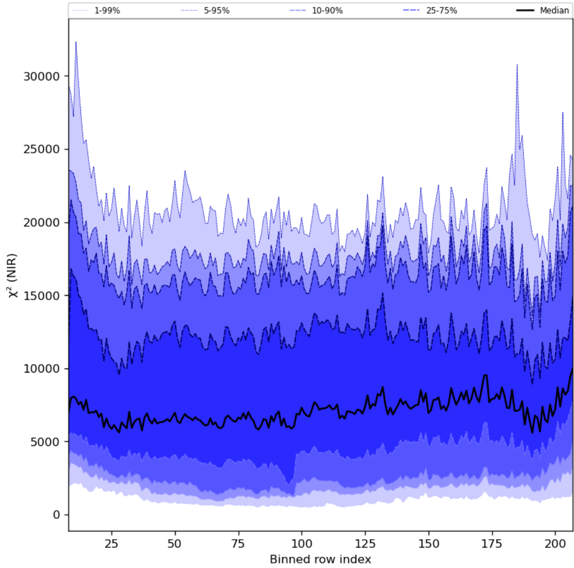
Figure 40: Along track statistics of “ \chi^2 (NIR)” for 2023-10-03 to 2023-10-05
