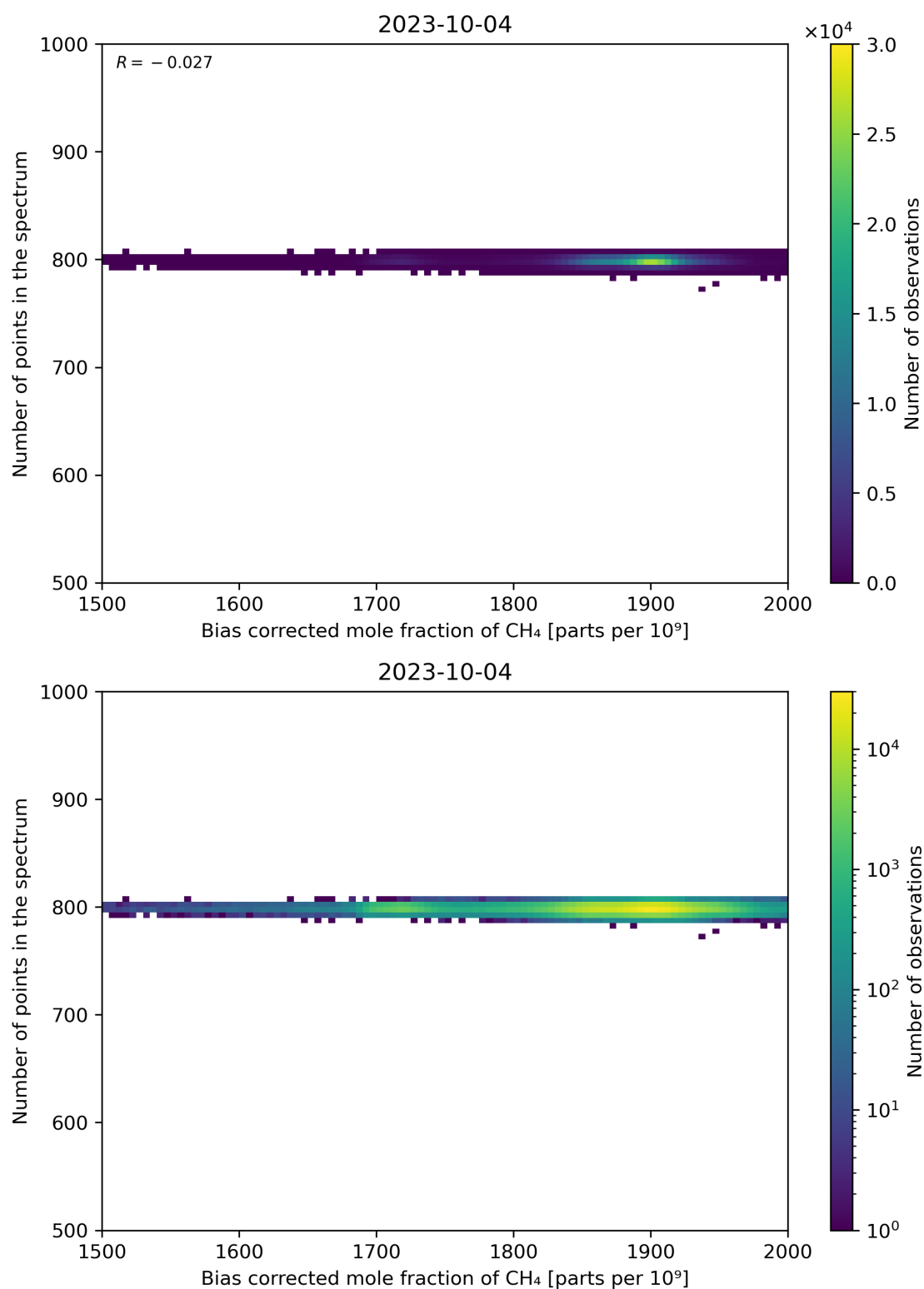
Figure 68: Scatter density plot of “Bias corrected mole fraction of CH 4 ” against “Number of points in the spectrum” for 2023-10-03 to 2023-10-05.
