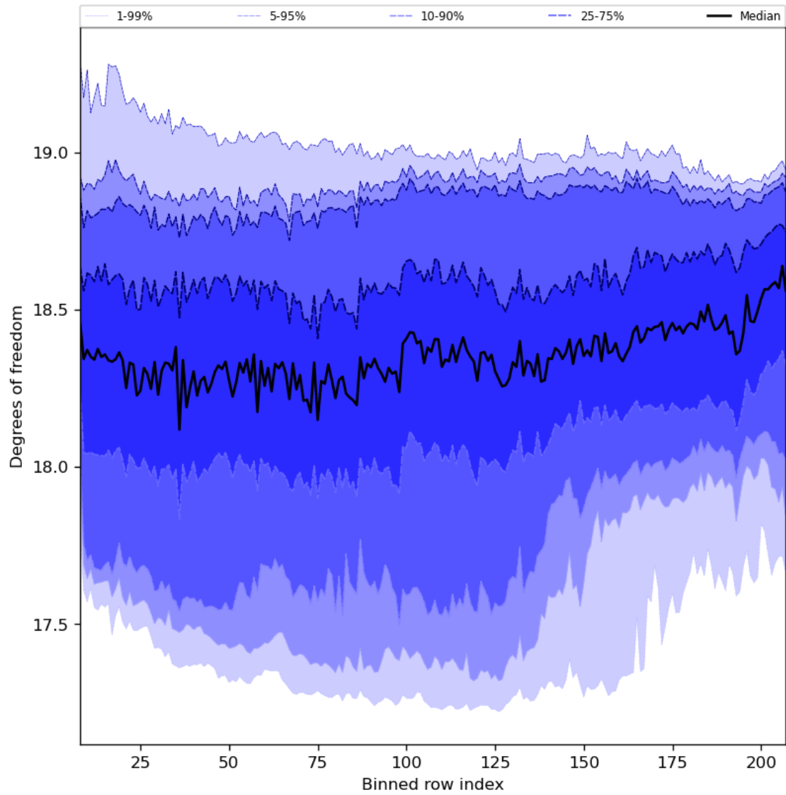
Figure 41: Along track statistics of “Degrees of freedom” for 2023-10-03 to 2023-10-05
