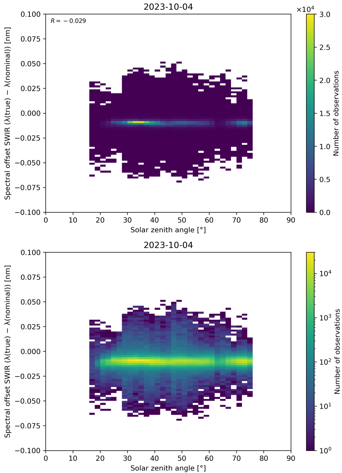
Figure 104: Scatter density plot of “Solar zenith angle” against “Spectral offset SWIR ( \lambda(\text{true}) - \lambda(\text{nominal}) )” for 2023-10-03 to 2023-10-05.
