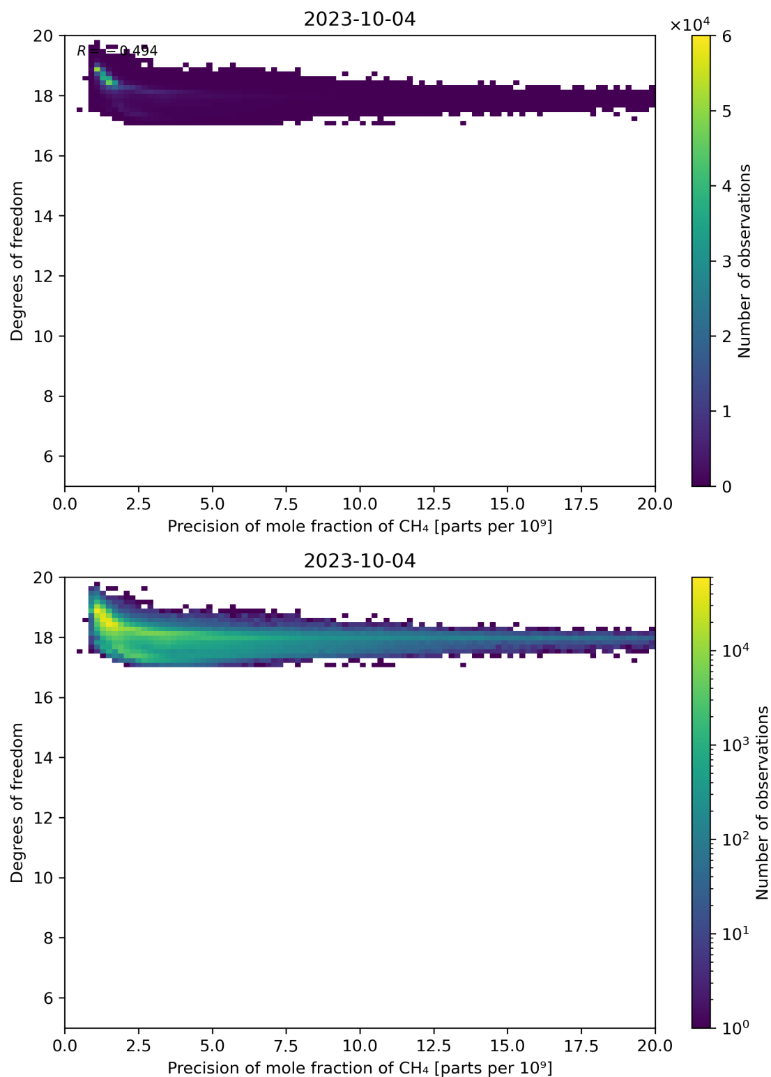
Figure 80: Scatter density plot of “Precision of mole fraction of CH 4 ” against “Degrees of freedom” for 2023-10-03 to 2023-10-05.
