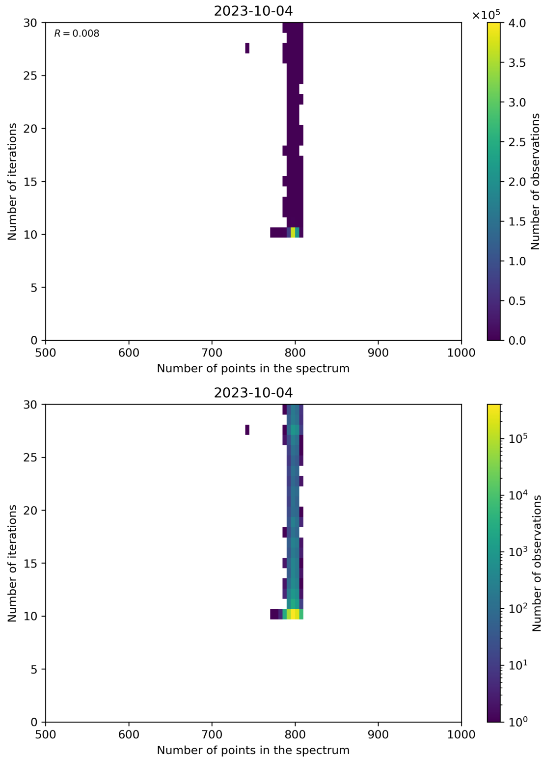
Figure 92: Scatter density plot of “Number of points in the spectrum” against “Number of iterations” for 2023-10-03 to 2023-10-05.
