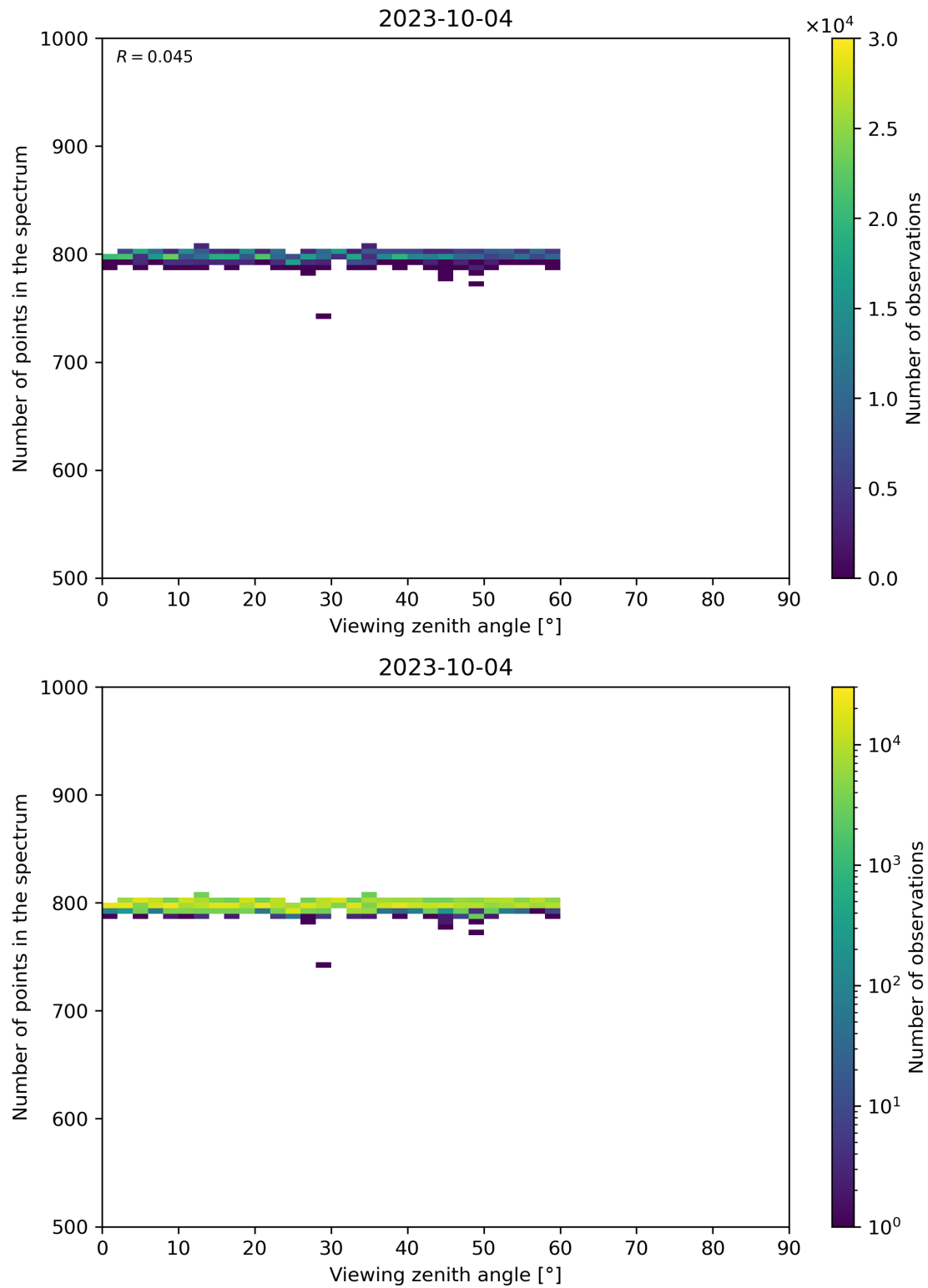
Figure 114: Scatter density plot of “Viewing zenith angle” against “Number of points in the spectrum” for 2023-10-03 to 2023-10-05.
