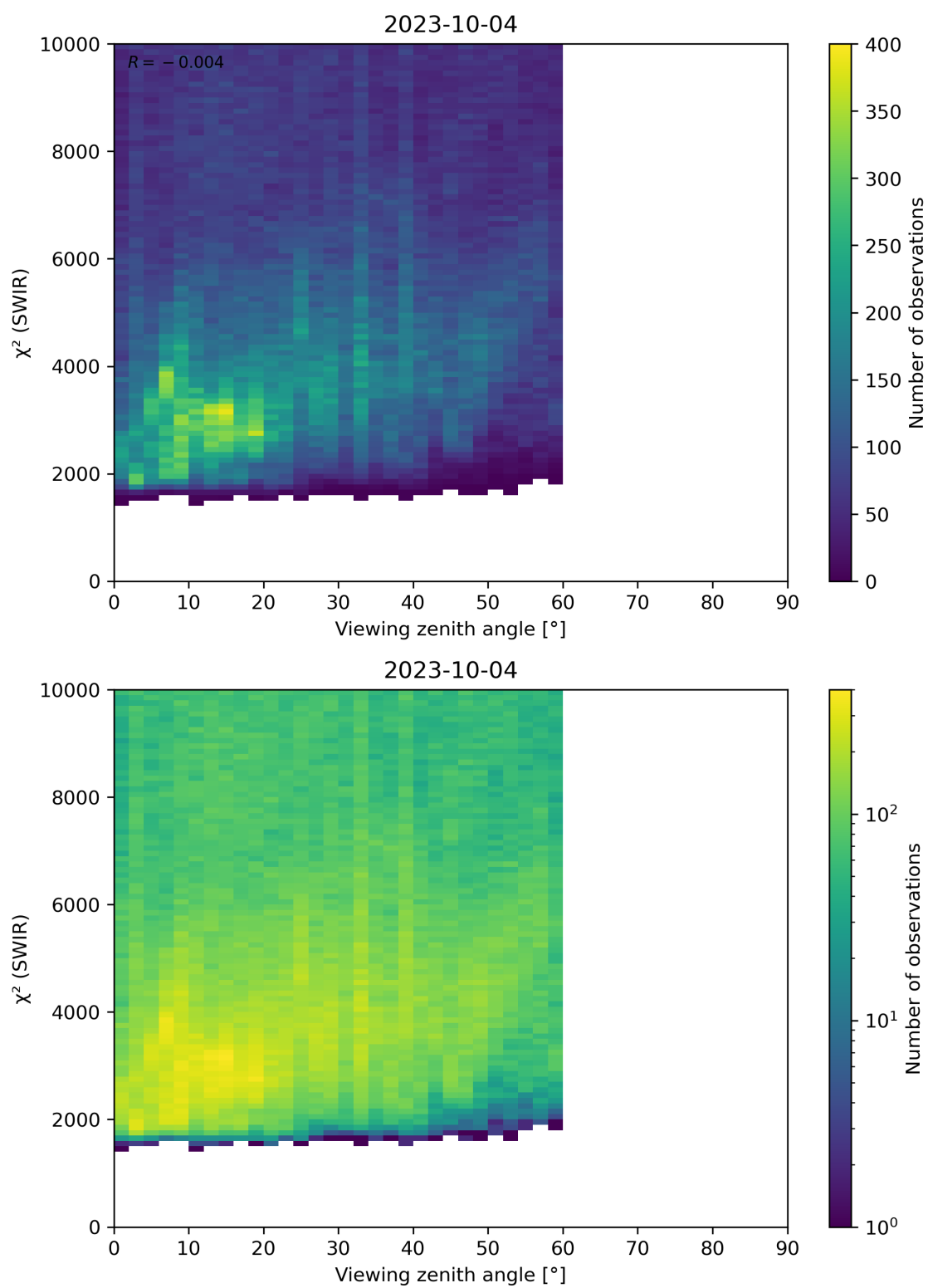
Figure 106: Scatter density plot of “Viewing zenith angle” against “ \chi^2 (SWIR)” for 2023-10-03 to 2023-10-05.
