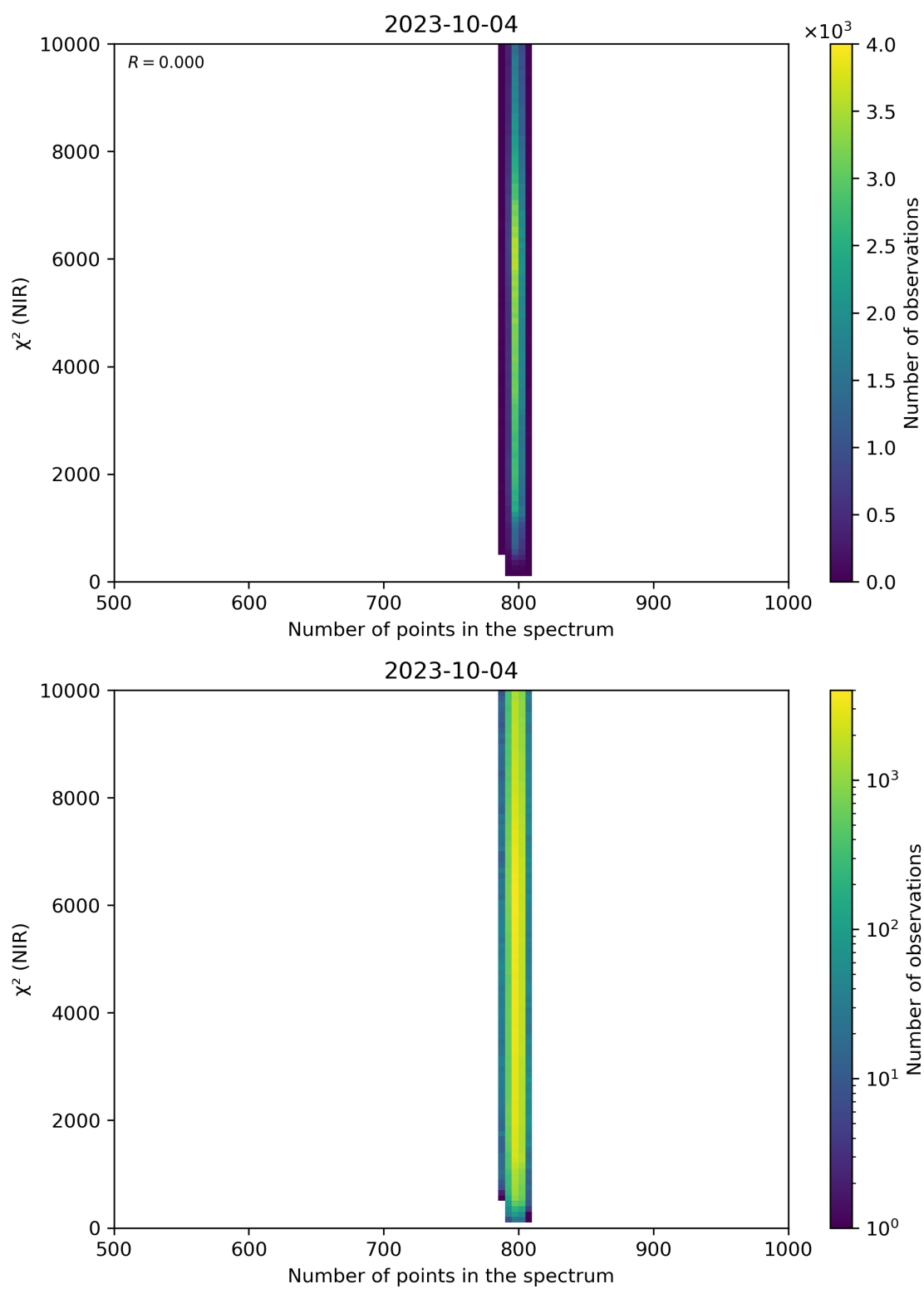
Figure 88: Scatter density plot of “Number of points in the spectrum” against “ \chi^2 (NIR)” for 2023-10-03 to 2023-10-05.
