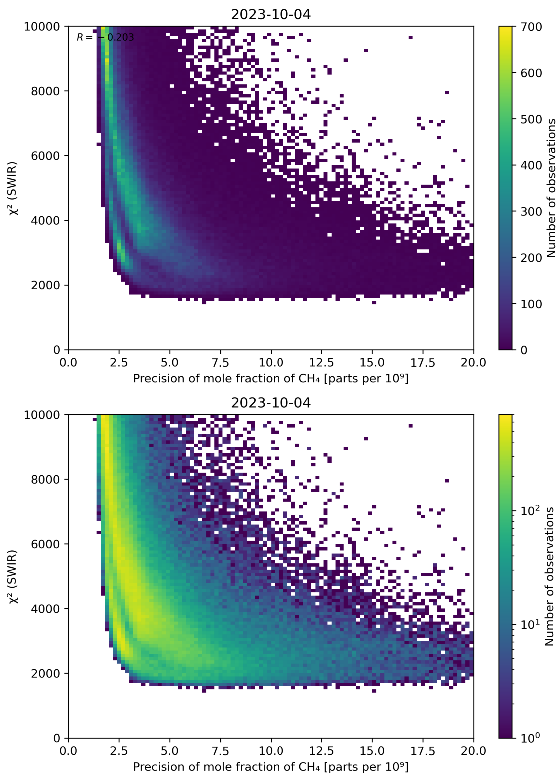
Figure 79: Scatter density plot of “Precision of mole fraction of CH 4 ” against “ \chi^2 (SWIR)” for 2023-10-03 to 2023-10-05.
