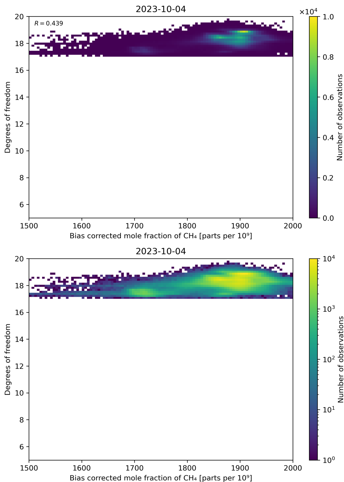
Figure 65: Scatter density plot of “Bias corrected mole fraction of CH 4 ” against “Degrees of freedom” for 2023-10-03 to 2023-10-05.
