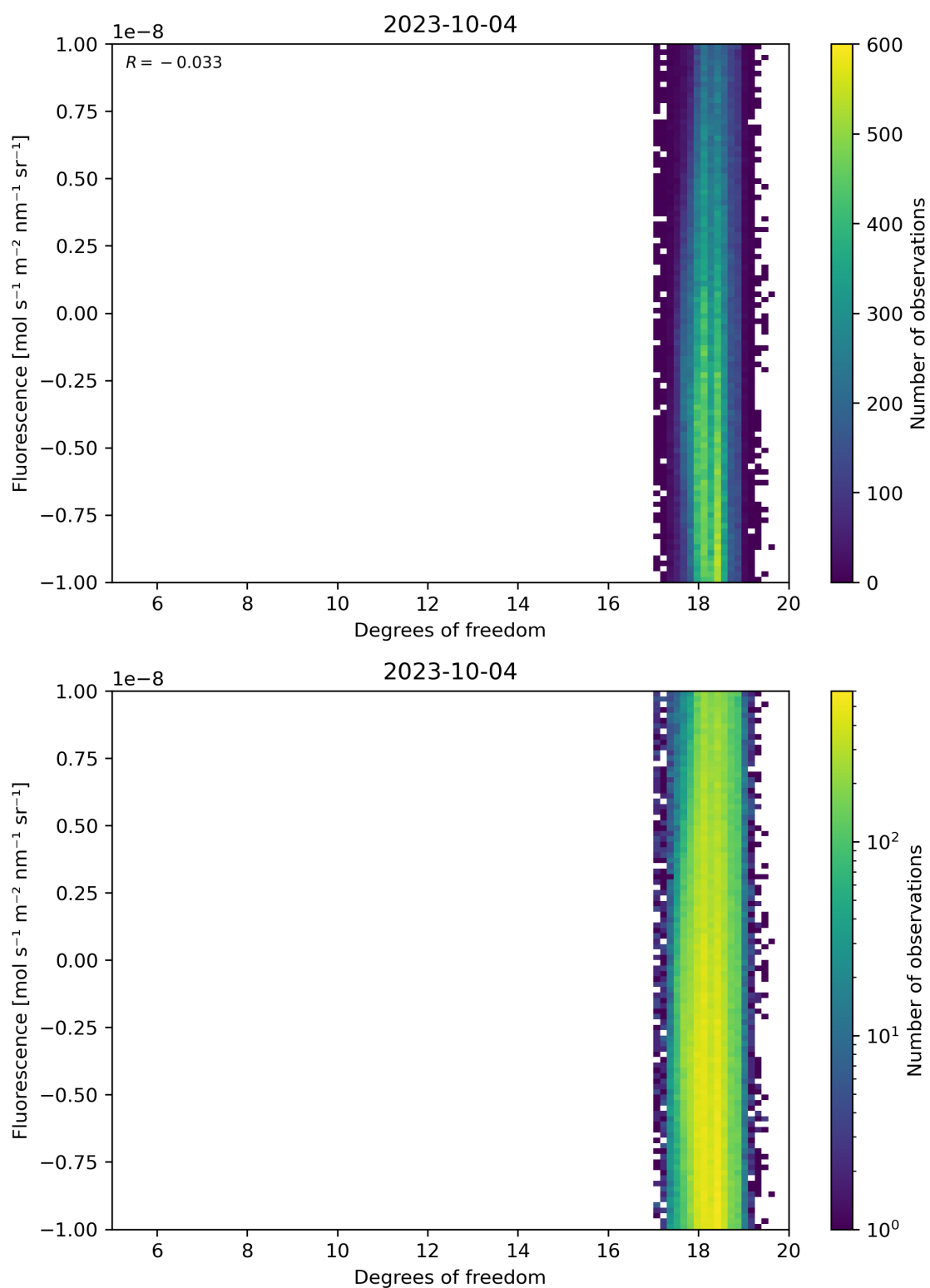
Figure 51: Scatter density plot of “Degrees of freedom” against “Fluorescence” for 2023-10-03 to 2023-10-05.
