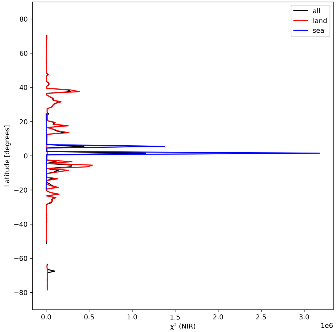
Figure 18: Zonal average of “ \chi^2 (NIR)” for 2023-10-03 to 2023-10-05.
