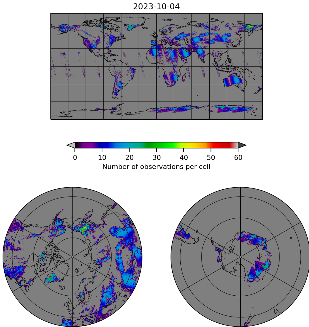
Figure 10: Map of the number of observations for 2023-10-03 to 2023-10-05
