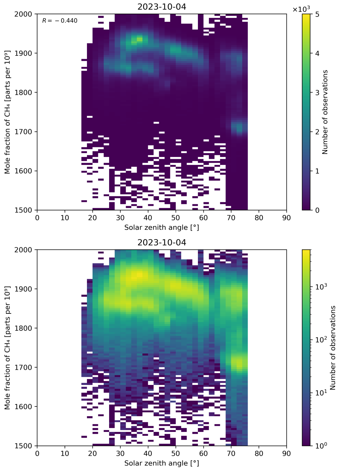
Figure 99: Scatter density plot of “Solar zenith angle” against “Mole fraction of \text{CH}_4 ” for 2023-10-03 to 2023-10-05.
