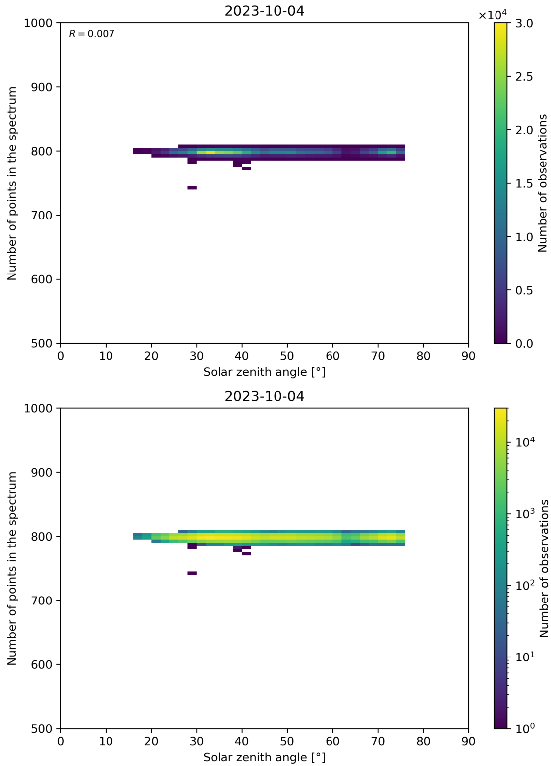
Figure 103: Scatter density plot of “Solar zenith angle” against “Number of points in the spectrum” for 2023-10-03 to 2023-10-05.
