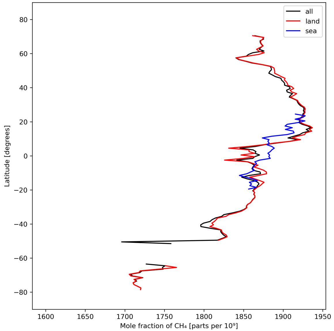
Figure 12: Zonal average of “Mole fraction of \text{CH}_4 ” for 2023-10-03 to 2023-10-05.
