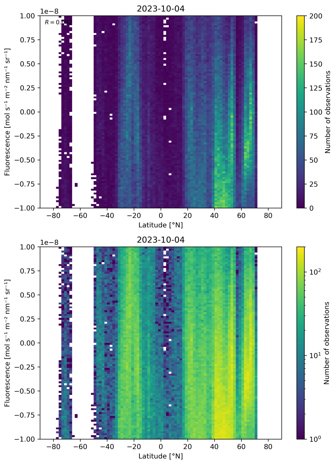
Figure 56: Scatter density plot of “Latitude” against “Fluorescence” for 2023-10-03 to 2023-10-05.
