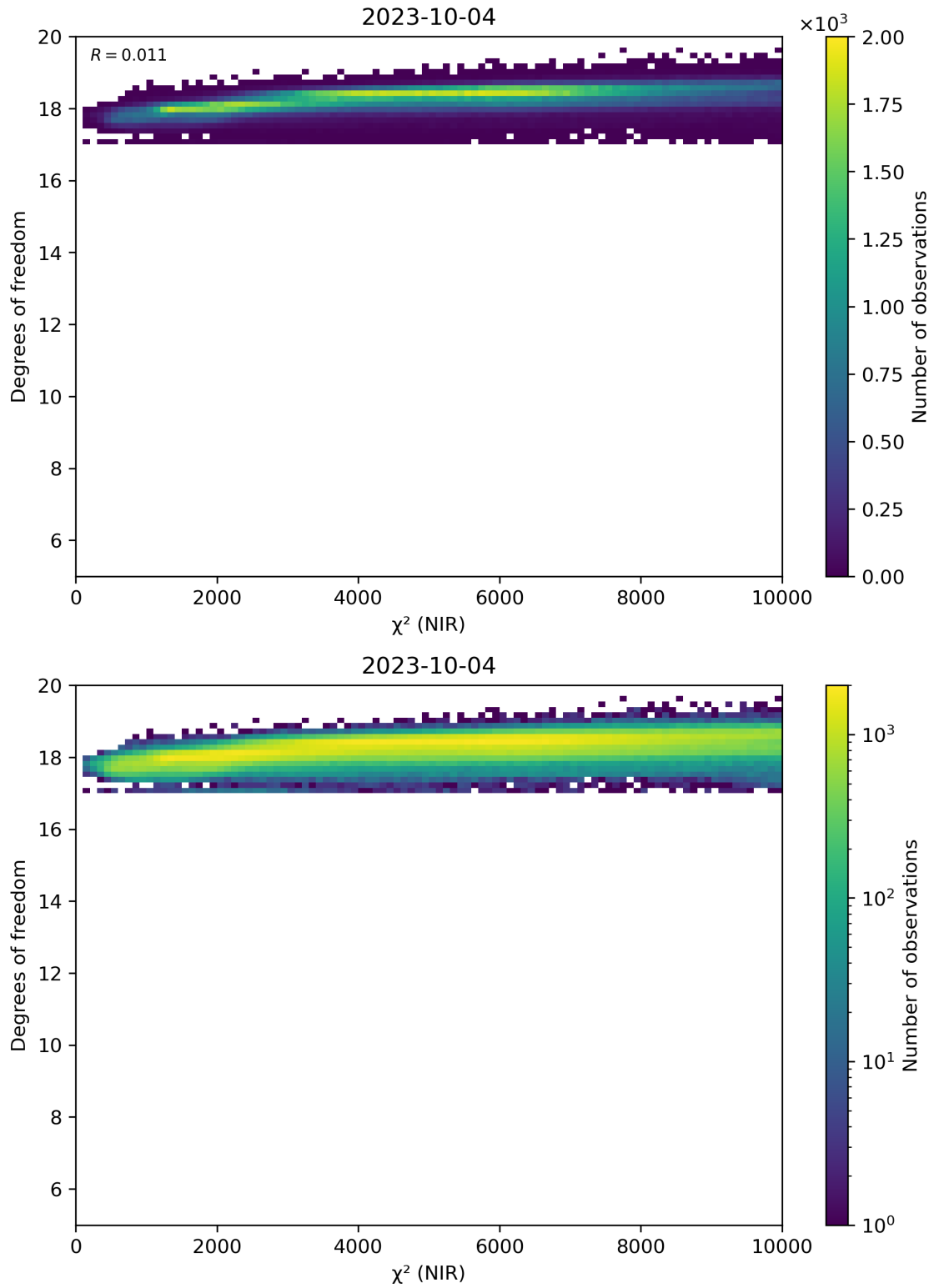
Figure 44: Scatter density plot of “ \chi^2 (NIR)” against “Degrees of freedom” for 2023-10-03 to 2023-10-05.
