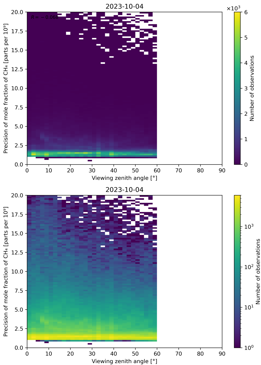
Figure 112: Scatter density plot of “Viewing zenith angle” against “Precision of mole fraction of CH 4 ” for 2023-10-03 to 2023-10-05.
