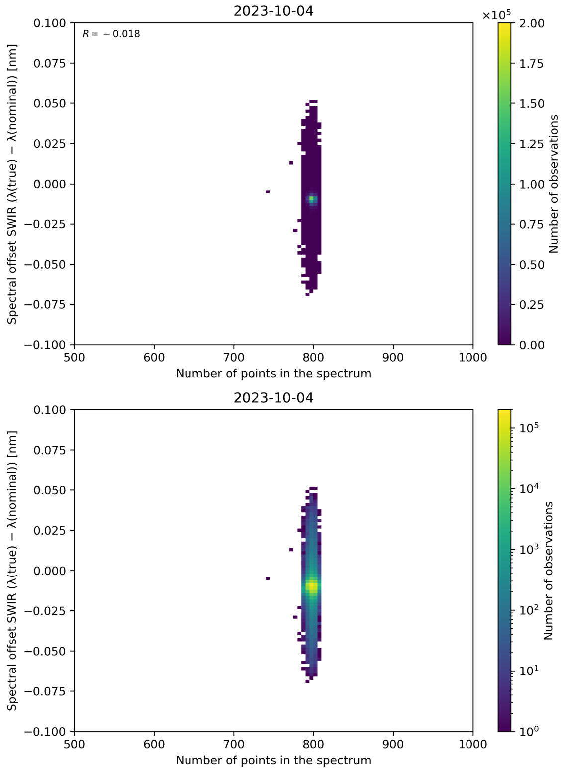
Figure 93: Scatter density plot of “Number of points in the spectrum” against “Spectral offset SWIR ( \lambda(\text{true}) - \lambda(\text{nominal}) )” for 2023-10-03 to 2023-10-05.
