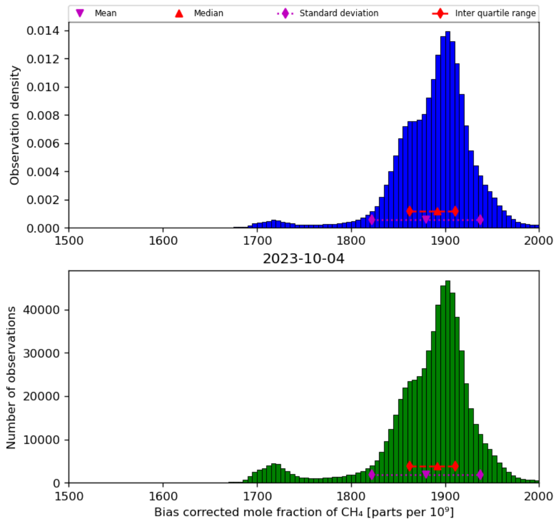
Figure 25: Histogram of “Bias corrected mole fraction of CH 4 ” for 2023-10-03 to 2023-10-05
