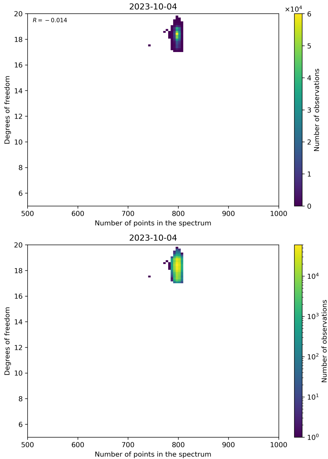
Figure 90: Scatter density plot of “Number of points in the spectrum” against “Degrees of freedom” for 2023-10-03 to 2023-10-05.
