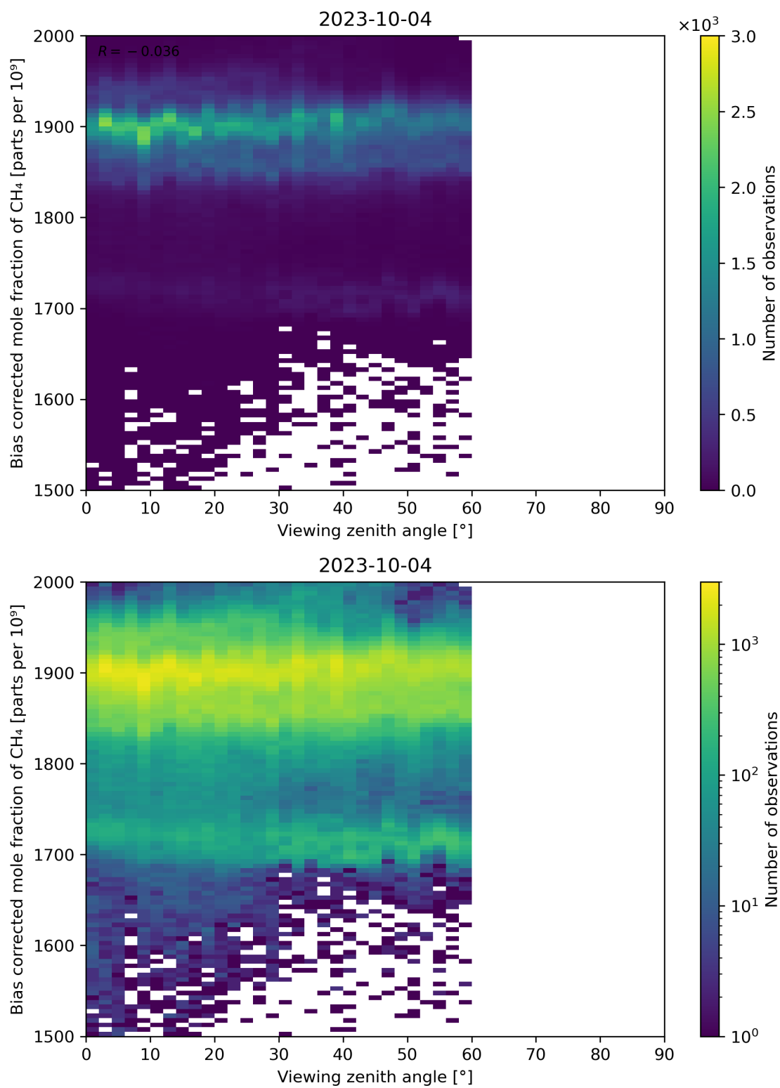
Figure 111: Scatter density plot of “Viewing zenith angle” against “Bias corrected mole fraction of CH 4 ” for 2023-10-03 to 2023-10-05.
