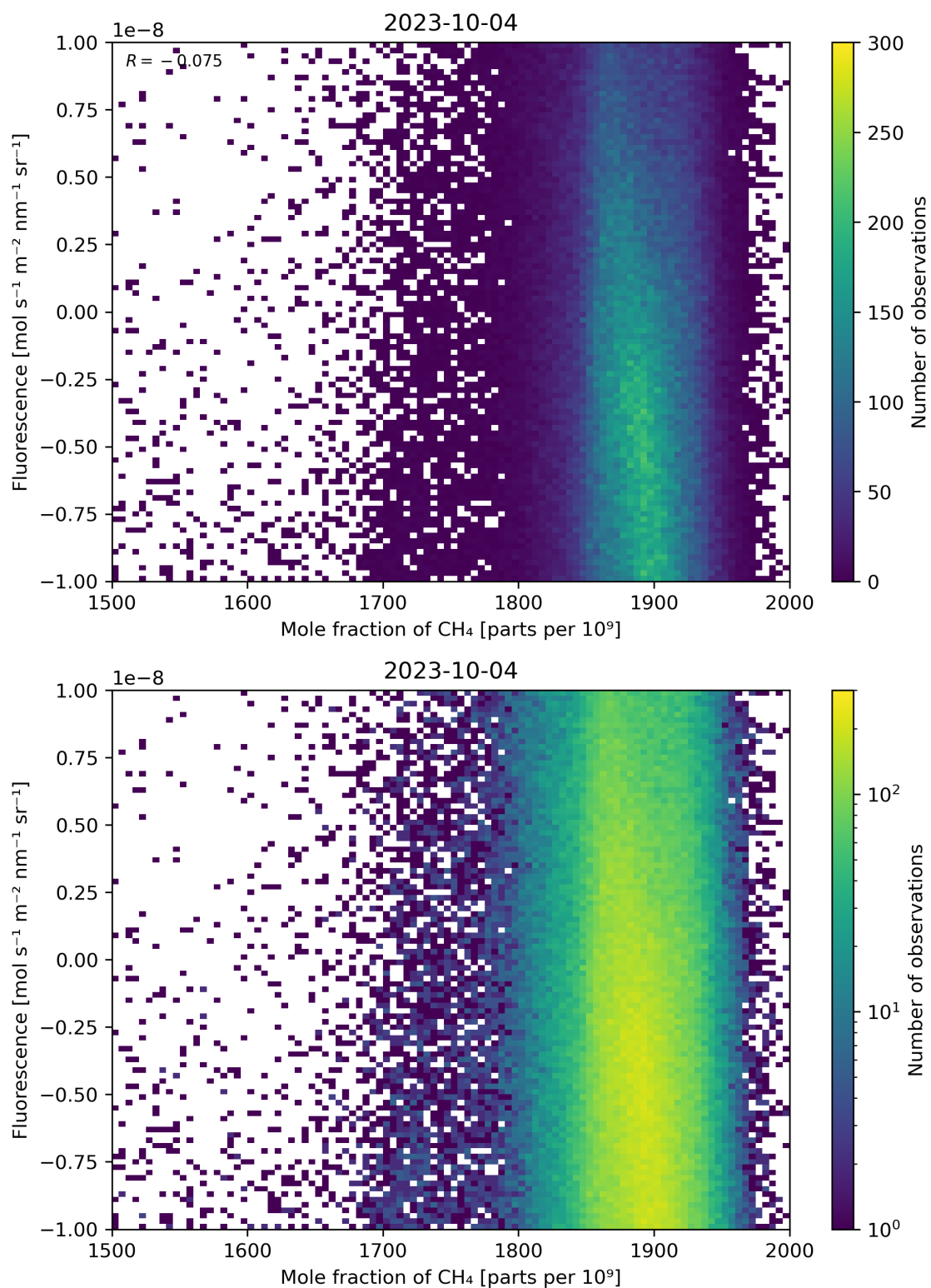
Figure 73: Scatter density plot of “Mole fraction of \text{CH}_4 ” against “Fluorescence” for 2023-10-03 to 2023-10-05.
