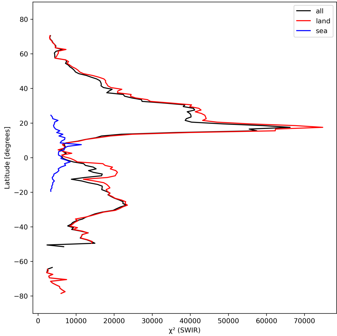
Figure 17: Zonal average of “ \chi^2 (SWIR)” for 2023-10-03 to 2023-10-05.
