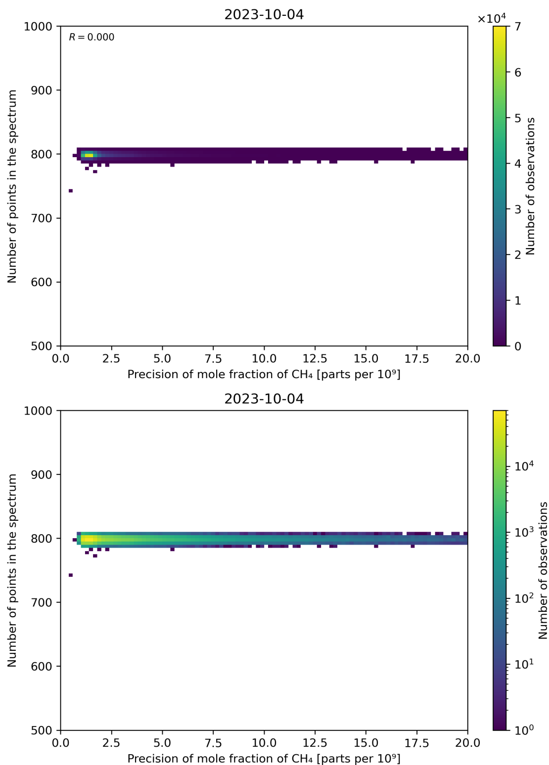
Figure 84: Scatter density plot of “Precision of mole fraction of \text{CH}_4 ” against “Number of points in the spectrum” for 2023-10-03 to 2023-10-05.
