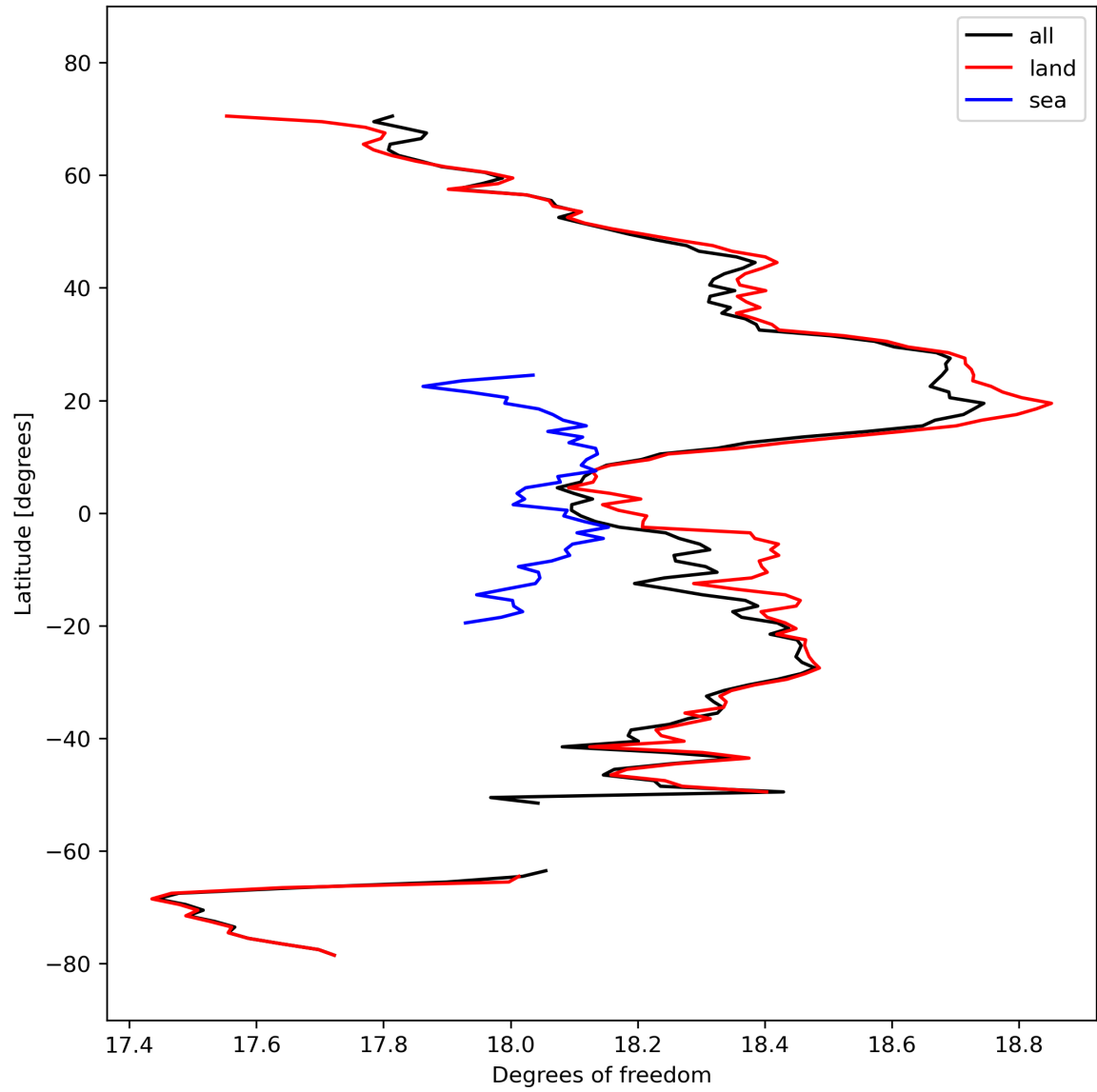
Figure 19: Zonal average of “Degrees of freedom” for 2023-10-03 to 2023-10-05.
