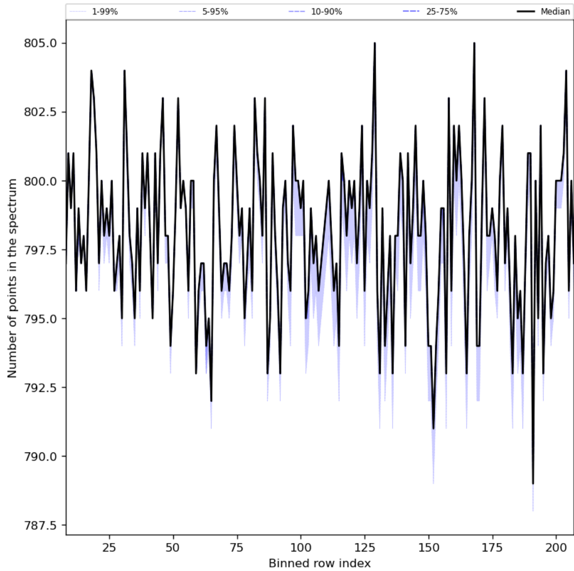
Figure 37: Along track statistics of “Number of points in the spectrum” for 2023-10-03 to 2023-10-05
