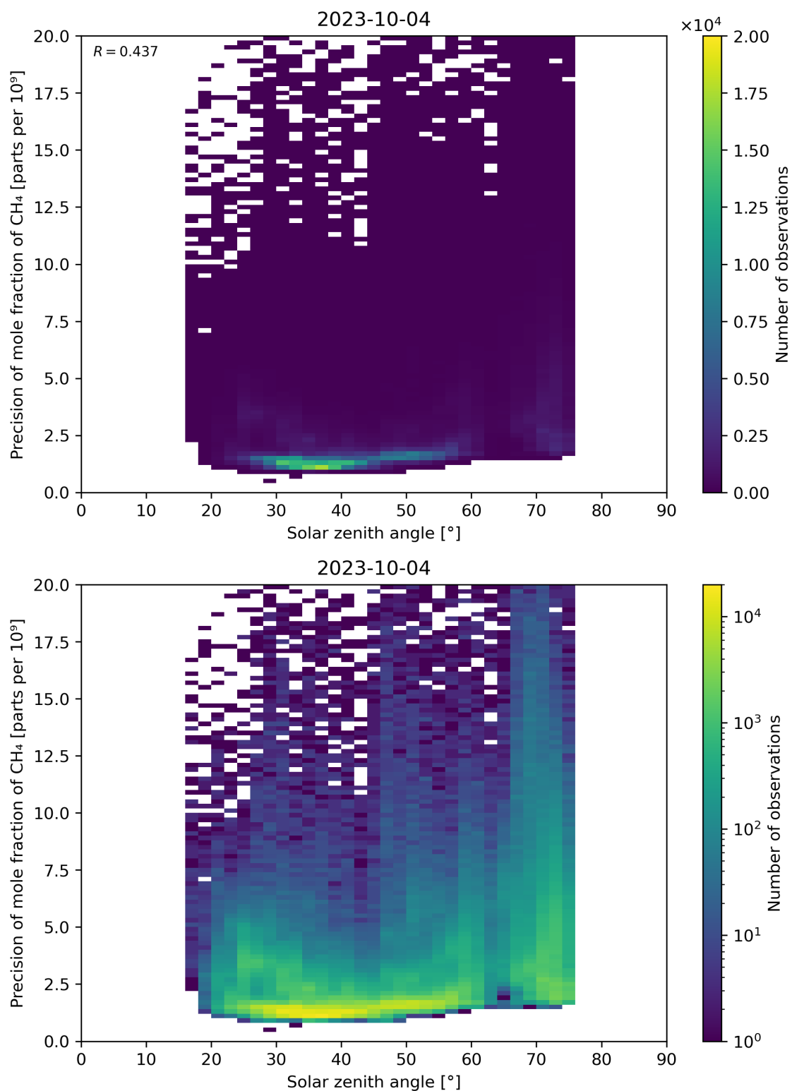
Figure 101: Scatter density plot of “Solar zenith angle” against “Precision of mole fraction of \text{CH}_4 ” for 2023-10-03 to 2023-10-05.
