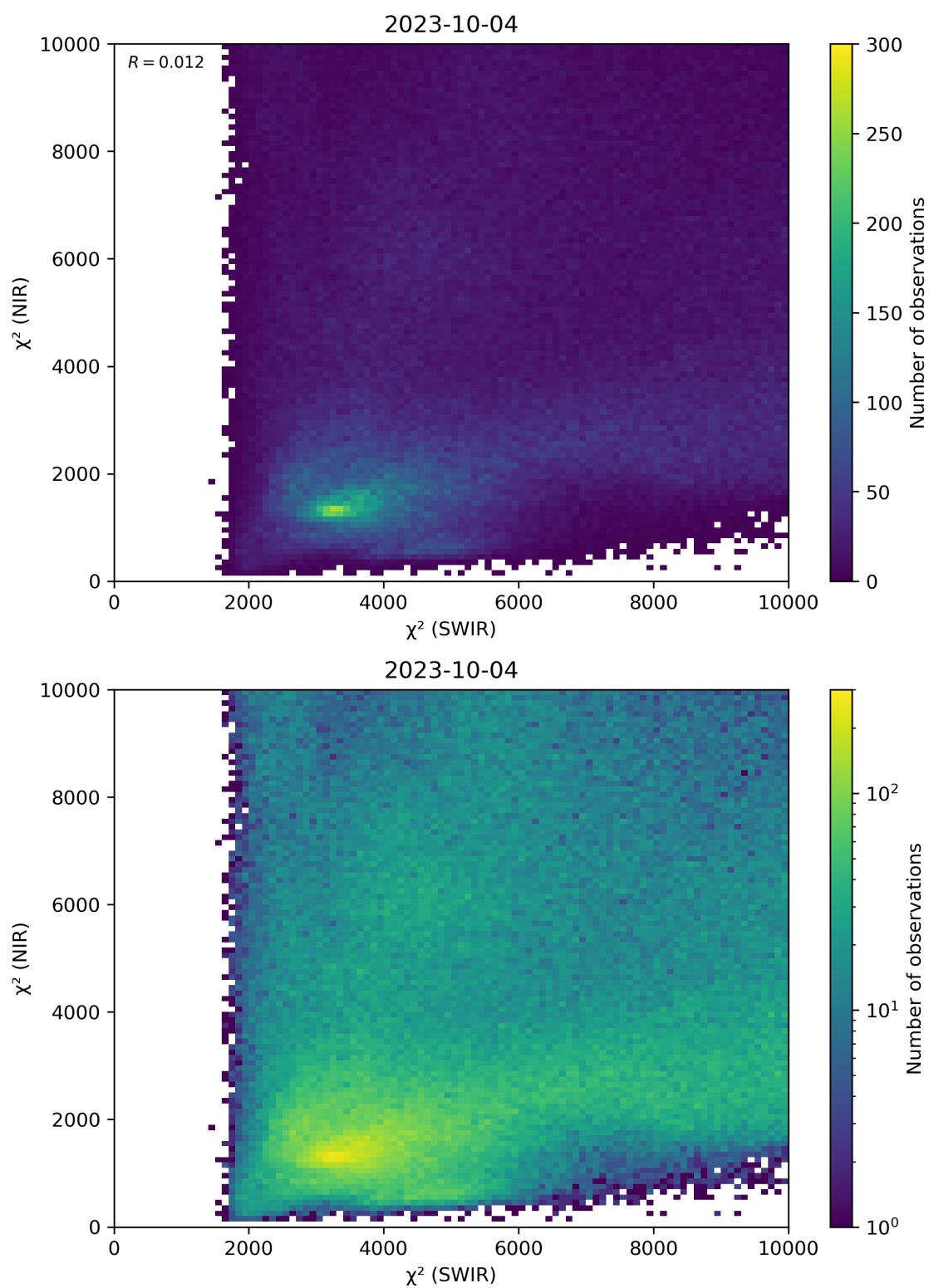
Figure 47: Scatter density plot of “ \chi^2 (SWIR)” against “ \chi^2 (NIR)” for 2023-10-03 to 2023-10-05.
