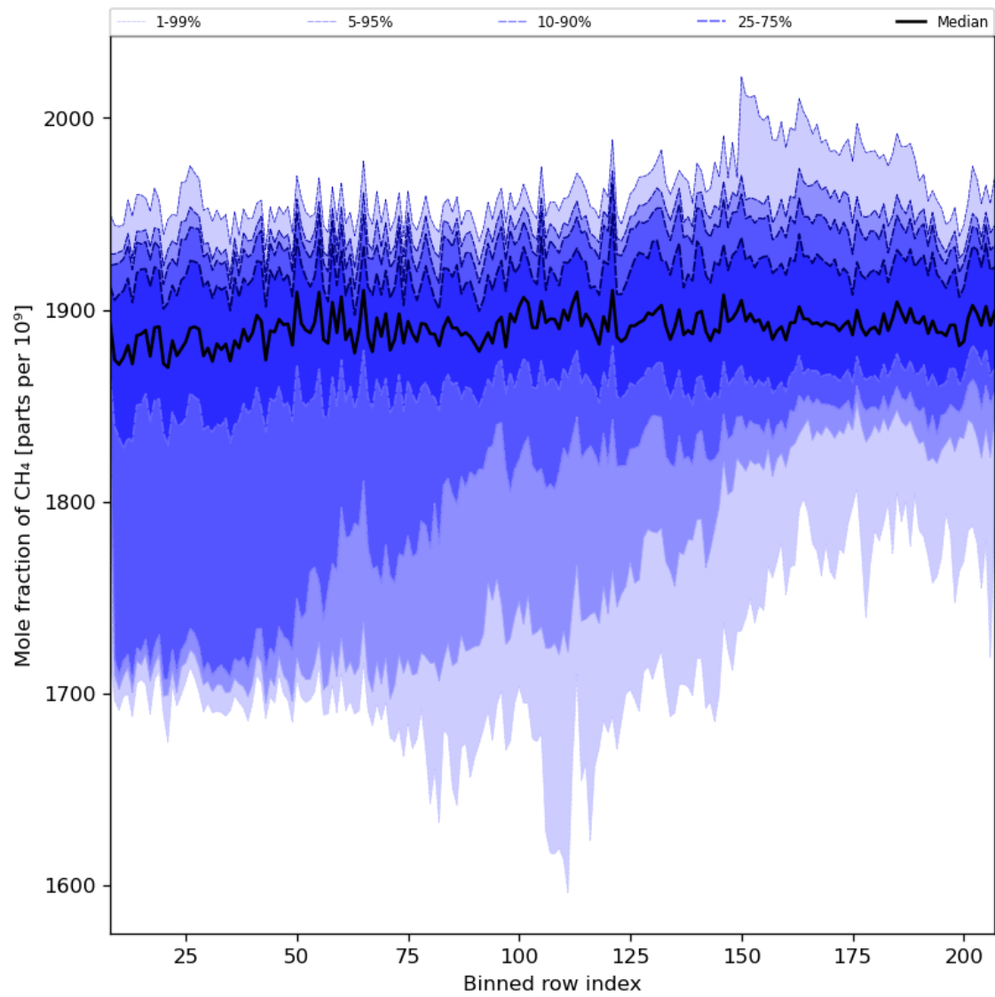
Figure 34: Along track statistics of “Mole fraction of CH 4 ” for 2023-10-03 to 2023-10-05
