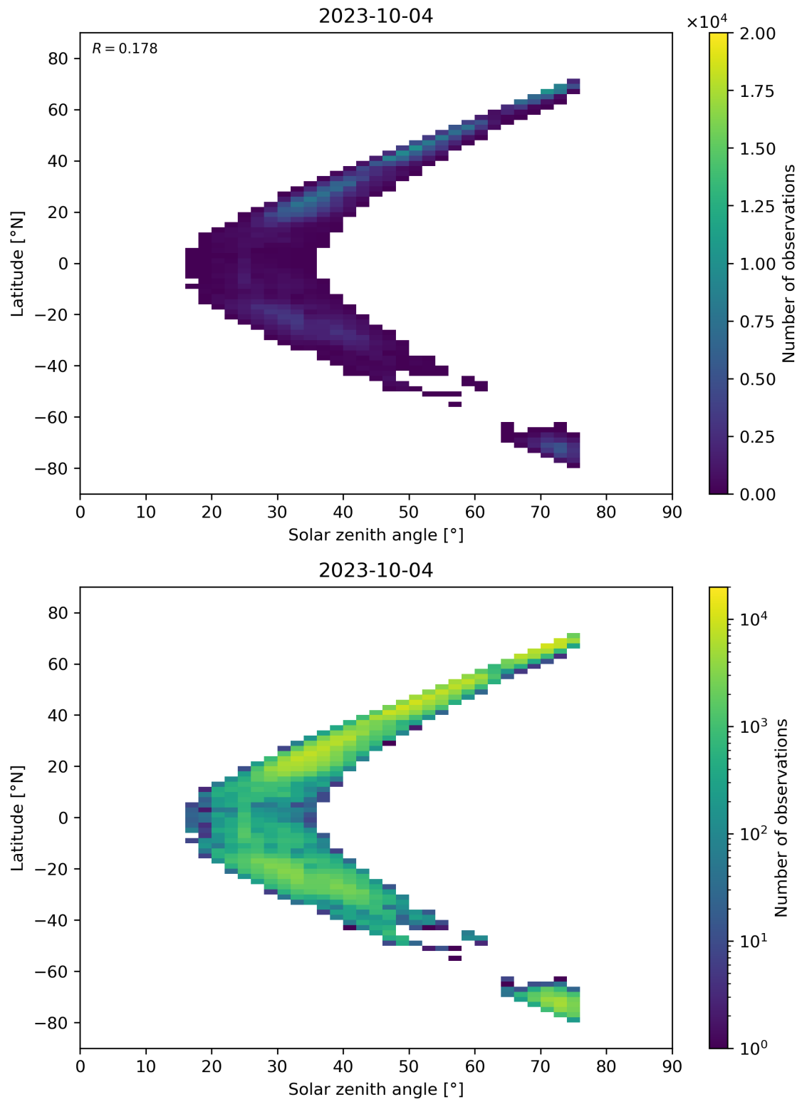
Figure 98: Scatter density plot of “Solar zenith angle” against “Latitude” for 2023-10-03 to 2023-10-05.
