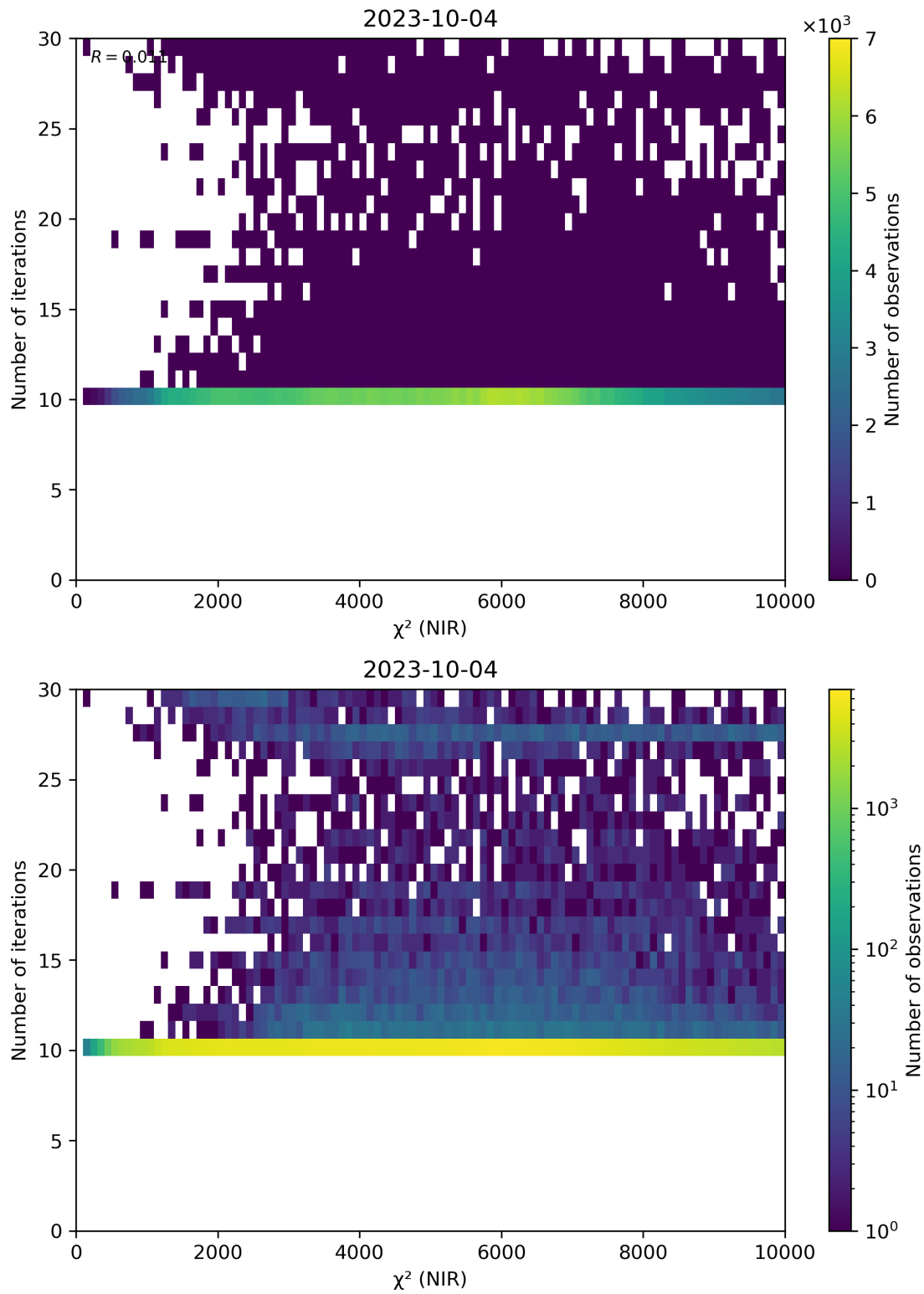
Figure 46: Scatter density plot of “ \chi^2 (NIR)” against “Number of iterations” for 2023-10-03 to 2023-10-05.
