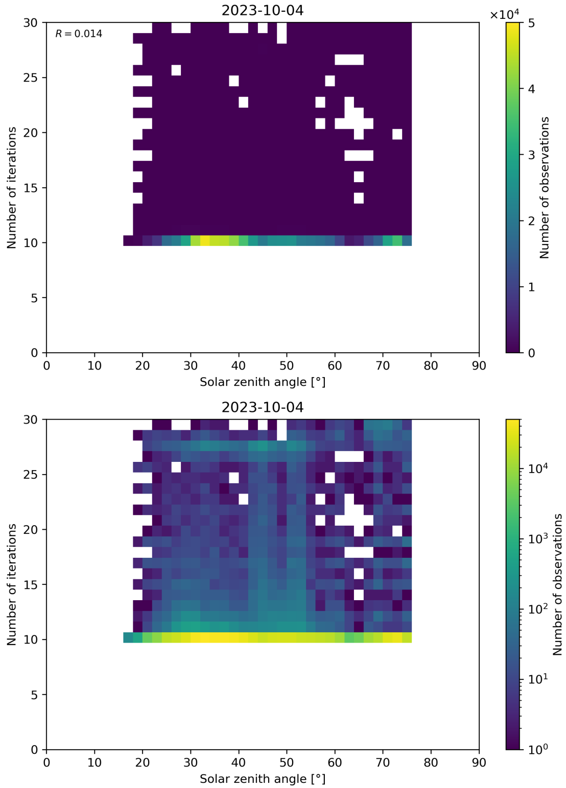
Figure 102: Scatter density plot of “Solar zenith angle” against “Number of iterations” for 2023-10-03 to 2023-10-05.
