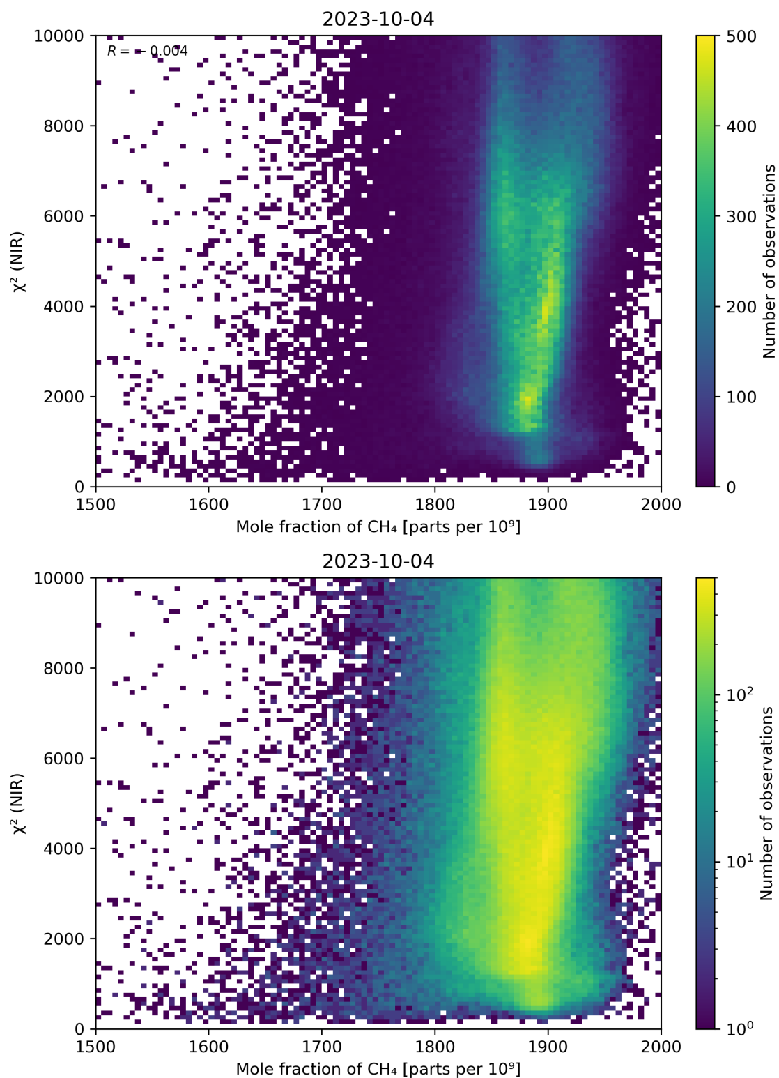
Figure 70: Scatter density plot of “Mole fraction of CH 4 ” against “ \chi^2 (NIR)” for 2023-10-03 to 2023-10-05.
