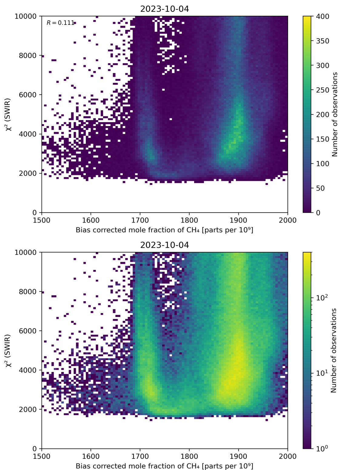
Figure 64: Scatter density plot of “Bias corrected mole fraction of CH 4 ” against “ \chi^2 (SWIR)” for 2023-10-03 to 2023-10-05.
