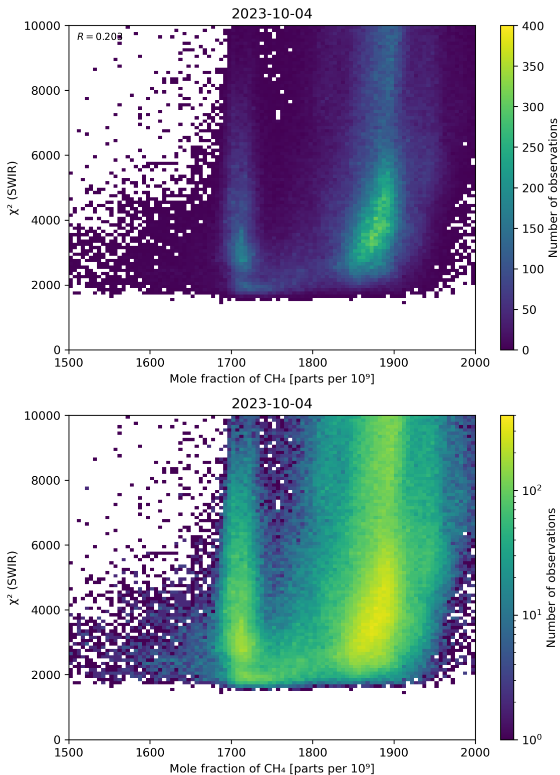
Figure 71: Scatter density plot of “Mole fraction of \text{CH}_4 ” against “ \chi^2 (SWIR)” for 2023-10-03 to 2023-10-05.
