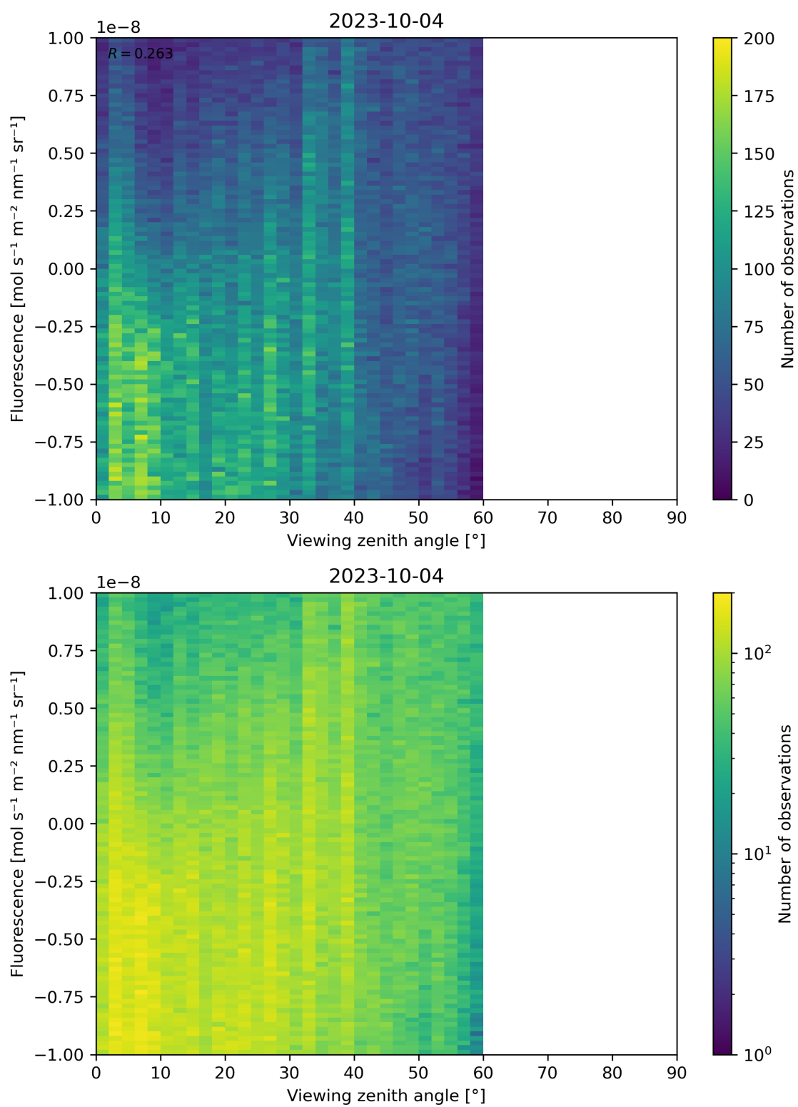
Figure 108: Scatter density plot of “Viewing zenith angle” against “Fluorescence” for 2023-10-03 to 2023-10-05.
