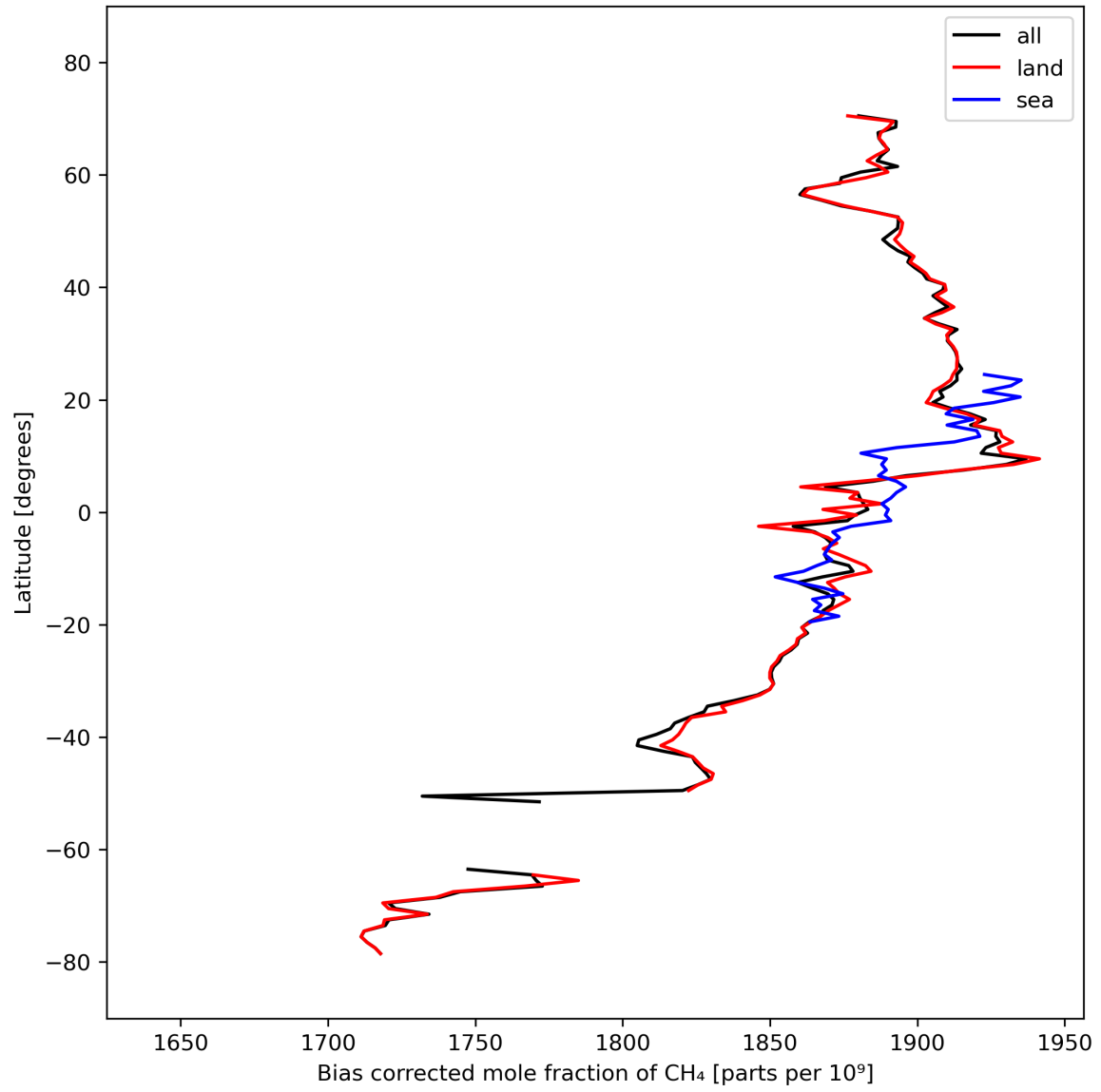
Figure 14: Zonal average of “Bias corrected mole fraction of CH 4 ” for 2023-10-03 to 2023-10-05.
