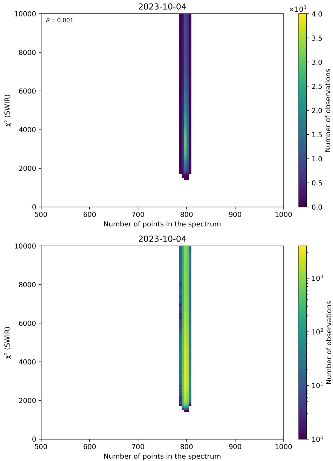
Figure 89: Scatter density plot of “Number of points in the spectrum” against “ \chi^2 (SWIR)” for 2023-10-03 to 2023-10-05.
