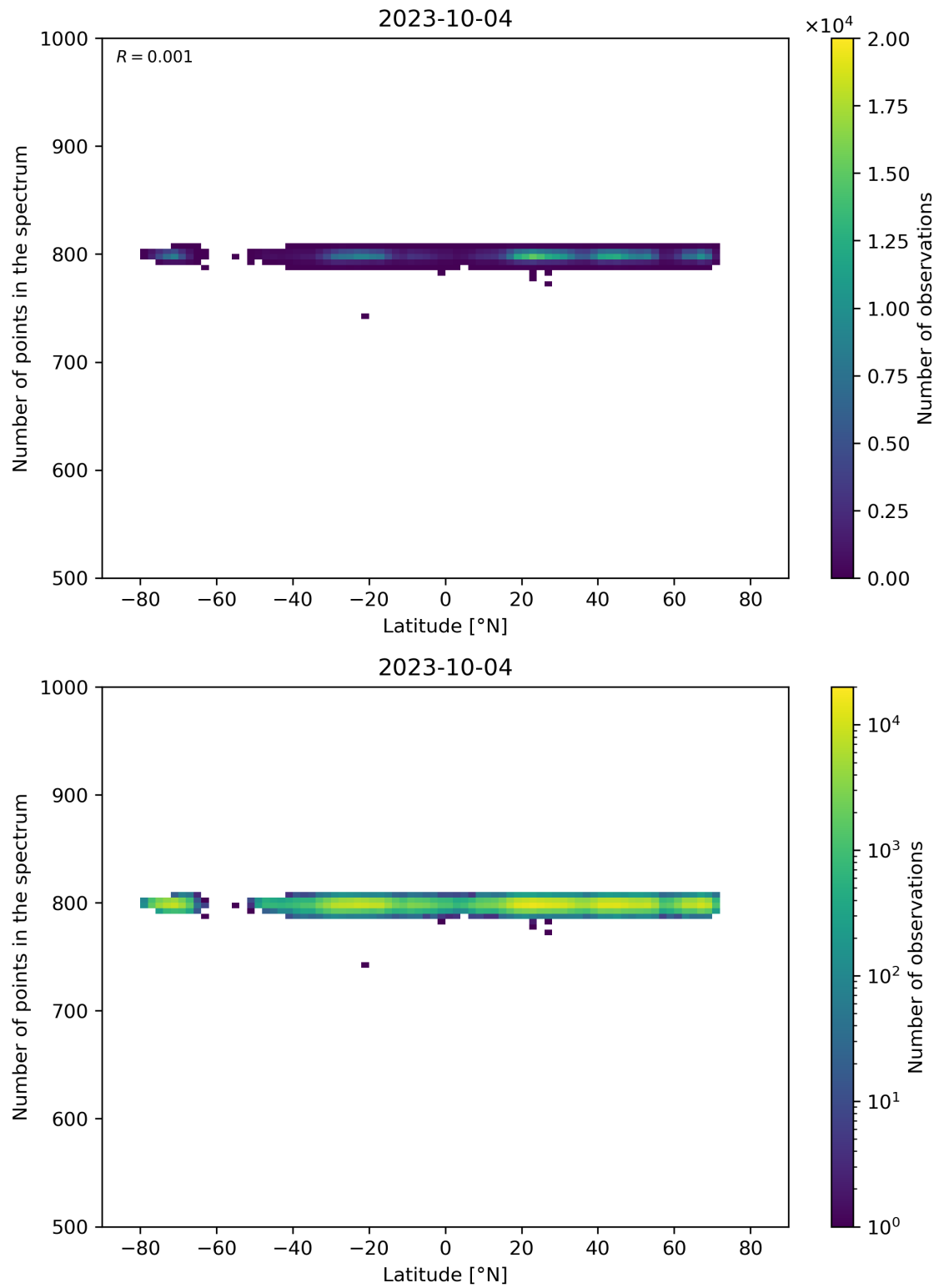
Figure 61: Scatter density plot of “Latitude” against “Number of points in the spectrum” for 2023-10-03 to 2023-10-05.
