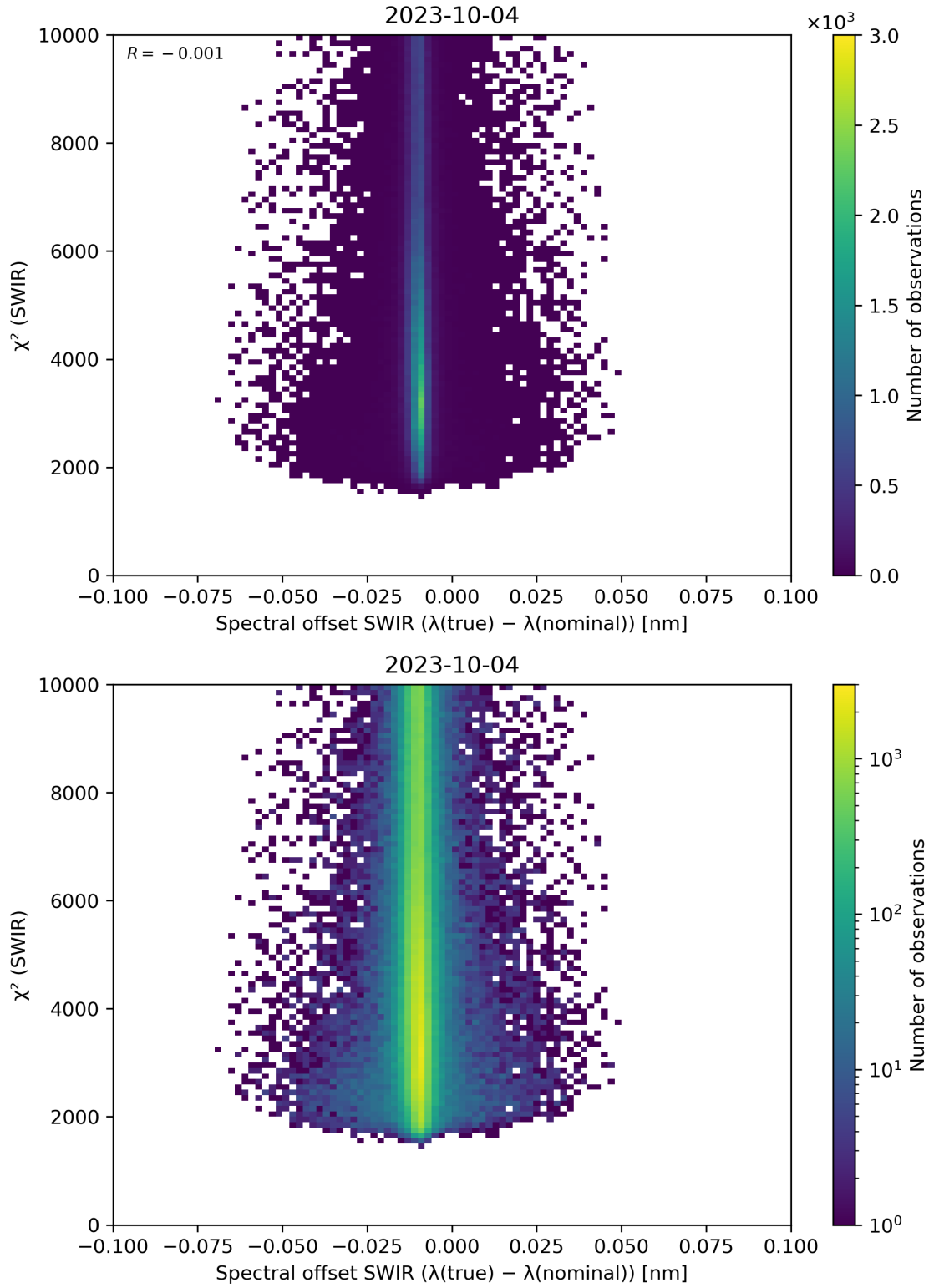
Figure 118: Scatter density plot of “Spectral offset SWIR ( \lambda(\text{true}) - \lambda(\text{nominal}) )” against “ \chi^2 (SWIR)” for 2023-10-03 to 2023-10-05.
