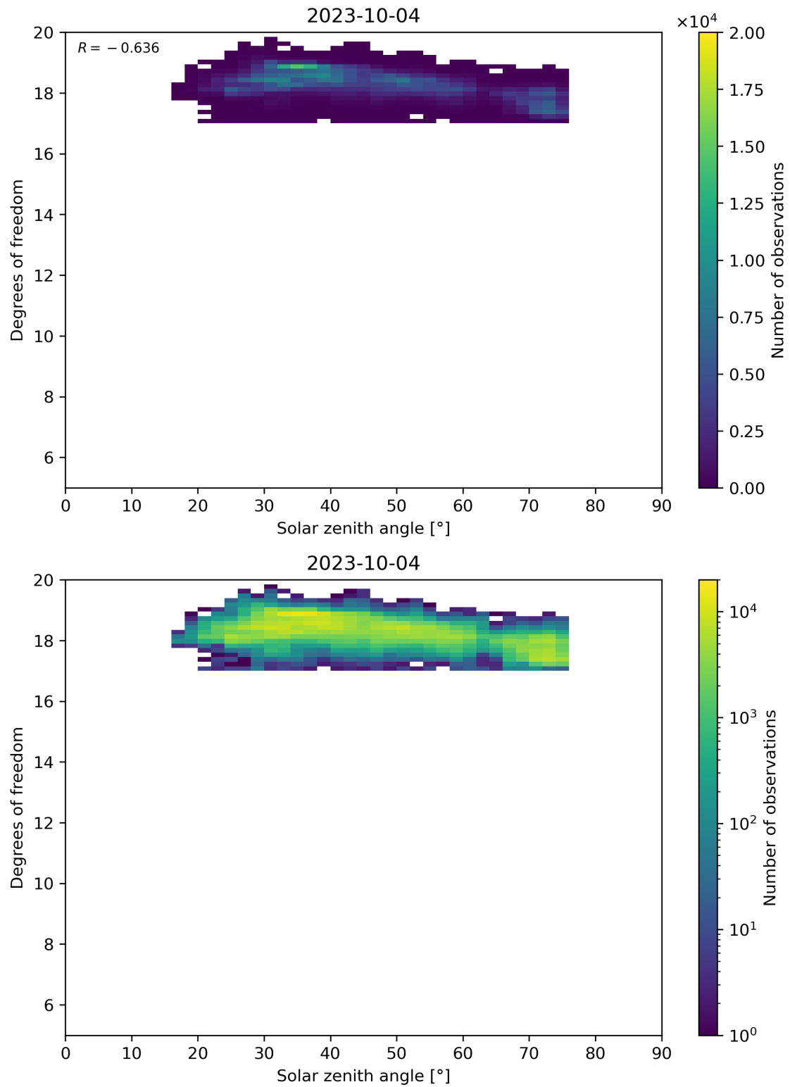
Figure 96: Scatter density plot of “Solar zenith angle” against “Degrees of freedom” for 2023-10-03 to 2023-10-05.
