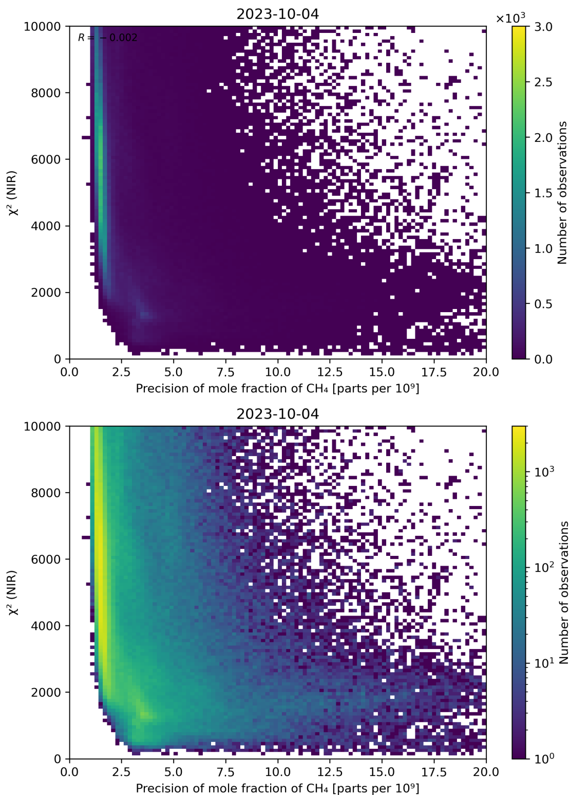
Figure 78: Scatter density plot of “Precision of mole fraction of CH 4 ” against “ \chi^2 (NIR)” for 2023-10-03 to 2023-10-05.
