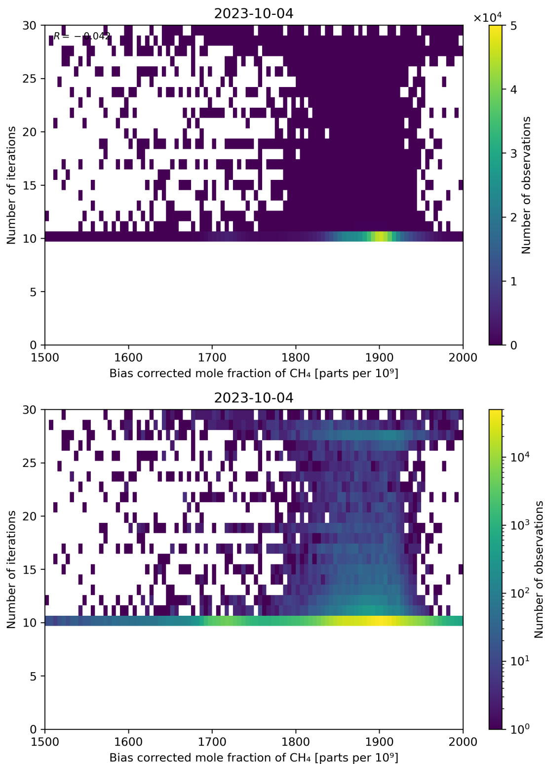
Figure 67: Scatter density plot of “Bias corrected mole fraction of CH 4 ” against “Number of iterations” for 2023-10-03 to 2023-10-05.
