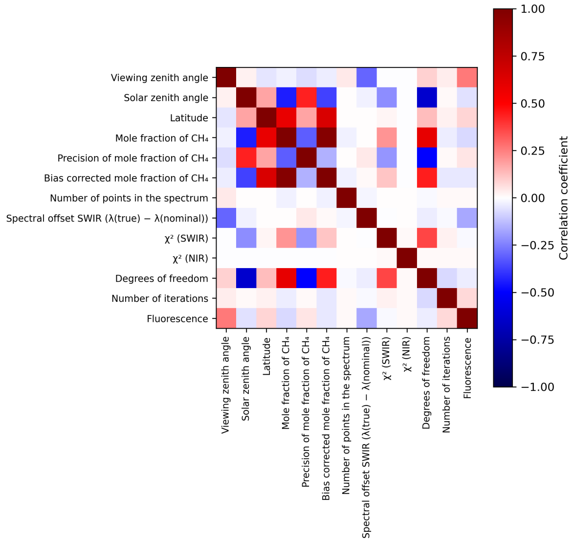
Figure 2: Map of correlation matrix for 2023-10-03 to 2023-10-05.
