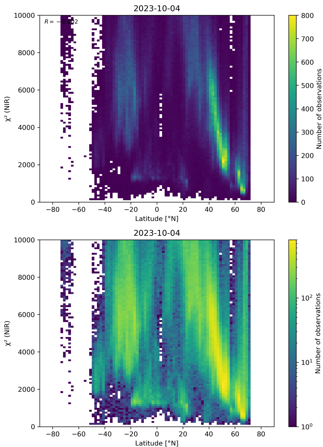
Figure 53: Scatter density plot of “Latitude” against “ \chi^2 (NIR)” for 2023-10-03 to 2023-10-05.
