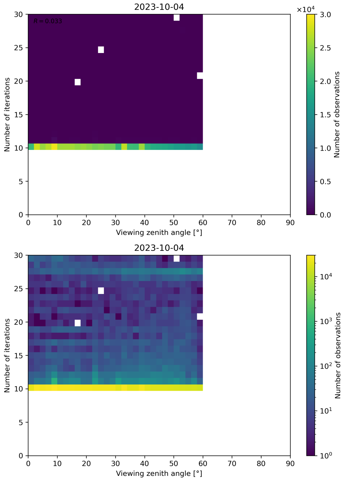
Figure 113: Scatter density plot of “Viewing zenith angle” against “Number of iterations” for 2023-10-03 to 2023-10-05.
