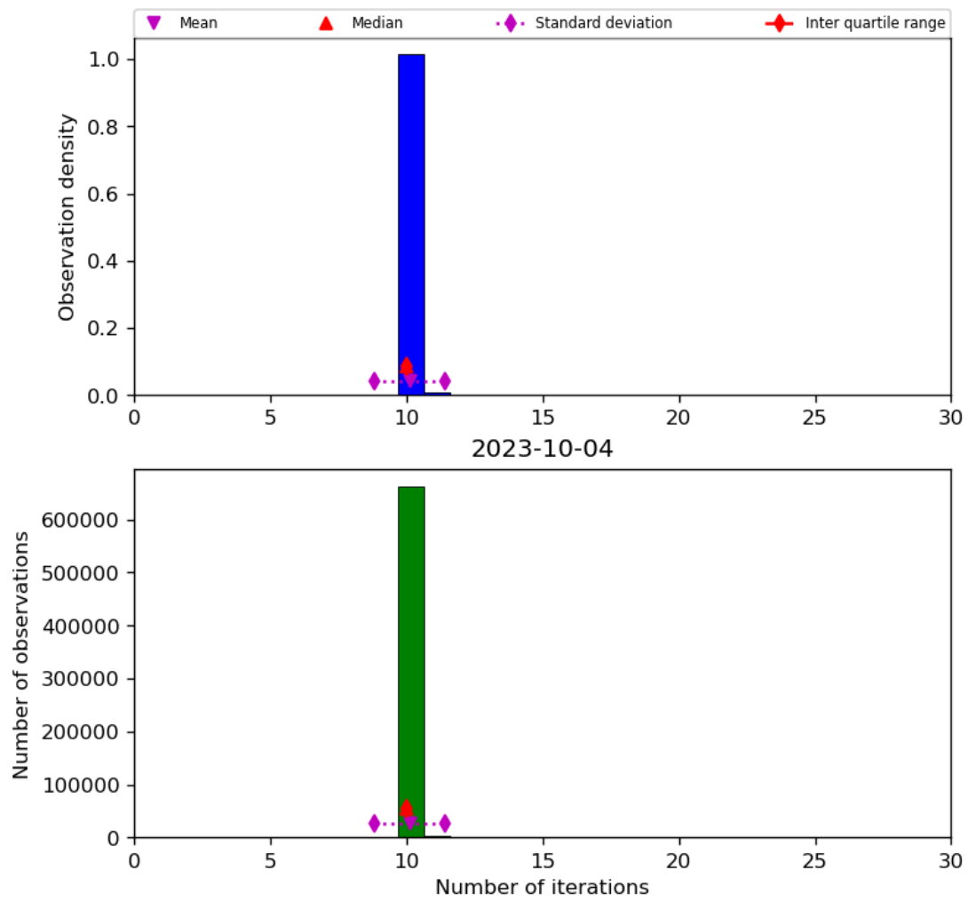
Figure 31: Histogram of “Number of iterations” for 2023-10-03 to 2023-10-05
