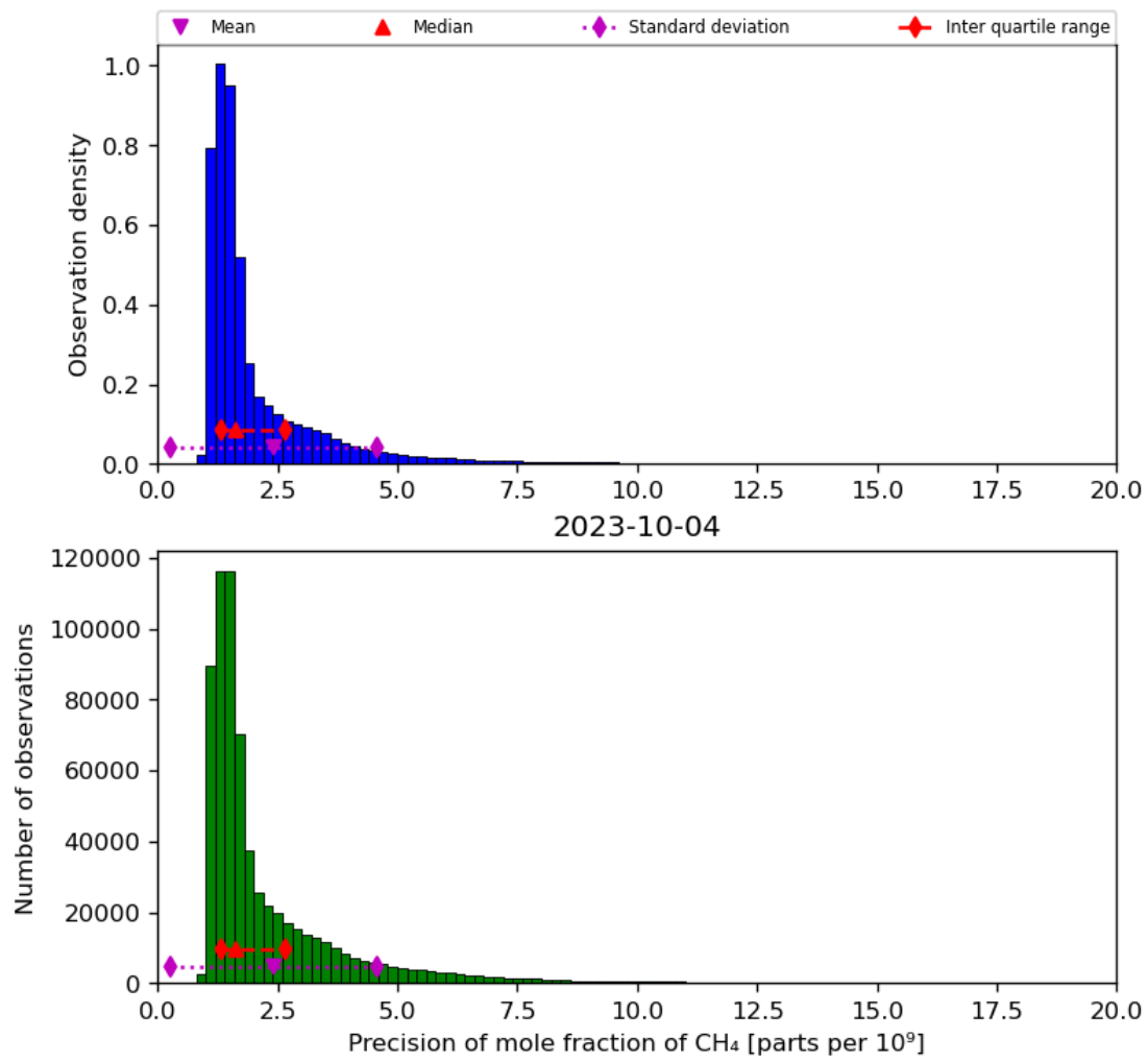
Figure 24: Histogram of “Precision of mole fraction of CH 4 ” for 2023-10-03 to 2023-10-05
