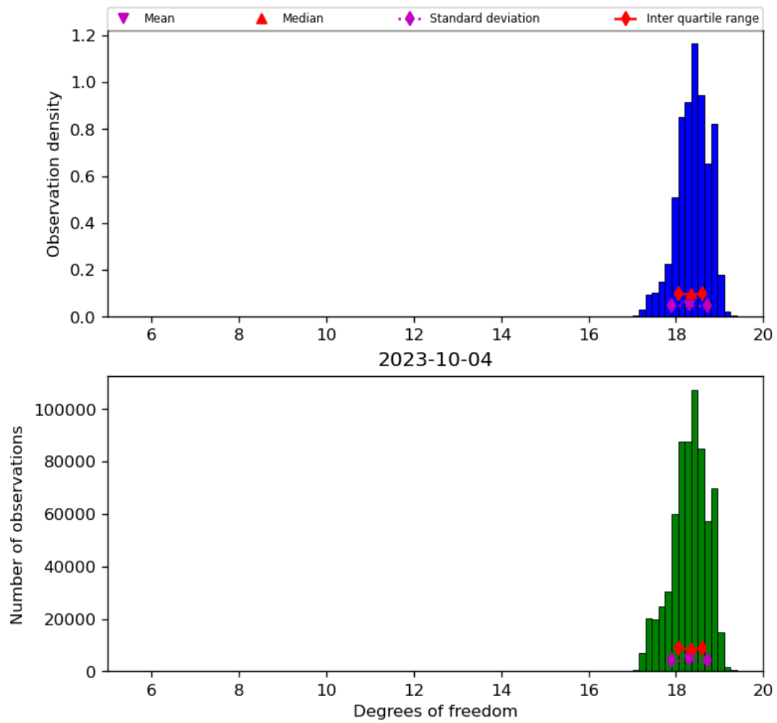
Figure 30: Histogram of “Degrees of freedom” for 2023-10-03 to 2023-10-05
