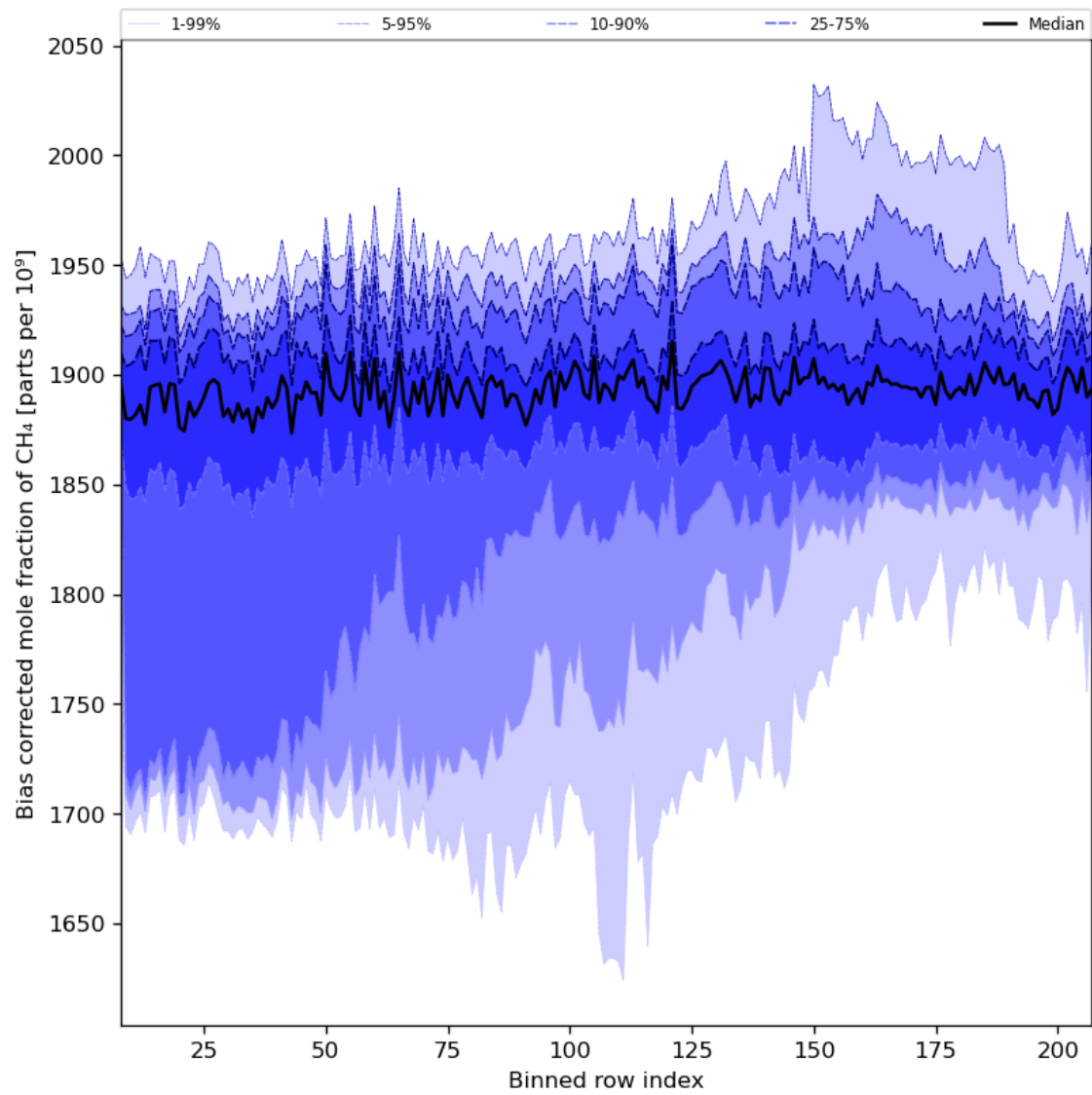
Figure 36: Along track statistics of “Bias corrected mole fraction of CH 4 ” for 2023-10-03 to 2023-10-05
