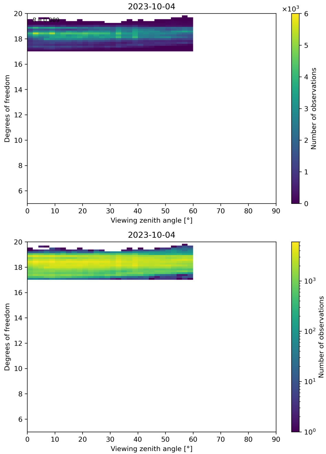
Figure 107: Scatter density plot of “Viewing zenith angle” against “Degrees of freedom” for 2023-10-03 to 2023-10-05.
