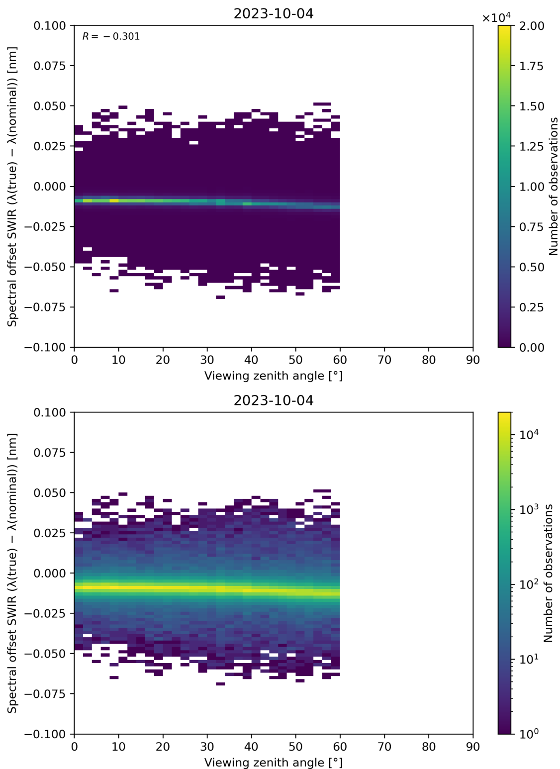
Figure 116: Scatter density plot of “Viewing zenith angle” against “Spectral offset SWIR ( \lambda(\text{true}) - \lambda(\text{nominal}) )” for 2023-10-03 to 2023-10-05.
