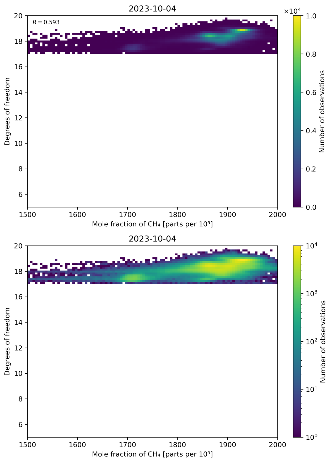
Figure 72: Scatter density plot of “Mole fraction of CH 4 ” against “Degrees of freedom” for 2023-10-03 to 2023-10-05.
