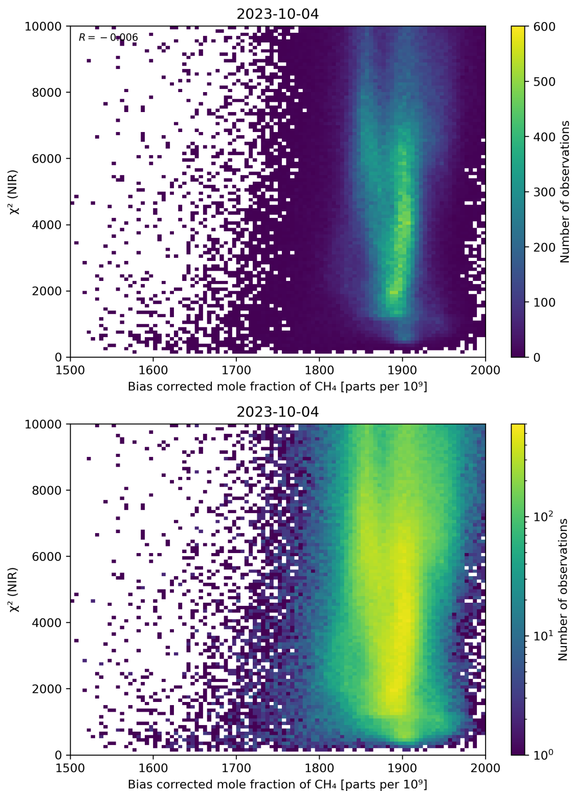
Figure 63: Scatter density plot of “Bias corrected mole fraction of CH 4 ” against “ \chi^2 (NIR)” for 2023-10-03 to 2023-10-05.
