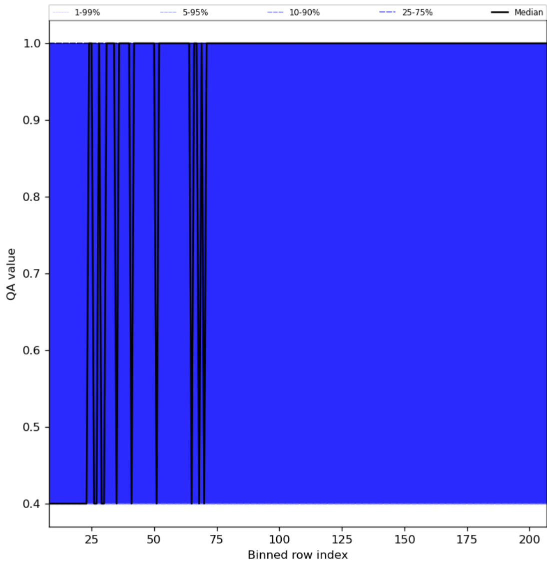
Figure 33: Along track statistics of “QA value” for 2023-10-03 to 2023-10-05
