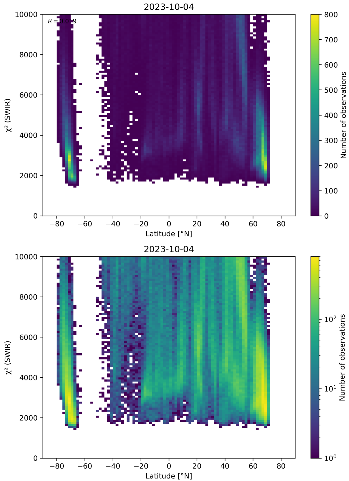
Figure 54: Scatter density plot of “Latitude” against “ \chi^2 (SWIR)” for 2023-10-03 to 2023-10-05.
