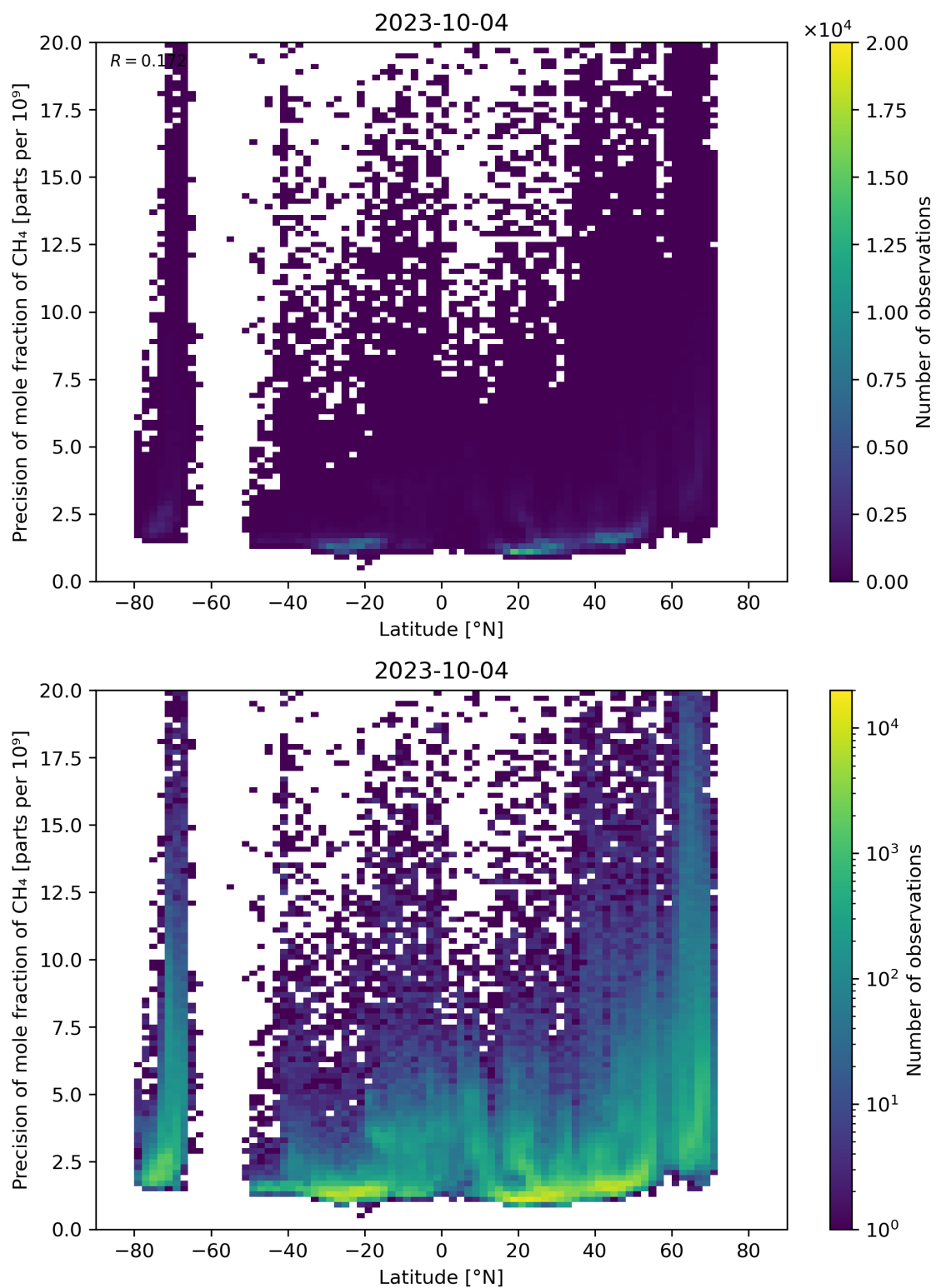
Figure 59: Scatter density plot of “Latitude” against “Precision of mole fraction of CH 4 ” for 2023-10-03 to 2023-10-05.
