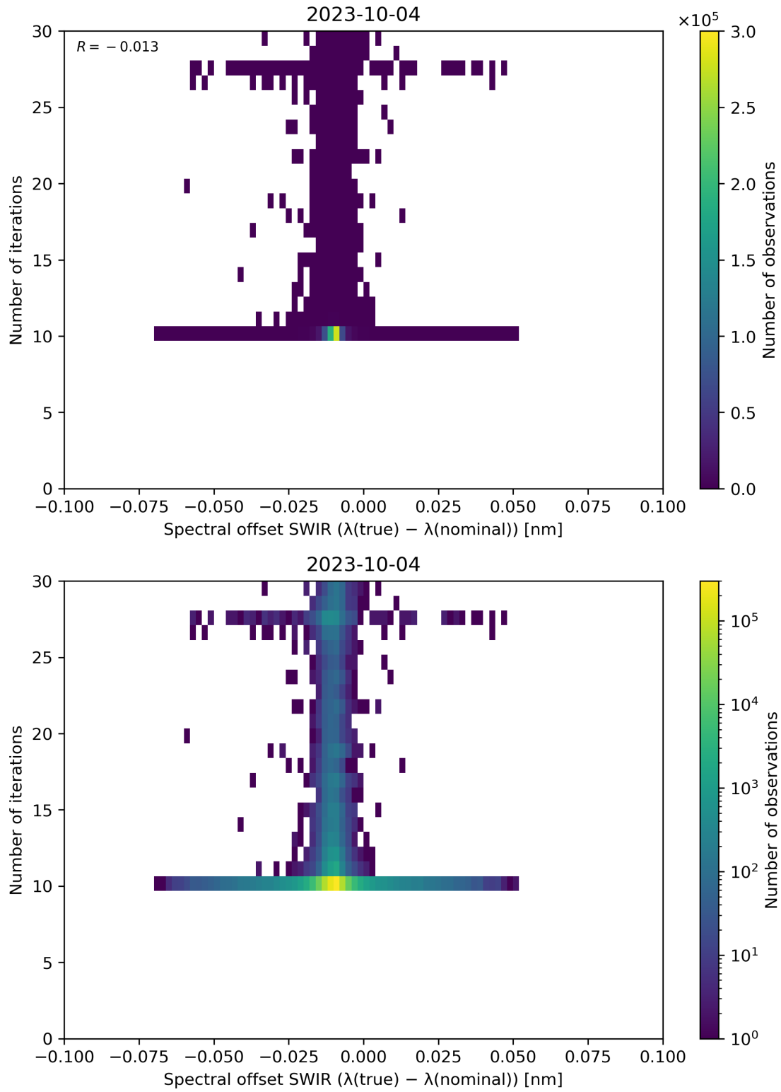
Figure 121: Scatter density plot of “Spectral offset SWIR ( \lambda(\text{true}) - \lambda(\text{nominal}) )” against “Number of iterations” for 2023-10-03 to 2023-10-05.
