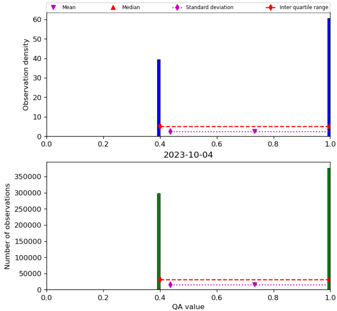
Figure 22: Histogram of “QA value” for 2023-10-03 to 2023-10-05
