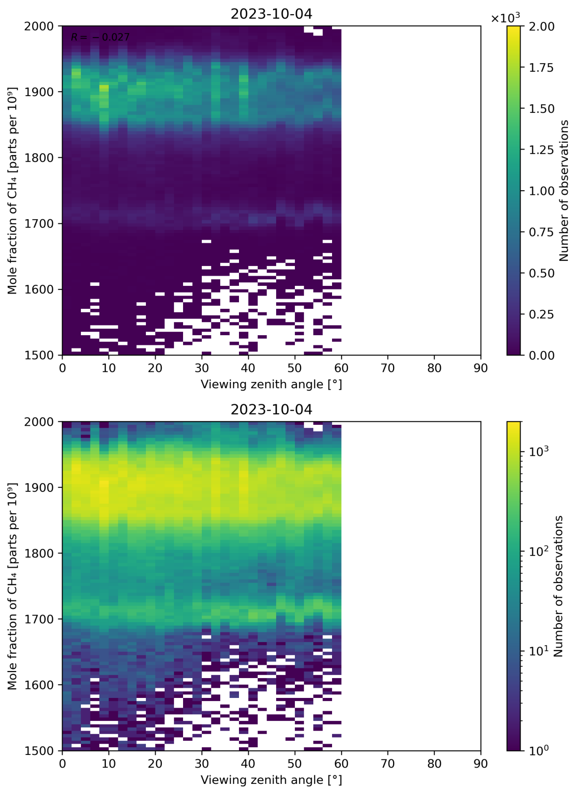
Figure 110: Scatter density plot of “Viewing zenith angle” against “Mole fraction of CH 4 ” for 2023-10-03 to 2023-10-05.
