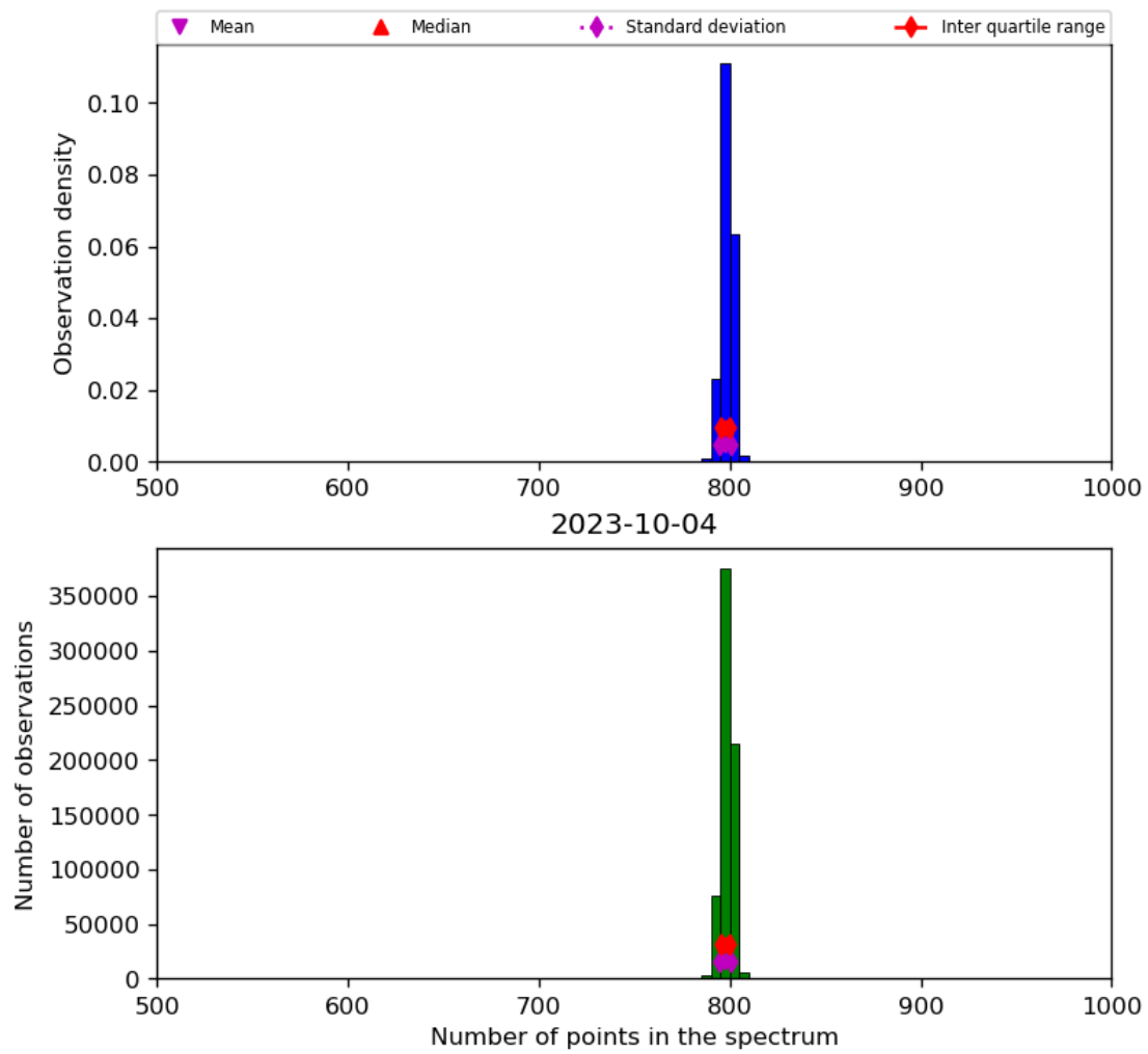
Figure 26: Histogram of “Number of points in the spectrum” for 2023-10-03 to 2023-10-05
