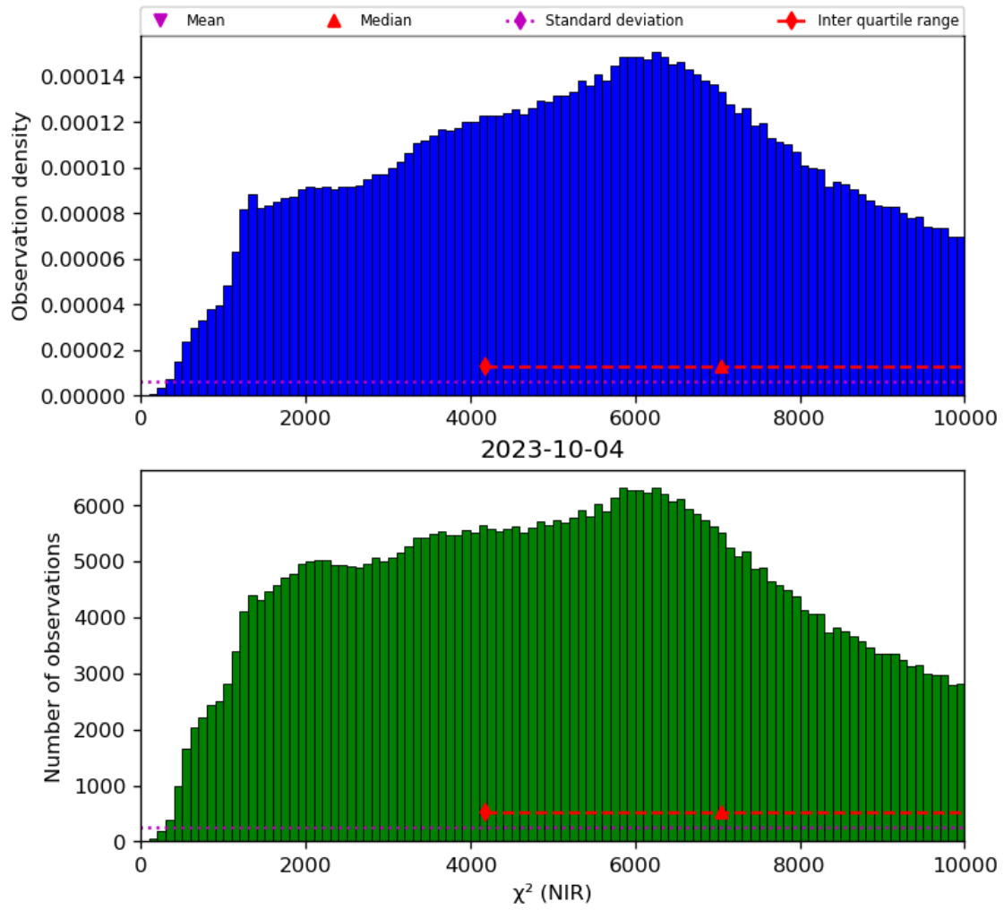
Figure 29: Histogram of “ \chi^2 (NIR)” for 2023-10-03 to 2023-10-05
