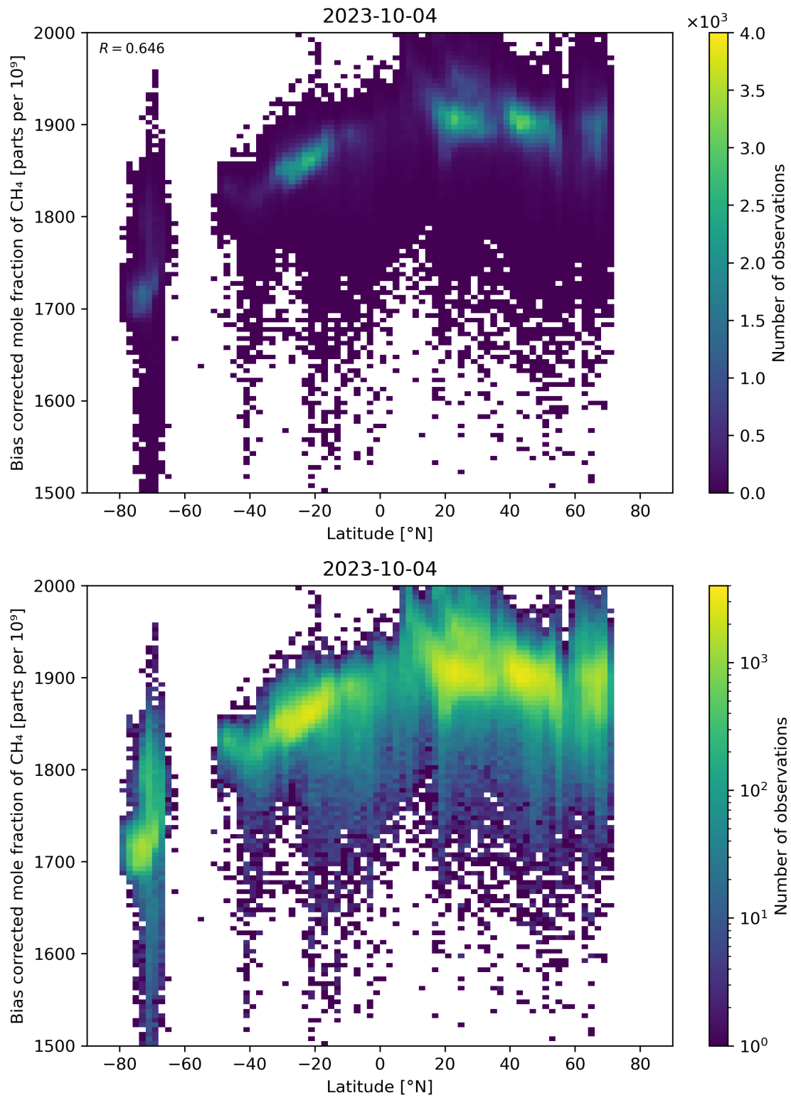
Figure 58: Scatter density plot of “Latitude” against “Bias corrected mole fraction of CH 4 ” for 2023-10-03 to 2023-10-05.
