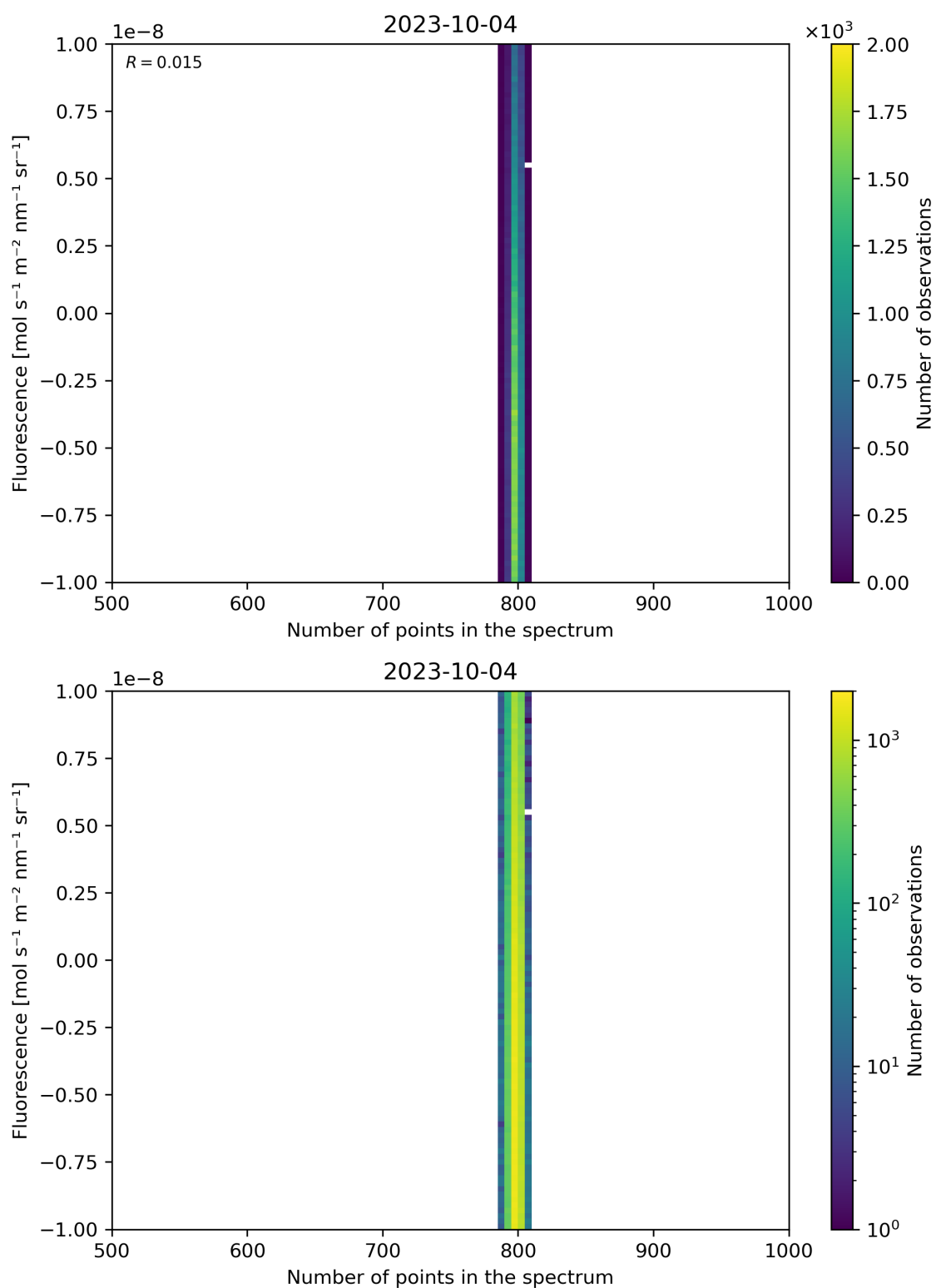
Figure 91: Scatter density plot of “Number of points in the spectrum” against “Fluorescence” for 2023-10-03 to 2023-10-05.
