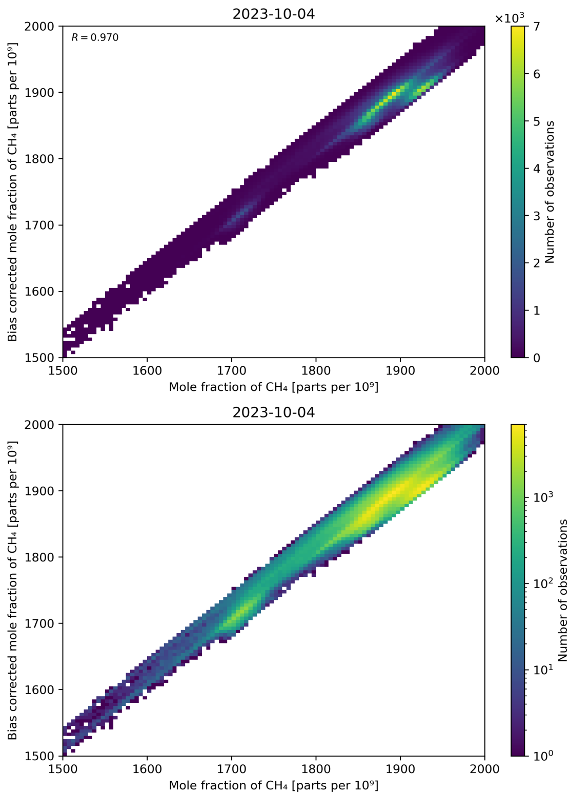
Figure 74: Scatter density plot of “Mole fraction of CH 4 ” against “Bias corrected mole fraction of CH 4 ” for 2023-10-03 to 2023-10-05.
