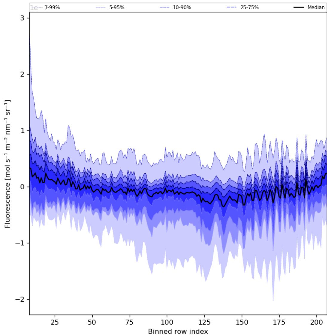
Figure 43: Along track statistics of “Fluorescence” for 2023-10-03 to 2023-10-05
