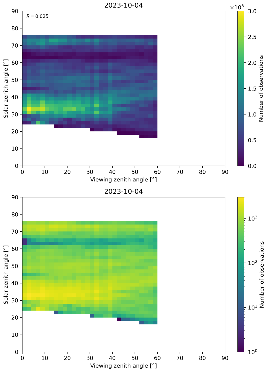
Figure 115: Scatter density plot of “Viewing zenith angle” against “Solar zenith angle” for 2023-10-03 to 2023-10-05.
