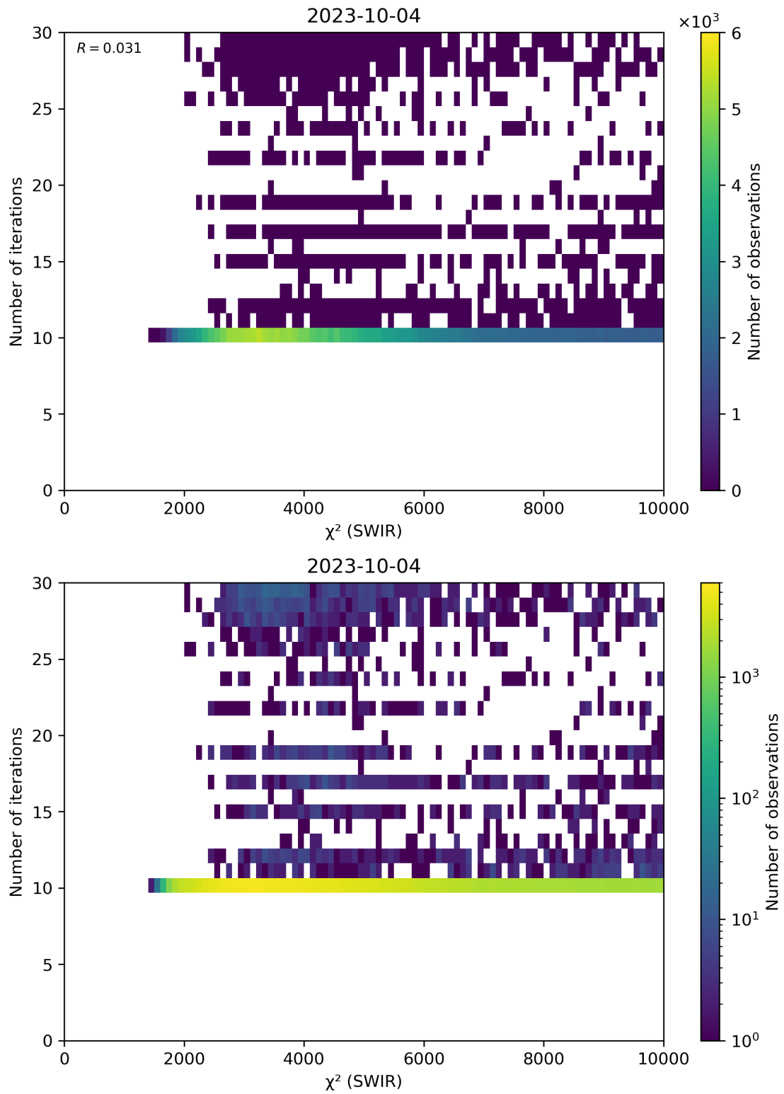
Figure 50: Scatter density plot of “ \chi^2 (SWIR)” against “Number of iterations” for 2023-10-03 to 2023-10-05.
