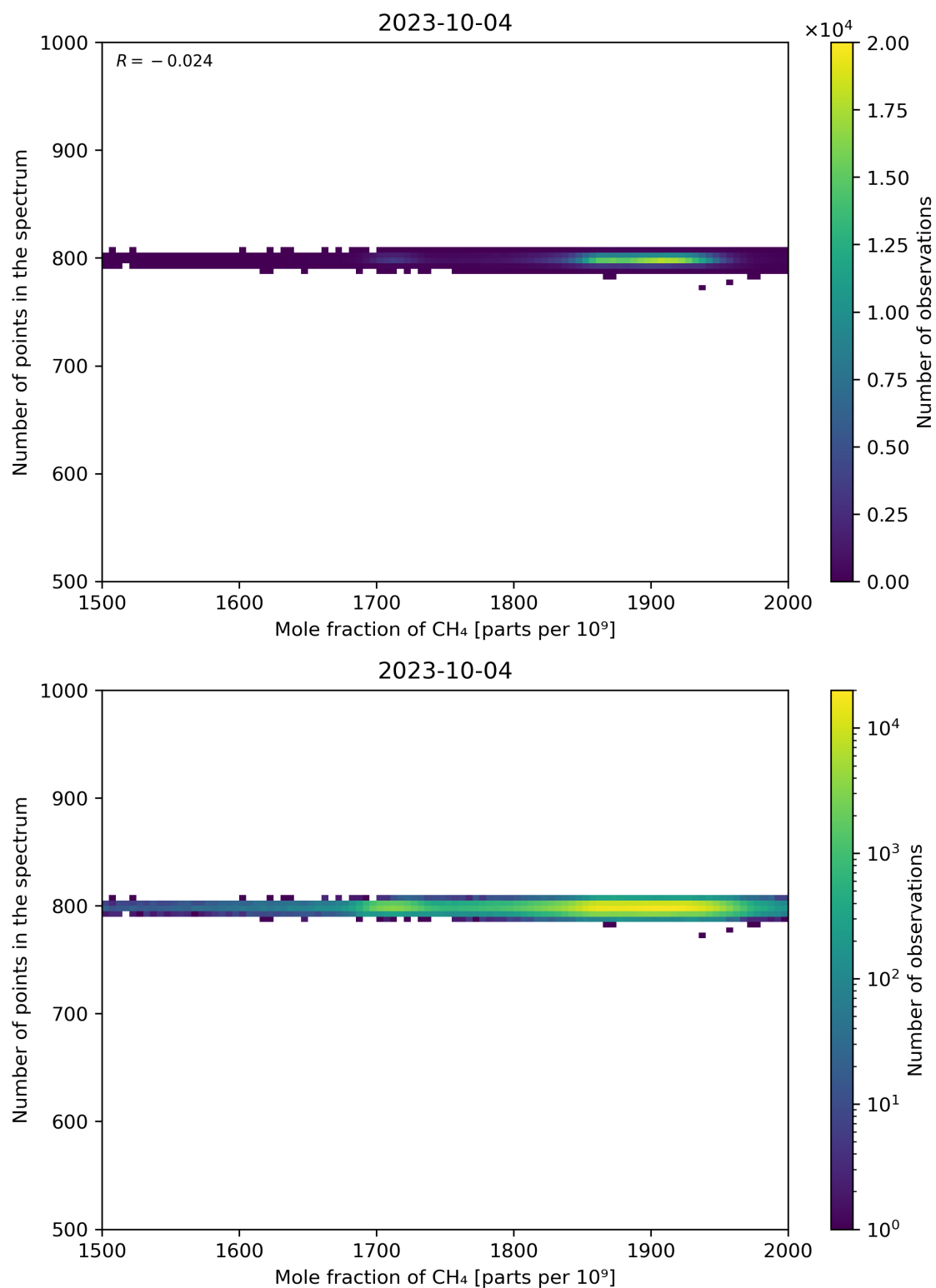
Figure 77: Scatter density plot of “Mole fraction of CH 4 ” against “Number of points in the spectrum” for 2023-10-03 to 2023-10-05.
