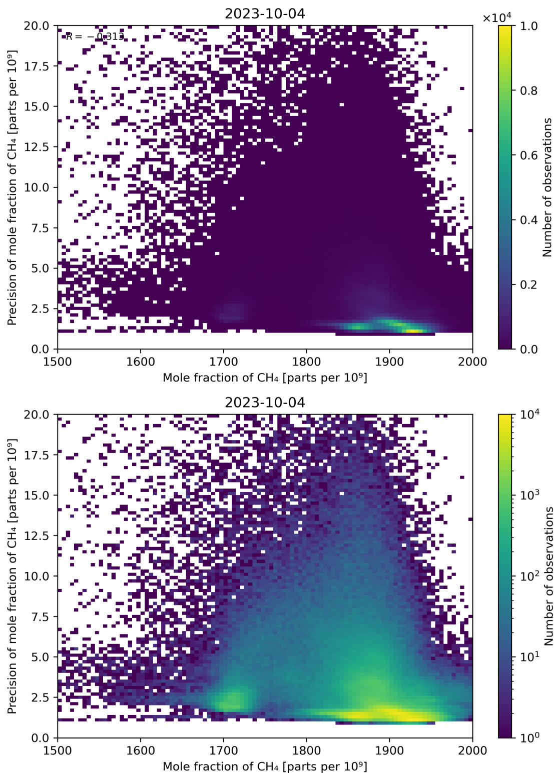
Figure 75: Scatter density plot of “Mole fraction of CH 4 ” against “Precision of mole fraction of CH 4 ” for 2023-10-03 to 2023-10-05.
