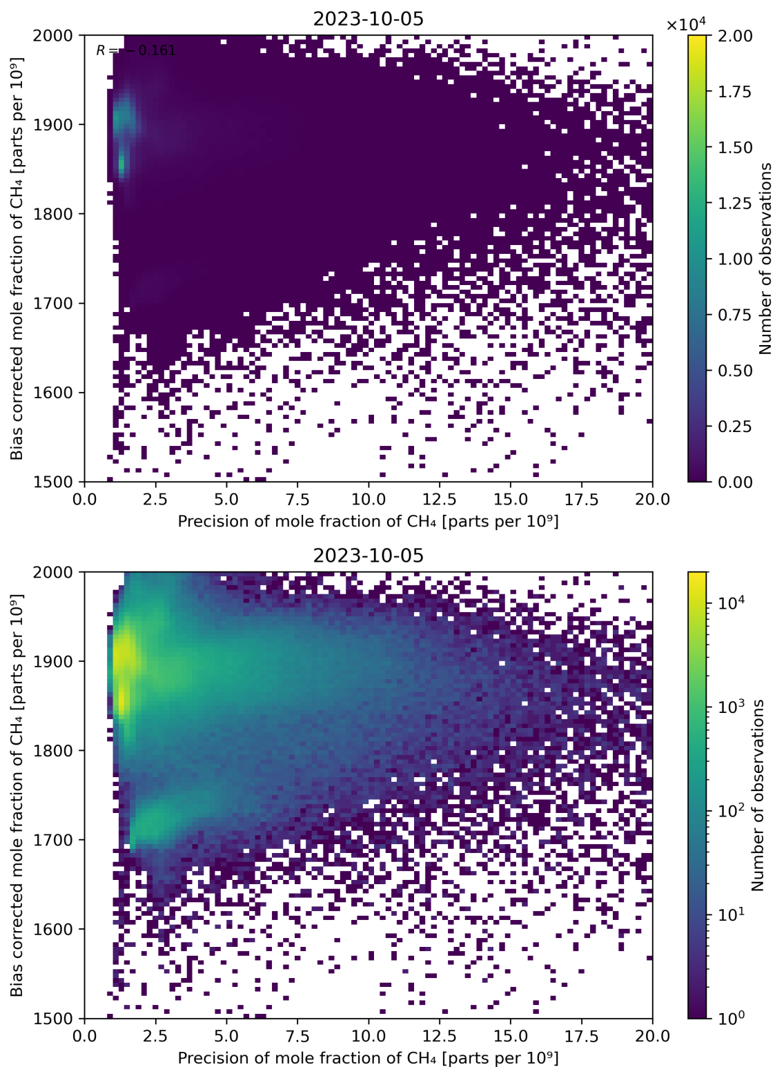
Figure 82: Scatter density plot of “Precision of mole fraction of CH 4 ” against “Bias corrected mole fraction of CH 4 ” for 2023-10-04 to 2023-10-06.
