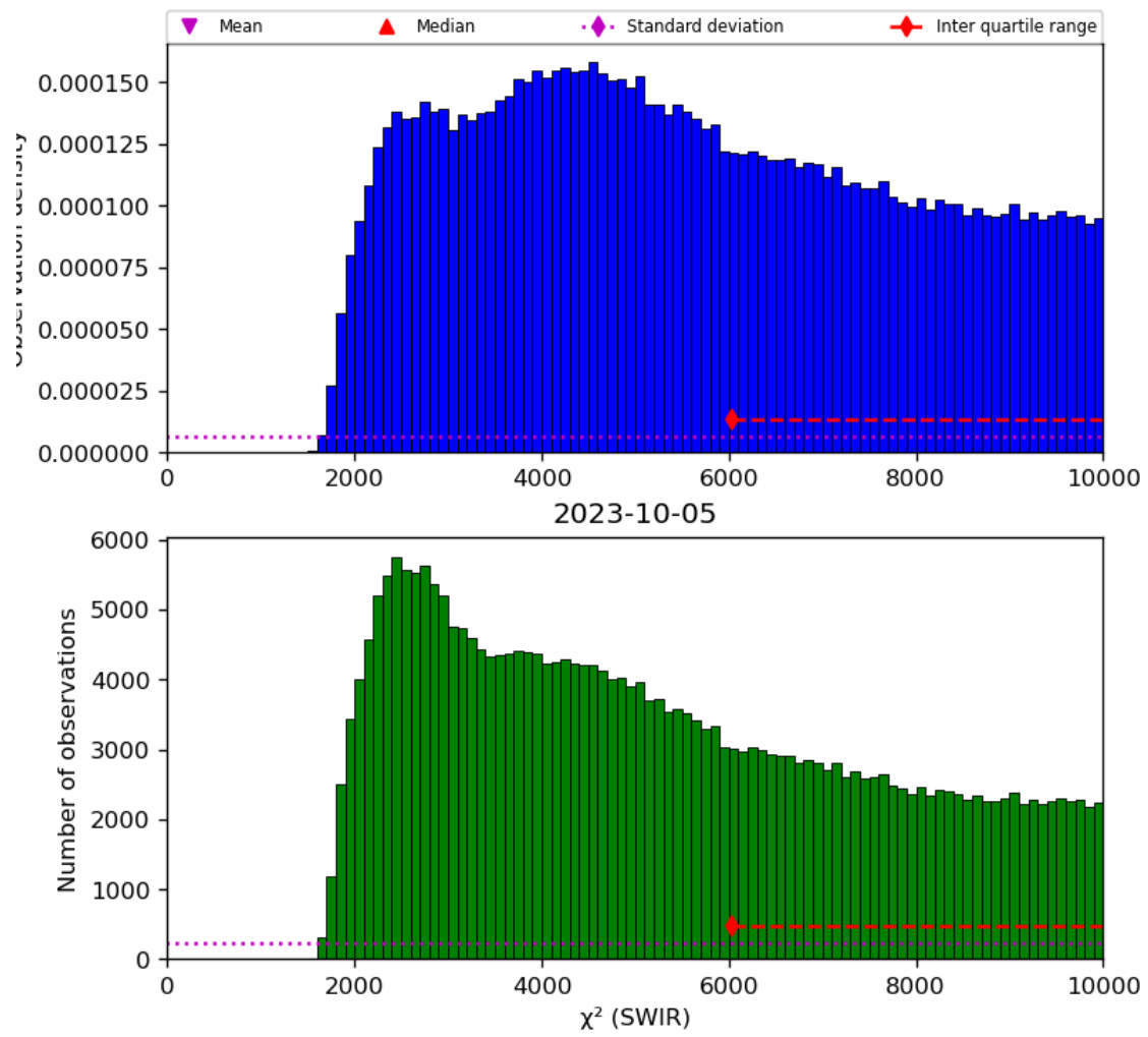
Figure 28: Histogram of “ \chi^2 (SWIR)” for 2023-10-04 to 2023-10-06
