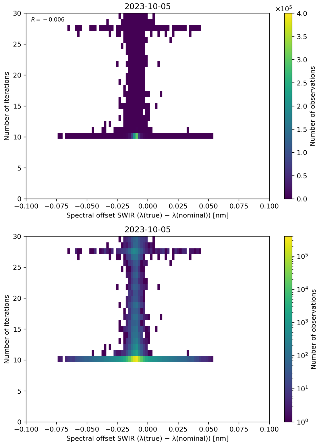
Figure 121: Scatter density plot of “Spectral offset SWIR ( \lambda(\text{true}) - \lambda(\text{nominal}) )” against “Number of iterations” for 2023-10-04 to 2023-10-06.
