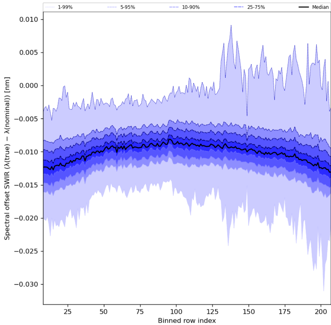
Figure 38: Along track statistics of “Spectral offset SWIR ( \lambda(\text{true}) - \lambda(\text{nominal}) )” for 2023-10-04 to 2023-10-06
