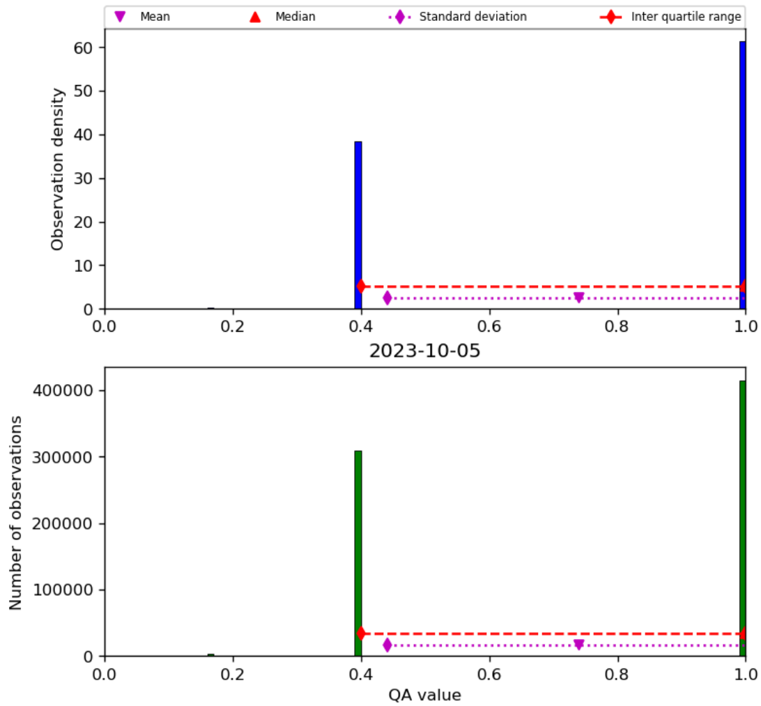
Figure 22: Histogram of “QA value” for 2023-10-04 to 2023-10-06
