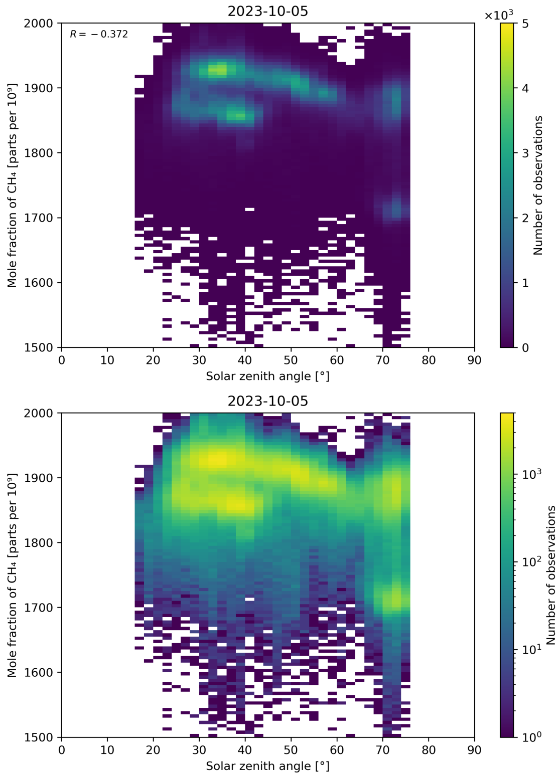
Figure 99: Scatter density plot of “Solar zenith angle” against “Mole fraction of CH 4 ” for 2023-10-04 to 2023-10-06.
