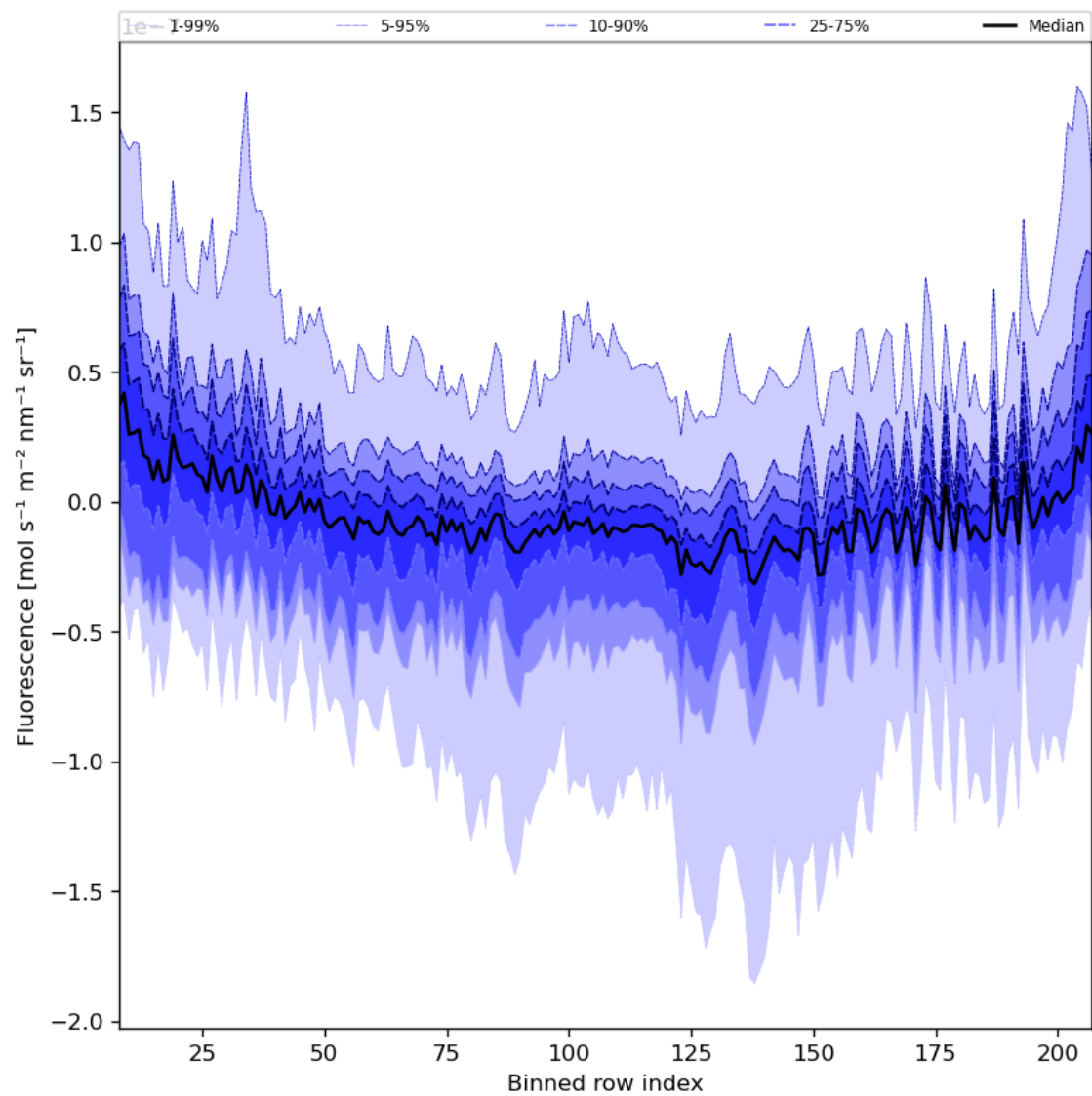
Figure 43: Along track statistics of “Fluorescence” for 2023-10-04 to 2023-10-06
