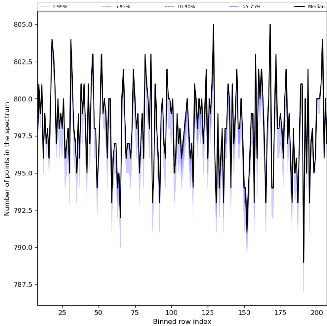
Figure 37: Along track statistics of “Number of points in the spectrum” for 2023-10-04 to 2023-10-06
