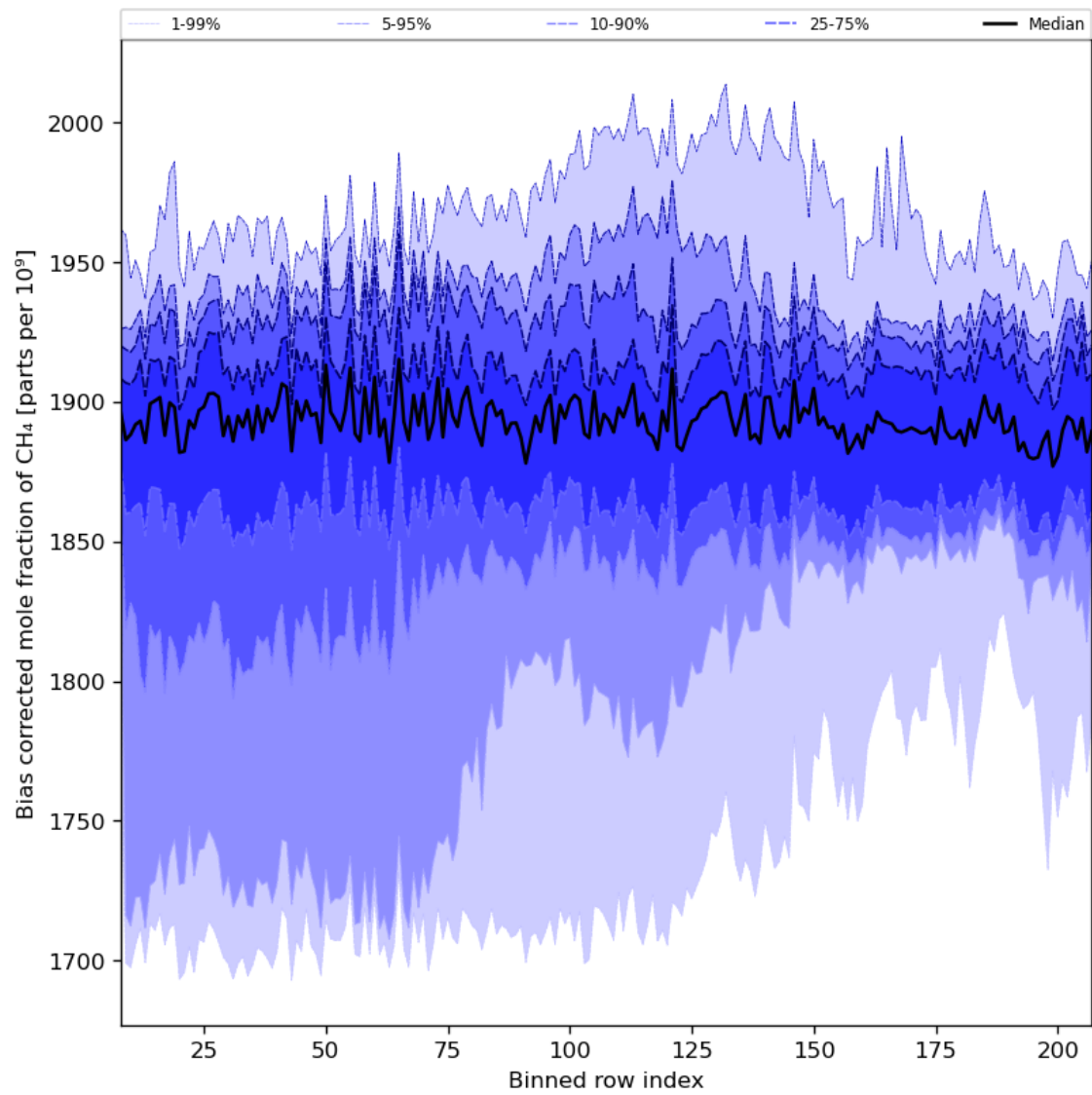
Figure 36: Along track statistics of “Bias corrected mole fraction of CH 4 ” for 2023-10-04 to 2023-10-06
