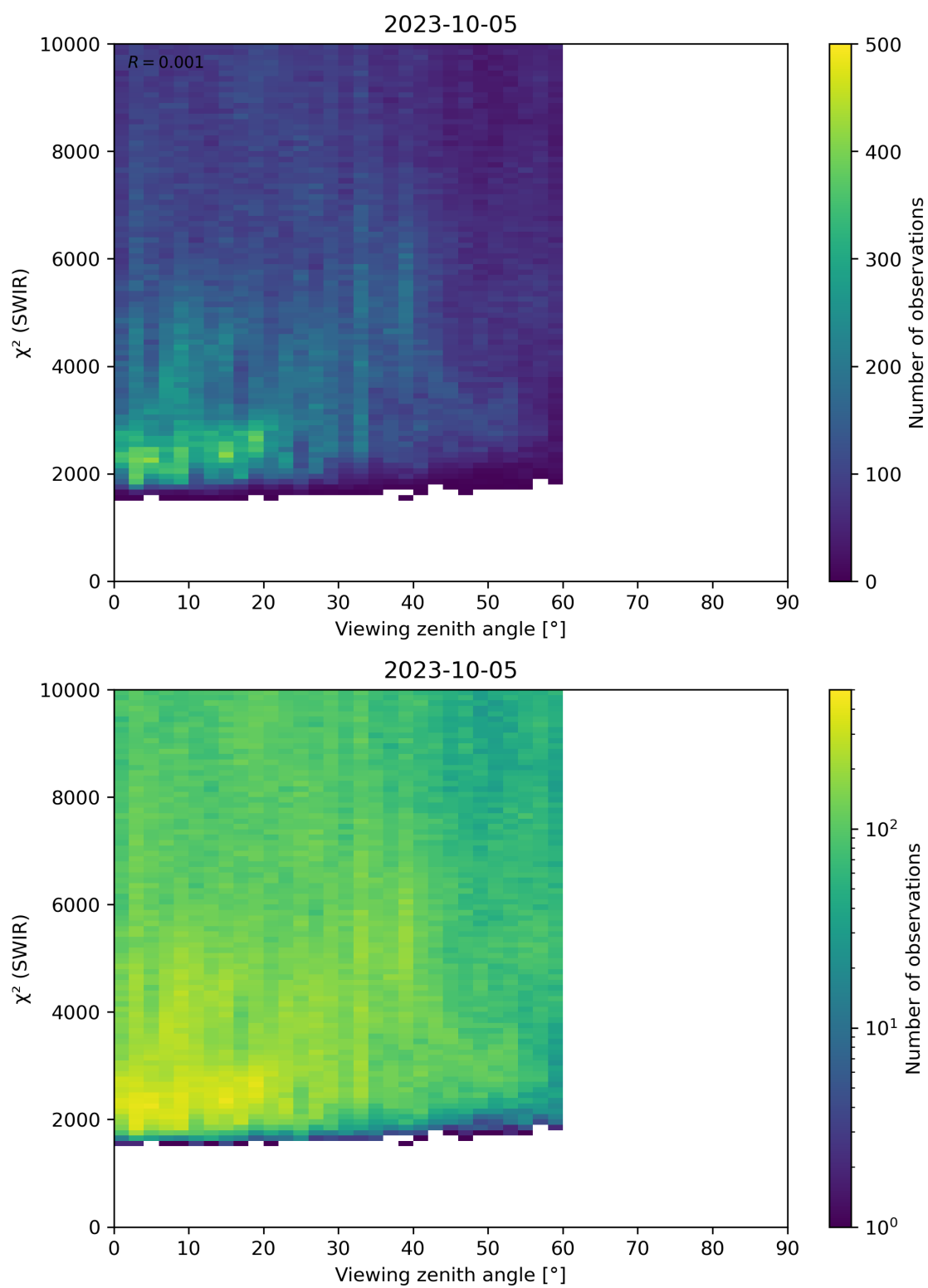
Figure 106: Scatter density plot of “Viewing zenith angle” against “ \chi^2 (SWIR)” for 2023-10-04 to 2023-10-06.
