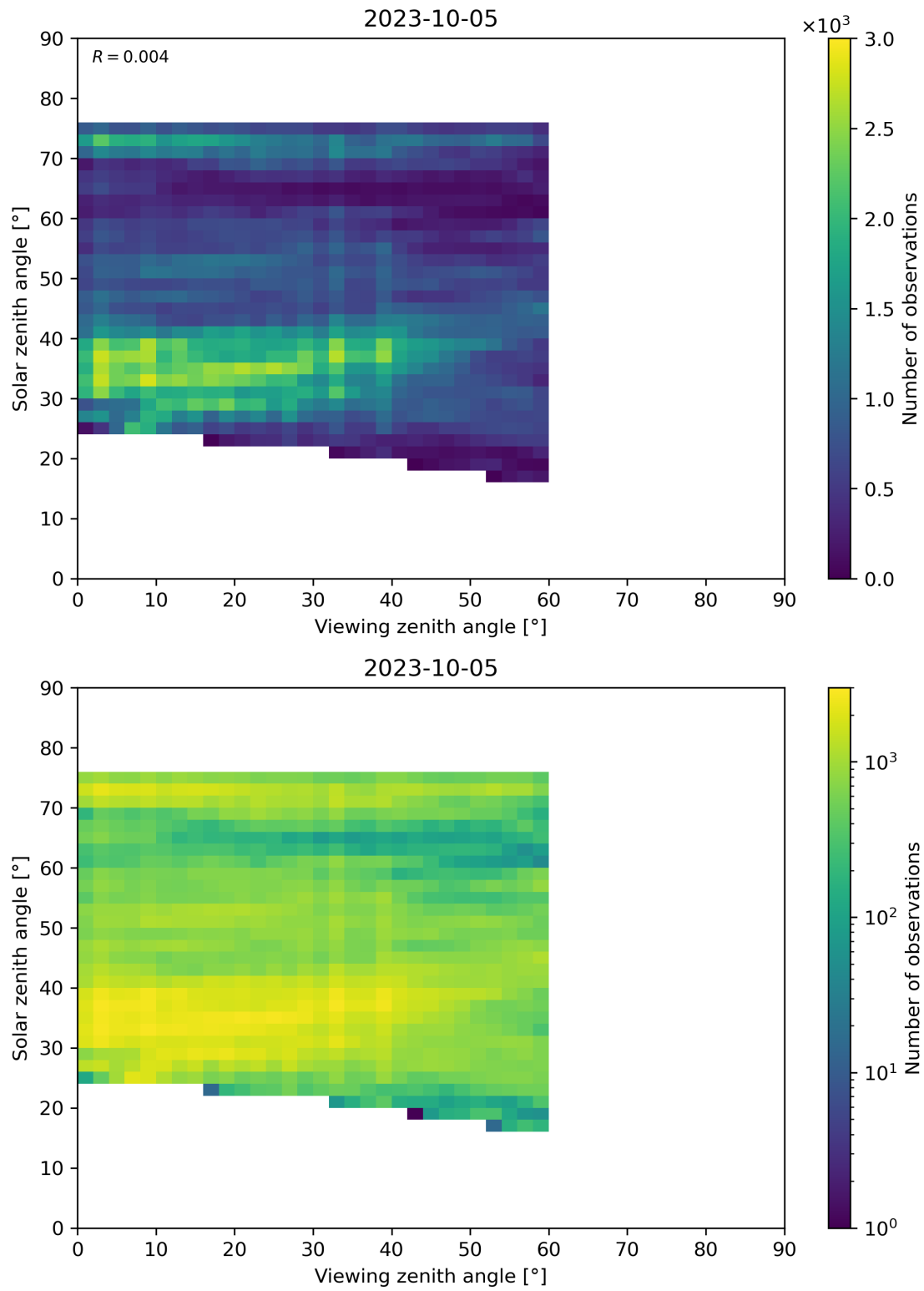
Figure 115: Scatter density plot of “Viewing zenith angle” against “Solar zenith angle” for 2023-10-04 to 2023-10-06.
