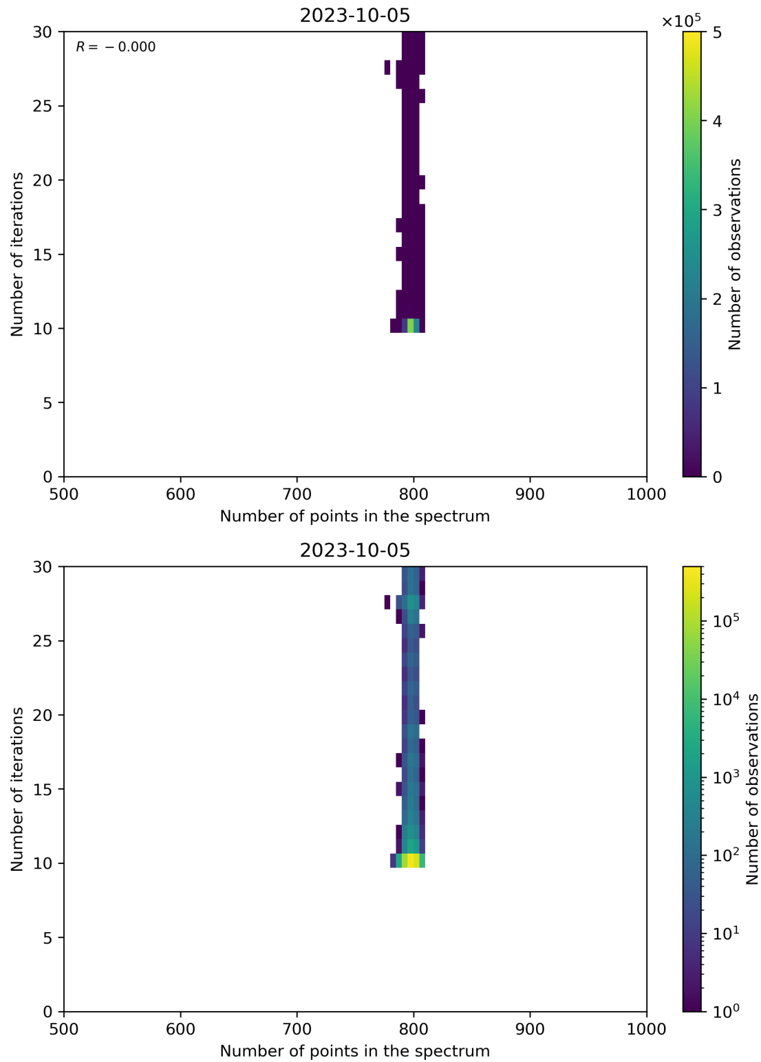
Figure 92: Scatter density plot of “Number of points in the spectrum” against “Number of iterations” for 2023-10-04 to 2023-10-06.
