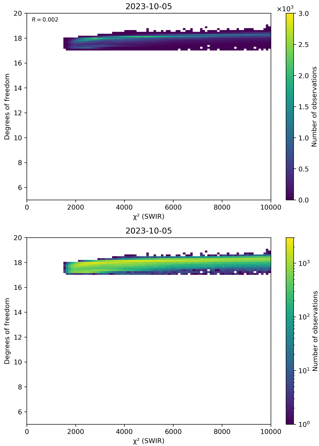
Figure 48: Scatter density plot of “ \chi^2 (SWIR)” against “Degrees of freedom” for 2023-10-04 to 2023-10-06.
