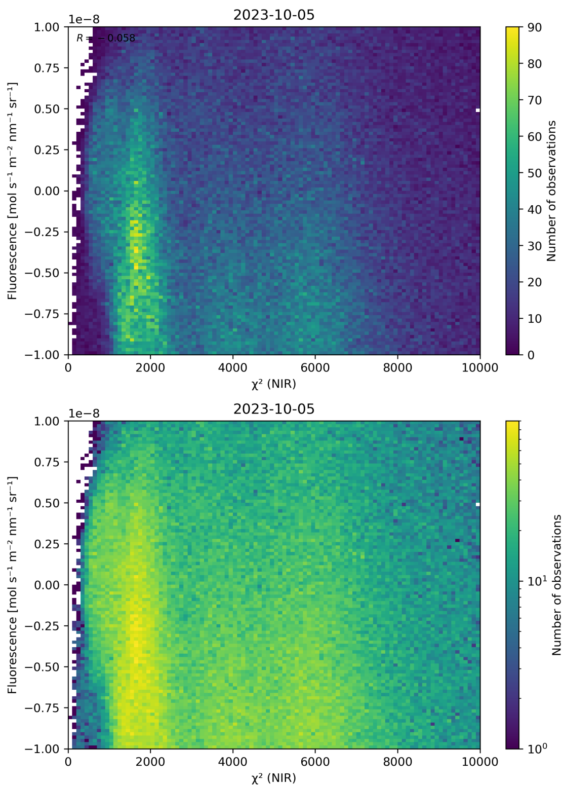
Figure 45: Scatter density plot of “ \chi^2 (NIR)” against “Fluorescence” for 2023-10-04 to 2023-10-06.
