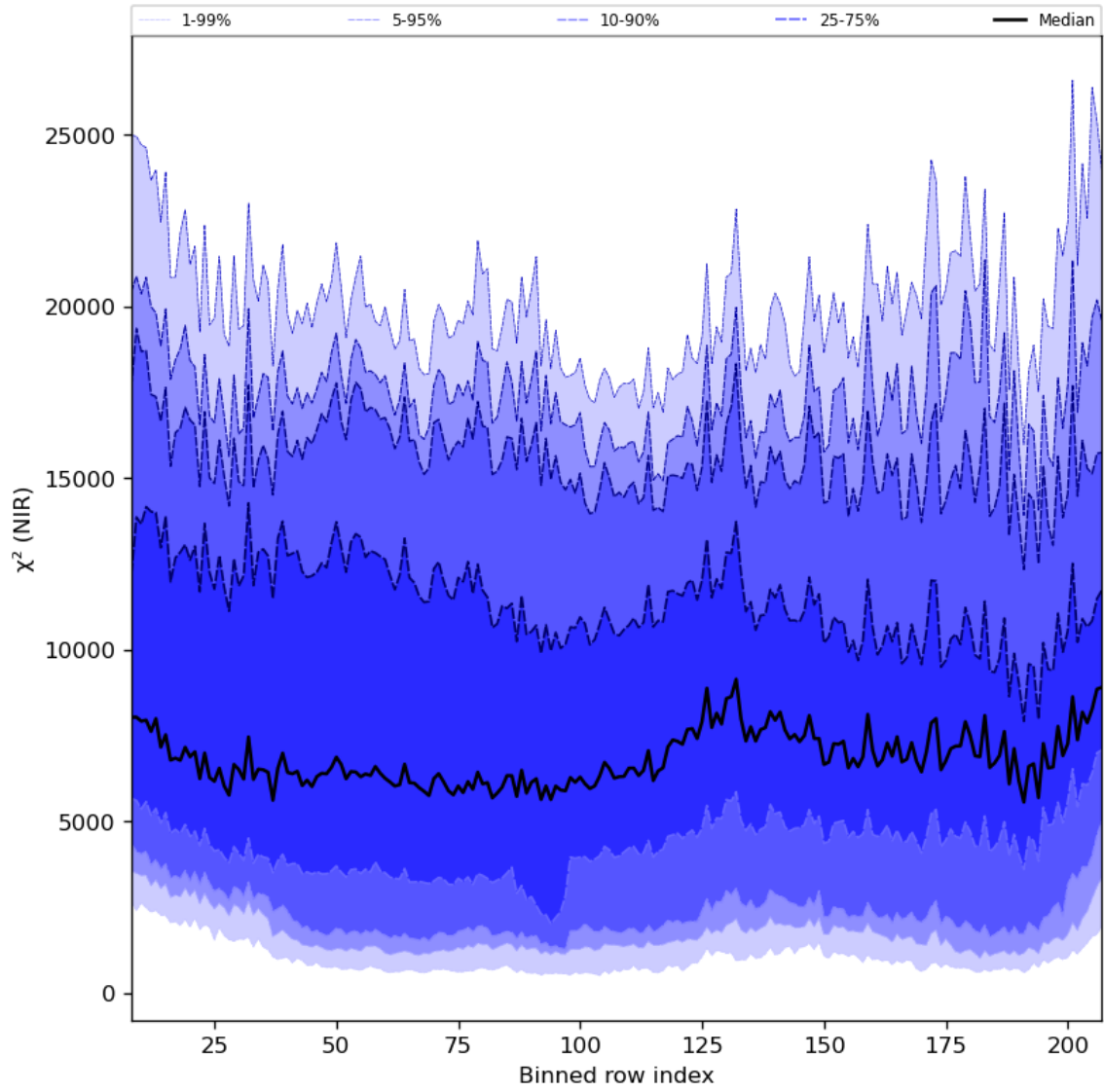
Figure 40: Along track statistics of " \chi^2 (NIR)" for 2023-10-04 to 2023-10-06
