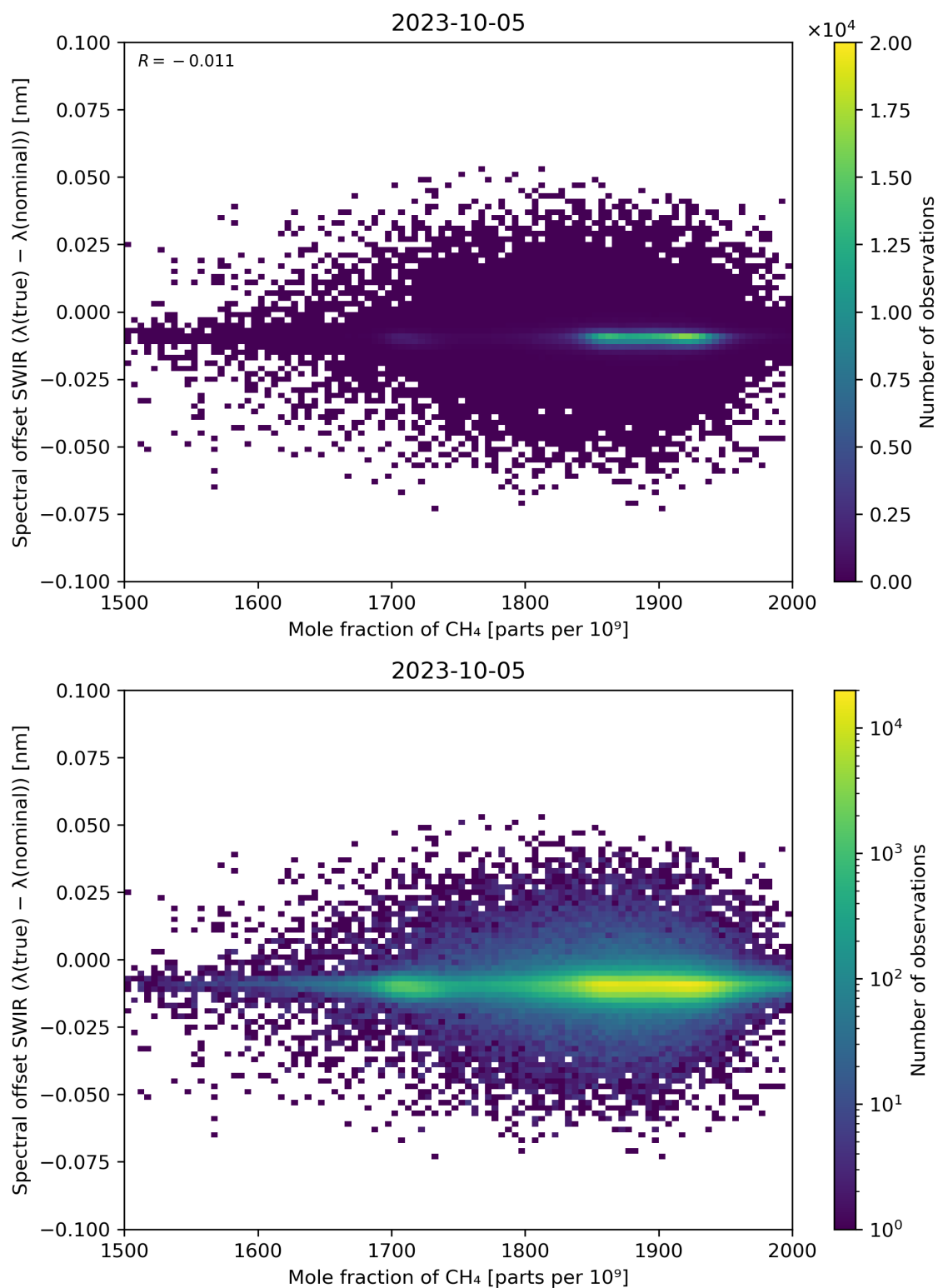
Figure 86: Scatter density plot of “Mole fraction of CH 4 ” against “Spectral offset SWIR ( \lambda(\text{true}) - \lambda(\text{nominal}) )” for 2023-10-04 to 2023-10-06.
