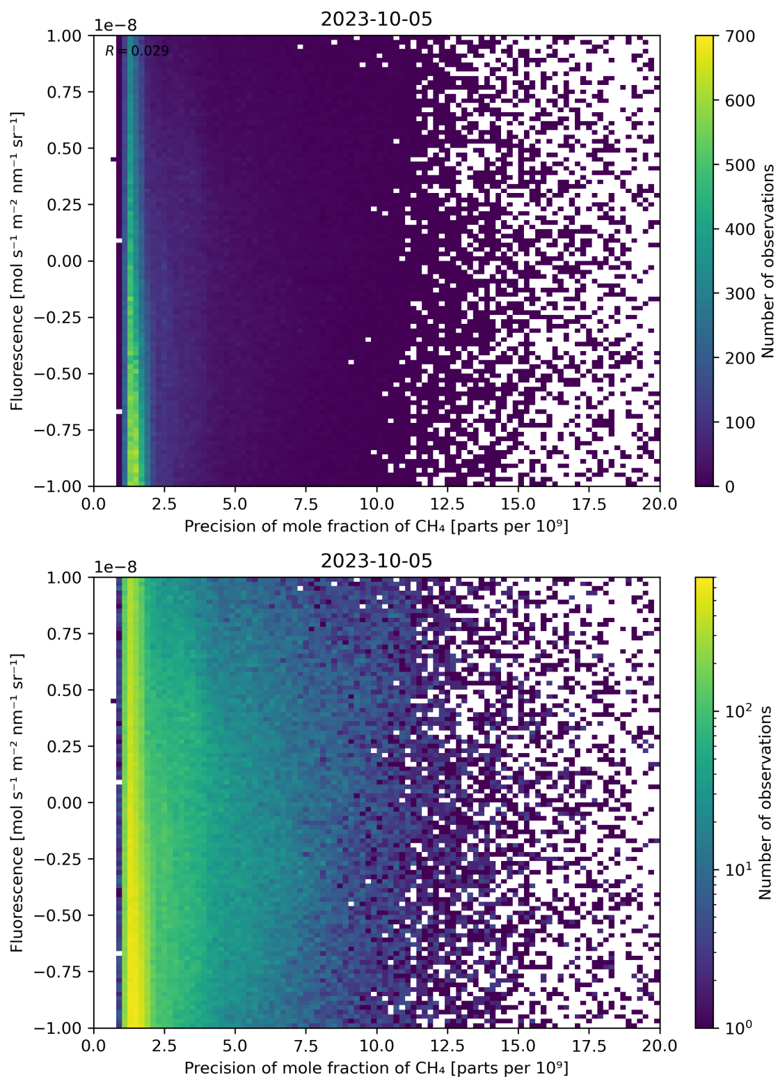
Figure 81: Scatter density plot of “Precision of mole fraction of \text{CH}_4 ” against “Fluorescence” for 2023-10-04 to 2023-10-06.
