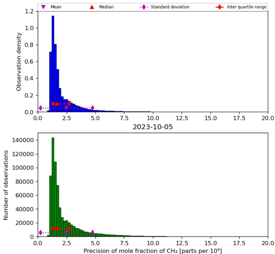
Figure 24: Histogram of “Precision of mole fraction of CH 4 ” for 2023-10-04 to 2023-10-06
