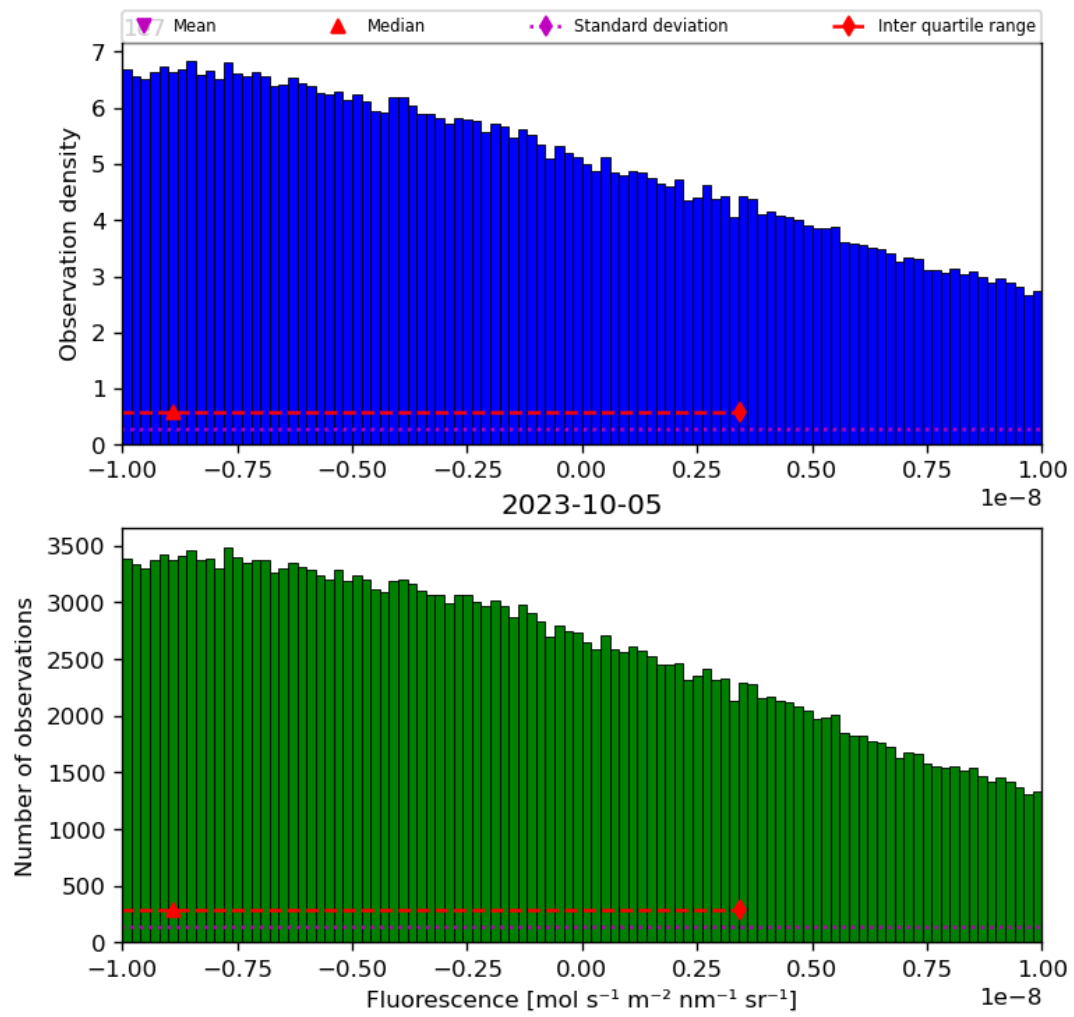
Figure 32: Histogram of “Fluorescence” for 2023-10-04 to 2023-10-06
