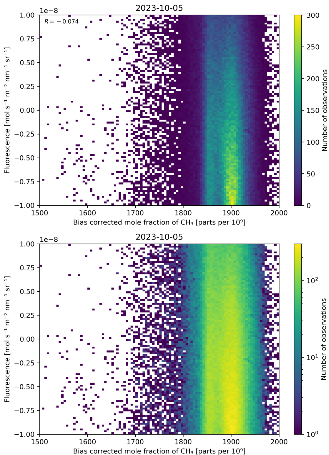
Figure 66: Scatter density plot of “Bias corrected mole fraction of \text{CH}_4 ” against “Fluorescence” for 2023-10-04 to 2023-10-06.
