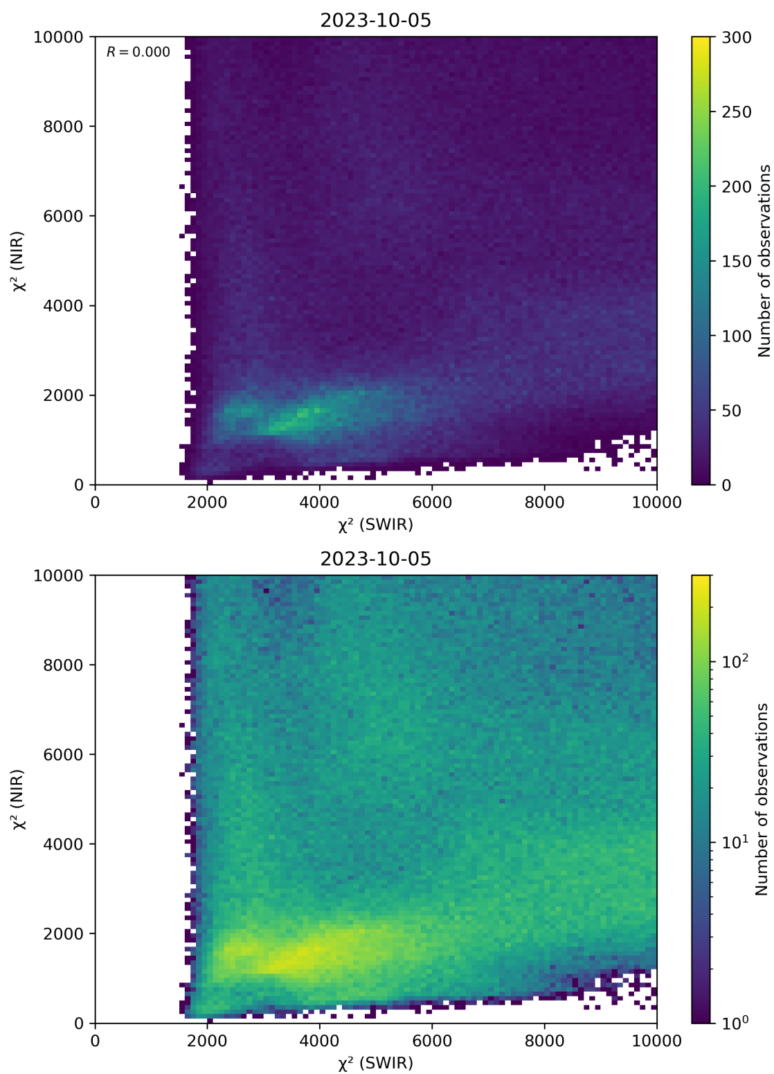
Figure 47: Scatter density plot of “ \chi^2 (SWIR)” against “ \chi^2 (NIR)” for 2023-10-04 to 2023-10-06.
