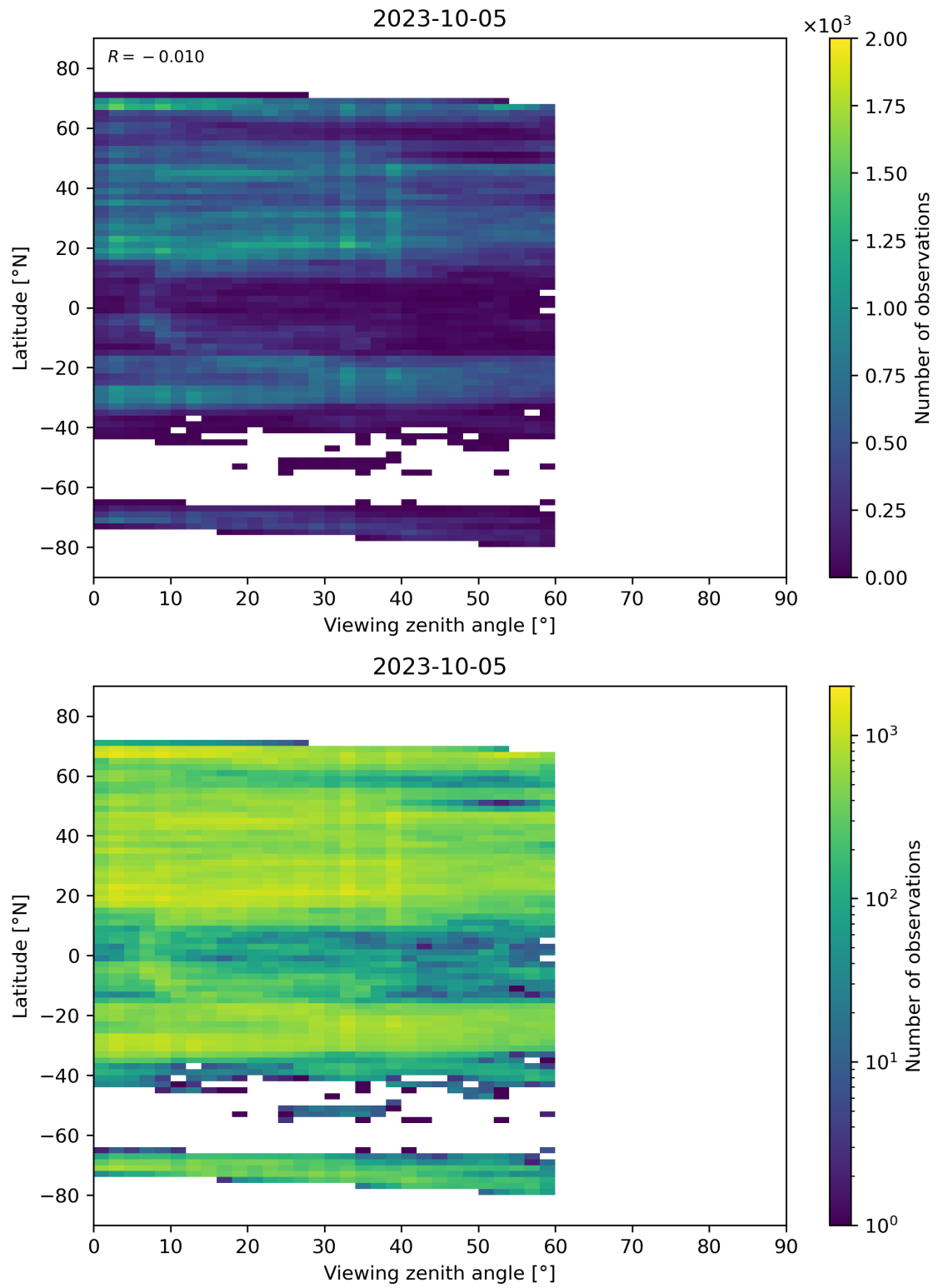
Figure 109: Scatter density plot of “Viewing zenith angle” against “Latitude” for 2023-10-04 to 2023-10-06.
