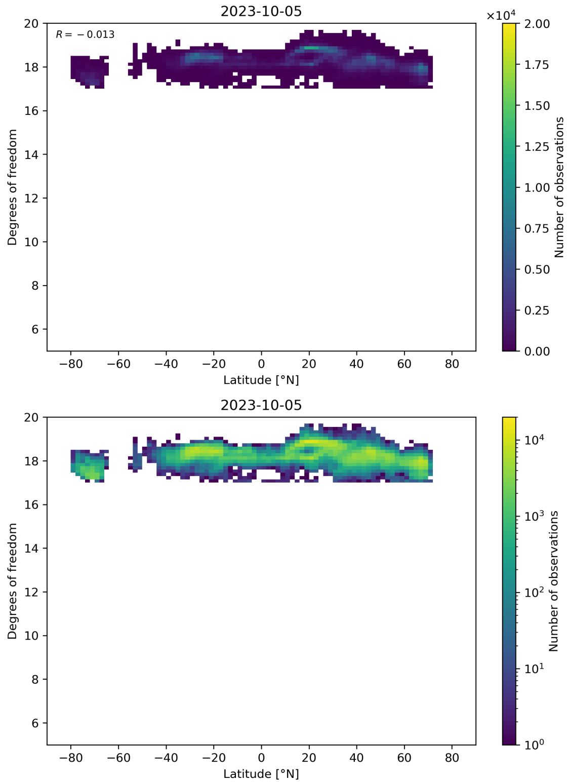
Figure 55: Scatter density plot of “Latitude” against “Degrees of freedom” for 2023-10-04 to 2023-10-06.
