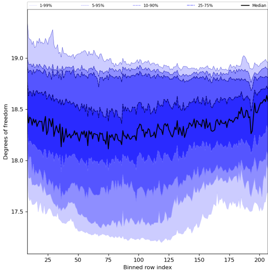
Figure 41: Along track statistics of “Degrees of freedom” for 2023-10-04 to 2023-10-06
