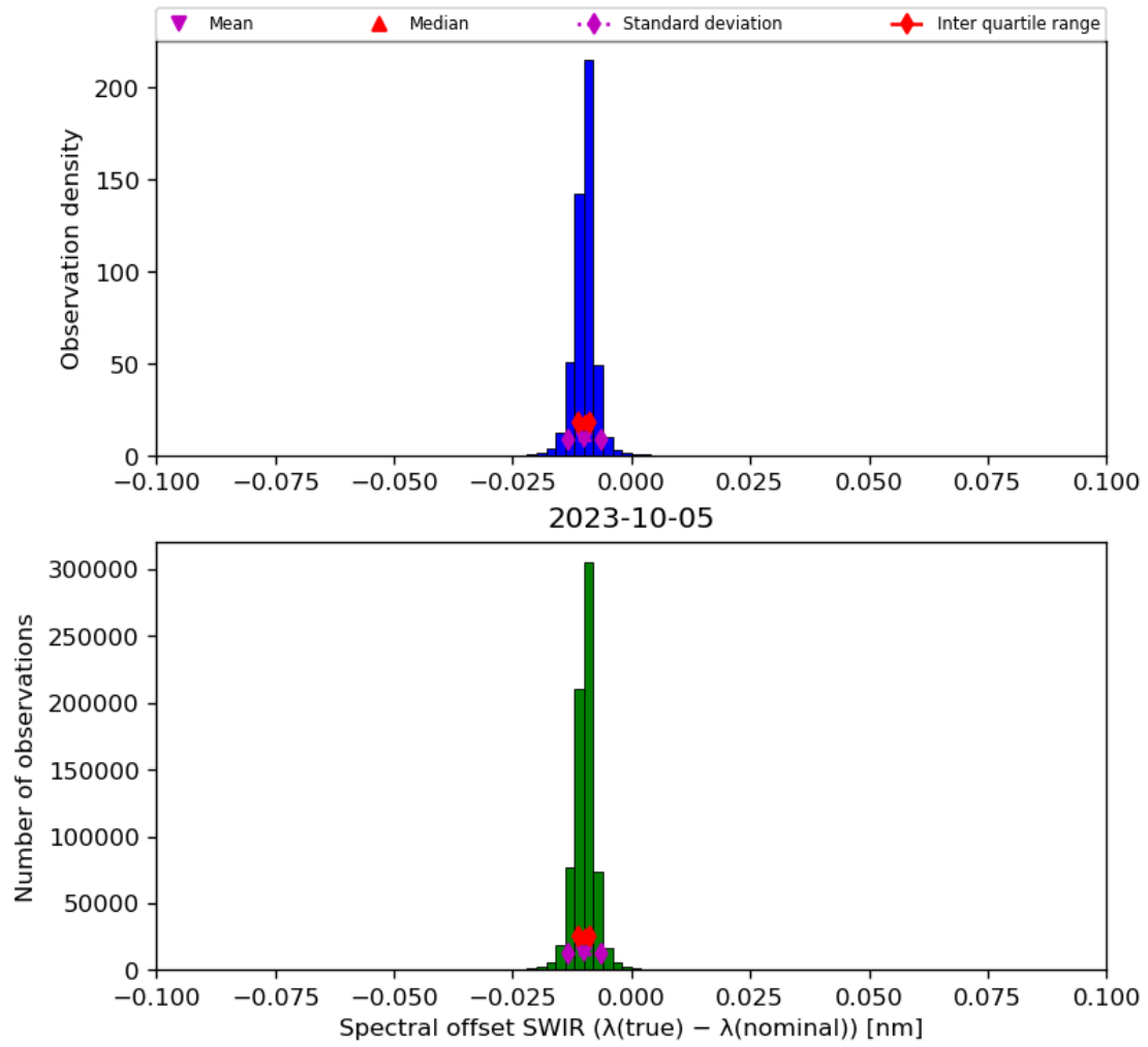
Figure 27: Histogram of “Spectral offset SWIR ( \lambda(\text{true}) - \lambda(\text{nominal}) )” for 2023-10-04 to 2023-10-06
