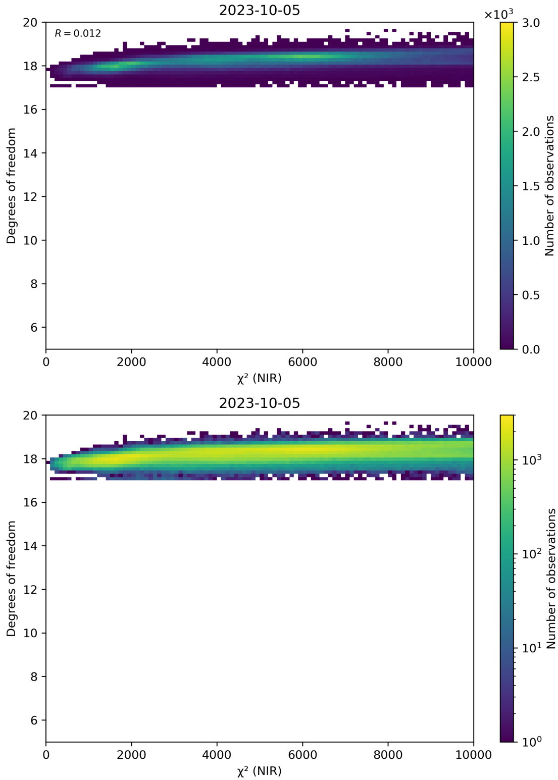
Figure 44: Scatter density plot of “ \chi^2 (NIR)” against “Degrees of freedom” for 2023-10-04 to 2023-10-06.
