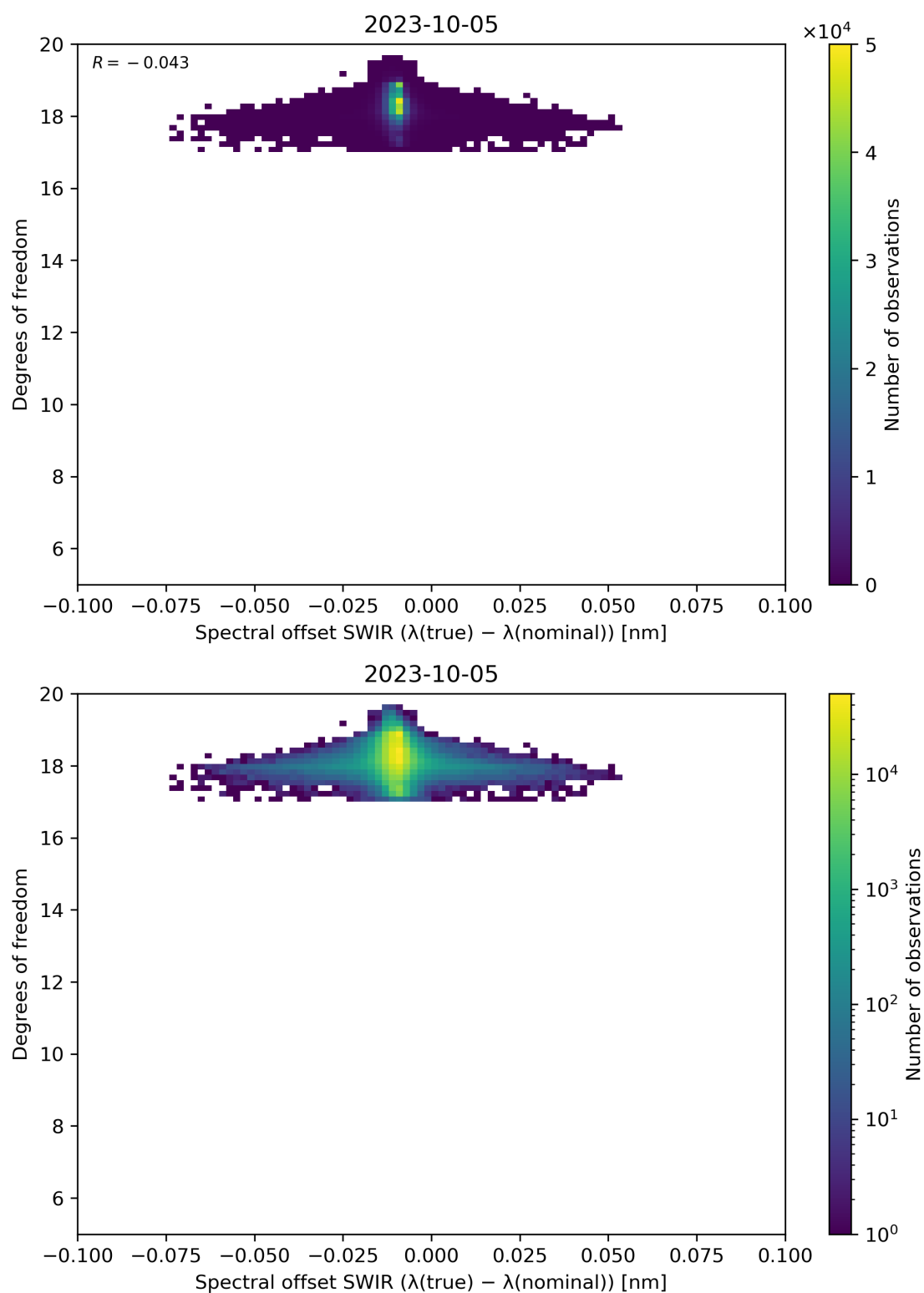
Figure 119: Scatter density plot of “Spectral offset SWIR ( \lambda(\text{true}) - \lambda(\text{nominal}) )” against “Degrees of freedom” for 2023-10-04 to 2023-10-06.
