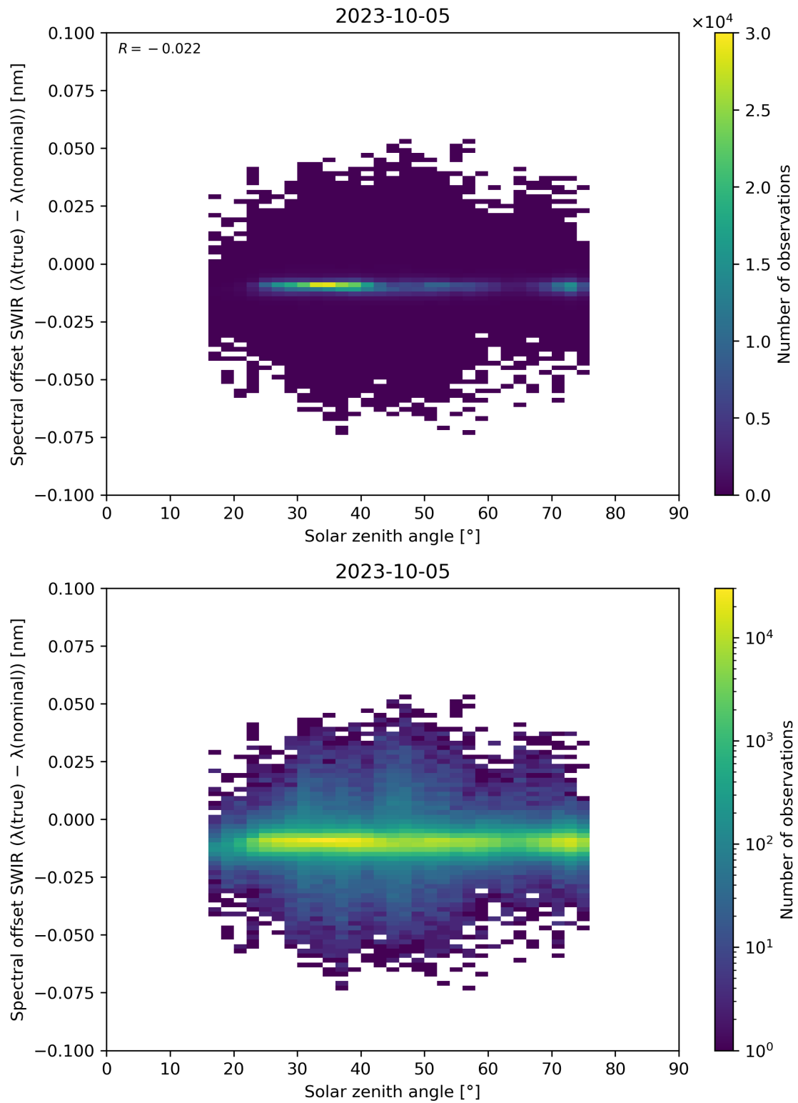
Figure 104: Scatter density plot of “Solar zenith angle” against “Spectral offset SWIR ( \lambda(\text{true}) - \lambda(\text{nominal}) )” for 2023-10-04 to 2023-10-06.
