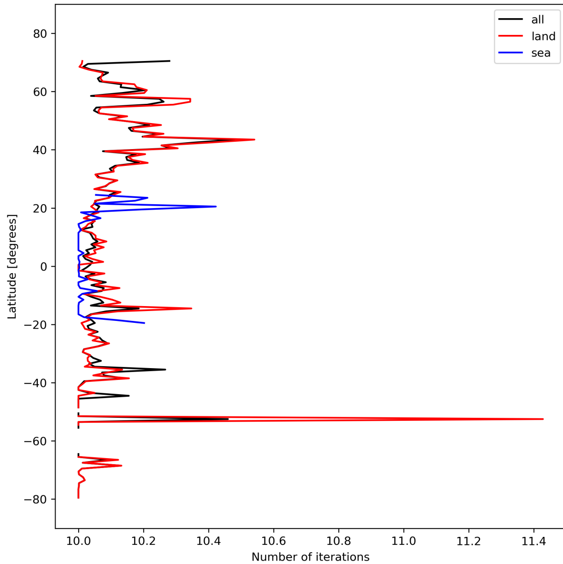
Figure 20: Zonal average of “Number of iterations” for 2023-10-04 to 2023-10-06.
