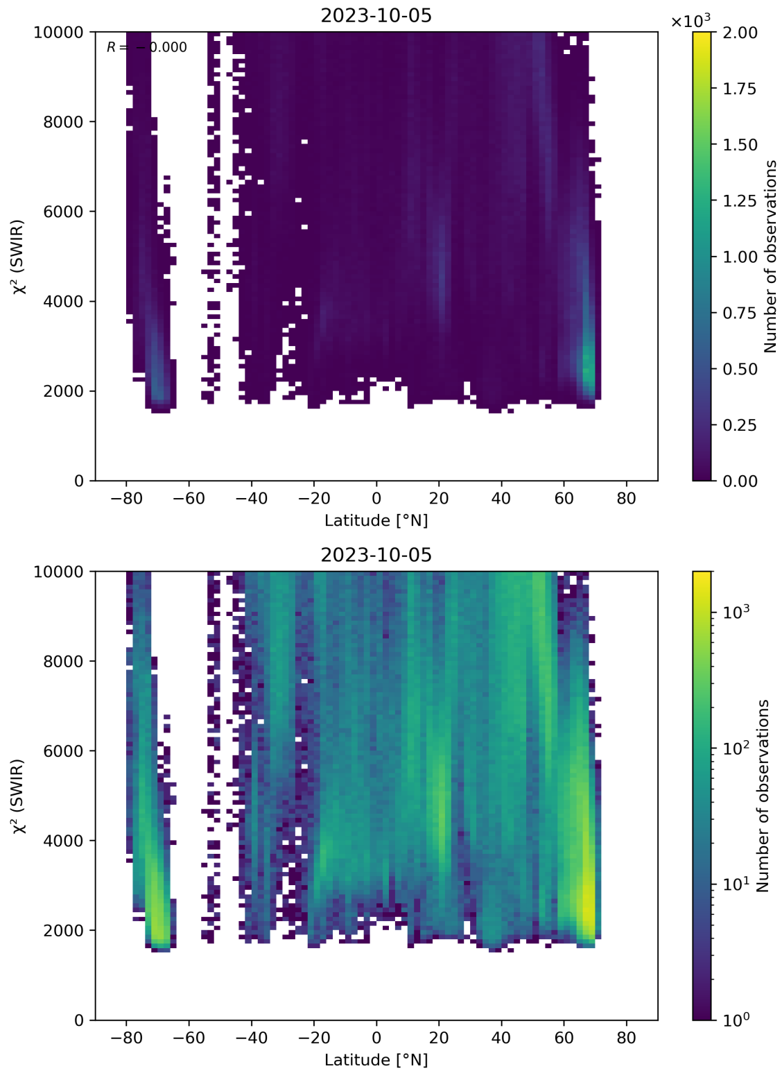
Figure 54: Scatter density plot of “Latitude” against “ \chi^2 (SWIR)” for 2023-10-04 to 2023-10-06.
