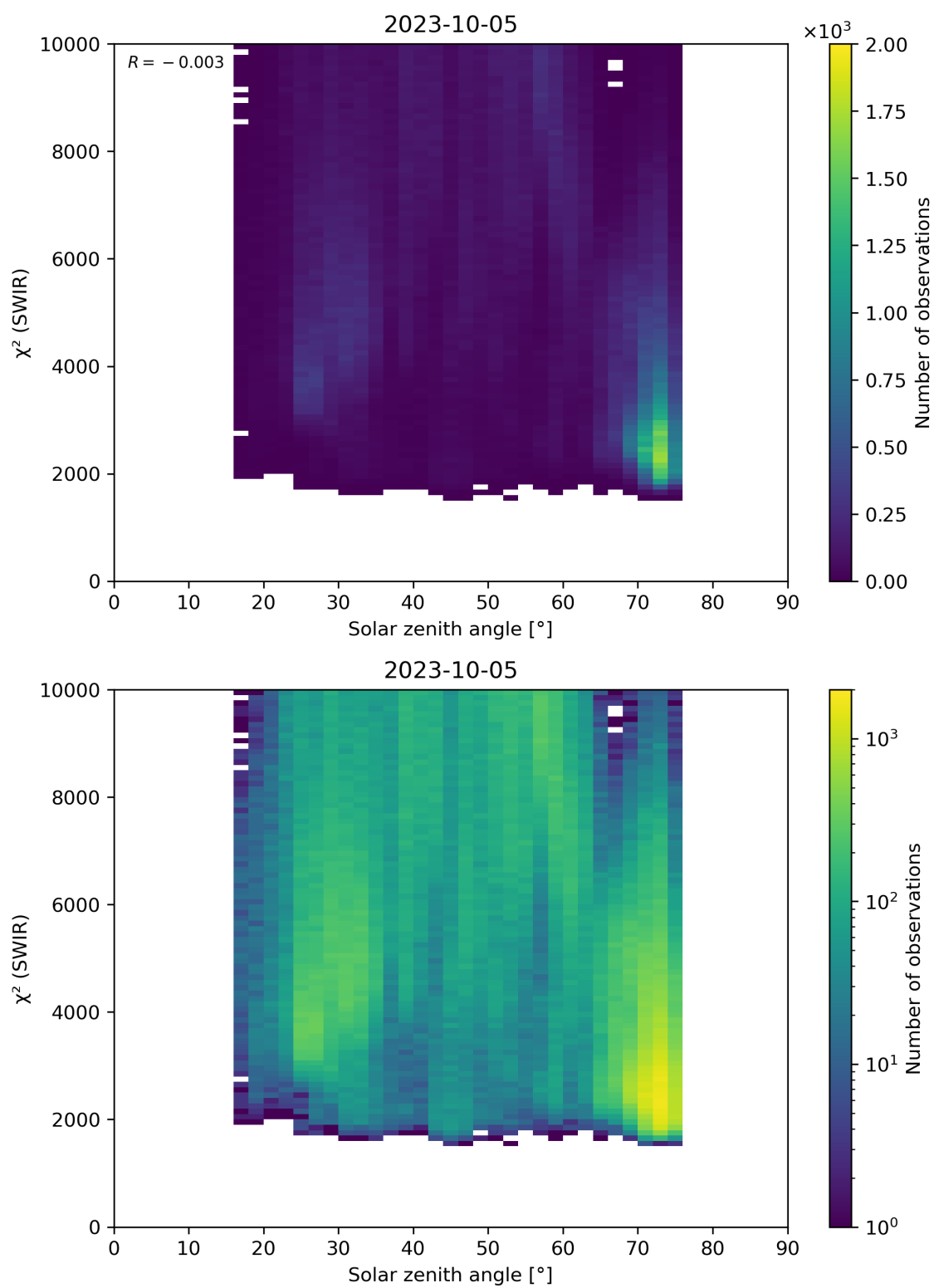
Figure 95: Scatter density plot of “Solar zenith angle” against “ \chi^2 (SWIR)” for 2023-10-04 to 2023-10-06.
