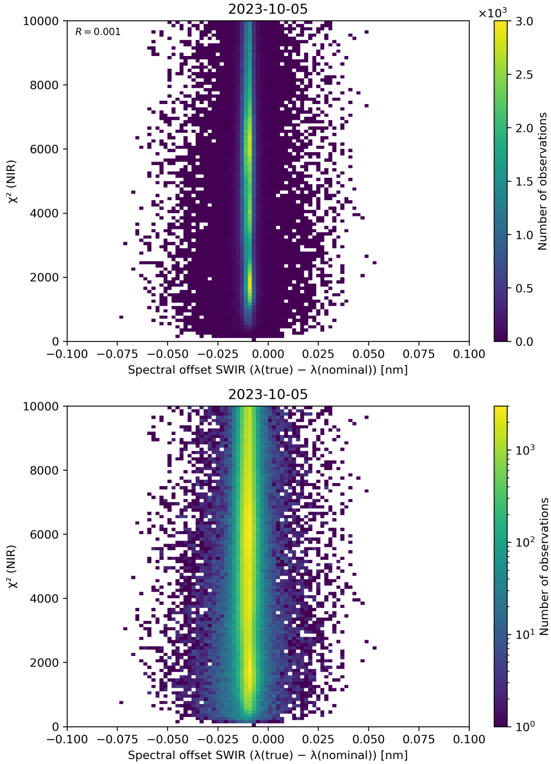
Figure 117: Scatter density plot of “Spectral offset SWIR ( \lambda(\text{true}) - \lambda(\text{nominal}) )” against “ \chi^2 (NIR)” for 2023-10-04 to 2023-10-06.
