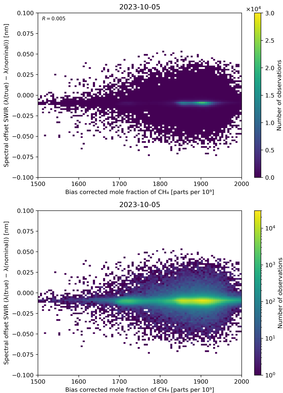
Figure 69: Scatter density plot of “Bias corrected mole fraction of \text{CH}_4 ” against “Spectral offset SWIR ( \lambda(\text{true}) - \lambda(\text{nominal}) )” for 2023-10-04 to 2023-10-06.
