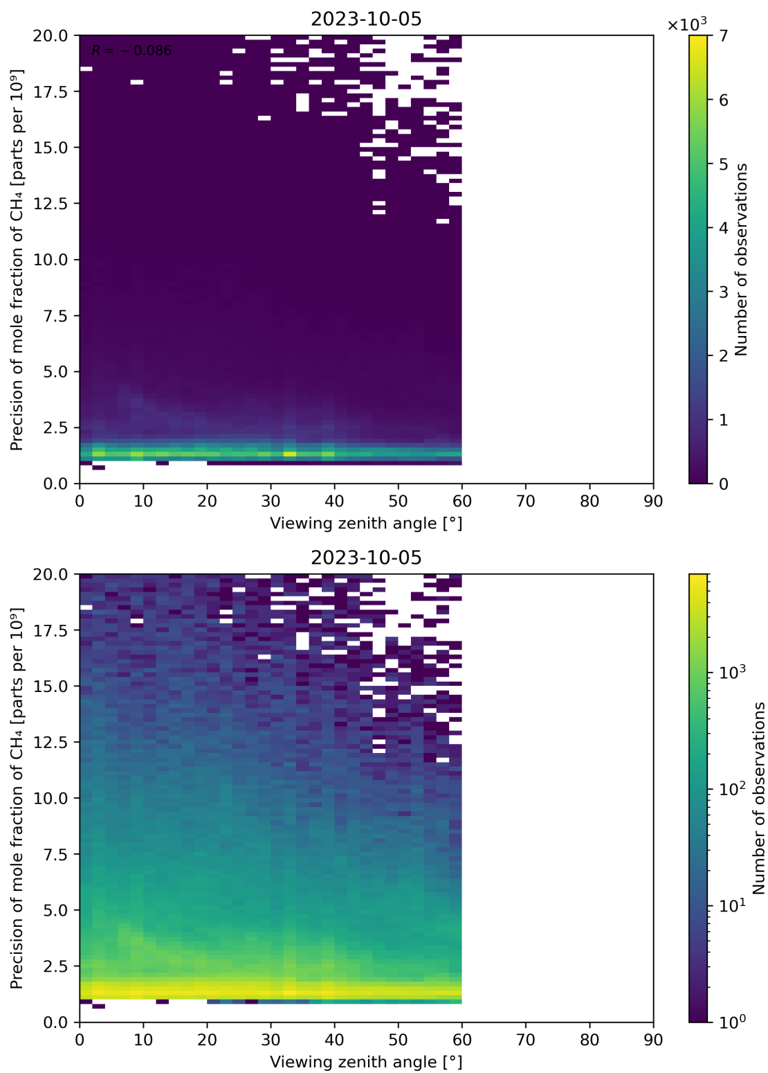
Figure 112: Scatter density plot of “Viewing zenith angle” against “Precision of mole fraction of CH 4 ” for 2023-10-04 to 2023-10-06.
