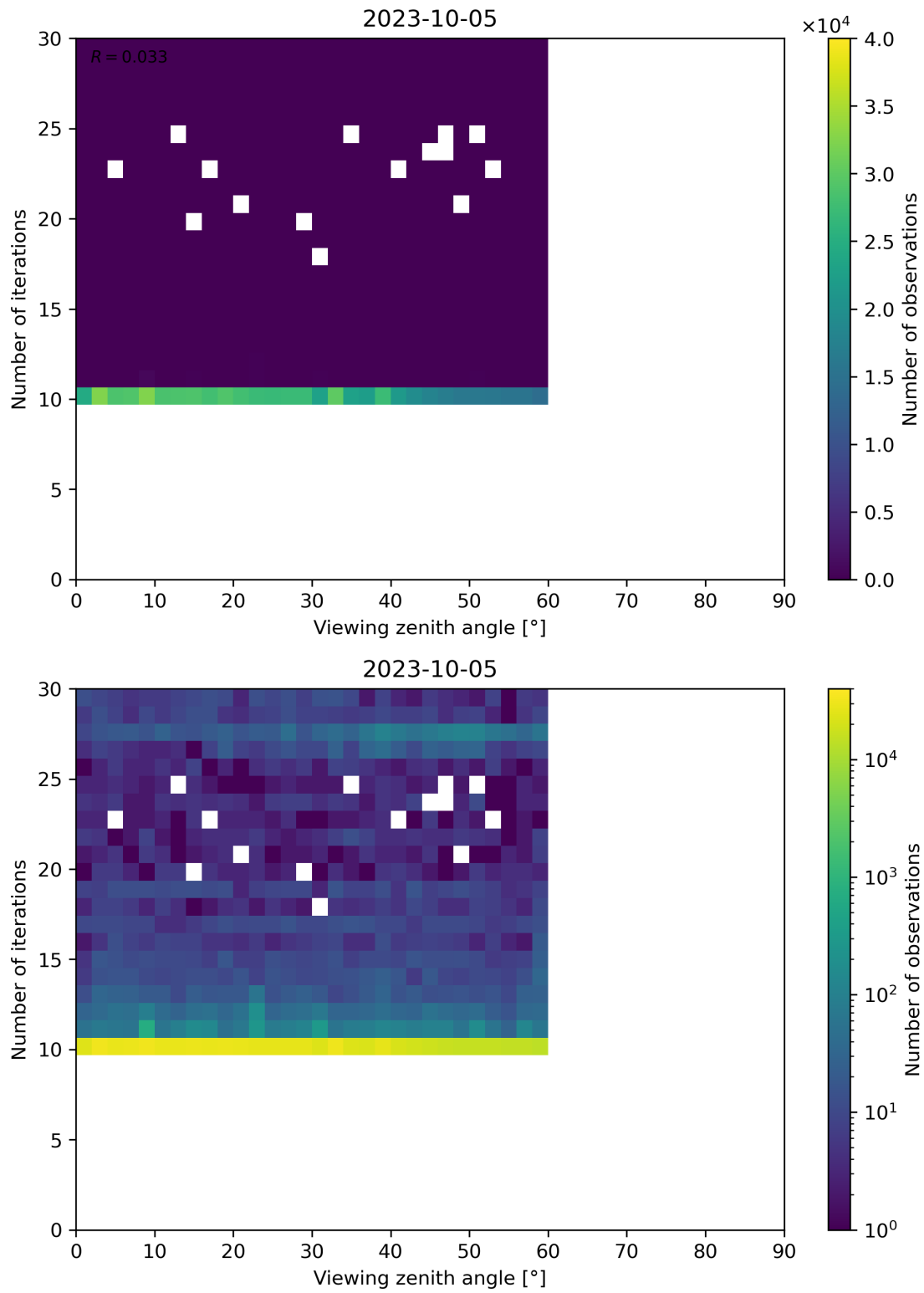
Figure 113: Scatter density plot of “Viewing zenith angle” against “Number of iterations” for 2023-10-04 to 2023-10-06.
