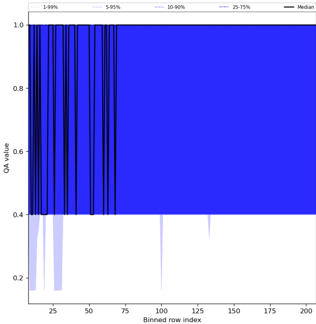
Figure 33: Along track statistics of “QA value” for 2023-10-04 to 2023-10-06
