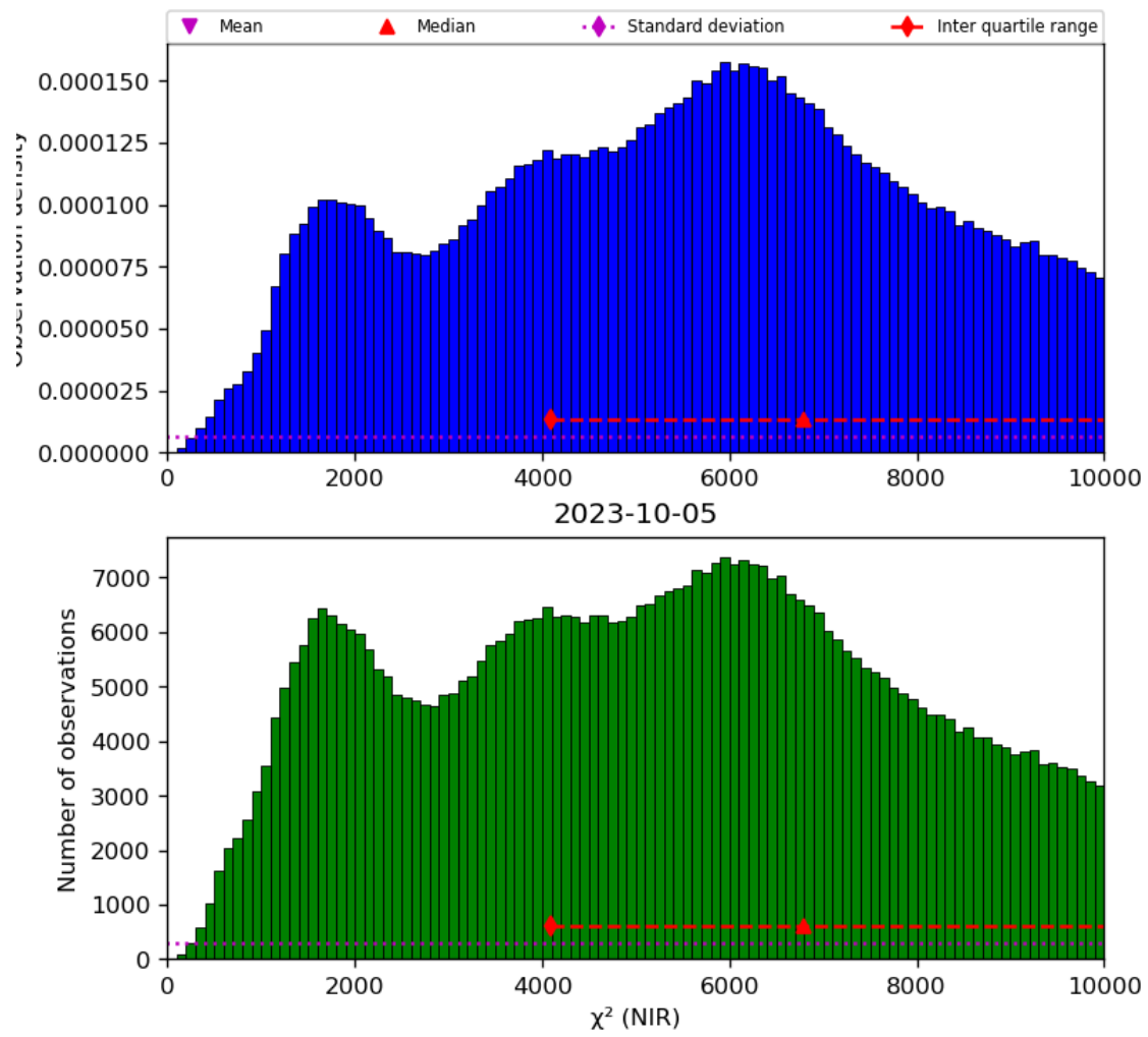
Figure 29: Histogram of “ \chi^2 (NIR)” for 2023-10-04 to 2023-10-06
