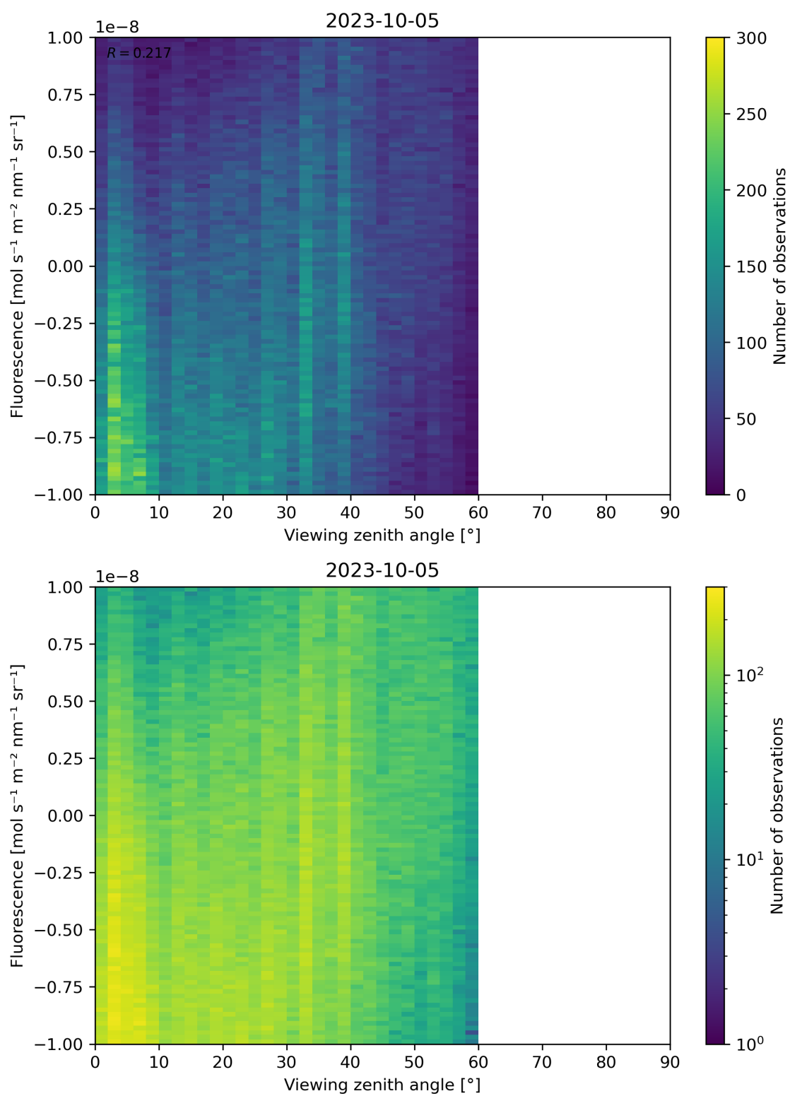
Figure 108: Scatter density plot of “Viewing zenith angle” against “Fluorescence” for 2023-10-04 to 2023-10-06.
