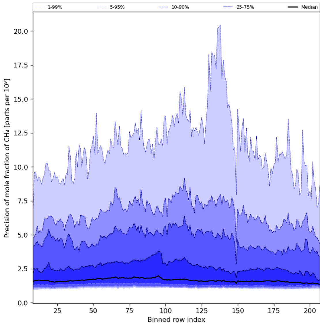
Figure 35: Along track statistics of “Precision of mole fraction of CH 4 ” for 2023-10-04 to 2023-10-06
