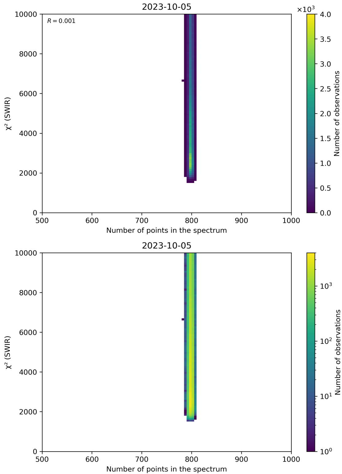
Figure 89: Scatter density plot of “Number of points in the spectrum” against “ \chi^2 (SWIR)” for 2023-10-04 to 2023-10-06.
