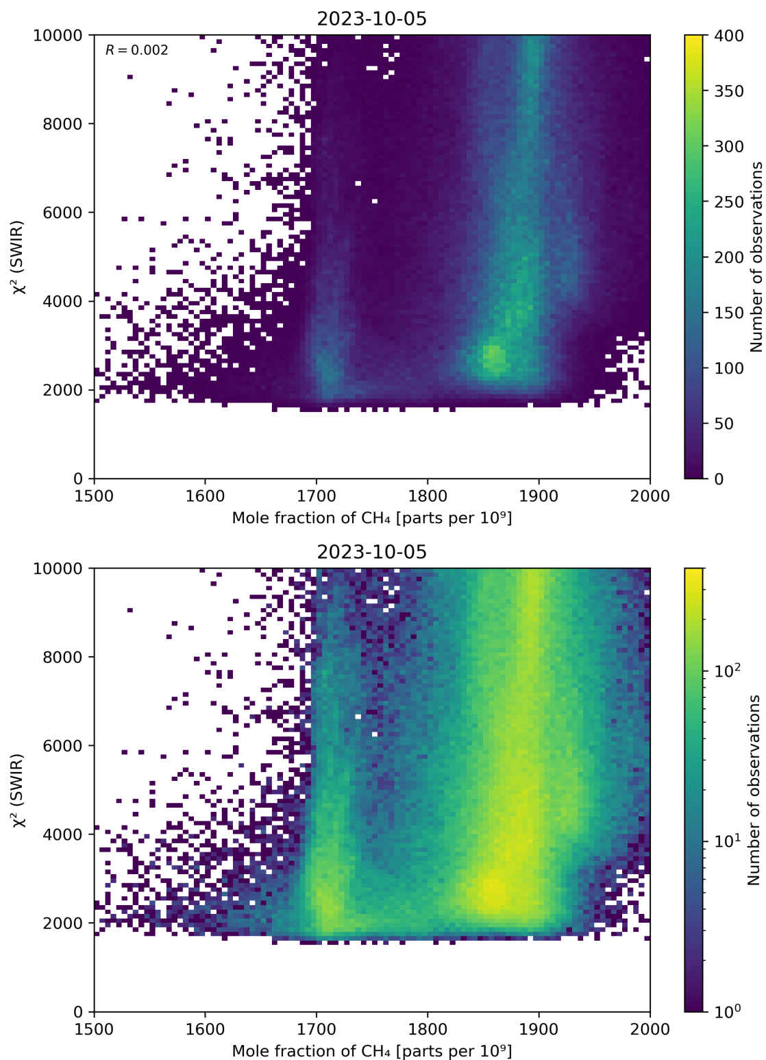
Figure 71: Scatter density plot of “Mole fraction of \text{CH}_4 ” against “ \chi^2 (SWIR)” for 2023-10-04 to 2023-10-06.
