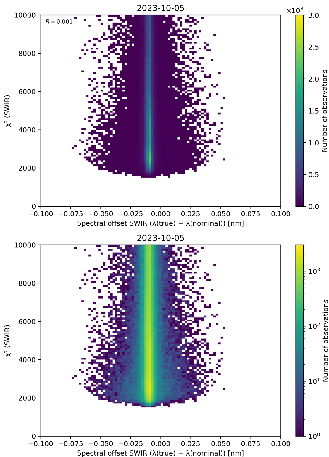
Figure 118: Scatter density plot of “Spectral offset SWIR ( \lambda(\text{true}) - \lambda(\text{nominal}) )” against “ \chi^2 (SWIR)” for 2023-10-04 to 2023-10-06.
