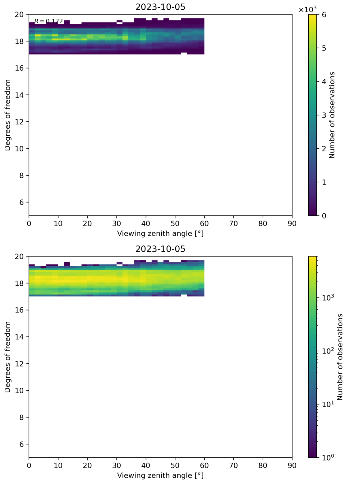
Figure 107: Scatter density plot of “Viewing zenith angle” against “Degrees of freedom” for 2023-10-04 to 2023-10-06.
