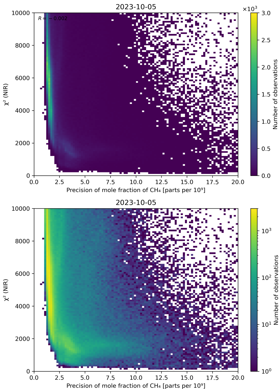
Figure 78: Scatter density plot of “Precision of mole fraction of CH 4 ” against “ \chi^2 (NIR)” for 2023-10-04 to 2023-10-06.
