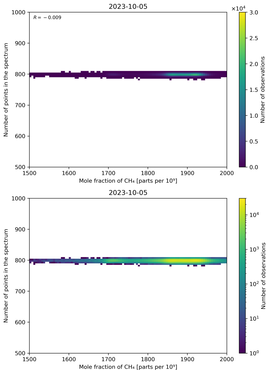
Figure 77: Scatter density plot of “Mole fraction of CH 4 ” against “Number of points in the spectrum” for 2023-10-04 to 2023-10-06.
