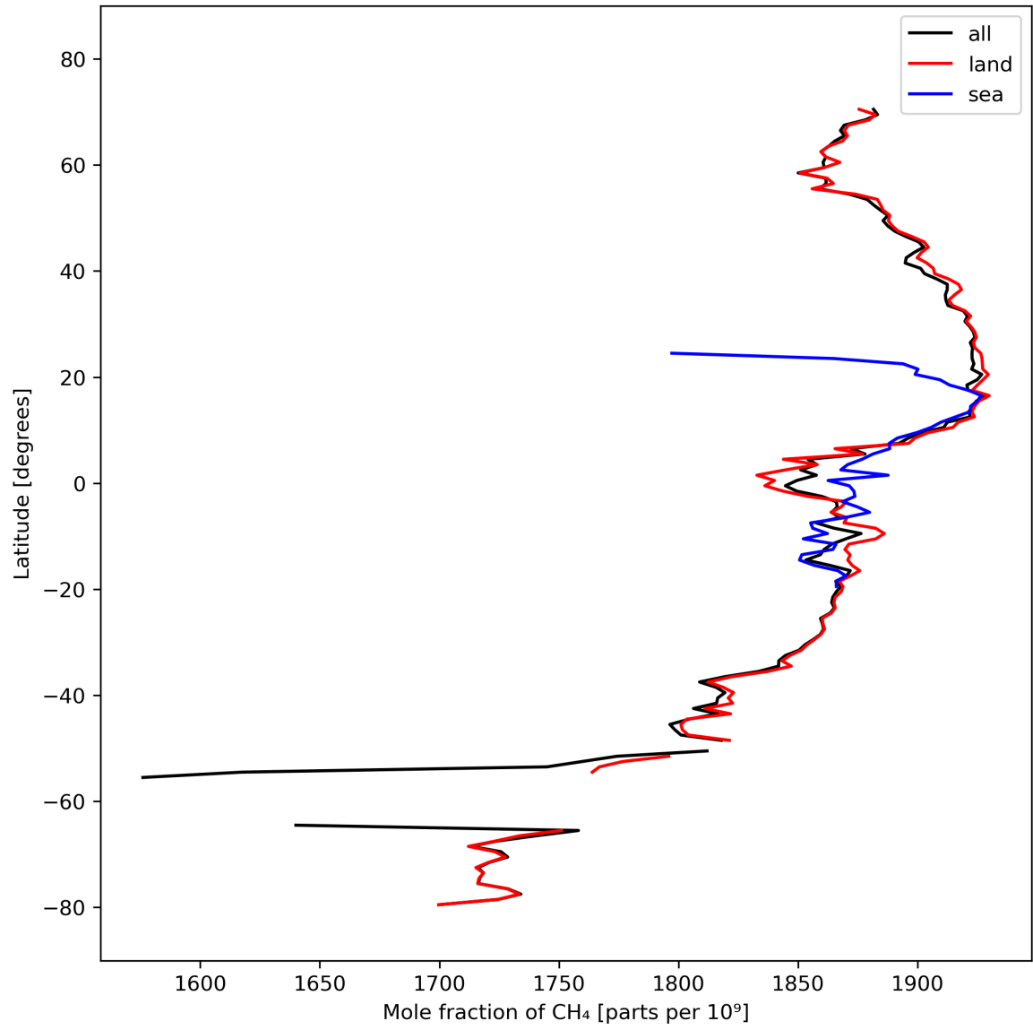
Figure 12: Zonal average of “Mole fraction of \text{CH}_4 ” for 2023-10-04 to 2023-10-06.
