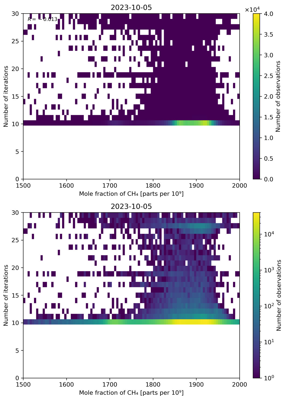
Figure 76: Scatter density plot of “Mole fraction of CH 4 ” against “Number of iterations” for 2023-10-04 to 2023-10-06.
