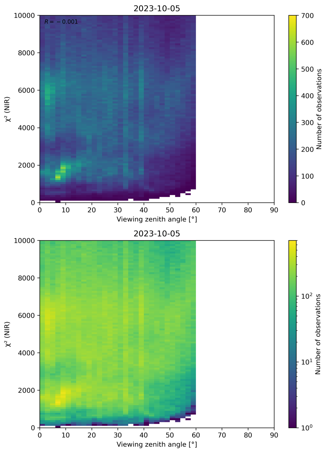
Figure 105: Scatter density plot of “Viewing zenith angle” against “ \chi^2 (NIR)” for 2023-10-04 to 2023-10-06.
