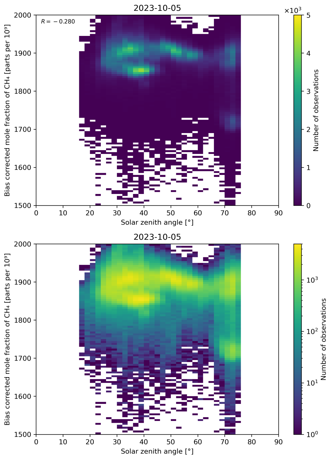
Figure 100: Scatter density plot of “Solar zenith angle” against “Bias corrected mole fraction of CH 4 ” for 2023-10-04 to 2023-10-06.
