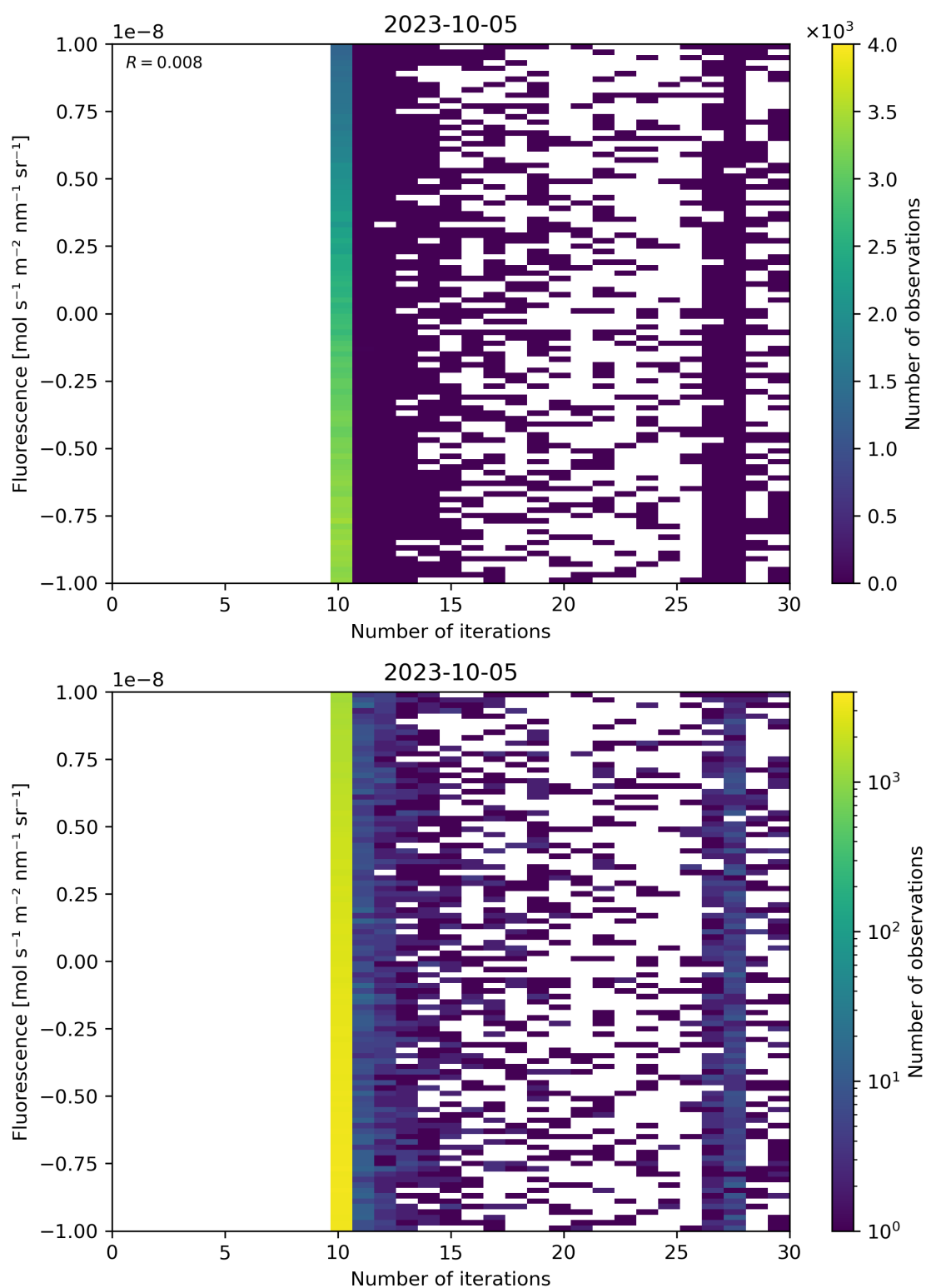
Figure 87: Scatter density plot of “Number of iterations” against “Fluorescence” for 2023-10-04 to 2023-10-06.
