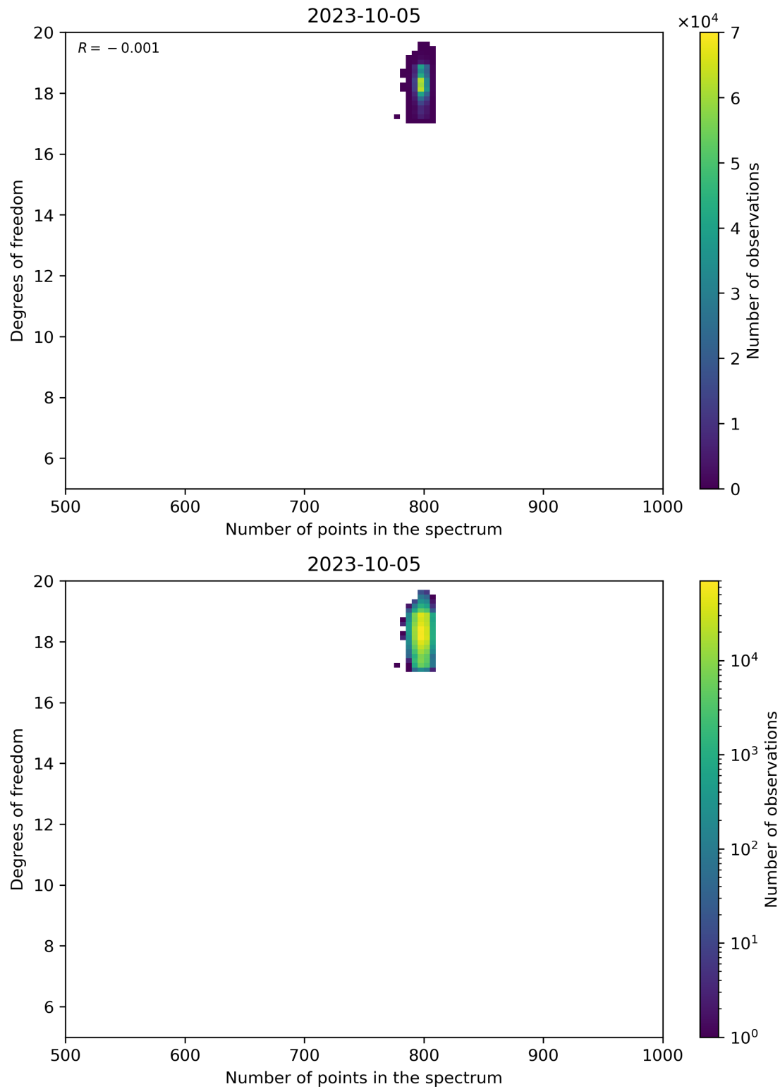
Figure 90: Scatter density plot of “Number of points in the spectrum” against “Degrees of freedom” for 2023-10-04 to 2023-10-06.
