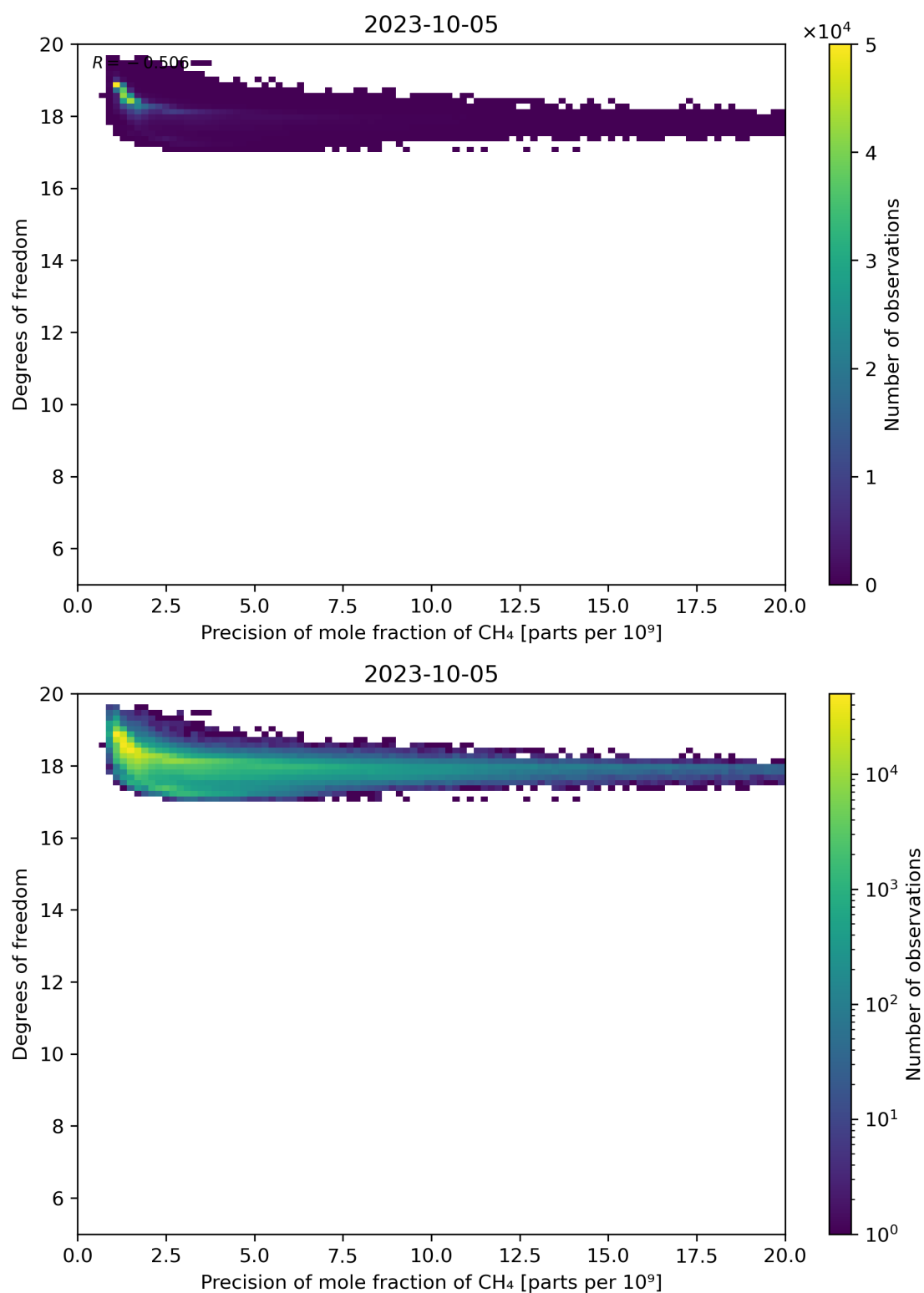
Figure 80: Scatter density plot of “Precision of mole fraction of CH 4 ” against “Degrees of freedom” for 2023-10-04 to 2023-10-06.
