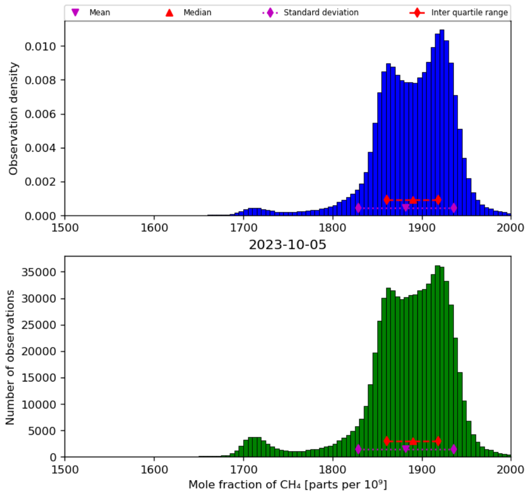
Figure 23: Histogram of “Mole fraction of CH 4 ” for 2023-10-04 to 2023-10-06
