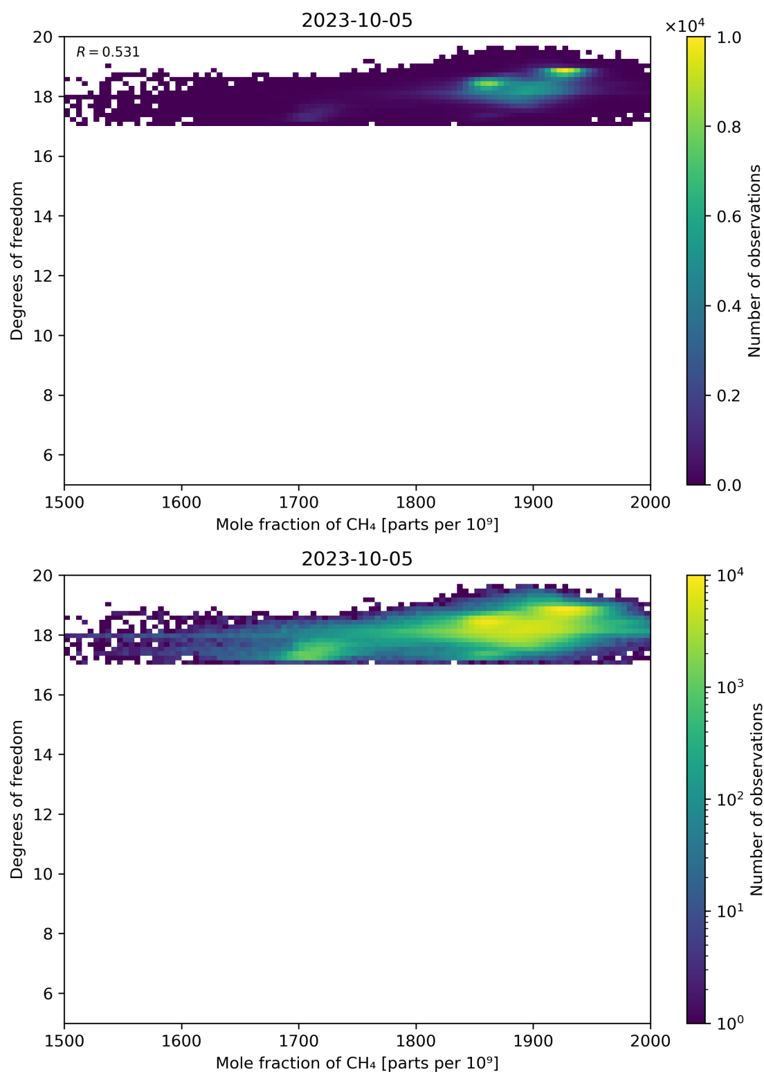
Figure 72: Scatter density plot of “Mole fraction of CH 4 ” against “Degrees of freedom” for 2023-10-04 to 2023-10-06.
