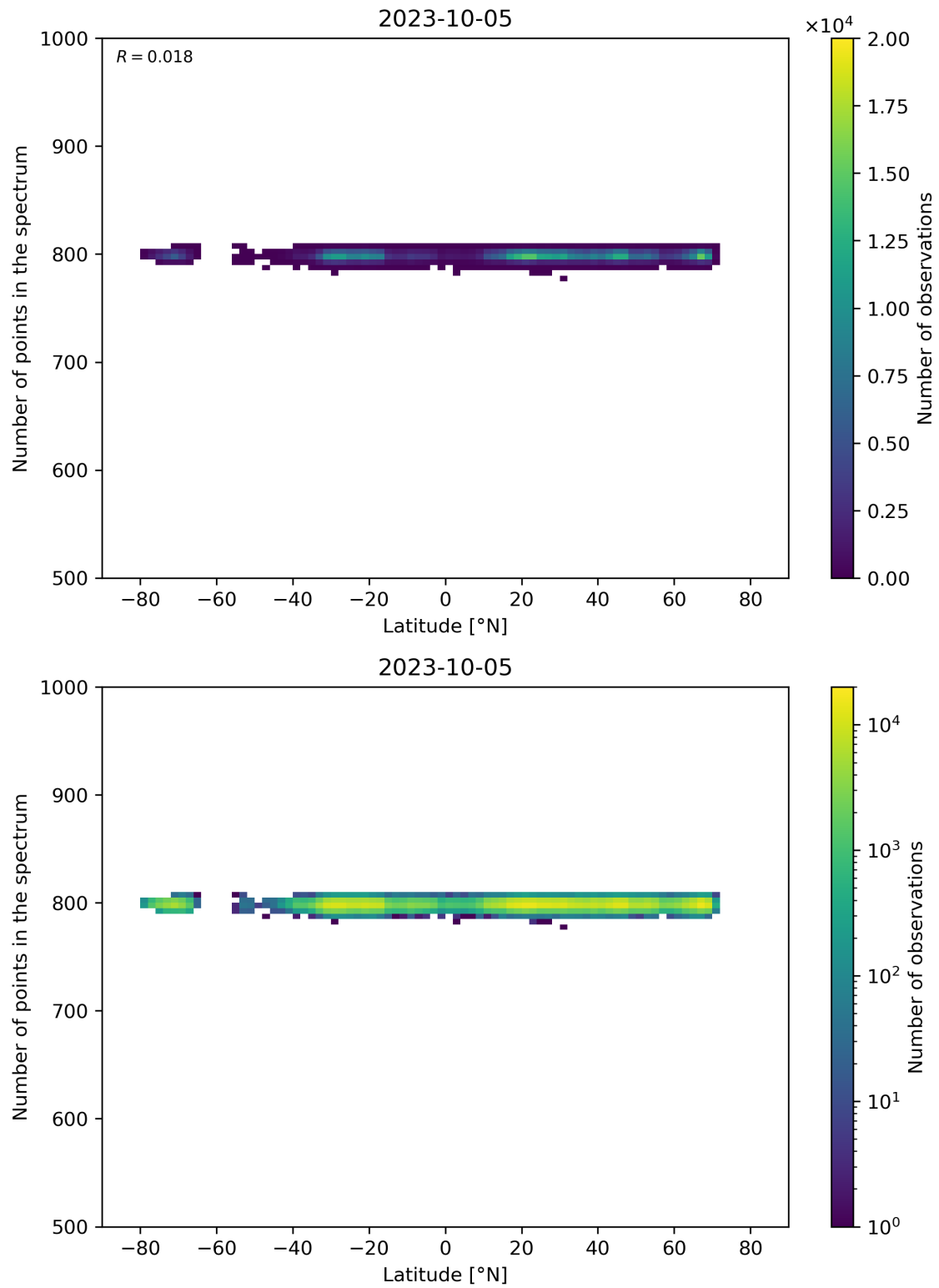
Figure 61: Scatter density plot of “Latitude” against “Number of points in the spectrum” for 2023-10-04 to 2023-10-06.
