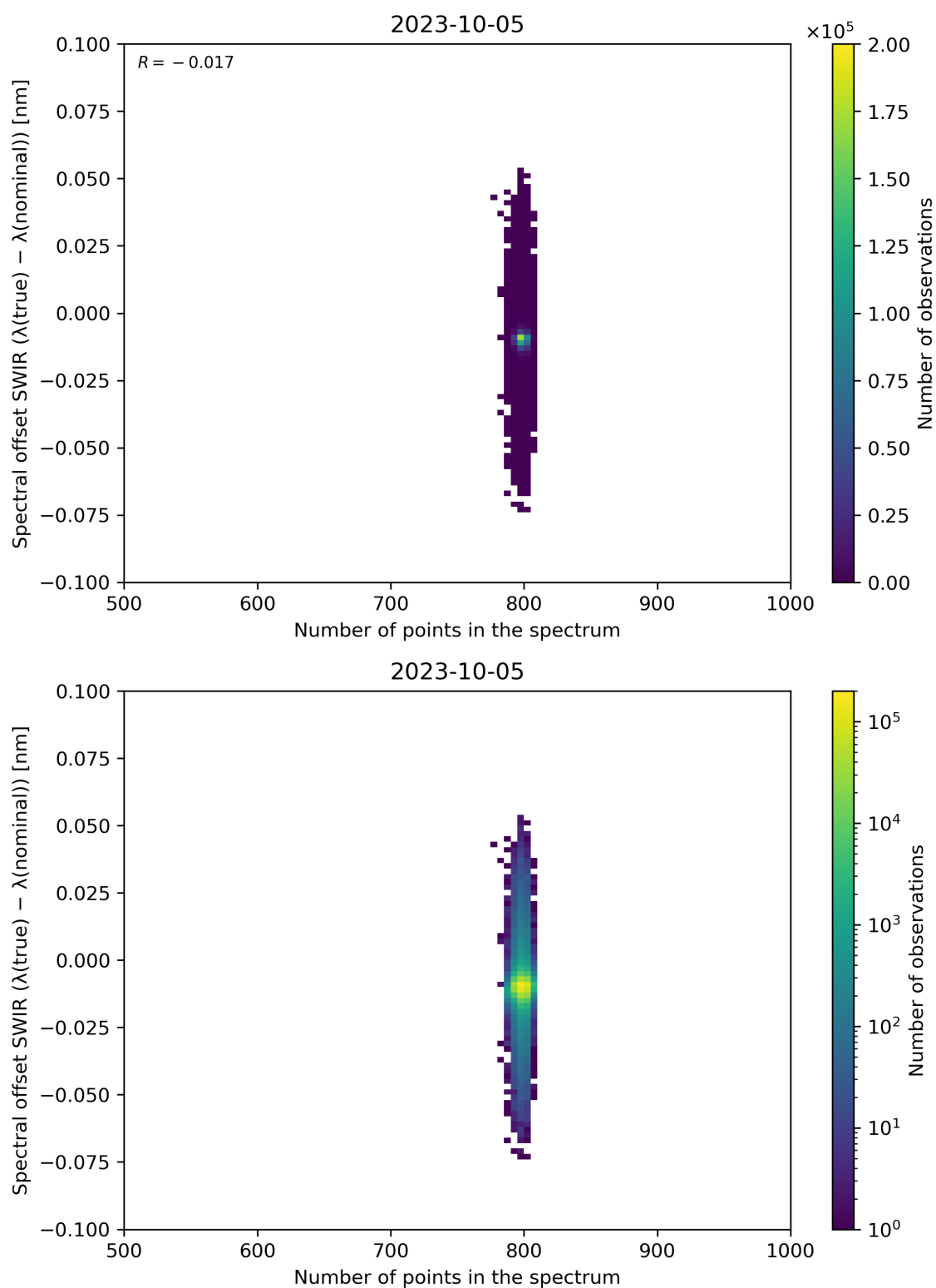
Figure 93: Scatter density plot of “Number of points in the spectrum” against “Spectral offset SWIR ( \lambda(\text{true}) - \lambda(\text{nominal}) )” for 2023-10-04 to 2023-10-06.
