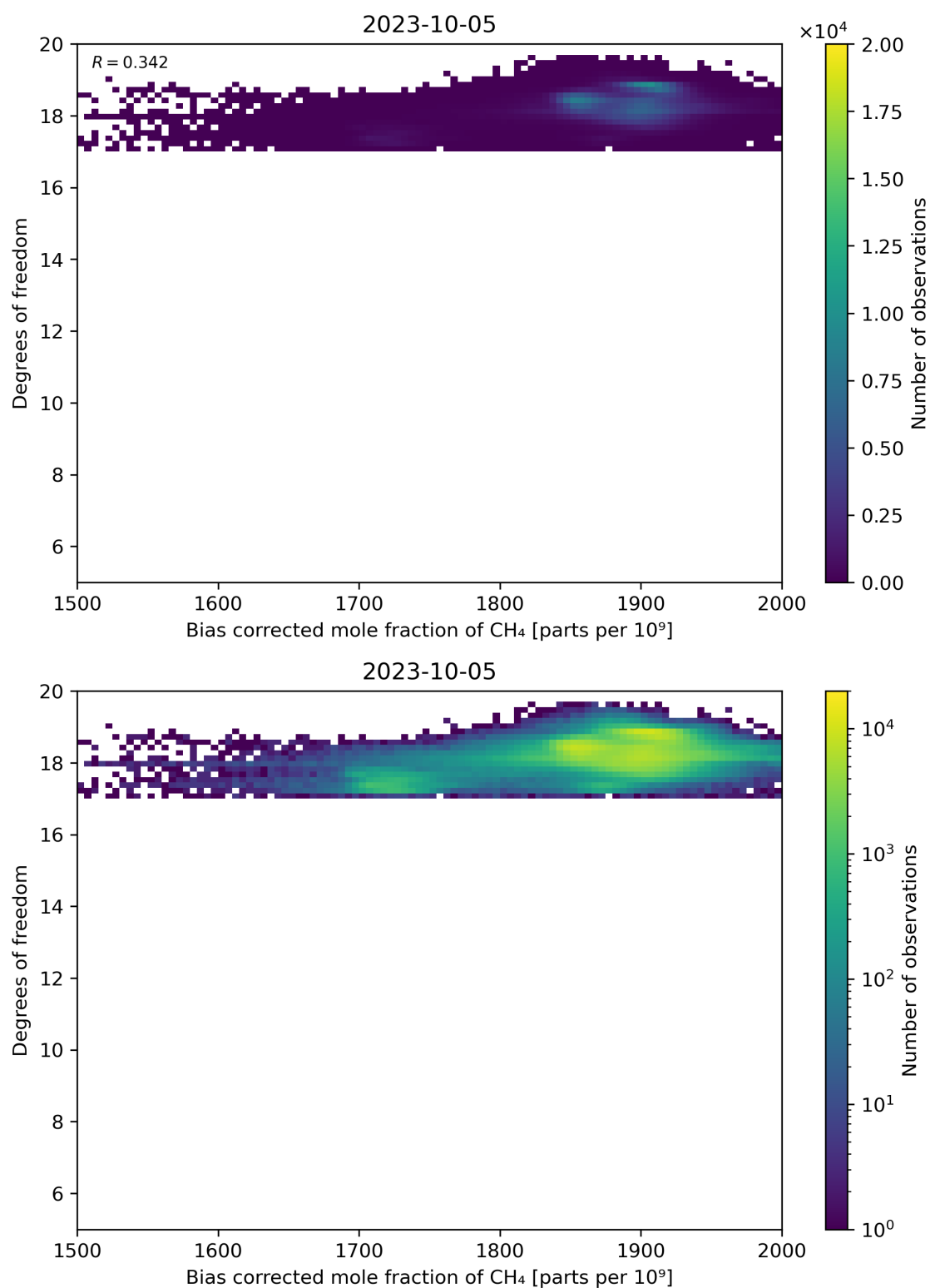
Figure 65: Scatter density plot of “Bias corrected mole fraction of CH 4 ” against “Degrees of freedom” for 2023-10-04 to 2023-10-06.
