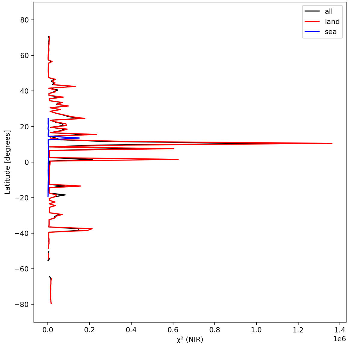
Figure 18: Zonal average of “ \chi^2 (NIR)” for 2023-10-04 to 2023-10-06.
