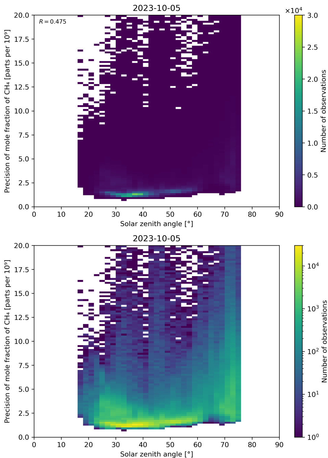
Figure 101: Scatter density plot of “Solar zenith angle” against “Precision of mole fraction of CH 4 ” for 2023-10-04 to 2023-10-06.
