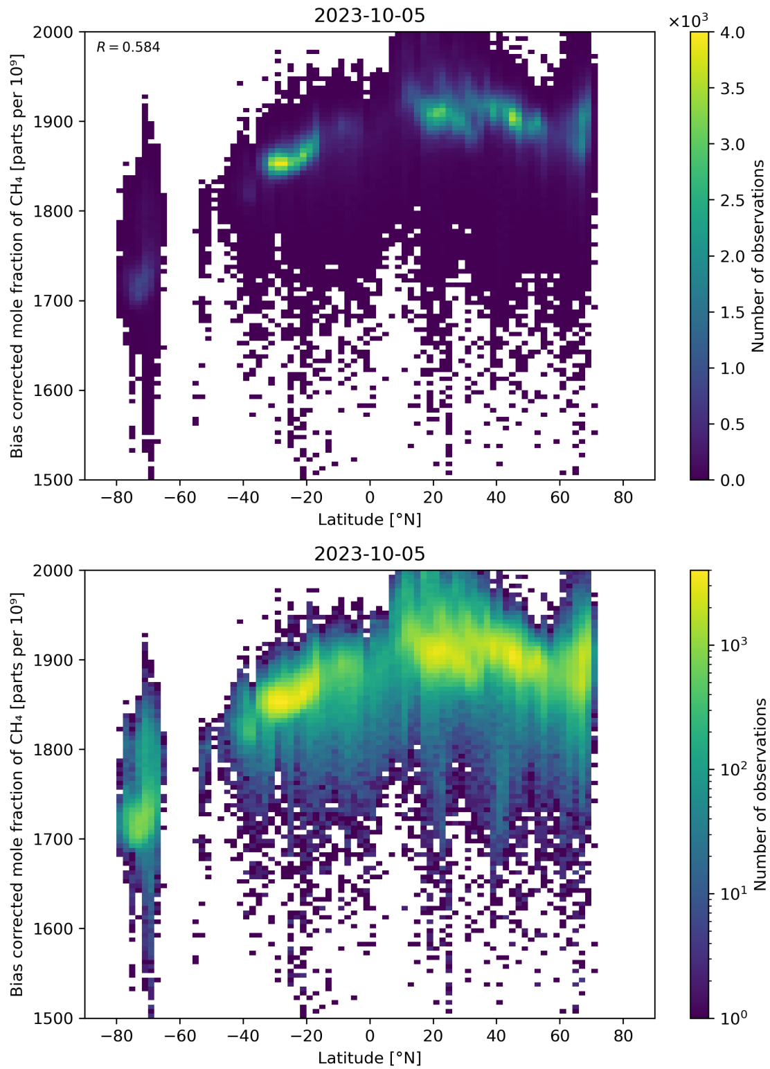
Figure 58: Scatter density plot of “Latitude” against “Bias corrected mole fraction of \text{CH}_4 ” for 2023-10-04 to 2023-10-06.
