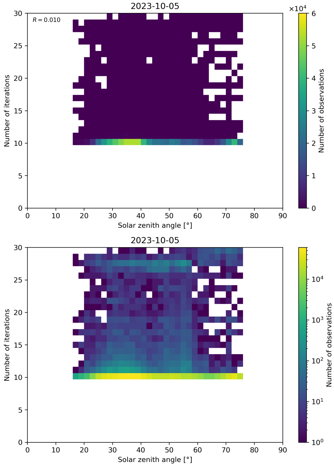
Figure 102: Scatter density plot of “Solar zenith angle” against “Number of iterations” for 2023-10-04 to 2023-10-06.
