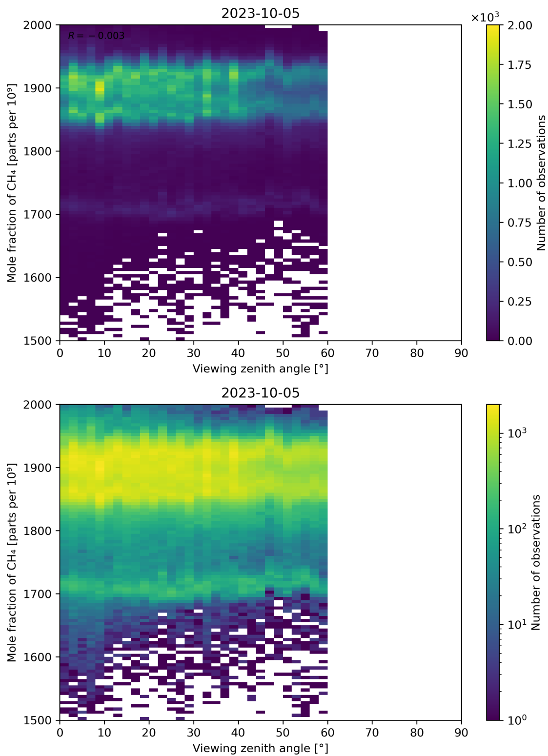
Figure 110: Scatter density plot of “Viewing zenith angle” against “Mole fraction of CH 4 ” for 2023-10-04 to 2023-10-06.
