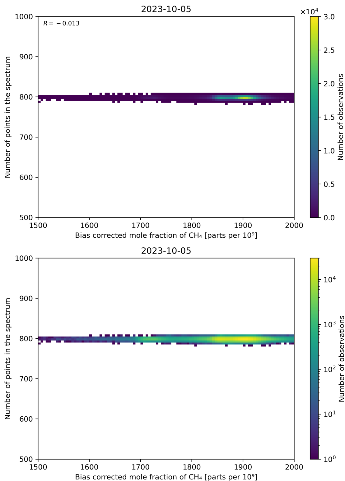
Figure 68: Scatter density plot of “Bias corrected mole fraction of CH 4 ” against “Number of points in the spectrum” for 2023-10-04 to 2023-10-06.
