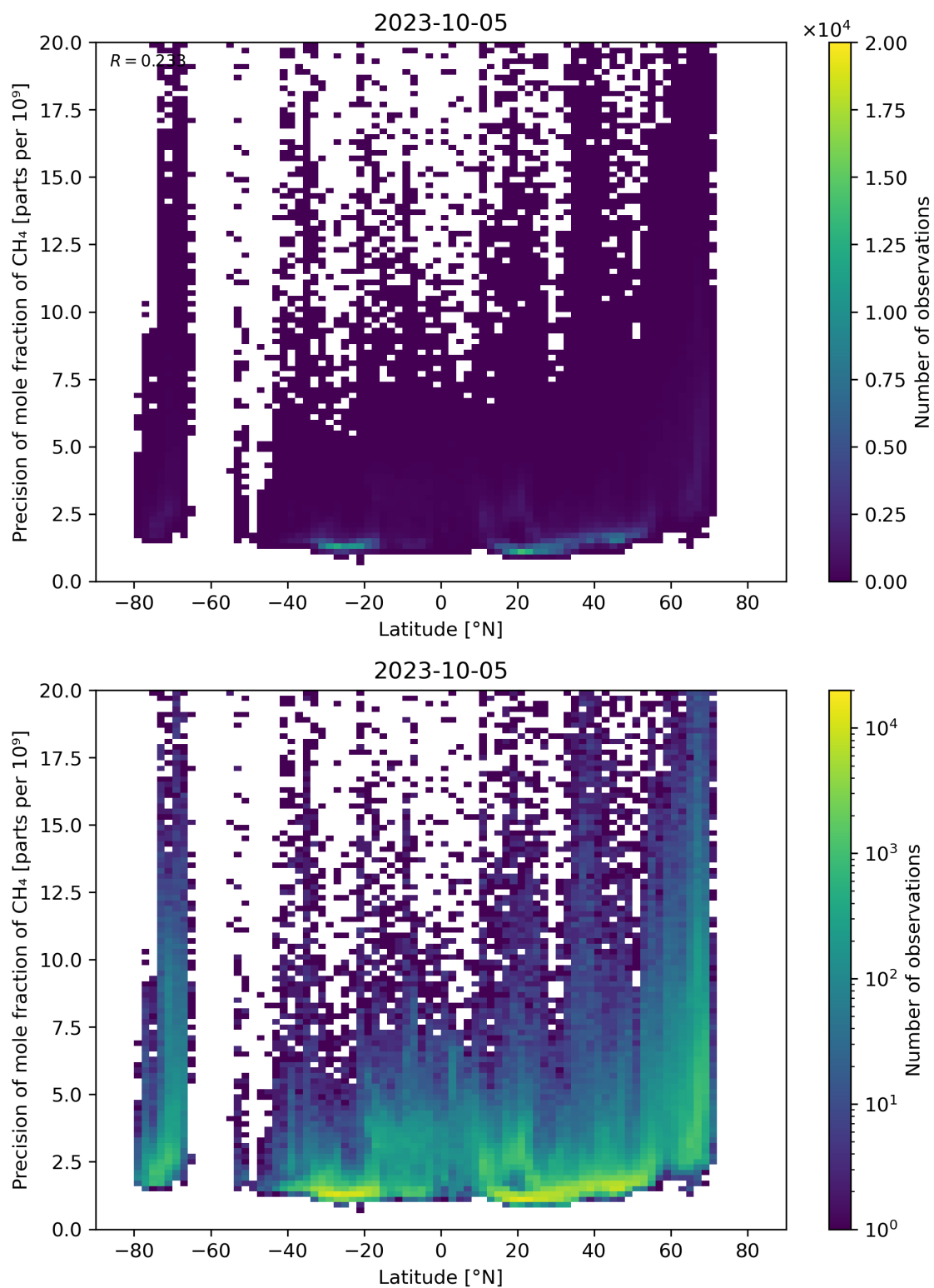
Figure 59: Scatter density plot of “Latitude” against “Precision of mole fraction of \text{CH}_4 ” for 2023-10-04 to 2023-10-06.
