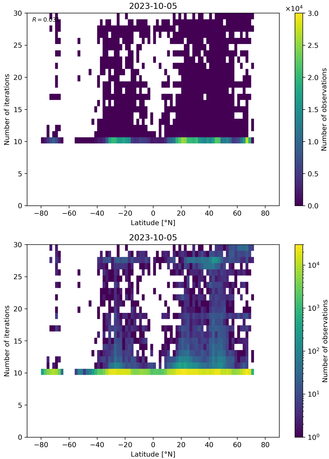
Figure 60: Scatter density plot of “Latitude” against “Number of iterations” for 2023-10-04 to 2023-10-06.
