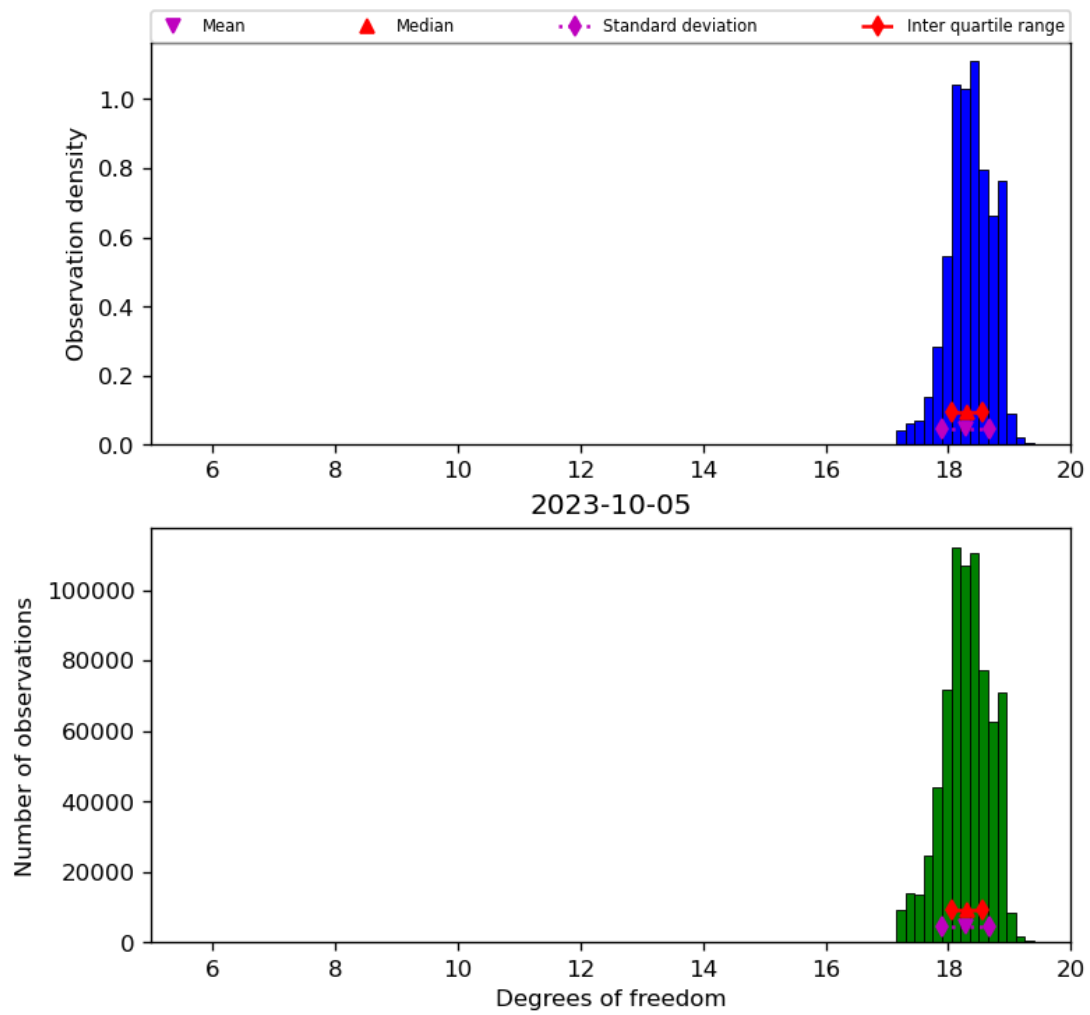
Figure 30: Histogram of “Degrees of freedom” for 2023-10-04 to 2023-10-06
