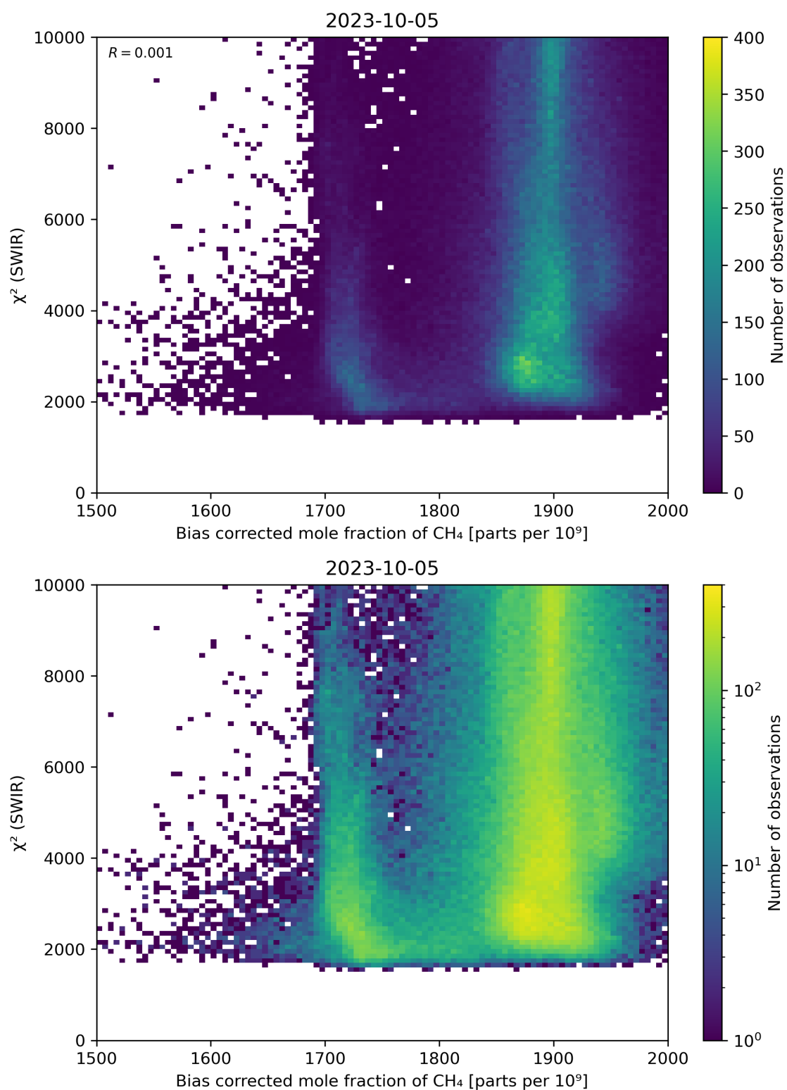
Figure 64: Scatter density plot of “Bias corrected mole fraction of CH 4 ” against “ \chi^2 (SWIR)” for 2023-10-04 to 2023-10-06.
