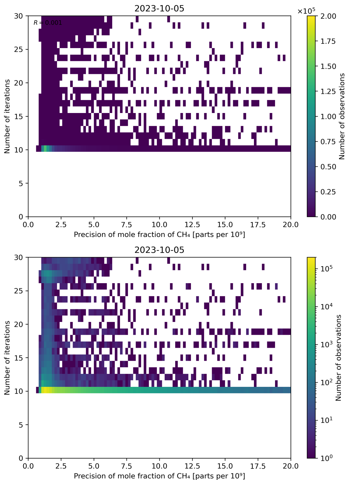
Figure 83: Scatter density plot of “Precision of mole fraction of CH 4 ” against “Number of iterations” for 2023-10-04 to 2023-10-06.
