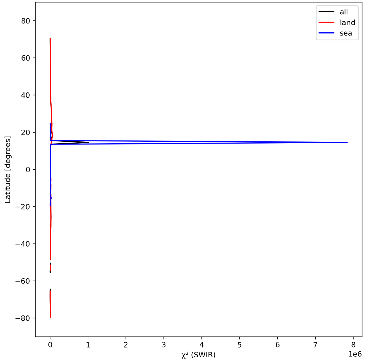
Figure 17: Zonal average of “ \chi^2 (SWIR)” for 2023-10-04 to 2023-10-06.
