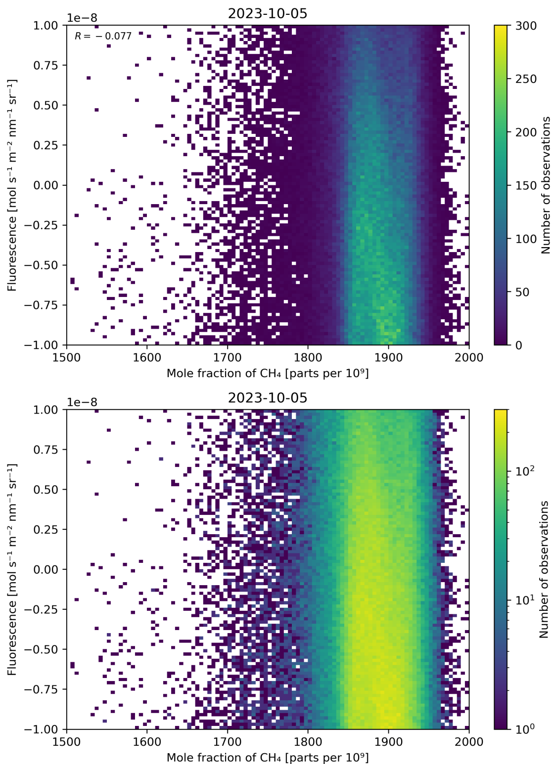
Figure 73: Scatter density plot of “Mole fraction of \text{CH}_4 ” against “Fluorescence” for 2023-10-04 to 2023-10-06.
