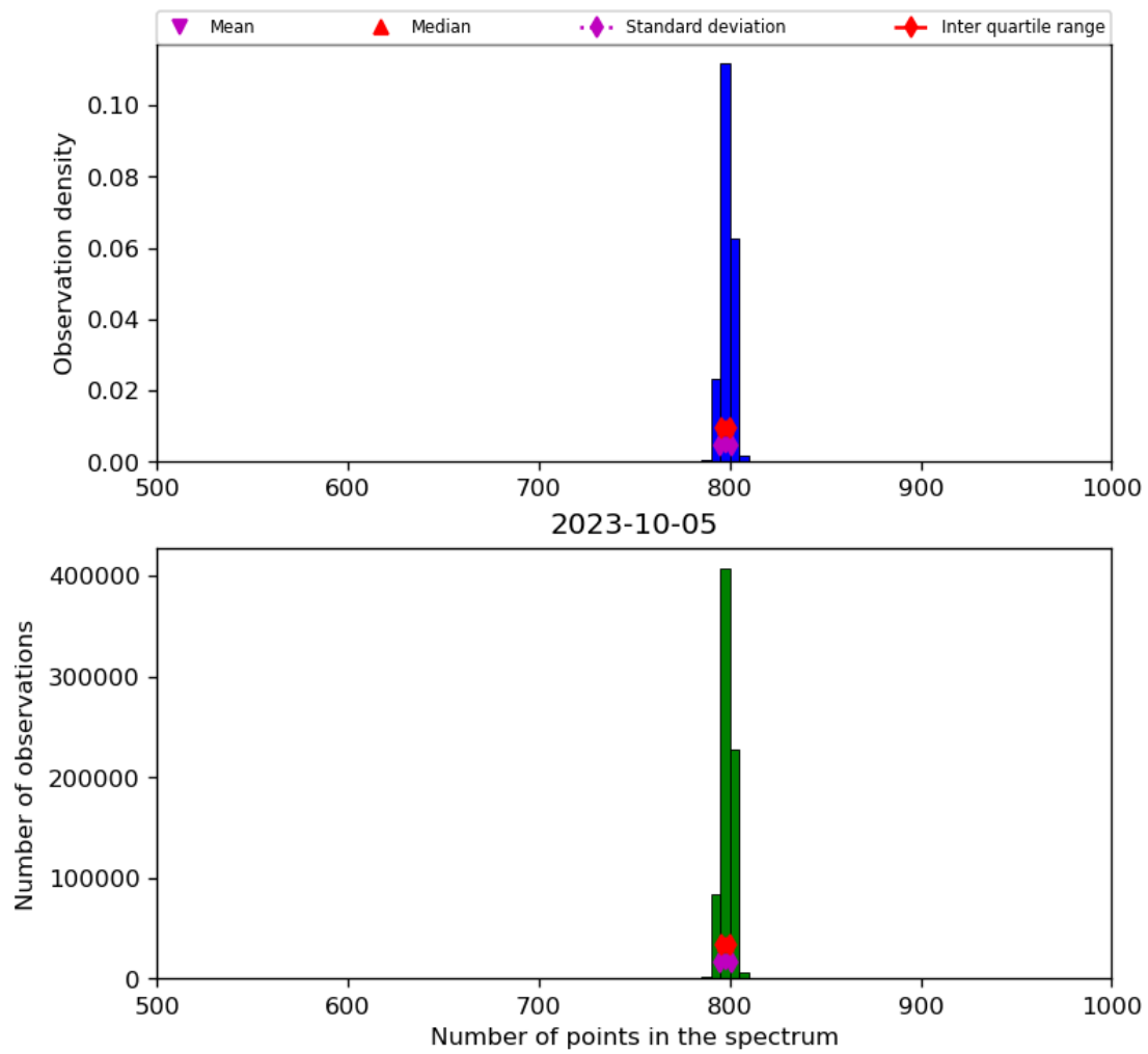
Figure 26: Histogram of “Number of points in the spectrum” for 2023-10-04 to 2023-10-06
