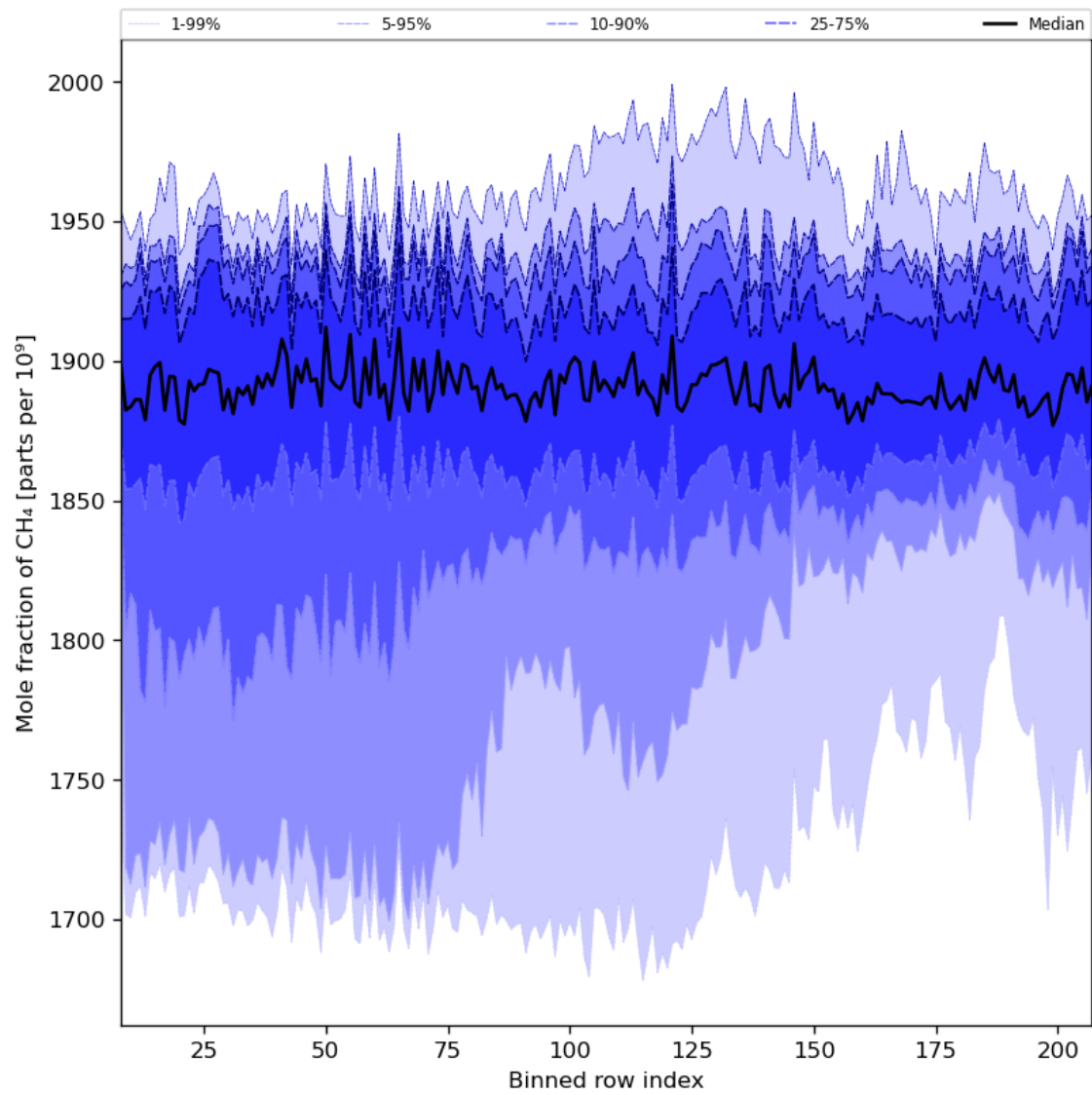
Figure 34: Along track statistics of “Mole fraction of CH 4 ” for 2023-10-04 to 2023-10-06
