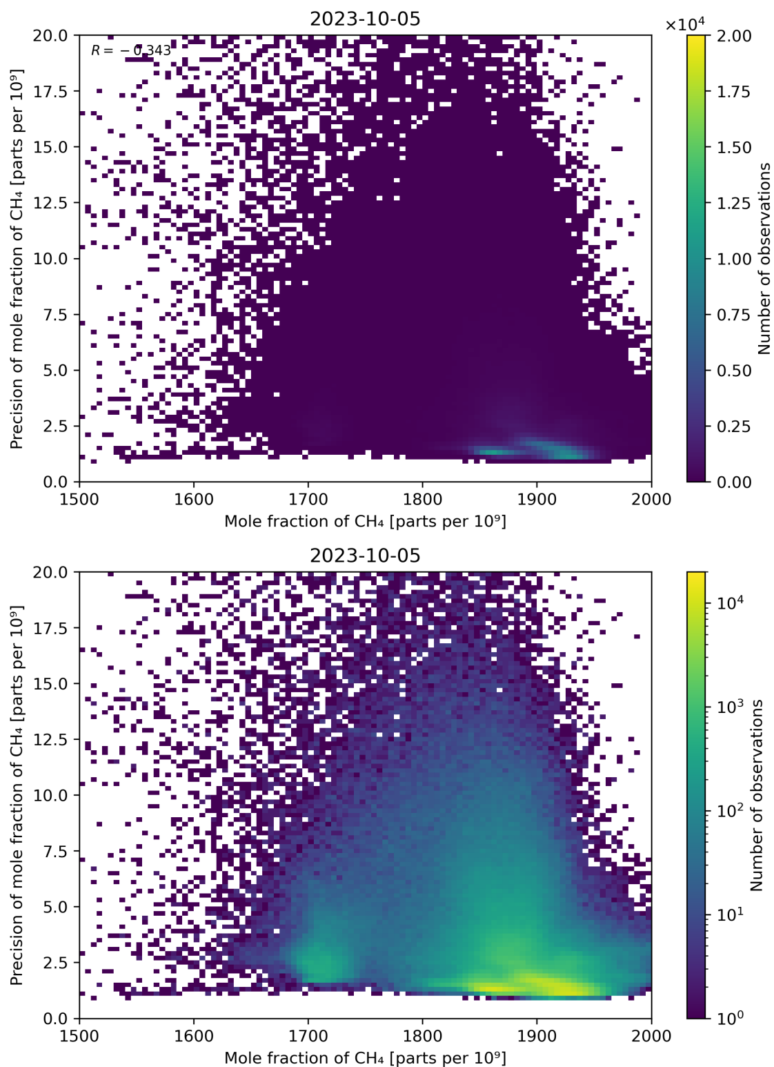
Figure 75: Scatter density plot of “Mole fraction of CH 4 ” against “Precision of mole fraction of CH 4 ” for 2023-10-04 to 2023-10-06.
