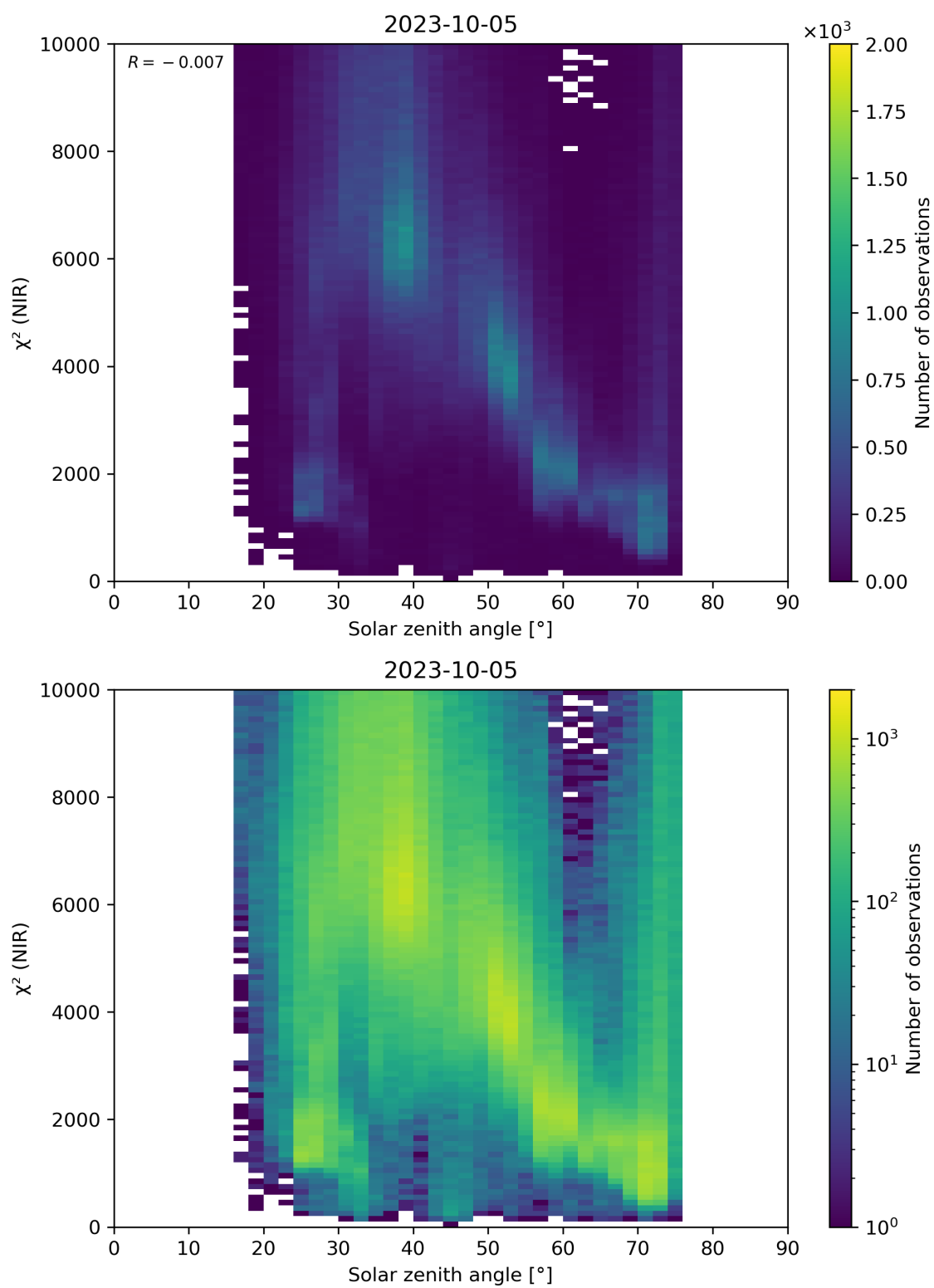
Figure 94: Scatter density plot of “Solar zenith angle” against “ \chi^2 (NIR)” for 2023-10-04 to 2023-10-06.
