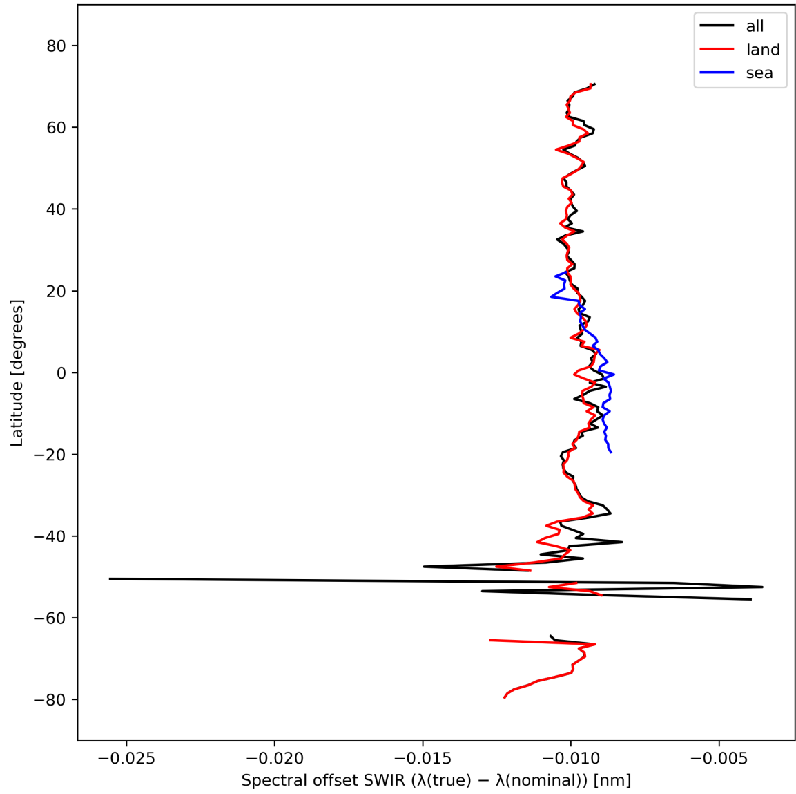
Figure 16: Zonal average of “Spectral offset SWIR ( \lambda(\text{true}) - \lambda(\text{nominal}) )” for 2023-10-04 to 2023-10-06.
