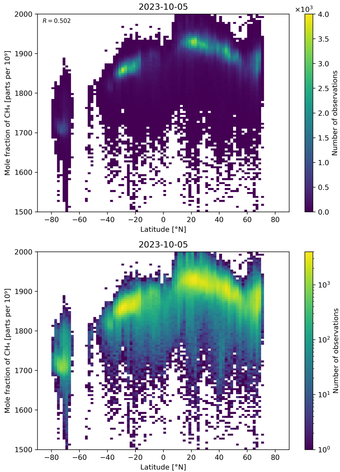
Figure 57: Scatter density plot of “Latitude” against “Mole fraction of CH 4 ” for 2023-10-04 to 2023-10-06.
