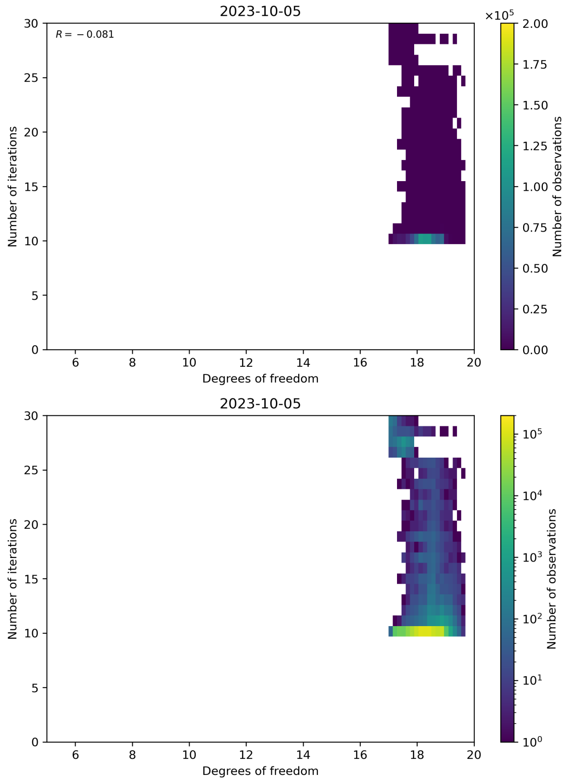
Figure 52: Scatter density plot of “Degrees of freedom” against “Number of iterations” for 2023-10-04 to 2023-10-06.
