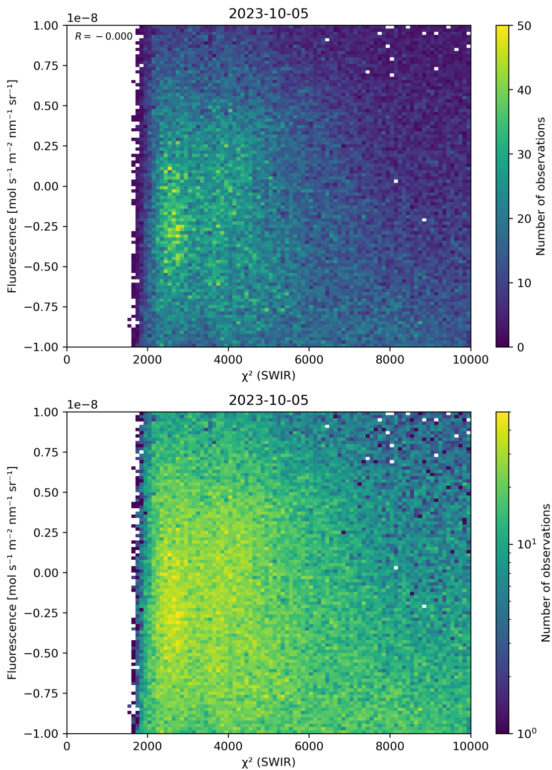
Figure 49: Scatter density plot of “ \chi^2 (SWIR)” against “Fluorescence” for 2023-10-04 to 2023-10-06.
