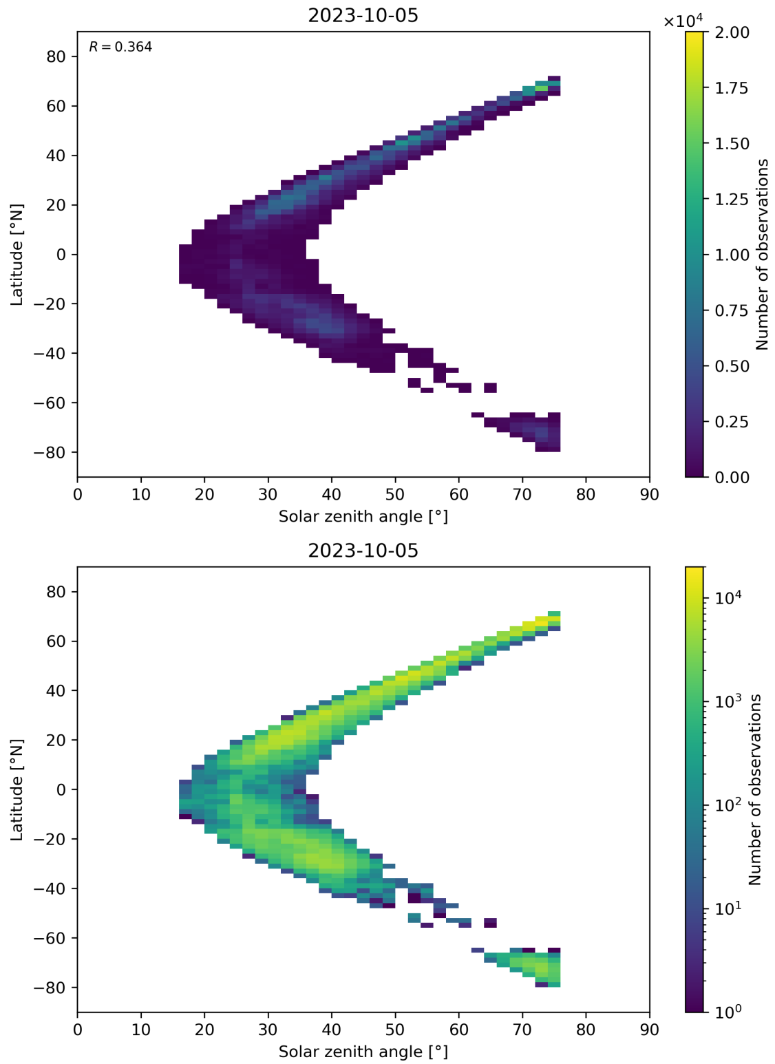
Figure 98: Scatter density plot of “Solar zenith angle” against “Latitude” for 2023-10-04 to 2023-10-06.
