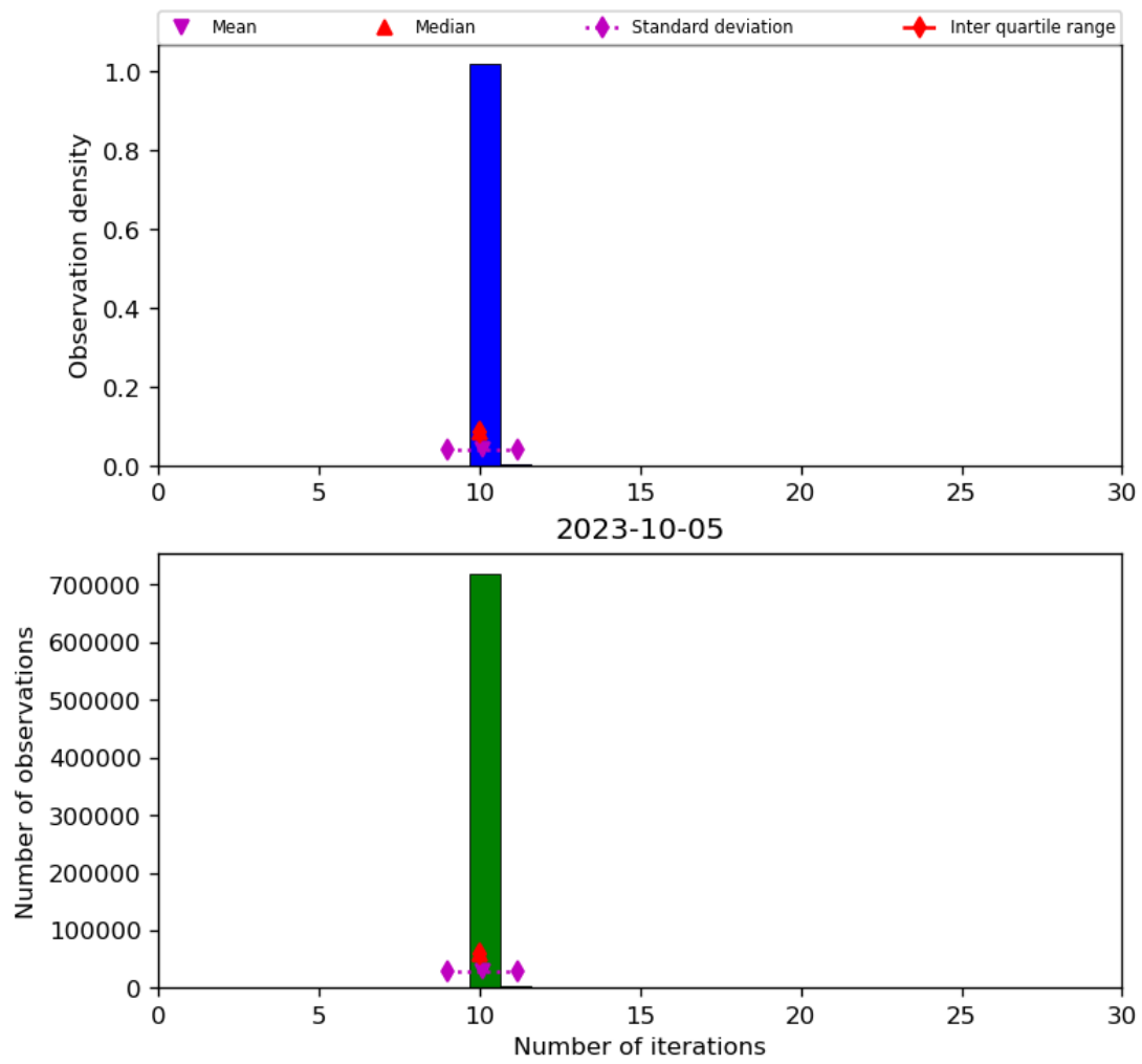
Figure 31: Histogram of “Number of iterations” for 2023-10-04 to 2023-10-06
