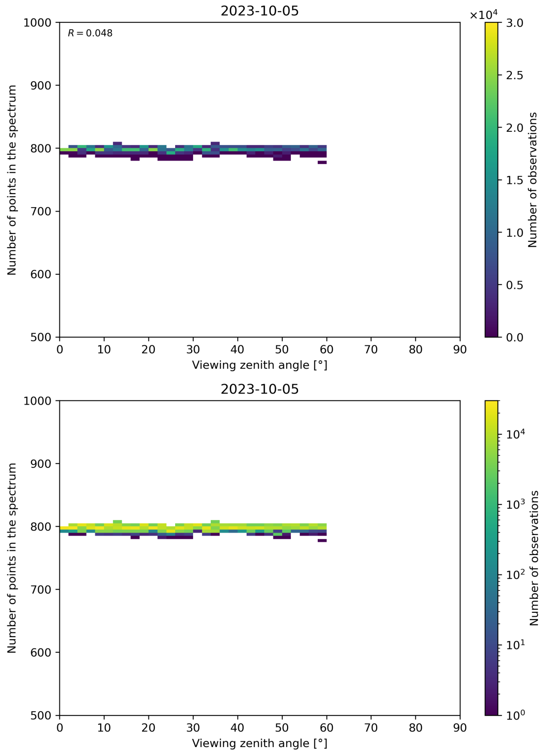
Figure 114: Scatter density plot of “Viewing zenith angle” against “Number of points in the spectrum” for 2023-10-04 to 2023-10-06.
