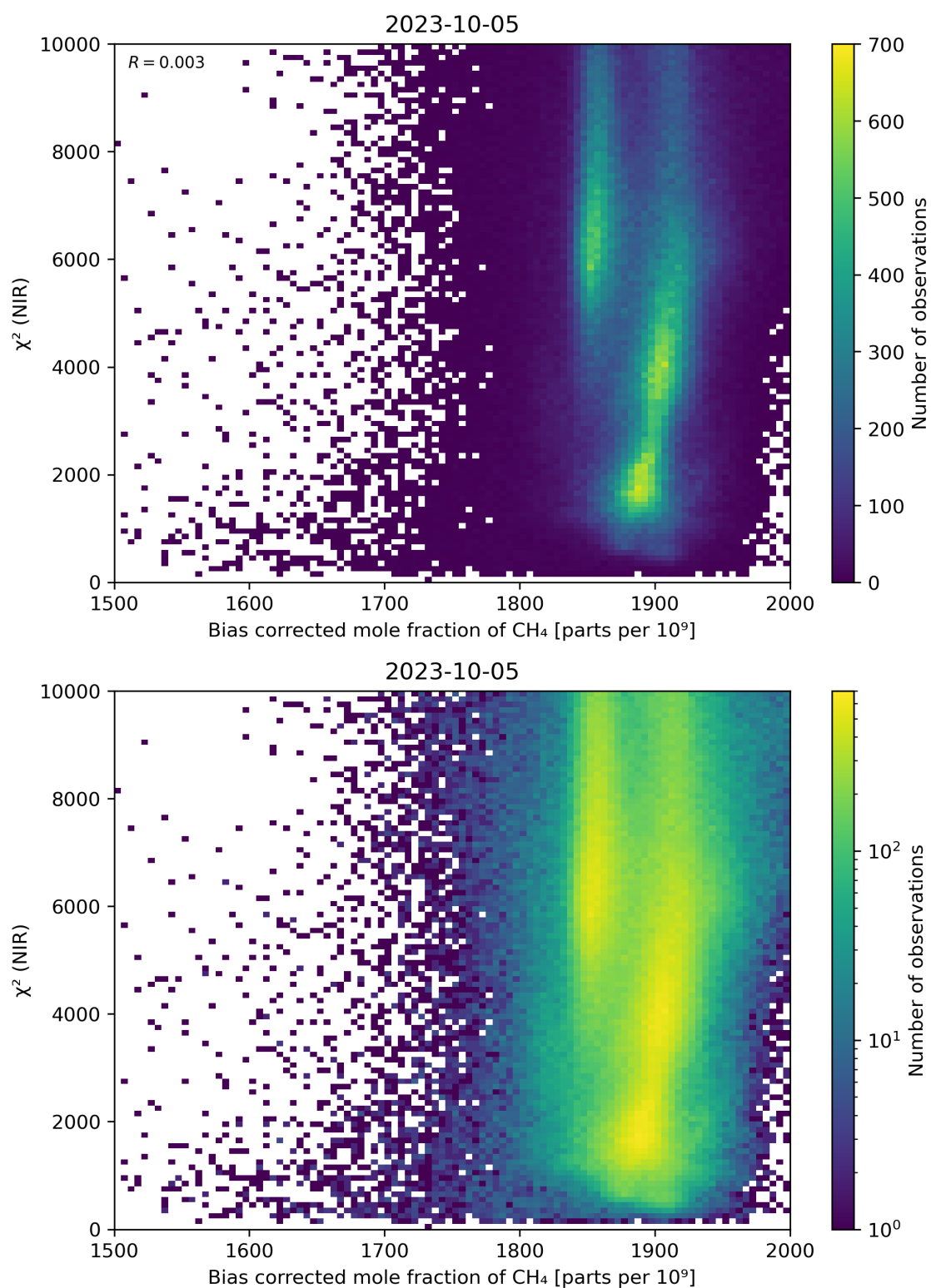
Figure 63: Scatter density plot of “Bias corrected mole fraction of CH 4 ” against “ \chi^2 (NIR)” for 2023-10-04 to 2023-10-06.
