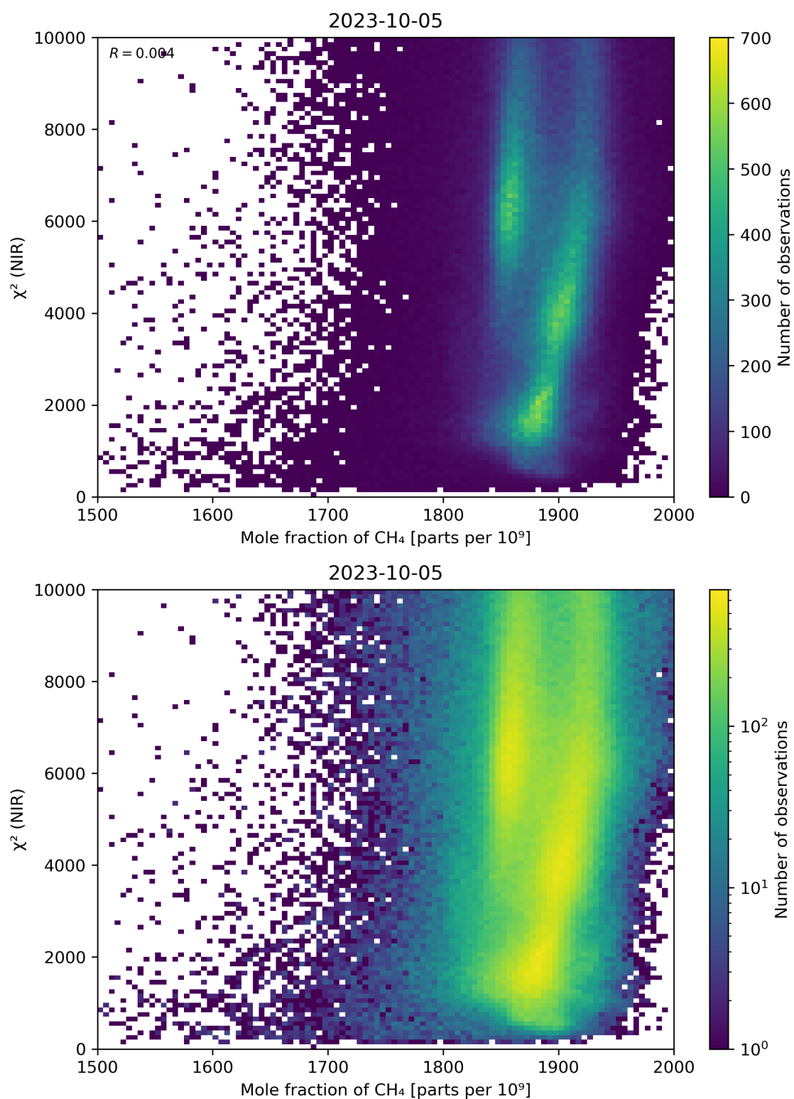
Figure 70: Scatter density plot of “Mole fraction of CH 4 ” against “ \chi^2 (NIR)” for 2023-10-04 to 2023-10-06.
