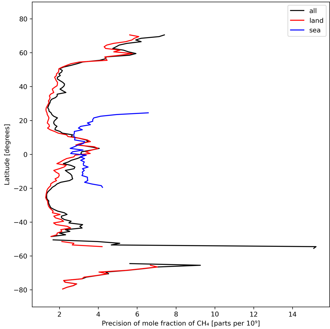
Figure 13: Zonal average of “Precision of mole fraction of CH 4 ” for 2023-10-04 to 2023-10-06.
