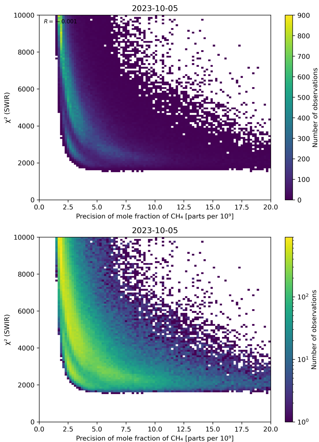
Figure 79: Scatter density plot of “Precision of mole fraction of \text{CH}_4 ” against “ \chi^2 (SWIR)” for 2023-10-04 to 2023-10-06.
