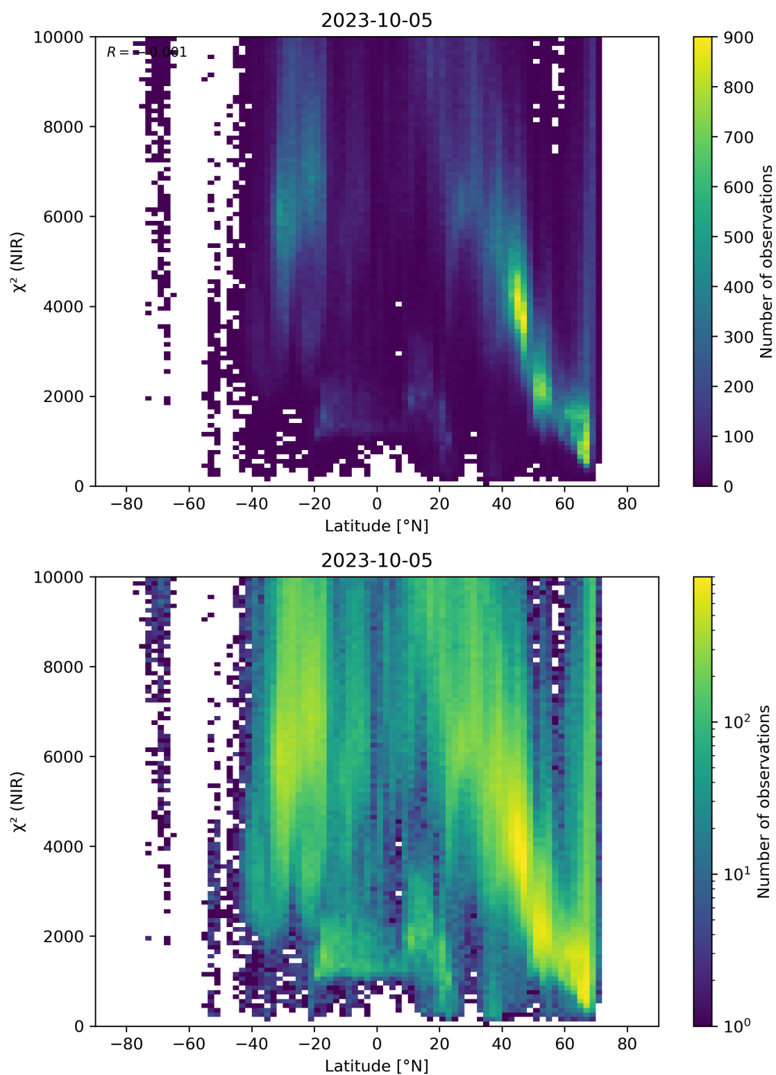
Figure 53: Scatter density plot of “Latitude” against “ \chi^2 (NIR)” for 2023-10-04 to 2023-10-06.
