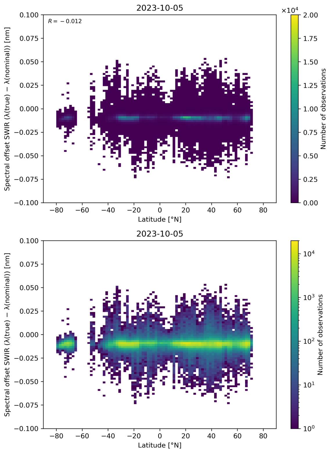
Figure 62: Scatter density plot of “Latitude” against “Spectral offset SWIR ( \lambda(\text{true}) - \lambda(\text{nominal}) )” for 2023-10-04 to 2023-10-06.
