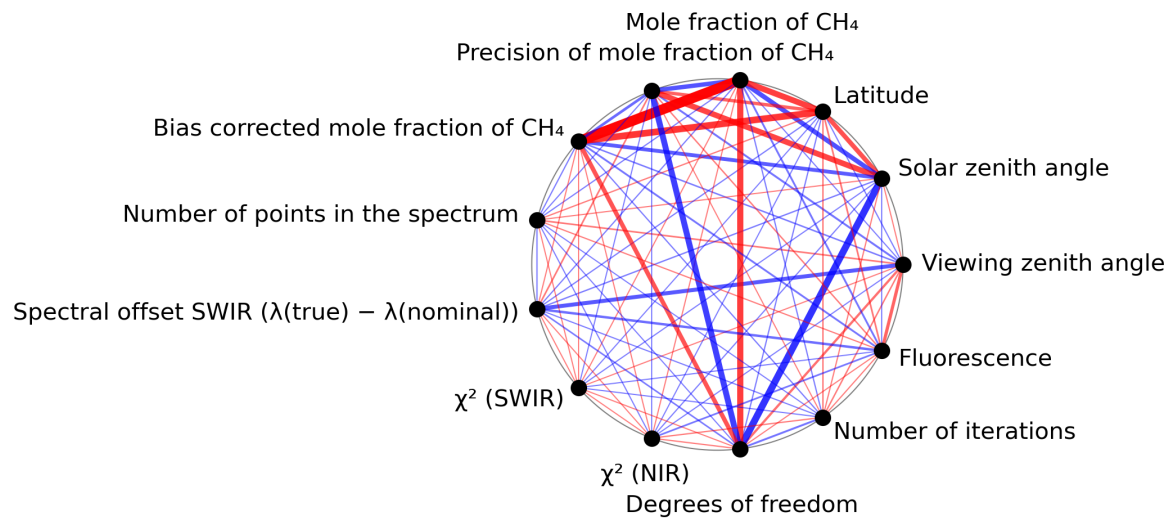
Figure 1: Map of correlation graph for 2023-10-04 to 2023-10-06.
