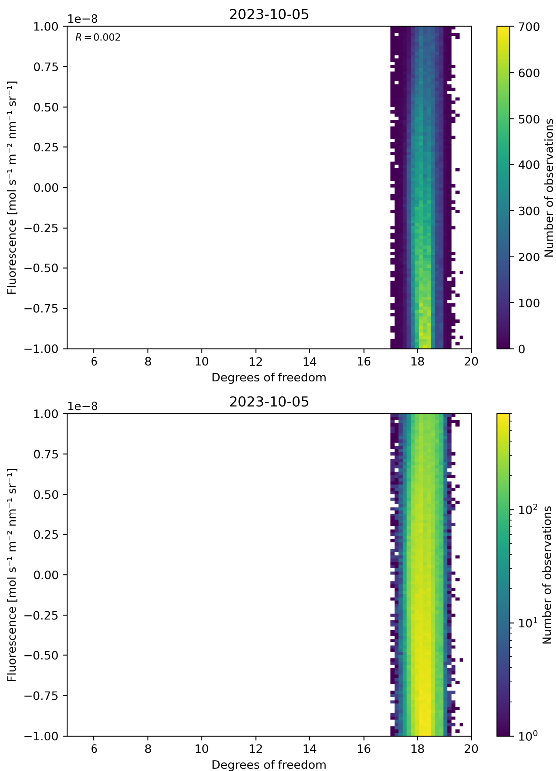
Figure 51: Scatter density plot of “Degrees of freedom” against “Fluorescence” for 2023-10-04 to 2023-10-06.
