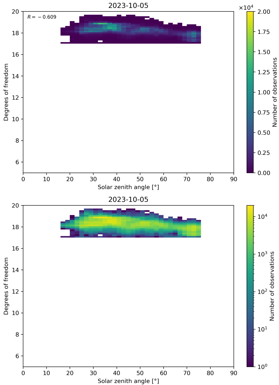
Figure 96: Scatter density plot of “Solar zenith angle” against “Degrees of freedom” for 2023-10-04 to 2023-10-06.
