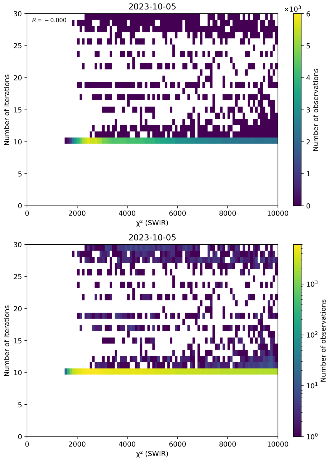
Figure 50: Scatter density plot of “ \chi^2 (SWIR)” against “Number of iterations” for 2023-10-04 to 2023-10-06.
