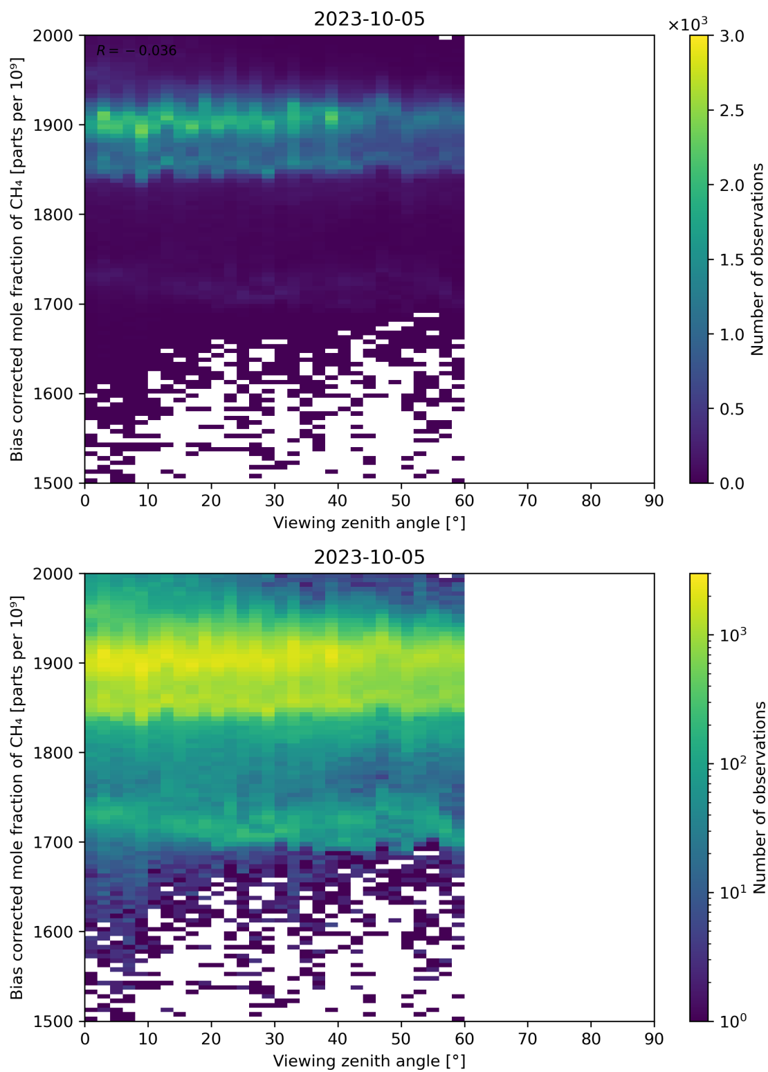
Figure 111: Scatter density plot of “Viewing zenith angle” against “Bias corrected mole fraction of CH 4 ” for 2023-10-04 to 2023-10-06.
