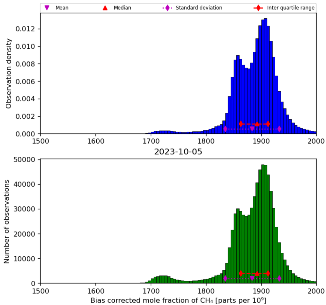
Figure 25: Histogram of “Bias corrected mole fraction of CH 4 ” for 2023-10-04 to 2023-10-06
