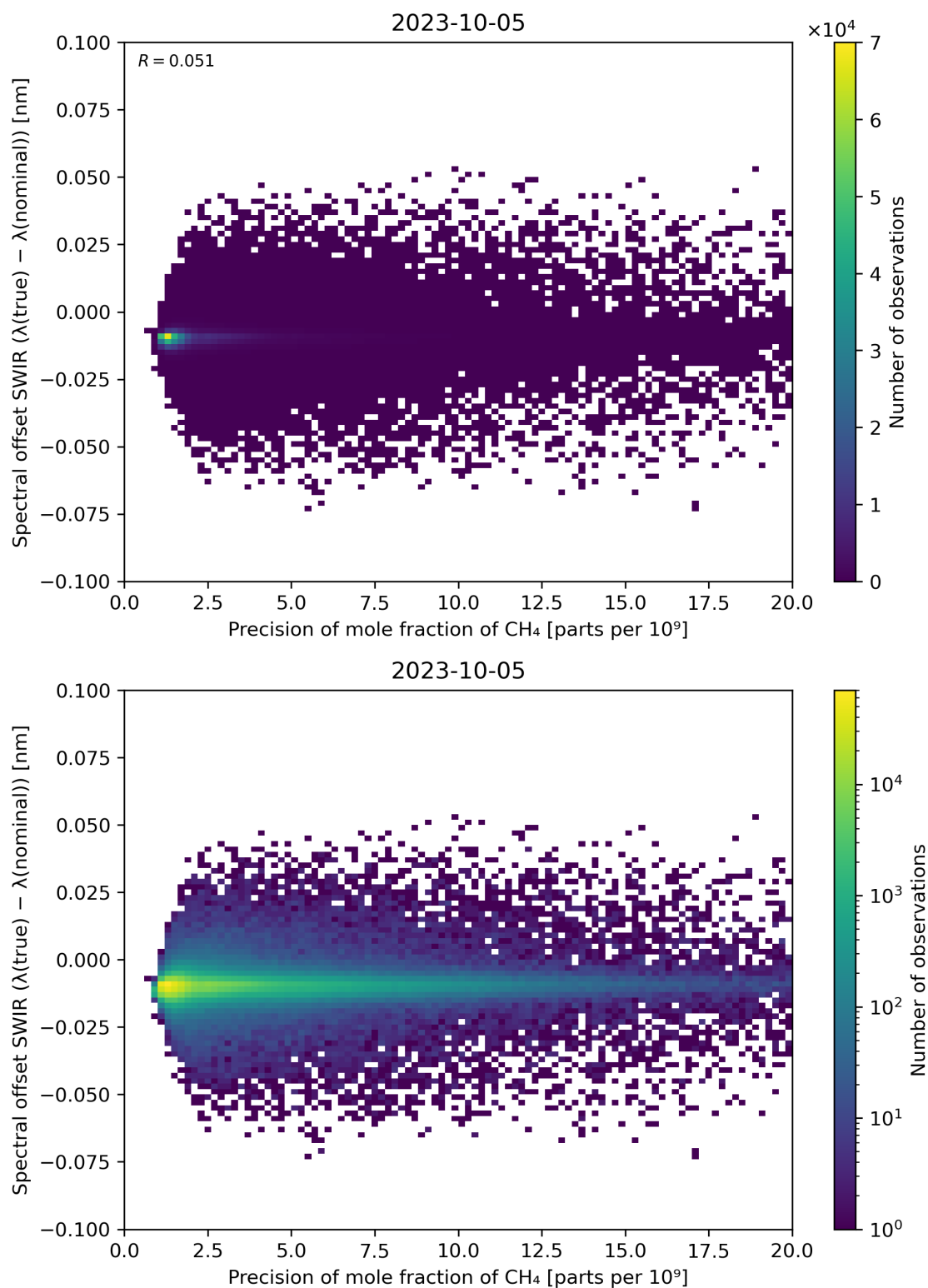
Figure 85: Scatter density plot of “Precision of mole fraction of CH 4 ” against “Spectral offset SWIR ( \lambda(\text{true}) - \lambda(\text{nominal}) )” for 2023-10-04 to 2023-10-06.
