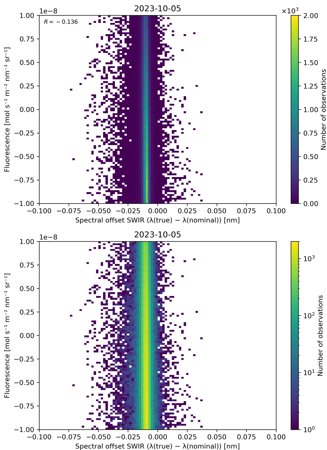
Figure 120: Scatter density plot of “Spectral offset SWIR ( \lambda(\text{true}) - \lambda(\text{nominal}) )” against “Fluorescence” for 2023-10-04 to 2023-10-06.
