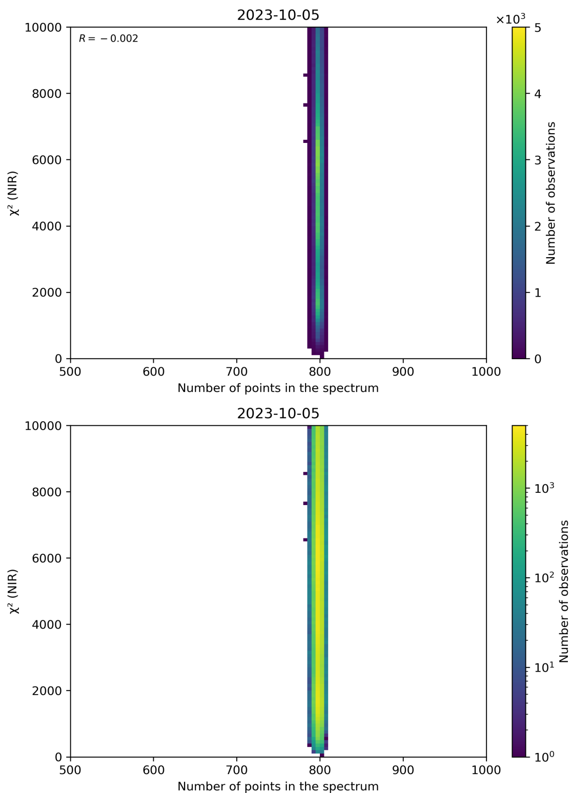
Figure 88: Scatter density plot of “Number of points in the spectrum” against “ \chi^2 (NIR)” for 2023-10-04 to 2023-10-06.
