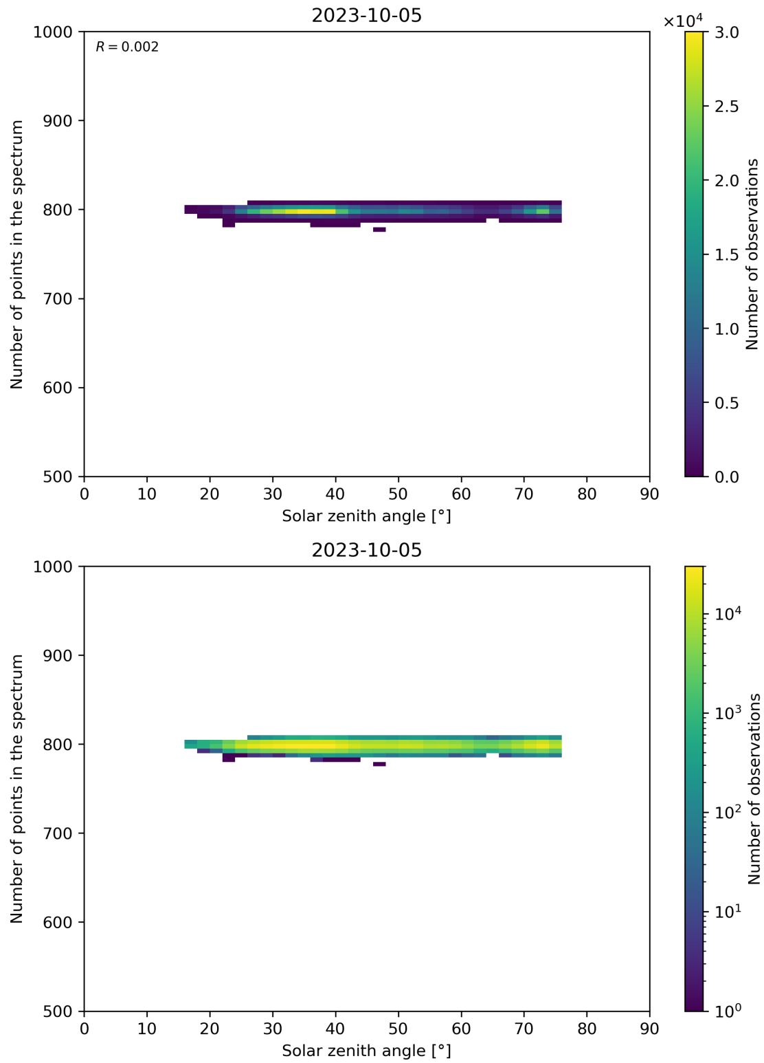
Figure 103: Scatter density plot of “Solar zenith angle” against “Number of points in the spectrum” for 2023-10-04 to 2023-10-06.
