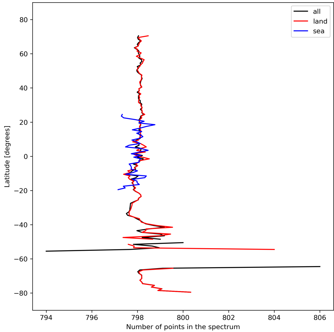
Figure 15: Zonal average of “Number of points in the spectrum” for 2023-10-04 to 2023-10-06.
