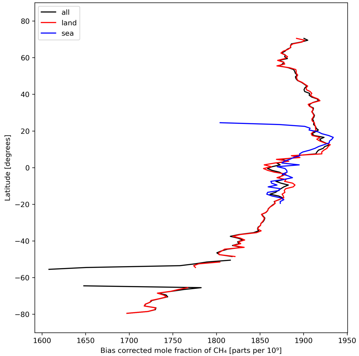
Figure 14: Zonal average of “Bias corrected mole fraction of CH 4 ” for 2023-10-04 to 2023-10-06.
