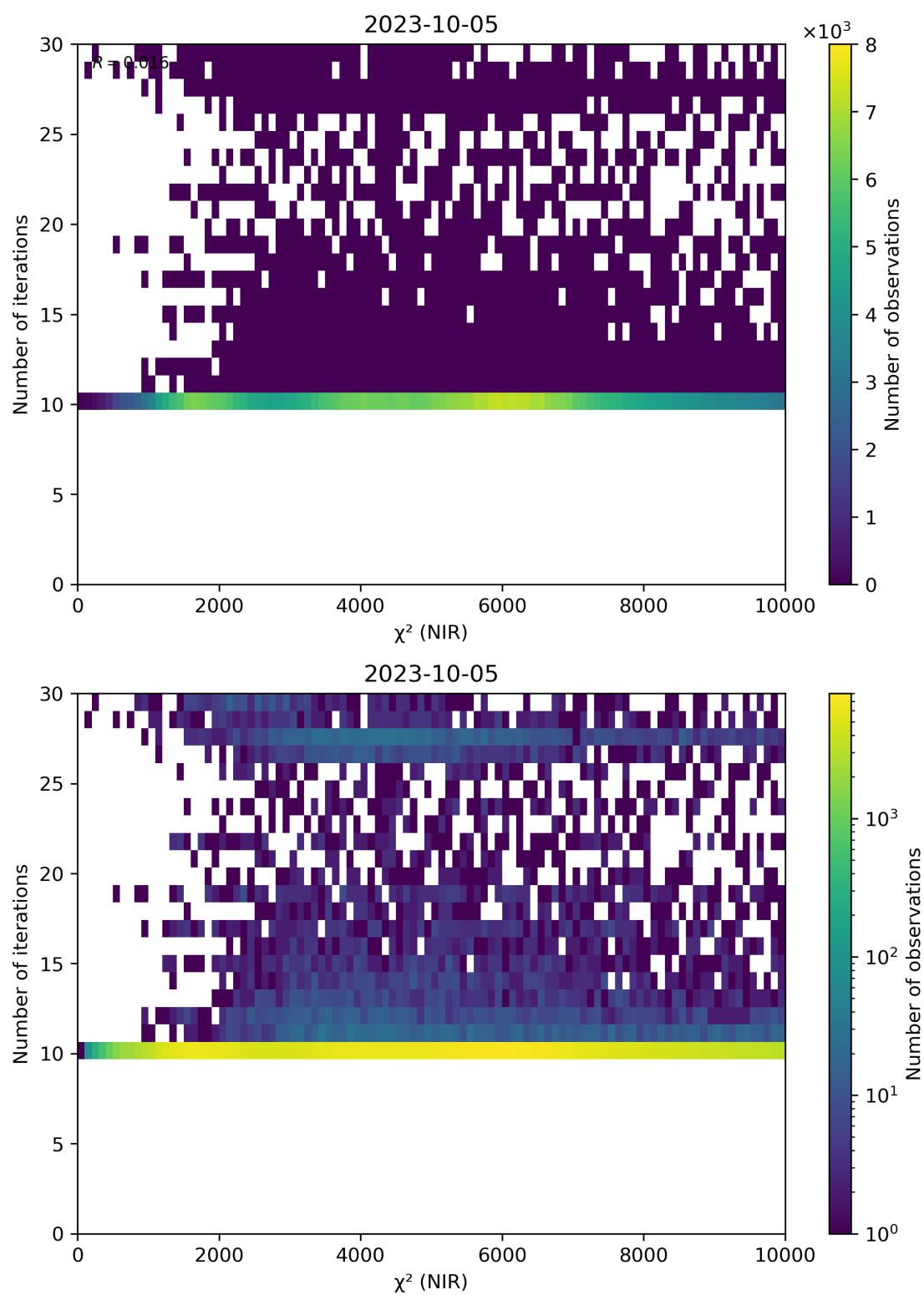
Figure 46: Scatter density plot of “ \chi^2 (NIR)” against “Number of iterations” for 2023-10-04 to 2023-10-06.
