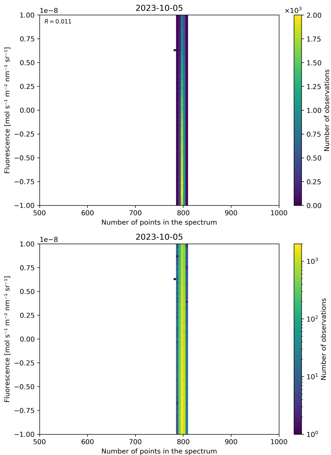
Figure 91: Scatter density plot of “Number of points in the spectrum” against “Fluorescence” for 2023-10-04 to 2023-10-06.
