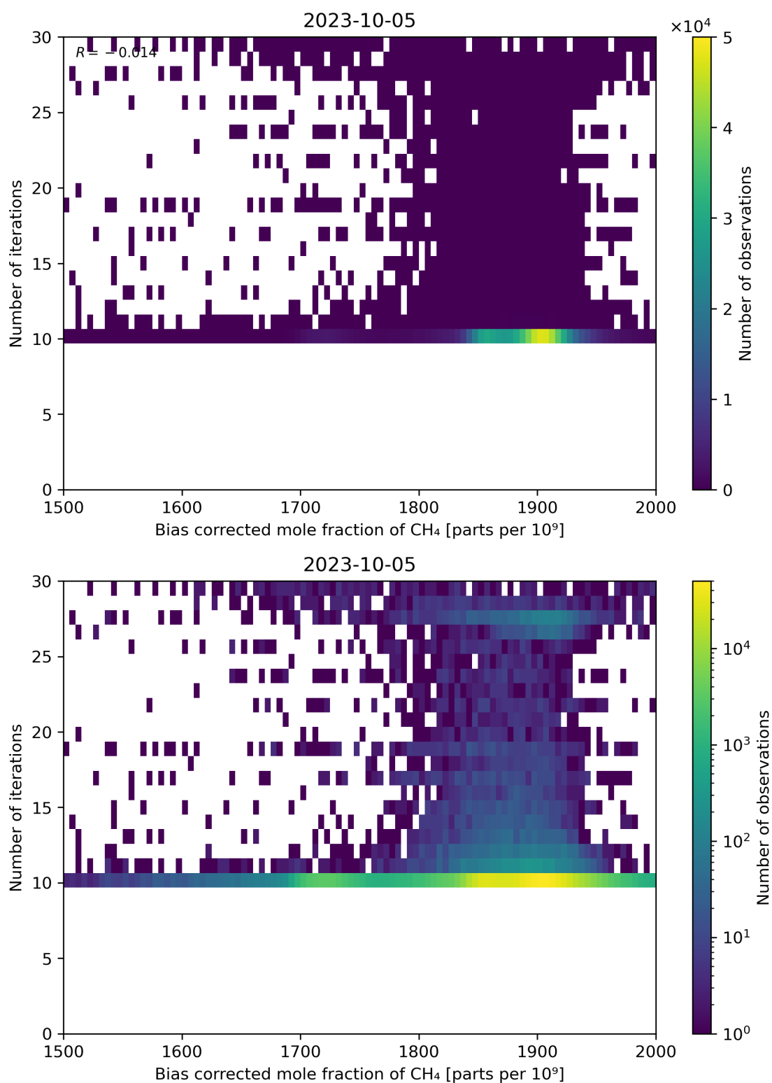
Figure 67: Scatter density plot of “Bias corrected mole fraction of CH 4 ” against “Number of iterations” for 2023-10-04 to 2023-10-06.
