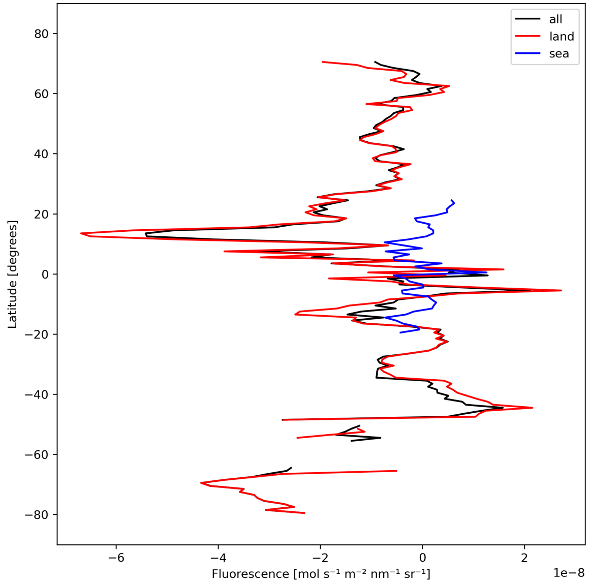
Figure 21: Zonal average of “Fluorescence” for 2023-10-04 to 2023-10-06.
