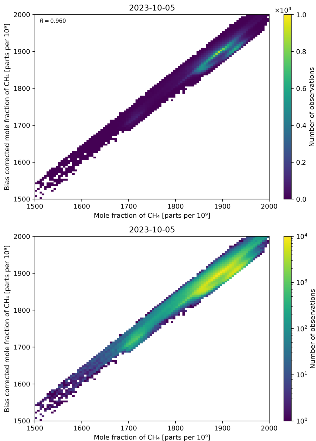
Figure 74: Scatter density plot of “Mole fraction of CH 4 ” against “Bias corrected mole fraction of CH 4 ” for 2023-10-04 to 2023-10-06.
