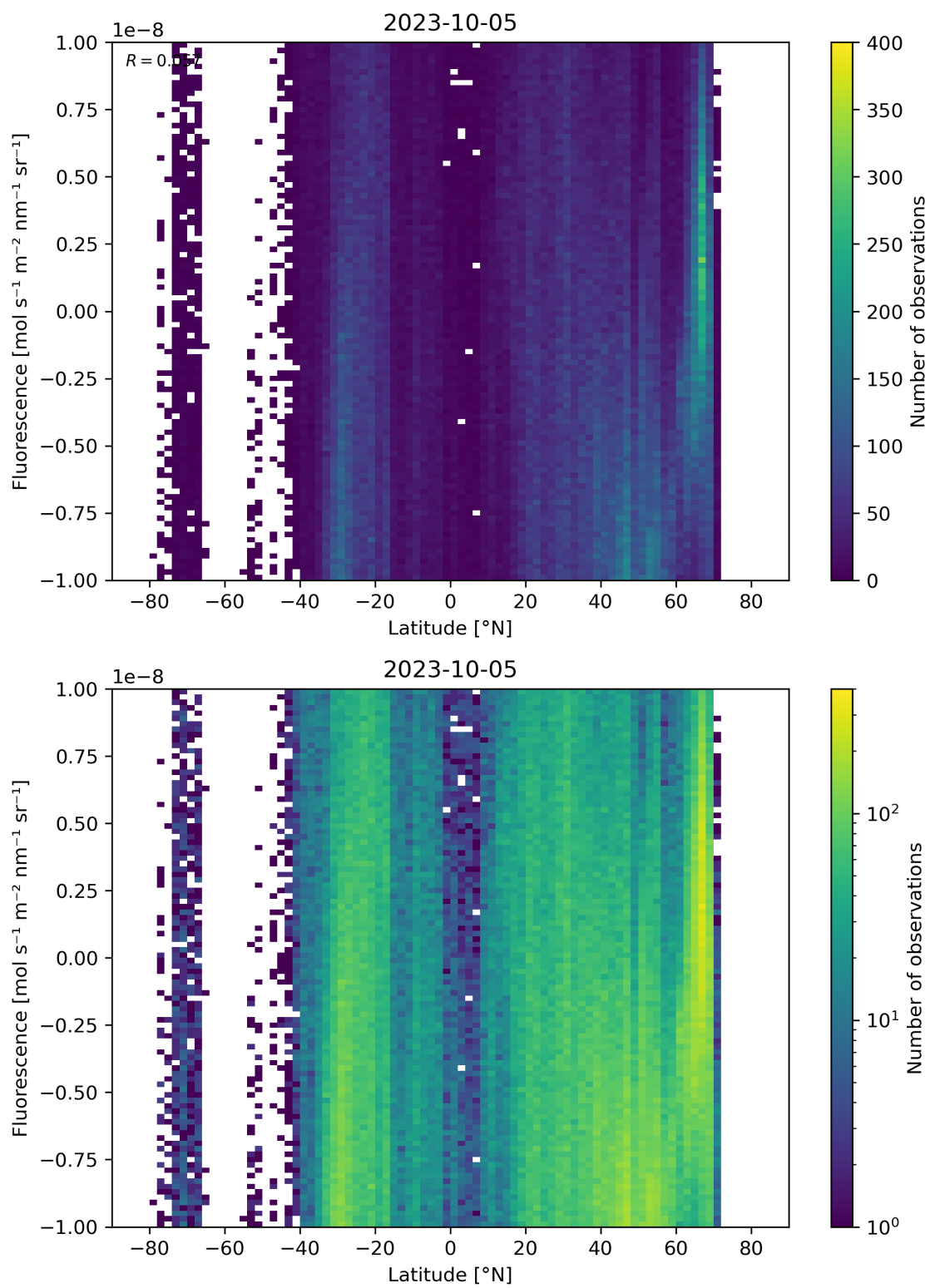
Figure 56: Scatter density plot of “Latitude” against “Fluorescence” for 2023-10-04 to 2023-10-06.
