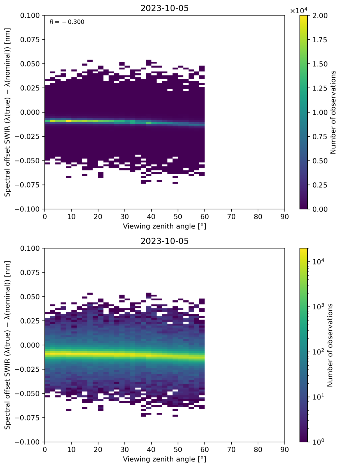
Figure 116: Scatter density plot of “Viewing zenith angle” against “Spectral offset SWIR ( \lambda(\text{true}) - \lambda(\text{nominal}) )” for 2023-10-04 to 2023-10-06.
