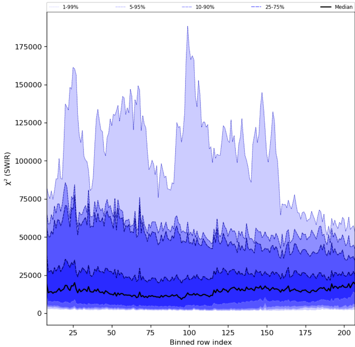
Figure 39: Along track statistics of “ \chi^2 (SWIR)” for 2023-10-04 to 2023-10-06
