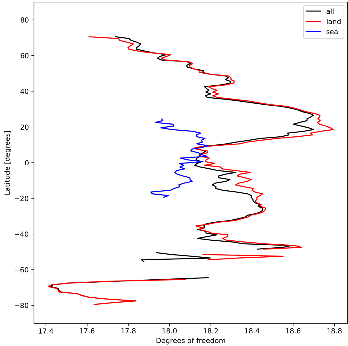
Figure 19: Zonal average of “Degrees of freedom” for 2023-10-04 to 2023-10-06.
