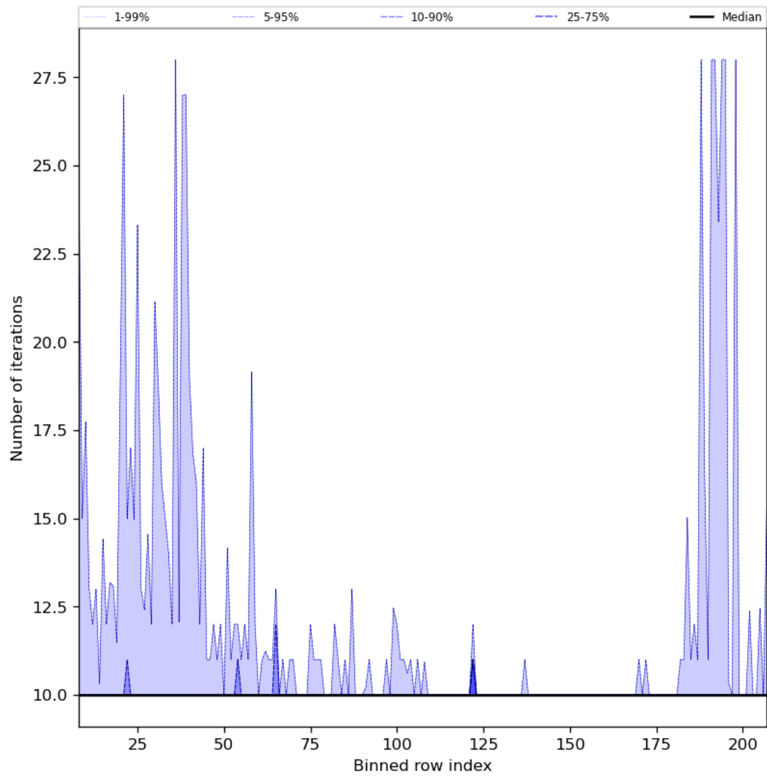
Figure 42: Along track statistics of “Number of iterations” for 2023-10-04 to 2023-10-06
