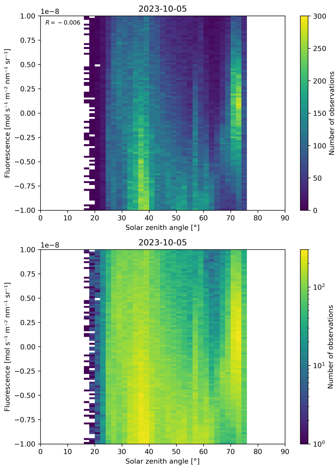
Figure 97: Scatter density plot of “Solar zenith angle” against “Fluorescence” for 2023-10-04 to 2023-10-06.
