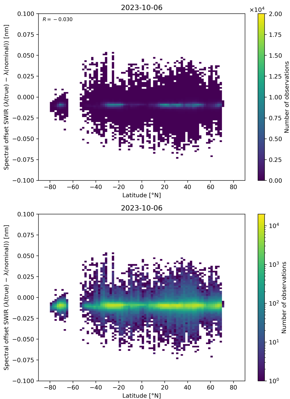
Figure 62: Scatter density plot of “Latitude” against “Spectral offset SWIR ( \lambda(\text{true}) - \lambda(\text{nominal}) )” for 2023-10-06 to 2023-10-07.
