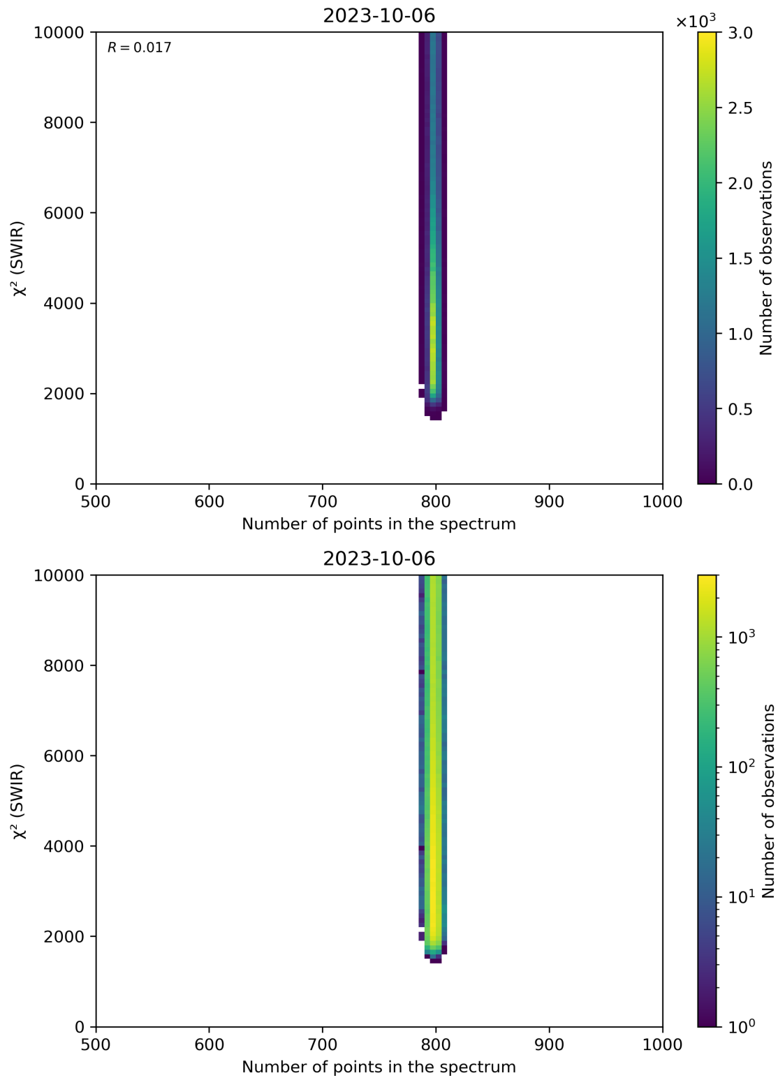
Figure 89: Scatter density plot of “Number of points in the spectrum” against “ \chi^2 (SWIR)” for 2023-10-06 to 2023-10-07.
