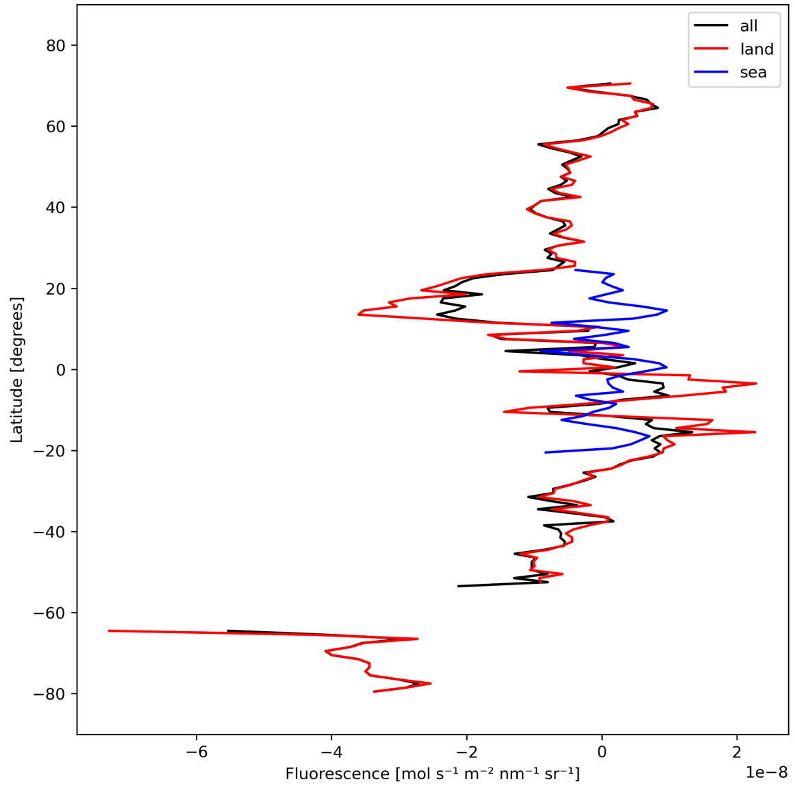
Figure 21: Zonal average of “Fluorescence” for 2023-10-06 to 2023-10-07.
