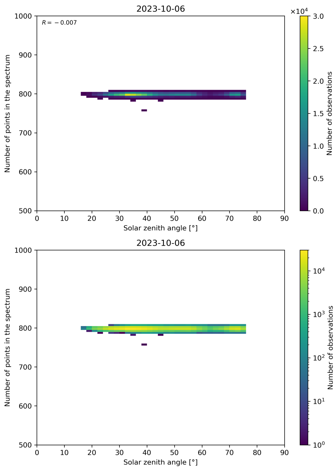
Figure 103: Scatter density plot of “Solar zenith angle” against “Number of points in the spectrum” for 2023-10-06 to 2023-10-07.
