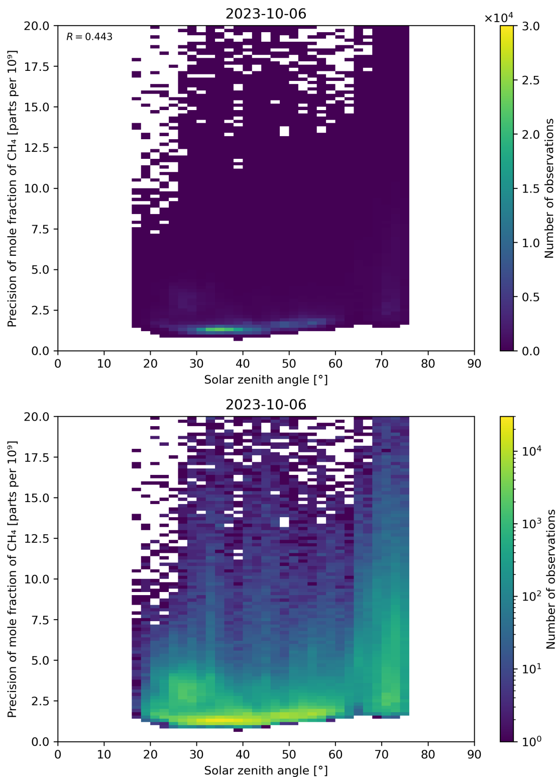
Figure 101: Scatter density plot of “Solar zenith angle” against “Precision of mole fraction of CH 4 ” for 2023-10-06 to 2023-10-07.
