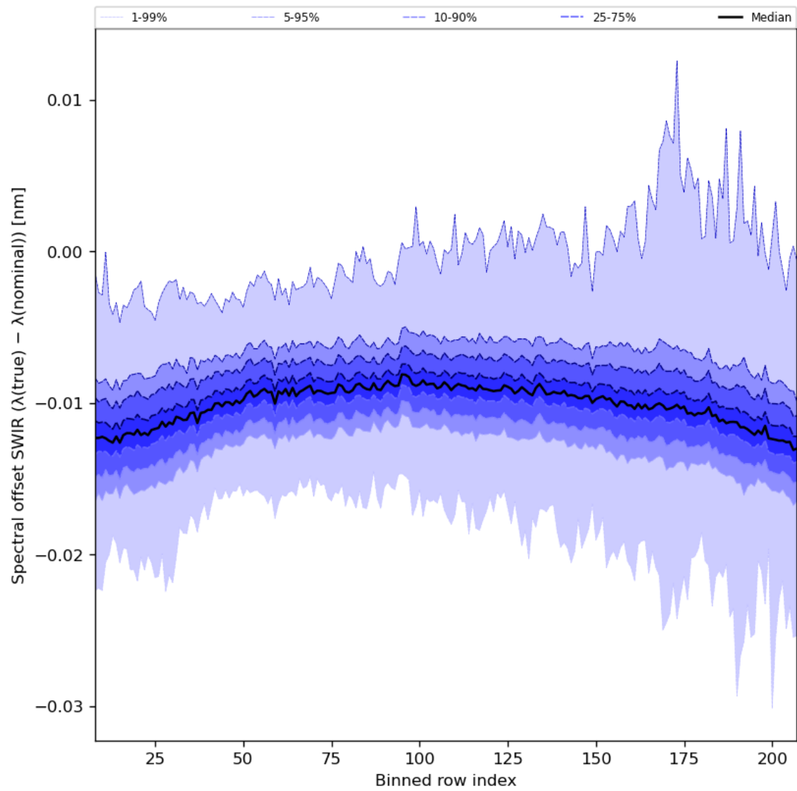
Figure 38: Along track statistics of “Spectral offset SWIR ( \lambda(\text{true}) - \lambda(\text{nominal}) )” for 2023-10-06 to 2023-10-07
