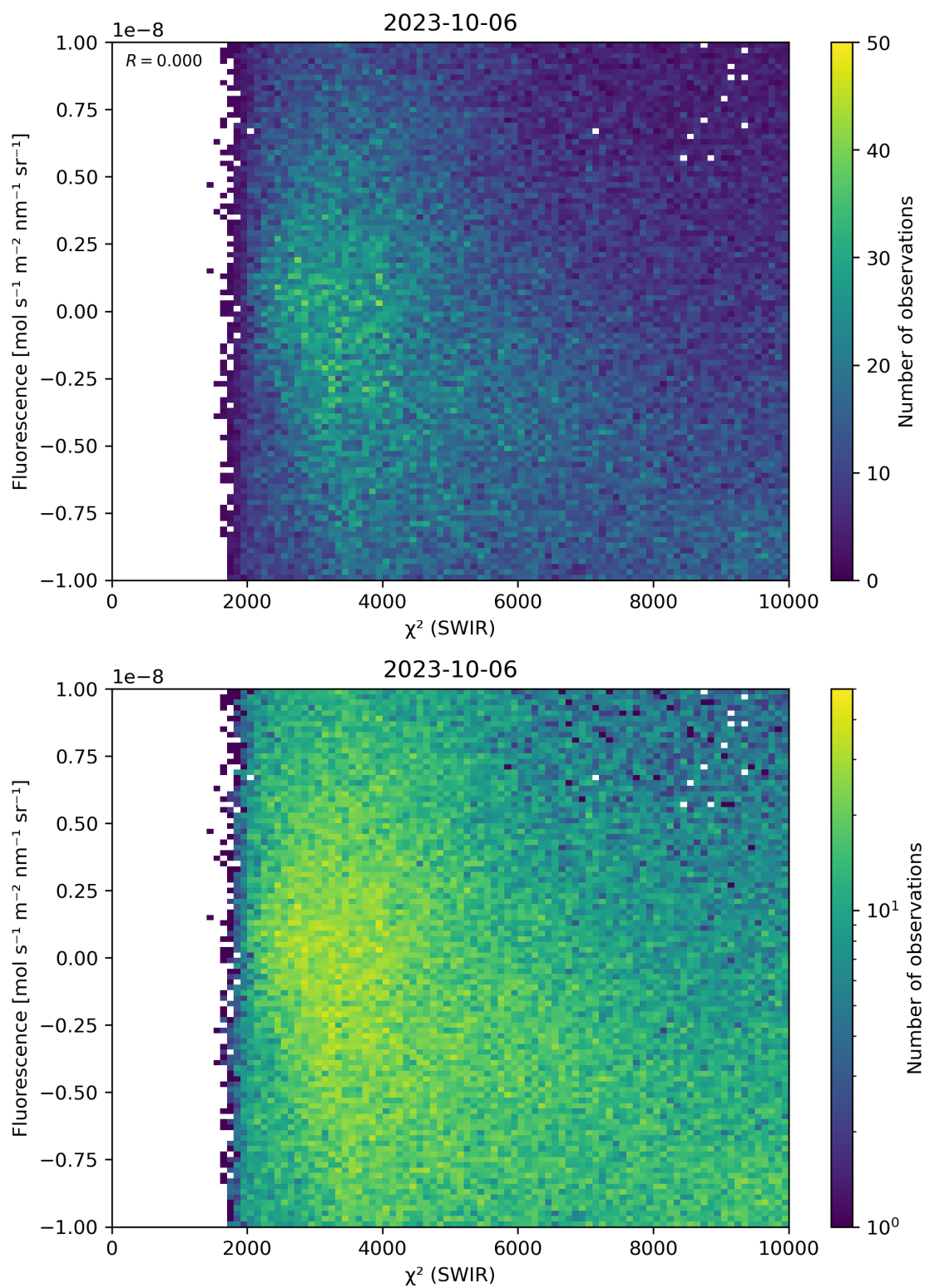
Figure 49: Scatter density plot of “ \chi^2 (SWIR)” against “Fluorescence” for 2023-10-06 to 2023-10-07.
