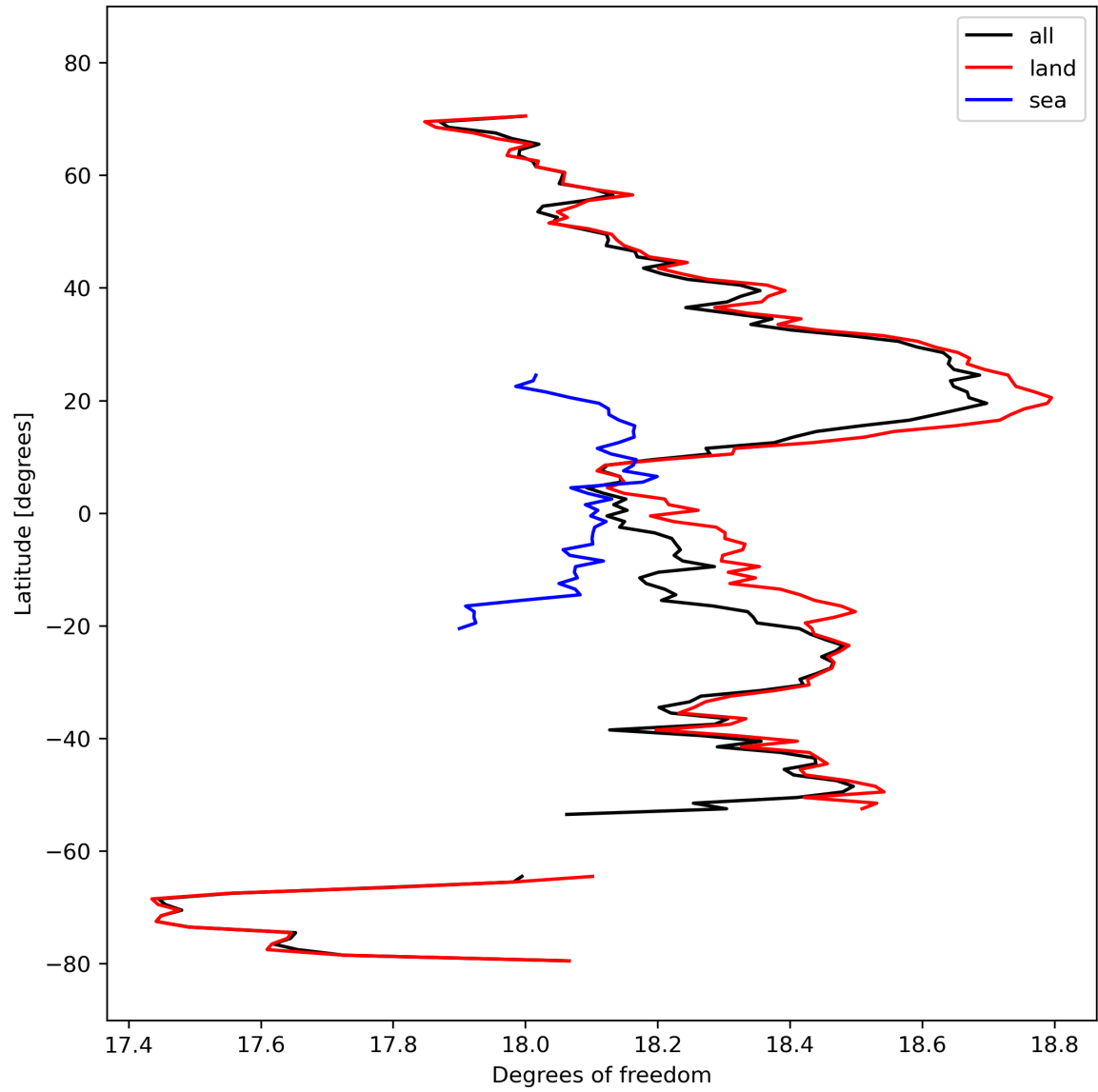
Figure 19: Zonal average of “Degrees of freedom” for 2023-10-06 to 2023-10-07.
