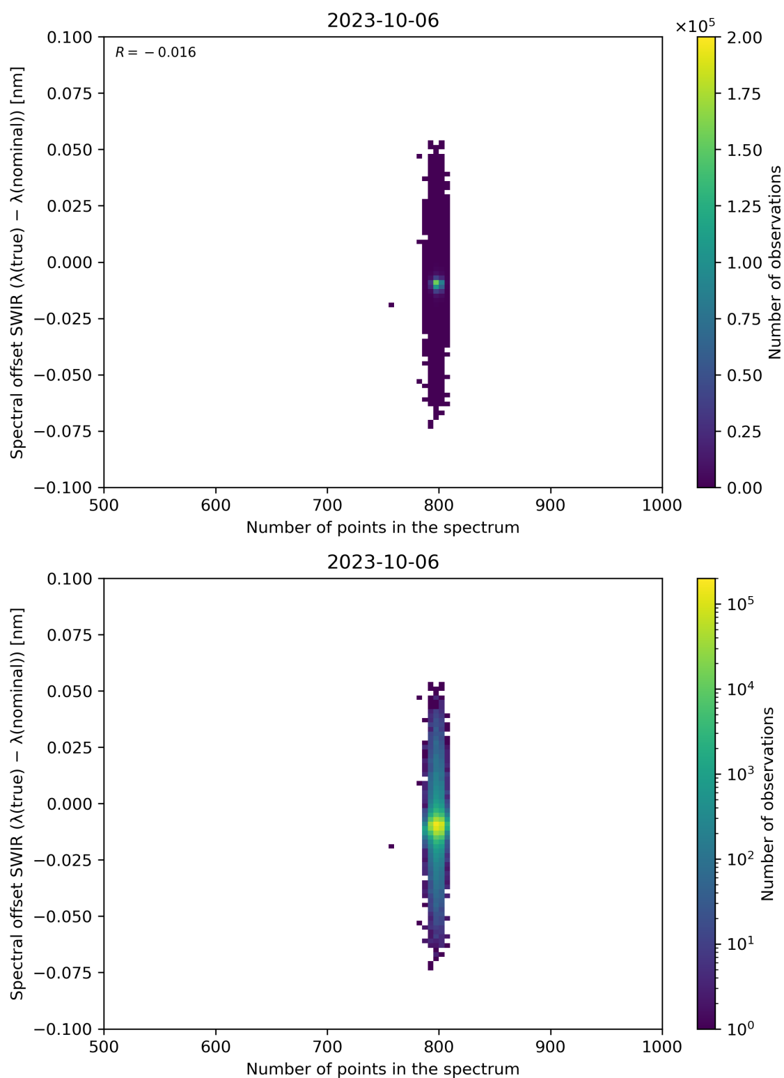
Figure 93: Scatter density plot of “Number of points in the spectrum” against “Spectral offset SWIR ( \lambda(\text{true}) - \lambda(\text{nominal}) )” for 2023-10-06 to 2023-10-07.
