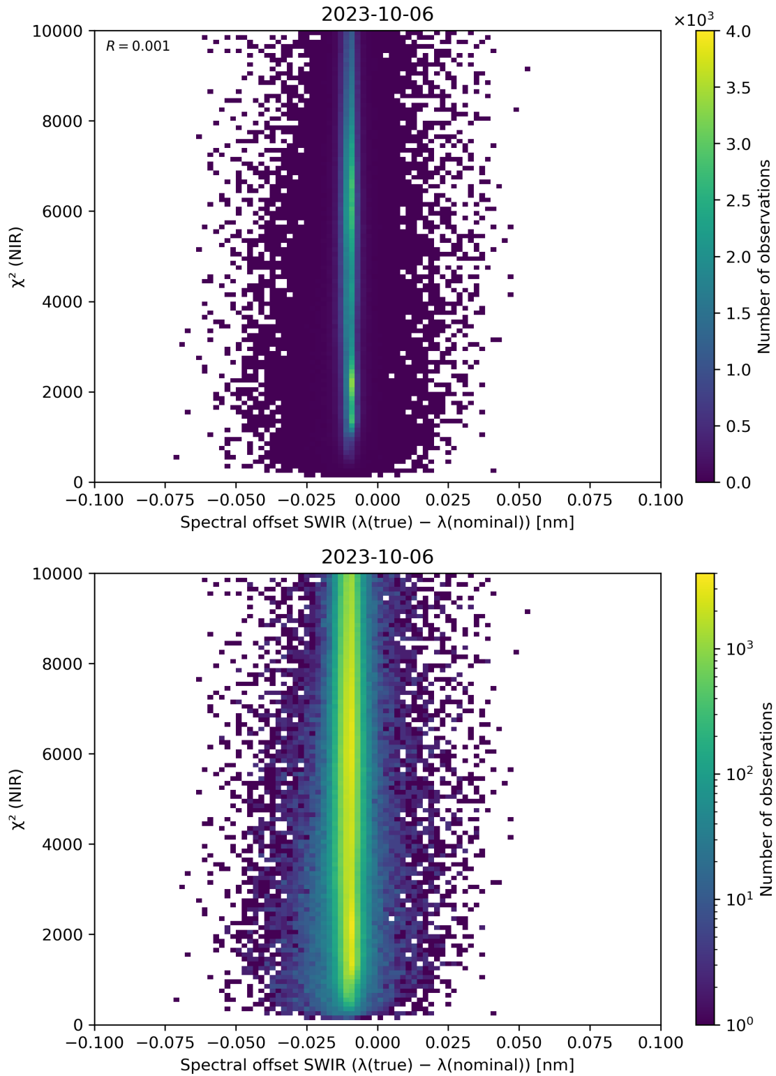
Figure 117: Scatter density plot of “Spectral offset SWIR ( \lambda(\text{true}) - \lambda(\text{nominal}) )” against “ \chi^2 (NIR)” for 2023-10-06 to 2023-10-07.
