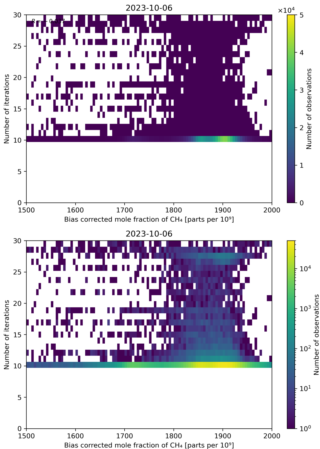
Figure 67: Scatter density plot of “Bias corrected mole fraction of \text{CH}_4 ” against “Number of iterations” for 2023-10-06 to 2023-10-07.
