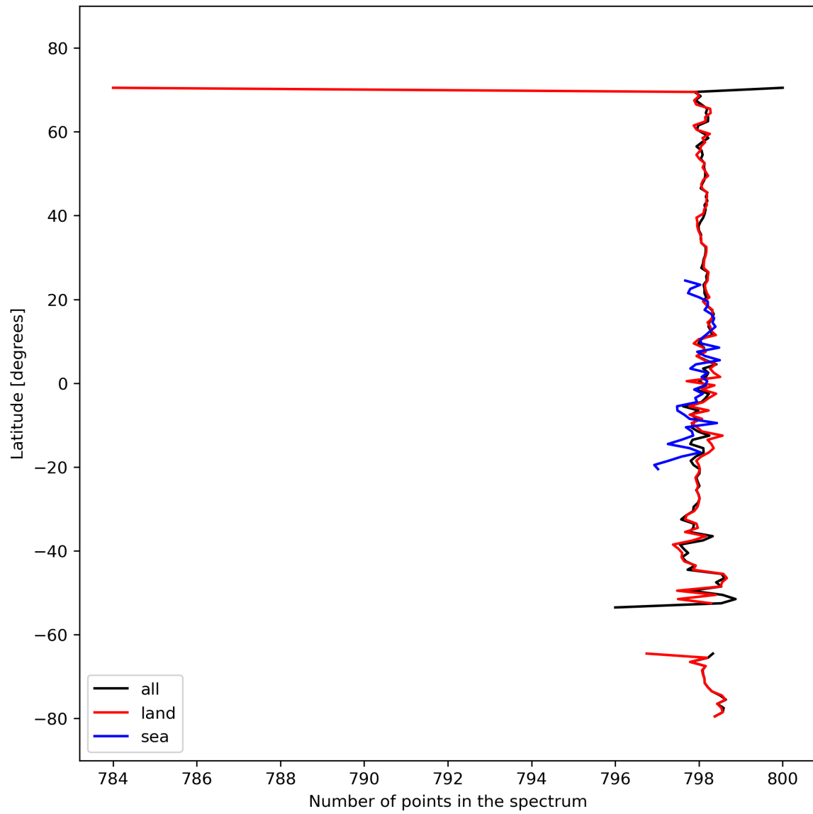
Figure 15: Zonal average of “Number of points in the spectrum” for 2023-10-06 to 2023-10-07.
