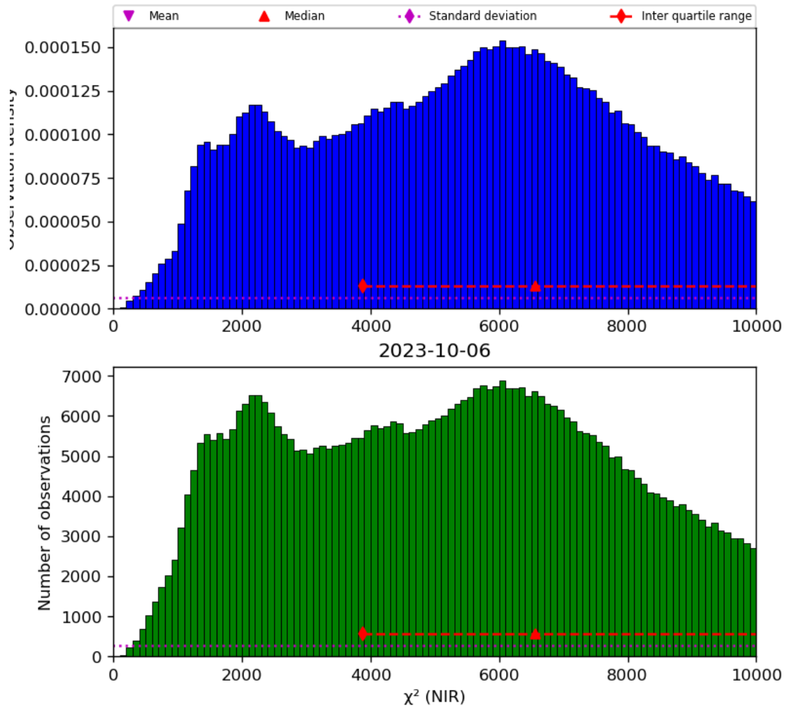
Figure 29: Histogram of “ \chi^2 (NIR)” for 2023-10-06 to 2023-10-07
