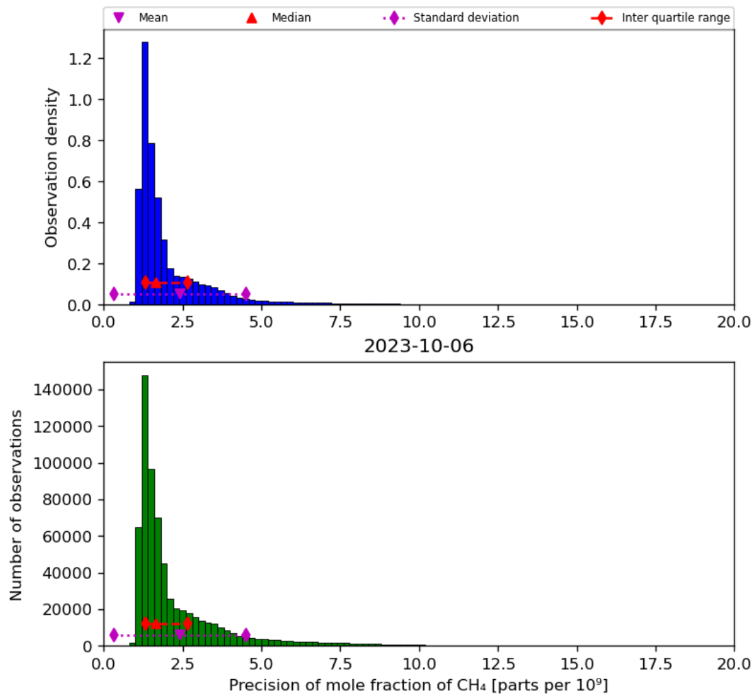
Figure 24: Histogram of “Precision of mole fraction of CH 4 ” for 2023-10-06 to 2023-10-07
