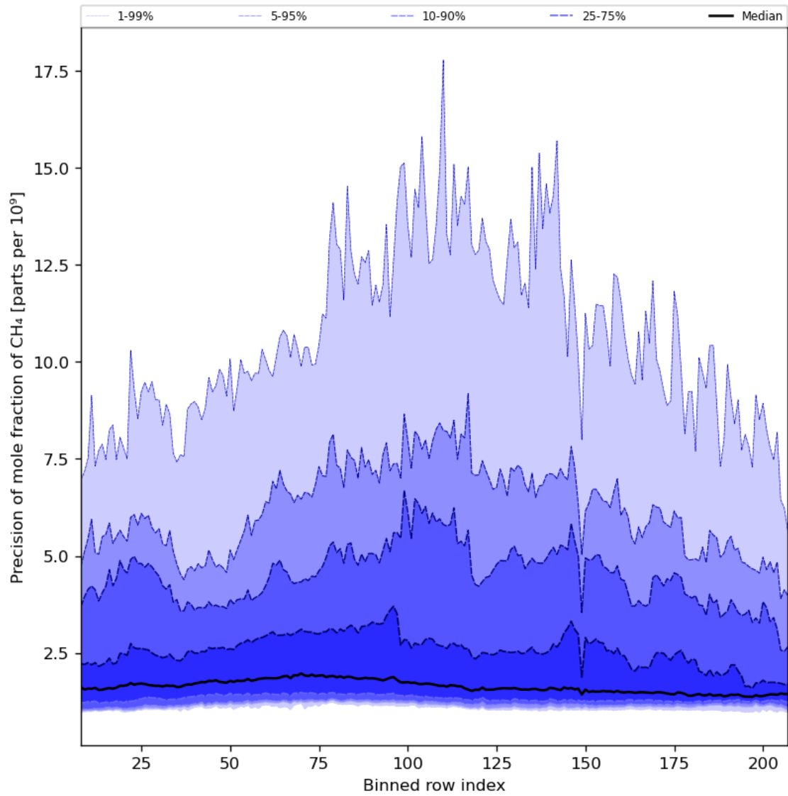
Figure 35: Along track statistics of “Precision of mole fraction of CH 4 ” for 2023-10-06 to 2023-10-07
