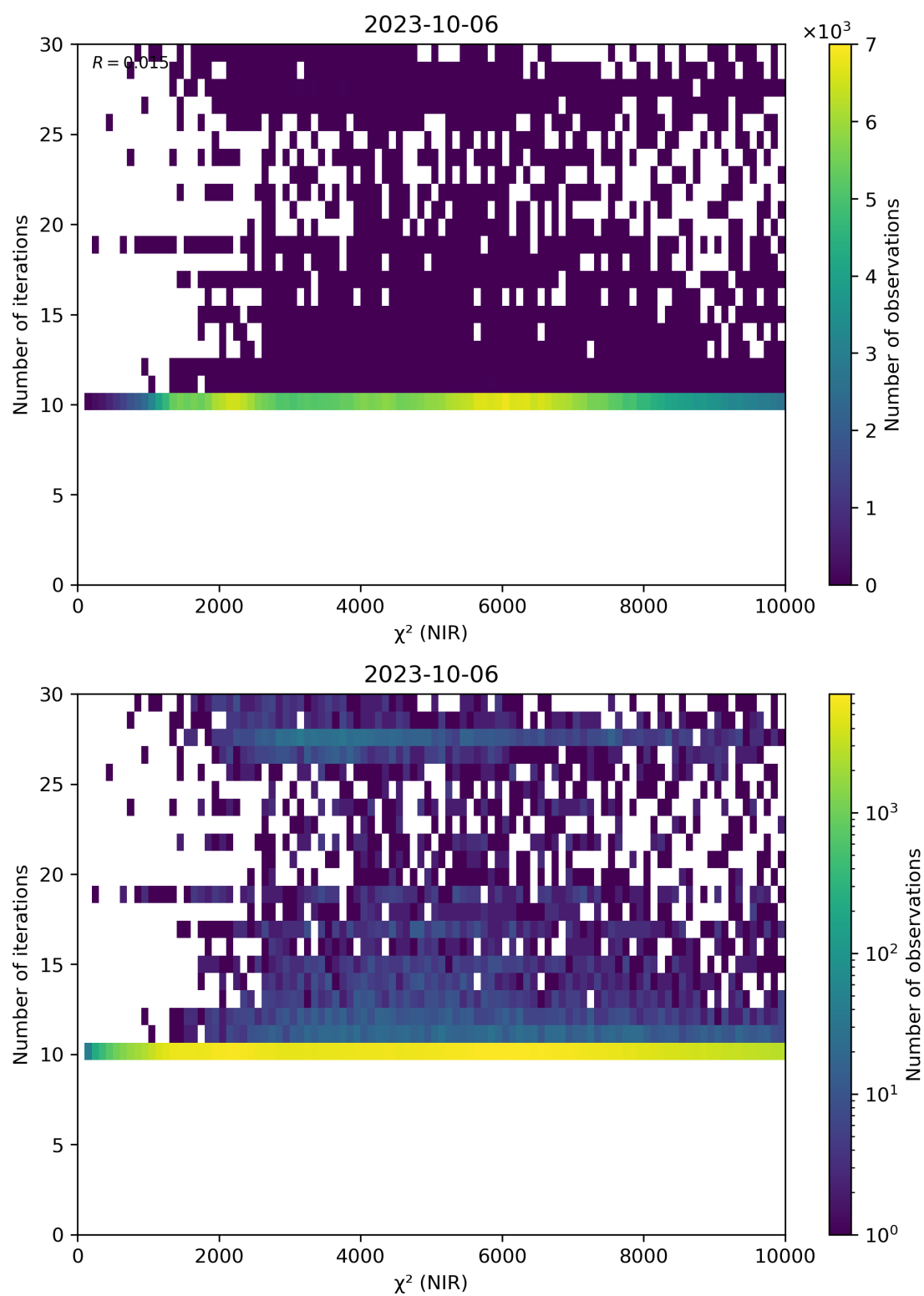
Figure 46: Scatter density plot of “ \chi^2 (NIR)” against “Number of iterations” for 2023-10-06 to 2023-10-07.
