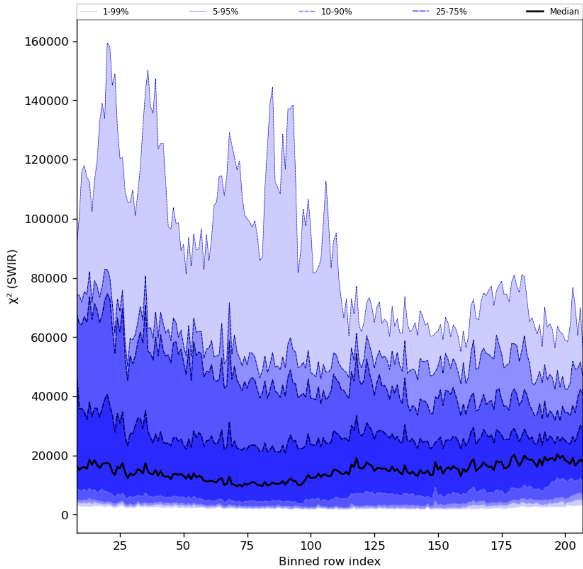
Figure 39: Along track statistics of " \chi^2 (SWIR)" for 2023-10-06 to 2023-10-07
