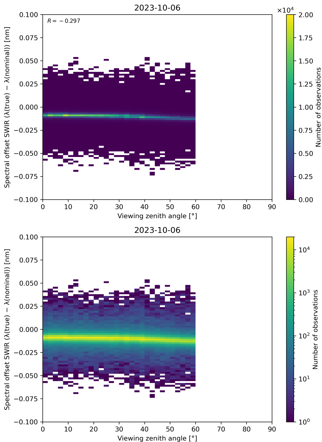
Figure 116: Scatter density plot of “Viewing zenith angle” against “Spectral offset SWIR ( \lambda(\text{true}) - \lambda(\text{nominal}) )” for 2023-10-06 to 2023-10-07.
