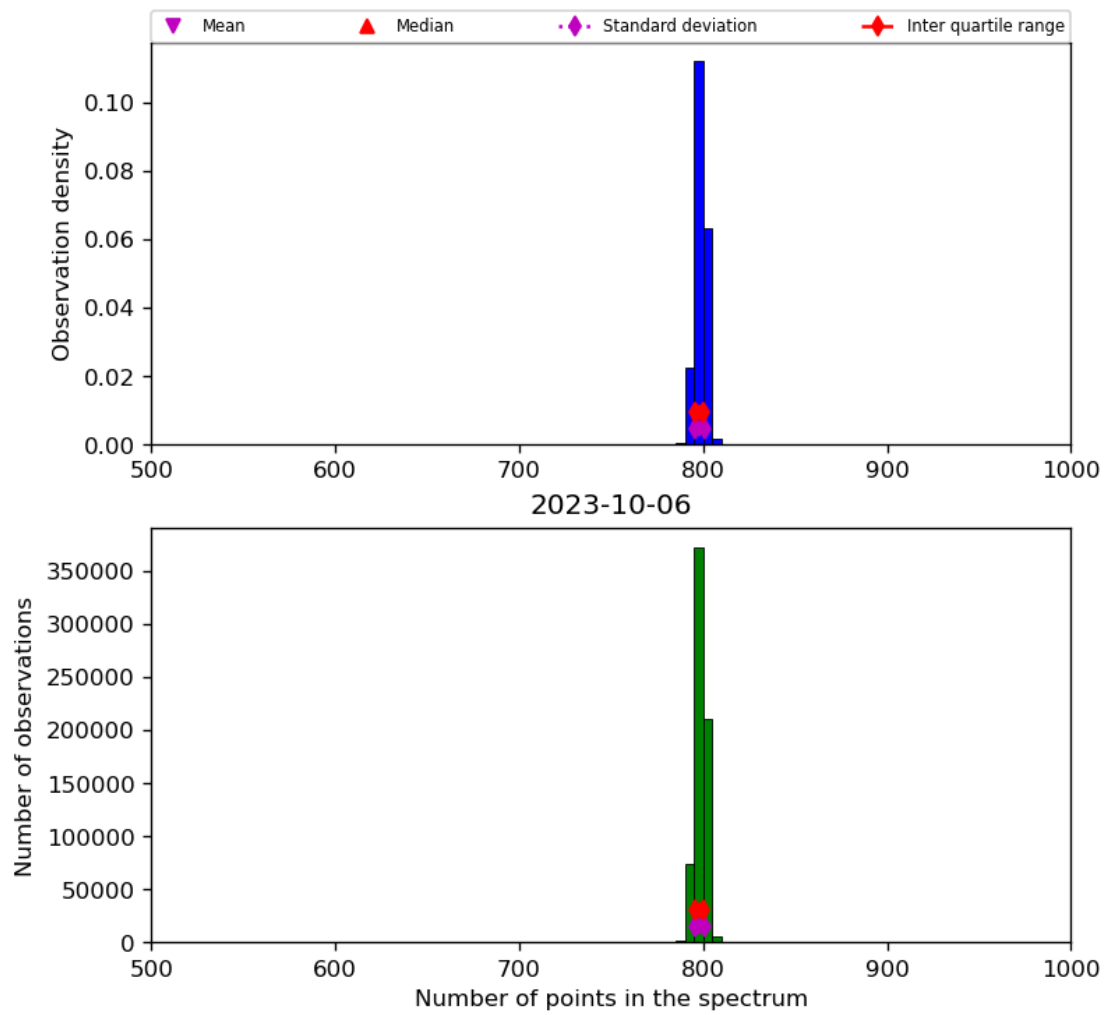
Figure 26: Histogram of “Number of points in the spectrum” for 2023-10-06 to 2023-10-07
