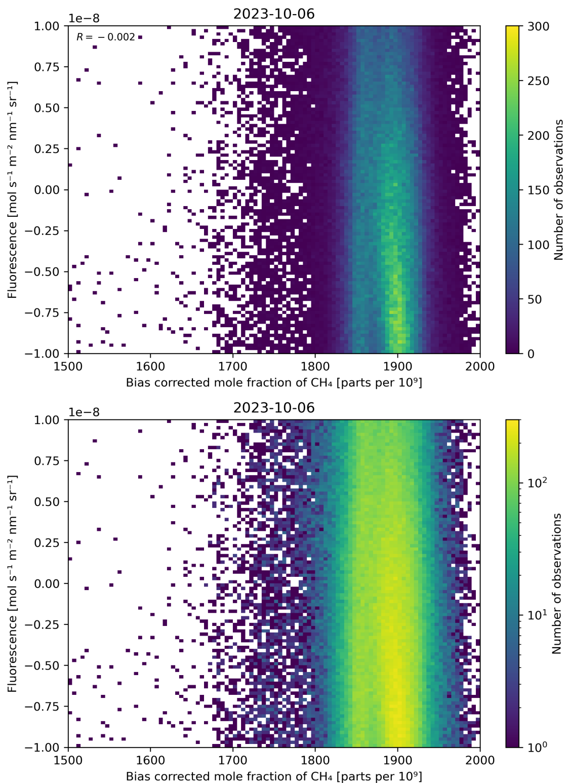
Figure 66: Scatter density plot of “Bias corrected mole fraction of \text{CH}_4 ” against “Fluorescence” for 2023-10-06 to 2023-10-07.
