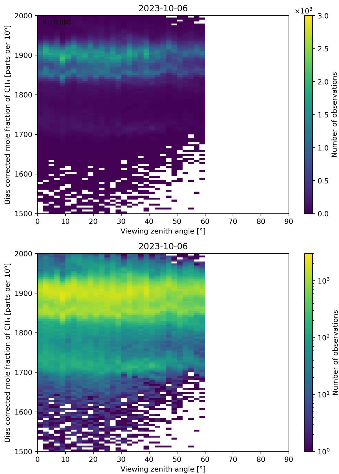
Figure 111: Scatter density plot of “Viewing zenith angle” against “Bias corrected mole fraction of CH 4 ” for 2023-10-06 to 2023-10-07.
