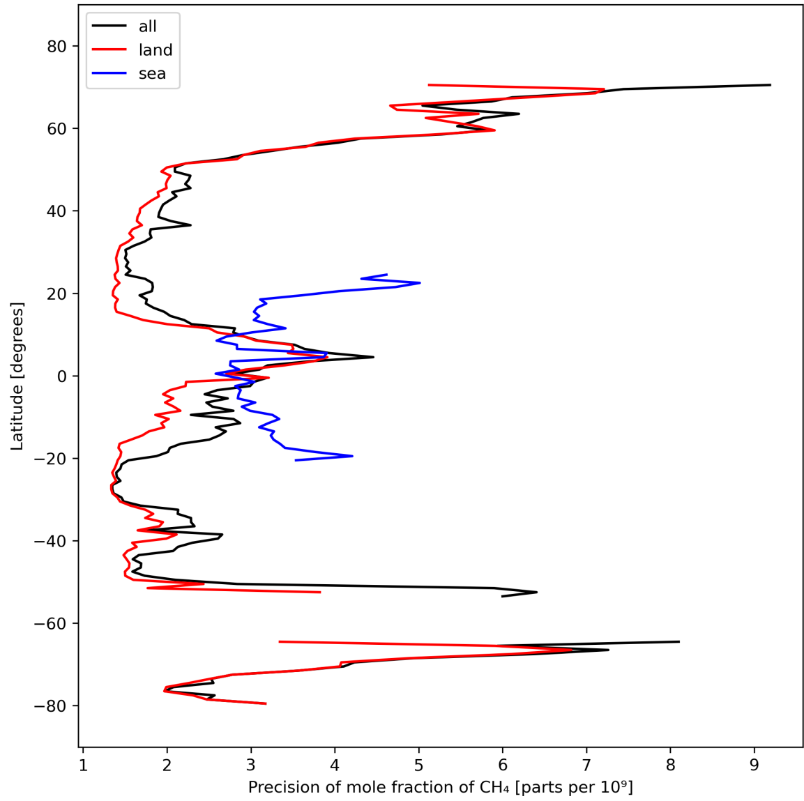
Figure 13: Zonal average of “Precision of mole fraction of CH 4 ” for 2023-10-06 to 2023-10-07.
