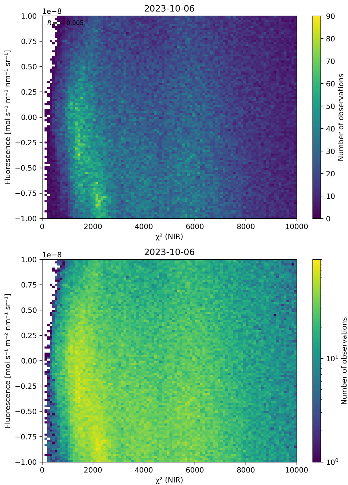
Figure 45: Scatter density plot of “ \chi^2 (NIR)” against “Fluorescence” for 2023-10-06 to 2023-10-07.
