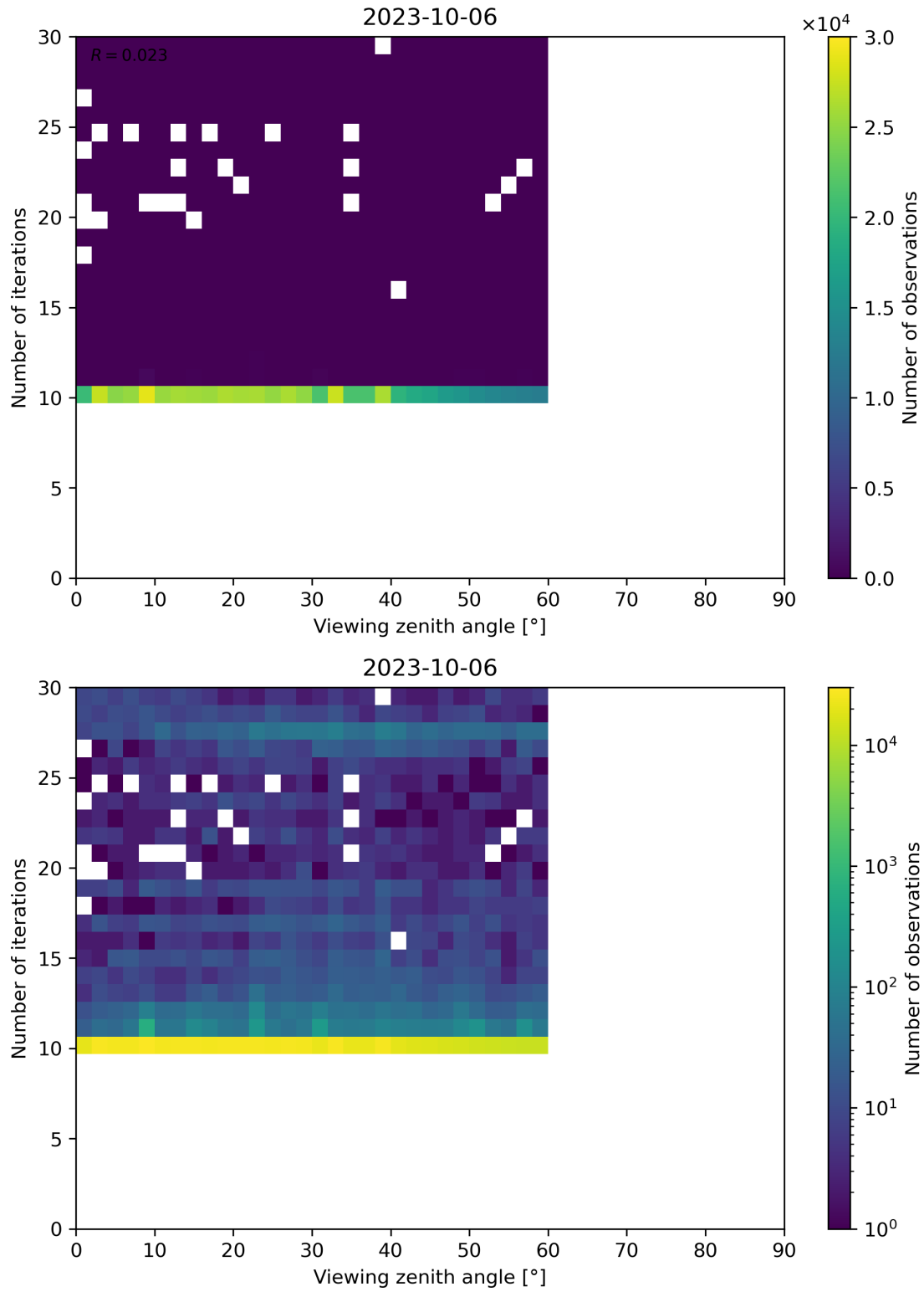
Figure 113: Scatter density plot of “Viewing zenith angle” against “Number of iterations” for 2023-10-06 to 2023-10-07.
