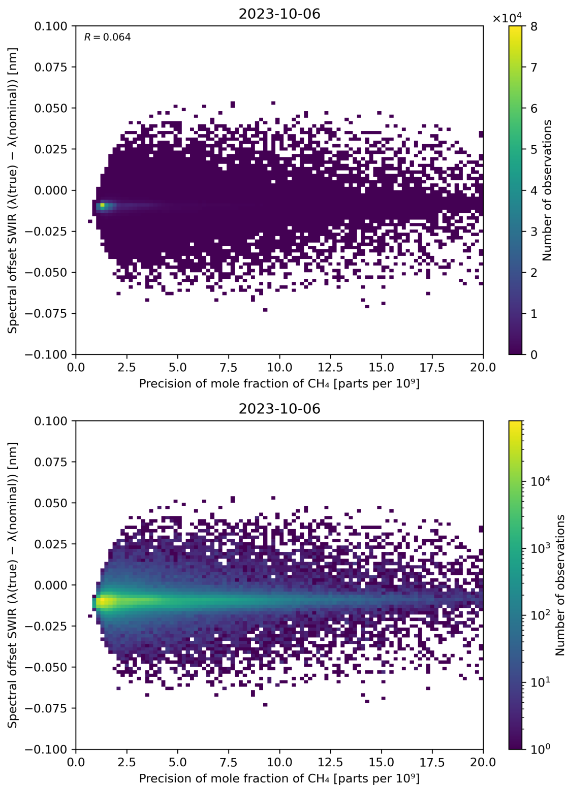
Figure 85: Scatter density plot of “Precision of mole fraction of \text{CH}_4 ” against “Spectral offset SWIR ( \lambda(\text{true}) - \lambda(\text{nominal}) )” for 2023-10-06 to 2023-10-07.
