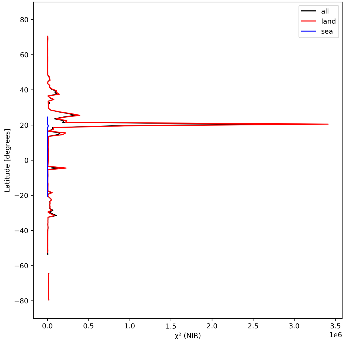
Figure 18: Zonal average of “ \chi^2 (NIR)” for 2023-10-06 to 2023-10-07.
