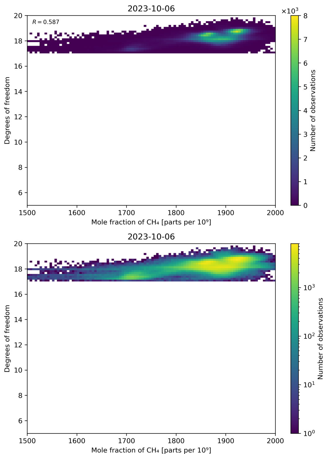
Figure 72: Scatter density plot of “Mole fraction of CH 4 ” against “Degrees of freedom” for 2023-10-06 to 2023-10-07.
