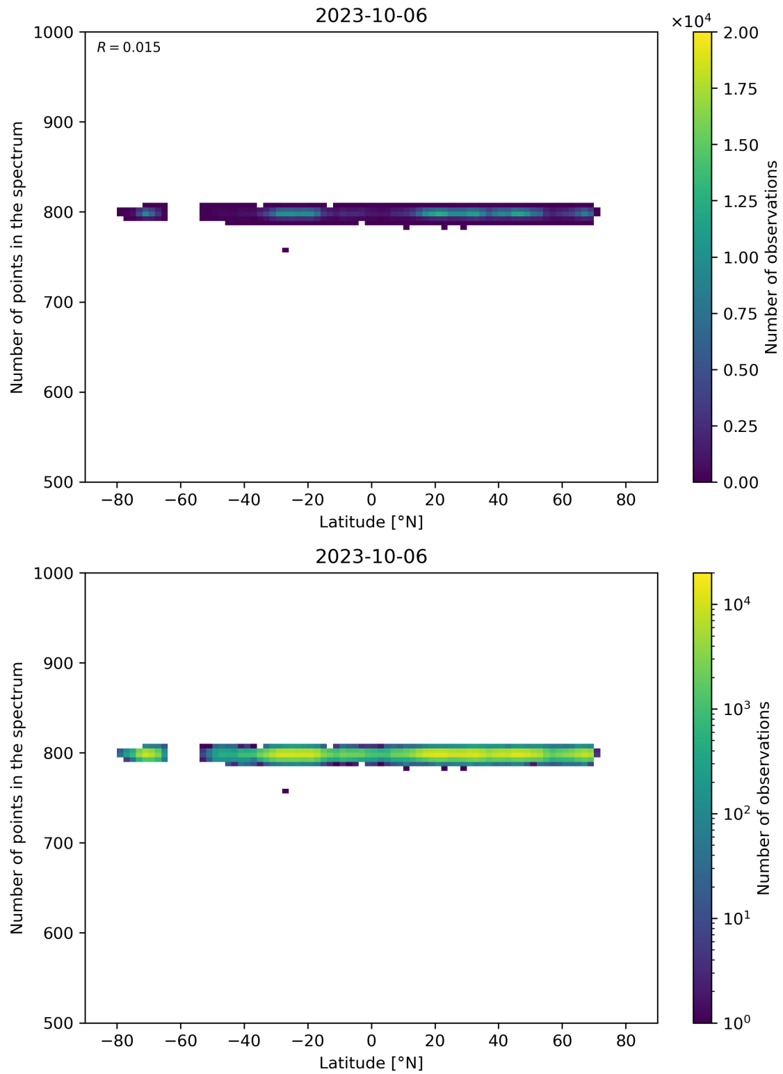
Figure 61: Scatter density plot of “Latitude” against “Number of points in the spectrum” for 2023-10-06 to 2023-10-07.
