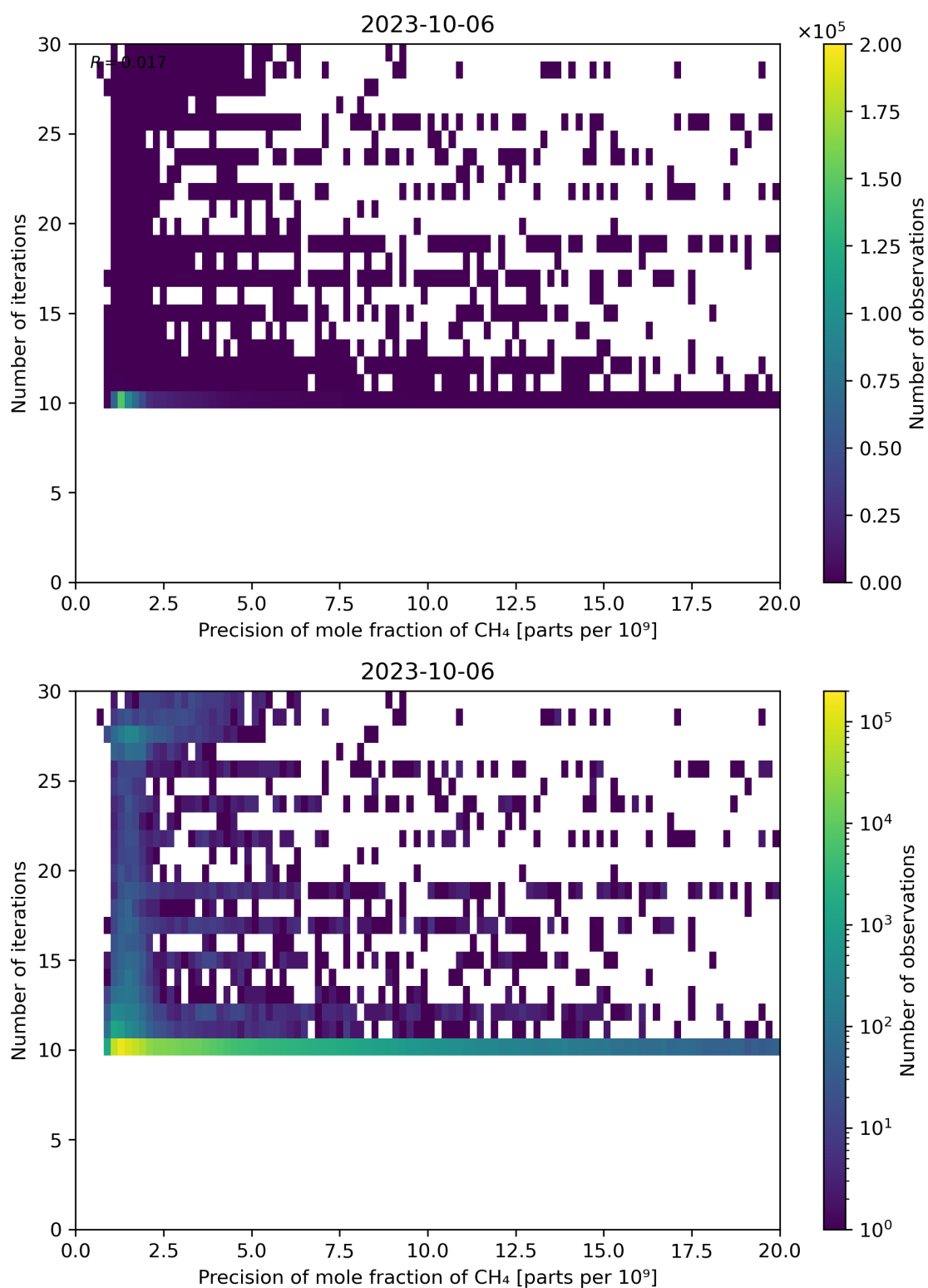
Figure 83: Scatter density plot of “Precision of mole fraction of CH 4 ” against “Number of iterations” for 2023-10-06 to 2023-10-07.
