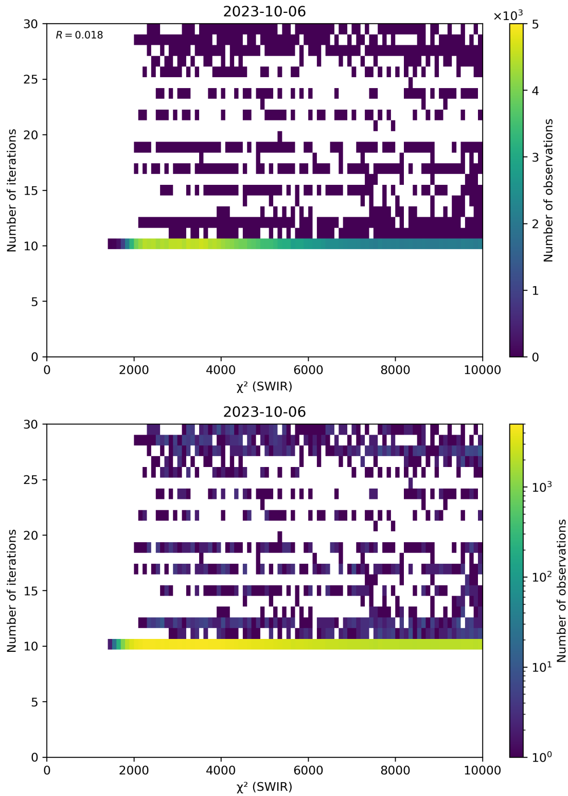
Figure 50: Scatter density plot of “ \chi^2 (SWIR)” against “Number of iterations” for 2023-10-06 to 2023-10-07.
