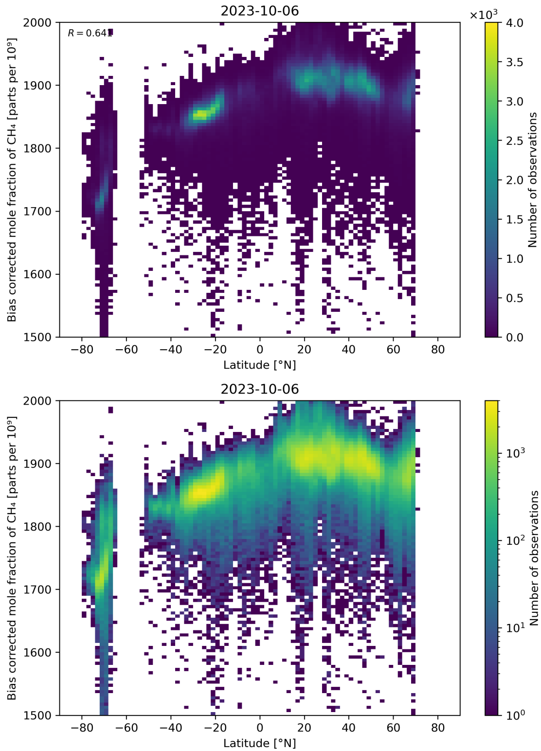
Figure 58: Scatter density plot of “Latitude” against “Bias corrected mole fraction of CH 4 ” for 2023-10-06 to 2023-10-07.
