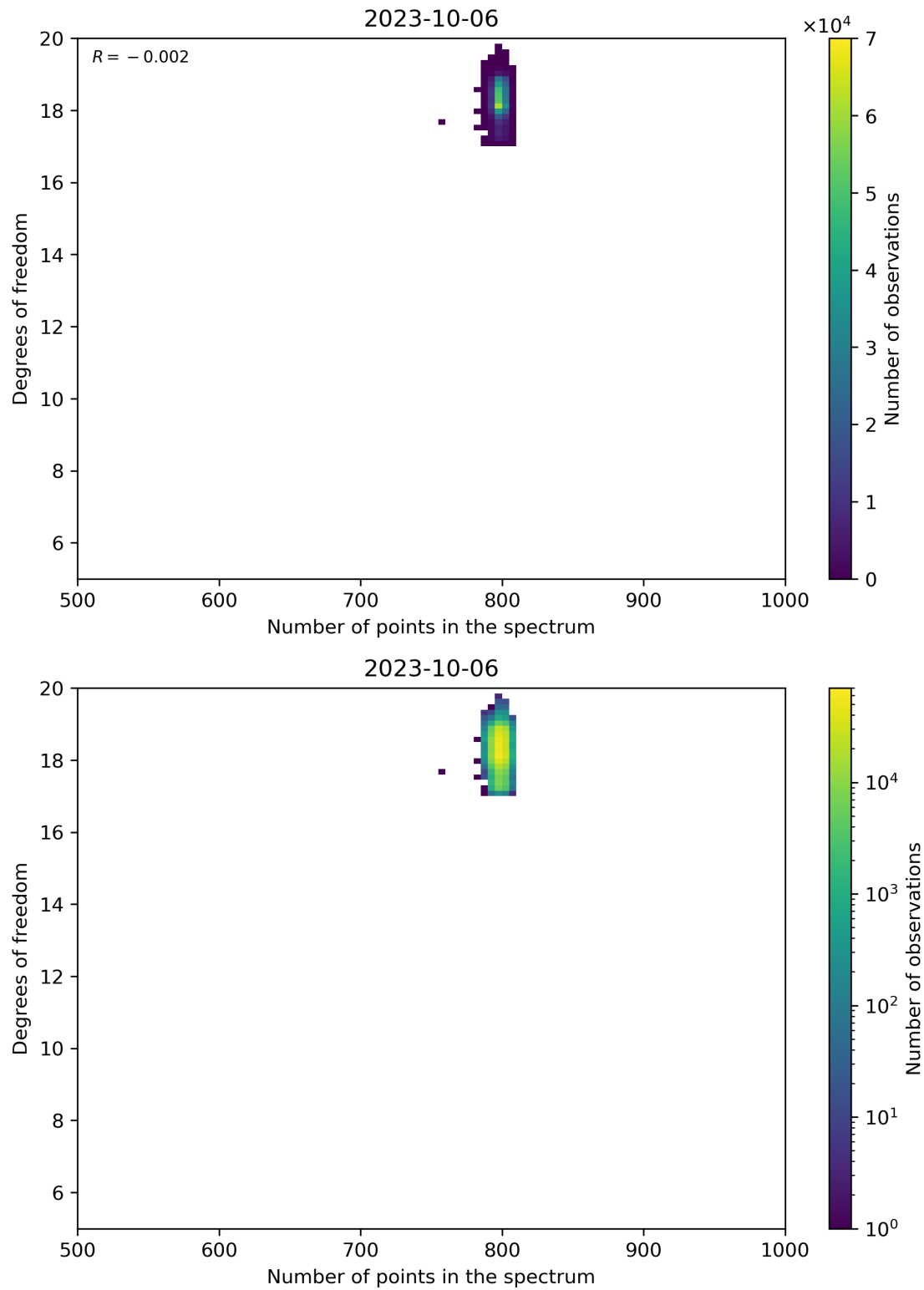
Figure 90: Scatter density plot of “Number of points in the spectrum” against “Degrees of freedom” for 2023-10-06 to 2023-10-07.
