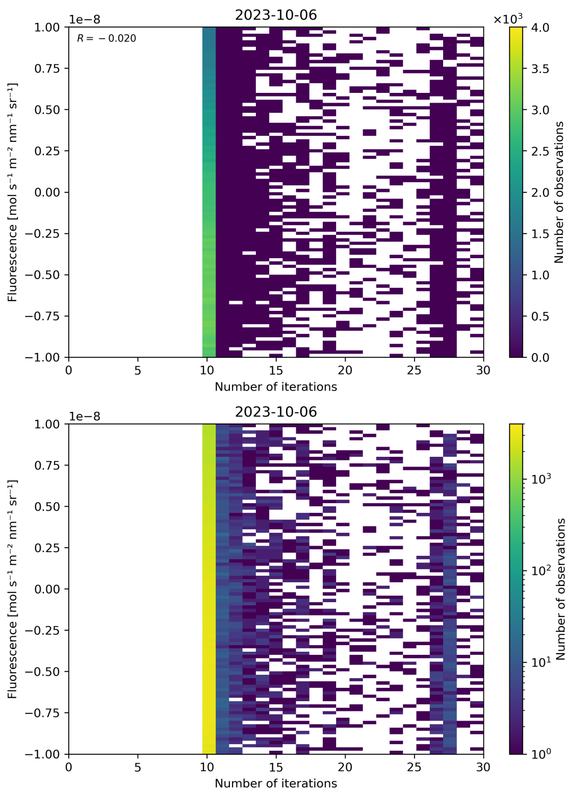
Figure 87: Scatter density plot of “Number of iterations” against “Fluorescence” for 2023-10-06 to 2023-10-07.
