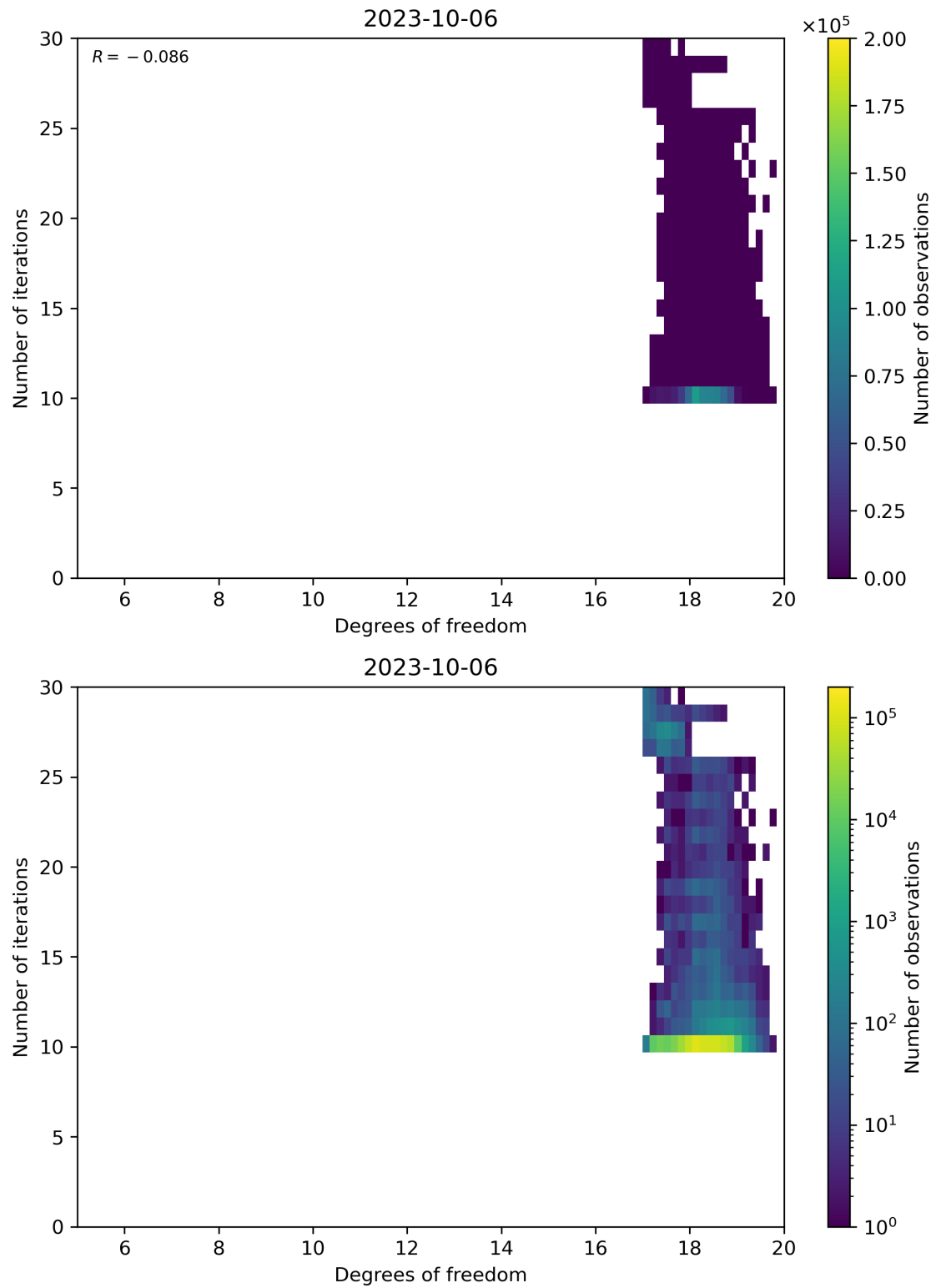
Figure 52: Scatter density plot of “Degrees of freedom” against “Number of iterations” for 2023-10-06 to 2023-10-07.
