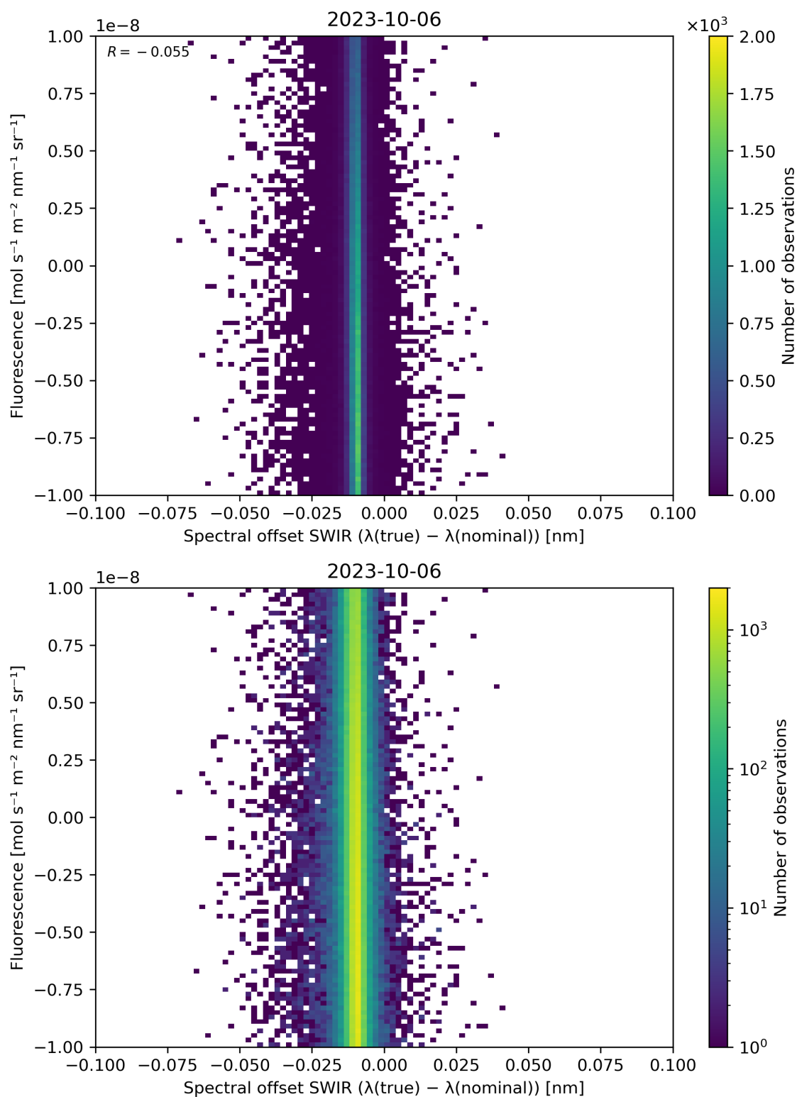
Figure 120: Scatter density plot of “Spectral offset SWIR ( \lambda(\text{true}) - \lambda(\text{nominal}) )” against “Fluorescence” for 2023-10-06 to 2023-10-07.
