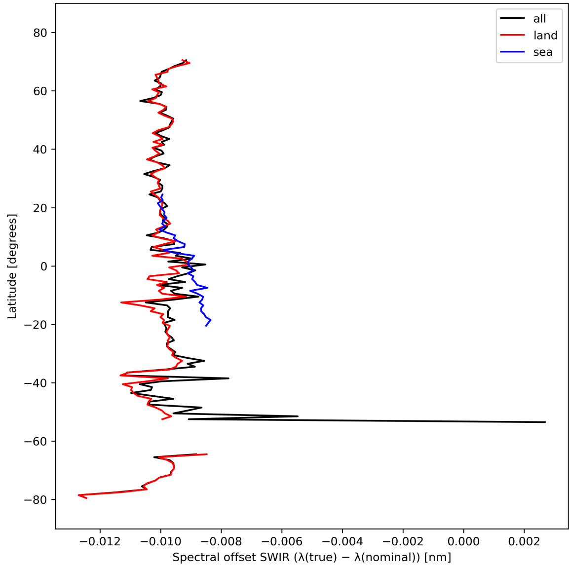
Figure 16: Zonal average of “Spectral offset SWIR ( \lambda(\text{true}) - \lambda(\text{nominal}) )” for 2023-10-06 to 2023-10-07.
