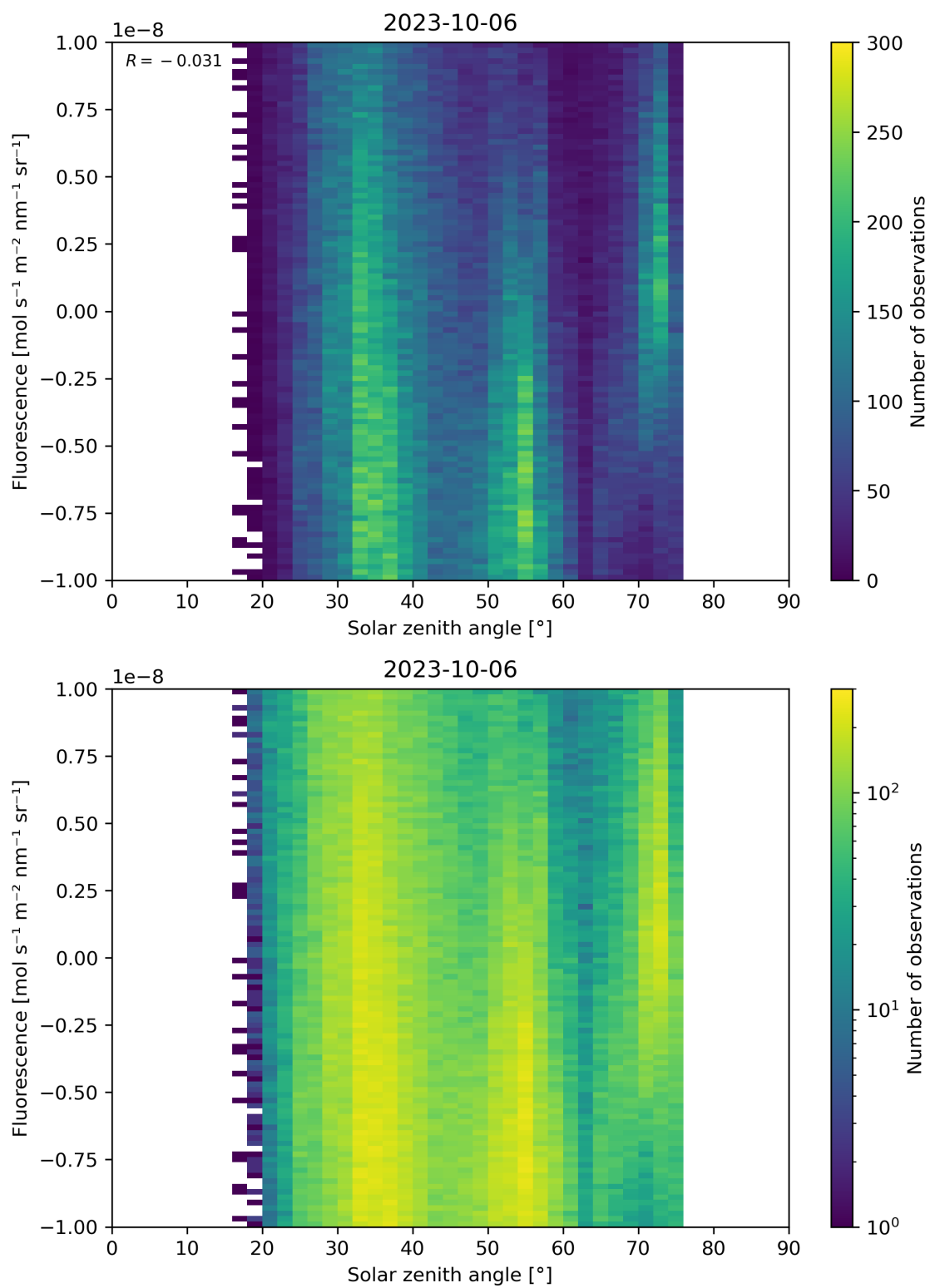
Figure 97: Scatter density plot of “Solar zenith angle” against “Fluorescence” for 2023-10-06 to 2023-10-07.
