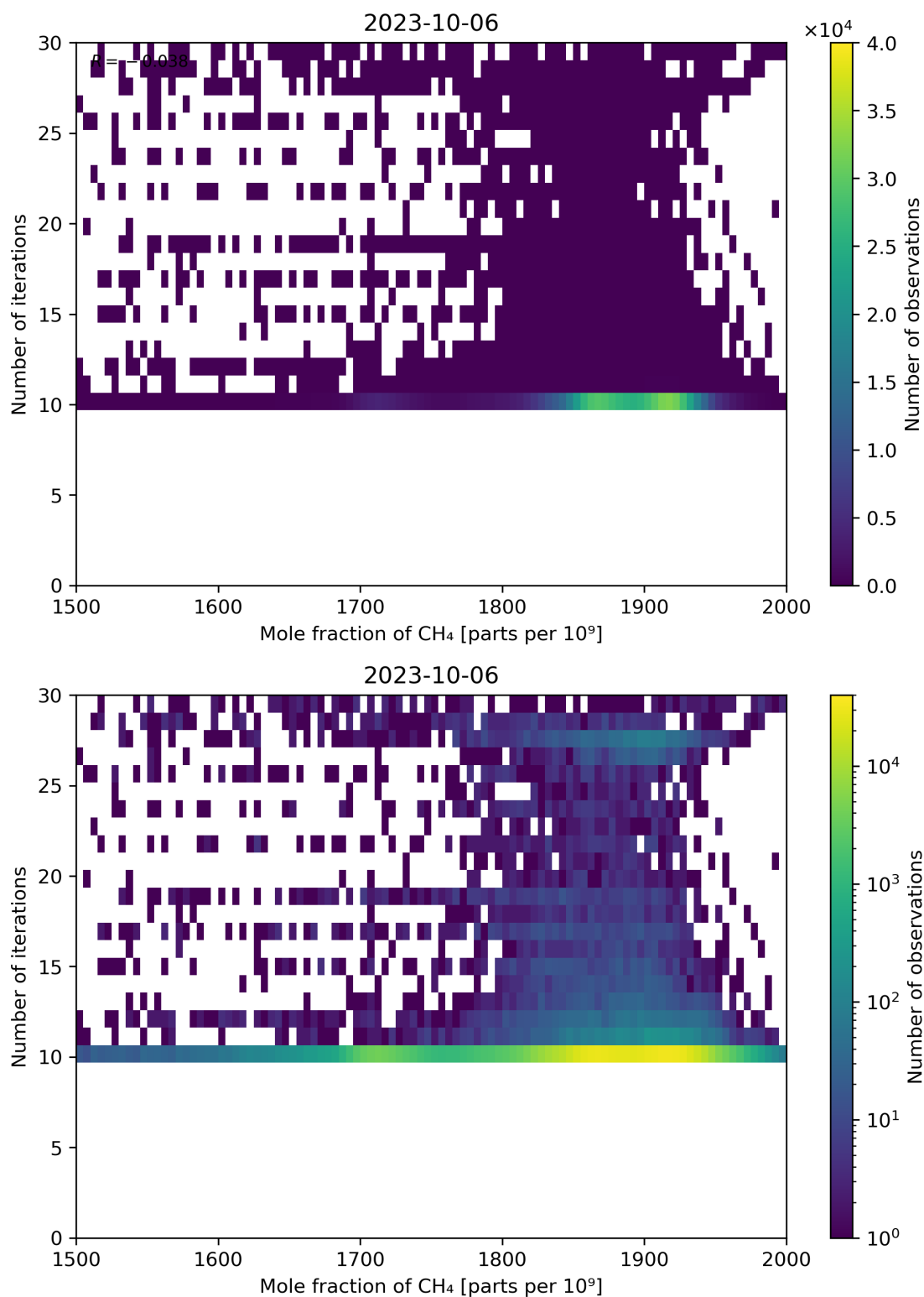
Figure 76: Scatter density plot of “Mole fraction of CH 4 ” against “Number of iterations” for 2023-10-06 to 2023-10-07.
