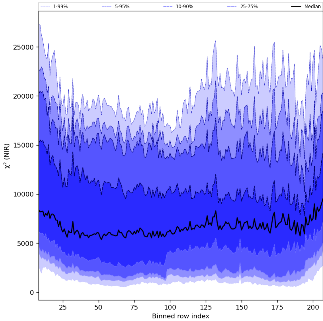
Figure 40: Along track statistics of “ \chi^2 (NIR)” for 2023-10-06 to 2023-10-07
