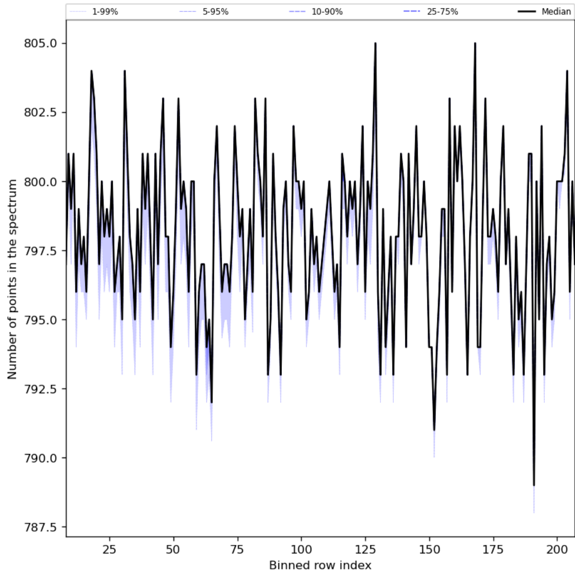
Figure 37: Along track statistics of “Number of points in the spectrum” for 2023-10-06 to 2023-10-07
