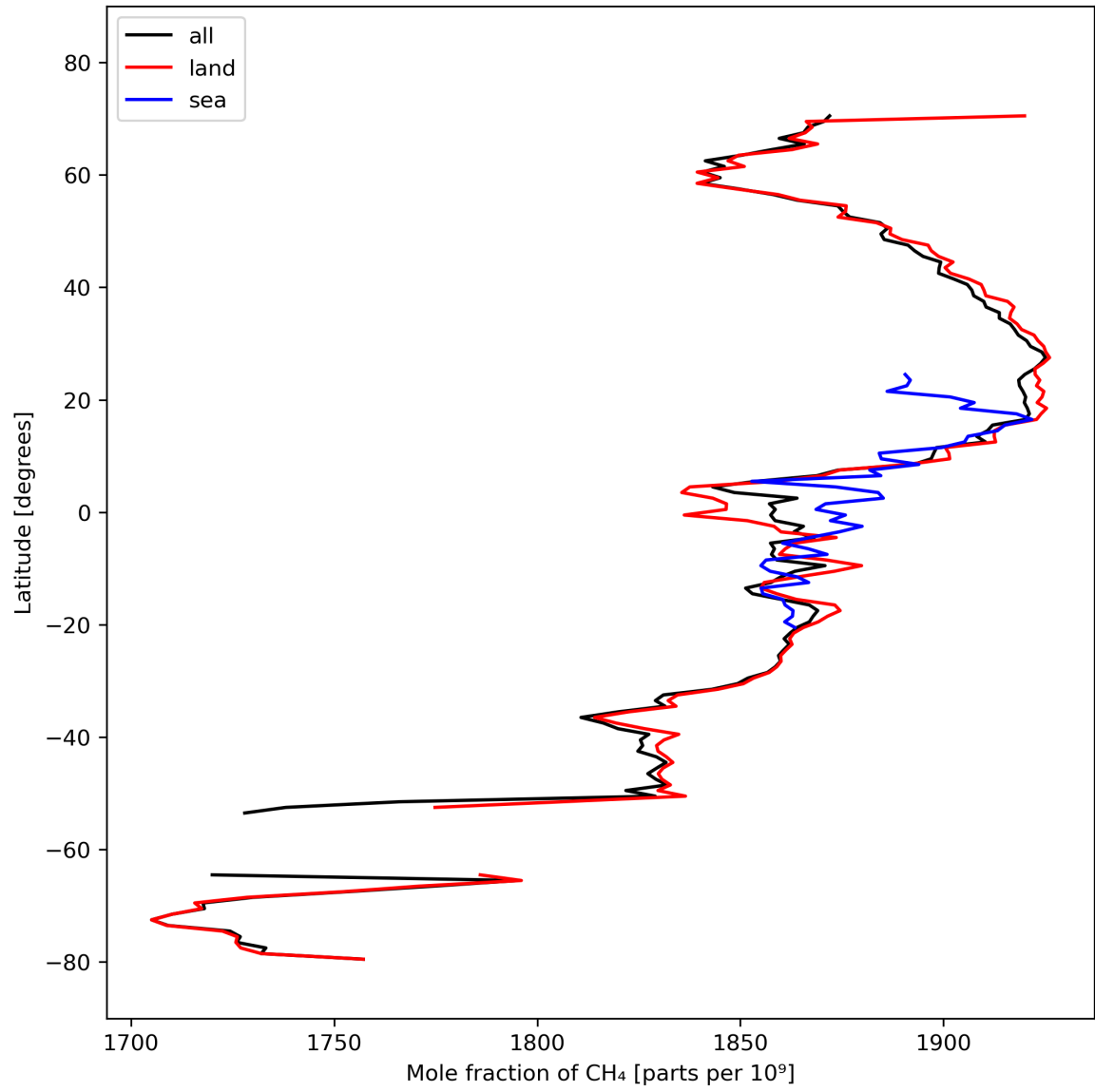
Figure 12: Zonal average of “Mole fraction of \text{CH}_4 ” for 2023-10-06 to 2023-10-07.
