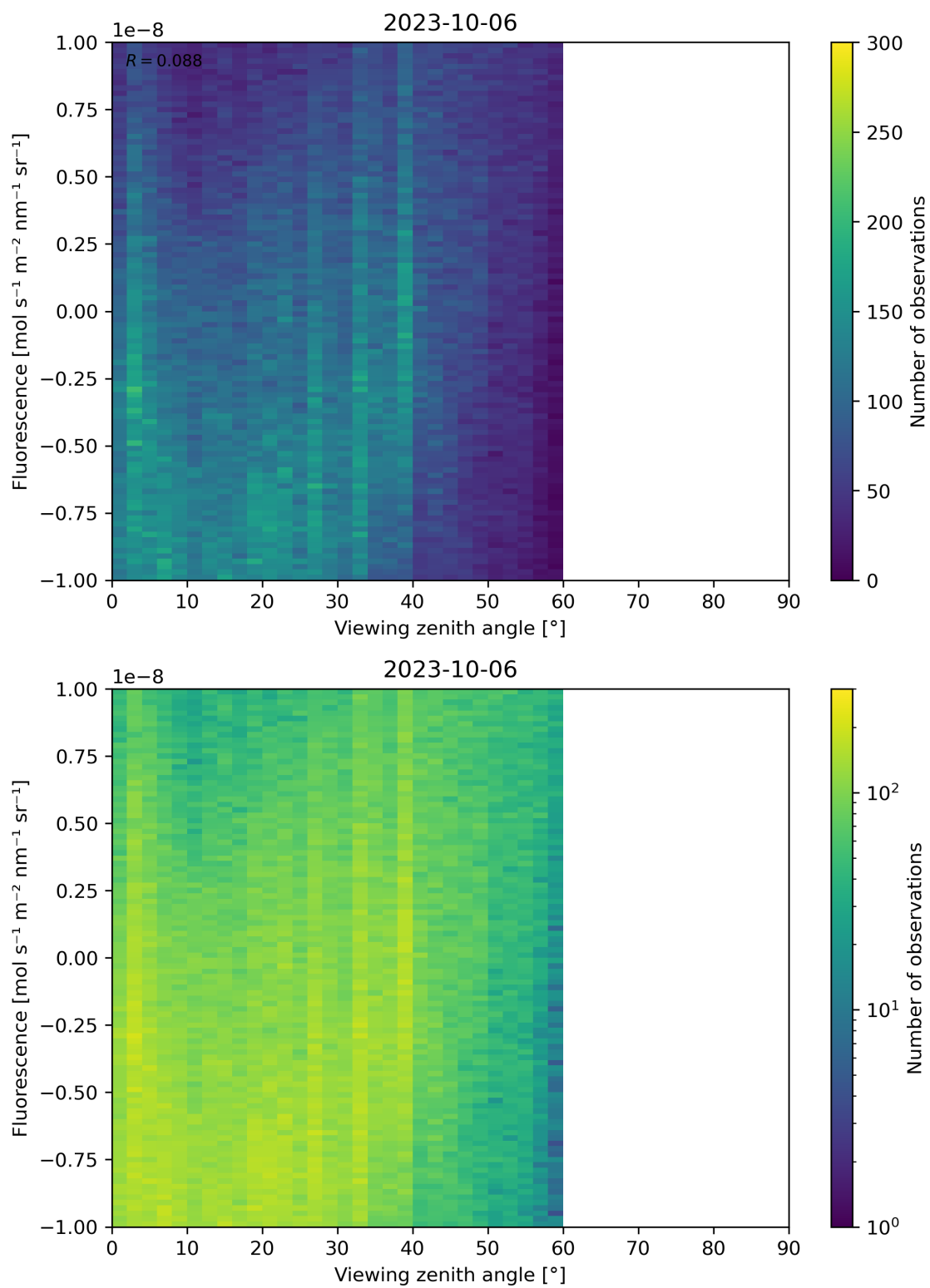
Figure 108: Scatter density plot of “Viewing zenith angle” against “Fluorescence” for 2023-10-06 to 2023-10-07.
