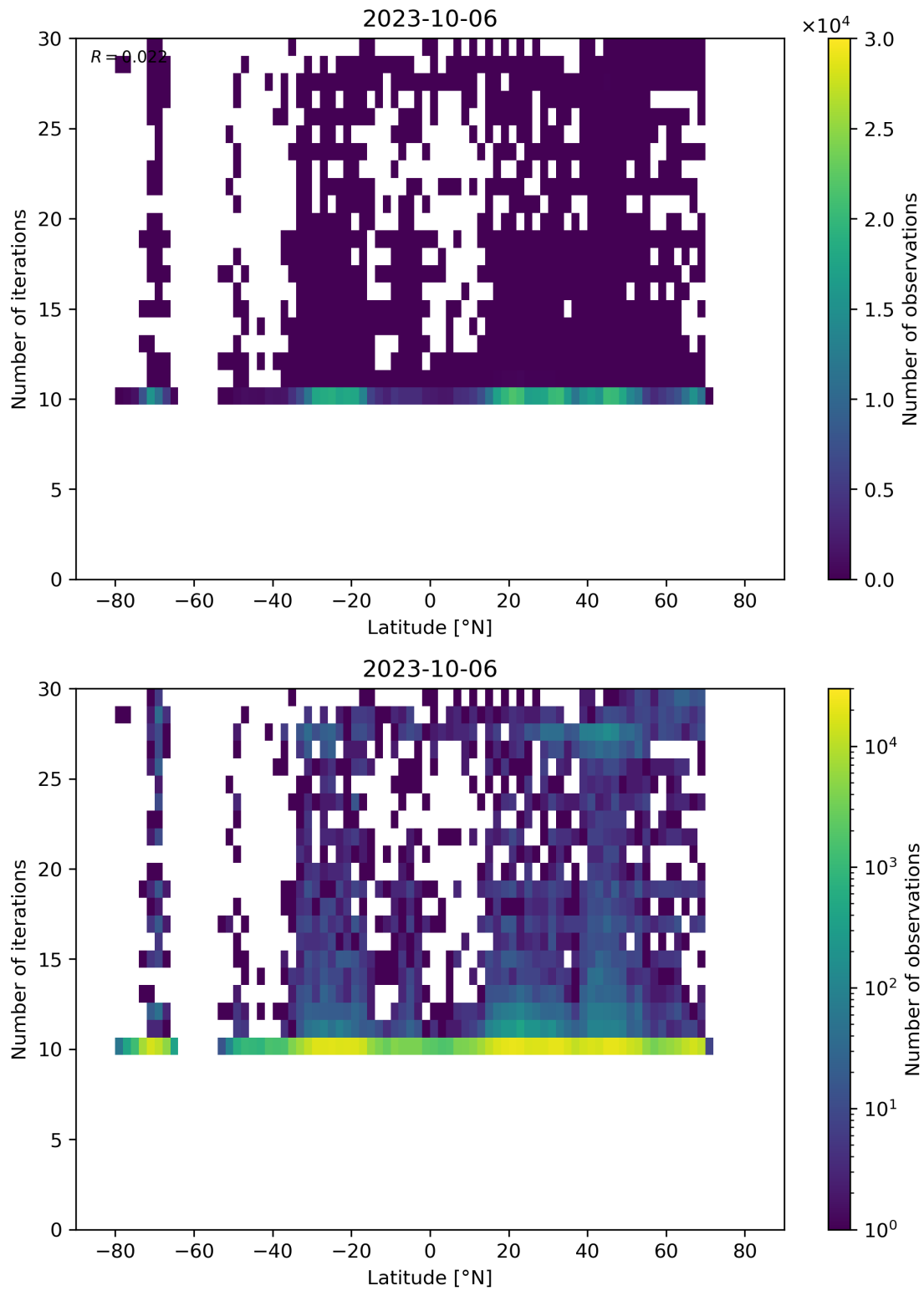
Figure 60: Scatter density plot of “Latitude” against “Number of iterations” for 2023-10-06 to 2023-10-07.
