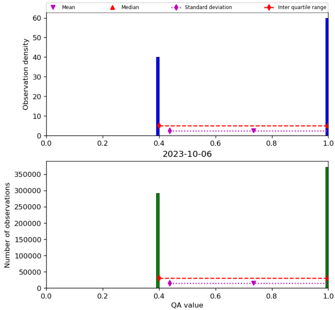
Figure 22: Histogram of “QA value” for 2023-10-06 to 2023-10-07
