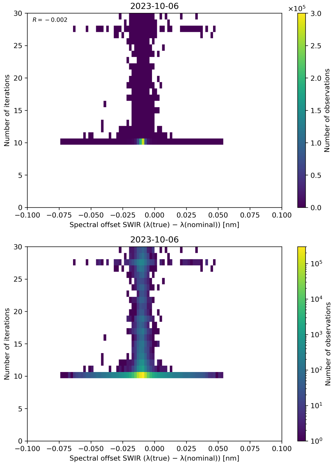
Figure 121: Scatter density plot of “Spectral offset SWIR ( \lambda(\text{true}) - \lambda(\text{nominal}) )” against “Number of iterations” for 2023-10-06 to 2023-10-07.
