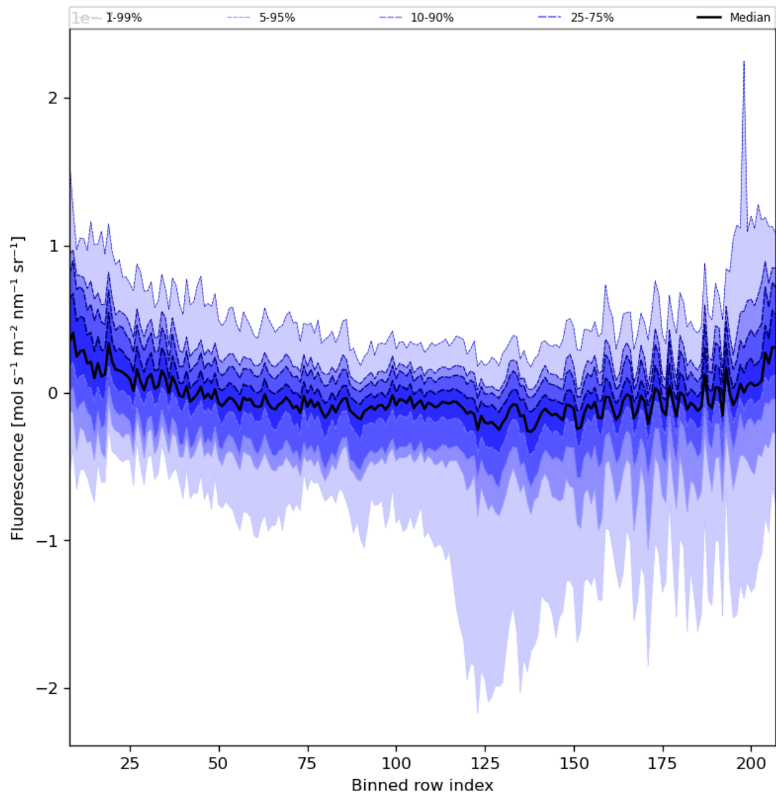
Figure 43: Along track statistics of “Fluorescence” for 2023-10-06 to 2023-10-07
