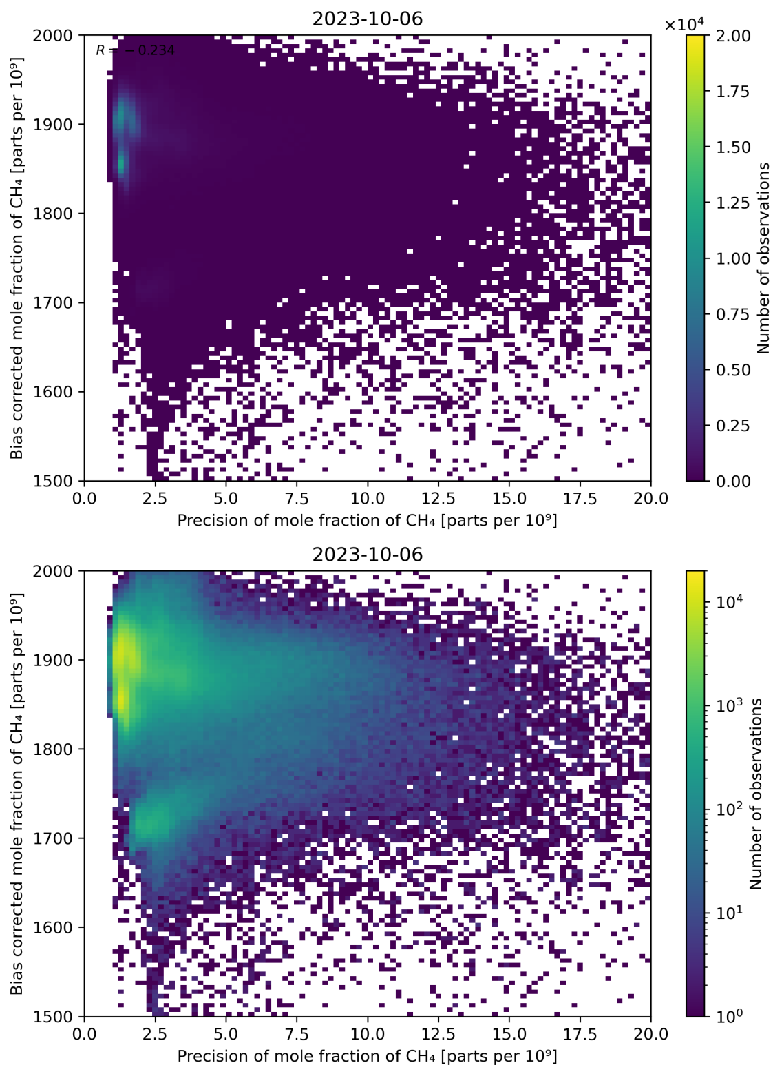
Figure 82: Scatter density plot of “Precision of mole fraction of CH 4 ” against “Bias corrected mole fraction of CH 4 ” for 2023-10-06 to 2023-10-07.
