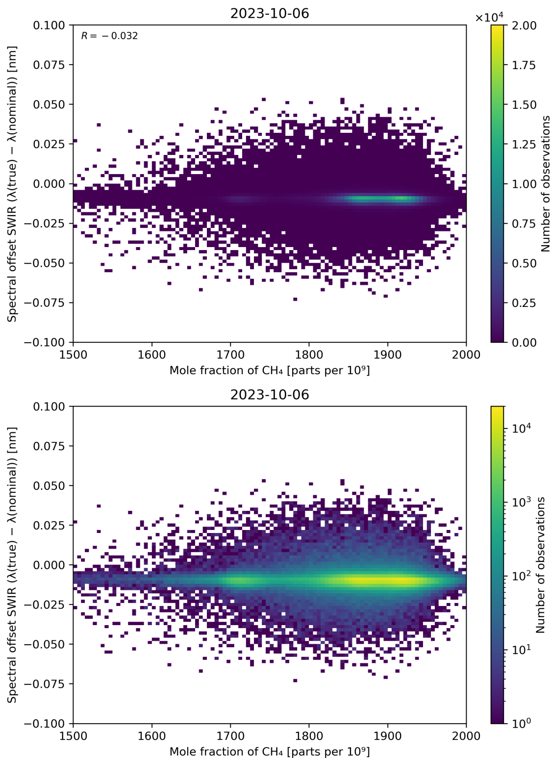
Figure 86: Scatter density plot of “Mole fraction of CH 4 ” against “Spectral offset SWIR ( \lambda(\text{true}) - \lambda(\text{nominal}) )” for 2023-10-06 to 2023-10-07.
