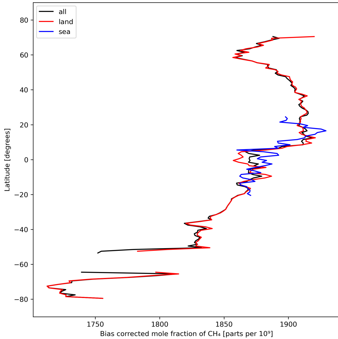
Figure 14: Zonal average of “Bias corrected mole fraction of CH 4 ” for 2023-10-06 to 2023-10-07.
