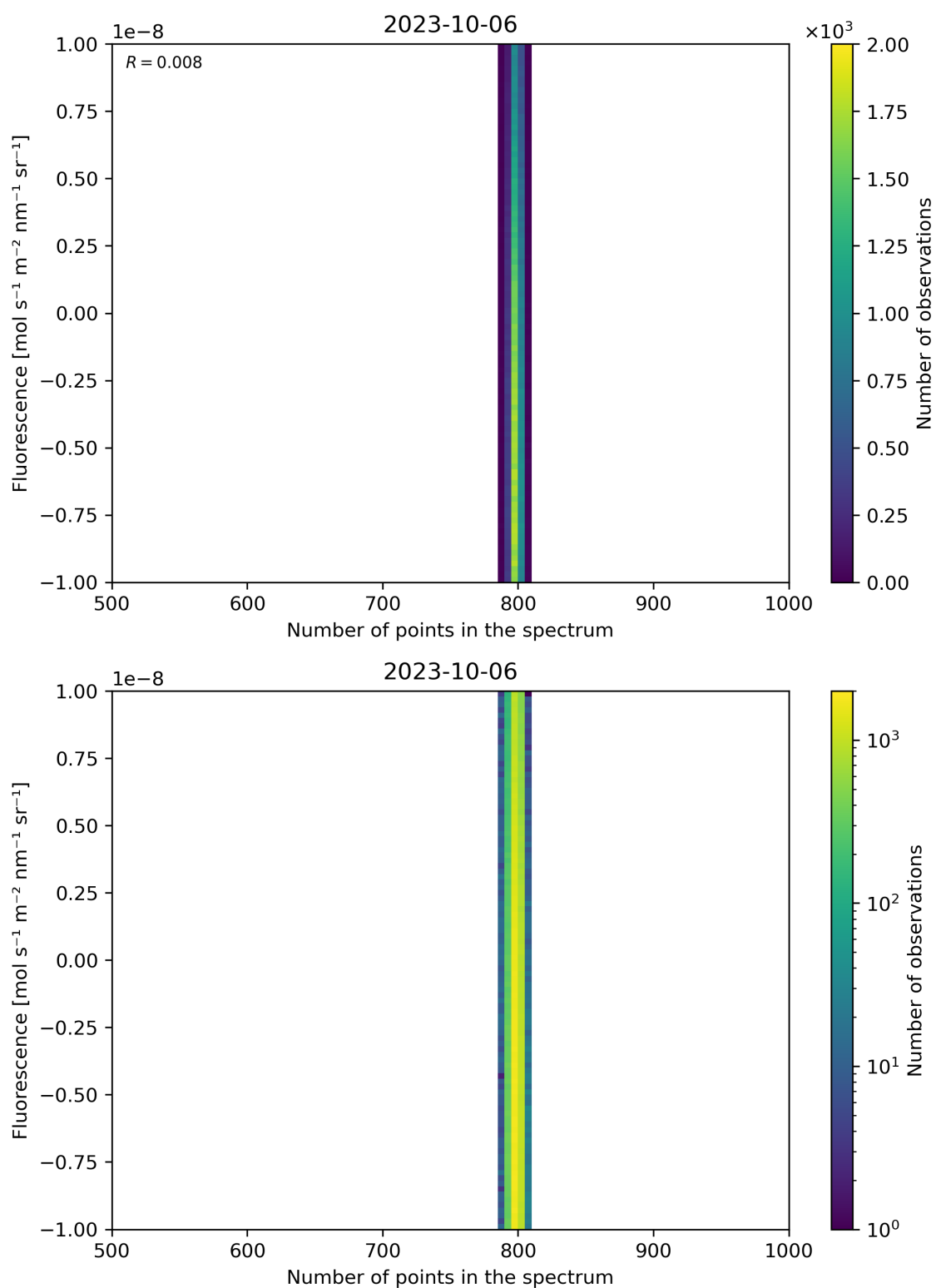
Figure 91: Scatter density plot of “Number of points in the spectrum” against “Fluorescence” for 2023-10-06 to 2023-10-07.
