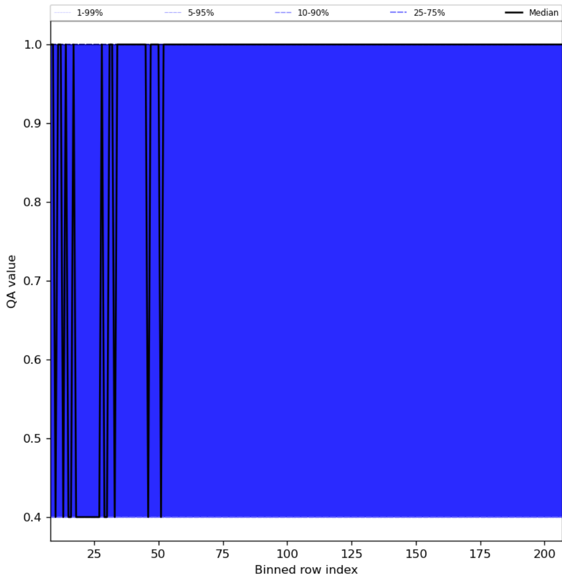
Figure 33: Along track statistics of “QA value” for 2023-10-06 to 2023-10-07
