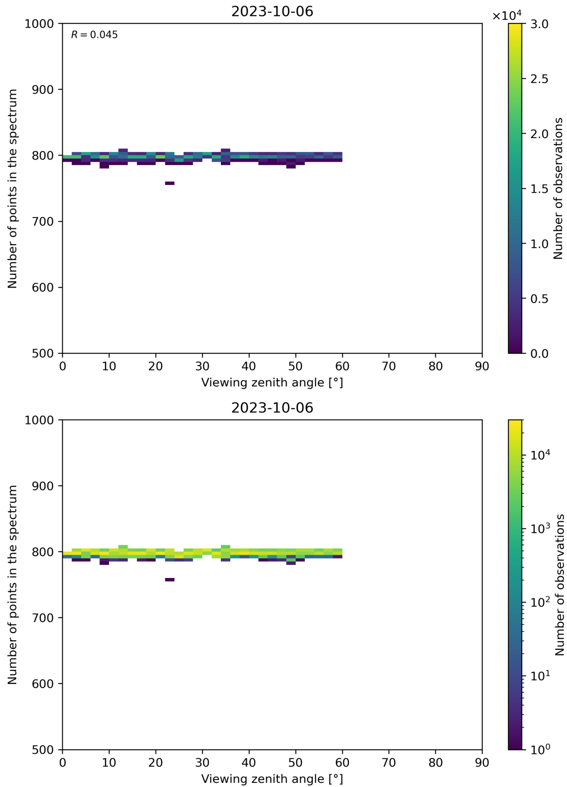
Figure 114: Scatter density plot of “Viewing zenith angle” against “Number of points in the spectrum” for 2023-10-06 to 2023-10-07.
