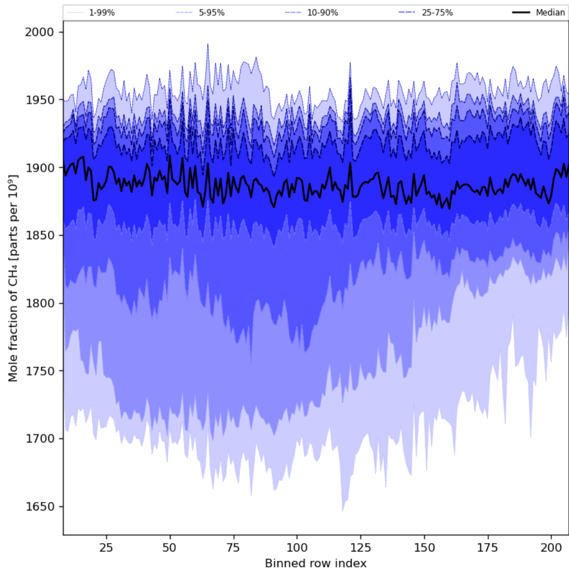
Figure 34: Along track statistics of “Mole fraction of CH 4 ” for 2023-10-06 to 2023-10-07
