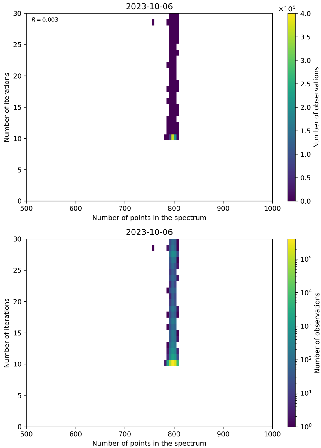
Figure 92: Scatter density plot of “Number of points in the spectrum” against “Number of iterations” for 2023-10-06 to 2023-10-07.
