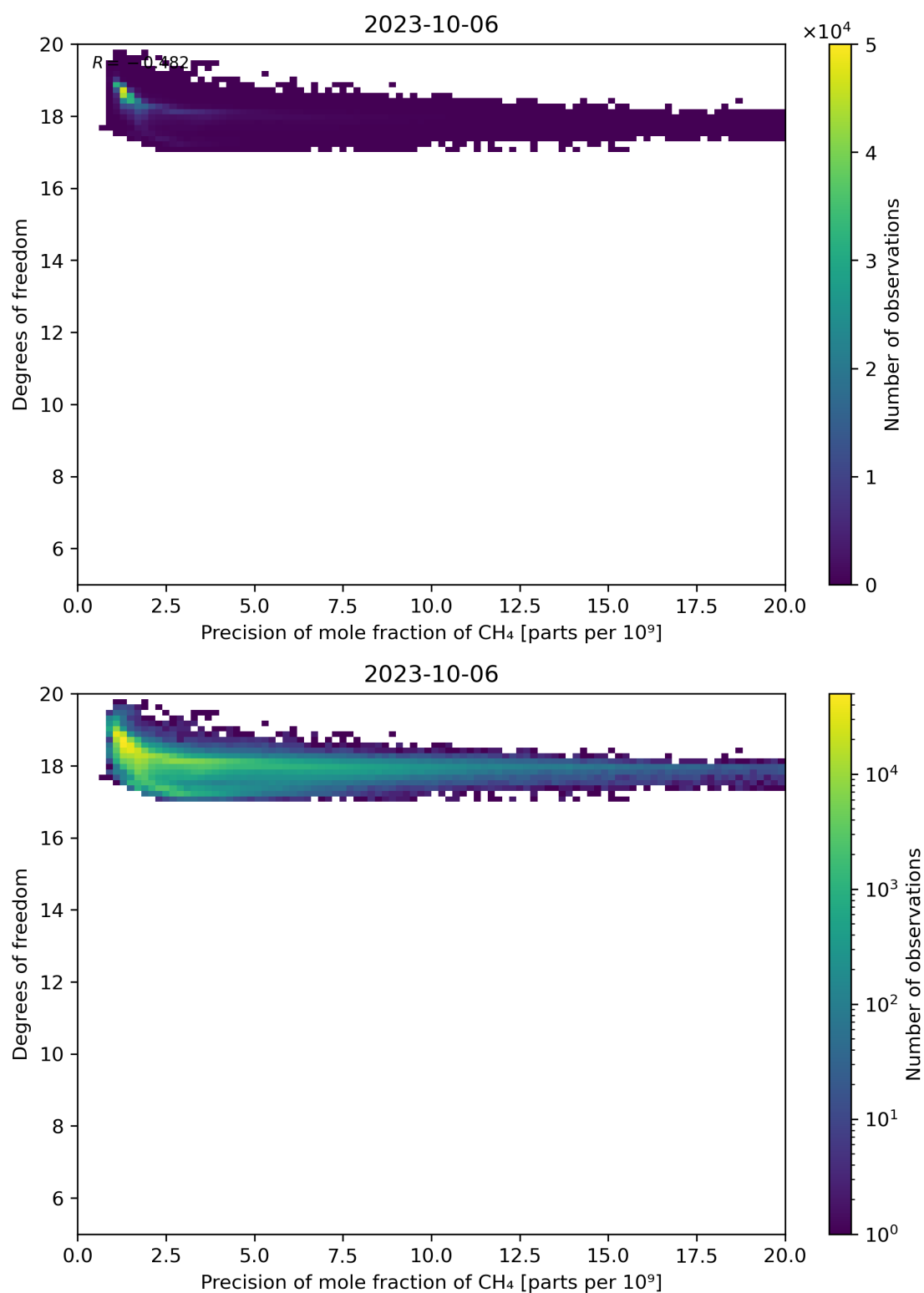
Figure 80: Scatter density plot of “Precision of mole fraction of CH 4 ” against “Degrees of freedom” for 2023-10-06 to 2023-10-07.
