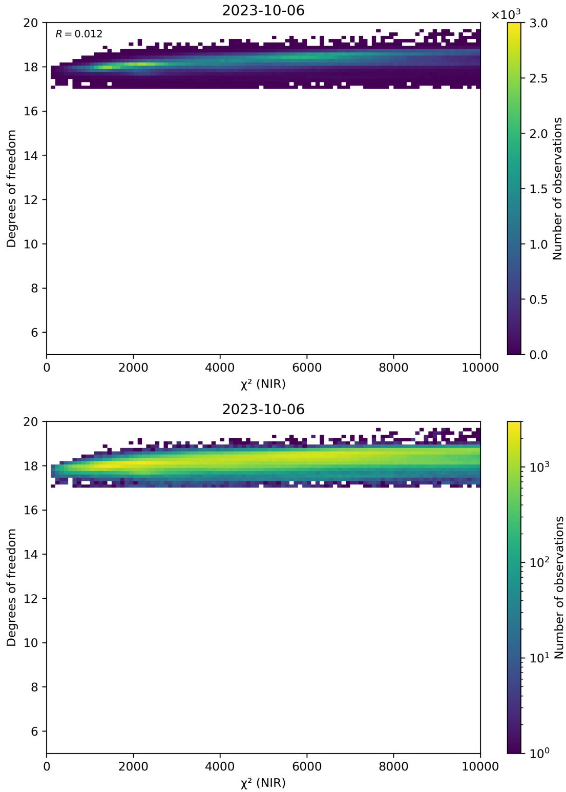
Figure 44: Scatter density plot of “ \chi^2 (NIR)” against “Degrees of freedom” for 2023-10-06 to 2023-10-07.
