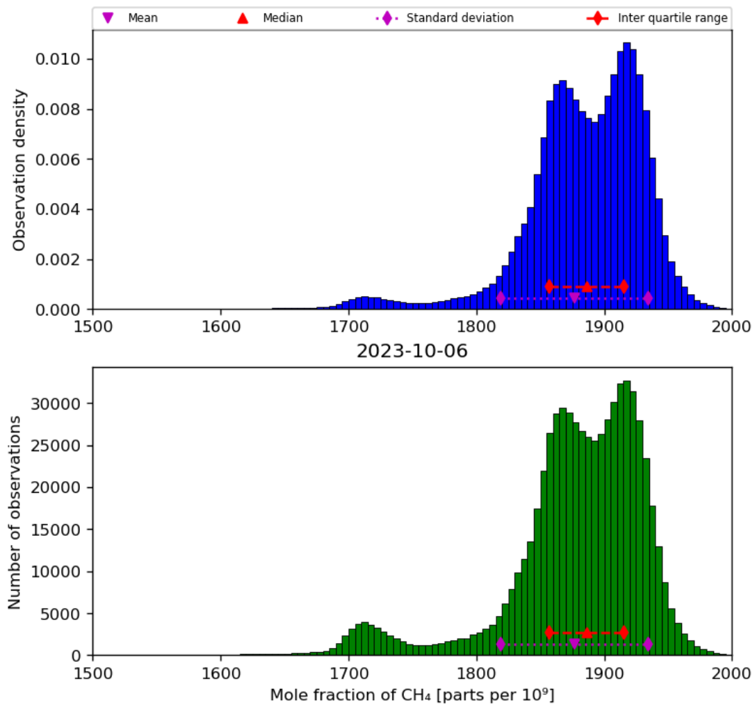
Figure 23: Histogram of “Mole fraction of CH 4 ” for 2023-10-06 to 2023-10-07
