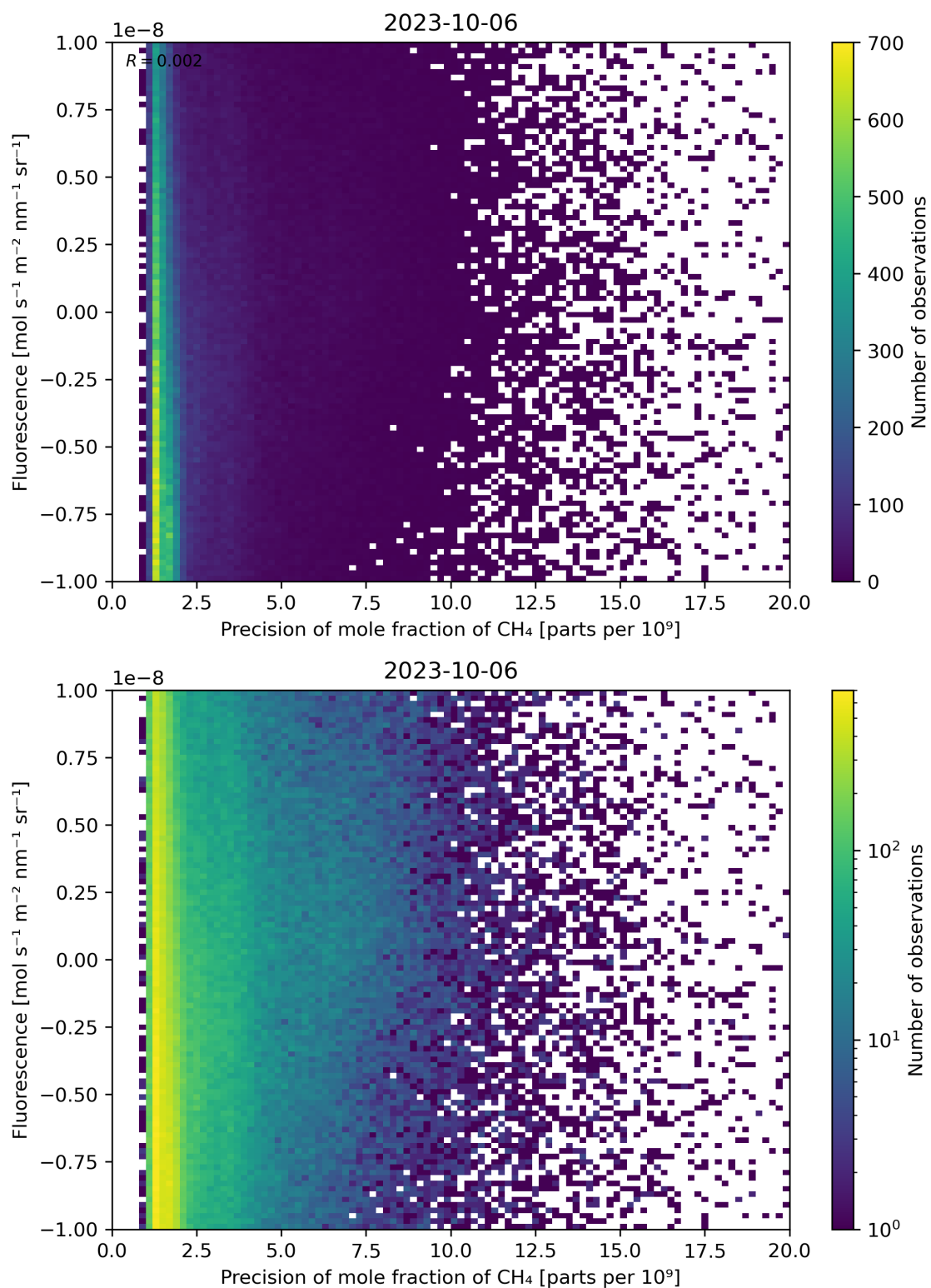
Figure 81: Scatter density plot of “Precision of mole fraction of \text{CH}_4 ” against “Fluorescence” for 2023-10-06 to 2023-10-07.
