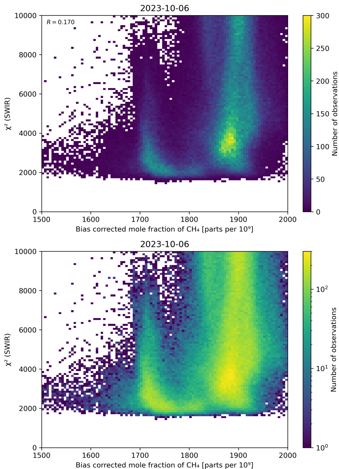
Figure 64: Scatter density plot of “Bias corrected mole fraction of CH 4 ” against “ \chi^2 (SWIR)” for 2023-10-06 to 2023-10-07.
