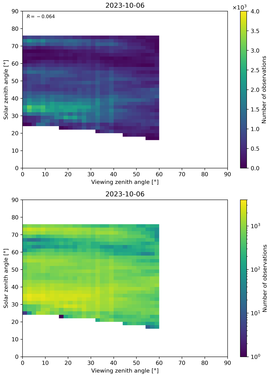
Figure 115: Scatter density plot of “Viewing zenith angle” against “Solar zenith angle” for 2023-10-06 to 2023-10-07.
