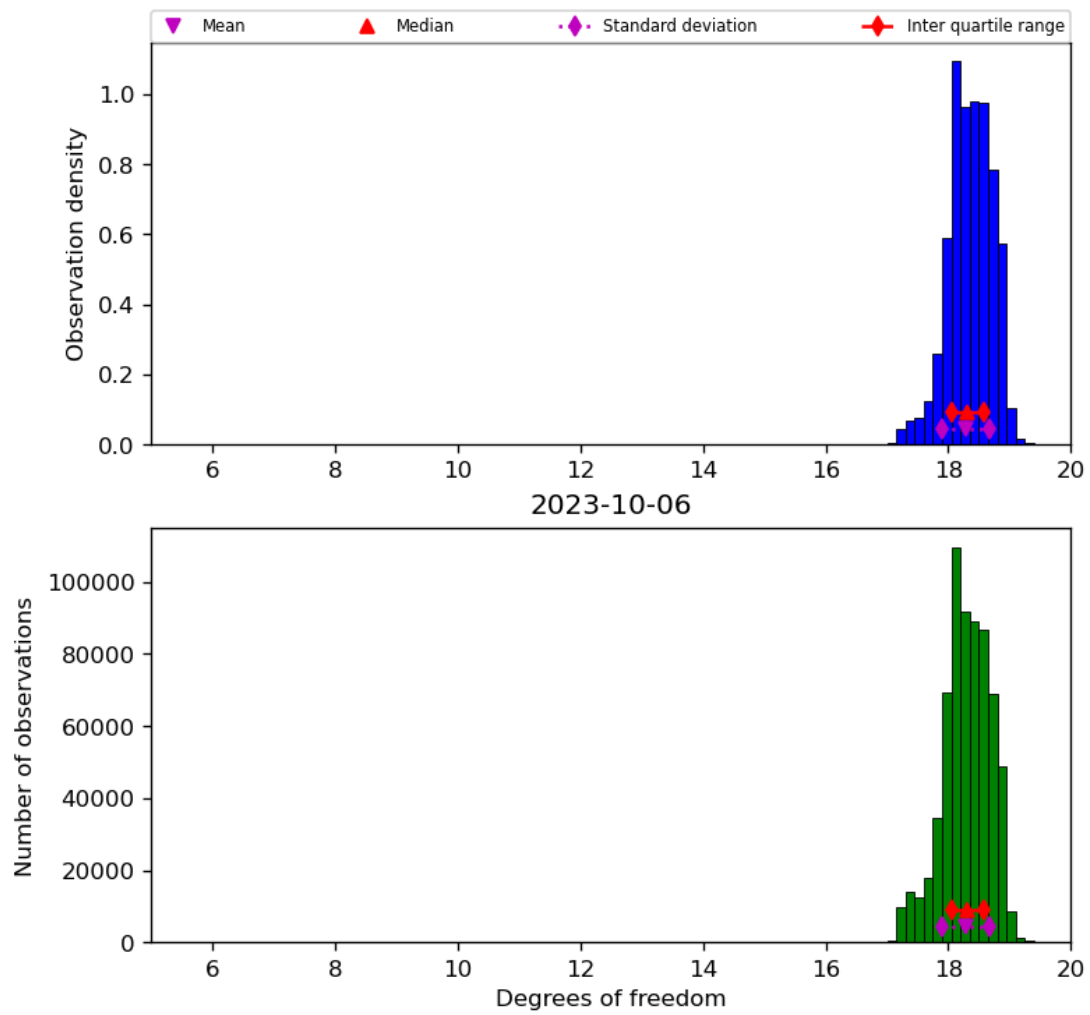
Figure 30: Histogram of “Degrees of freedom” for 2023-10-06 to 2023-10-07
