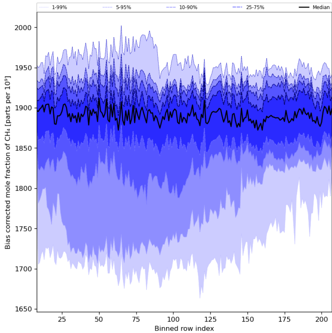
Figure 36: Along track statistics of “Bias corrected mole fraction of CH 4 ” for 2023-10-06 to 2023-10-07
