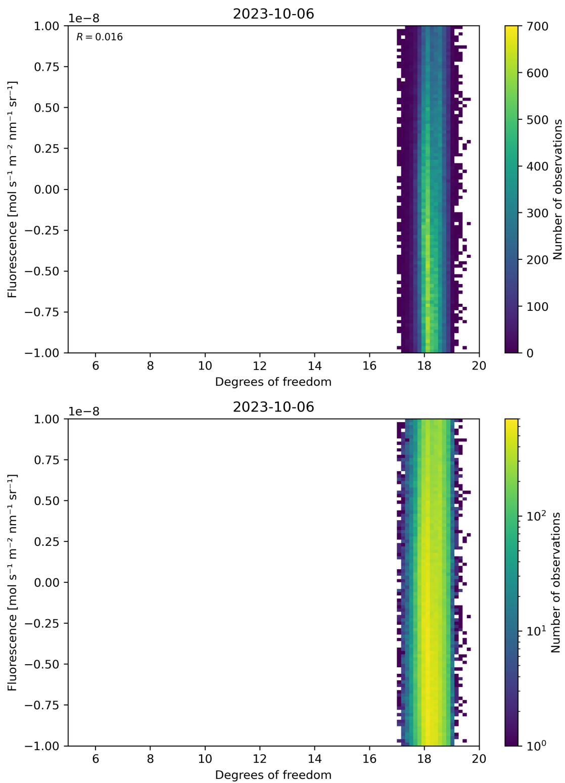
Figure 51: Scatter density plot of “Degrees of freedom” against “Fluorescence” for 2023-10-06 to 2023-10-07.
