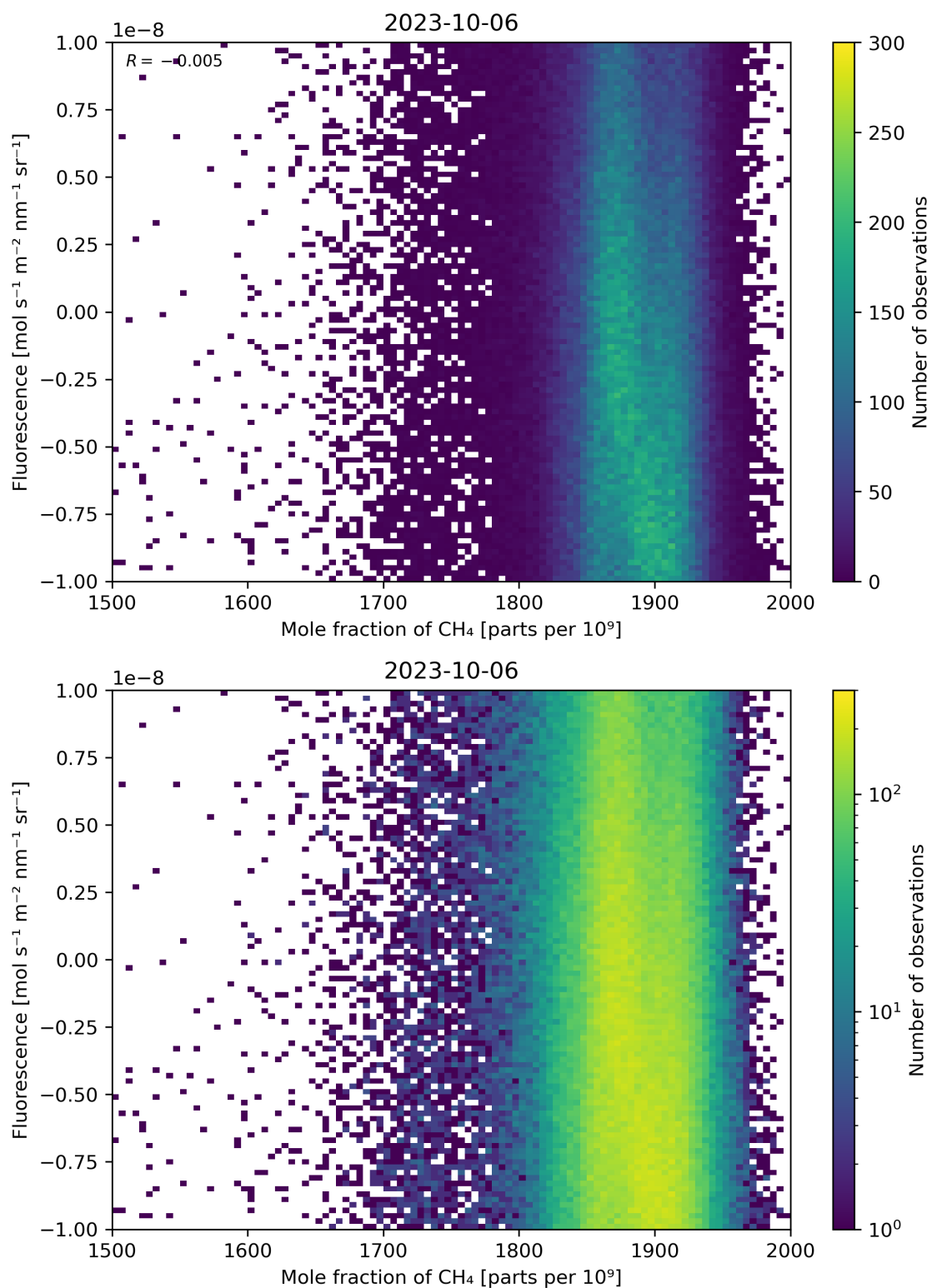
Figure 73: Scatter density plot of “Mole fraction of \text{CH}_4 ” against “Fluorescence” for 2023-10-06 to 2023-10-07.
