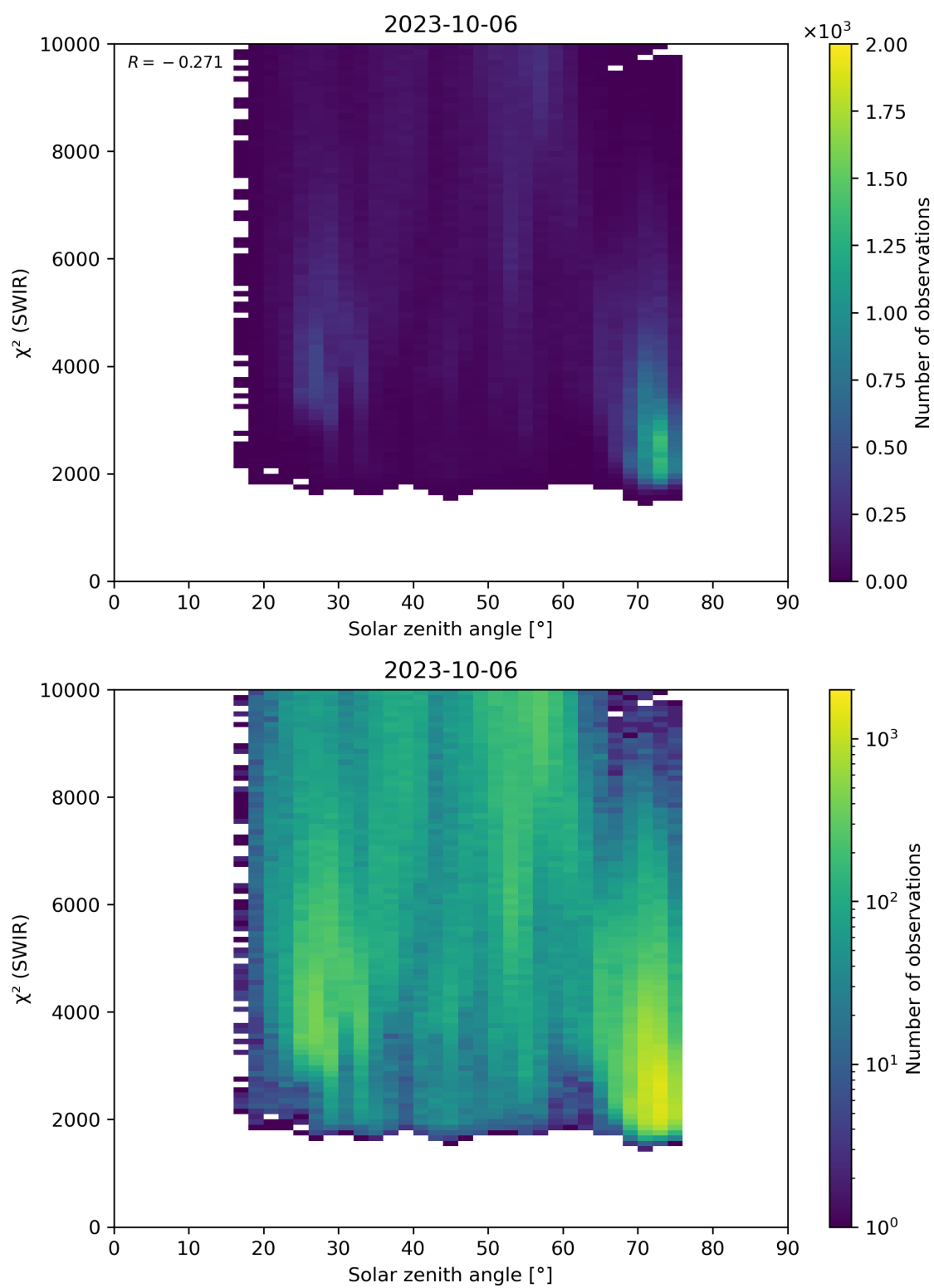
Figure 95: Scatter density plot of “Solar zenith angle” against “ \chi^2 (SWIR)” for 2023-10-06 to 2023-10-07.
