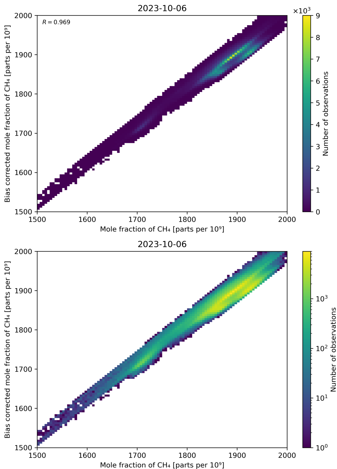
Figure 74: Scatter density plot of “Mole fraction of CH 4 ” against “Bias corrected mole fraction of CH 4 ” for 2023-10-06 to 2023-10-07.
