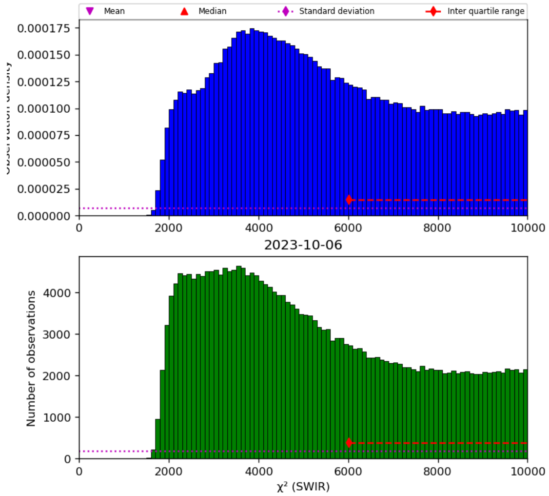
Figure 28: Histogram of “ \chi^2 (SWIR)” for 2023-10-06 to 2023-10-07
