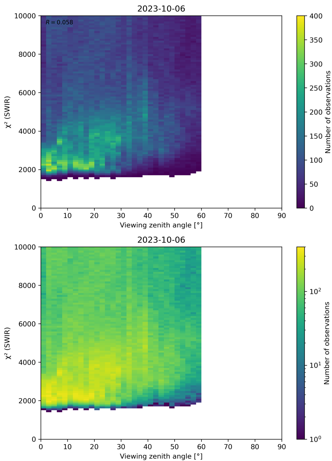
Figure 106: Scatter density plot of “Viewing zenith angle” against “ \chi^2 (SWIR)” for 2023-10-06 to 2023-10-07.
