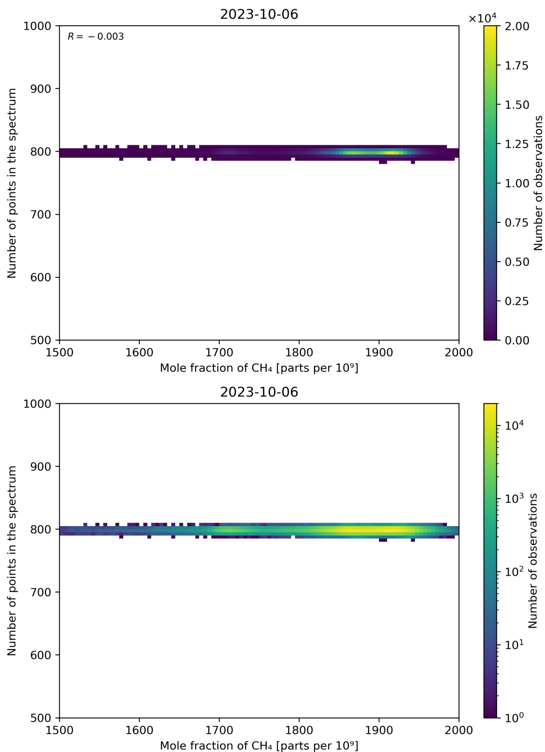
Figure 77: Scatter density plot of “Mole fraction of CH 4 ” against “Number of points in the spectrum” for 2023-10-06 to 2023-10-07.
