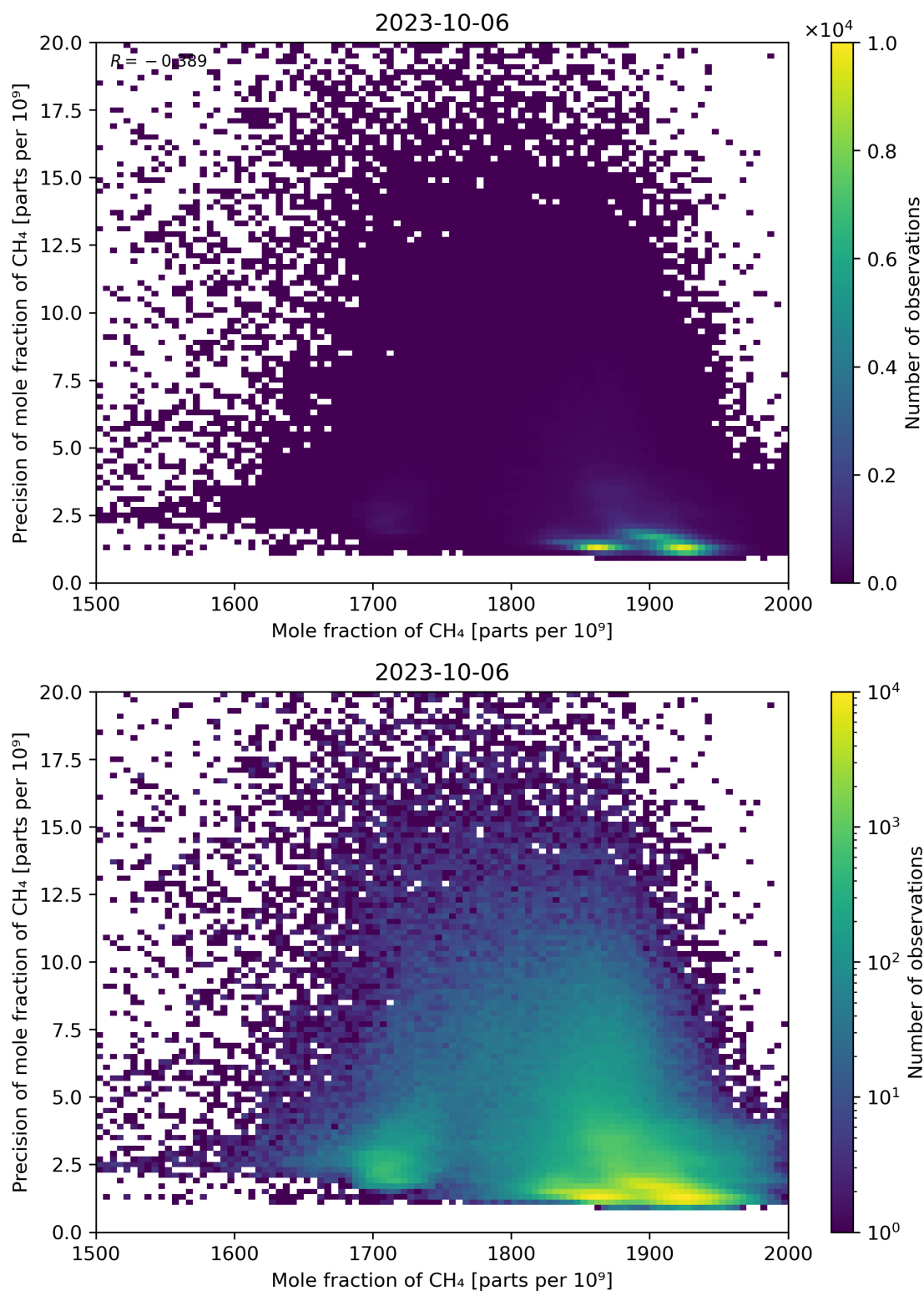
Figure 75: Scatter density plot of “Mole fraction of CH 4 ” against “Precision of mole fraction of CH 4 ” for 2023-10-06 to 2023-10-07.
