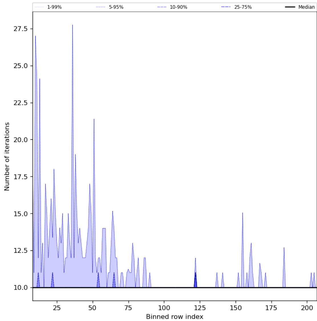
Figure 42: Along track statistics of “Number of iterations” for 2023-10-06 to 2023-10-07
