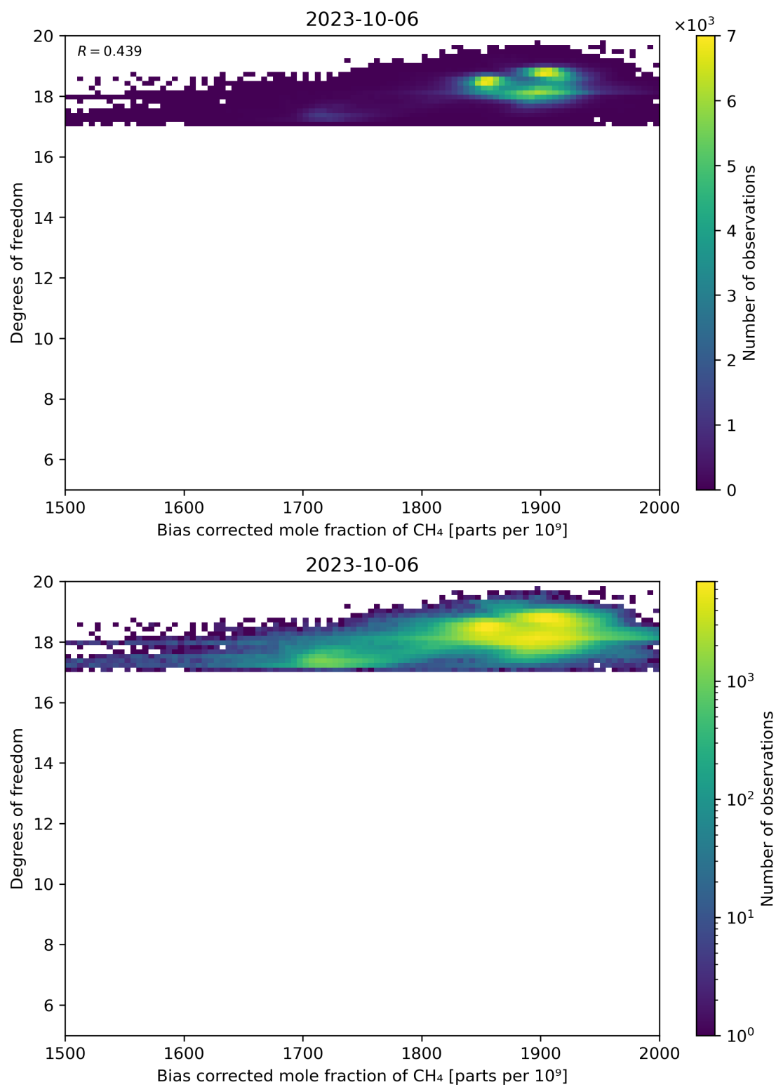
Figure 65: Scatter density plot of “Bias corrected mole fraction of CH 4 ” against “Degrees of freedom” for 2023-10-06 to 2023-10-07.
