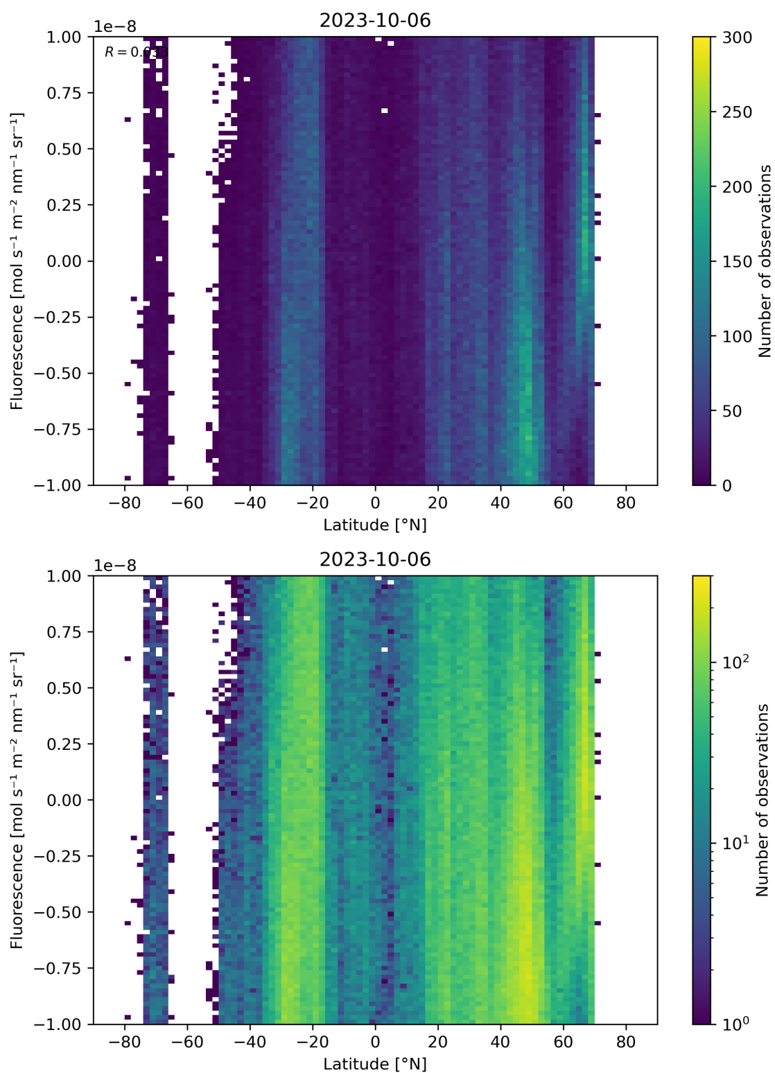
Figure 56: Scatter density plot of “Latitude” against “Fluorescence” for 2023-10-06 to 2023-10-07.
