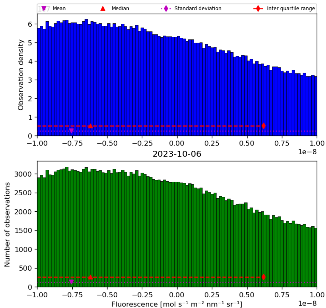
Figure 32: Histogram of “Fluorescence” for 2023-10-06 to 2023-10-07
