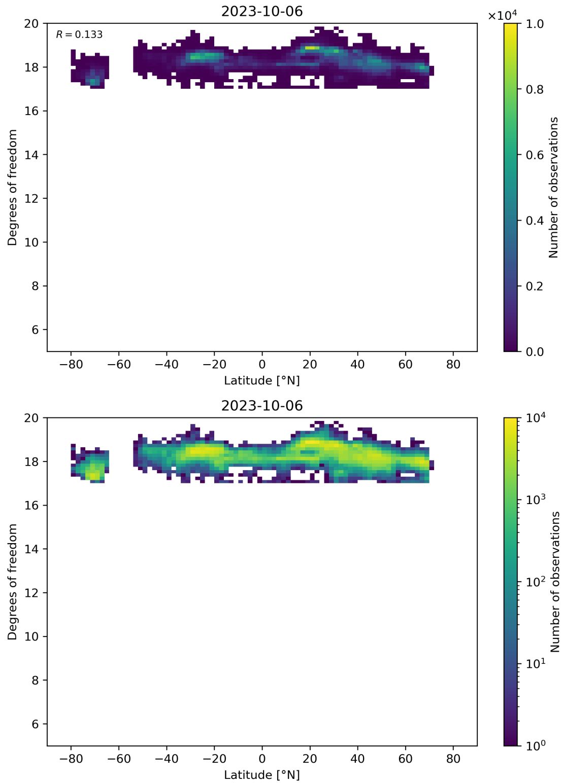
Figure 55: Scatter density plot of “Latitude” against “Degrees of freedom” for 2023-10-06 to 2023-10-07.
