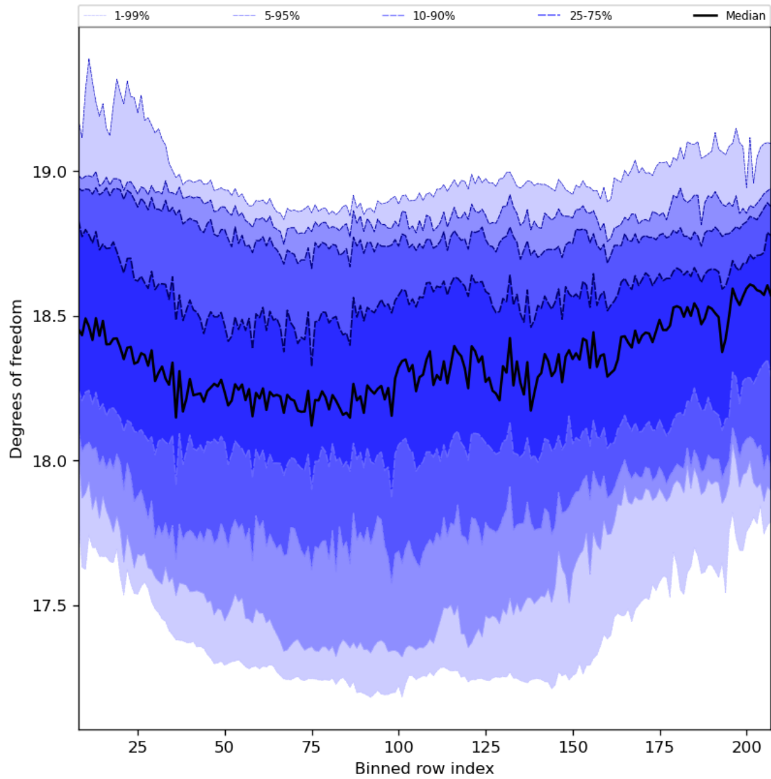
Figure 41: Along track statistics of “Degrees of freedom” for 2023-10-06 to 2023-10-07
