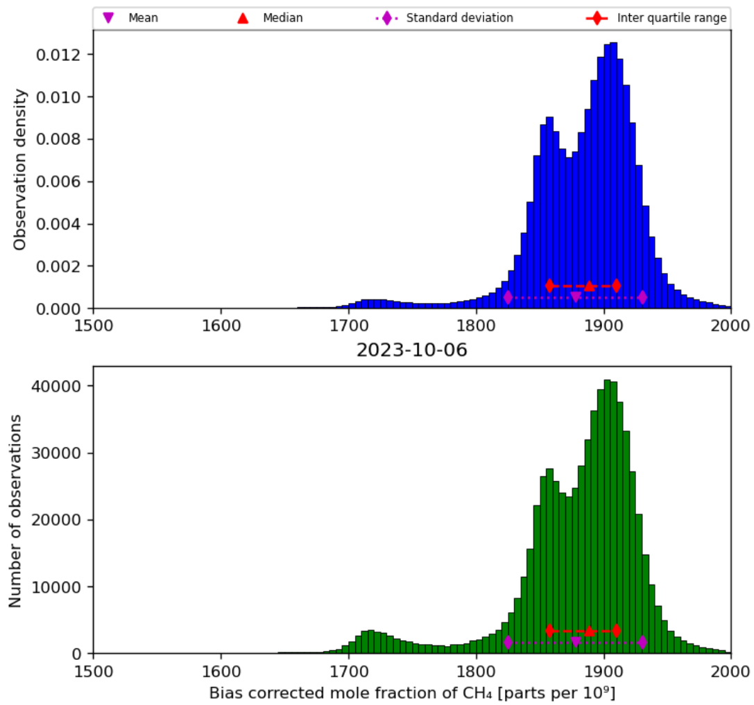
Figure 25: Histogram of “Bias corrected mole fraction of CH 4 ” for 2023-10-06 to 2023-10-07
