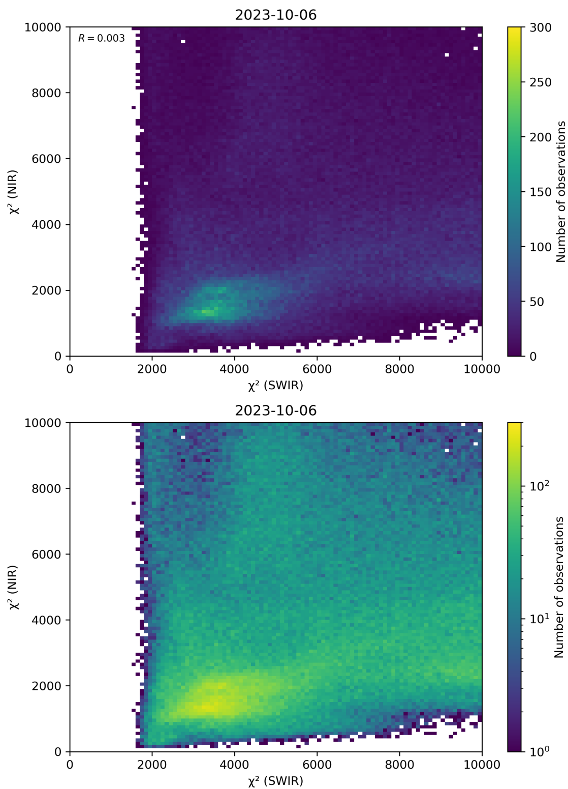
Figure 47: Scatter density plot of “ \chi^2 (SWIR)” against “ \chi^2 (NIR)” for 2023-10-06 to 2023-10-07.
