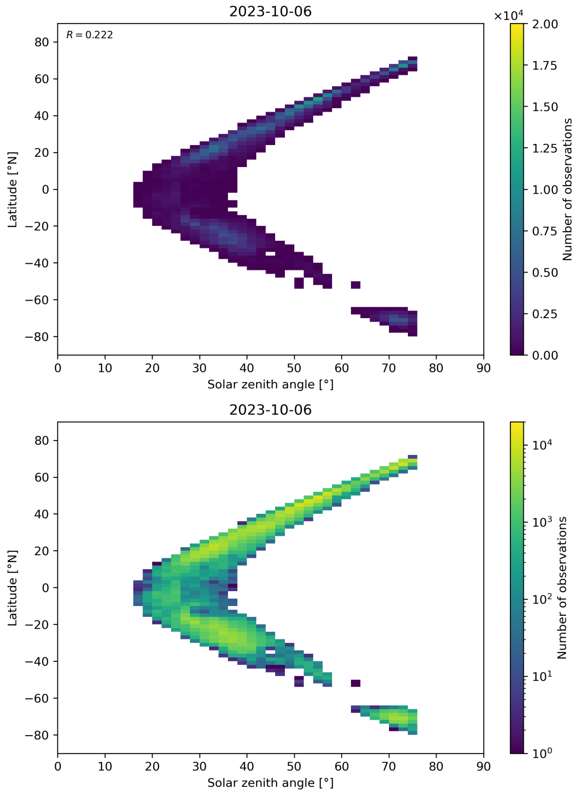
Figure 98: Scatter density plot of “Solar zenith angle” against “Latitude” for 2023-10-06 to 2023-10-07.
