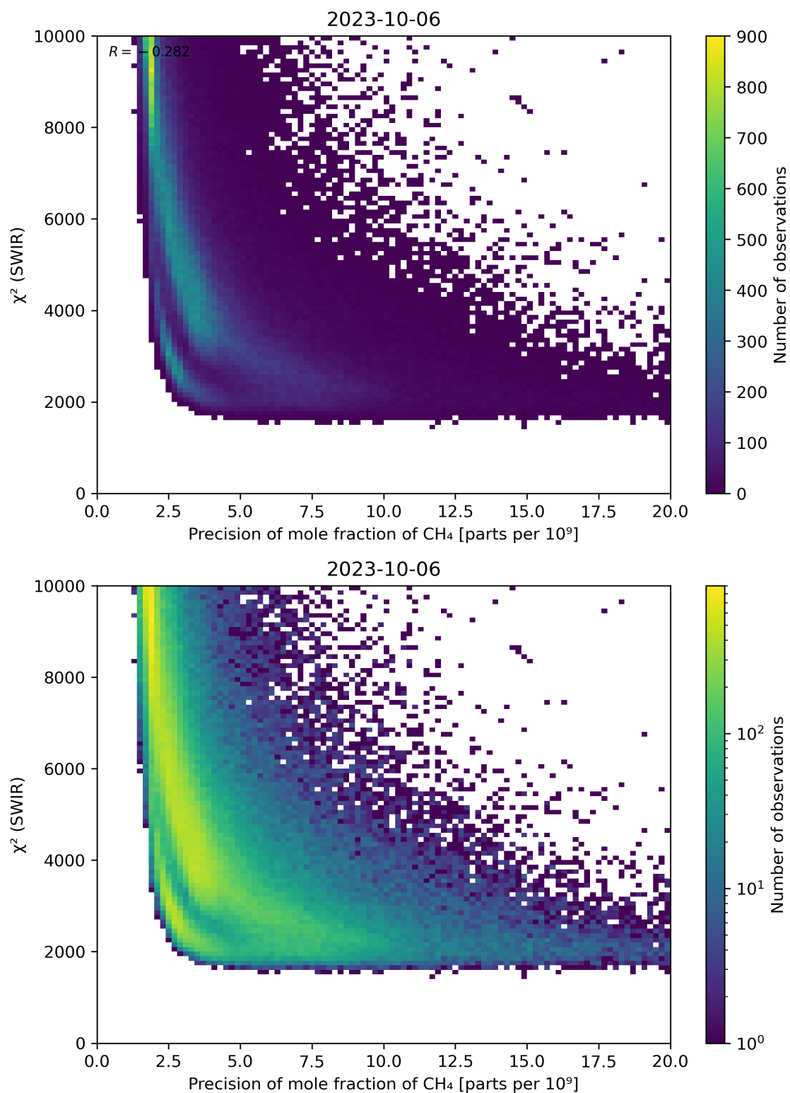
Figure 79: Scatter density plot of “Precision of mole fraction of CH 4 ” against “ \chi^2 (SWIR)” for 2023-10-06 to 2023-10-07.
