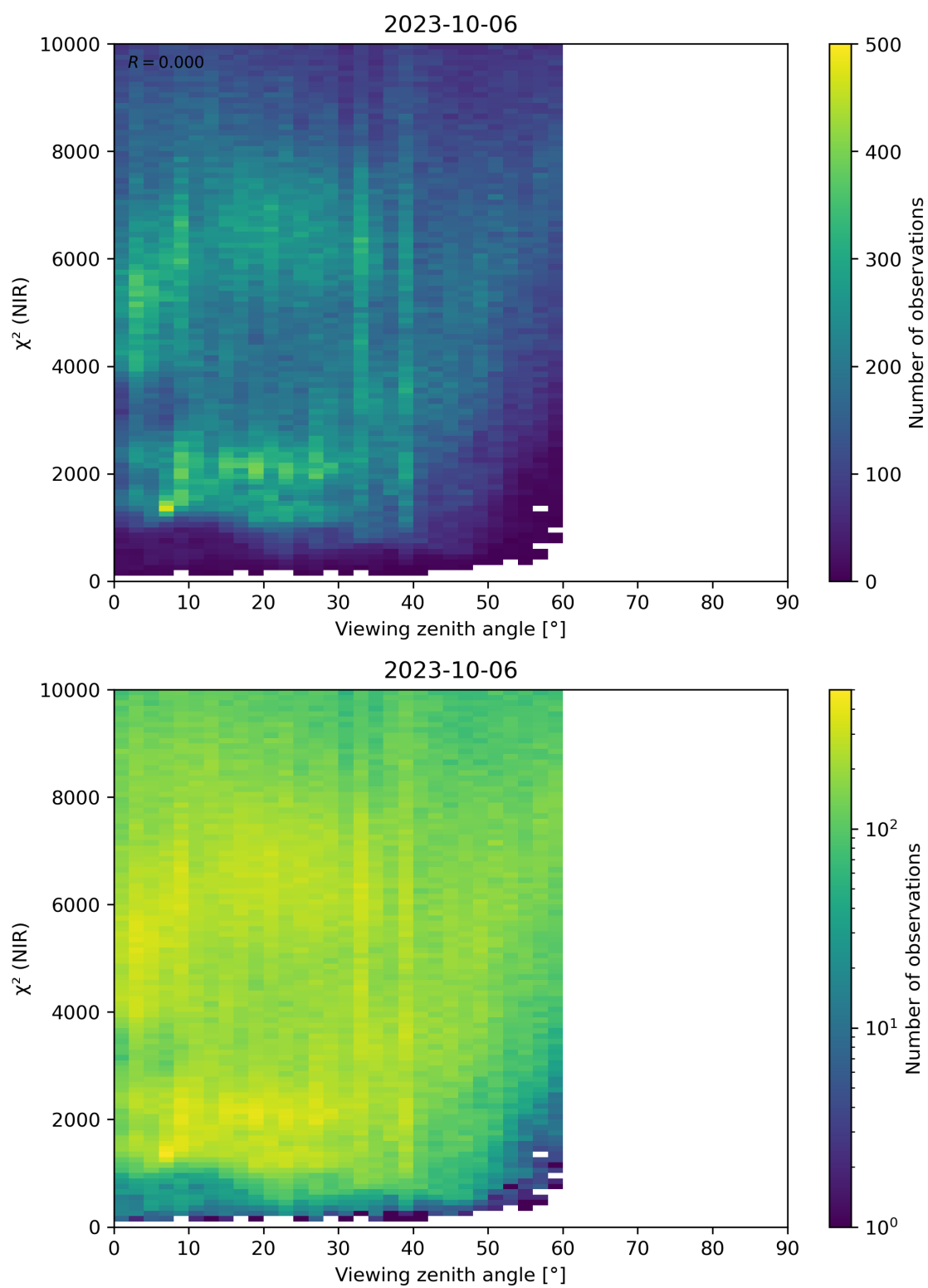
Figure 105: Scatter density plot of “Viewing zenith angle” against “ \chi^2 (NIR)” for 2023-10-06 to 2023-10-07.
