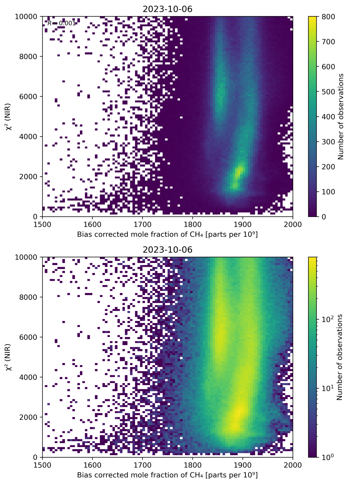
Figure 63: Scatter density plot of “Bias corrected mole fraction of CH 4 ” against “ \chi^2 (NIR)” for 2023-10-06 to 2023-10-07.
