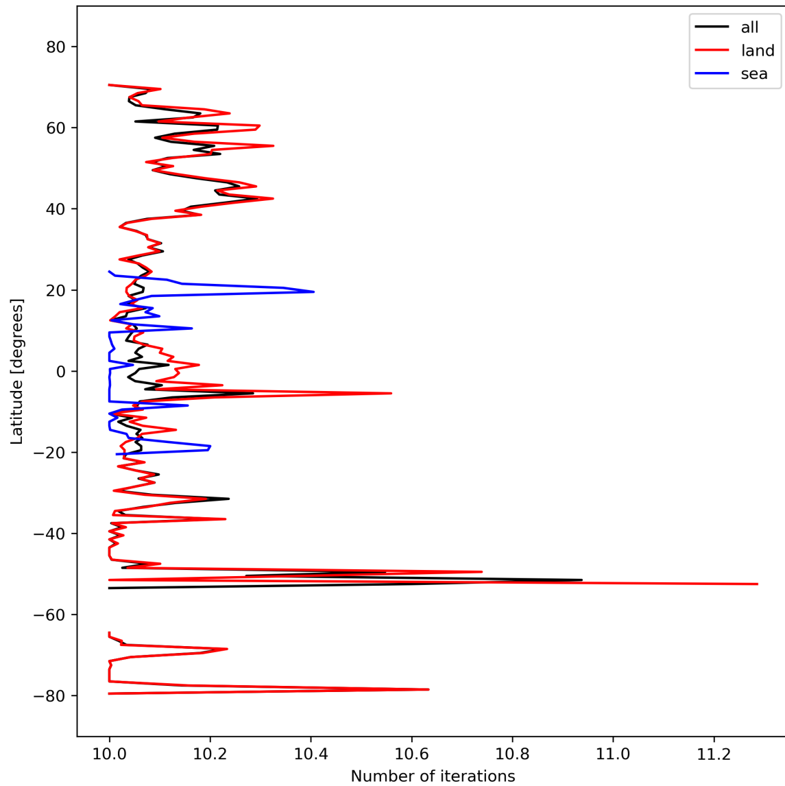
Figure 20: Zonal average of “Number of iterations” for 2023-10-06 to 2023-10-07.
