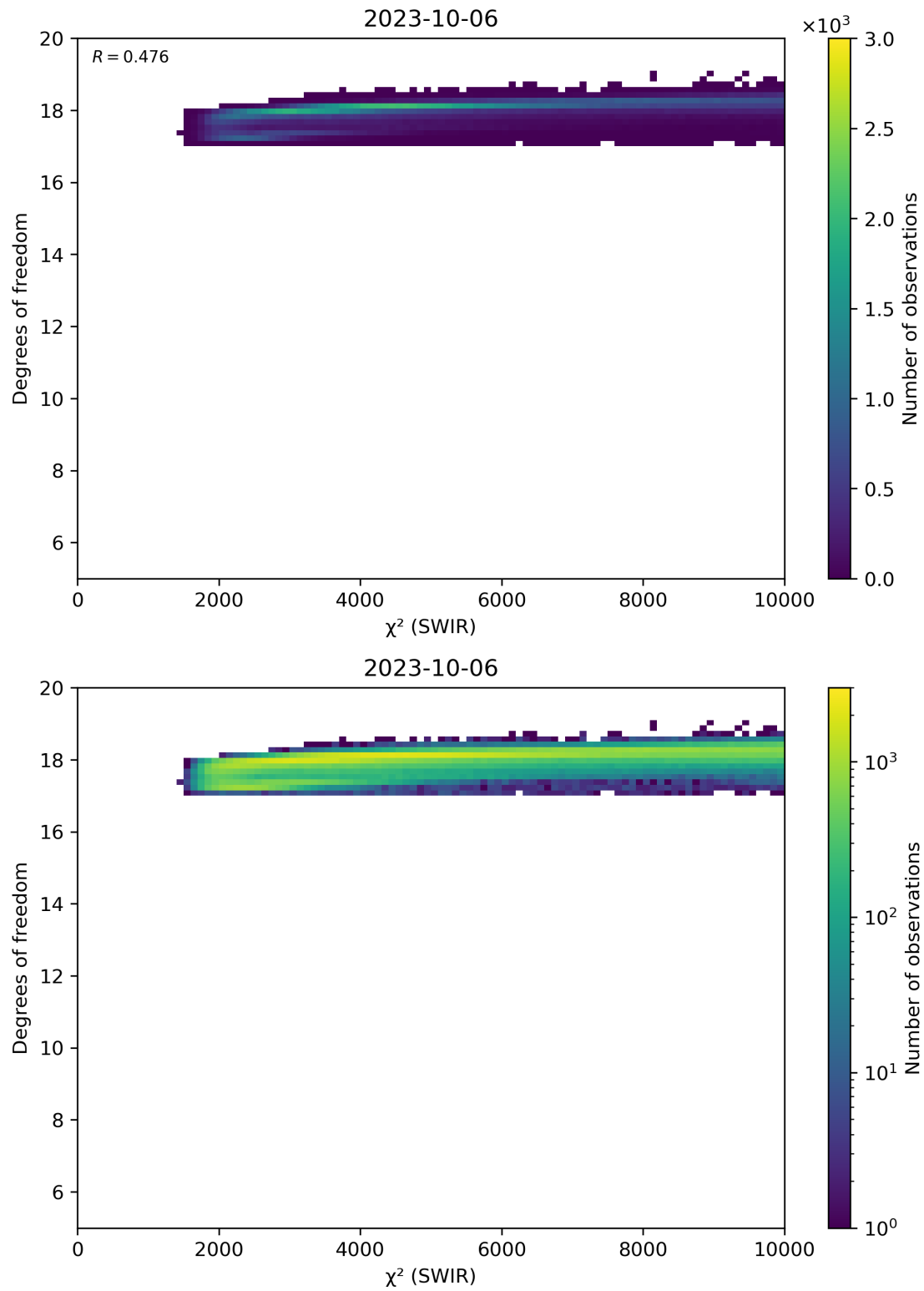
Figure 48: Scatter density plot of “ \chi^2 (SWIR)” against “Degrees of freedom” for 2023-10-06 to 2023-10-07.
