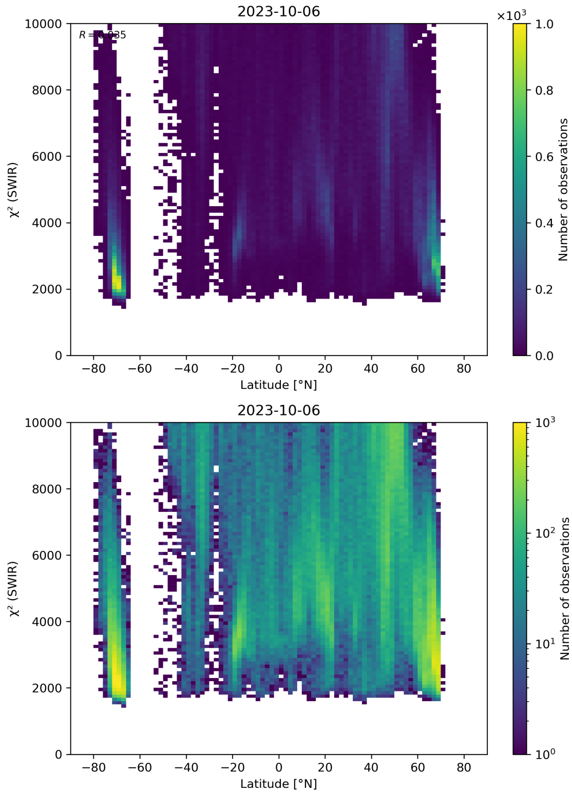
Figure 54: Scatter density plot of “Latitude” against “ \chi^2 (SWIR)” for 2023-10-06 to 2023-10-07.
