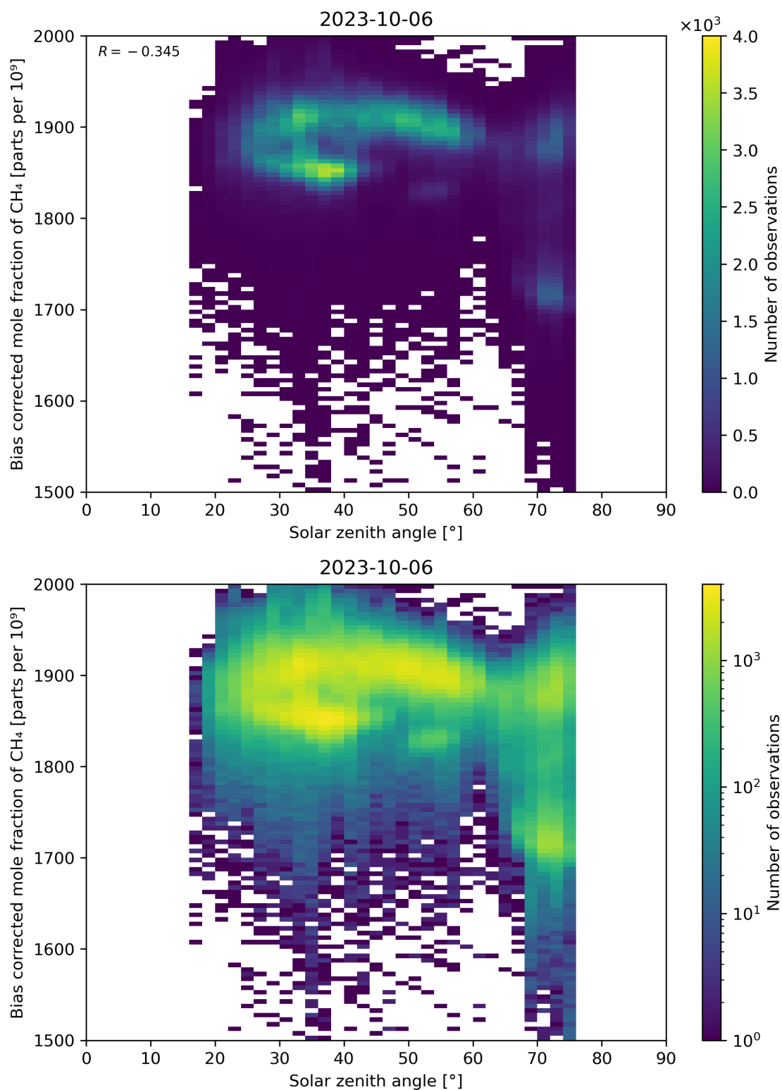
Figure 100: Scatter density plot of “Solar zenith angle” against “Bias corrected mole fraction of CH 4 ” for 2023-10-06 to 2023-10-07.
