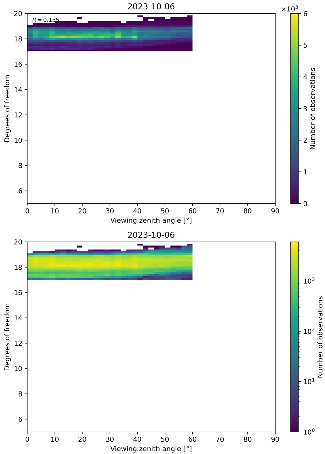
Figure 107: Scatter density plot of “Viewing zenith angle” against “Degrees of freedom” for 2023-10-06 to 2023-10-07.
