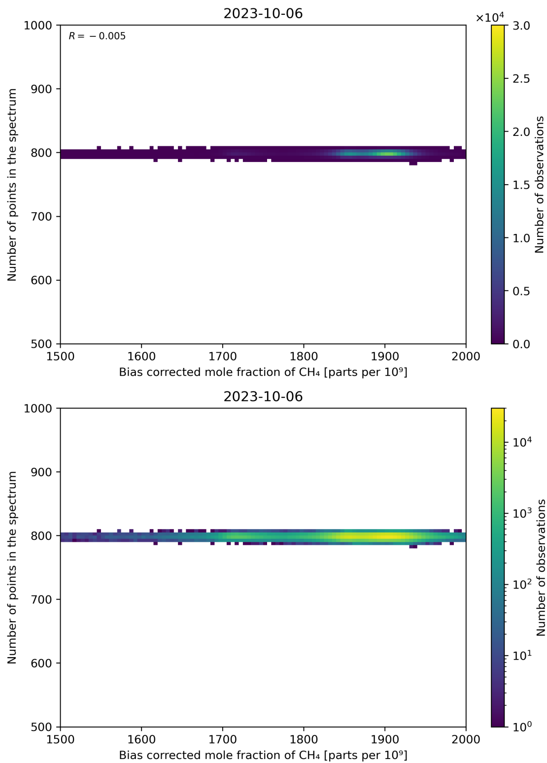
Figure 68: Scatter density plot of “Bias corrected mole fraction of CH 4 ” against “Number of points in the spectrum” for 2023-10-06 to 2023-10-07.
