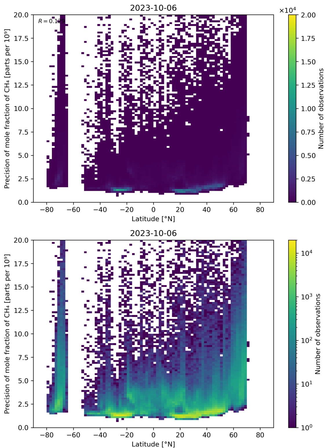
Figure 59: Scatter density plot of “Latitude” against “Precision of mole fraction of CH 4 ” for 2023-10-06 to 2023-10-07.
