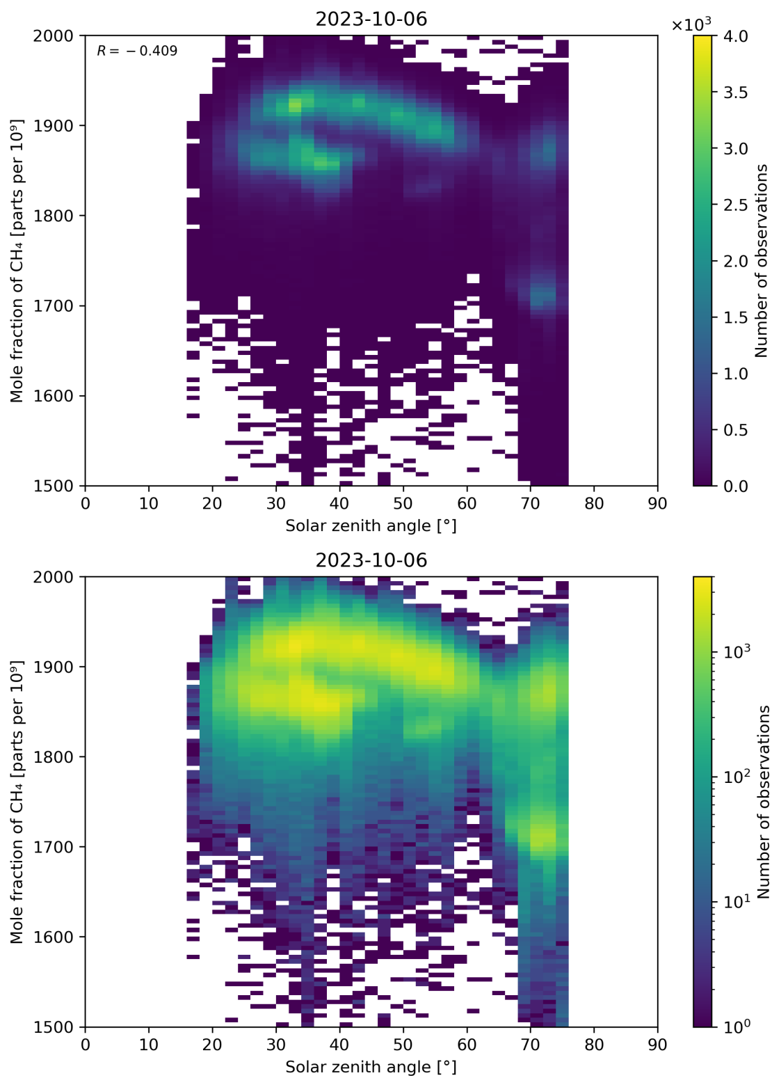
Figure 99: Scatter density plot of “Solar zenith angle” against “Mole fraction of CH 4 ” for 2023-10-06 to 2023-10-07.
