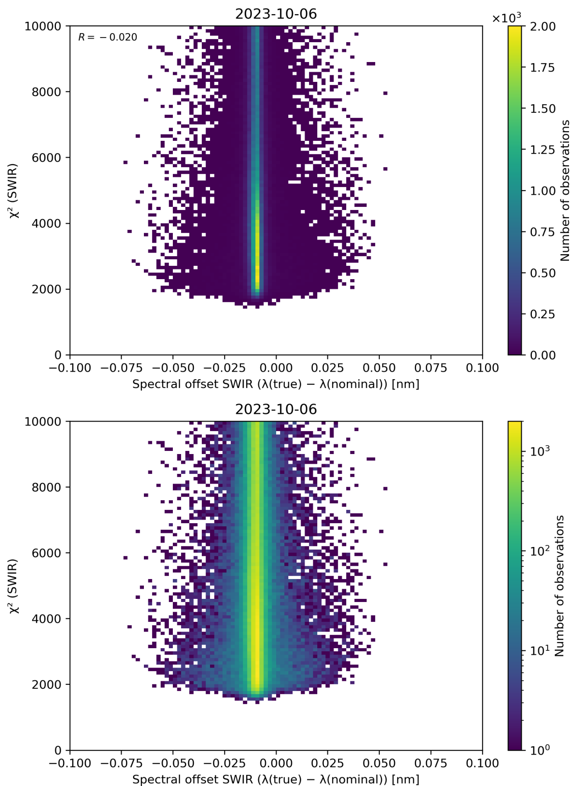
Figure 118: Scatter density plot of “Spectral offset SWIR ( \lambda(\text{true}) - \lambda(\text{nominal}) )” against “ \chi^2 (SWIR)” for 2023-10-06 to 2023-10-07.
