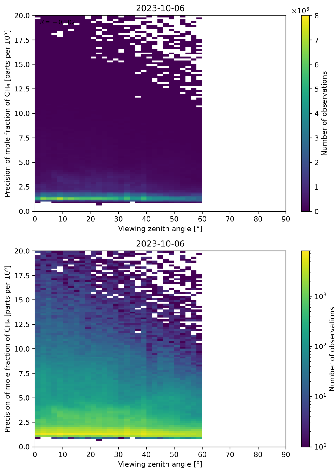
Figure 112: Scatter density plot of “Viewing zenith angle” against “Precision of mole fraction of CH 4 ” for 2023-10-06 to 2023-10-07.
