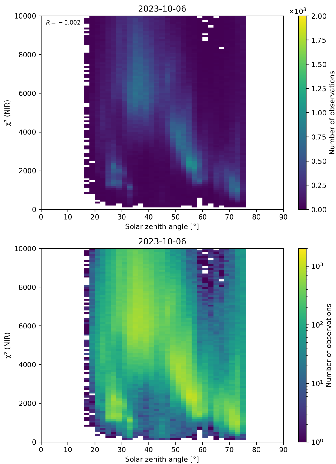
Figure 94: Scatter density plot of “Solar zenith angle” against “ \chi^2 (NIR)” for 2023-10-06 to 2023-10-07.
