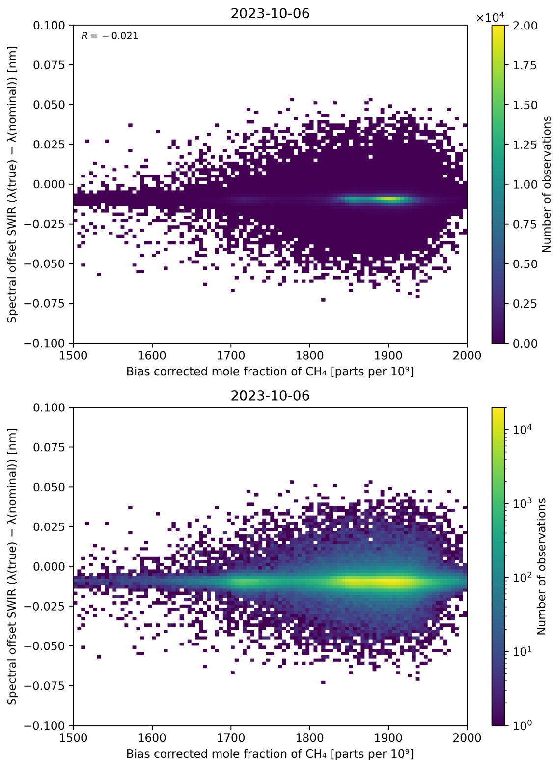
Figure 69: Scatter density plot of “Bias corrected mole fraction of \text{CH}_4 ” against “Spectral offset SWIR ( \lambda(\text{true}) - \lambda(\text{nominal}) )” for 2023-10-06 to 2023-10-07.
