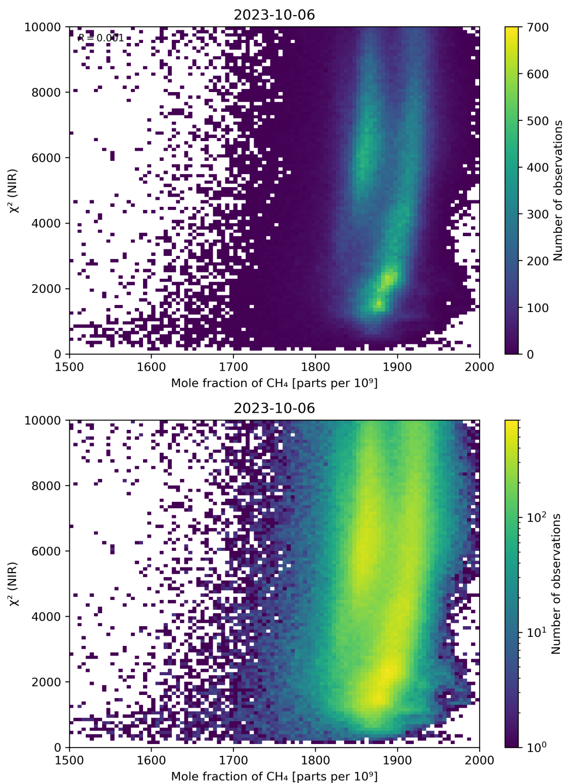
Figure 70: Scatter density plot of “Mole fraction of \text{CH}_4 ” against “ \chi^2 (NIR)” for 2023-10-06 to 2023-10-07.
