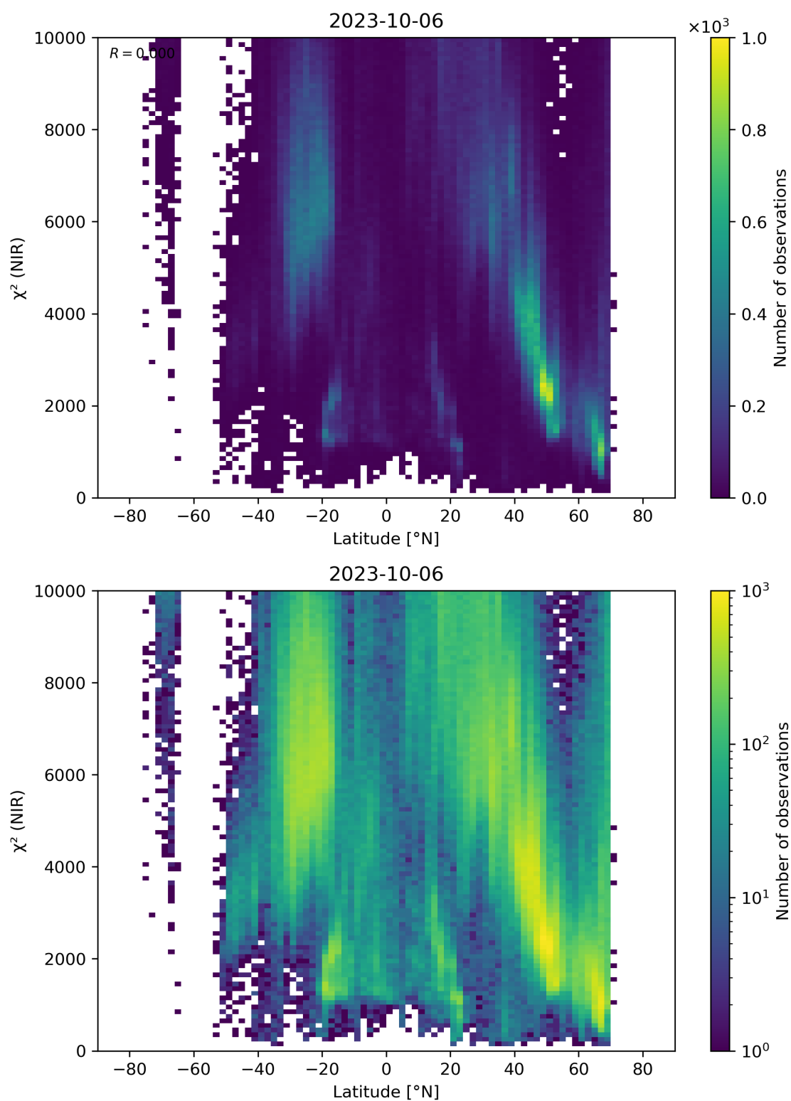
Figure 53: Scatter density plot of “Latitude” against “ \chi^2 (NIR)” for 2023-10-06 to 2023-10-07.
