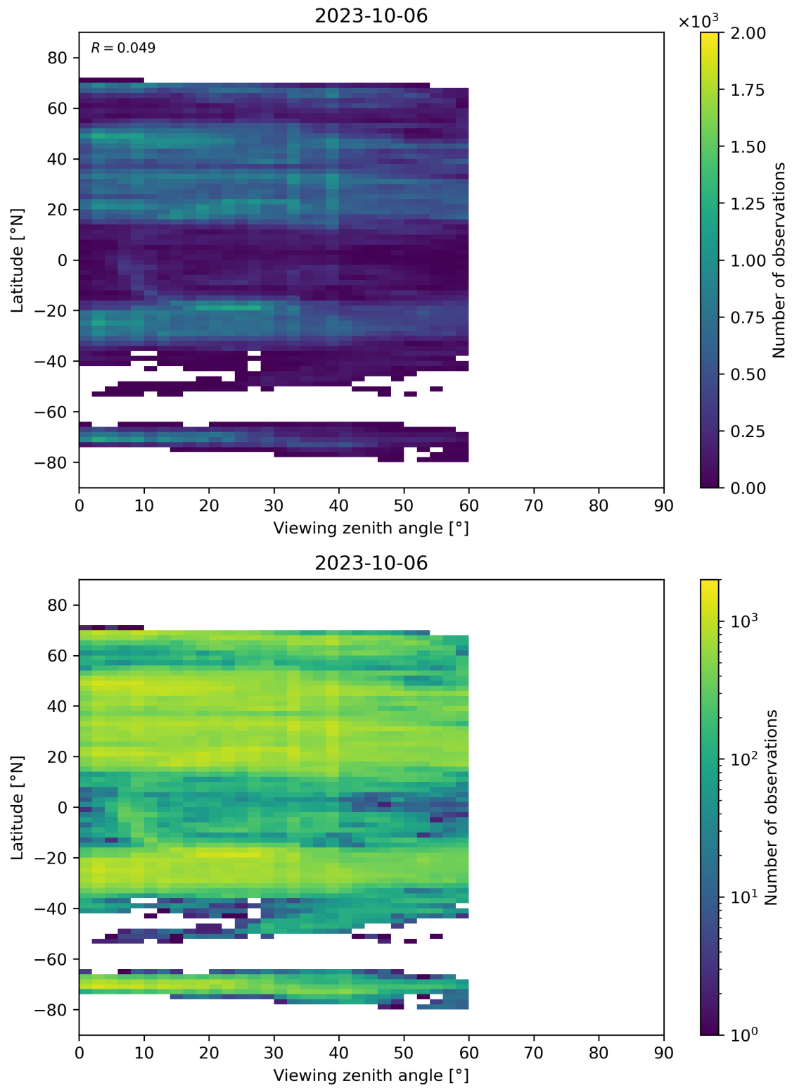
Figure 109: Scatter density plot of “Viewing zenith angle” against “Latitude” for 2023-10-06 to 2023-10-07.
