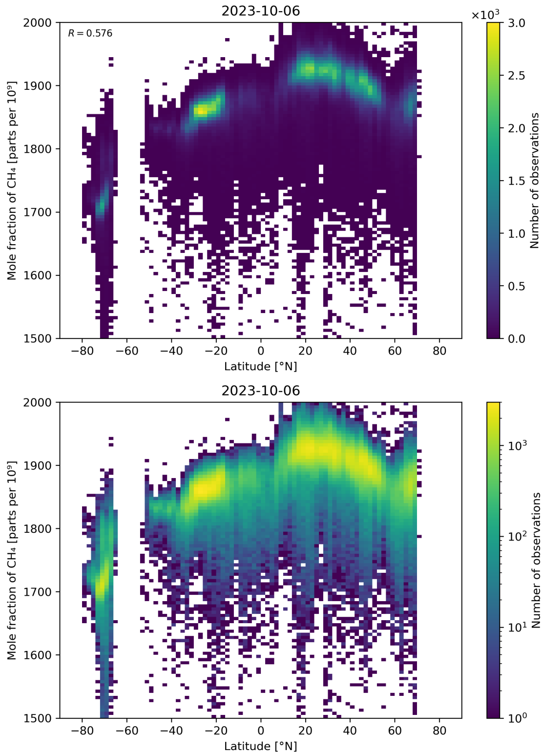
Figure 57: Scatter density plot of “Latitude” against “Mole fraction of \text{CH}_4 ” for 2023-10-06 to 2023-10-07.
