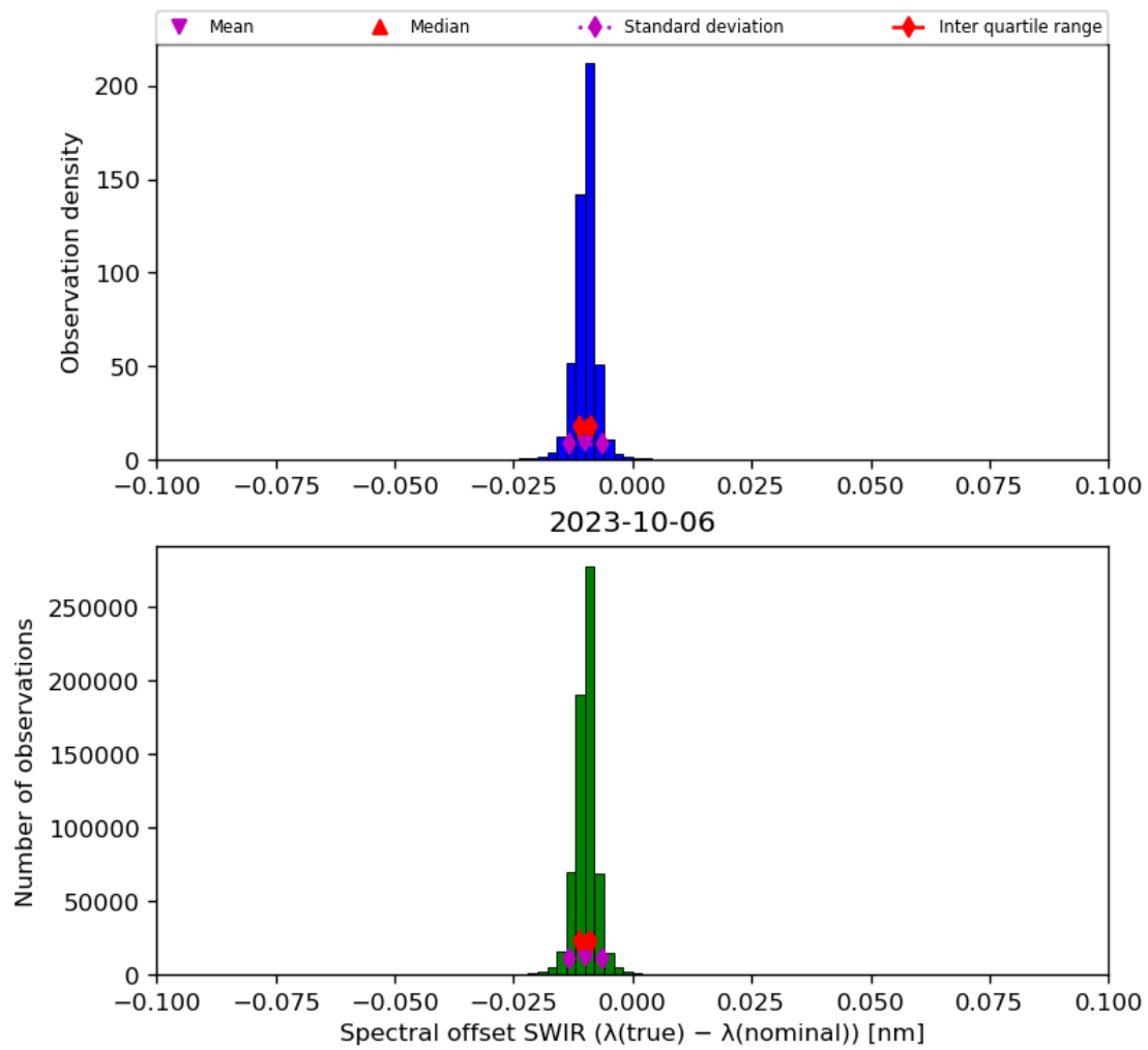
Figure 27: Histogram of “Spectral offset SWIR ( \lambda(\text{true}) - \lambda(\text{nominal}) )” for 2023-10-06 to 2023-10-07
