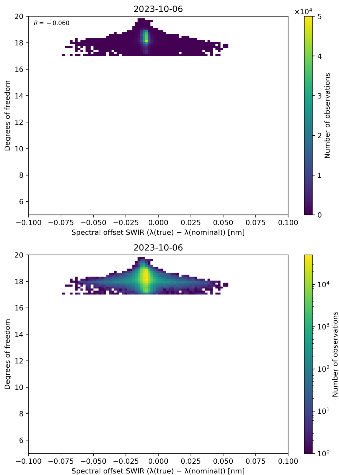
Figure 119: Scatter density plot of “Spectral offset SWIR ( \lambda(\text{true}) - \lambda(\text{nominal}) )” against “Degrees of freedom” for 2023-10-06 to 2023-10-07.
