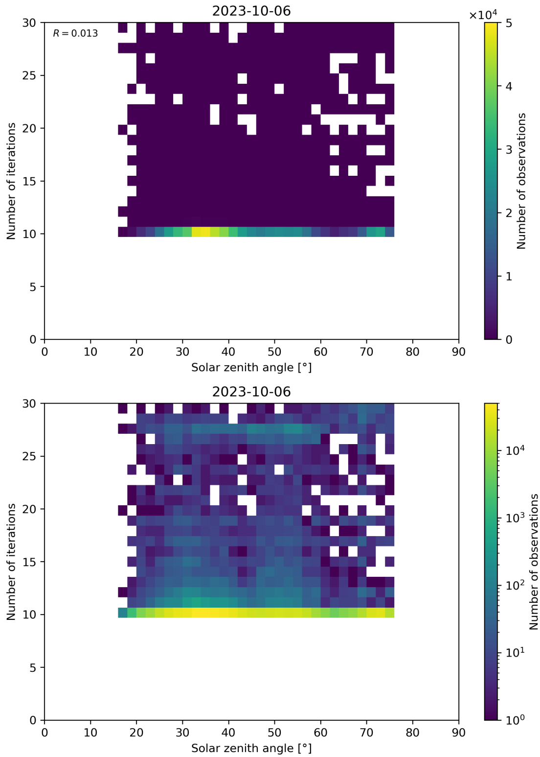
Figure 102: Scatter density plot of “Solar zenith angle” against “Number of iterations” for 2023-10-06 to 2023-10-07.
