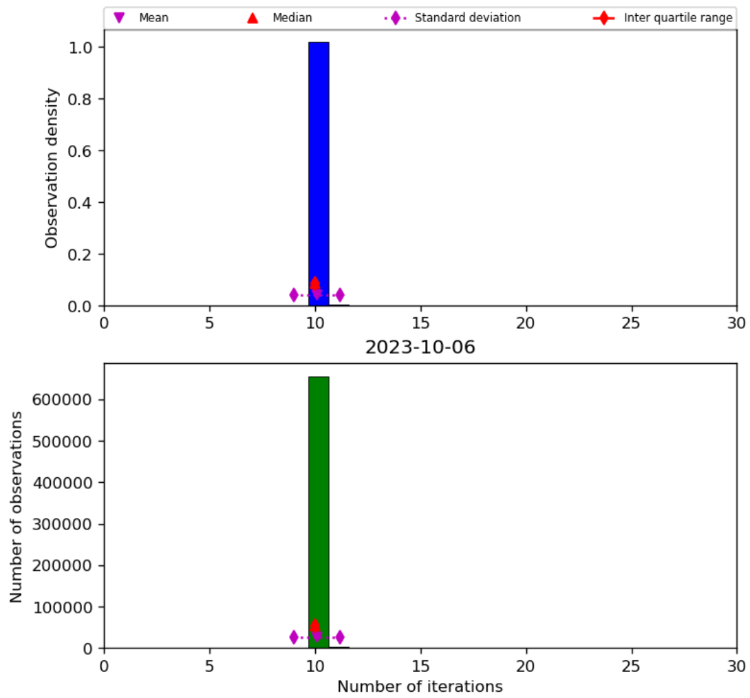
Figure 31: Histogram of “Number of iterations” for 2023-10-06 to 2023-10-07
