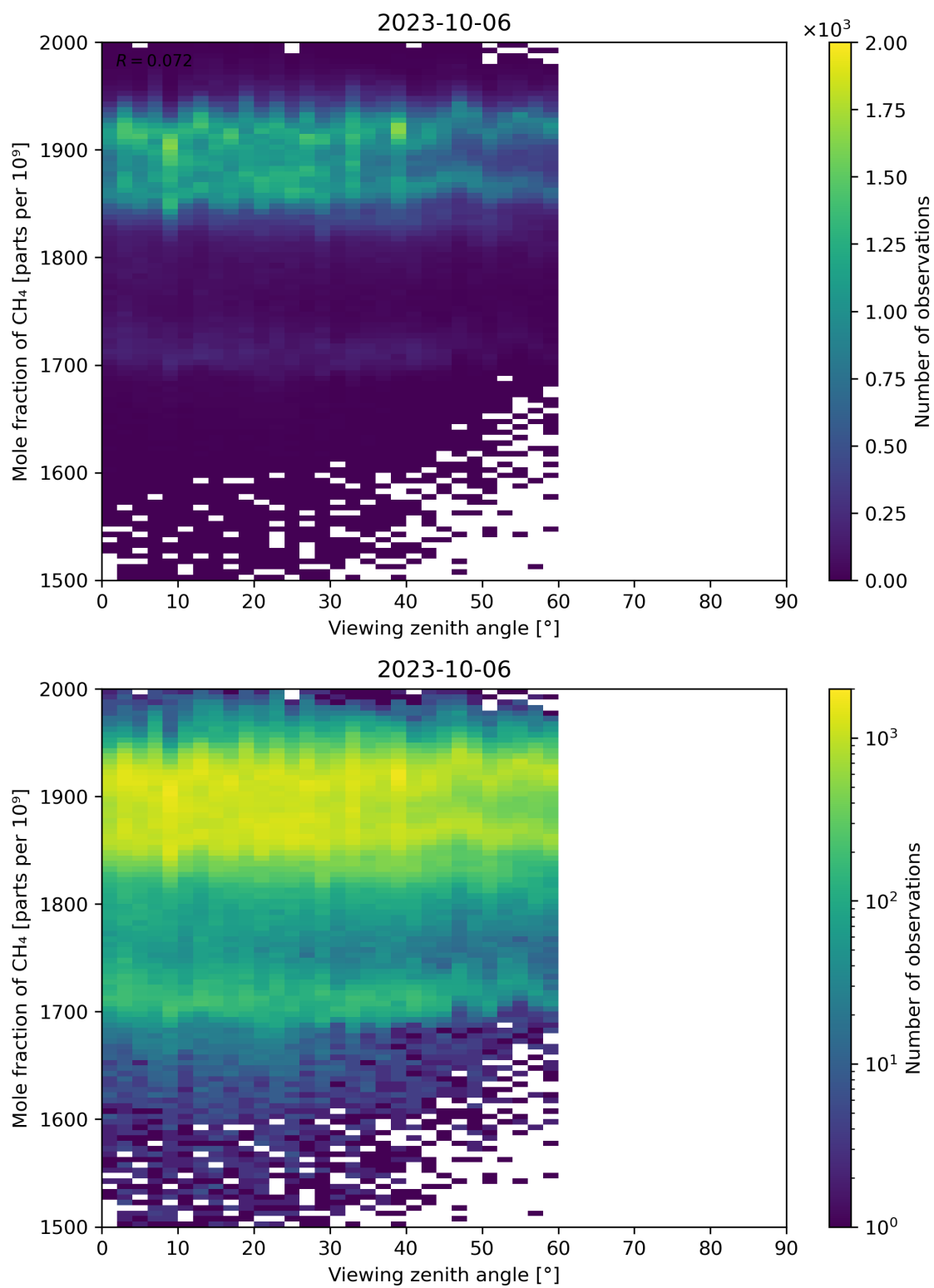
Figure 110: Scatter density plot of “Viewing zenith angle” against “Mole fraction of CH 4 ” for 2023-10-06 to 2023-10-07.
