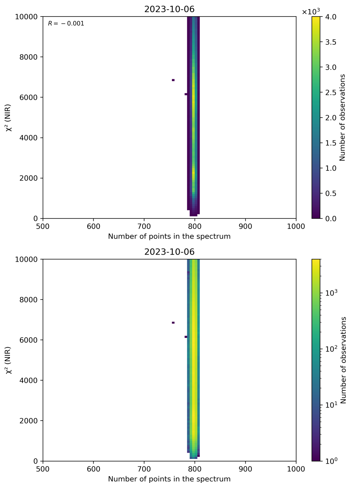
Figure 88: Scatter density plot of “Number of points in the spectrum” against “ \chi^2 (NIR)” for 2023-10-06 to 2023-10-07.
