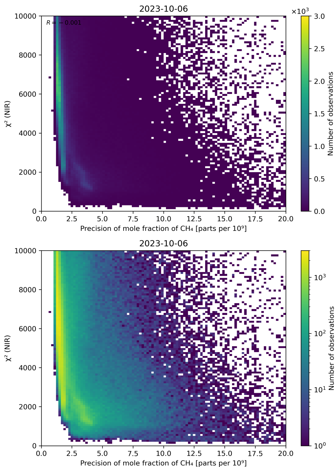
Figure 78: Scatter density plot of “Precision of mole fraction of CH 4 ” against “ \chi^2 (NIR)” for 2023-10-06 to 2023-10-07.
