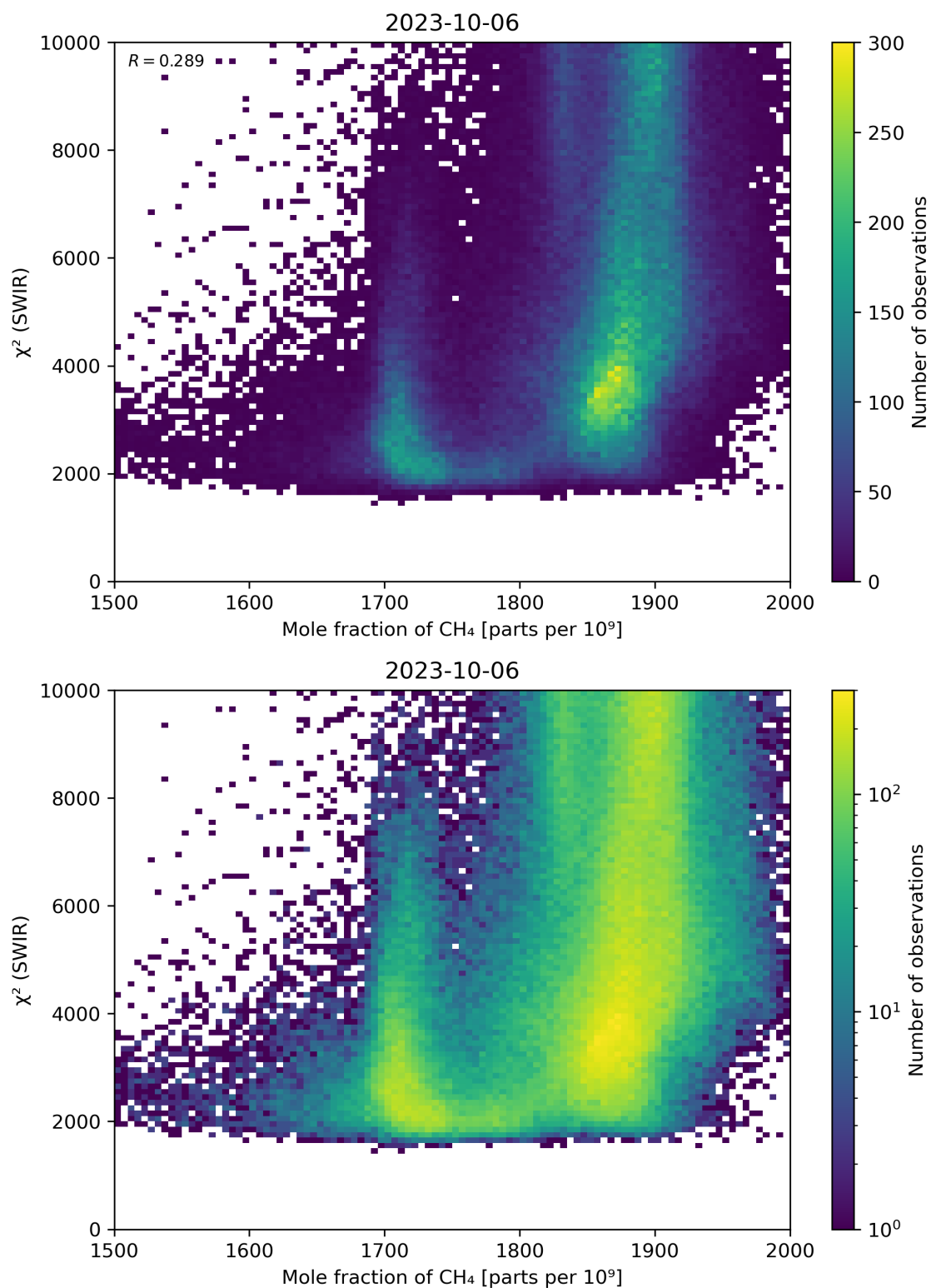
Figure 71: Scatter density plot of “Mole fraction of \text{CH}_4 ” against “ \chi^2 (SWIR)” for 2023-10-06 to 2023-10-07.
