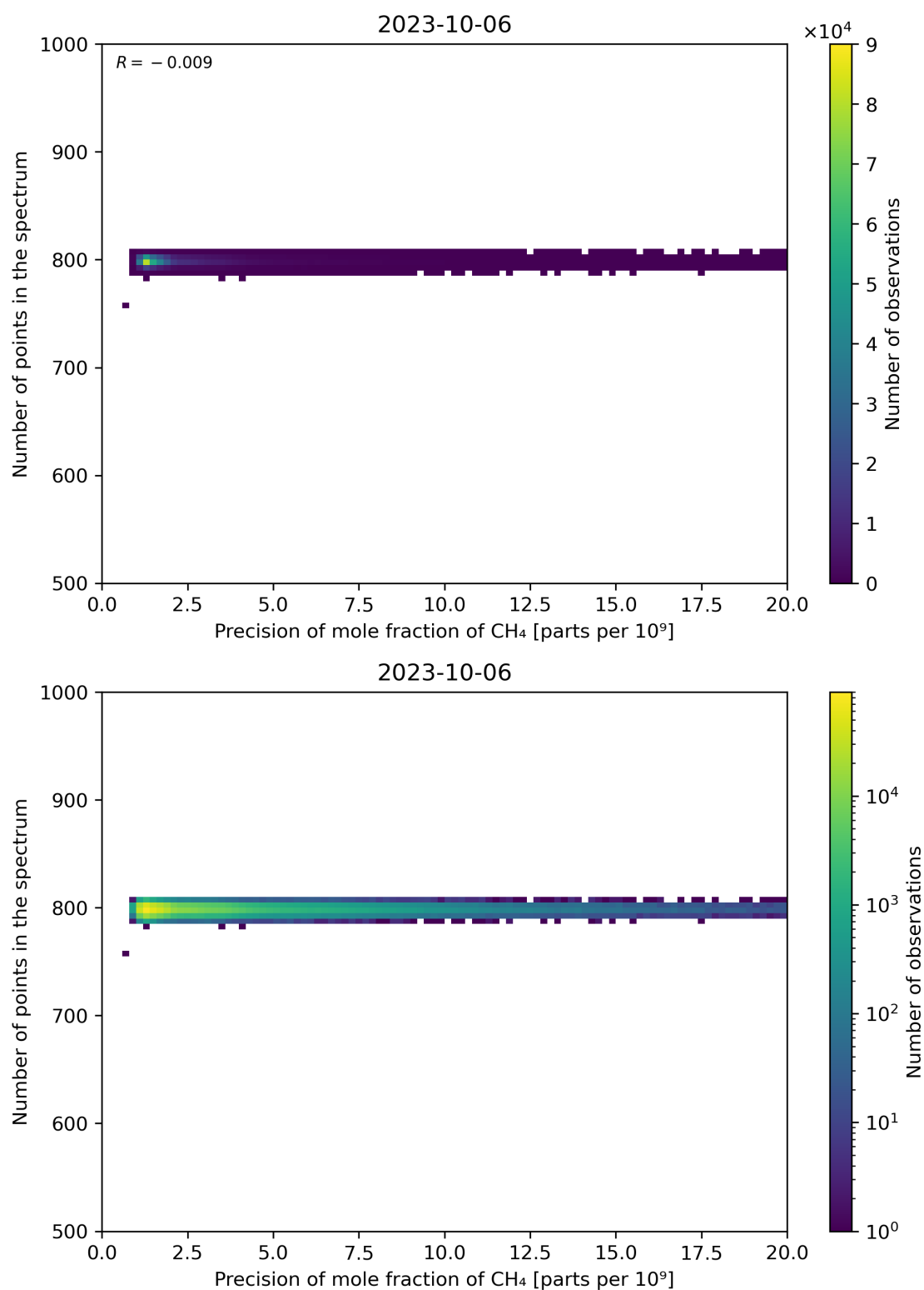
Figure 84: Scatter density plot of “Precision of mole fraction of CH 4 ” against “Number of points in the spectrum” for 2023-10-06 to 2023-10-07.
