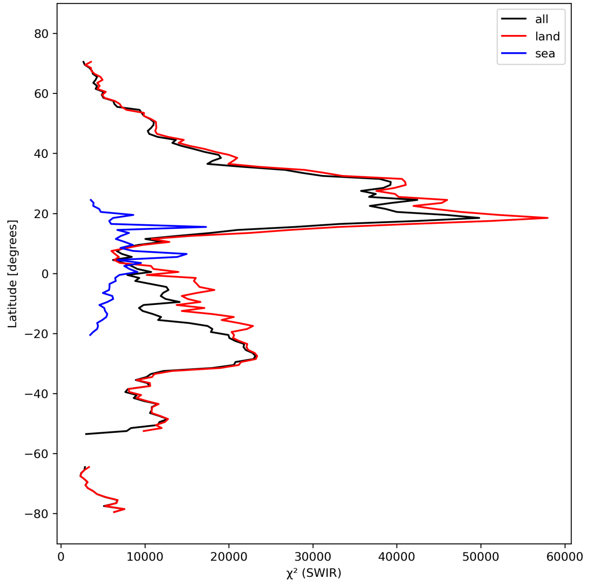
Figure 17: Zonal average of “ \chi^2 (SWIR)” for 2023-10-06 to 2023-10-07.
