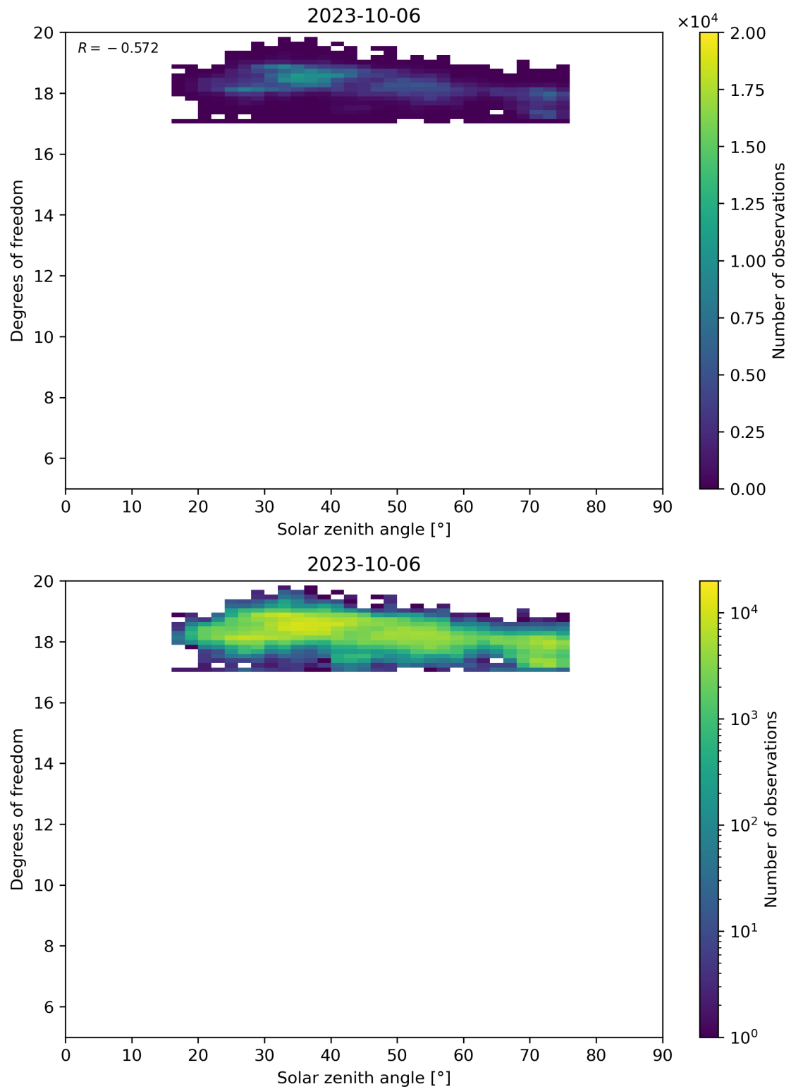
Figure 96: Scatter density plot of “Solar zenith angle” against “Degrees of freedom” for 2023-10-06 to 2023-10-07.
