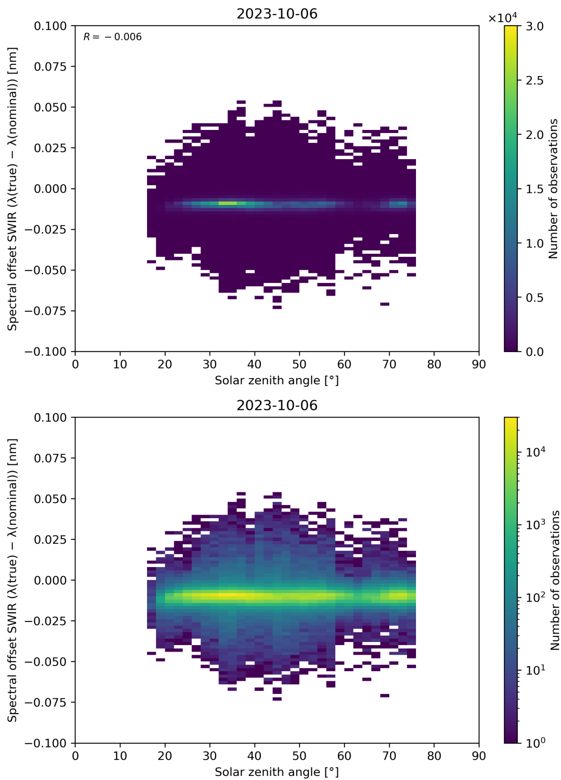
Figure 104: Scatter density plot of “Solar zenith angle” against “Spectral offset SWIR ( \lambda(\text{true}) - \lambda(\text{nominal}) )” for 2023-10-06 to 2023-10-07.
