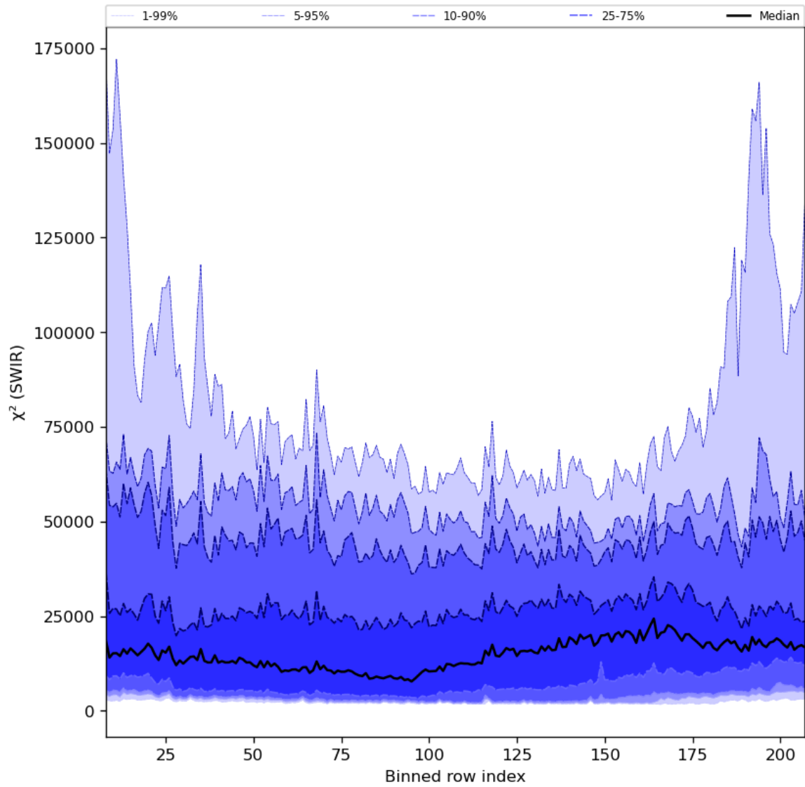
Figure 39: Along track statistics of " \chi^2 (SWIR)" for 2023-10-06 to 2023-10-08
