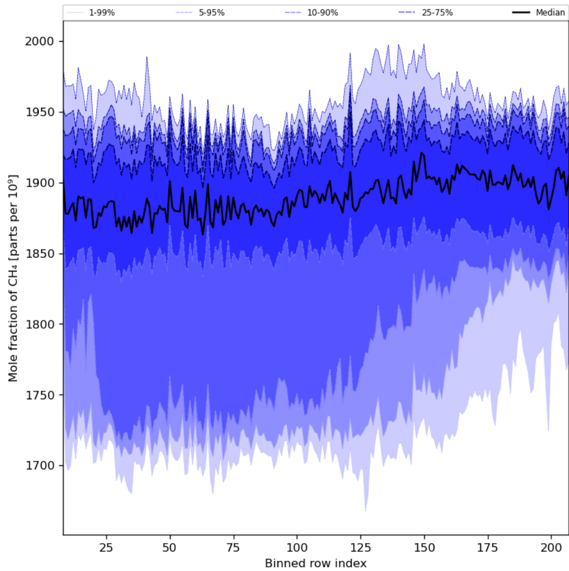
Figure 34: Along track statistics of “Mole fraction of CH 4 ” for 2023-10-06 to 2023-10-08
