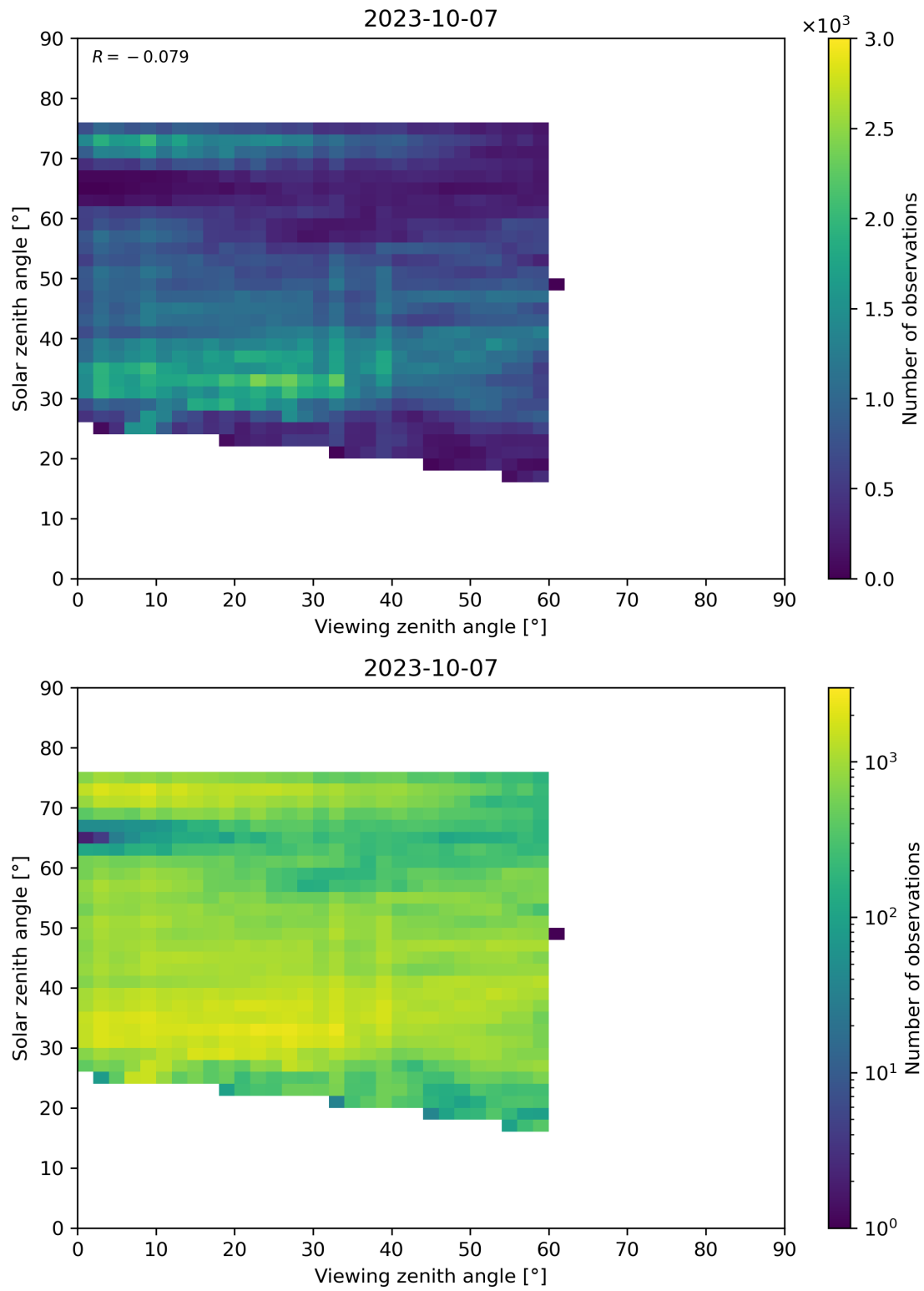
Figure 115: Scatter density plot of “Viewing zenith angle” against “Solar zenith angle” for 2023-10-06 to 2023-10-08.
