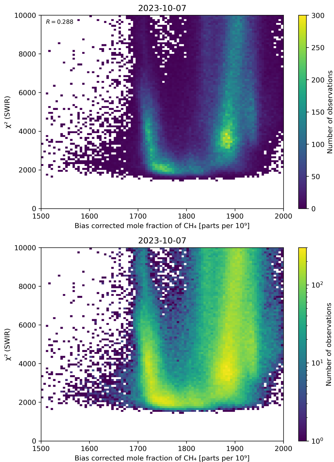
Figure 64: Scatter density plot of “Bias corrected mole fraction of CH 4 ” against “ \chi^2 (SWIR)” for 2023-10-06 to 2023-10-08.
