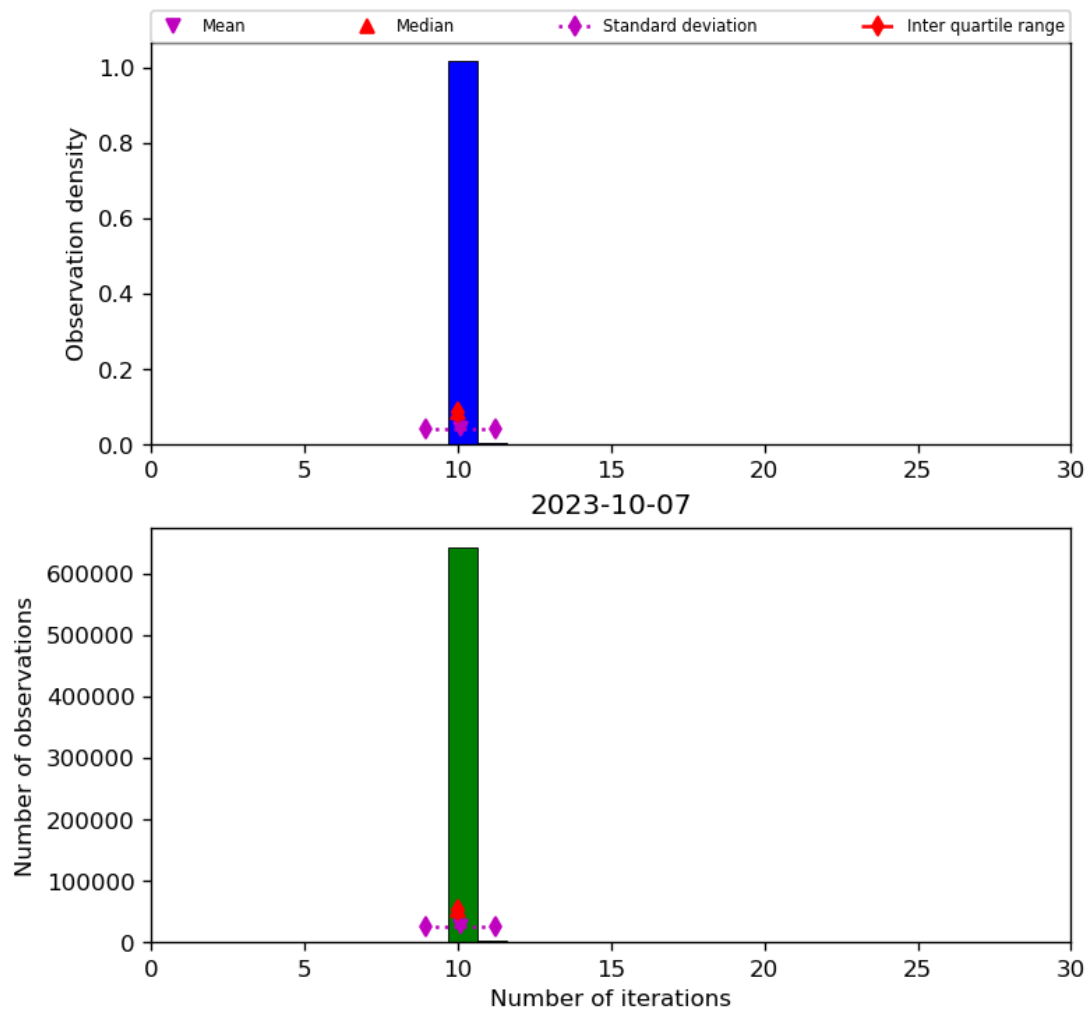
Figure 31: Histogram of “Number of iterations” for 2023-10-06 to 2023-10-08
