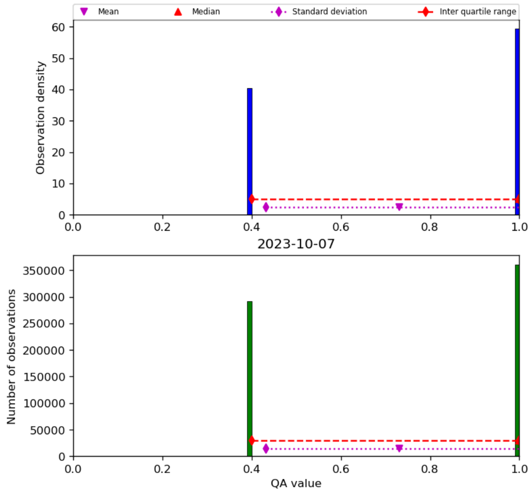
Figure 22: Histogram of “QA value” for 2023-10-06 to 2023-10-08
