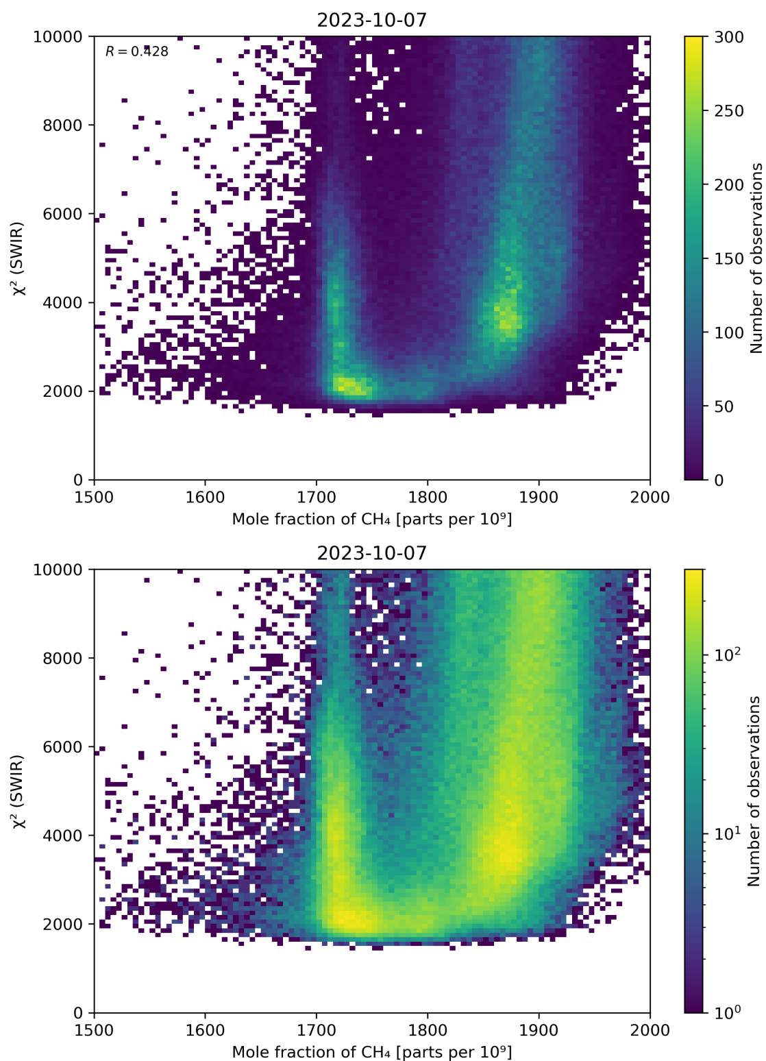
Figure 71: Scatter density plot of “Mole fraction of \text{CH}_4 ” against “ \chi^2 (SWIR)” for 2023-10-06 to 2023-10-08.
