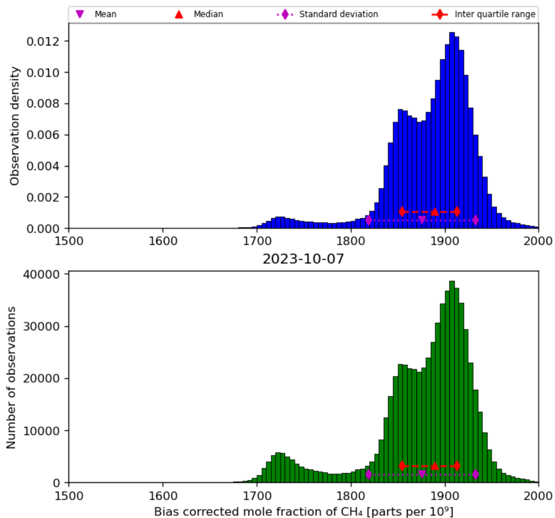
Figure 25: Histogram of “Bias corrected mole fraction of CH 4 ” for 2023-10-06 to 2023-10-08
