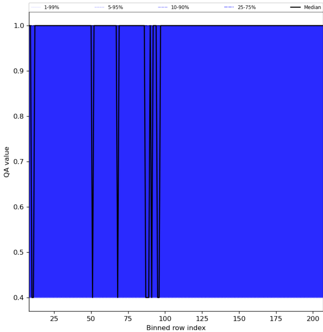
Figure 33: Along track statistics of “QA value” for 2023-10-06 to 2023-10-08
