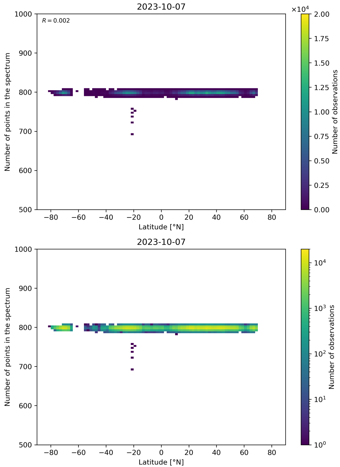
Figure 61: Scatter density plot of “Latitude” against “Number of points in the spectrum” for 2023-10-06 to 2023-10-08.
