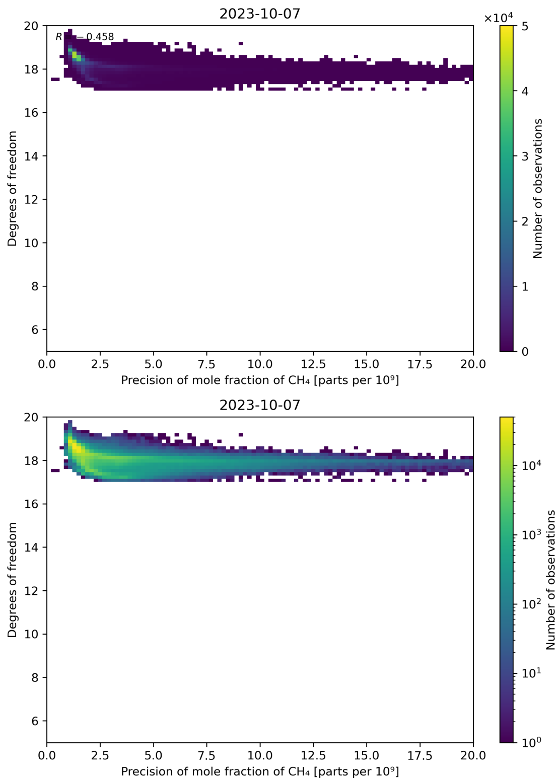
Figure 80: Scatter density plot of “Precision of mole fraction of CH 4 ” against “Degrees of freedom” for 2023-10-06 to 2023-10-08.
