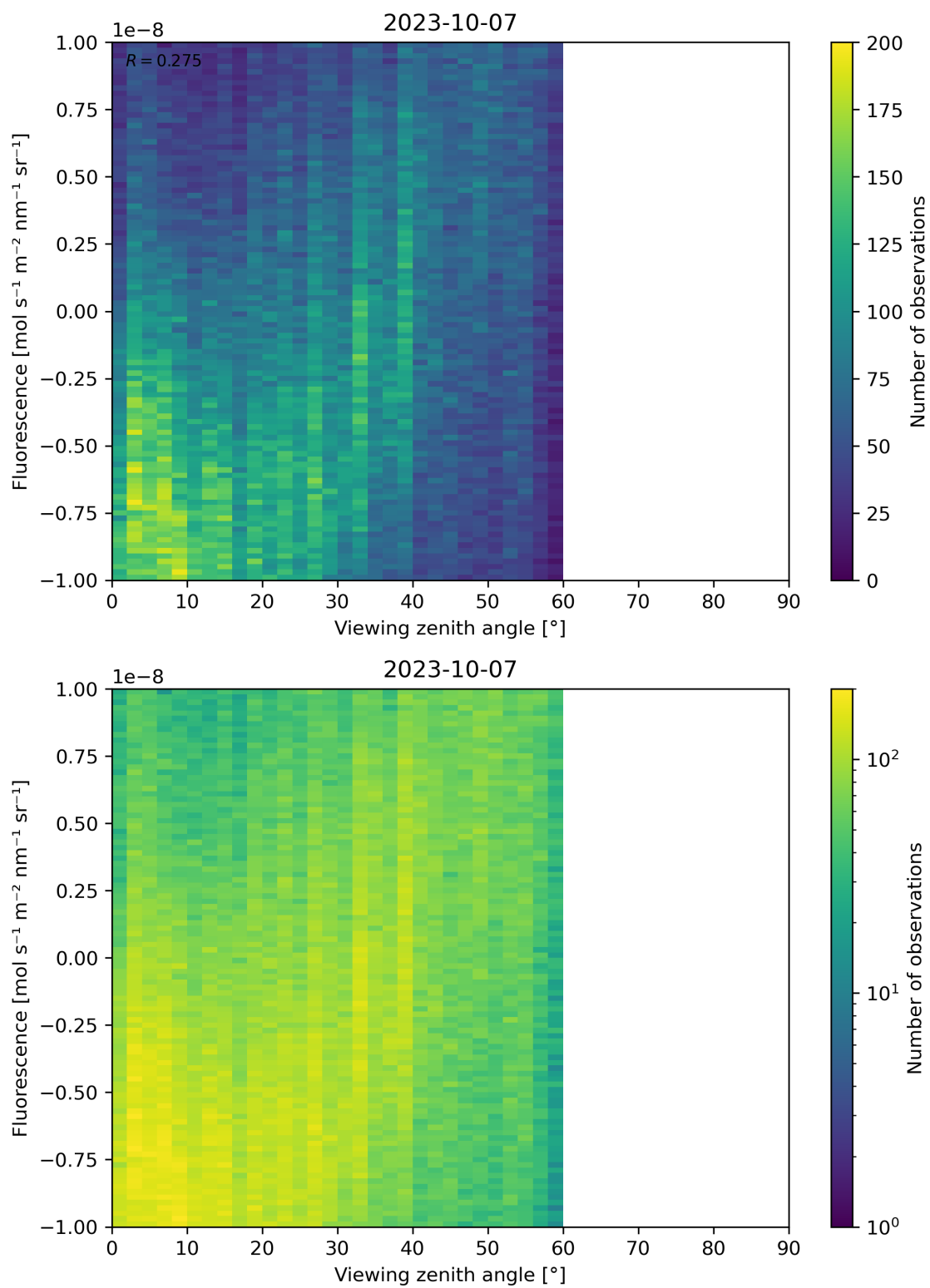
Figure 108: Scatter density plot of “Viewing zenith angle” against “Fluorescence” for 2023-10-06 to 2023-10-08.
