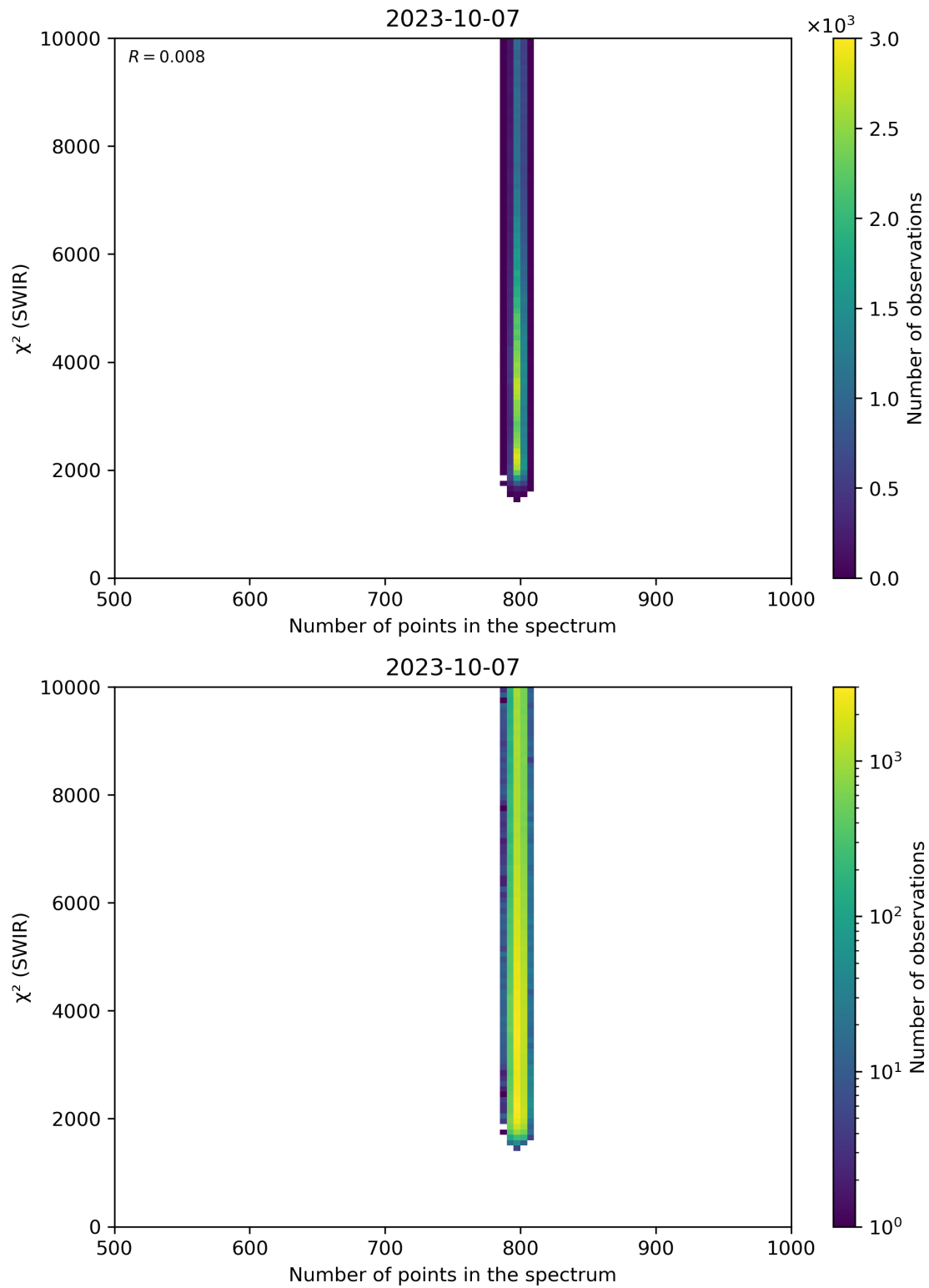
Figure 89: Scatter density plot of “Number of points in the spectrum” against “ \chi^2 (SWIR)” for 2023-10-06 to 2023-10-08.
