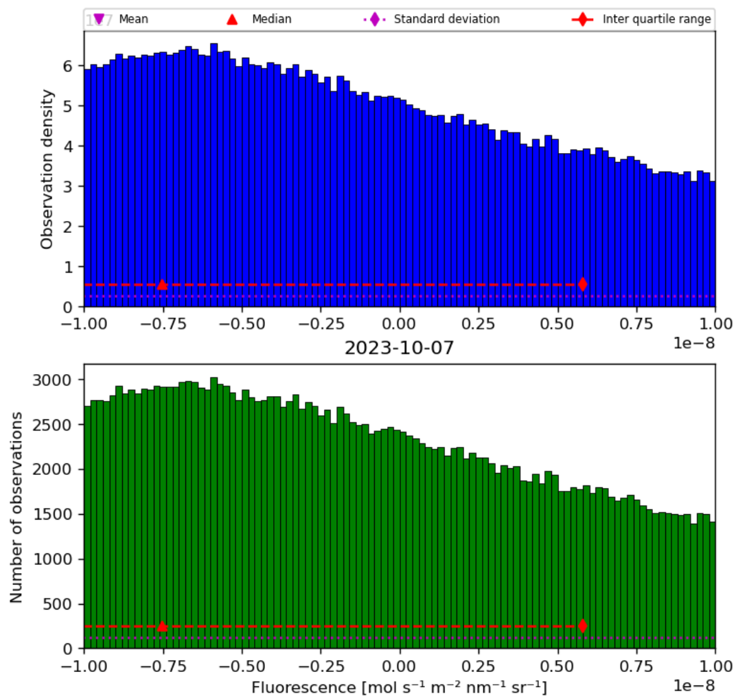
Figure 32: Histogram of “Fluorescence” for 2023-10-06 to 2023-10-08
