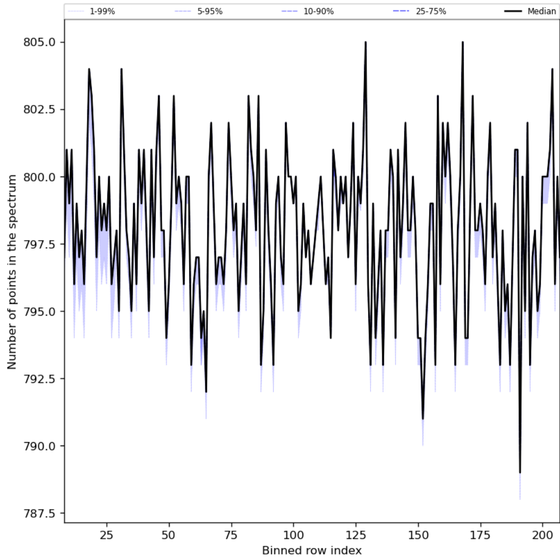
Figure 37: Along track statistics of “Number of points in the spectrum” for 2023-10-06 to 2023-10-08
