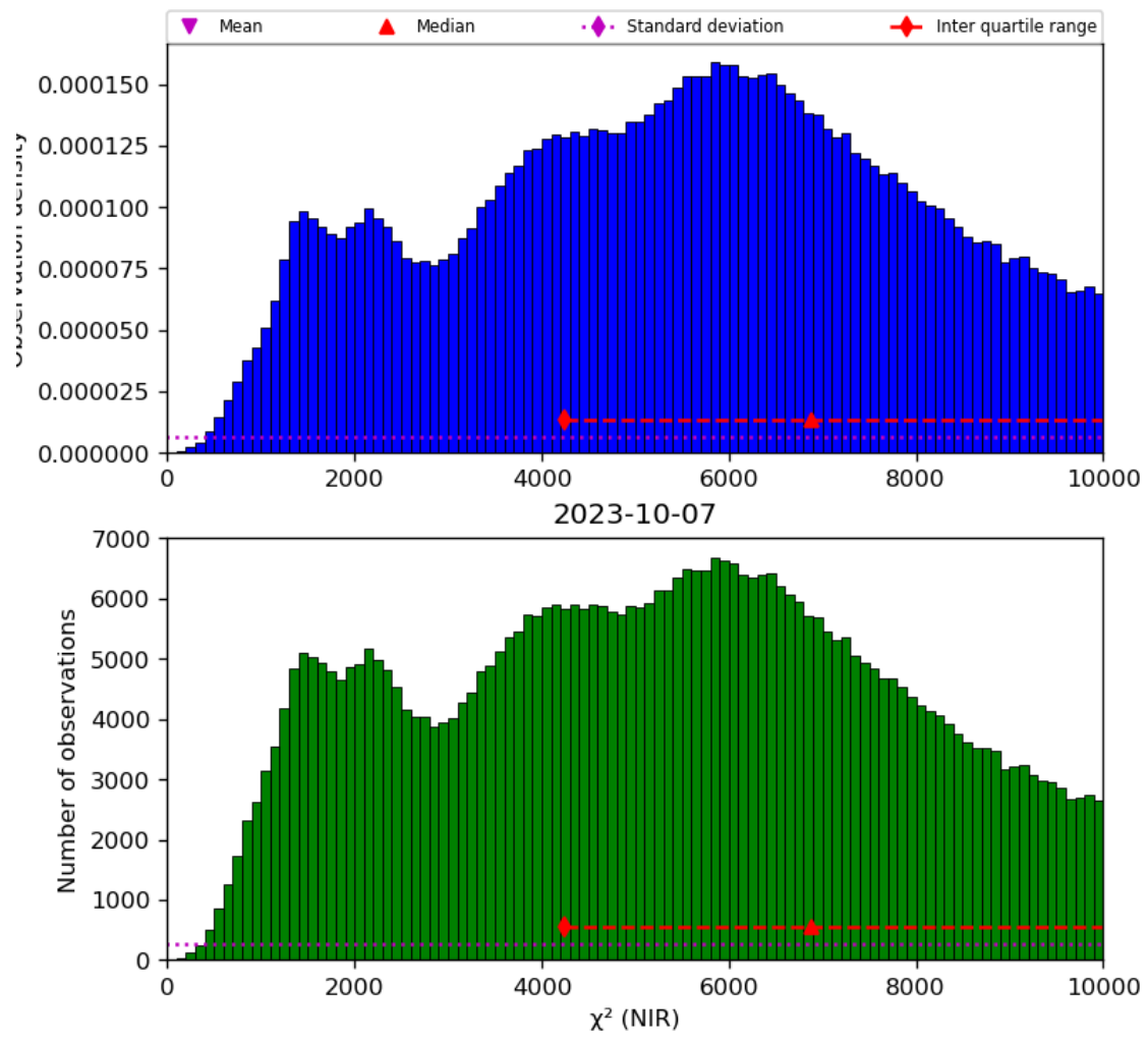
Figure 29: Histogram of “ \chi^2 (NIR)” for 2023-10-06 to 2023-10-08
