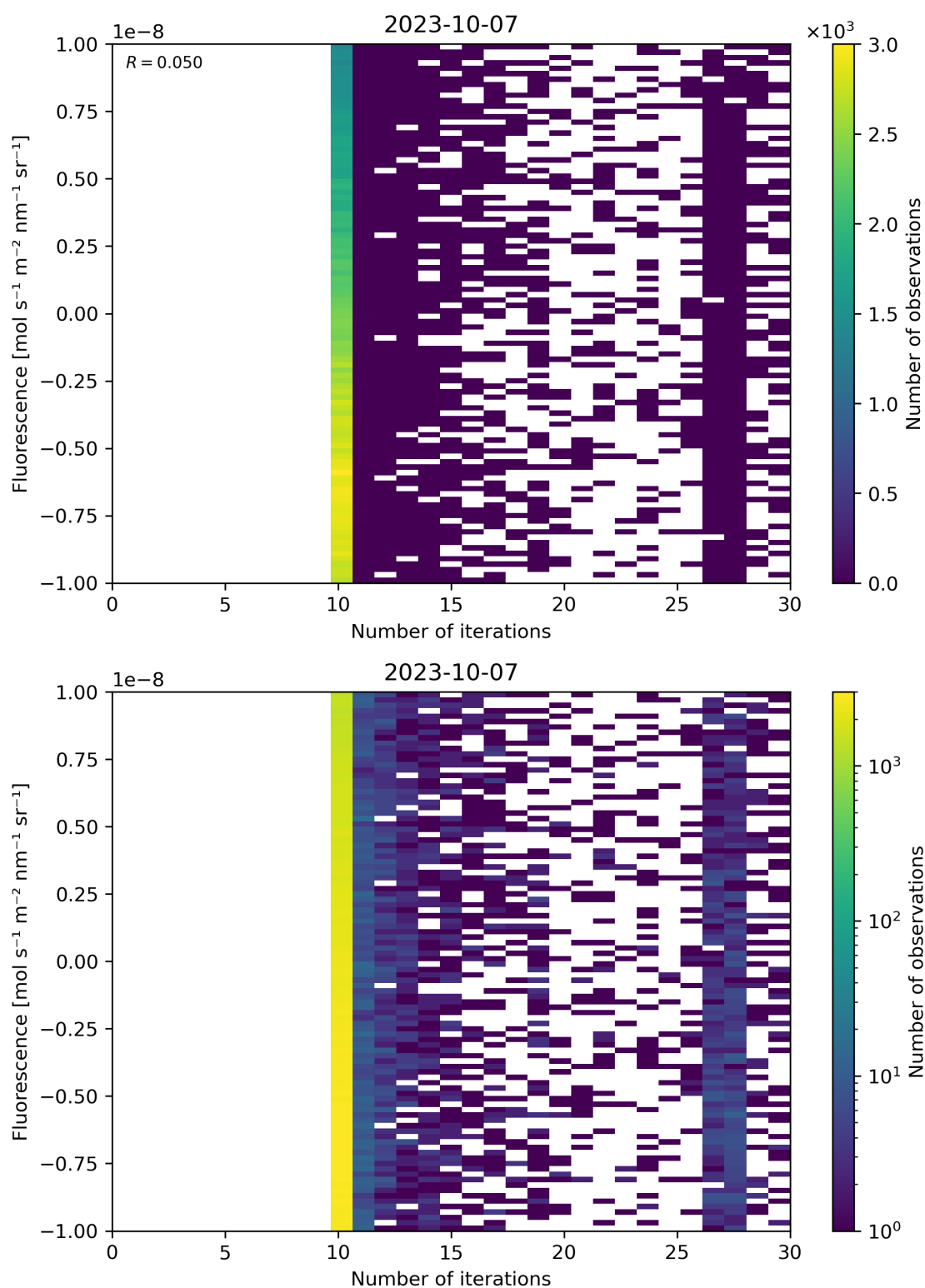
Figure 87: Scatter density plot of “Number of iterations” against “Fluorescence” for 2023-10-06 to 2023-10-08.
