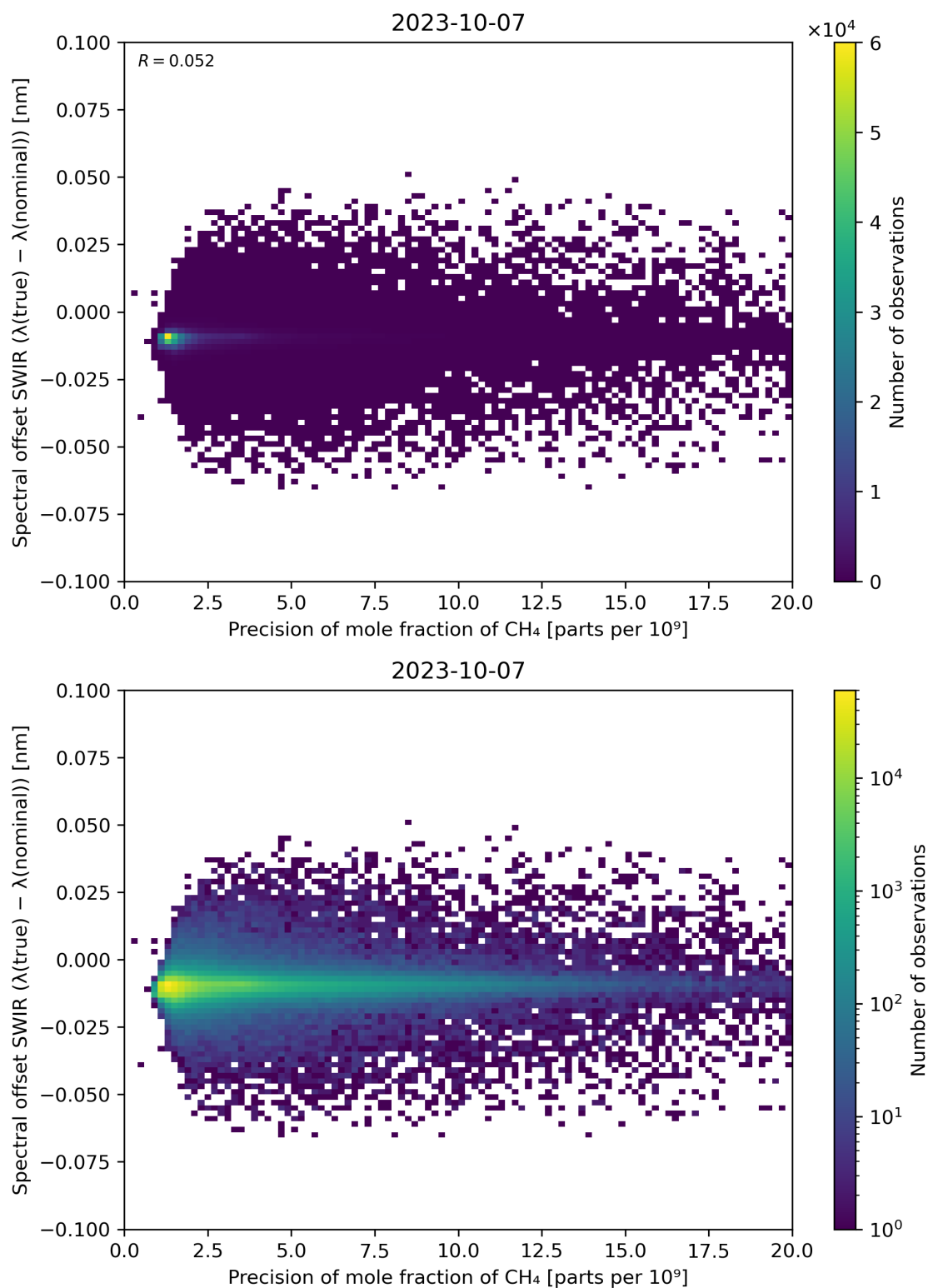
Figure 85: Scatter density plot of “Precision of mole fraction of CH 4 ” against “Spectral offset SWIR ( \lambda(\text{true}) - \lambda(\text{nominal}) )” for 2023-10-06 to 2023-10-08.
