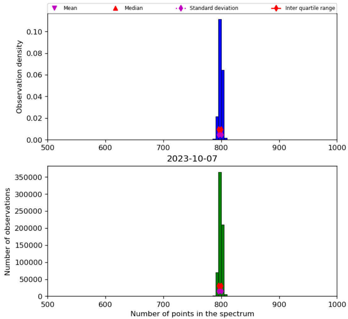
Figure 26: Histogram of “Number of points in the spectrum” for 2023-10-06 to 2023-10-08
