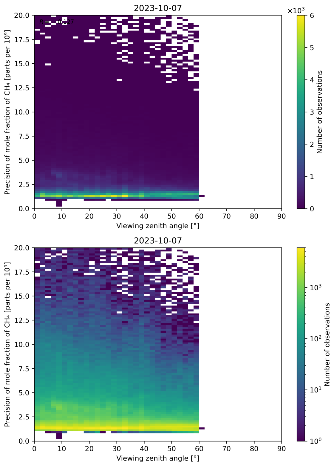
Figure 112: Scatter density plot of “Viewing zenith angle” against “Precision of mole fraction of CH 4 ” for 2023-10-06 to 2023-10-08.
