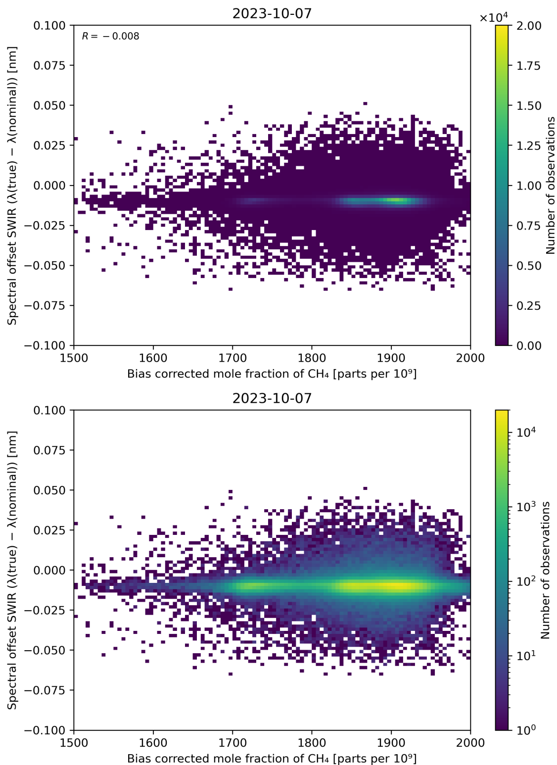
Figure 69: Scatter density plot of “Bias corrected mole fraction of \text{CH}_4 ” against “Spectral offset SWIR ( \lambda(\text{true}) - \lambda(\text{nominal}) )” for 2023-10-06 to 2023-10-08.
