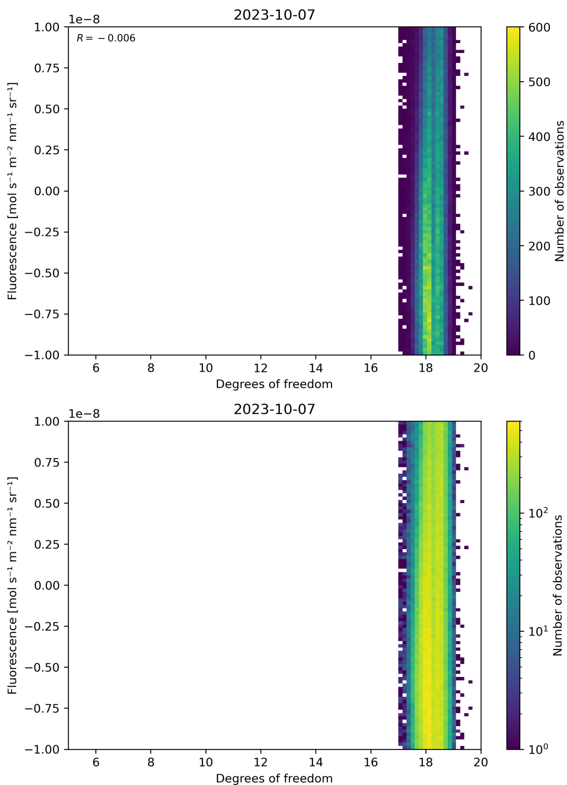
Figure 51: Scatter density plot of “Degrees of freedom” against “Fluorescence” for 2023-10-06 to 2023-10-08.
