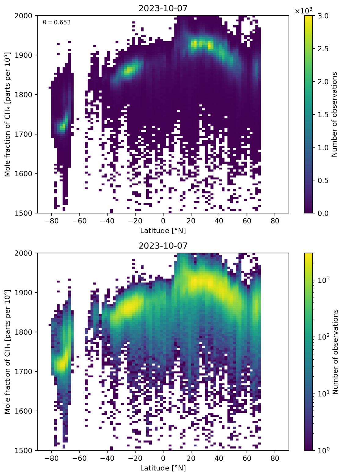
Figure 57: Scatter density plot of “Latitude” against “Mole fraction of CH 4 ” for 2023-10-06 to 2023-10-08.
