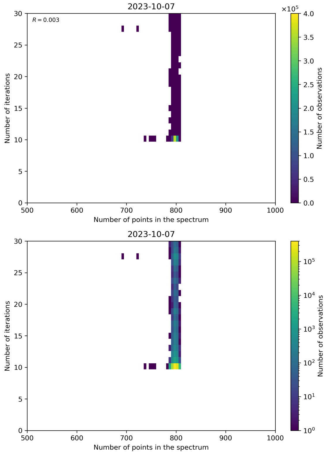
Figure 92: Scatter density plot of “Number of points in the spectrum” against “Number of iterations” for 2023-10-06 to 2023-10-08.
