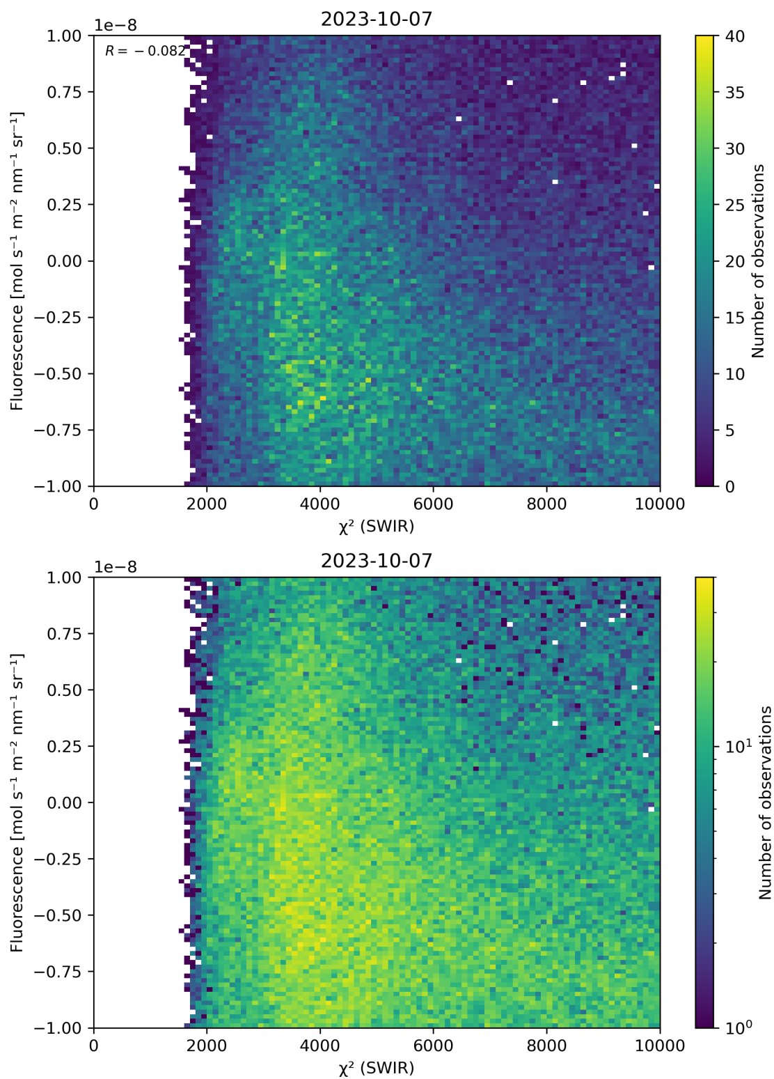
Figure 49: Scatter density plot of “ \chi^2 (SWIR)” against “Fluorescence” for 2023-10-06 to 2023-10-08.
