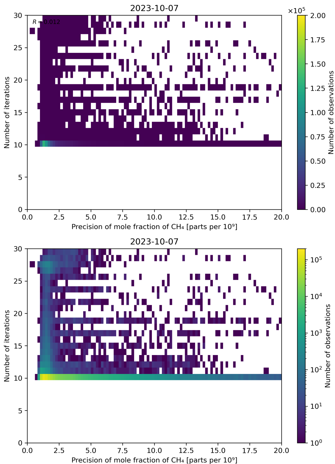
Figure 83: Scatter density plot of “Precision of mole fraction of CH 4 ” against “Number of iterations” for 2023-10-06 to 2023-10-08.
