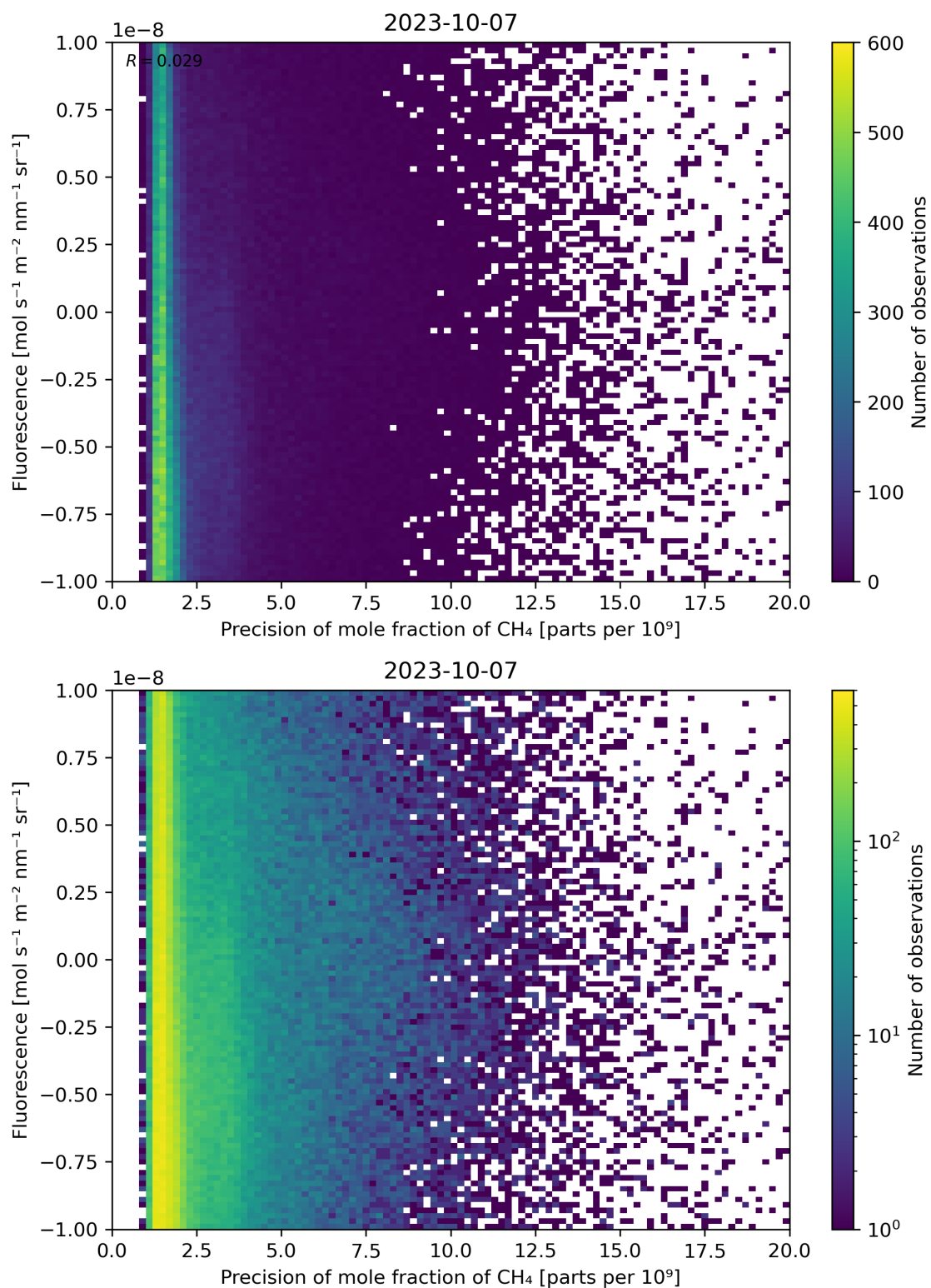
Figure 81: Scatter density plot of “Precision of mole fraction of \text{CH}_4 ” against “Fluorescence” for 2023-10-06 to 2023-10-08.
