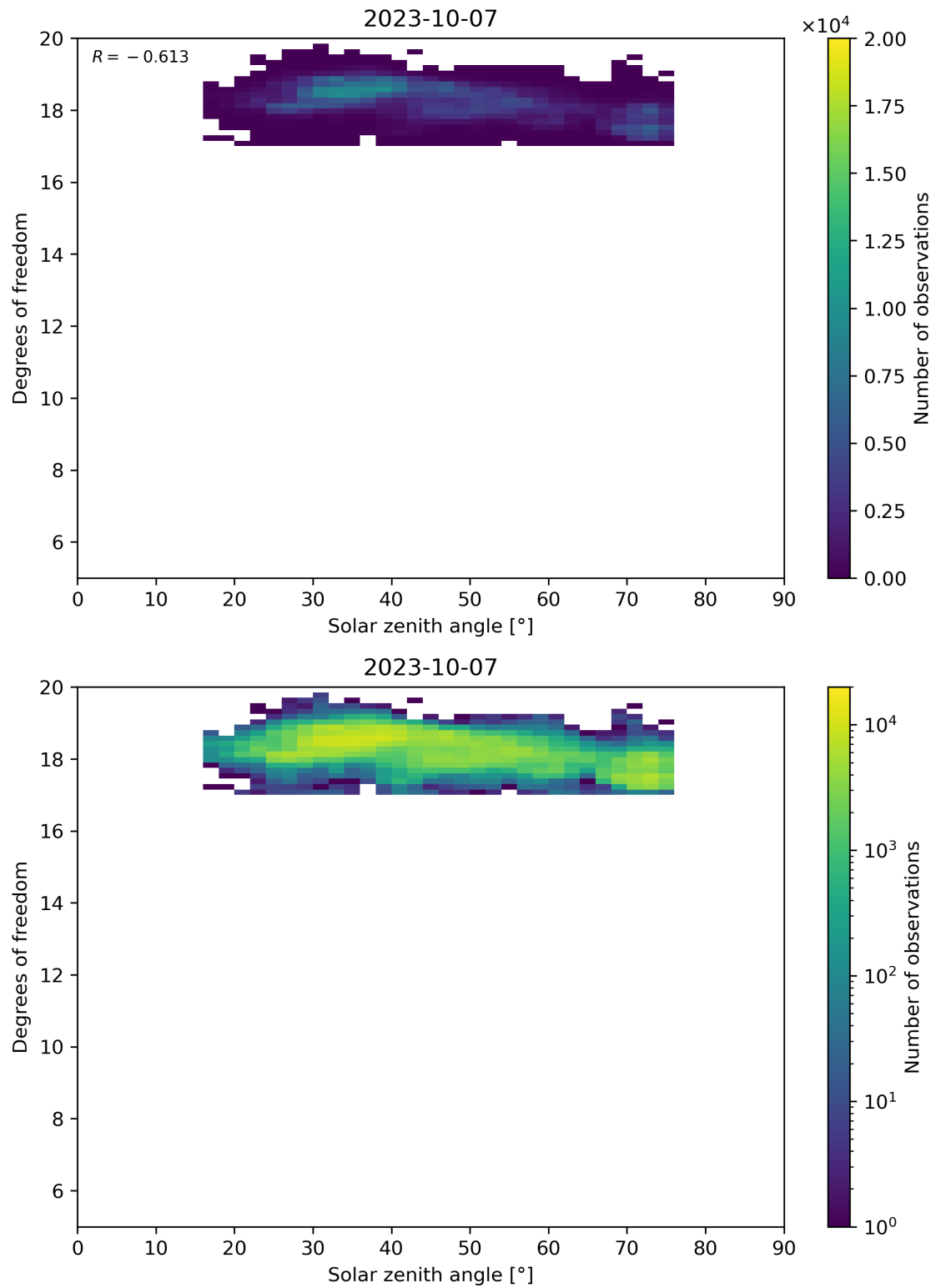
Figure 96: Scatter density plot of “Solar zenith angle” against “Degrees of freedom” for 2023-10-06 to 2023-10-08.
