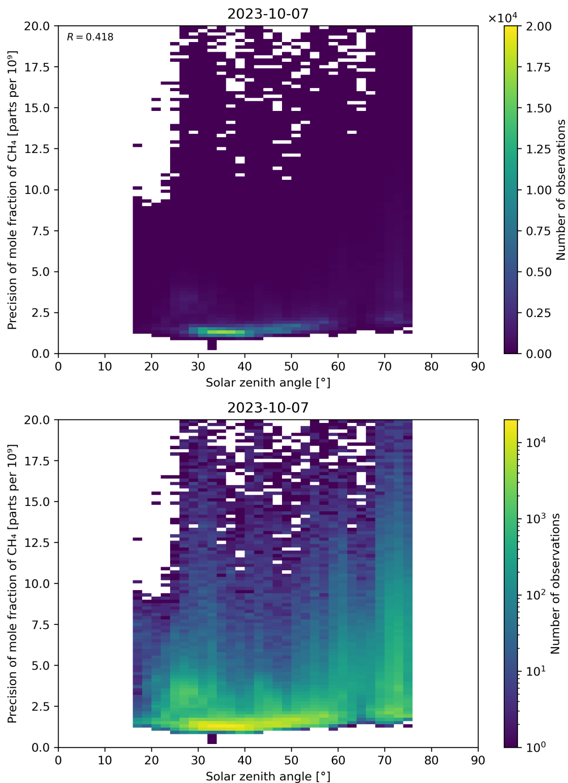
Figure 101: Scatter density plot of “Solar zenith angle” against “Precision of mole fraction of CH 4 ” for 2023-10-06 to 2023-10-08.
