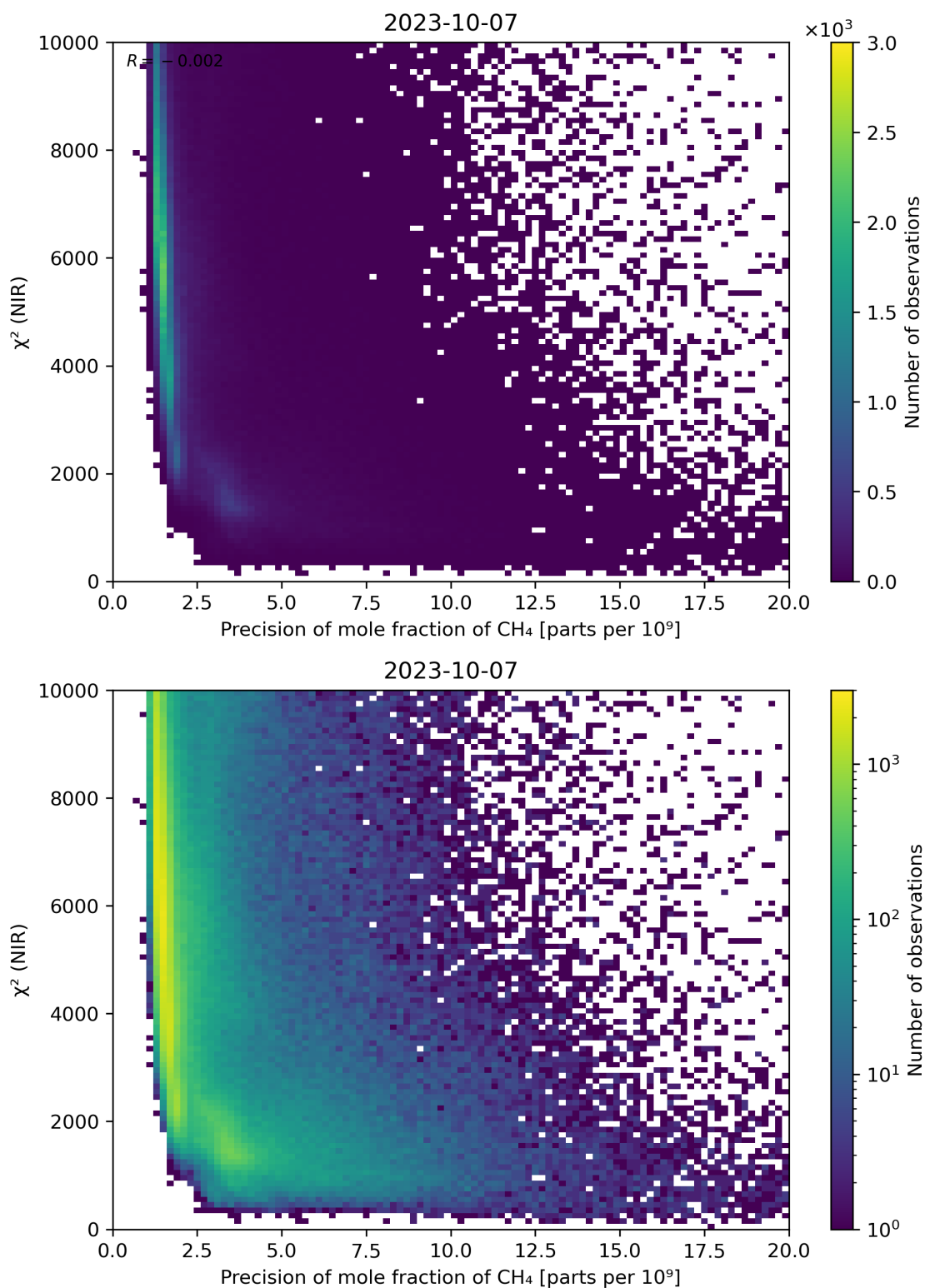
Figure 78: Scatter density plot of “Precision of mole fraction of CH 4 ” against “ \chi^2 (NIR)” for 2023-10-06 to 2023-10-08.
