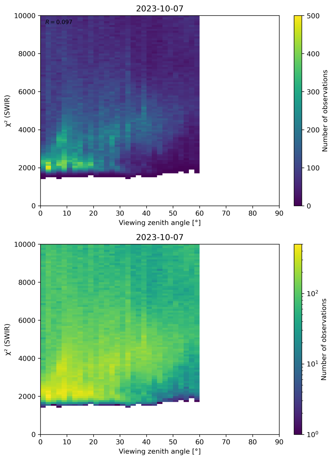
Figure 106: Scatter density plot of “Viewing zenith angle” against “ \chi^2 (SWIR)” for 2023-10-06 to 2023-10-08.
