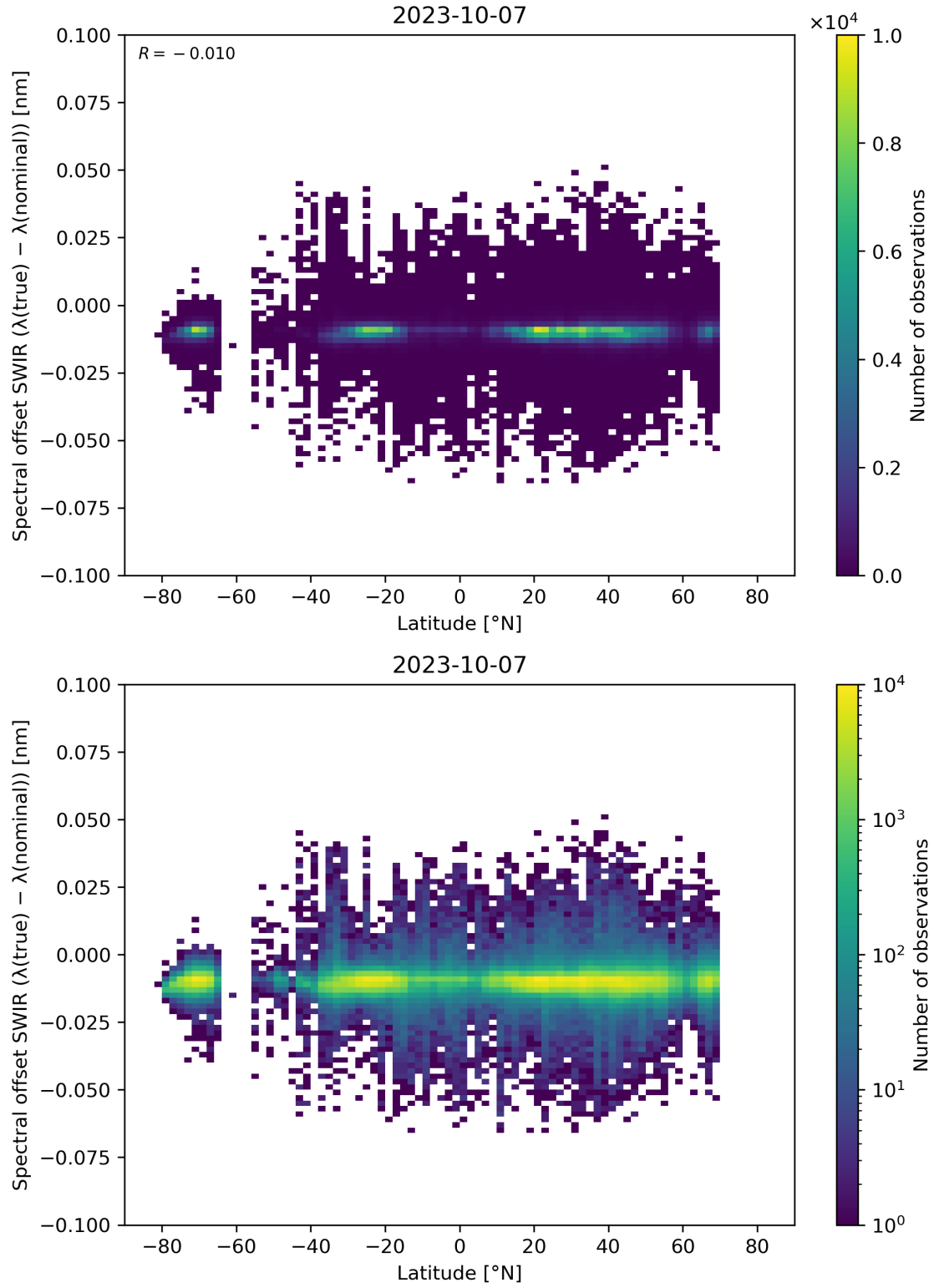
Figure 62: Scatter density plot of “Latitude” against “Spectral offset SWIR ( \lambda(\text{true}) - \lambda(\text{nominal}) )” for 2023-10-06 to 2023-10-08.
