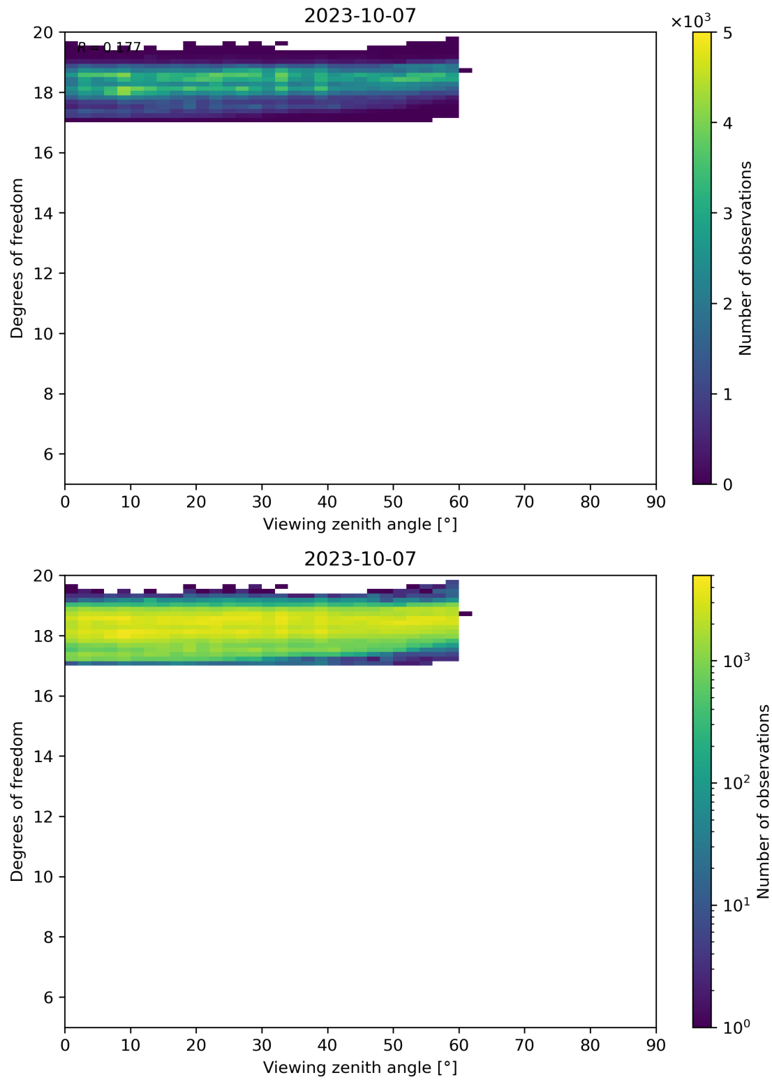
Figure 107: Scatter density plot of “Viewing zenith angle” against “Degrees of freedom” for 2023-10-06 to 2023-10-08.
