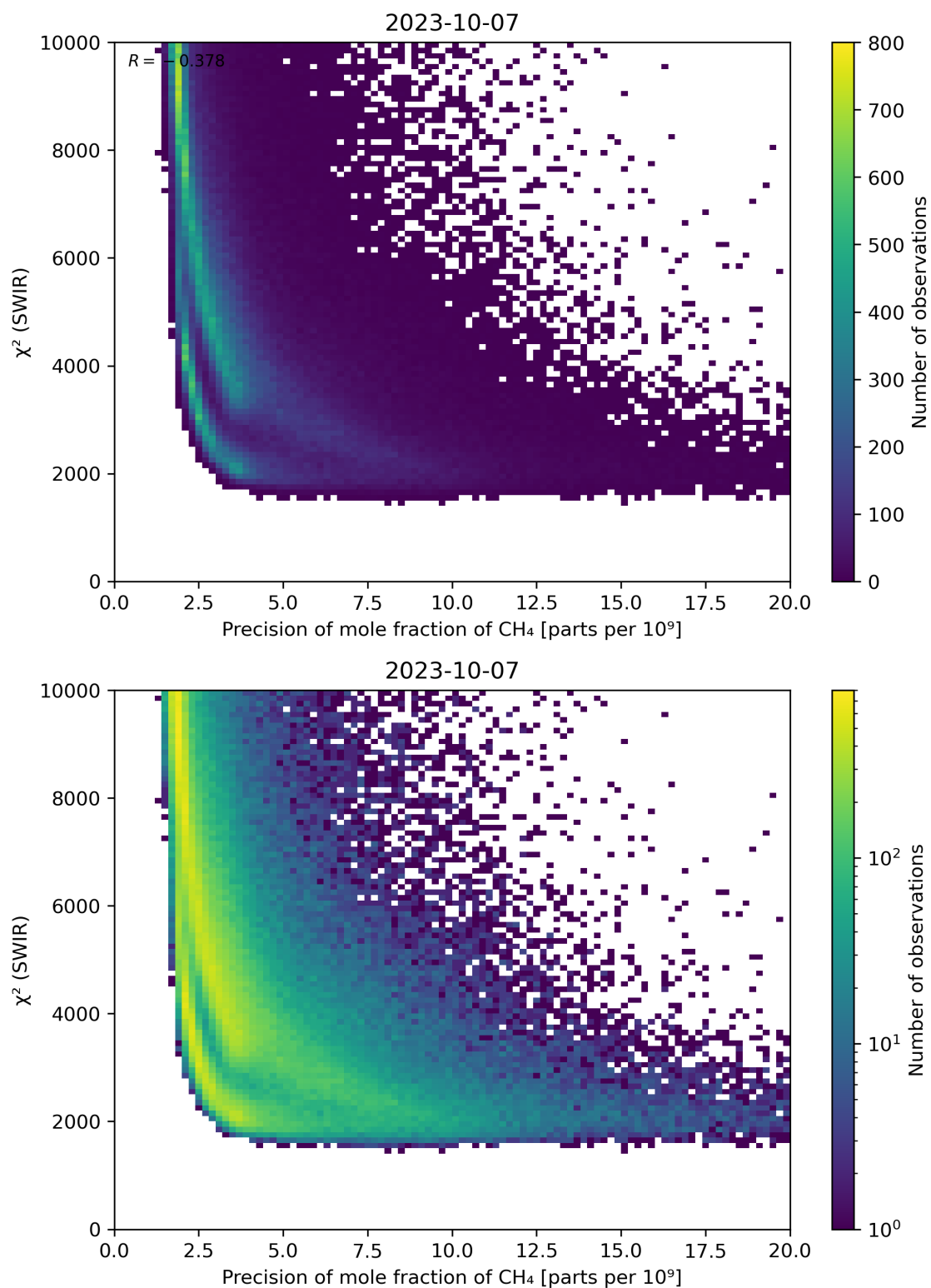
Figure 79: Scatter density plot of “Precision of mole fraction of CH 4 ” against “ \chi^2 (SWIR)” for 2023-10-06 to 2023-10-08.
