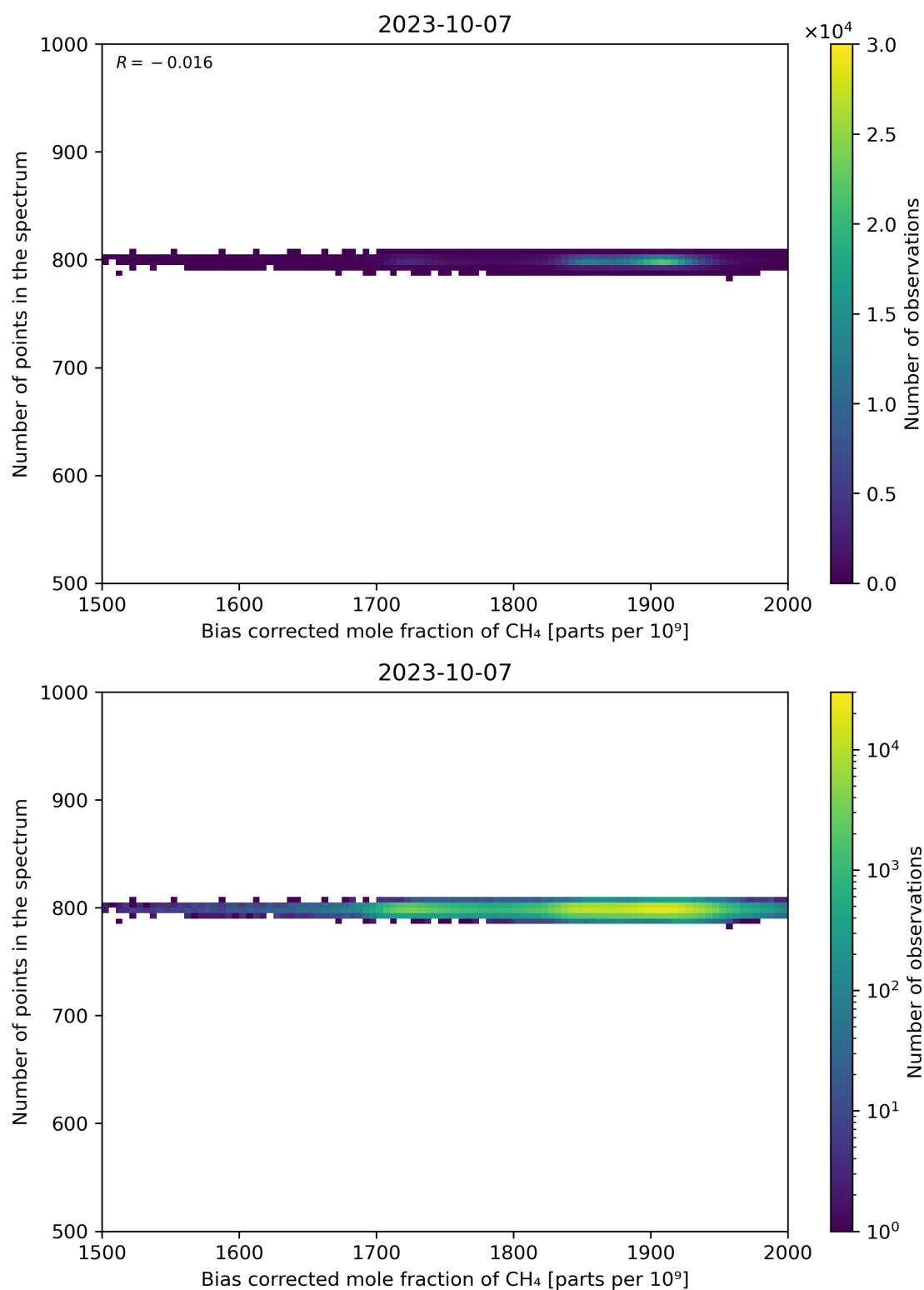
Figure 68: Scatter density plot of “Bias corrected mole fraction of CH 4 ” against “Number of points in the spectrum” for 2023-10-06 to 2023-10-08.
