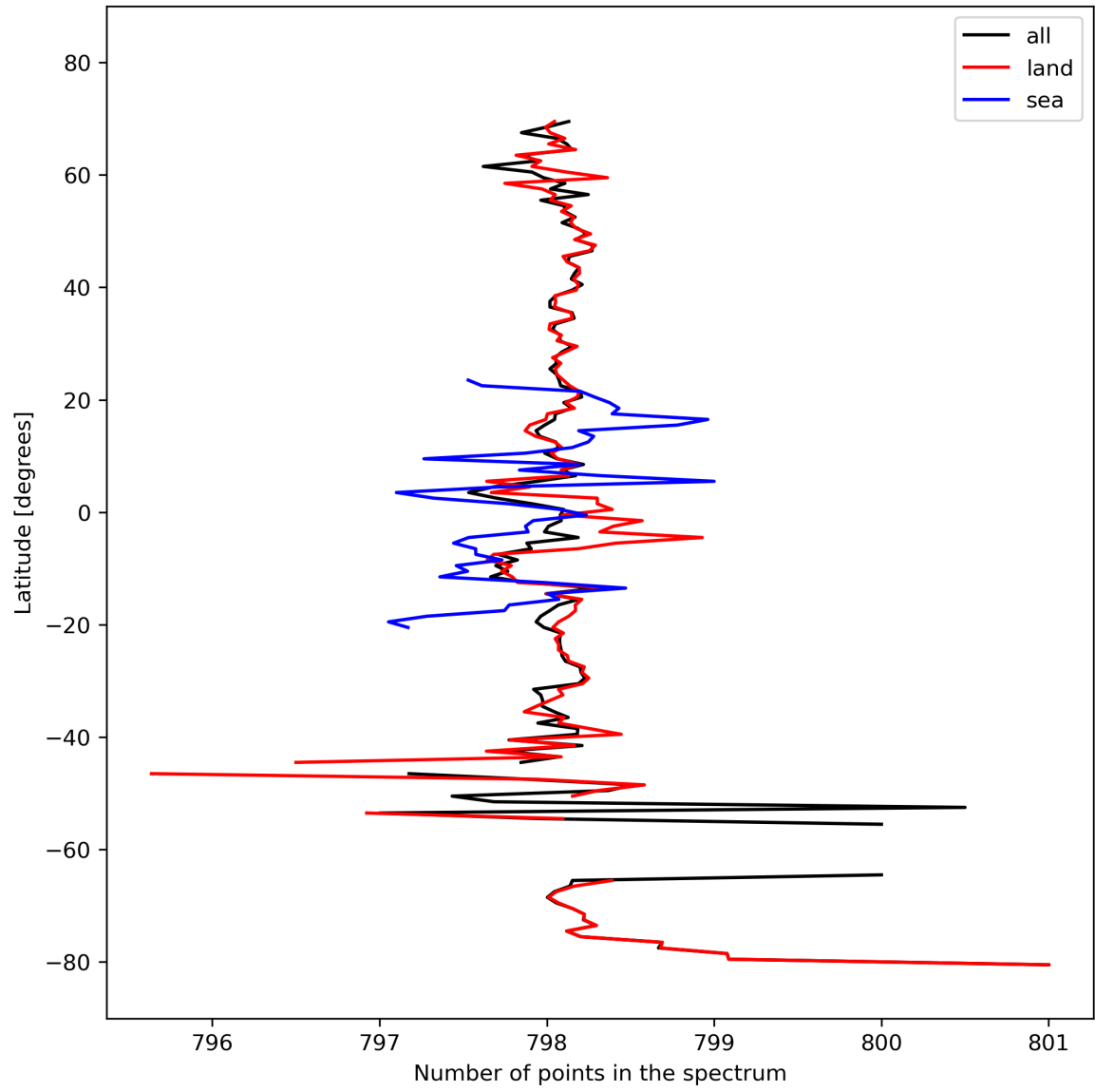
Figure 15: Zonal average of “Number of points in the spectrum” for 2023-10-06 to 2023-10-08.
