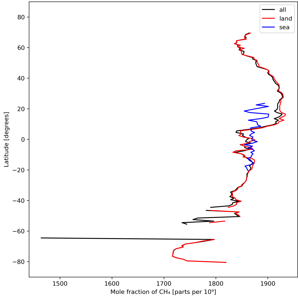
Figure 12: Zonal average of “Mole fraction of \text{CH}_4 ” for 2023-10-06 to 2023-10-08.
