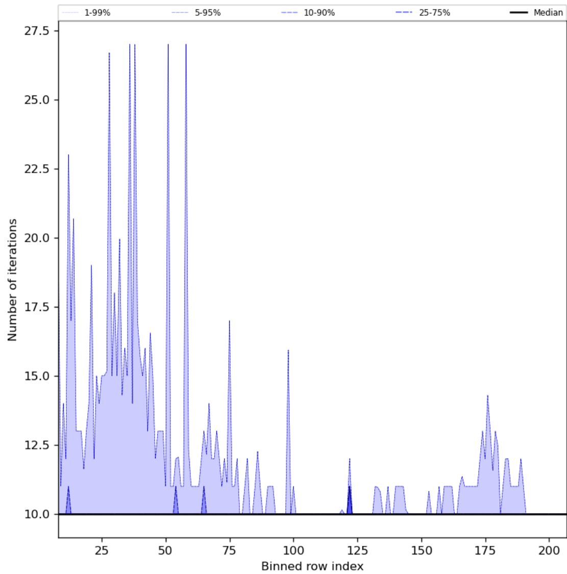
Figure 42: Along track statistics of “Number of iterations” for 2023-10-06 to 2023-10-08
