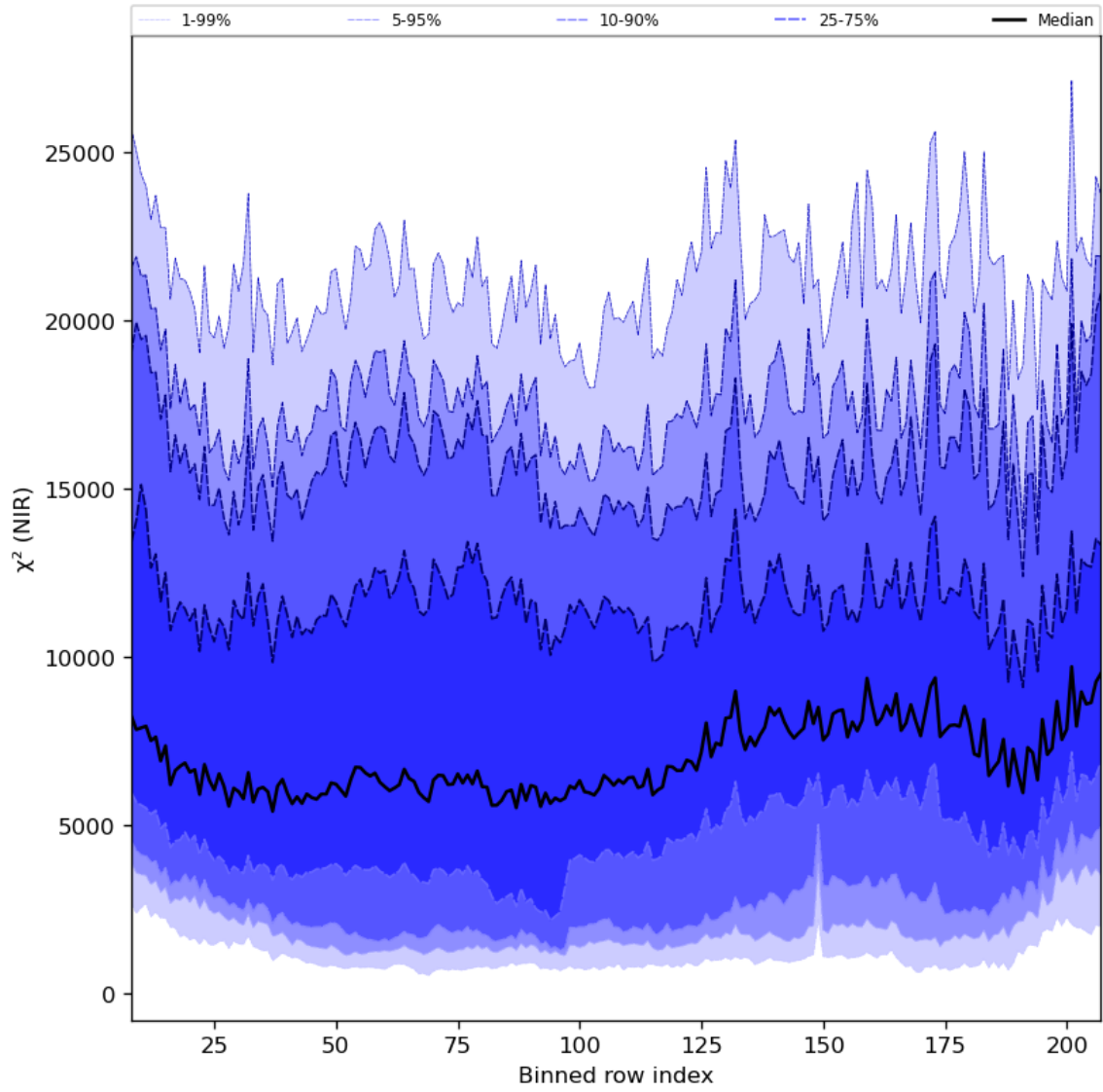
Figure 40: Along track statistics of “ \chi^2 (NIR)” for 2023-10-06 to 2023-10-08
