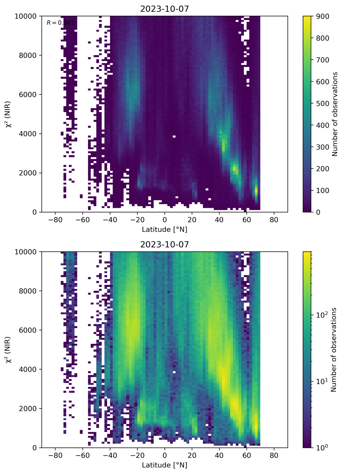
Figure 53: Scatter density plot of “Latitude” against “ \chi^2 (NIR)” for 2023-10-06 to 2023-10-08.
