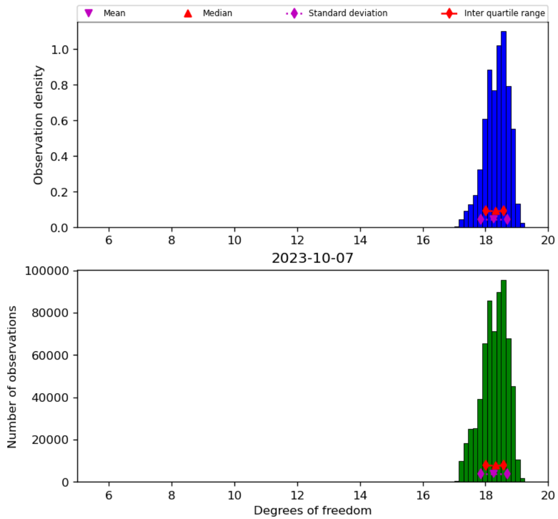
Figure 30: Histogram of “Degrees of freedom” for 2023-10-06 to 2023-10-08
