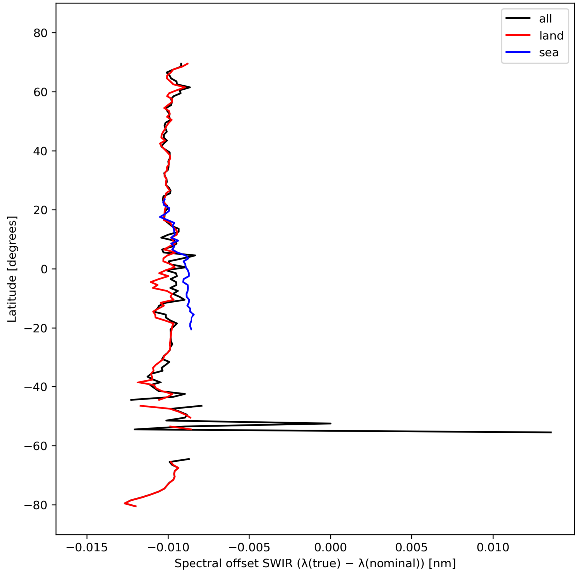
Figure 16: Zonal average of “Spectral offset SWIR ( \lambda(\text{true}) - \lambda(\text{nominal}) )” for 2023-10-06 to 2023-10-08.
