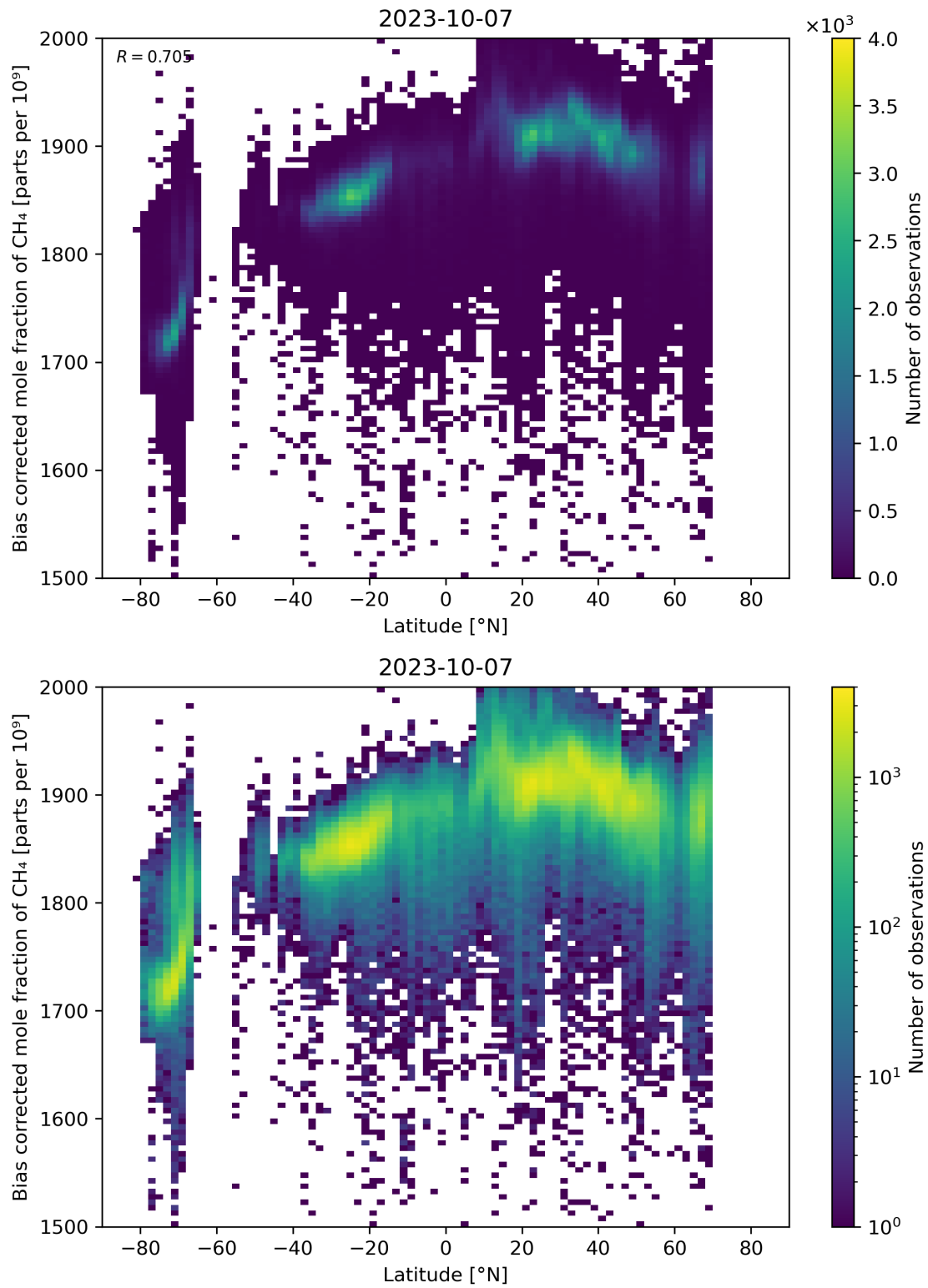
Figure 58: Scatter density plot of “Latitude” against “Bias corrected mole fraction of CH 4 ” for 2023-10-06 to 2023-10-08.
