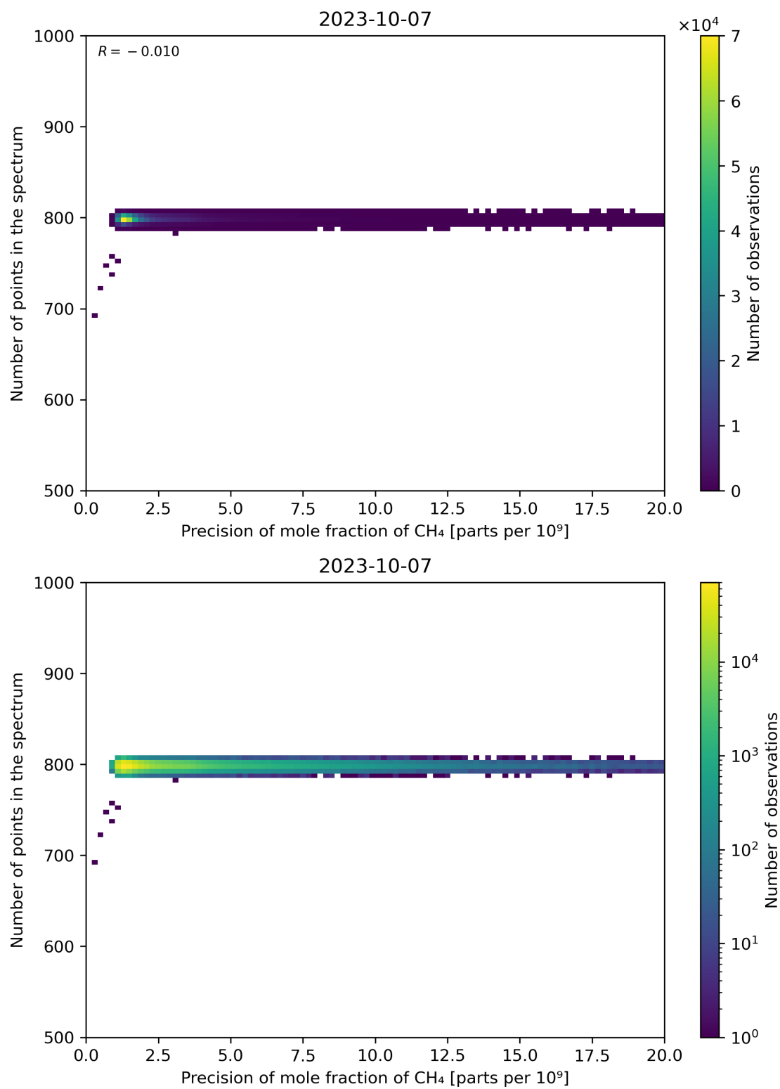
Figure 84: Scatter density plot of “Precision of mole fraction of CH 4 ” against “Number of points in the spectrum” for 2023-10-06 to 2023-10-08.
