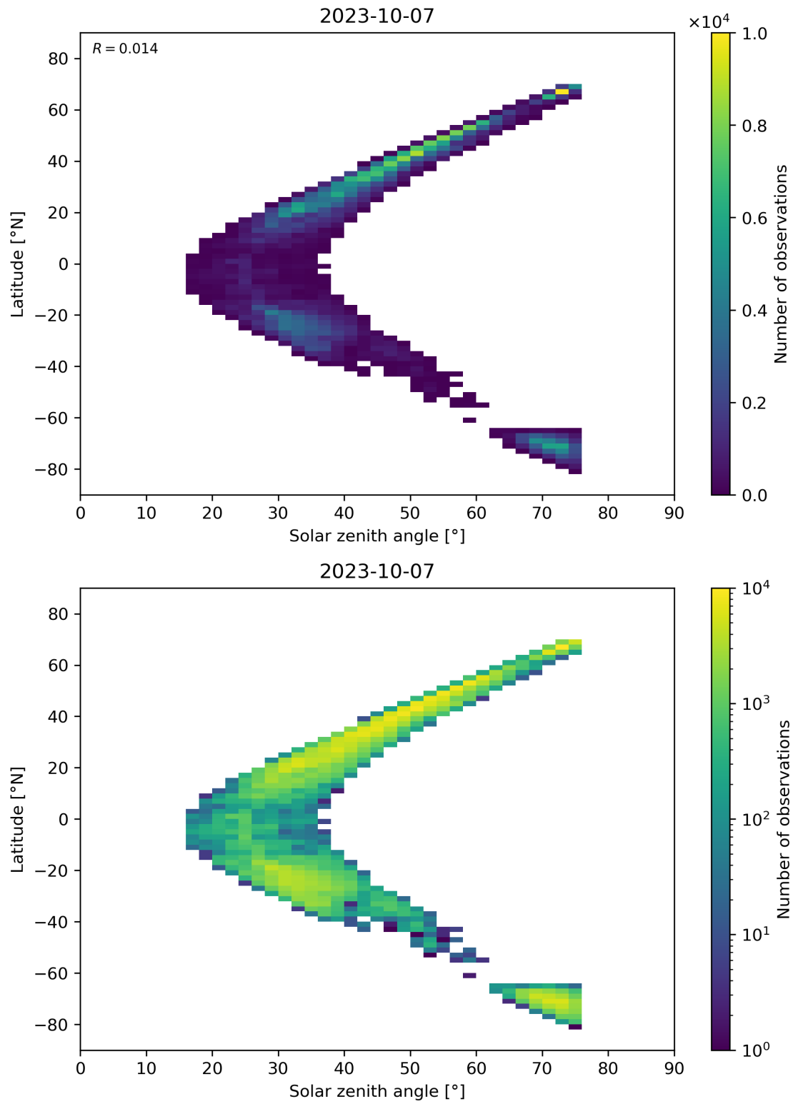
Figure 98: Scatter density plot of “Solar zenith angle” against “Latitude” for 2023-10-06 to 2023-10-08.
