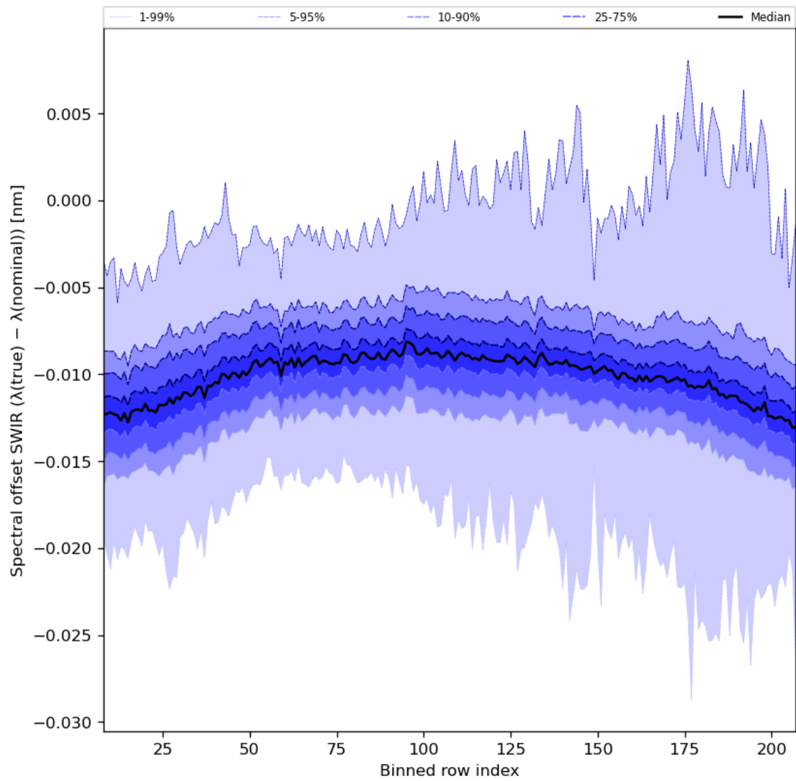
Figure 38: Along track statistics of “Spectral offset SWIR ( \lambda(\text{true}) - \lambda(\text{nominal}) )” for 2023-10-06 to 2023-10-08
