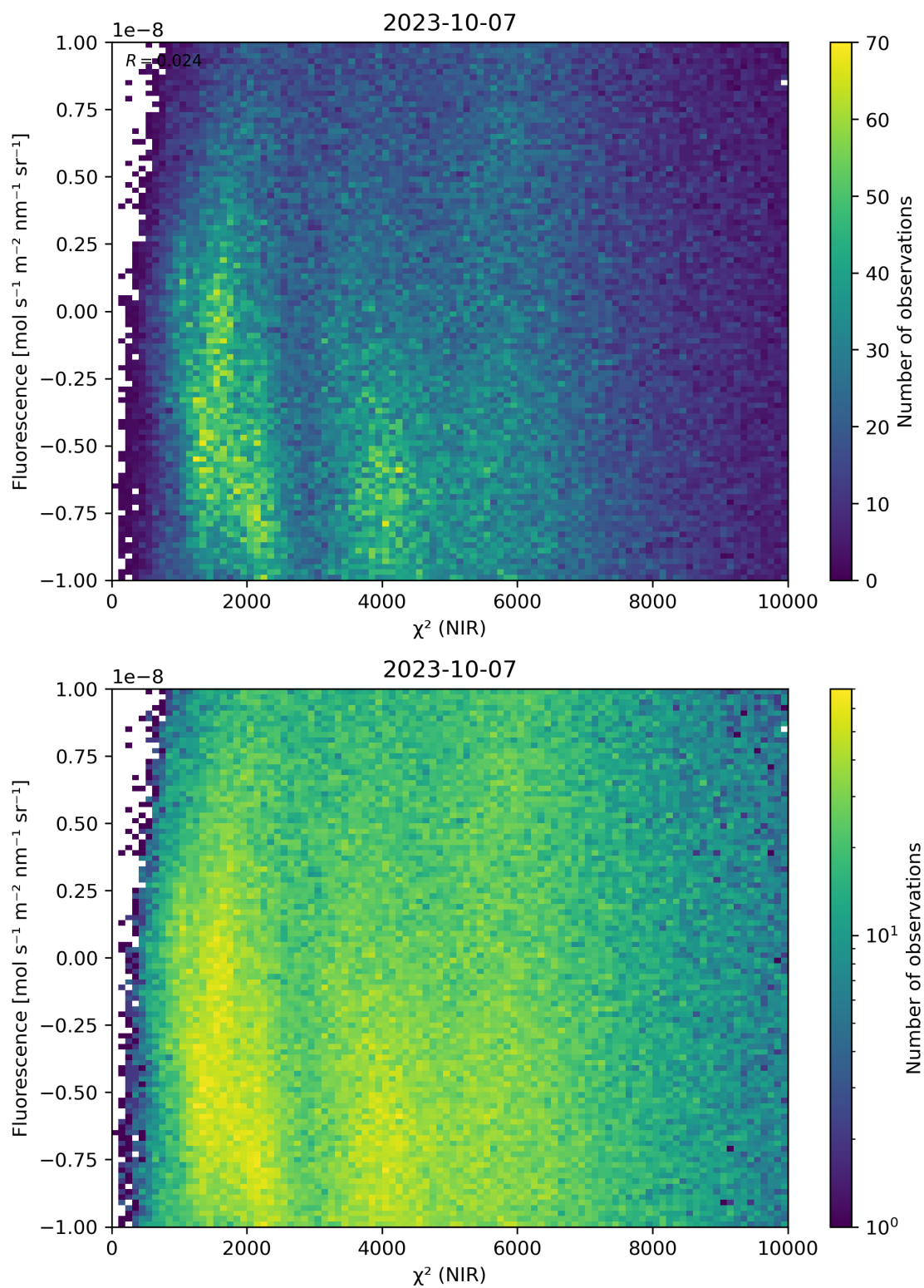
Figure 45: Scatter density plot of “ \chi^2 (NIR)” against “Fluorescence” for 2023-10-06 to 2023-10-08.
