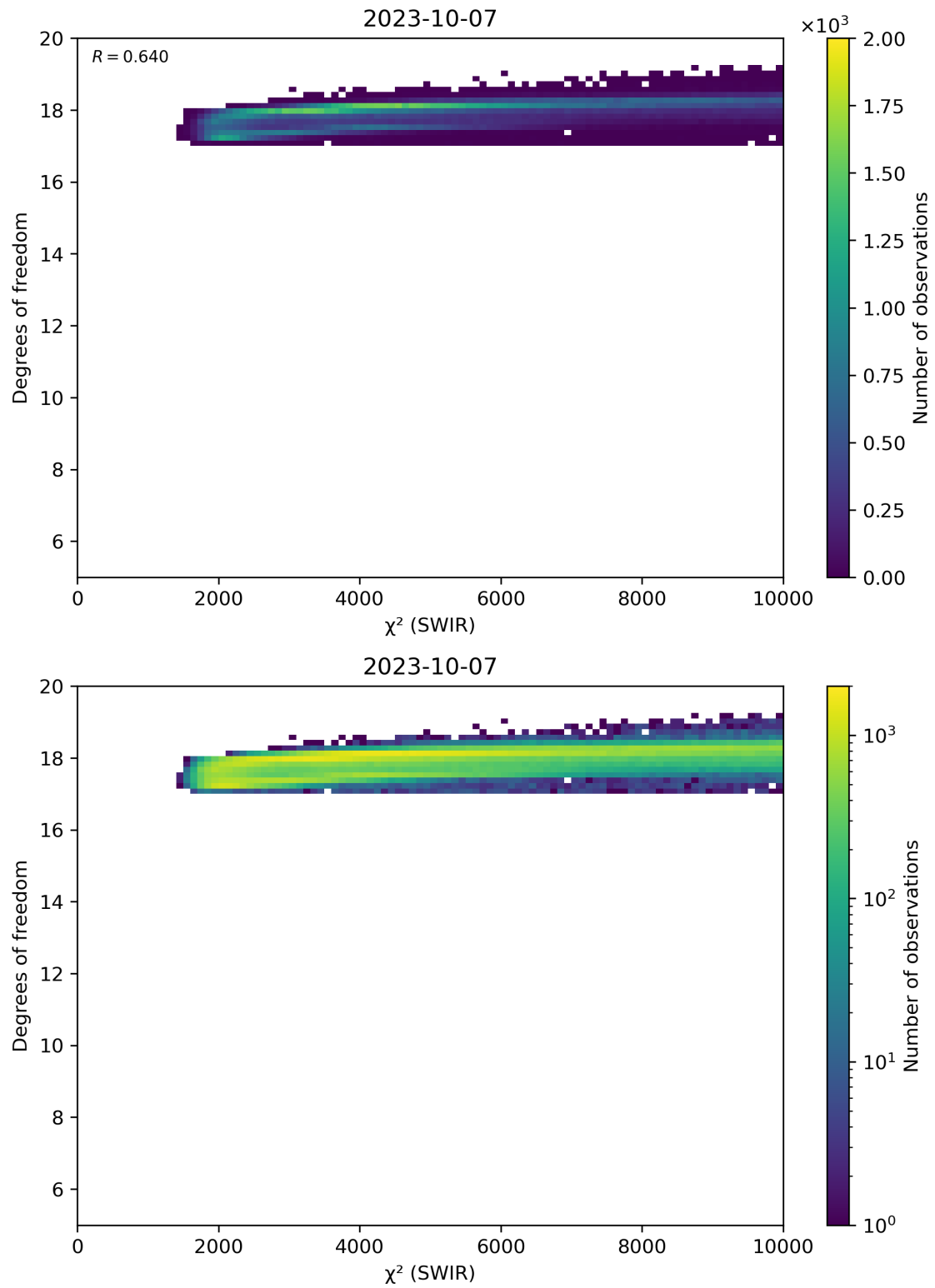
Figure 48: Scatter density plot of “ \chi^2 (SWIR)” against “Degrees of freedom” for 2023-10-06 to 2023-10-08.
