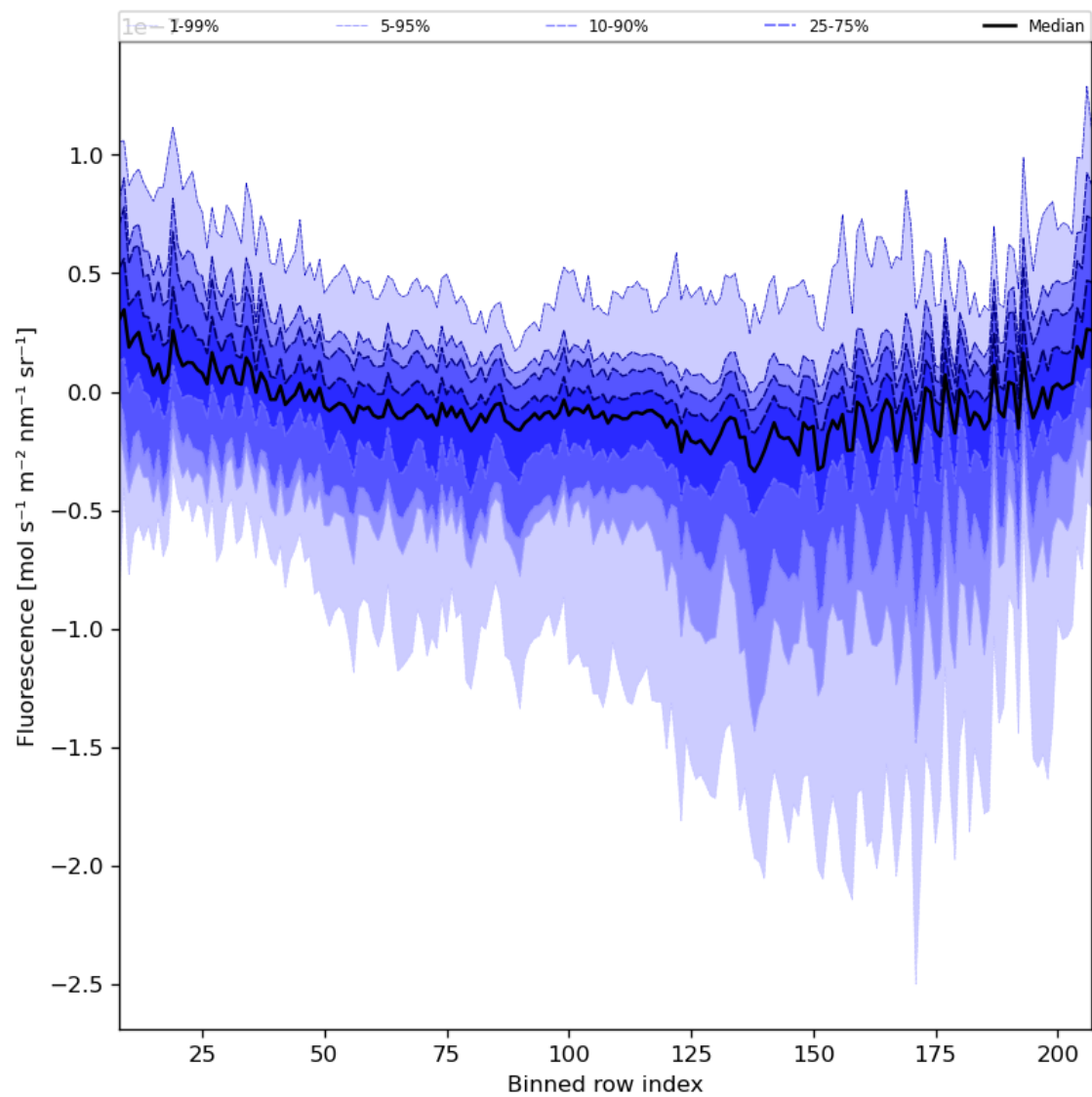
Figure 43: Along track statistics of “Fluorescence” for 2023-10-06 to 2023-10-08
