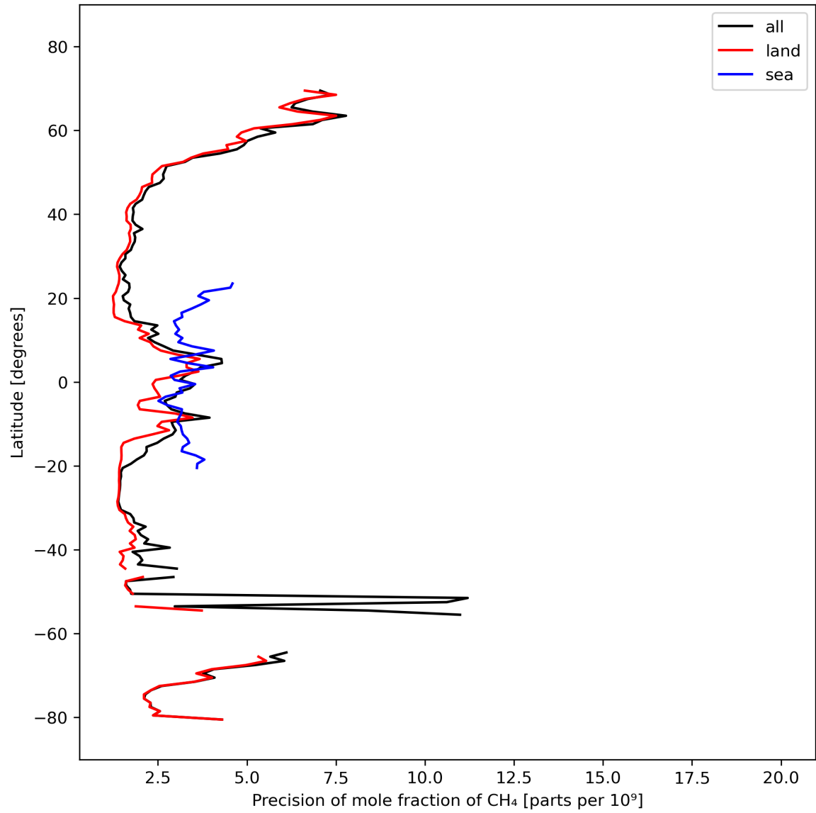
Figure 13: Zonal average of “Precision of mole fraction of CH 4 ” for 2023-10-06 to 2023-10-08.
