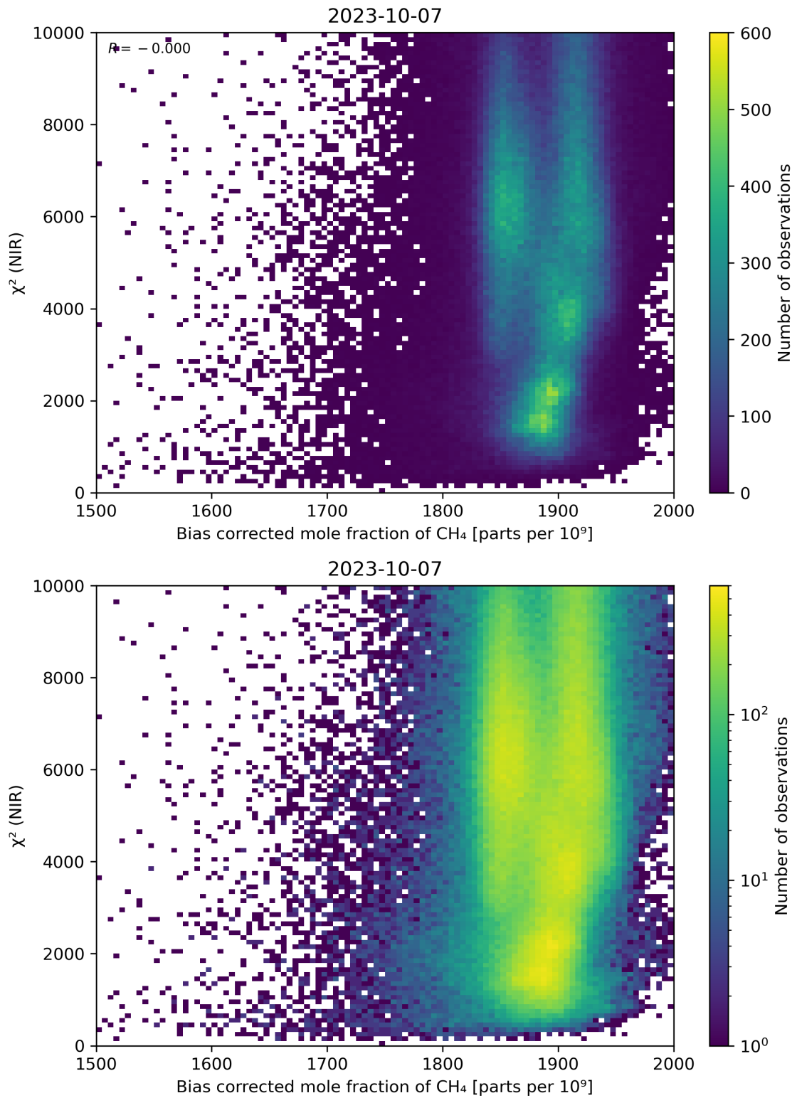
Figure 63: Scatter density plot of “Bias corrected mole fraction of CH 4 ” against “ \chi^2 (NIR)” for 2023-10-06 to 2023-10-08.
