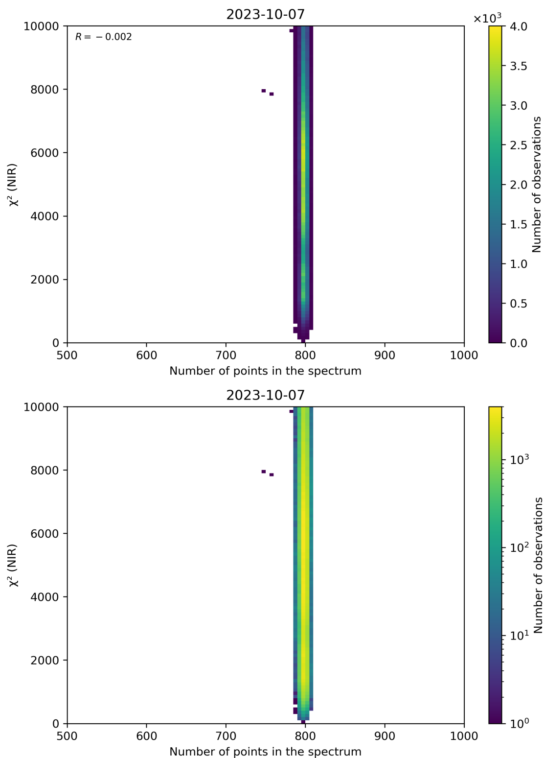
Figure 88: Scatter density plot of “Number of points in the spectrum” against “ \chi^2 (NIR)” for 2023-10-06 to 2023-10-08.
