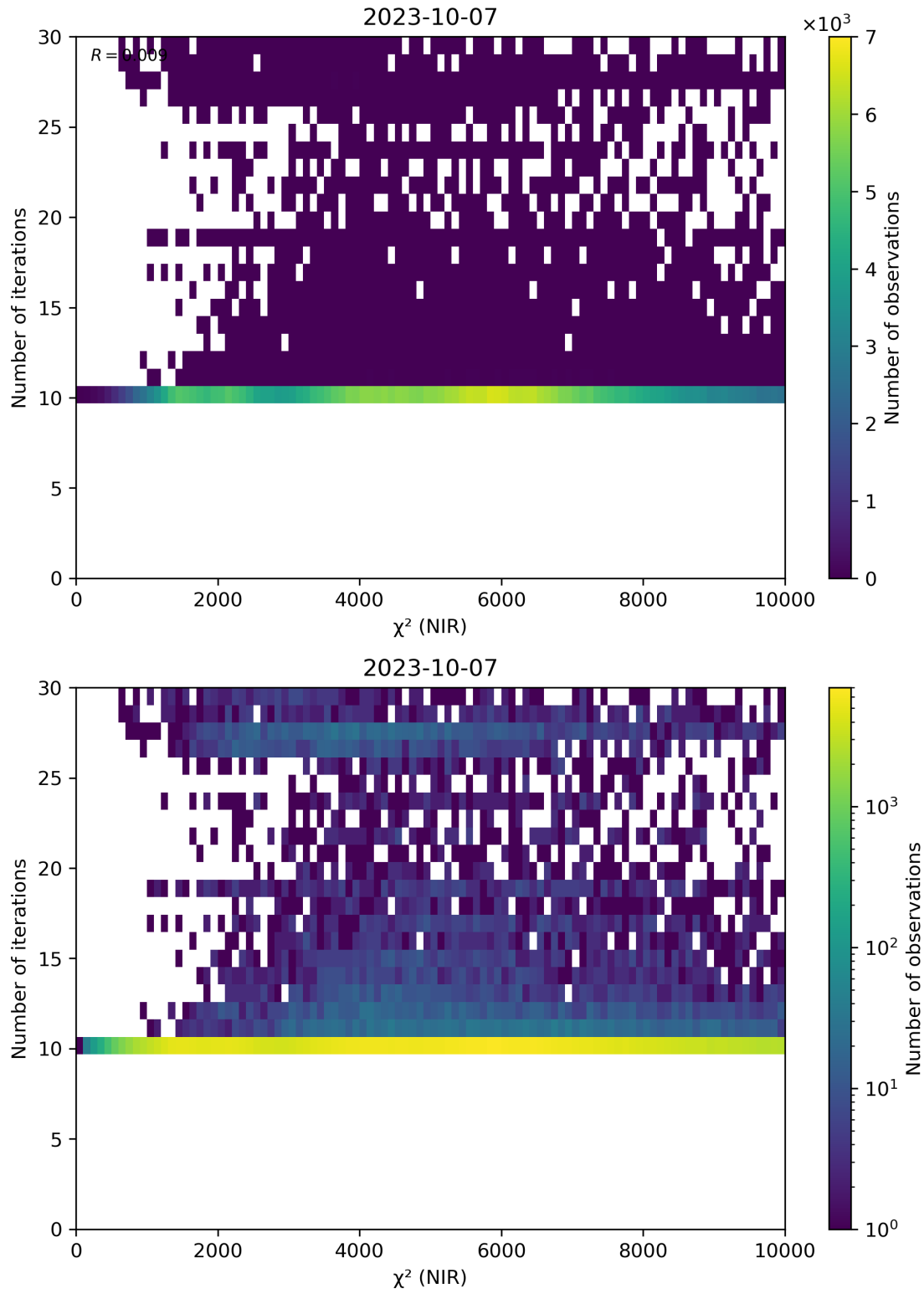
Figure 46: Scatter density plot of “ \chi^2 (NIR)” against “Number of iterations” for 2023-10-06 to 2023-10-08.
