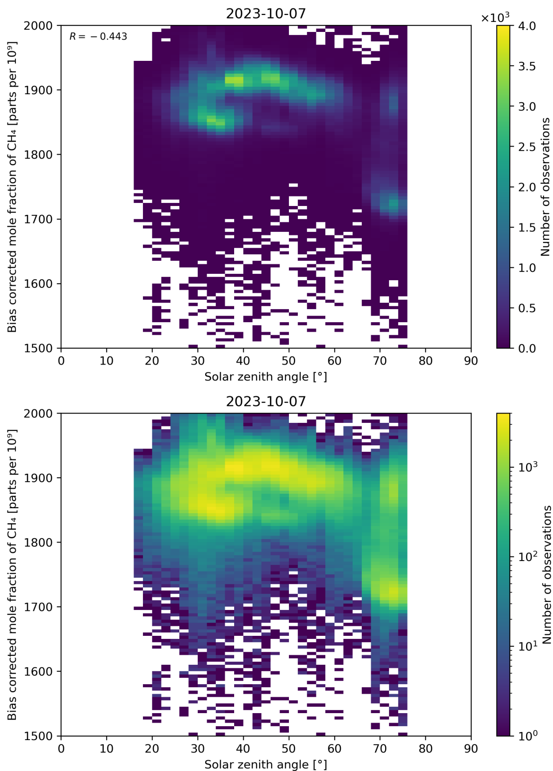
Figure 100: Scatter density plot of “Solar zenith angle” against “Bias corrected mole fraction of CH 4 ” for 2023-10-06 to 2023-10-08.
