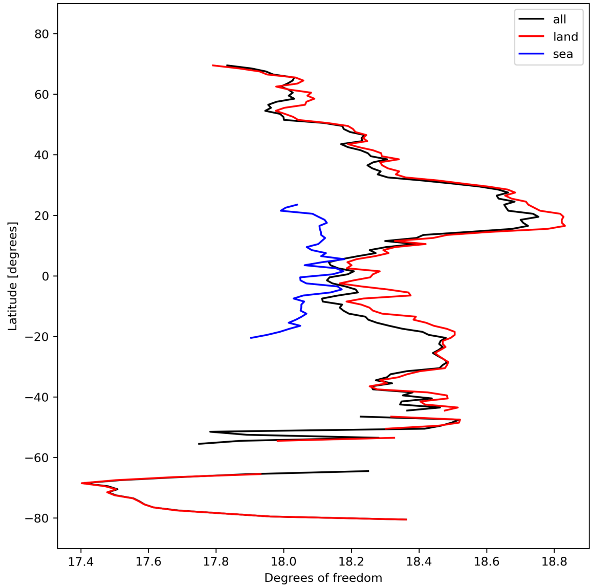
Figure 19: Zonal average of “Degrees of freedom” for 2023-10-06 to 2023-10-08.
