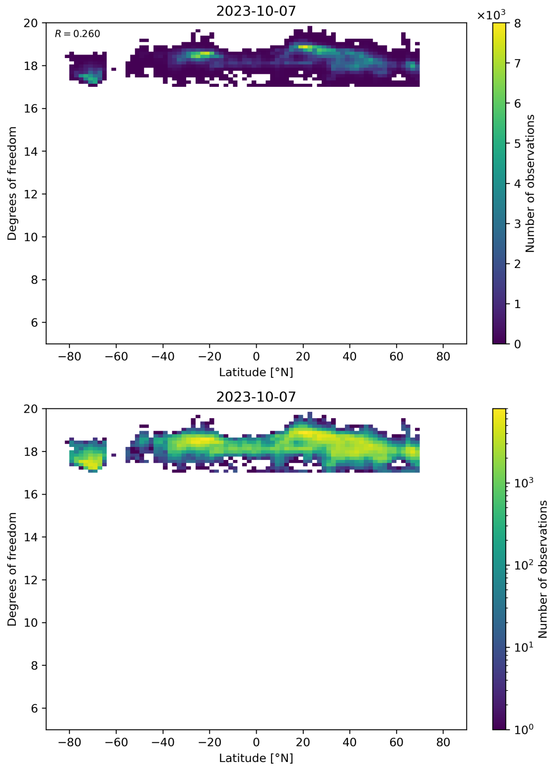
Figure 55: Scatter density plot of “Latitude” against “Degrees of freedom” for 2023-10-06 to 2023-10-08.
