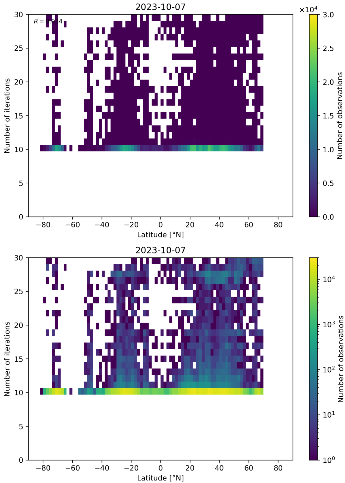
Figure 60: Scatter density plot of “Latitude” against “Number of iterations” for 2023-10-06 to 2023-10-08.
