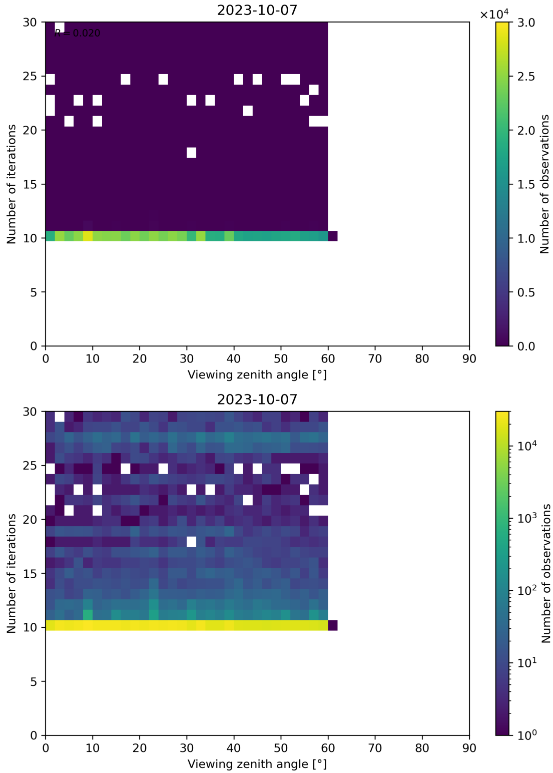
Figure 113: Scatter density plot of “Viewing zenith angle” against “Number of iterations” for 2023-10-06 to 2023-10-08.
