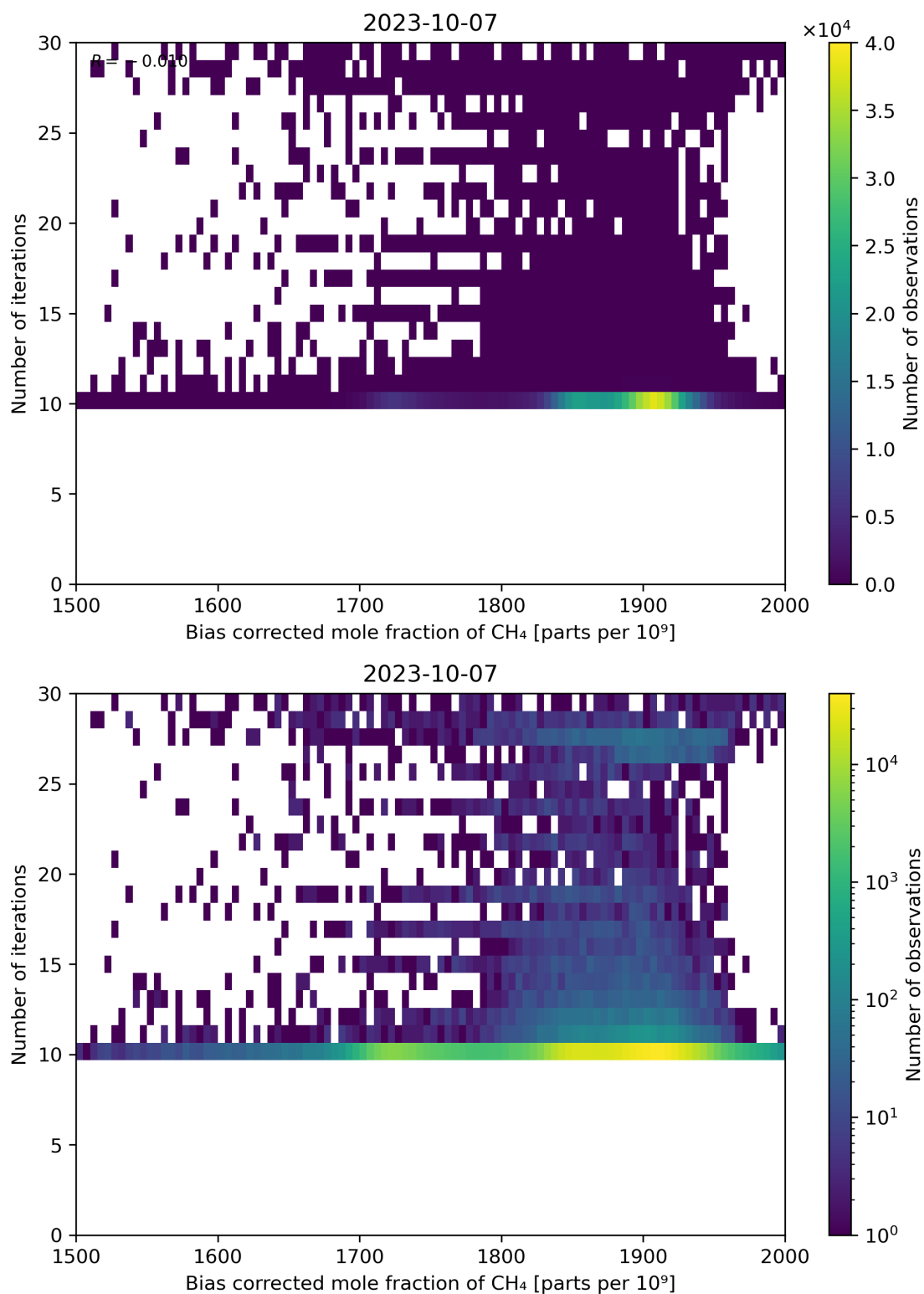
Figure 67: Scatter density plot of “Bias corrected mole fraction of CH 4 ” against “Number of iterations” for 2023-10-06 to 2023-10-08.
