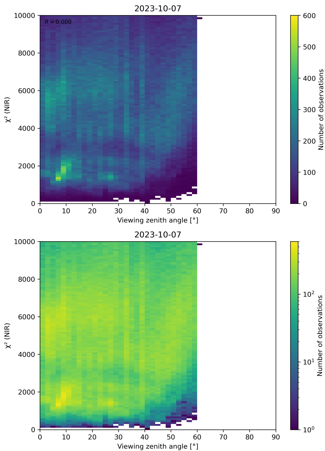
Figure 105: Scatter density plot of “Viewing zenith angle” against “ \chi^2 (NIR)” for 2023-10-06 to 2023-10-08.
