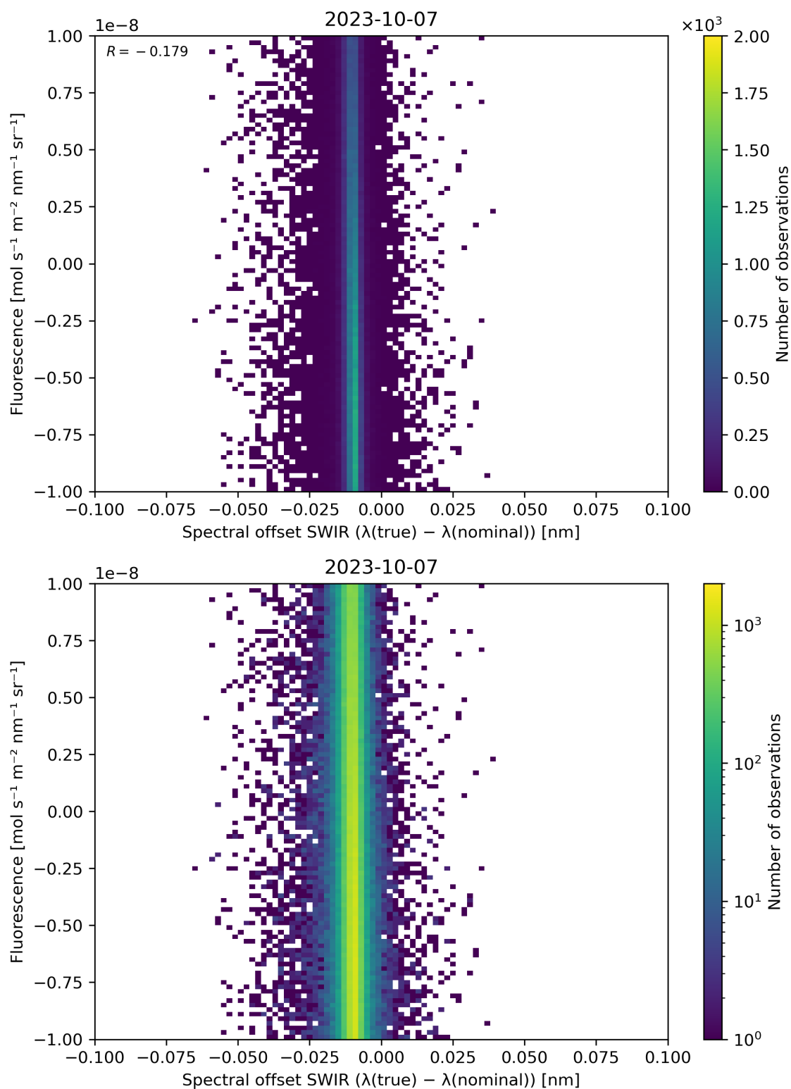
Figure 120: Scatter density plot of “Spectral offset SWIR ( \lambda(\text{true}) - \lambda(\text{nominal}) )” against “Fluorescence” for 2023-10-06 to 2023-10-08.
