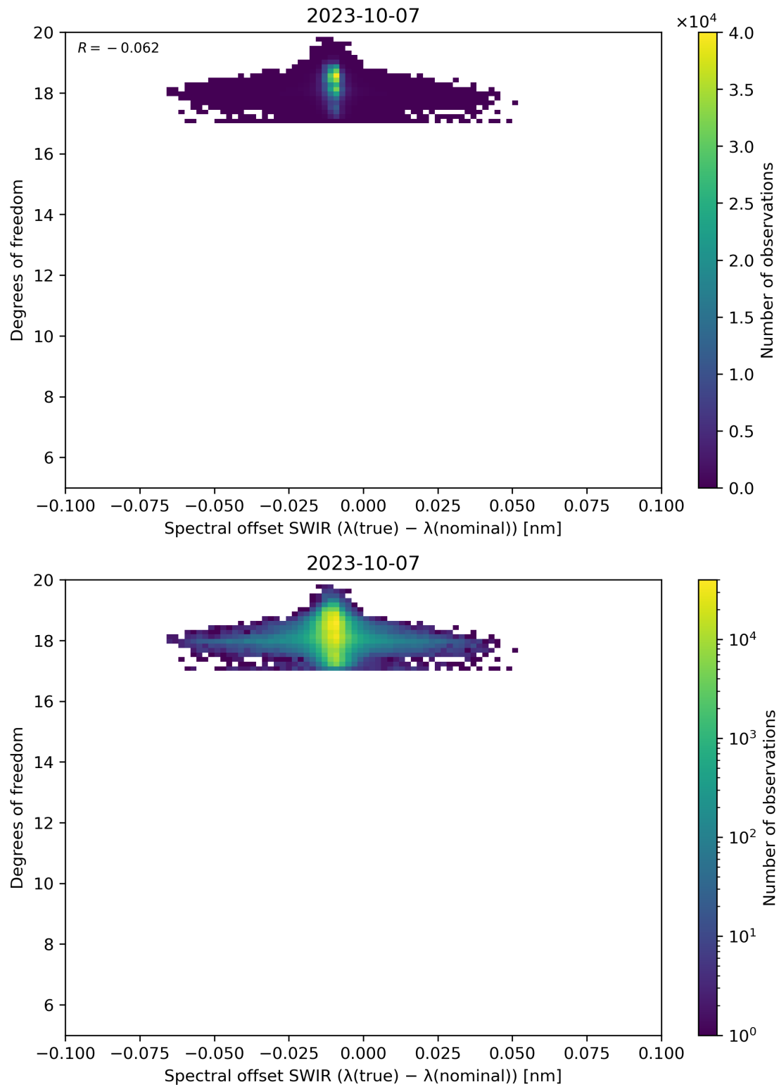
Figure 119: Scatter density plot of “Spectral offset SWIR ( \lambda(\text{true}) - \lambda(\text{nominal}) )” against “Degrees of freedom” for 2023-10-06 to 2023-10-08.
