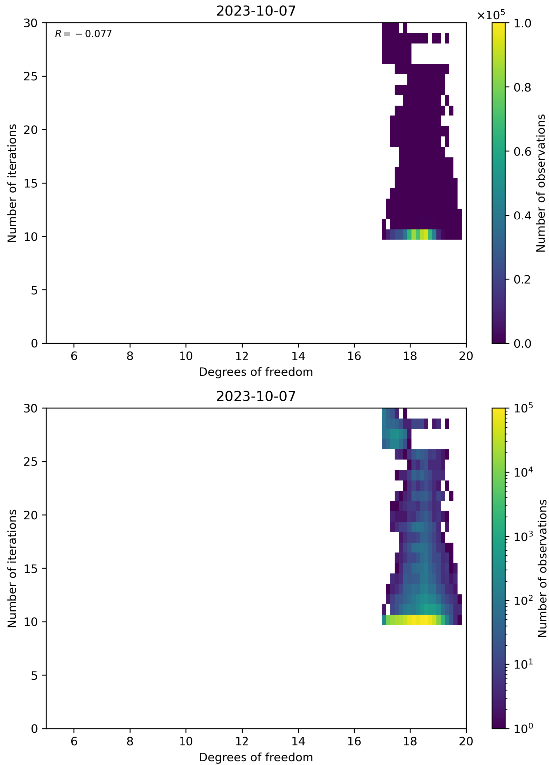
Figure 52: Scatter density plot of “Degrees of freedom” against “Number of iterations” for 2023-10-06 to 2023-10-08.
