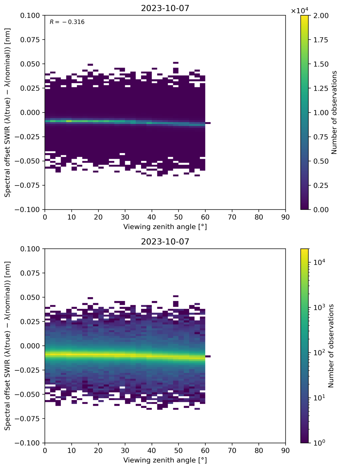
Figure 116: Scatter density plot of “Viewing zenith angle” against “Spectral offset SWIR ( \lambda(\text{true}) - \lambda(\text{nominal}) )” for 2023-10-06 to 2023-10-08.
