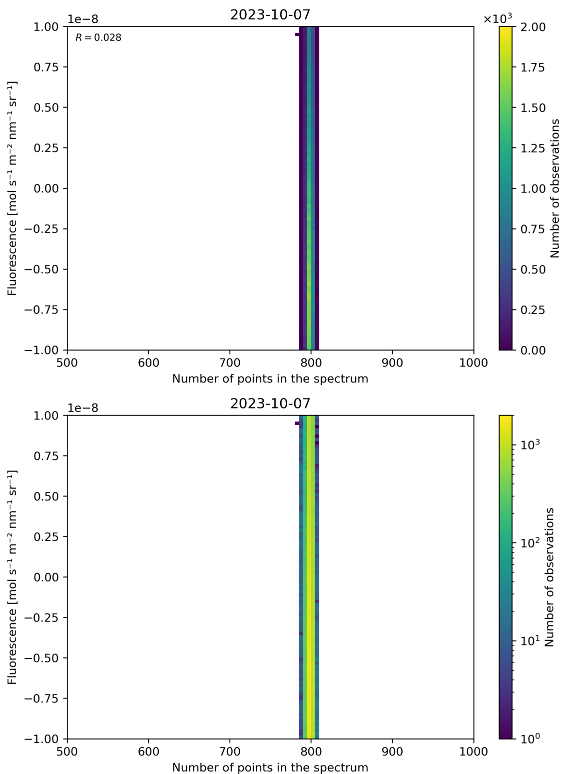
Figure 91: Scatter density plot of “Number of points in the spectrum” against “Fluorescence” for 2023-10-06 to 2023-10-08.
