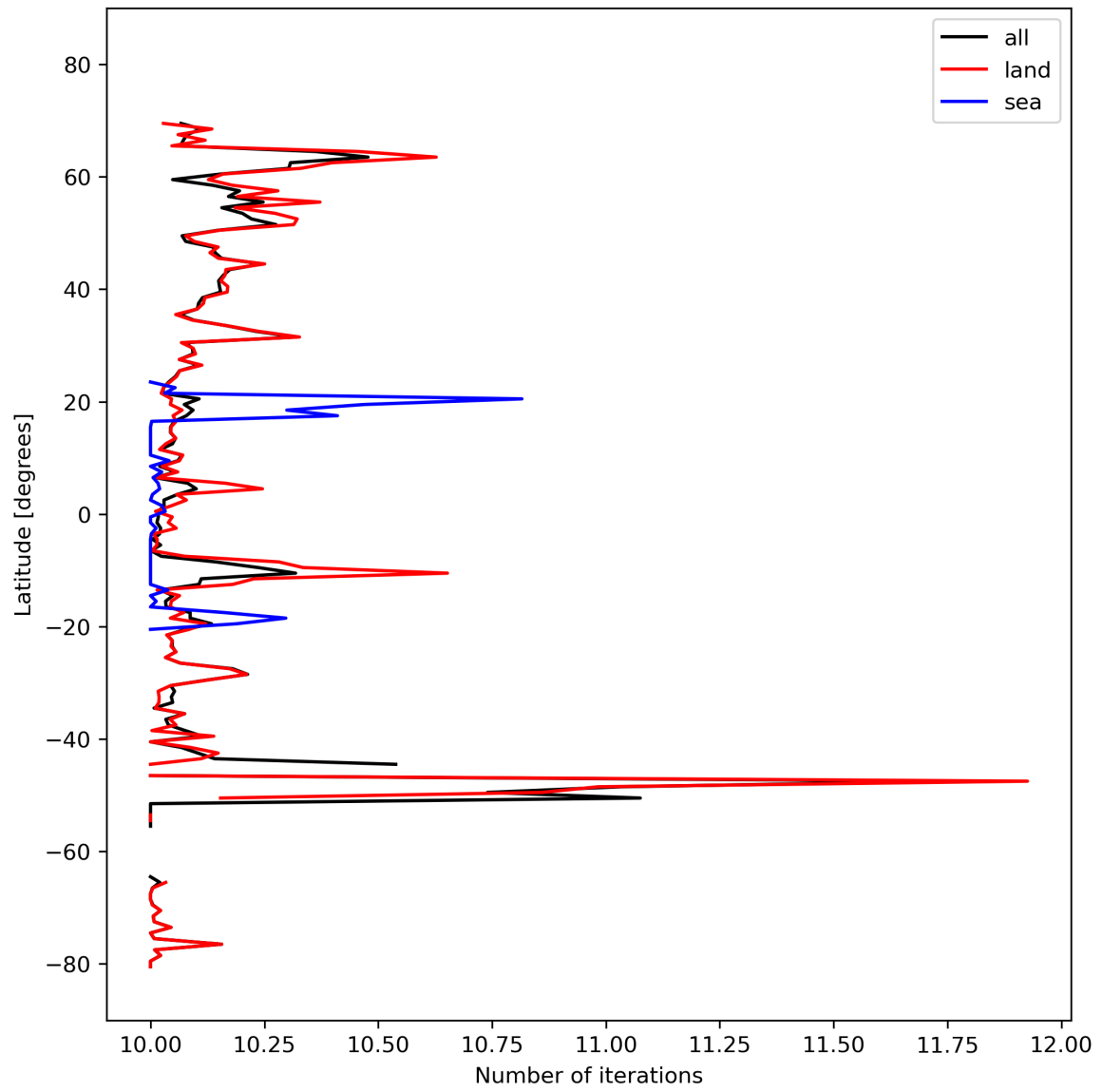
Figure 20: Zonal average of “Number of iterations” for 2023-10-06 to 2023-10-08.
