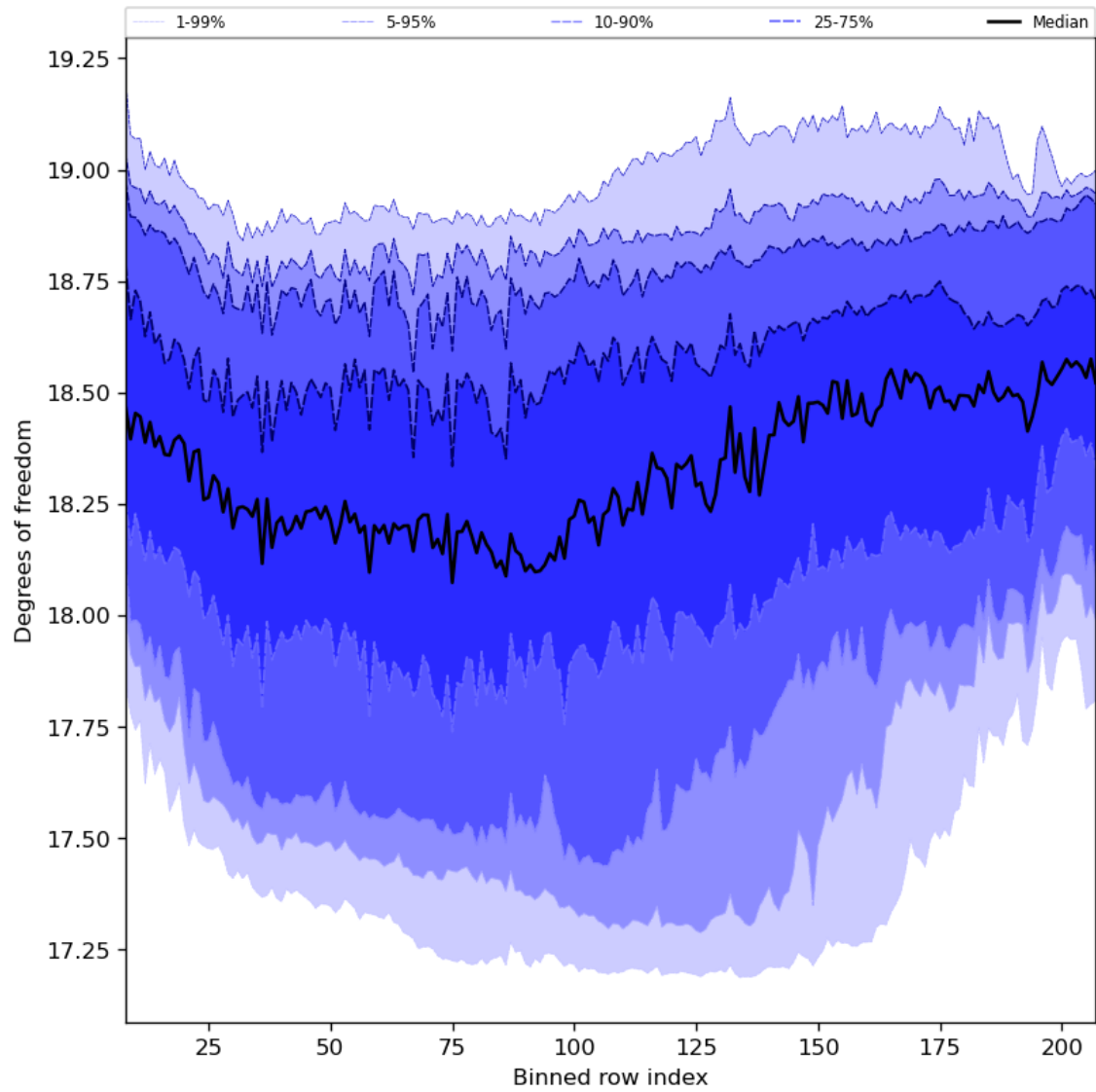
Figure 41: Along track statistics of “Degrees of freedom” for 2023-10-06 to 2023-10-08
