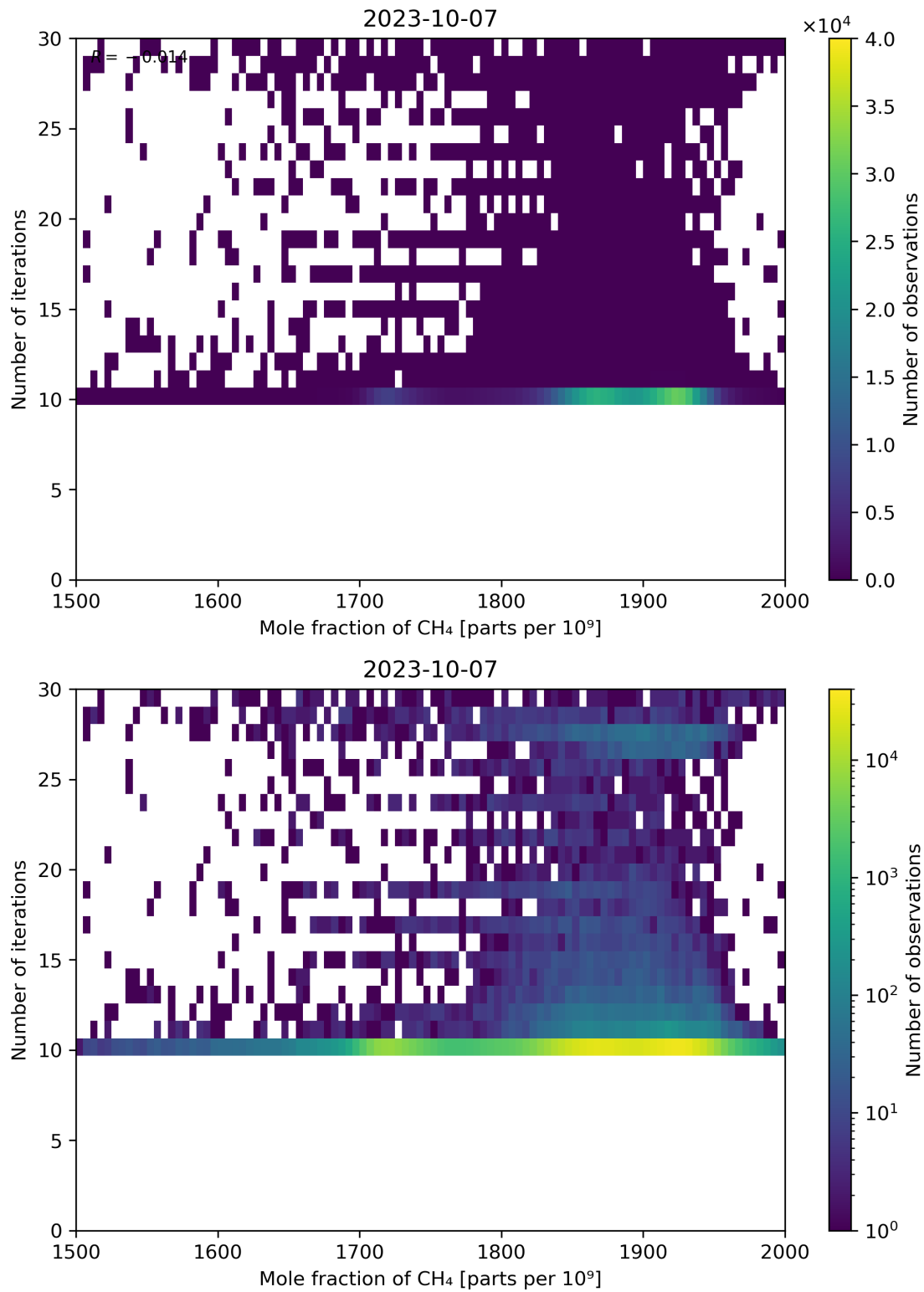
Figure 76: Scatter density plot of “Mole fraction of CH 4 ” against “Number of iterations” for 2023-10-06 to 2023-10-08.
