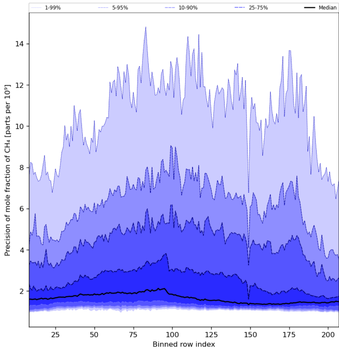
Figure 35: Along track statistics of “Precision of mole fraction of CH 4 ” for 2023-10-06 to 2023-10-08
