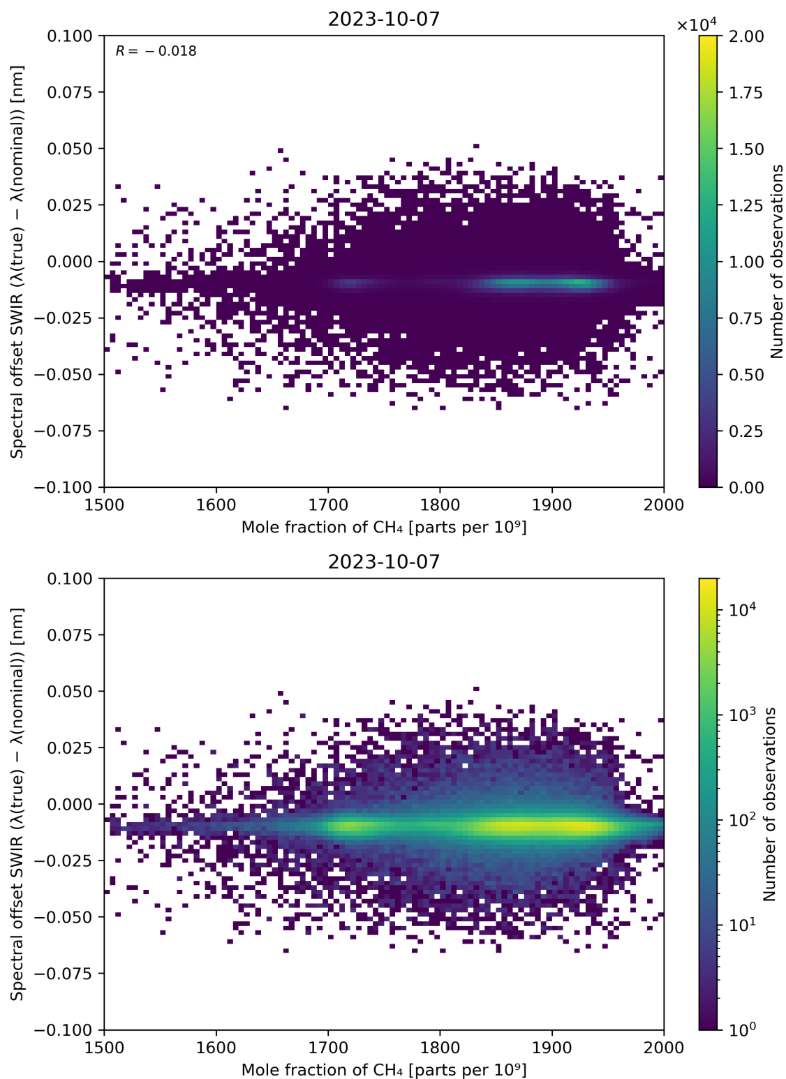
Figure 86: Scatter density plot of “Mole fraction of CH 4 ” against “Spectral offset SWIR ( \lambda(\text{true}) - \lambda(\text{nominal}) )” for 2023-10-06 to 2023-10-08.
