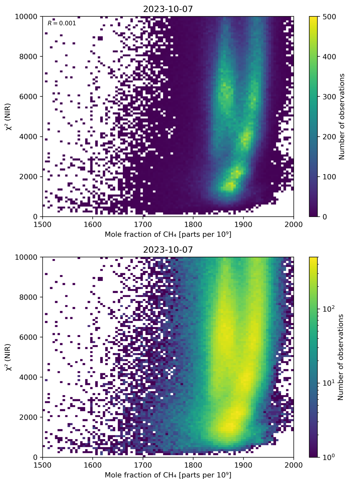
Figure 70: Scatter density plot of “Mole fraction of CH 4 ” against “ \chi^2 (NIR)” for 2023-10-06 to 2023-10-08.
