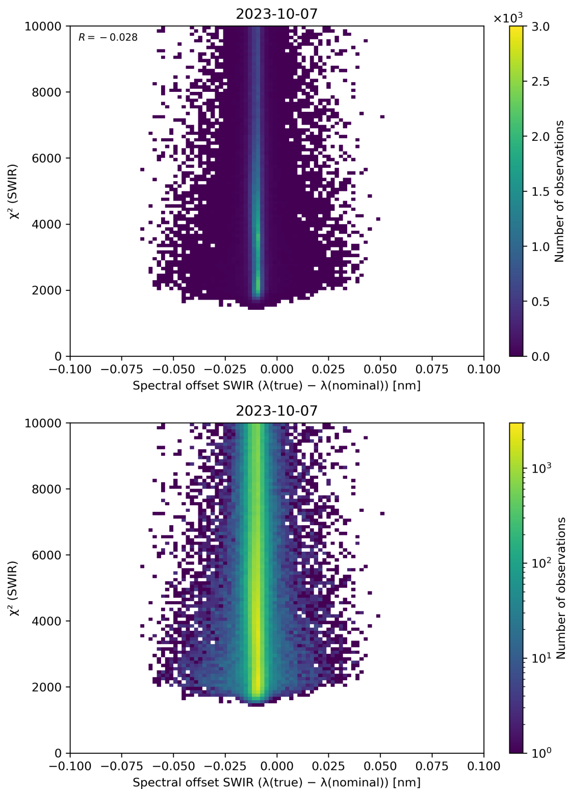
Figure 118: Scatter density plot of “Spectral offset SWIR ( \lambda(\text{true}) - \lambda(\text{nominal}) )” against “ \chi^2 (SWIR)” for 2023-10-06 to 2023-10-08.
