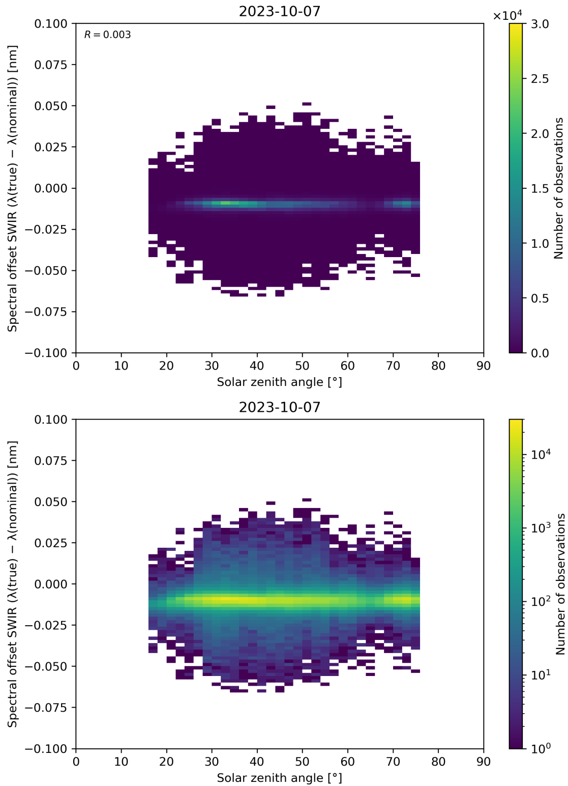
Figure 104: Scatter density plot of “Solar zenith angle” against “Spectral offset SWIR ( \lambda(\text{true}) - \lambda(\text{nominal}) )” for 2023-10-06 to 2023-10-08.
