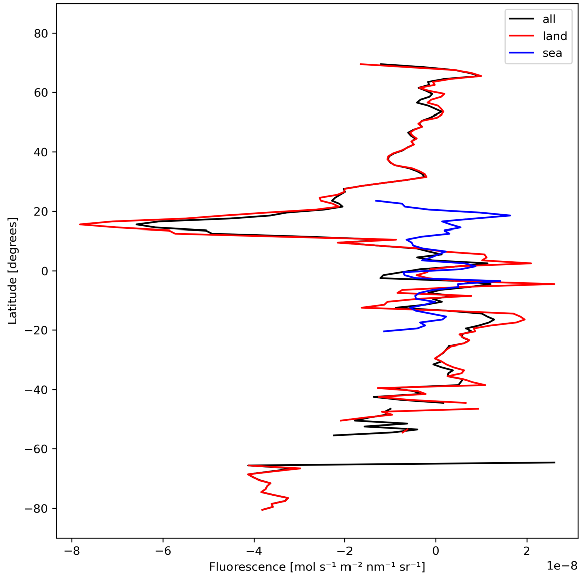
Figure 21: Zonal average of “Fluorescence” for 2023-10-06 to 2023-10-08.
