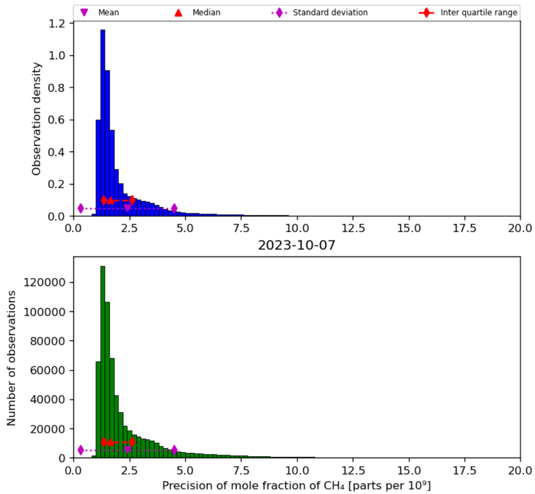
Figure 24: Histogram of “Precision of mole fraction of CH 4 ” for 2023-10-06 to 2023-10-08
