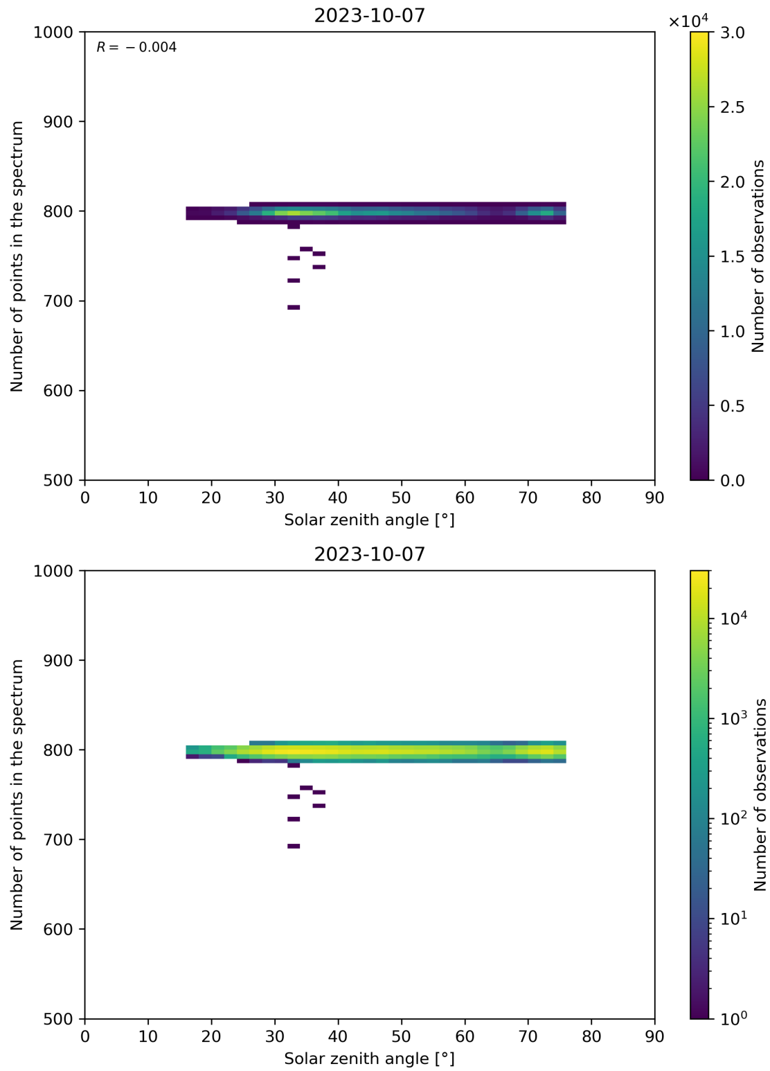
Figure 103: Scatter density plot of “Solar zenith angle” against “Number of points in the spectrum” for 2023-10-06 to 2023-10-08.
