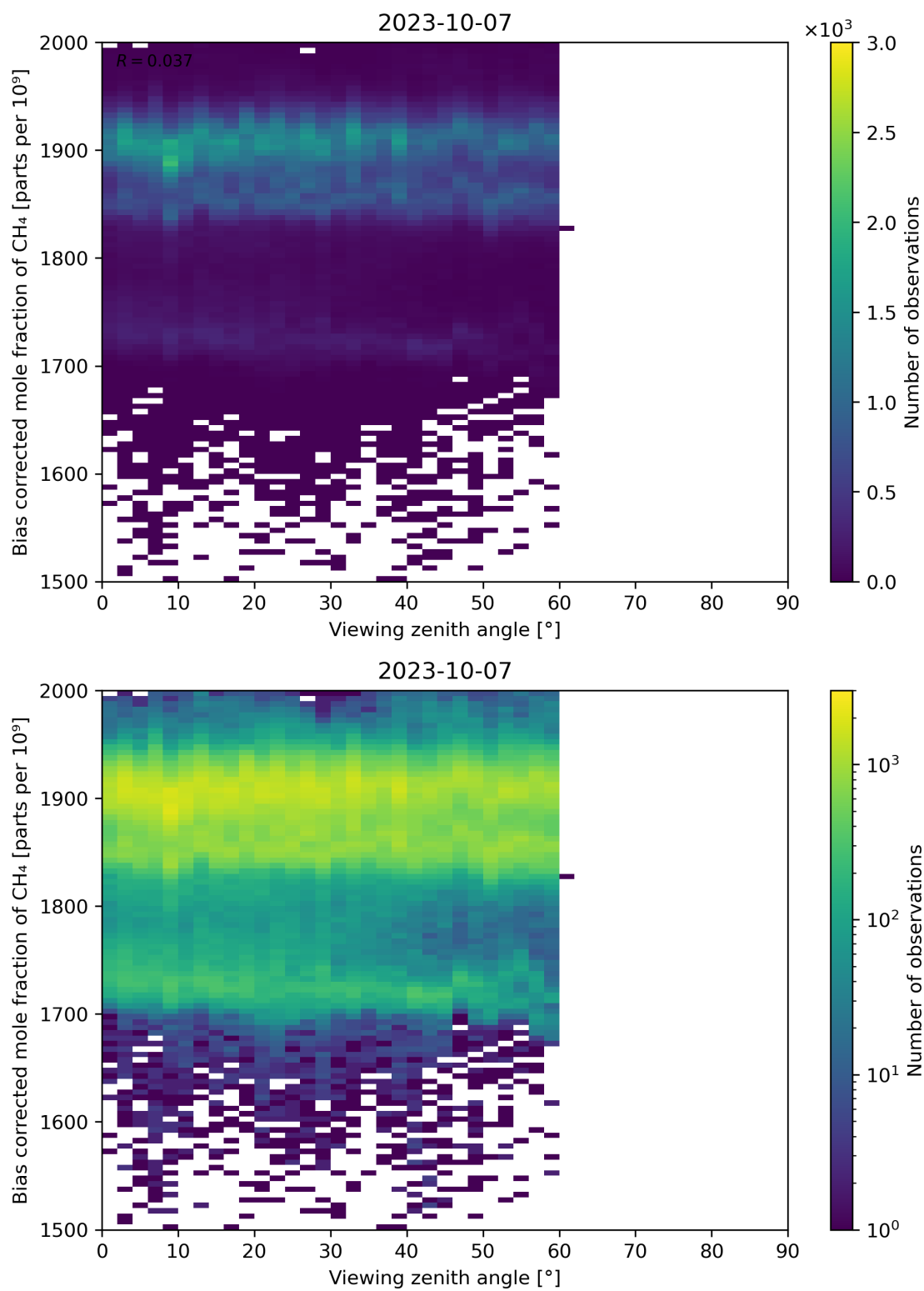
Figure 111: Scatter density plot of “Viewing zenith angle” against “Bias corrected mole fraction of CH 4 ” for 2023-10-06 to 2023-10-08.
