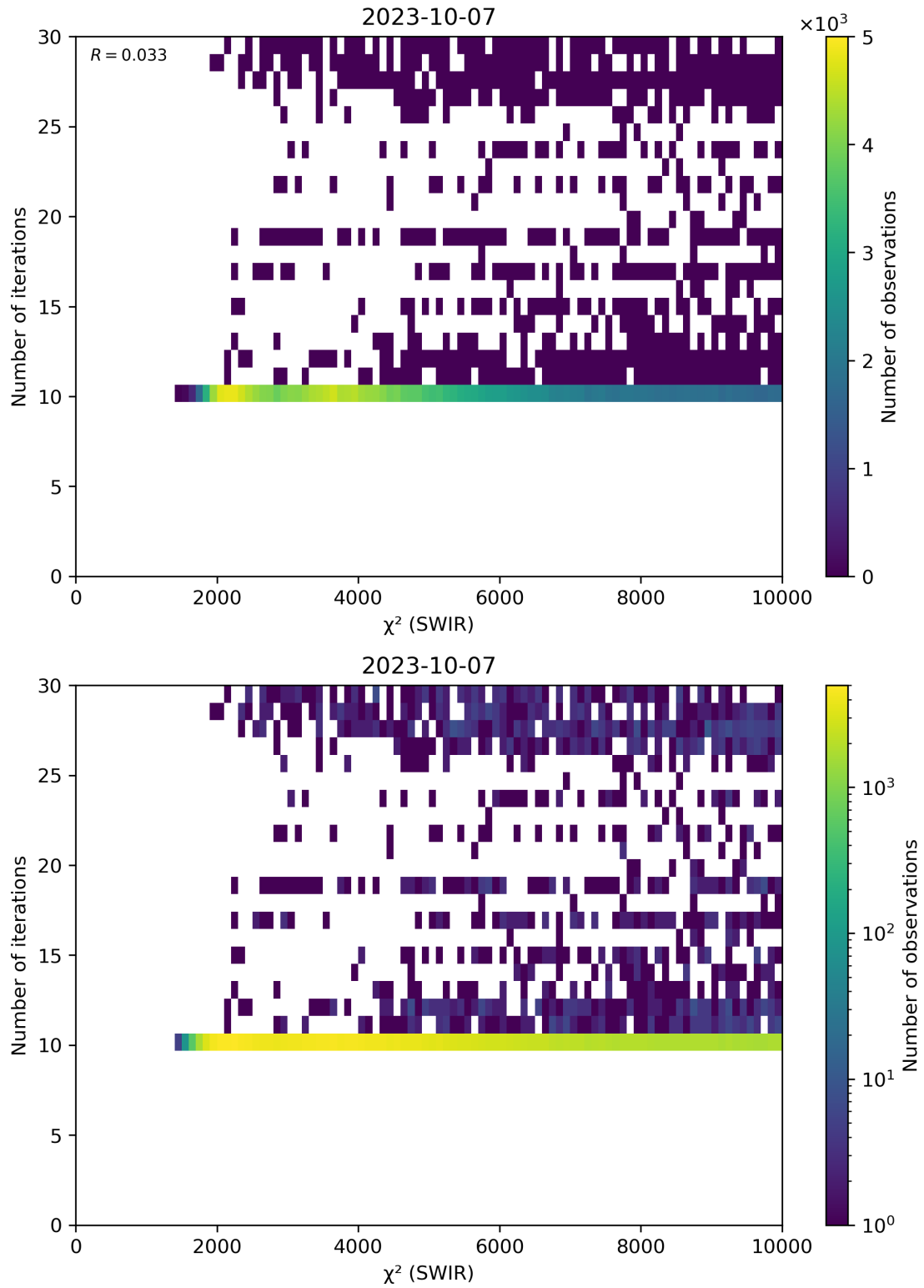
Figure 50: Scatter density plot of “ \chi^2 (SWIR)” against “Number of iterations” for 2023-10-06 to 2023-10-08.
