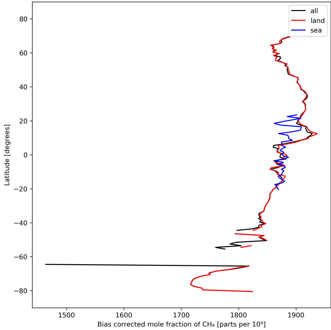
Figure 14: Zonal average of “Bias corrected mole fraction of CH 4 ” for 2023-10-06 to 2023-10-08.
