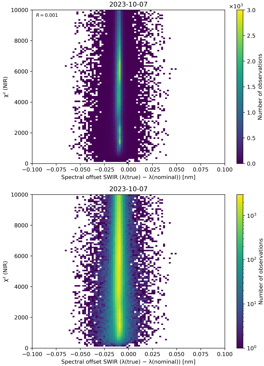
Figure 117: Scatter density plot of “Spectral offset SWIR ( \lambda(\text{true}) - \lambda(\text{nominal}) )” against “ \chi^2 (NIR)” for 2023-10-06 to 2023-10-08.
