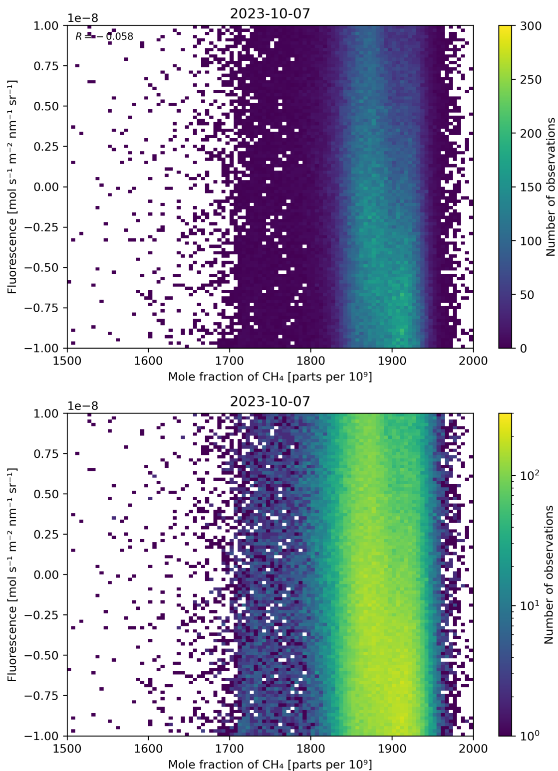
Figure 73: Scatter density plot of “Mole fraction of \text{CH}_4 ” against “Fluorescence” for 2023-10-06 to 2023-10-08.
