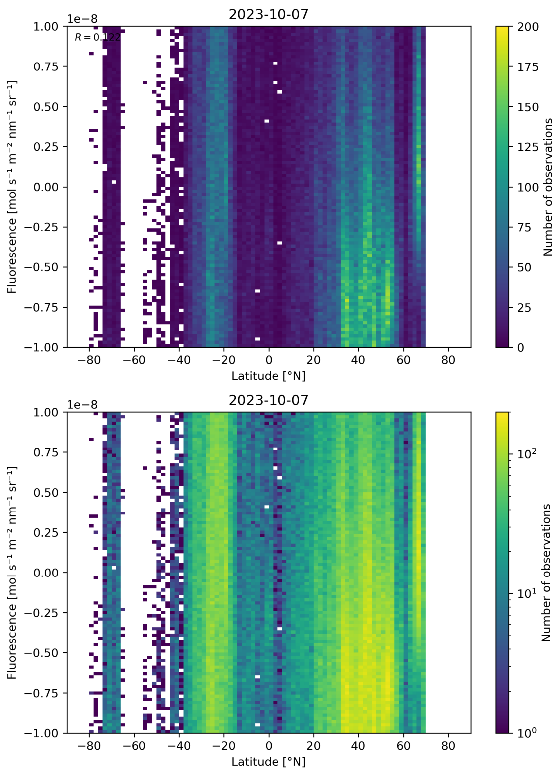
Figure 56: Scatter density plot of “Latitude” against “Fluorescence” for 2023-10-06 to 2023-10-08.
