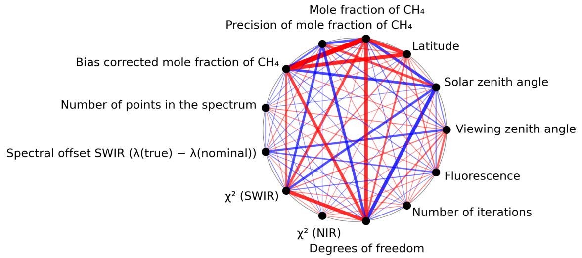
Figure 1: Map of correlation graph for 2023-10-06 to 2023-10-08.
