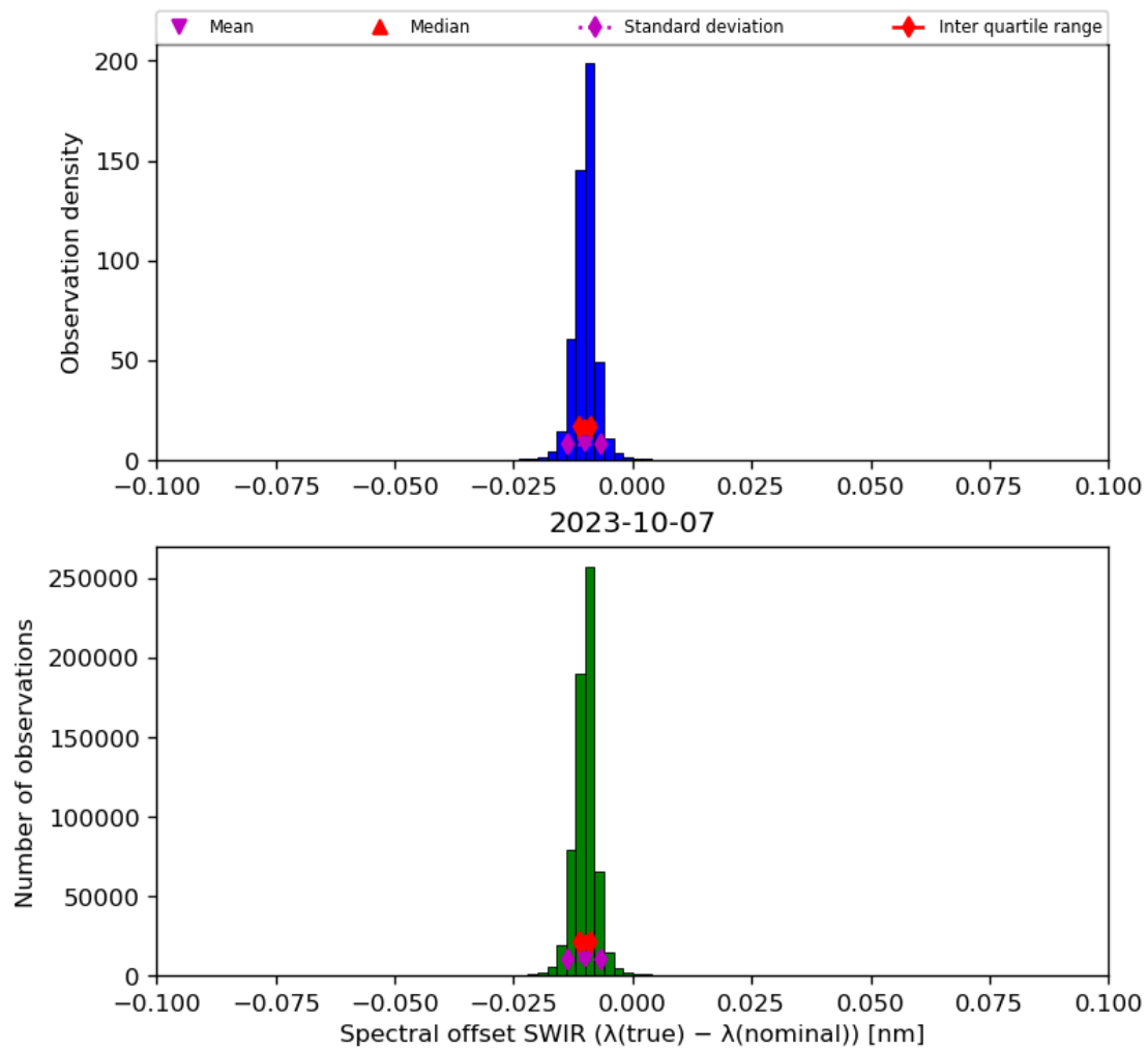
Figure 27: Histogram of “Spectral offset SWIR ( \lambda(\text{true}) - \lambda(\text{nominal}) )” for 2023-10-06 to 2023-10-08
