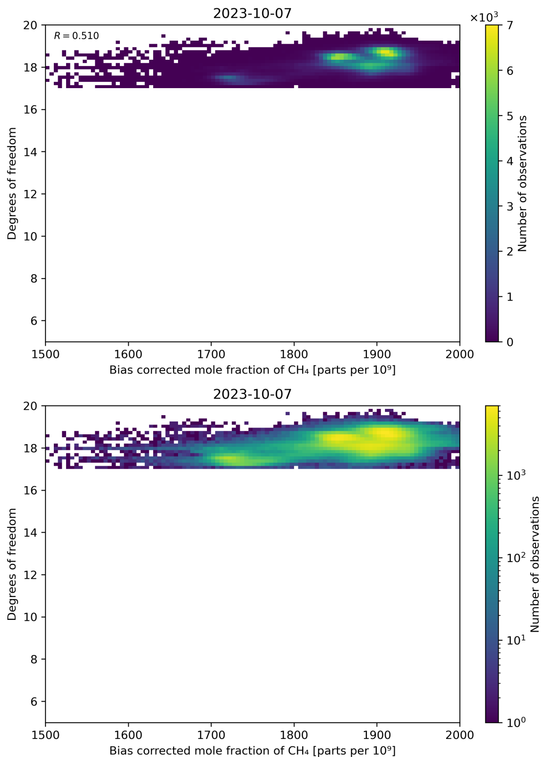
Figure 65: Scatter density plot of “Bias corrected mole fraction of CH 4 ” against “Degrees of freedom” for 2023-10-06 to 2023-10-08.
