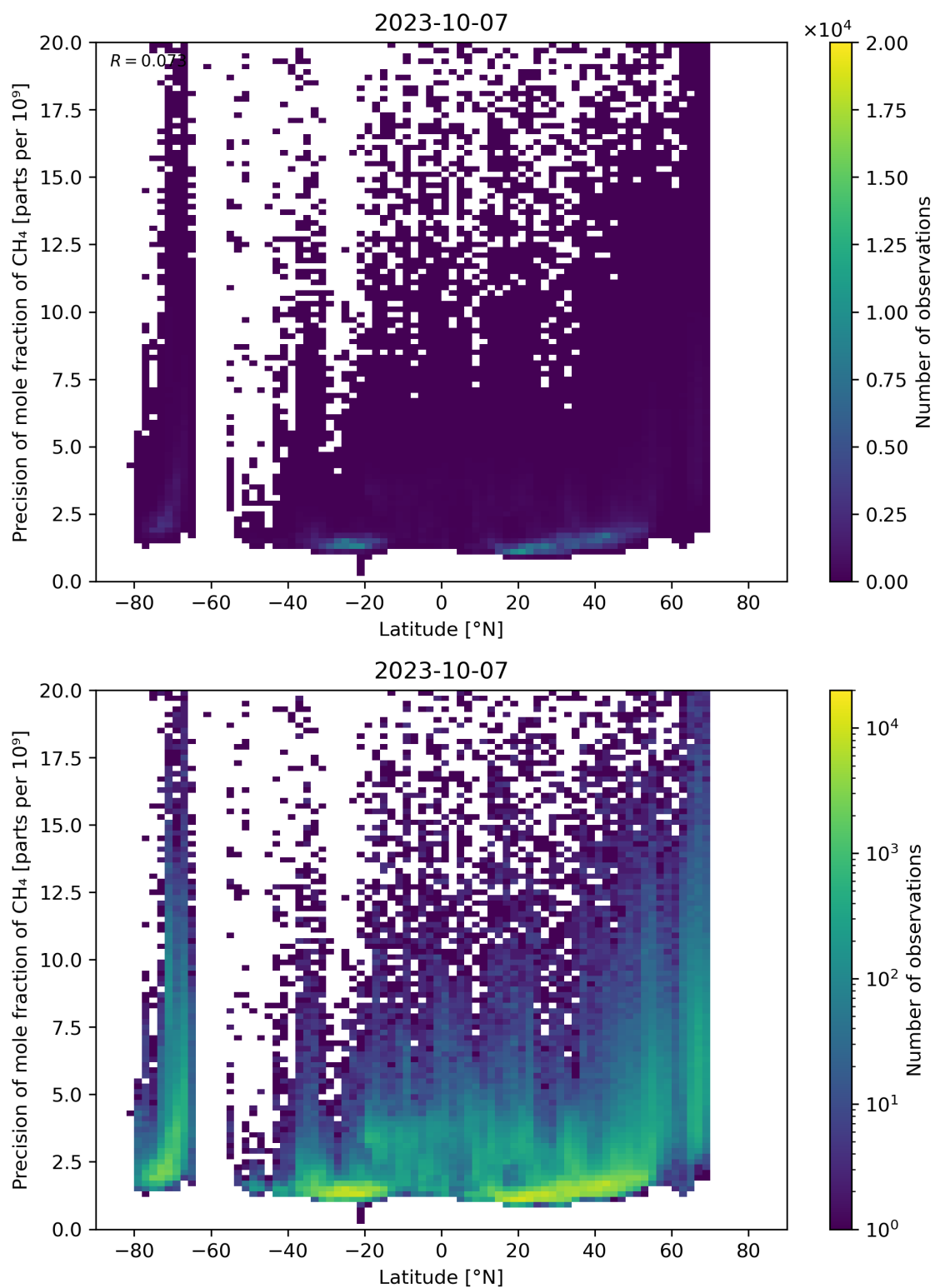
Figure 59: Scatter density plot of “Latitude” against “Precision of mole fraction of CH 4 ” for 2023-10-06 to 2023-10-08.
