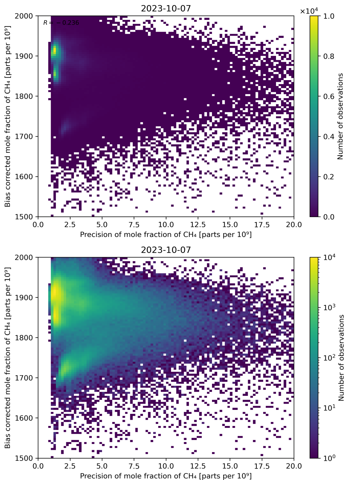
Figure 82: Scatter density plot of “Precision of mole fraction of CH 4 ” against “Bias corrected mole fraction of CH 4 ” for 2023-10-06 to 2023-10-08.
