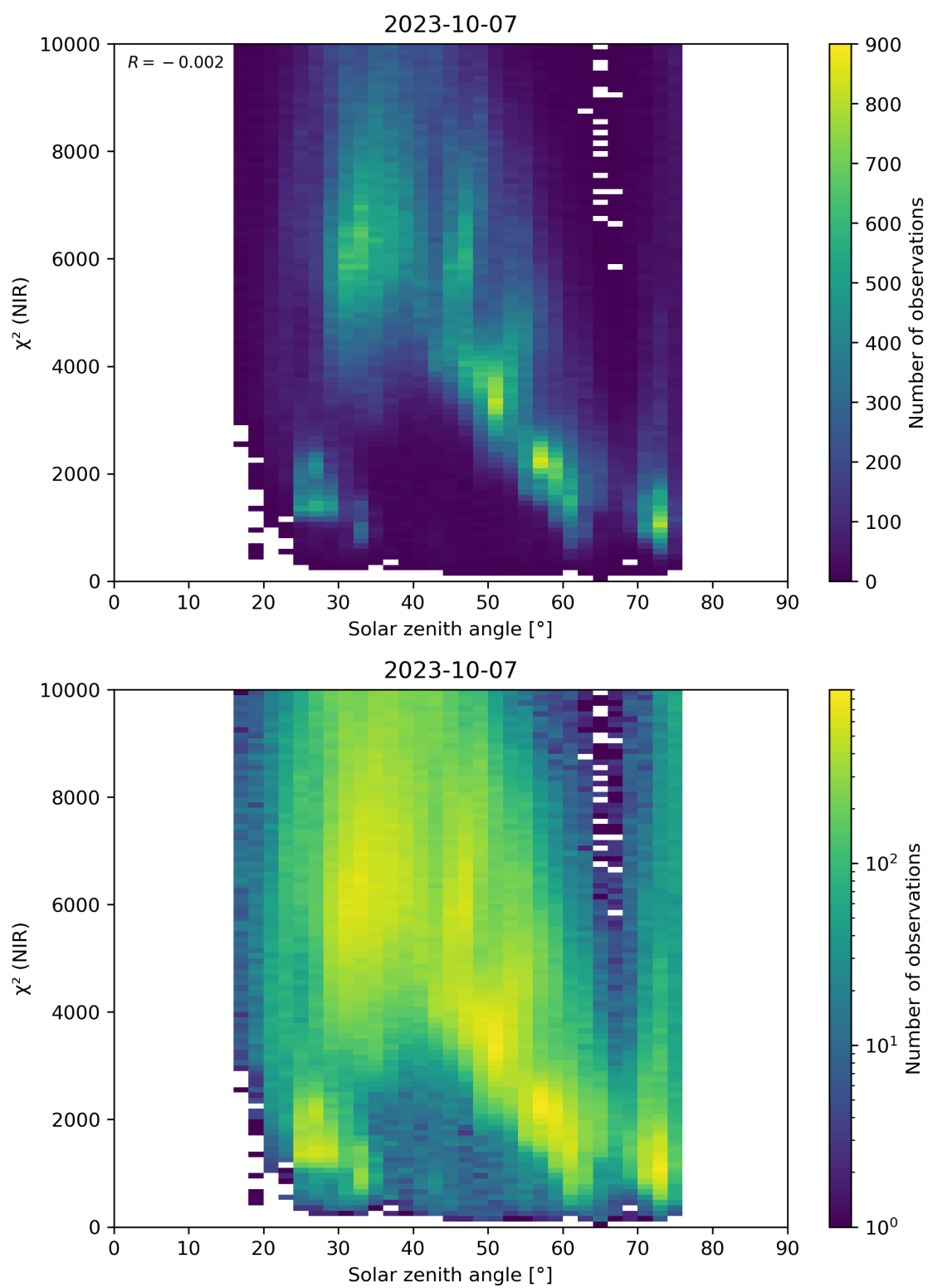
Figure 94: Scatter density plot of “Solar zenith angle” against “ \chi^2 (NIR)” for 2023-10-06 to 2023-10-08.
