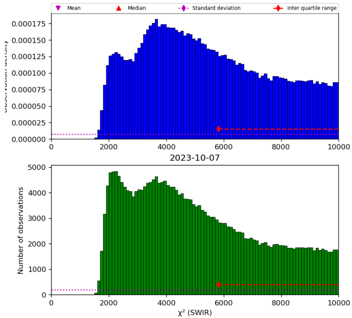
Figure 28: Histogram of “ \chi^2 (SWIR)” for 2023-10-06 to 2023-10-08
