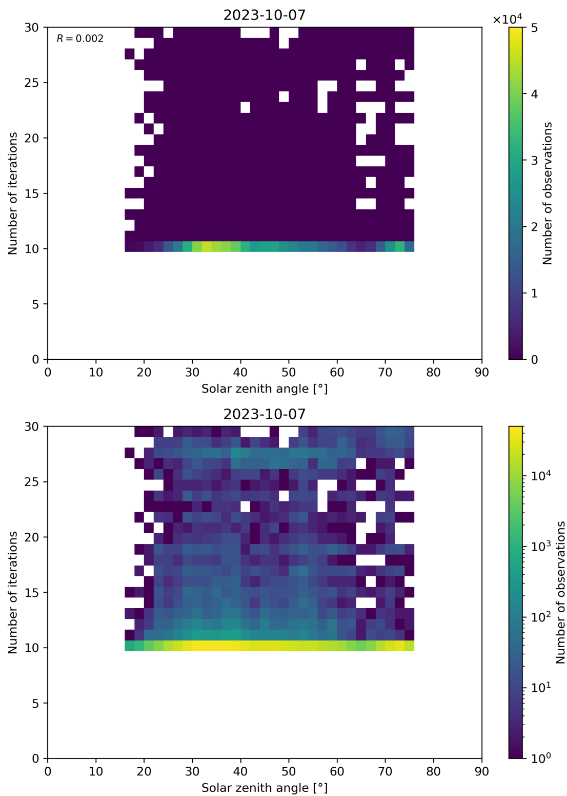
Figure 102: Scatter density plot of “Solar zenith angle” against “Number of iterations” for 2023-10-06 to 2023-10-08.
