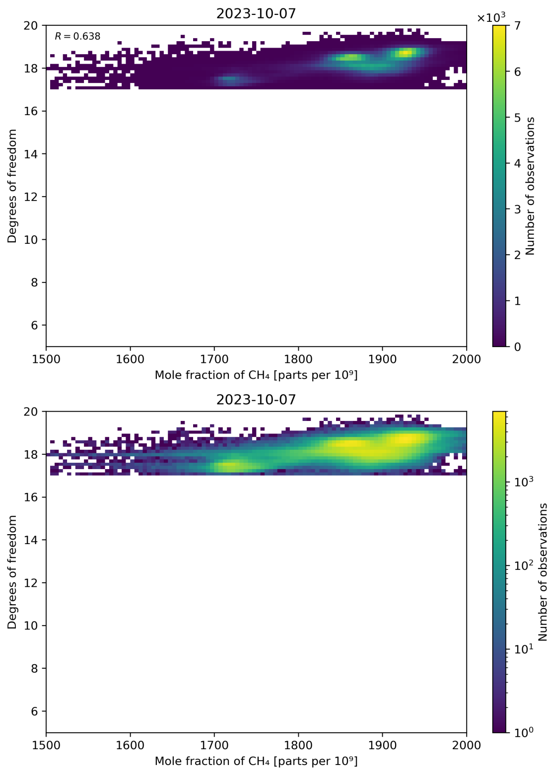
Figure 72: Scatter density plot of “Mole fraction of CH 4 ” against “Degrees of freedom” for 2023-10-06 to 2023-10-08.
