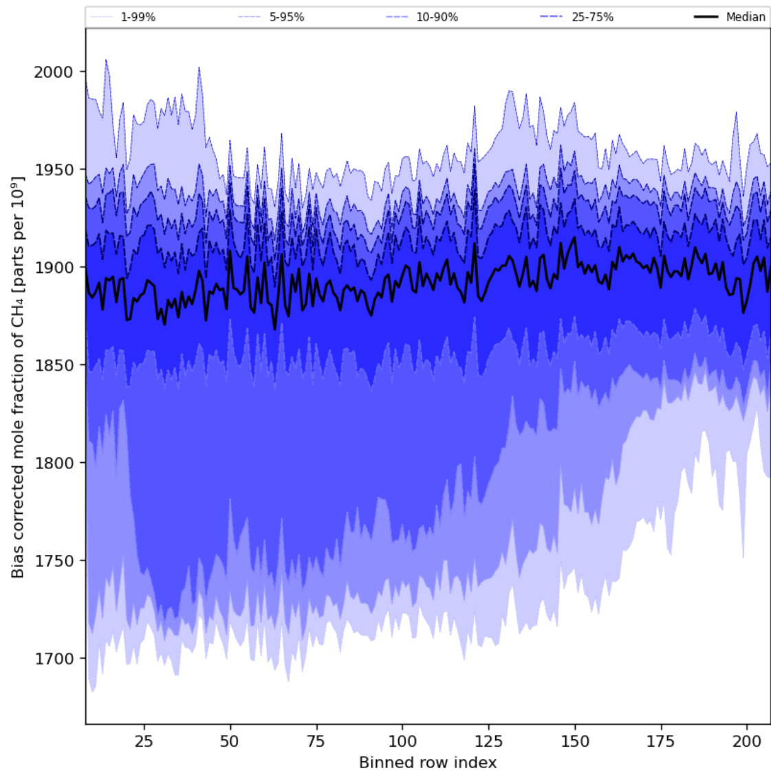
Figure 36: Along track statistics of “Bias corrected mole fraction of CH 4 ” for 2023-10-06 to 2023-10-08
