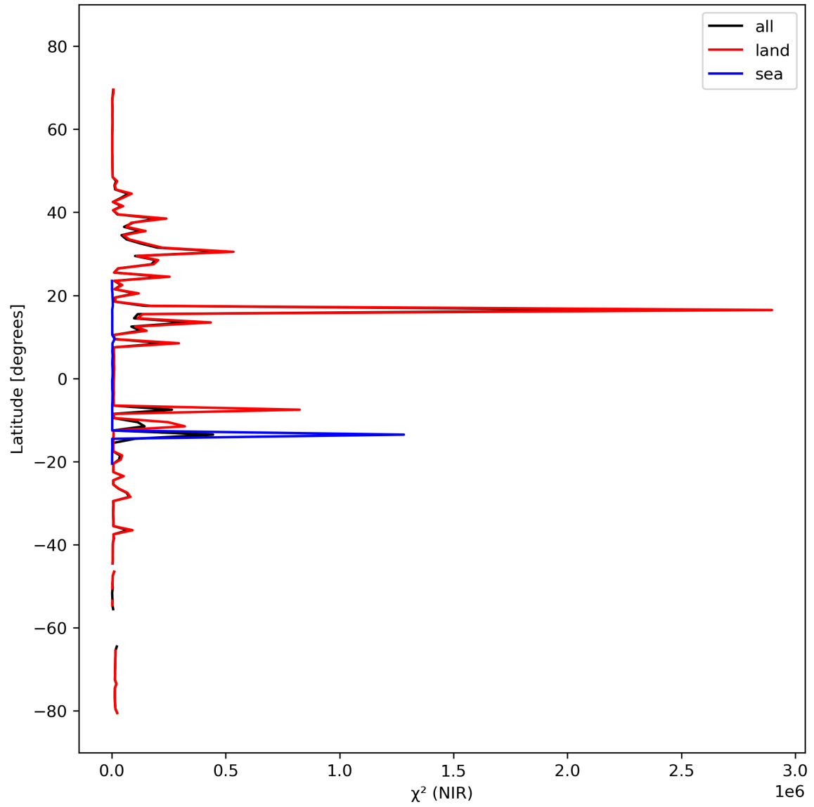
Figure 18: Zonal average of “ \chi^2 (NIR)” for 2023-10-06 to 2023-10-08.
