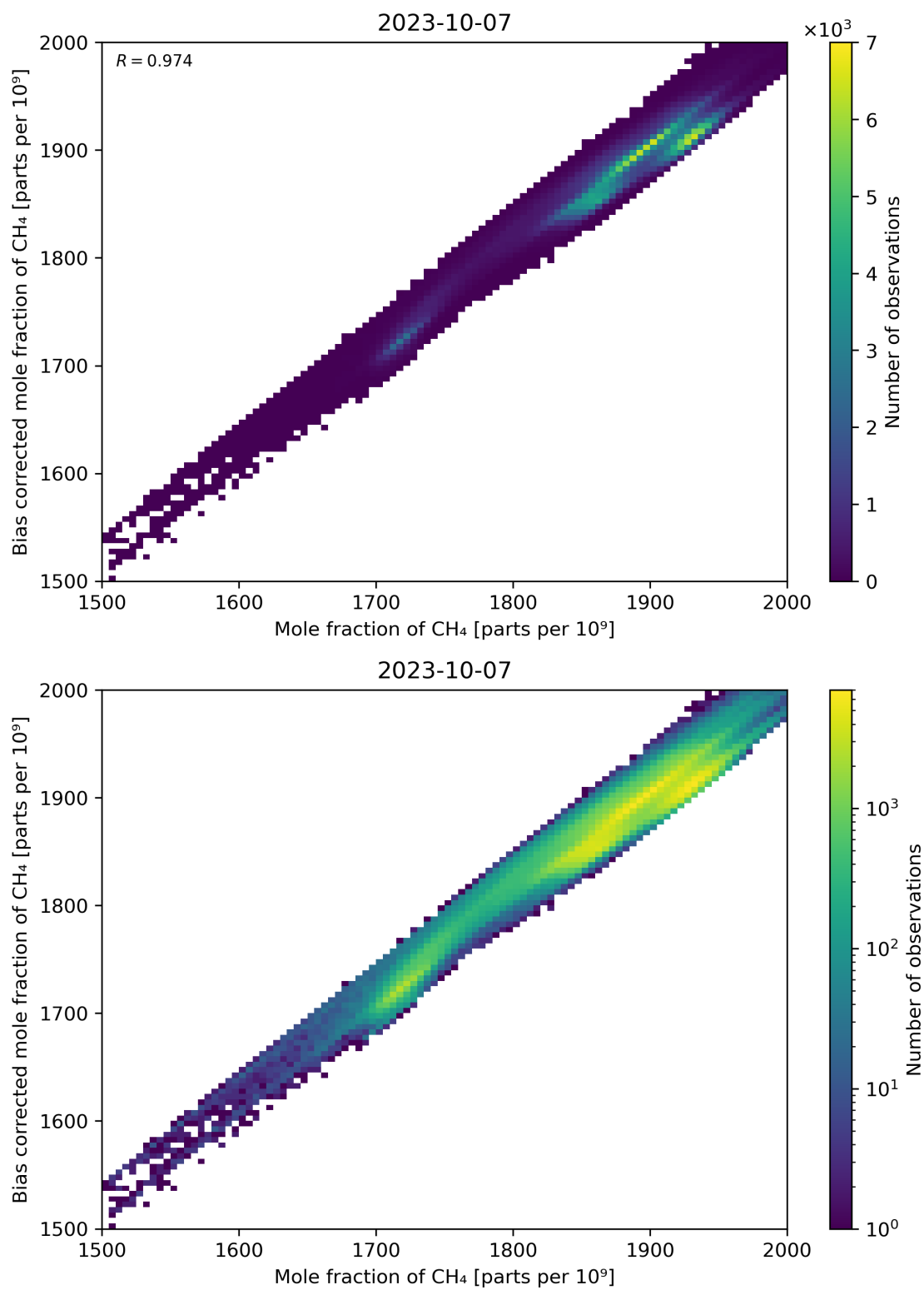
Figure 74: Scatter density plot of “Mole fraction of CH 4 ” against “Bias corrected mole fraction of CH 4 ” for 2023-10-06 to 2023-10-08.
