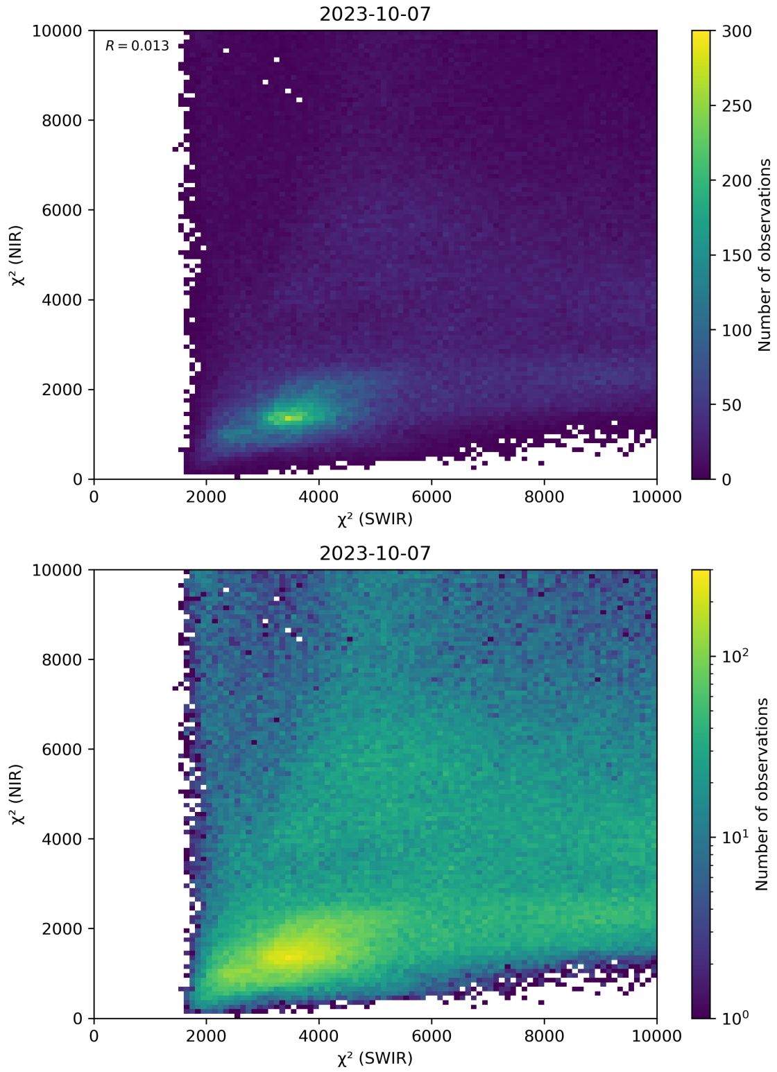
Figure 47: Scatter density plot of “ \chi^2 (SWIR)” against “ \chi^2 (NIR)” for 2023-10-06 to 2023-10-08.
