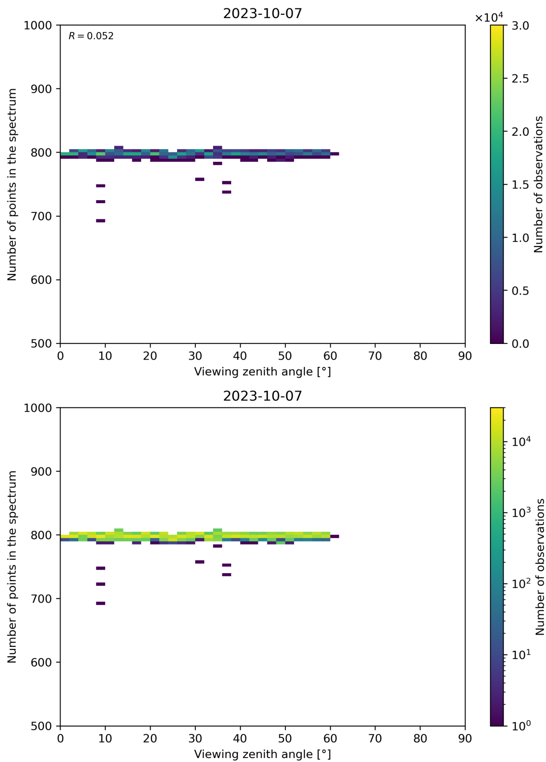
Figure 114: Scatter density plot of “Viewing zenith angle” against “Number of points in the spectrum” for 2023-10-06 to 2023-10-08.
