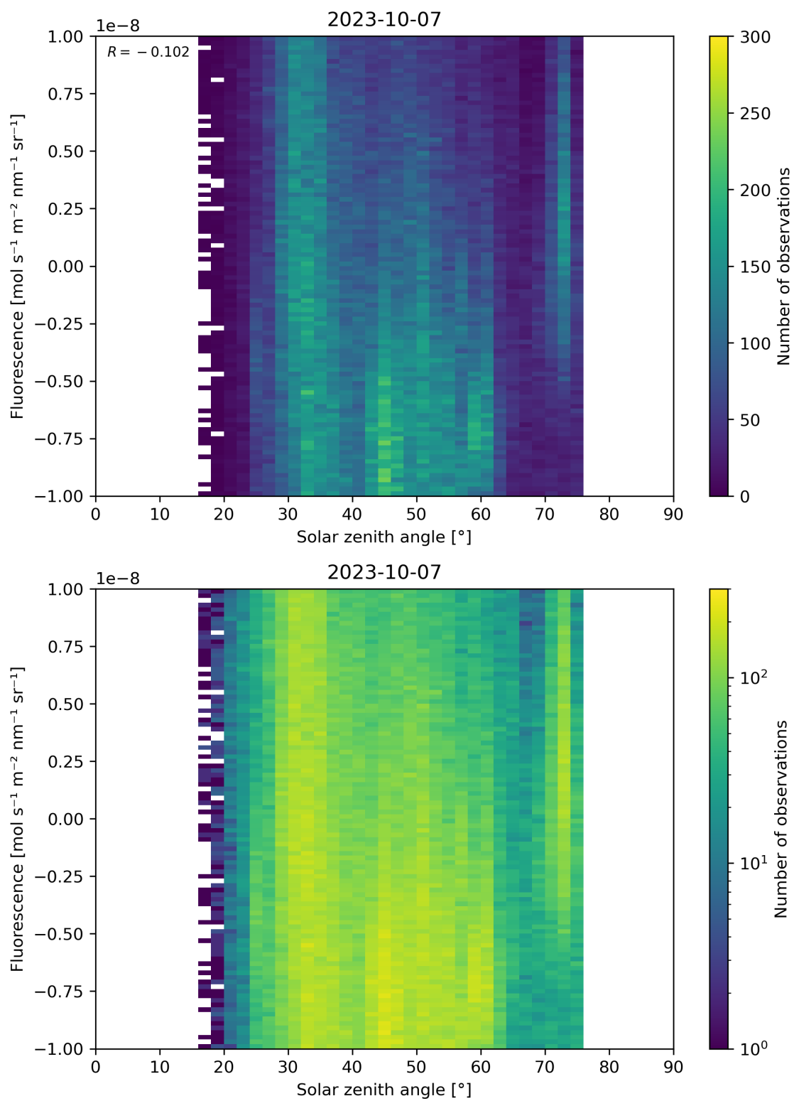
Figure 97: Scatter density plot of “Solar zenith angle” against “Fluorescence” for 2023-10-06 to 2023-10-08.
