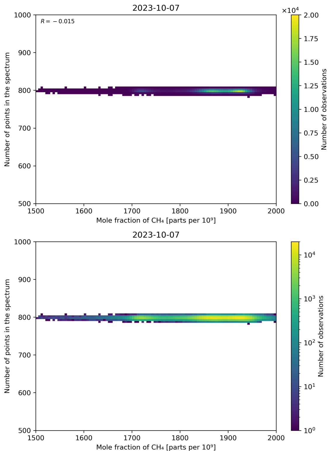
Figure 77: Scatter density plot of “Mole fraction of CH 4 ” against “Number of points in the spectrum” for 2023-10-06 to 2023-10-08.
