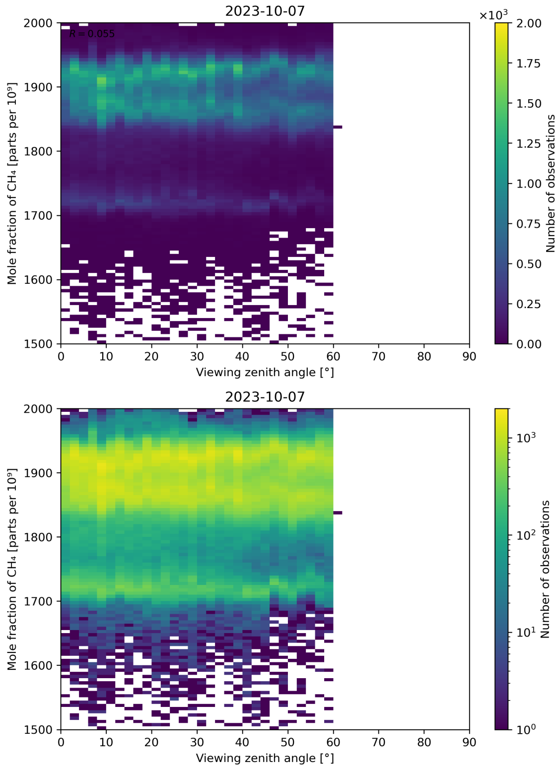
Figure 110: Scatter density plot of “Viewing zenith angle” against “Mole fraction of CH 4 ” for 2023-10-06 to 2023-10-08.
