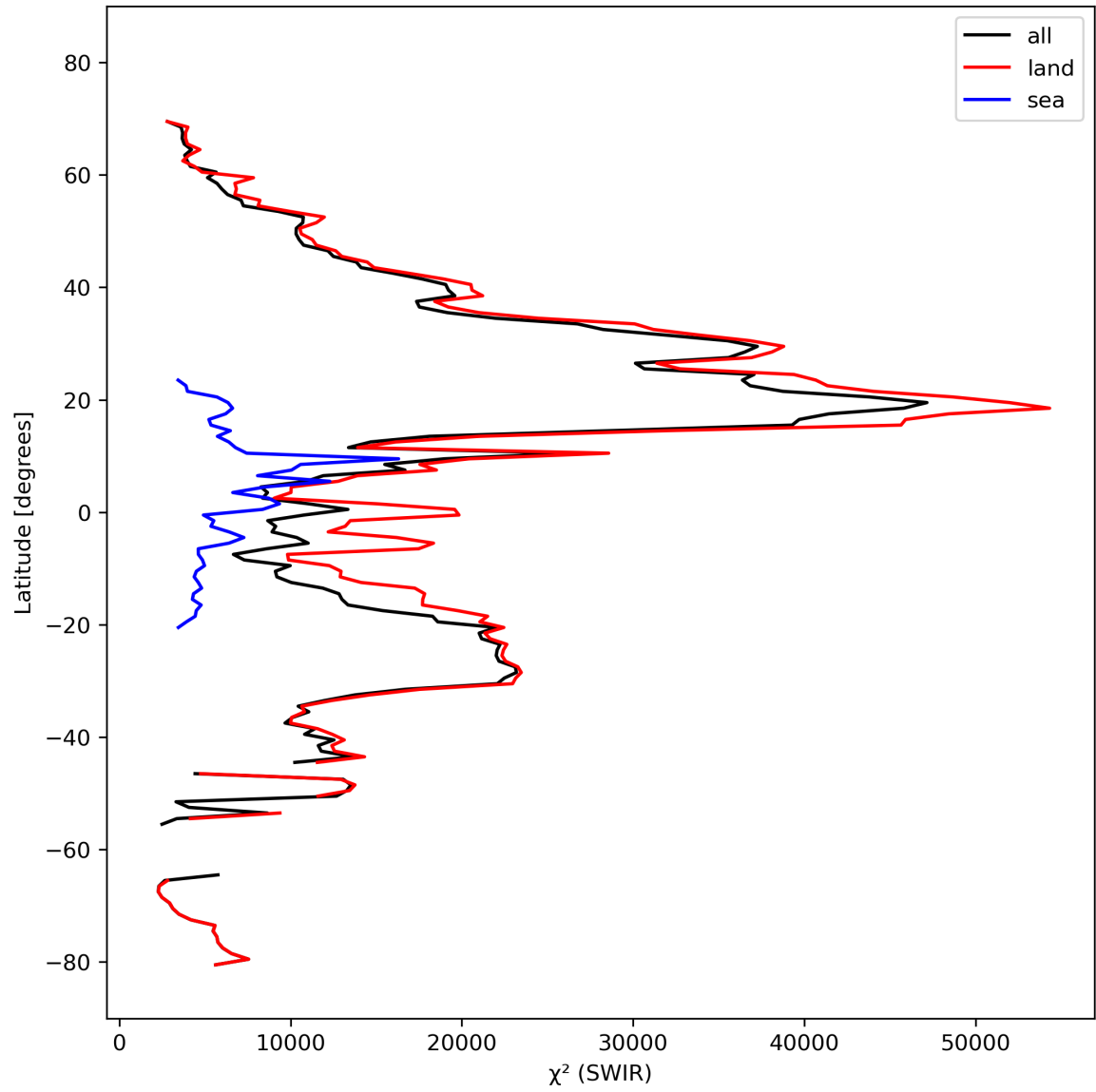
Figure 17: Zonal average of “ \chi^2 (SWIR)” for 2023-10-06 to 2023-10-08.
