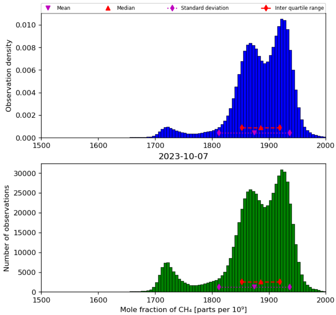
Figure 23: Histogram of “Mole fraction of CH 4 ” for 2023-10-06 to 2023-10-08
