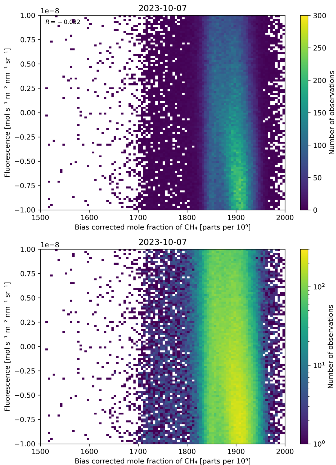
Figure 66: Scatter density plot of “Bias corrected mole fraction of \text{CH}_4 ” against “Fluorescence” for 2023-10-06 to 2023-10-08.
