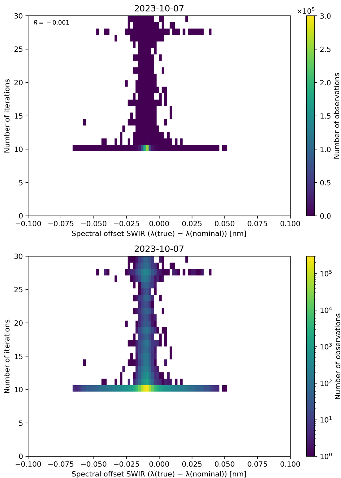
Figure 121: Scatter density plot of “Spectral offset SWIR ( \lambda(\text{true}) - \lambda(\text{nominal}) )” against “Number of iterations” for 2023-10-06 to 2023-10-08.
