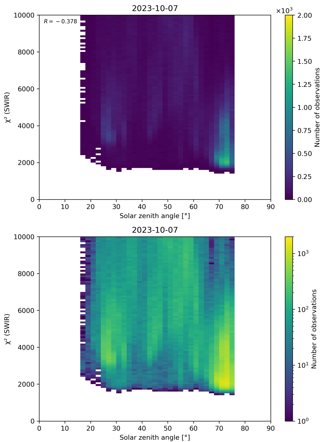
Figure 95: Scatter density plot of “Solar zenith angle” against “ \chi^2 (SWIR)” for 2023-10-06 to 2023-10-08.
