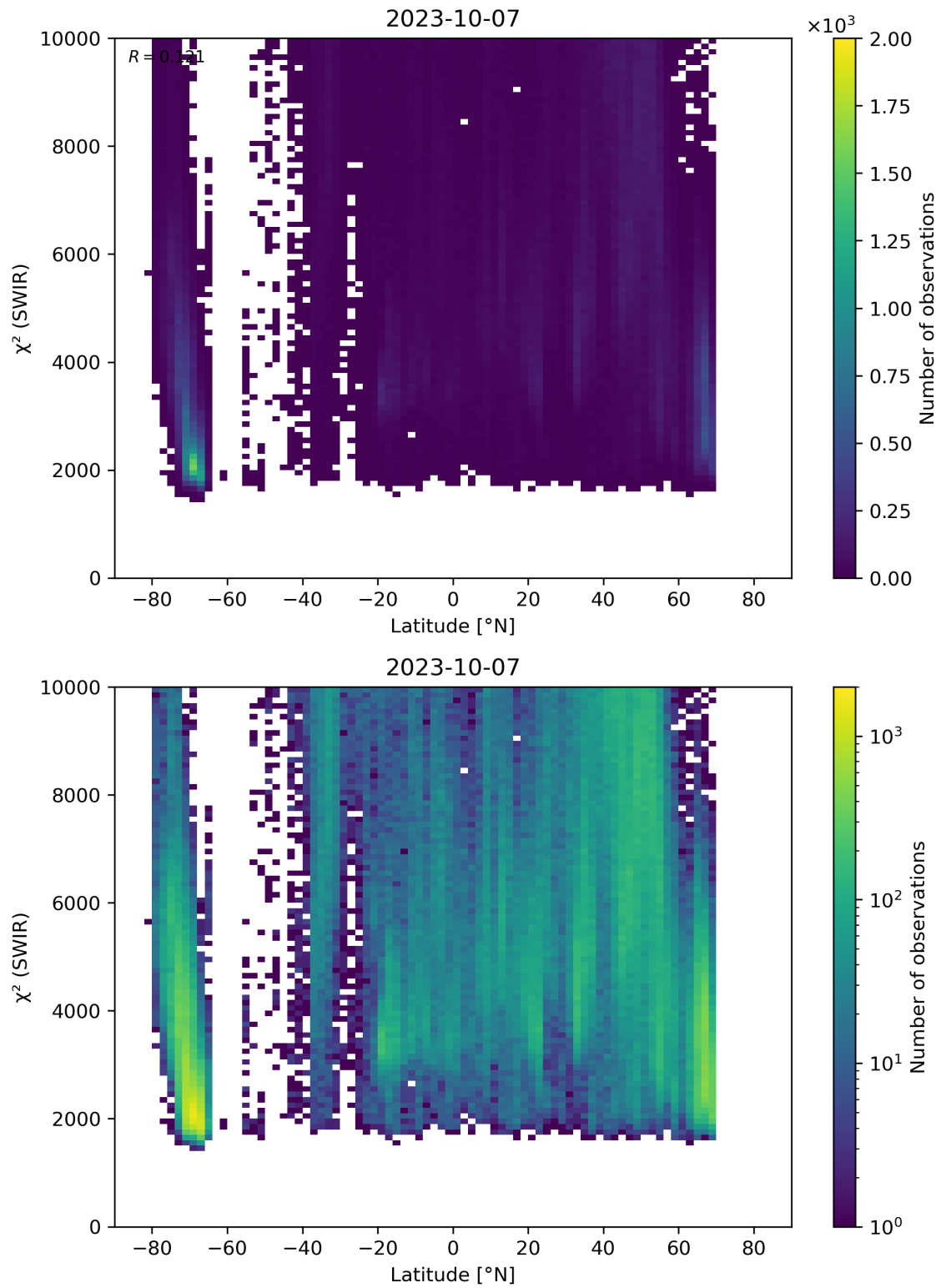
Figure 54: Scatter density plot of “Latitude” against “ \chi^2 (SWIR)” for 2023-10-06 to 2023-10-08.
