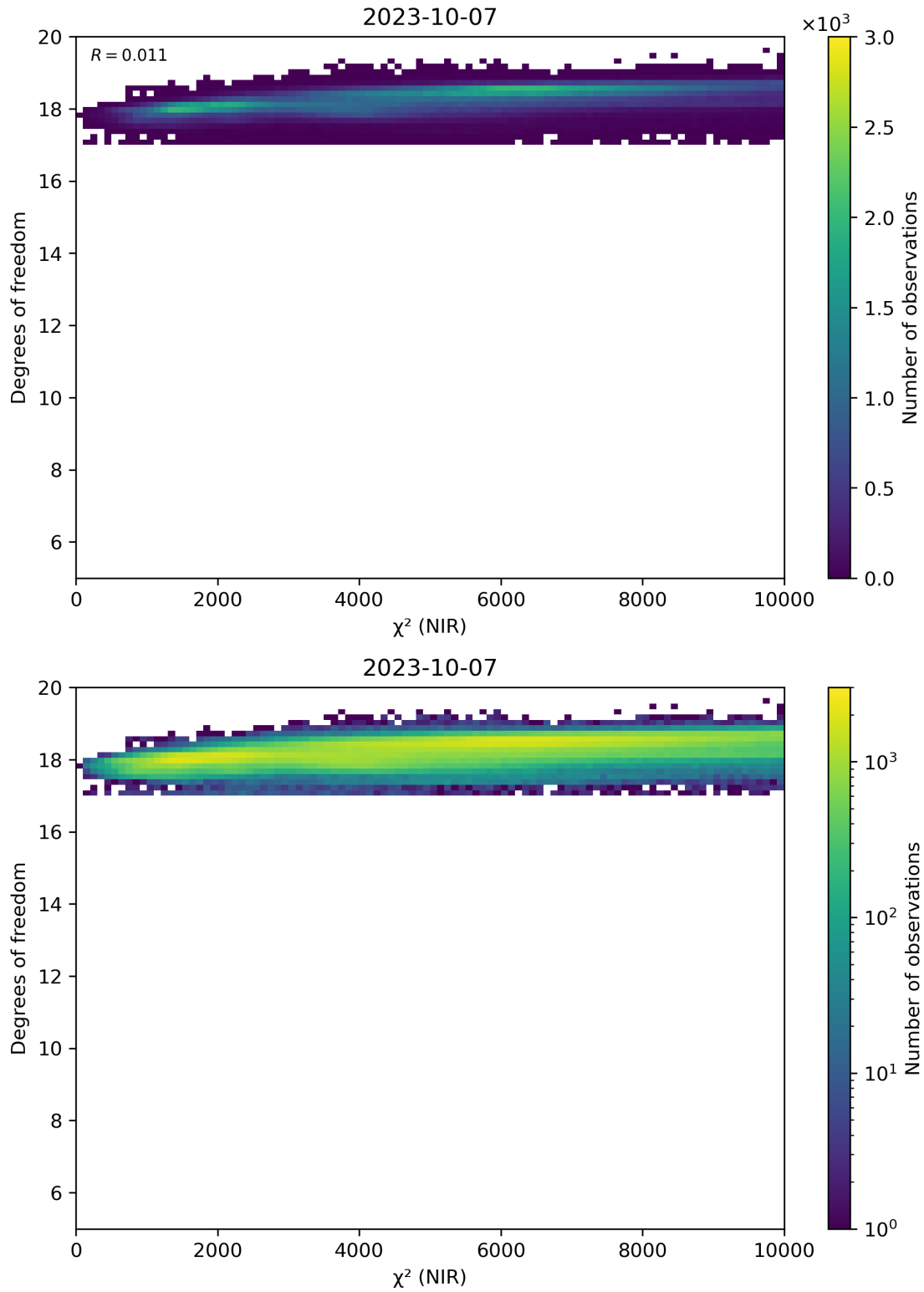
Figure 44: Scatter density plot of “ \chi^2 (NIR)” against “Degrees of freedom” for 2023-10-06 to 2023-10-08.
