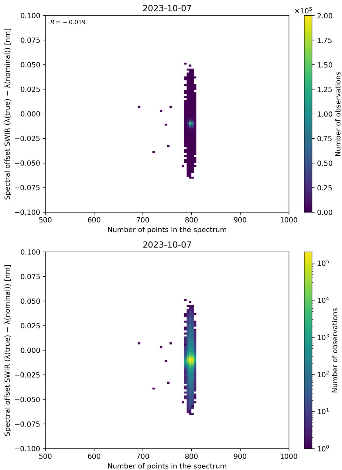
Figure 93: Scatter density plot of “Number of points in the spectrum” against “Spectral offset SWIR ( \lambda(\text{true}) - \lambda(\text{nominal}) )” for 2023-10-06 to 2023-10-08.
