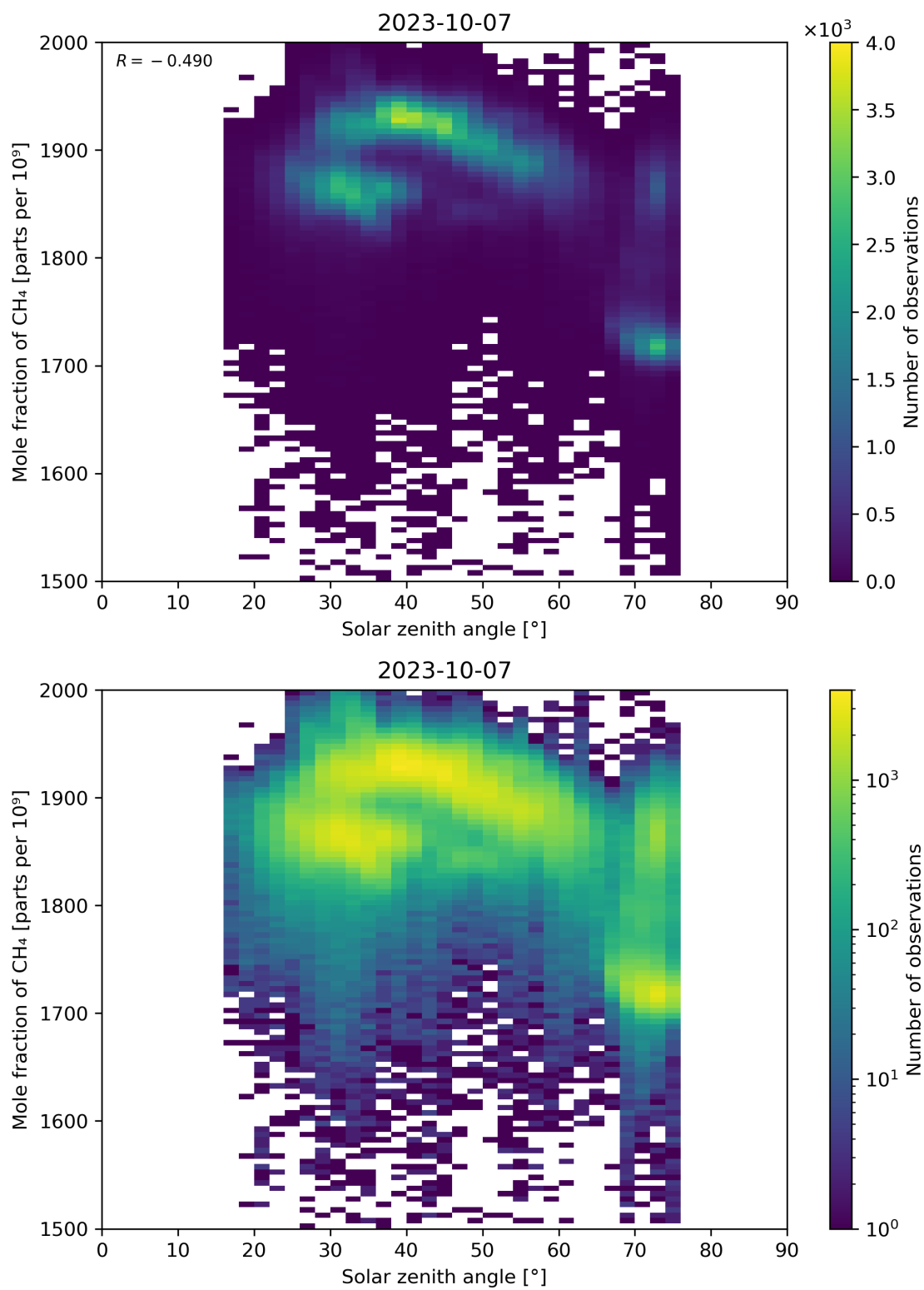
Figure 99: Scatter density plot of “Solar zenith angle” against “Mole fraction of CH 4 ” for 2023-10-06 to 2023-10-08.
