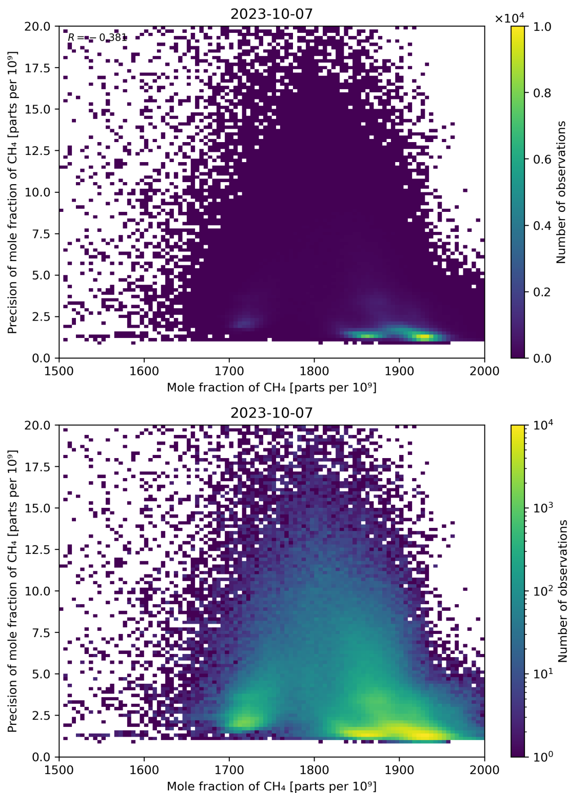
Figure 75: Scatter density plot of “Mole fraction of CH 4 ” against “Precision of mole fraction of CH 4 ” for 2023-10-06 to 2023-10-08.
