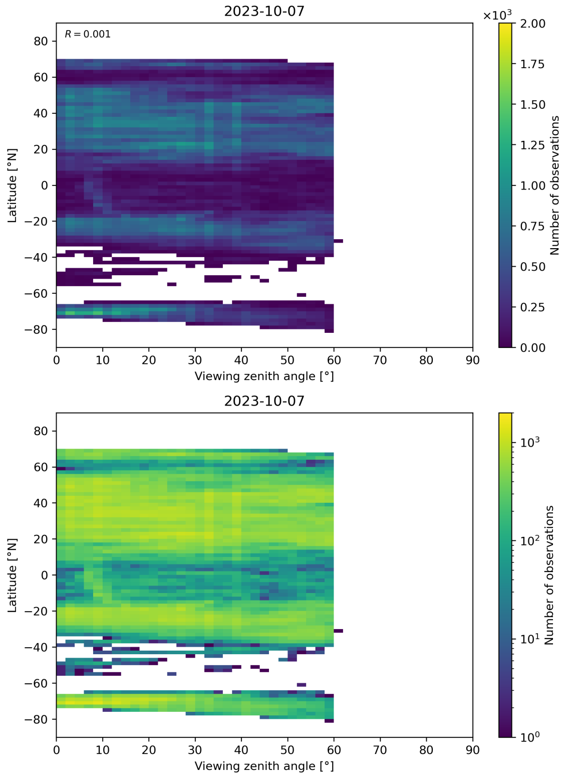
Figure 109: Scatter density plot of “Viewing zenith angle” against “Latitude” for 2023-10-06 to 2023-10-08.
