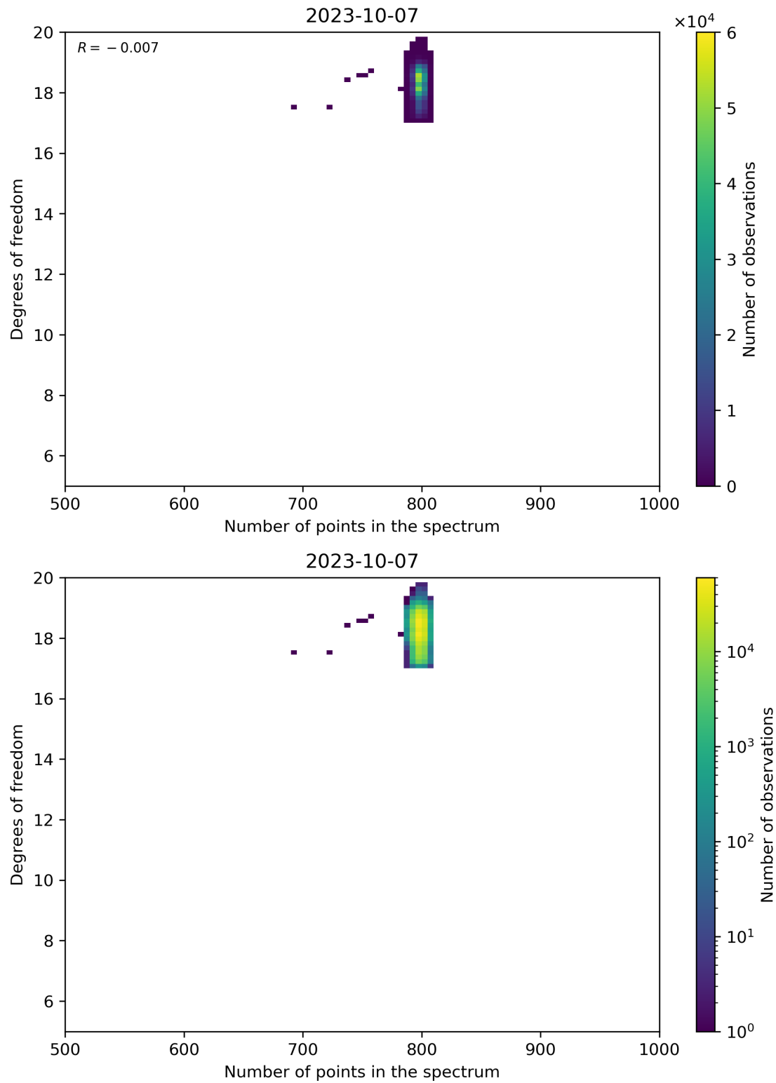
Figure 90: Scatter density plot of “Number of points in the spectrum” against “Degrees of freedom” for 2023-10-06 to 2023-10-08.
