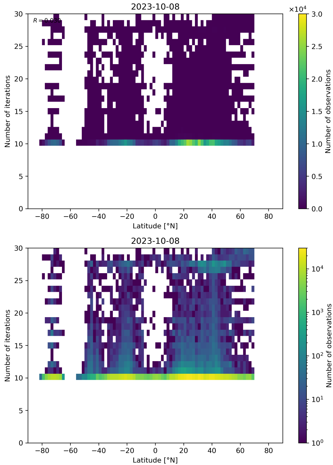
Figure 60: Scatter density plot of “Latitude” against “Number of iterations” for 2023-10-07 to 2023-10-09.
