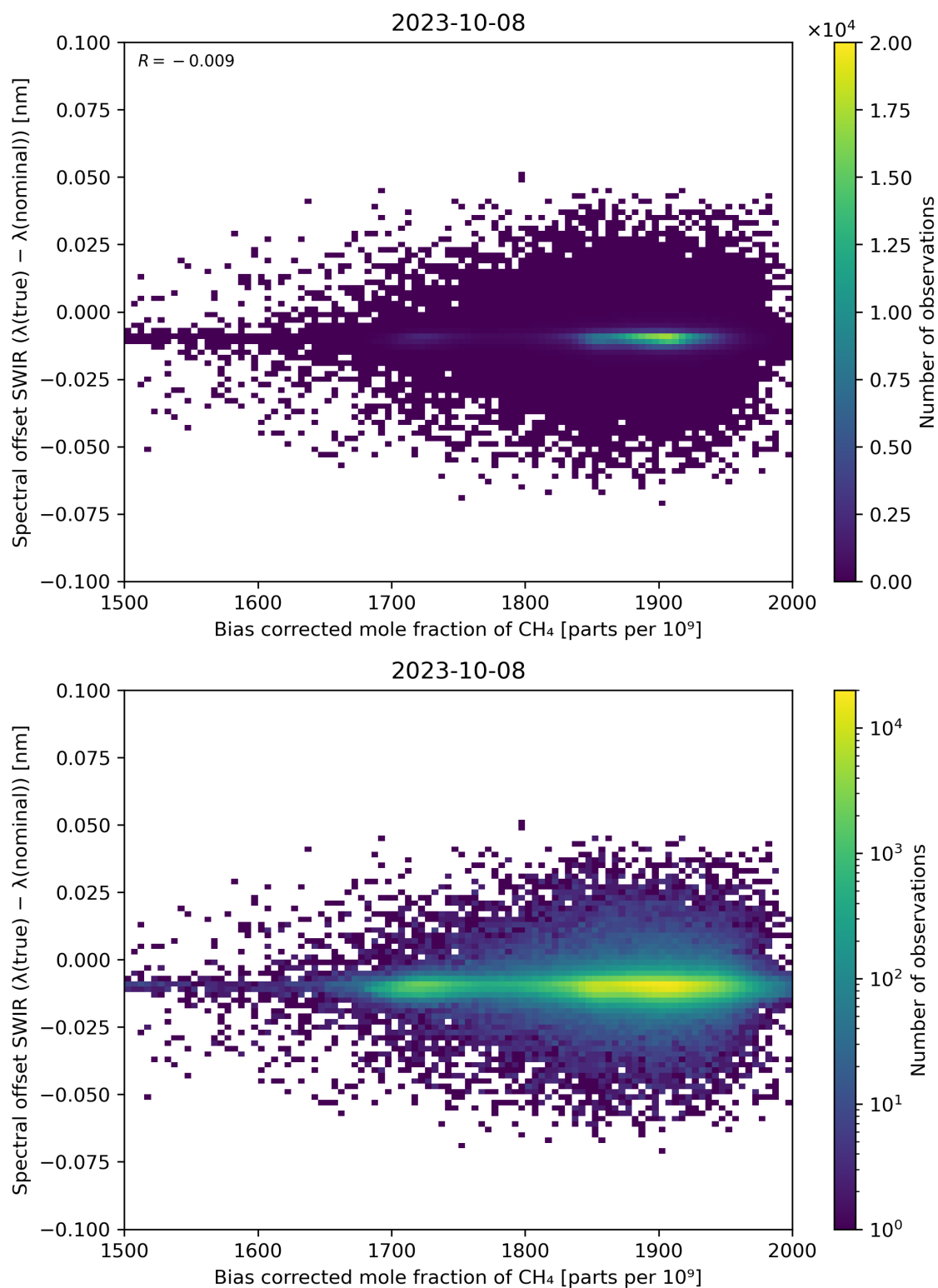
Figure 69: Scatter density plot of “Bias corrected mole fraction of \text{CH}_4 ” against “Spectral offset SWIR ( \lambda(\text{true}) - \lambda(\text{nominal}) )” for 2023-10-07 to 2023-10-09.
