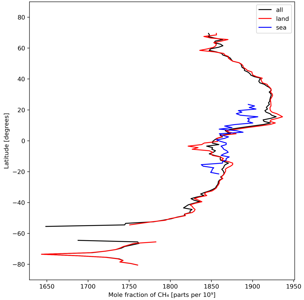
Figure 12: Zonal average of “Mole fraction of \text{CH}_4 ” for 2023-10-07 to 2023-10-09.
