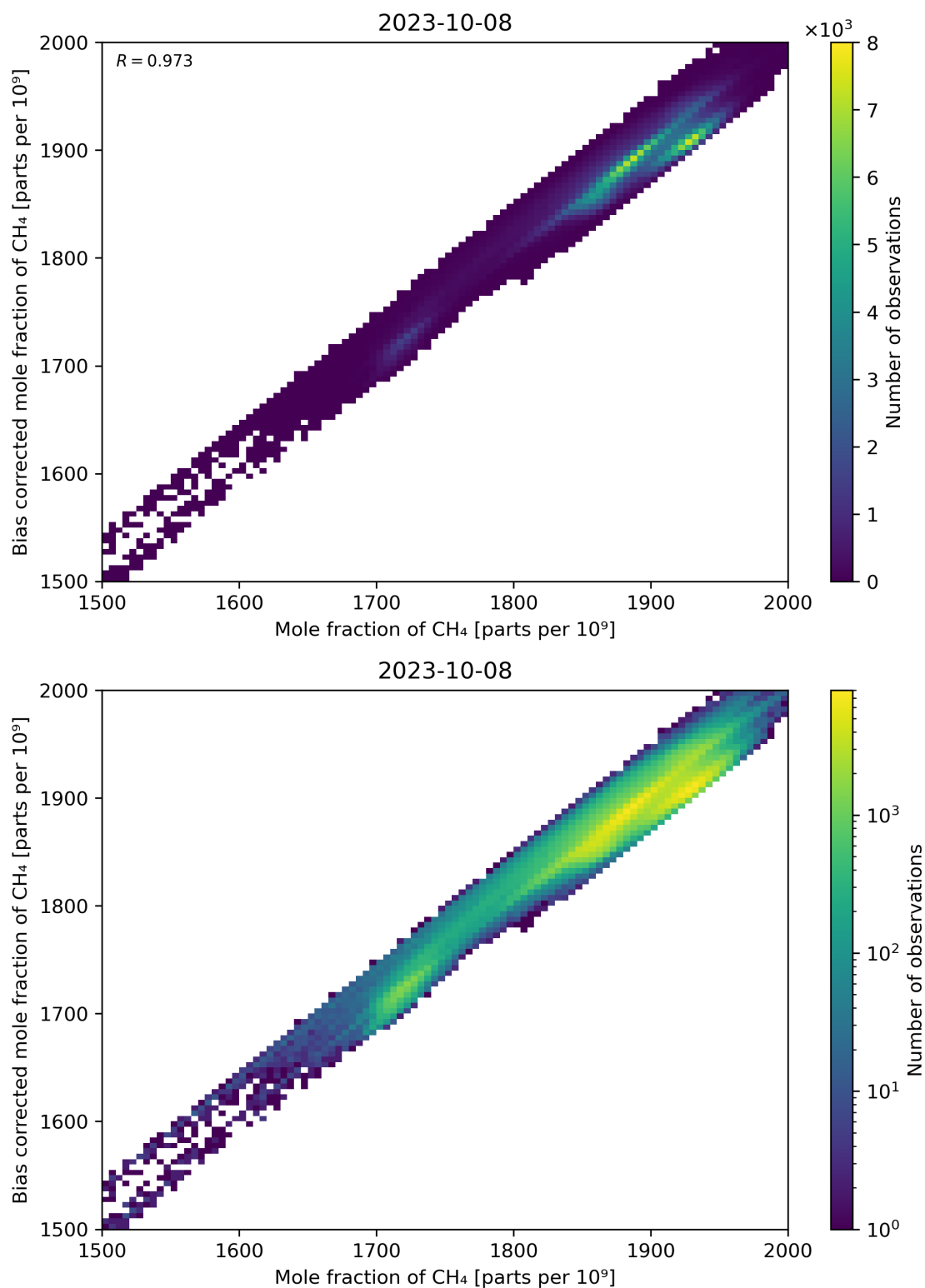
Figure 74: Scatter density plot of “Mole fraction of CH 4 ” against “Bias corrected mole fraction of CH 4 ” for 2023-10-07 to 2023-10-09.
