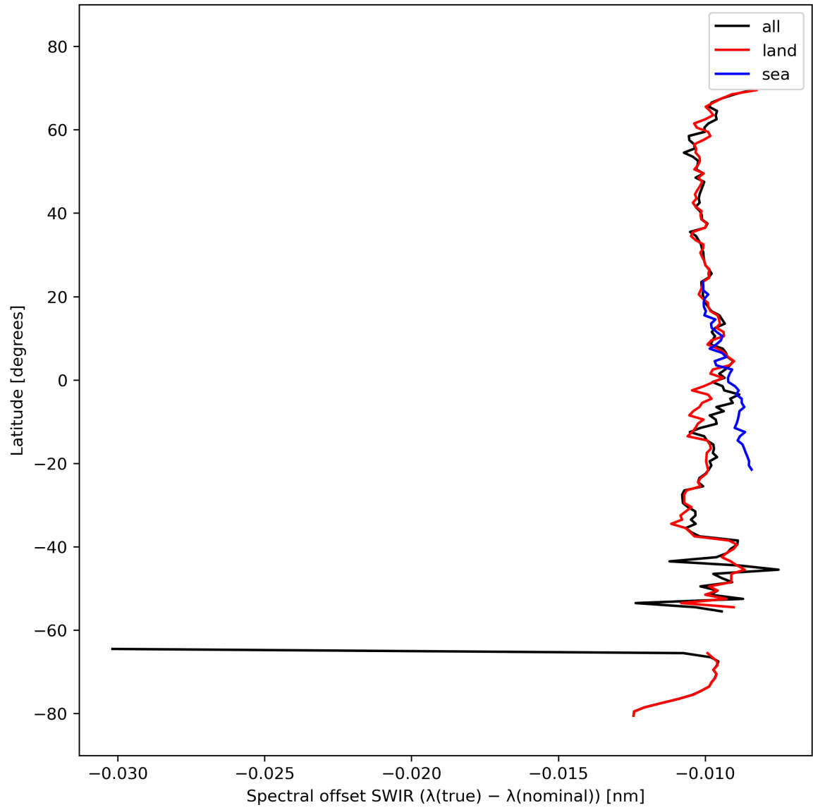
Figure 16: Zonal average of “Spectral offset SWIR ( \lambda(\text{true}) - \lambda(\text{nominal}) )” for 2023-10-07 to 2023-10-09.
