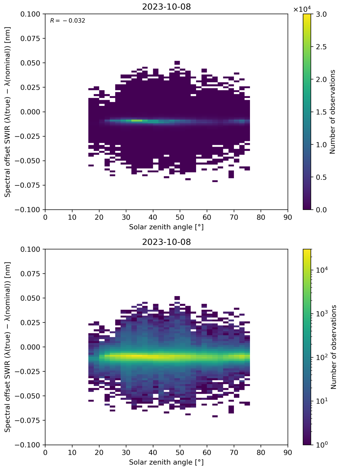
Figure 104: Scatter density plot of “Solar zenith angle” against “Spectral offset SWIR ( \lambda(\text{true}) - \lambda(\text{nominal}) )” for 2023-10-07 to 2023-10-09.
