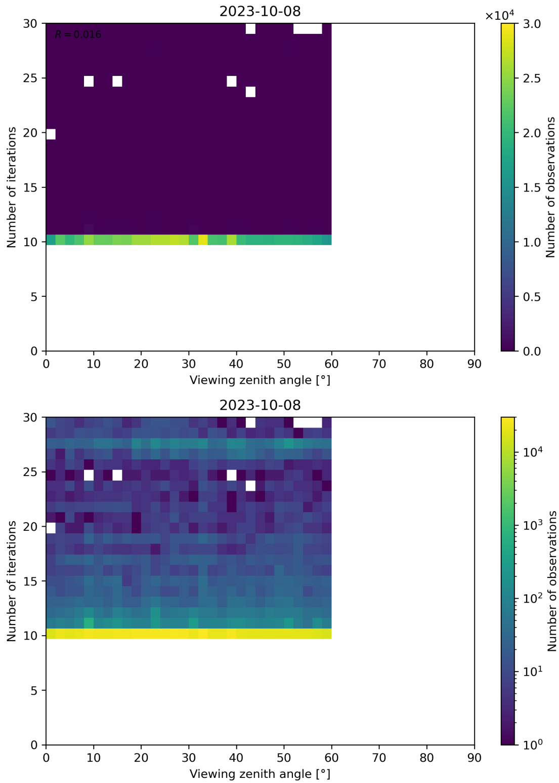
Figure 113: Scatter density plot of “Viewing zenith angle” against “Number of iterations” for 2023-10-07 to 2023-10-09.
