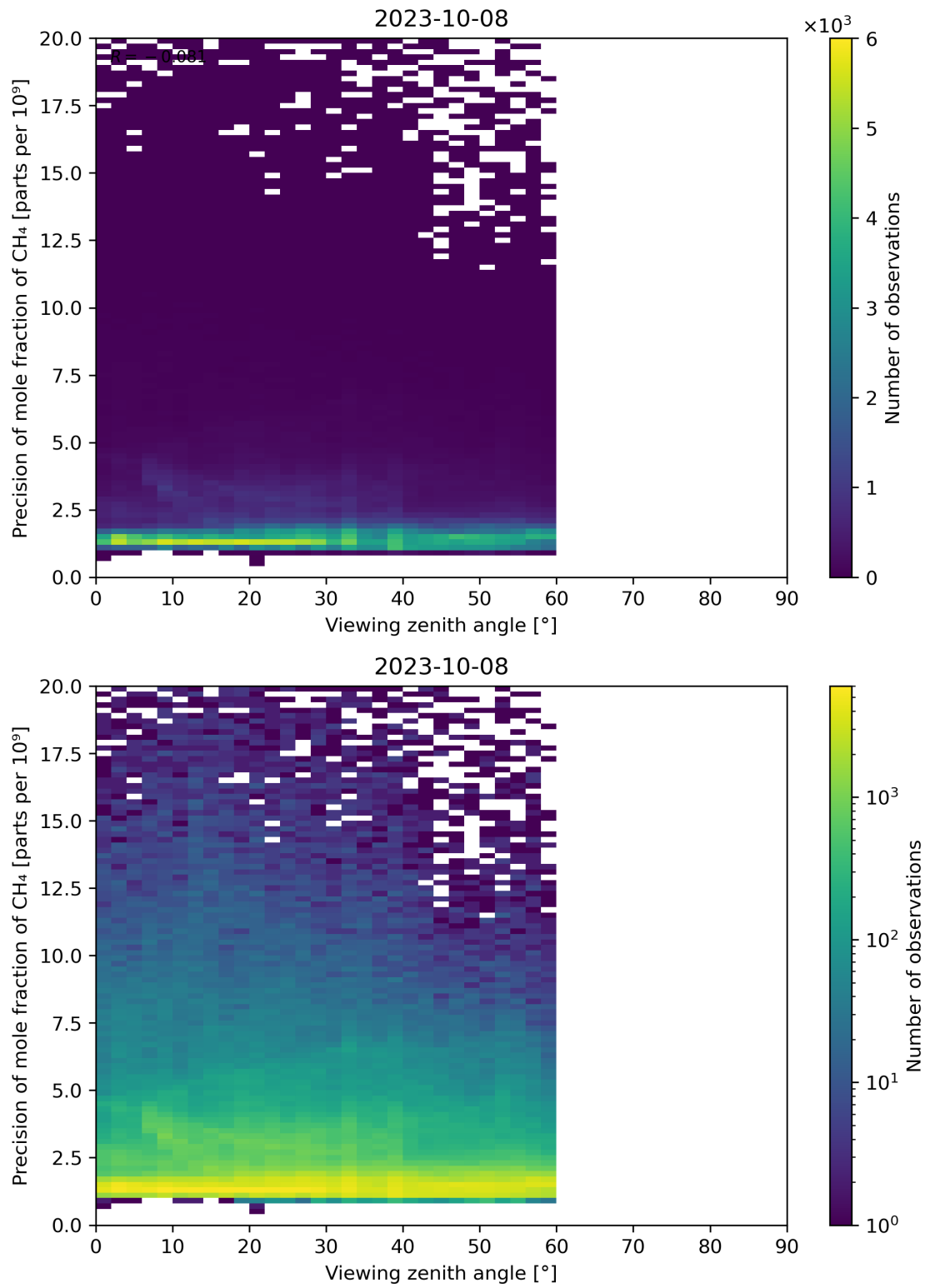
Figure 112: Scatter density plot of “Viewing zenith angle” against “Precision of mole fraction of CH 4 ” for 2023-10-07 to 2023-10-09.
