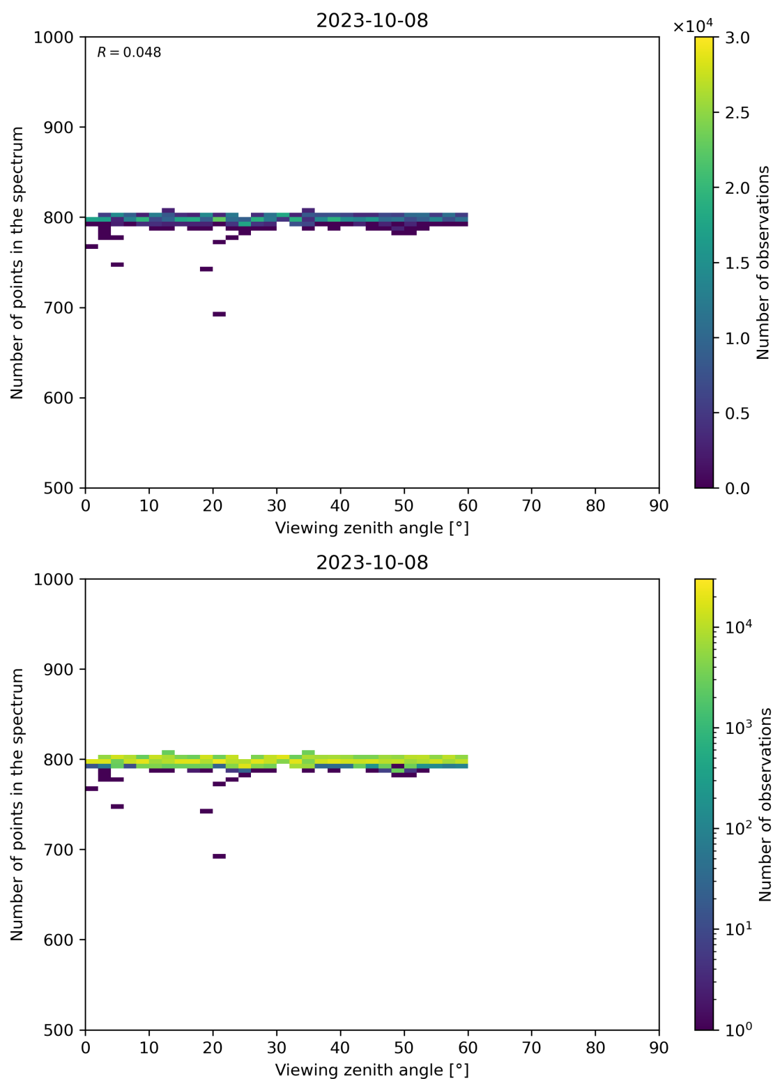
Figure 114: Scatter density plot of “Viewing zenith angle” against “Number of points in the spectrum” for 2023-10-07 to 2023-10-09.
