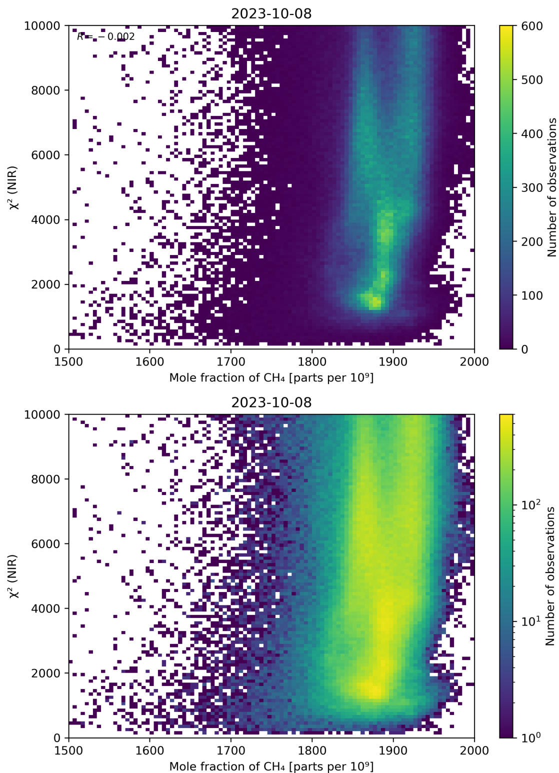
Figure 70: Scatter density plot of “Mole fraction of \text{CH}_4 ” against “ \chi^2 (NIR)” for 2023-10-07 to 2023-10-09.
