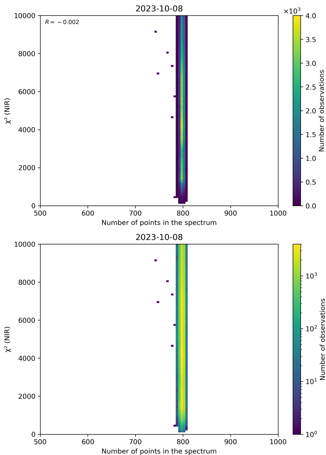
Figure 88: Scatter density plot of “Number of points in the spectrum” against “ \chi^2 (NIR)” for 2023-10-07 to 2023-10-09.
