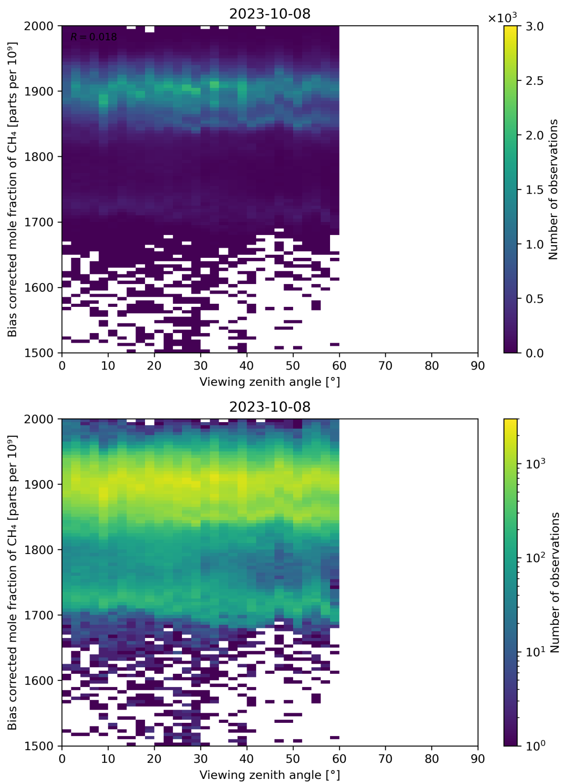
Figure 111: Scatter density plot of “Viewing zenith angle” against “Bias corrected mole fraction of CH 4 ” for 2023-10-07 to 2023-10-09.
