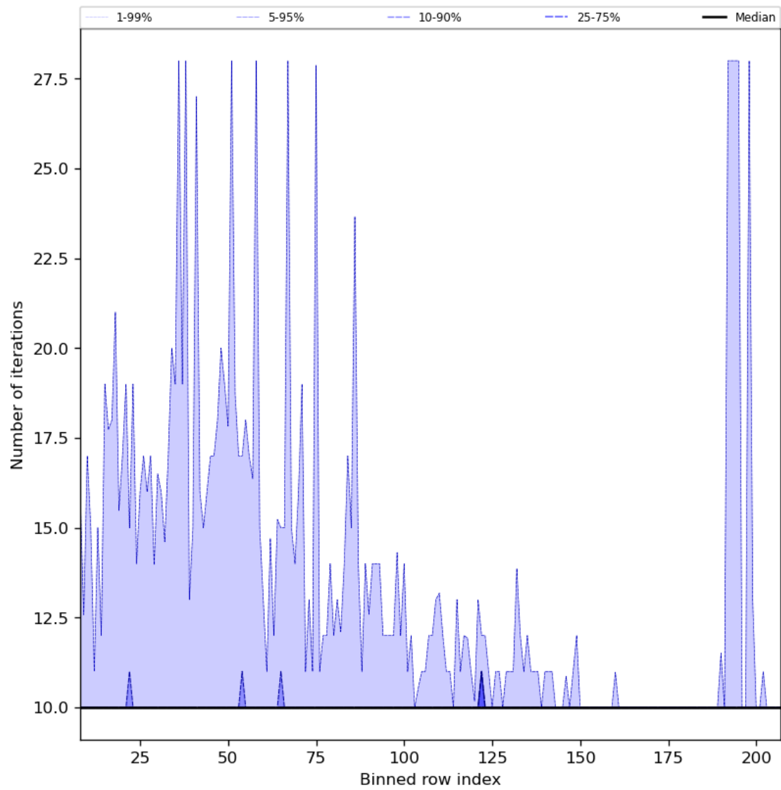
Figure 42: Along track statistics of “Number of iterations” for 2023-10-07 to 2023-10-09
