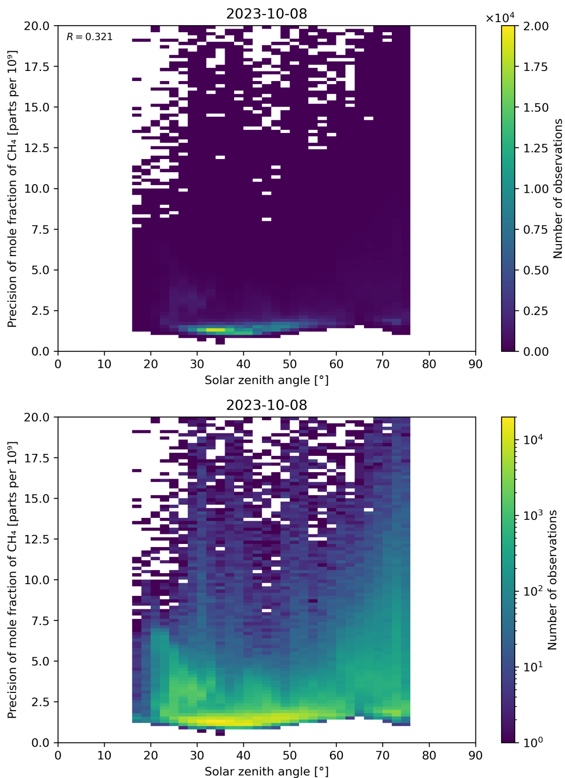
Figure 101: Scatter density plot of “Solar zenith angle” against “Precision of mole fraction of CH 4 ” for 2023-10-07 to 2023-10-09.
