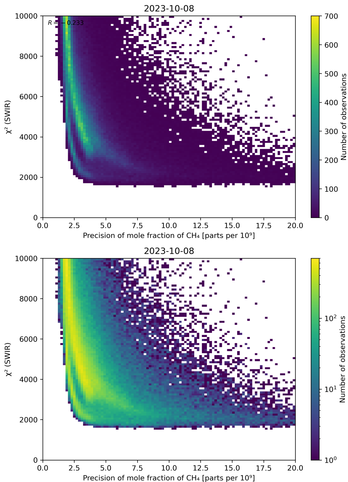
Figure 79: Scatter density plot of “Precision of mole fraction of CH 4 ” against “ \chi^2 (SWIR)” for 2023-10-07 to 2023-10-09.
