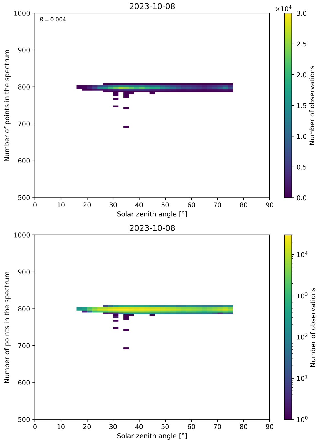
Figure 103: Scatter density plot of “Solar zenith angle” against “Number of points in the spectrum” for 2023-10-07 to 2023-10-09.
