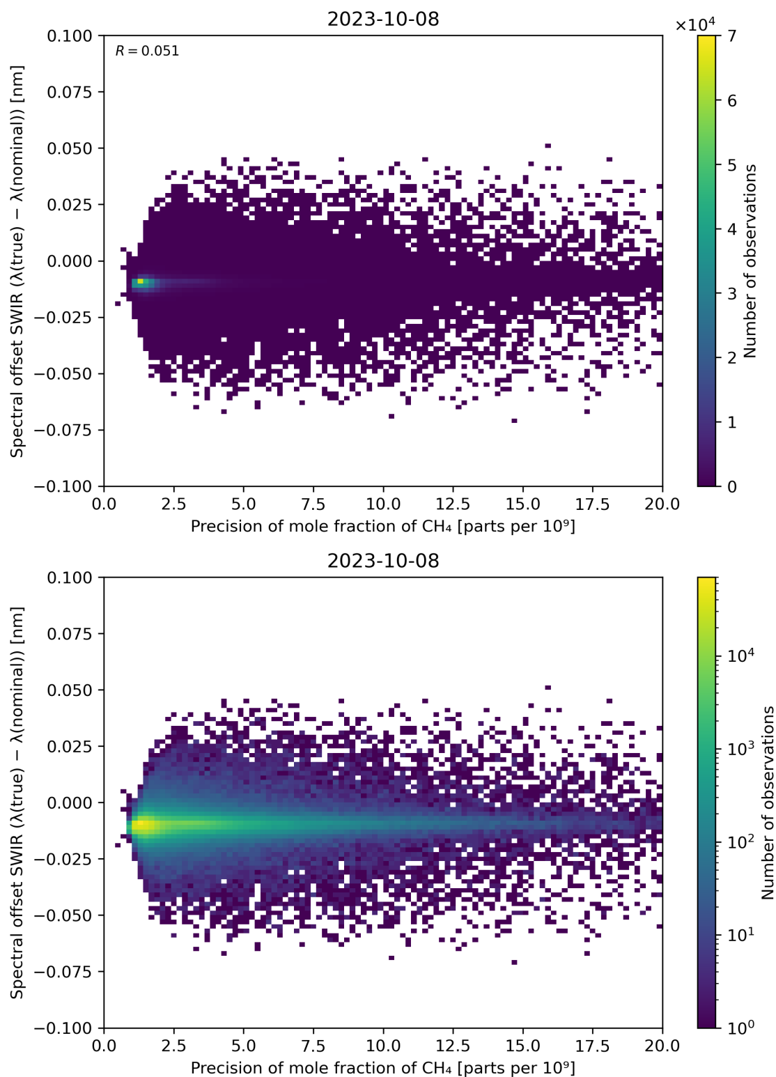
Figure 85: Scatter density plot of “Precision of mole fraction of CH 4 ” against “Spectral offset SWIR ( \lambda(\text{true}) - \lambda(\text{nominal}) )” for 2023-10-07 to 2023-10-09.
