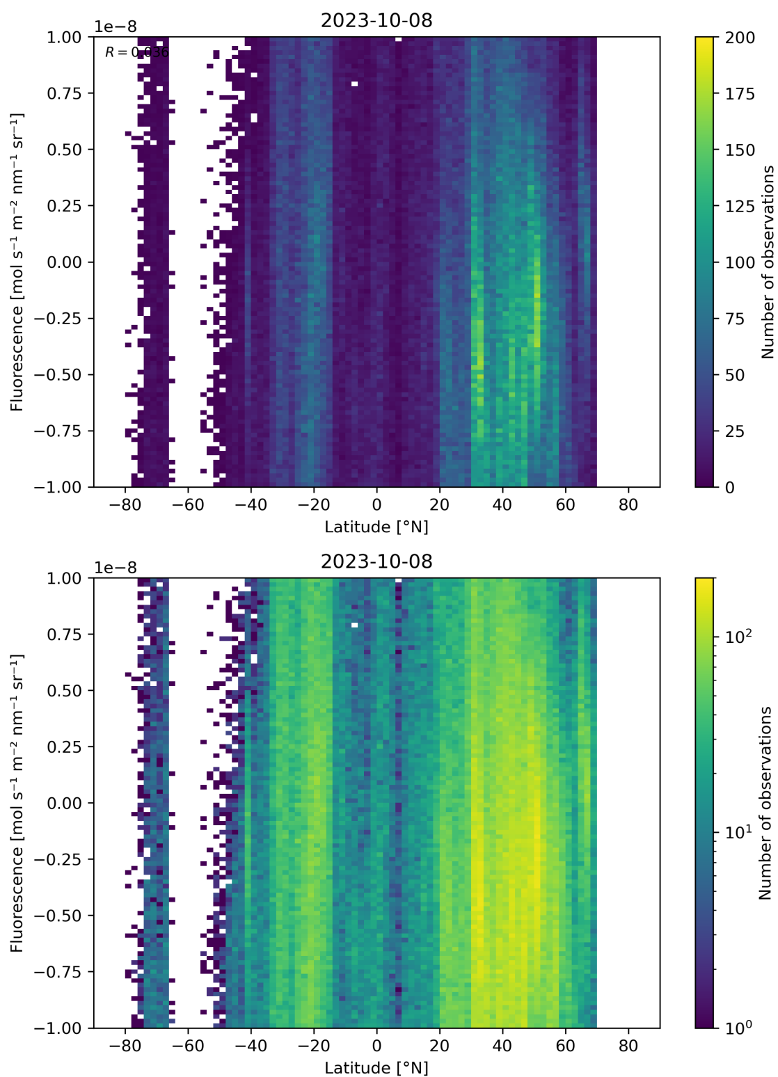
Figure 56: Scatter density plot of “Latitude” against “Fluorescence” for 2023-10-07 to 2023-10-09.
