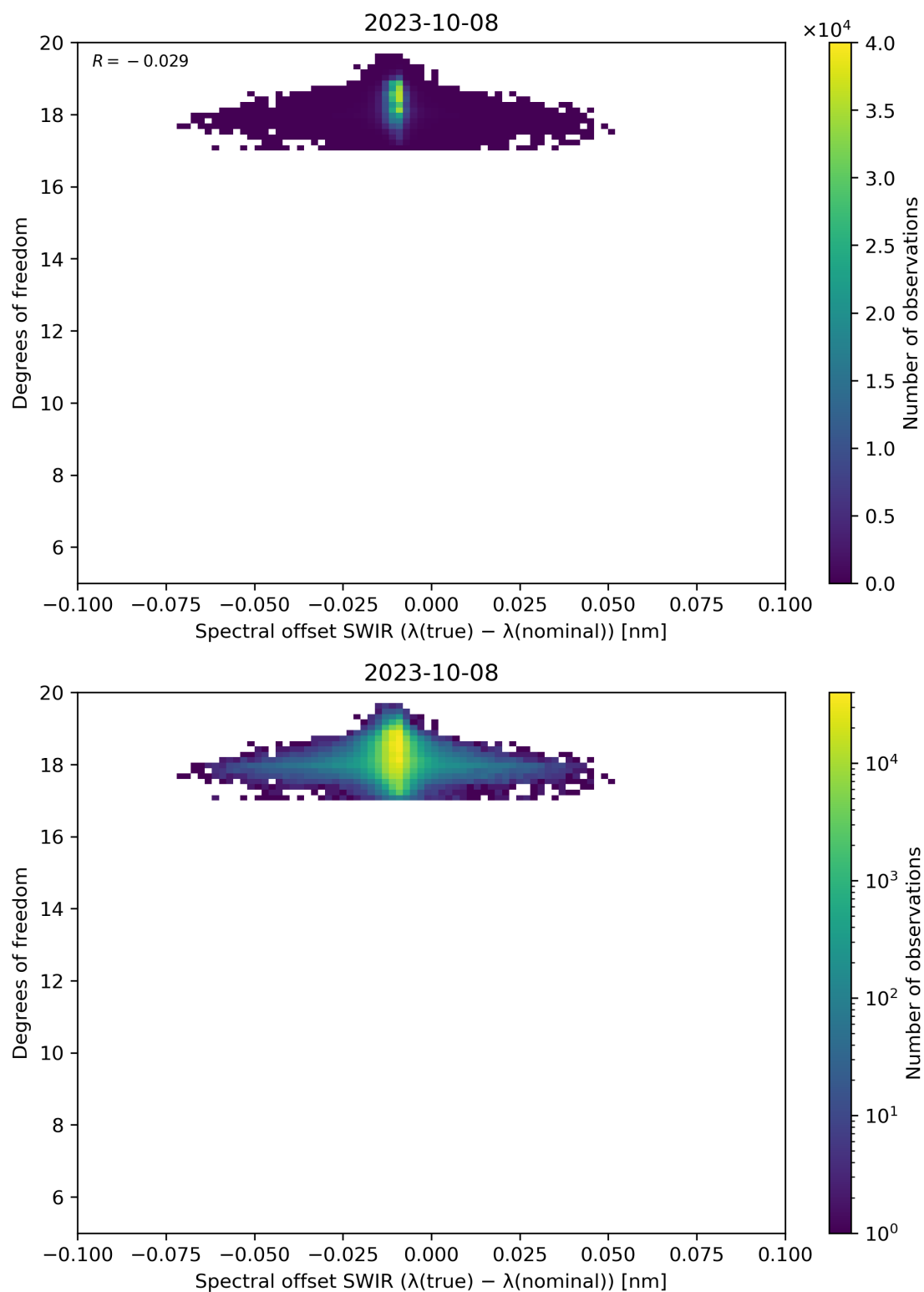
Figure 119: Scatter density plot of “Spectral offset SWIR ( \lambda(\text{true}) - \lambda(\text{nominal}) )” against “Degrees of freedom” for 2023-10-07 to 2023-10-09.
