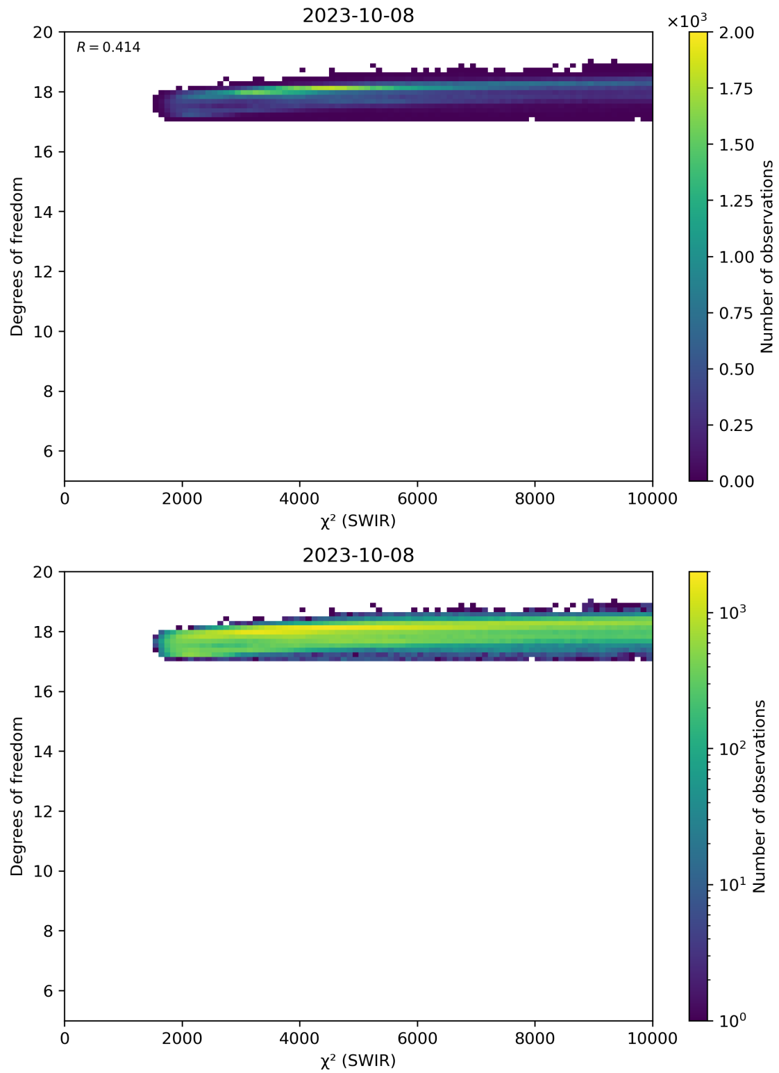
Figure 48: Scatter density plot of “ \chi^2 (SWIR)” against “Degrees of freedom” for 2023-10-07 to 2023-10-09.
