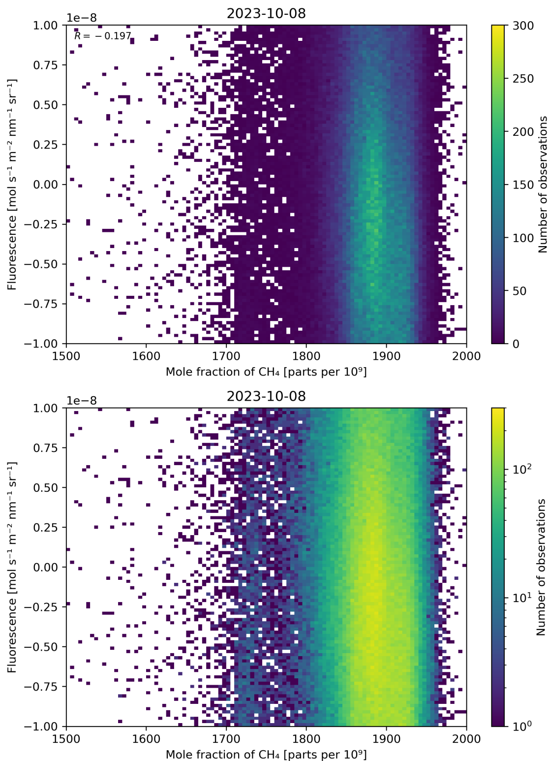
Figure 73: Scatter density plot of “Mole fraction of \text{CH}_4 ” against “Fluorescence” for 2023-10-07 to 2023-10-09.
