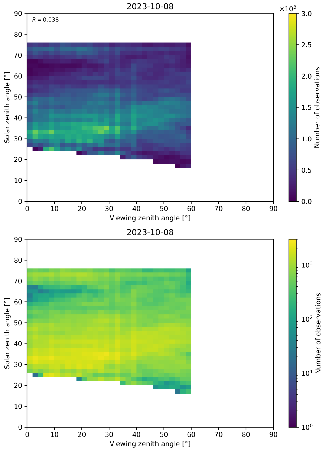
Figure 115: Scatter density plot of “Viewing zenith angle” against “Solar zenith angle” for 2023-10-07 to 2023-10-09.
