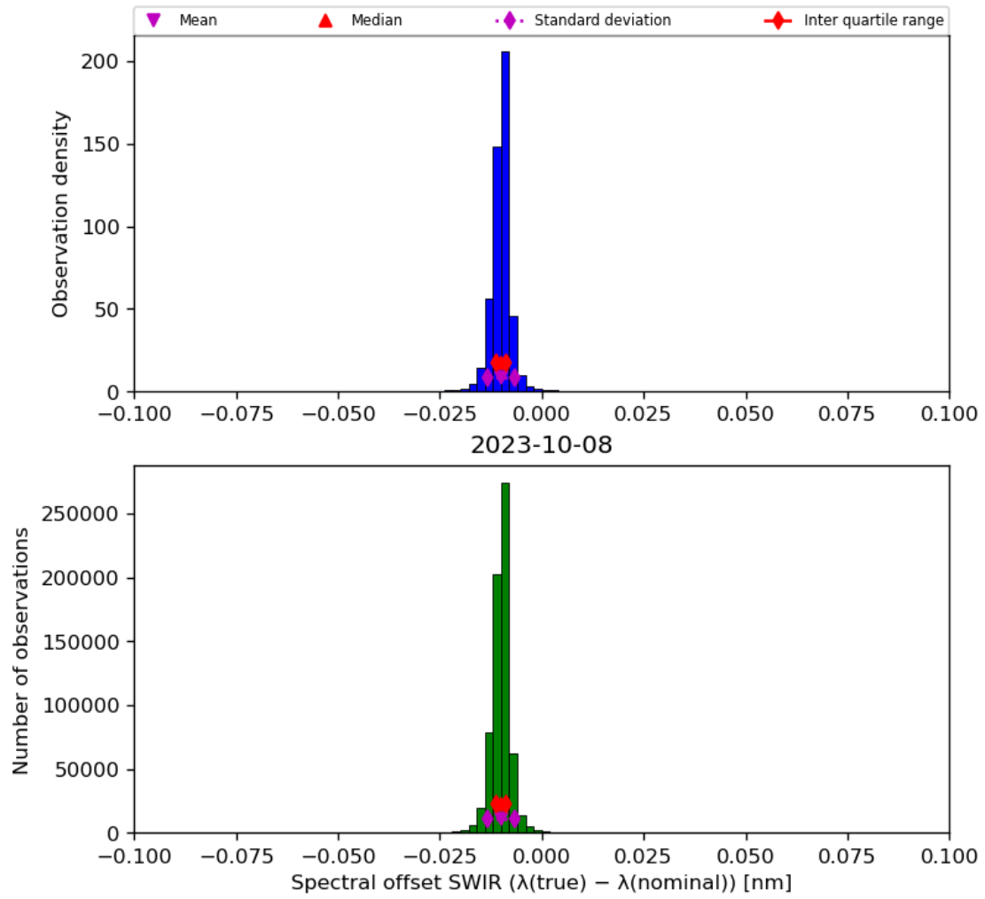
Figure 27: Histogram of “Spectral offset SWIR ( \lambda(\text{true}) - \lambda(\text{nominal}) )” for 2023-10-07 to 2023-10-09
