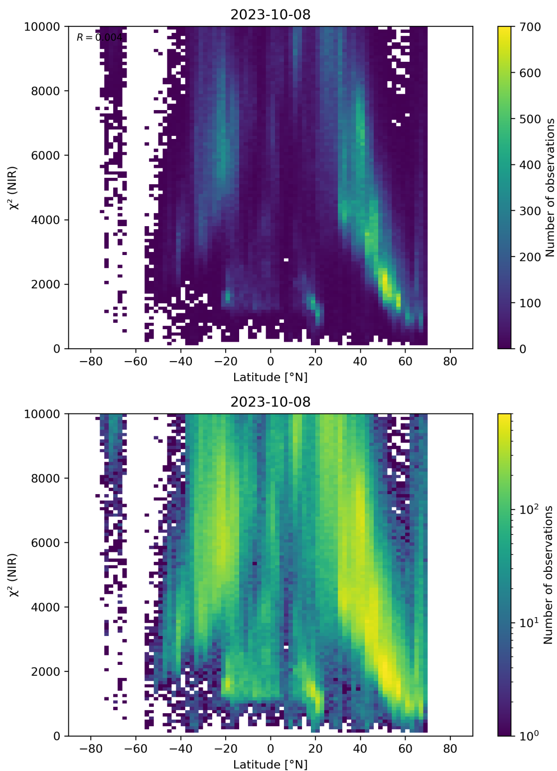
Figure 53: Scatter density plot of “Latitude” against “ \chi^2 (NIR)” for 2023-10-07 to 2023-10-09.
