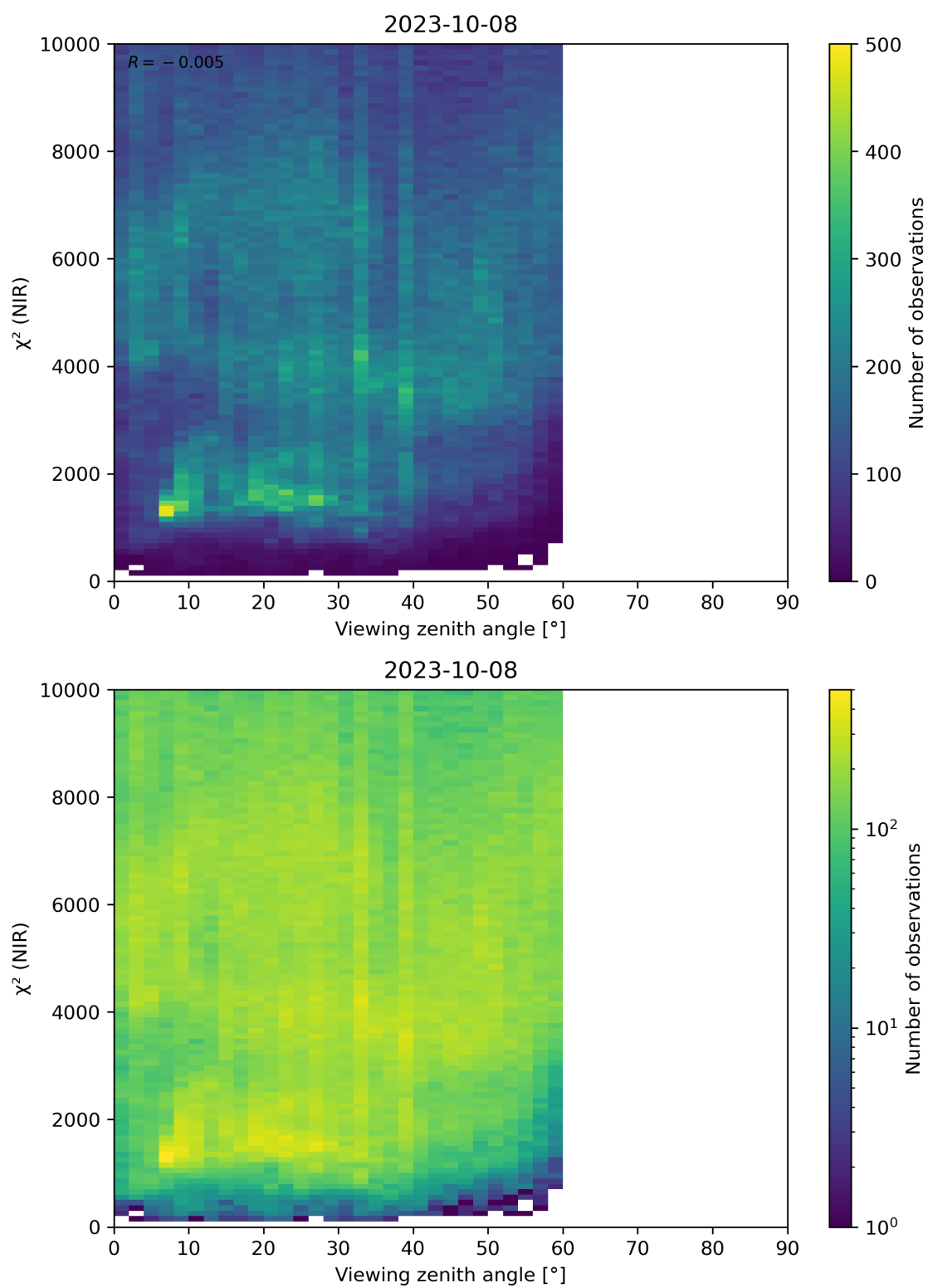
Figure 105: Scatter density plot of “Viewing zenith angle” against “ \chi^2 (NIR)” for 2023-10-07 to 2023-10-09.
