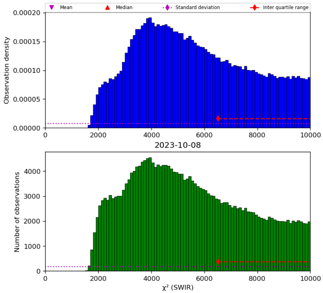
Figure 28: Histogram of “ \chi^2 (SWIR)” for 2023-10-07 to 2023-10-09
