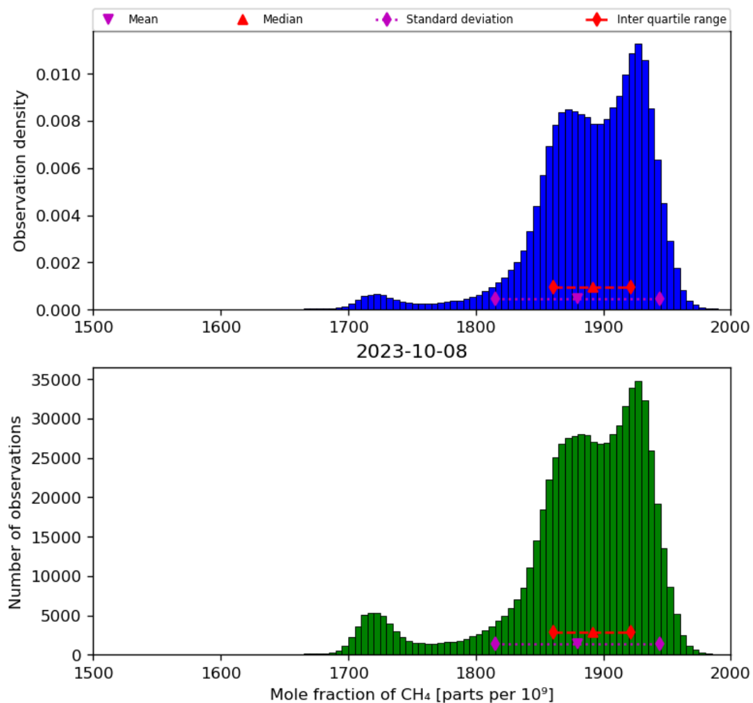
Figure 23: Histogram of “Mole fraction of CH 4 ” for 2023-10-07 to 2023-10-09
