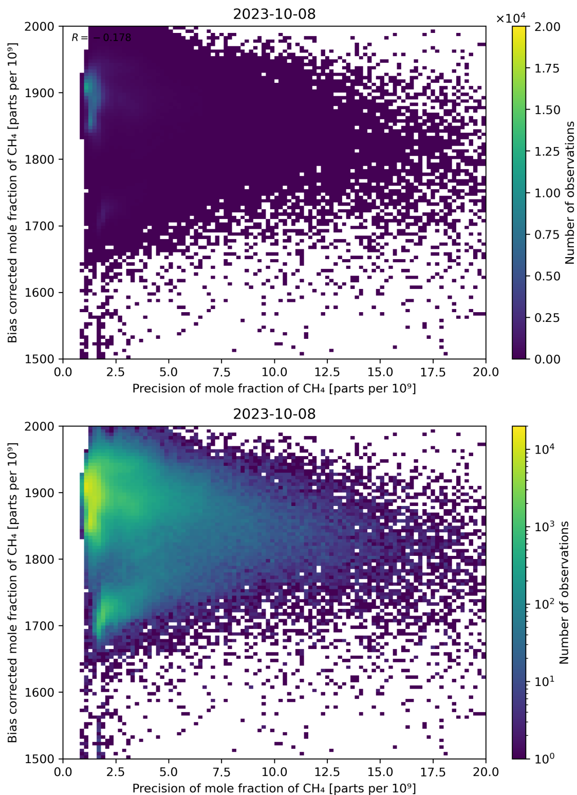
Figure 82: Scatter density plot of “Precision of mole fraction of CH 4 ” against “Bias corrected mole fraction of CH 4 ” for 2023-10-07 to 2023-10-09.
