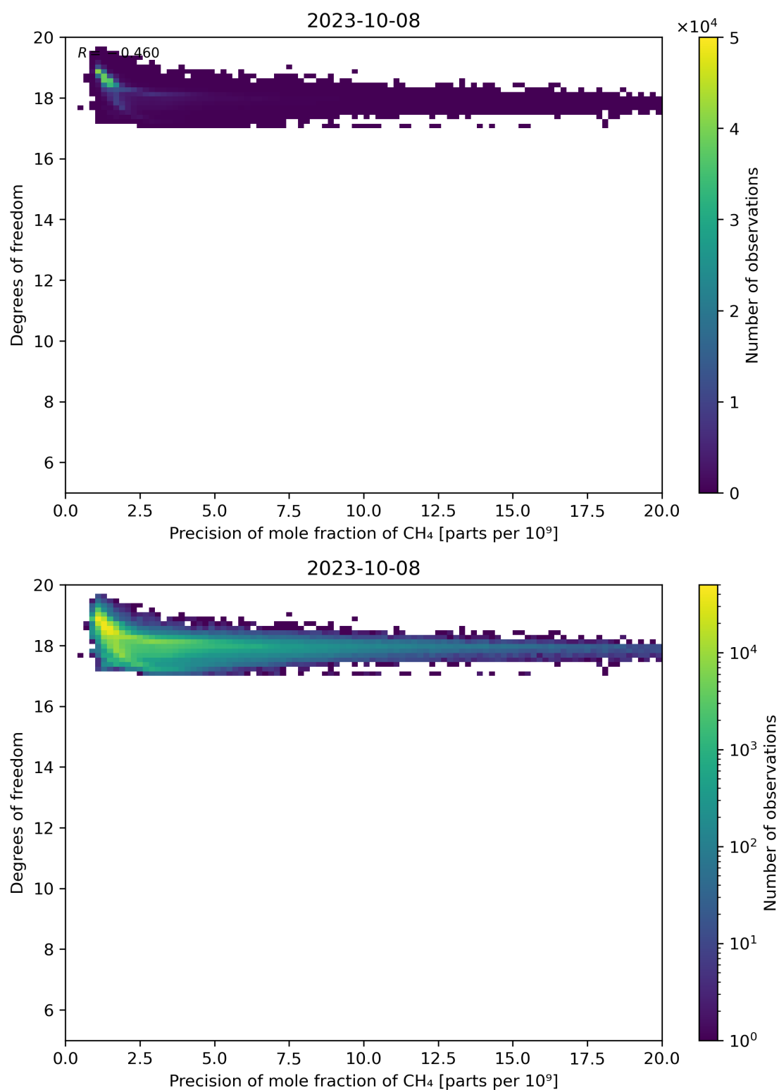
Figure 80: Scatter density plot of “Precision of mole fraction of CH 4 ” against “Degrees of freedom” for 2023-10-07 to 2023-10-09.
