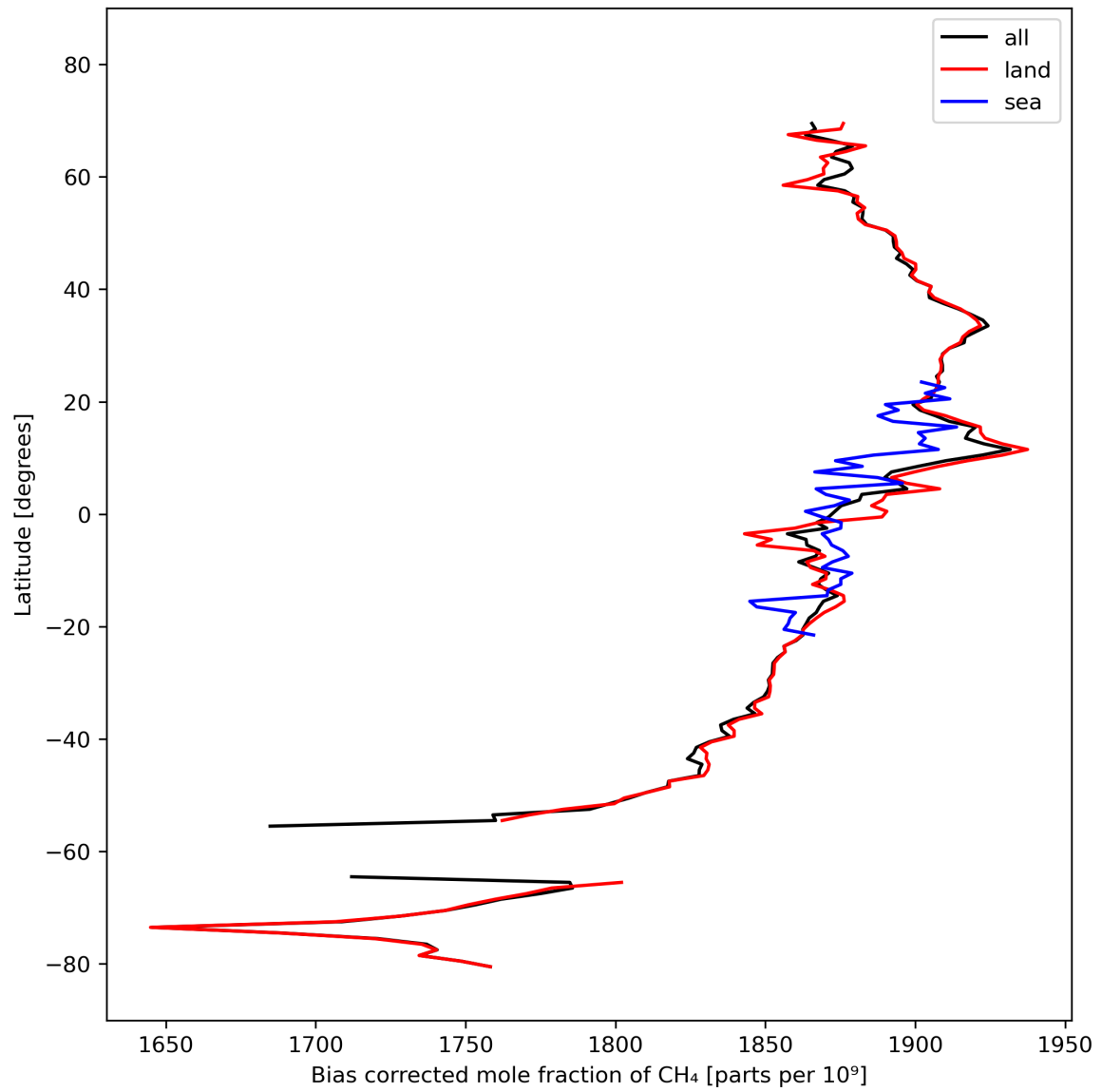
Figure 14: Zonal average of “Bias corrected mole fraction of CH 4 ” for 2023-10-07 to 2023-10-09.
