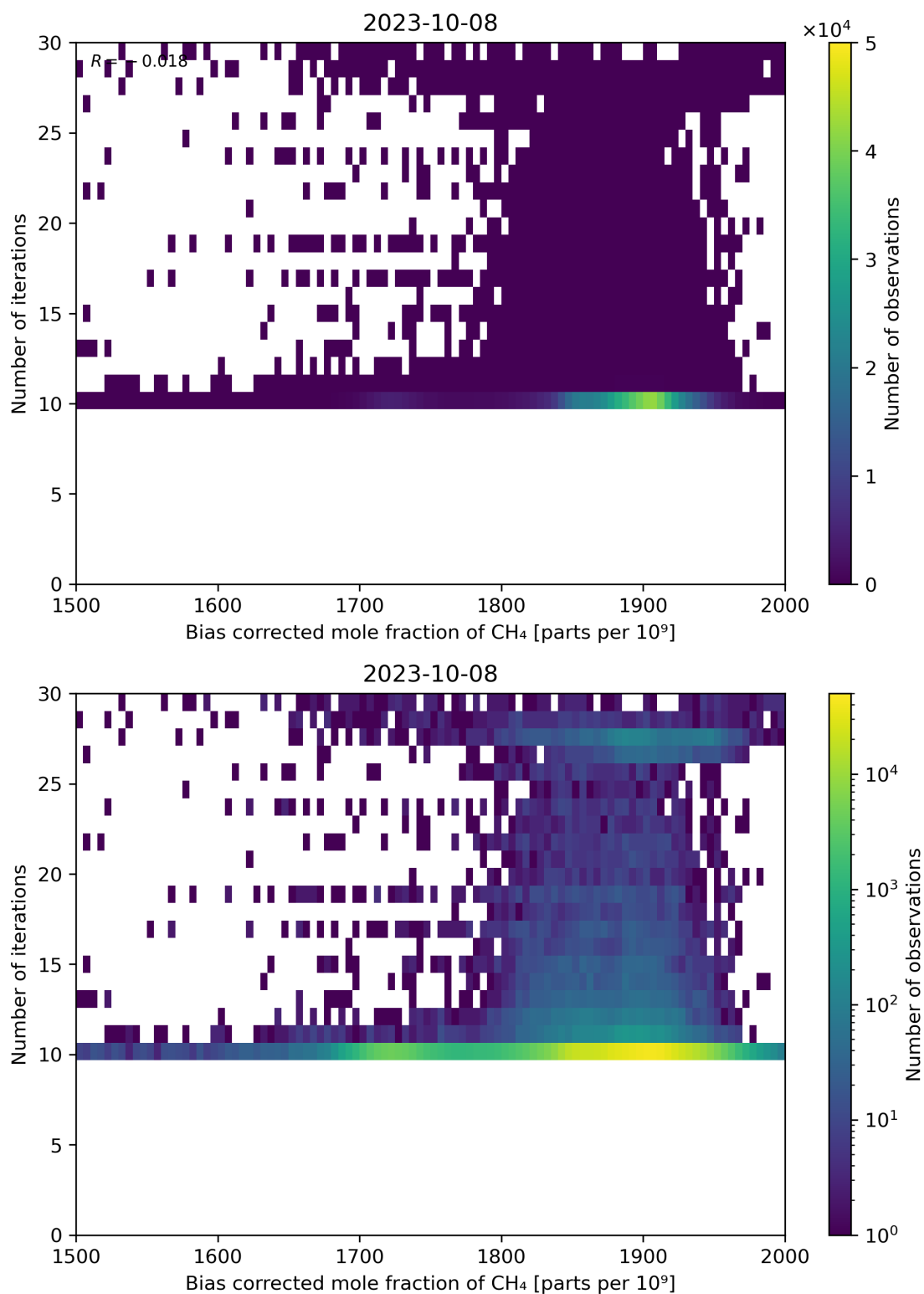
Figure 67: Scatter density plot of “Bias corrected mole fraction of \text{CH}_4 ” against “Number of iterations” for 2023-10-07 to 2023-10-09.
