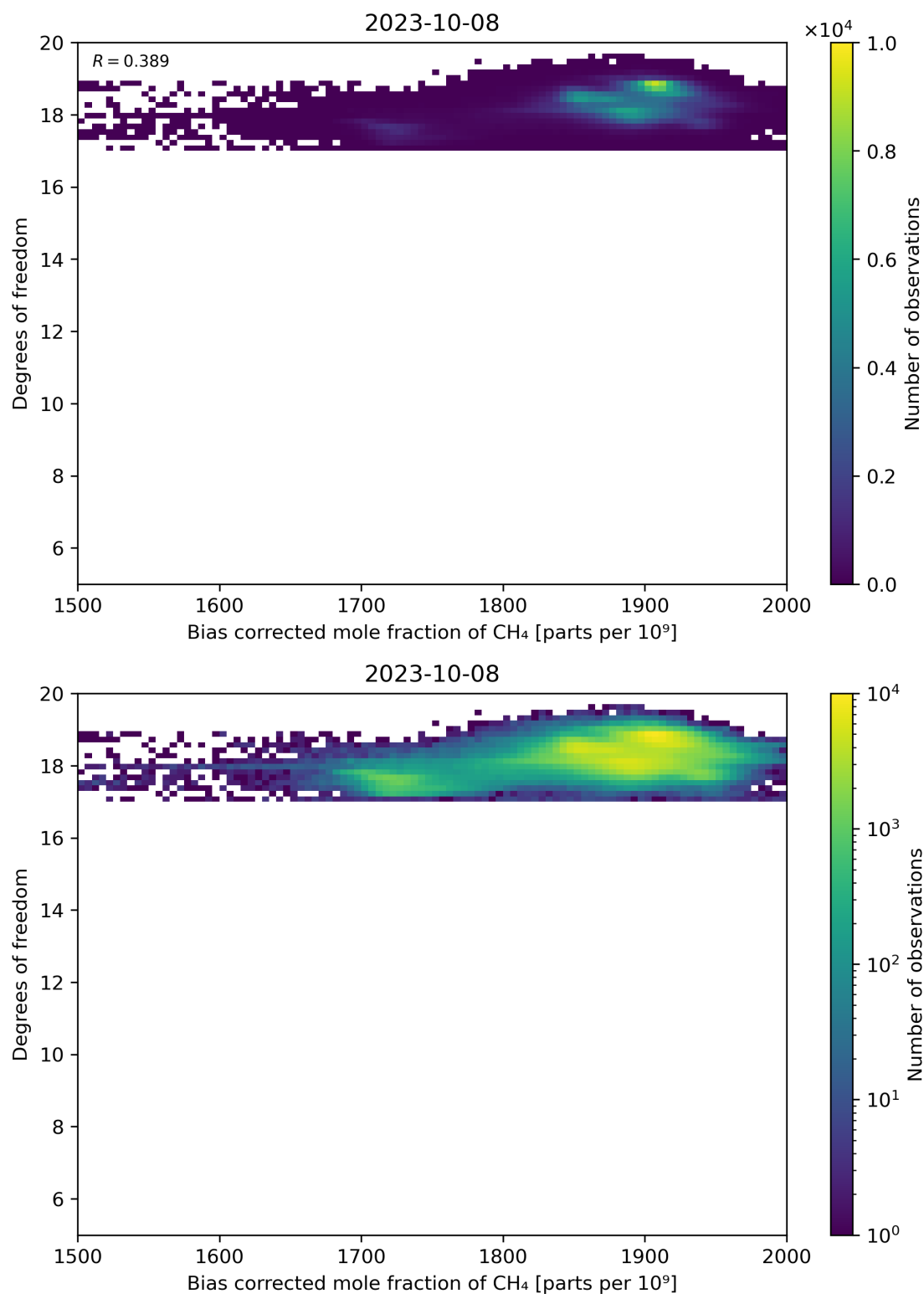
Figure 65: Scatter density plot of “Bias corrected mole fraction of CH 4 ” against “Degrees of freedom” for 2023-10-07 to 2023-10-09.
