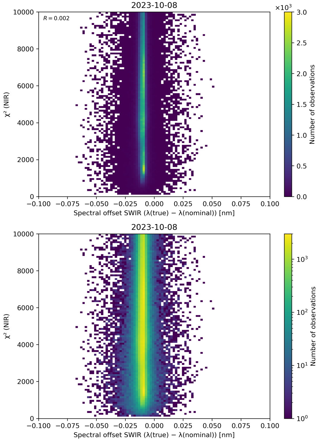
Figure 117: Scatter density plot of “Spectral offset SWIR ( \lambda(\text{true}) - \lambda(\text{nominal}) )” against “ \chi^2 (NIR)” for 2023-10-07 to 2023-10-09.
