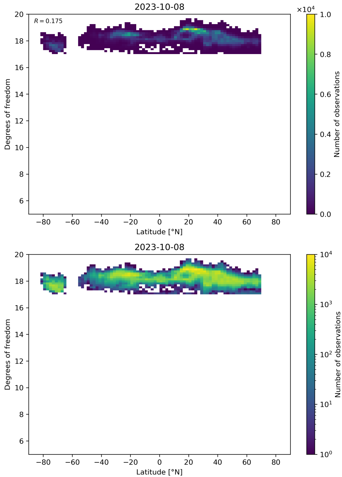
Figure 55: Scatter density plot of “Latitude” against “Degrees of freedom” for 2023-10-07 to 2023-10-09.
