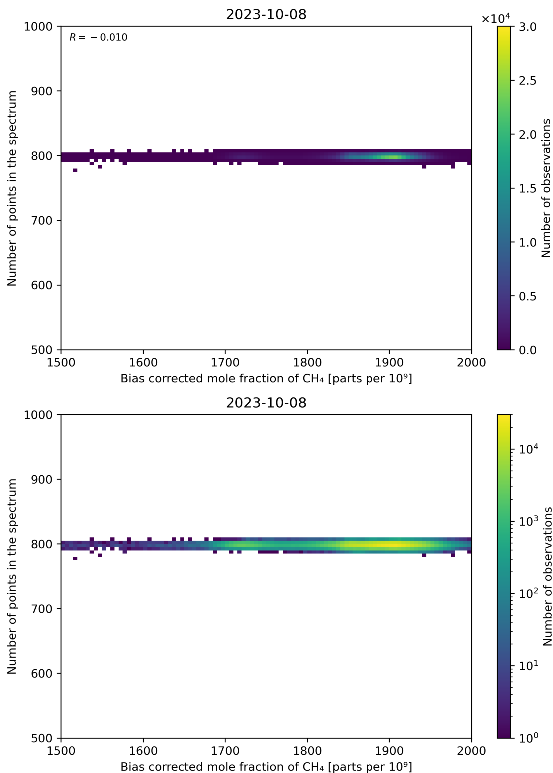
Figure 68: Scatter density plot of “Bias corrected mole fraction of CH 4 ” against “Number of points in the spectrum” for 2023-10-07 to 2023-10-09.
