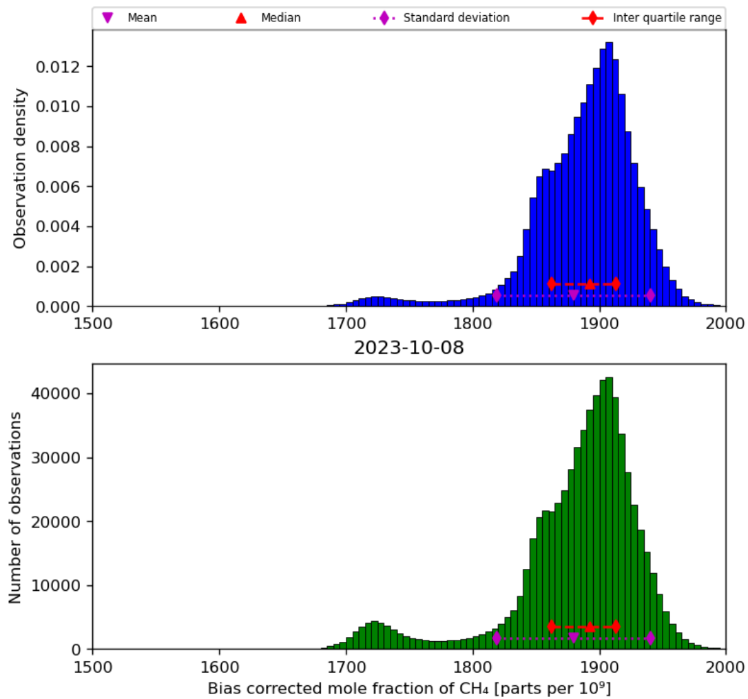
Figure 25: Histogram of “Bias corrected mole fraction of CH 4 ” for 2023-10-07 to 2023-10-09
