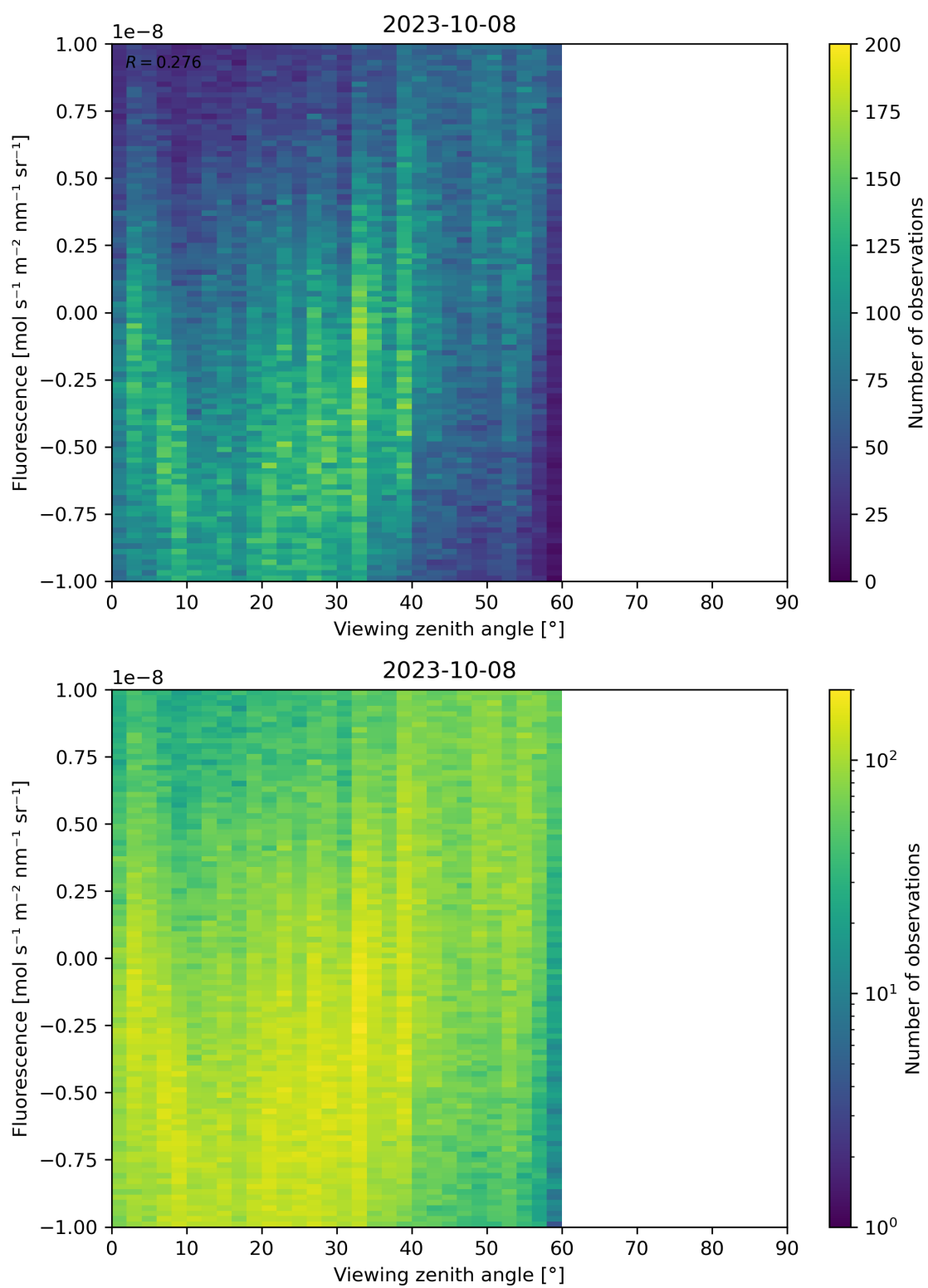
Figure 108: Scatter density plot of “Viewing zenith angle” against “Fluorescence” for 2023-10-07 to 2023-10-09.
