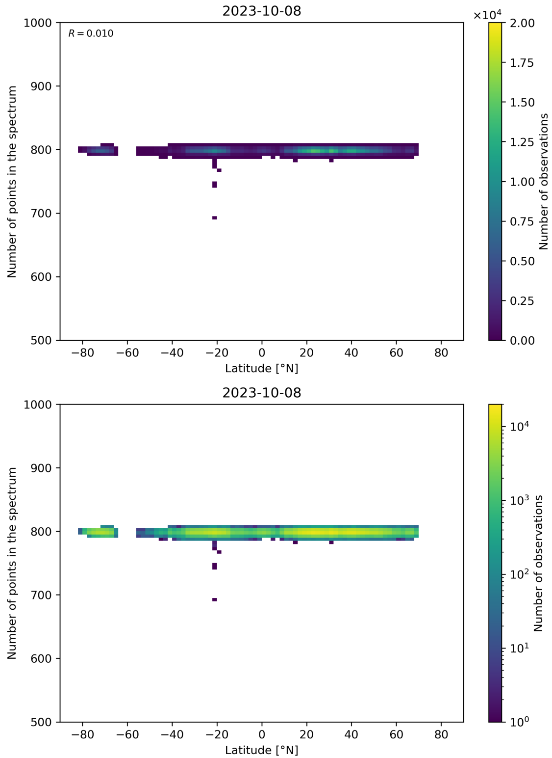
Figure 61: Scatter density plot of “Latitude” against “Number of points in the spectrum” for 2023-10-07 to 2023-10-09.
