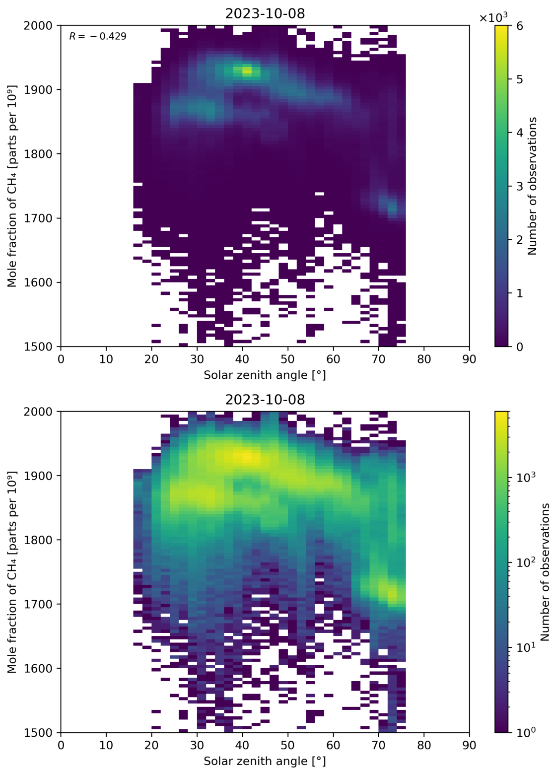
Figure 99: Scatter density plot of “Solar zenith angle” against “Mole fraction of CH 4 ” for 2023-10-07 to 2023-10-09.
