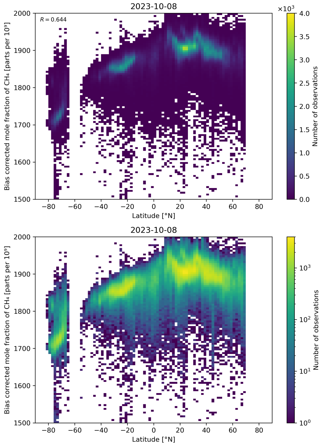
Figure 58: Scatter density plot of “Latitude” against “Bias corrected mole fraction of \text{CH}_4 ” for 2023-10-07 to 2023-10-09.
