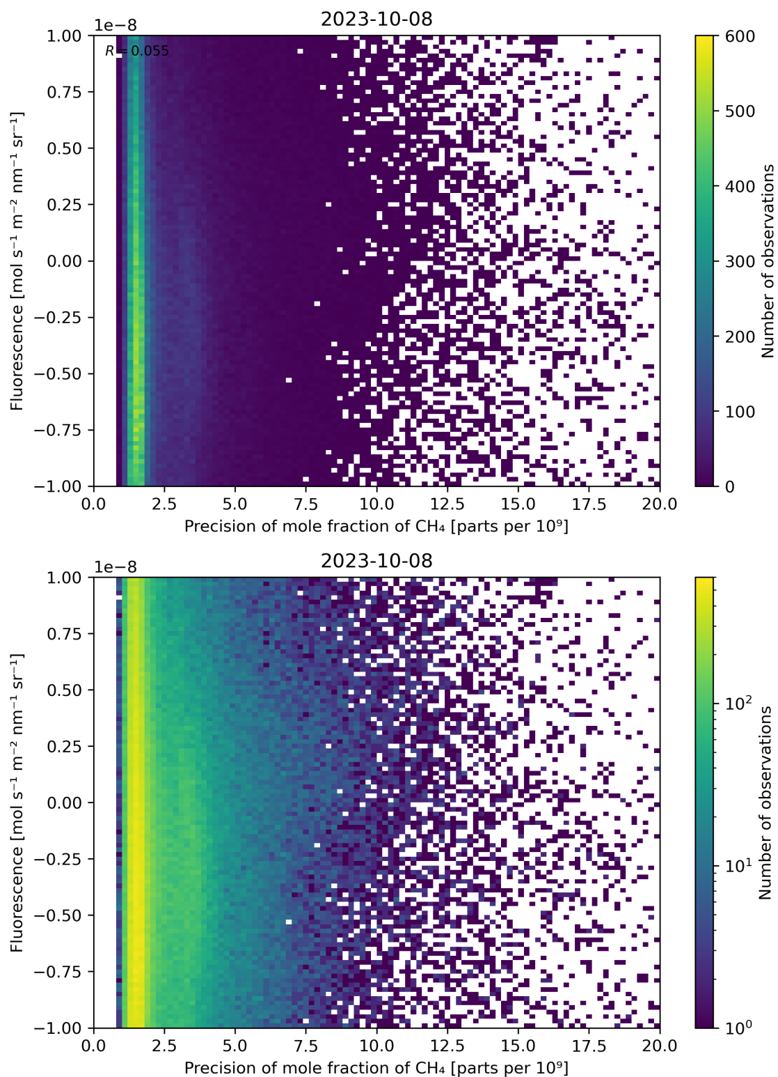
Figure 81: Scatter density plot of “Precision of mole fraction of CH 4 ” against “Fluorescence” for 2023-10-07 to 2023-10-09.
