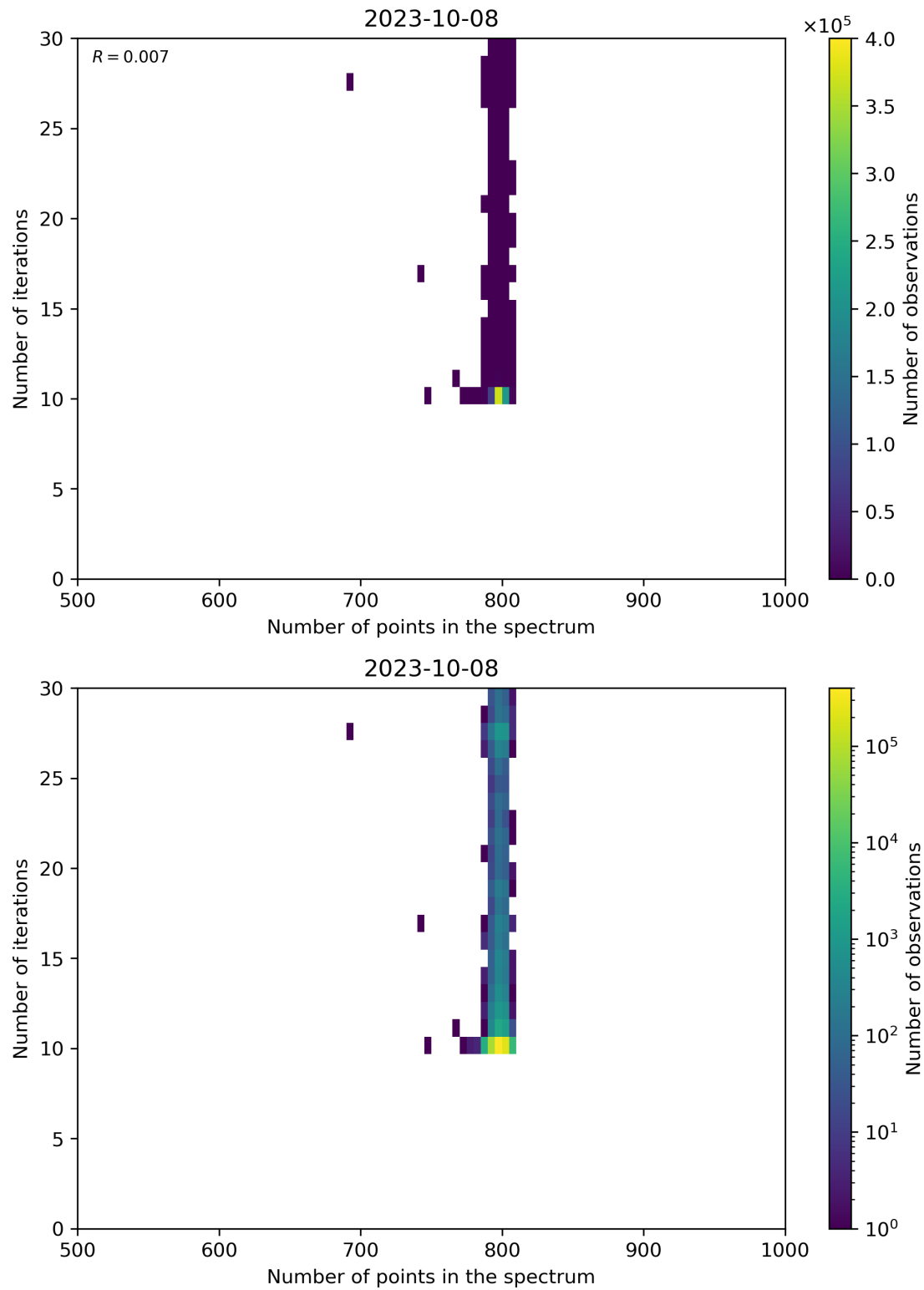
Figure 92: Scatter density plot of “Number of points in the spectrum” against “Number of iterations” for 2023-10-07 to 2023-10-09.
