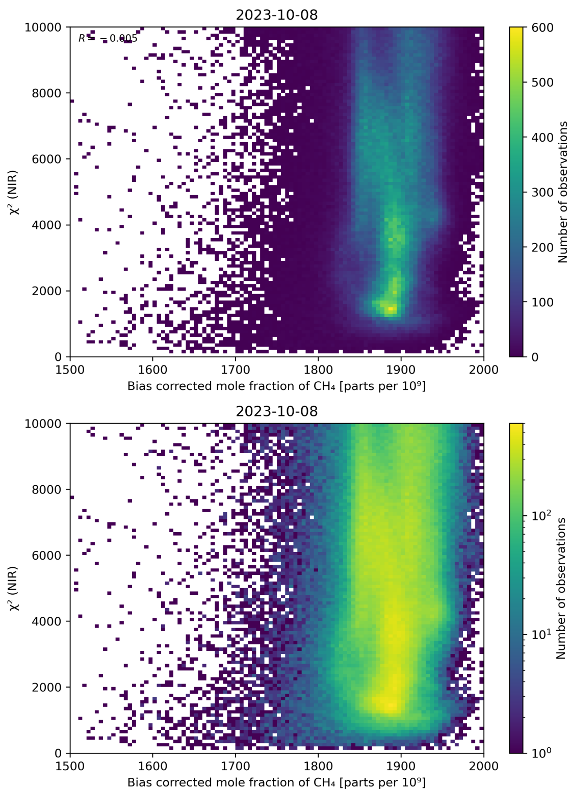
Figure 63: Scatter density plot of “Bias corrected mole fraction of \text{CH}_4 ” against “ \chi^2 (NIR)” for 2023-10-07 to 2023-10-09.
