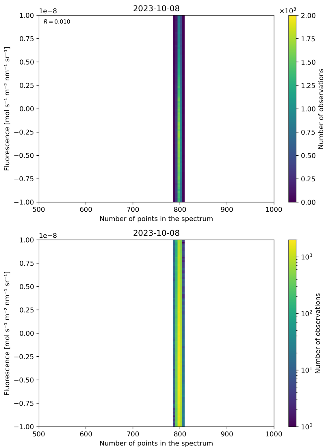
Figure 91: Scatter density plot of “Number of points in the spectrum” against “Fluorescence” for 2023-10-07 to 2023-10-09.
