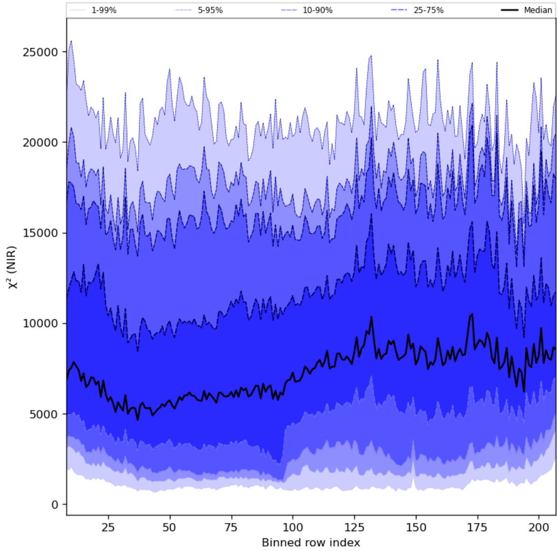
Figure 40: Along track statistics of “ \chi^2 (NIR)” for 2023-10-07 to 2023-10-09
