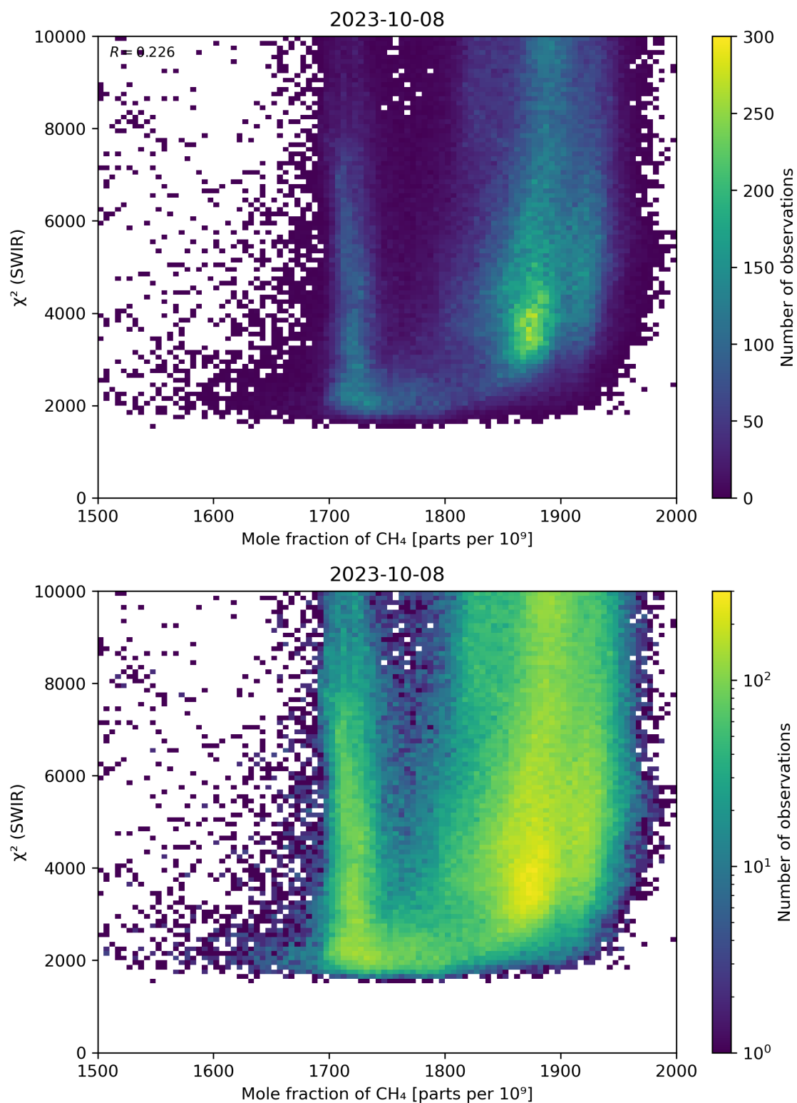
Figure 71: Scatter density plot of “Mole fraction of \text{CH}_4 ” against “ \chi^2 (SWIR)” for 2023-10-07 to 2023-10-09.
