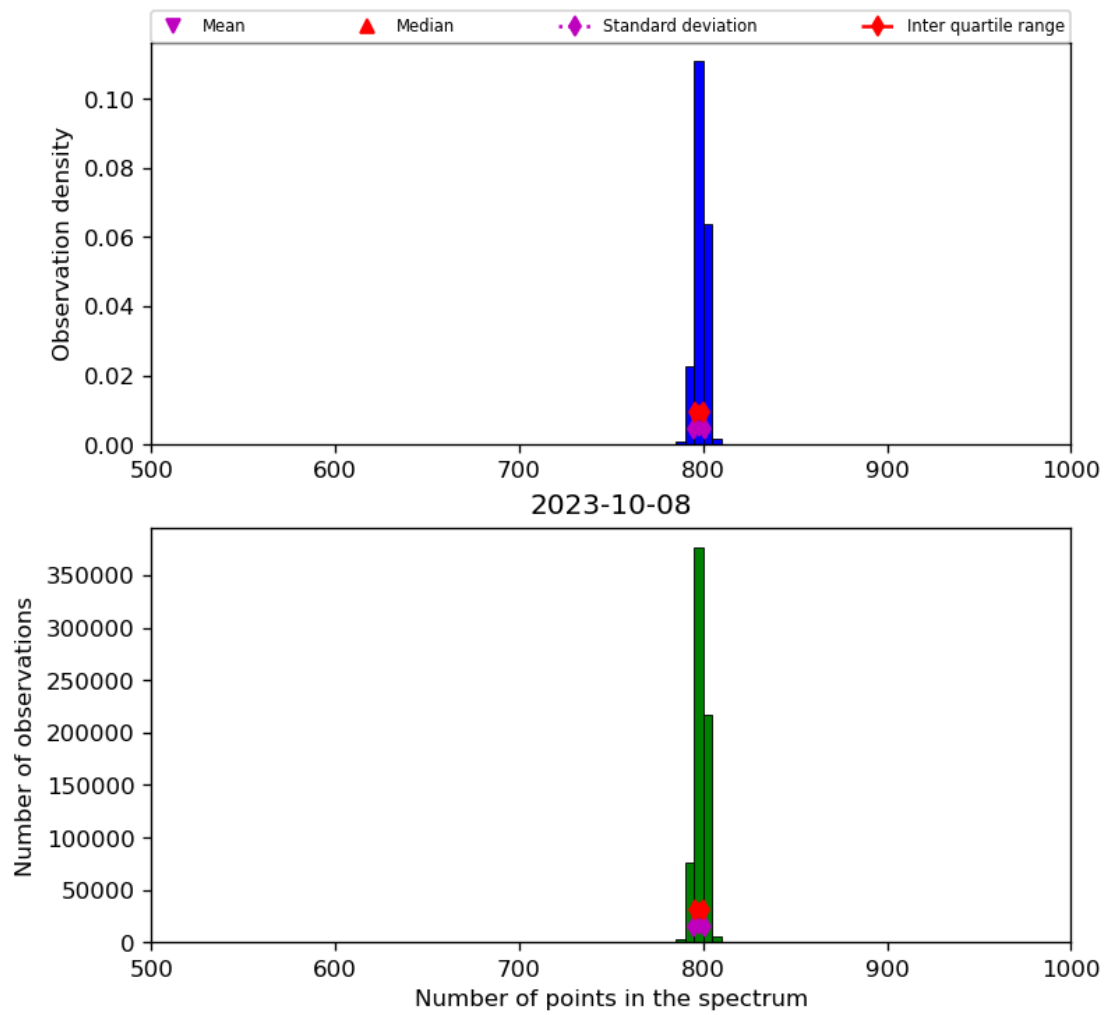
Figure 26: Histogram of “Number of points in the spectrum” for 2023-10-07 to 2023-10-09
