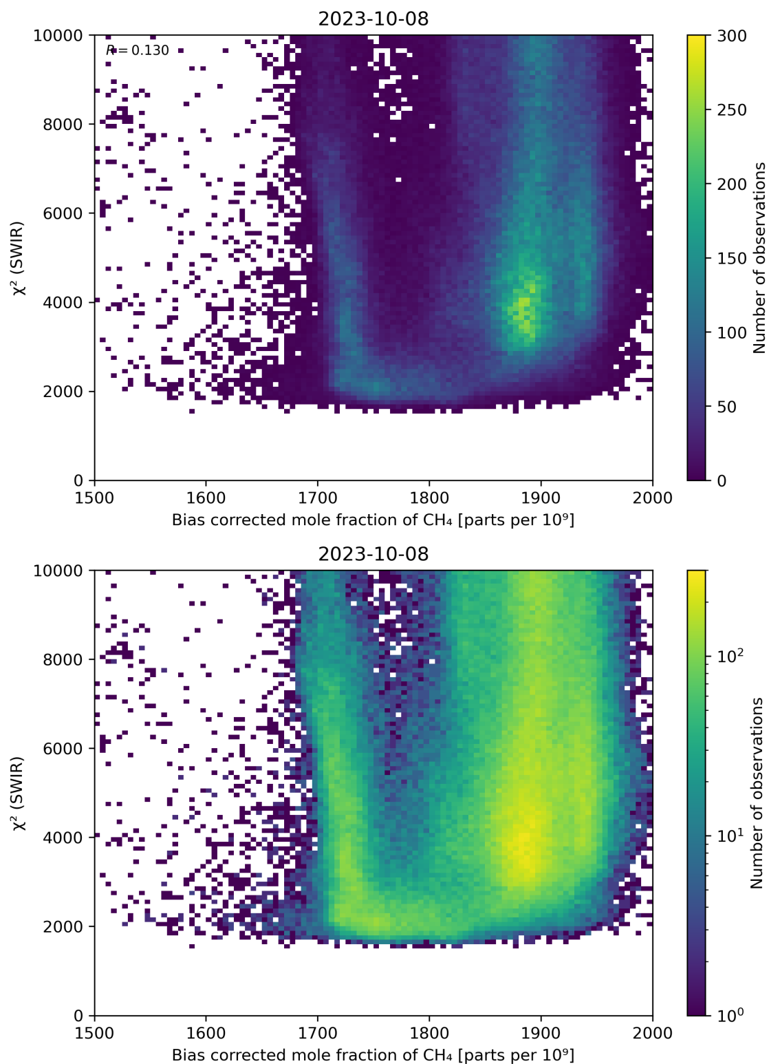
Figure 64: Scatter density plot of “Bias corrected mole fraction of \text{CH}_4 ” against “ \chi^2 (SWIR)” for 2023-10-07 to 2023-10-09.
