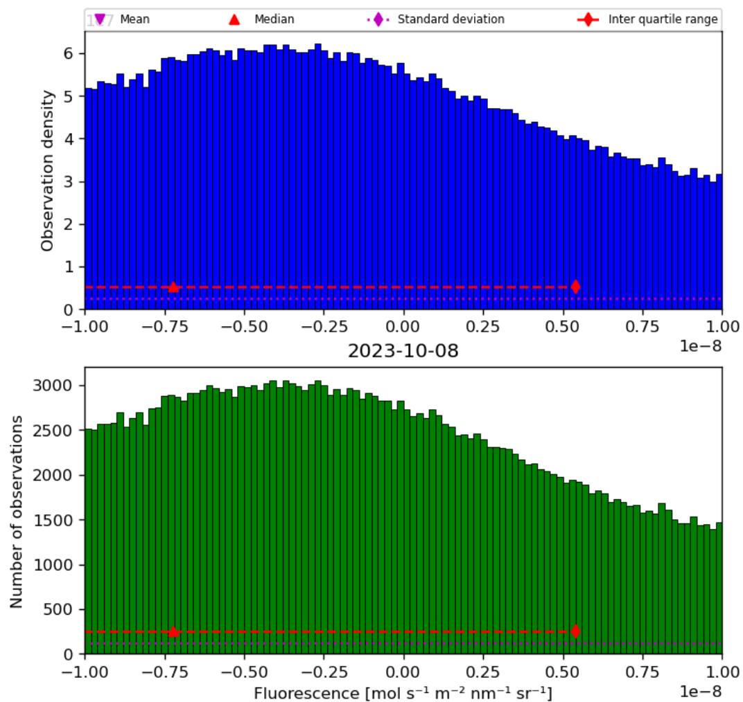
Figure 32: Histogram of “Fluorescence” for 2023-10-07 to 2023-10-09
