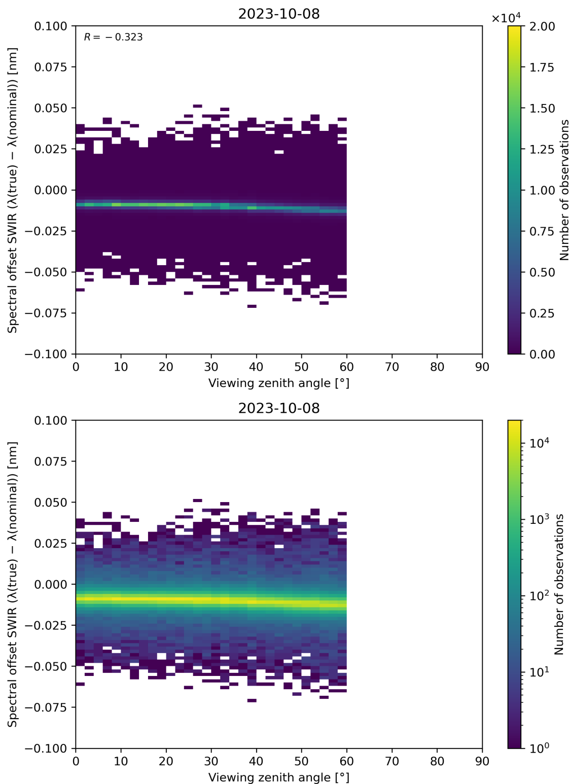
Figure 116: Scatter density plot of “Viewing zenith angle” against “Spectral offset SWIR ( \lambda(\text{true}) - \lambda(\text{nominal}) )” for 2023-10-07 to 2023-10-09.
