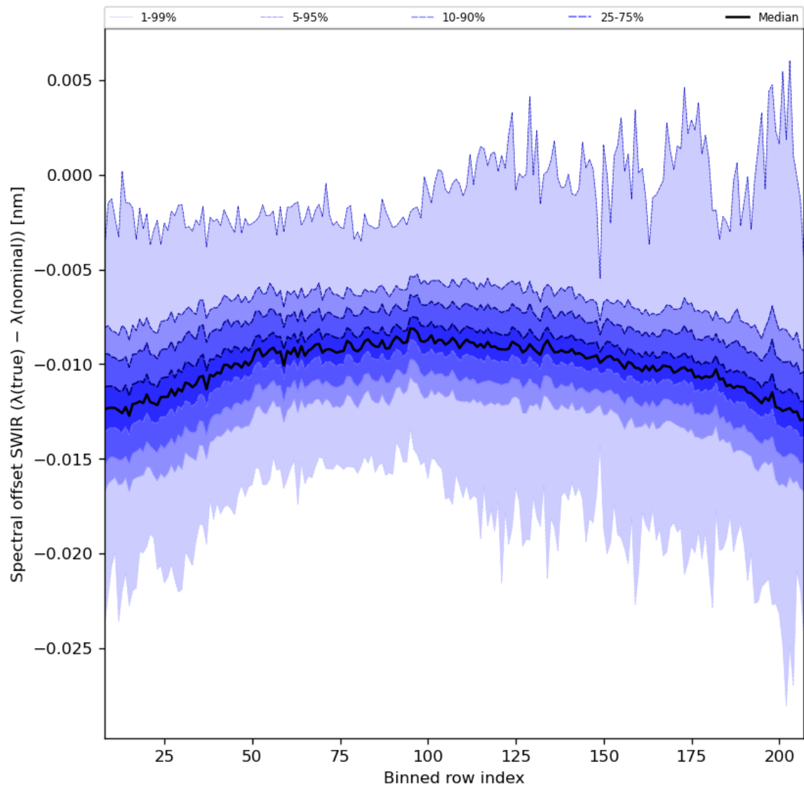
Figure 38: Along track statistics of “Spectral offset SWIR ( \lambda(\text{true}) - \lambda(\text{nominal}) )” for 2023-10-07 to 2023-10-09
