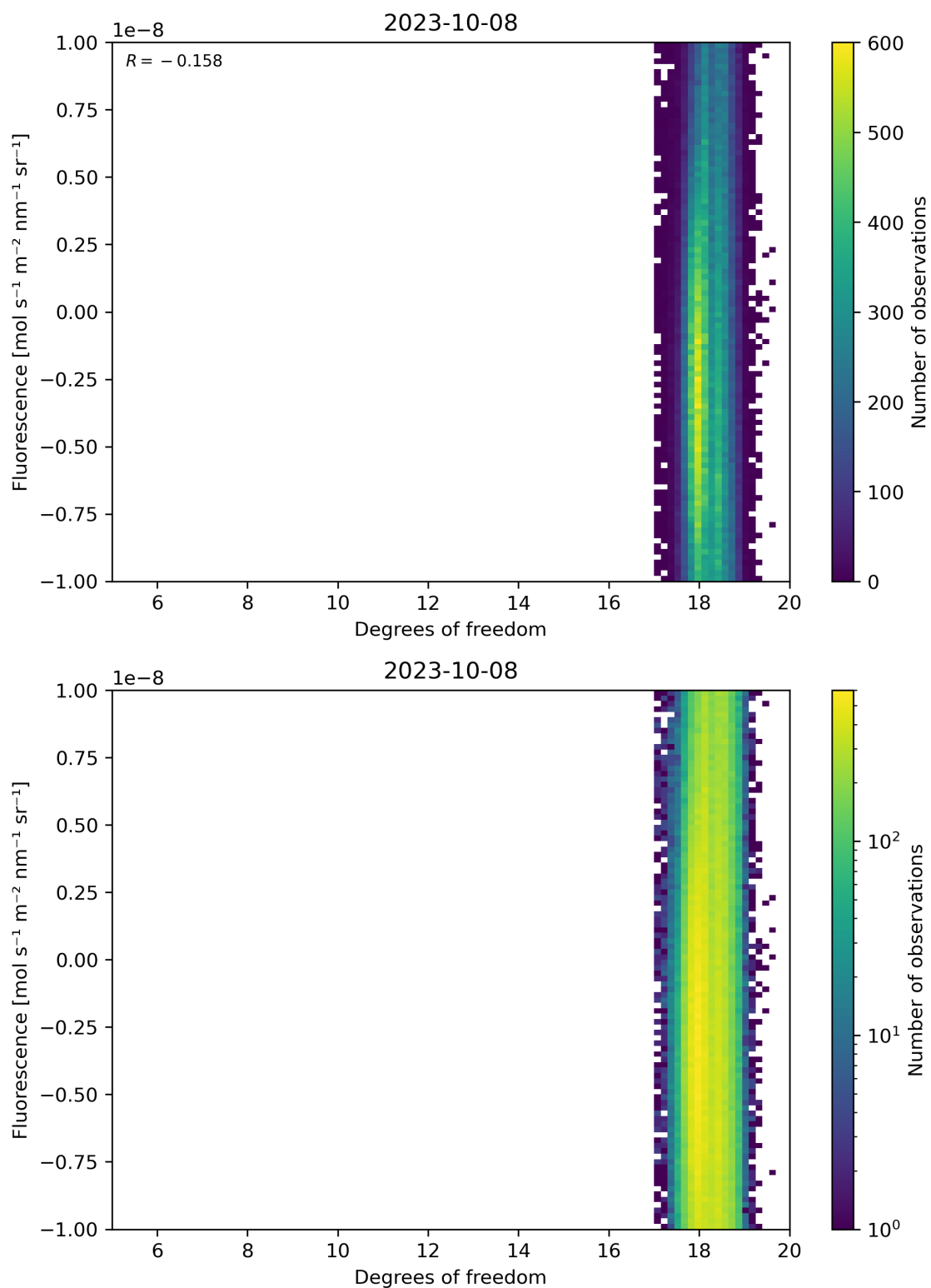
Figure 51: Scatter density plot of “Degrees of freedom” against “Fluorescence” for 2023-10-07 to 2023-10-09.
