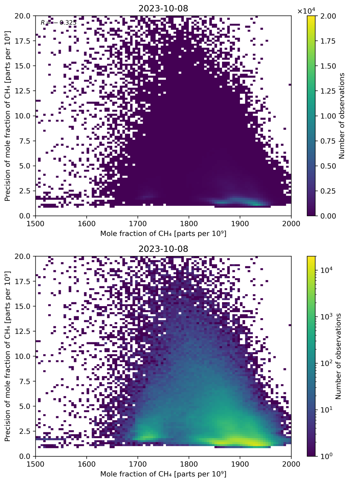
Figure 75: Scatter density plot of “Mole fraction of CH 4 ” against “Precision of mole fraction of CH 4 ” for 2023-10-07 to 2023-10-09.
