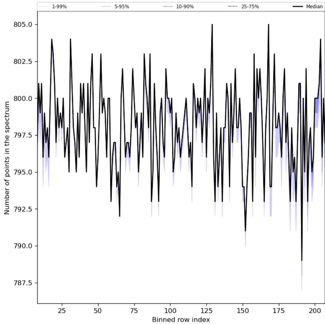
Figure 37: Along track statistics of “Number of points in the spectrum” for 2023-10-07 to 2023-10-09
