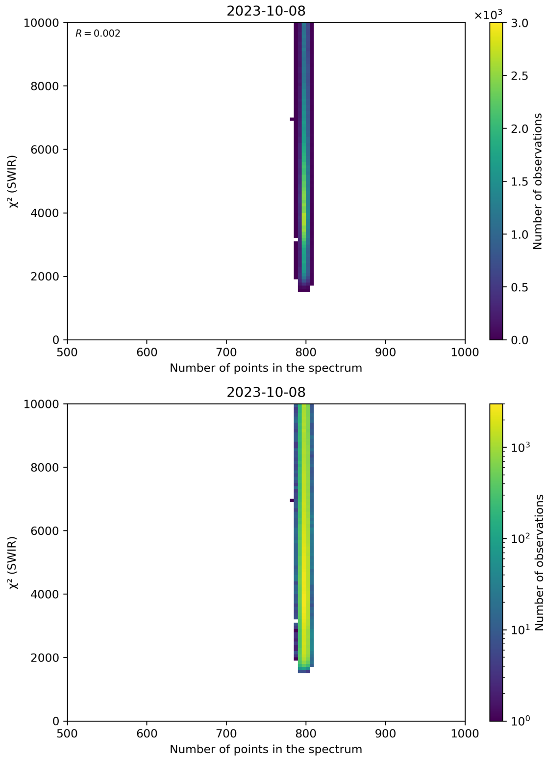
Figure 89: Scatter density plot of “Number of points in the spectrum” against “ \chi^2 (SWIR)” for 2023-10-07 to 2023-10-09.
