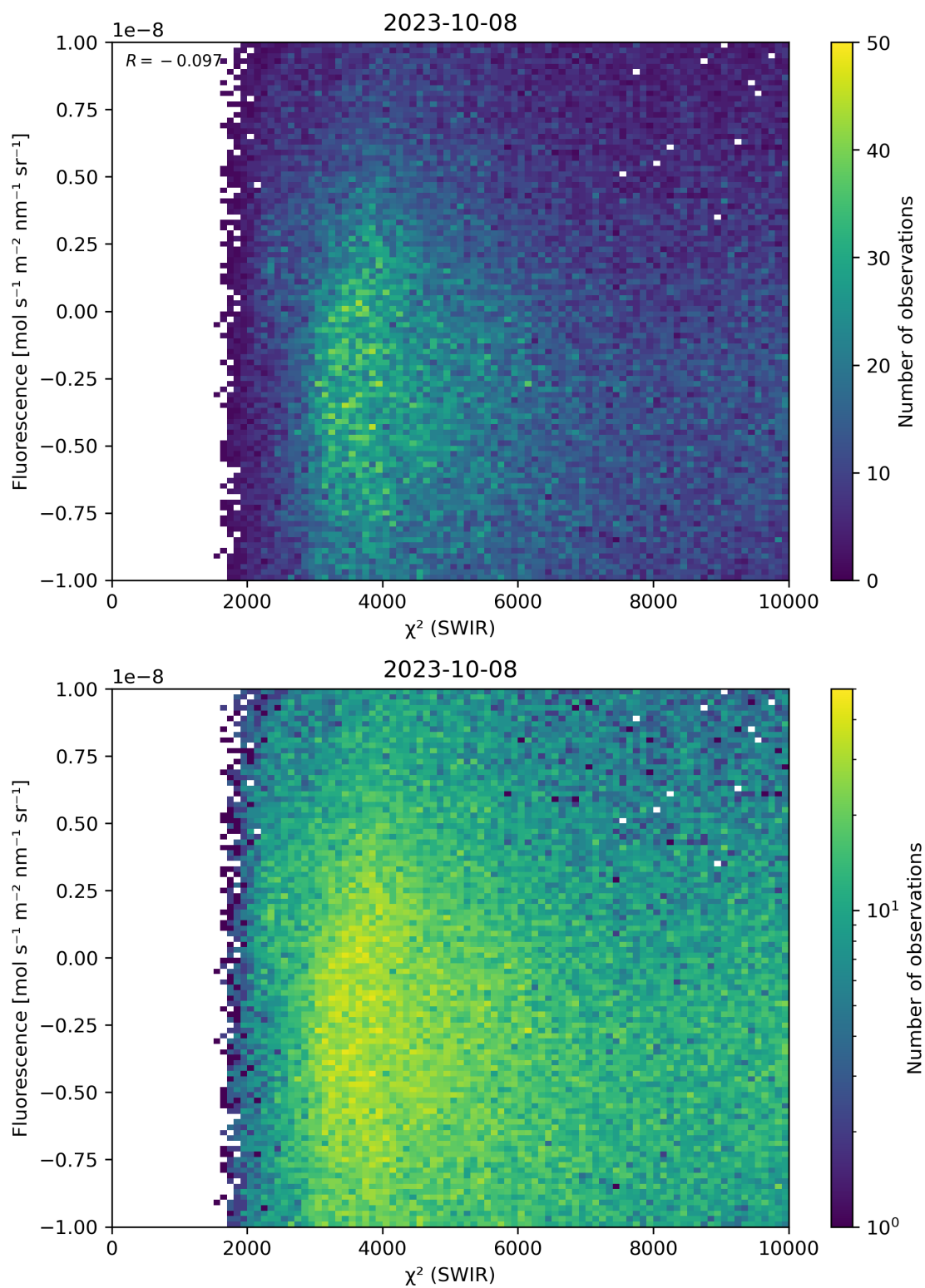
Figure 49: Scatter density plot of “ \chi^2 (SWIR)” against “Fluorescence” for 2023-10-07 to 2023-10-09.
