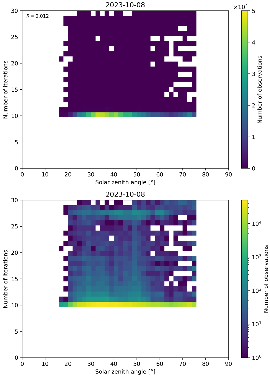
Figure 102: Scatter density plot of “Solar zenith angle” against “Number of iterations” for 2023-10-07 to 2023-10-09.
