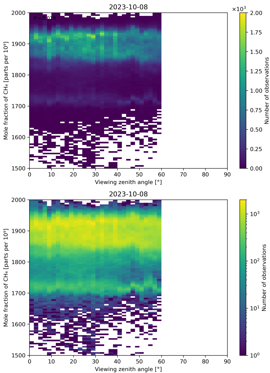
Figure 110: Scatter density plot of “Viewing zenith angle” against “Mole fraction of CH 4 ” for 2023-10-07 to 2023-10-09.
