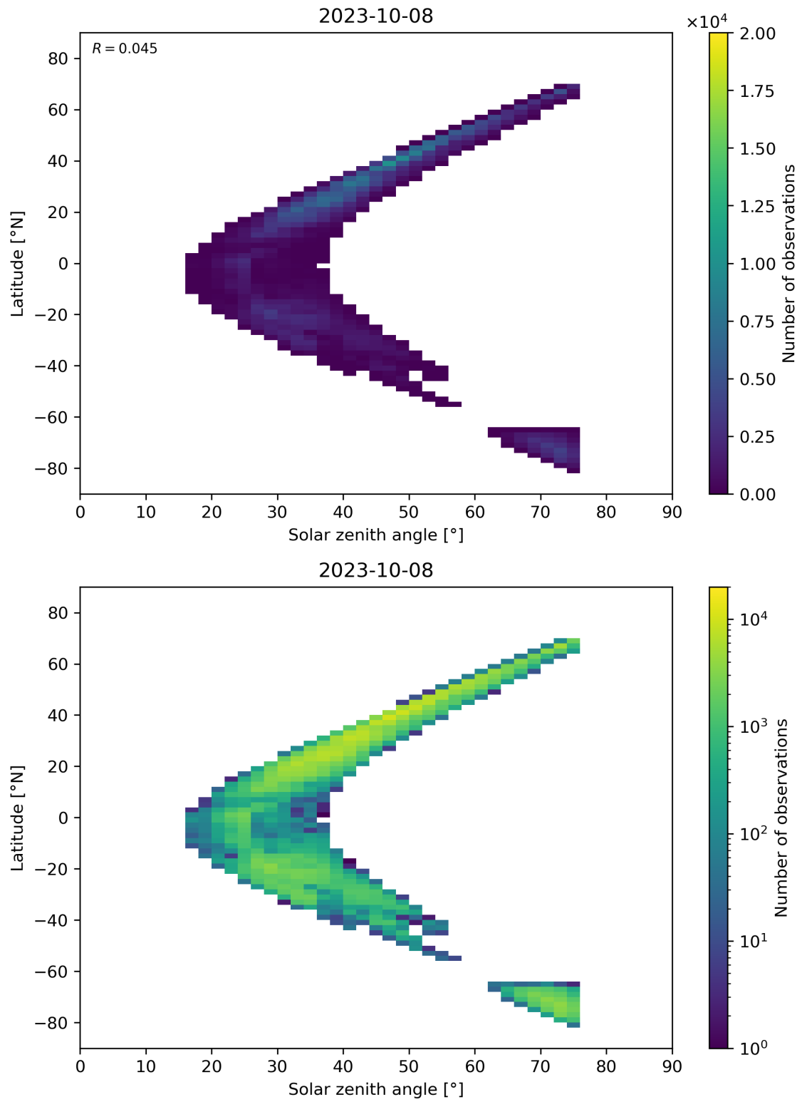
Figure 98: Scatter density plot of “Solar zenith angle” against “Latitude” for 2023-10-07 to 2023-10-09.
