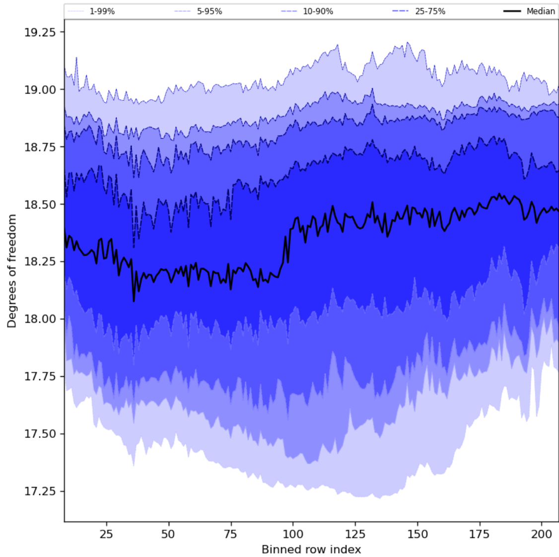
Figure 41: Along track statistics of “Degrees of freedom” for 2023-10-07 to 2023-10-09
