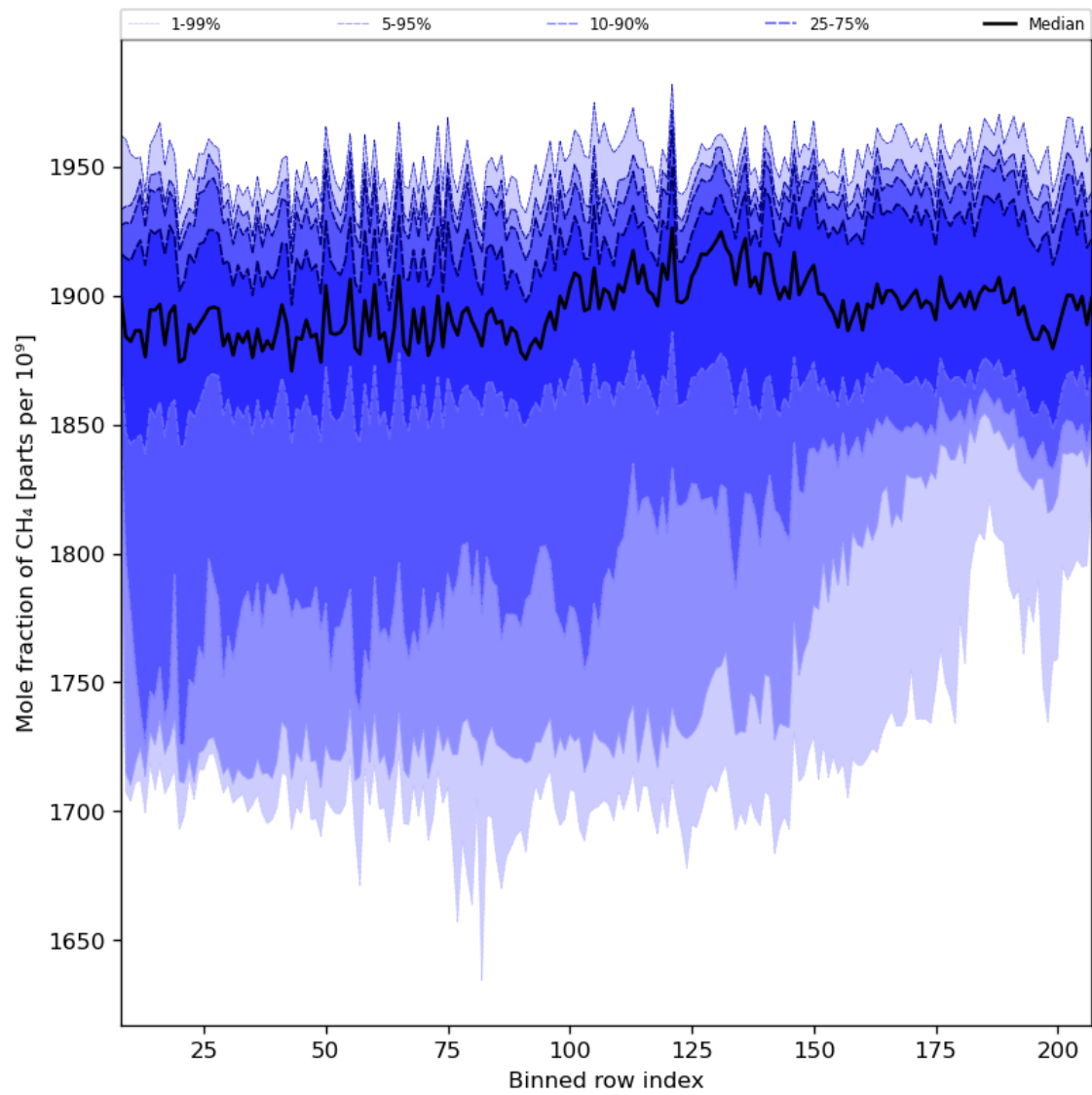
Figure 34: Along track statistics of “Mole fraction of CH 4 ” for 2023-10-07 to 2023-10-09
