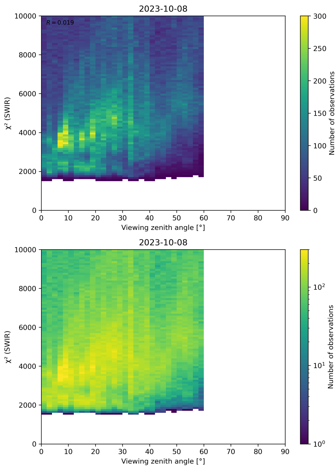
Figure 106: Scatter density plot of “Viewing zenith angle” against “ \chi^2 (SWIR)” for 2023-10-07 to 2023-10-09.
