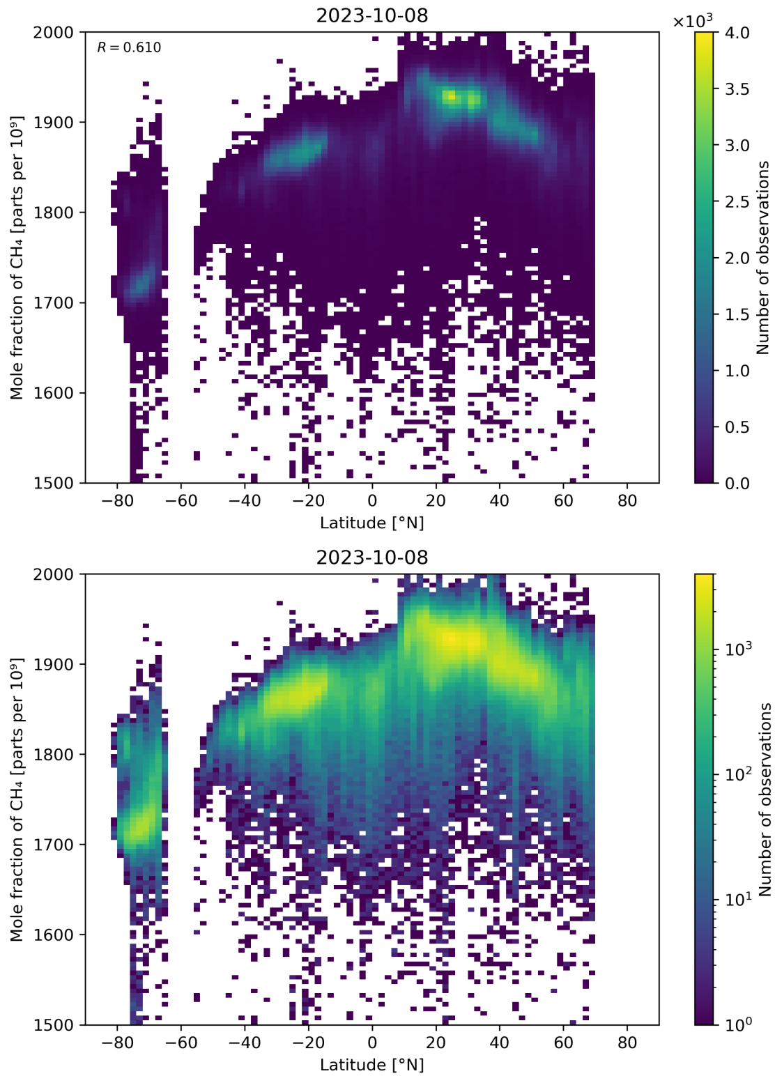
Figure 57: Scatter density plot of “Latitude” against “Mole fraction of CH 4 ” for 2023-10-07 to 2023-10-09.
