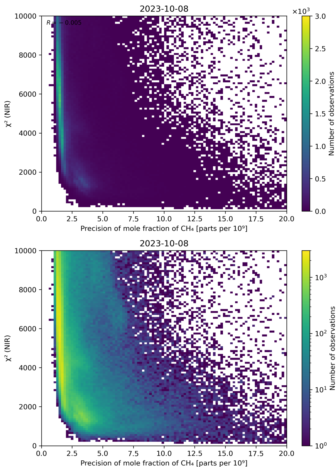
Figure 78: Scatter density plot of “Precision of mole fraction of CH 4 ” against “ \chi^2 (NIR)” for 2023-10-07 to 2023-10-09.
