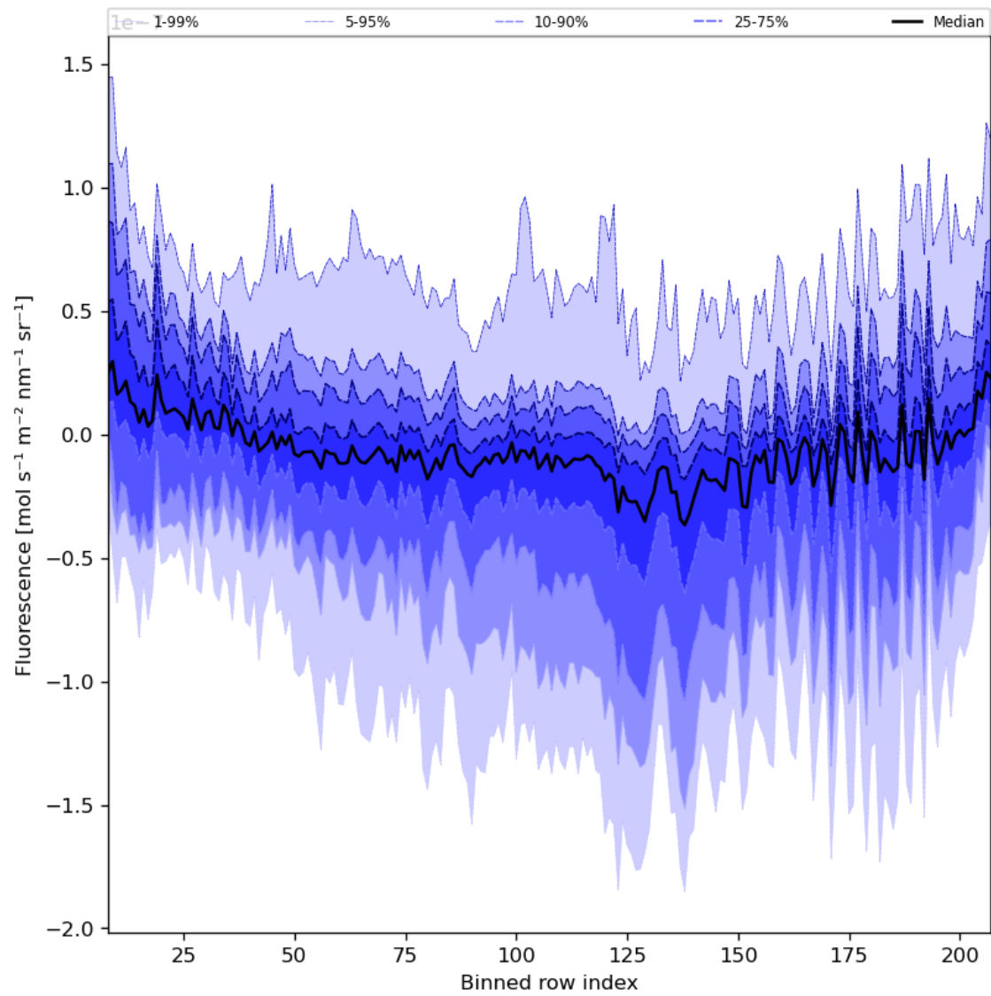
Figure 43: Along track statistics of “Fluorescence” for 2023-10-07 to 2023-10-09
