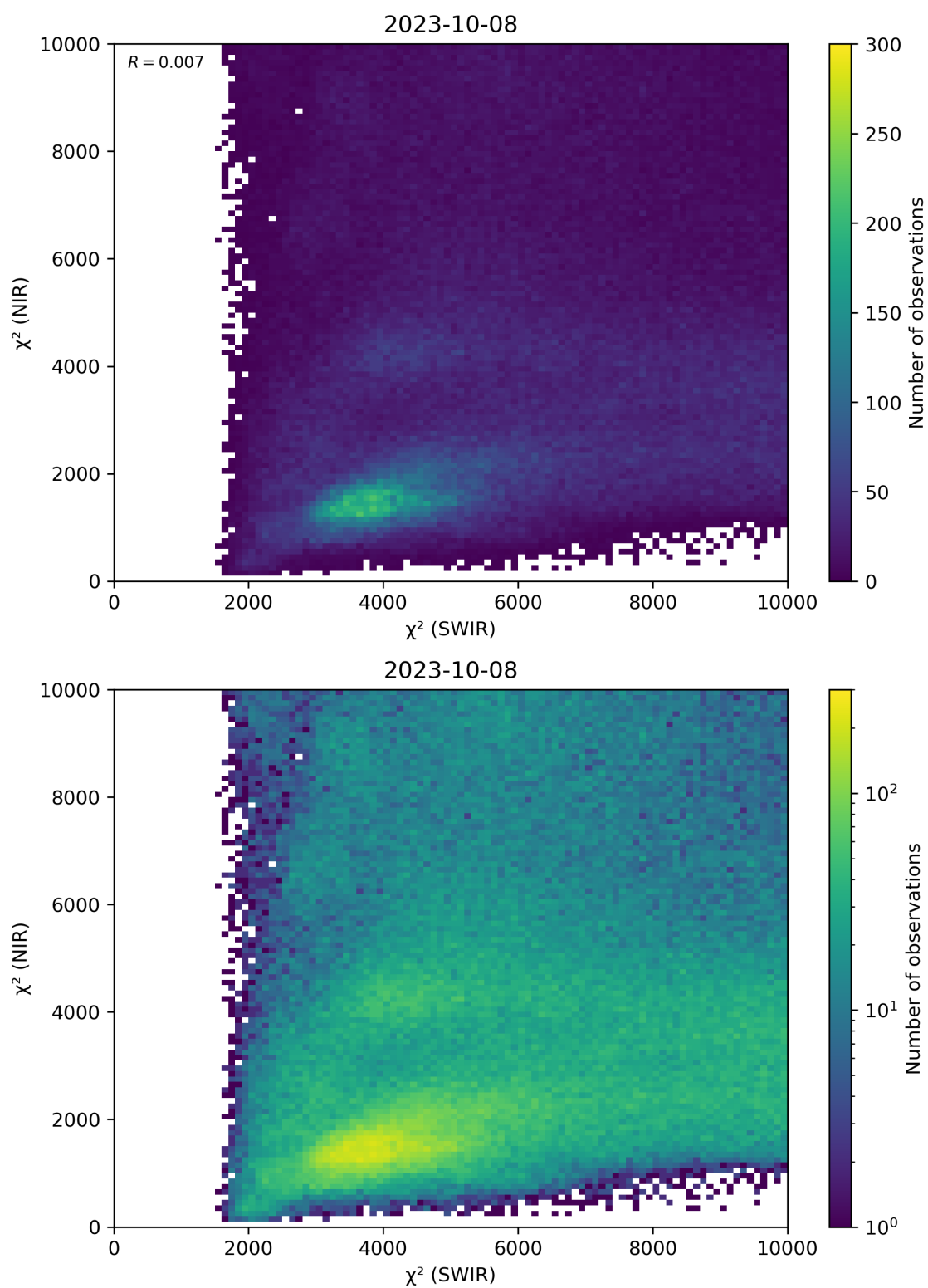
Figure 47: Scatter density plot of “ \chi^2 (SWIR)” against “ \chi^2 (NIR)” for 2023-10-07 to 2023-10-09.
