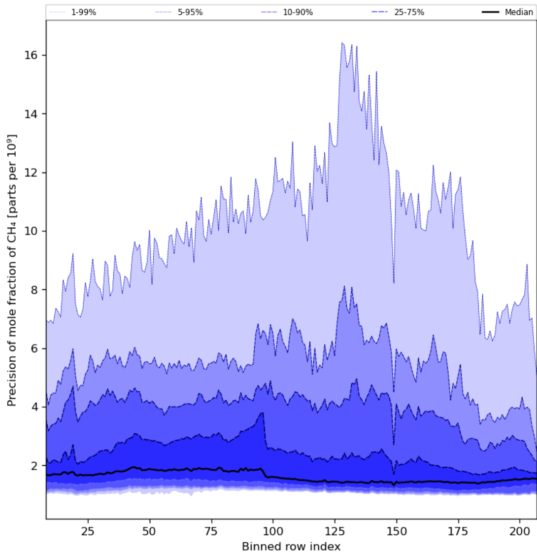
Figure 35: Along track statistics of “Precision of mole fraction of CH 4 ” for 2023-10-07 to 2023-10-09
