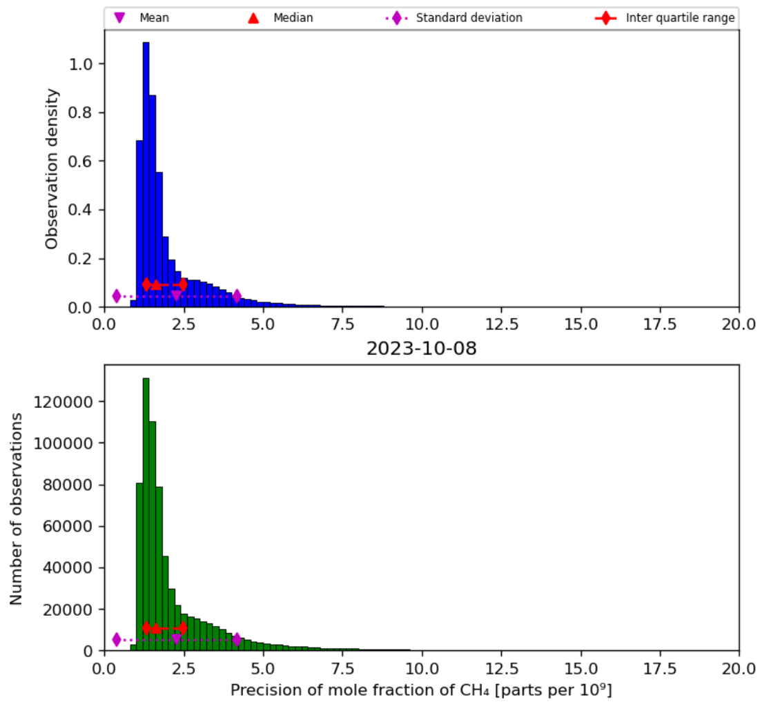
Figure 24: Histogram of “Precision of mole fraction of CH 4 ” for 2023-10-07 to 2023-10-09
