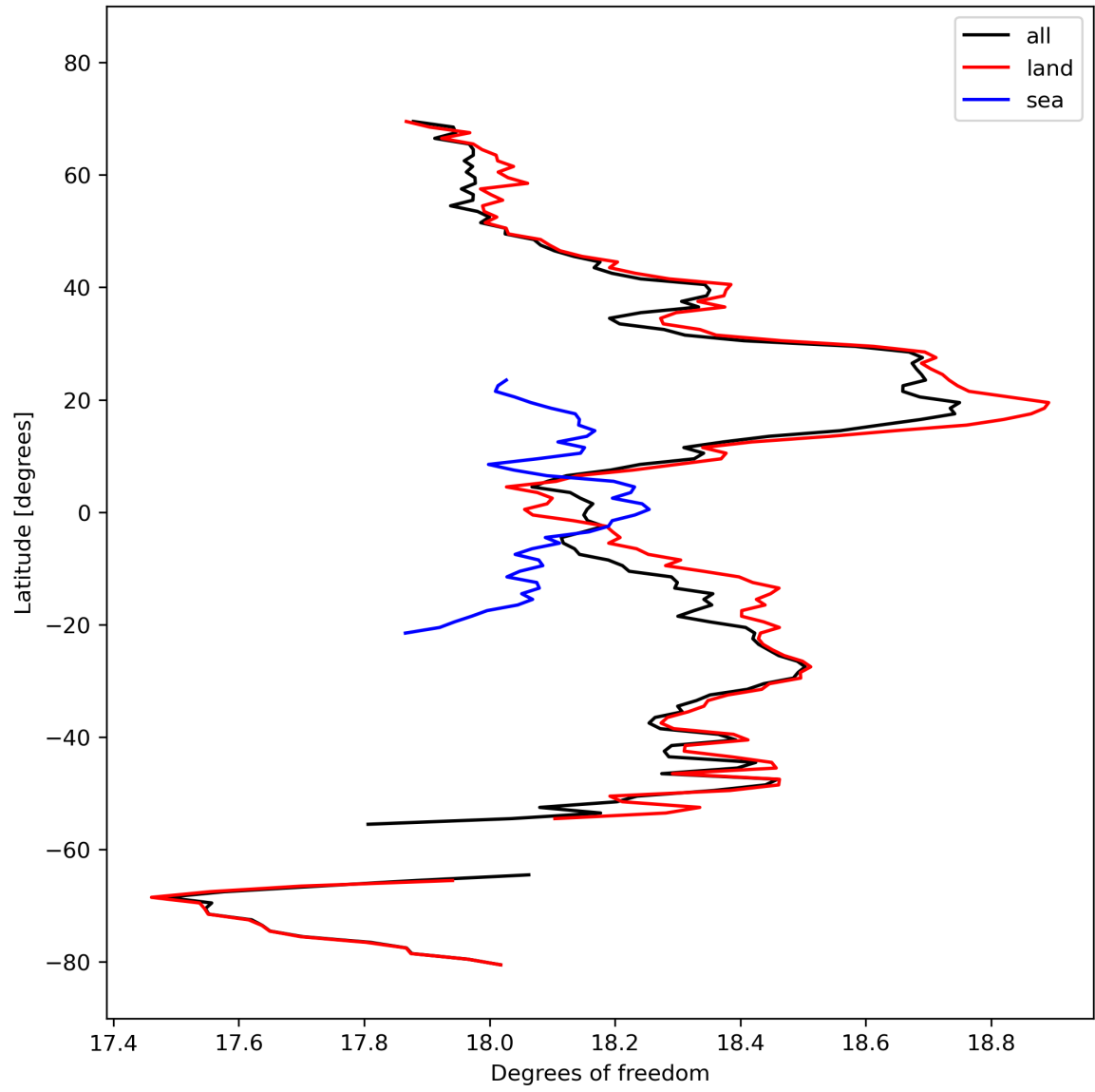
Figure 19: Zonal average of “Degrees of freedom” for 2023-10-07 to 2023-10-09.
