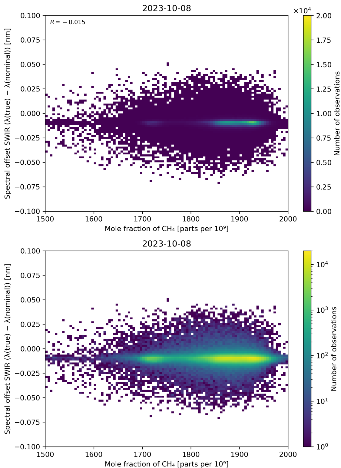
Figure 86: Scatter density plot of “Mole fraction of CH 4 ” against “Spectral offset SWIR ( \lambda(\text{true}) - \lambda(\text{nominal}) )” for 2023-10-07 to 2023-10-09.
