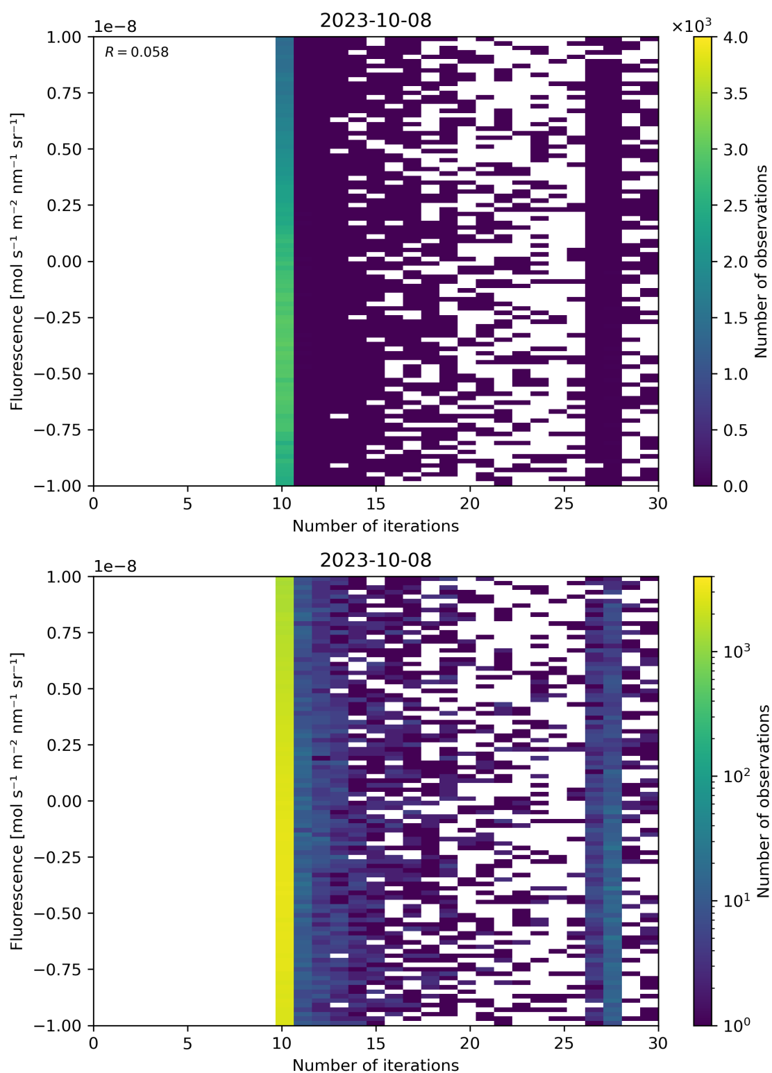
Figure 87: Scatter density plot of “Number of iterations” against “Fluorescence” for 2023-10-07 to 2023-10-09.
