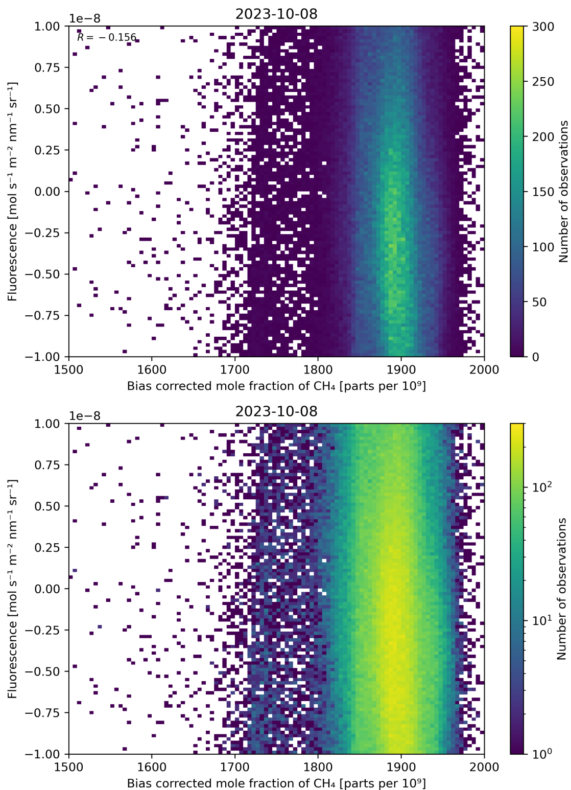
Figure 66: Scatter density plot of “Bias corrected mole fraction of \text{CH}_4 ” against “Fluorescence” for 2023-10-07 to 2023-10-09.
