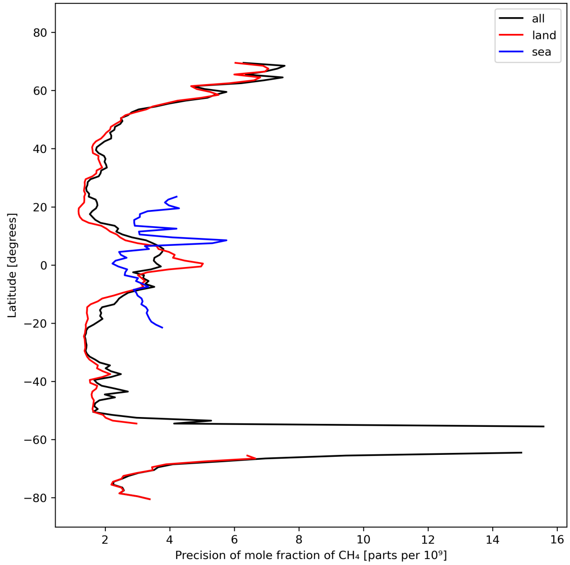
Figure 13: Zonal average of “Precision of mole fraction of \text{CH}_4 ” for 2023-10-07 to 2023-10-09.
