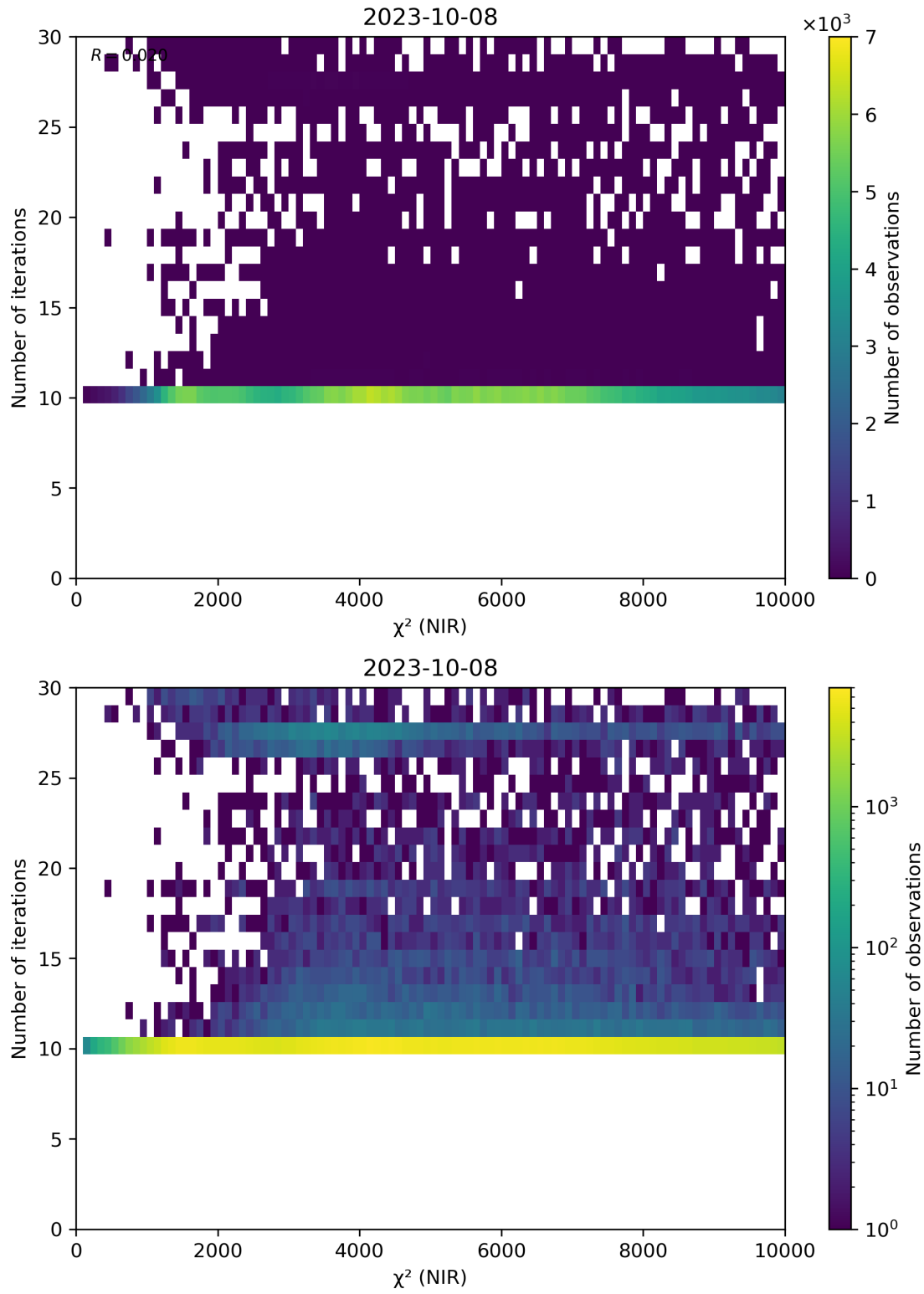
Figure 46: Scatter density plot of “ \chi^2 (NIR)” against “Number of iterations” for 2023-10-07 to 2023-10-09.
