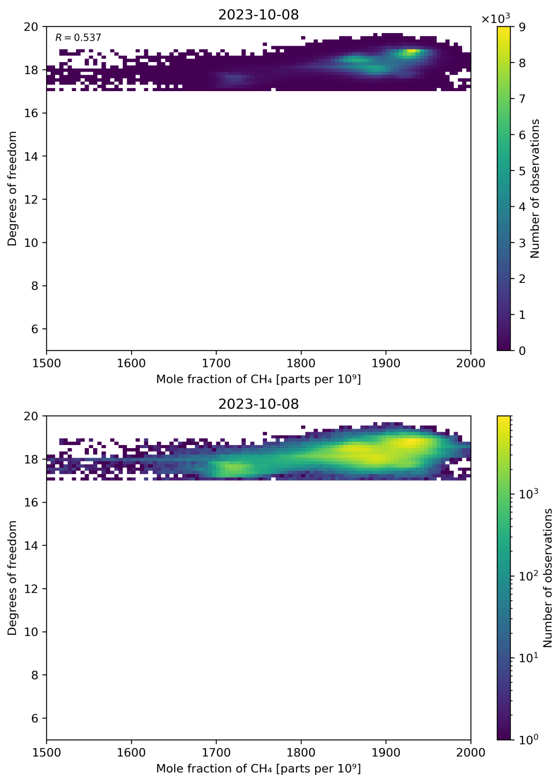
Figure 72: Scatter density plot of “Mole fraction of CH 4 ” against “Degrees of freedom” for 2023-10-07 to 2023-10-09.
