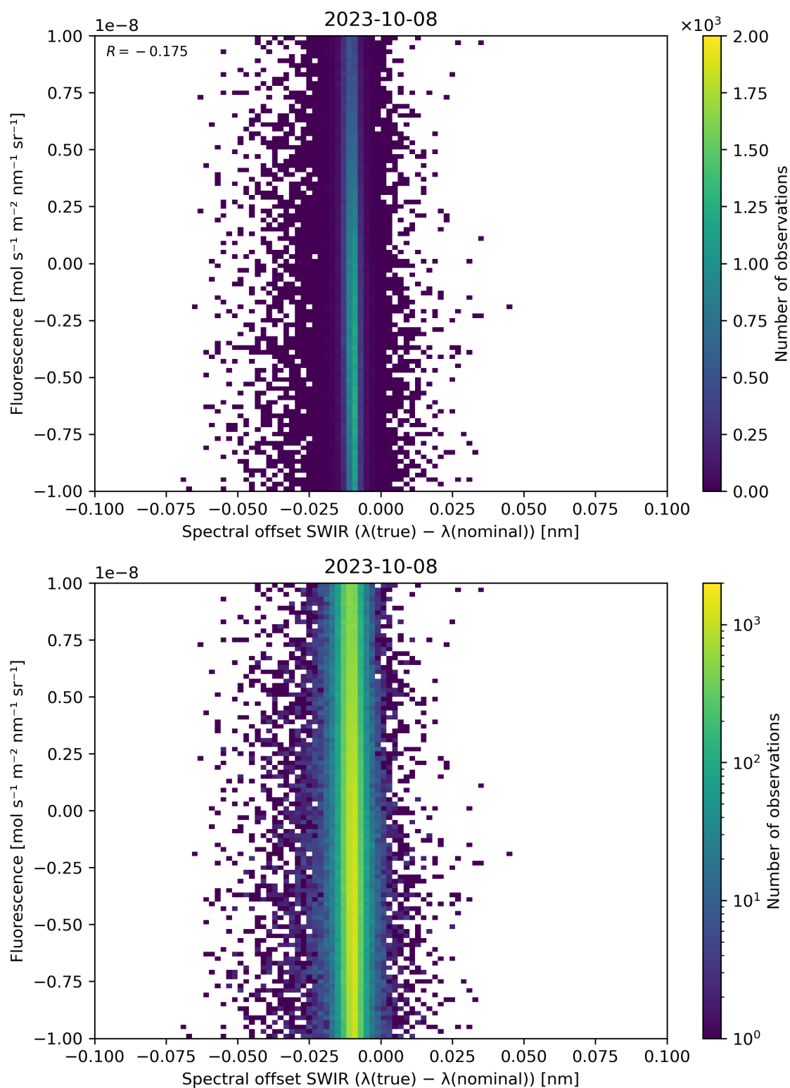
Figure 120: Scatter density plot of “Spectral offset SWIR ( \lambda(\text{true}) - \lambda(\text{nominal}) )” against “Fluorescence” for 2023-10-07 to 2023-10-09.
