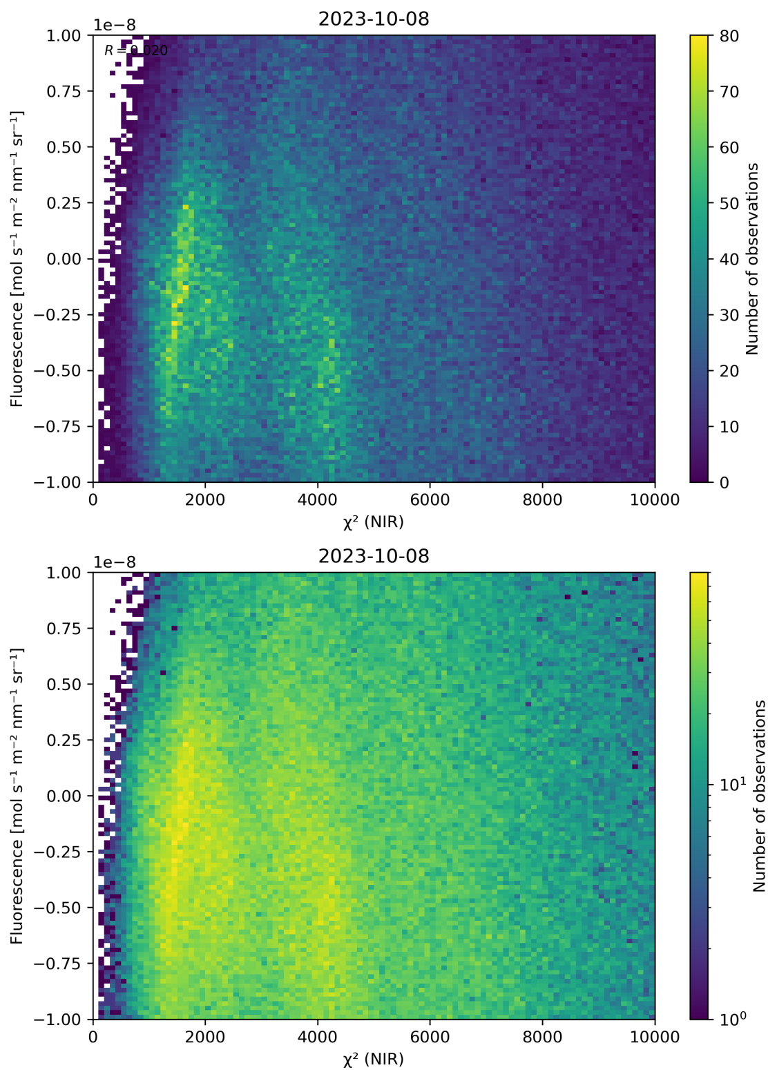
Figure 45: Scatter density plot of “ \chi^2 (NIR)” against “Fluorescence” for 2023-10-07 to 2023-10-09.
