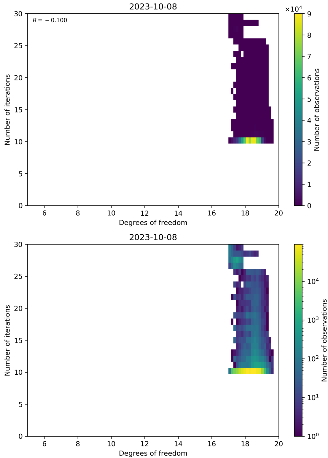
Figure 52: Scatter density plot of “Degrees of freedom” against “Number of iterations” for 2023-10-07 to 2023-10-09.
