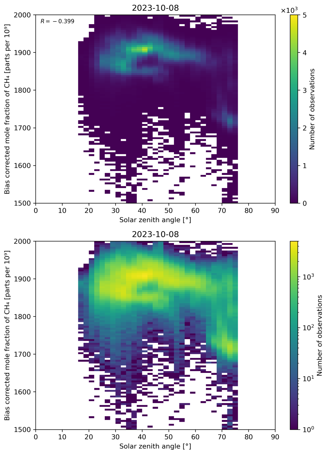
Figure 100: Scatter density plot of “Solar zenith angle” against “Bias corrected mole fraction of CH 4 ” for 2023-10-07 to 2023-10-09.
