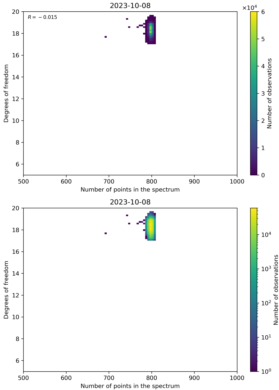
Figure 90: Scatter density plot of “Number of points in the spectrum” against “Degrees of freedom” for 2023-10-07 to 2023-10-09.
