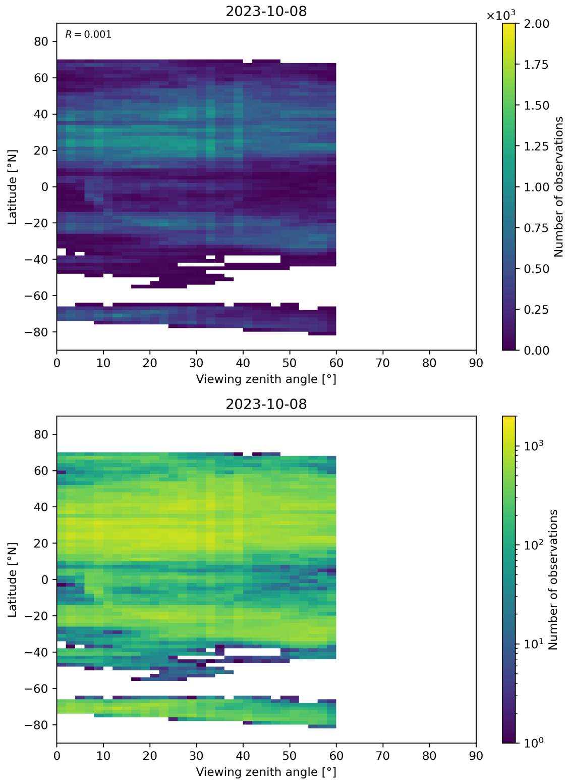
Figure 109: Scatter density plot of “Viewing zenith angle” against “Latitude” for 2023-10-07 to 2023-10-09.
