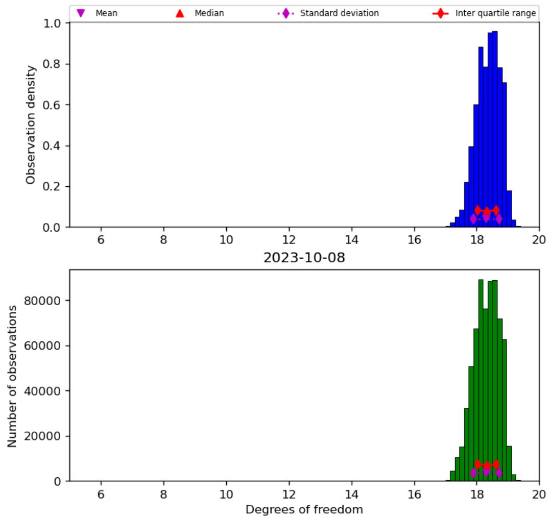
Figure 30: Histogram of “Degrees of freedom” for 2023-10-07 to 2023-10-09
