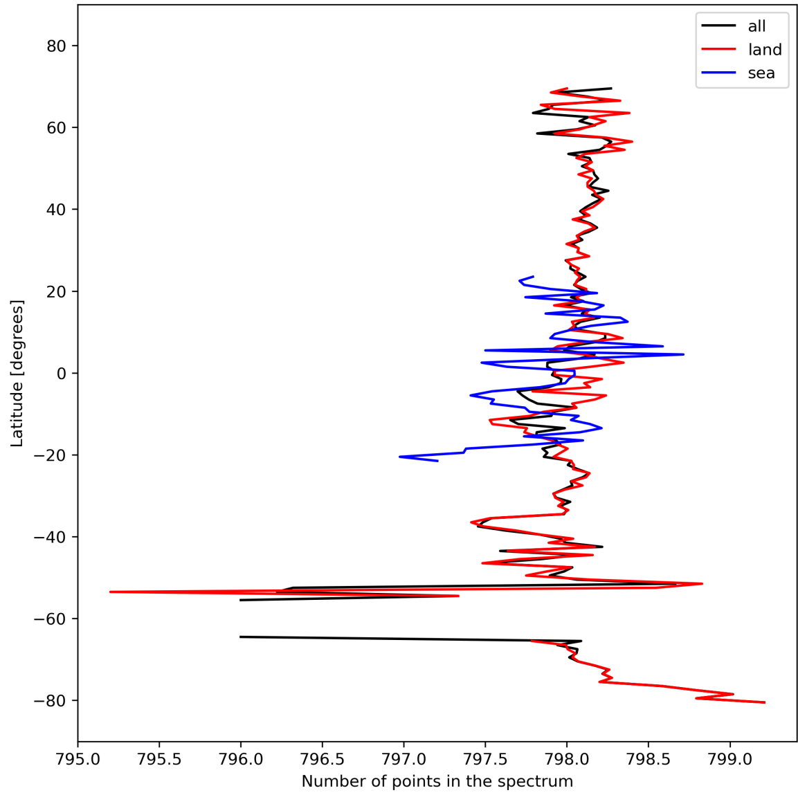
Figure 15: Zonal average of “Number of points in the spectrum” for 2023-10-07 to 2023-10-09.
