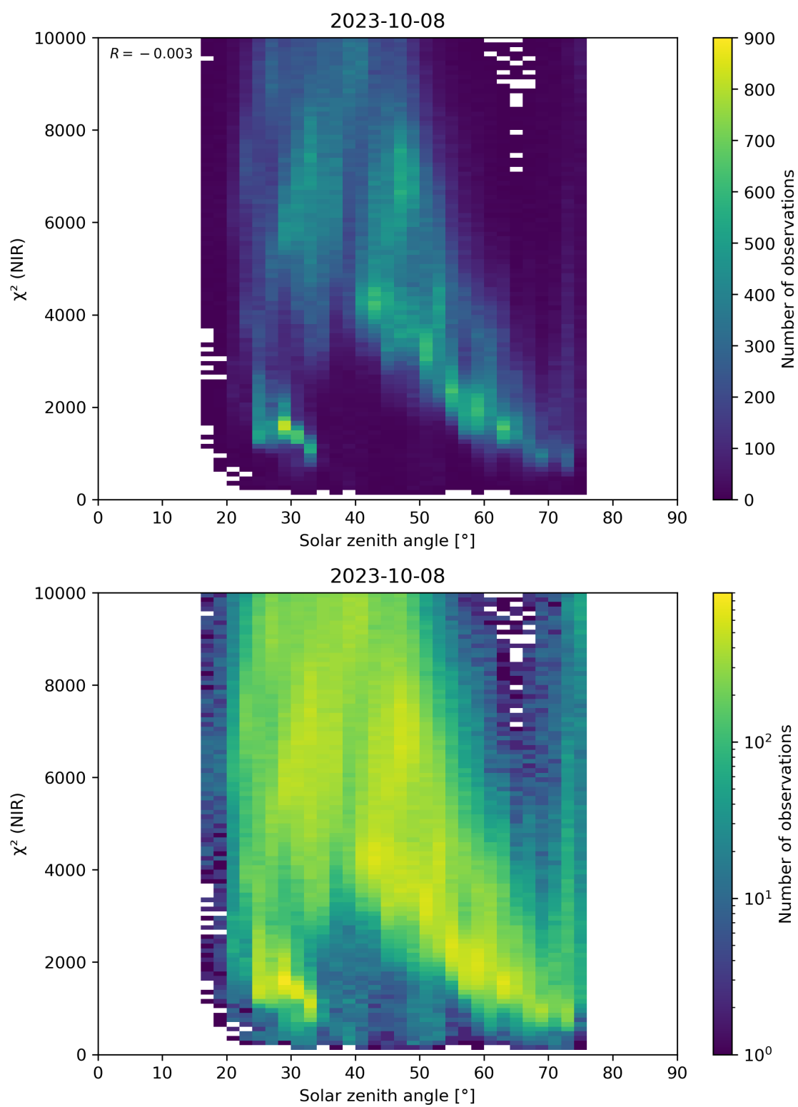
Figure 94: Scatter density plot of “Solar zenith angle” against “ \chi^2 (NIR)” for 2023-10-07 to 2023-10-09.
