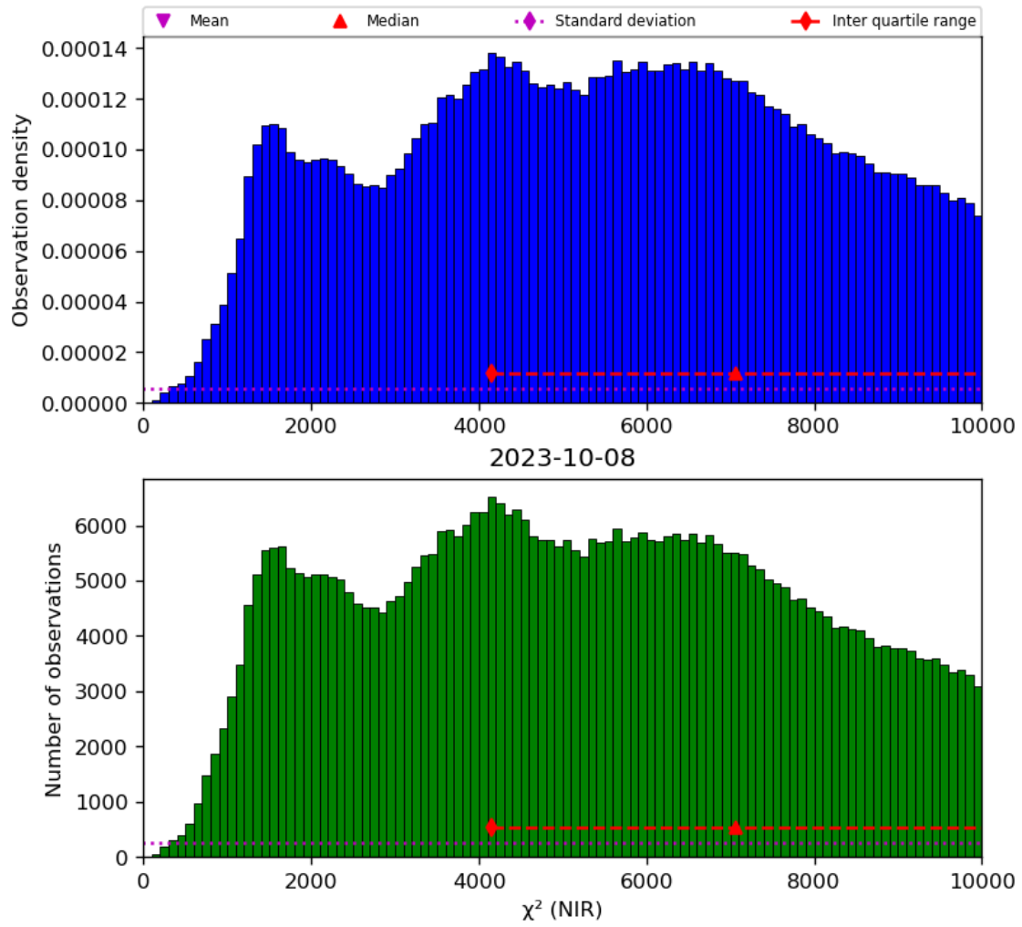
Figure 29: Histogram of “ \chi^2 (NIR)” for 2023-10-07 to 2023-10-09
