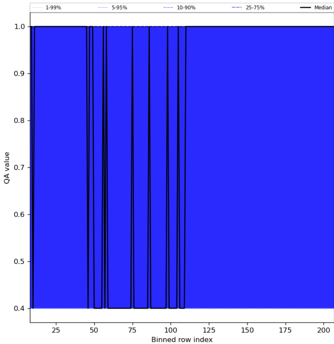
Figure 33: Along track statistics of “QA value” for 2023-10-07 to 2023-10-09
