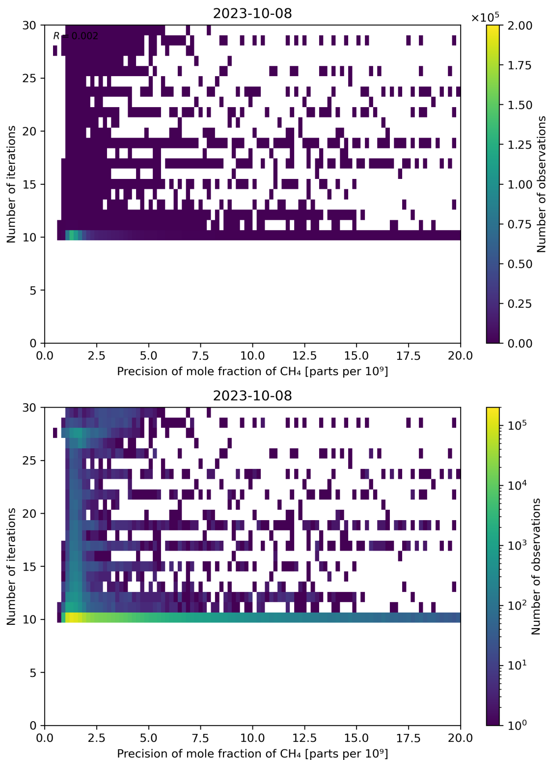
Figure 83: Scatter density plot of “Precision of mole fraction of CH 4 ” against “Number of iterations” for 2023-10-07 to 2023-10-09.
