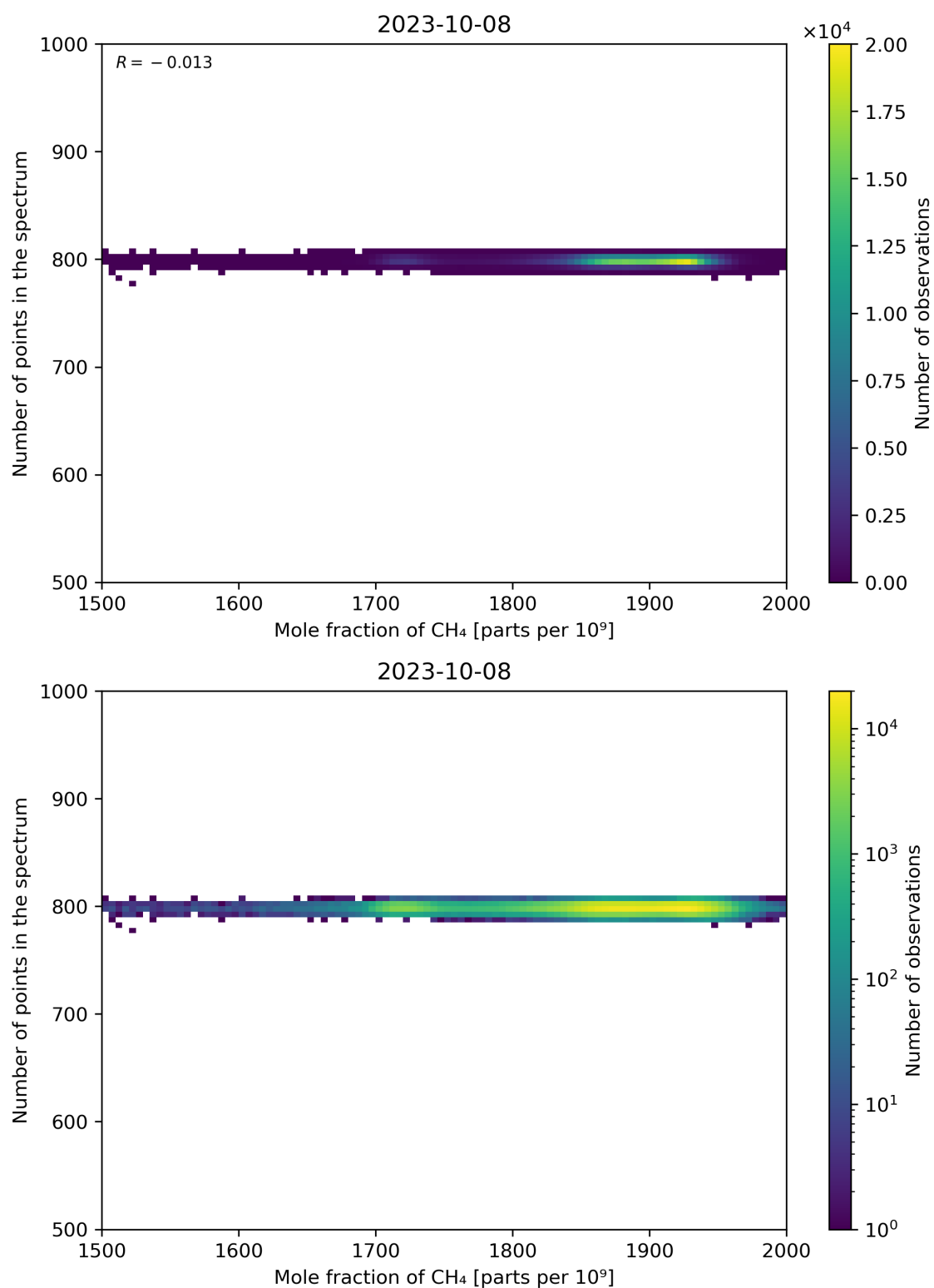
Figure 77: Scatter density plot of “Mole fraction of CH 4 ” against “Number of points in the spectrum” for 2023-10-07 to 2023-10-09.
