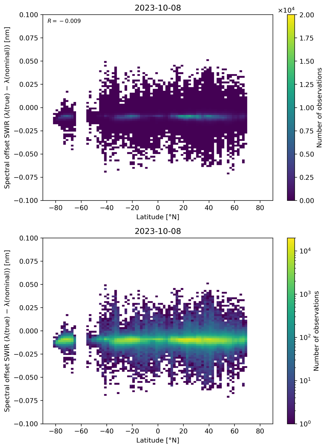
Figure 62: Scatter density plot of “Latitude” against “Spectral offset SWIR ( \lambda(\text{true}) - \lambda(\text{nominal}) )” for 2023-10-07 to 2023-10-09.
