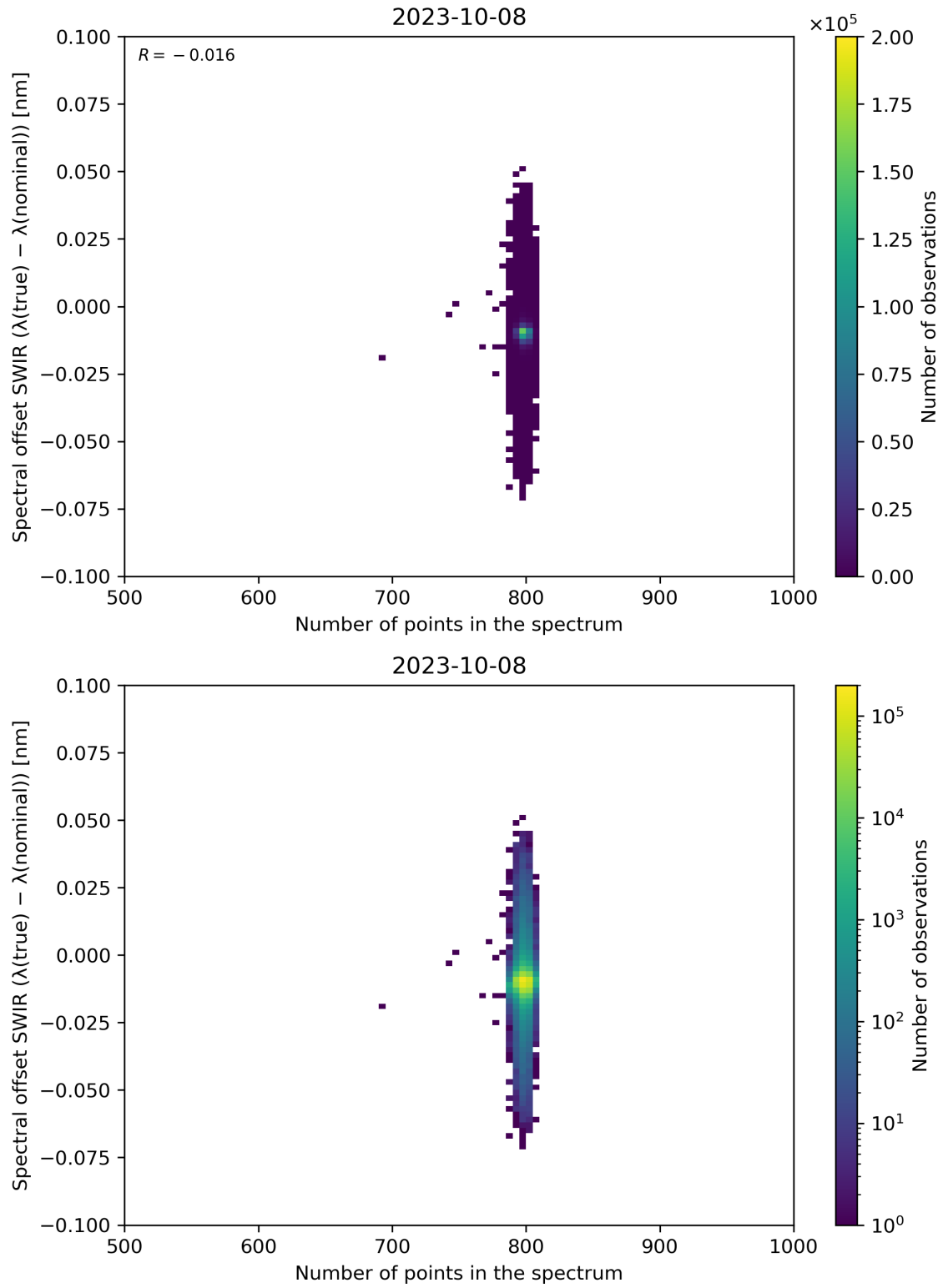
Figure 93: Scatter density plot of “Number of points in the spectrum” against “Spectral offset SWIR ( \lambda(\text{true}) - \lambda(\text{nominal}) )” for 2023-10-07 to 2023-10-09.
