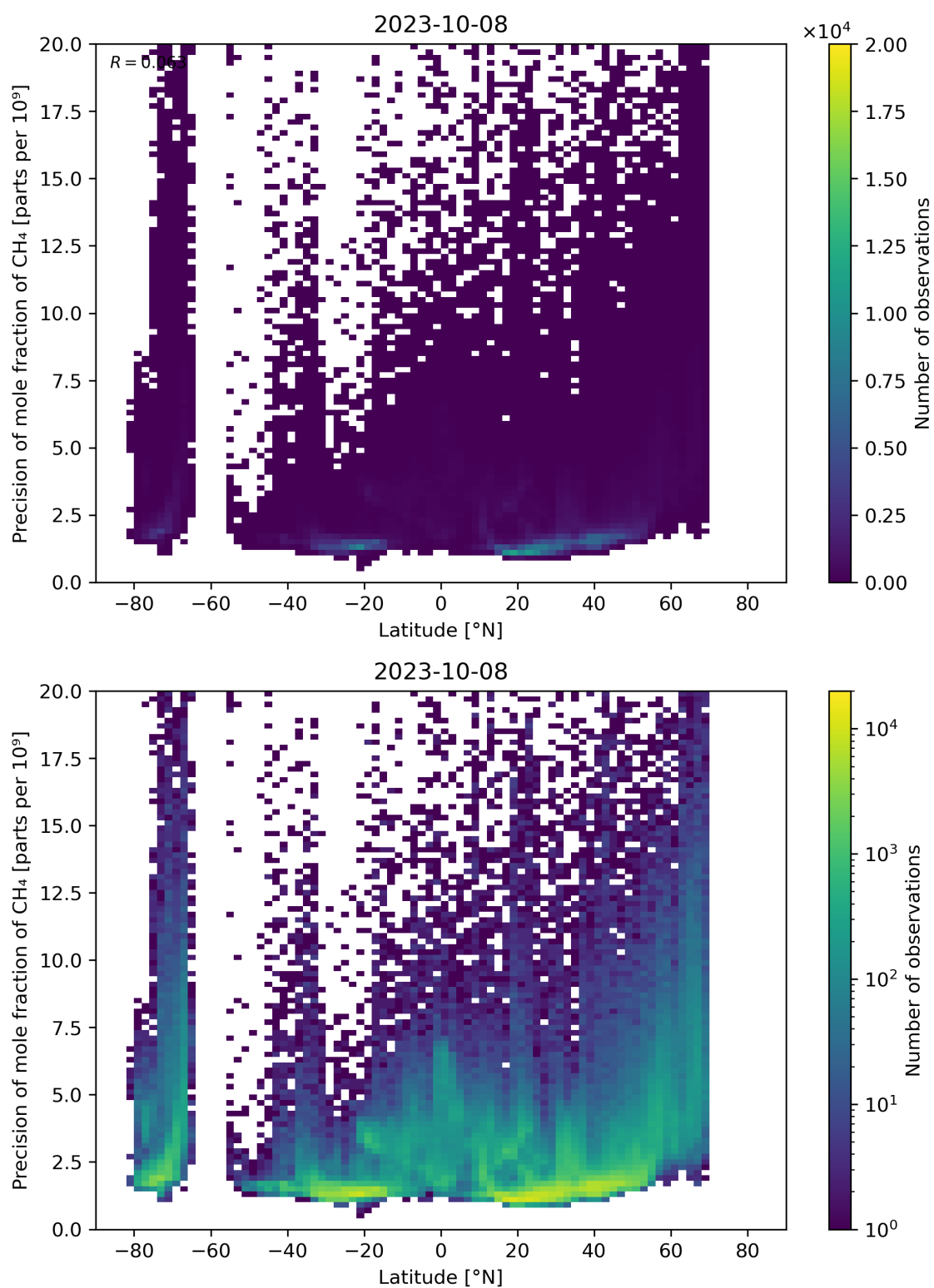
Figure 59: Scatter density plot of “Latitude” against “Precision of mole fraction of CH 4 ” for 2023-10-07 to 2023-10-09.
