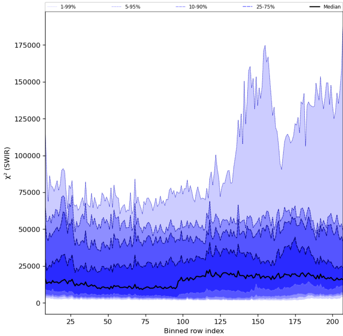
Figure 39: Along track statistics of “ \chi^2 (SWIR)” for 2023-10-07 to 2023-10-09
