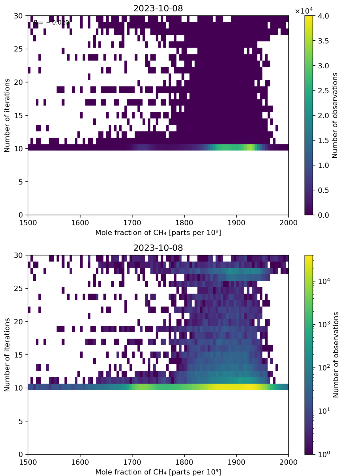
Figure 76: Scatter density plot of “Mole fraction of CH 4 ” against “Number of iterations” for 2023-10-07 to 2023-10-09.
