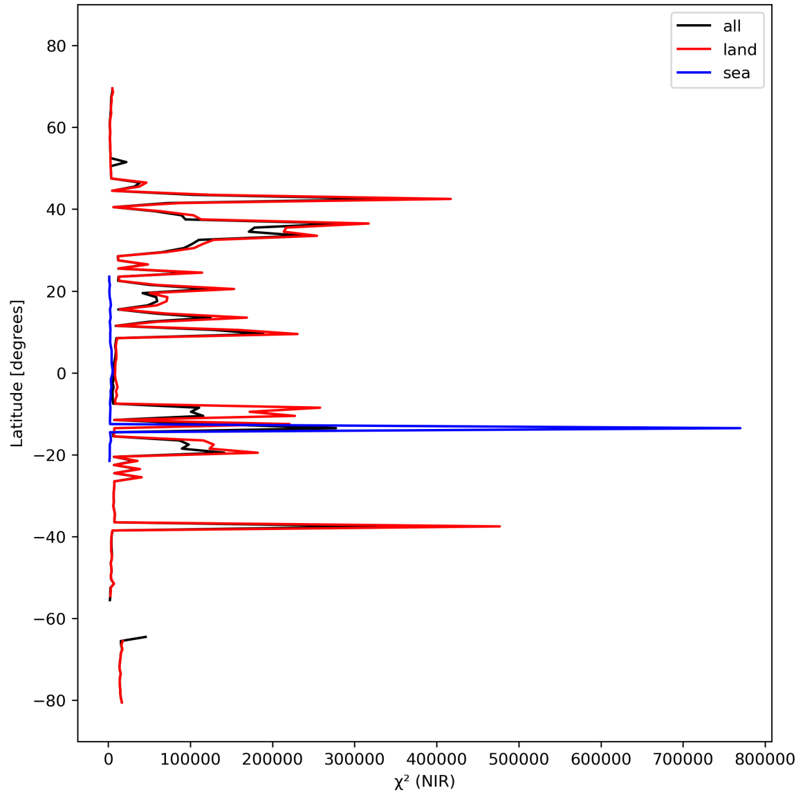
Figure 18: Zonal average of “ \chi^2 (NIR)” for 2023-10-07 to 2023-10-09.
