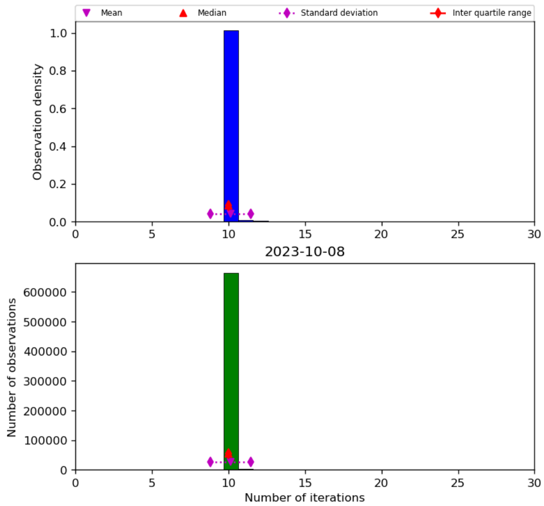
Figure 31: Histogram of “Number of iterations” for 2023-10-07 to 2023-10-09
