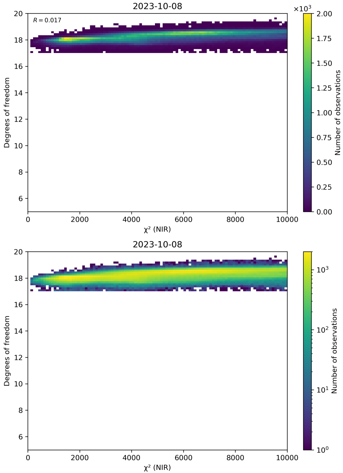
Figure 44: Scatter density plot of “ \chi^2 (NIR)” against “Degrees of freedom” for 2023-10-07 to 2023-10-09.
