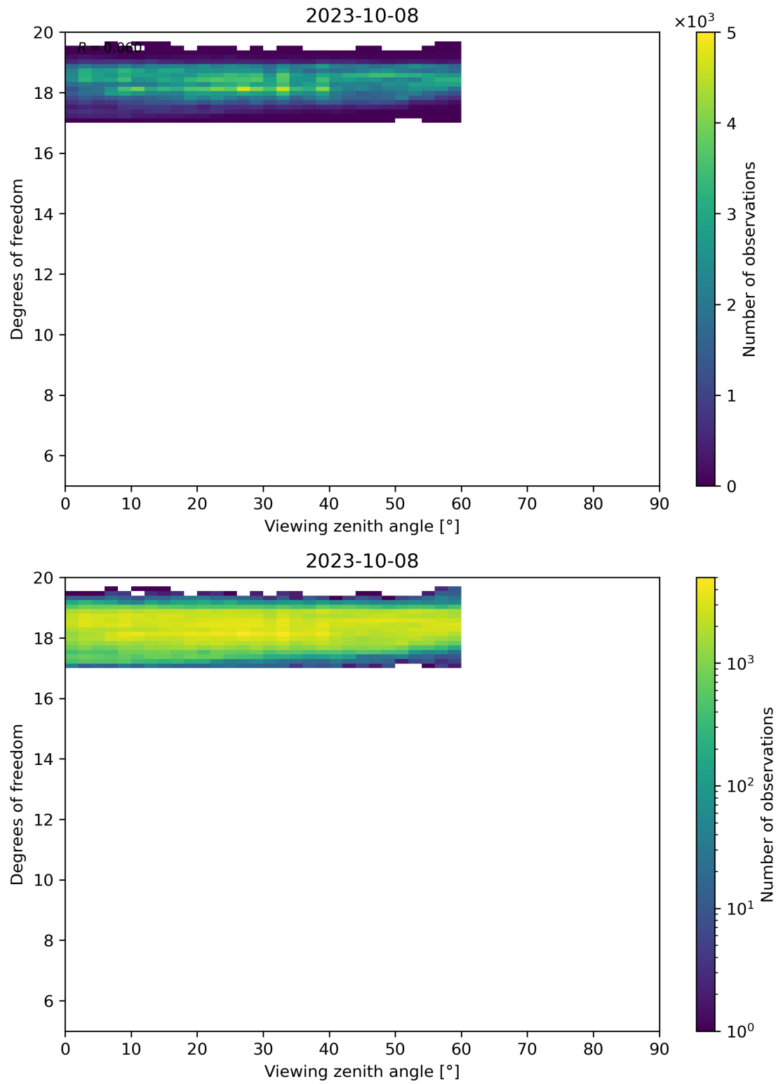
Figure 107: Scatter density plot of “Viewing zenith angle” against “Degrees of freedom” for 2023-10-07 to 2023-10-09.
