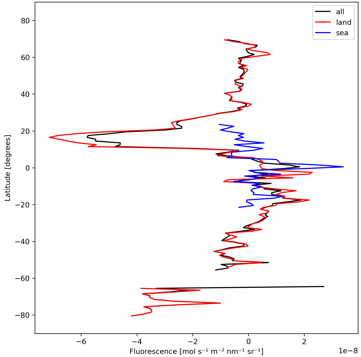
Figure 21: Zonal average of “Fluorescence” for 2023-10-07 to 2023-10-09.
