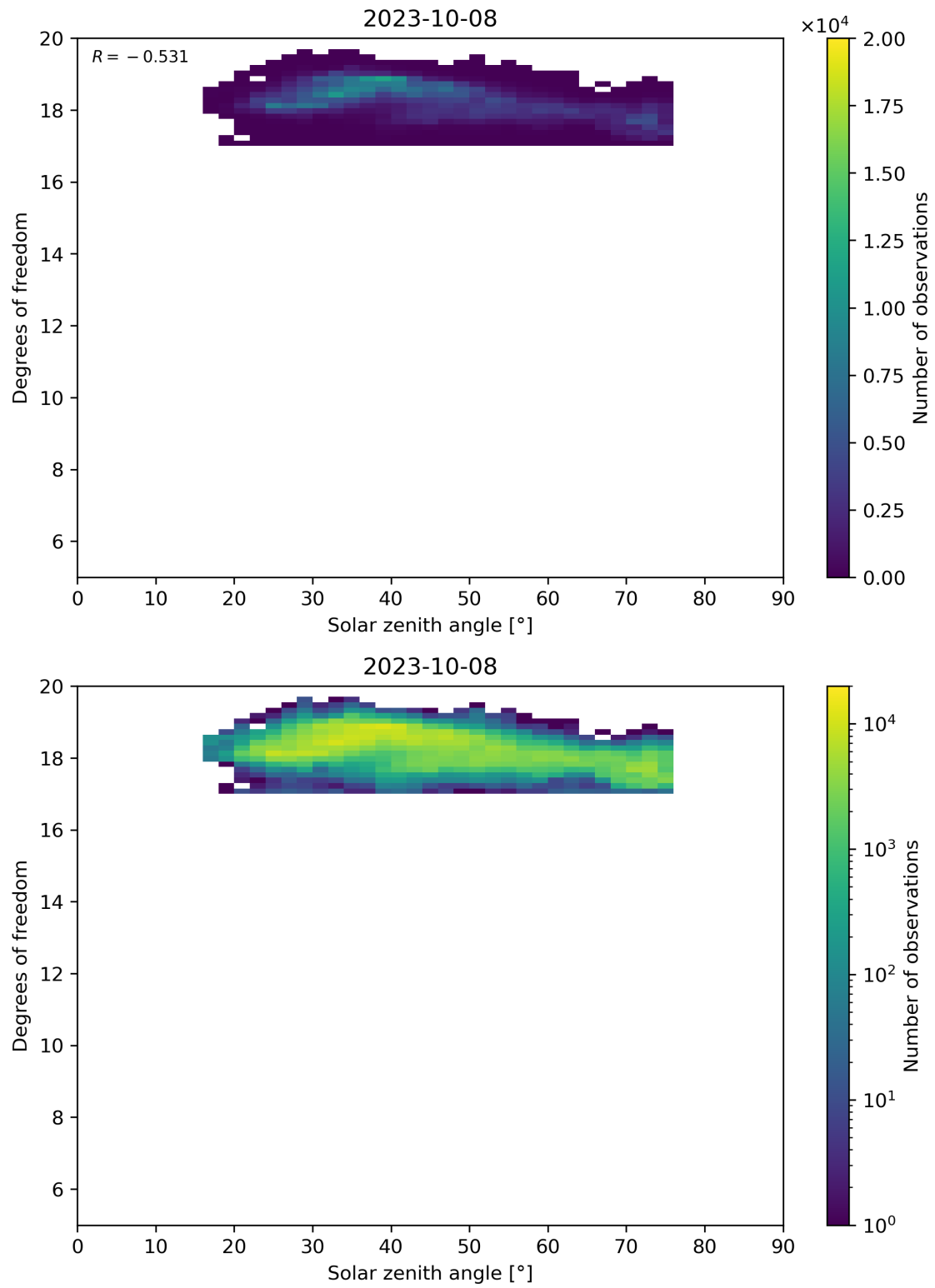
Figure 96: Scatter density plot of “Solar zenith angle” against “Degrees of freedom” for 2023-10-07 to 2023-10-09.
