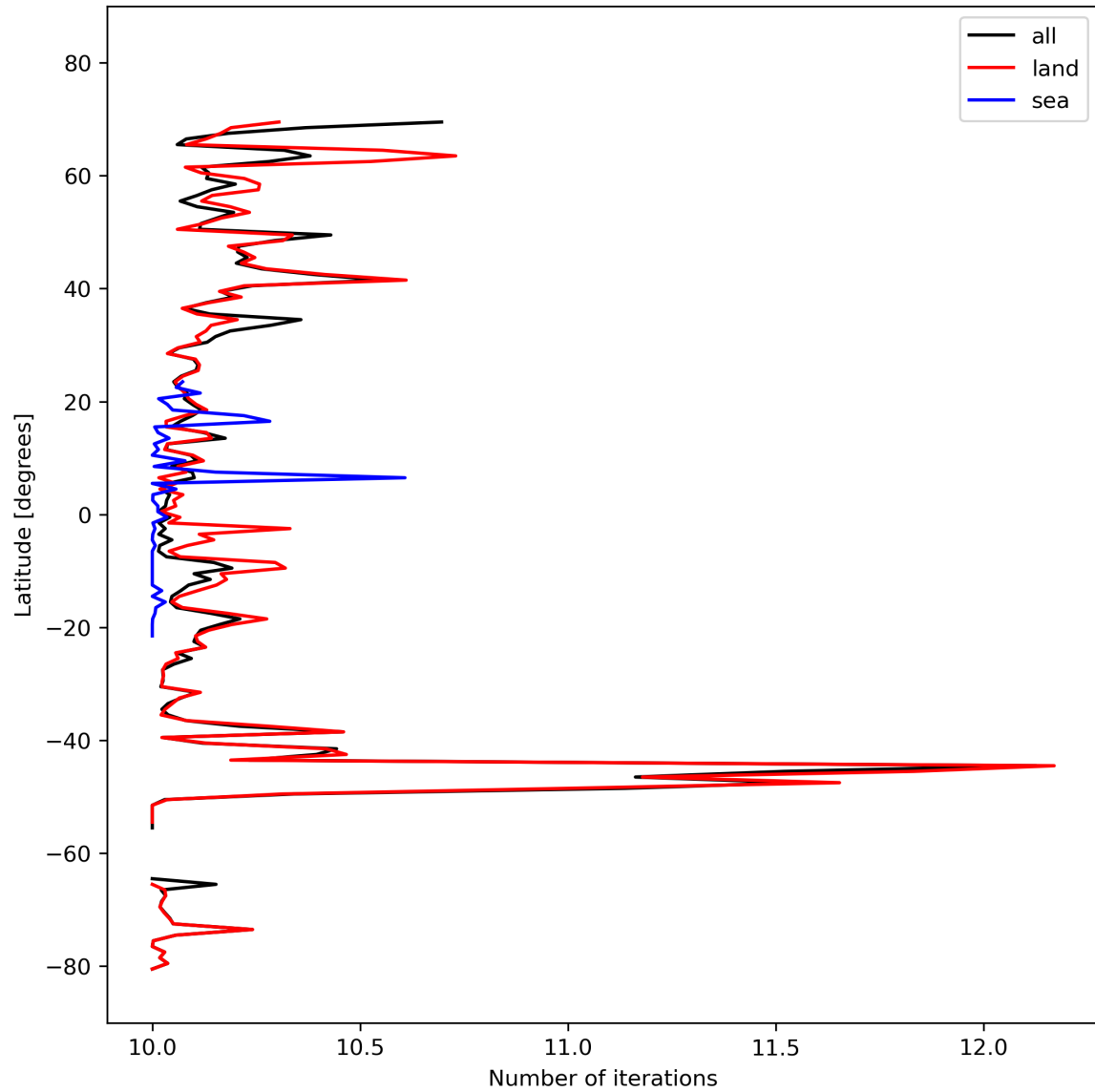
Figure 20: Zonal average of “Number of iterations” for 2023-10-07 to 2023-10-09.
