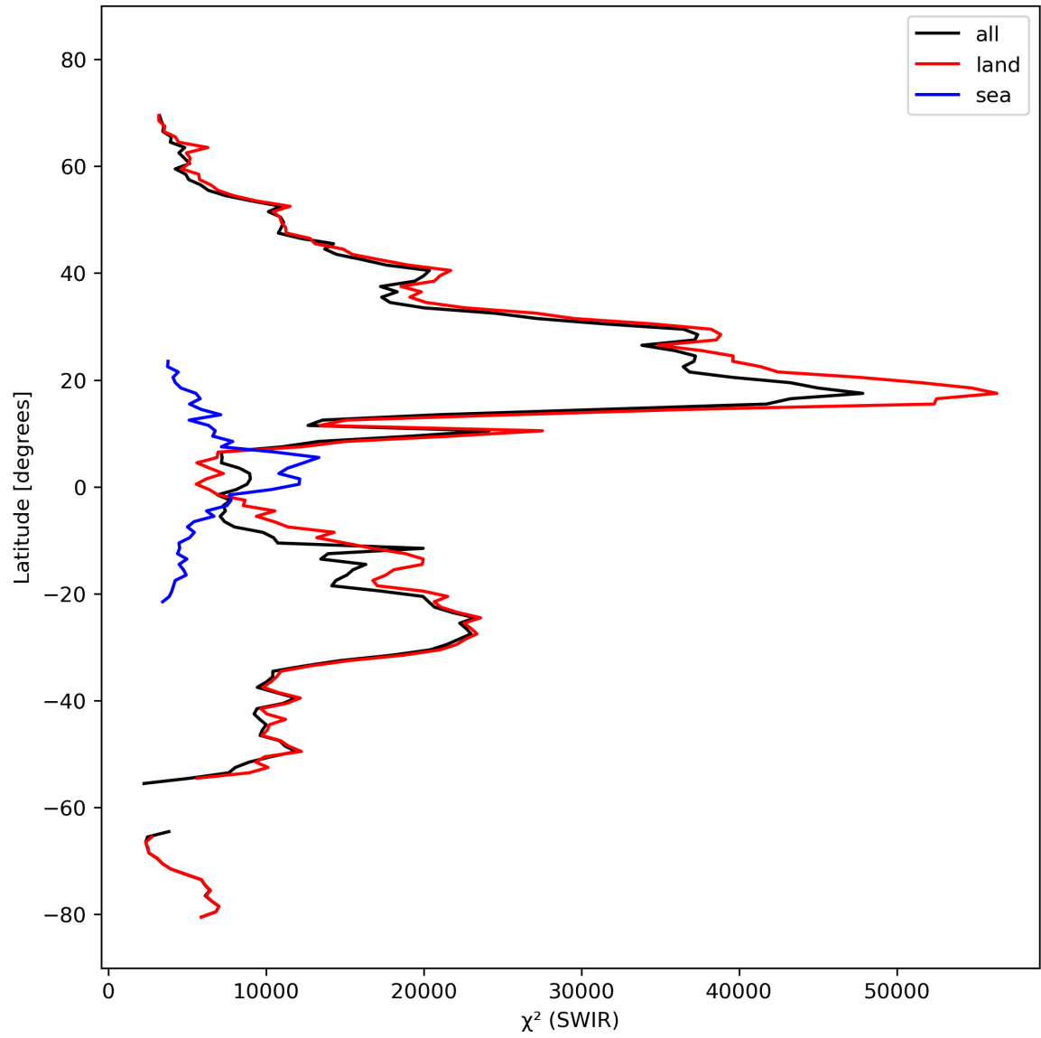
Figure 17: Zonal average of “ \chi^2 (SWIR)” for 2023-10-07 to 2023-10-09.
