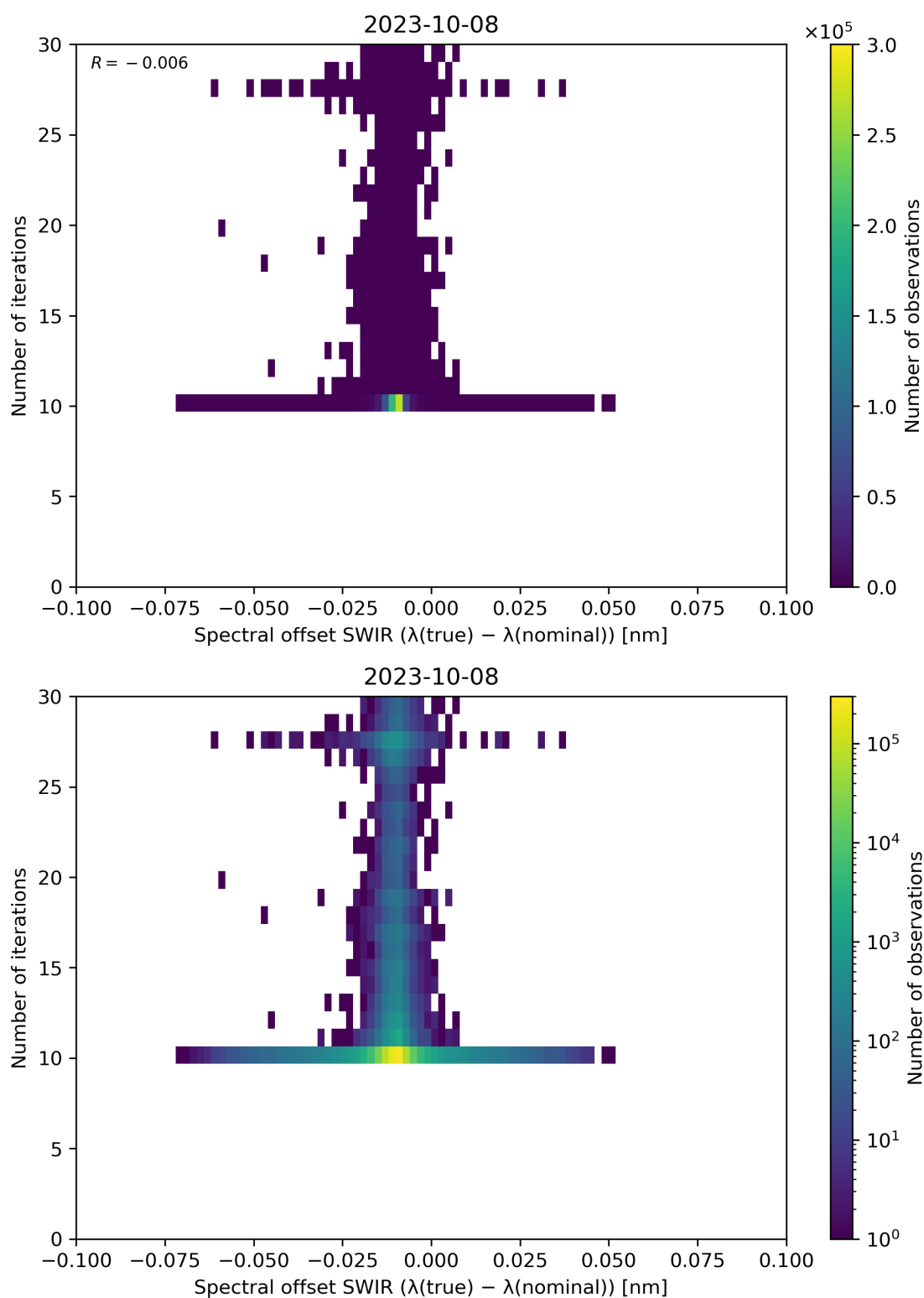
Figure 121: Scatter density plot of “Spectral offset SWIR ( \lambda(\text{true}) - \lambda(\text{nominal}) )” against “Number of iterations” for 2023-10-07 to 2023-10-09.
