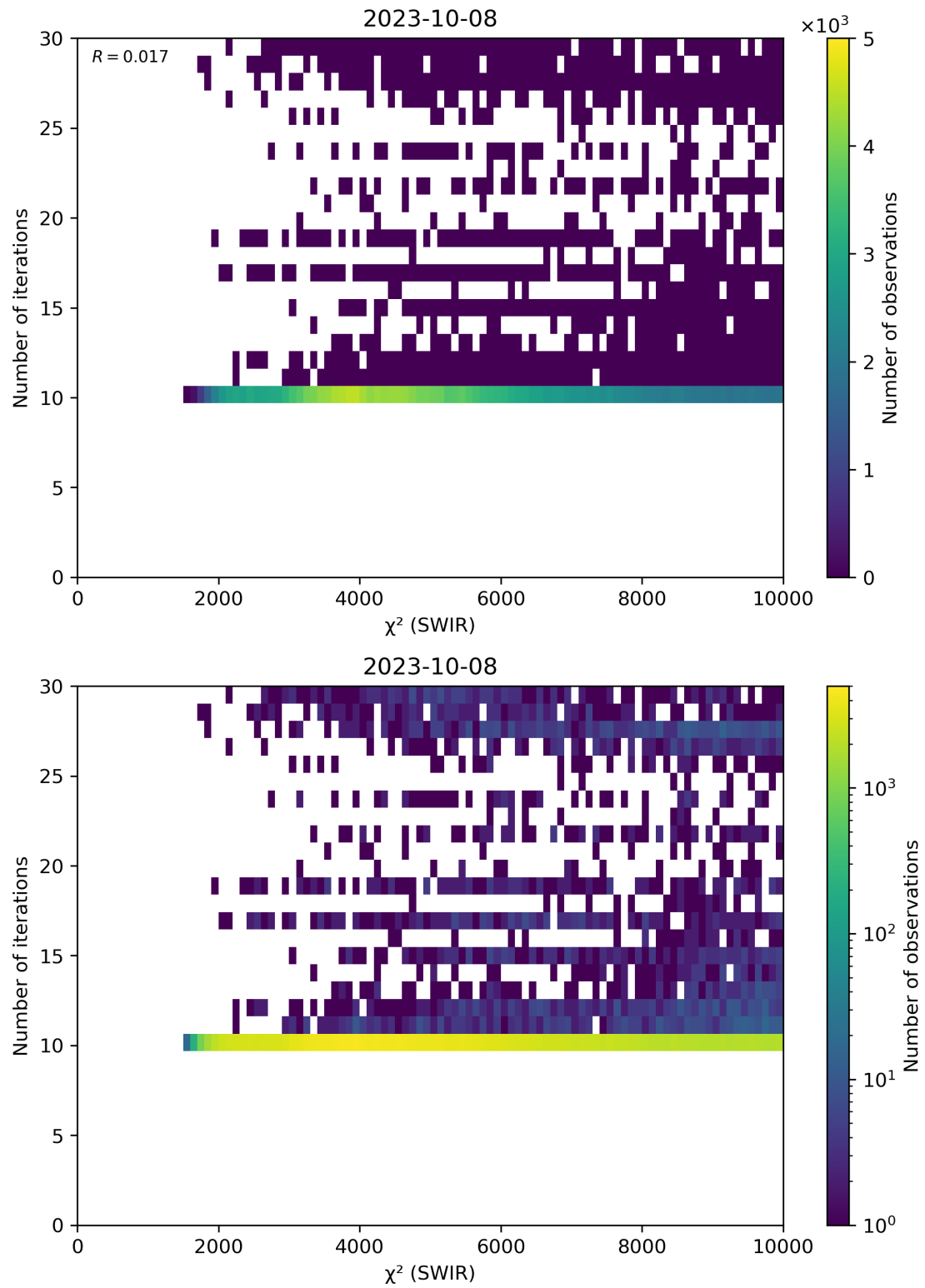
Figure 50: Scatter density plot of “ \chi^2 (SWIR)” against “Number of iterations” for 2023-10-07 to 2023-10-09.
