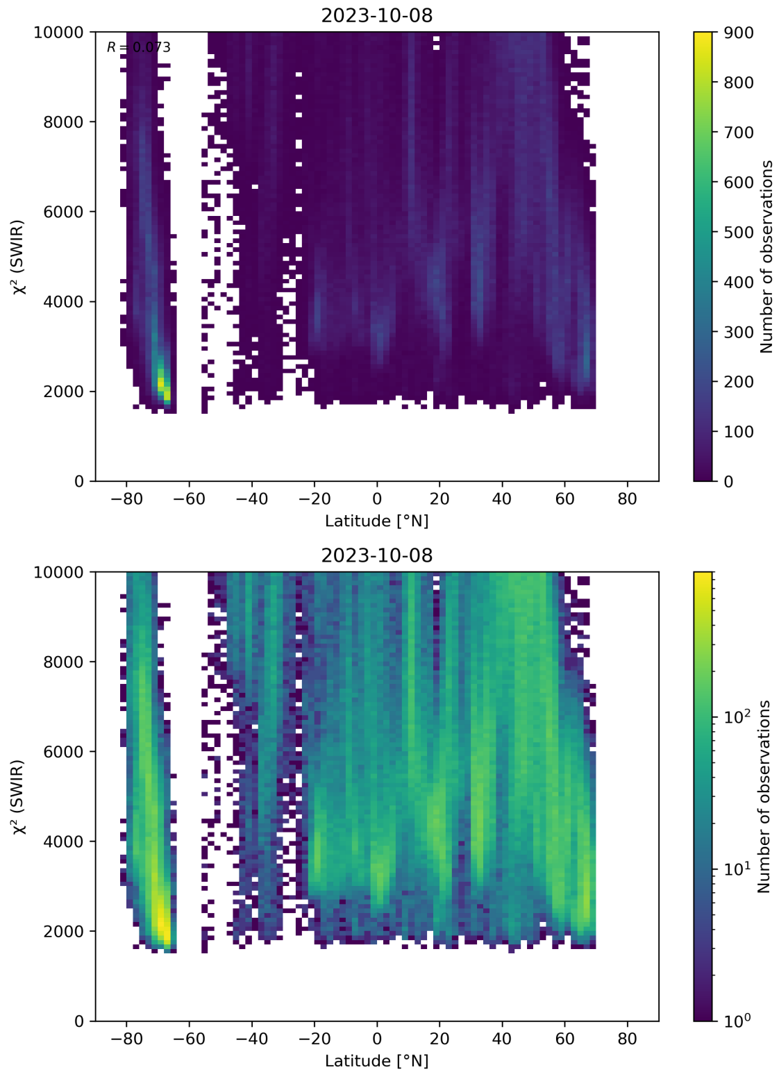
Figure 54: Scatter density plot of “Latitude” against “ \chi^2 (SWIR)” for 2023-10-07 to 2023-10-09.
