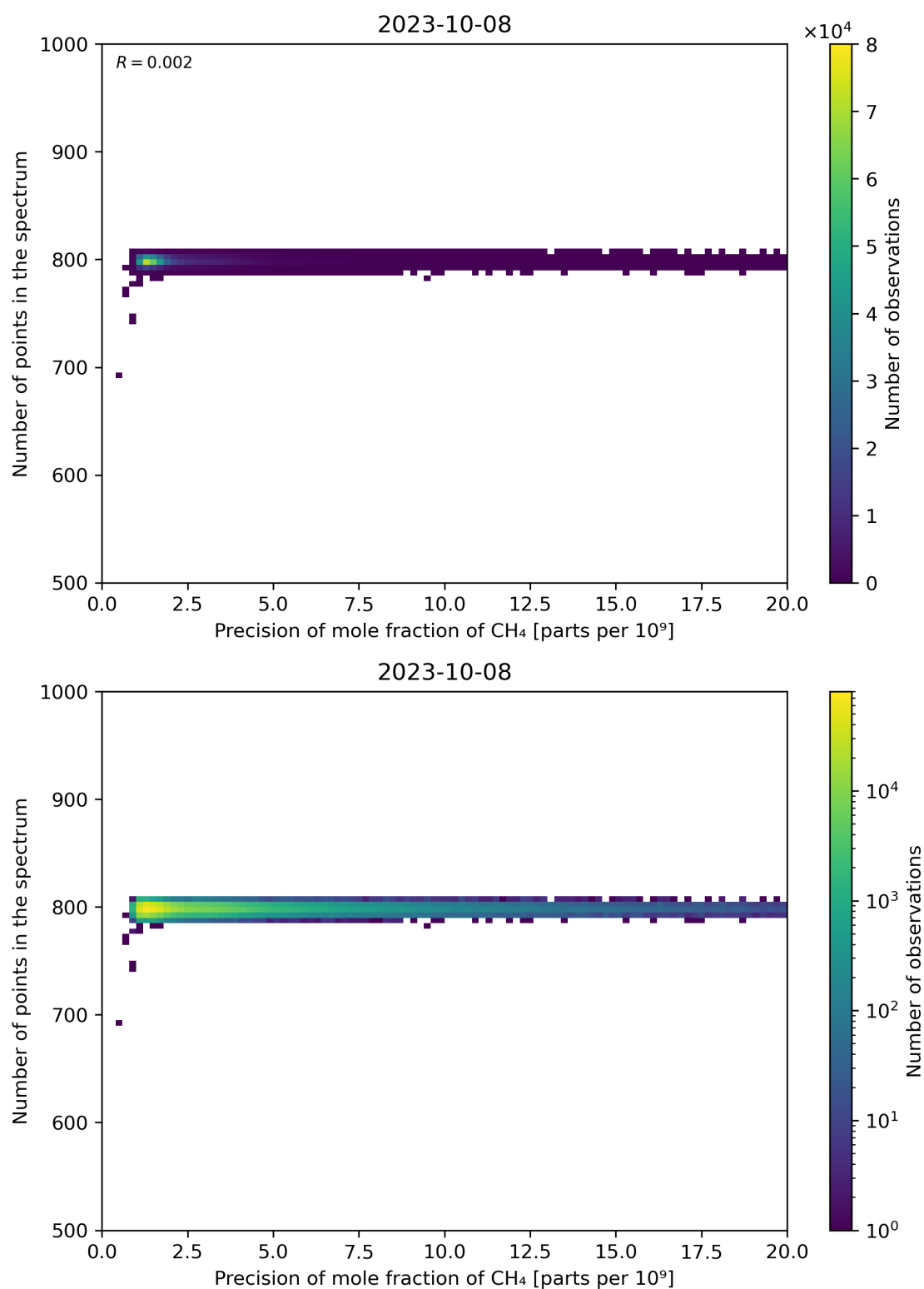
Figure 84: Scatter density plot of “Precision of mole fraction of \text{CH}_4 ” against “Number of points in the spectrum” for 2023-10-07 to 2023-10-09.
