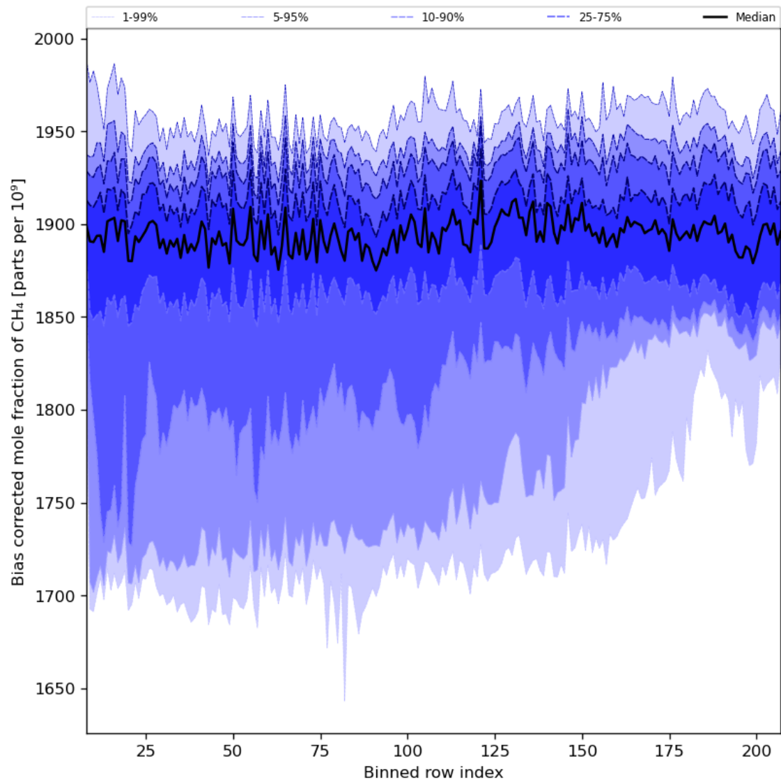
Figure 36: Along track statistics of “Bias corrected mole fraction of CH 4 ” for 2023-10-07 to 2023-10-09
