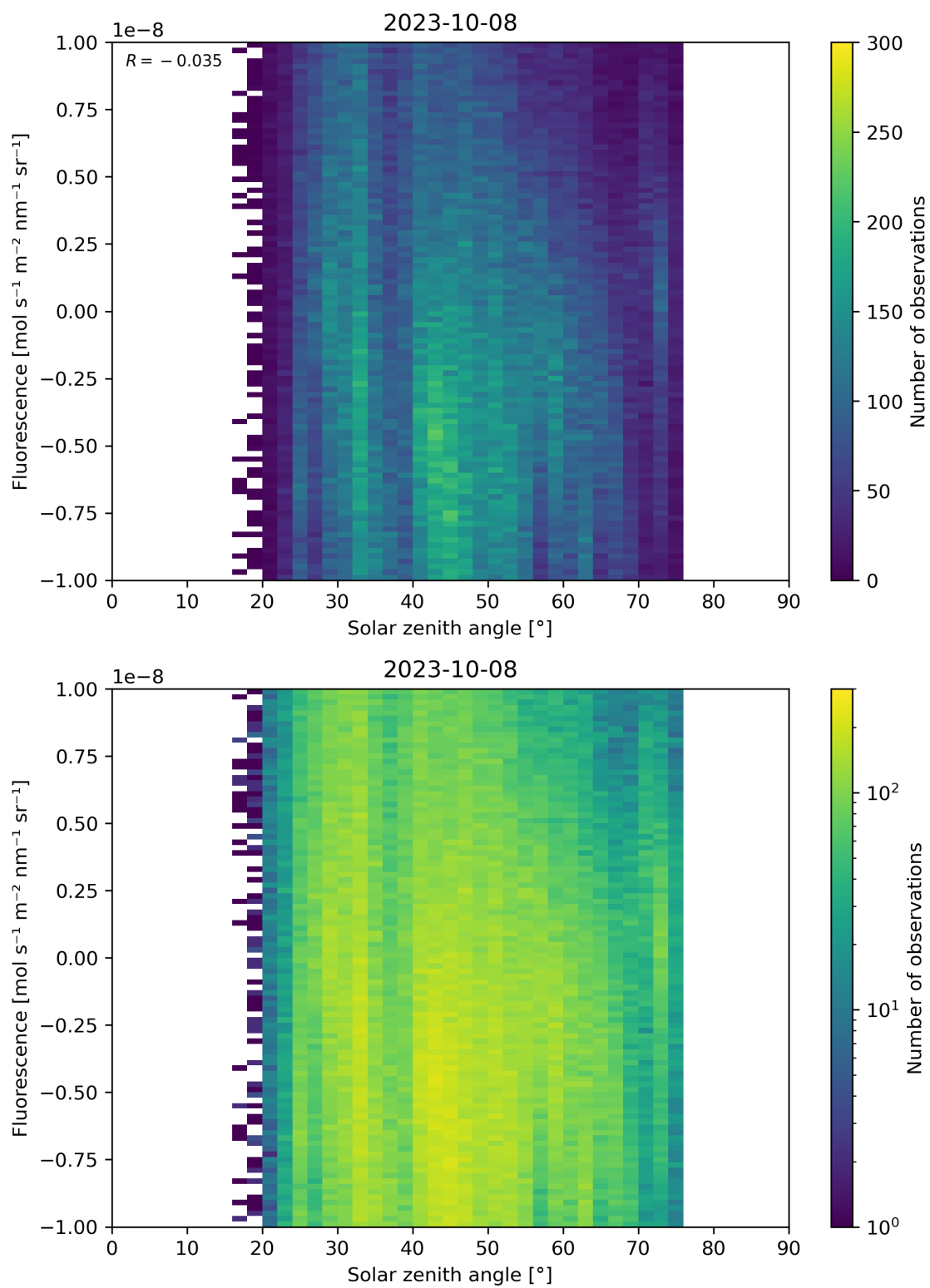
Figure 97: Scatter density plot of “Solar zenith angle” against “Fluorescence” for 2023-10-07 to 2023-10-09.
