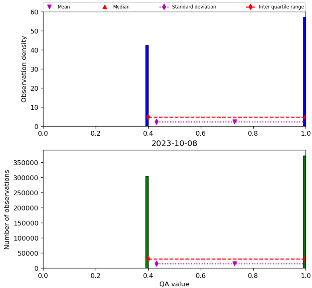
Figure 22: Histogram of “QA value” for 2023-10-07 to 2023-10-09
