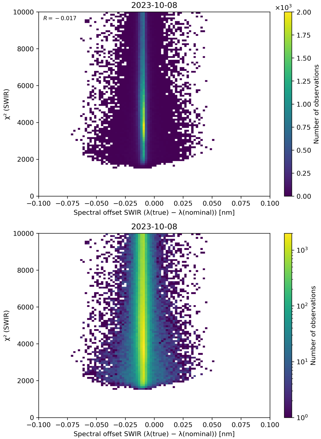
Figure 118: Scatter density plot of “Spectral offset SWIR ( \lambda(\text{true}) - \lambda(\text{nominal}) )” against “ \chi^2 (SWIR)” for 2023-10-07 to 2023-10-09.
