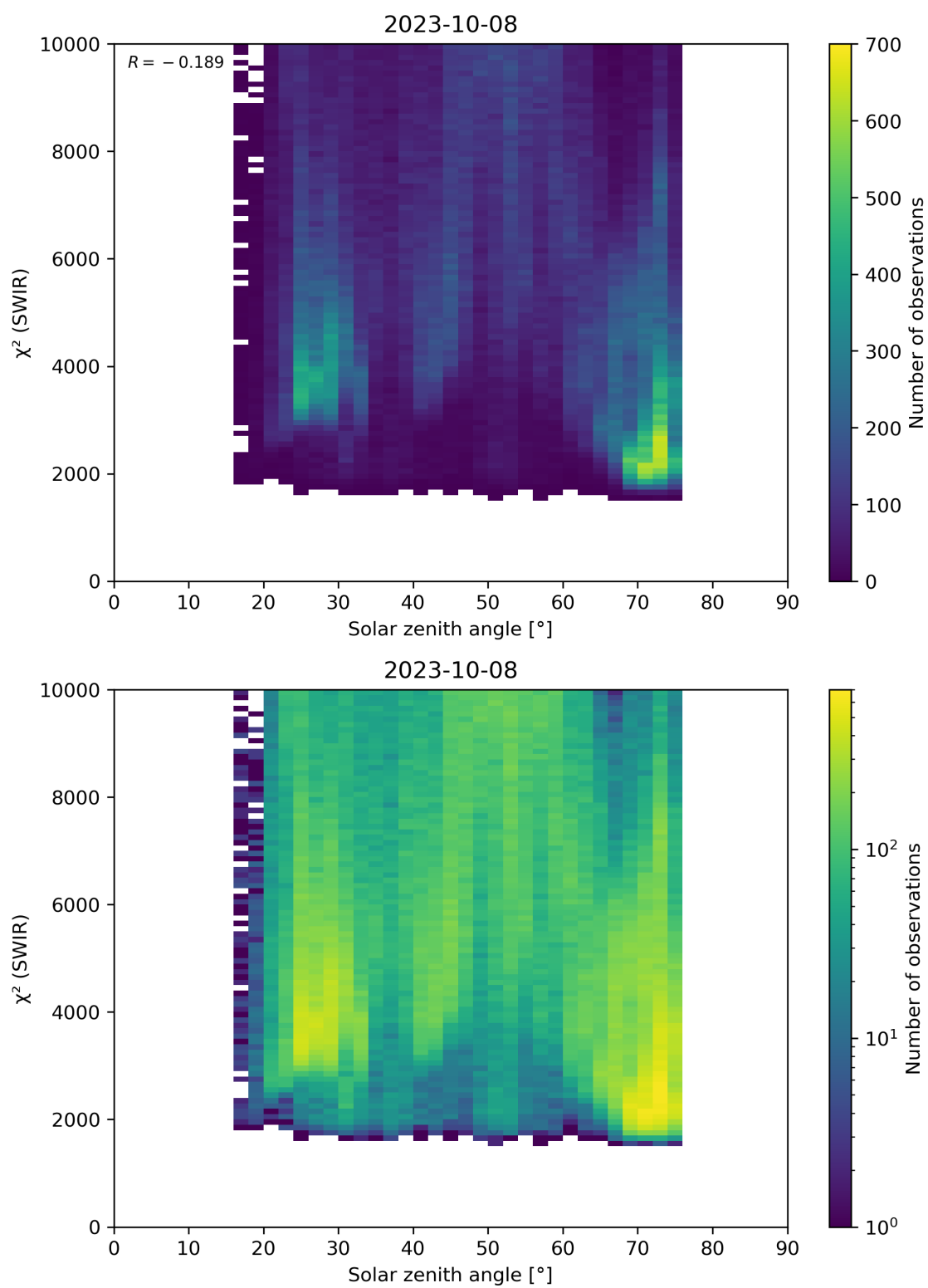
Figure 95: Scatter density plot of “Solar zenith angle” against “ \chi^2 (SWIR)” for 2023-10-07 to 2023-10-09.
