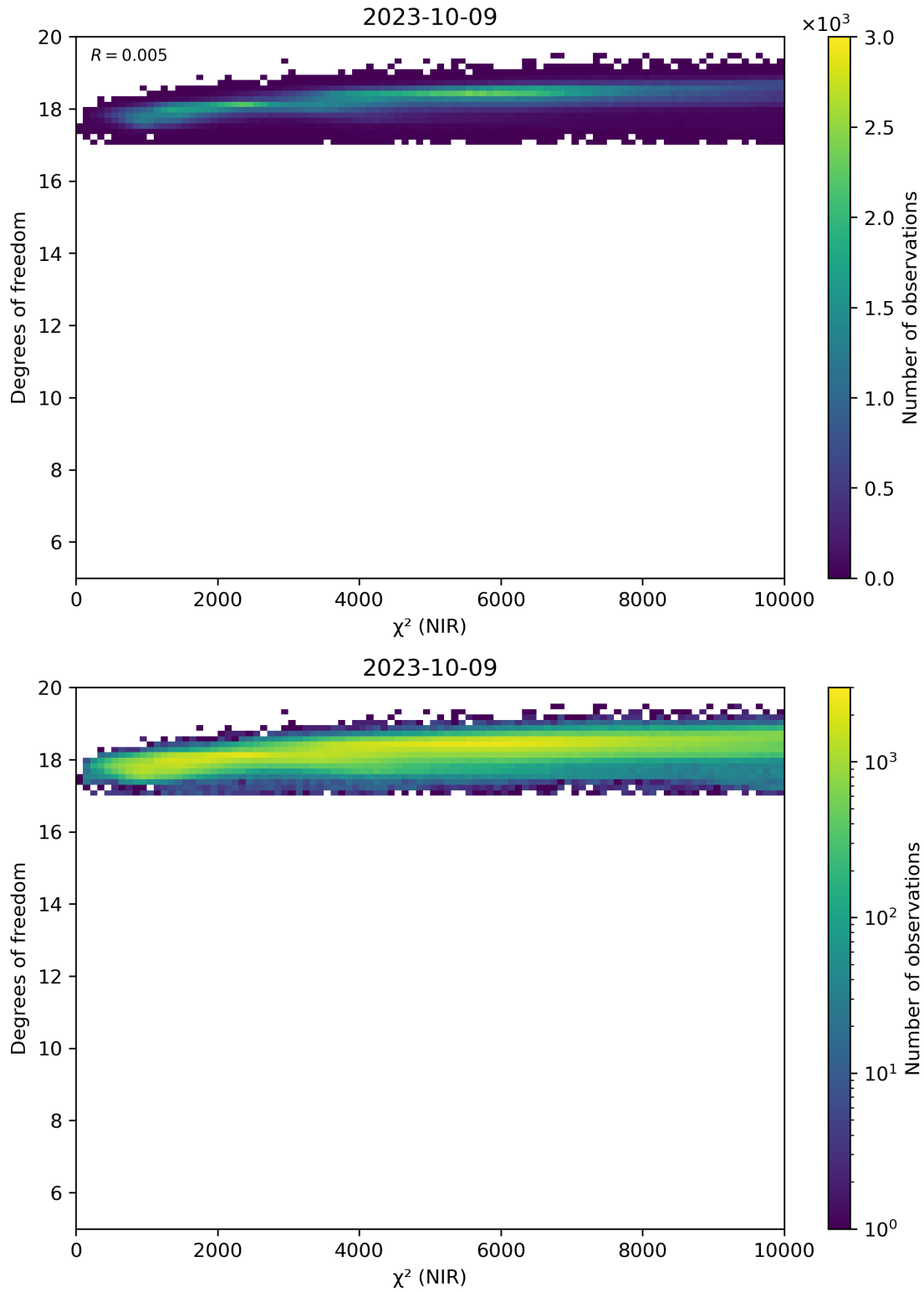
Figure 44: Scatter density plot of “ \chi^2 (NIR)” against “Degrees of freedom” for 2023-10-08 to 2023-10-10.
