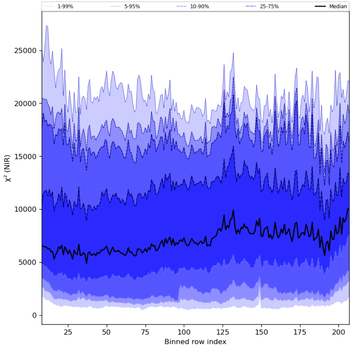
Figure 40: Along track statistics of “ \chi^2 (NIR)” for 2023-10-08 to 2023-10-10
