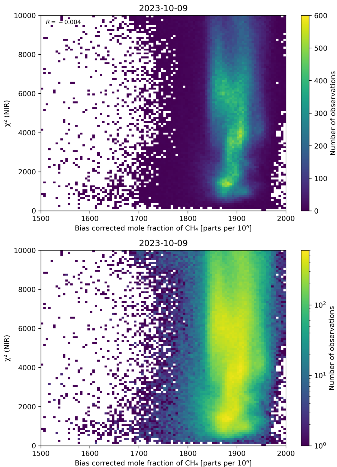
Figure 63: Scatter density plot of “Bias corrected mole fraction of CH 4 ” against “ \chi^2 (NIR)” for 2023-10-08 to 2023-10-10.
