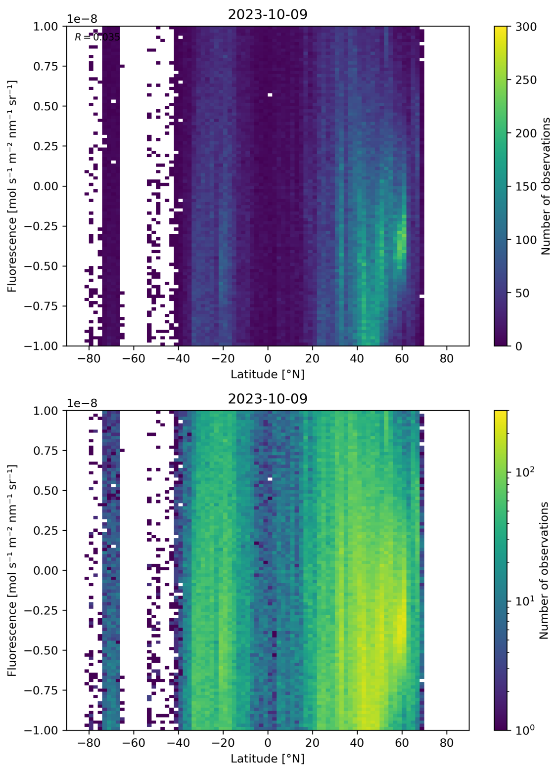
Figure 56: Scatter density plot of “Latitude” against “Fluorescence” for 2023-10-08 to 2023-10-10.
