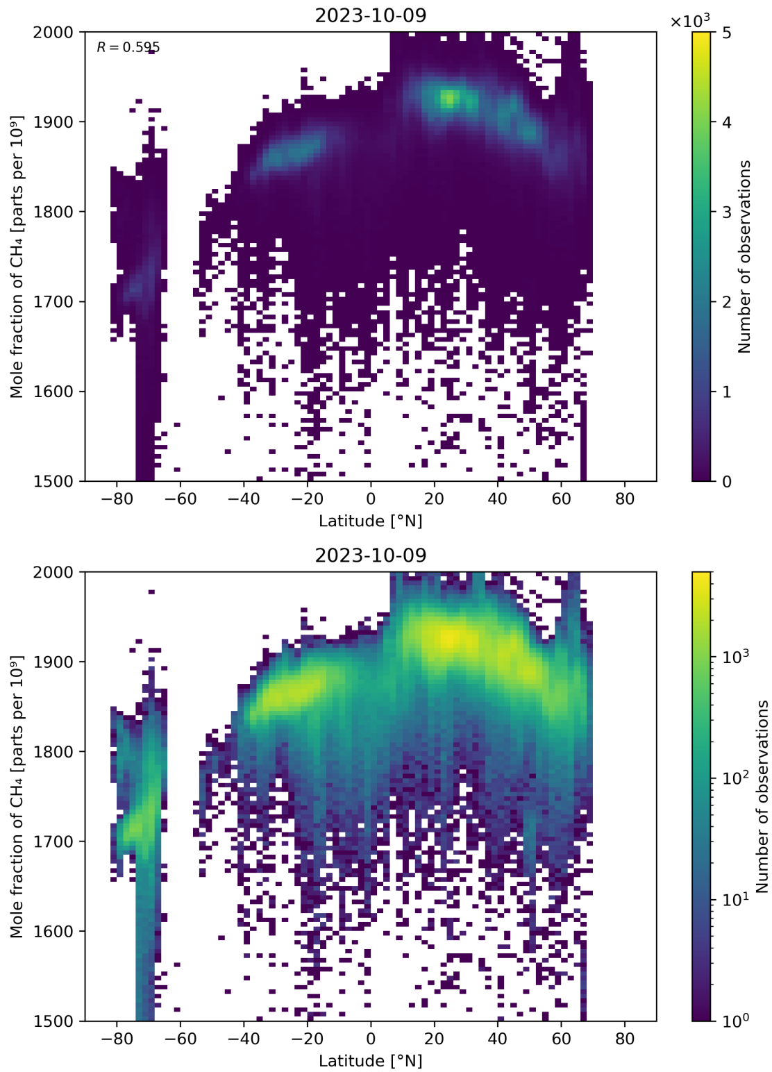
Figure 57: Scatter density plot of “Latitude” against “Mole fraction of CH 4 ” for 2023-10-08 to 2023-10-10.
