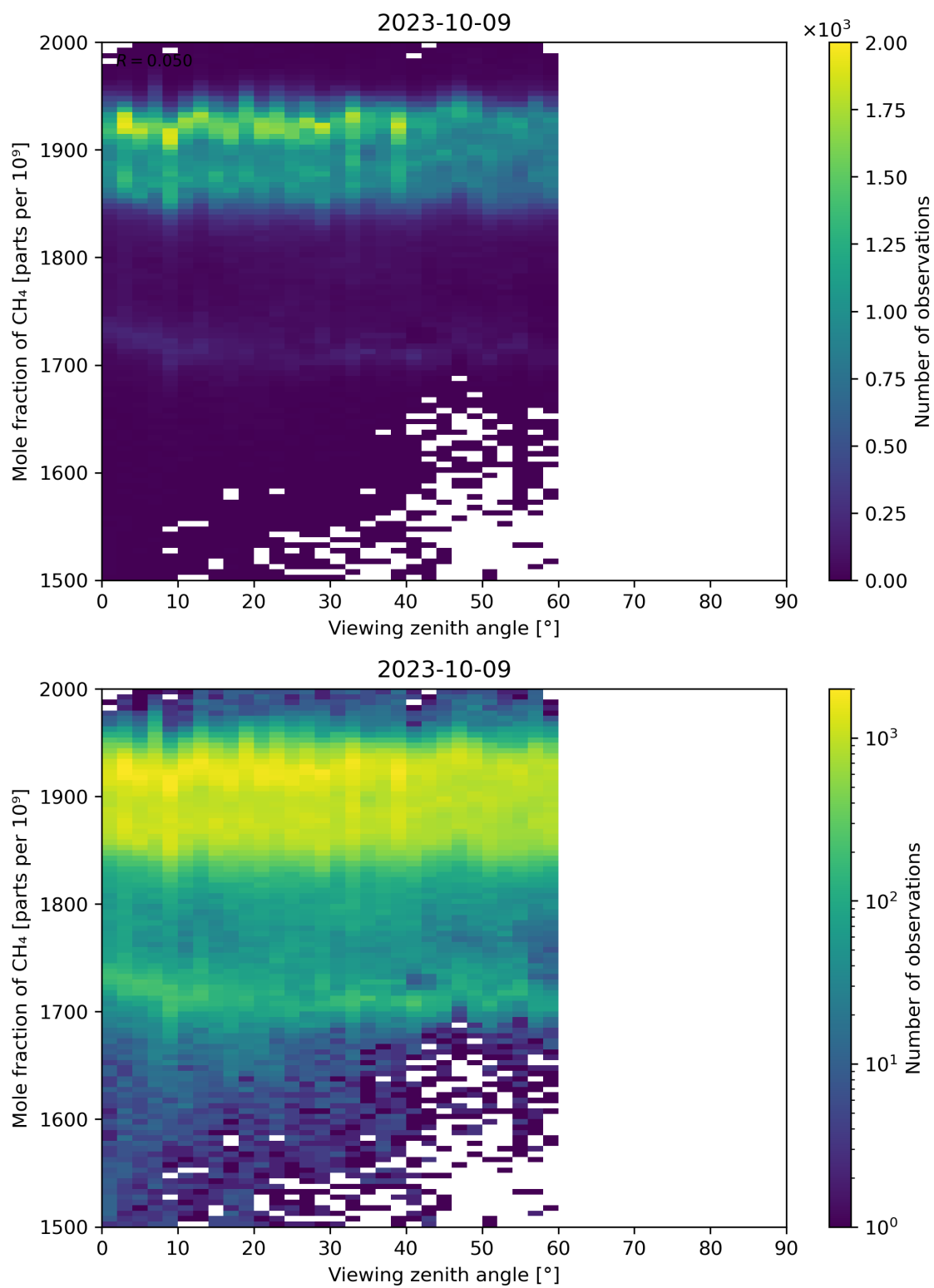
Figure 110: Scatter density plot of “Viewing zenith angle” against “Mole fraction of CH 4 ” for 2023-10-08 to 2023-10-10.
