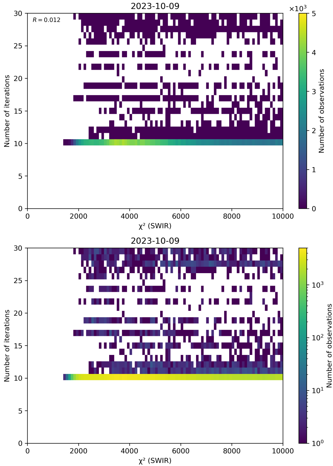
Figure 50: Scatter density plot of “ \chi^2 (SWIR)” against “Number of iterations” for 2023-10-08 to 2023-10-10.
