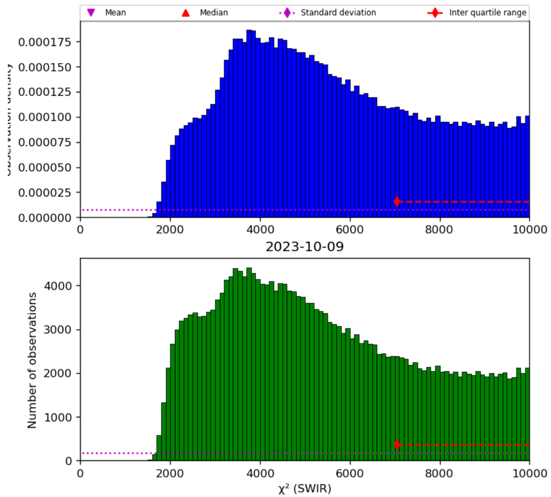
Figure 28: Histogram of “ \chi^2 (SWIR)” for 2023-10-08 to 2023-10-10
