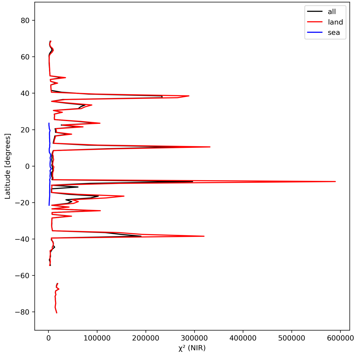
Figure 18: Zonal average of “ \chi^2 (NIR)” for 2023-10-08 to 2023-10-10.
