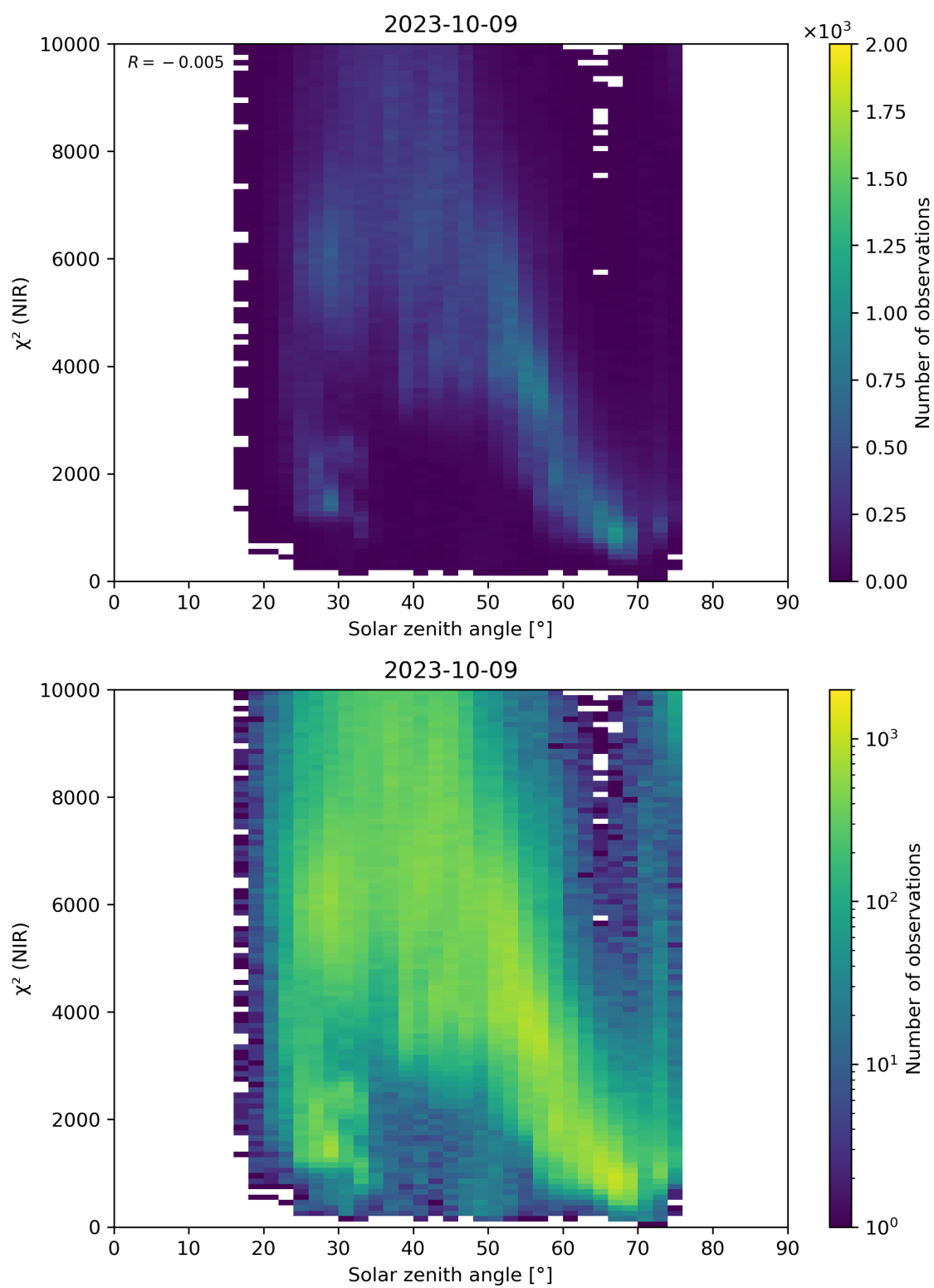
Figure 94: Scatter density plot of “Solar zenith angle” against “ \chi^2 (NIR)” for 2023-10-08 to 2023-10-10.
