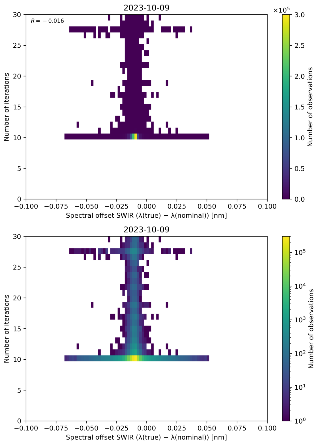
Figure 121: Scatter density plot of “Spectral offset SWIR ( \lambda(\text{true}) - \lambda(\text{nominal}) )” against “Number of iterations” for 2023-10-08 to 2023-10-10.
