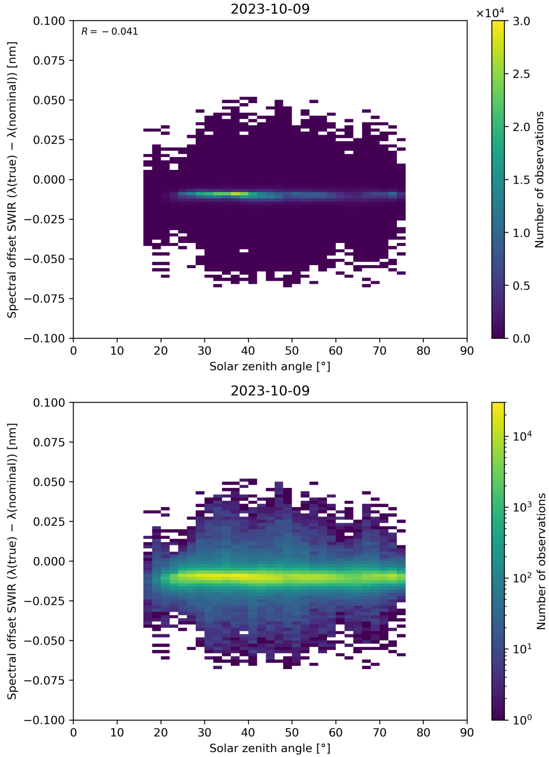
Figure 104: Scatter density plot of “Solar zenith angle” against “Spectral offset SWIR ( \lambda(\text{true}) - \lambda(\text{nominal}) )” for 2023-10-08 to 2023-10-10.
