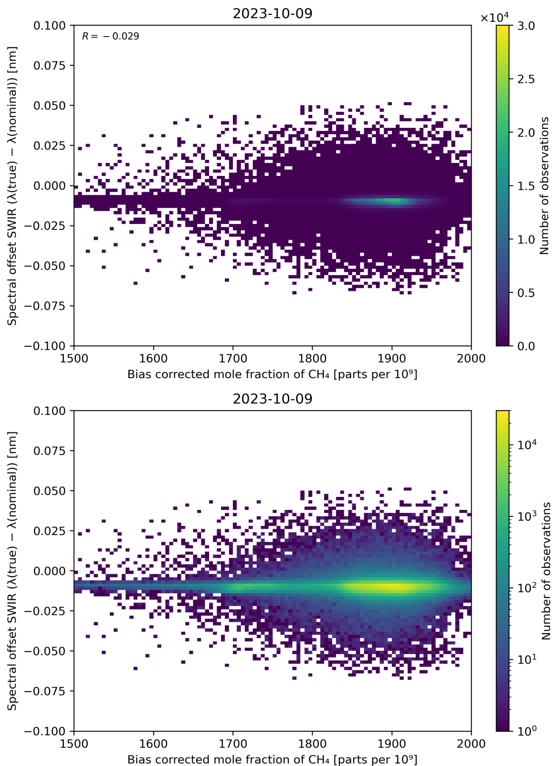
Figure 69: Scatter density plot of “Bias corrected mole fraction of \text{CH}_4 ” against “Spectral offset SWIR ( \lambda(\text{true}) - \lambda(\text{nominal}) )” for 2023-10-08 to 2023-10-10.
