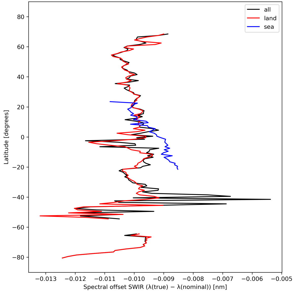
Figure 16: Zonal average of “Spectral offset SWIR ( \lambda(\text{true}) - \lambda(\text{nominal}) )” for 2023-10-08 to 2023-10-10.
