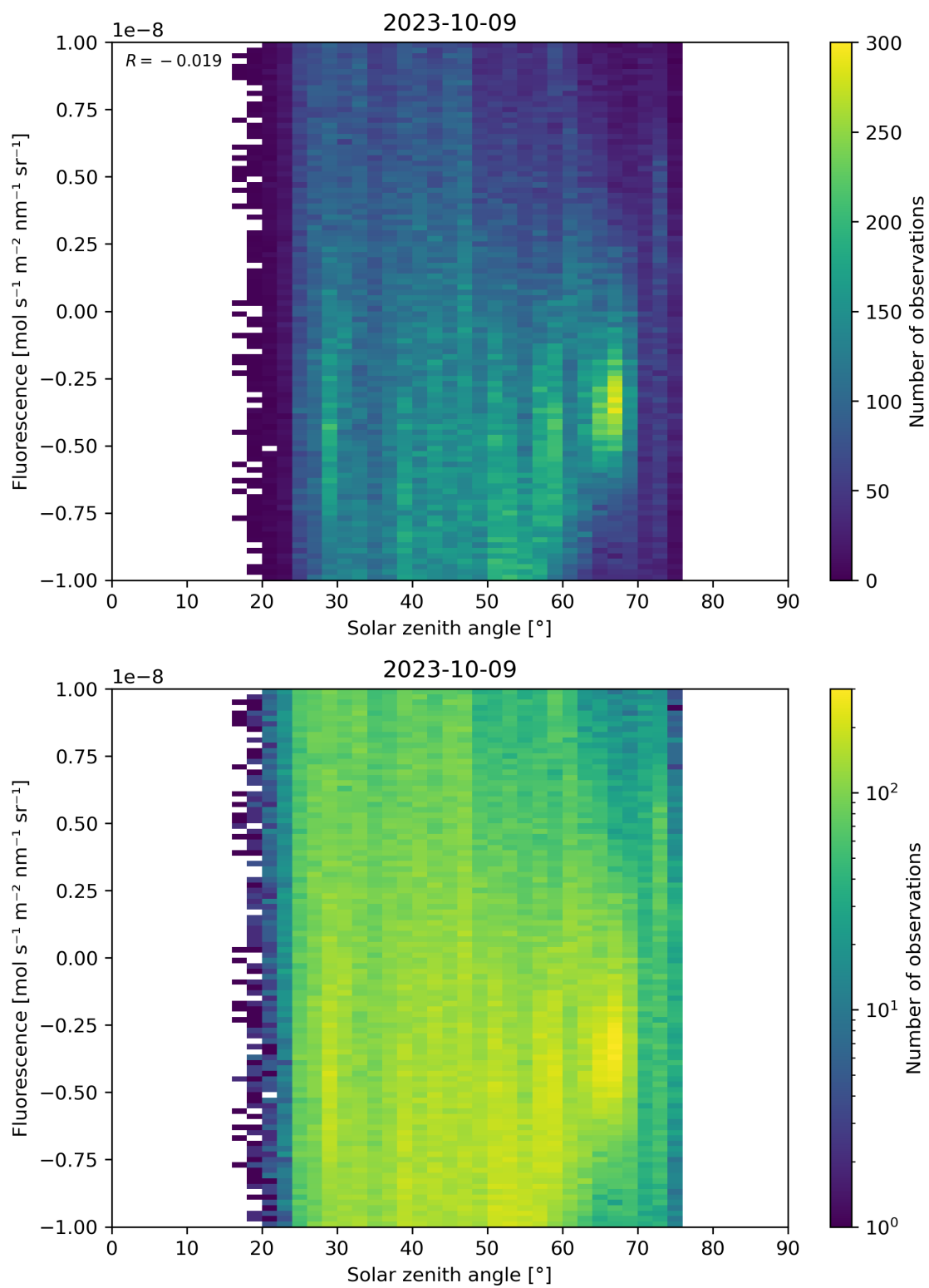
Figure 97: Scatter density plot of “Solar zenith angle” against “Fluorescence” for 2023-10-08 to 2023-10-10.
