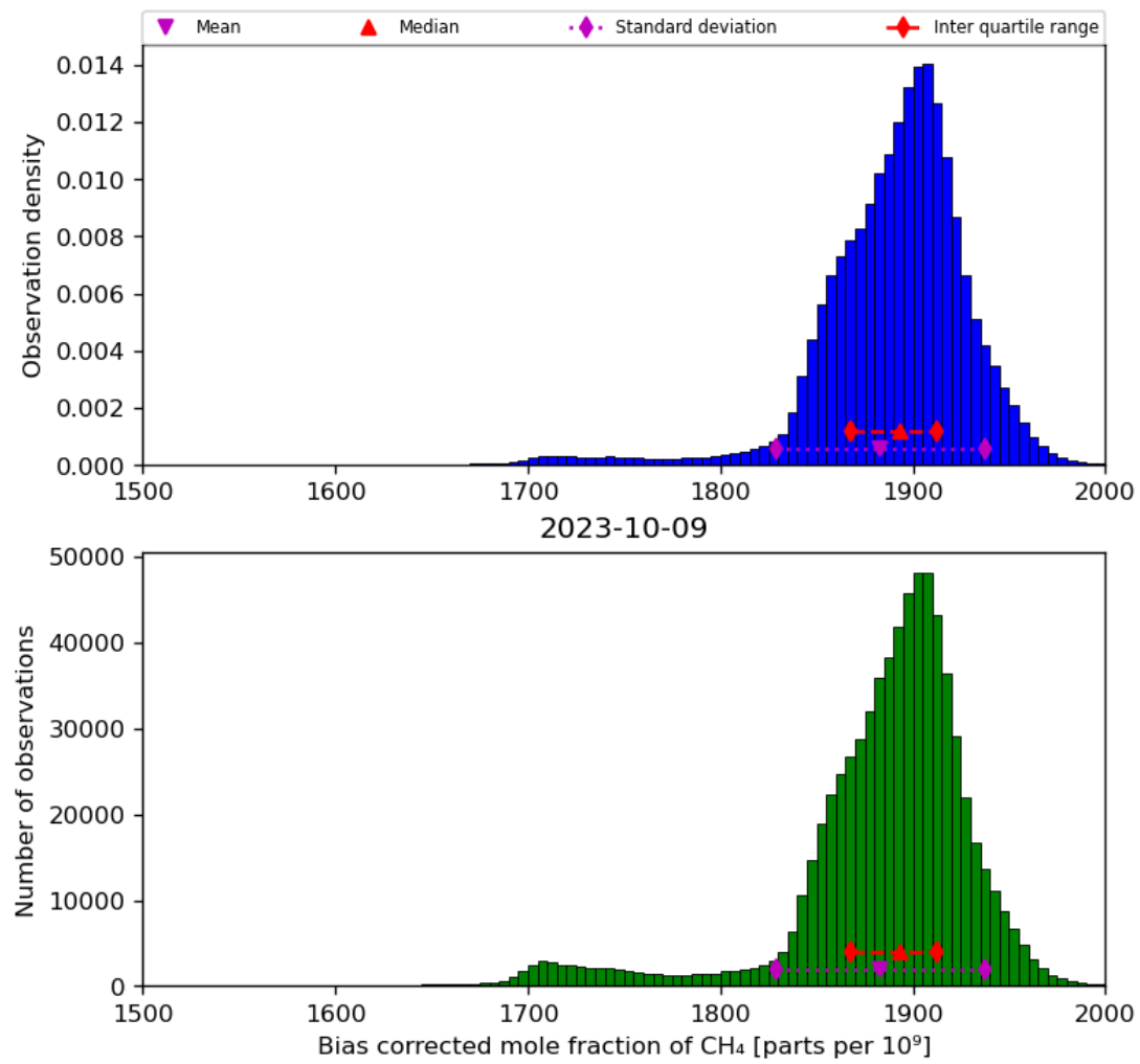
Figure 25: Histogram of “Bias corrected mole fraction of CH 4 ” for 2023-10-08 to 2023-10-10
