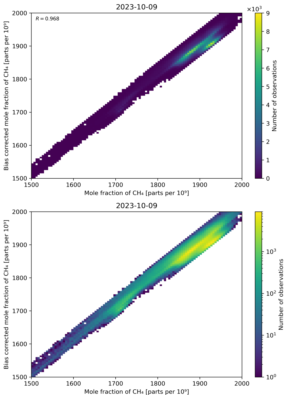
Figure 74: Scatter density plot of “Mole fraction of CH 4 ” against “Bias corrected mole fraction of CH 4 ” for 2023-10-08 to 2023-10-10.
