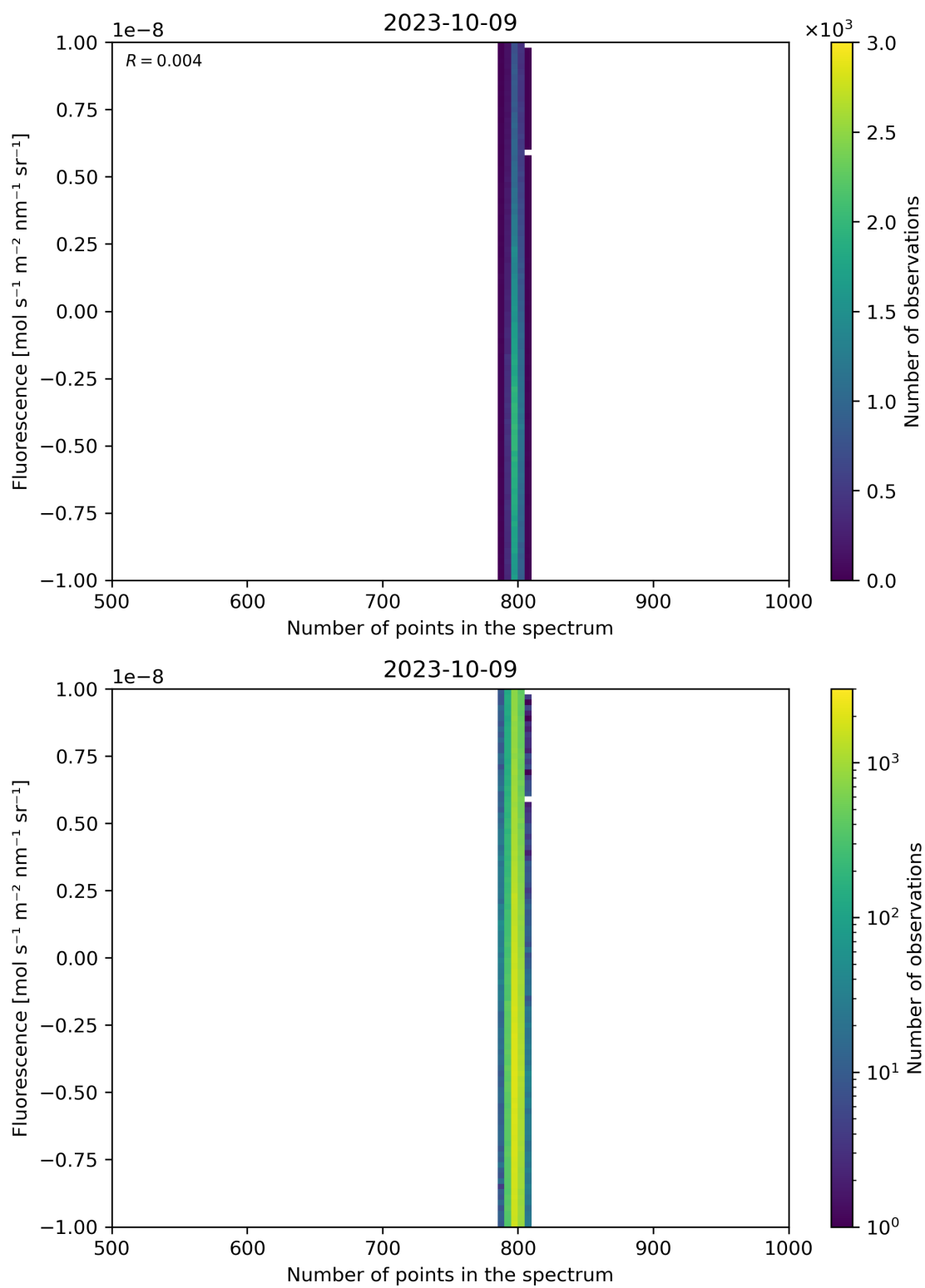
Figure 91: Scatter density plot of “Number of points in the spectrum” against “Fluorescence” for 2023-10-08 to 2023-10-10.
