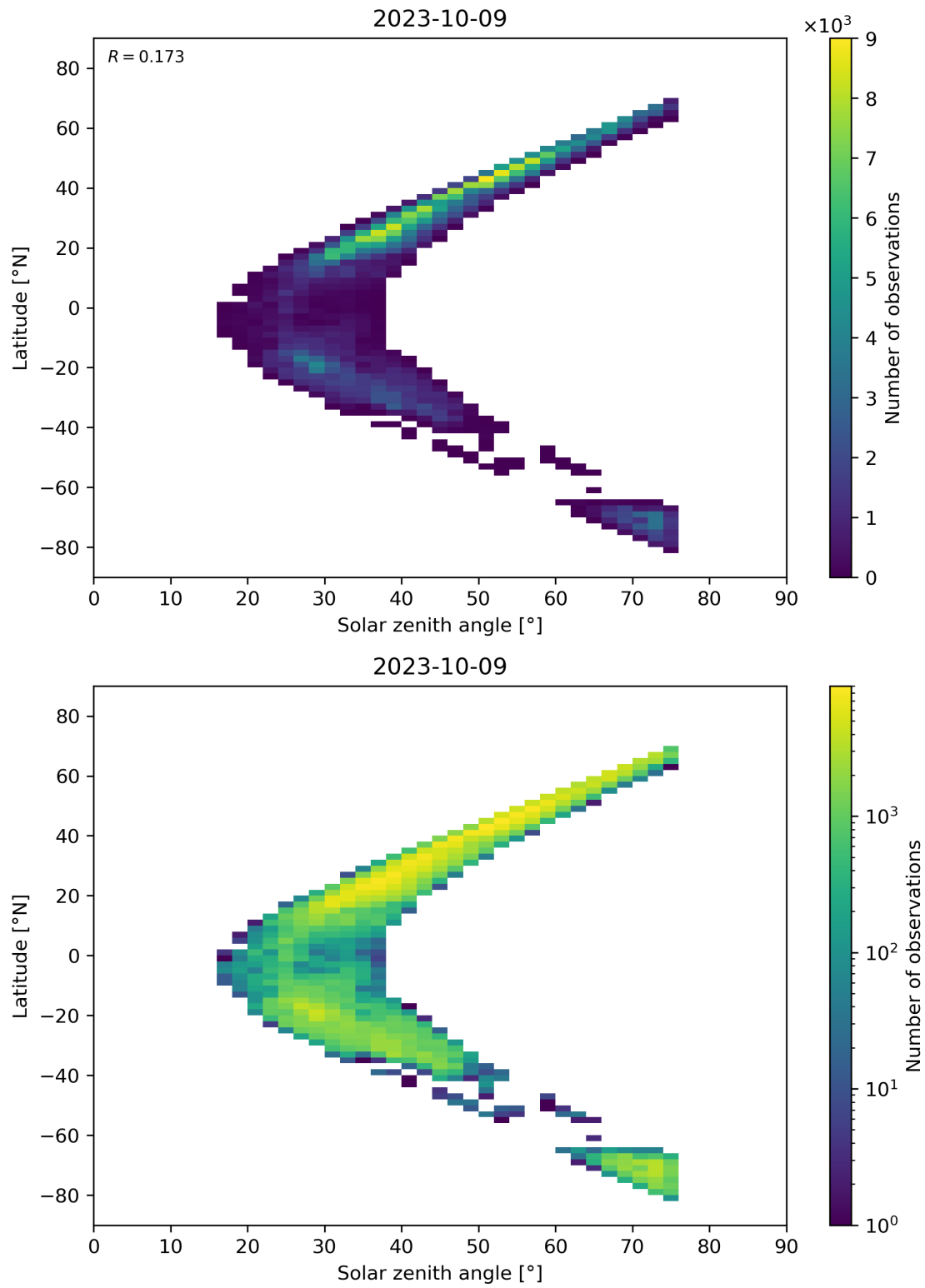
Figure 98: Scatter density plot of “Solar zenith angle” against “Latitude” for 2023-10-08 to 2023-10-10.
