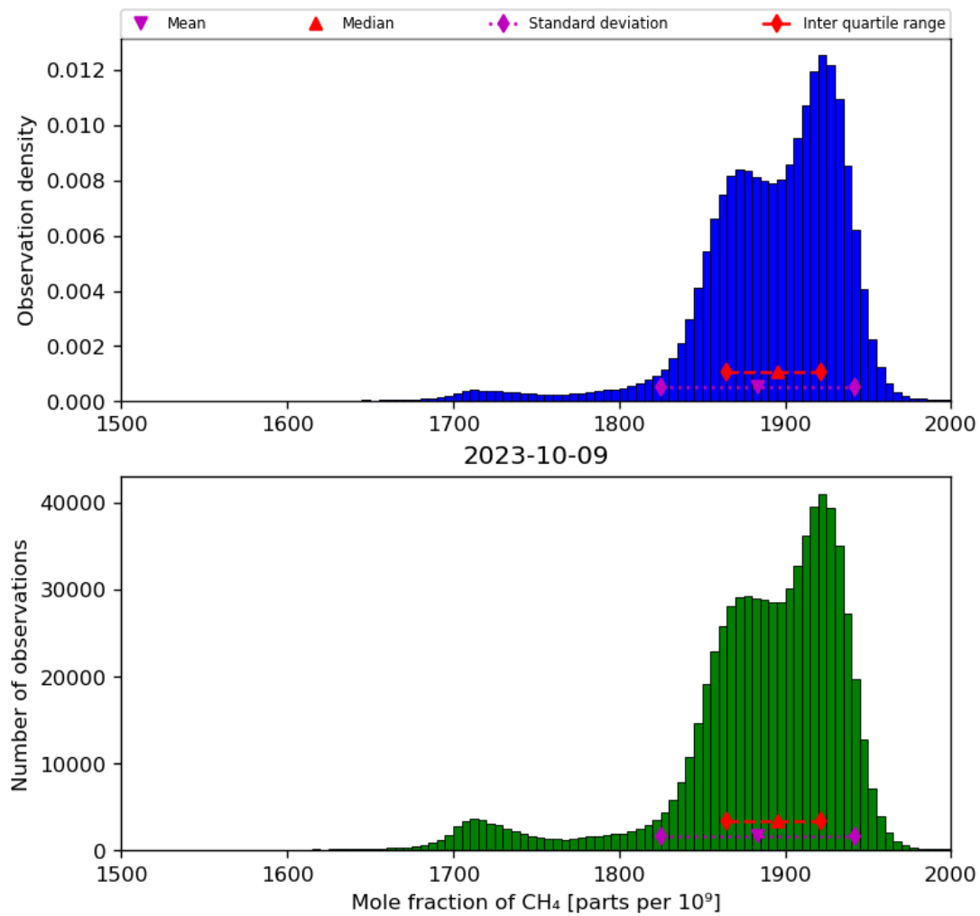
Figure 23: Histogram of “Mole fraction of CH 4 ” for 2023-10-08 to 2023-10-10
