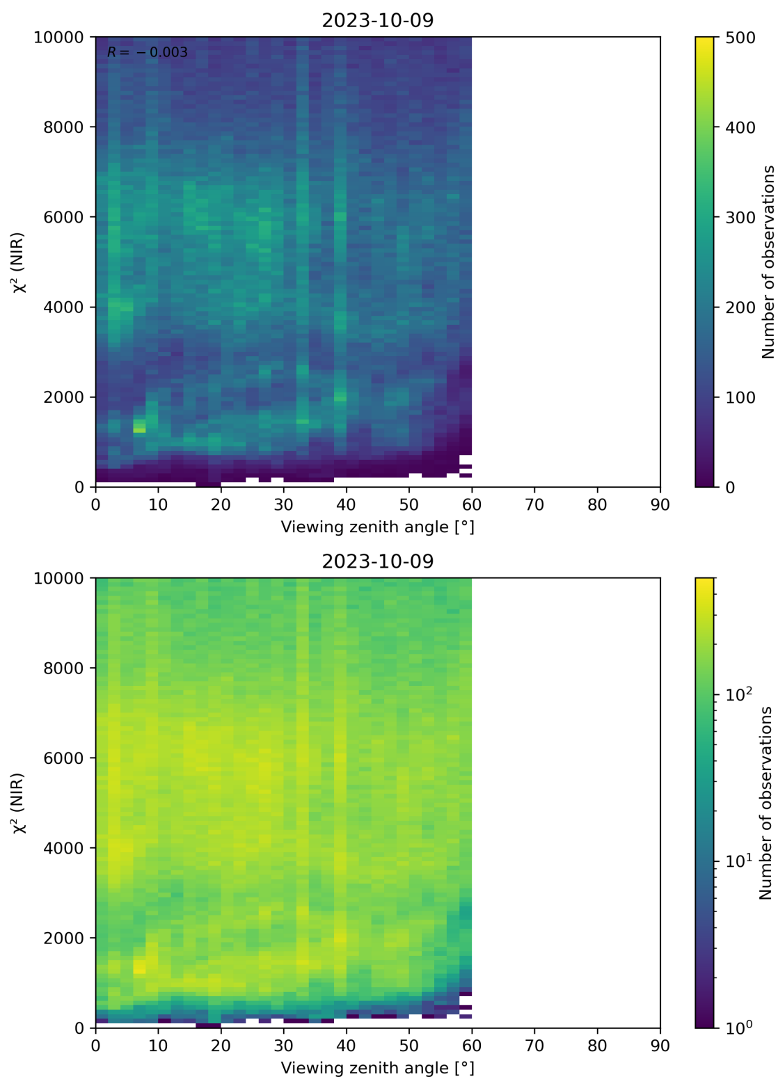
Figure 105: Scatter density plot of “Viewing zenith angle” against “ \chi^2 (NIR)” for 2023-10-08 to 2023-10-10.
