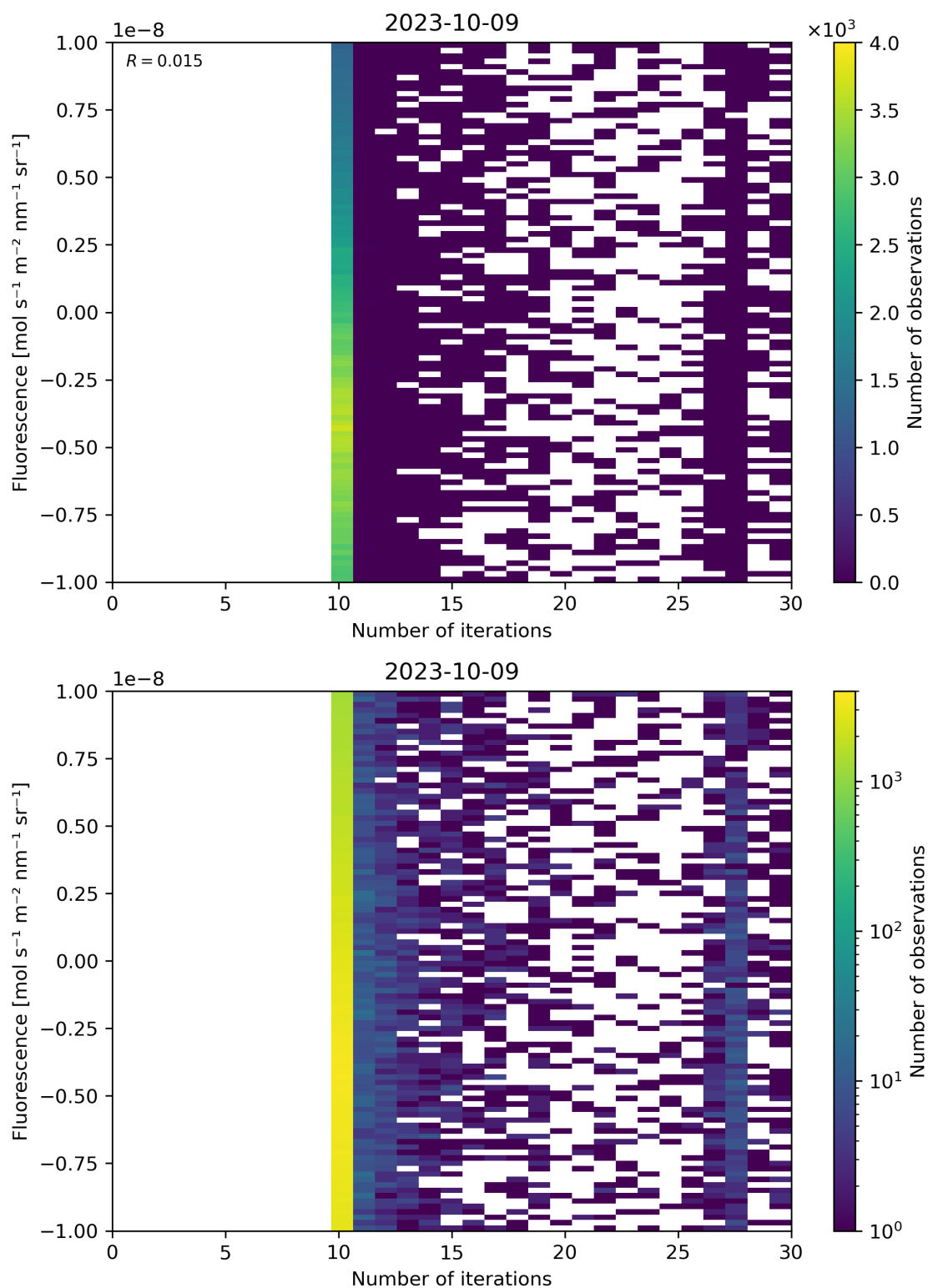
Figure 87: Scatter density plot of “Number of iterations” against “Fluorescence” for 2023-10-08 to 2023-10-10.
