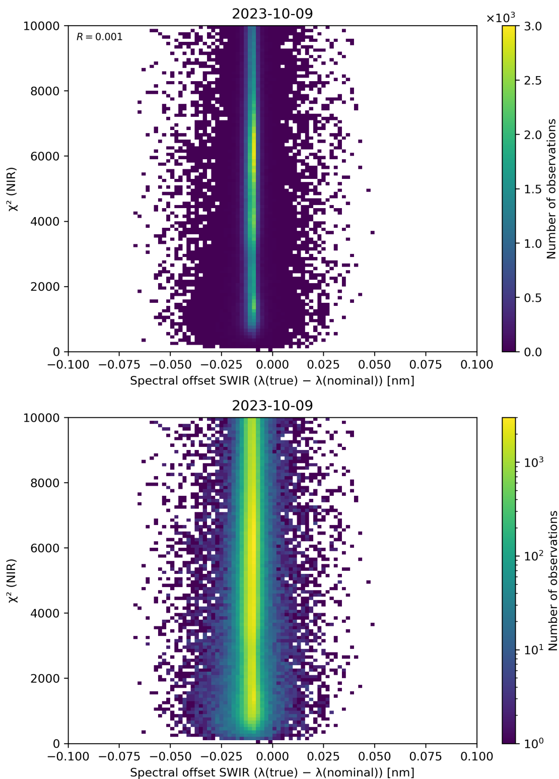
Figure 117: Scatter density plot of “Spectral offset SWIR ( \lambda(\text{true}) - \lambda(\text{nominal}) )” against “ \chi^2 (NIR)” for 2023-10-08 to 2023-10-10.
