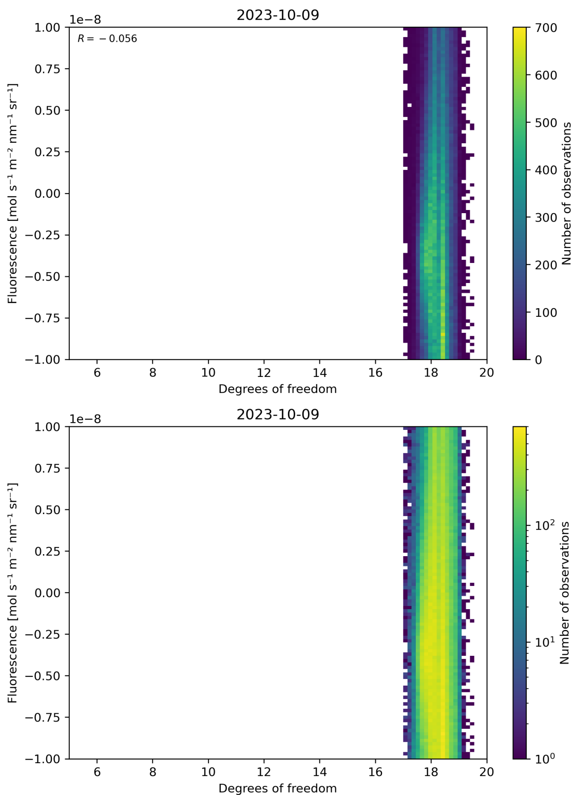
Figure 51: Scatter density plot of “Degrees of freedom” against “Fluorescence” for 2023-10-08 to 2023-10-10.
