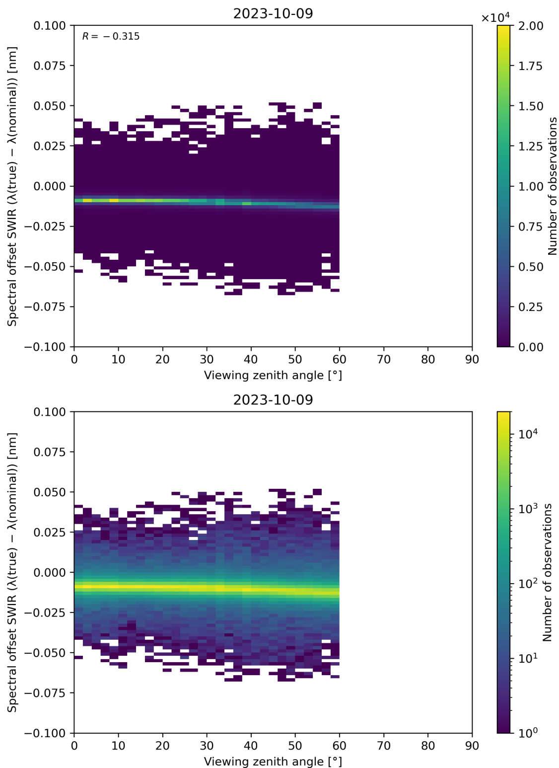
Figure 116: Scatter density plot of “Viewing zenith angle” against “Spectral offset SWIR ( \lambda(\text{true}) - \lambda(\text{nominal}) )” for 2023-10-08 to 2023-10-10.
