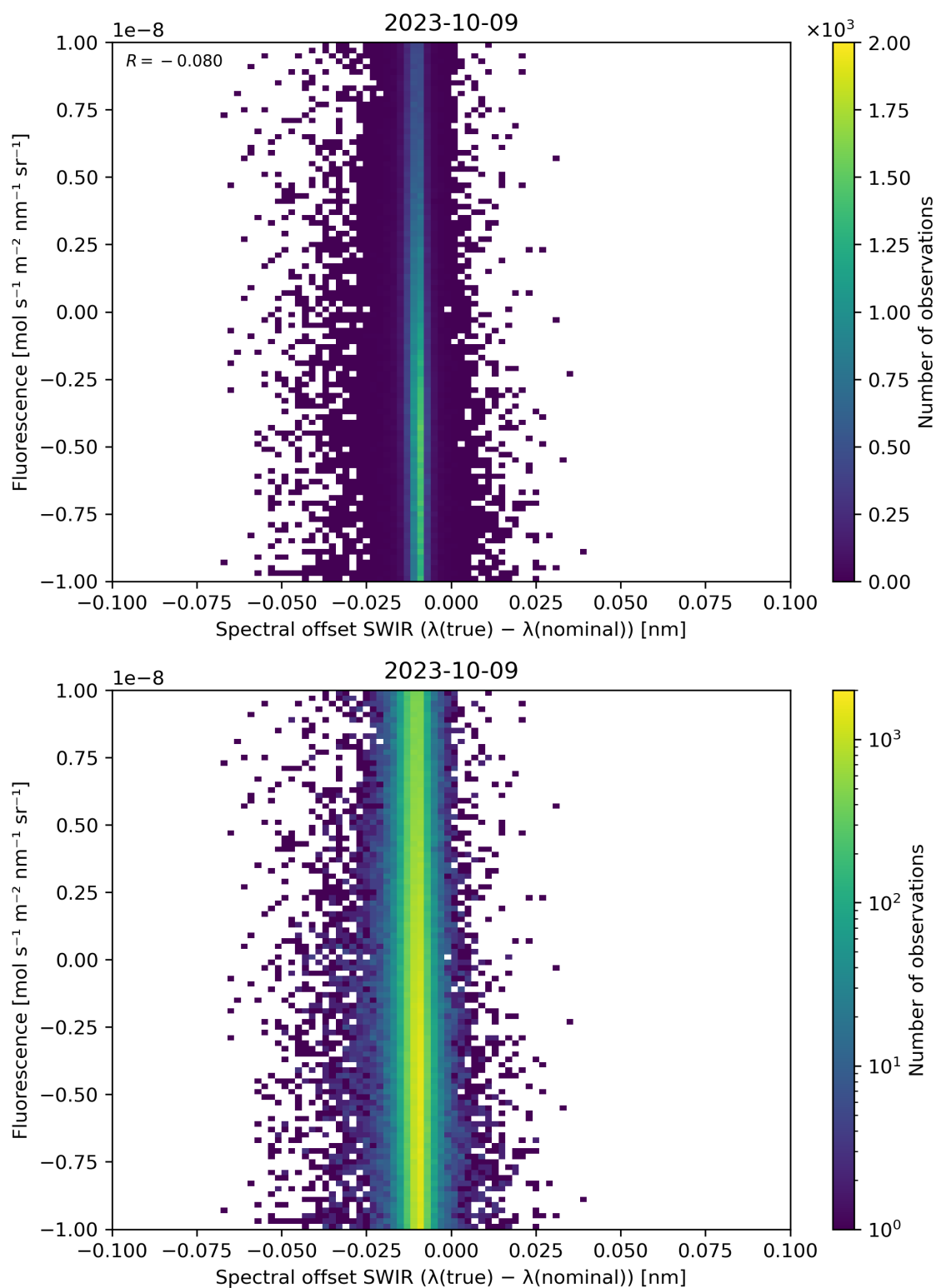
Figure 120: Scatter density plot of “Spectral offset SWIR ( \lambda(\text{true}) - \lambda(\text{nominal}) )” against “Fluorescence” for 2023-10-08 to 2023-10-10.
