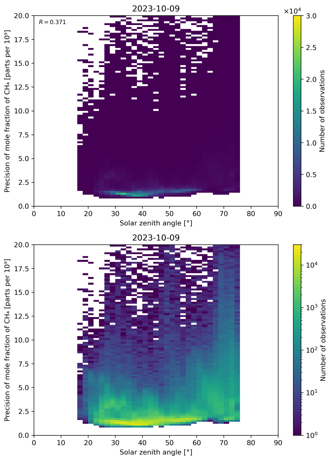
Figure 101: Scatter density plot of “Solar zenith angle” against “Precision of mole fraction of CH 4 ” for 2023-10-08 to 2023-10-10.
