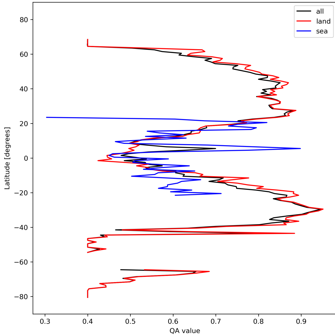
Figure 11: Zonal average of “QA value” for 2023-10-08 to 2023-10-10.
