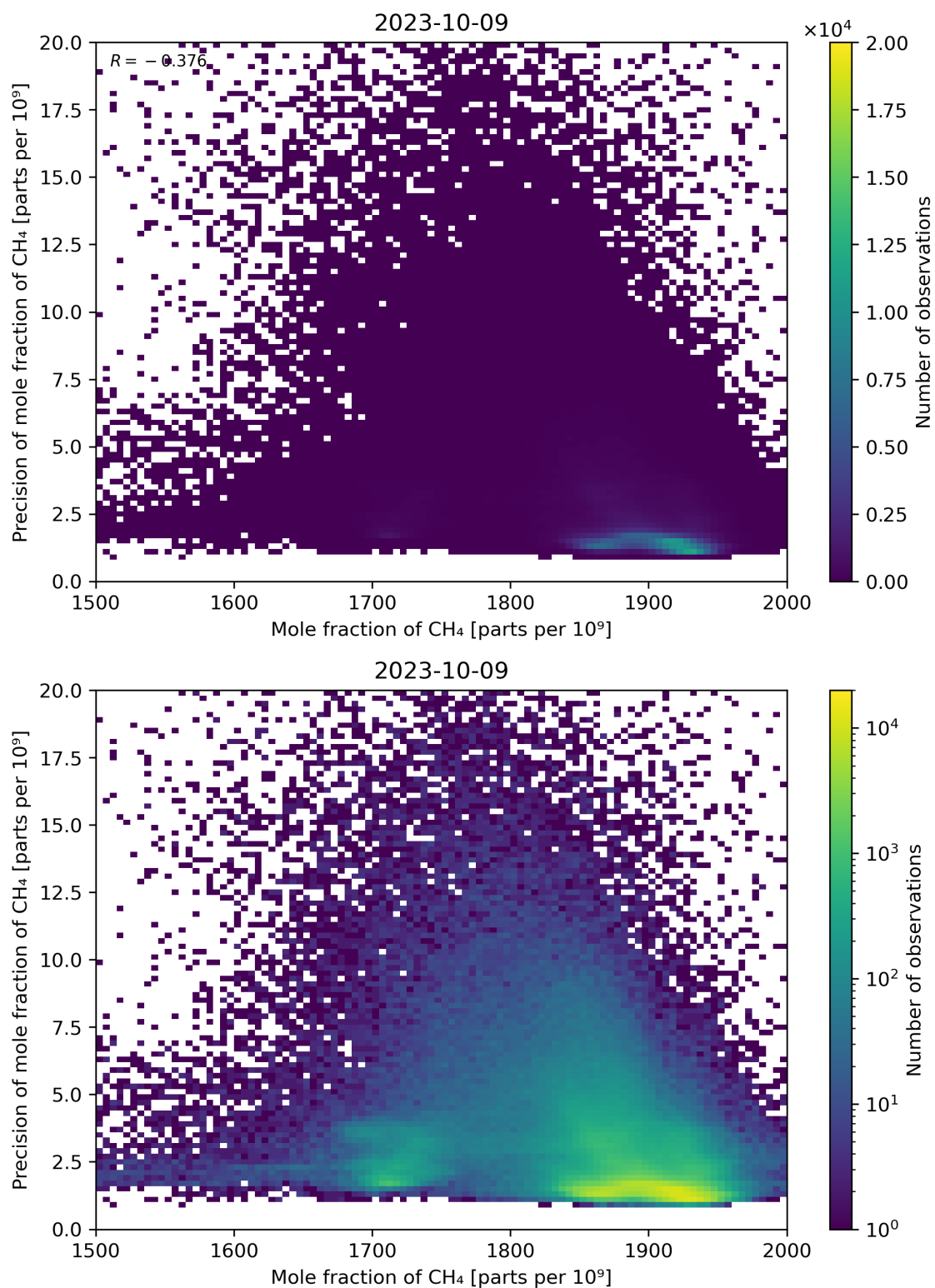
Figure 75: Scatter density plot of “Mole fraction of CH 4 ” against “Precision of mole fraction of CH 4 ” for 2023-10-08 to 2023-10-10.
