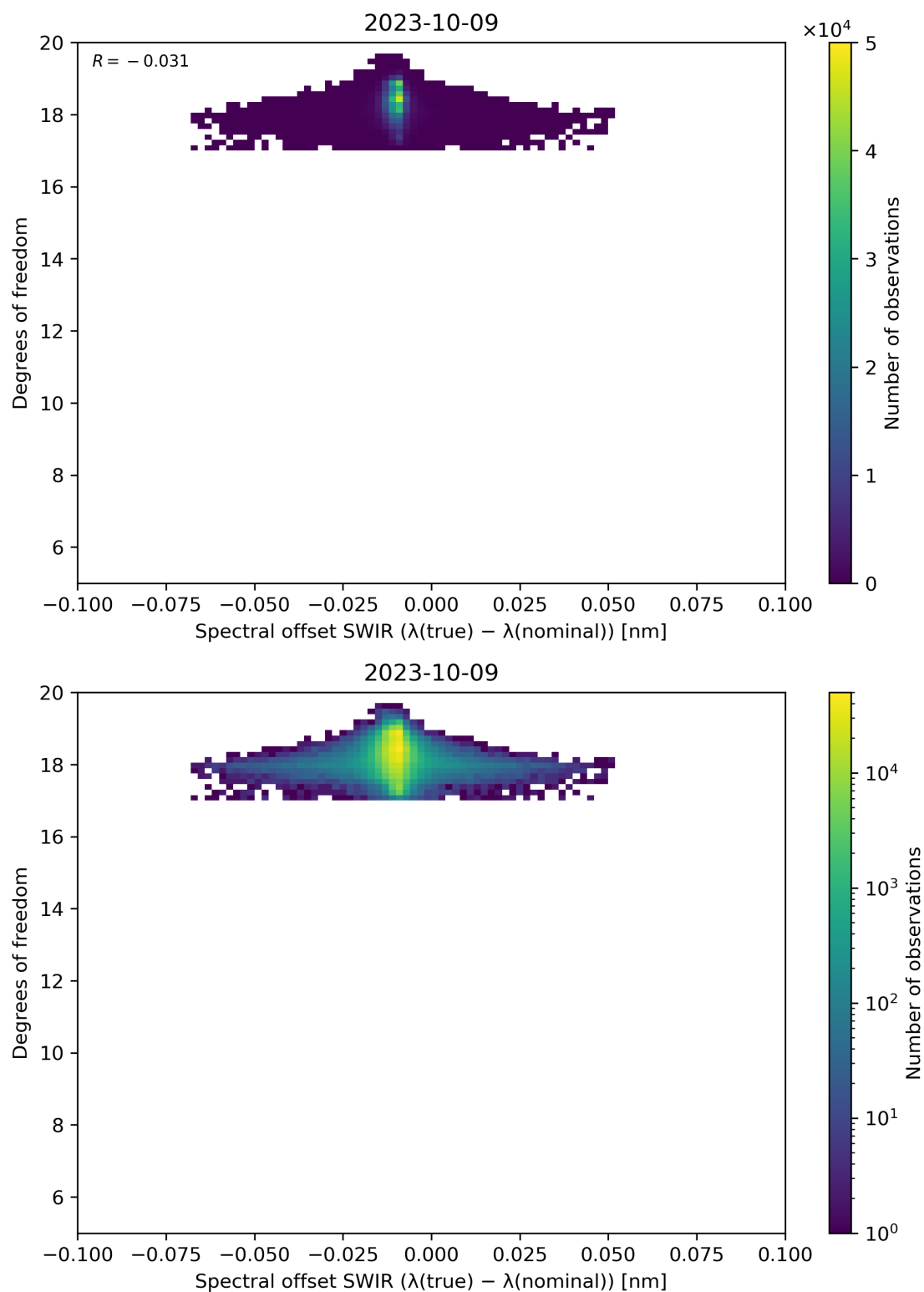
Figure 119: Scatter density plot of “Spectral offset SWIR ( \lambda(\text{true}) - \lambda(\text{nominal}) )” against “Degrees of freedom” for 2023-10-08 to 2023-10-10.
