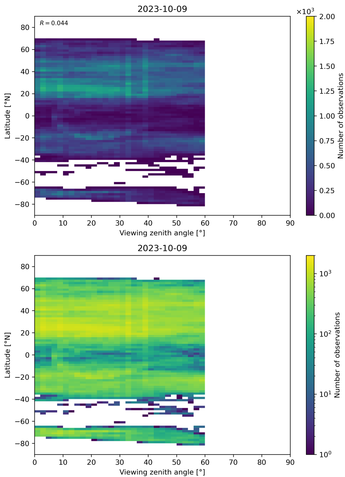
Figure 109: Scatter density plot of “Viewing zenith angle” against “Latitude” for 2023-10-08 to 2023-10-10.
