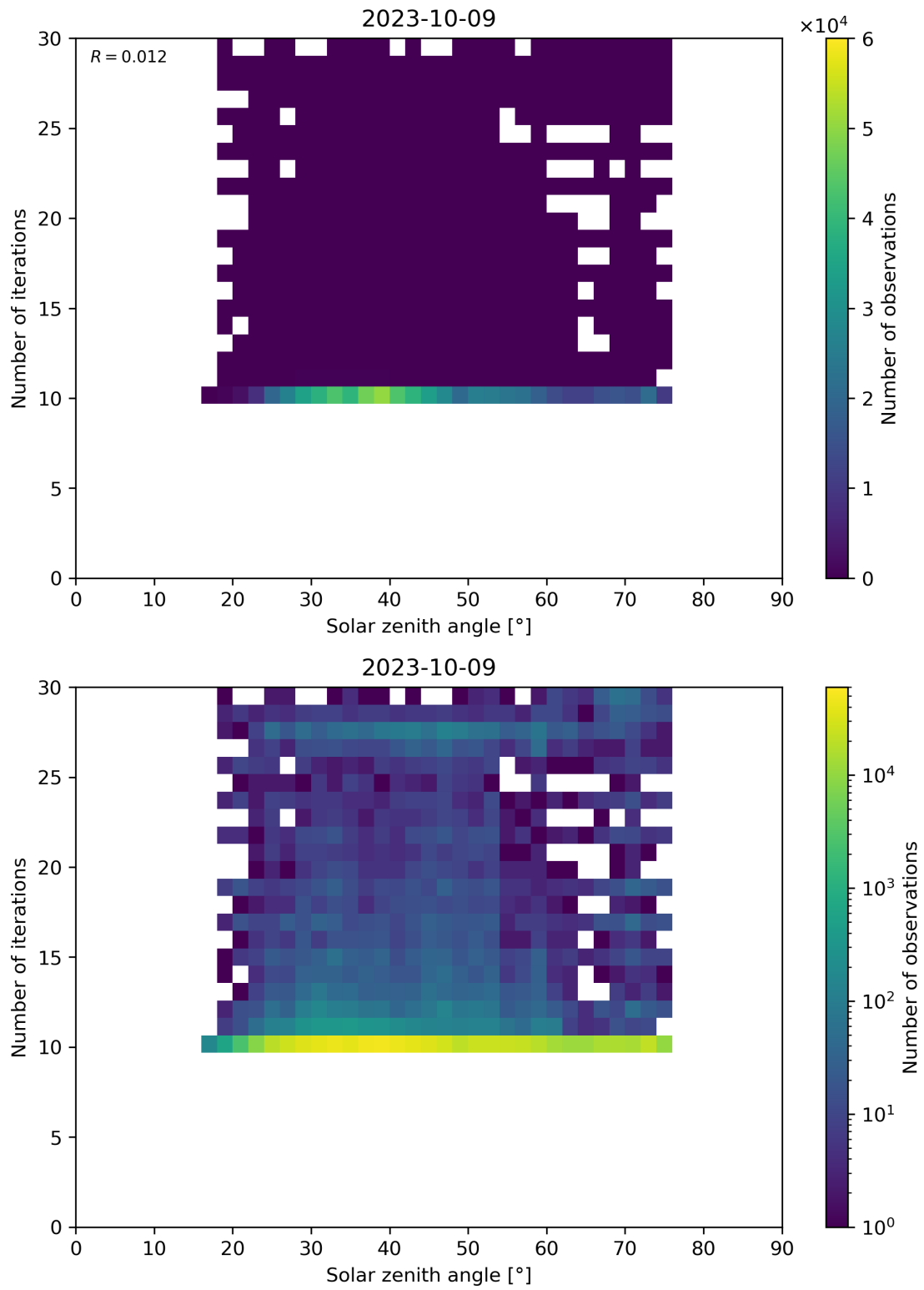
Figure 102: Scatter density plot of “Solar zenith angle” against “Number of iterations” for 2023-10-08 to 2023-10-10.
