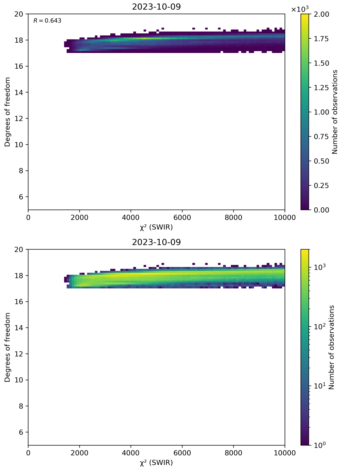
Figure 48: Scatter density plot of “ \chi^2 (SWIR)” against “Degrees of freedom” for 2023-10-08 to 2023-10-10.
