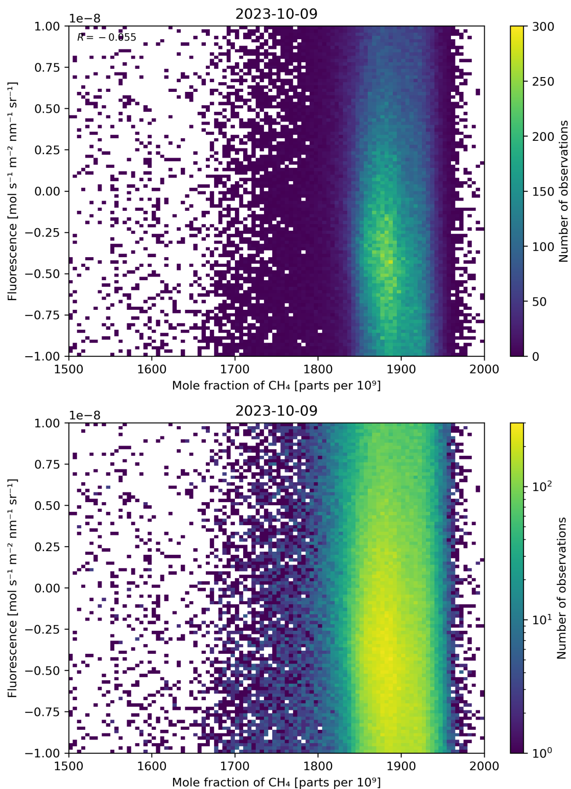
Figure 73: Scatter density plot of “Mole fraction of \text{CH}_4 ” against “Fluorescence” for 2023-10-08 to 2023-10-10.
