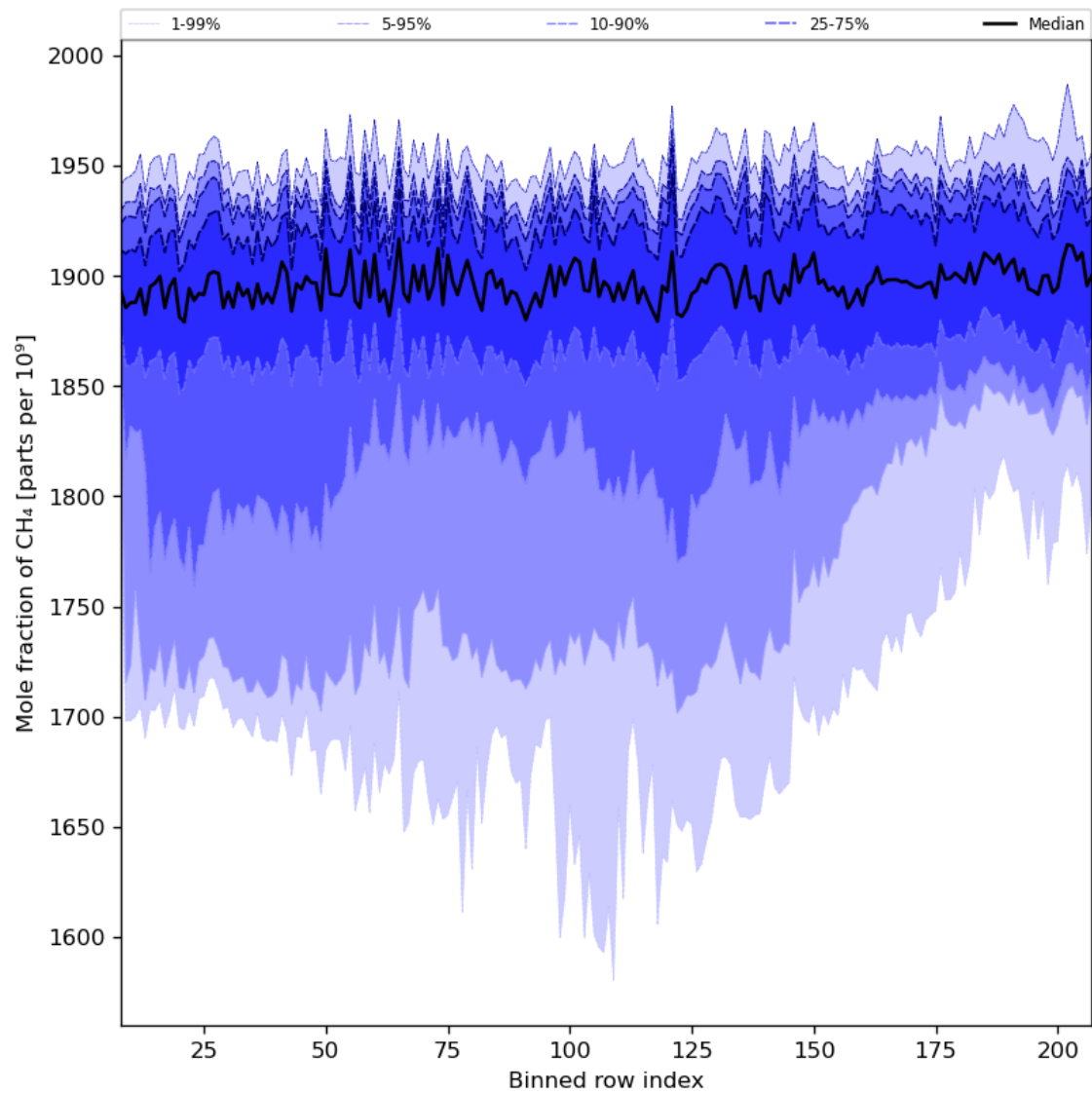
Figure 34: Along track statistics of “Mole fraction of CH 4 ” for 2023-10-08 to 2023-10-10
