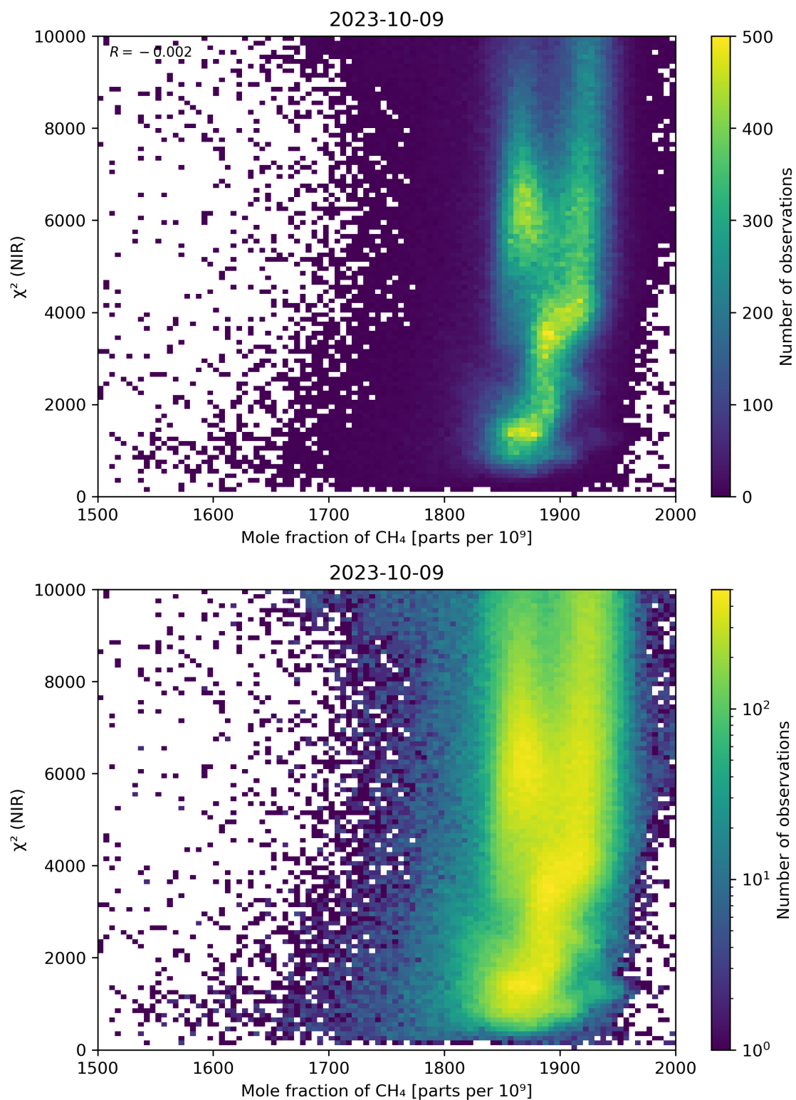
Figure 70: Scatter density plot of “Mole fraction of CH 4 ” against “ \chi^2 (NIR)” for 2023-10-08 to 2023-10-10.
