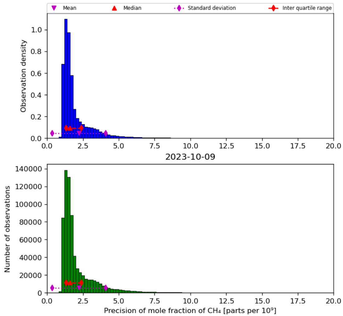
Figure 24: Histogram of “Precision of mole fraction of CH 4 ” for 2023-10-08 to 2023-10-10
