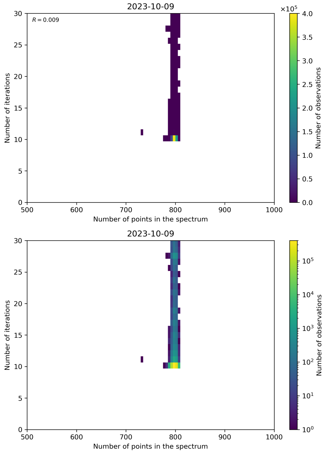
Figure 92: Scatter density plot of “Number of points in the spectrum” against “Number of iterations” for 2023-10-08 to 2023-10-10.
