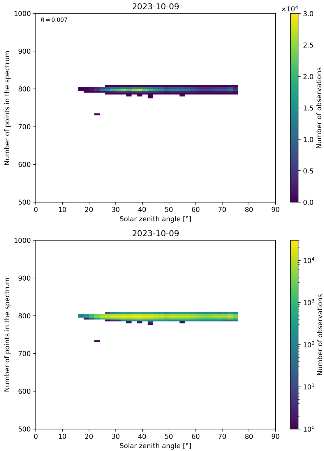
Figure 103: Scatter density plot of “Solar zenith angle” against “Number of points in the spectrum” for 2023-10-08 to 2023-10-10.
