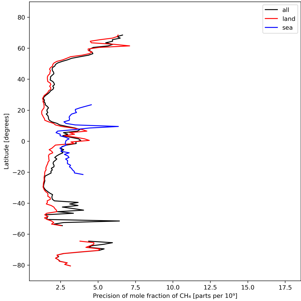
Figure 13: Zonal average of “Precision of mole fraction of CH 4 ” for 2023-10-08 to 2023-10-10.
