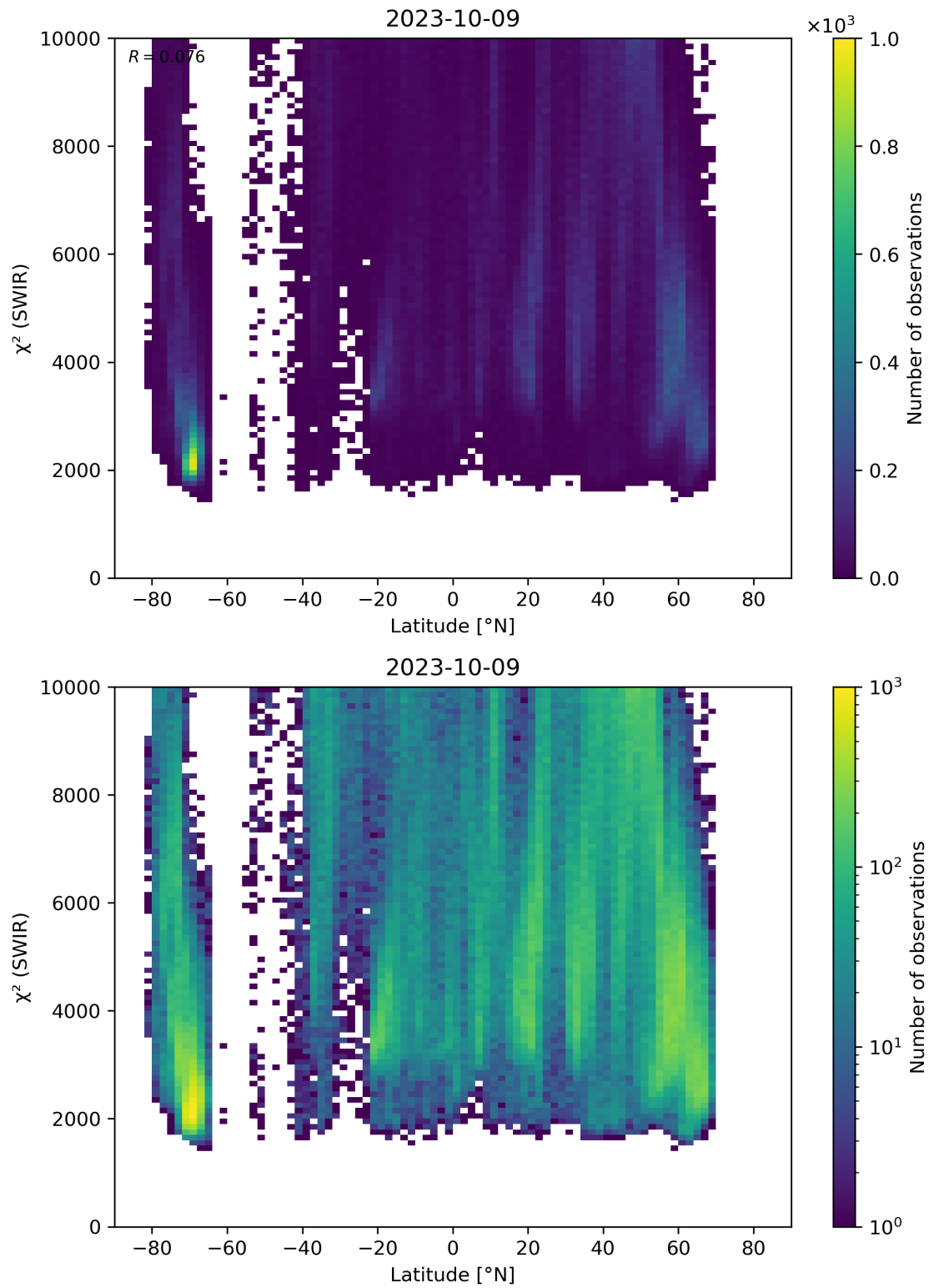
Figure 54: Scatter density plot of “Latitude” against “ \chi^2 (SWIR)” for 2023-10-08 to 2023-10-10.
