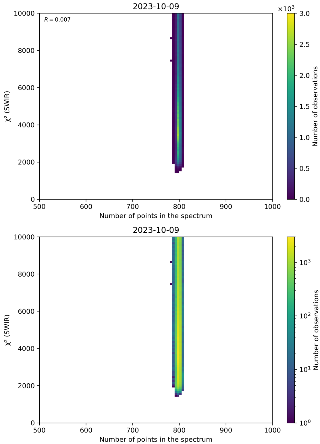
Figure 89: Scatter density plot of “Number of points in the spectrum” against “ \chi^2 (SWIR)” for 2023-10-08 to 2023-10-10.
