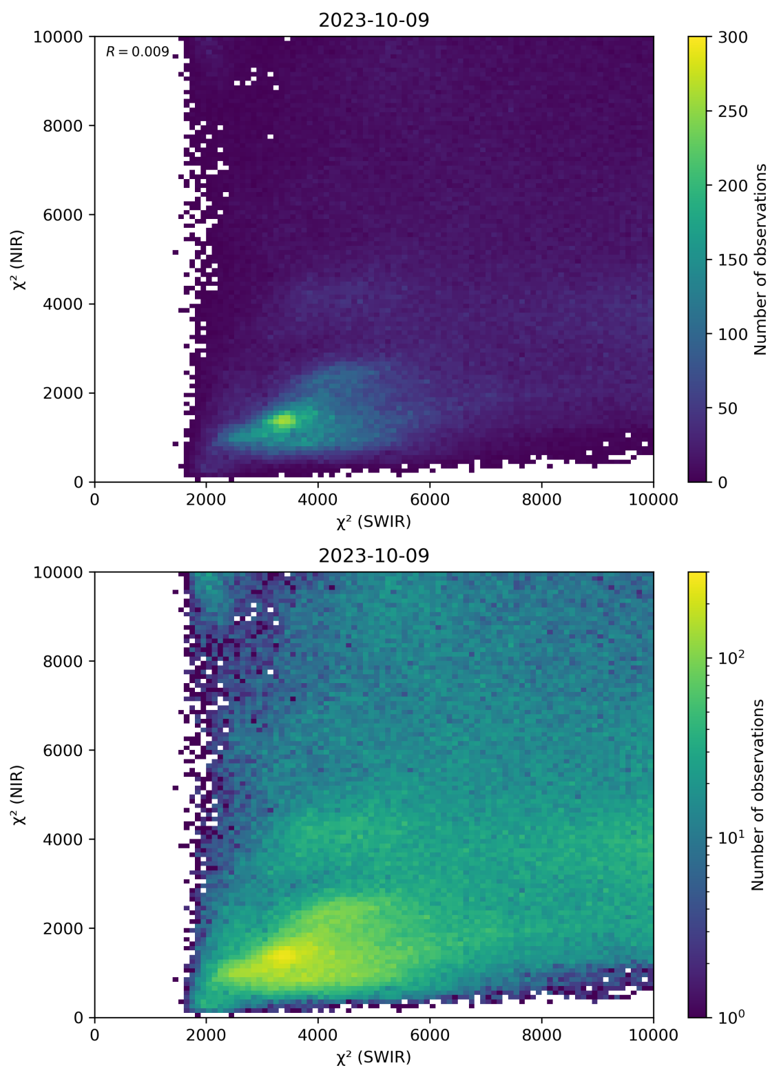
Figure 47: Scatter density plot of “ \chi^2 (SWIR)” against “ \chi^2 (NIR)” for 2023-10-08 to 2023-10-10.
