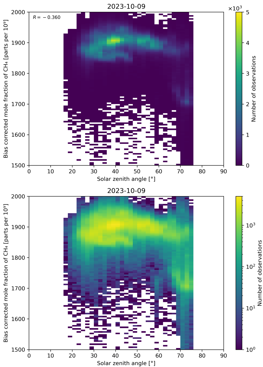
Figure 100: Scatter density plot of “Solar zenith angle” against “Bias corrected mole fraction of CH 4 ” for 2023-10-08 to 2023-10-10.
