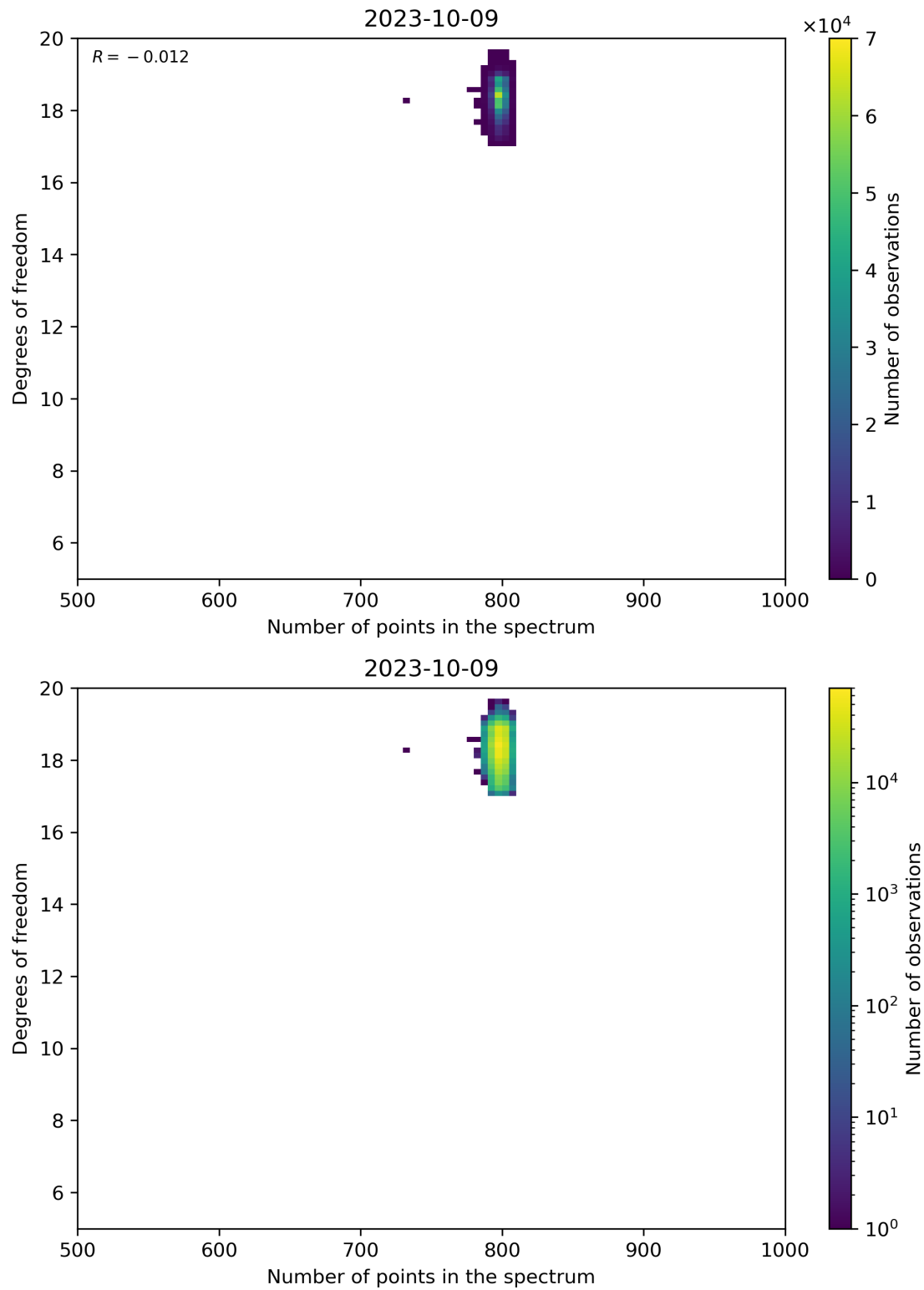
Figure 90: Scatter density plot of “Number of points in the spectrum” against “Degrees of freedom” for 2023-10-08 to 2023-10-10.
