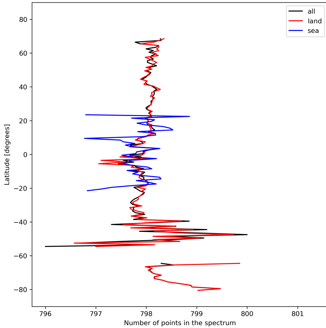
Figure 15: Zonal average of “Number of points in the spectrum” for 2023-10-08 to 2023-10-10.
