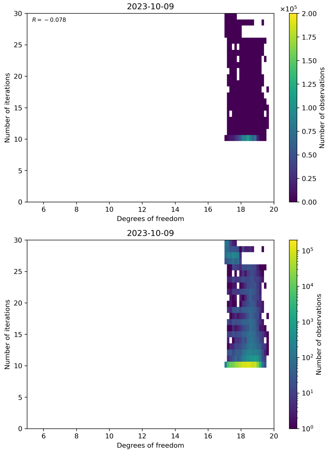
Figure 52: Scatter density plot of “Degrees of freedom” against “Number of iterations” for 2023-10-08 to 2023-10-10.
