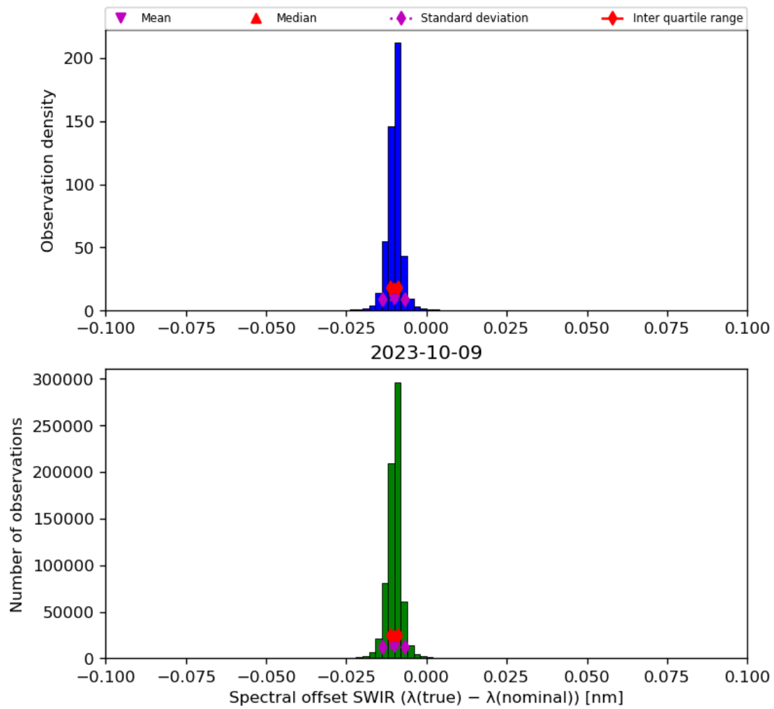
Figure 27: Histogram of “Spectral offset SWIR ( \lambda(\text{true}) - \lambda(\text{nominal}) )” for 2023-10-08 to 2023-10-10
