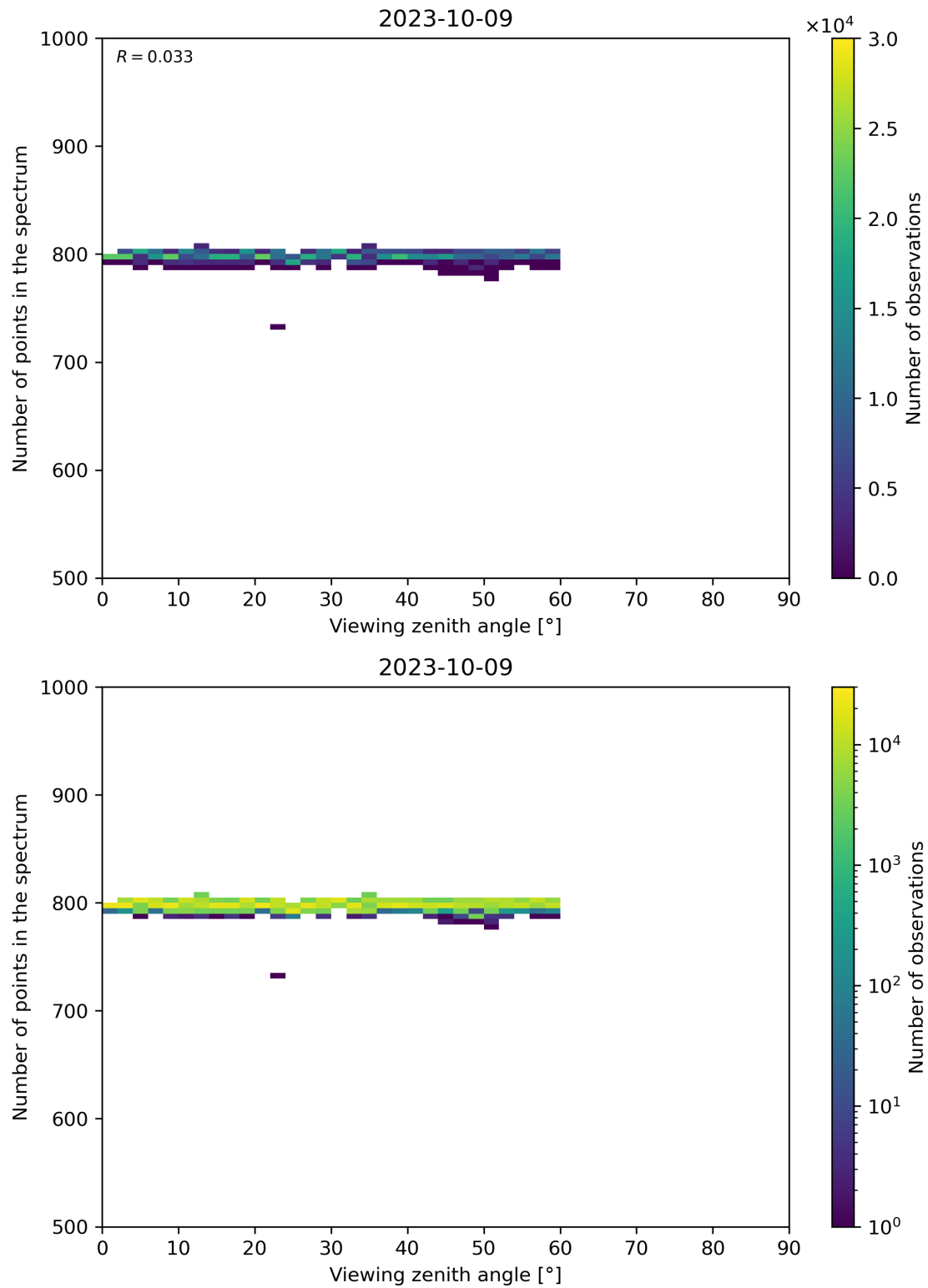
Figure 114: Scatter density plot of “Viewing zenith angle” against “Number of points in the spectrum” for 2023-10-08 to 2023-10-10.
