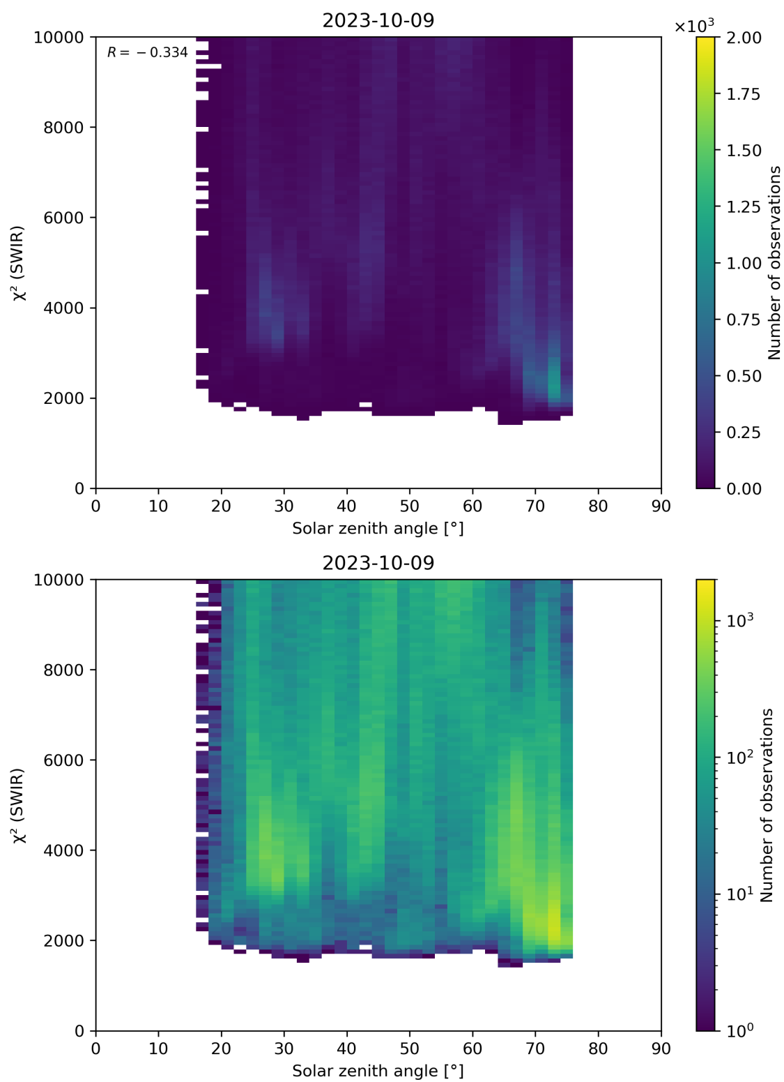
Figure 95: Scatter density plot of “Solar zenith angle” against “ \chi^2 (SWIR)” for 2023-10-08 to 2023-10-10.
