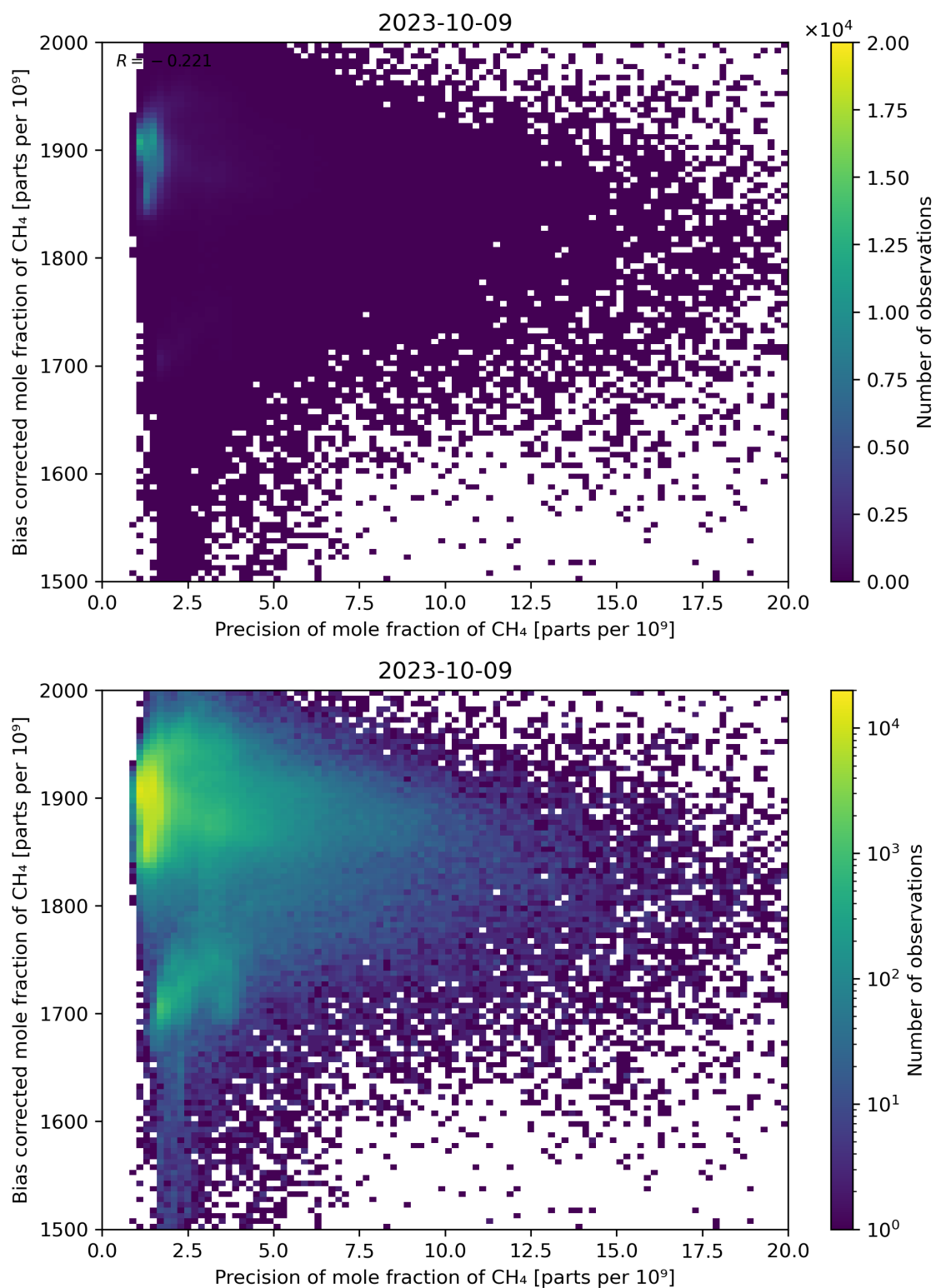
Figure 82: Scatter density plot of “Precision of mole fraction of CH 4 ” against “Bias corrected mole fraction of CH 4 ” for 2023-10-08 to 2023-10-10.
