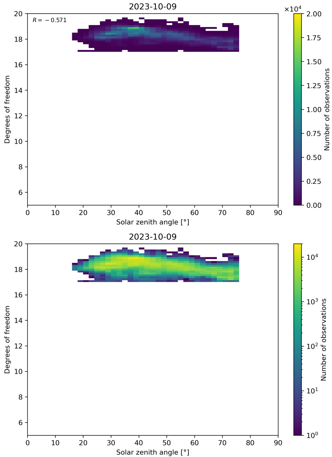
Figure 96: Scatter density plot of “Solar zenith angle” against “Degrees of freedom” for 2023-10-08 to 2023-10-10.
