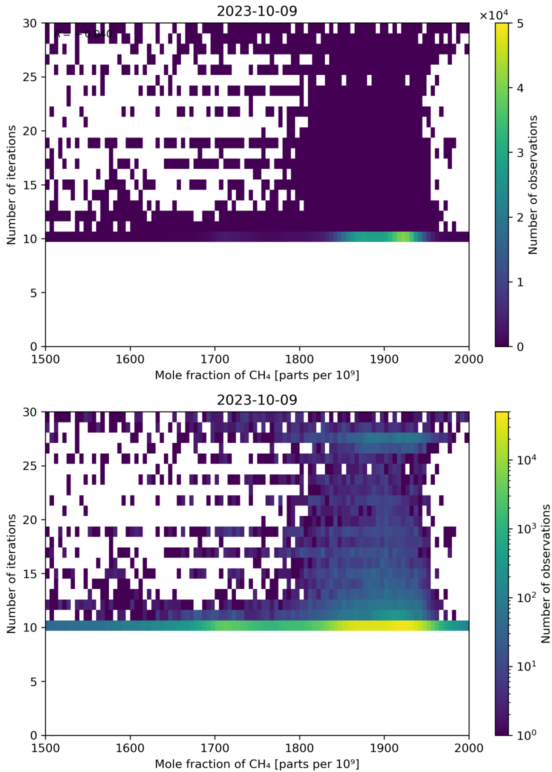
Figure 76: Scatter density plot of “Mole fraction of CH 4 ” against “Number of iterations” for 2023-10-08 to 2023-10-10.
