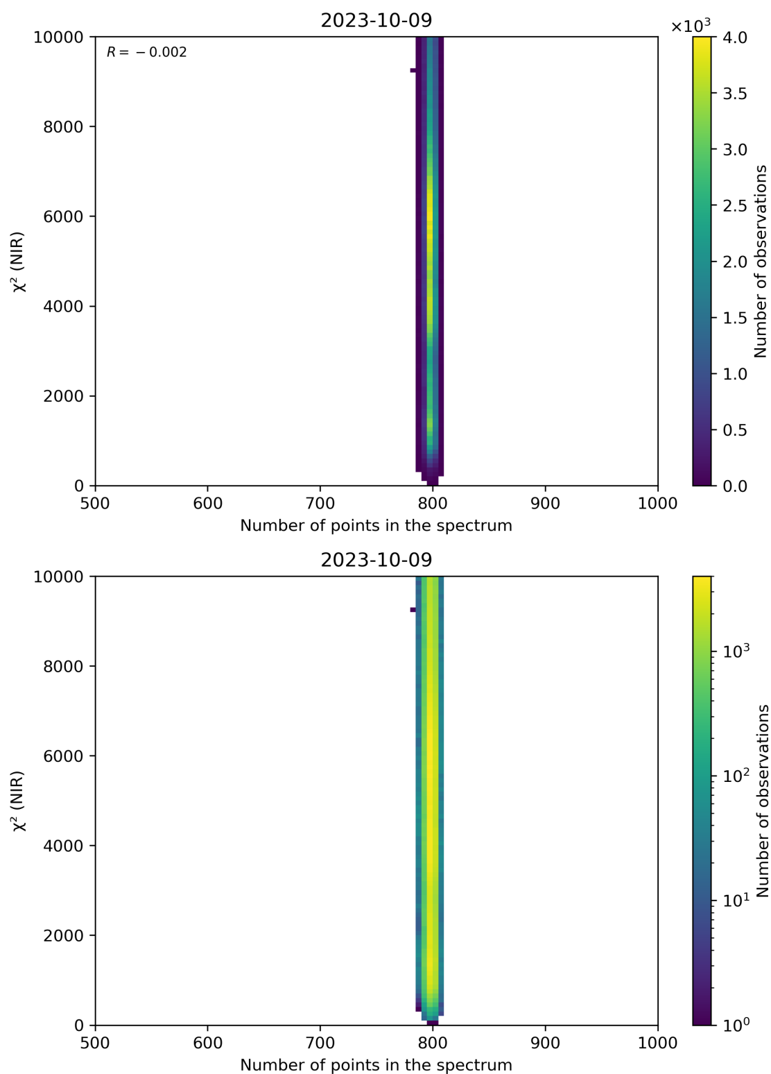
Figure 88: Scatter density plot of “Number of points in the spectrum” against “ \chi^2 (NIR)” for 2023-10-08 to 2023-10-10.
