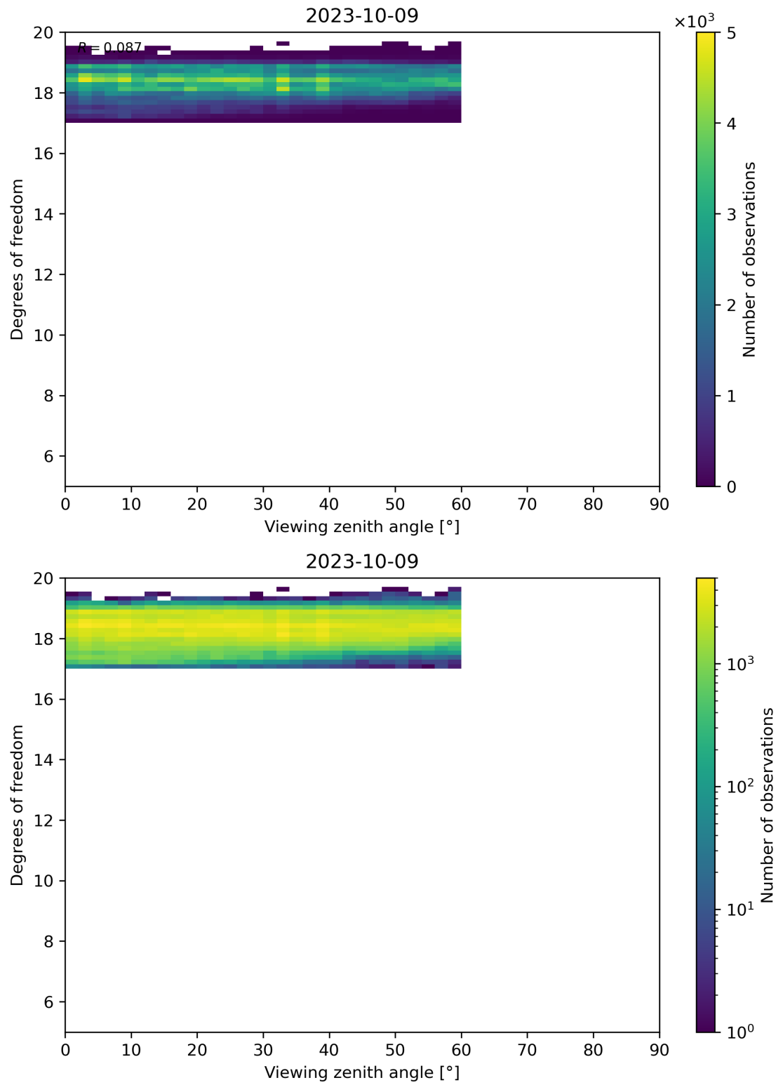
Figure 107: Scatter density plot of “Viewing zenith angle” against “Degrees of freedom” for 2023-10-08 to 2023-10-10.
