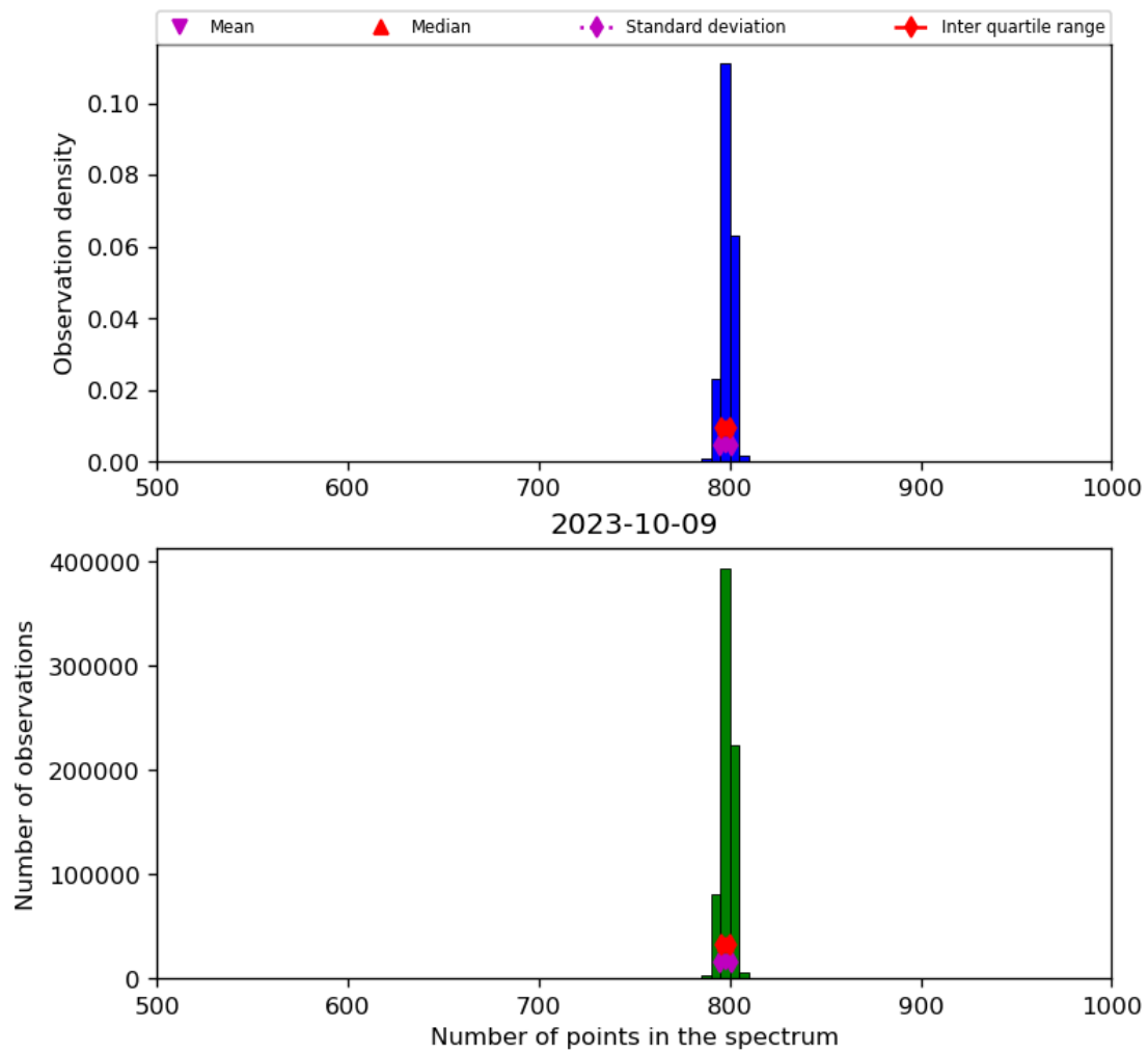
Figure 26: Histogram of “Number of points in the spectrum” for 2023-10-08 to 2023-10-10
