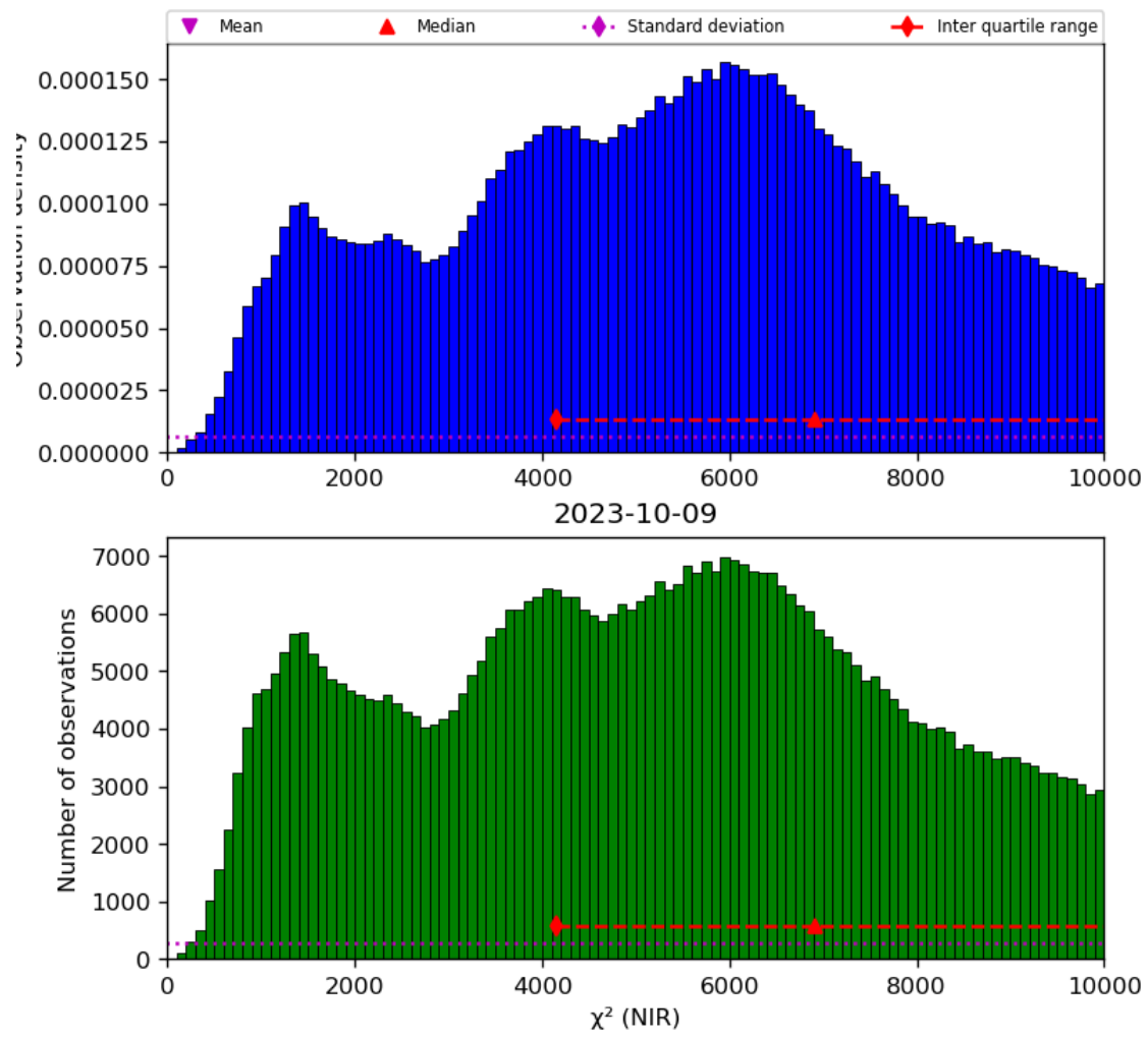
Figure 29: Histogram of “ \chi^2 (NIR)” for 2023-10-08 to 2023-10-10
