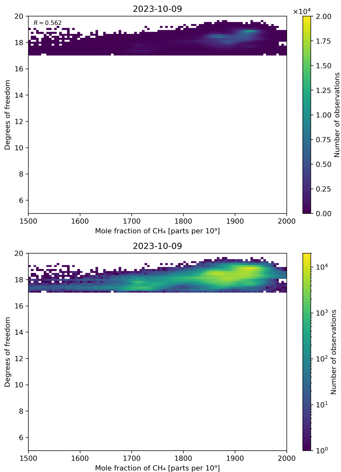
Figure 72: Scatter density plot of “Mole fraction of CH 4 ” against “Degrees of freedom” for 2023-10-08 to 2023-10-10.
