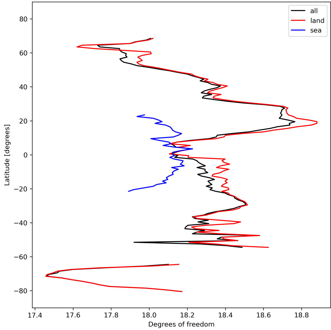
Figure 19: Zonal average of “Degrees of freedom” for 2023-10-08 to 2023-10-10.
