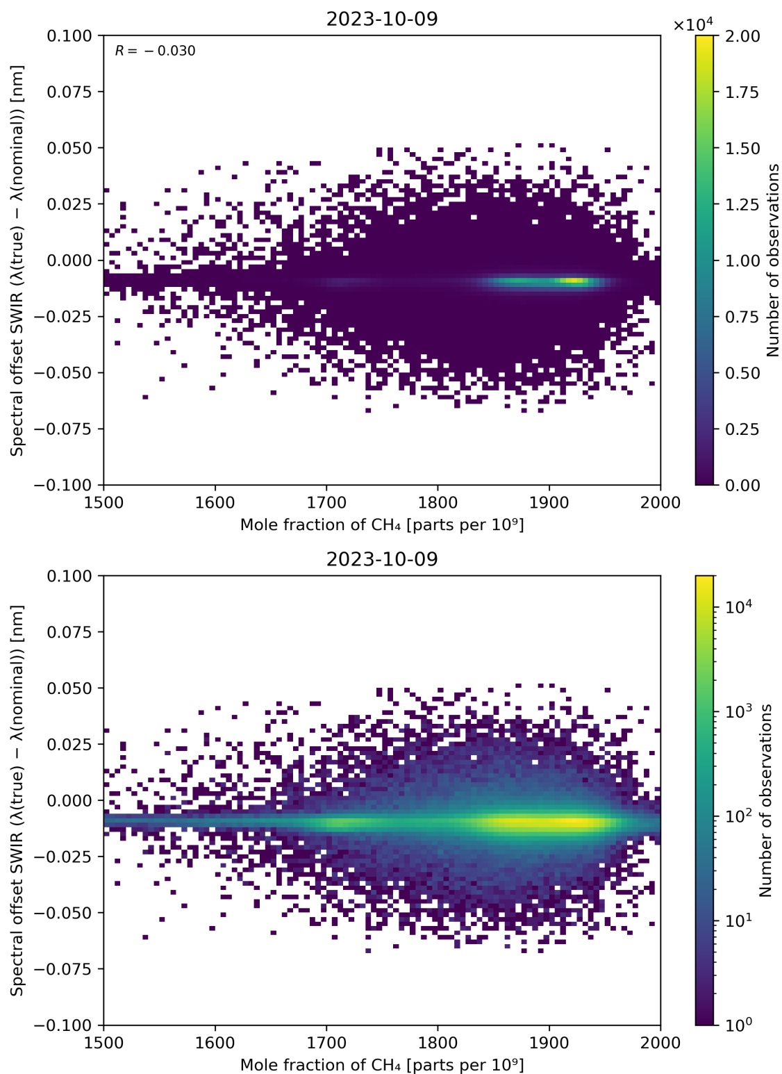
Figure 86: Scatter density plot of “Mole fraction of CH 4 ” against “Spectral offset SWIR ( \lambda(\text{true}) - \lambda(\text{nominal}) )” for 2023-10-08 to 2023-10-10.
