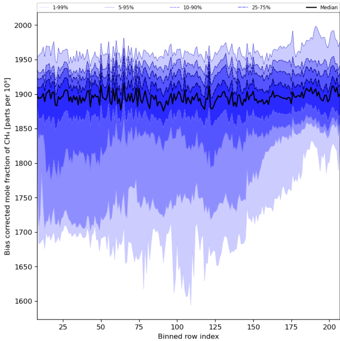
Figure 36: Along track statistics of “Bias corrected mole fraction of CH 4 ” for 2023-10-08 to 2023-10-10
