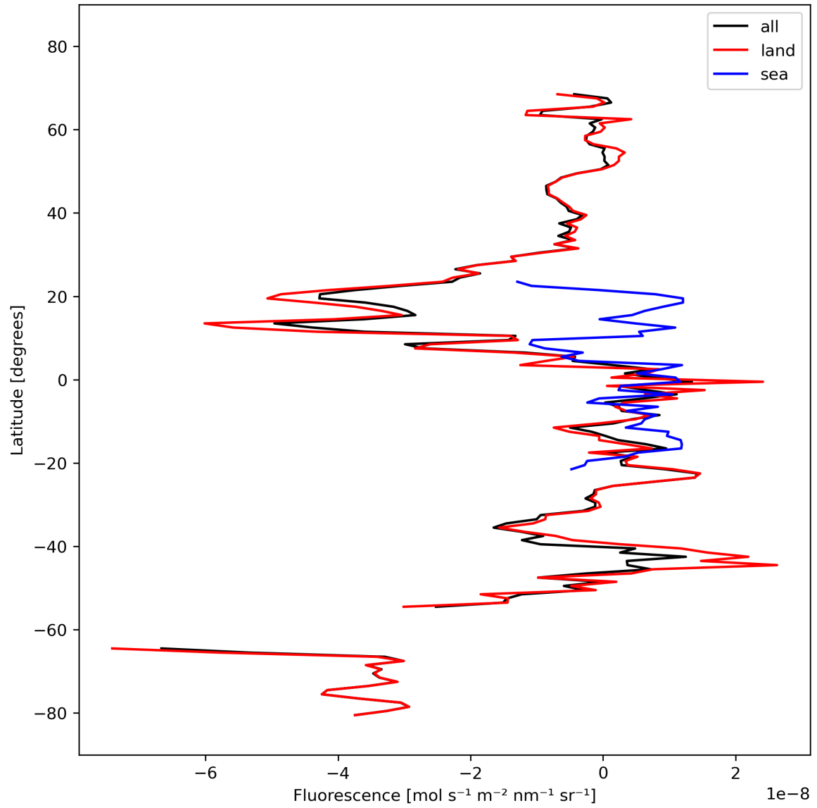
Figure 21: Zonal average of “Fluorescence” for 2023-10-08 to 2023-10-10.
