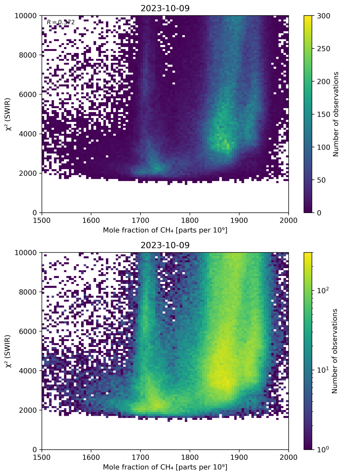
Figure 71: Scatter density plot of “Mole fraction of CH 4 ” against “ \chi^2 (SWIR)” for 2023-10-08 to 2023-10-10.
