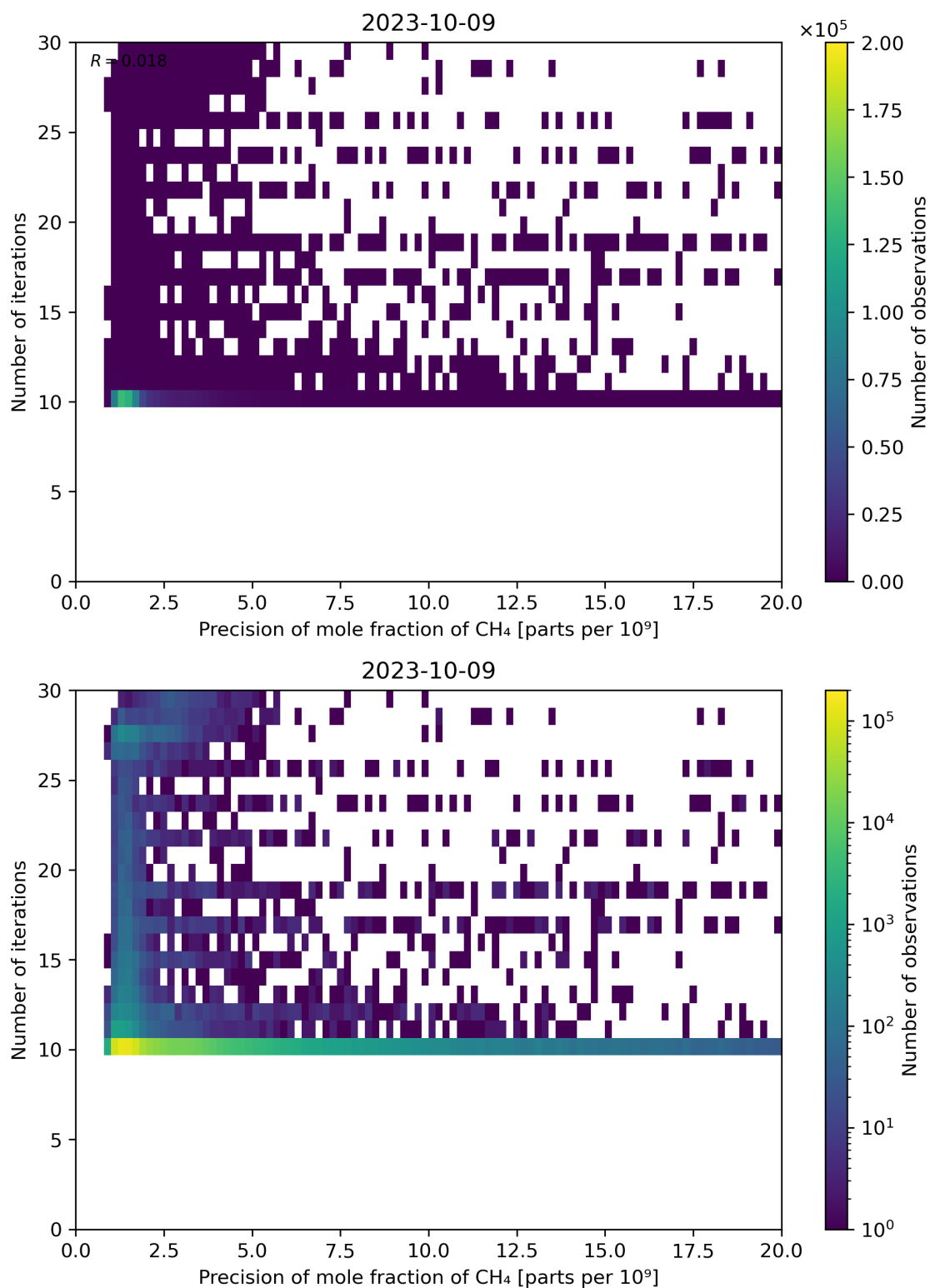
Figure 83: Scatter density plot of “Precision of mole fraction of CH 4 ” against “Number of iterations” for 2023-10-08 to 2023-10-10.
