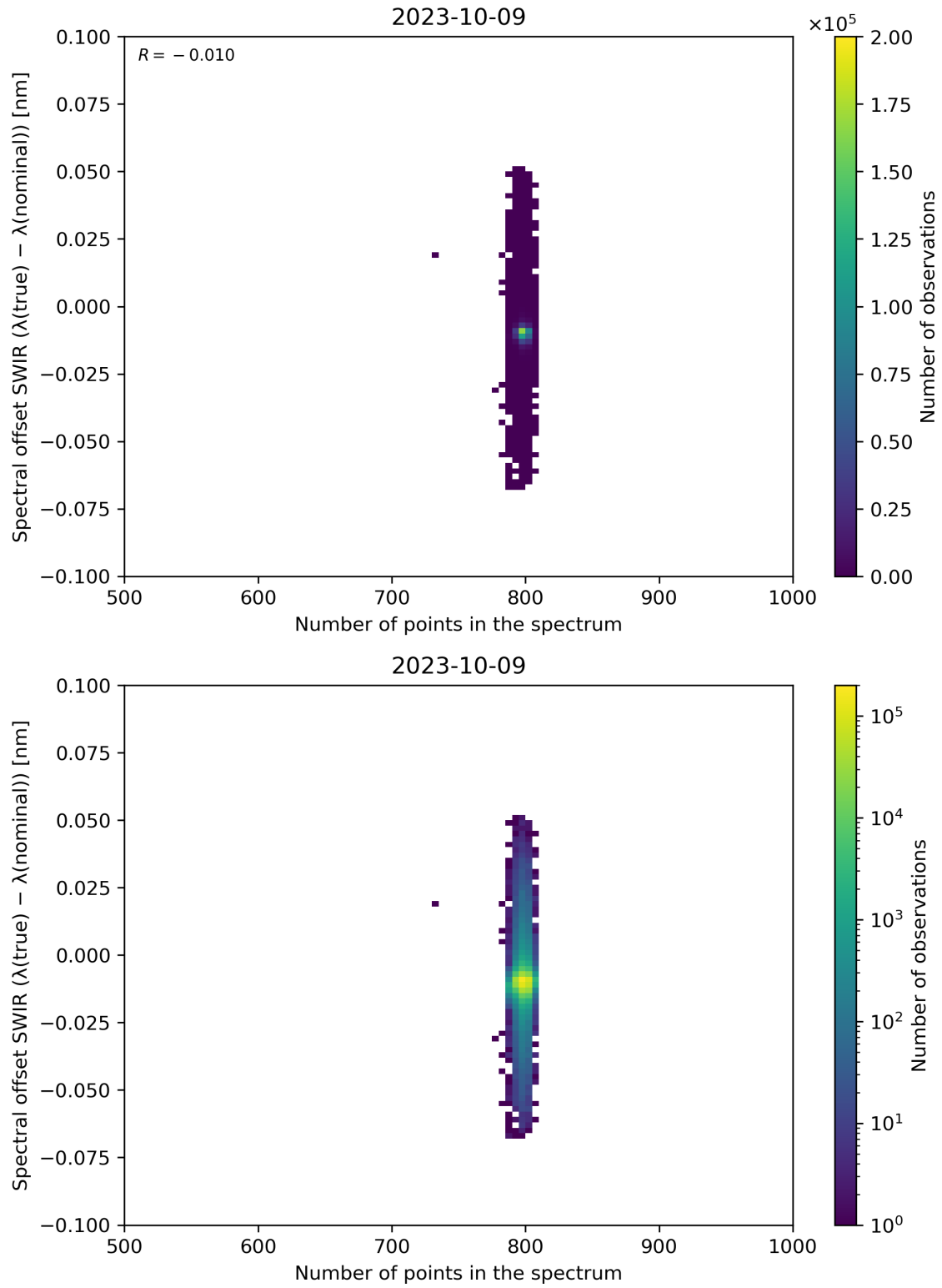
Figure 93: Scatter density plot of “Number of points in the spectrum” against “Spectral offset SWIR ( \lambda(\text{true}) - \lambda(\text{nominal}) )” for 2023-10-08 to 2023-10-10.
