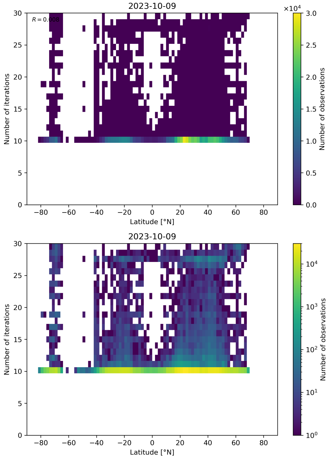
Figure 60: Scatter density plot of “Latitude” against “Number of iterations” for 2023-10-08 to 2023-10-10.
