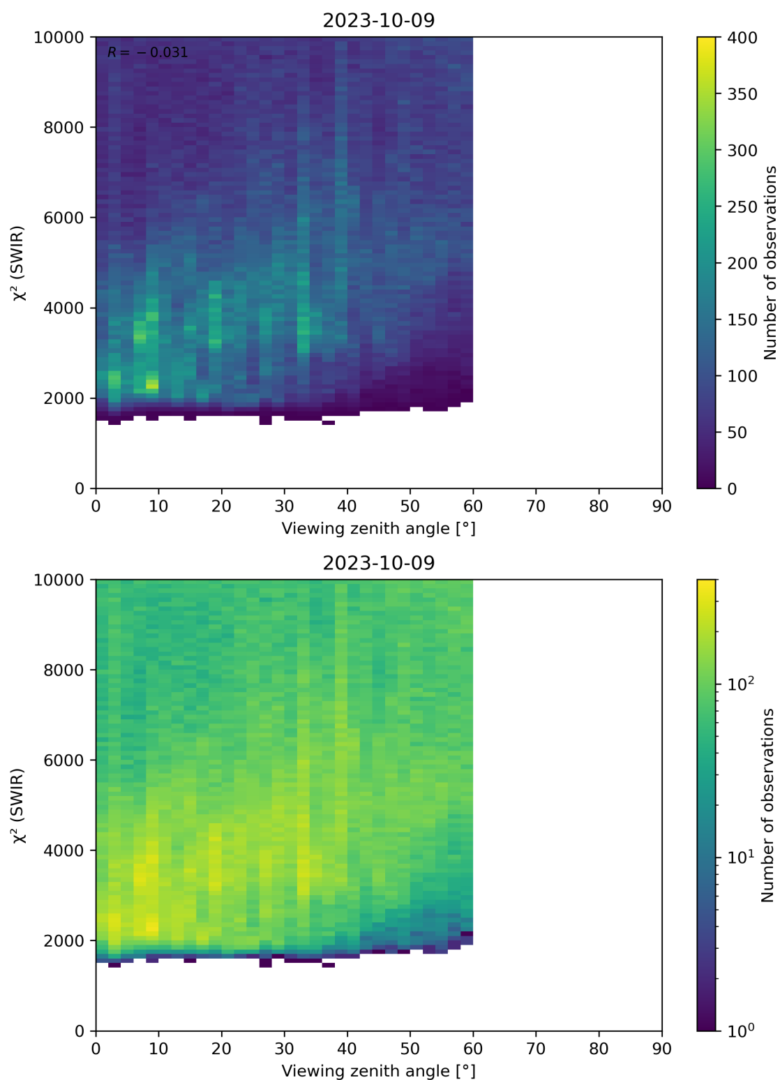
Figure 106: Scatter density plot of “Viewing zenith angle” against “ \chi^2 (SWIR)” for 2023-10-08 to 2023-10-10.
