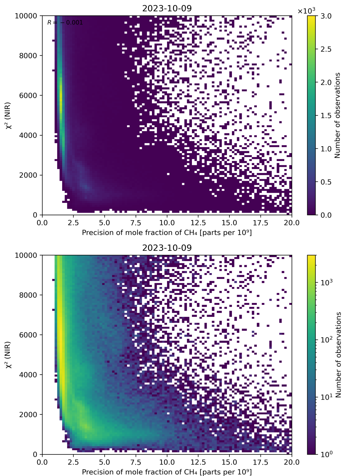
Figure 78: Scatter density plot of “Precision of mole fraction of CH 4 ” against “ \chi^2 (NIR)” for 2023-10-08 to 2023-10-10.
