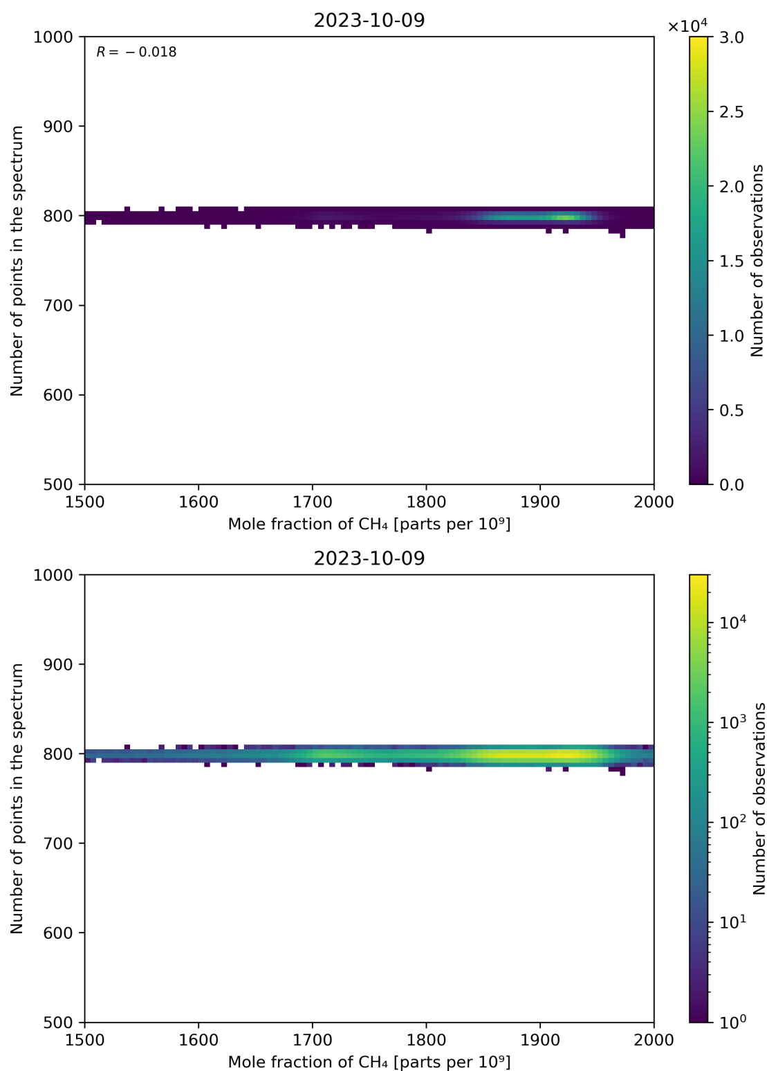
Figure 77: Scatter density plot of “Mole fraction of CH 4 ” against “Number of points in the spectrum” for 2023-10-08 to 2023-10-10.
