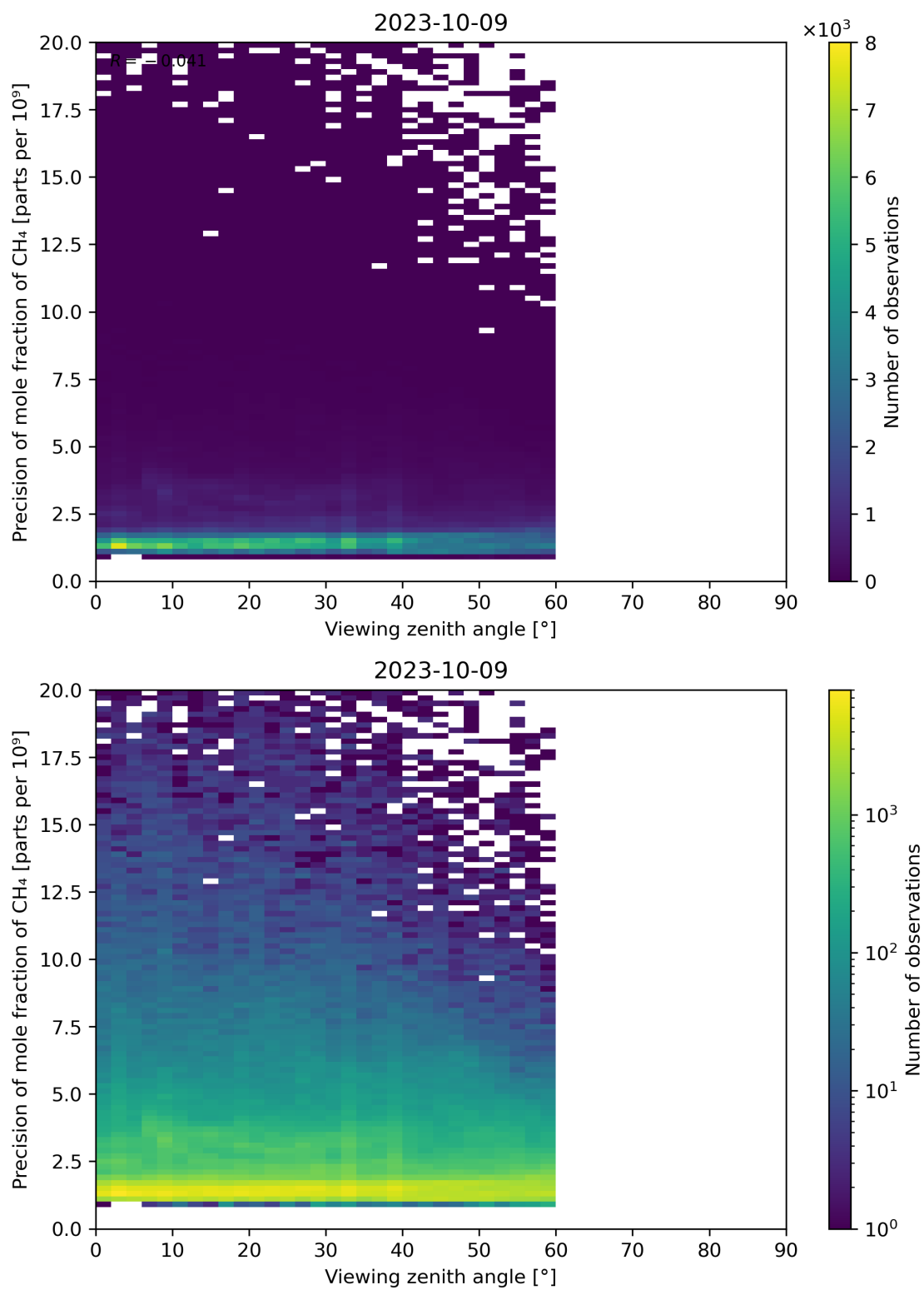
Figure 112: Scatter density plot of “Viewing zenith angle” against “Precision of mole fraction of CH 4 ” for 2023-10-08 to 2023-10-10.
