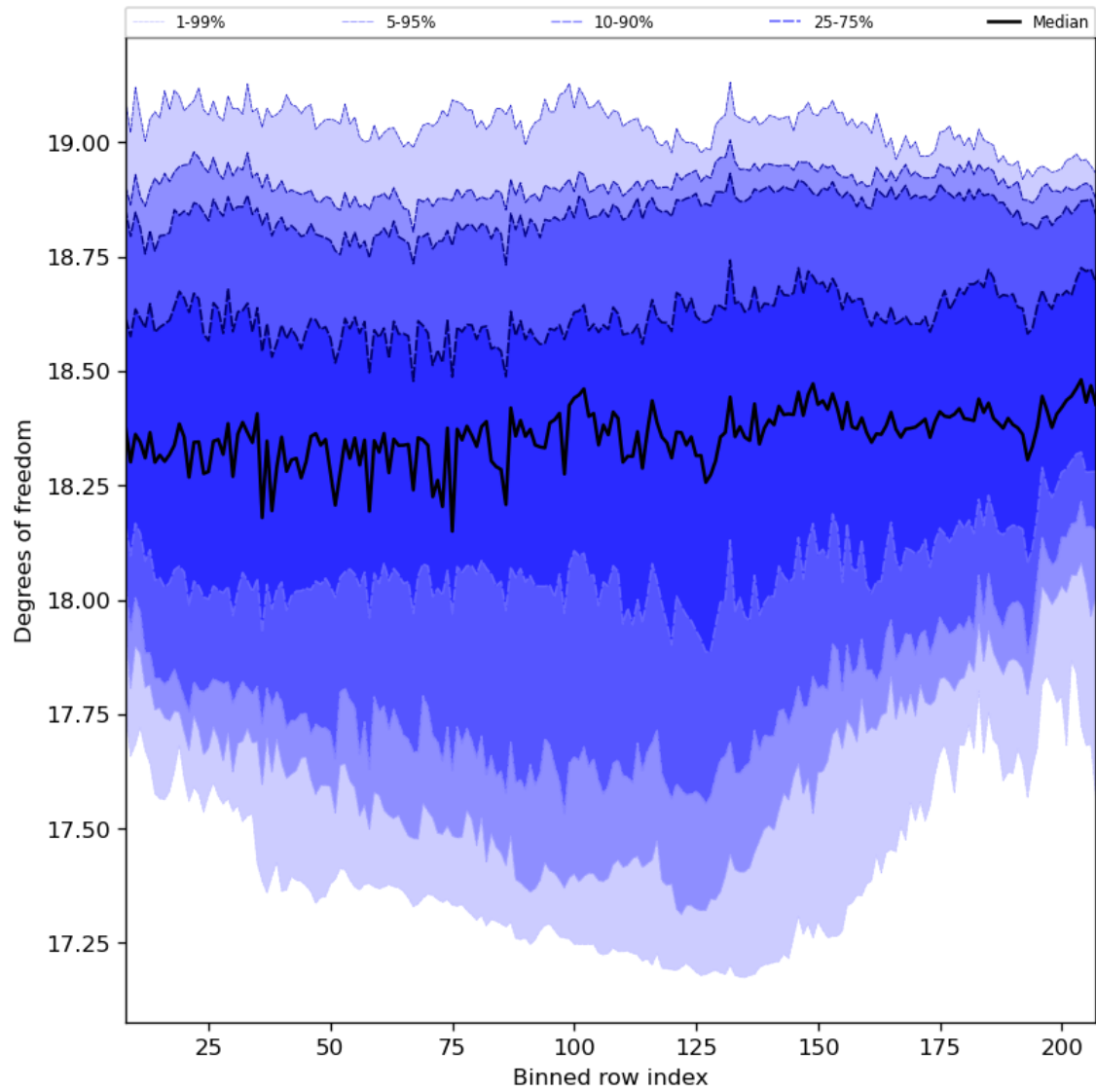
Figure 41: Along track statistics of “Degrees of freedom” for 2023-10-08 to 2023-10-10
