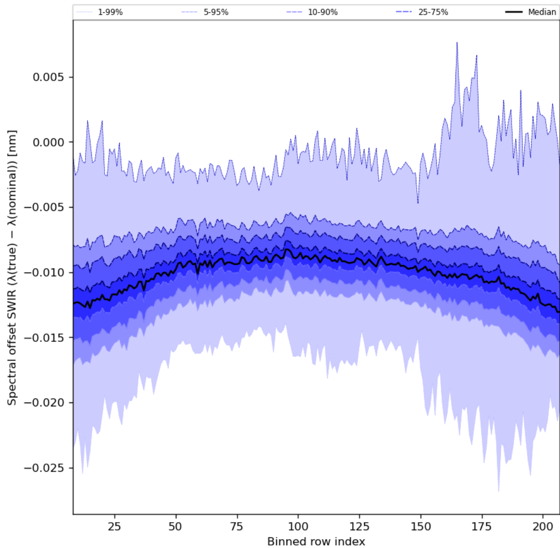
Figure 38: Along track statistics of “Spectral offset SWIR ( \lambda(\text{true}) - \lambda(\text{nominal}) )” for 2023-10-08 to 2023-10-10
