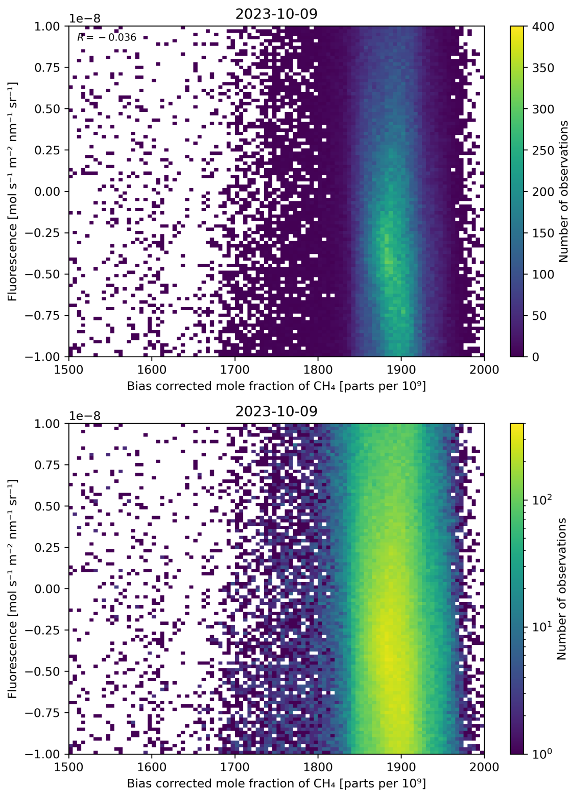
Figure 66: Scatter density plot of “Bias corrected mole fraction of \text{CH}_4 ” against “Fluorescence” for 2023-10-08 to 2023-10-10.
