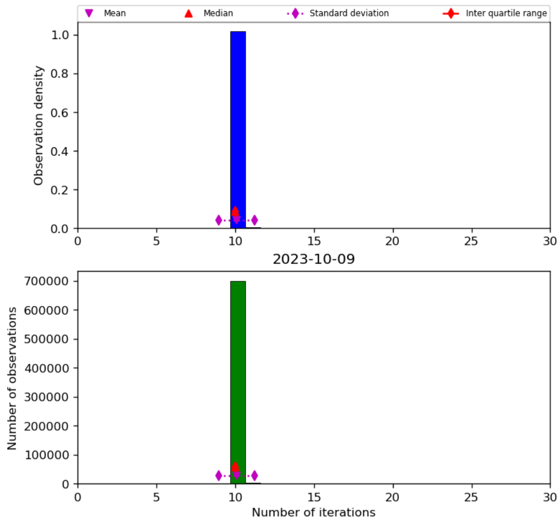
Figure 31: Histogram of “Number of iterations” for 2023-10-08 to 2023-10-10
