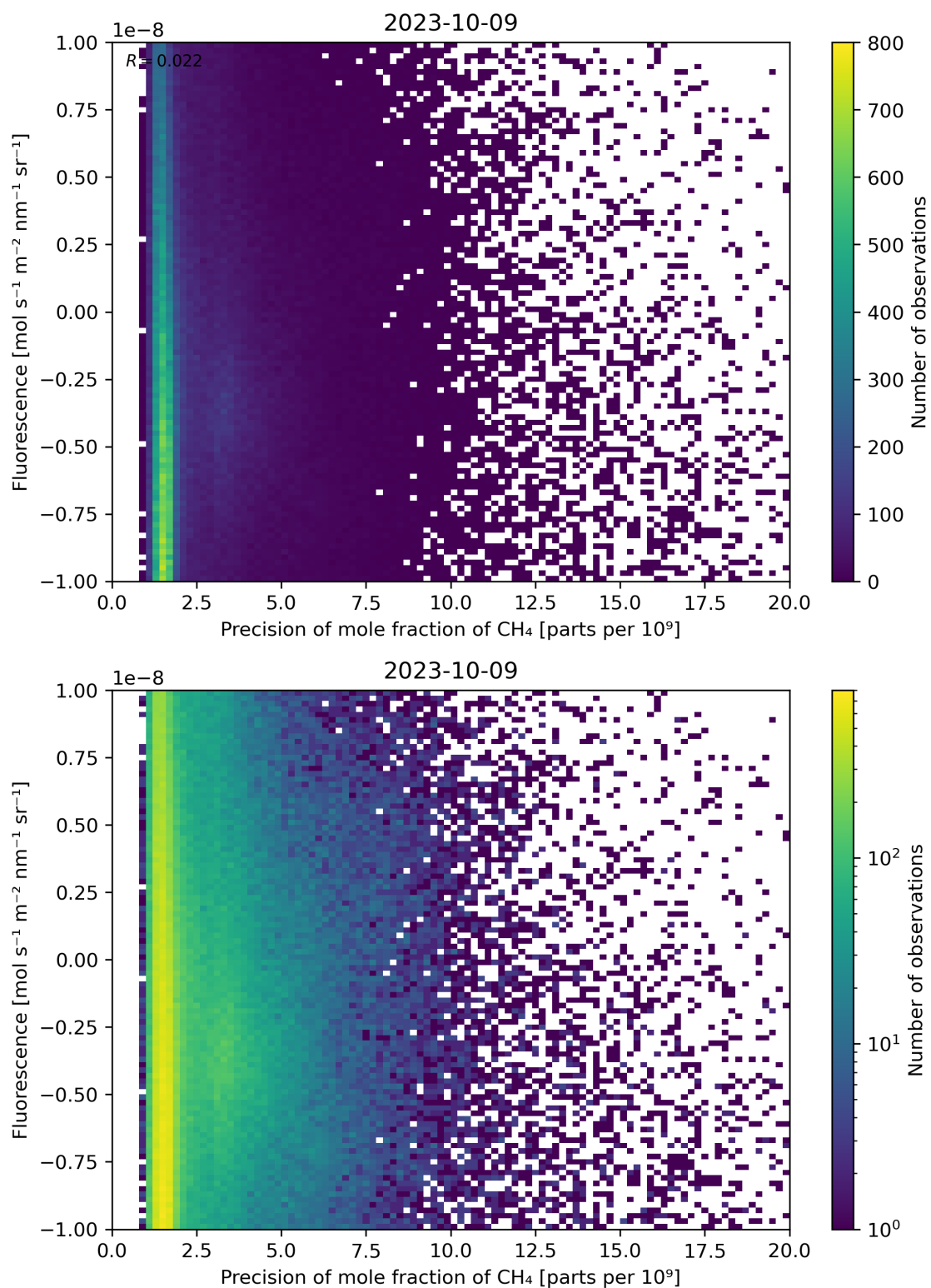
Figure 81: Scatter density plot of “Precision of mole fraction of \text{CH}_4 ” against “Fluorescence” for 2023-10-08 to 2023-10-10.
