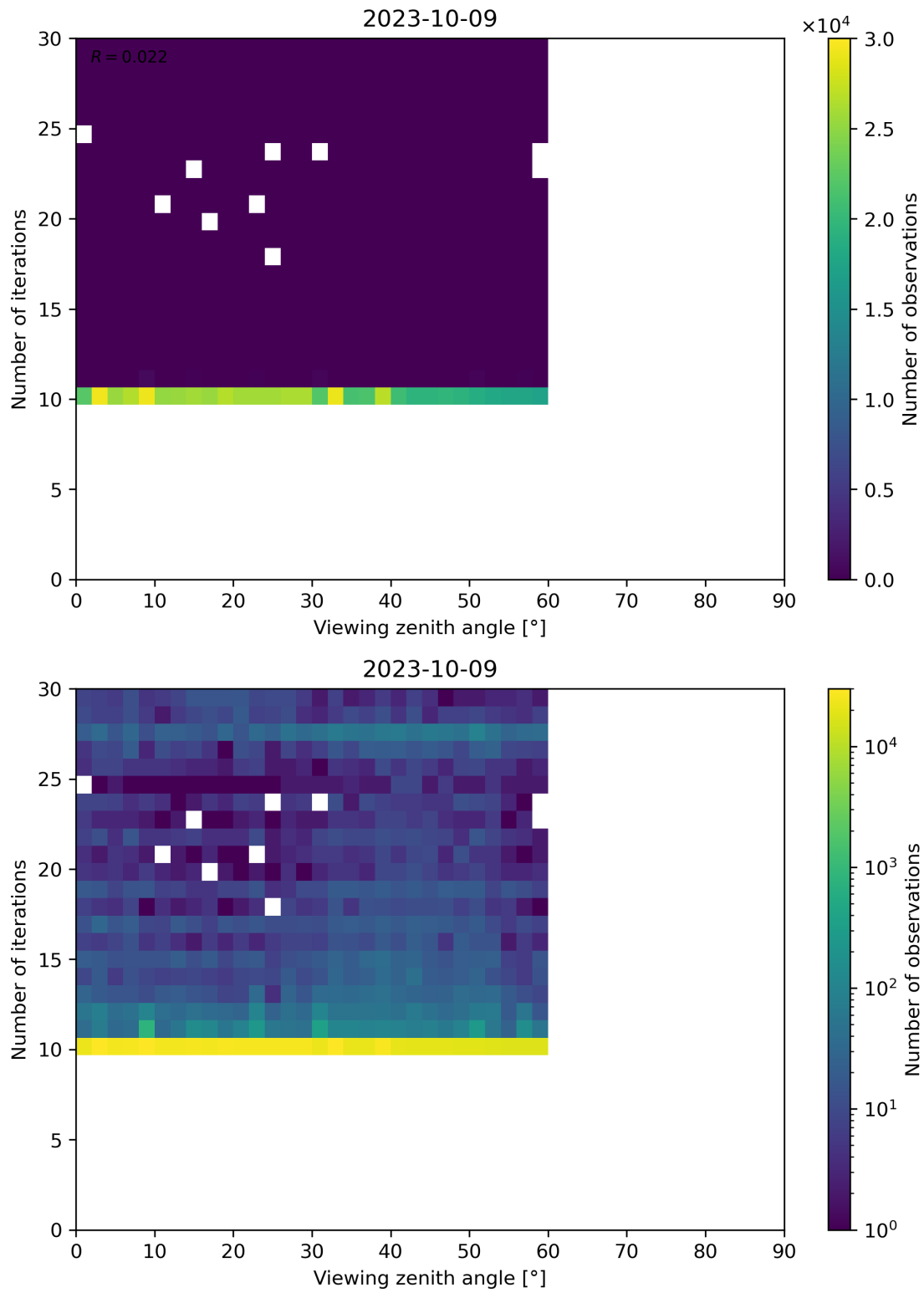
Figure 113: Scatter density plot of “Viewing zenith angle” against “Number of iterations” for 2023-10-08 to 2023-10-10.
