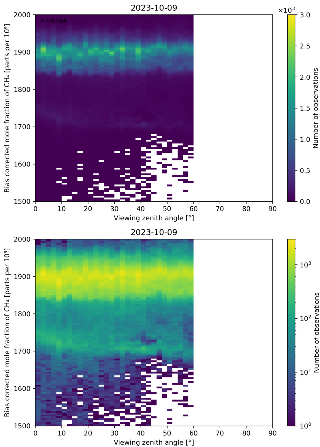
Figure 111: Scatter density plot of “Viewing zenith angle” against “Bias corrected mole fraction of CH 4 ” for 2023-10-08 to 2023-10-10.
