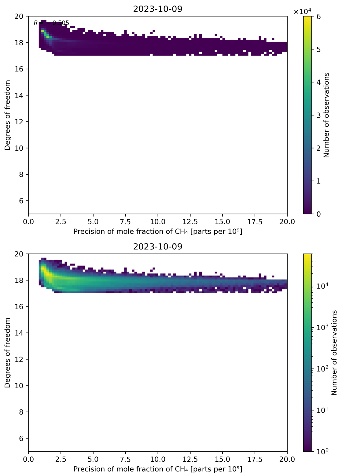
Figure 80: Scatter density plot of “Precision of mole fraction of CH 4 ” against “Degrees of freedom” for 2023-10-08 to 2023-10-10.
