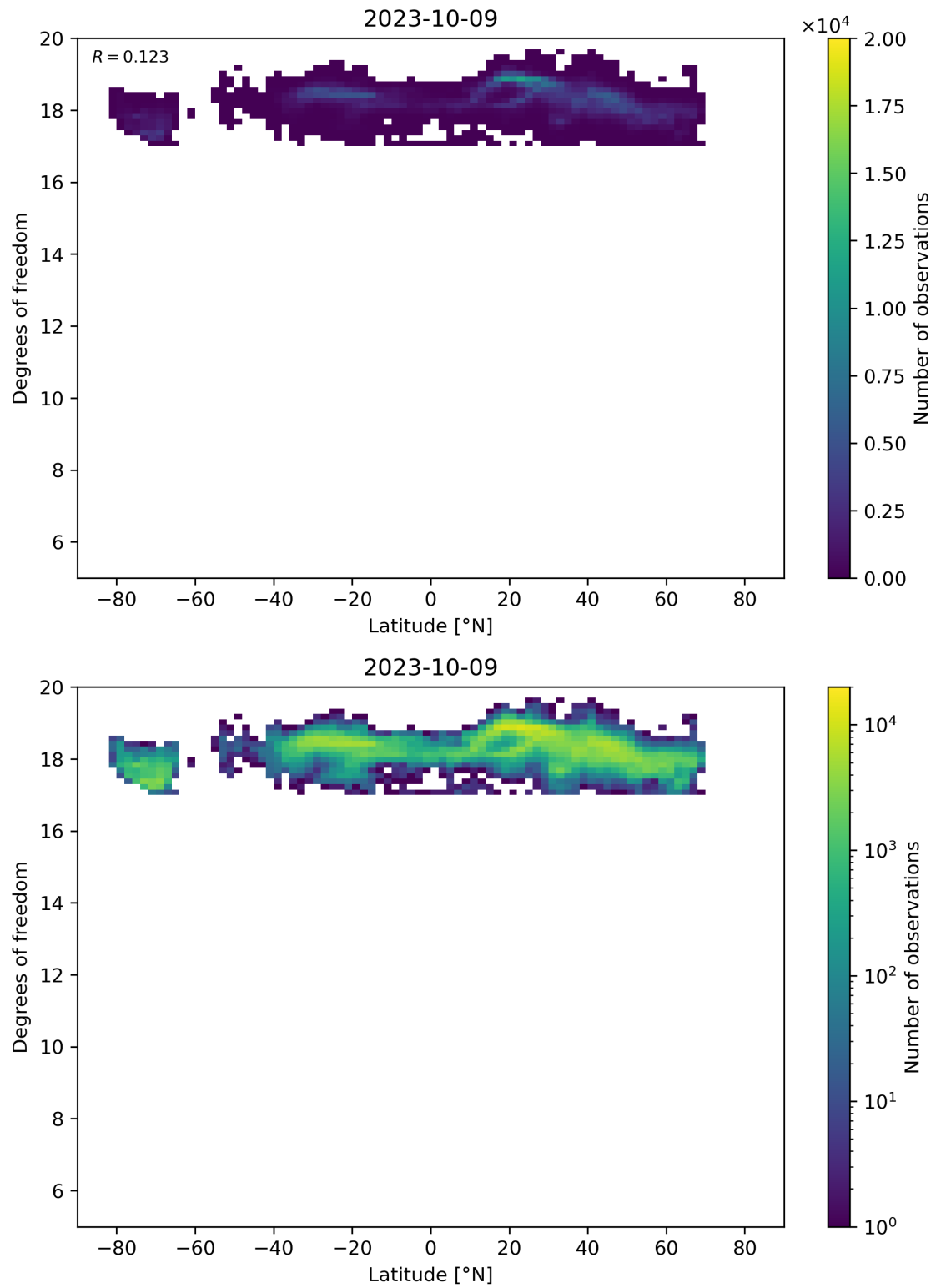
Figure 55: Scatter density plot of “Latitude” against “Degrees of freedom” for 2023-10-08 to 2023-10-10.
