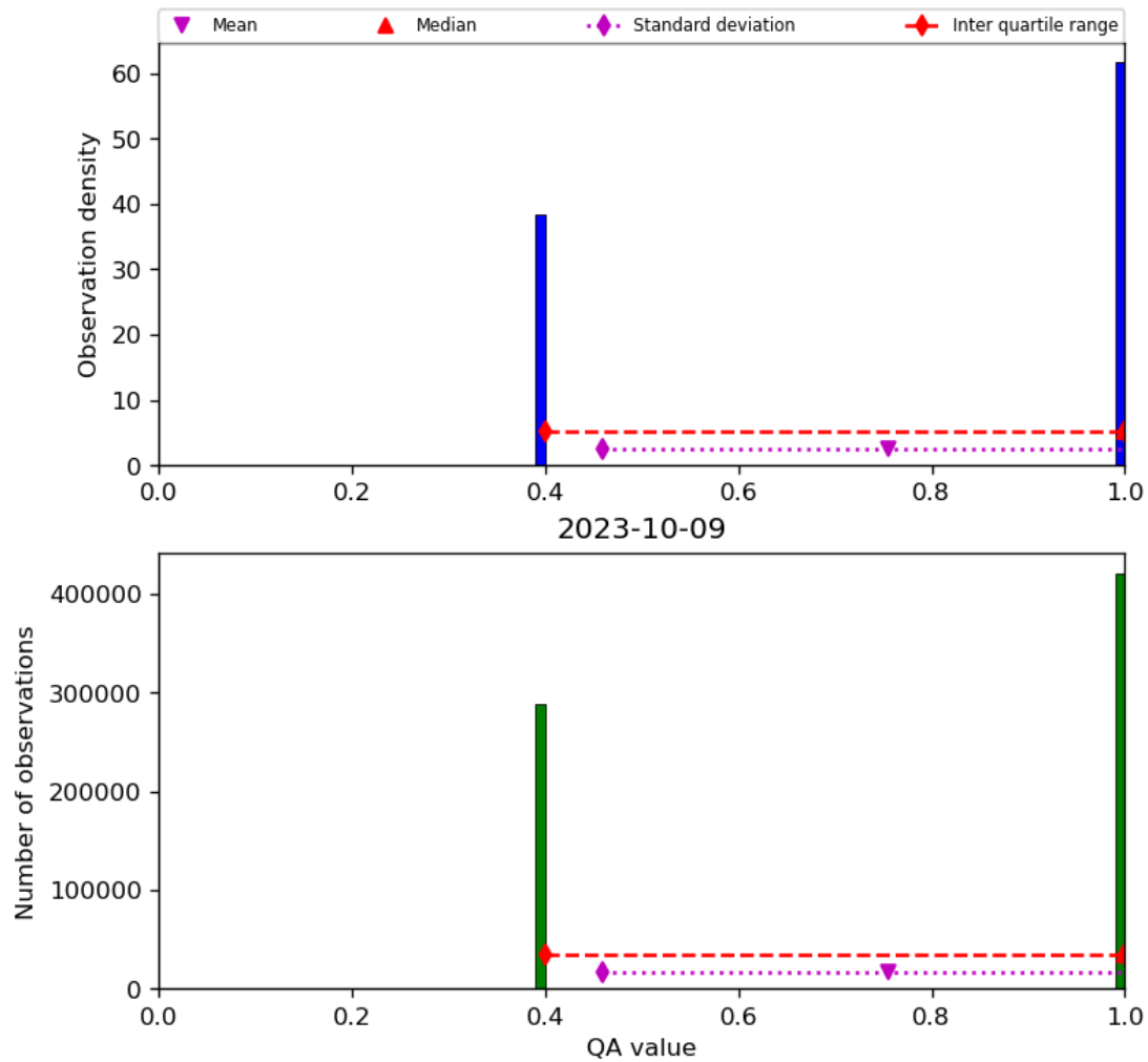
Figure 22: Histogram of “QA value” for 2023-10-08 to 2023-10-10
