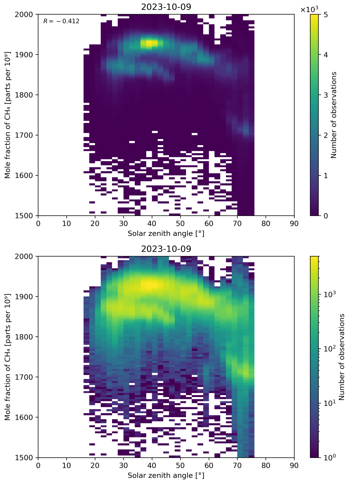
Figure 99: Scatter density plot of “Solar zenith angle” against “Mole fraction of CH 4 ” for 2023-10-08 to 2023-10-10.
