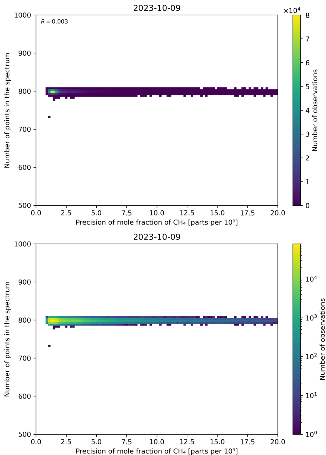
Figure 84: Scatter density plot of “Precision of mole fraction of \text{CH}_4 ” against “Number of points in the spectrum” for 2023-10-08 to 2023-10-10.
