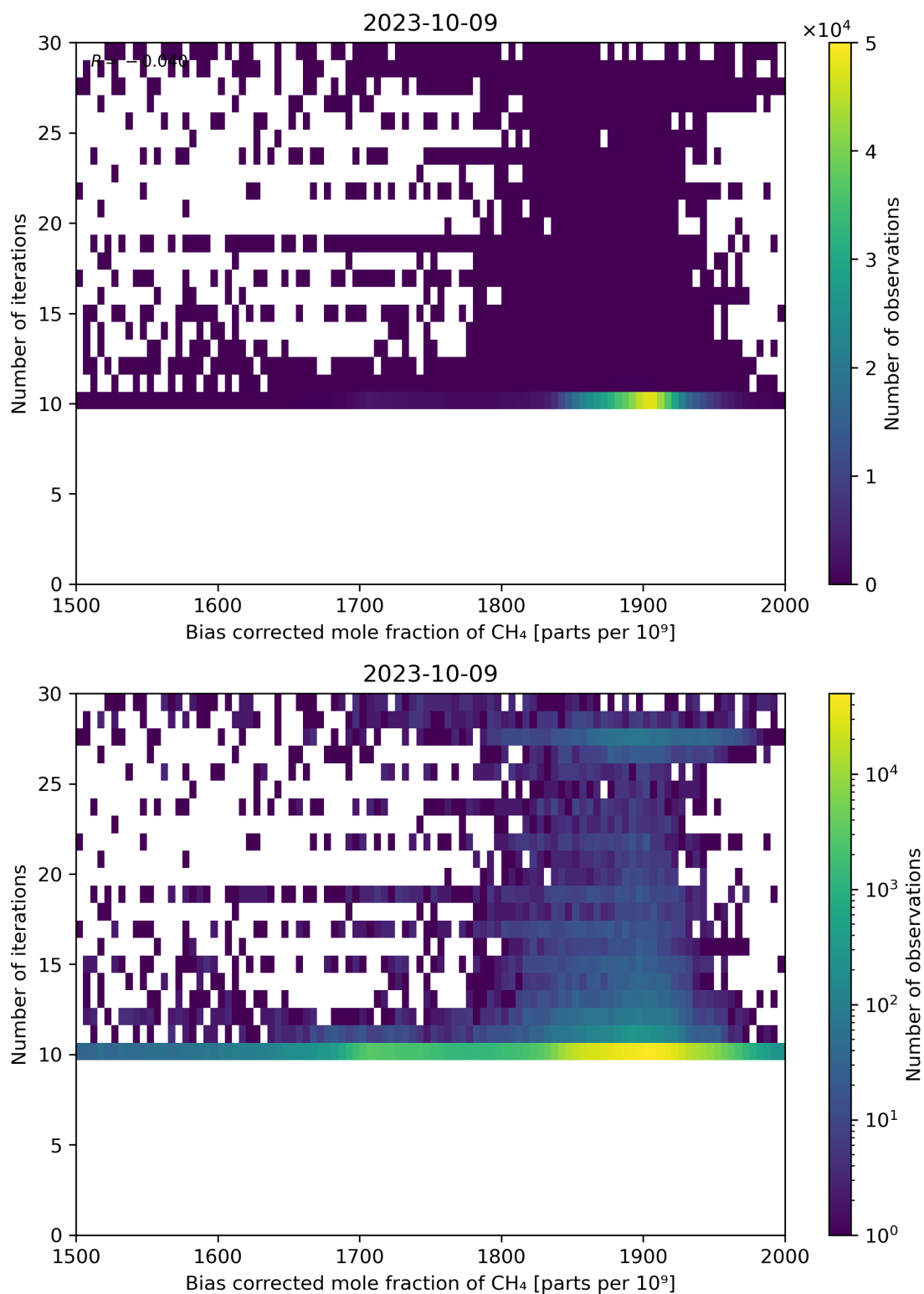
Figure 67: Scatter density plot of “Bias corrected mole fraction of CH 4 ” against “Number of iterations” for 2023-10-08 to 2023-10-10.
