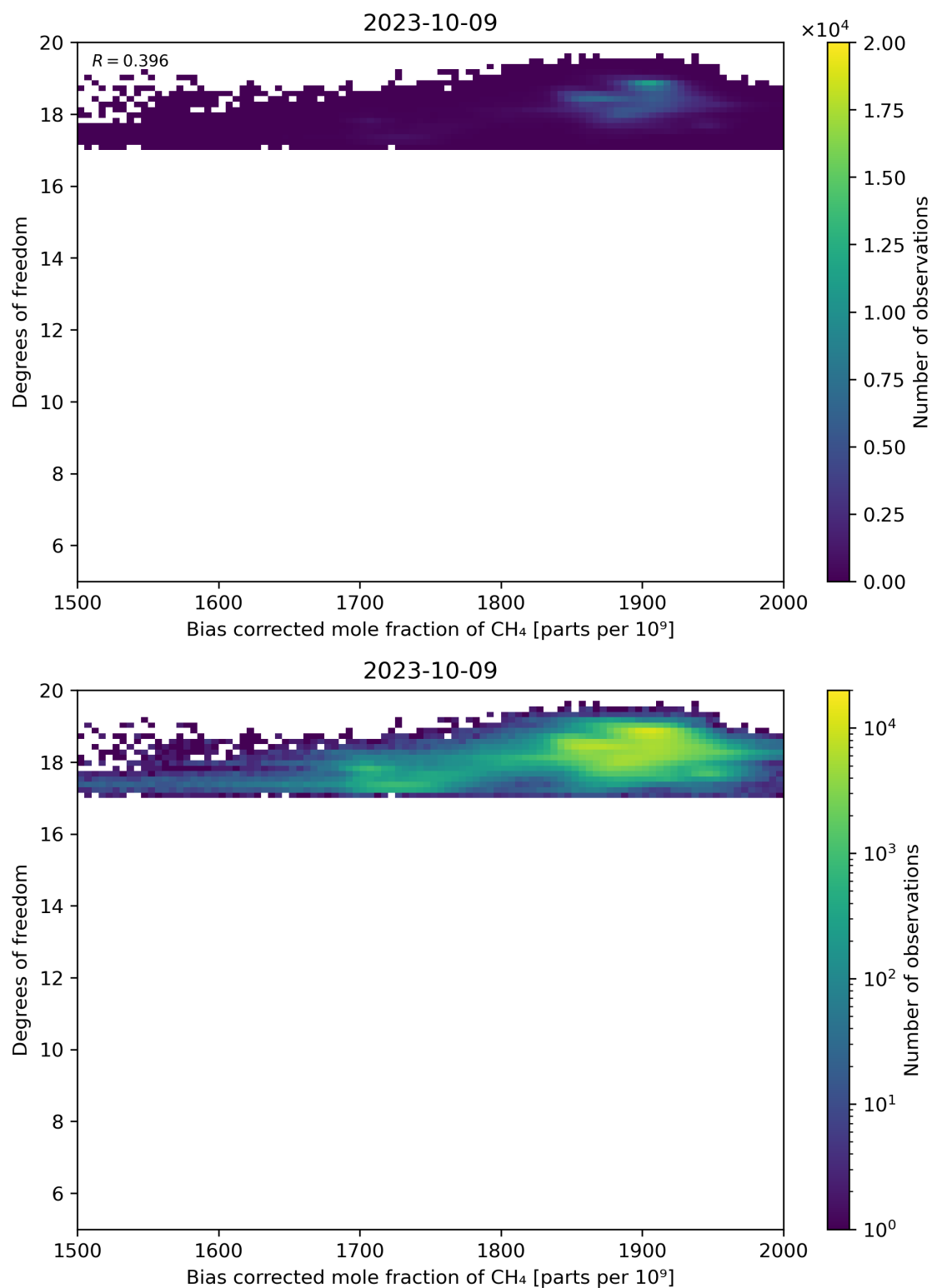
Figure 65: Scatter density plot of “Bias corrected mole fraction of CH 4 ” against “Degrees of freedom” for 2023-10-08 to 2023-10-10.
