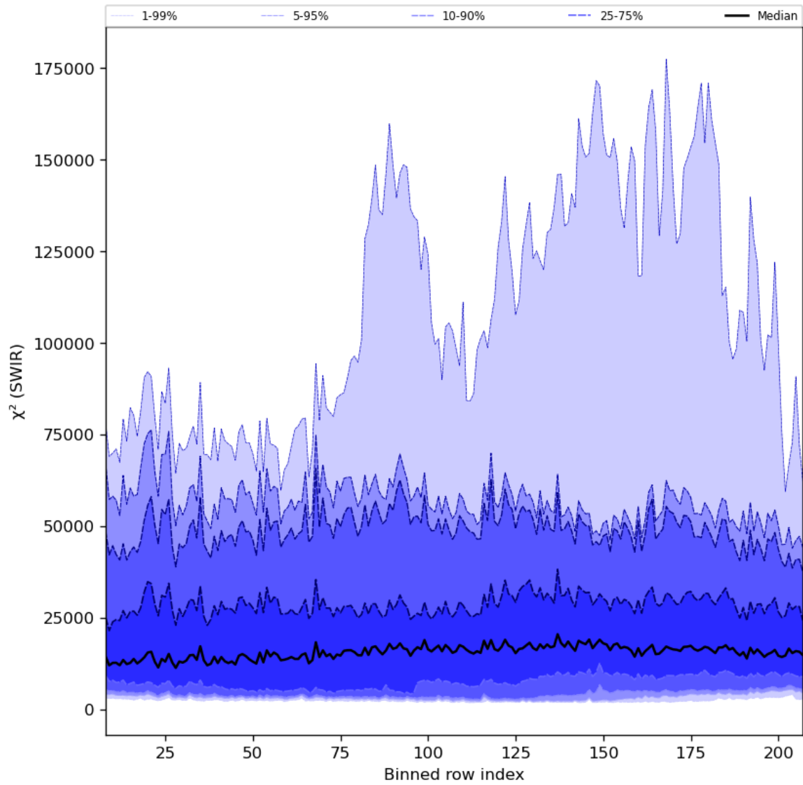
Figure 39: Along track statistics of " \chi^2 (SWIR)" for 2023-10-08 to 2023-10-10
