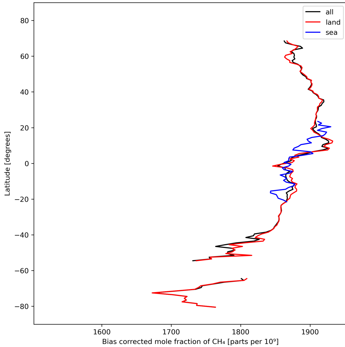
Figure 14: Zonal average of “Bias corrected mole fraction of CH 4 ” for 2023-10-08 to 2023-10-10.
