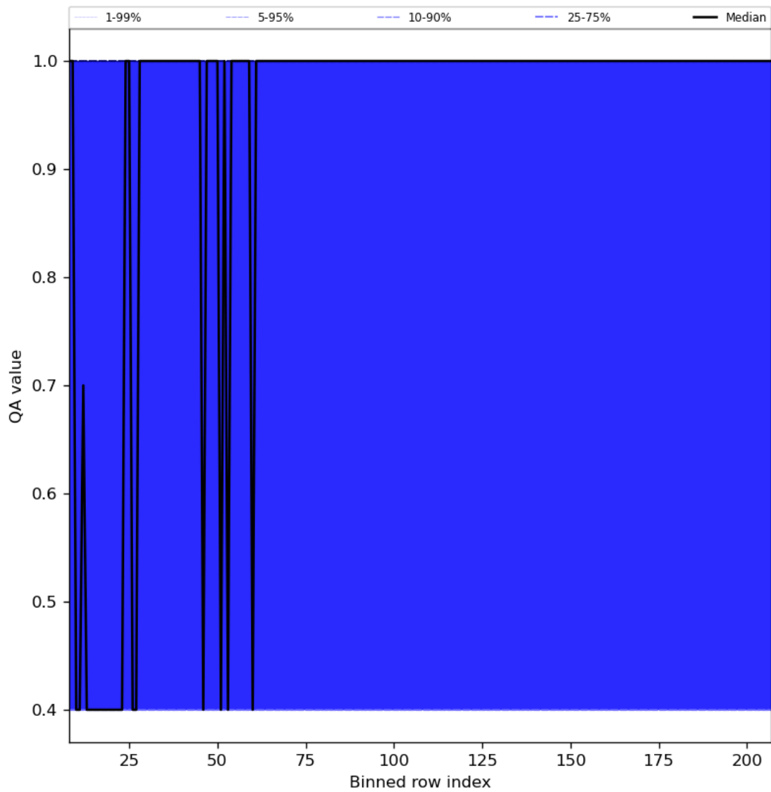
Figure 33: Along track statistics of “QA value” for 2023-10-08 to 2023-10-10
