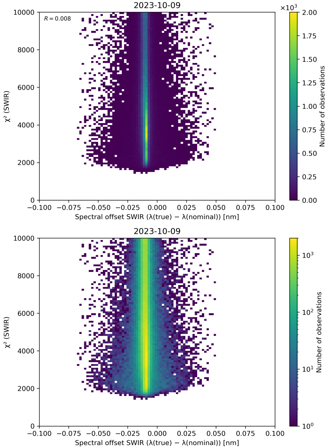
Figure 118: Scatter density plot of “Spectral offset SWIR ( \lambda(\text{true}) - \lambda(\text{nominal}) )” against “ \chi^2 (SWIR)” for 2023-10-08 to 2023-10-10.
