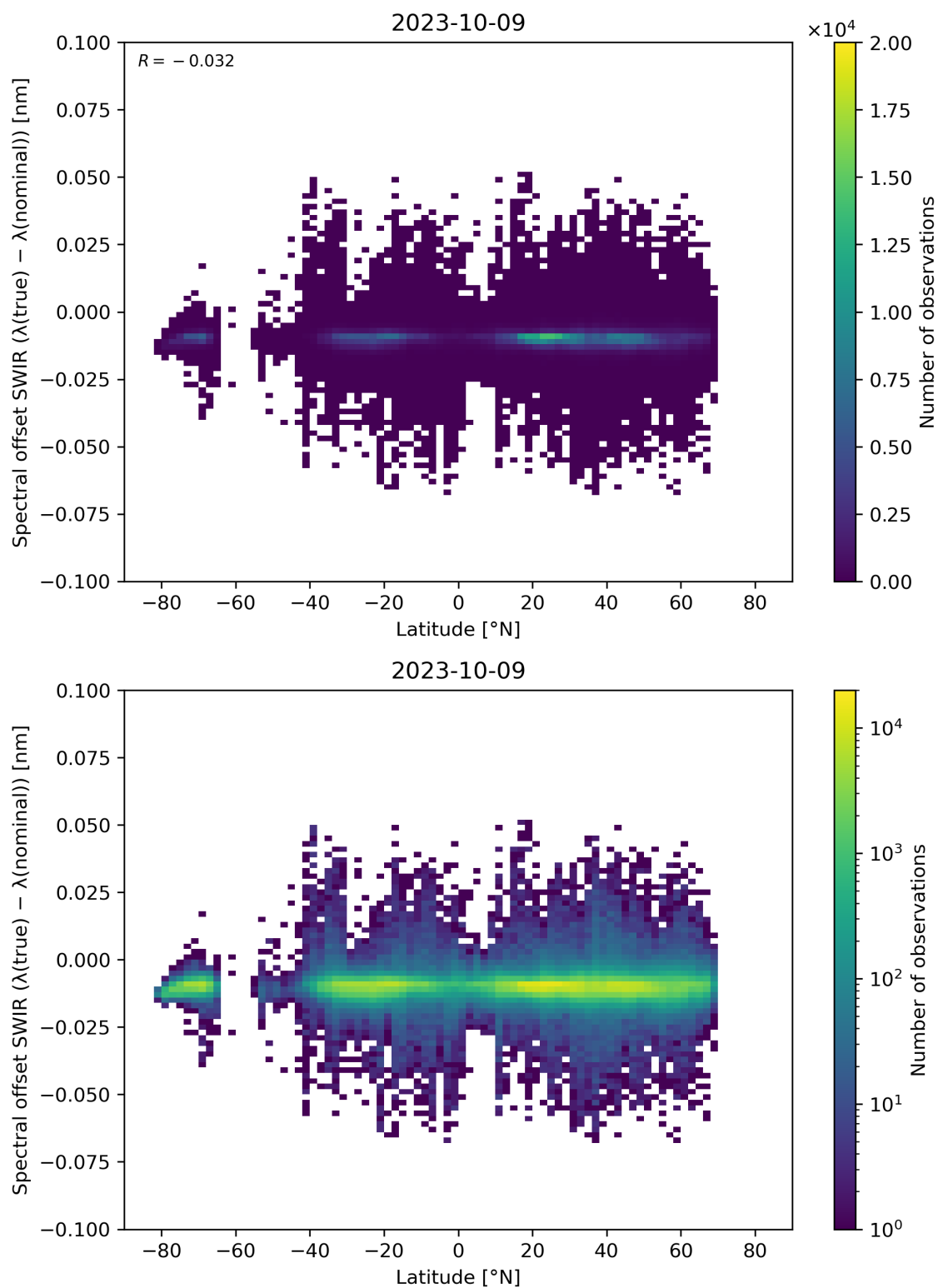
Figure 62: Scatter density plot of “Latitude” against “Spectral offset SWIR ( \lambda(\text{true}) - \lambda(\text{nominal}) )” for 2023-10-08 to 2023-10-10.
