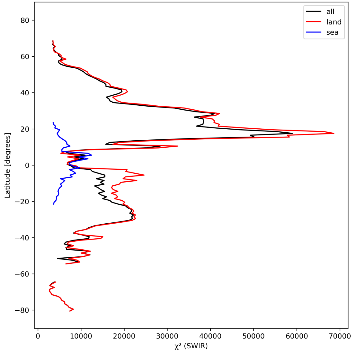
Figure 17: Zonal average of “ \chi^2 (SWIR)” for 2023-10-08 to 2023-10-10.
