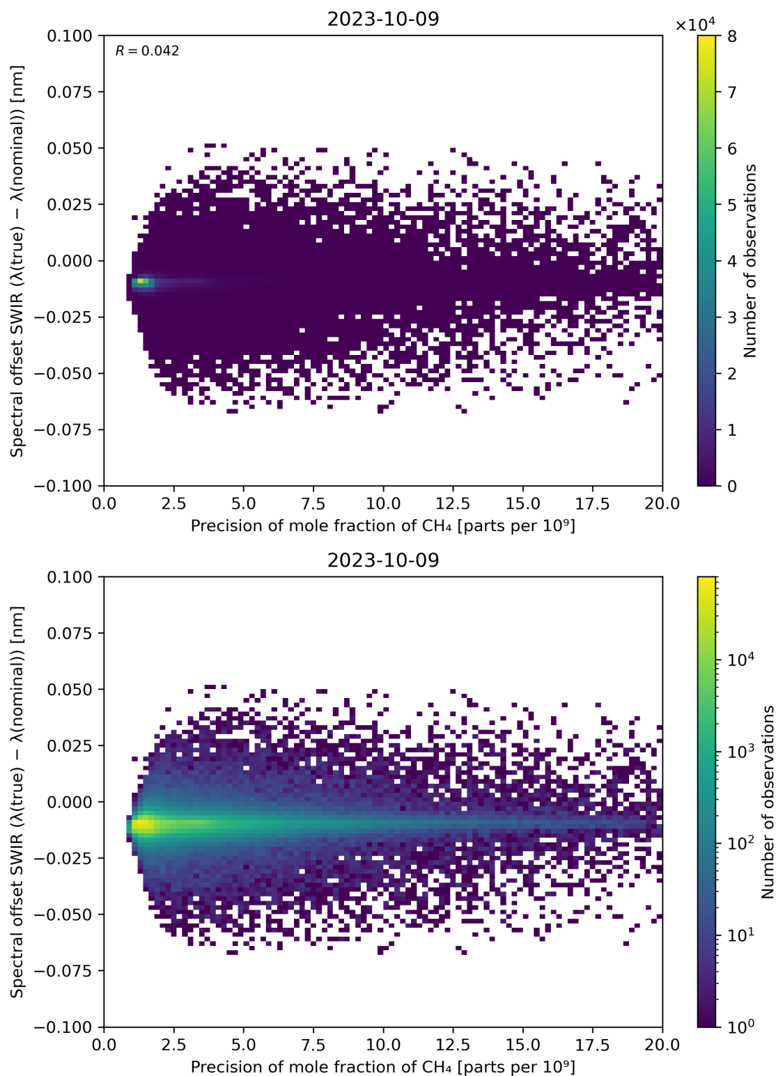
Figure 85: Scatter density plot of “Precision of mole fraction of CH 4 ” against “Spectral offset SWIR ( \lambda(\text{true}) - \lambda(\text{nominal}) )” for 2023-10-08 to 2023-10-10.
