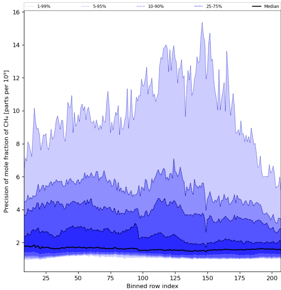
Figure 35: Along track statistics of “Precision of mole fraction of CH 4 ” for 2023-10-08 to 2023-10-10
