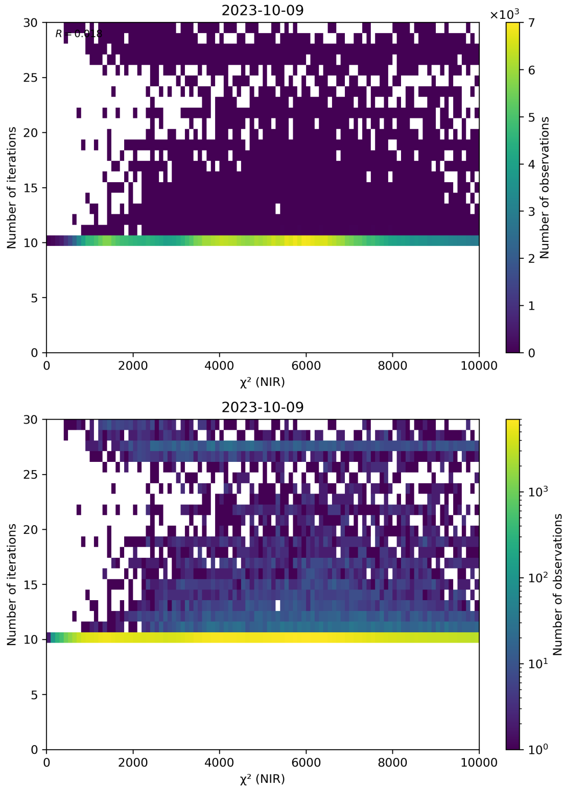
Figure 46: Scatter density plot of “ \chi^2 (NIR)” against “Number of iterations” for 2023-10-08 to 2023-10-10.
