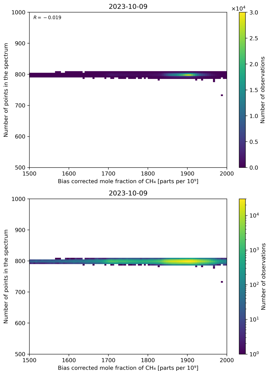
Figure 68: Scatter density plot of “Bias corrected mole fraction of CH 4 ” against “Number of points in the spectrum” for 2023-10-08 to 2023-10-10.
