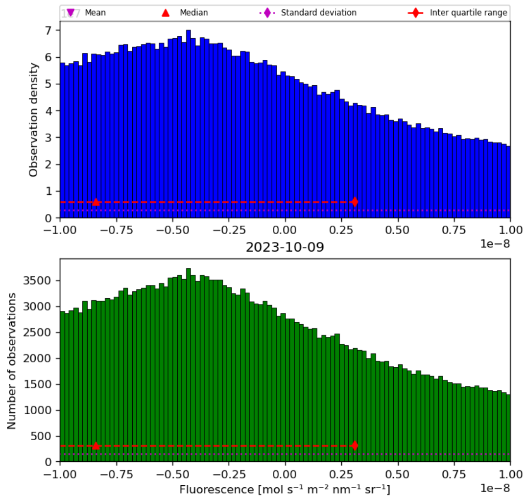
Figure 32: Histogram of “Fluorescence” for 2023-10-08 to 2023-10-10
