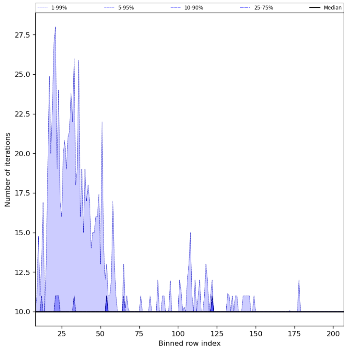
Figure 42: Along track statistics of “Number of iterations” for 2023-10-08 to 2023-10-10
