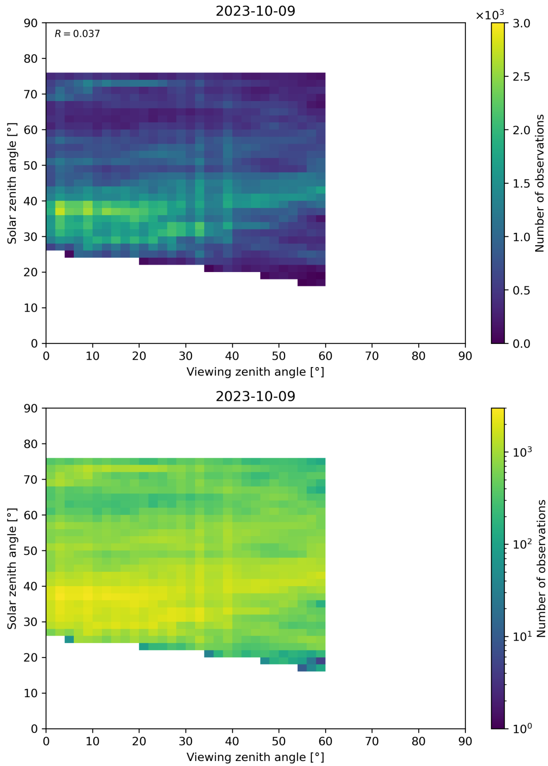
Figure 115: Scatter density plot of “Viewing zenith angle” against “Solar zenith angle” for 2023-10-08 to 2023-10-10.
