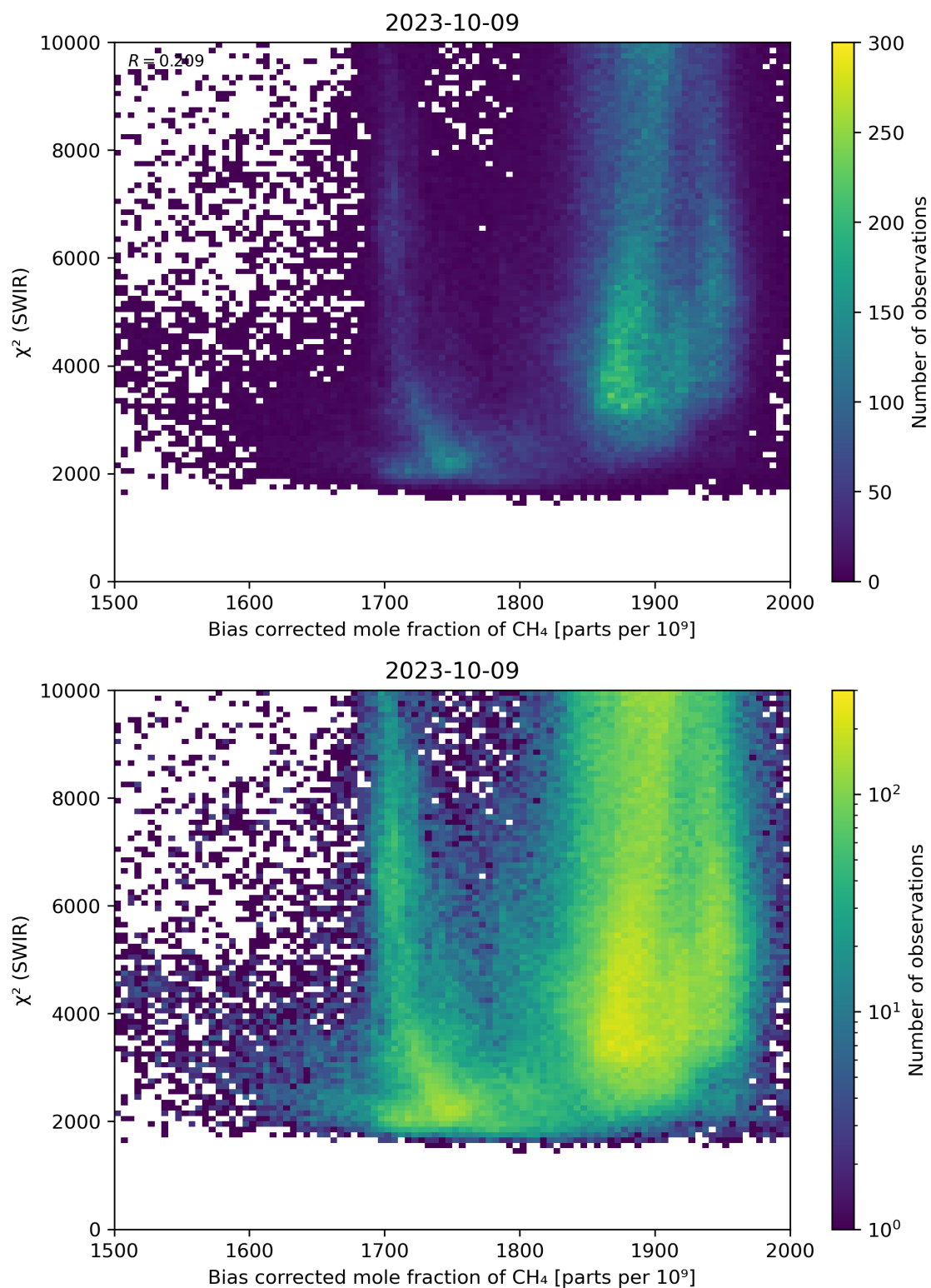
Figure 64: Scatter density plot of “Bias corrected mole fraction of CH 4 ” against “ \chi^2 (SWIR)” for 2023-10-08 to 2023-10-10.
