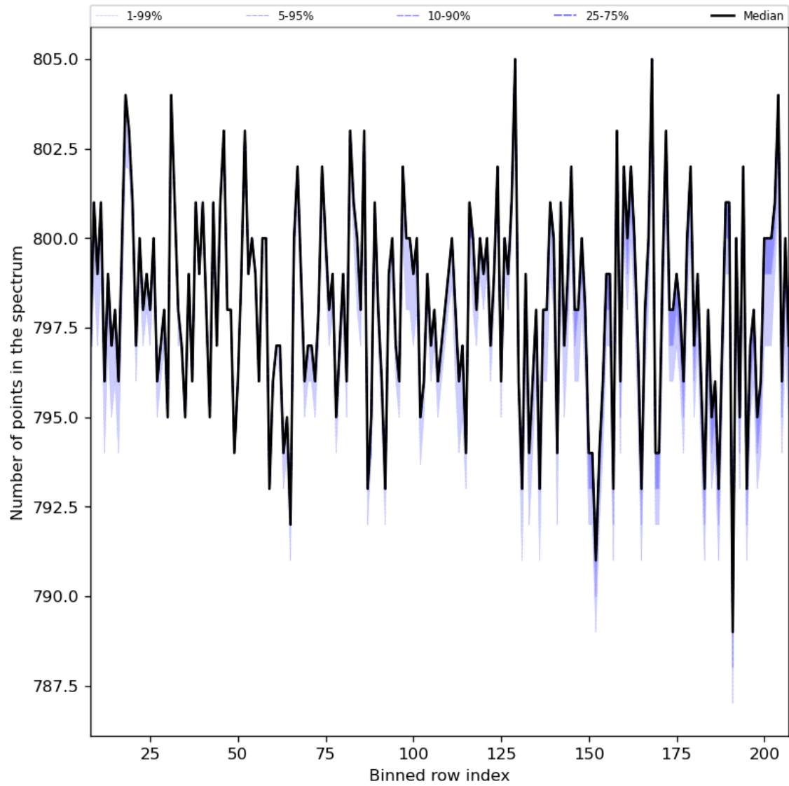
Figure 37: Along track statistics of “Number of points in the spectrum” for 2023-10-08 to 2023-10-10
