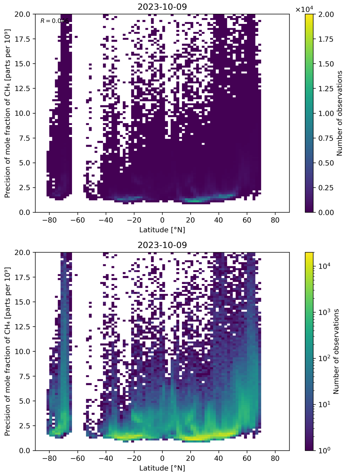
Figure 59: Scatter density plot of “Latitude” against “Precision of mole fraction of CH 4 ” for 2023-10-08 to 2023-10-10.
