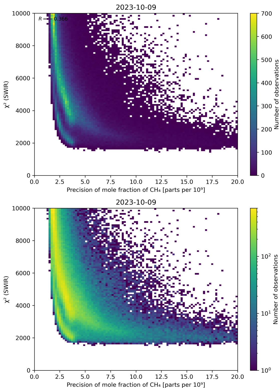
Figure 79: Scatter density plot of “Precision of mole fraction of \text{CH}_4 ” against “ \chi^2 (SWIR)” for 2023-10-08 to 2023-10-10.
