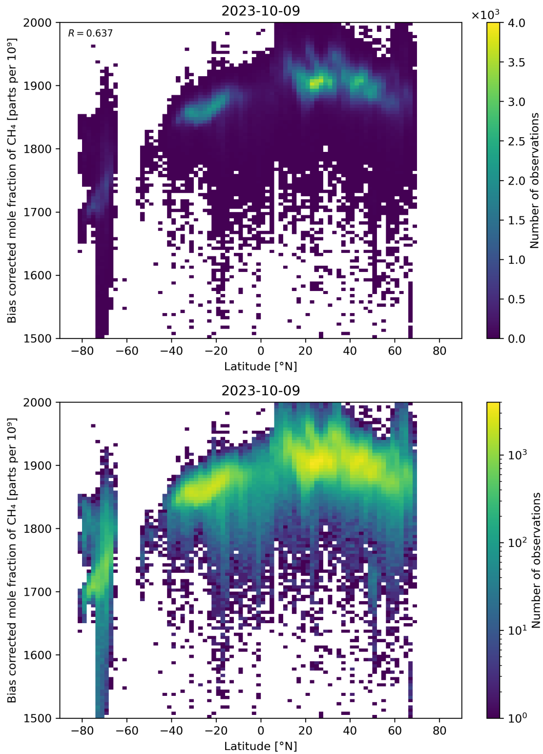
Figure 58: Scatter density plot of “Latitude” against “Bias corrected mole fraction of \text{CH}_4 ” for 2023-10-08 to 2023-10-10.
