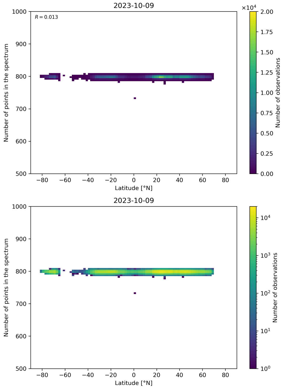
Figure 61: Scatter density plot of “Latitude” against “Number of points in the spectrum” for 2023-10-08 to 2023-10-10.
