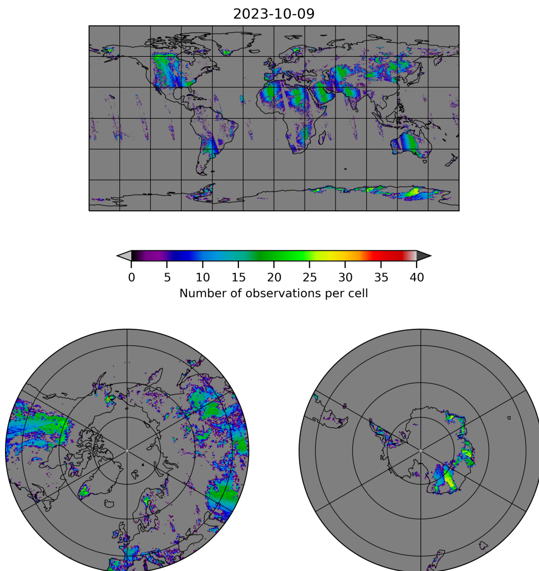
Figure 10: Map of the number of observations for 2023-10-08 to 2023-10-10
