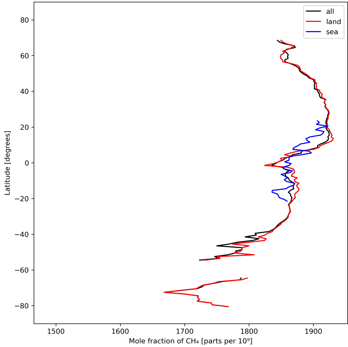
Figure 12: Zonal average of “Mole fraction of \text{CH}_4 ” for 2023-10-08 to 2023-10-10.
