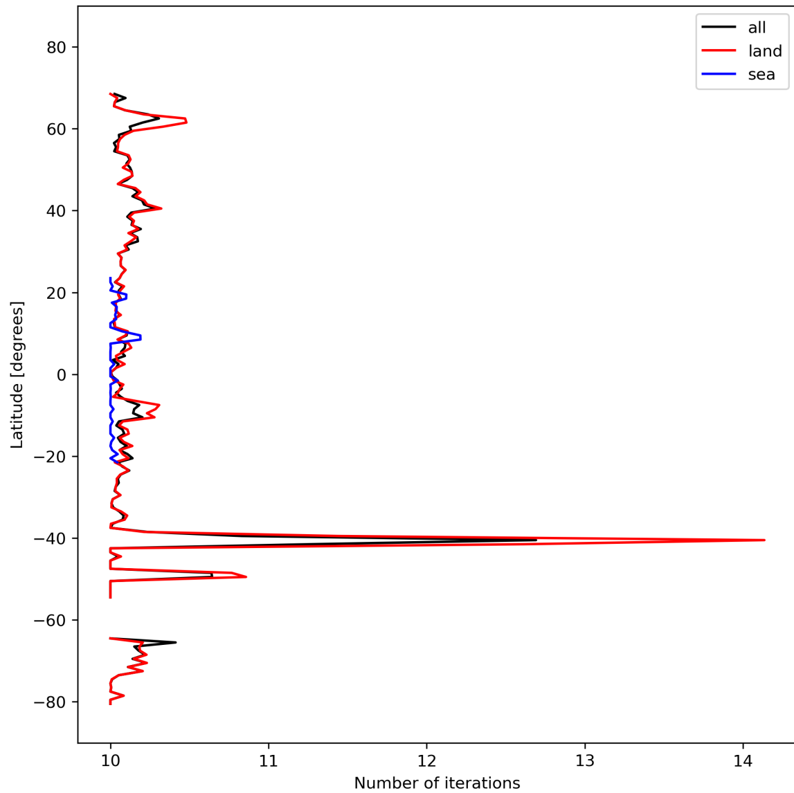
Figure 20: Zonal average of “Number of iterations” for 2023-10-08 to 2023-10-10.
