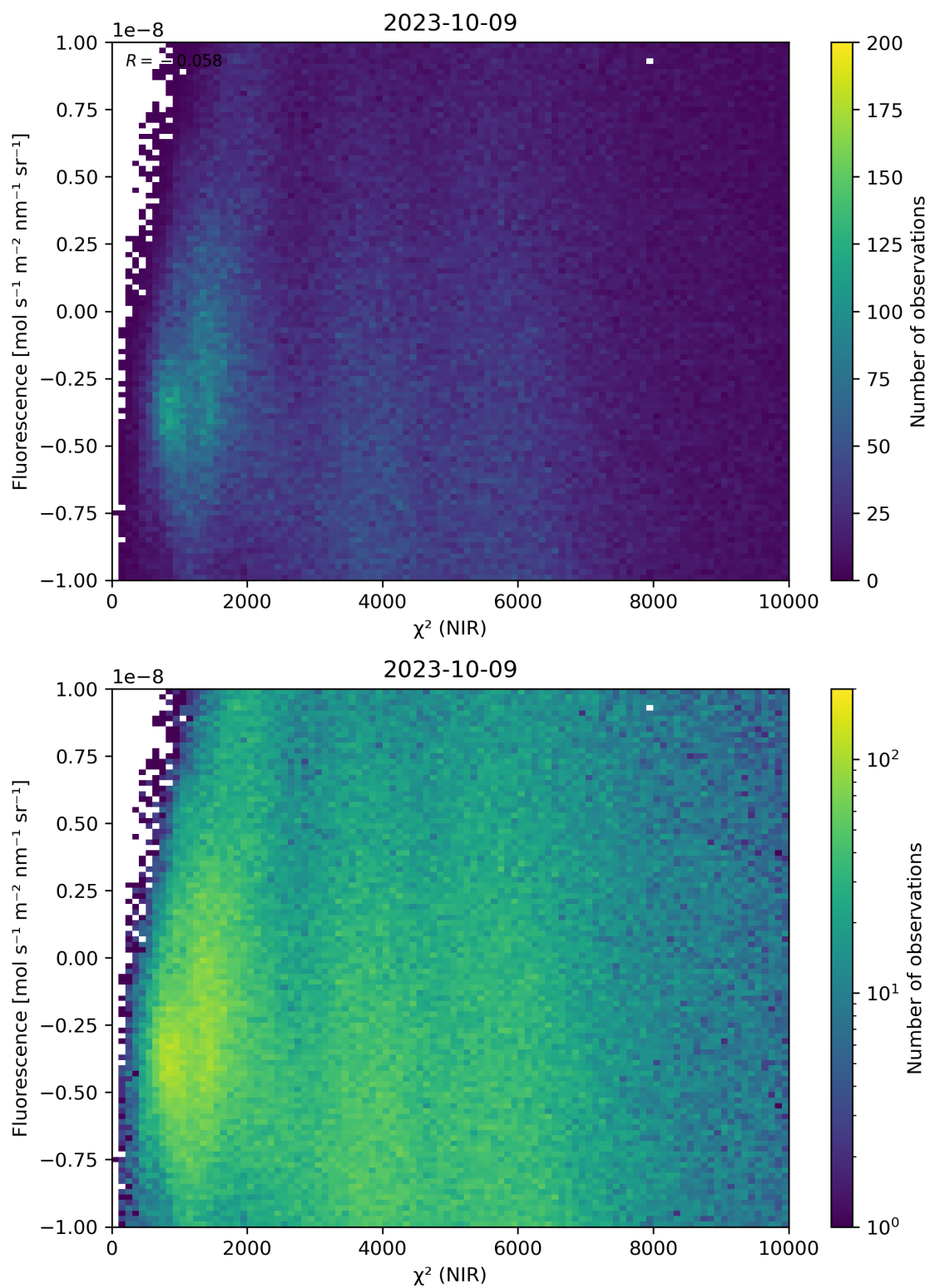
Figure 45: Scatter density plot of “ \chi^2 (NIR)” against “Fluorescence” for 2023-10-08 to 2023-10-10.
