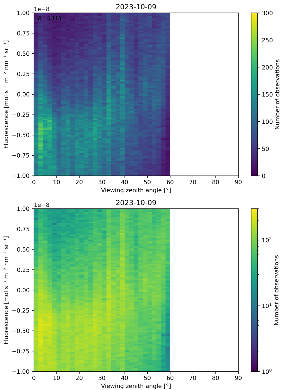
Figure 108: Scatter density plot of “Viewing zenith angle” against “Fluorescence” for 2023-10-08 to 2023-10-10.
