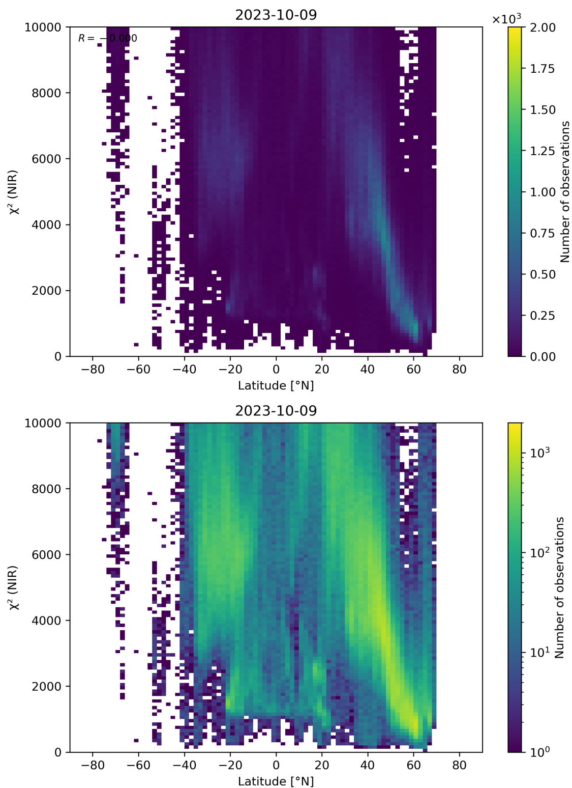
Figure 53: Scatter density plot of “Latitude” against “ \chi^2 (NIR)” for 2023-10-08 to 2023-10-10.
