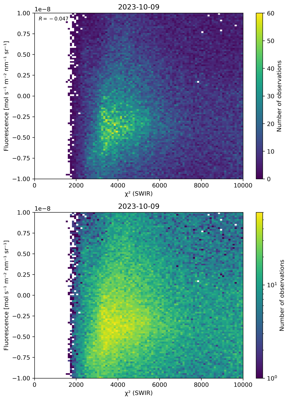
Figure 49: Scatter density plot of “ \chi^2 (SWIR)” against “Fluorescence” for 2023-10-08 to 2023-10-10.
