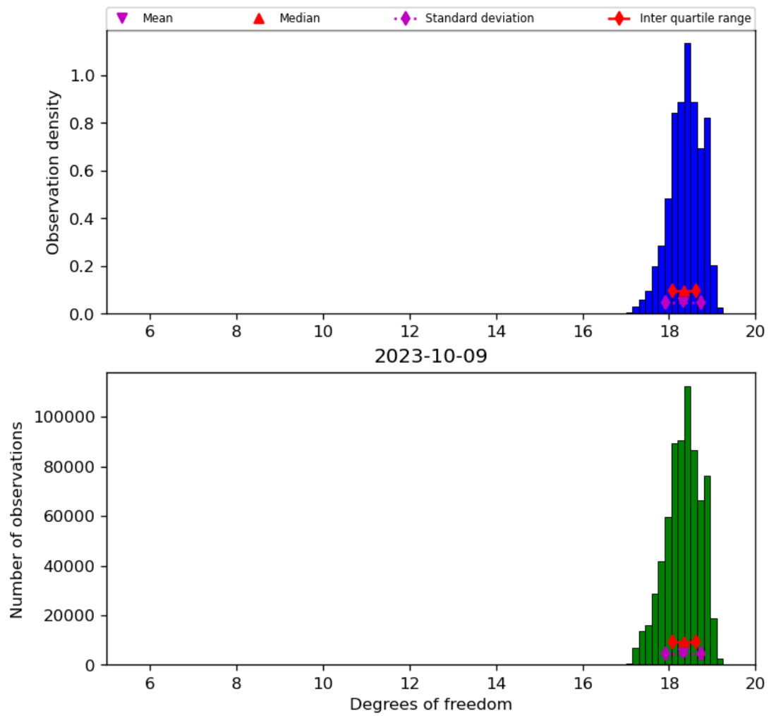
Figure 30: Histogram of “Degrees of freedom” for 2023-10-08 to 2023-10-10
