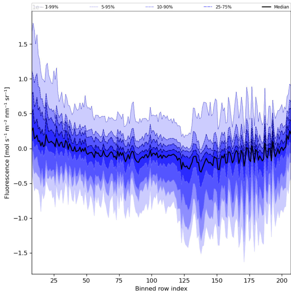
Figure 43: Along track statistics of “Fluorescence” for 2023-10-08 to 2023-10-10
