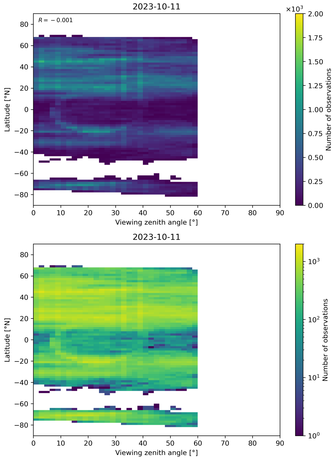
Figure 109: Scatter density plot of “Viewing zenith angle” against “Latitude” for 2023-10-10 to 2023-10-12.
