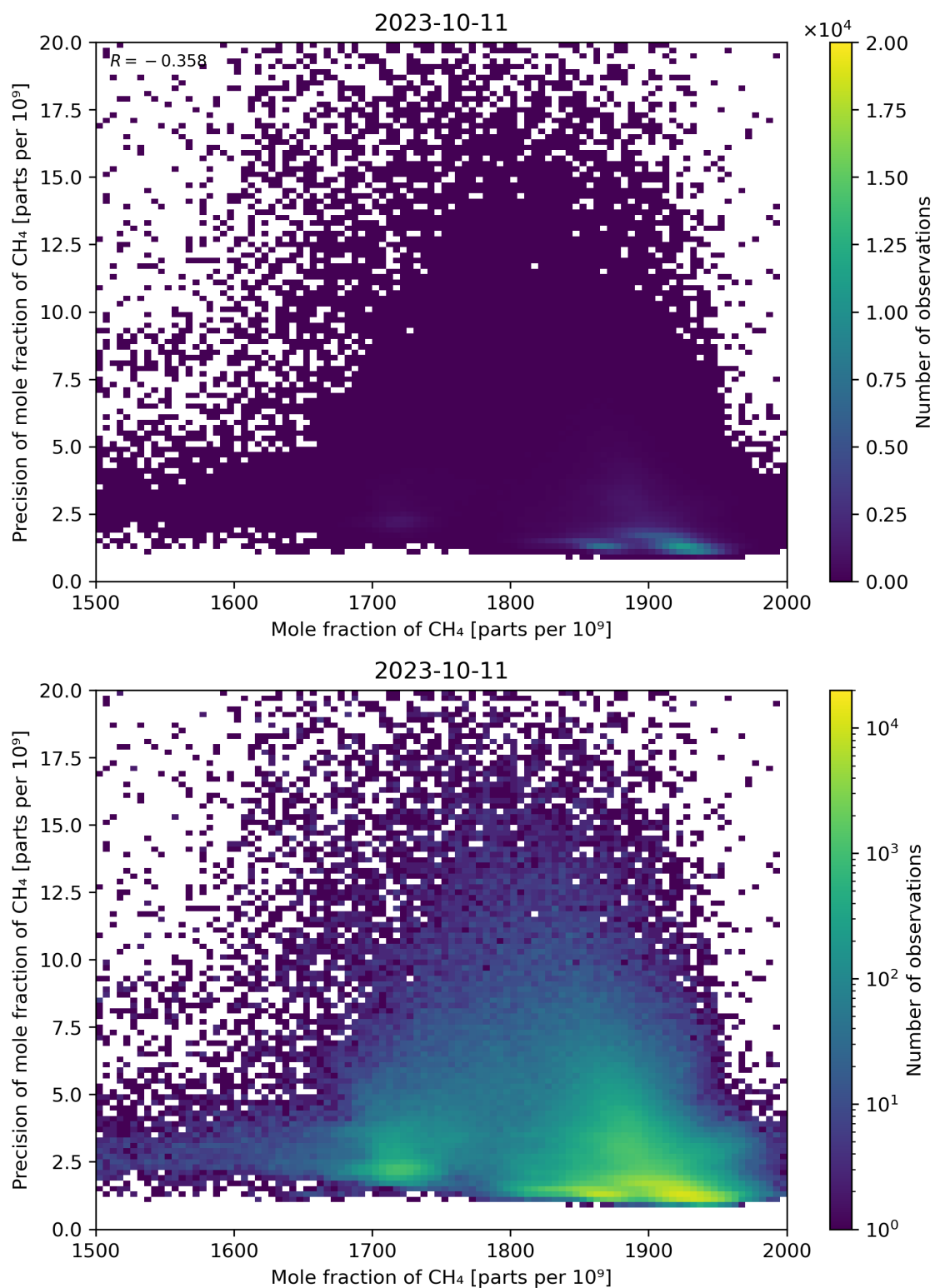
Figure 75: Scatter density plot of “Mole fraction of CH 4 ” against “Precision of mole fraction of CH 4 ” for 2023-10-10 to 2023-10-12.
