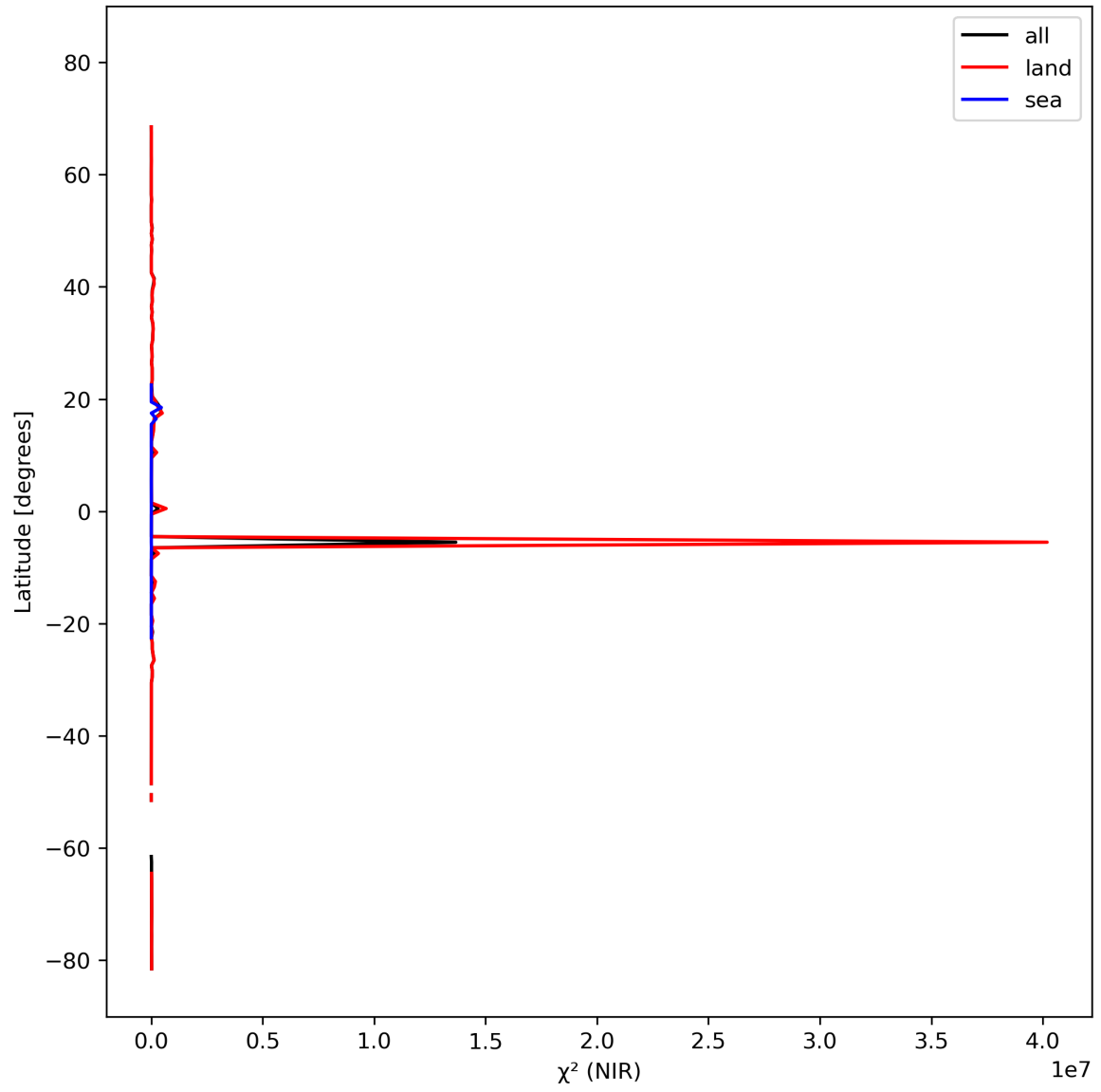
Figure 18: Zonal average of “ \chi^2 (NIR)” for 2023-10-10 to 2023-10-12.
