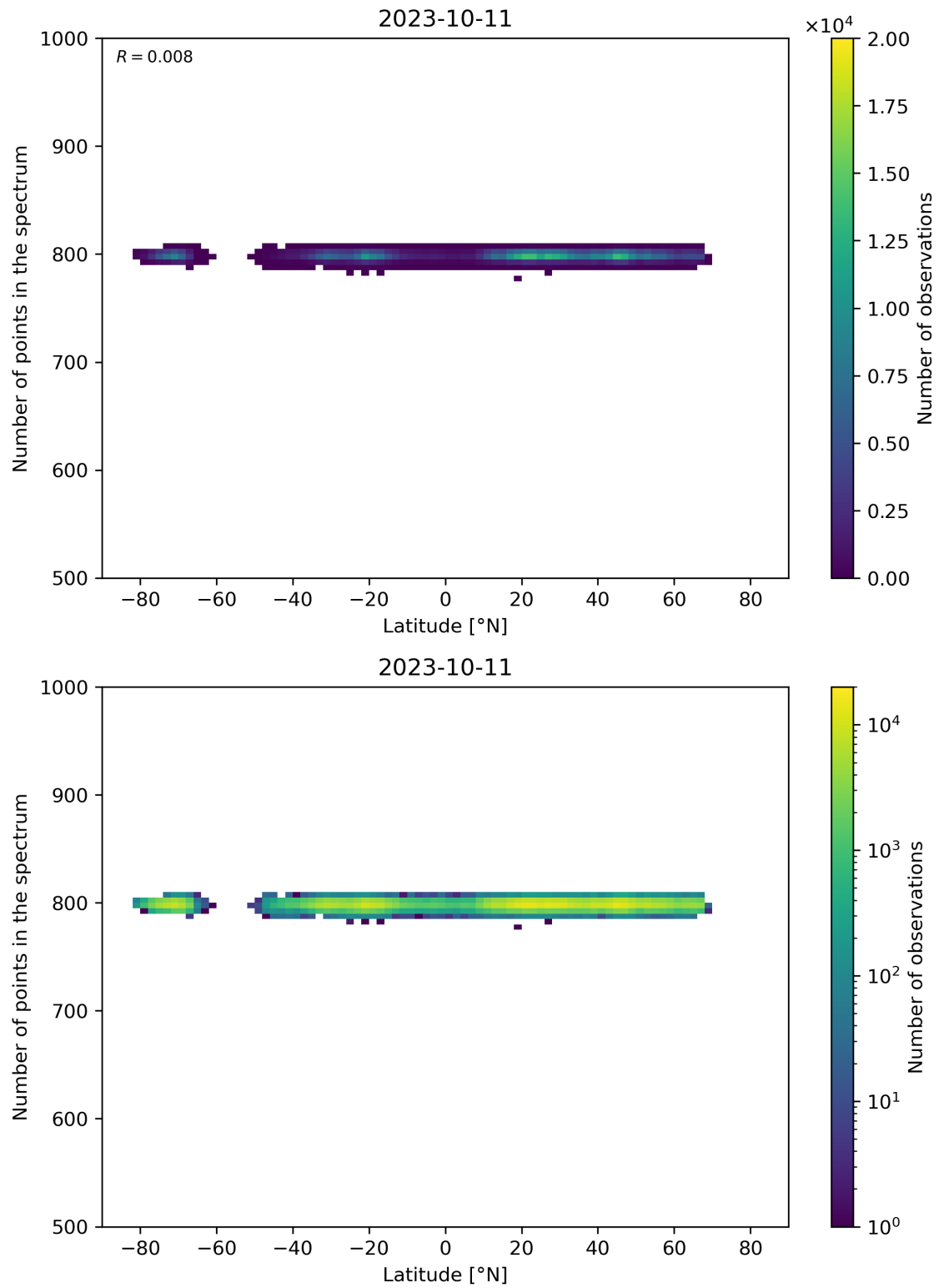
Figure 61: Scatter density plot of “Latitude” against “Number of points in the spectrum” for 2023-10-10 to 2023-10-12.
