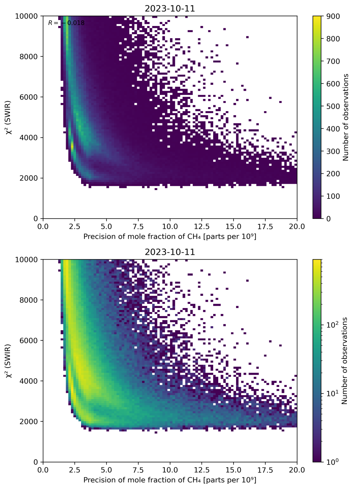
Figure 79: Scatter density plot of “Precision of mole fraction of \text{CH}_4 ” against “ \chi^2 (SWIR)” for 2023-10-10 to 2023-10-12.
