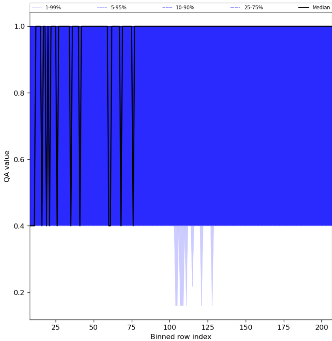
Figure 33: Along track statistics of “QA value” for 2023-10-10 to 2023-10-12
