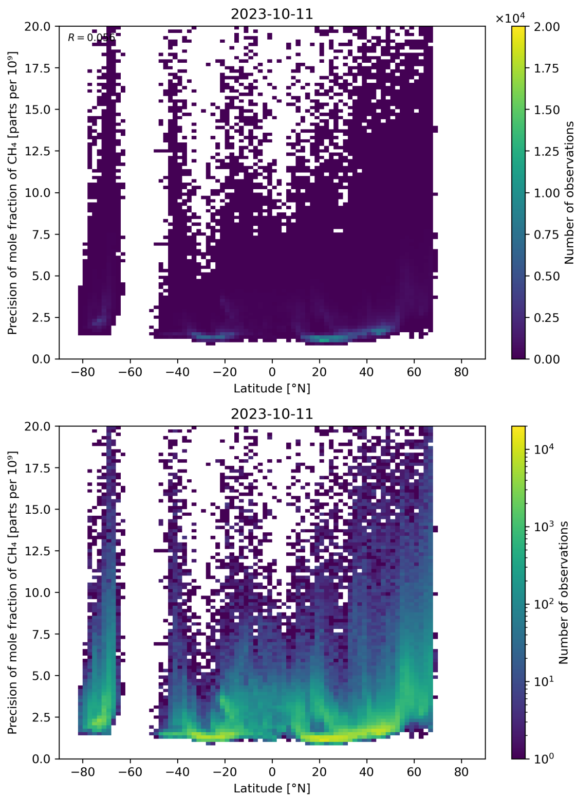
Figure 59: Scatter density plot of “Latitude” against “Precision of mole fraction of \text{CH}_4 ” for 2023-10-10 to 2023-10-12.
