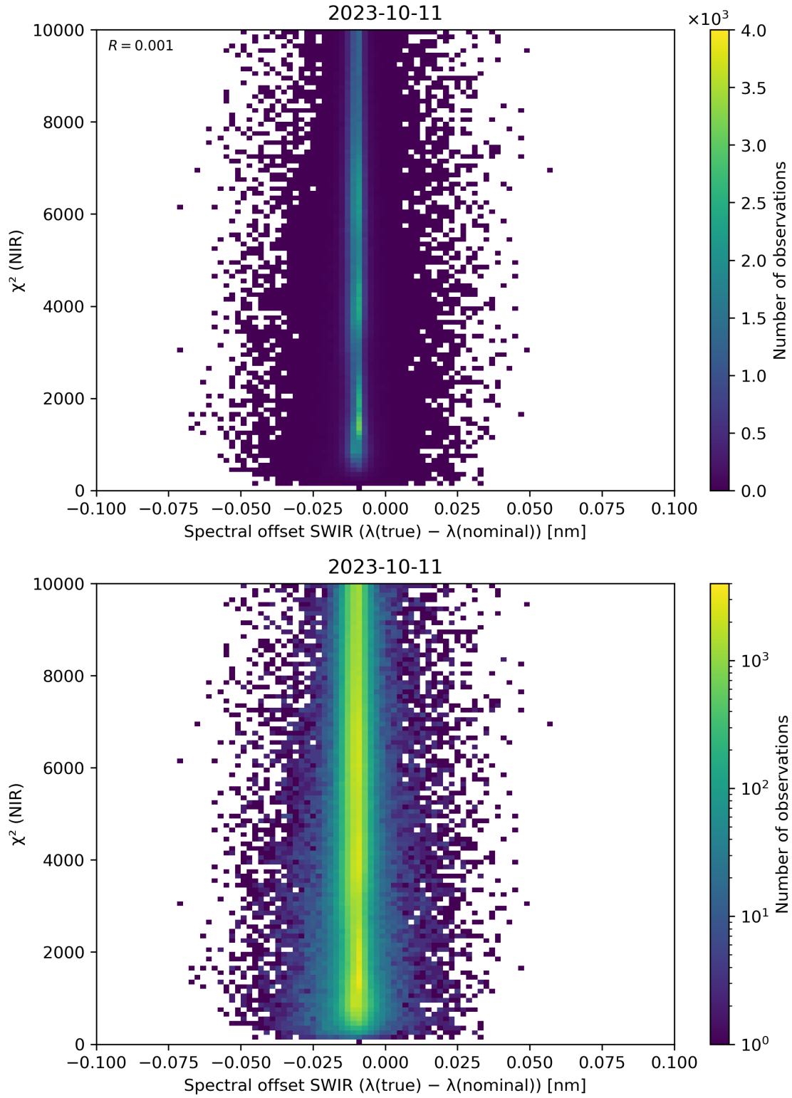
Figure 117: Scatter density plot of “Spectral offset SWIR ( \lambda(\text{true}) - \lambda(\text{nominal}) )” against “ \chi^2 (NIR)” for 2023-10-10 to 2023-10-12.
