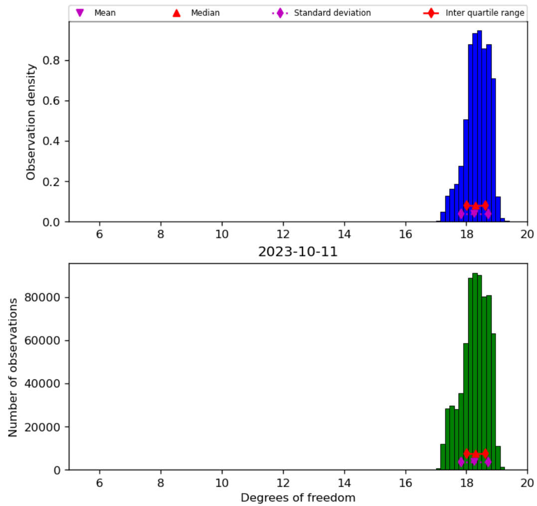
Figure 30: Histogram of “Degrees of freedom” for 2023-10-10 to 2023-10-12
