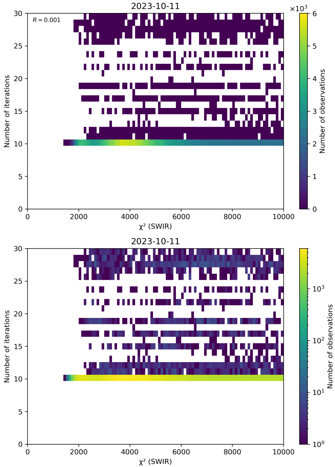
Figure 50: Scatter density plot of “ \chi^2 (SWIR)” against “Number of iterations” for 2023-10-10 to 2023-10-12.
