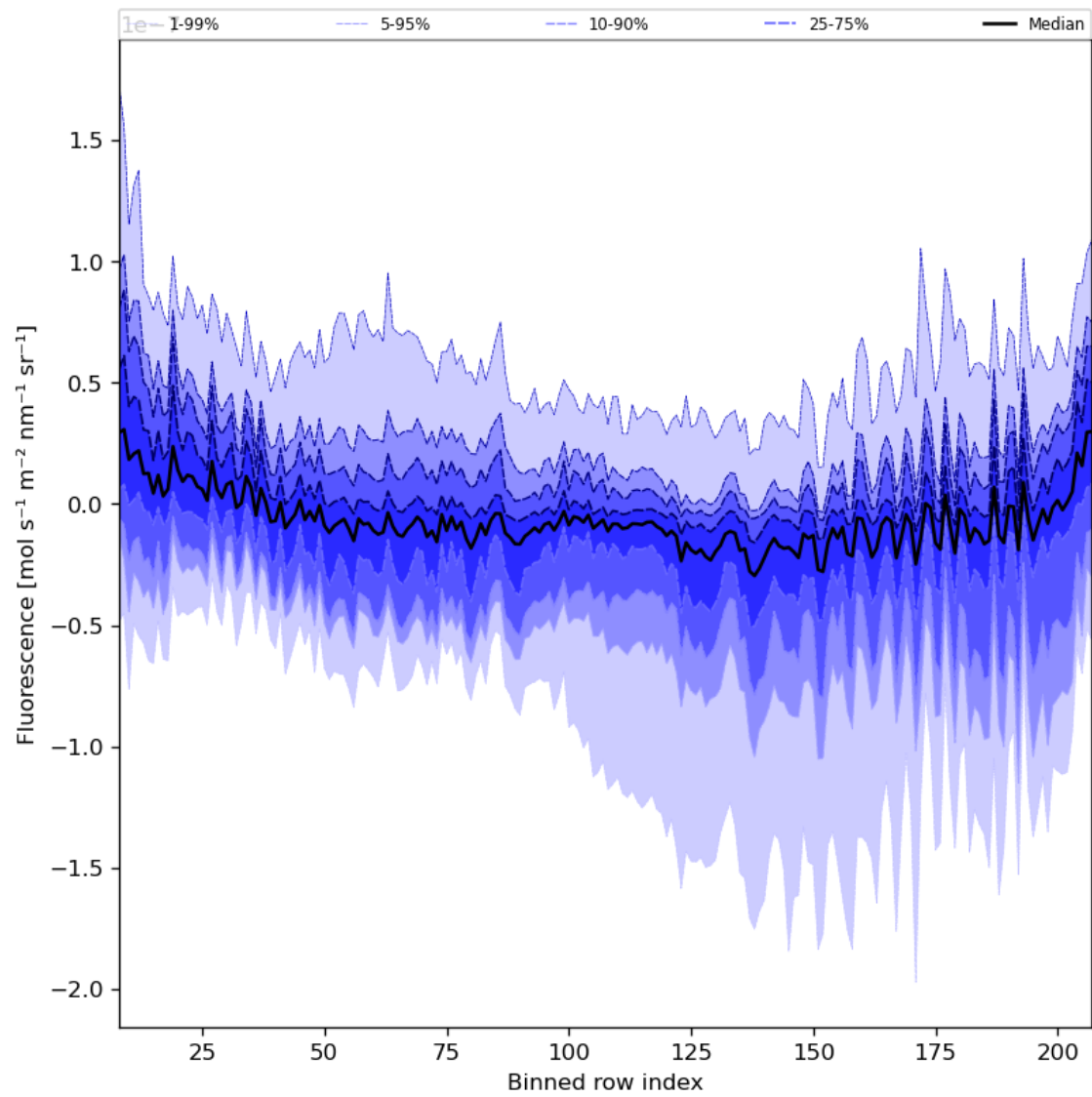
Figure 43: Along track statistics of “Fluorescence” for 2023-10-10 to 2023-10-12
