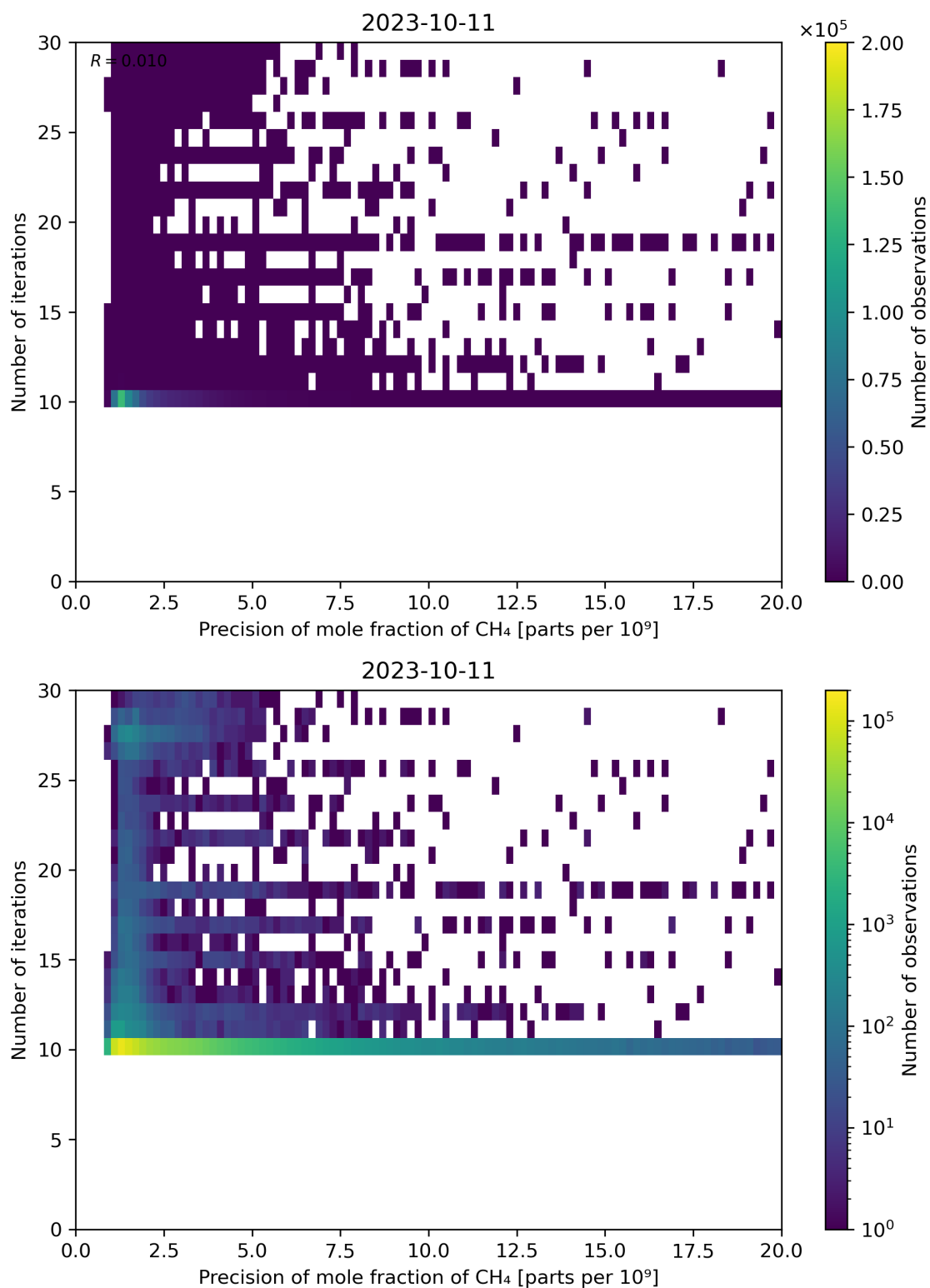
Figure 83: Scatter density plot of “Precision of mole fraction of CH 4 ” against “Number of iterations” for 2023-10-10 to 2023-10-12.
