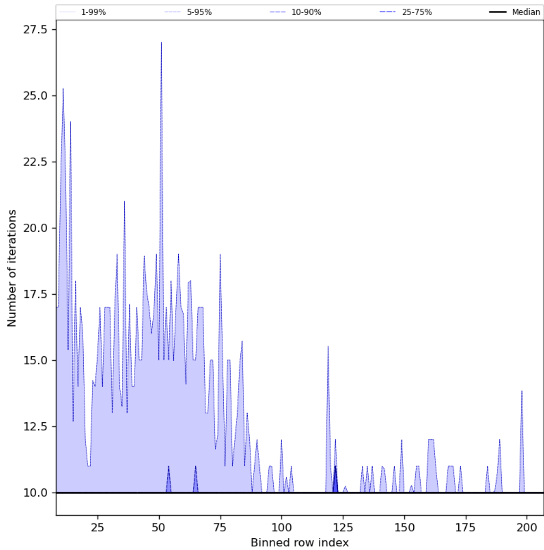
Figure 42: Along track statistics of “Number of iterations” for 2023-10-10 to 2023-10-12
