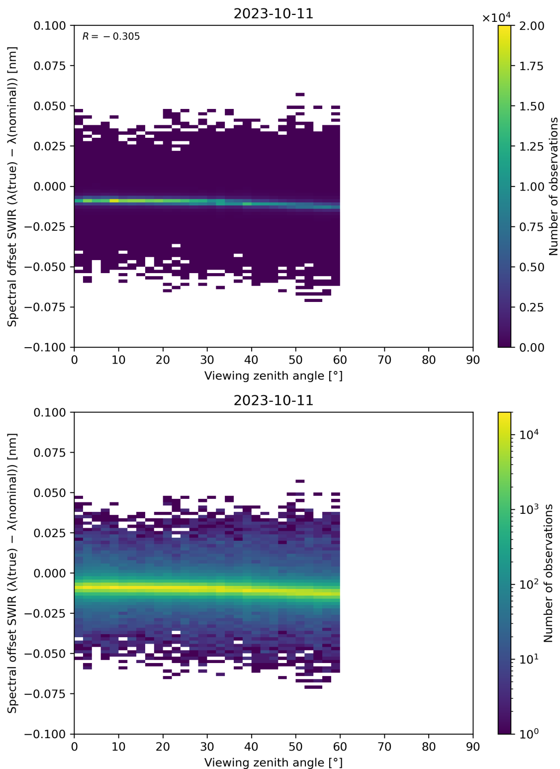
Figure 116: Scatter density plot of “Viewing zenith angle” against “Spectral offset SWIR ( \lambda(\text{true}) - \lambda(\text{nominal}) )” for 2023-10-10 to 2023-10-12.
