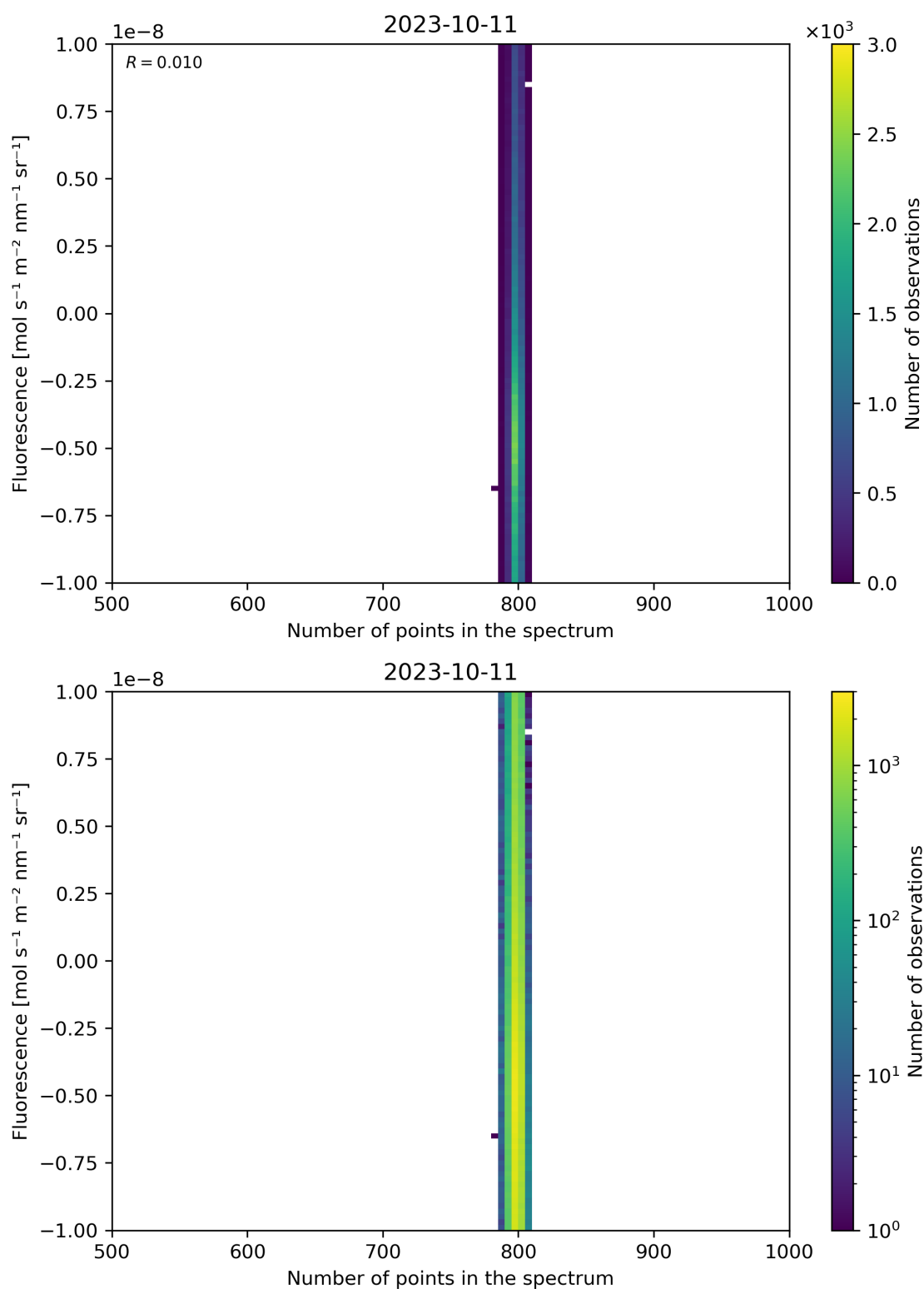
Figure 91: Scatter density plot of “Number of points in the spectrum” against “Fluorescence” for 2023-10-10 to 2023-10-12.
