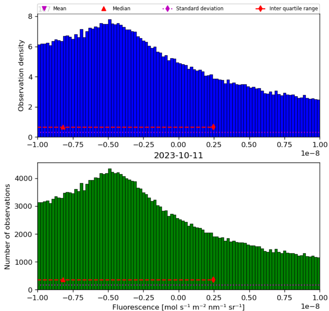
Figure 32: Histogram of “Fluorescence” for 2023-10-10 to 2023-10-12
