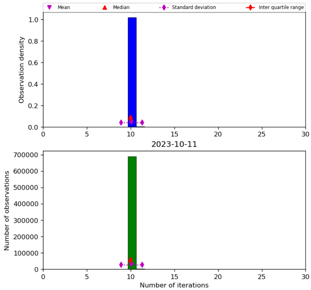
Figure 31: Histogram of “Number of iterations” for 2023-10-10 to 2023-10-12
