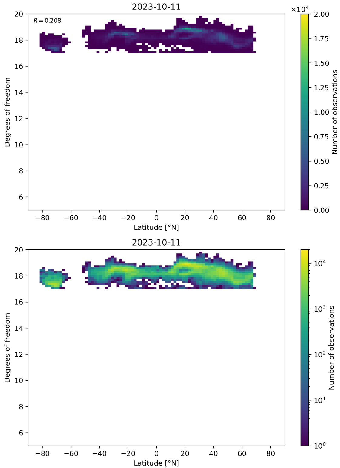
Figure 55: Scatter density plot of “Latitude” against “Degrees of freedom” for 2023-10-10 to 2023-10-12.
