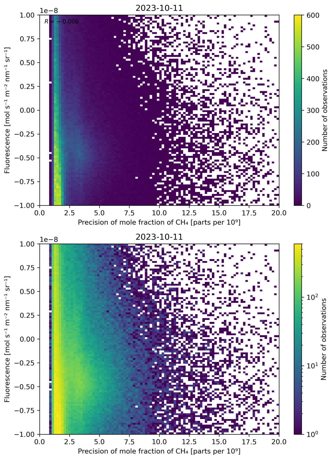
Figure 81: Scatter density plot of “Precision of mole fraction of \text{CH}_4 ” against “Fluorescence” for 2023-10-10 to 2023-10-12.
