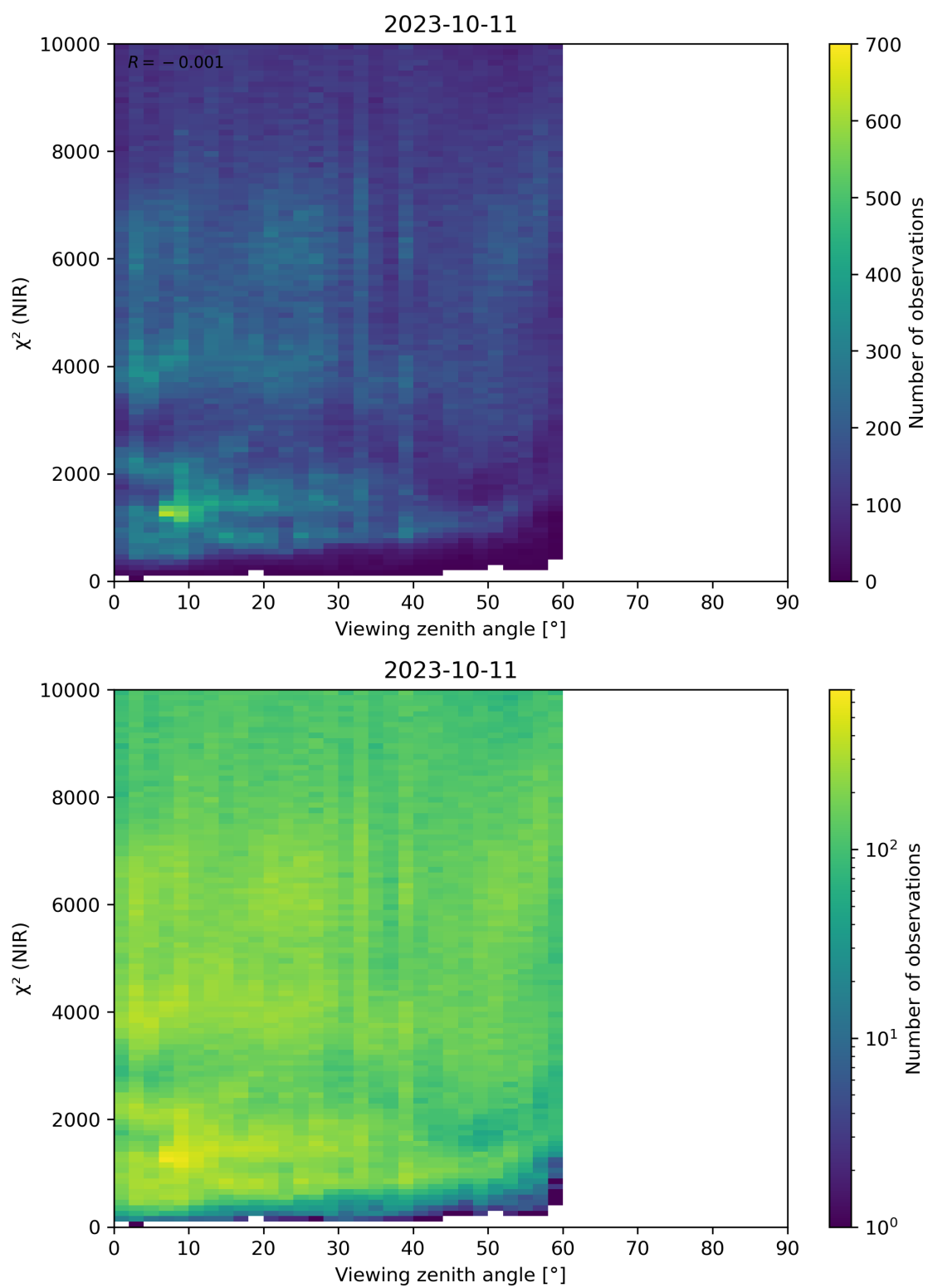
Figure 105: Scatter density plot of “Viewing zenith angle” against “ \chi^2 (NIR)” for 2023-10-10 to 2023-10-12.
