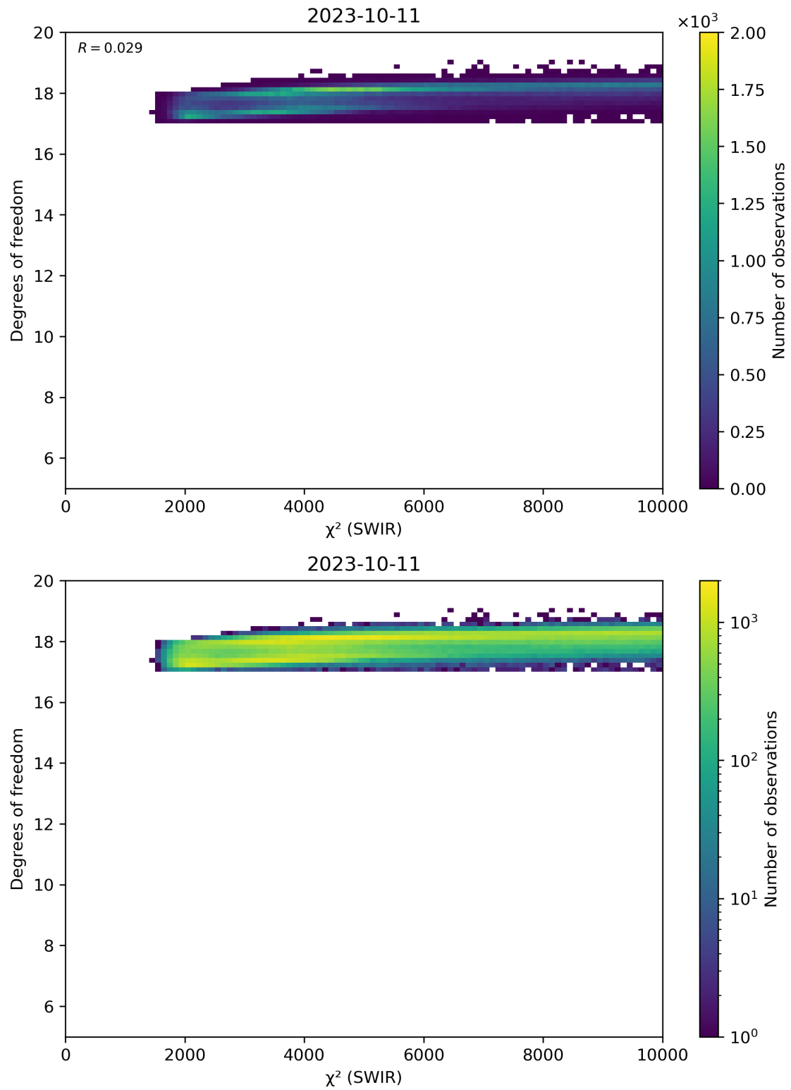
Figure 48: Scatter density plot of “ \chi^2 (SWIR)” against “Degrees of freedom” for 2023-10-10 to 2023-10-12.
