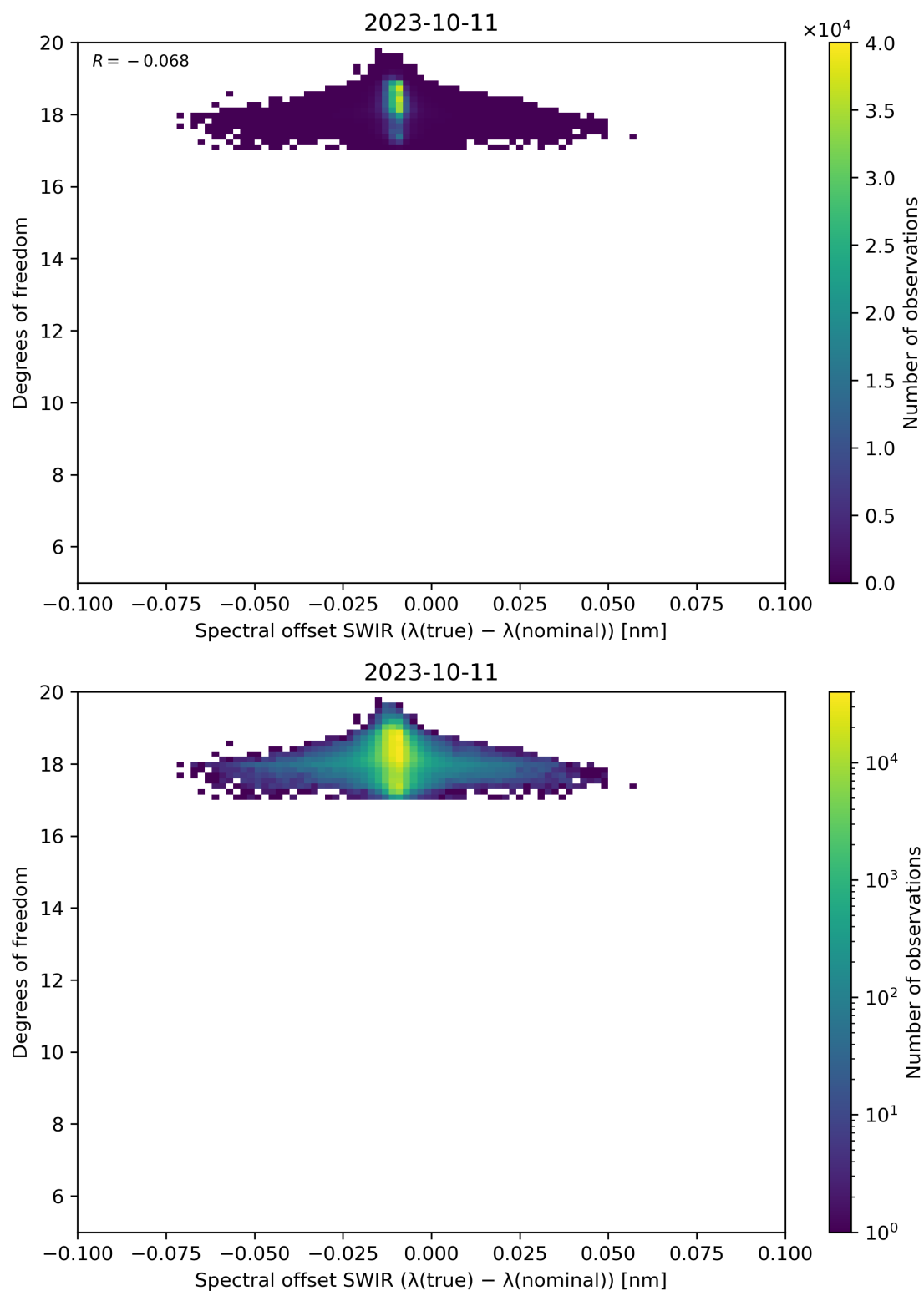
Figure 119: Scatter density plot of “Spectral offset SWIR ( \lambda(\text{true}) - \lambda(\text{nominal}) )” against “Degrees of freedom” for 2023-10-10 to 2023-10-12.
