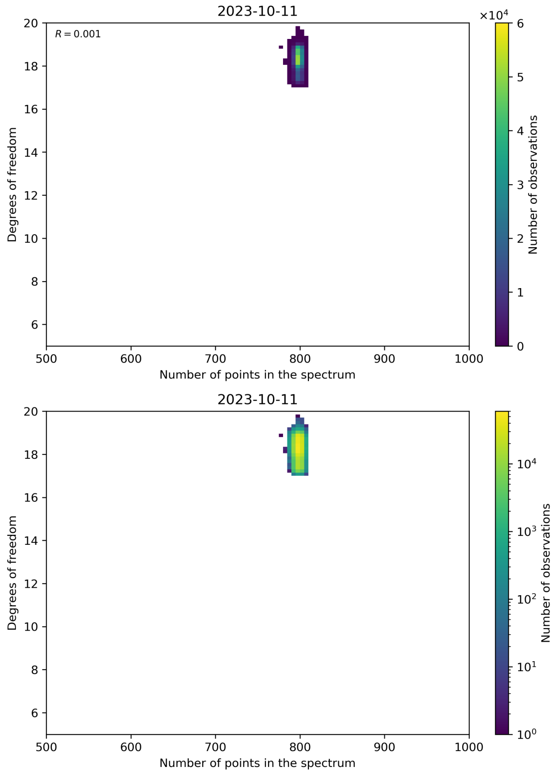
Figure 90: Scatter density plot of “Number of points in the spectrum” against “Degrees of freedom” for 2023-10-10 to 2023-10-12.
