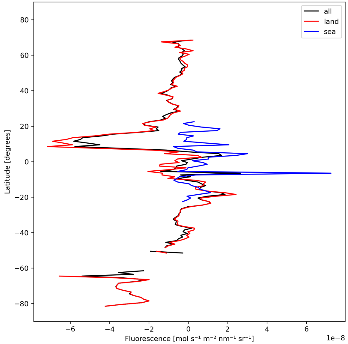
Figure 21: Zonal average of “Fluorescence” for 2023-10-10 to 2023-10-12.
