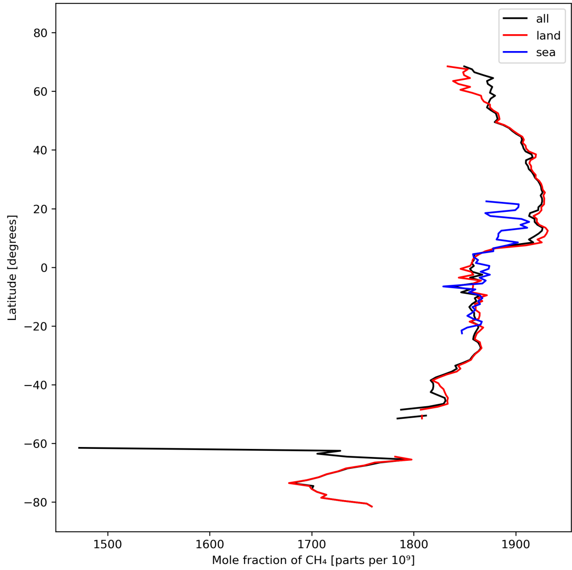
Figure 12: Zonal average of “Mole fraction of \text{CH}_4 ” for 2023-10-10 to 2023-10-12.
