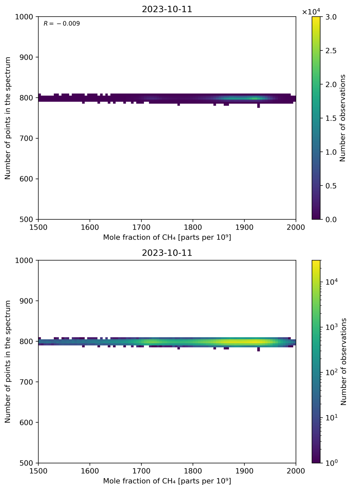
Figure 77: Scatter density plot of “Mole fraction of CH 4 ” against “Number of points in the spectrum” for 2023-10-10 to 2023-10-12.
