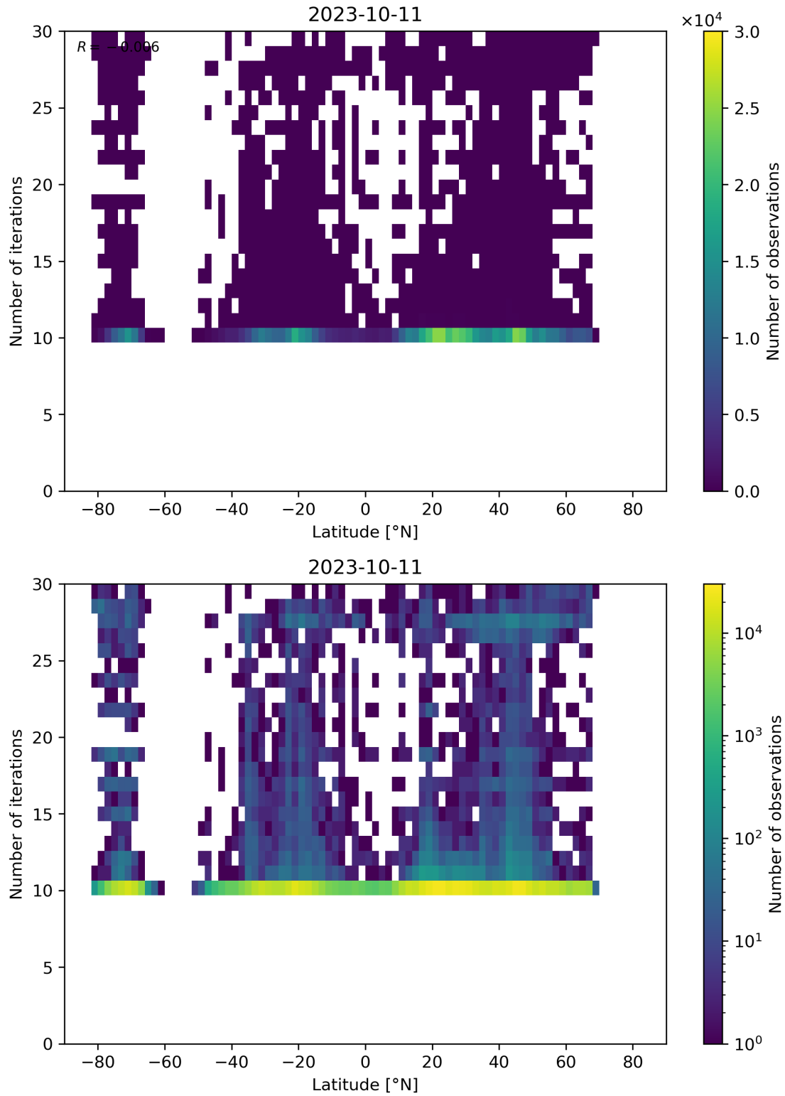
Figure 60: Scatter density plot of “Latitude” against “Number of iterations” for 2023-10-10 to 2023-10-12.
