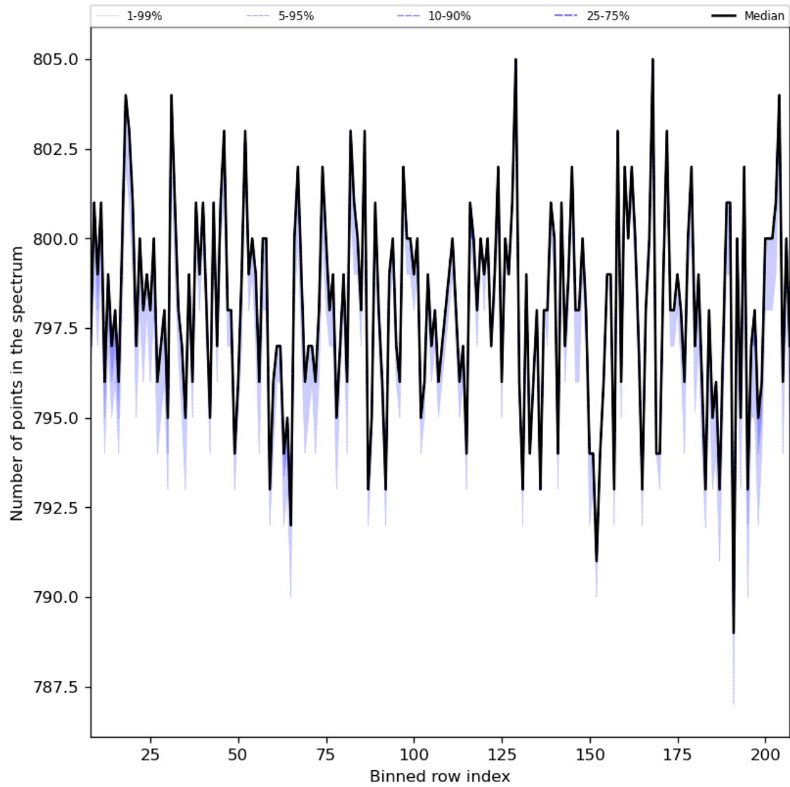
Figure 37: Along track statistics of “Number of points in the spectrum” for 2023-10-10 to 2023-10-12
