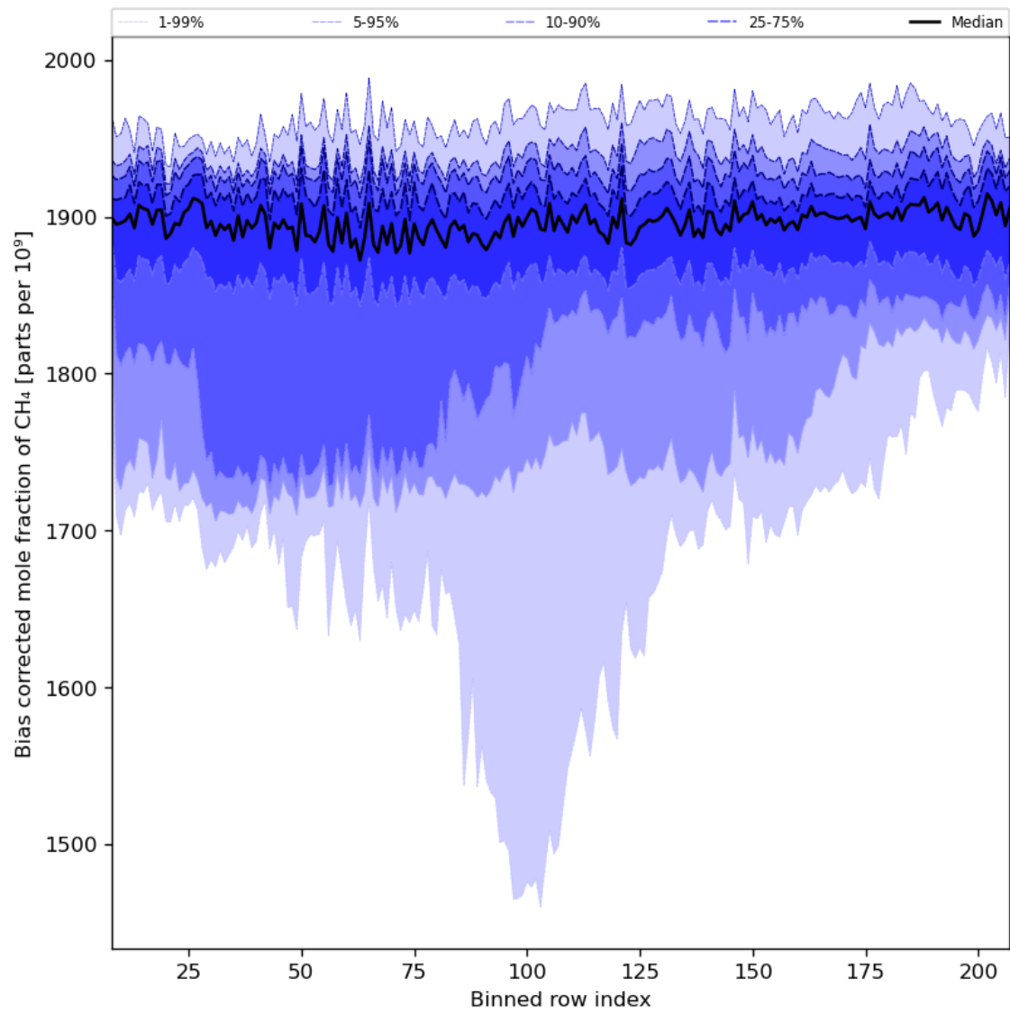
Figure 36: Along track statistics of “Bias corrected mole fraction of CH 4 ” for 2023-10-10 to 2023-10-12
