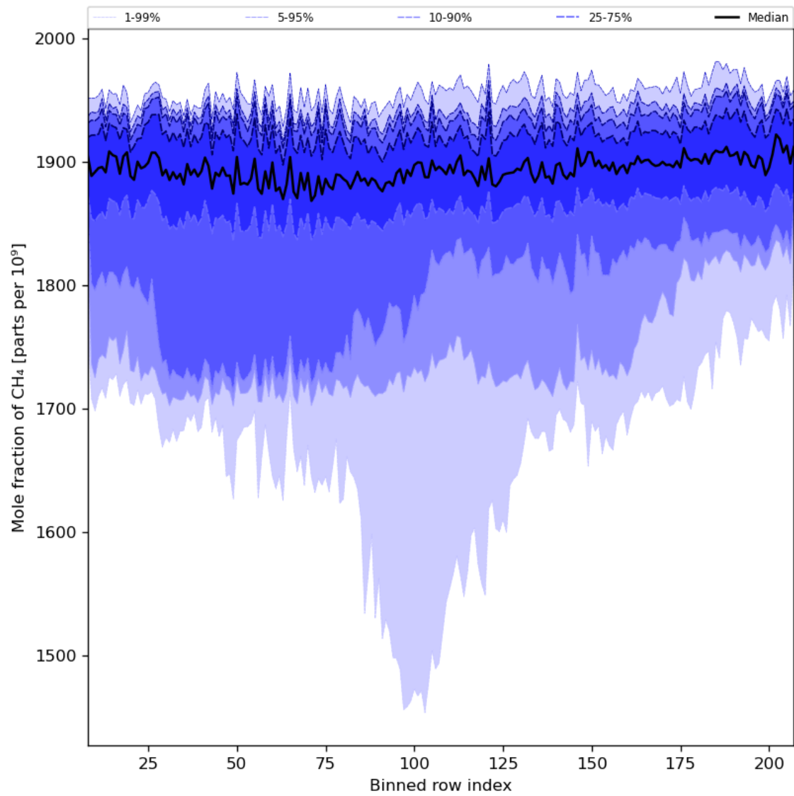
Figure 34: Along track statistics of “Mole fraction of CH 4 ” for 2023-10-10 to 2023-10-12
