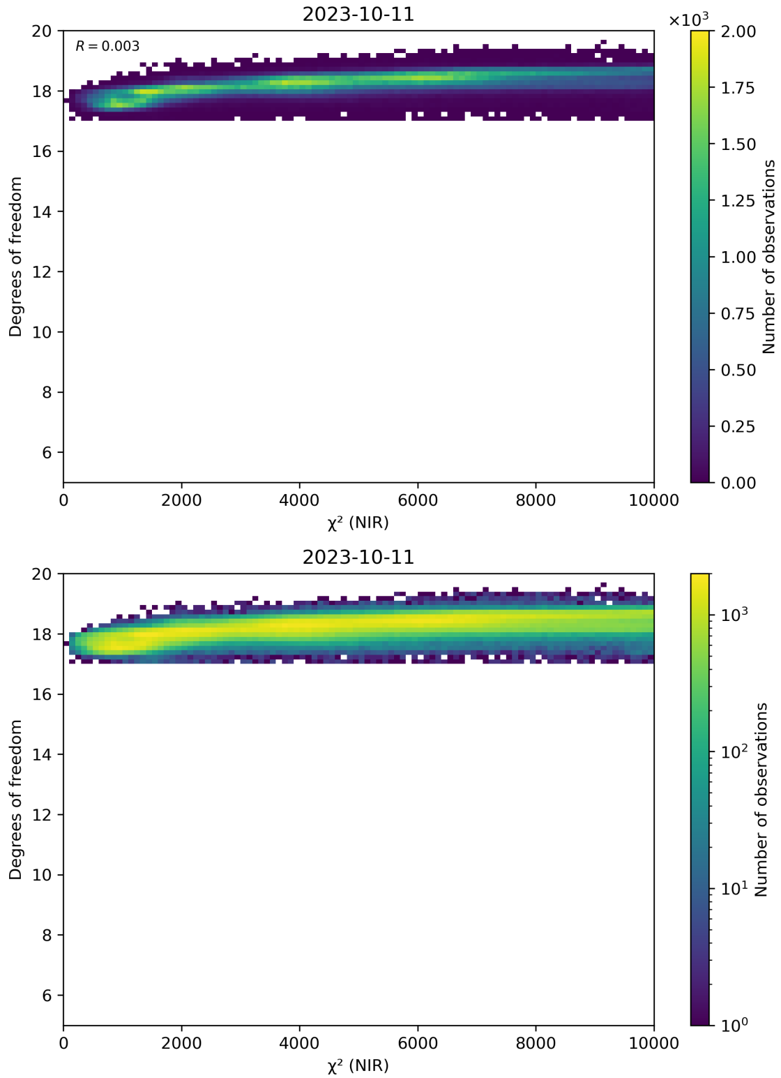
Figure 44: Scatter density plot of “ \chi^2 (NIR)” against “Degrees of freedom” for 2023-10-10 to 2023-10-12.
