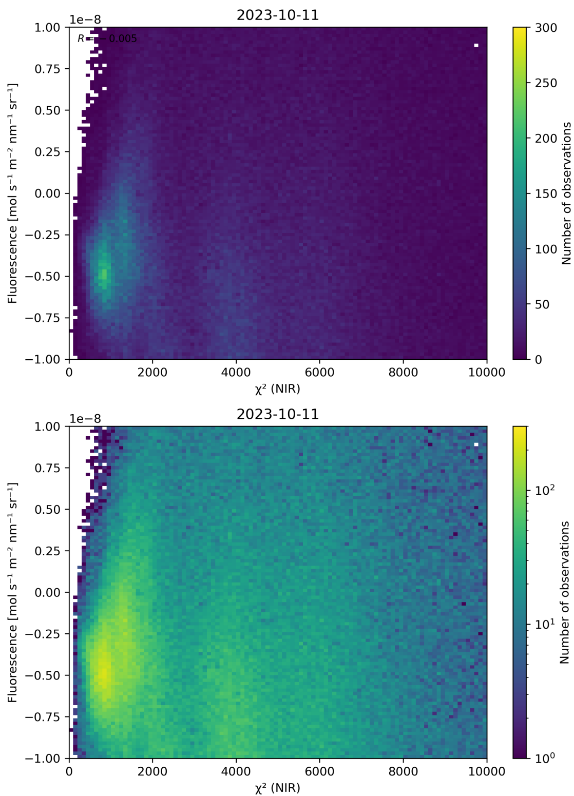
Figure 45: Scatter density plot of “ \chi^2 (NIR)” against “Fluorescence” for 2023-10-10 to 2023-10-12.
