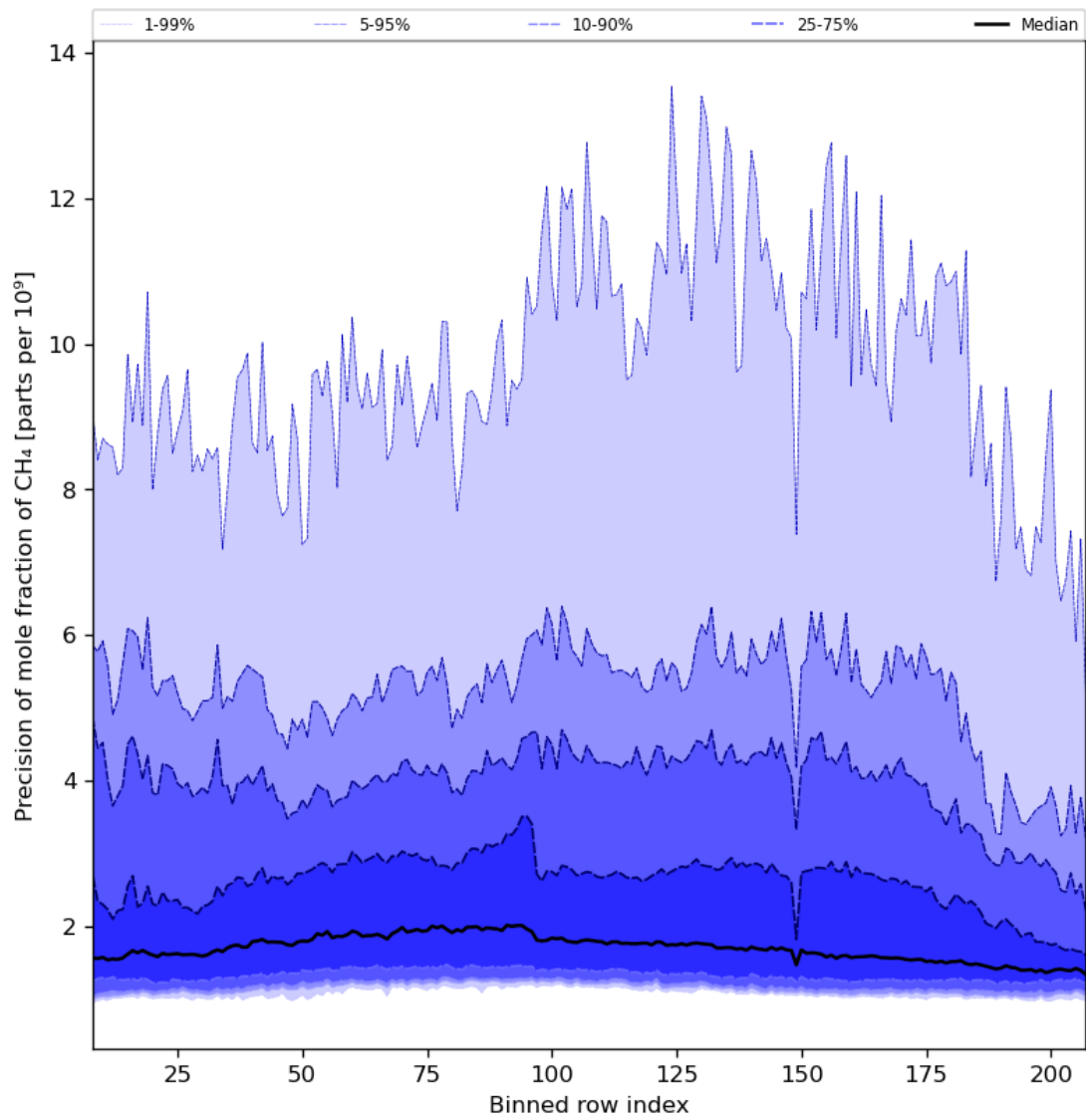
Figure 35: Along track statistics of “Precision of mole fraction of CH 4 ” for 2023-10-10 to 2023-10-12
