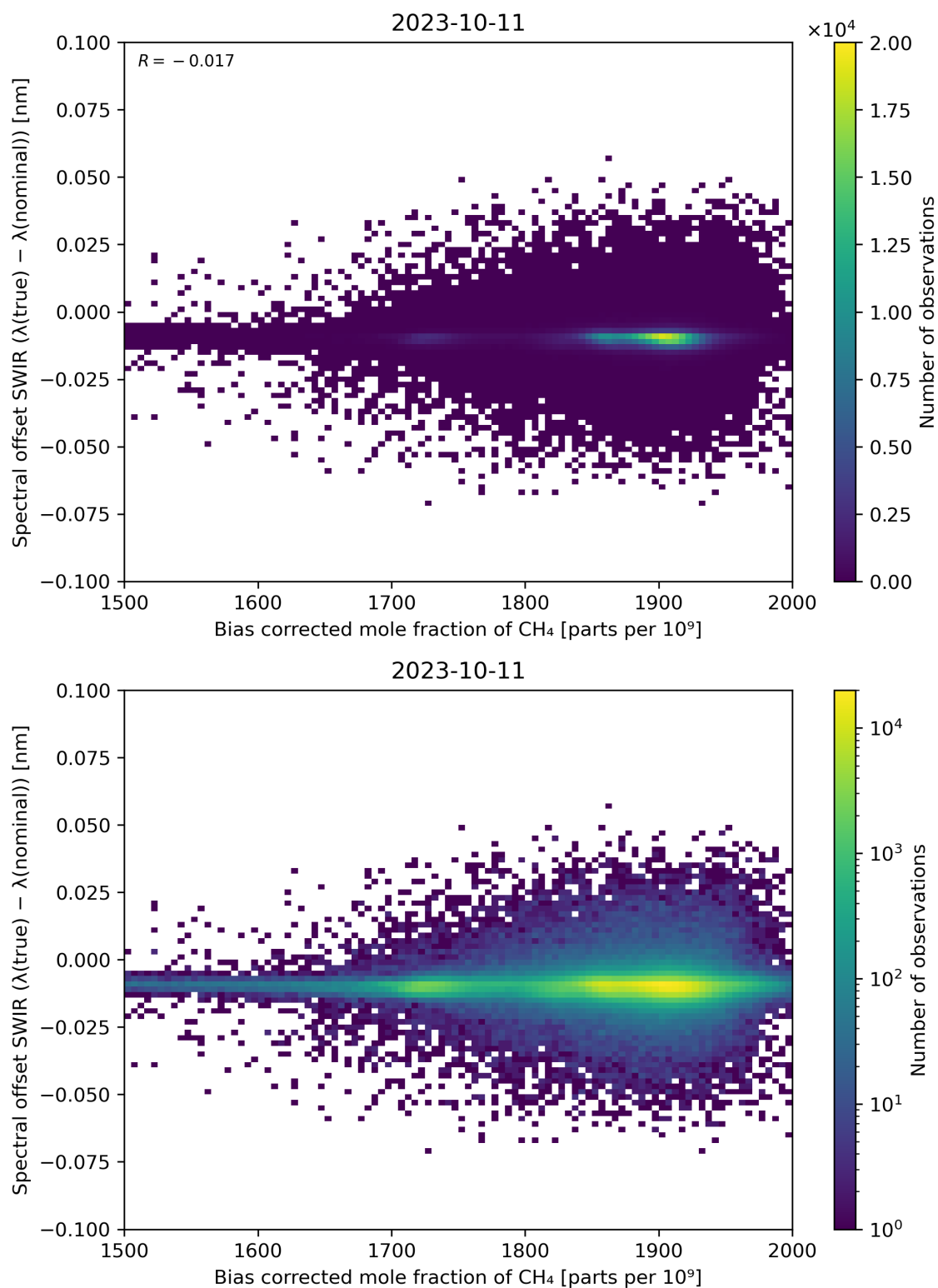
Figure 69: Scatter density plot of “Bias corrected mole fraction of \text{CH}_4 ” against “Spectral offset SWIR ( \lambda(\text{true}) - \lambda(\text{nominal}) )” for 2023-10-10 to 2023-10-12.
