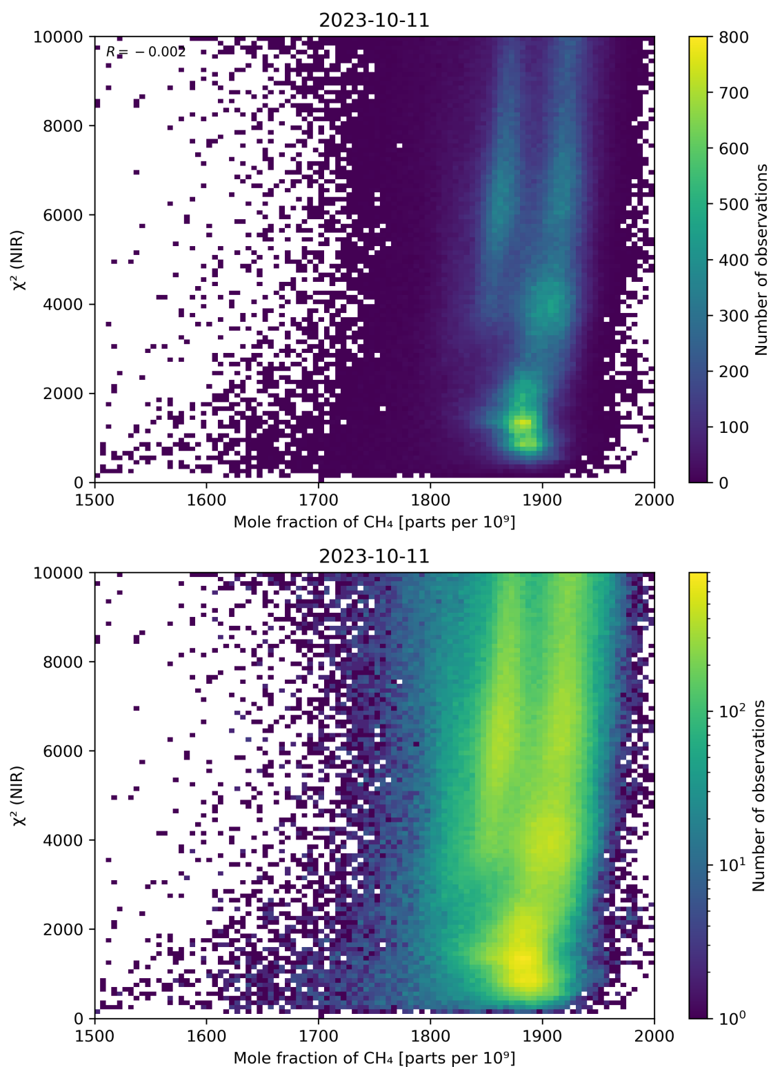
Figure 70: Scatter density plot of “Mole fraction of CH 4 ” against “ \chi^2 (NIR)” for 2023-10-10 to 2023-10-12.
