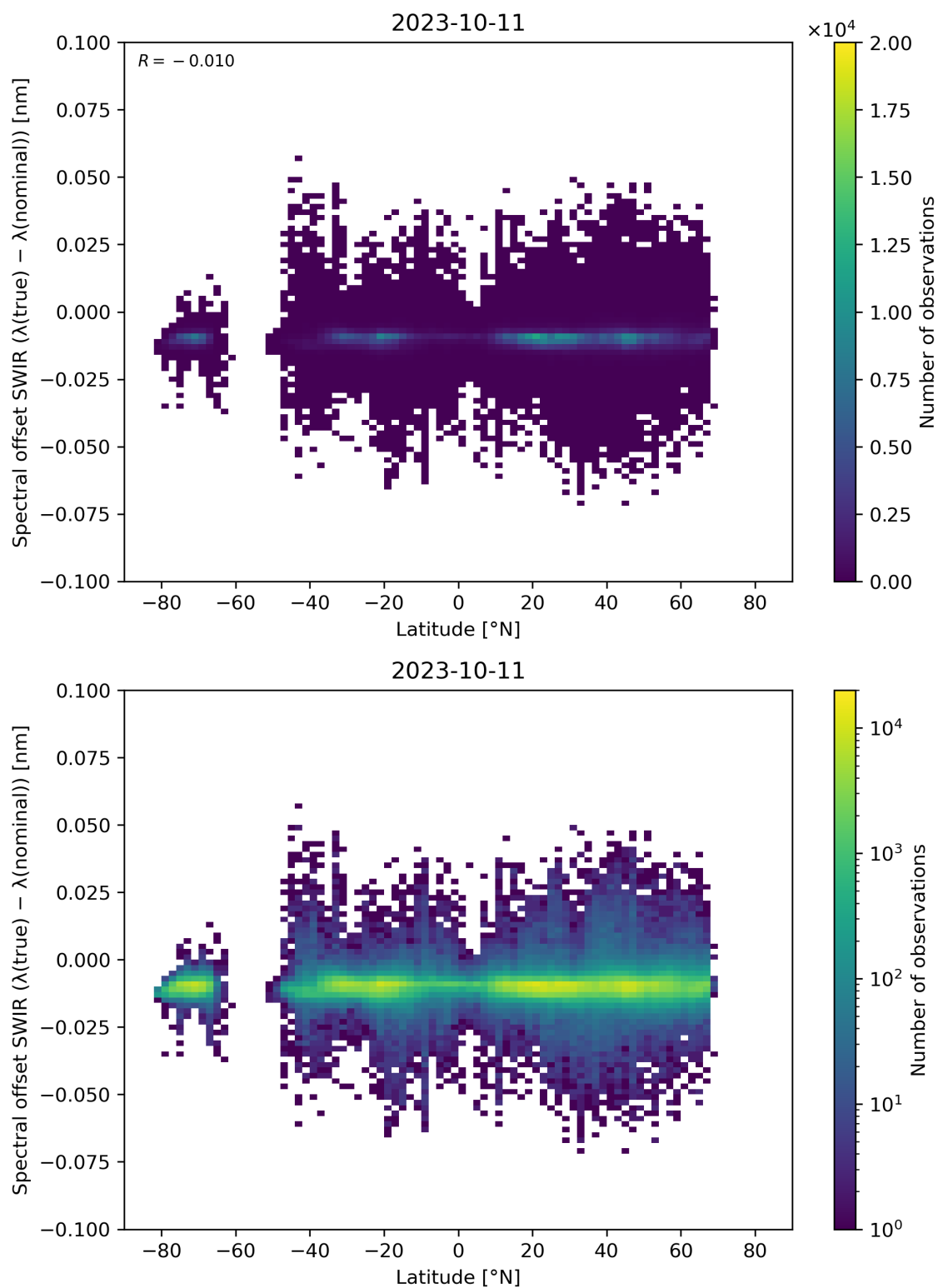
Figure 62: Scatter density plot of “Latitude” against “Spectral offset SWIR ( \lambda(\text{true}) - \lambda(\text{nominal}) )” for 2023-10-10 to 2023-10-12.
