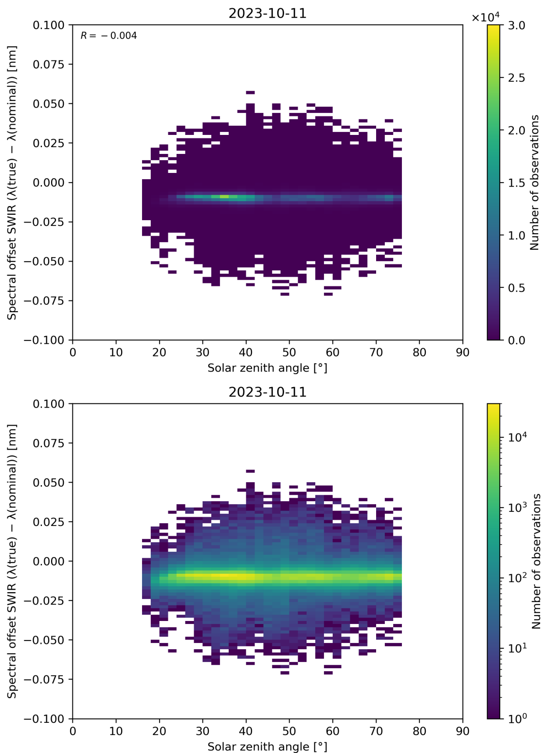
Figure 104: Scatter density plot of “Solar zenith angle” against “Spectral offset SWIR ( \lambda(\text{true}) - \lambda(\text{nominal}) )” for 2023-10-10 to 2023-10-12.
