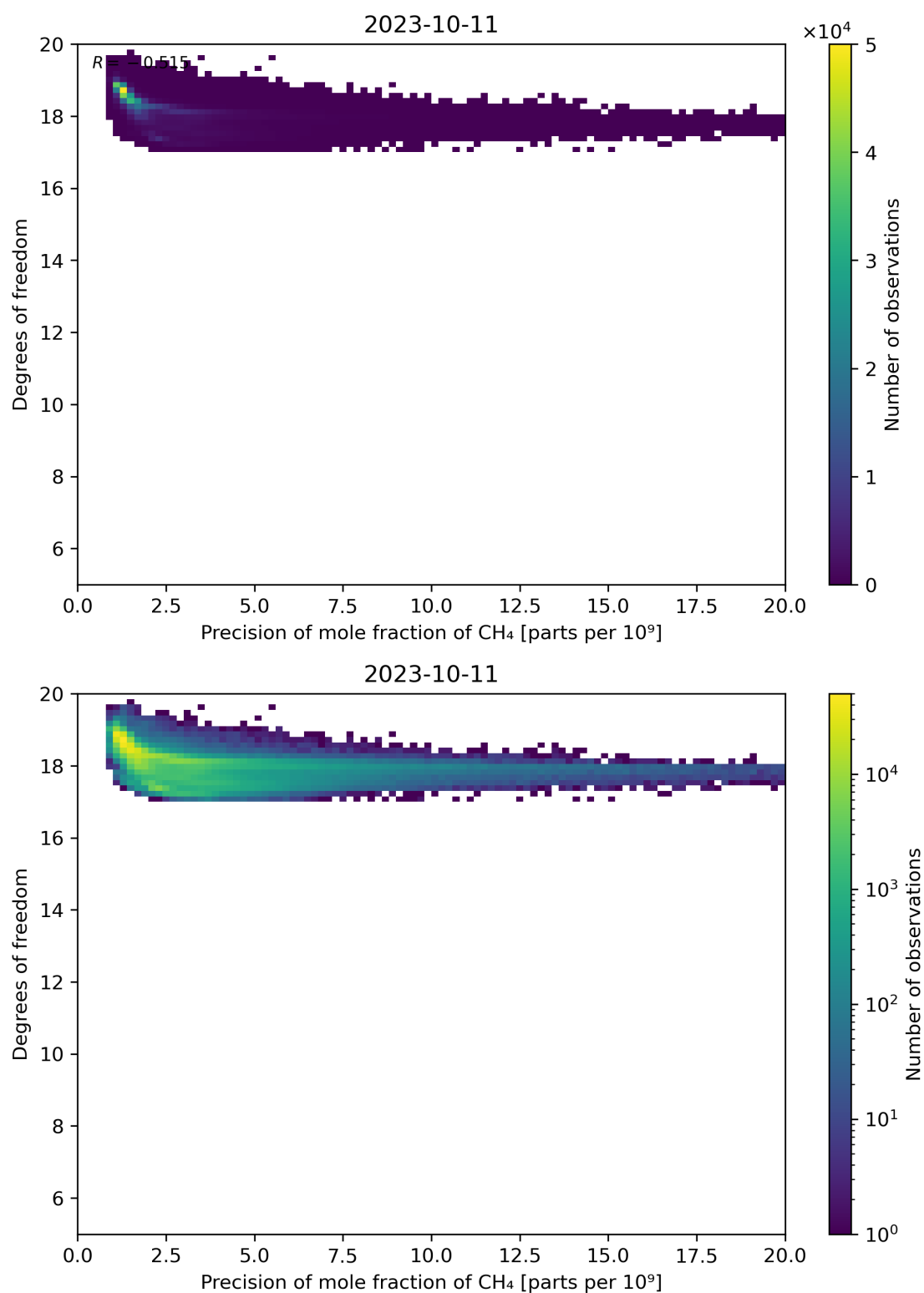
Figure 80: Scatter density plot of “Precision of mole fraction of CH 4 ” against “Degrees of freedom” for 2023-10-10 to 2023-10-12.
