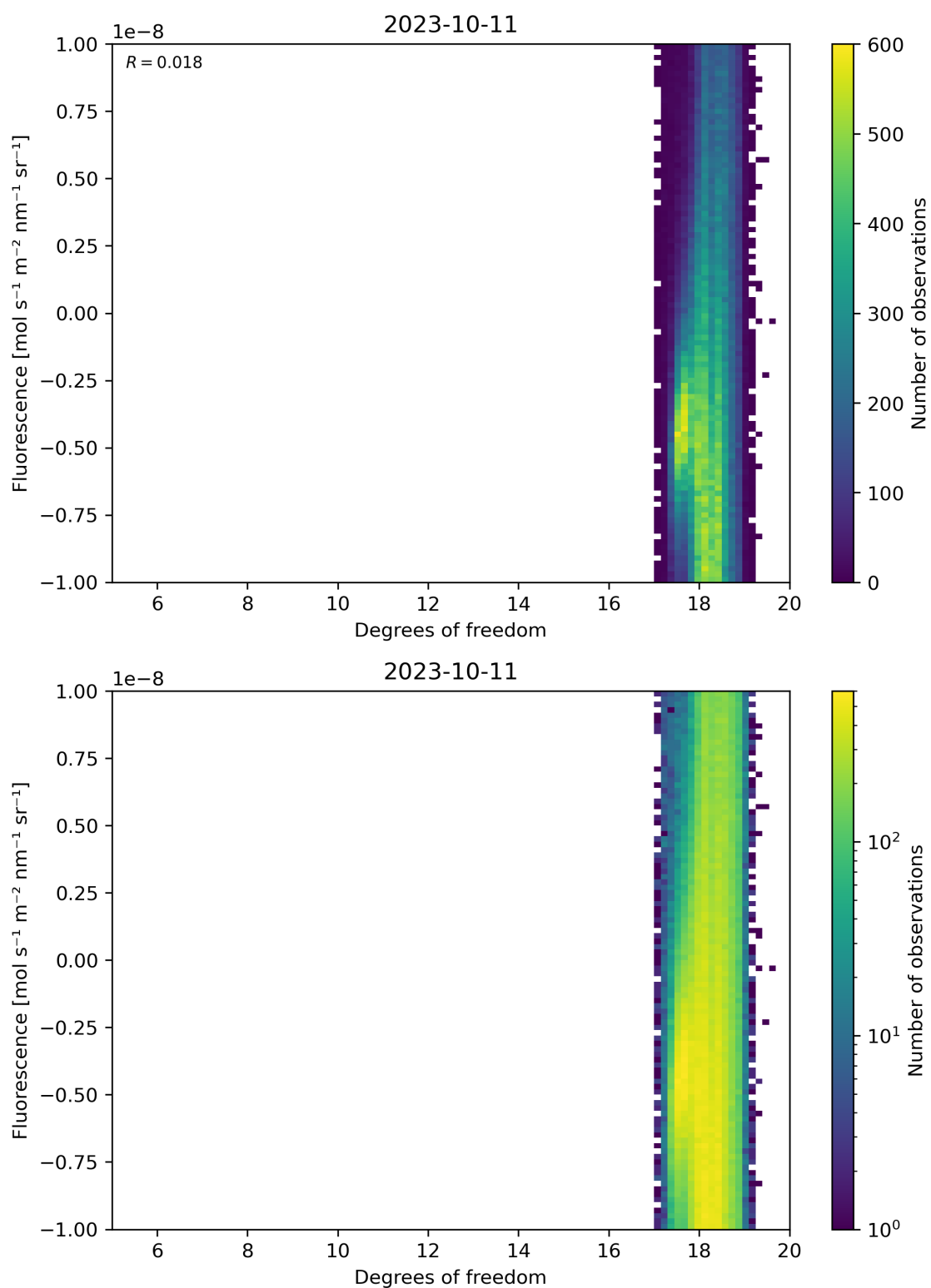
Figure 51: Scatter density plot of “Degrees of freedom” against “Fluorescence” for 2023-10-10 to 2023-10-12.
