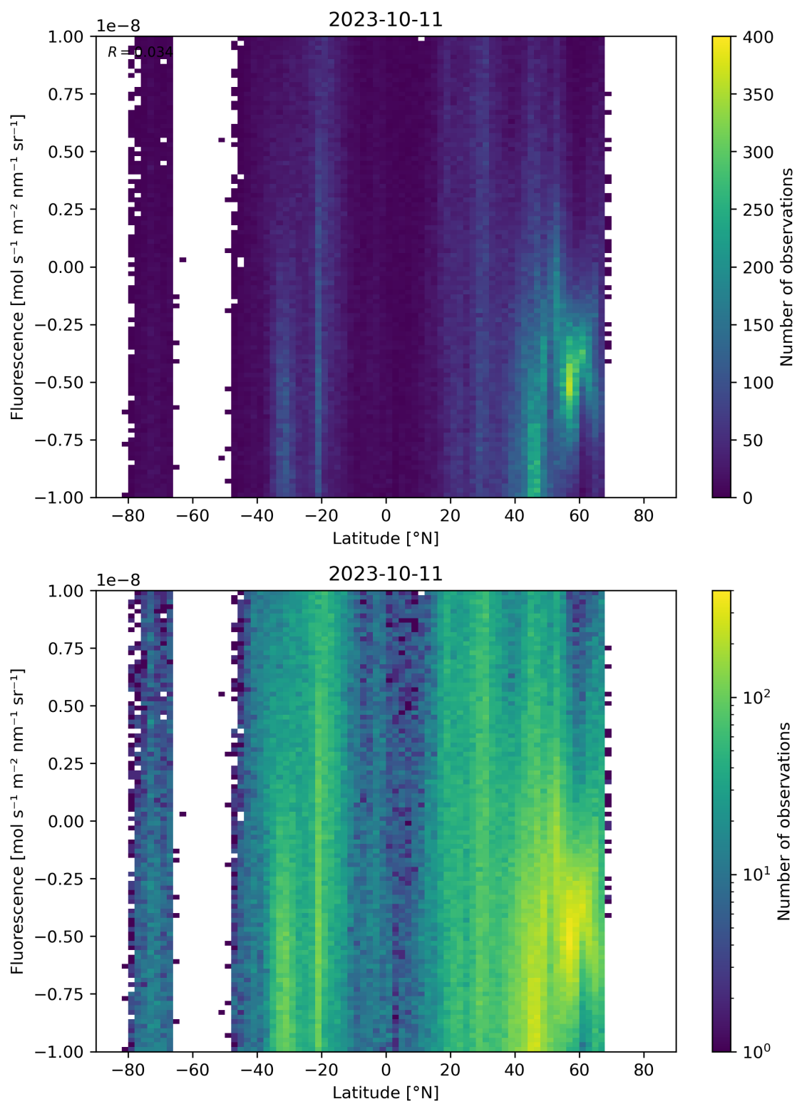
Figure 56: Scatter density plot of “Latitude” against “Fluorescence” for 2023-10-10 to 2023-10-12.
