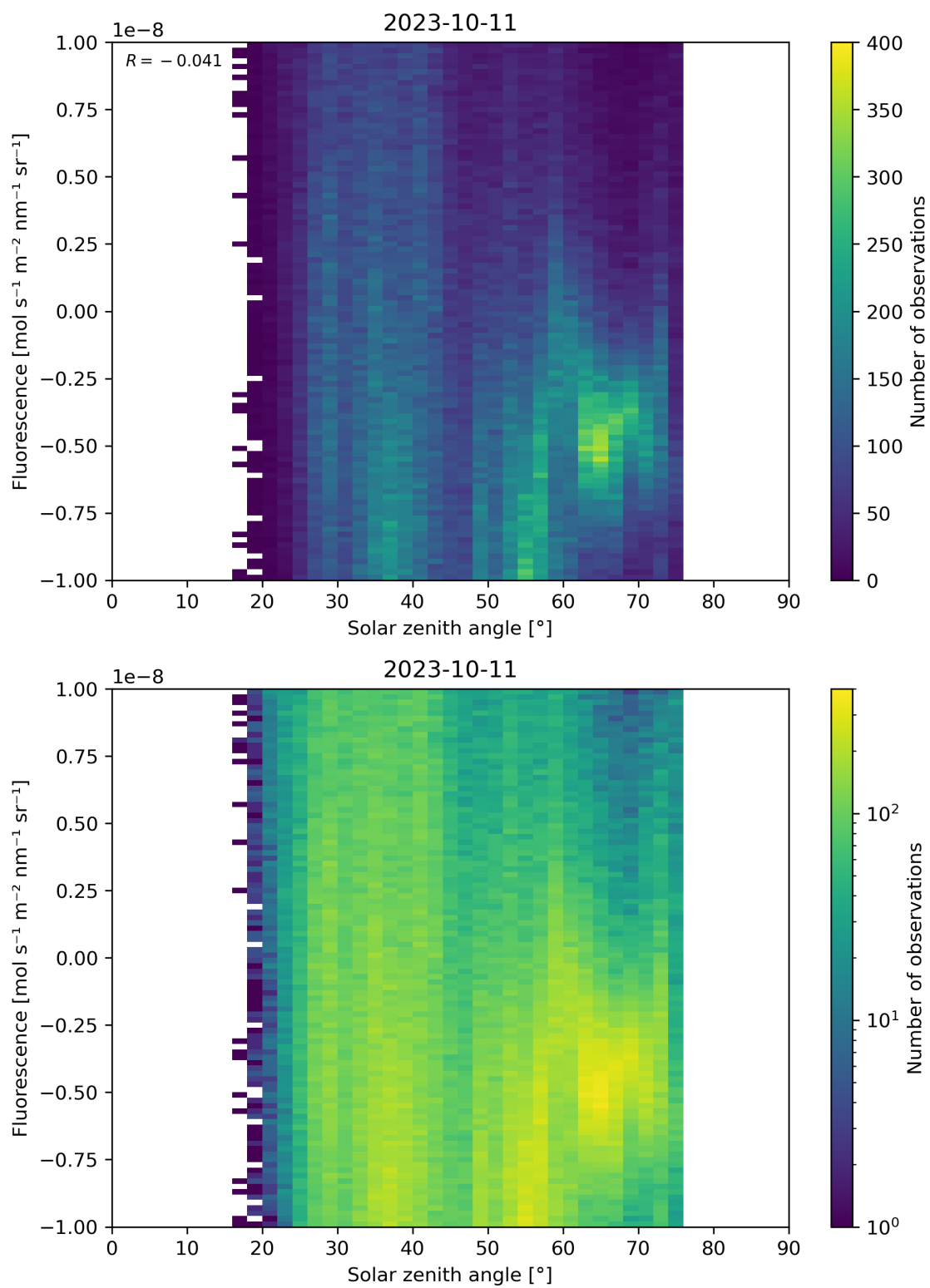
Figure 97: Scatter density plot of “Solar zenith angle” against “Fluorescence” for 2023-10-10 to 2023-10-12.
