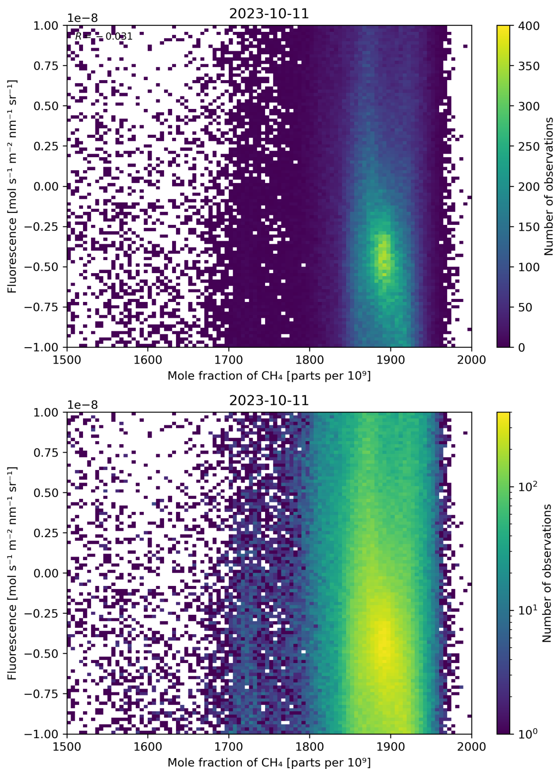
Figure 73: Scatter density plot of “Mole fraction of CH 4 ” against “Fluorescence” for 2023-10-10 to 2023-10-12.
