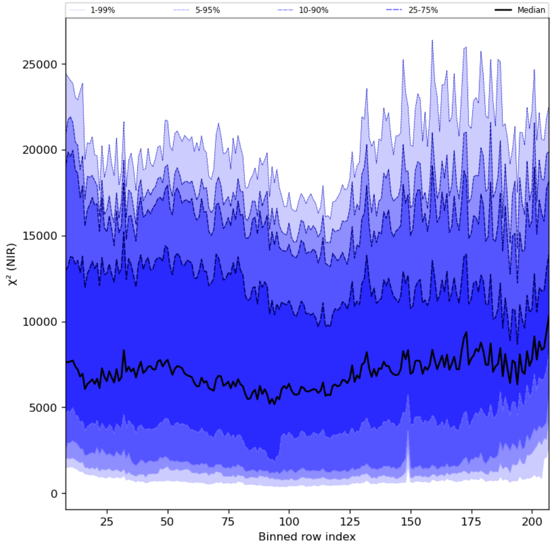
Figure 40: Along track statistics of “ \chi^2 (NIR)” for 2023-10-10 to 2023-10-12
