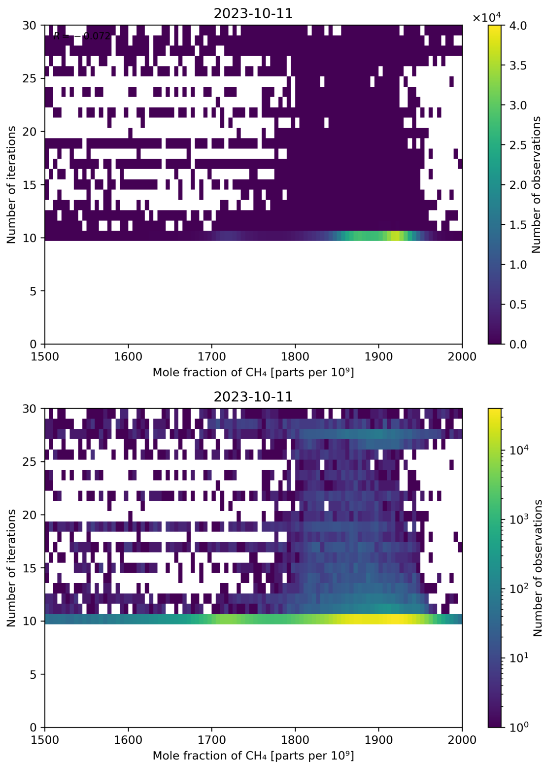
Figure 76: Scatter density plot of “Mole fraction of CH 4 ” against “Number of iterations” for 2023-10-10 to 2023-10-12.
