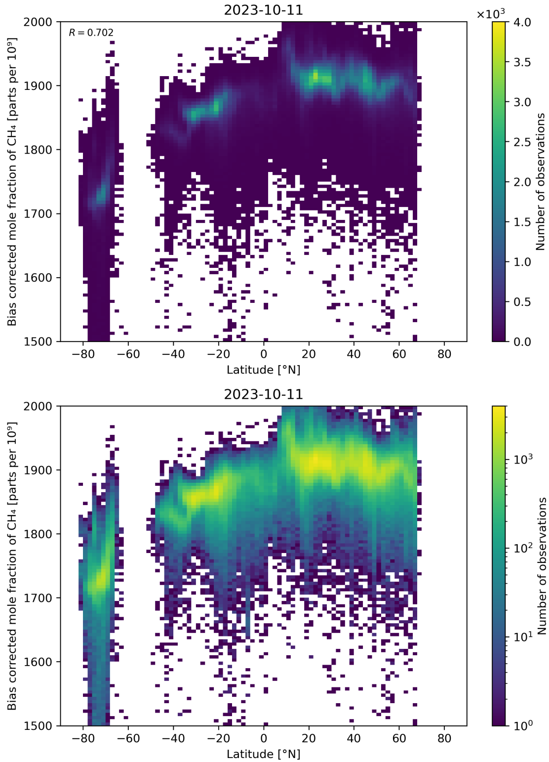
Figure 58: Scatter density plot of “Latitude” against “Bias corrected mole fraction of \text{CH}_4 ” for 2023-10-10 to 2023-10-12.
