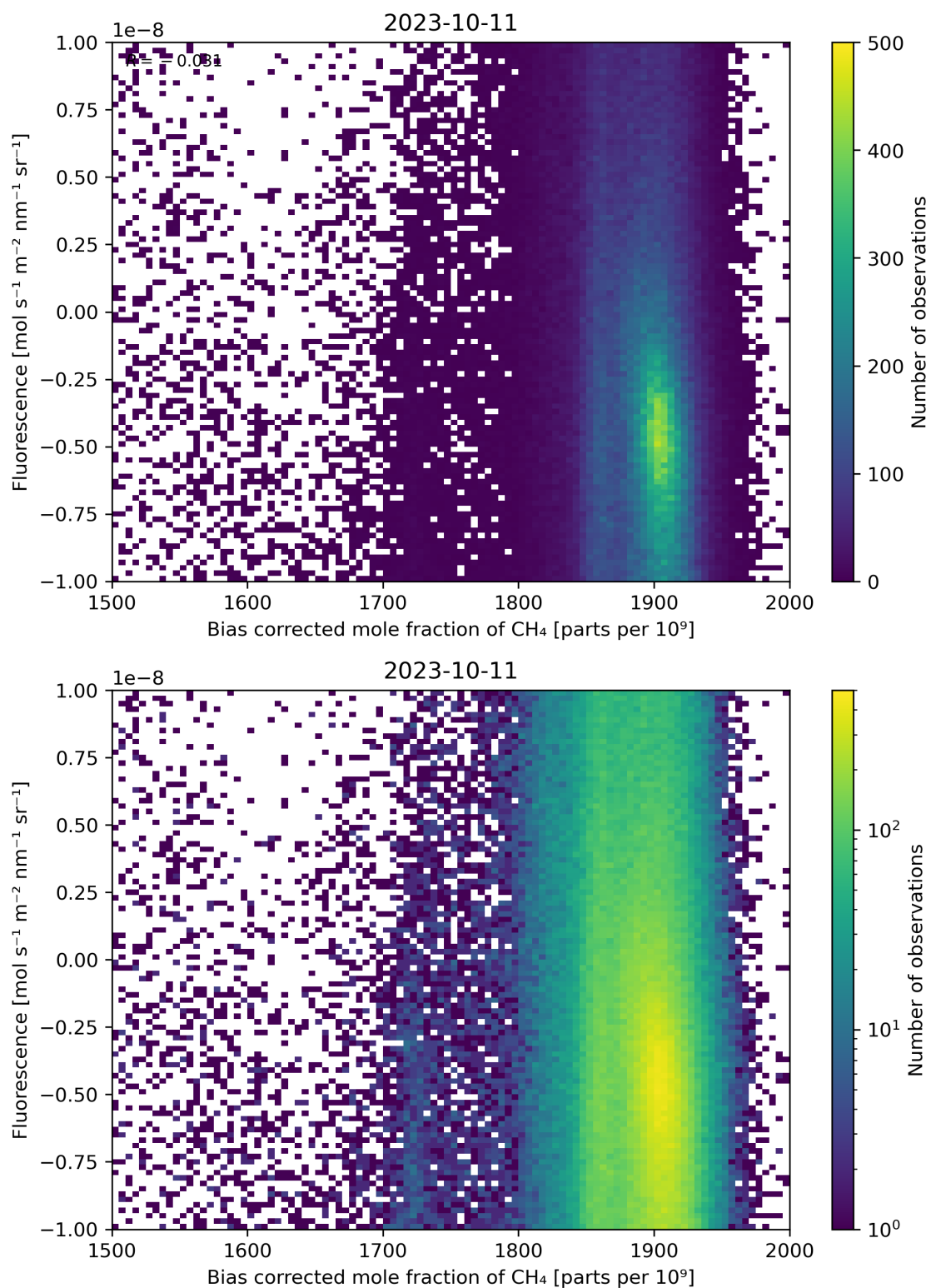
Figure 66: Scatter density plot of “Bias corrected mole fraction of \text{CH}_4 ” against “Fluorescence” for 2023-10-10 to 2023-10-12.
