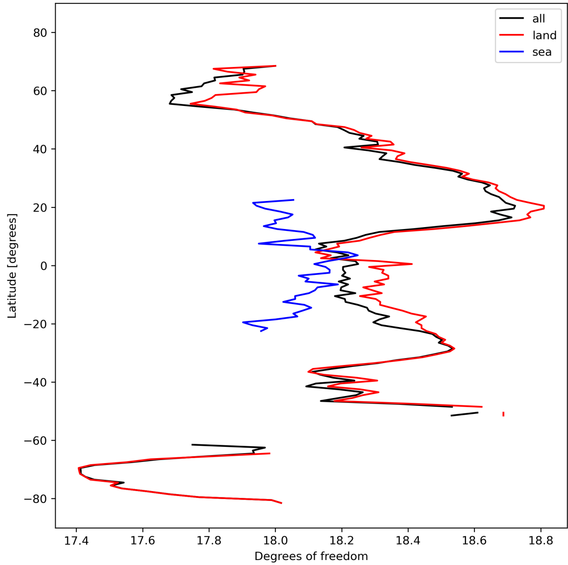
Figure 19: Zonal average of “Degrees of freedom” for 2023-10-10 to 2023-10-12.
