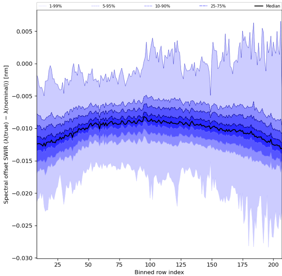
Figure 38: Along track statistics of “Spectral offset SWIR ( \lambda(\text{true}) - \lambda(\text{nominal}) )” for 2023-10-10 to 2023-10-12
