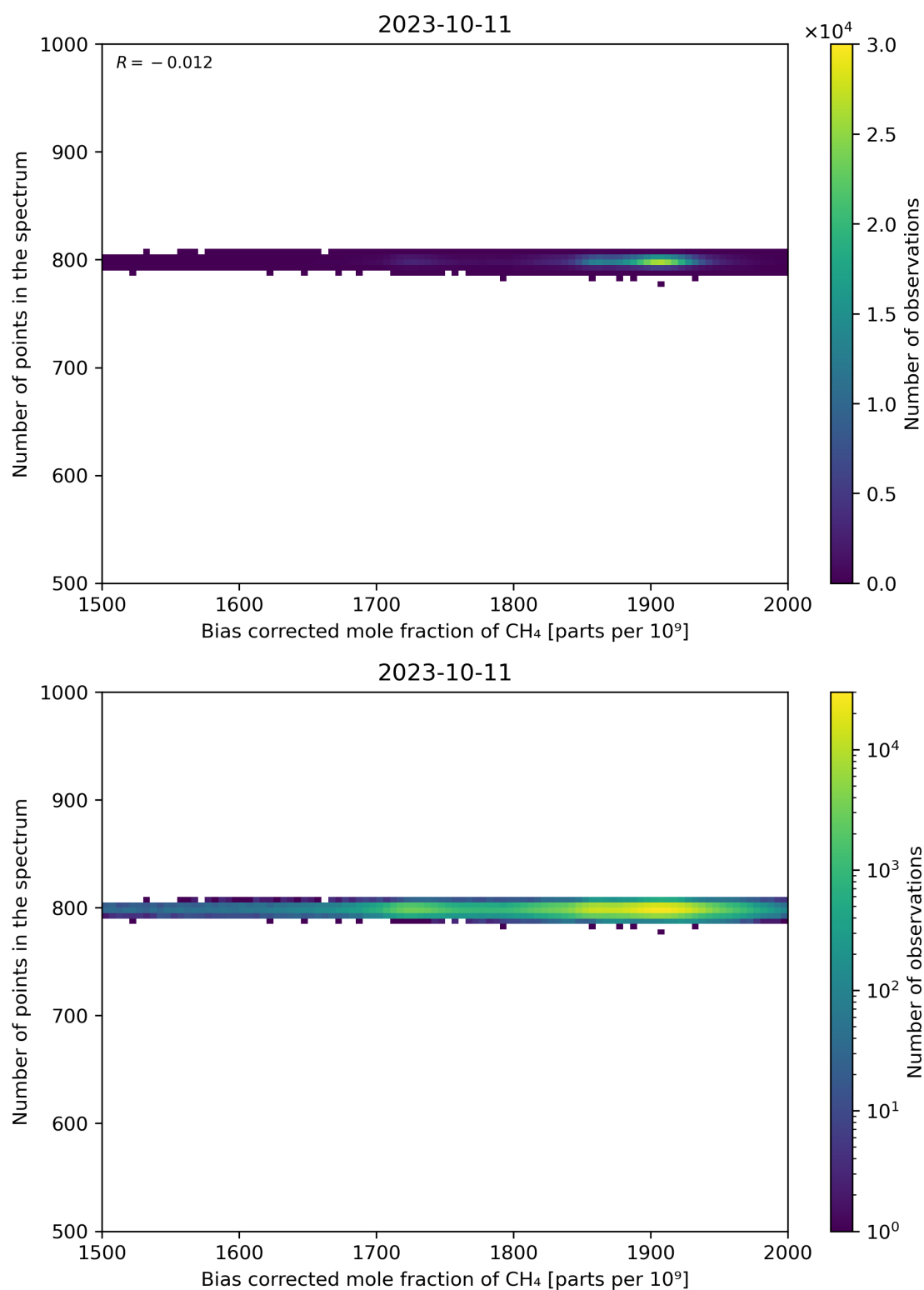
Figure 68: Scatter density plot of “Bias corrected mole fraction of CH 4 ” against “Number of points in the spectrum” for 2023-10-10 to 2023-10-12.
