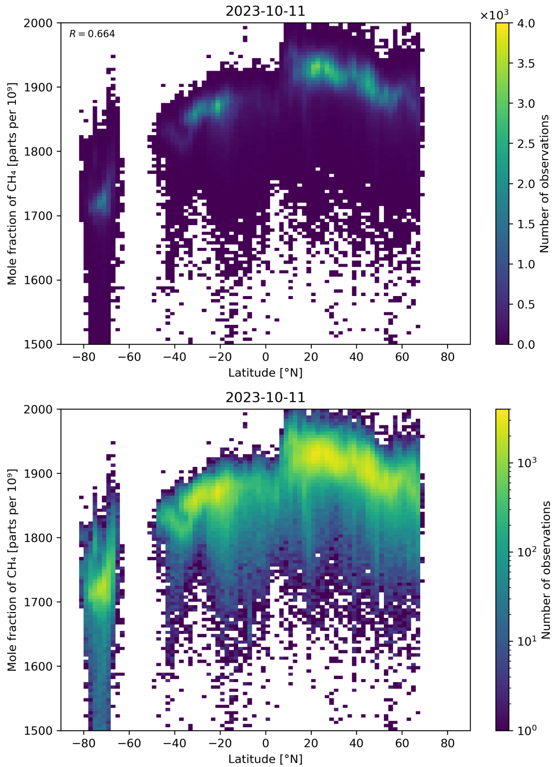
Figure 57: Scatter density plot of “Latitude” against “Mole fraction of CH 4 ” for 2023-10-10 to 2023-10-12.
