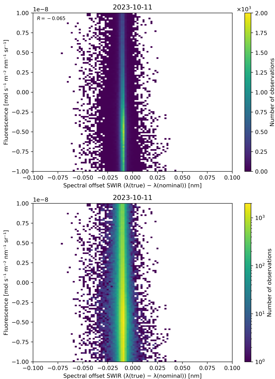
Figure 120: Scatter density plot of “Spectral offset SWIR ( \lambda(\text{true}) - \lambda(\text{nominal}) )” against “Fluorescence” for 2023-10-10 to 2023-10-12.
