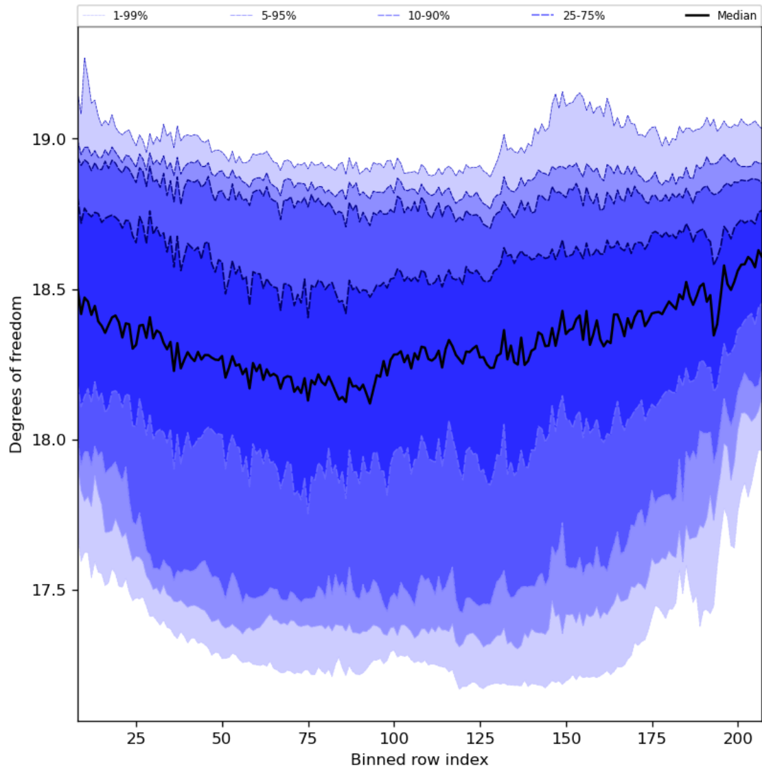
Figure 41: Along track statistics of “Degrees of freedom” for 2023-10-10 to 2023-10-12
