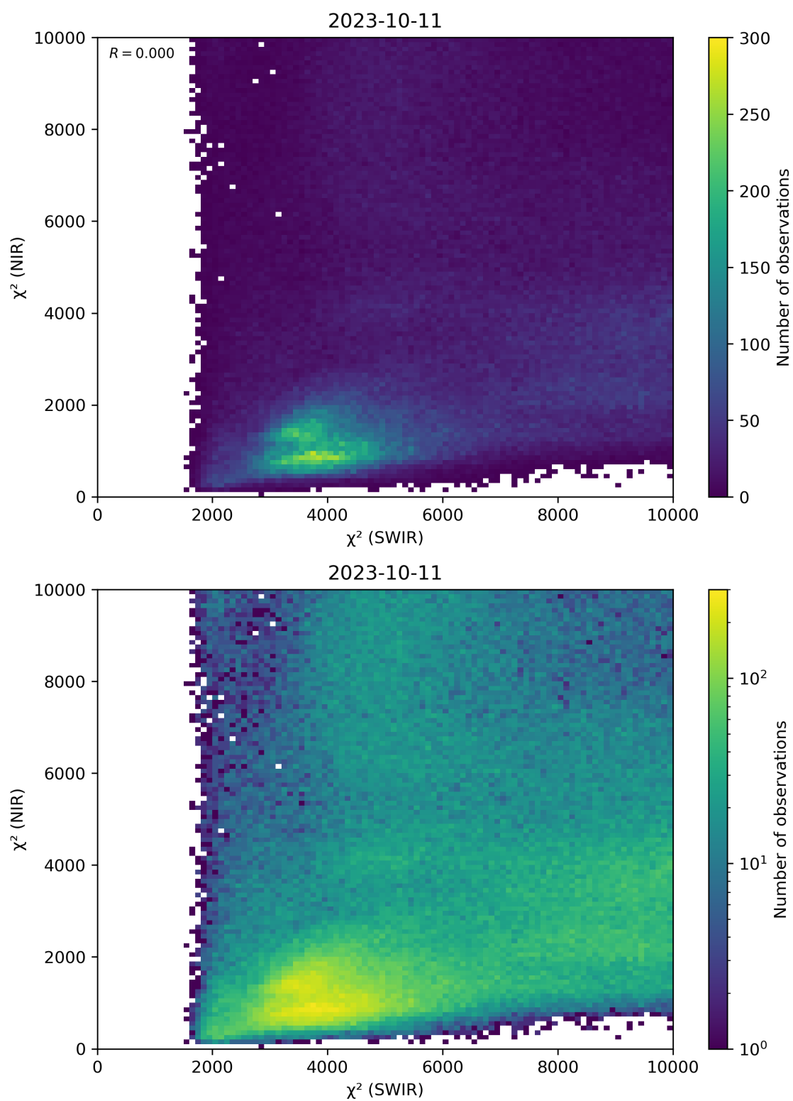
Figure 47: Scatter density plot of “ \chi^2 (SWIR)” against “ \chi^2 (NIR)” for 2023-10-10 to 2023-10-12.
