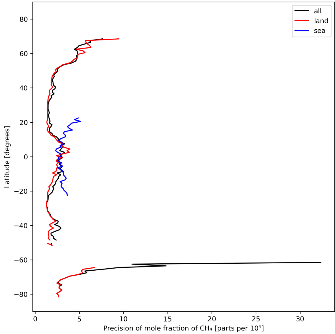
Figure 13: Zonal average of “Precision of mole fraction of CH 4 ” for 2023-10-10 to 2023-10-12.
