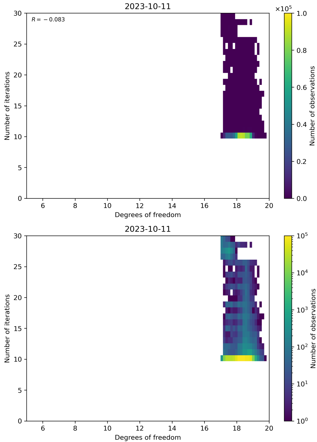
Figure 52: Scatter density plot of “Degrees of freedom” against “Number of iterations” for 2023-10-10 to 2023-10-12.
