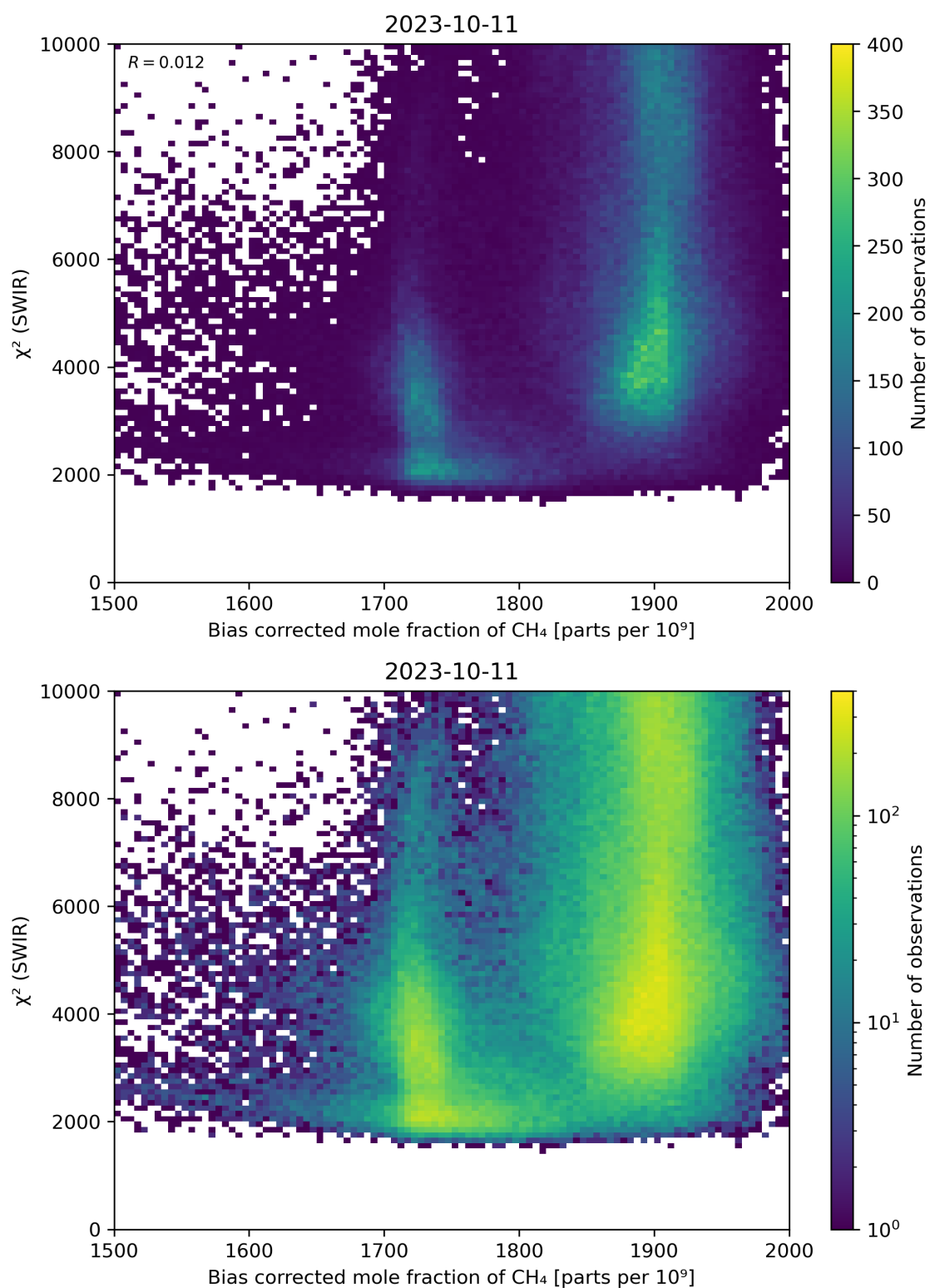
Figure 64: Scatter density plot of “Bias corrected mole fraction of CH 4 ” against “ \chi^2 (SWIR)” for 2023-10-10 to 2023-10-12.
