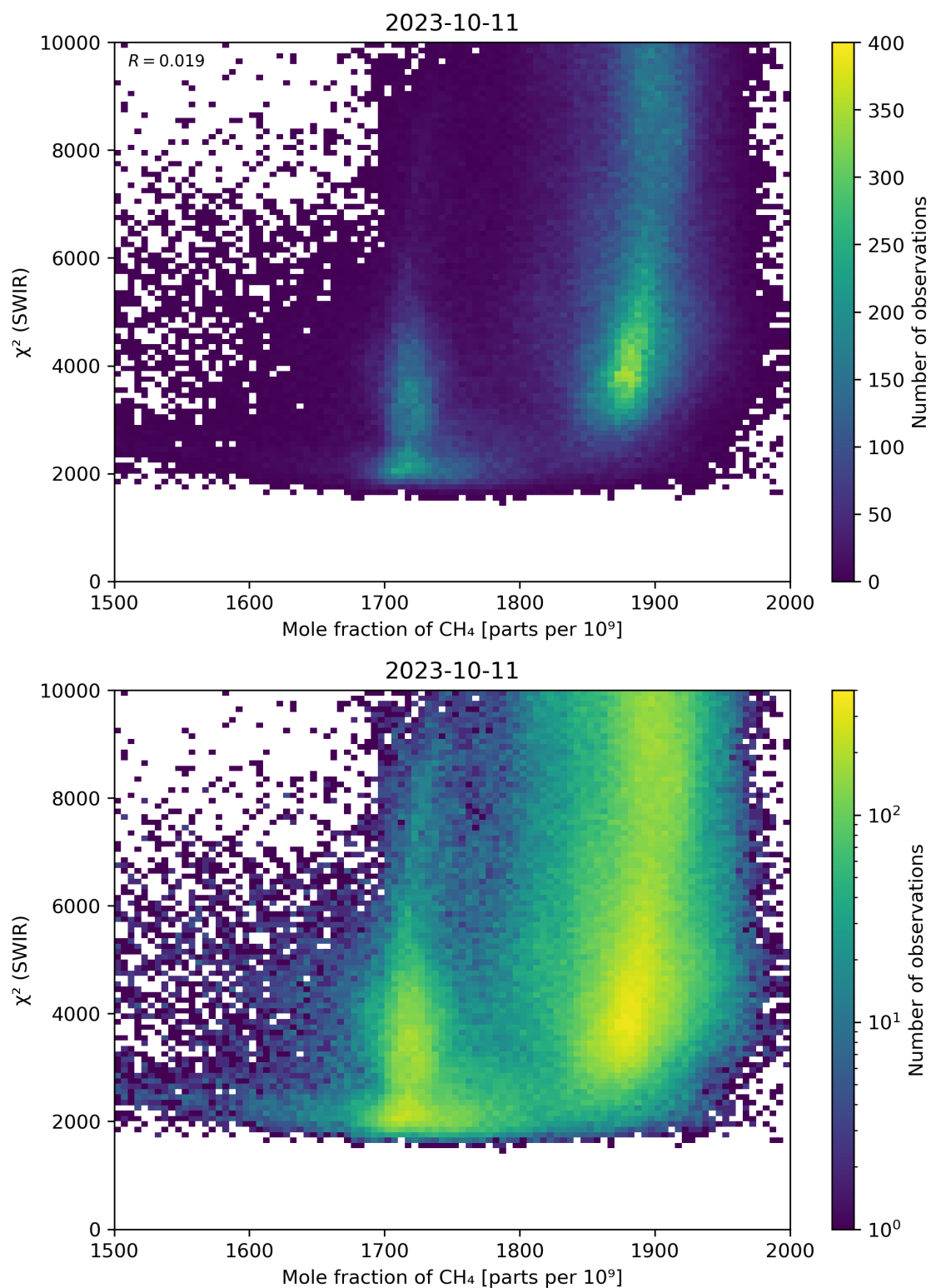
Figure 71: Scatter density plot of “Mole fraction of CH 4 ” against “ \chi^2 (SWIR)” for 2023-10-10 to 2023-10-12.
