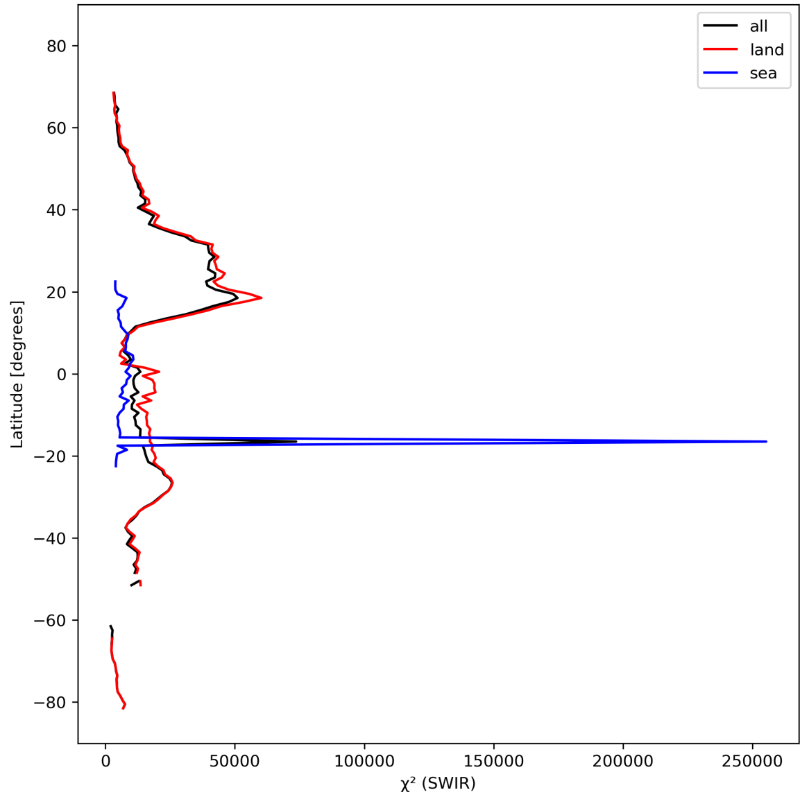
Figure 17: Zonal average of “ \chi^2 (SWIR)” for 2023-10-10 to 2023-10-12.
