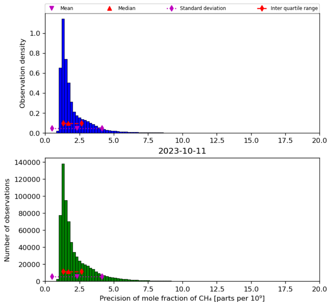
Figure 24: Histogram of “Precision of mole fraction of CH 4 ” for 2023-10-10 to 2023-10-12
