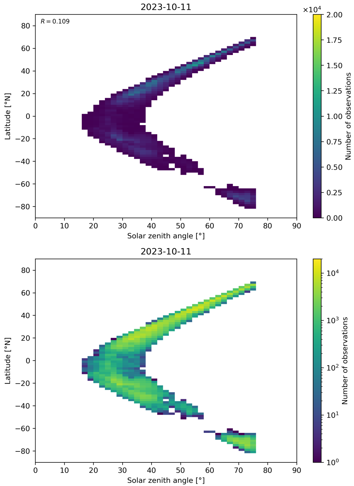
Figure 98: Scatter density plot of “Solar zenith angle” against “Latitude” for 2023-10-10 to 2023-10-12.
