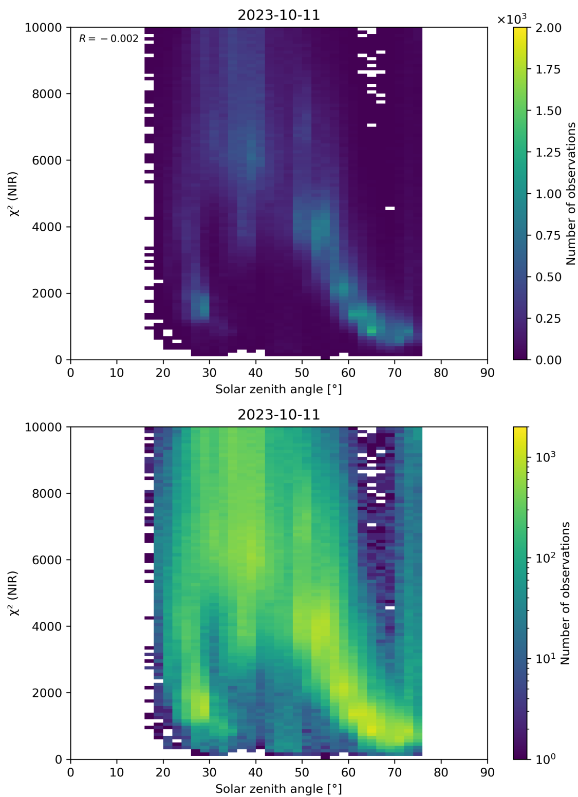
Figure 94: Scatter density plot of “Solar zenith angle” against “ \chi^2 (NIR)” for 2023-10-10 to 2023-10-12.
