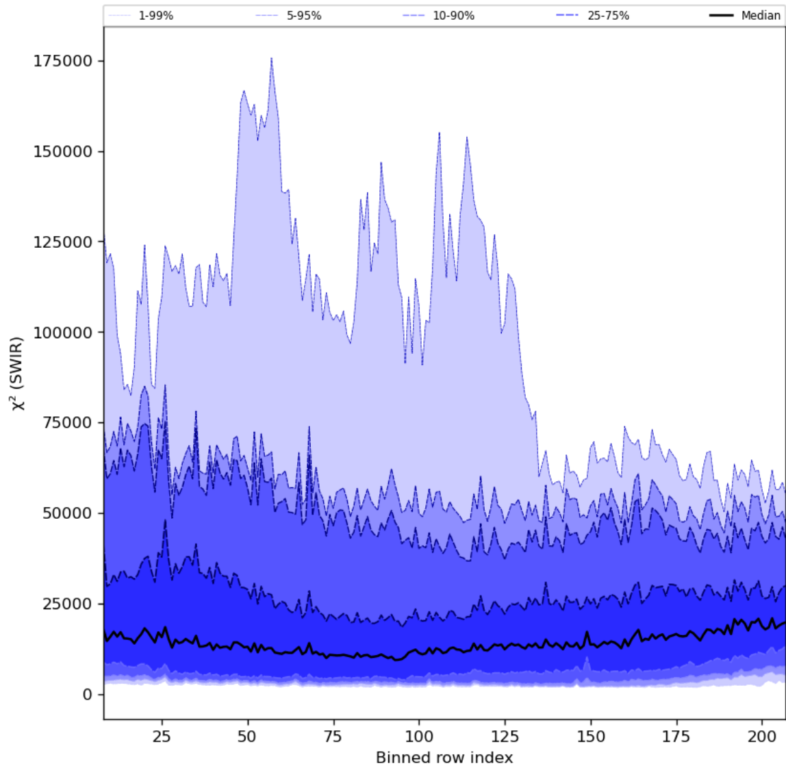
Figure 39: Along track statistics of “ \chi^2 (SWIR)” for 2023-10-10 to 2023-10-12
