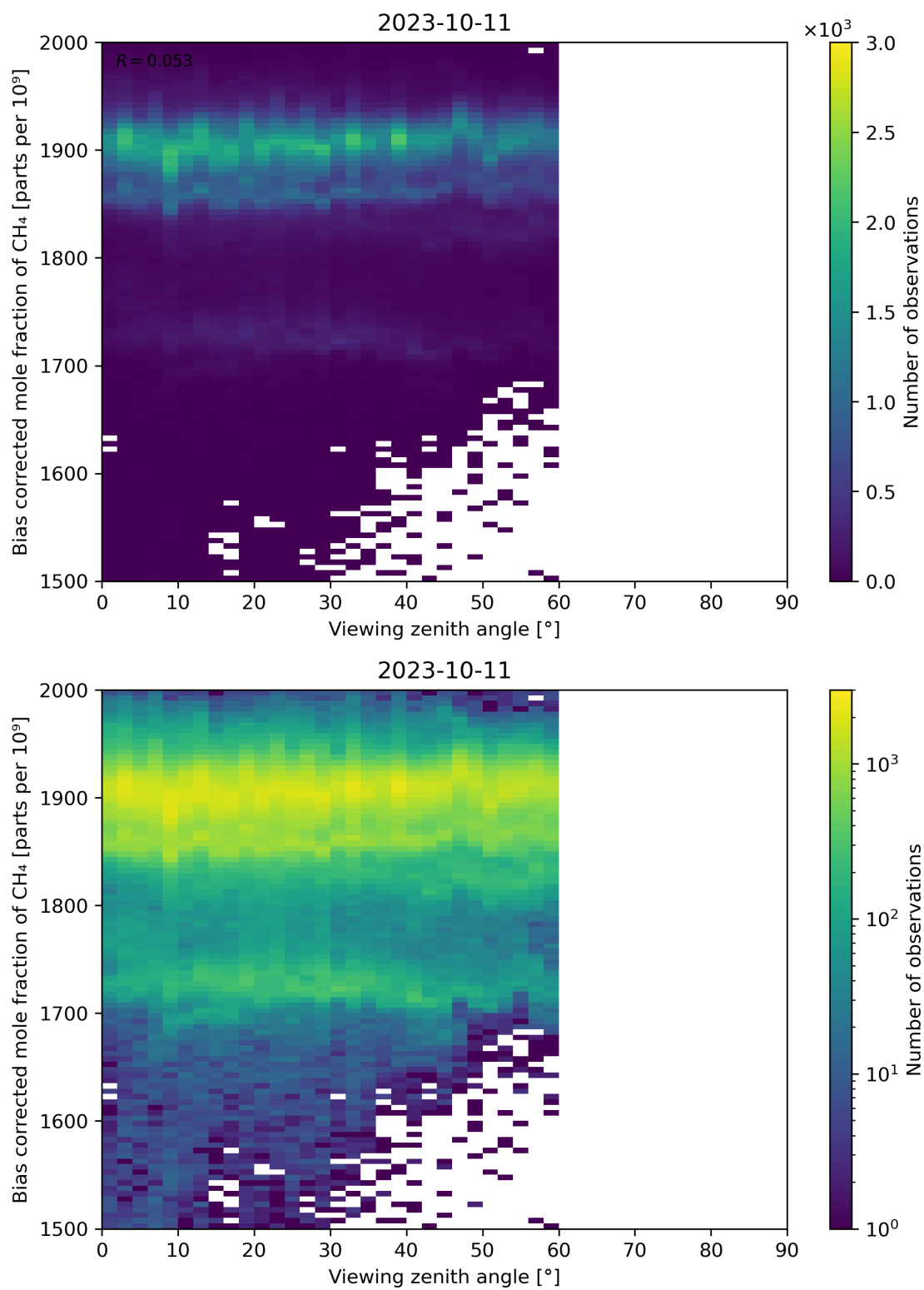
Figure 111: Scatter density plot of “Viewing zenith angle” against “Bias corrected mole fraction of CH 4 ” for 2023-10-10 to 2023-10-12.
