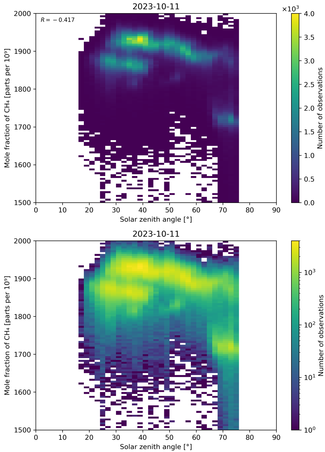
Figure 99: Scatter density plot of “Solar zenith angle” against “Mole fraction of CH 4 ” for 2023-10-10 to 2023-10-12.
