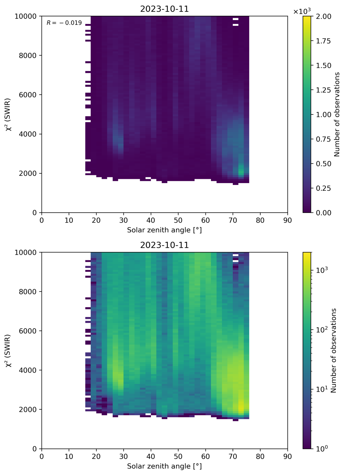
Figure 95: Scatter density plot of “Solar zenith angle” against “ \chi^2 (SWIR)” for 2023-10-10 to 2023-10-12.
