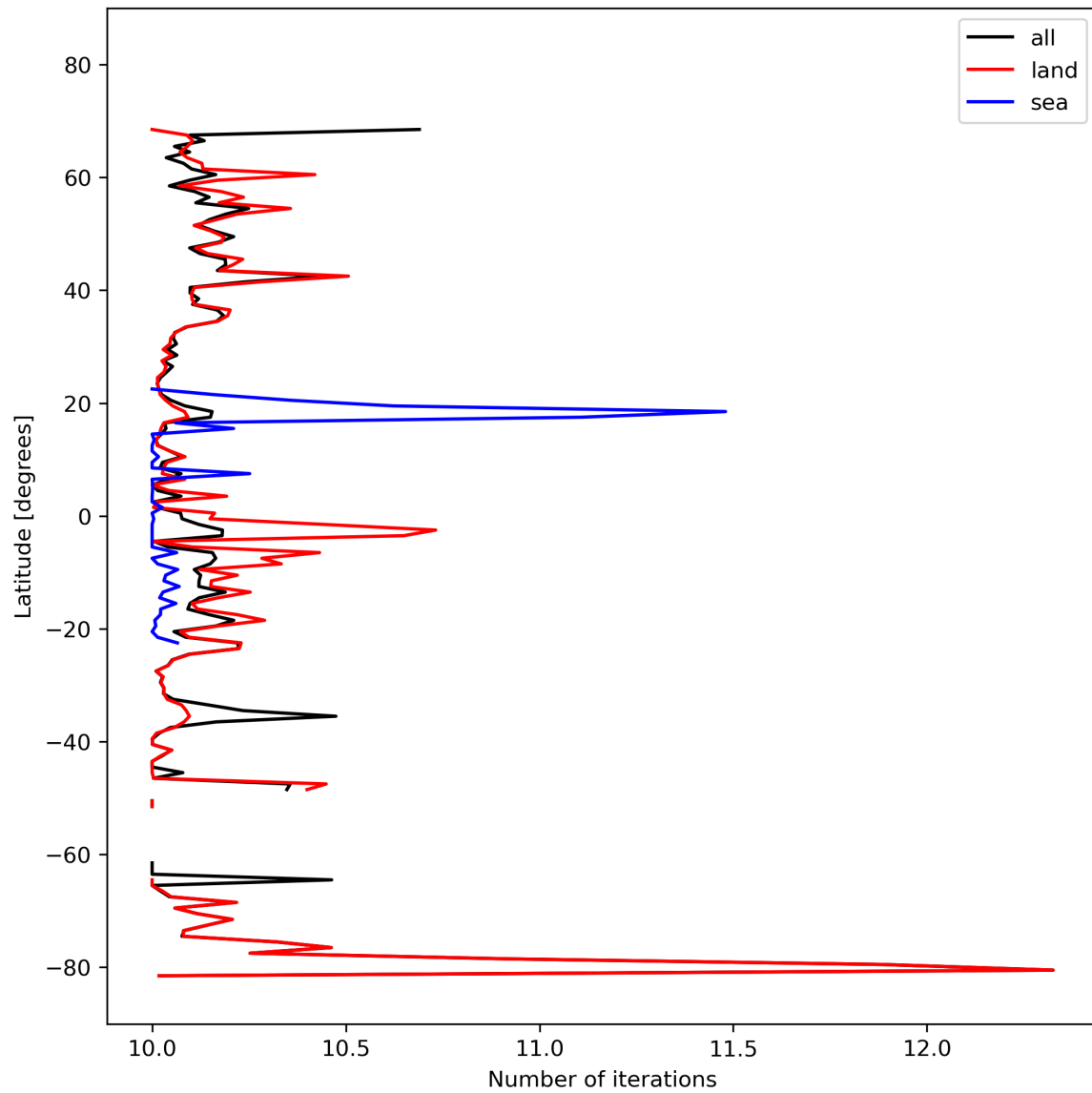
Figure 20: Zonal average of “Number of iterations” for 2023-10-10 to 2023-10-12.
