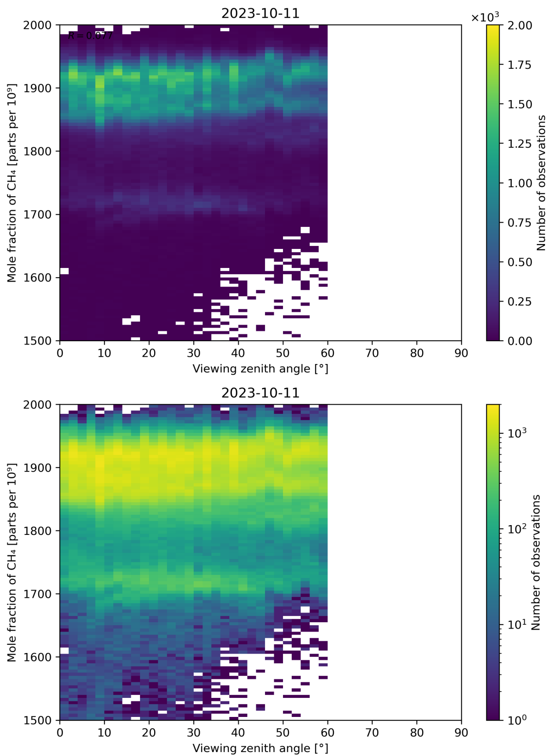
Figure 110: Scatter density plot of “Viewing zenith angle” against “Mole fraction of CH 4 ” for 2023-10-10 to 2023-10-12.
