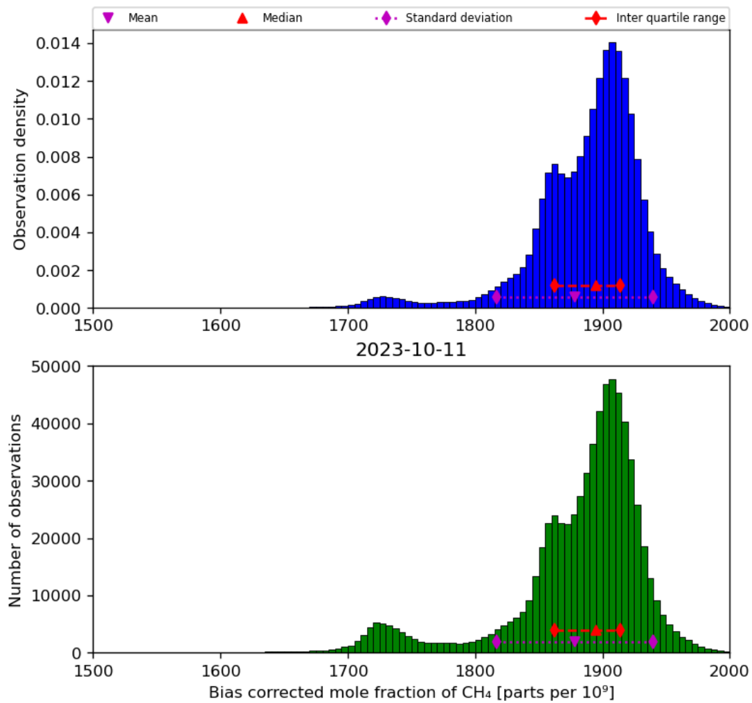
Figure 25: Histogram of “Bias corrected mole fraction of CH 4 ” for 2023-10-10 to 2023-10-12
