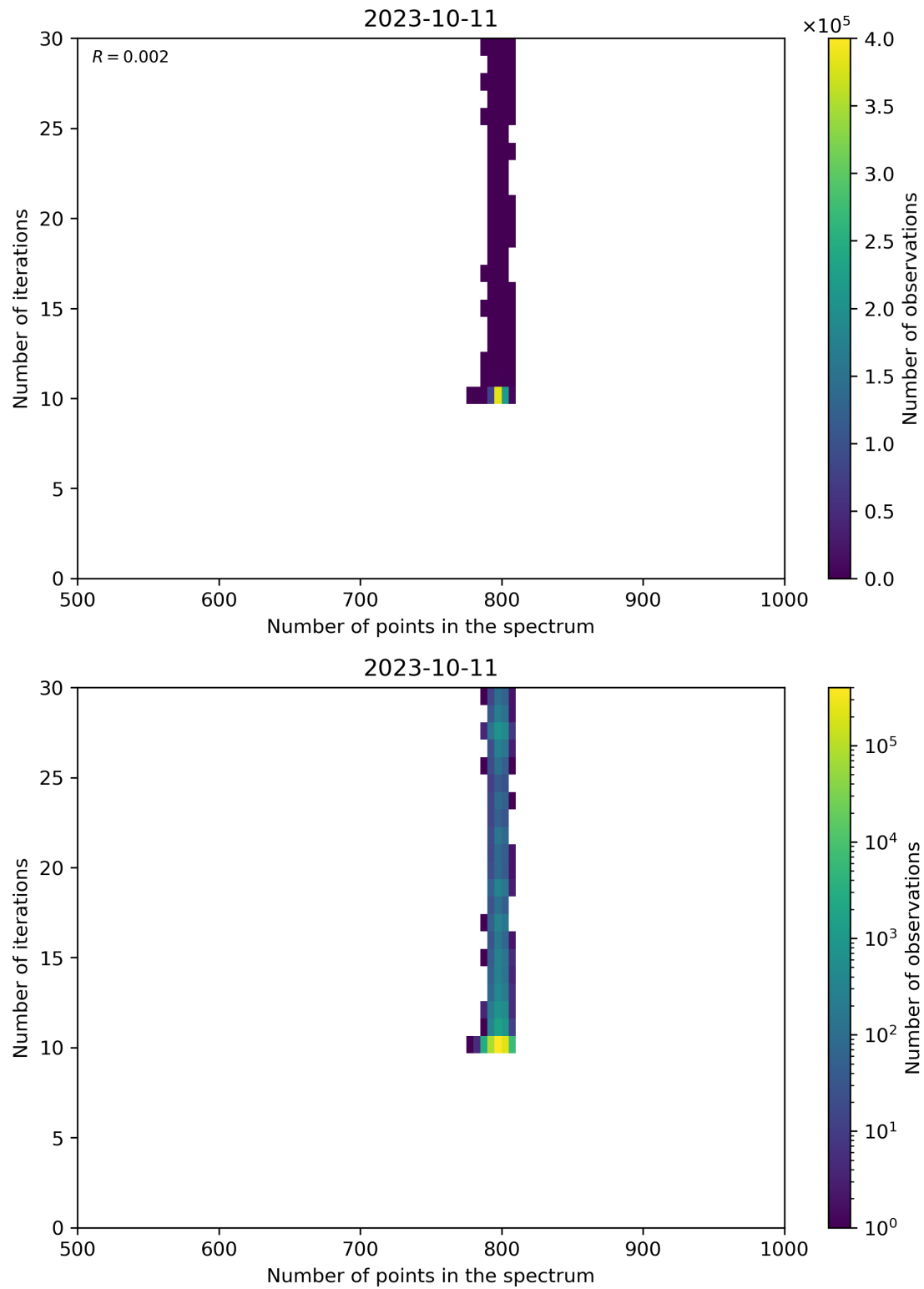
Figure 92: Scatter density plot of “Number of points in the spectrum” against “Number of iterations” for 2023-10-10 to 2023-10-12.
