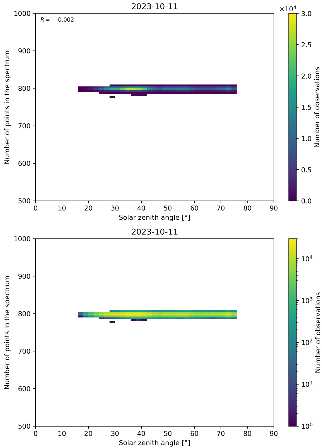
Figure 103: Scatter density plot of “Solar zenith angle” against “Number of points in the spectrum” for 2023-10-10 to 2023-10-12.
