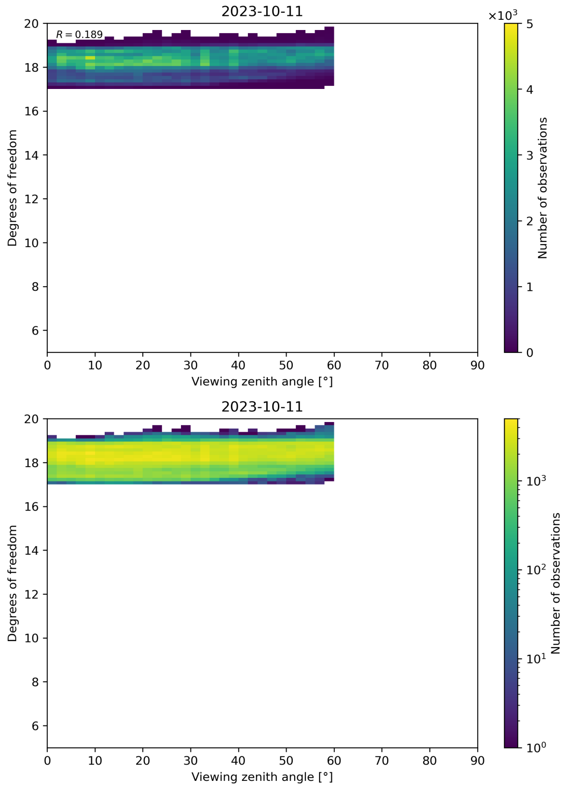
Figure 107: Scatter density plot of “Viewing zenith angle” against “Degrees of freedom” for 2023-10-10 to 2023-10-12.
