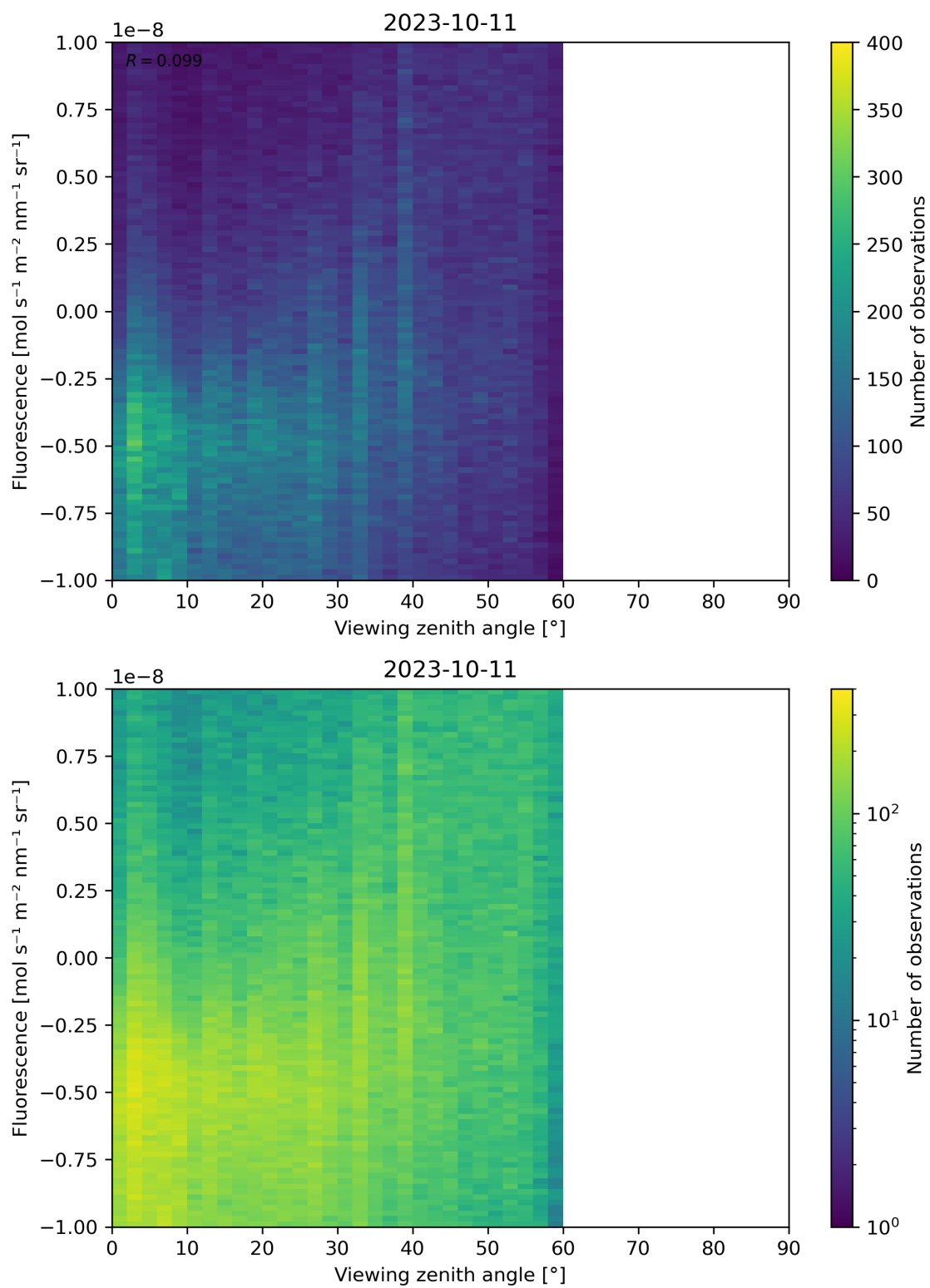
Figure 108: Scatter density plot of “Viewing zenith angle” against “Fluorescence” for 2023-10-10 to 2023-10-12.
