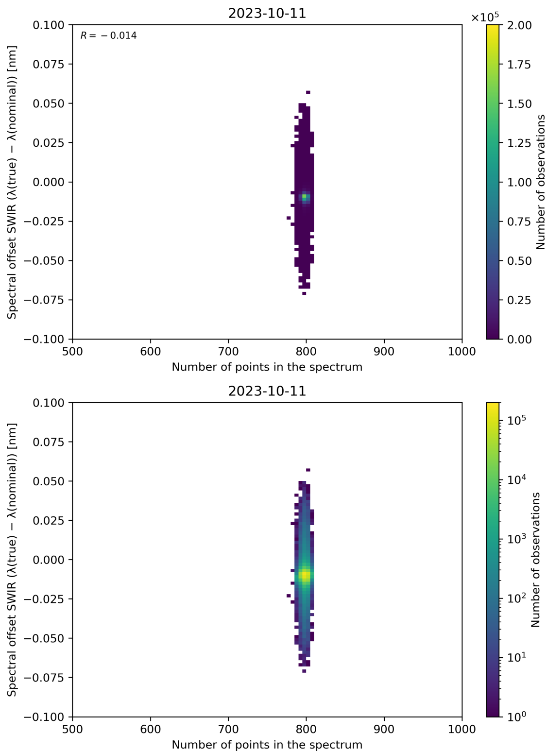
Figure 93: Scatter density plot of “Number of points in the spectrum” against “Spectral offset SWIR ( \lambda(\text{true}) - \lambda(\text{nominal}) )” for 2023-10-10 to 2023-10-12.
