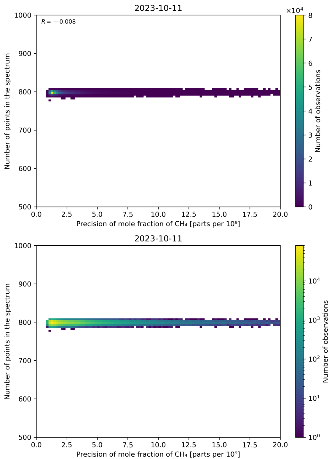
Figure 84: Scatter density plot of “Precision of mole fraction of CH 4 ” against “Number of points in the spectrum” for 2023-10-10 to 2023-10-12.
