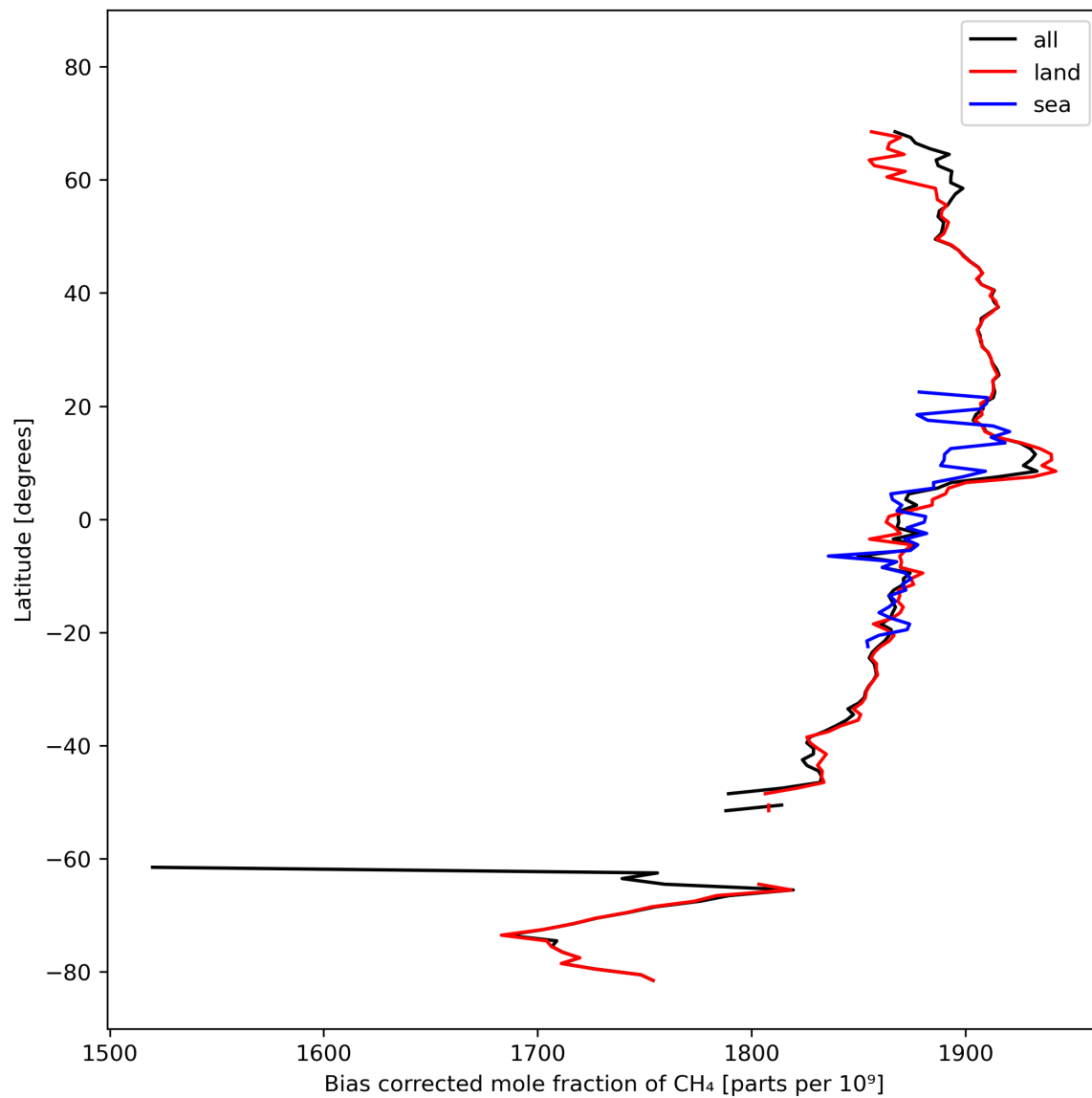
Figure 14: Zonal average of “Bias corrected mole fraction of CH 4 ” for 2023-10-10 to 2023-10-12.
