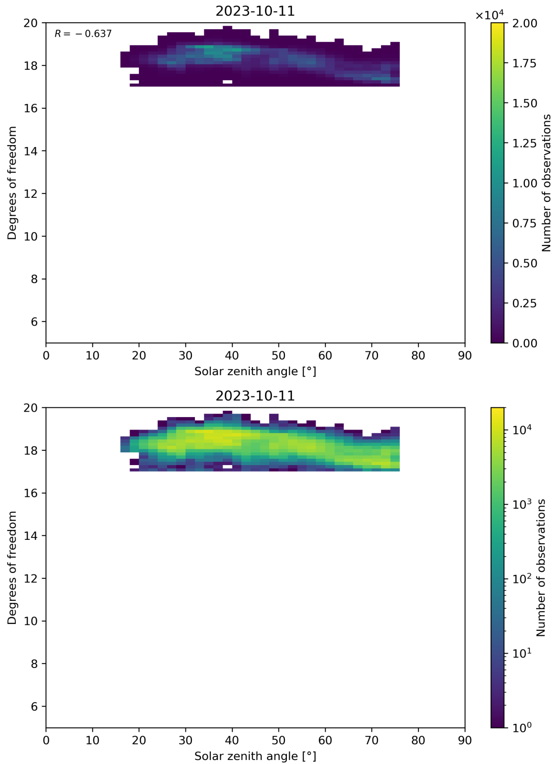
Figure 96: Scatter density plot of “Solar zenith angle” against “Degrees of freedom” for 2023-10-10 to 2023-10-12.
