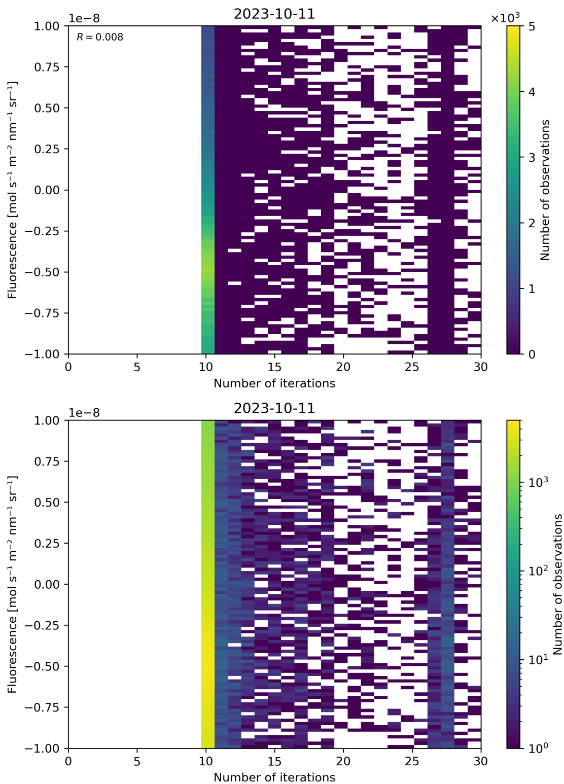
Figure 87: Scatter density plot of “Number of iterations” against “Fluorescence” for 2023-10-10 to 2023-10-12.
