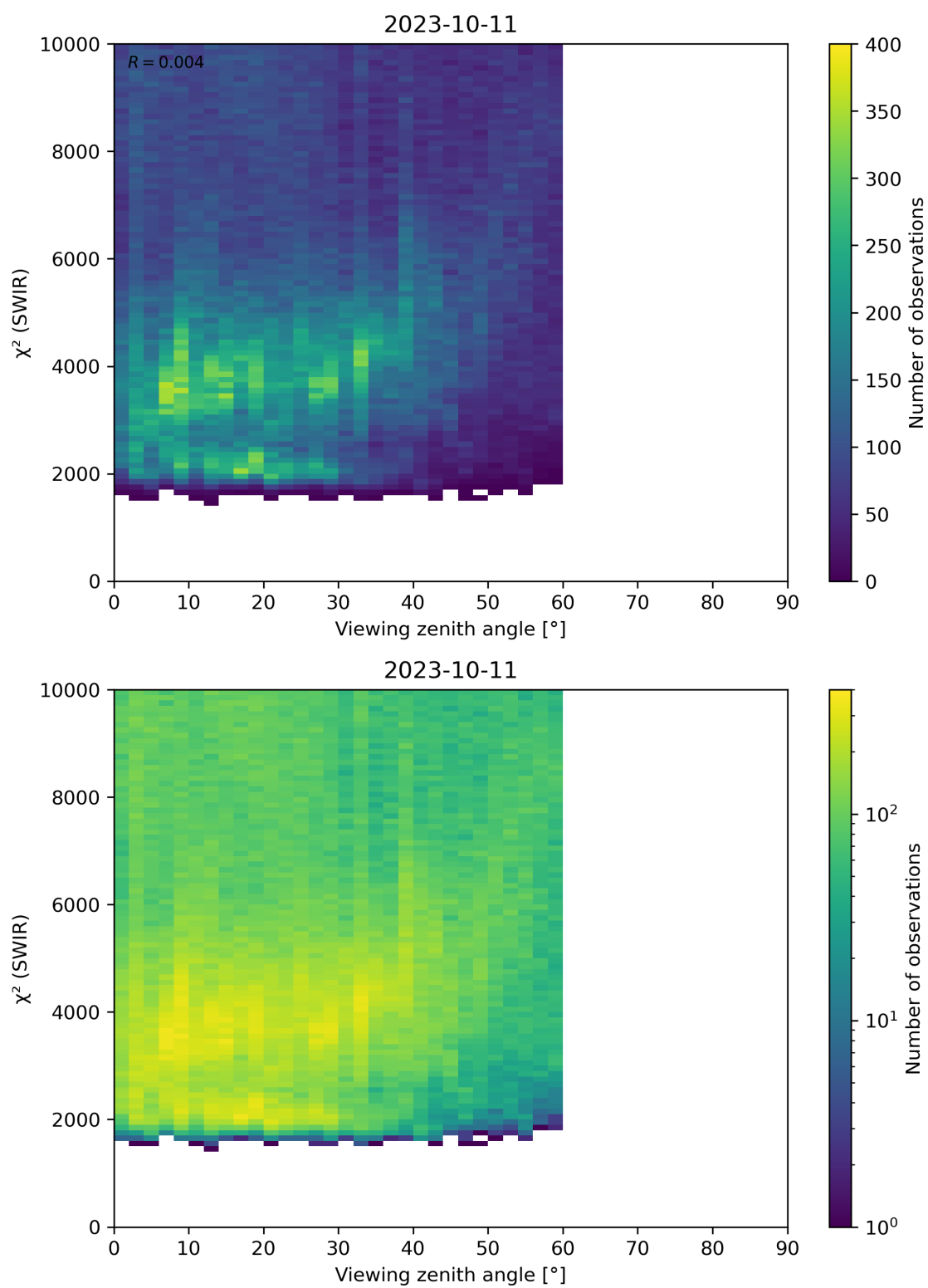
Figure 106: Scatter density plot of “Viewing zenith angle” against “ \chi^2 (SWIR)” for 2023-10-10 to 2023-10-12.
