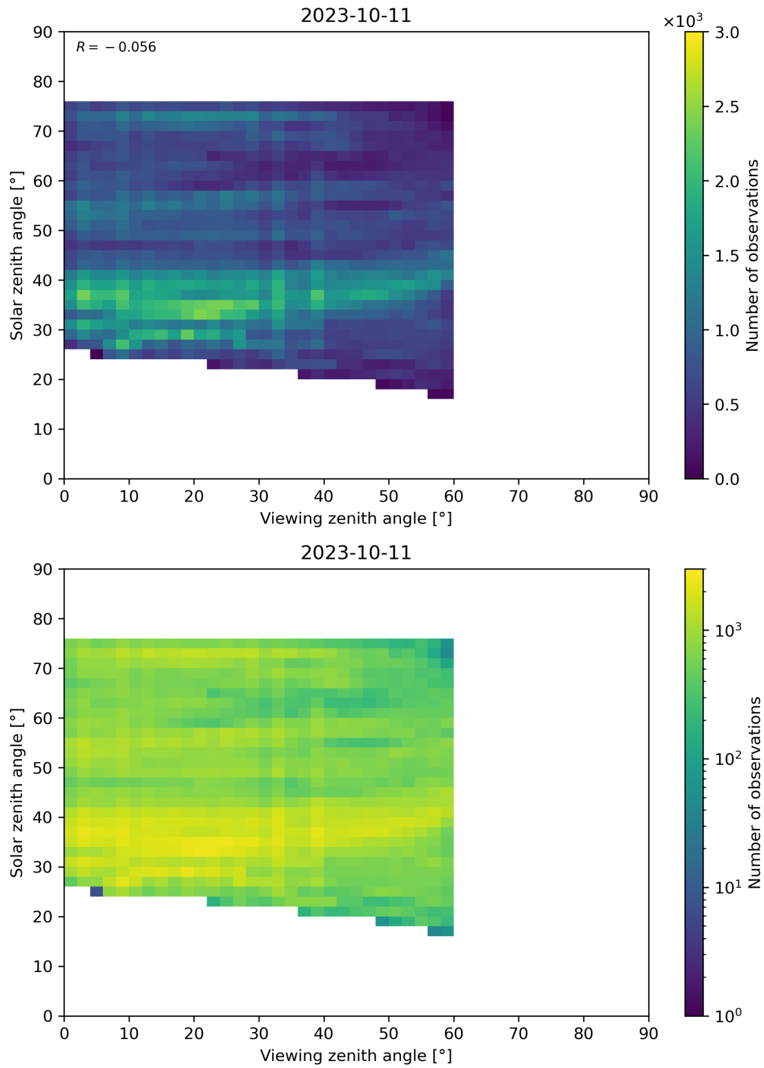
Figure 115: Scatter density plot of “Viewing zenith angle” against “Solar zenith angle” for 2023-10-10 to 2023-10-12.
