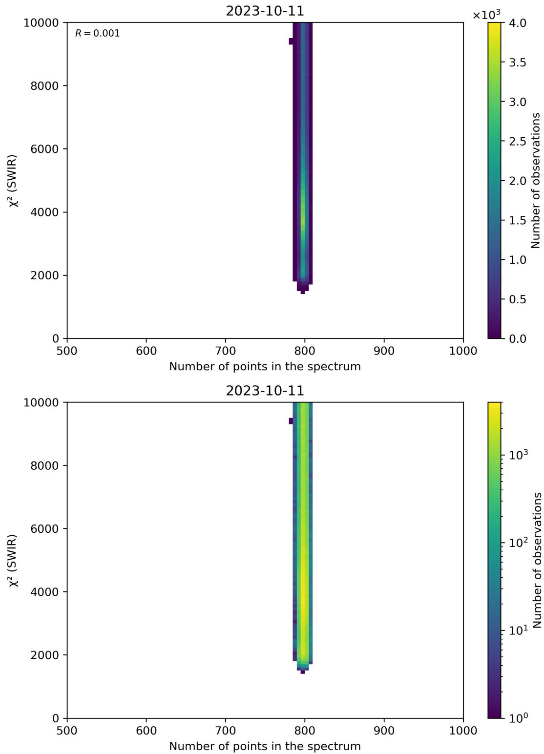
Figure 89: Scatter density plot of “Number of points in the spectrum” against “ \chi^2 (SWIR)” for 2023-10-10 to 2023-10-12.
