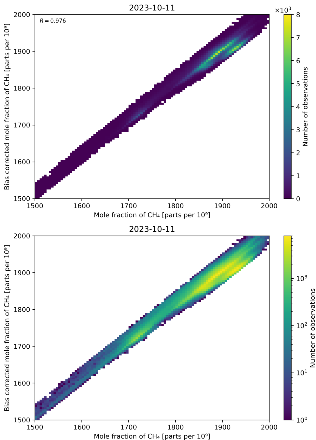
Figure 74: Scatter density plot of “Mole fraction of CH 4 ” against “Bias corrected mole fraction of CH 4 ” for 2023-10-10 to 2023-10-12.
