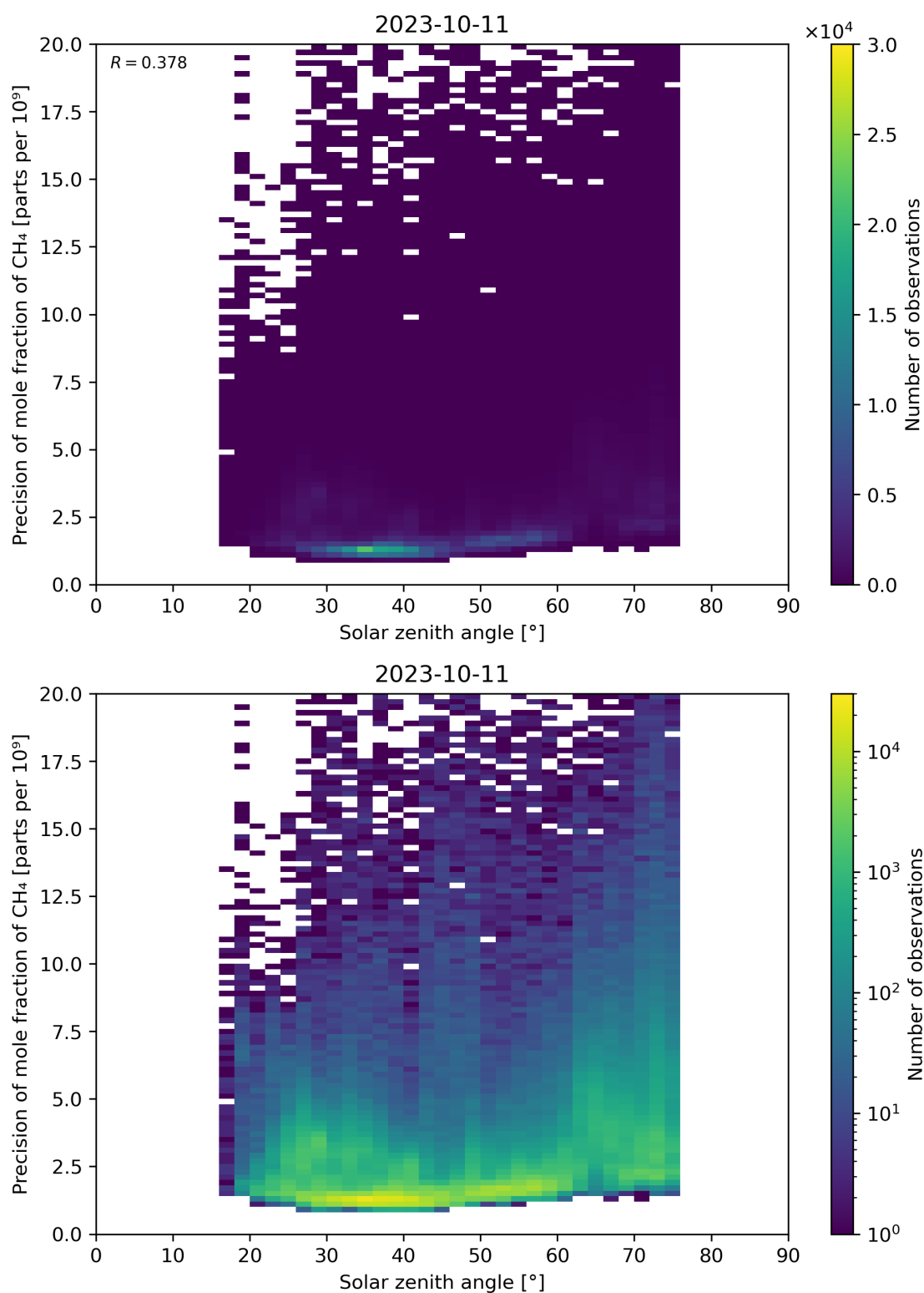
Figure 101: Scatter density plot of “Solar zenith angle” against “Precision of mole fraction of CH 4 ” for 2023-10-10 to 2023-10-12.
