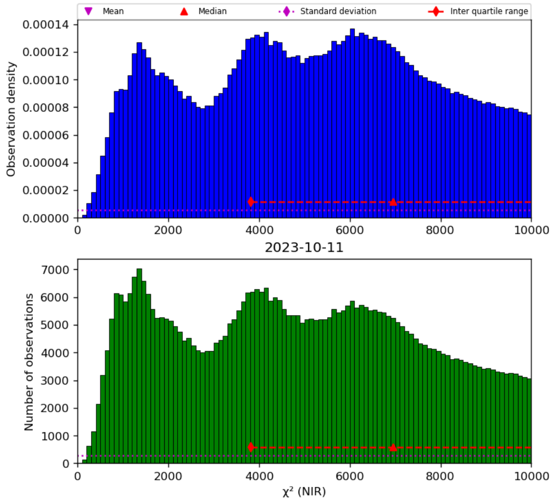
Figure 29: Histogram of “ \chi^2 (NIR)” for 2023-10-10 to 2023-10-12
