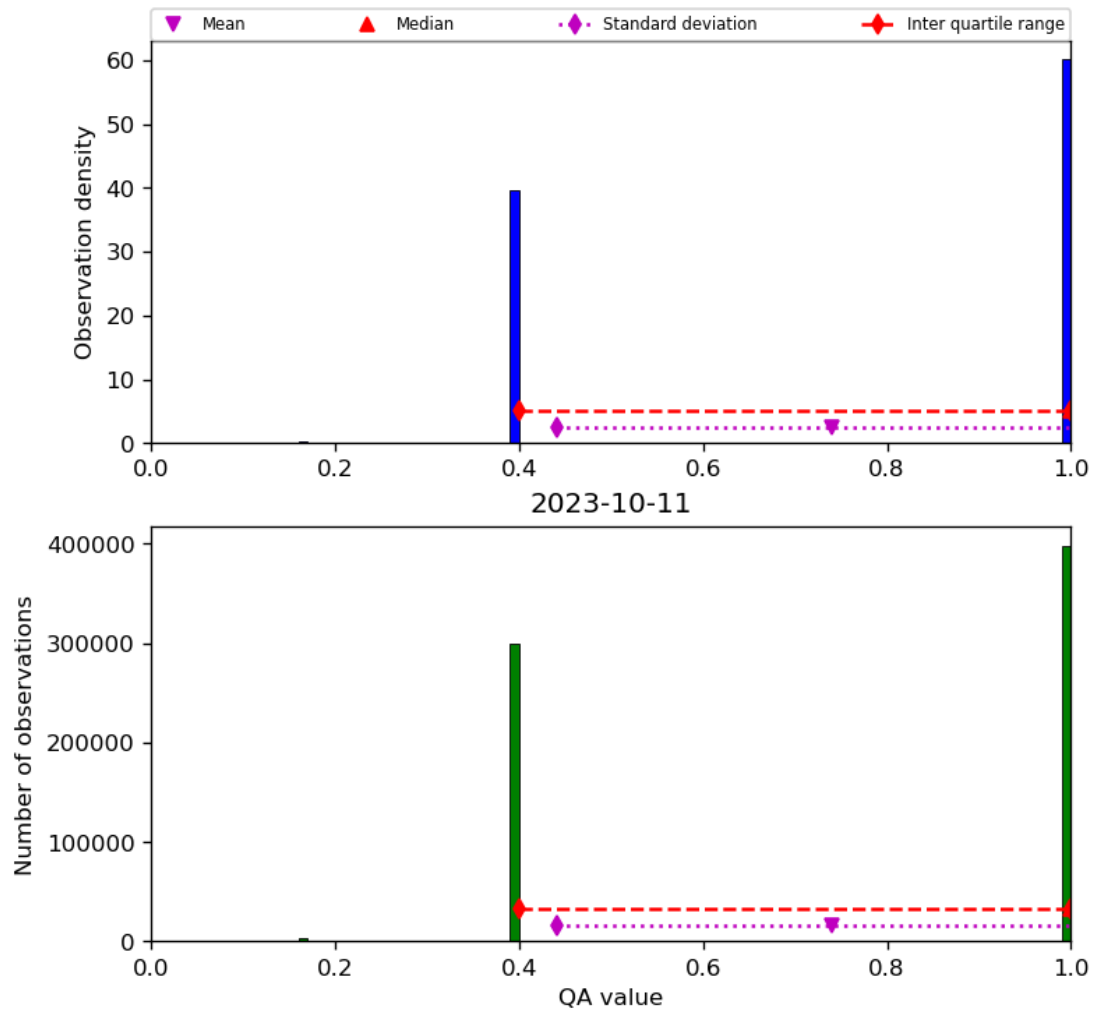
Figure 22: Histogram of “QA value” for 2023-10-10 to 2023-10-12
