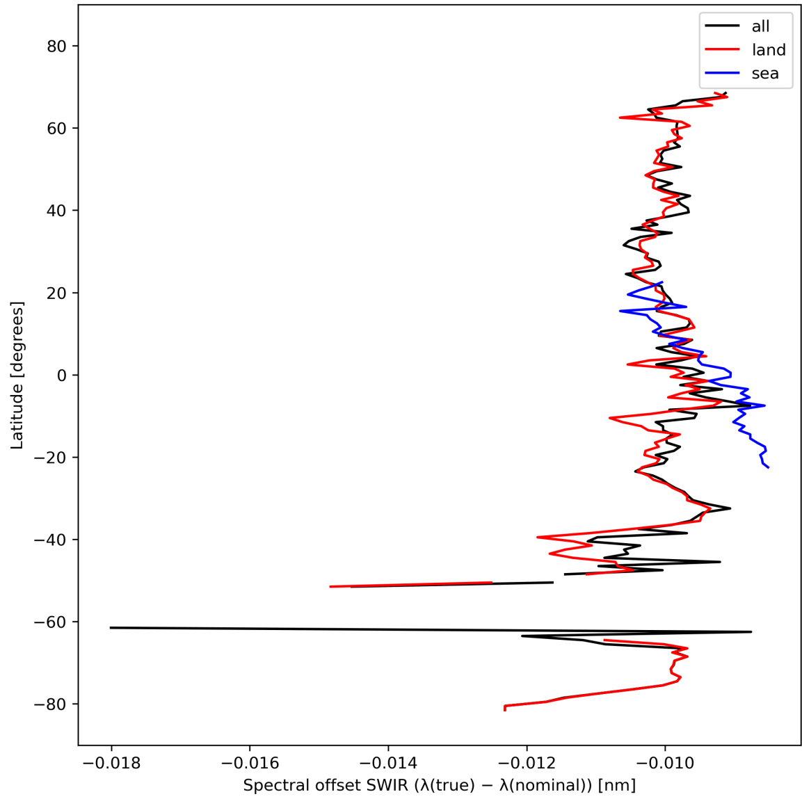
Figure 16: Zonal average of “Spectral offset SWIR ( \lambda(\text{true}) - \lambda(\text{nominal}) )” for 2023-10-10 to 2023-10-12.
