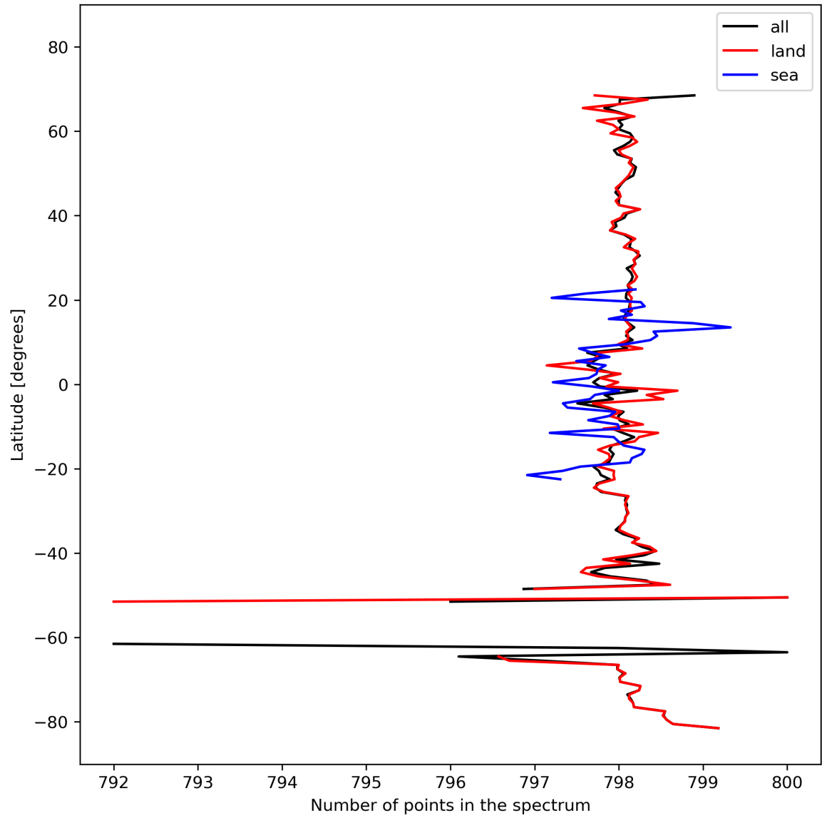
Figure 15: Zonal average of “Number of points in the spectrum” for 2023-10-10 to 2023-10-12.
