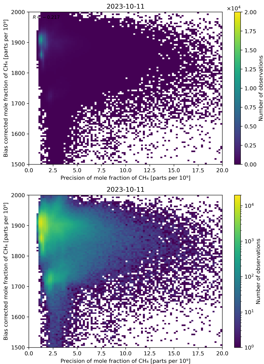
Figure 82: Scatter density plot of “Precision of mole fraction of CH 4 ” against “Bias corrected mole fraction of CH 4 ” for 2023-10-10 to 2023-10-12.
