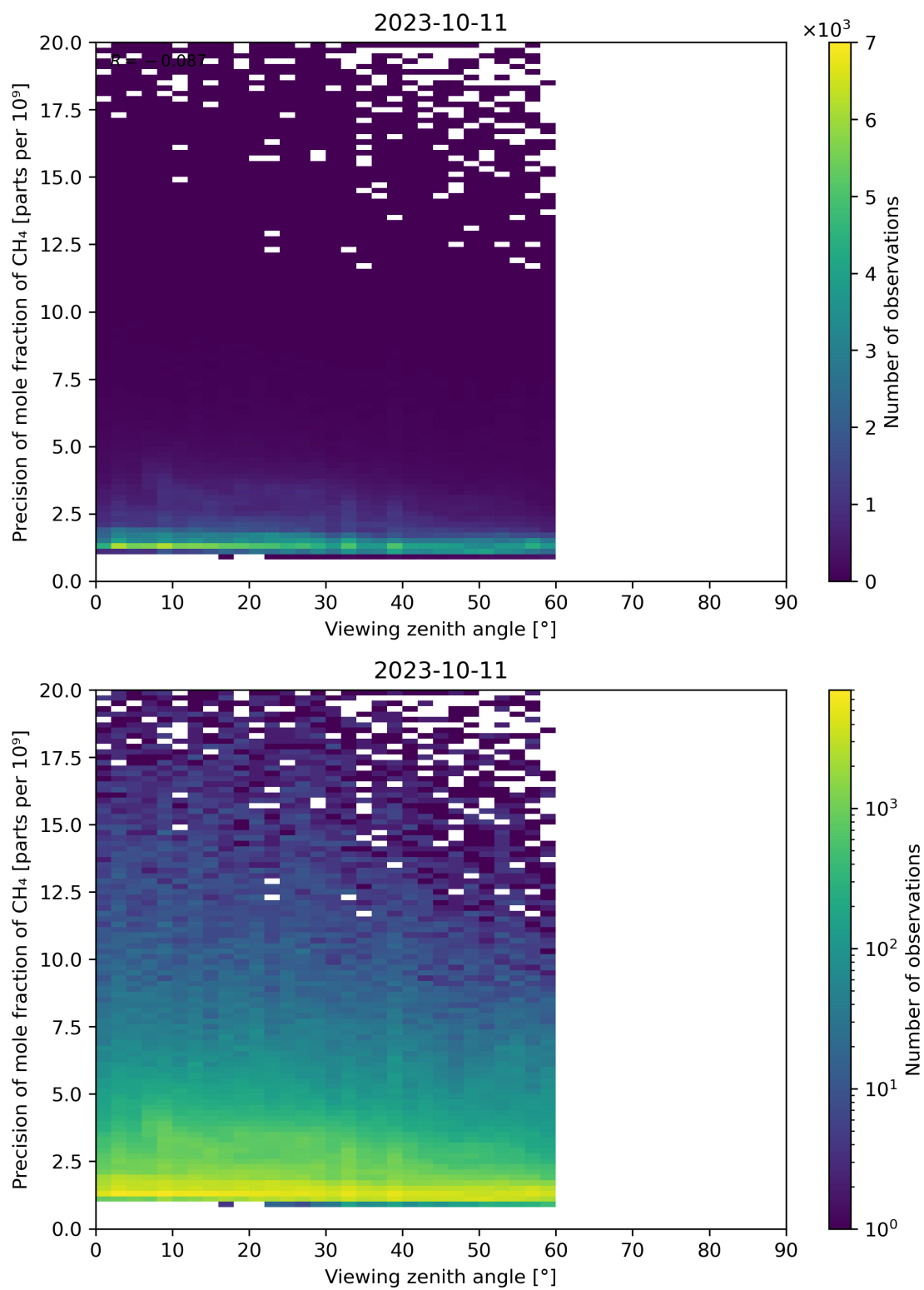
Figure 112: Scatter density plot of “Viewing zenith angle” against “Precision of mole fraction of CH 4 ” for 2023-10-10 to 2023-10-12.
