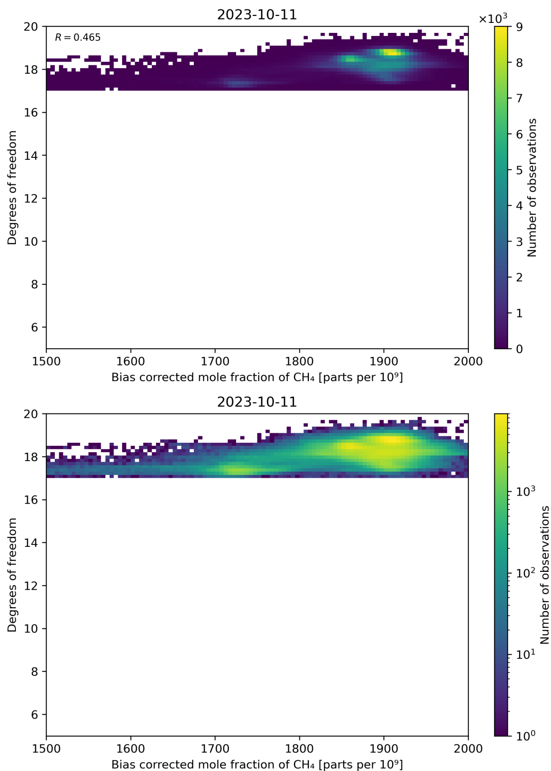
Figure 65: Scatter density plot of “Bias corrected mole fraction of CH 4 ” against “Degrees of freedom” for 2023-10-10 to 2023-10-12.
