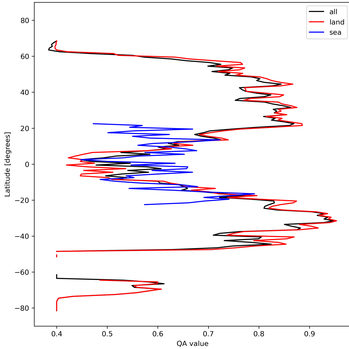
Figure 11: Zonal average of “QA value” for 2023-10-10 to 2023-10-12.
