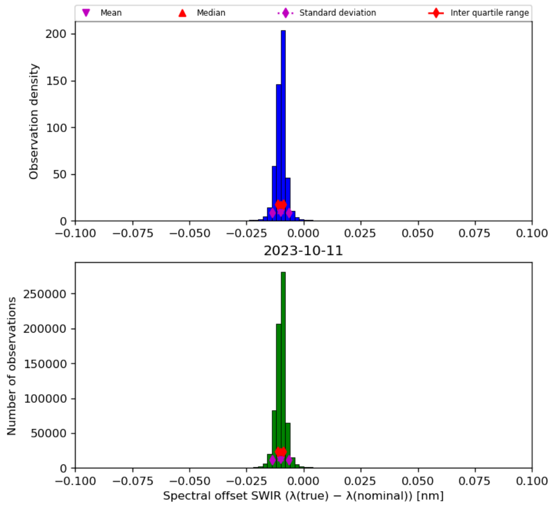
Figure 27: Histogram of “Spectral offset SWIR ( \lambda(\text{true}) - \lambda(\text{nominal}) )” for 2023-10-10 to 2023-10-12
