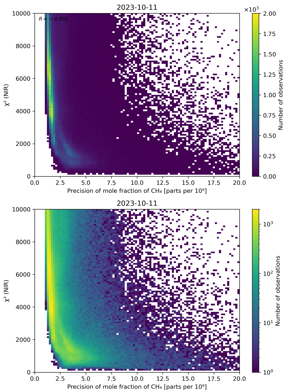
Figure 78: Scatter density plot of “Precision of mole fraction of CH 4 ” against “ \chi^2 (NIR)” for 2023-10-10 to 2023-10-12.
