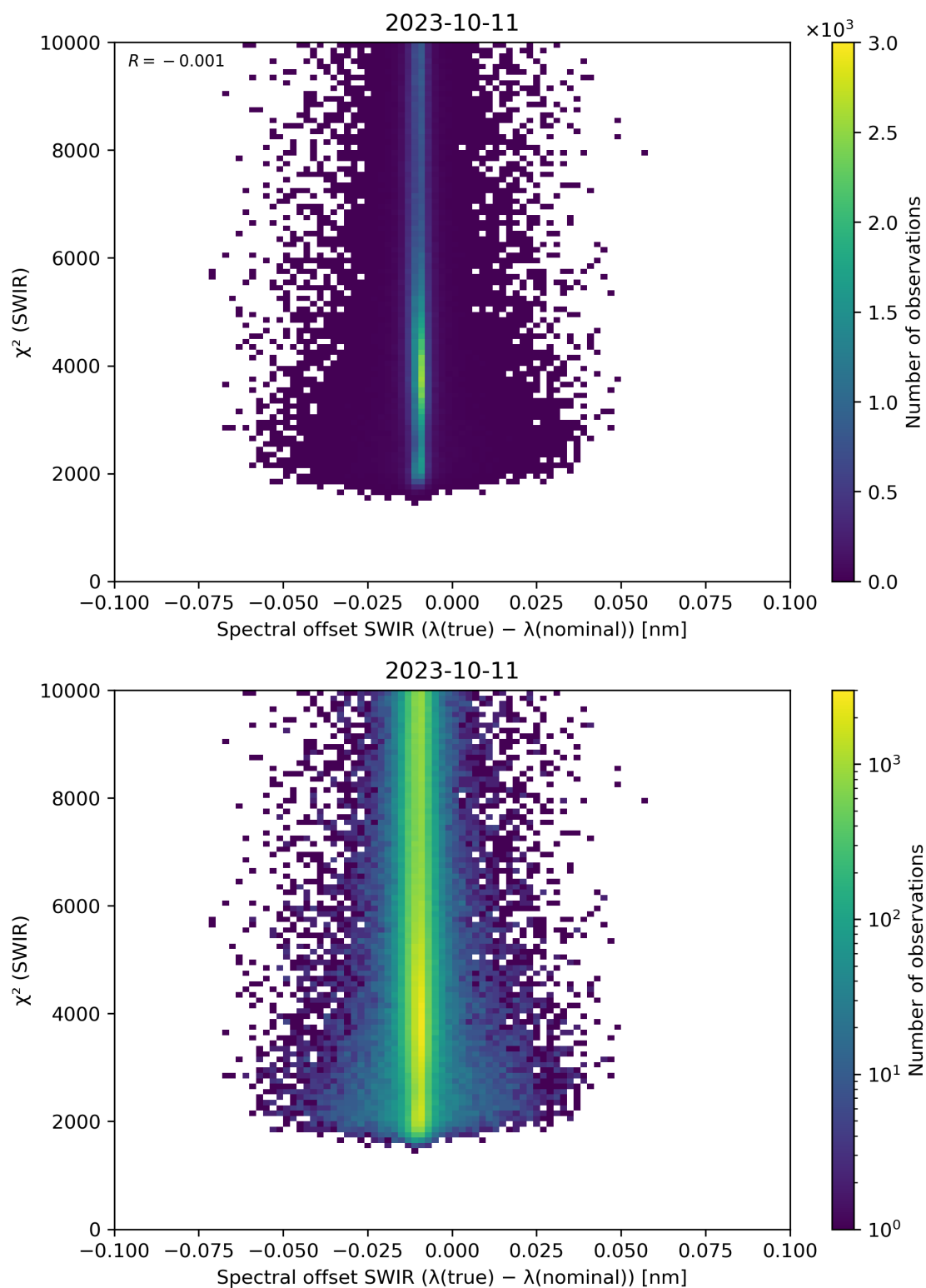
Figure 118: Scatter density plot of “Spectral offset SWIR ( \lambda(\text{true}) - \lambda(\text{nominal}) )” against “ \chi^2 (SWIR)” for 2023-10-10 to 2023-10-12.
