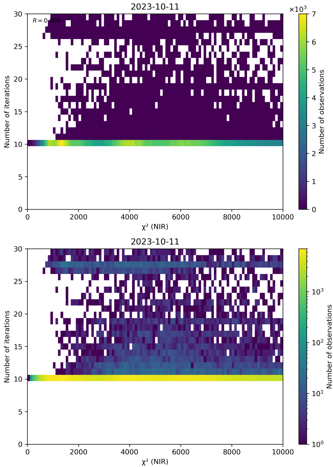
Figure 46: Scatter density plot of “ \chi^2 (NIR)” against “Number of iterations” for 2023-10-10 to 2023-10-12.
