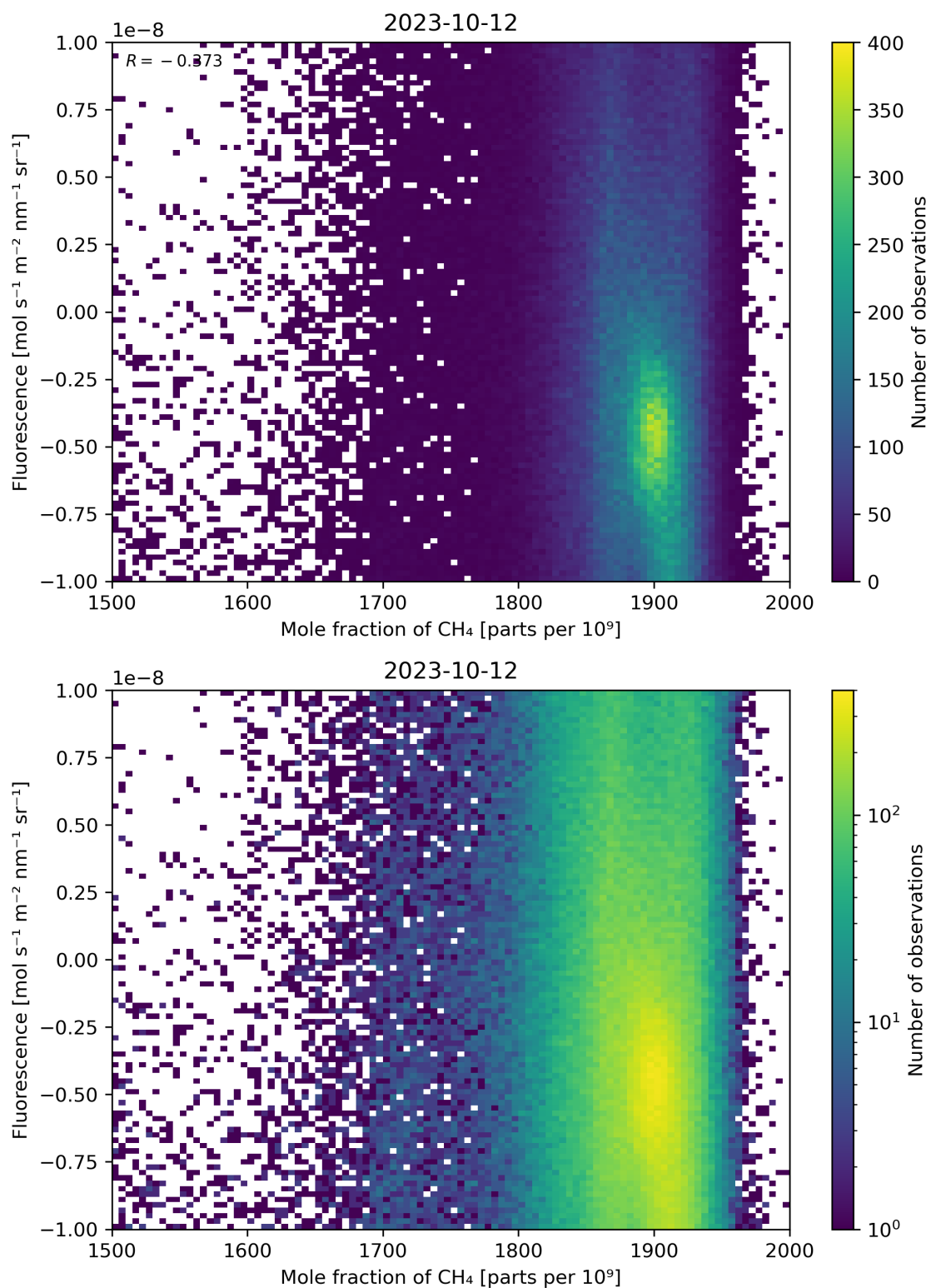
Figure 73: Scatter density plot of “Mole fraction of \text{CH}_4 ” against “Fluorescence” for 2023-10-12 to 2023-10-13.
