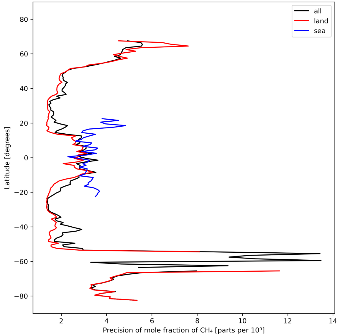
Figure 13: Zonal average of “Precision of mole fraction of CH 4 ” for 2023-10-12 to 2023-10-13.
