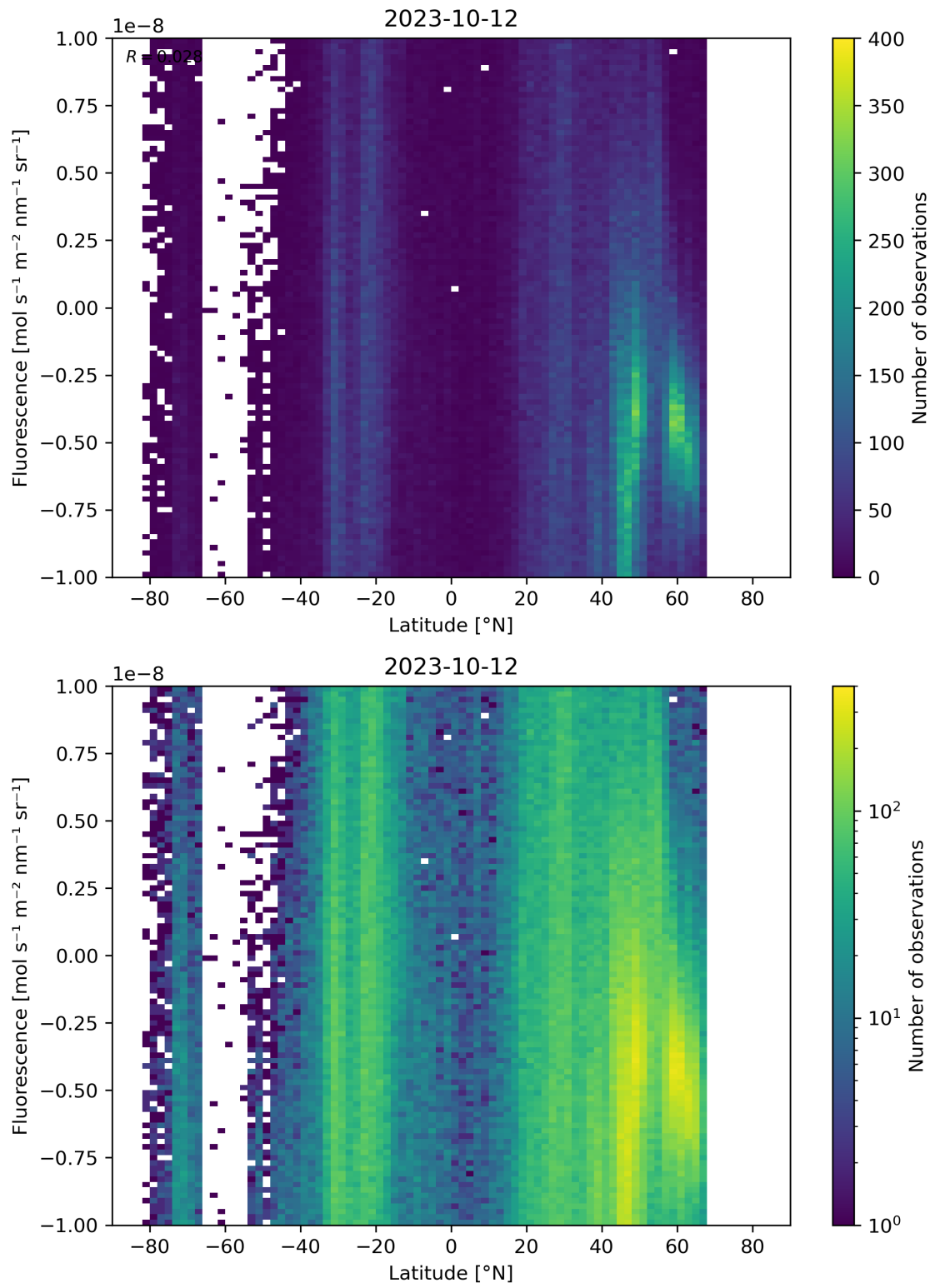
Figure 56: Scatter density plot of “Latitude” against “Fluorescence” for 2023-10-12 to 2023-10-13.
