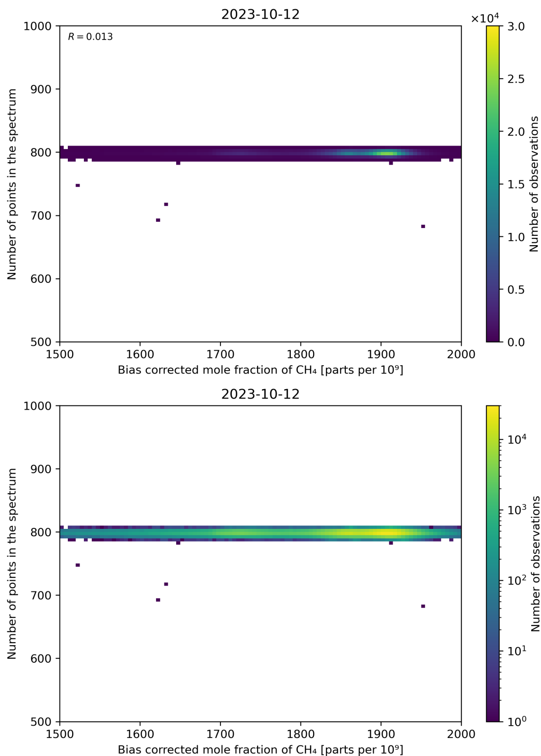
Figure 68: Scatter density plot of “Bias corrected mole fraction of CH 4 ” against “Number of points in the spectrum” for 2023-10-12 to 2023-10-13.
