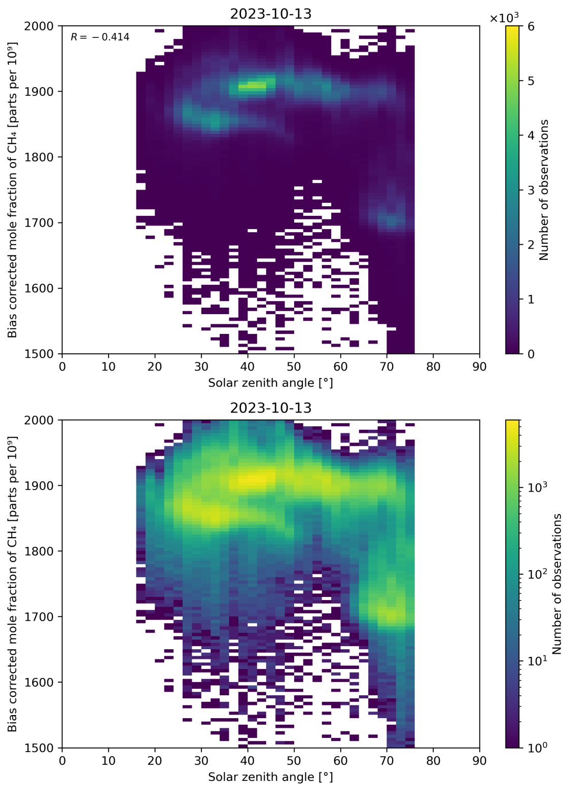
Figure 100: Scatter density plot of “Solar zenith angle” against “Bias corrected mole fraction of CH 4 ” for 2023-10-12 to 2023-10-14.
