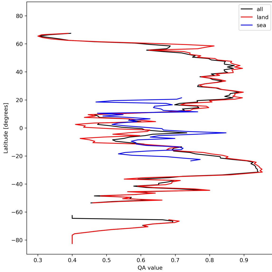
Figure 11: Zonal average of “QA value” for 2023-10-12 to 2023-10-14.
