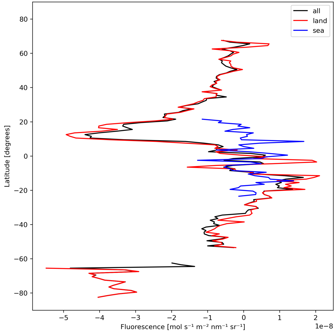
Figure 21: Zonal average of “Fluorescence” for 2023-10-12 to 2023-10-14.
