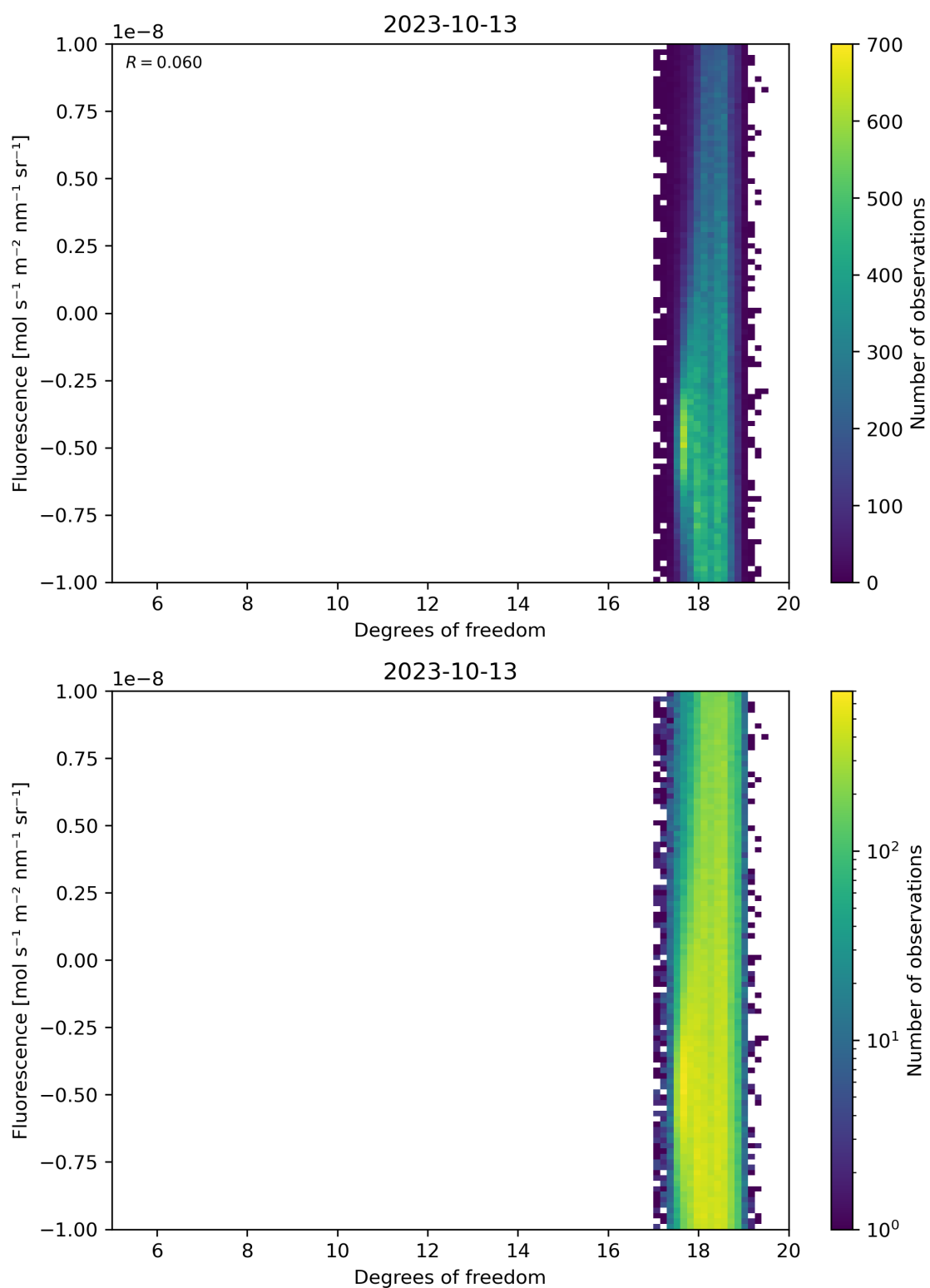
Figure 51: Scatter density plot of “Degrees of freedom” against “Fluorescence” for 2023-10-12 to 2023-10-14.
