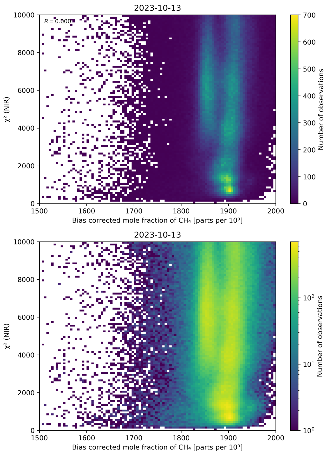
Figure 63: Scatter density plot of “Bias corrected mole fraction of CH 4 ” against “ \chi^2 (NIR)” for 2023-10-12 to 2023-10-14.
