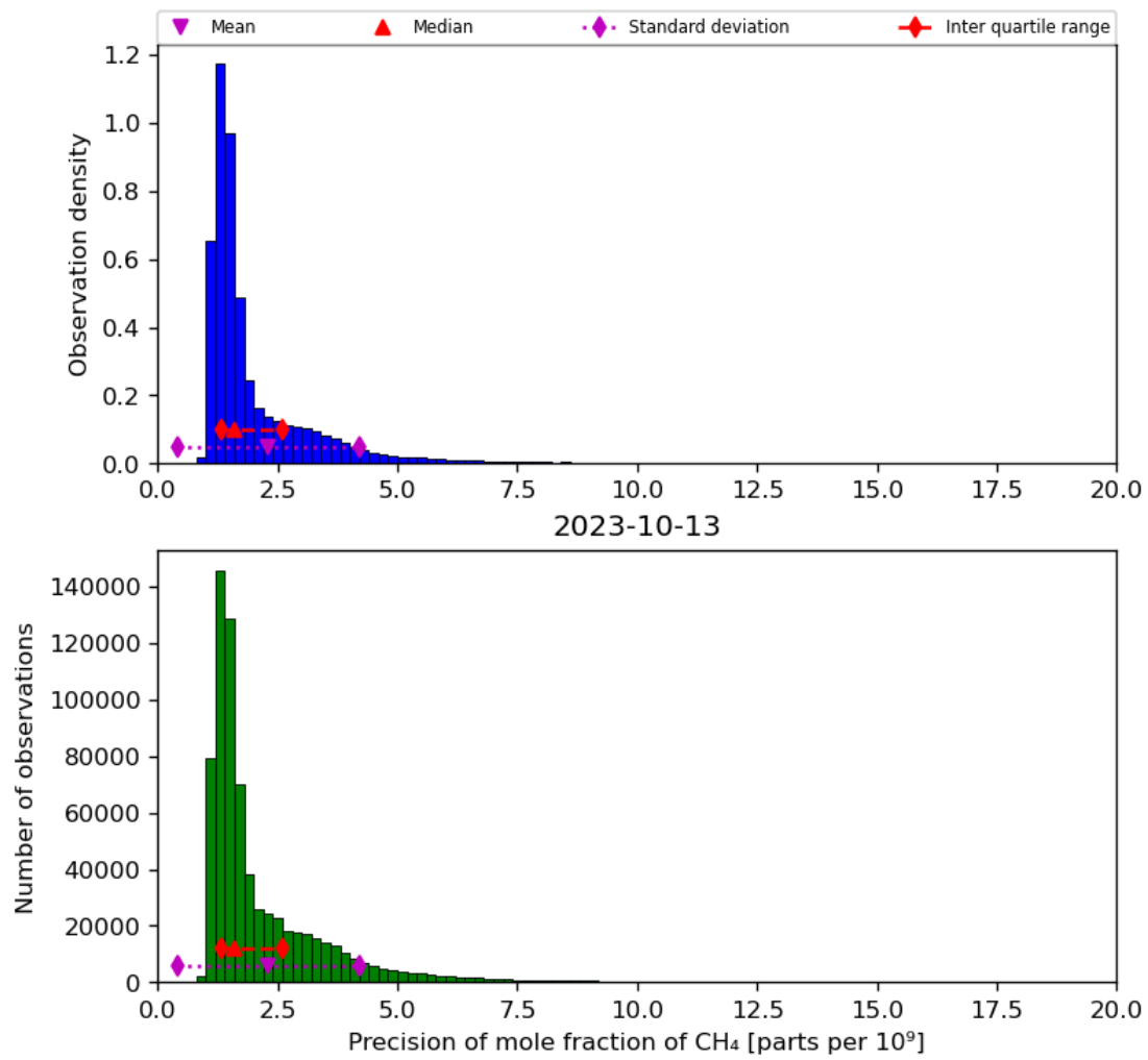
Figure 24: Histogram of “Precision of mole fraction of CH 4 ” for 2023-10-12 to 2023-10-14
