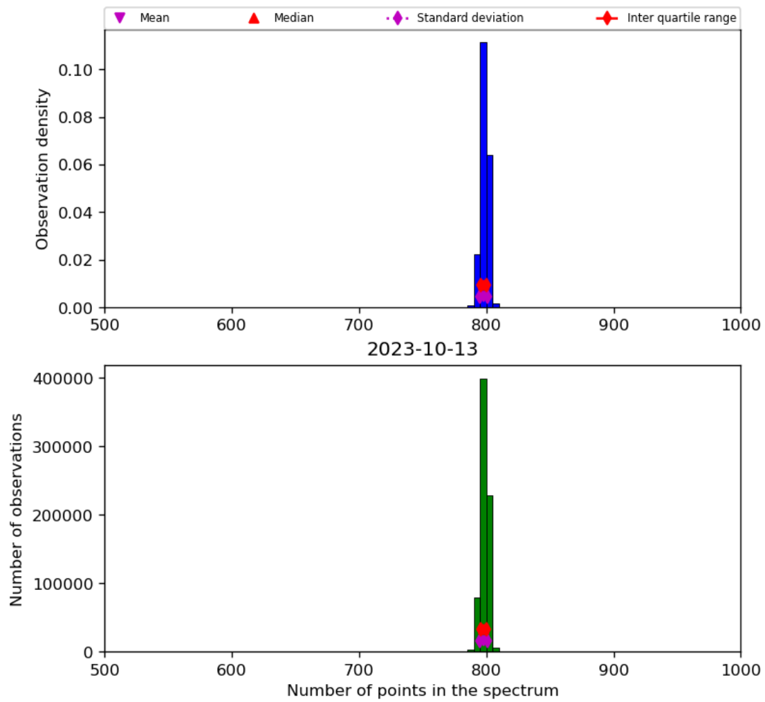
Figure 26: Histogram of “Number of points in the spectrum” for 2023-10-12 to 2023-10-14
