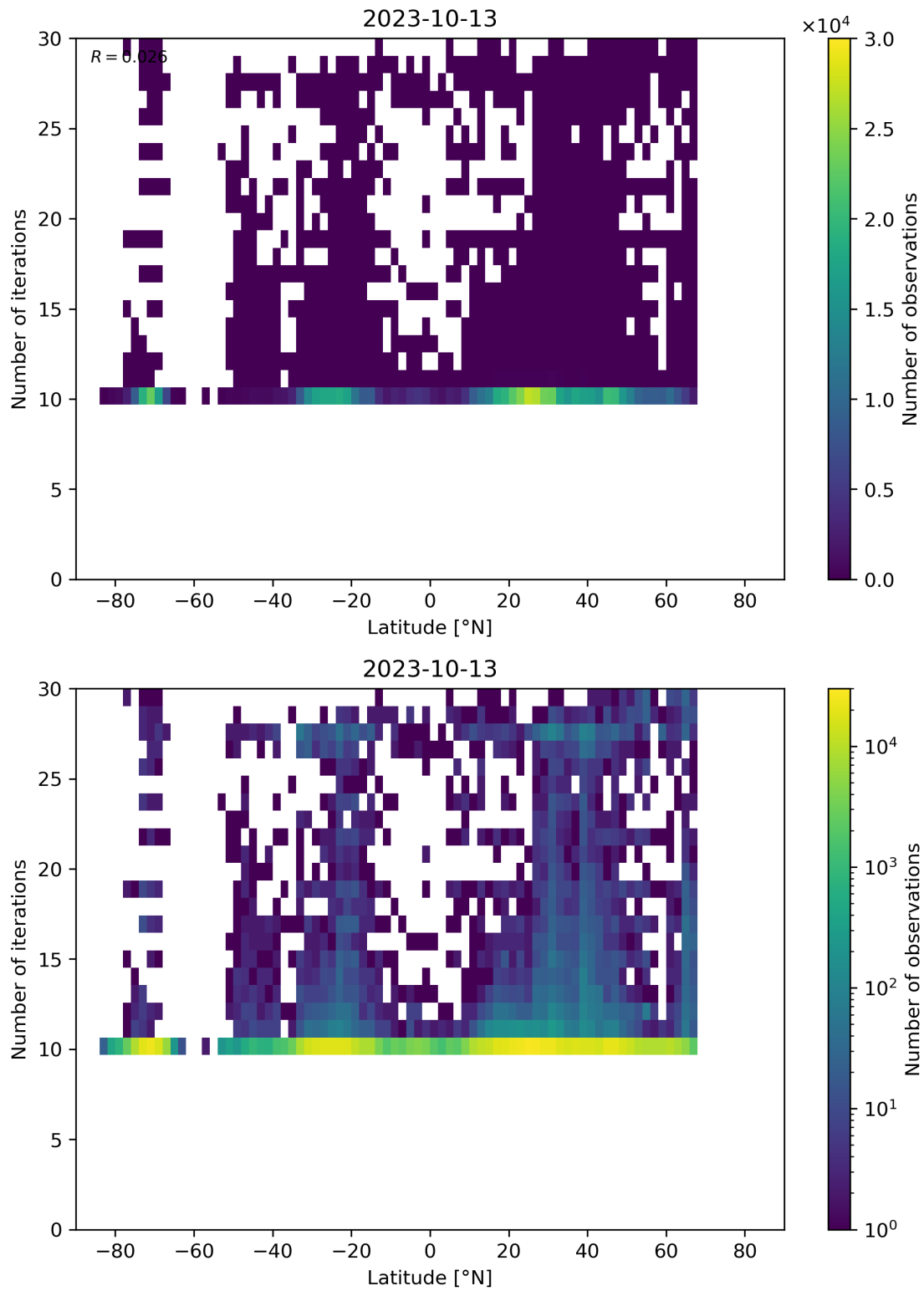
Figure 60: Scatter density plot of “Latitude” against “Number of iterations” for 2023-10-12 to 2023-10-14.
