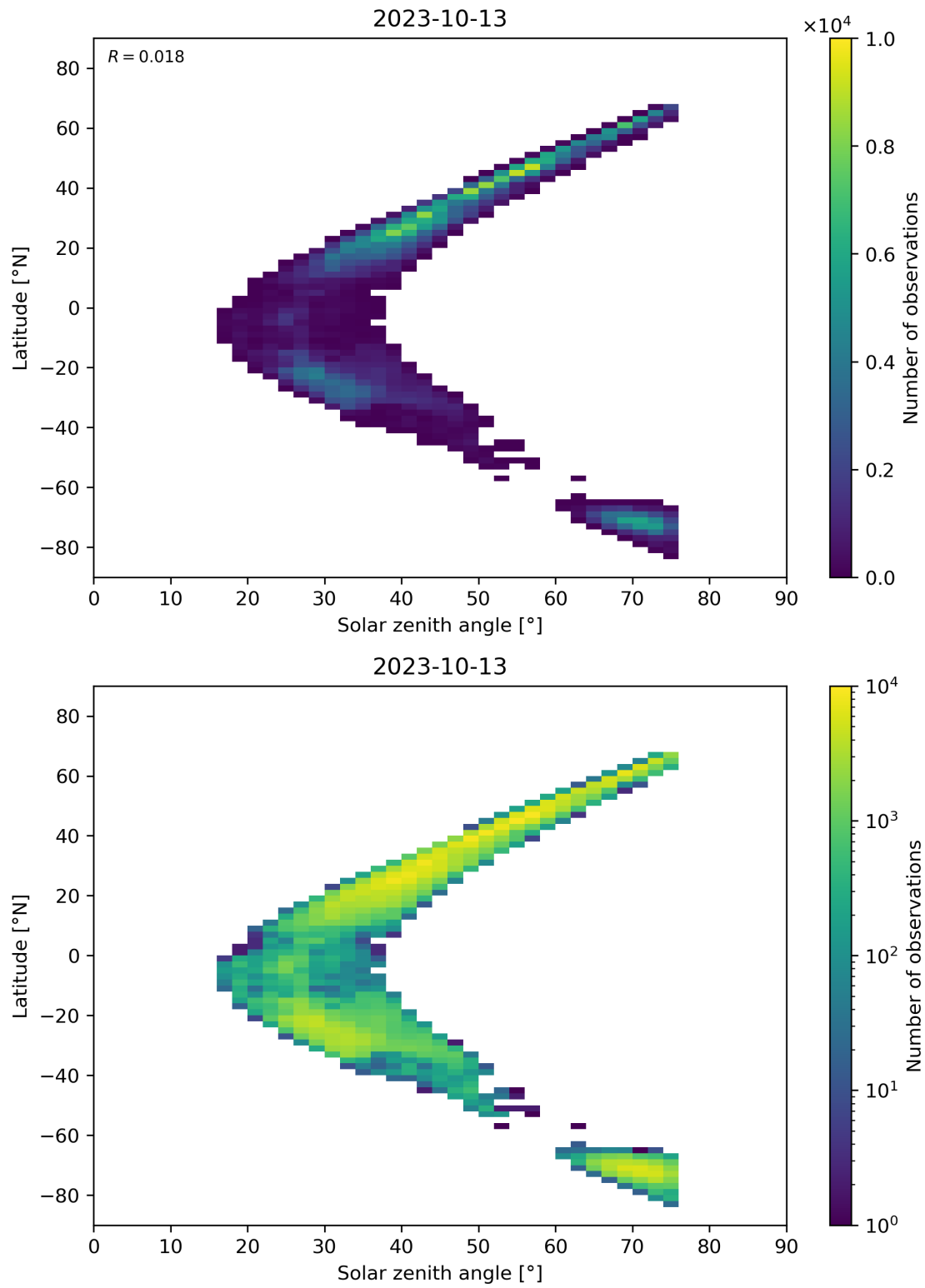
Figure 98: Scatter density plot of “Solar zenith angle” against “Latitude” for 2023-10-12 to 2023-10-14.
