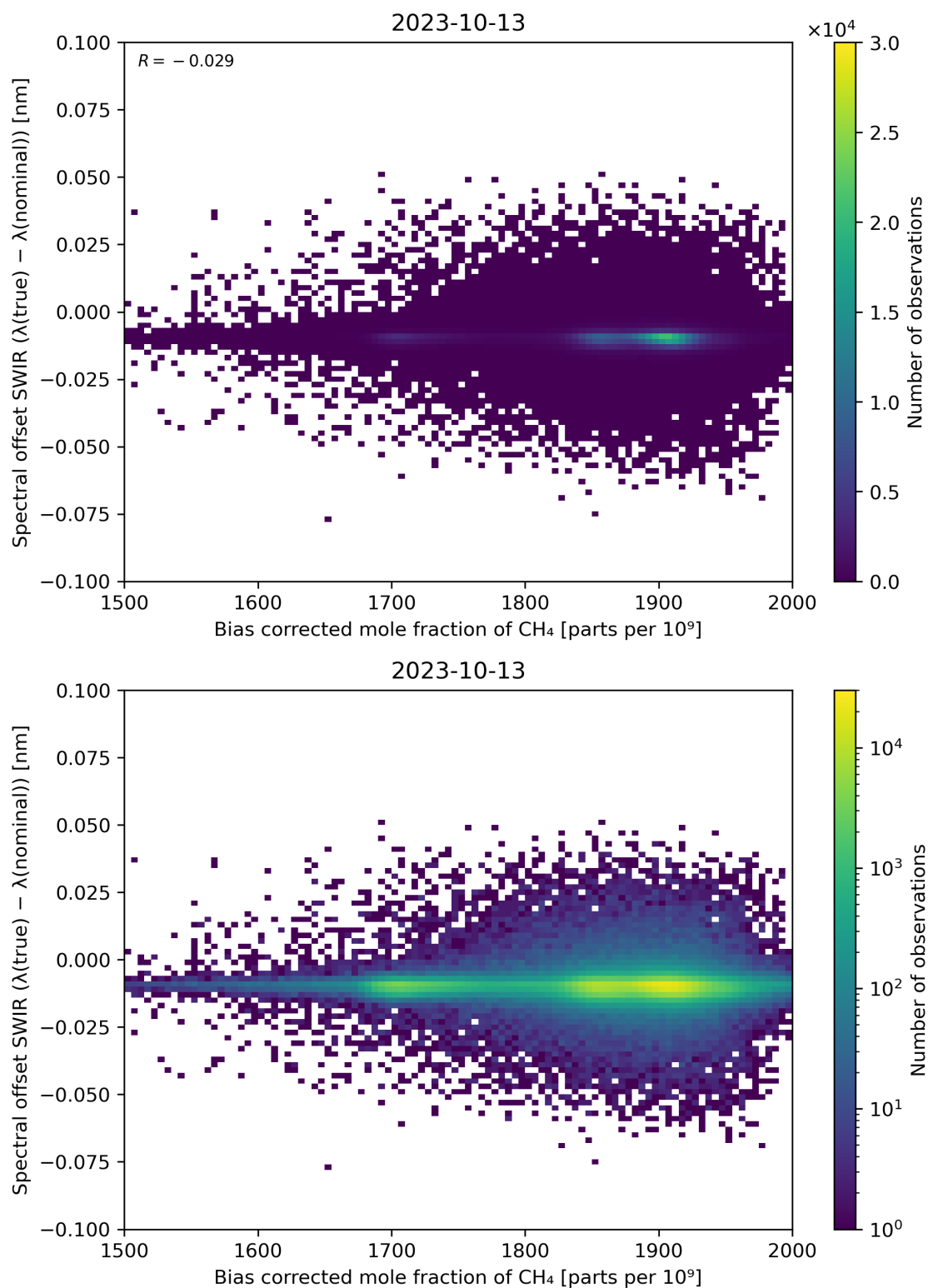
Figure 69: Scatter density plot of “Bias corrected mole fraction of \text{CH}_4 ” against “Spectral offset SWIR ( \lambda(\text{true}) - \lambda(\text{nominal}) )” for 2023-10-12 to 2023-10-14.
