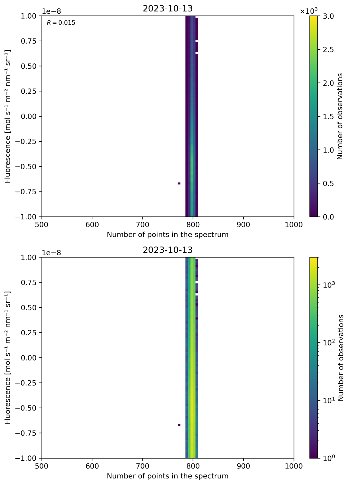
Figure 91: Scatter density plot of “Number of points in the spectrum” against “Fluorescence” for 2023-10-12 to 2023-10-14.
