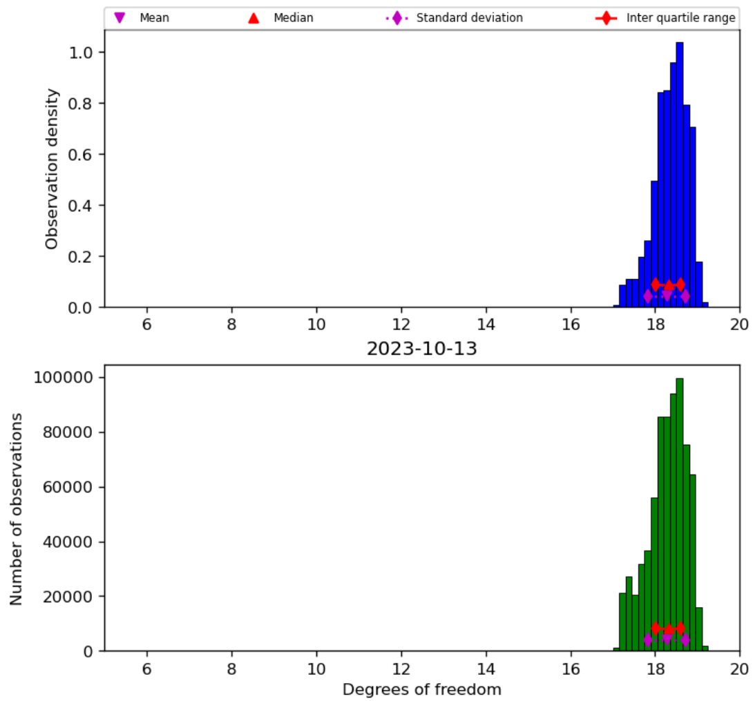
Figure 30: Histogram of “Degrees of freedom” for 2023-10-12 to 2023-10-14
