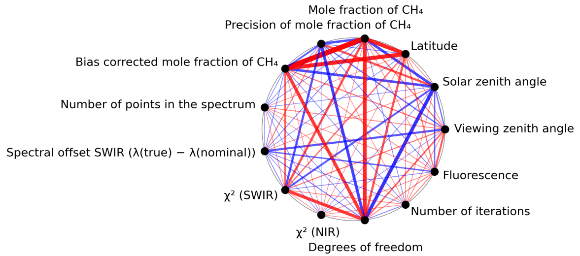
Figure 1: Map of correlation graph for 2023-10-12 to 2023-10-14.
