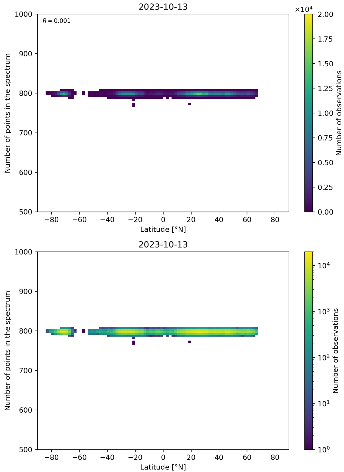
Figure 61: Scatter density plot of “Latitude” against “Number of points in the spectrum” for 2023-10-12 to 2023-10-14.
