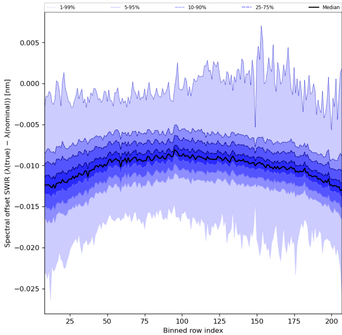
Figure 38: Along track statistics of “Spectral offset SWIR ( \lambda(\text{true}) - \lambda(\text{nominal}) )” for 2023-10-12 to 2023-10-14
