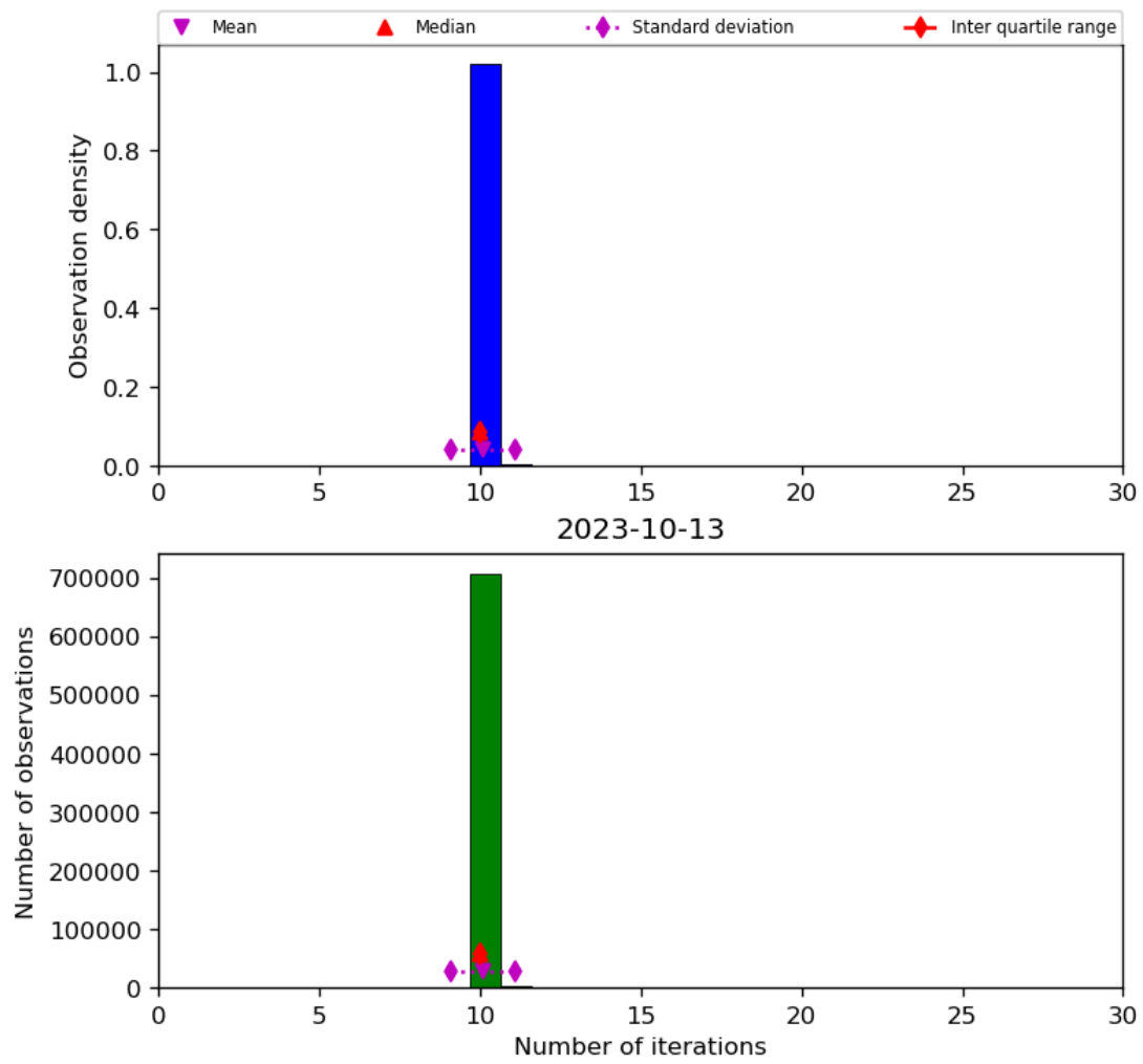
Figure 31: Histogram of “Number of iterations” for 2023-10-12 to 2023-10-14
