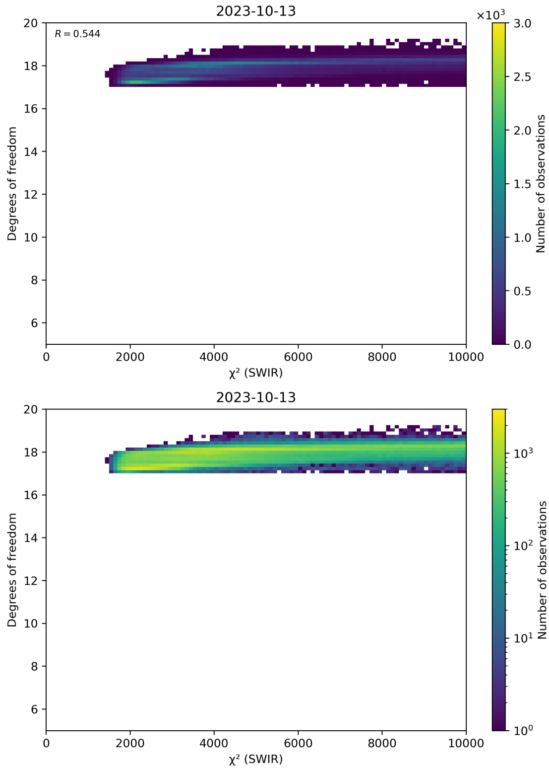
Figure 48: Scatter density plot of “ \chi^2 (SWIR)” against “Degrees of freedom” for 2023-10-12 to 2023-10-14.
