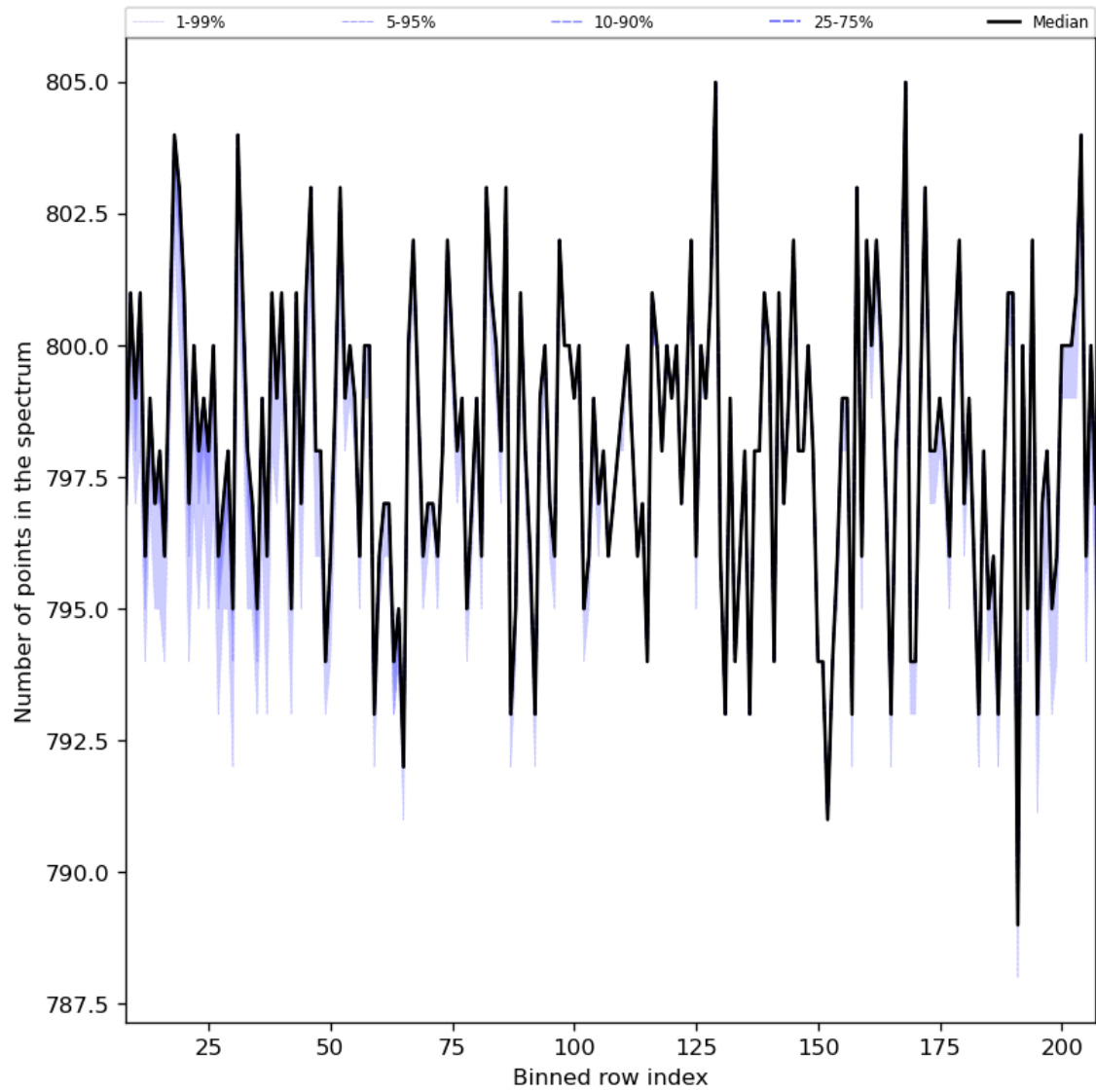
Figure 37: Along track statistics of “Number of points in the spectrum” for 2023-10-12 to 2023-10-14
