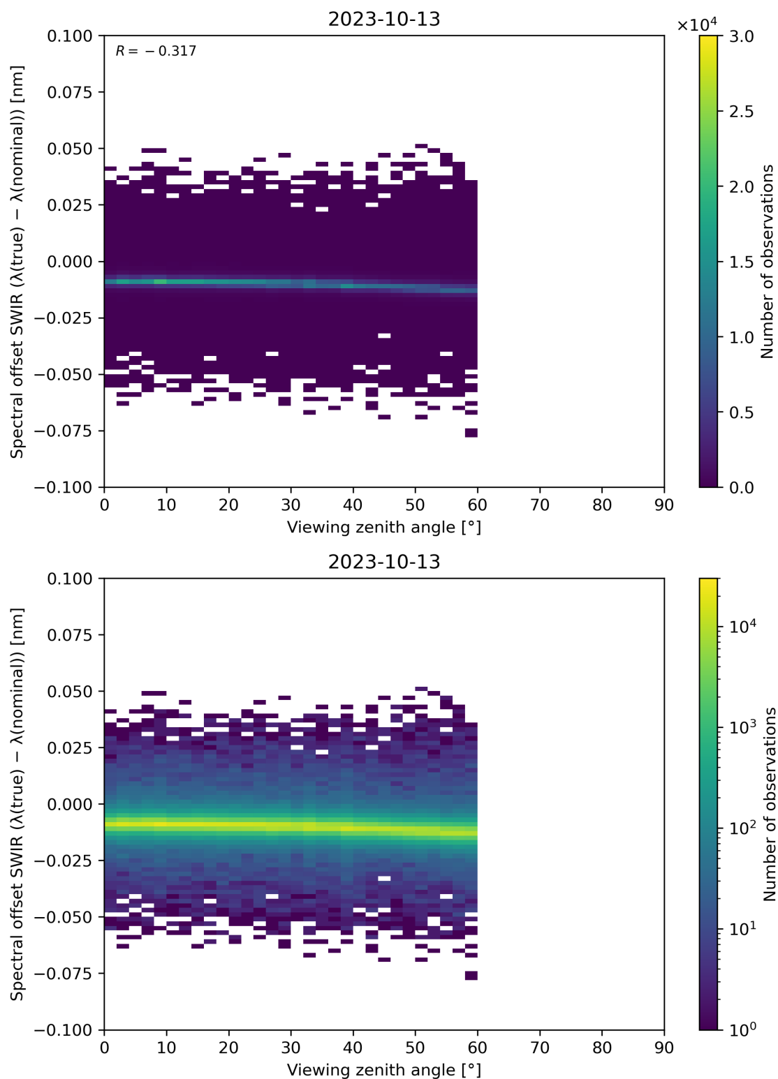
Figure 116: Scatter density plot of “Viewing zenith angle” against “Spectral offset SWIR ( \lambda(\text{true}) - \lambda(\text{nominal}) )” for 2023-10-12 to 2023-10-14.
