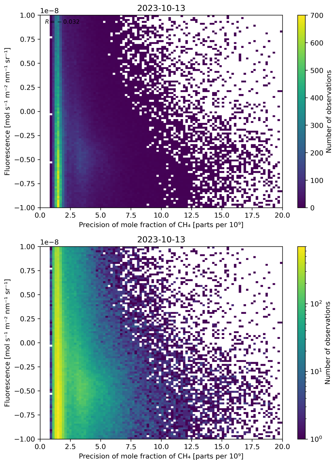
Figure 81: Scatter density plot of “Precision of mole fraction of \text{CH}_4 ” against “Fluorescence” for 2023-10-12 to 2023-10-14.
