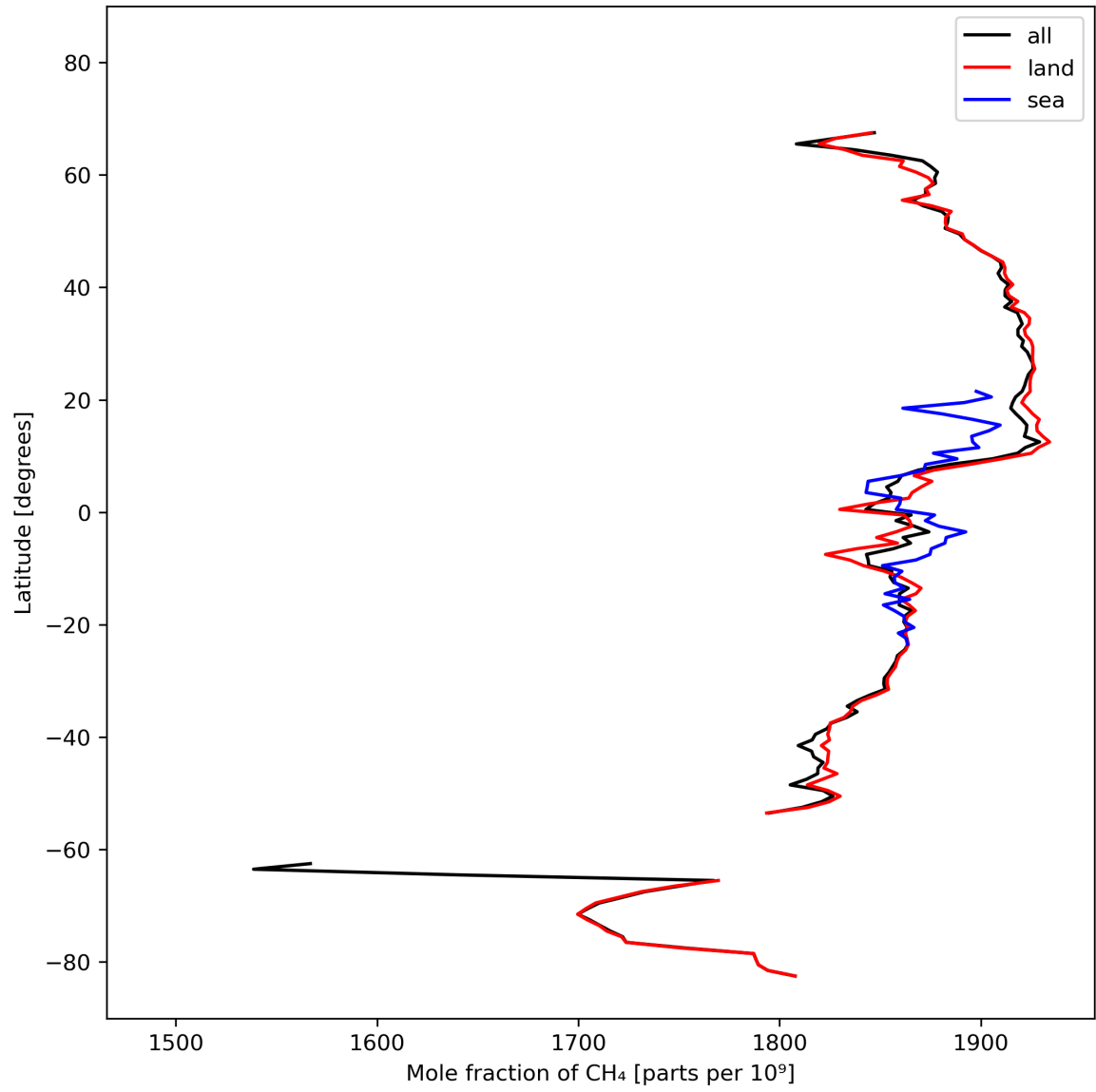
Figure 12: Zonal average of “Mole fraction of \text{CH}_4 ” for 2023-10-12 to 2023-10-14.
