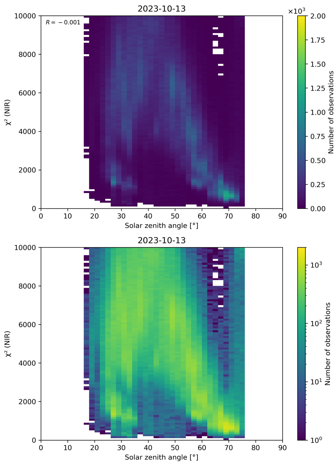
Figure 94: Scatter density plot of “Solar zenith angle” against “ \chi^2 (NIR)” for 2023-10-12 to 2023-10-14.
