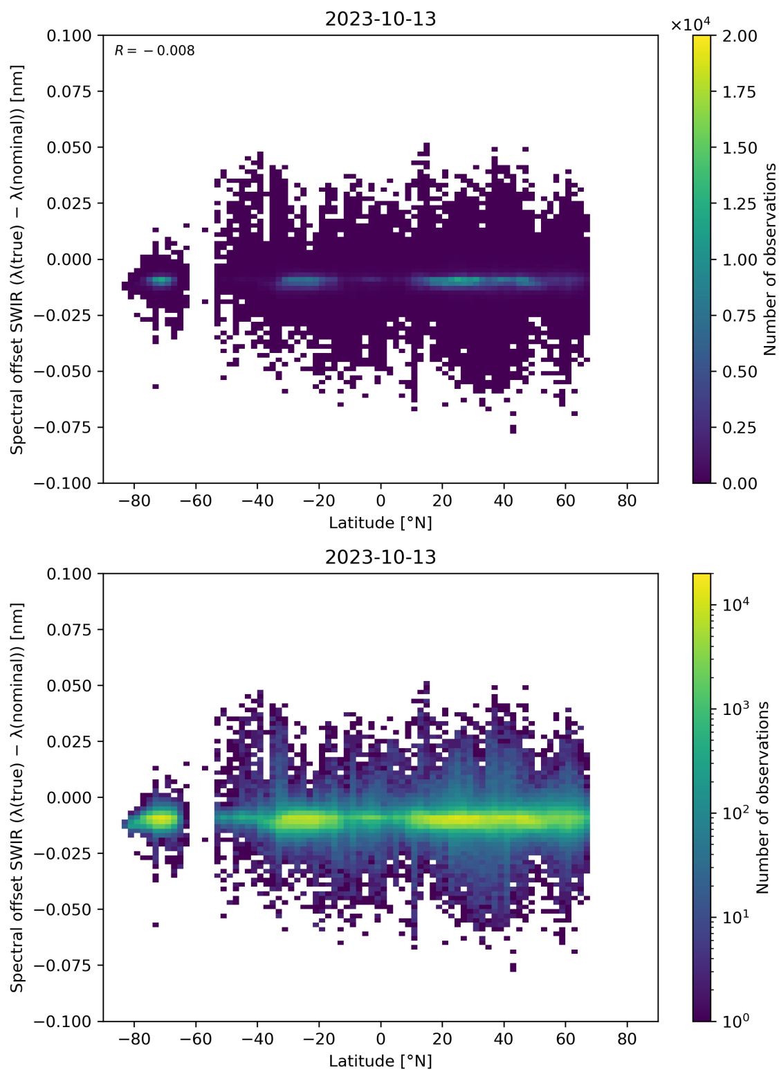
Figure 62: Scatter density plot of “Latitude” against “Spectral offset SWIR ( \lambda(\text{true}) - \lambda(\text{nominal}) )” for 2023-10-12 to 2023-10-14.
