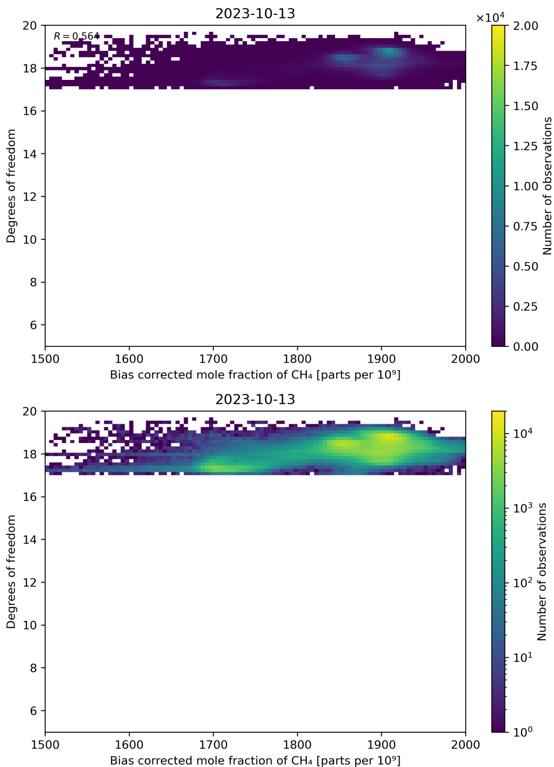
Figure 65: Scatter density plot of “Bias corrected mole fraction of CH 4 ” against “Degrees of freedom” for 2023-10-12 to 2023-10-14.
