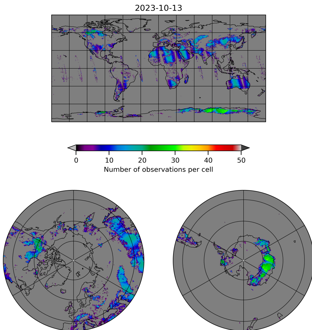
Figure 10: Map of the number of observations for 2023-10-12 to 2023-10-14
