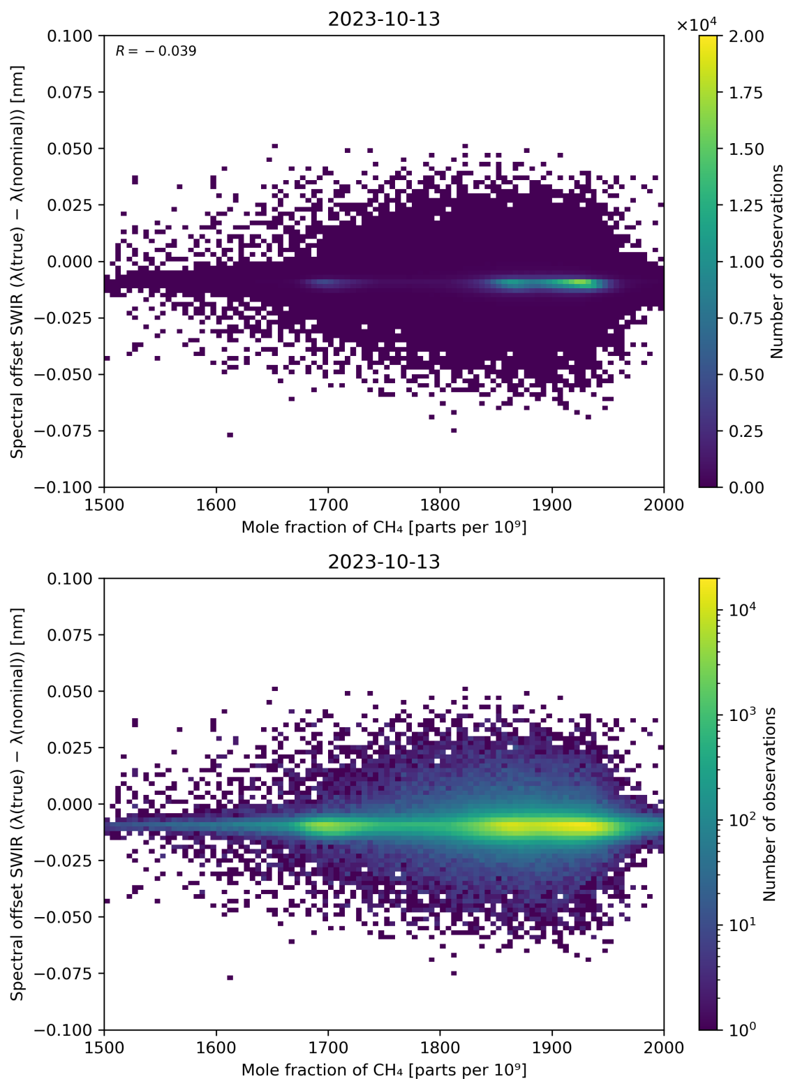
Figure 86: Scatter density plot of “Mole fraction of CH 4 ” against “Spectral offset SWIR ( \lambda(\text{true}) - \lambda(\text{nominal}) )” for 2023-10-12 to 2023-10-14.
