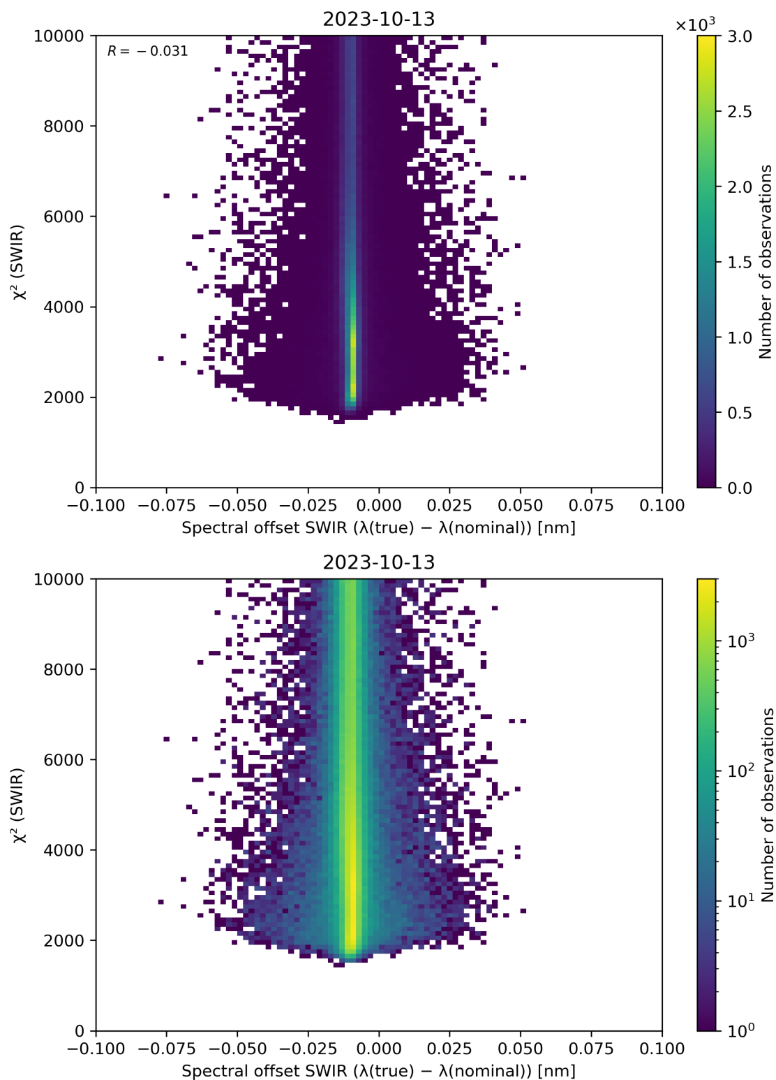
Figure 118: Scatter density plot of “Spectral offset SWIR ( \lambda(\text{true}) - \lambda(\text{nominal}) )” against “ \chi^2 (SWIR)” for 2023-10-12 to 2023-10-14.
