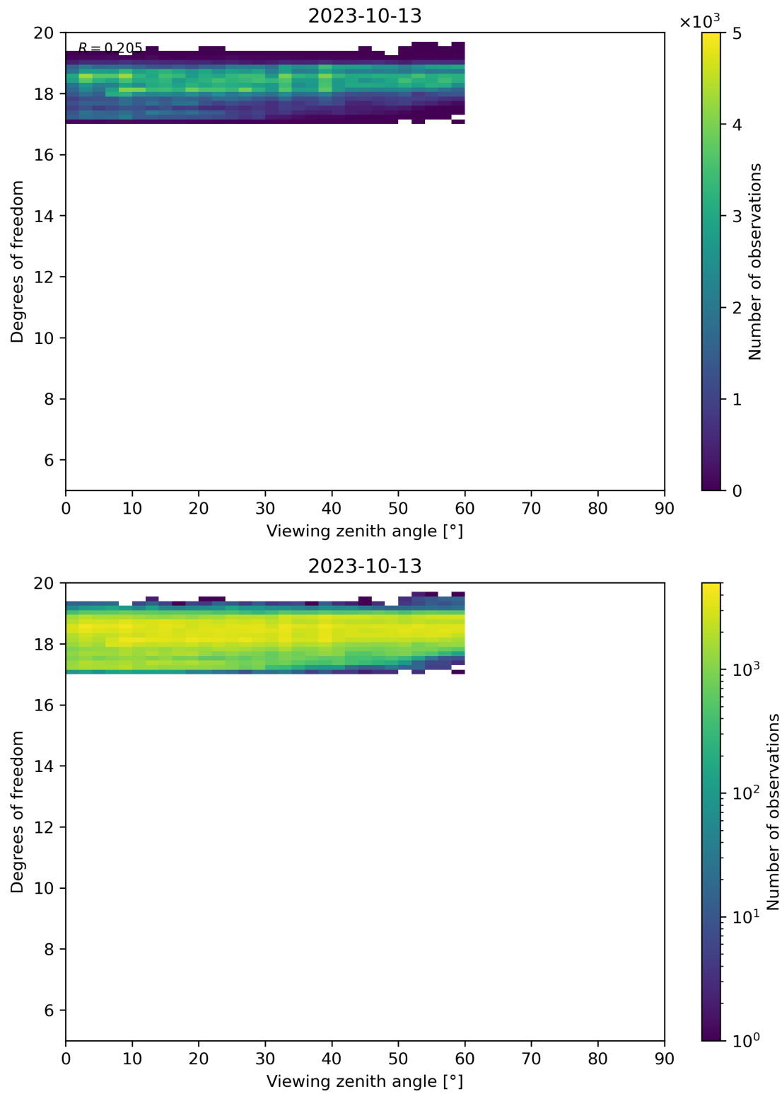
Figure 107: Scatter density plot of “Viewing zenith angle” against “Degrees of freedom” for 2023-10-12 to 2023-10-14.
