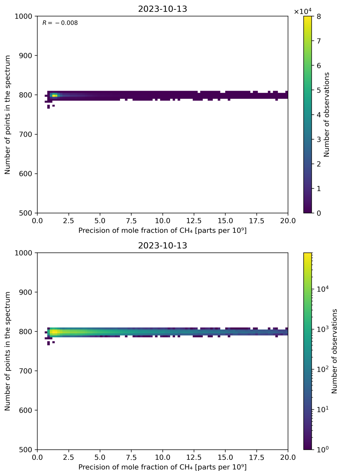
Figure 84: Scatter density plot of “Precision of mole fraction of CH 4 ” against “Number of points in the spectrum” for 2023-10-12 to 2023-10-14.
