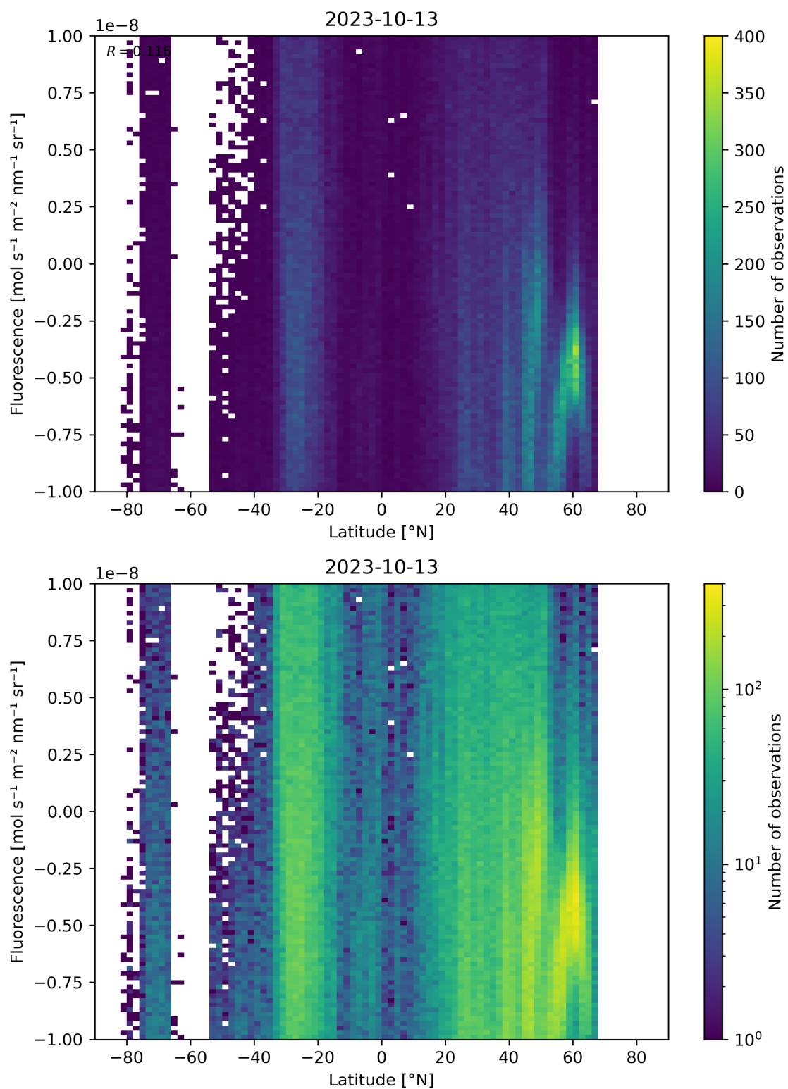
Figure 56: Scatter density plot of “Latitude” against “Fluorescence” for 2023-10-12 to 2023-10-14.
