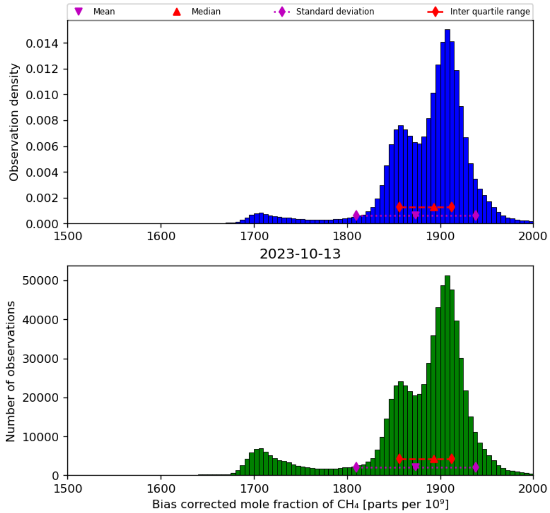
Figure 25: Histogram of “Bias corrected mole fraction of CH 4 ” for 2023-10-12 to 2023-10-14
