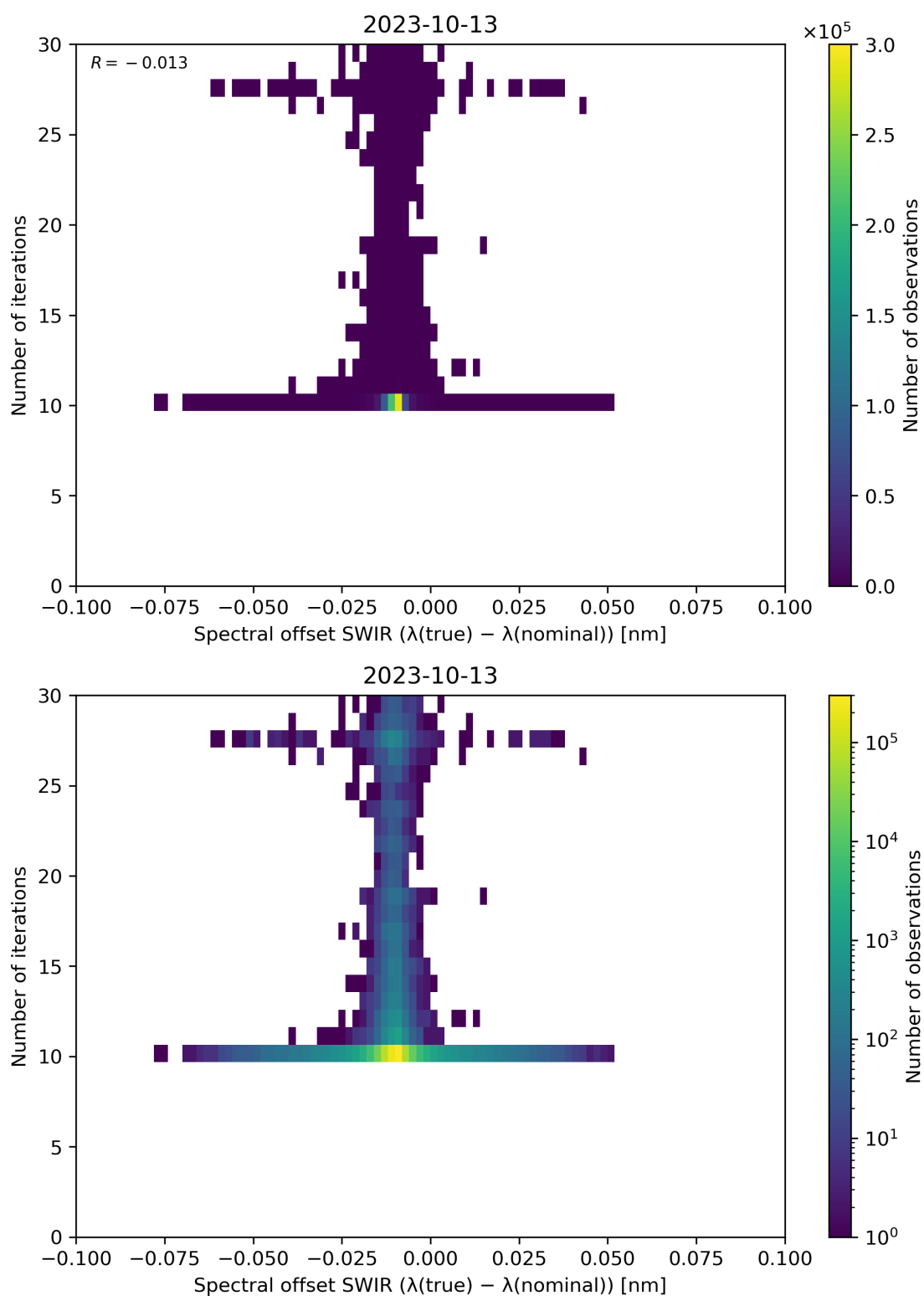
Figure 121: Scatter density plot of “Spectral offset SWIR ( \lambda(\text{true}) - \lambda(\text{nominal}) )” against “Number of iterations” for 2023-10-12 to 2023-10-14.
