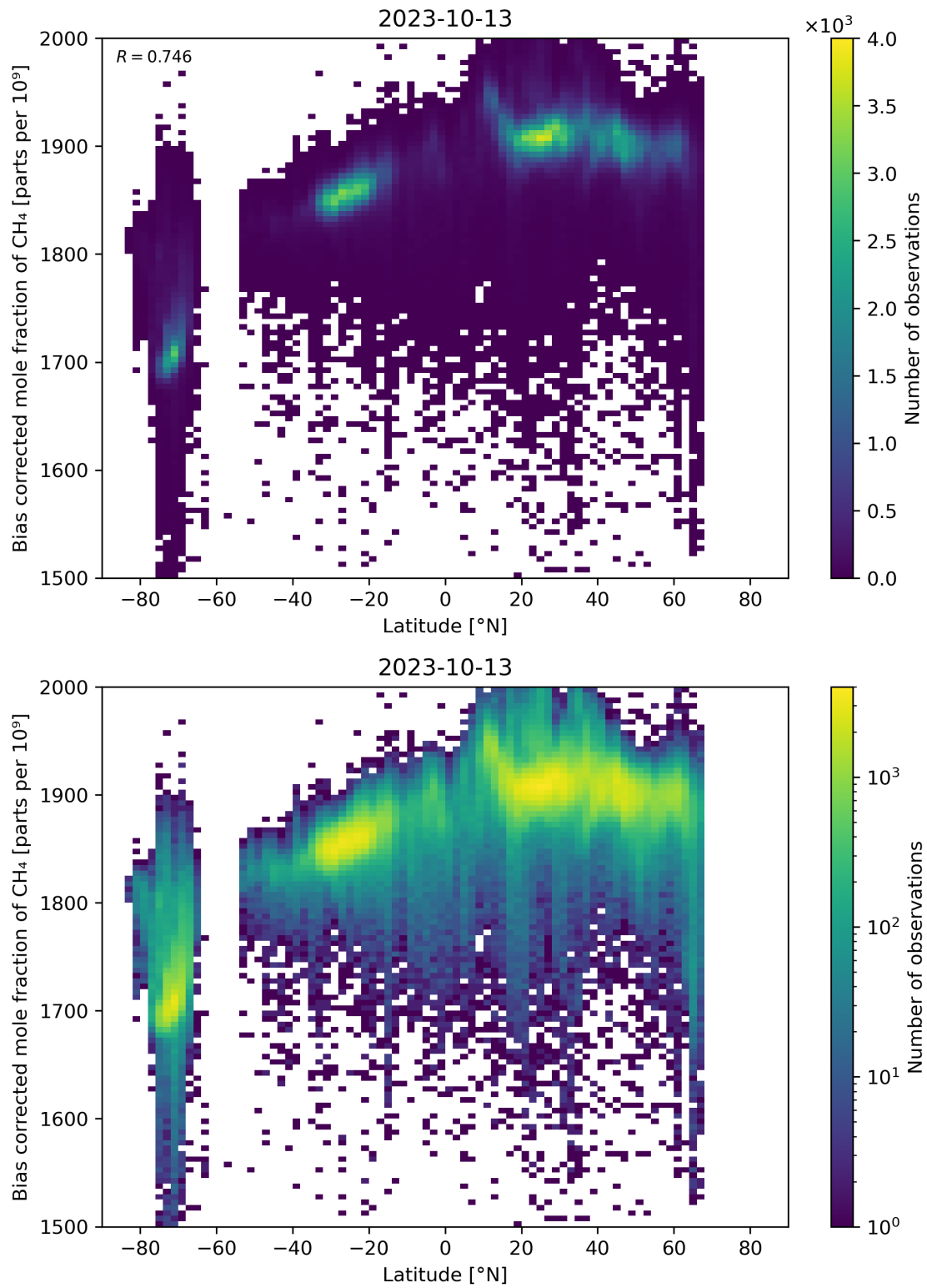
Figure 58: Scatter density plot of “Latitude” against “Bias corrected mole fraction of CH 4 ” for 2023-10-12 to 2023-10-14.
