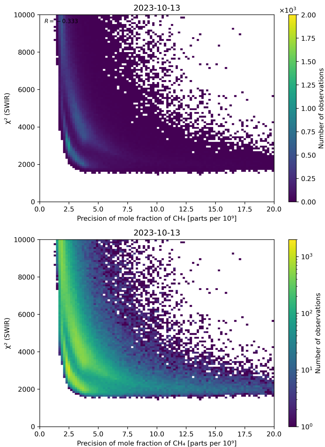
Figure 79: Scatter density plot of “Precision of mole fraction of \text{CH}_4 ” against “ \chi^2 (SWIR)” for 2023-10-12 to 2023-10-14.
