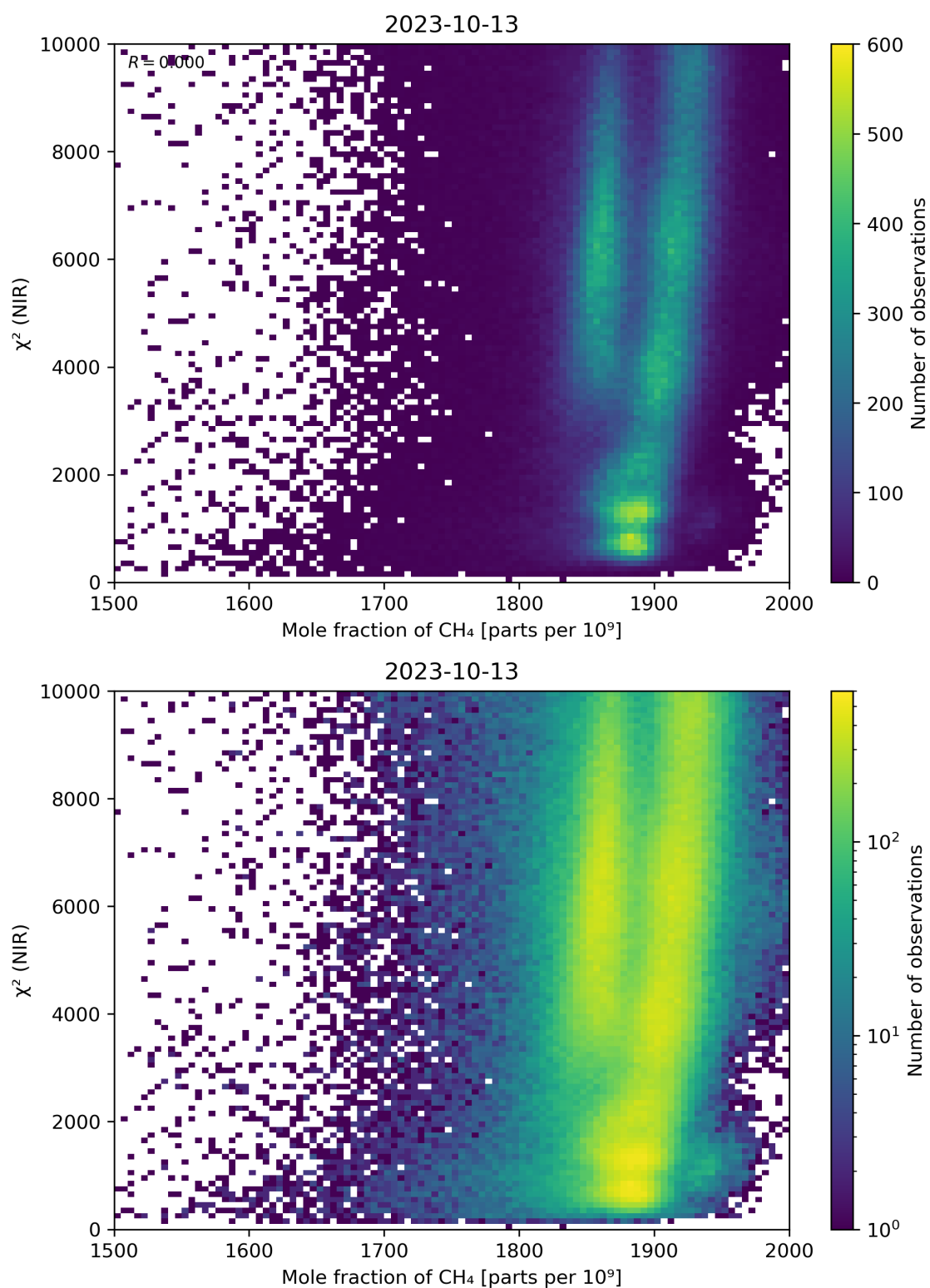
Figure 70: Scatter density plot of “Mole fraction of \text{CH}_4 ” against “ \chi^2 (NIR)” for 2023-10-12 to 2023-10-14.
