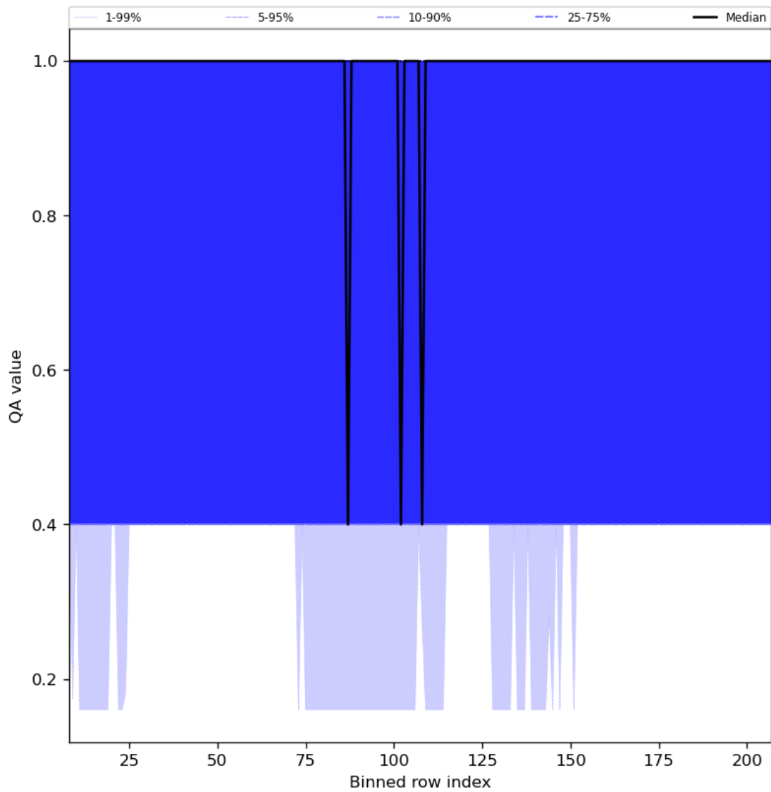
Figure 33: Along track statistics of “QA value” for 2023-10-12 to 2023-10-14
