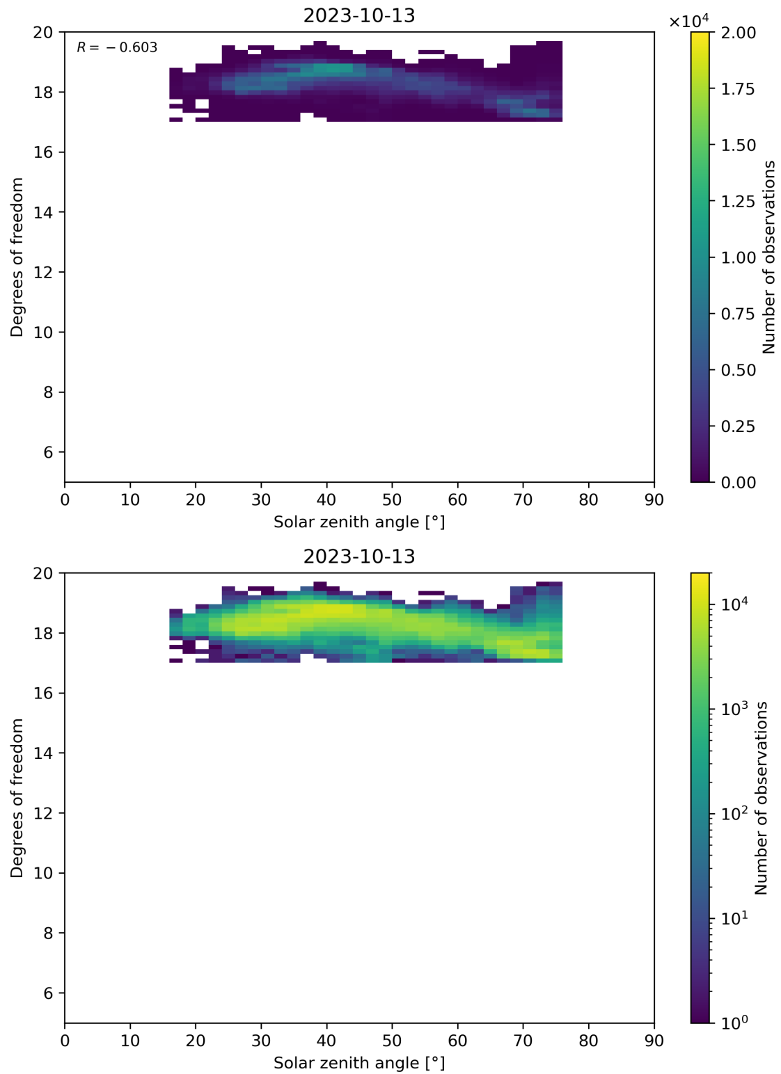
Figure 96: Scatter density plot of “Solar zenith angle” against “Degrees of freedom” for 2023-10-12 to 2023-10-14.
