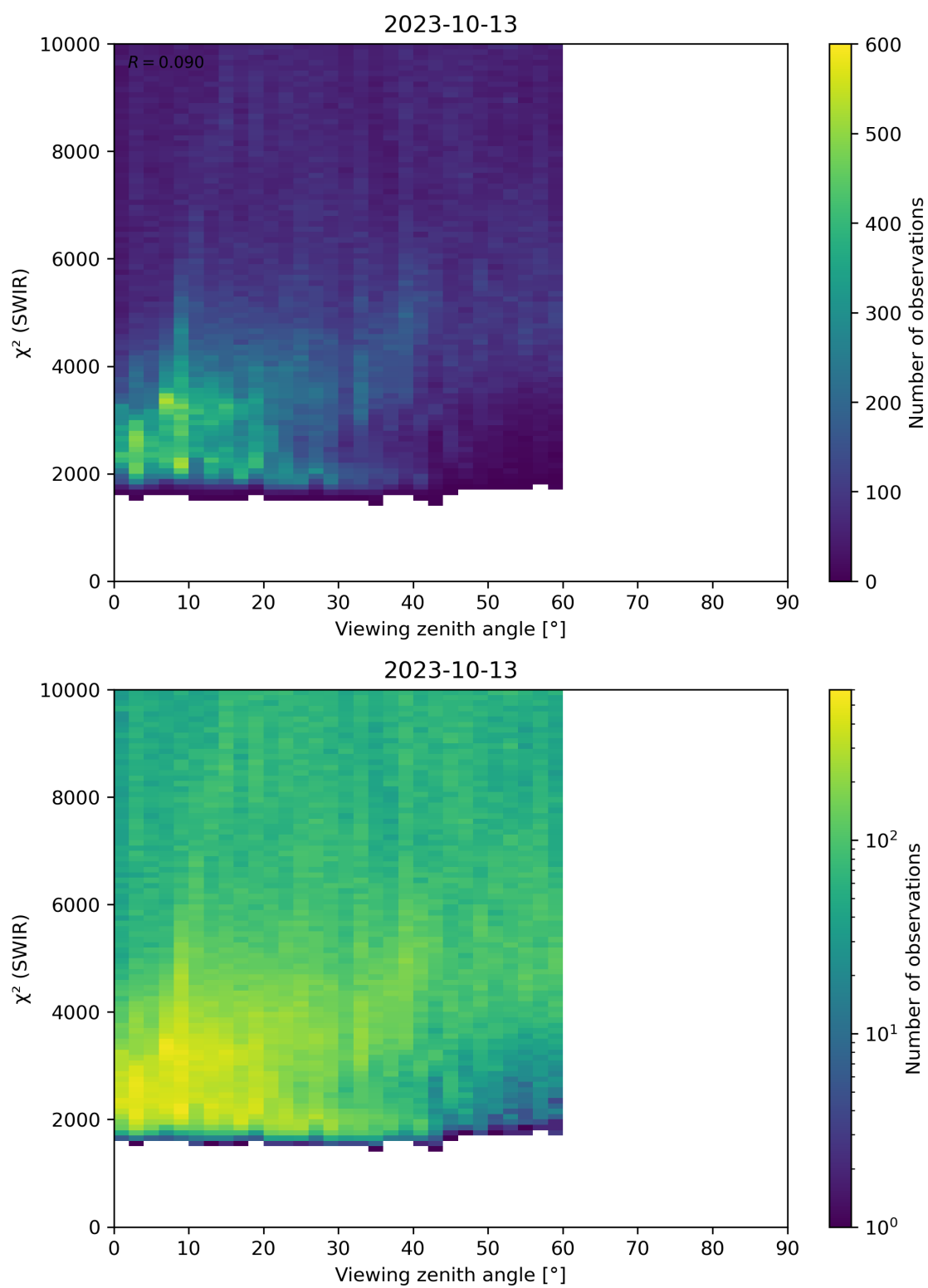
Figure 106: Scatter density plot of “Viewing zenith angle” against “ \chi^2 (SWIR)” for 2023-10-12 to 2023-10-14.
