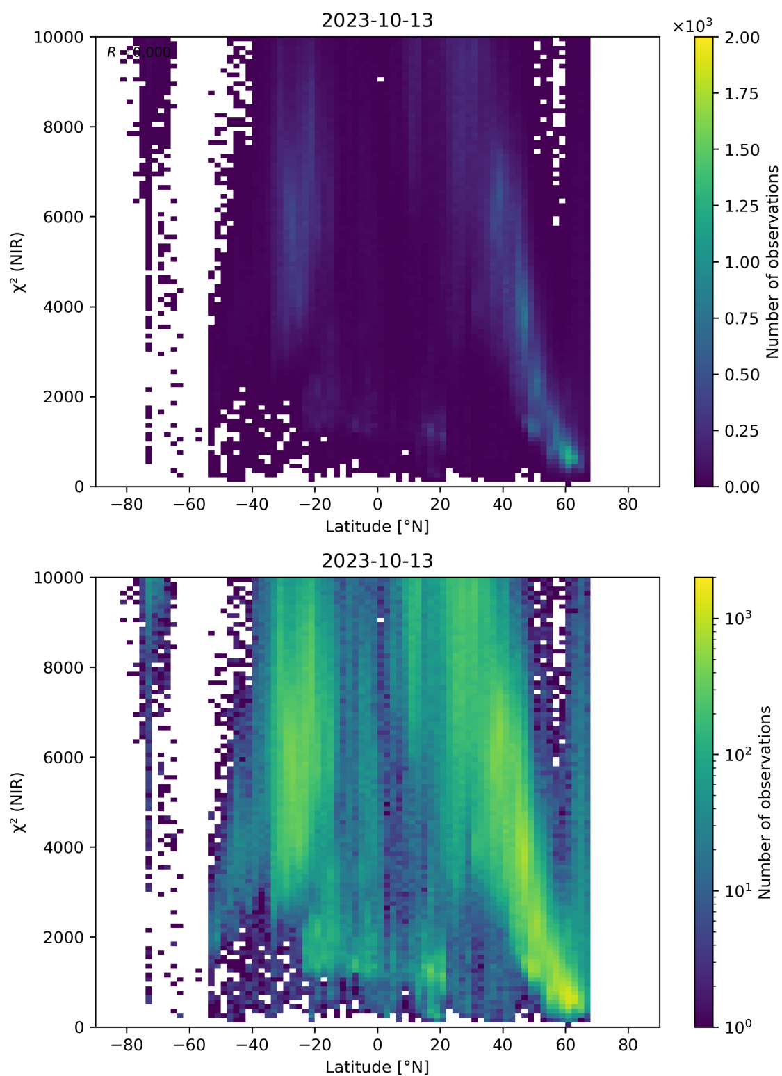
Figure 53: Scatter density plot of “Latitude” against “ \chi^2 (NIR)” for 2023-10-12 to 2023-10-14.
