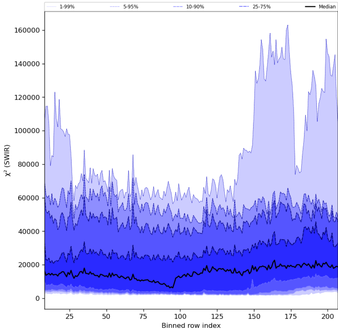
Figure 39: Along track statistics of “ \chi^2 (SWIR)” for 2023-10-12 to 2023-10-14
