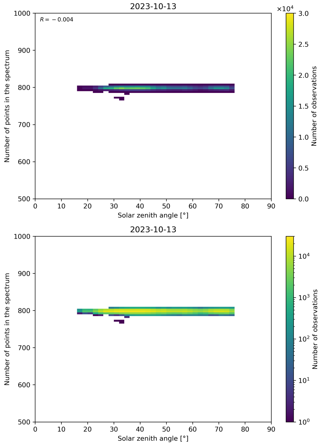
Figure 103: Scatter density plot of “Solar zenith angle” against “Number of points in the spectrum” for 2023-10-12 to 2023-10-14.
