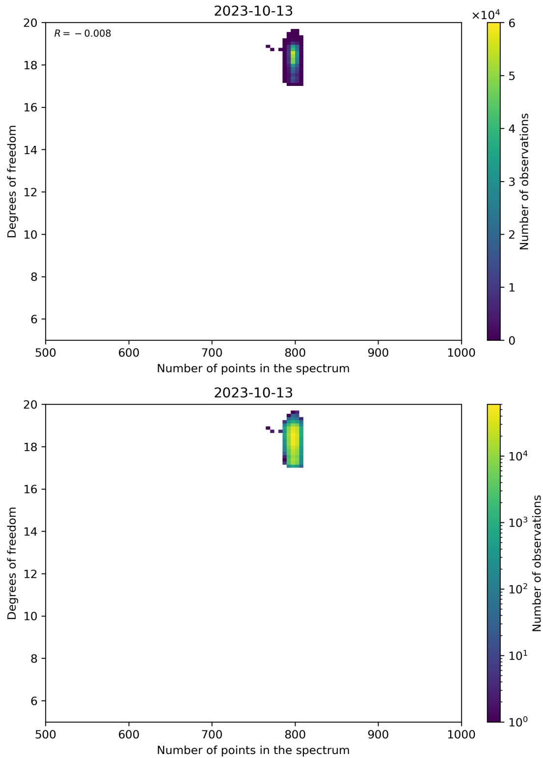
Figure 90: Scatter density plot of “Number of points in the spectrum” against “Degrees of freedom” for 2023-10-12 to 2023-10-14.
