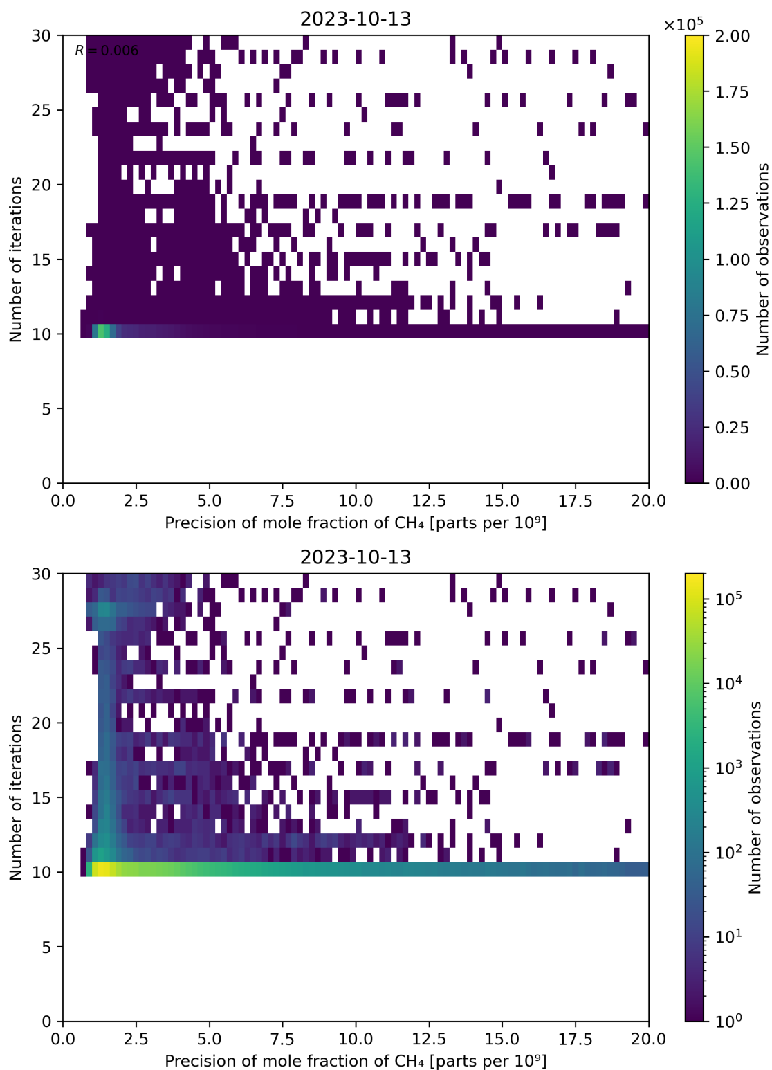
Figure 83: Scatter density plot of “Precision of mole fraction of CH 4 ” against “Number of iterations” for 2023-10-12 to 2023-10-14.
