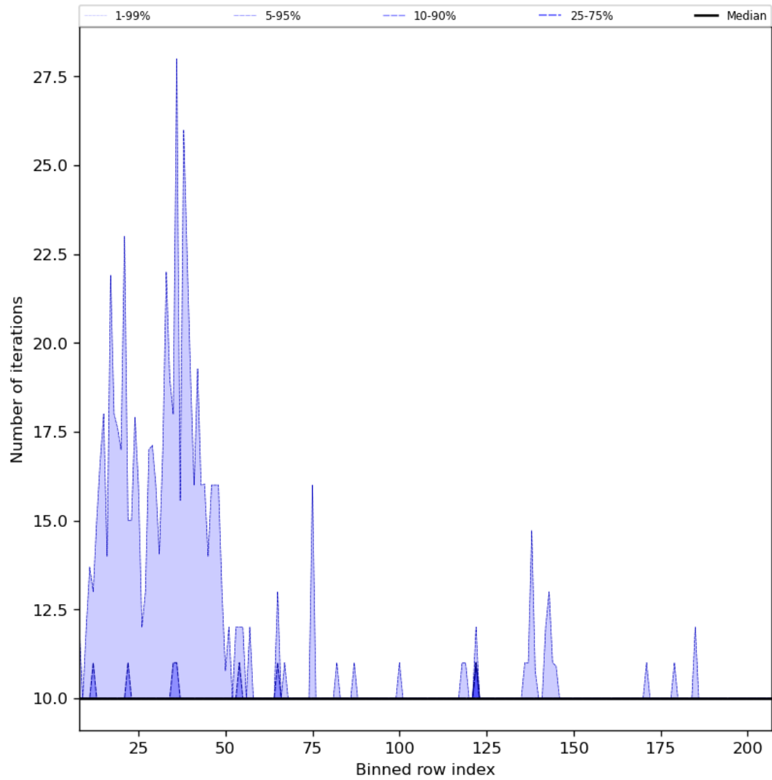
Figure 42: Along track statistics of “Number of iterations” for 2023-10-12 to 2023-10-14
