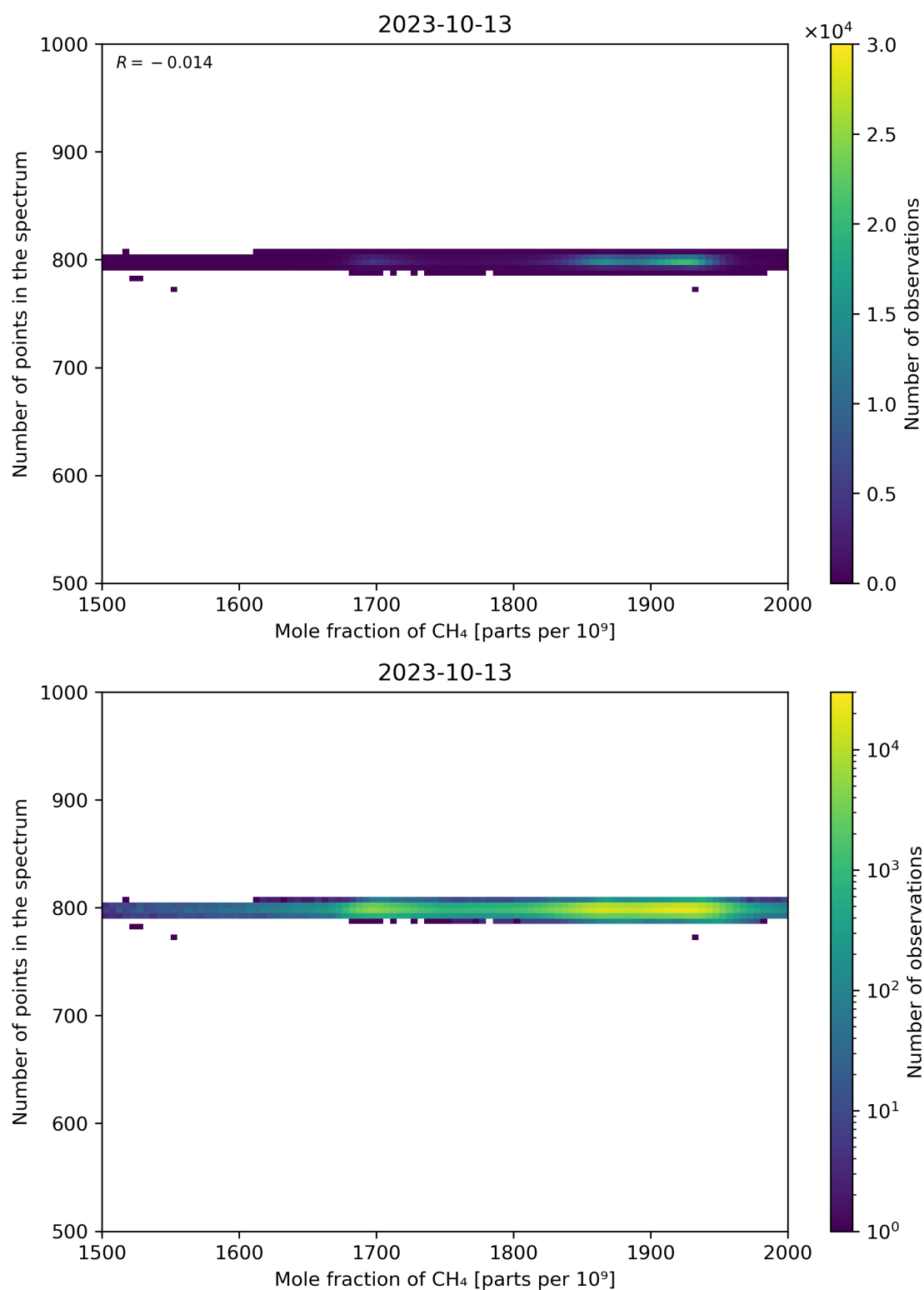
Figure 77: Scatter density plot of “Mole fraction of CH 4 ” against “Number of points in the spectrum” for 2023-10-12 to 2023-10-14.
