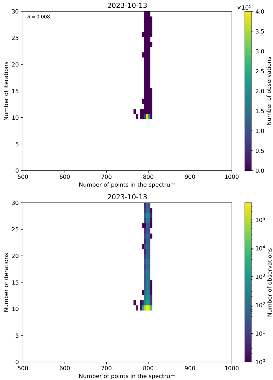
Figure 92: Scatter density plot of “Number of points in the spectrum” against “Number of iterations” for 2023-10-12 to 2023-10-14.
