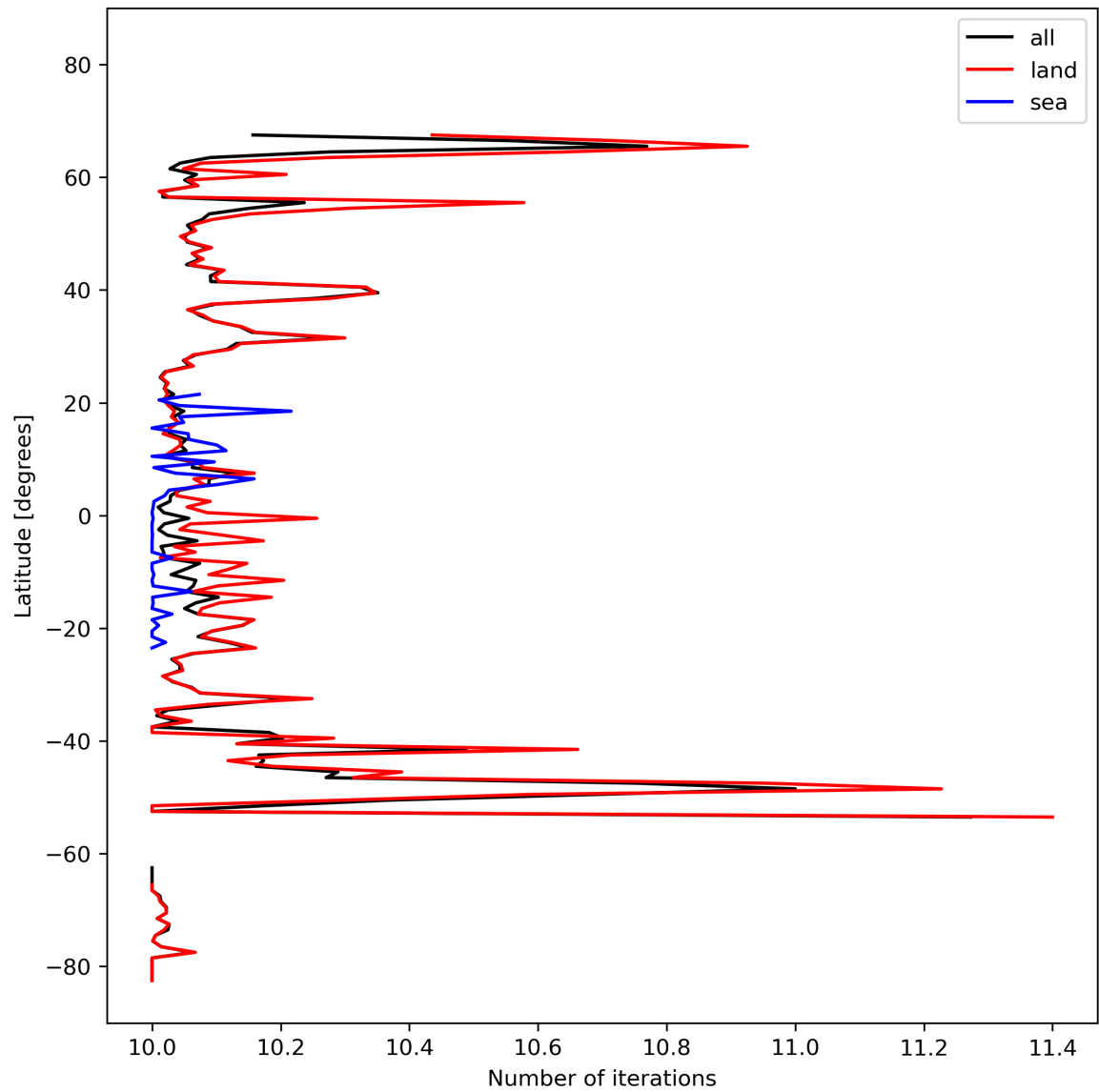
Figure 20: Zonal average of “Number of iterations” for 2023-10-12 to 2023-10-14.
