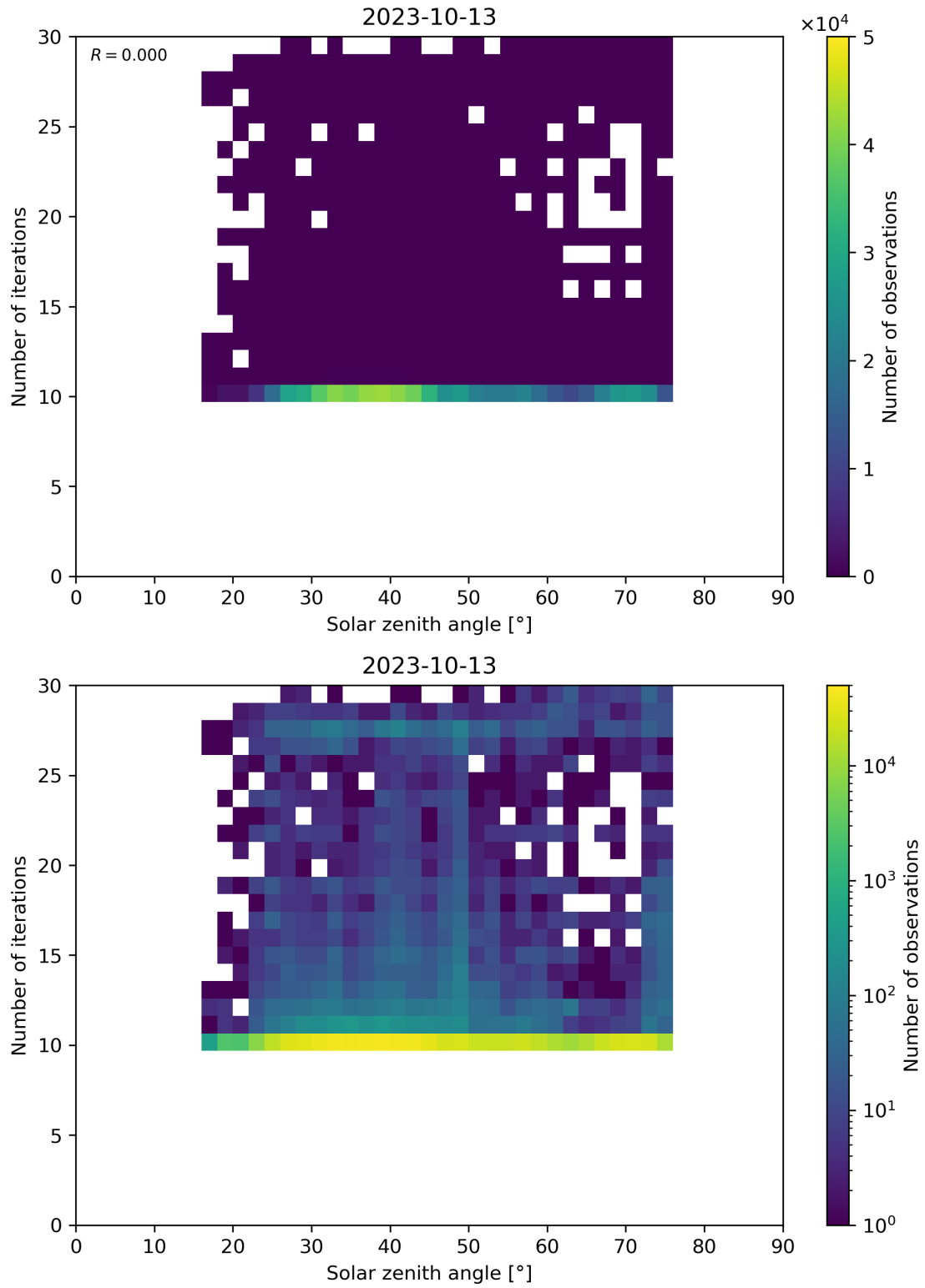
Figure 102: Scatter density plot of “Solar zenith angle” against “Number of iterations” for 2023-10-12 to 2023-10-14.
