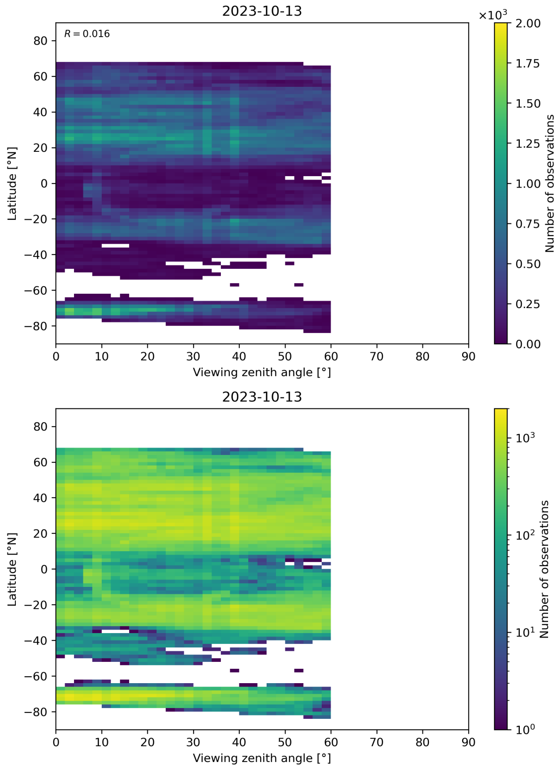
Figure 109: Scatter density plot of “Viewing zenith angle” against “Latitude” for 2023-10-12 to 2023-10-14.
