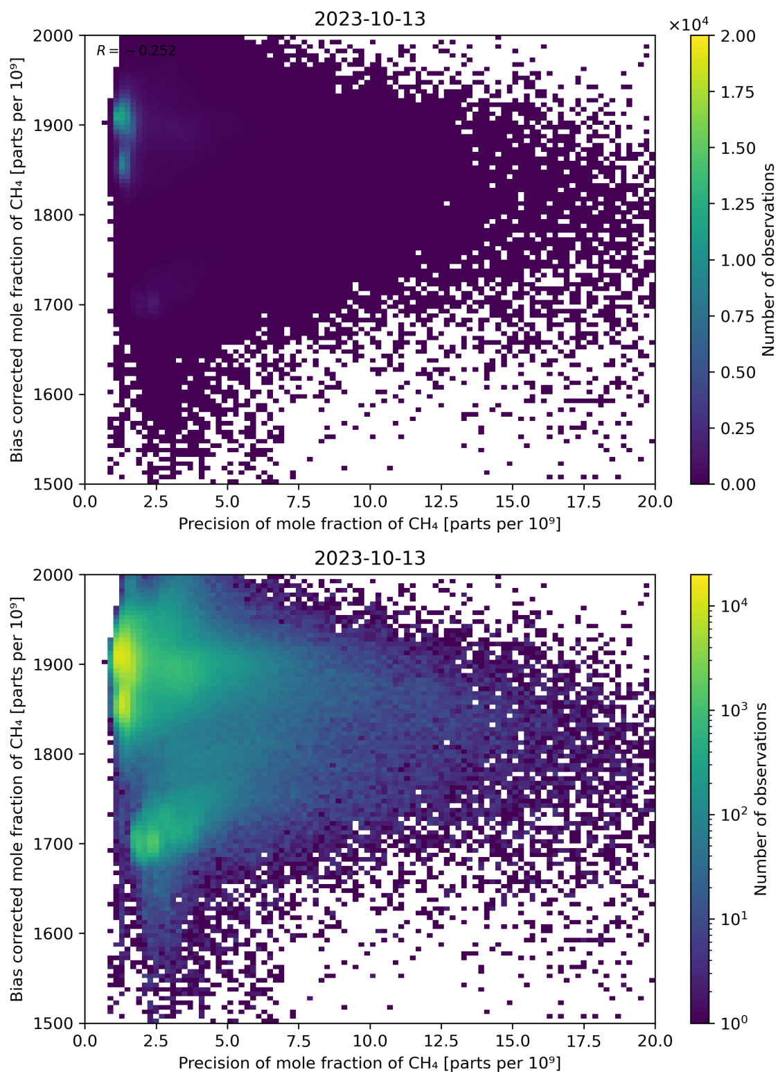
Figure 82: Scatter density plot of “Precision of mole fraction of CH 4 ” against “Bias corrected mole fraction of CH 4 ” for 2023-10-12 to 2023-10-14.
