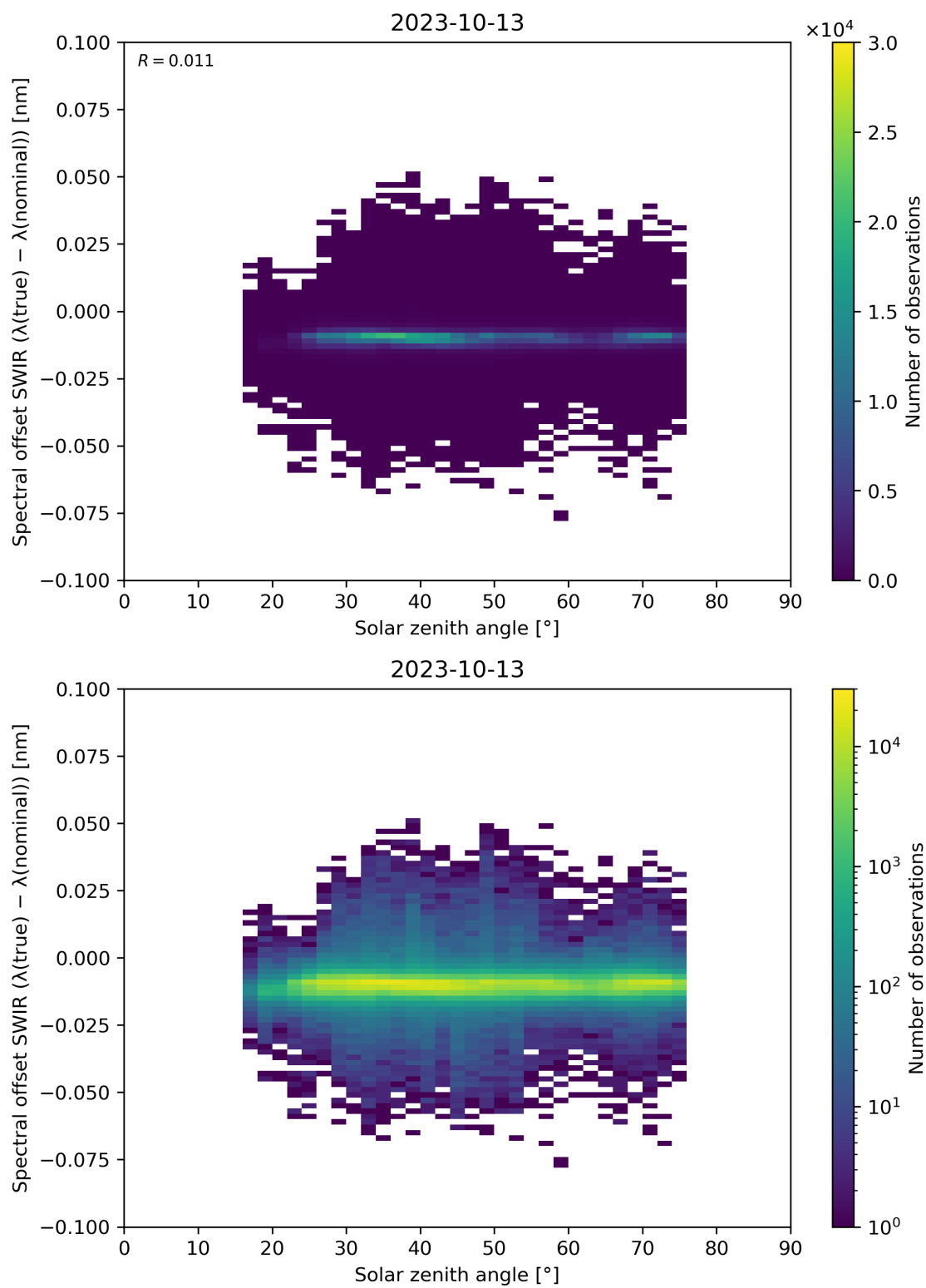
Figure 104: Scatter density plot of “Solar zenith angle” against “Spectral offset SWIR ( \lambda(\text{true}) - \lambda(\text{nominal}) )” for 2023-10-12 to 2023-10-14.
