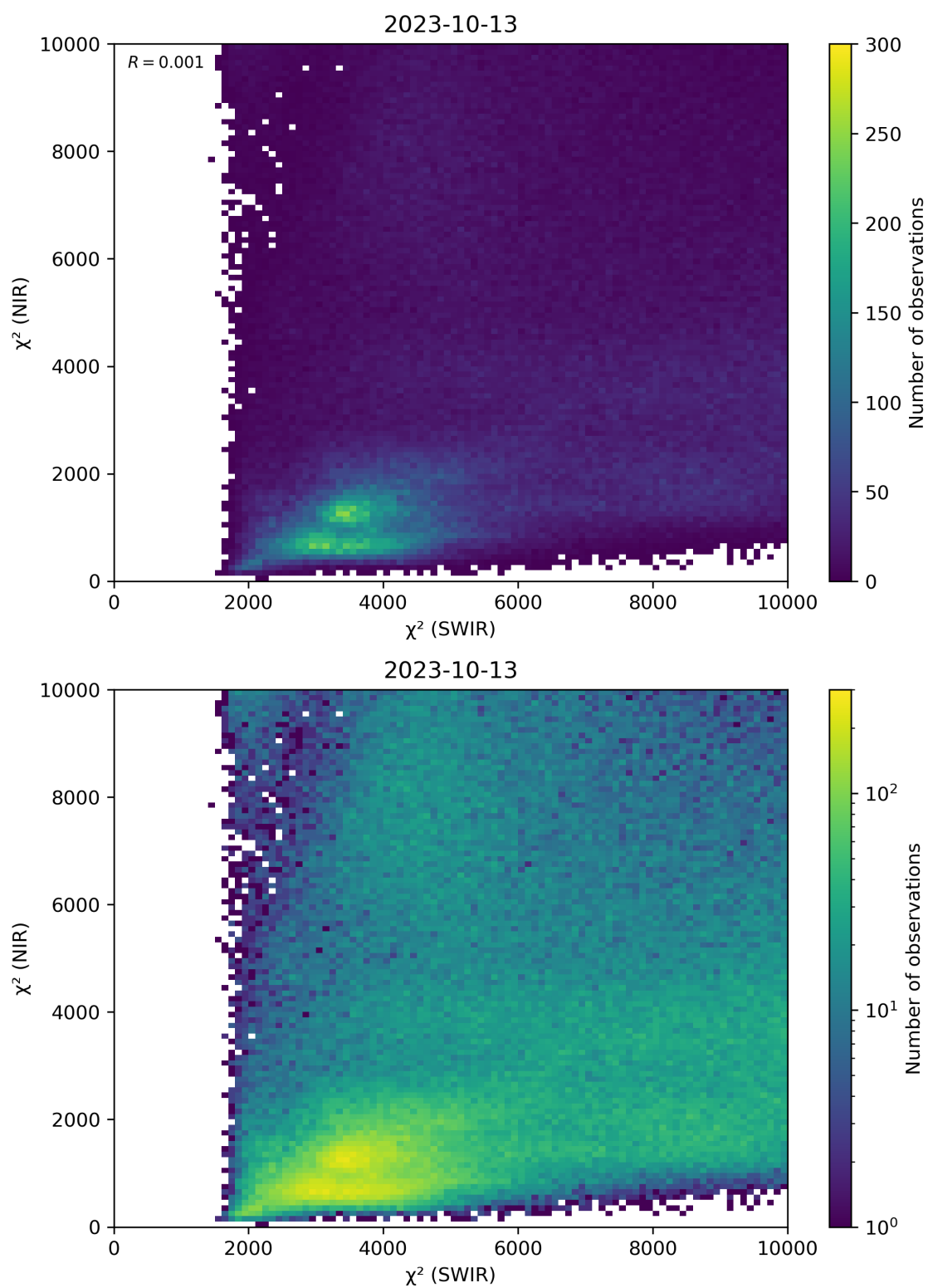
Figure 47: Scatter density plot of “ \chi^2 (SWIR)” against “ \chi^2 (NIR)” for 2023-10-12 to 2023-10-14.
