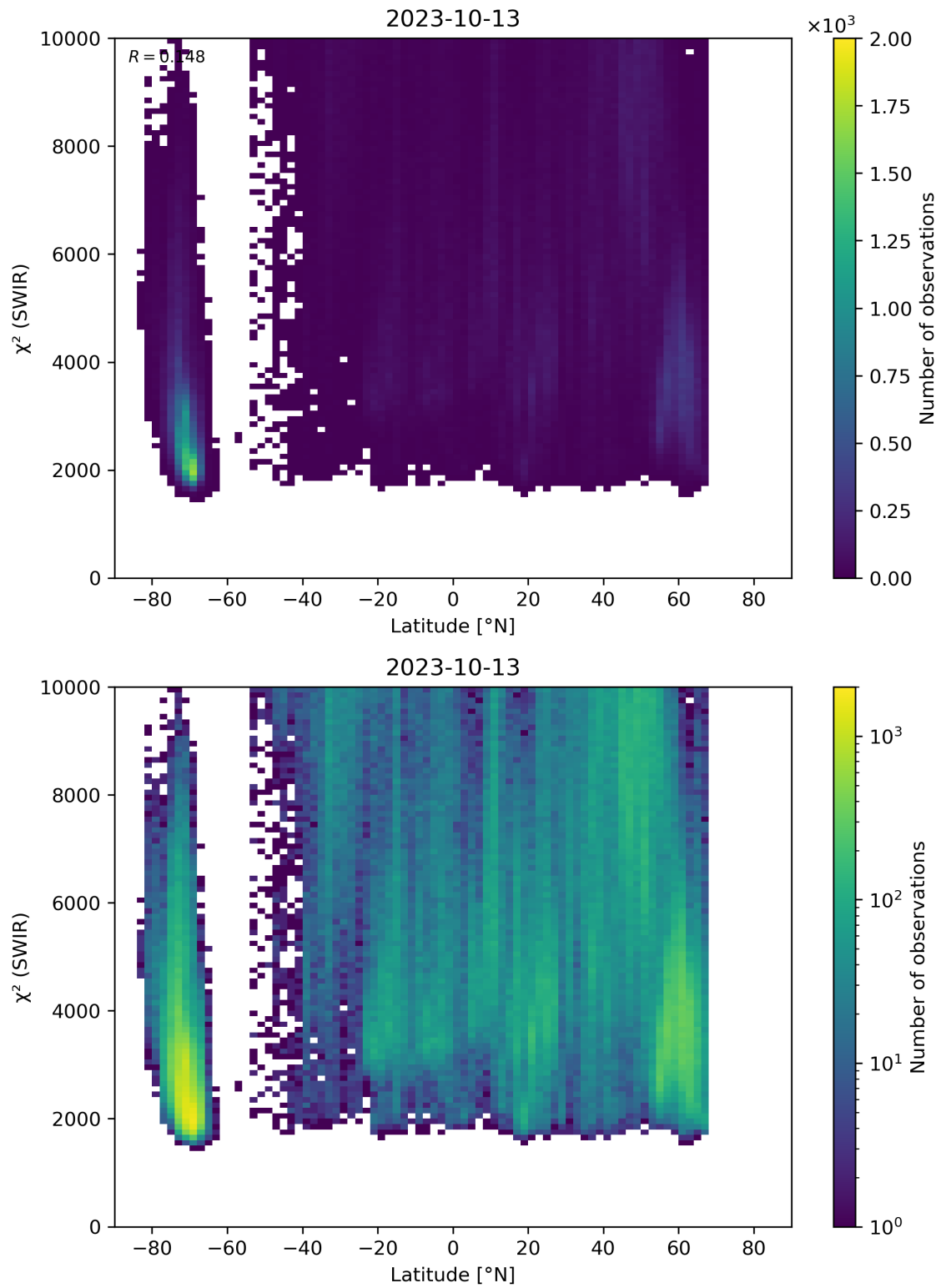
Figure 54: Scatter density plot of “Latitude” against “ \chi^2 (SWIR)” for 2023-10-12 to 2023-10-14.
