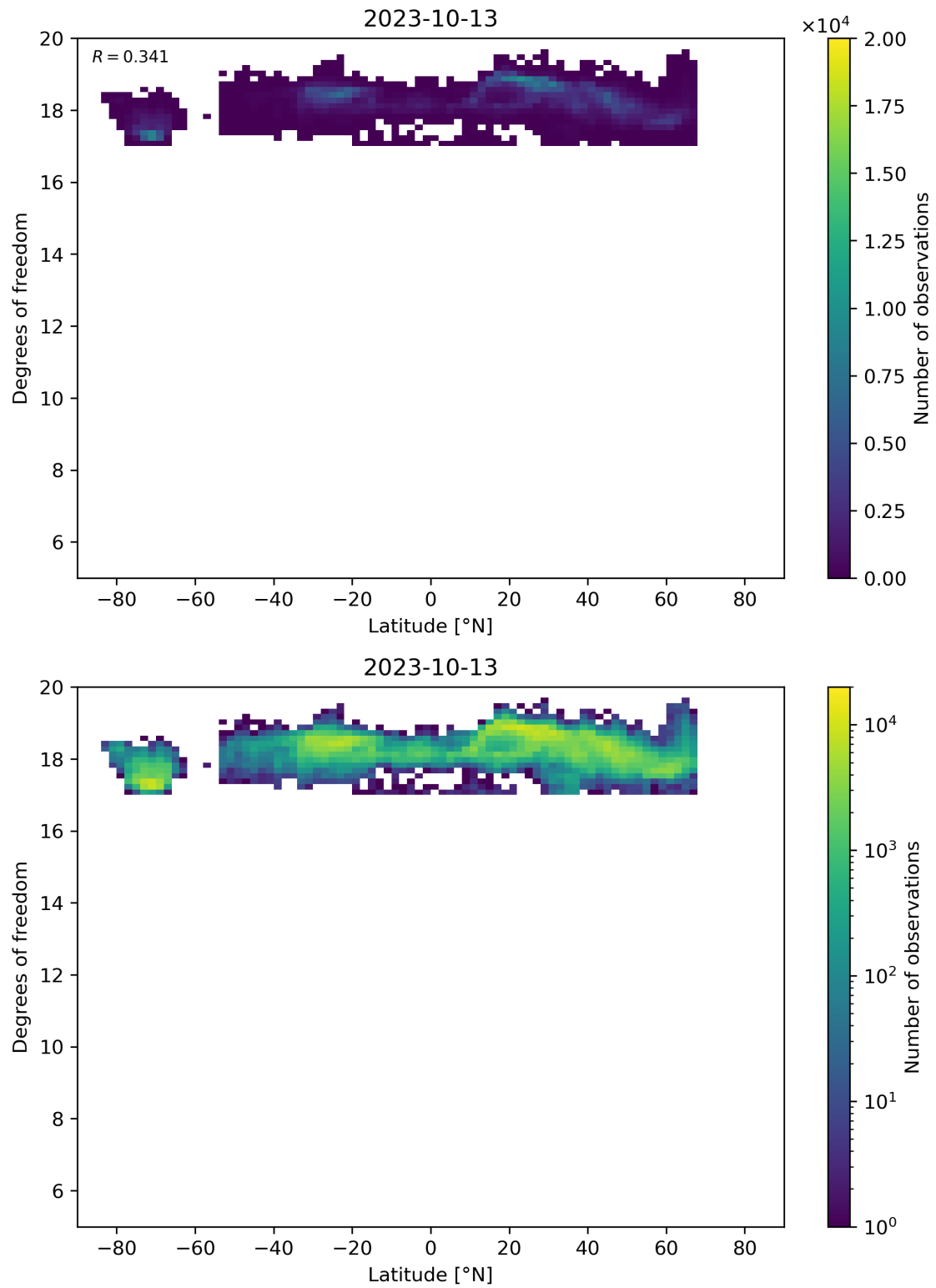
Figure 55: Scatter density plot of “Latitude” against “Degrees of freedom” for 2023-10-12 to 2023-10-14.
