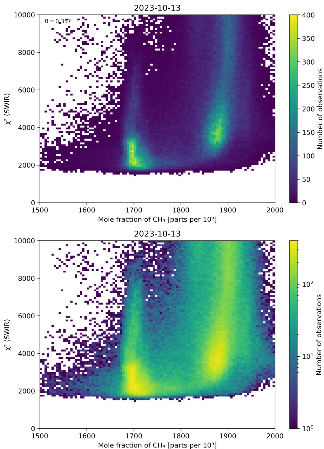
Figure 71: Scatter density plot of “Mole fraction of \text{CH}_4 ” against “ \chi^2 (SWIR)” for 2023-10-12 to 2023-10-14.
