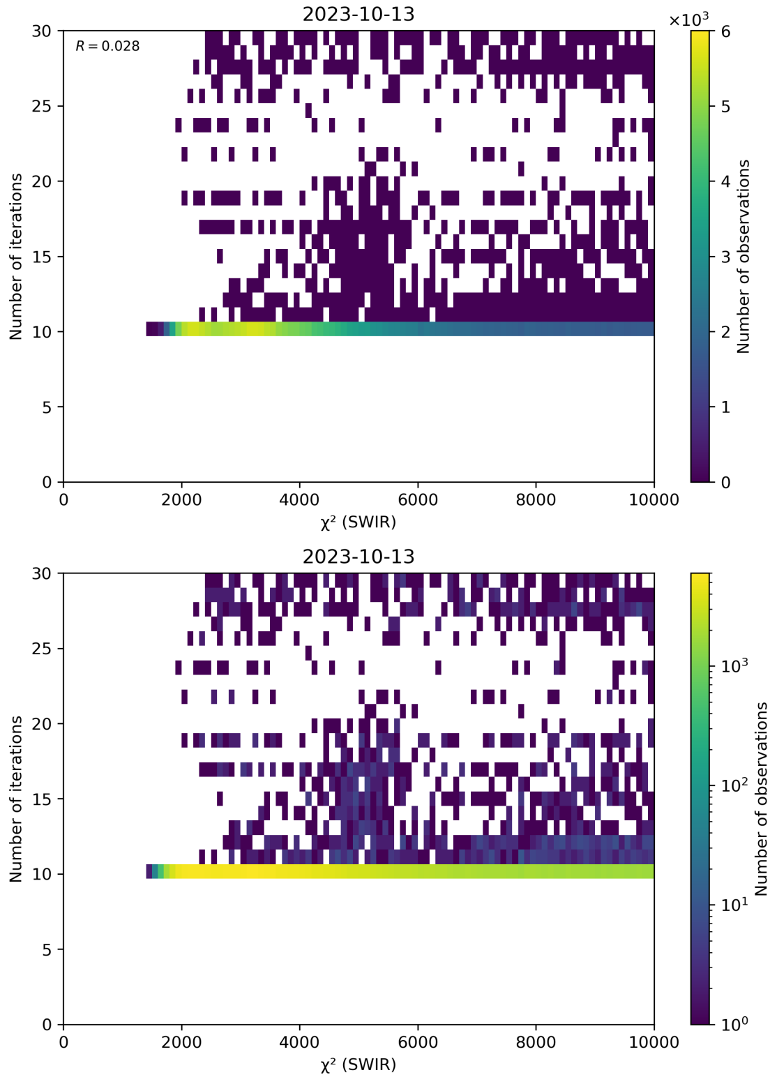
Figure 50: Scatter density plot of “ \chi^2 (SWIR)” against “Number of iterations” for 2023-10-12 to 2023-10-14.
