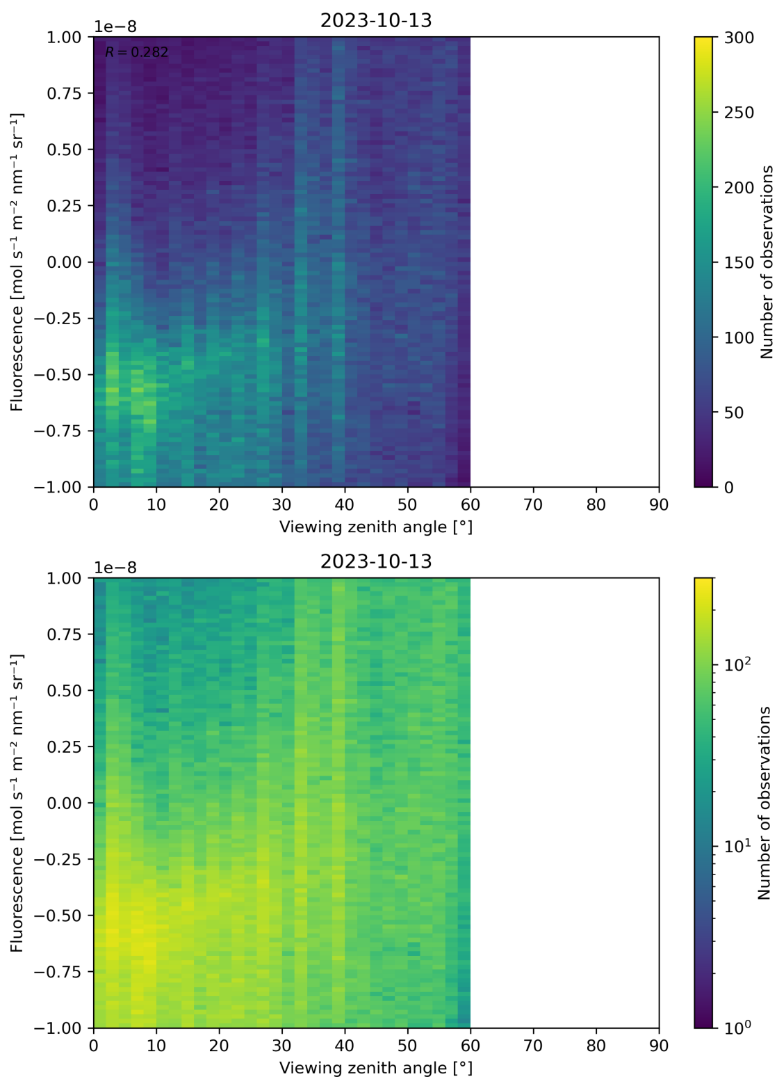
Figure 108: Scatter density plot of “Viewing zenith angle” against “Fluorescence” for 2023-10-12 to 2023-10-14.
