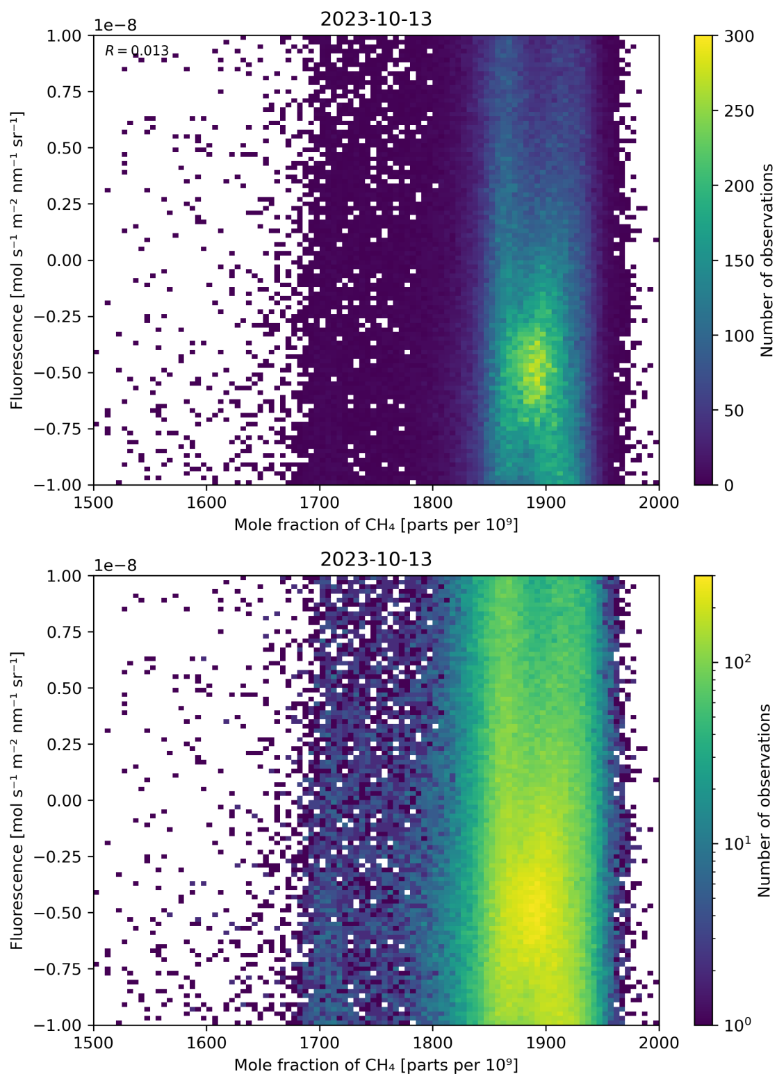
Figure 73: Scatter density plot of “Mole fraction of \text{CH}_4 ” against “Fluorescence” for 2023-10-12 to 2023-10-14.
