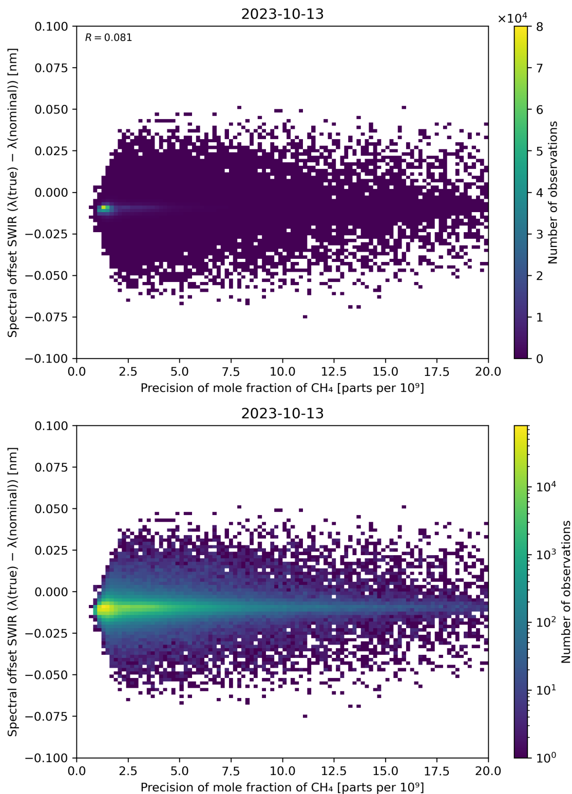
Figure 85: Scatter density plot of “Precision of mole fraction of CH 4 ” against “Spectral offset SWIR ( \lambda(\text{true}) - \lambda(\text{nominal}) )” for 2023-10-12 to 2023-10-14.
