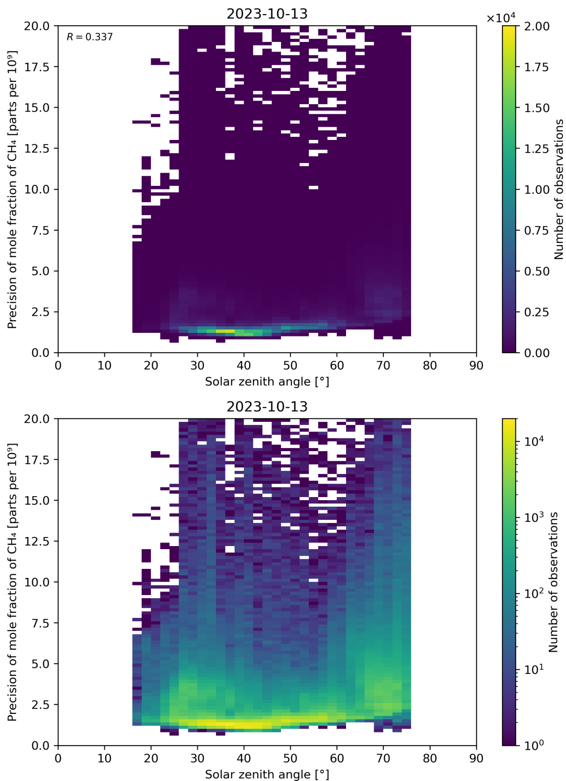
Figure 101: Scatter density plot of “Solar zenith angle” against “Precision of mole fraction of CH 4 ” for 2023-10-12 to 2023-10-14.
