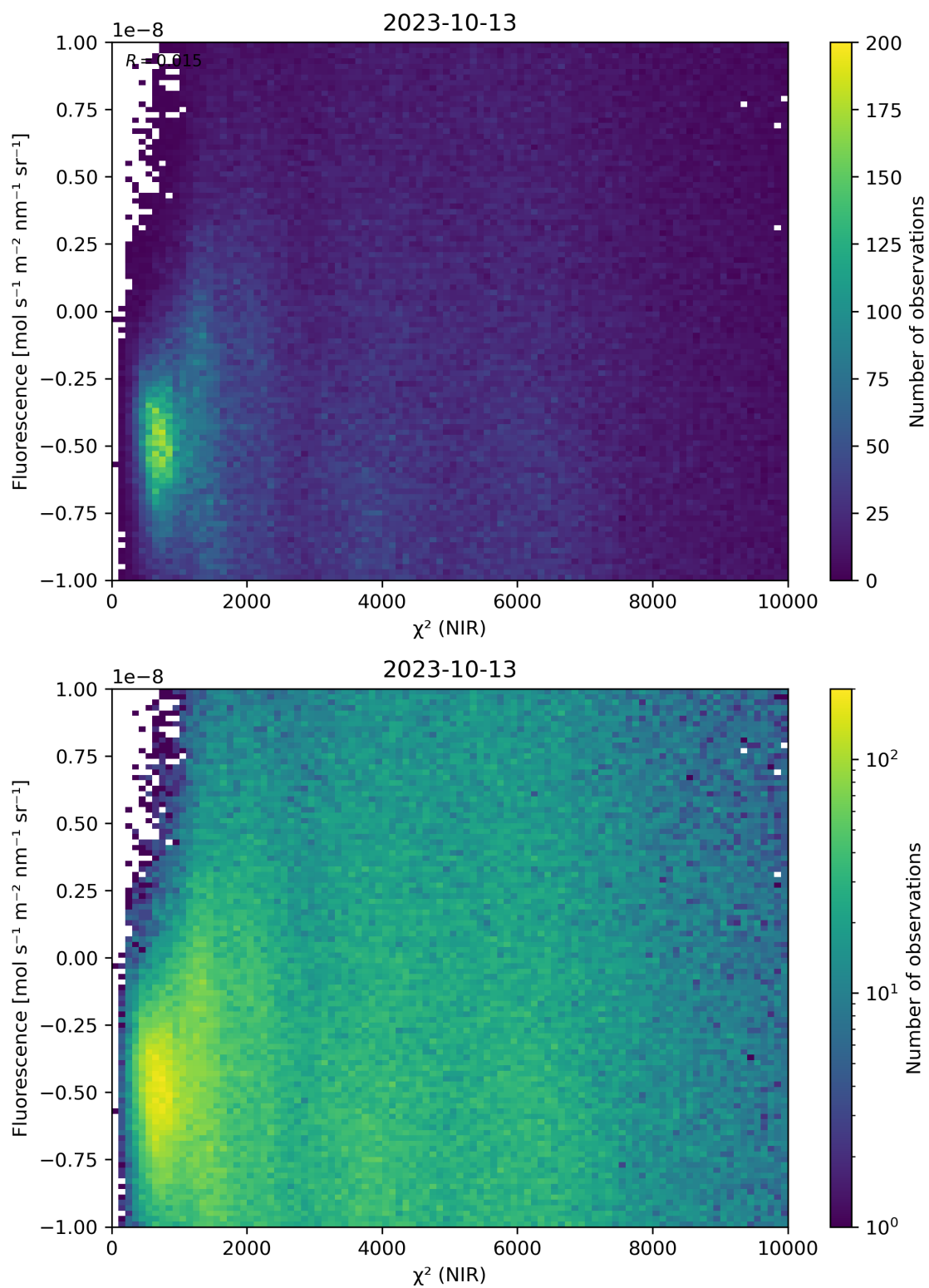
Figure 45: Scatter density plot of “ \chi^2 (NIR)” against “Fluorescence” for 2023-10-12 to 2023-10-14.
