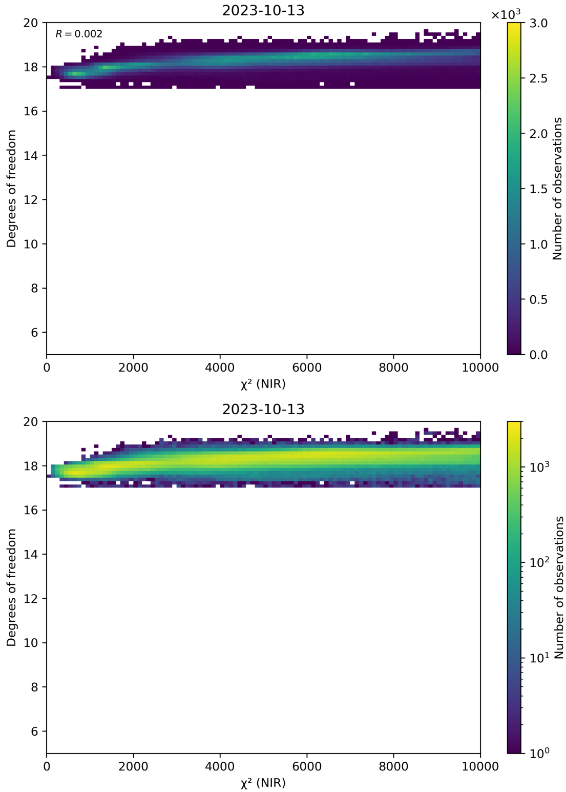
Figure 44: Scatter density plot of “ \chi^2 (NIR)” against “Degrees of freedom” for 2023-10-12 to 2023-10-14.
