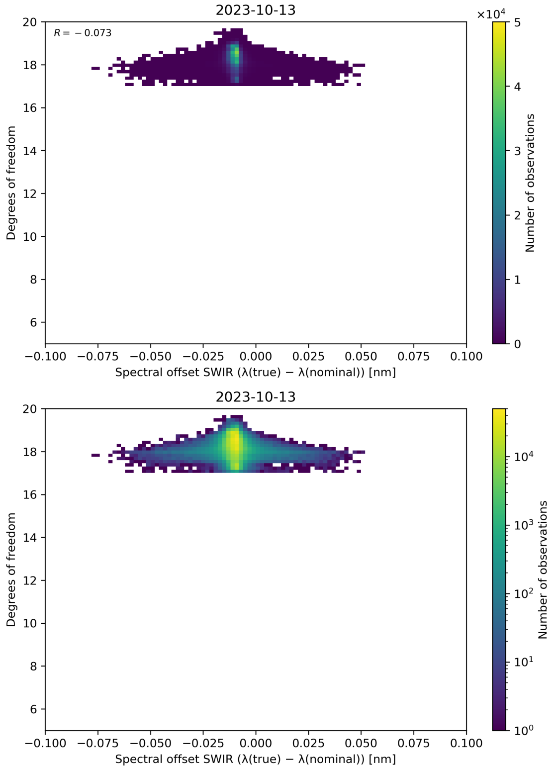
Figure 119: Scatter density plot of “Spectral offset SWIR ( \lambda(\text{true}) - \lambda(\text{nominal}) )” against “Degrees of freedom” for 2023-10-12 to 2023-10-14.
