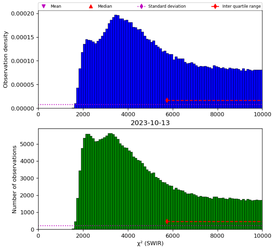
Figure 28: Histogram of “ \chi^2 (SWIR)” for 2023-10-12 to 2023-10-14
