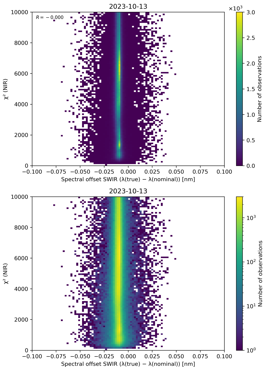
Figure 117: Scatter density plot of “Spectral offset SWIR ( \lambda(\text{true}) - \lambda(\text{nominal}) )” against “ \chi^2 (NIR)” for 2023-10-12 to 2023-10-14.
