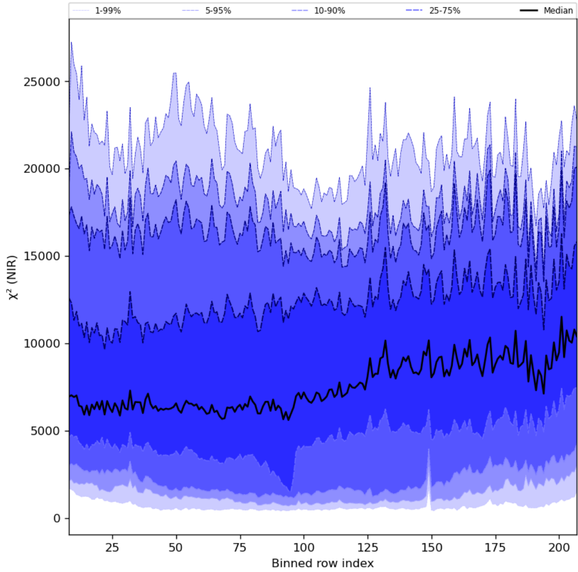
Figure 40: Along track statistics of “ \chi^2 (NIR)” for 2023-10-12 to 2023-10-14
