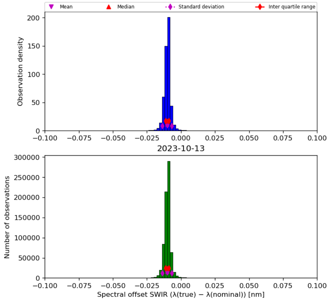
Figure 27: Histogram of “Spectral offset SWIR ( \lambda(\text{true}) - \lambda(\text{nominal}) )” for 2023-10-12 to 2023-10-14
