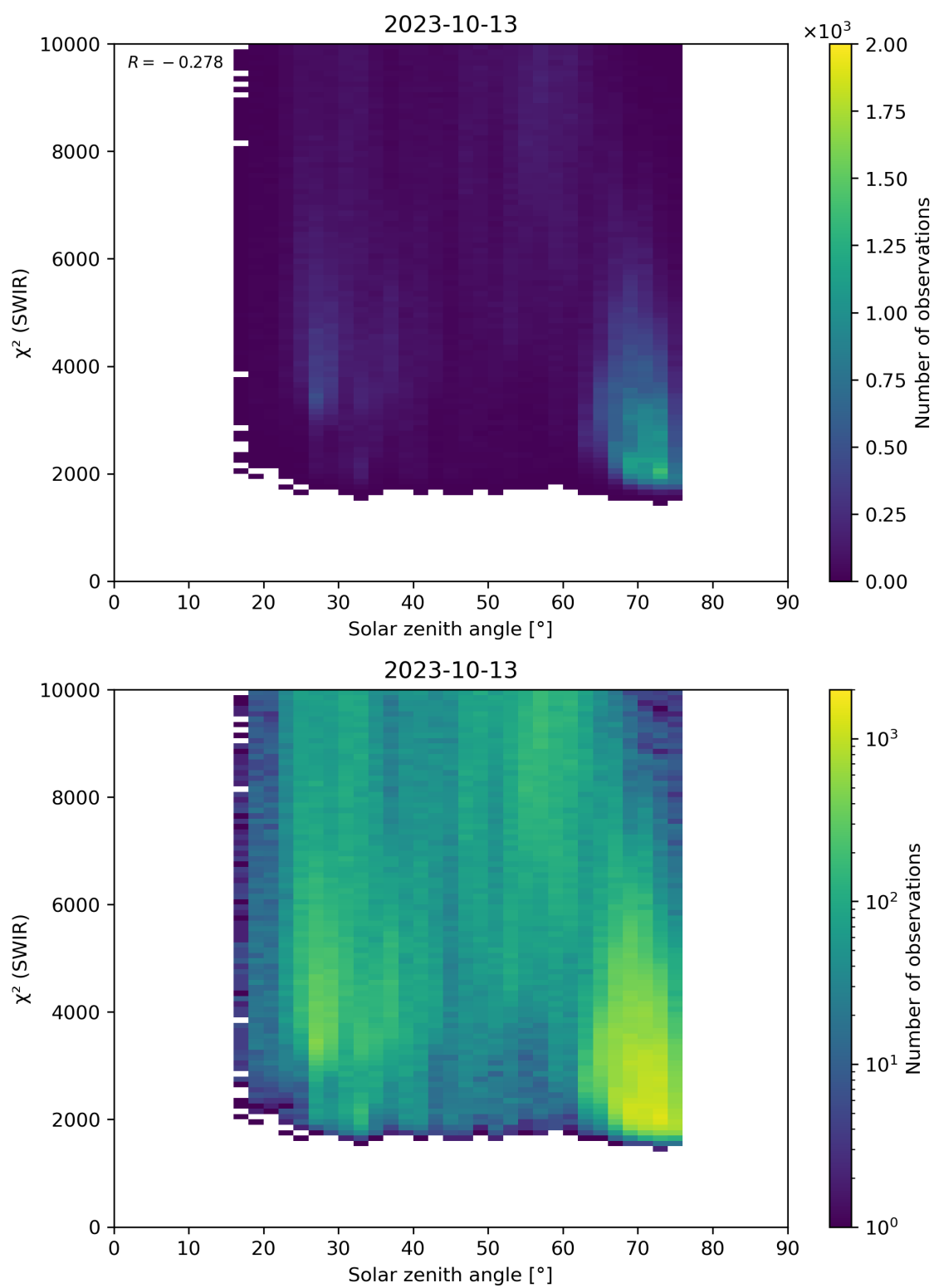
Figure 95: Scatter density plot of “Solar zenith angle” against “ \chi^2 (SWIR)” for 2023-10-12 to 2023-10-14.
