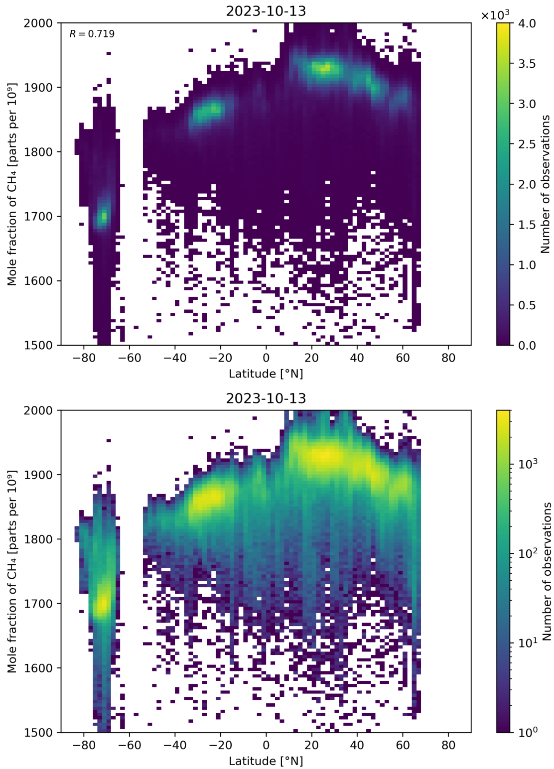
Figure 57: Scatter density plot of “Latitude” against “Mole fraction of CH 4 ” for 2023-10-12 to 2023-10-14.
