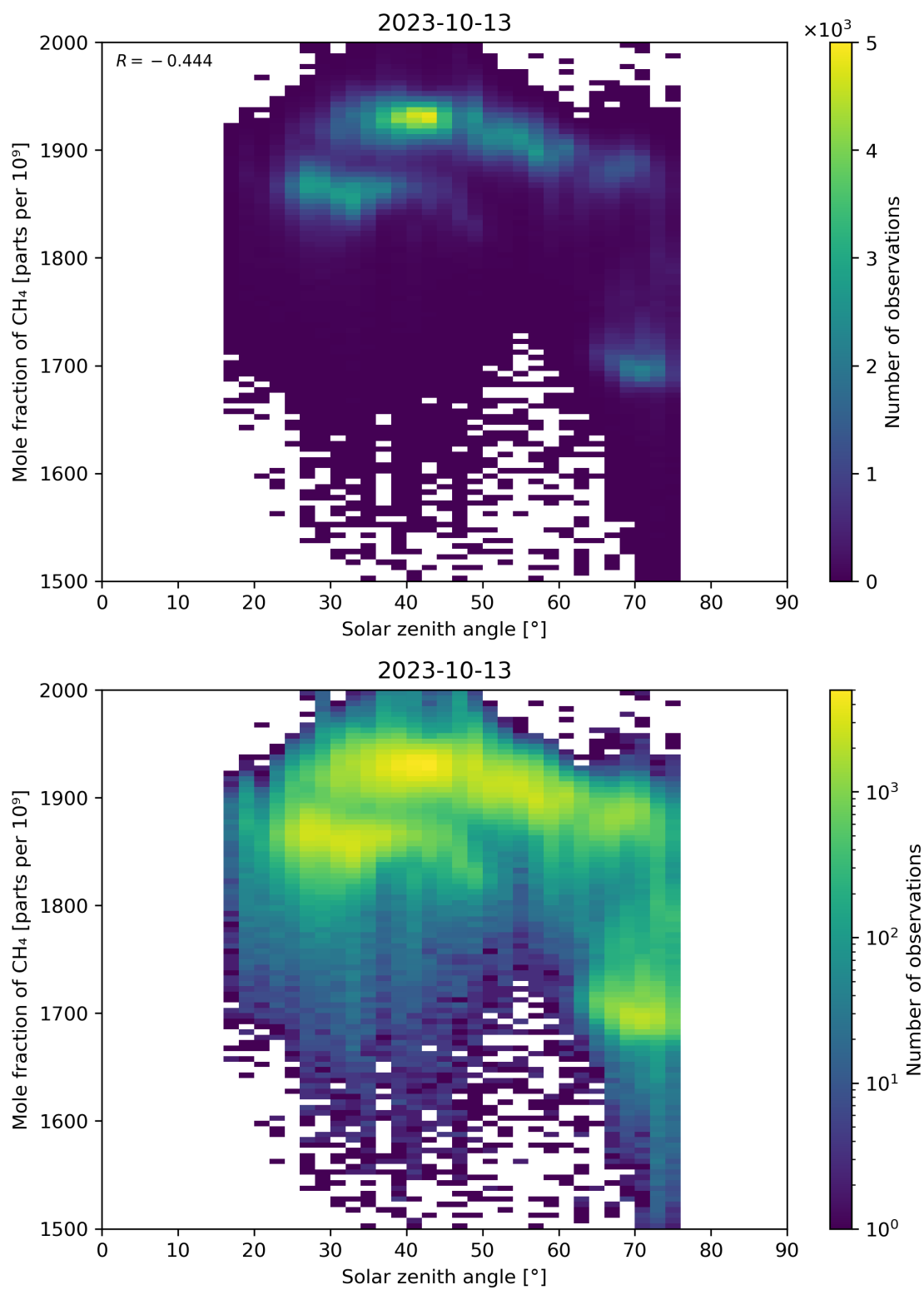
Figure 99: Scatter density plot of “Solar zenith angle” against “Mole fraction of CH 4 ” for 2023-10-12 to 2023-10-14.
