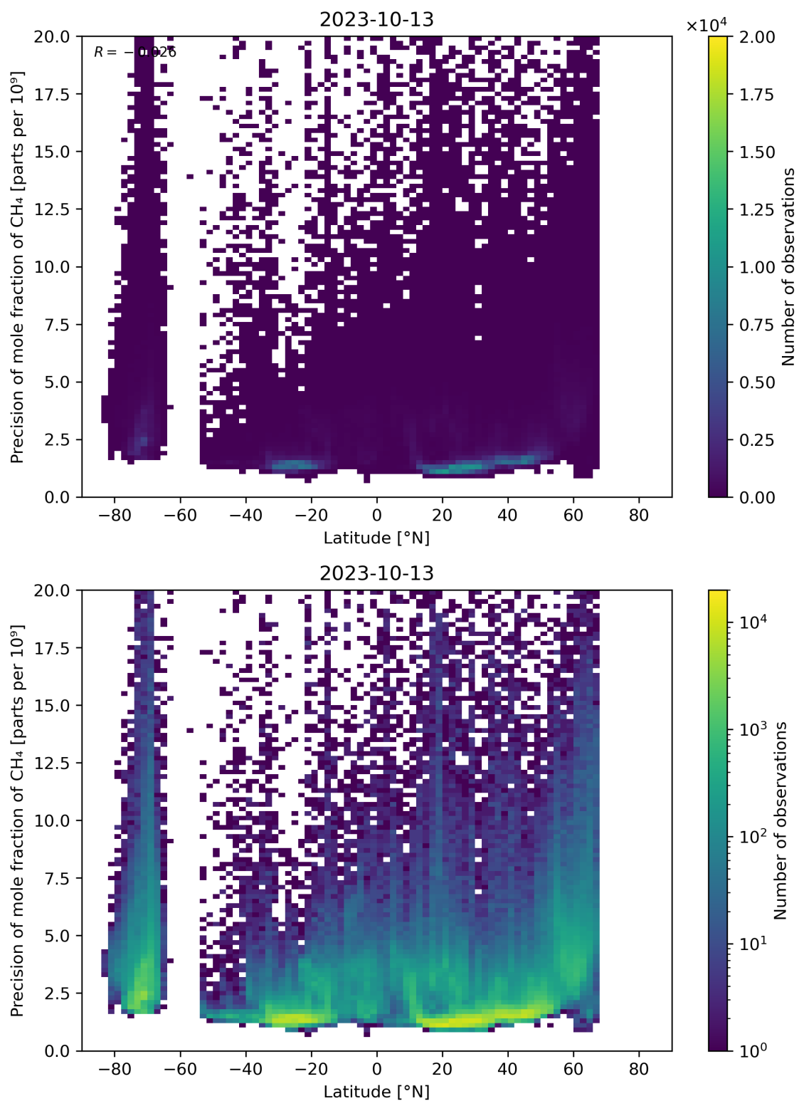
Figure 59: Scatter density plot of “Latitude” against “Precision of mole fraction of CH 4 ” for 2023-10-12 to 2023-10-14.
