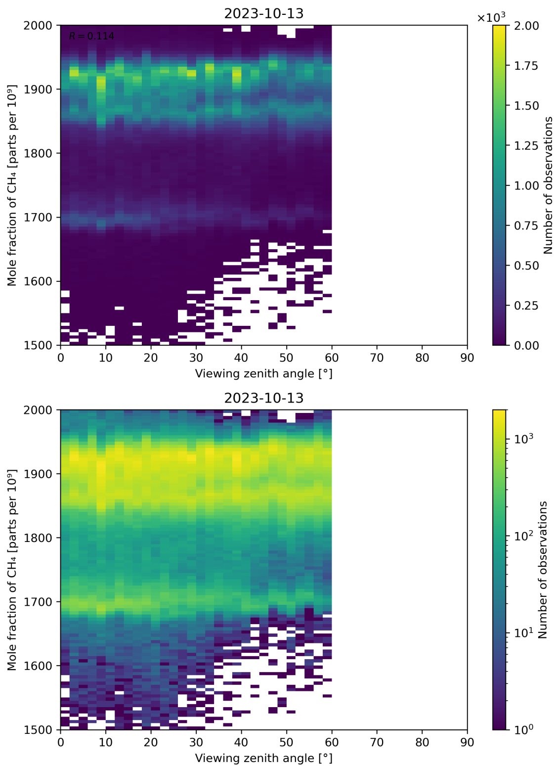
Figure 110: Scatter density plot of “Viewing zenith angle” against “Mole fraction of \text{CH}_4 ” for 2023-10-12 to 2023-10-14.
