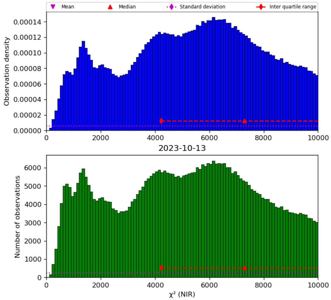
Figure 29: Histogram of “ \chi^2 (NIR)” for 2023-10-12 to 2023-10-14
