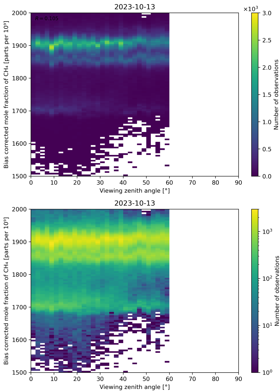
Figure 111: Scatter density plot of “Viewing zenith angle” against “Bias corrected mole fraction of CH 4 ” for 2023-10-12 to 2023-10-14.
