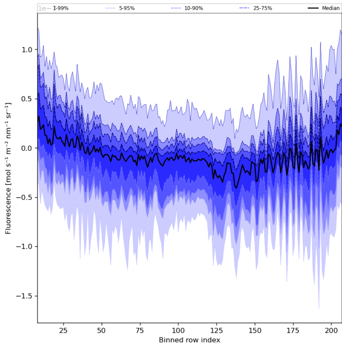
Figure 43: Along track statistics of “Fluorescence” for 2023-10-12 to 2023-10-14
