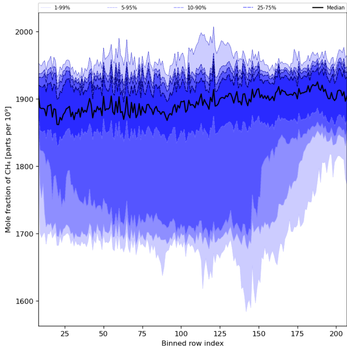
Figure 34: Along track statistics of “Mole fraction of CH 4 ” for 2023-10-12 to 2023-10-14
