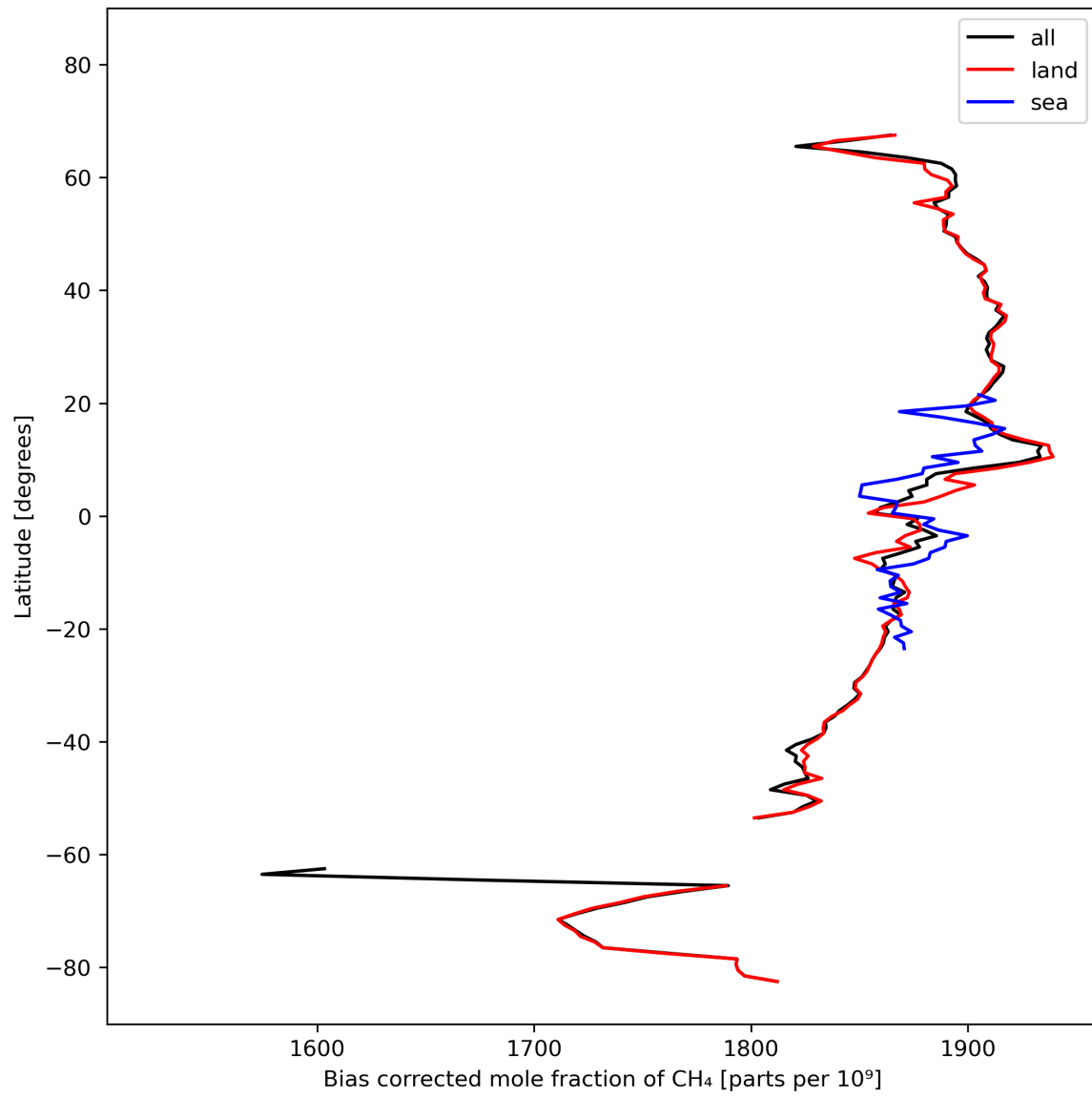
Figure 14: Zonal average of “Bias corrected mole fraction of CH 4 ” for 2023-10-12 to 2023-10-14.
