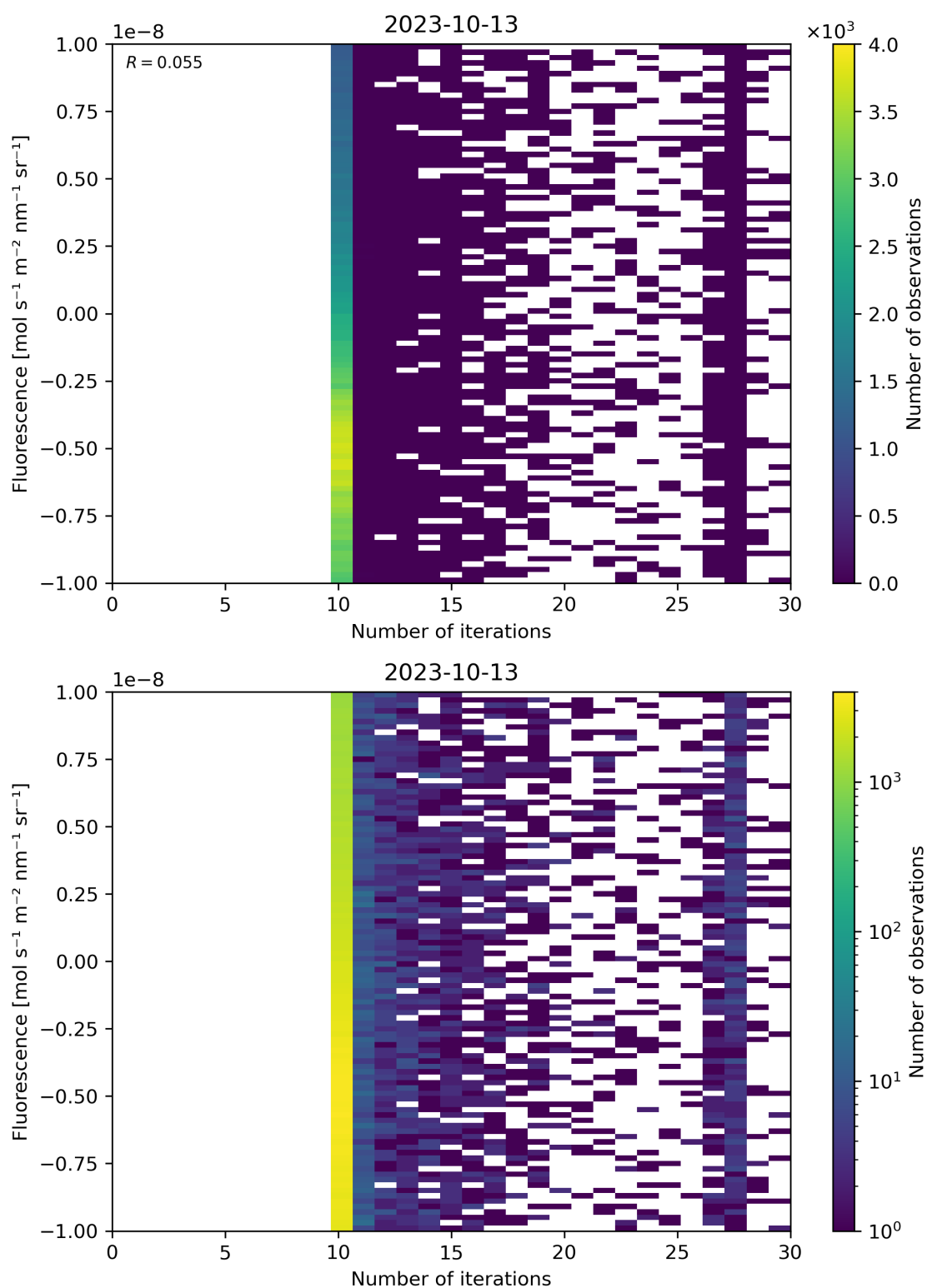
Figure 87: Scatter density plot of “Number of iterations” against “Fluorescence” for 2023-10-12 to 2023-10-14.
