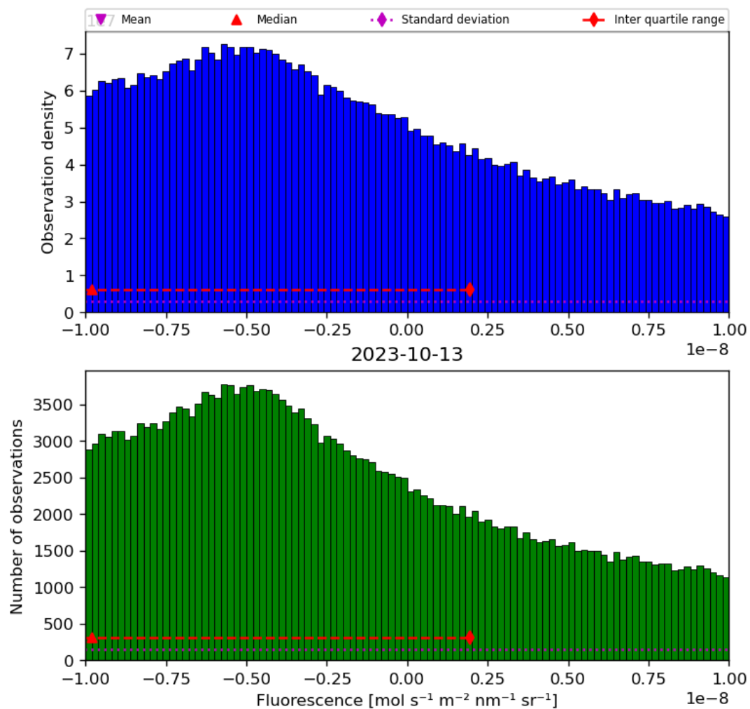
Figure 32: Histogram of “Fluorescence” for 2023-10-12 to 2023-10-14
