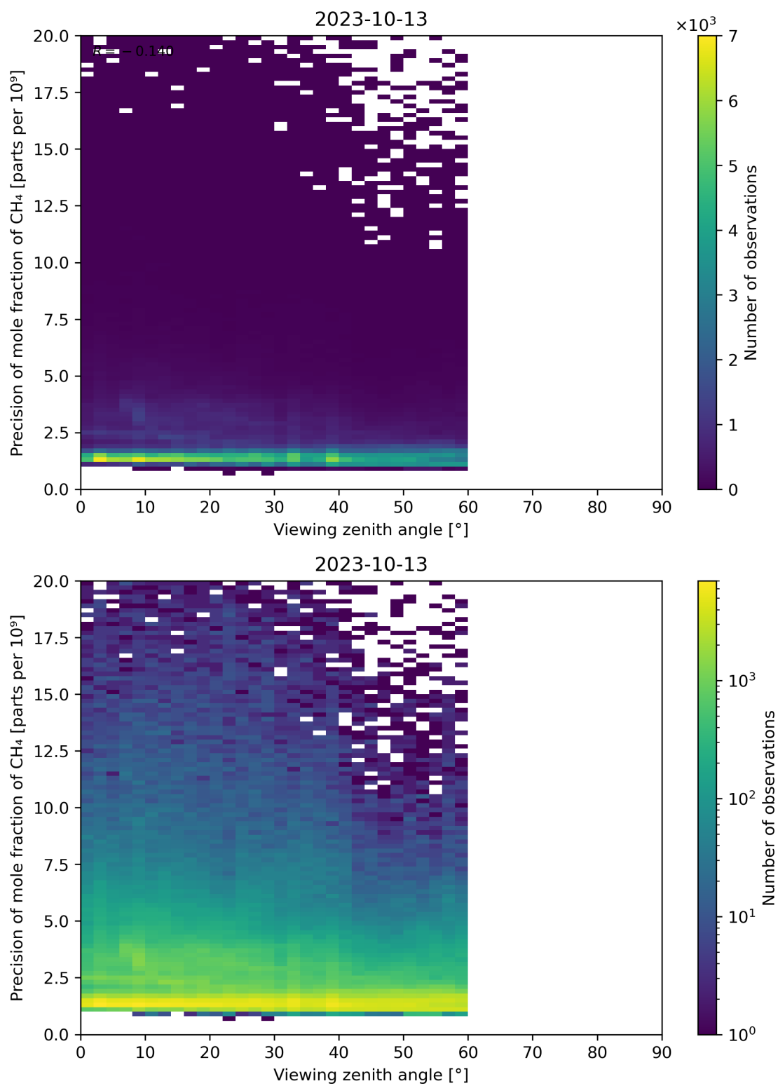
Figure 112: Scatter density plot of “Viewing zenith angle” against “Precision of mole fraction of CH 4 ” for 2023-10-12 to 2023-10-14.
