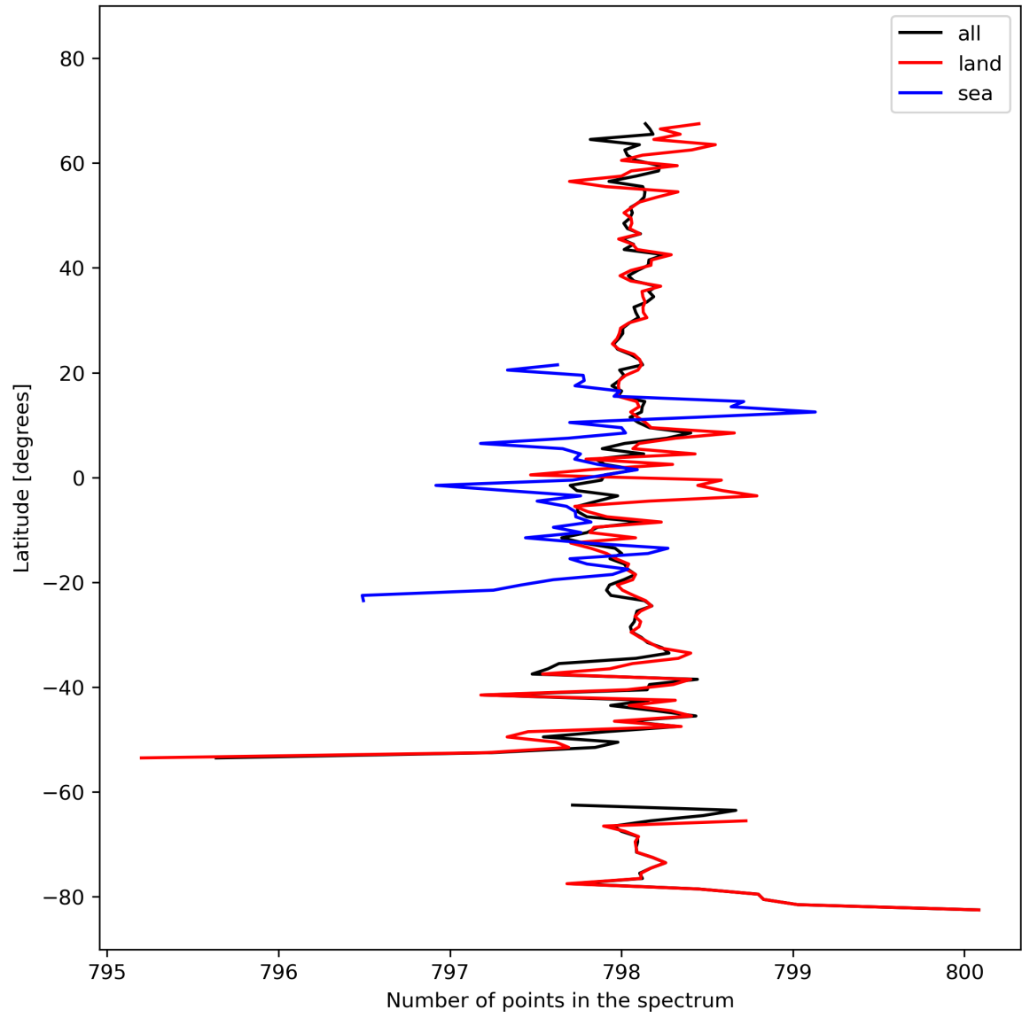
Figure 15: Zonal average of “Number of points in the spectrum” for 2023-10-12 to 2023-10-14.
