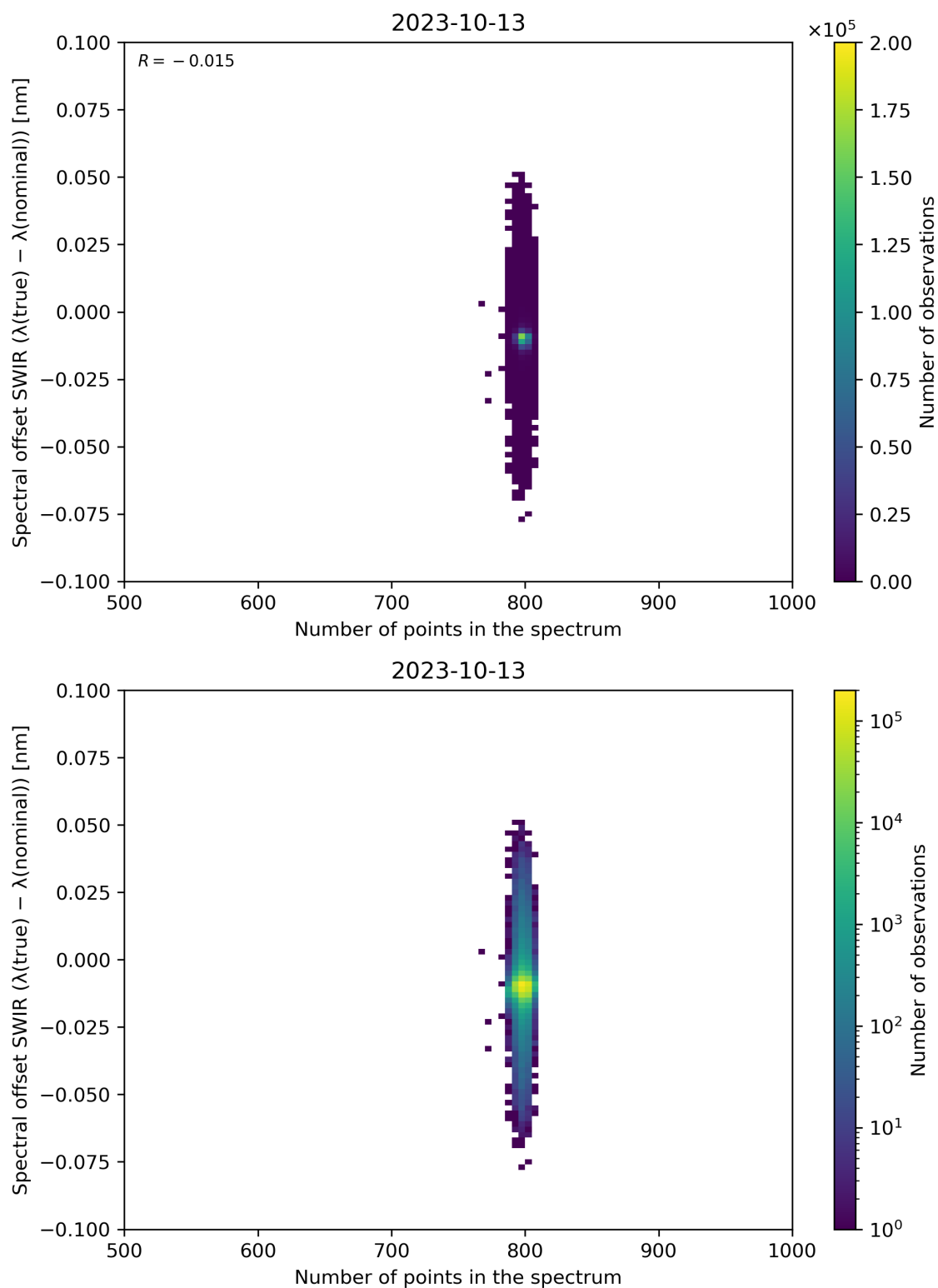
Figure 93: Scatter density plot of “Number of points in the spectrum” against “Spectral offset SWIR ( \lambda(\text{true}) - \lambda(\text{nominal}) )” for 2023-10-12 to 2023-10-14.
