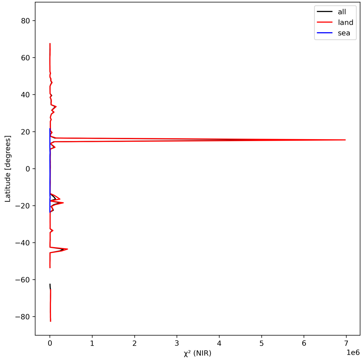
Figure 18: Zonal average of “ \chi^2 (NIR)” for 2023-10-12 to 2023-10-14.
