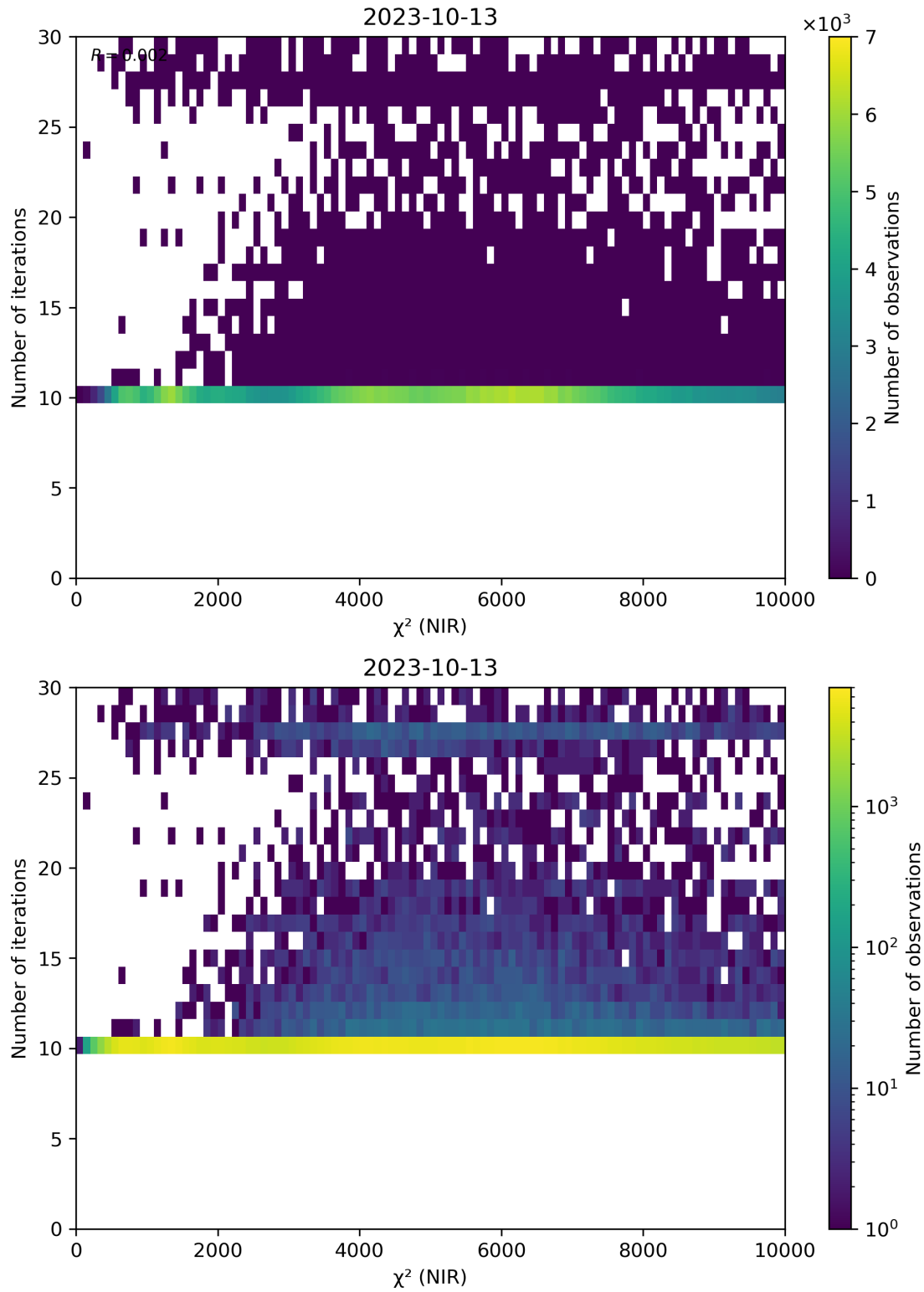
Figure 46: Scatter density plot of “ \chi^2 (NIR)” against “Number of iterations” for 2023-10-12 to 2023-10-14.
