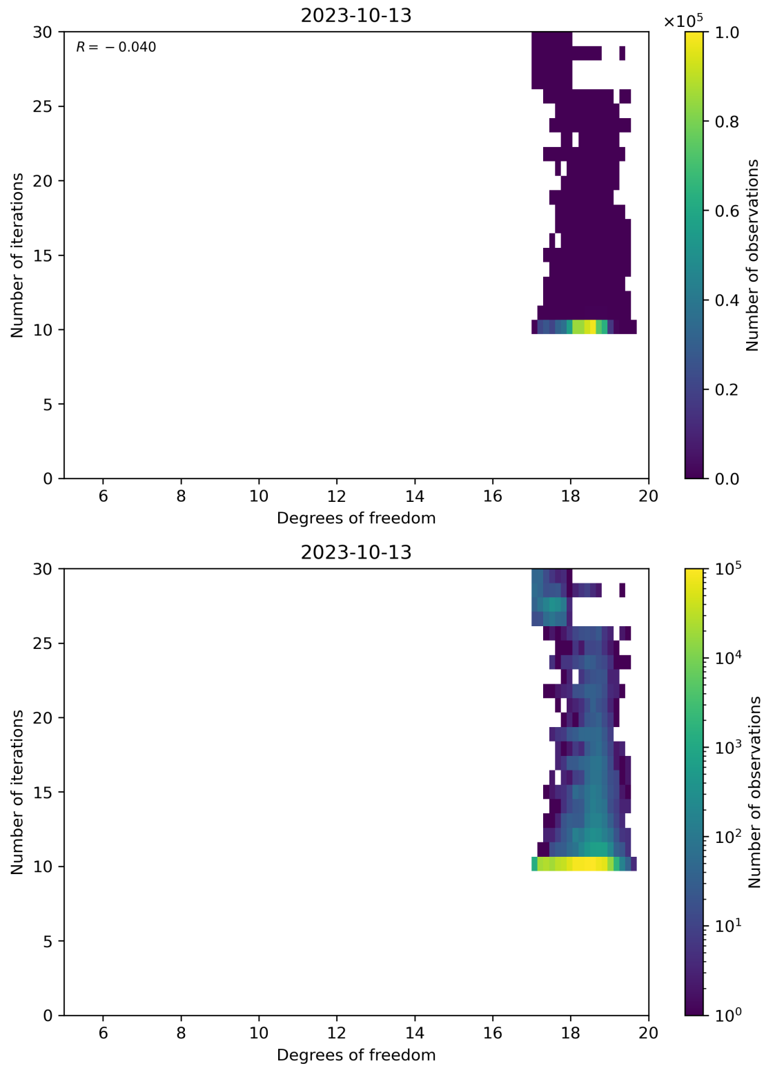
Figure 52: Scatter density plot of “Degrees of freedom” against “Number of iterations” for 2023-10-12 to 2023-10-14.
