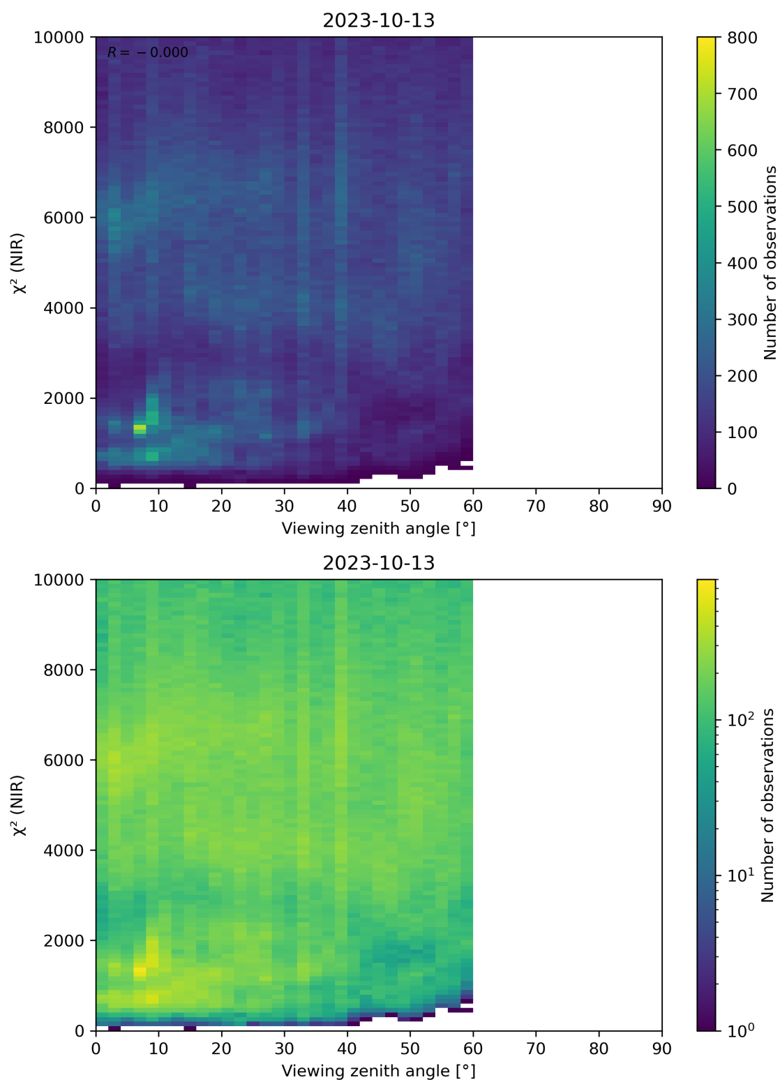
Figure 105: Scatter density plot of “Viewing zenith angle” against “ \chi^2 (NIR)” for 2023-10-12 to 2023-10-14.
