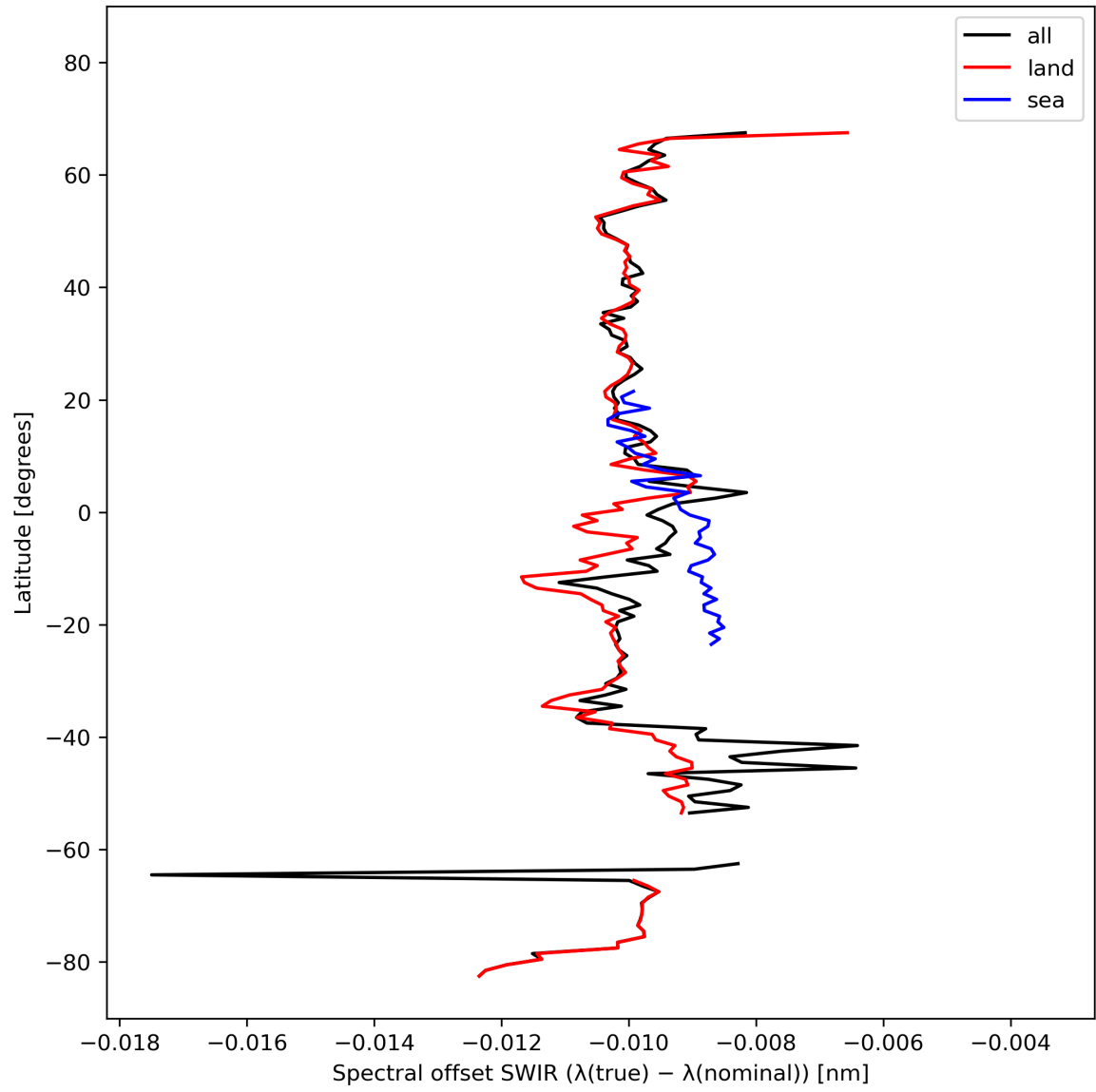
Figure 16: Zonal average of “Spectral offset SWIR ( \lambda(\text{true}) - \lambda(\text{nominal}) )” for 2023-10-12 to 2023-10-14.
