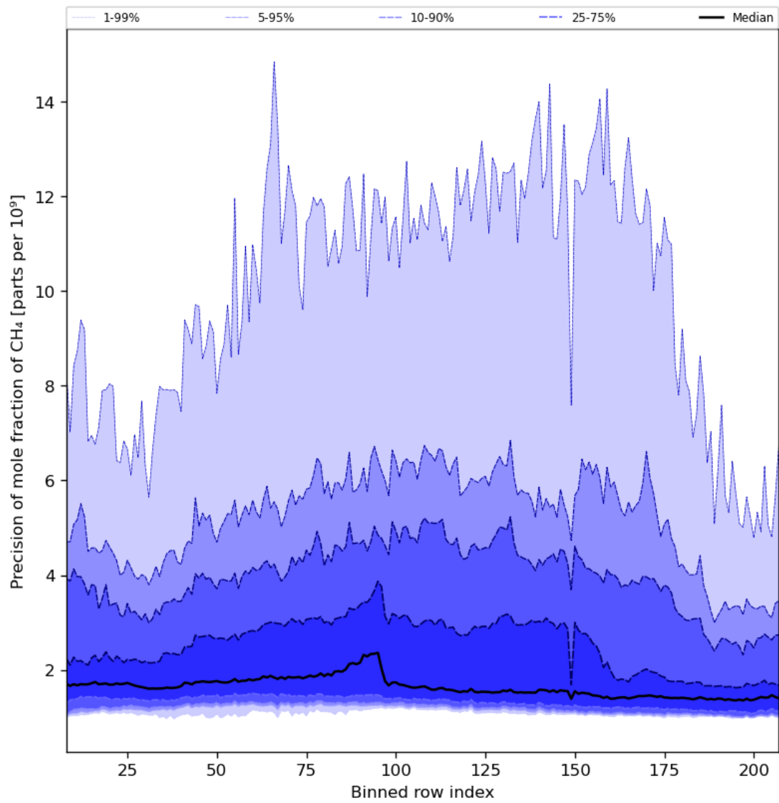
Figure 35: Along track statistics of “Precision of mole fraction of CH 4 ” for 2023-10-12 to 2023-10-14
