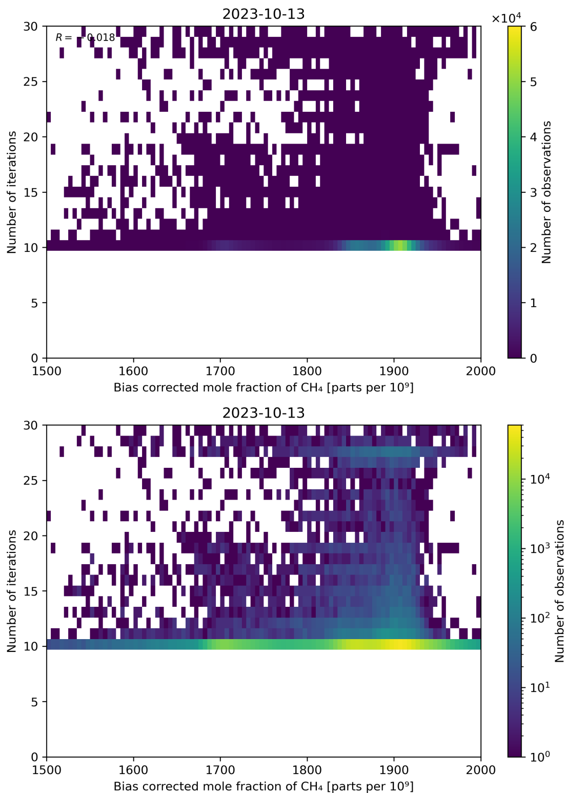
Figure 67: Scatter density plot of “Bias corrected mole fraction of CH 4 ” against “Number of iterations” for 2023-10-12 to 2023-10-14.
