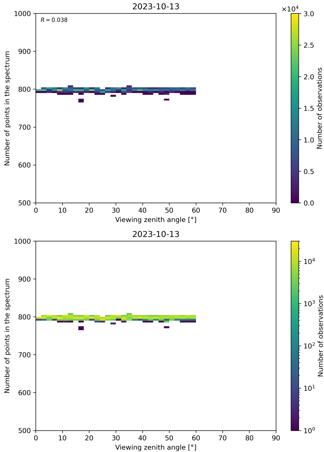
Figure 114: Scatter density plot of “Viewing zenith angle” against “Number of points in the spectrum” for 2023-10-12 to 2023-10-14.
