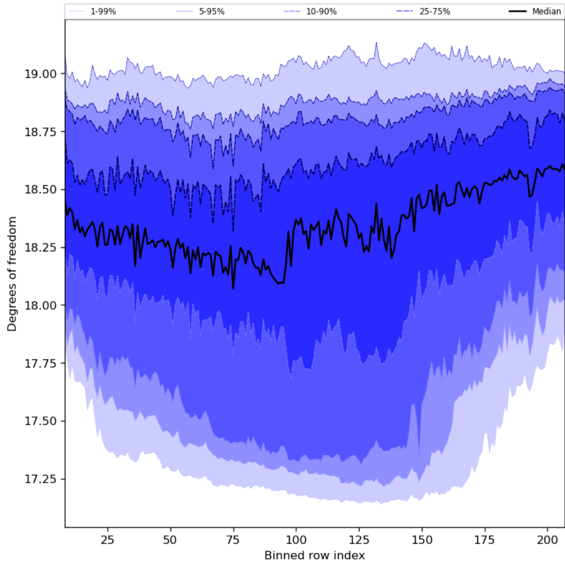
Figure 41: Along track statistics of “Degrees of freedom” for 2023-10-12 to 2023-10-14
