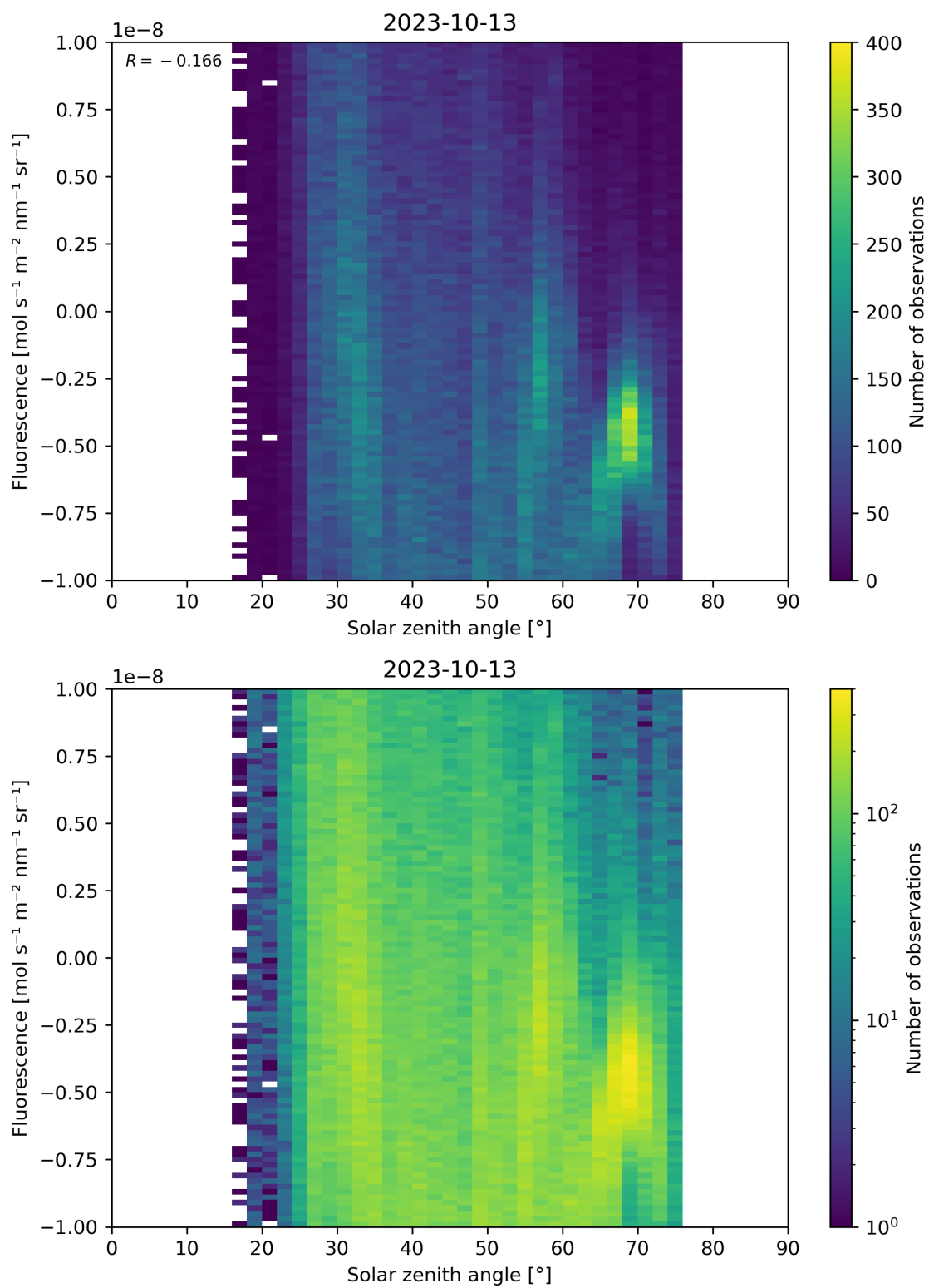
Figure 97: Scatter density plot of “Solar zenith angle” against “Fluorescence” for 2023-10-12 to 2023-10-14.
