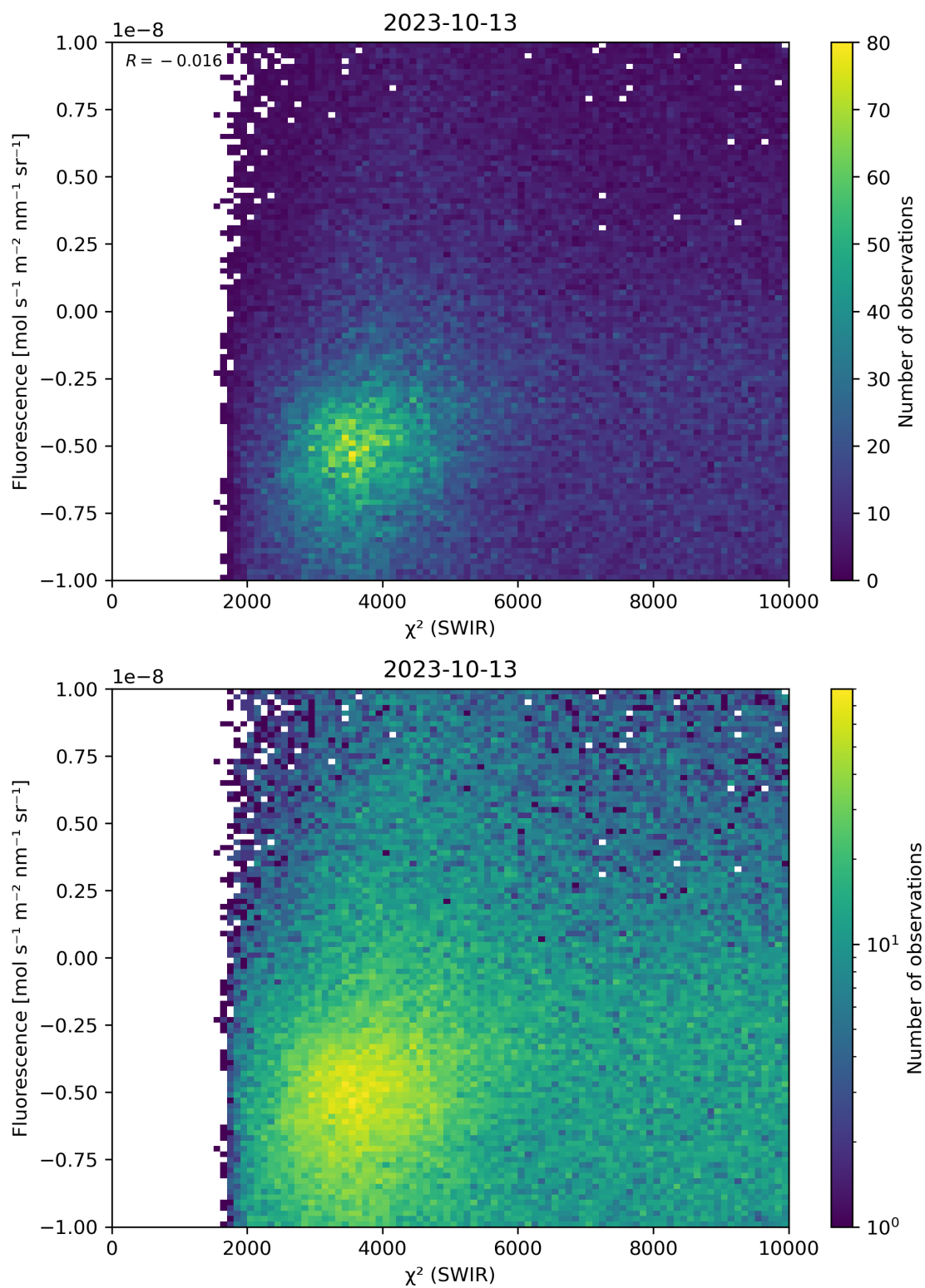
Figure 49: Scatter density plot of “ \chi^2 (SWIR)” against “Fluorescence” for 2023-10-12 to 2023-10-14.
