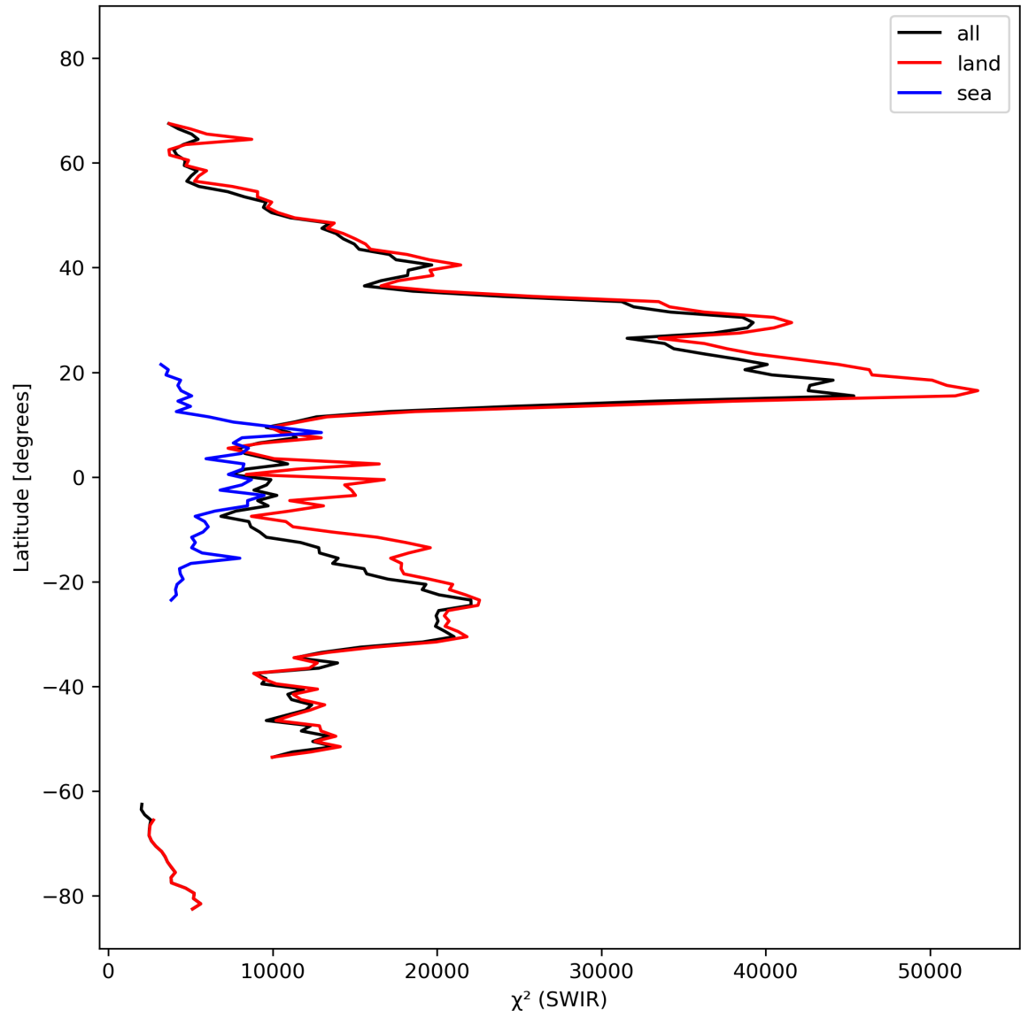
Figure 17: Zonal average of “ \chi^2 (SWIR)” for 2023-10-12 to 2023-10-14.
