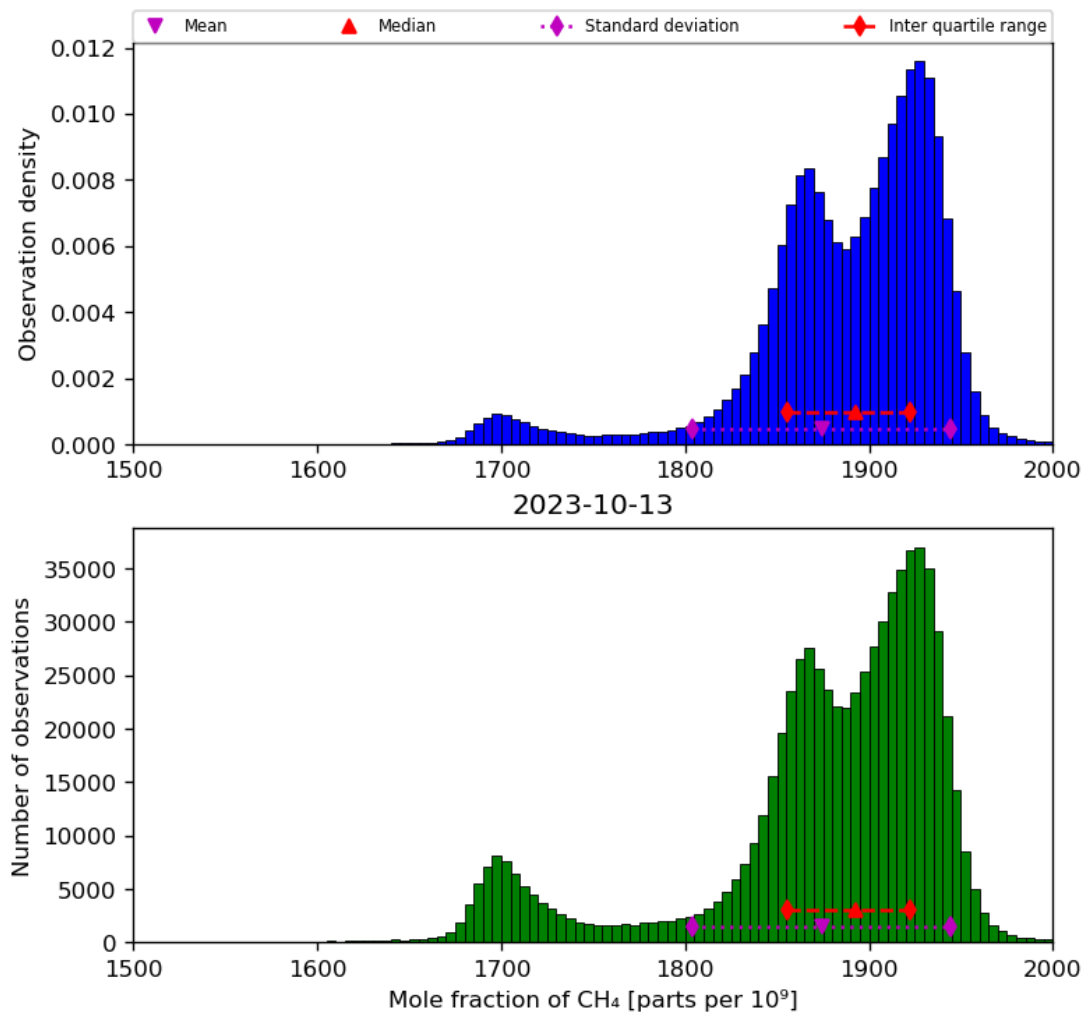
Figure 23: Histogram of “Mole fraction of CH 4 ” for 2023-10-12 to 2023-10-14
