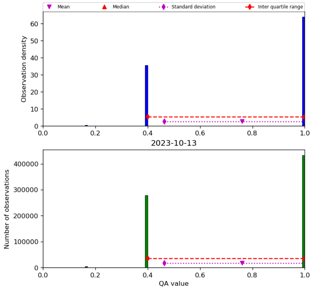
Figure 22: Histogram of “QA value” for 2023-10-12 to 2023-10-14
