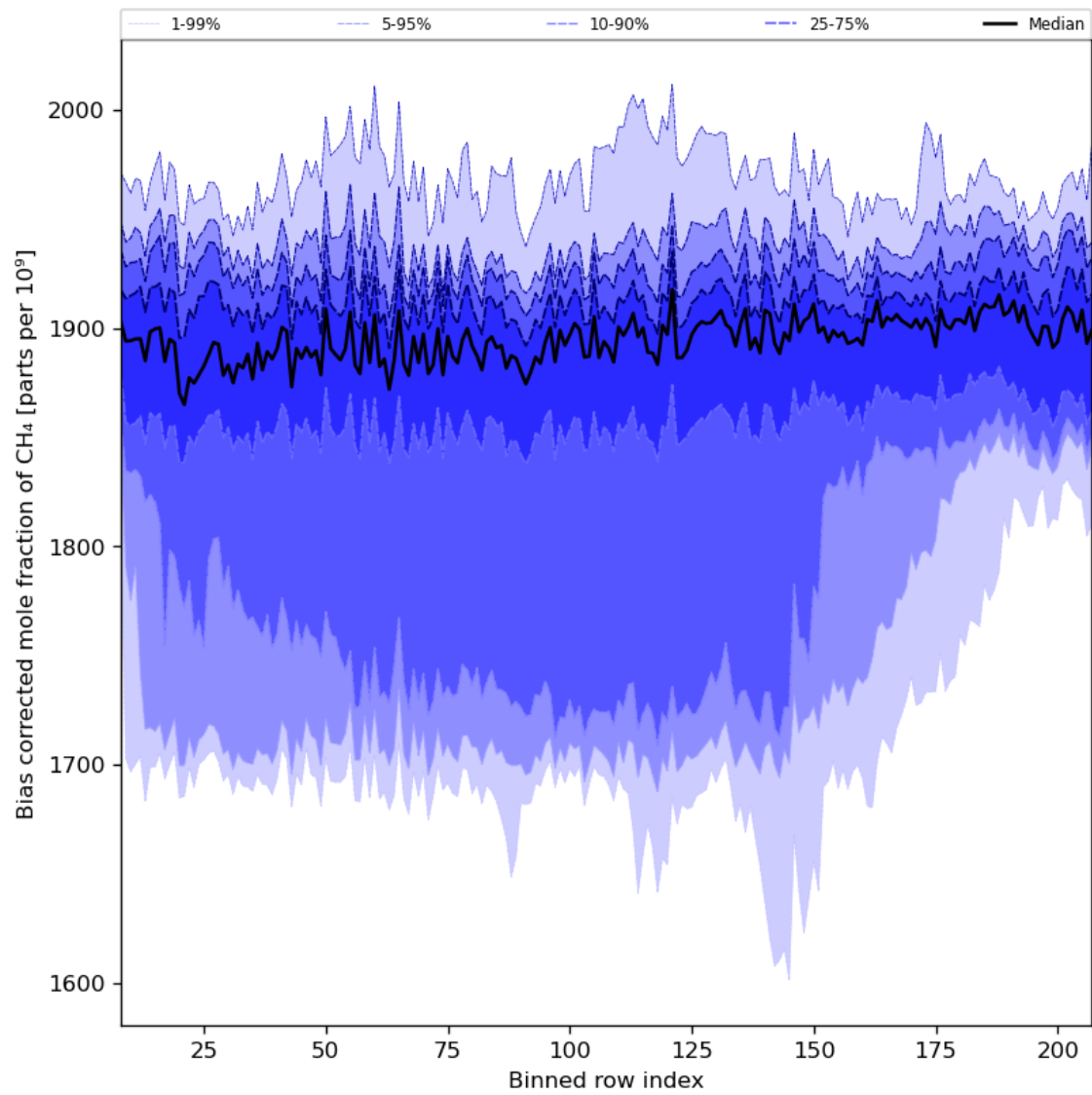
Figure 36: Along track statistics of “Bias corrected mole fraction of CH 4 ” for 2023-10-12 to 2023-10-14
