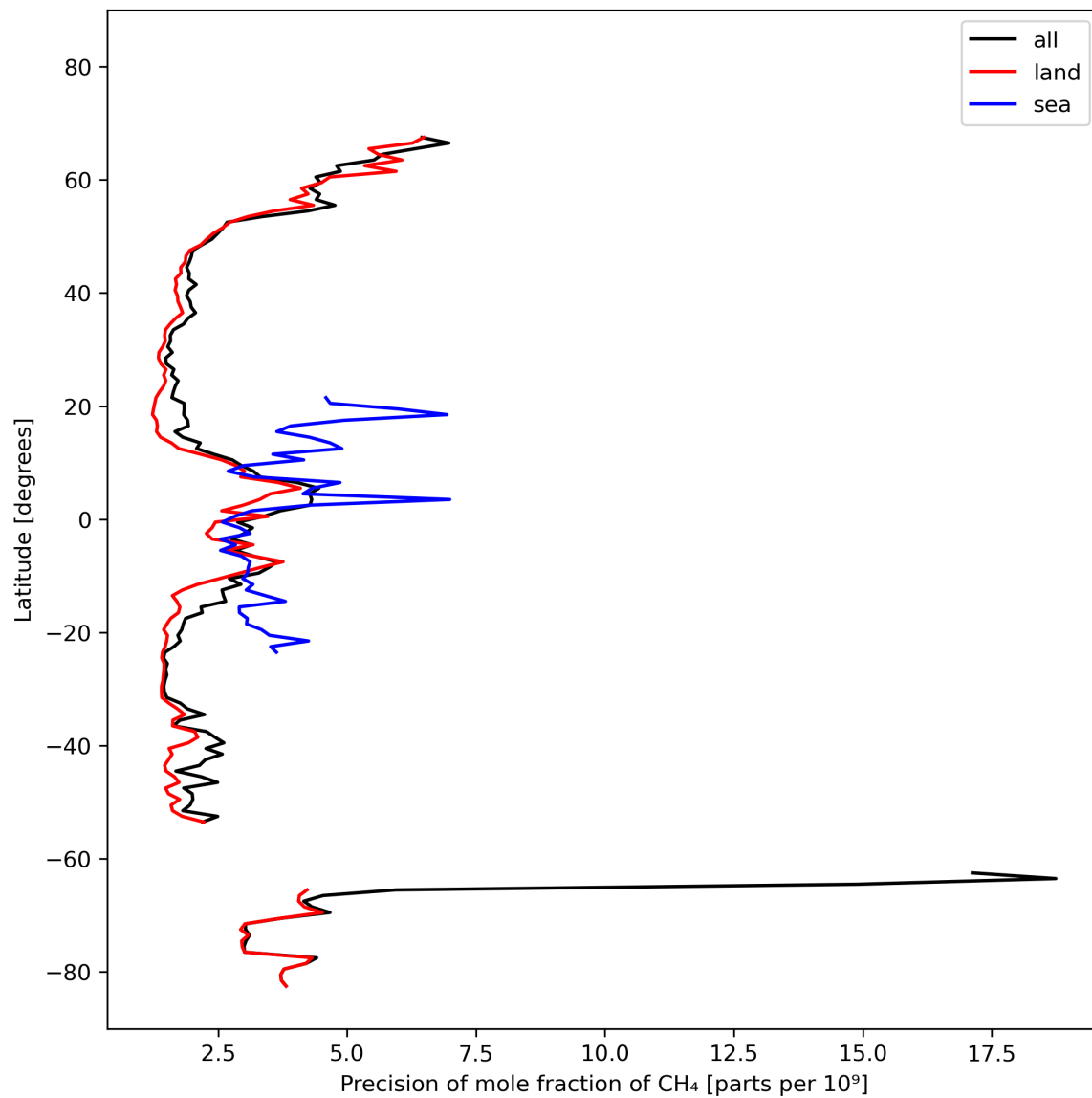
Figure 13: Zonal average of “Precision of mole fraction of CH 4 ” for 2023-10-12 to 2023-10-14.
