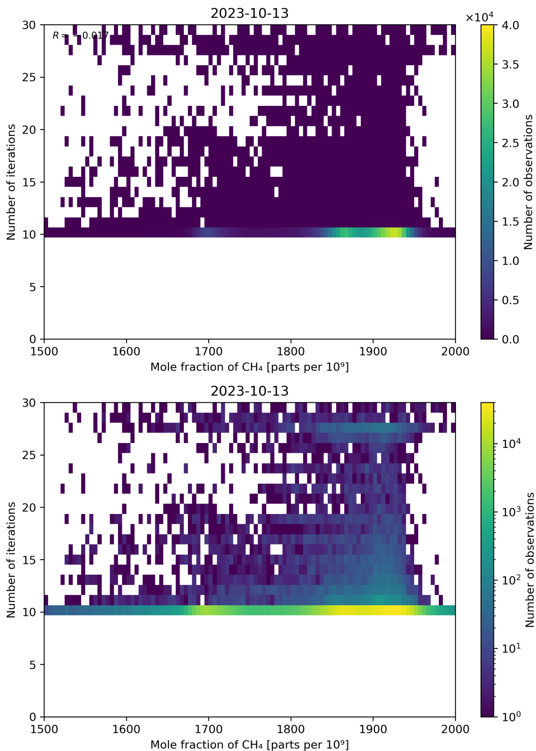
Figure 76: Scatter density plot of “Mole fraction of CH 4 ” against “Number of iterations” for 2023-10-12 to 2023-10-14.
