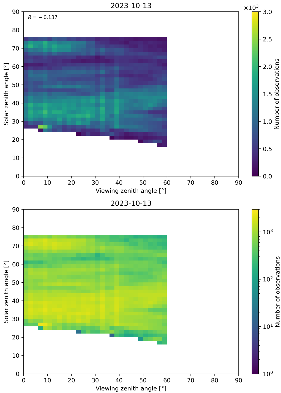
Figure 115: Scatter density plot of “Viewing zenith angle” against “Solar zenith angle” for 2023-10-12 to 2023-10-14.
