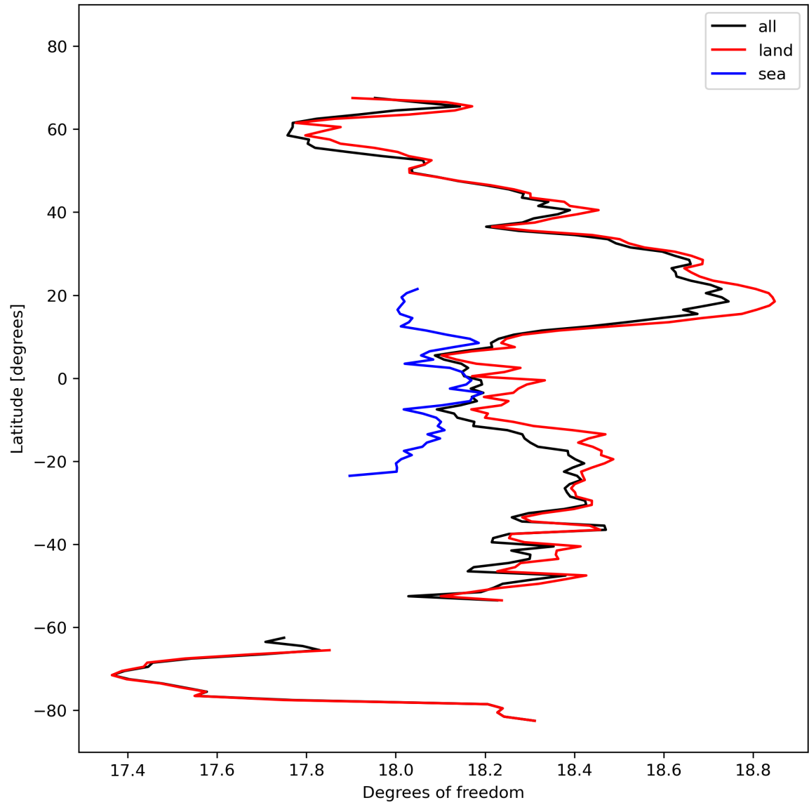
Figure 19: Zonal average of “Degrees of freedom” for 2023-10-12 to 2023-10-14.
