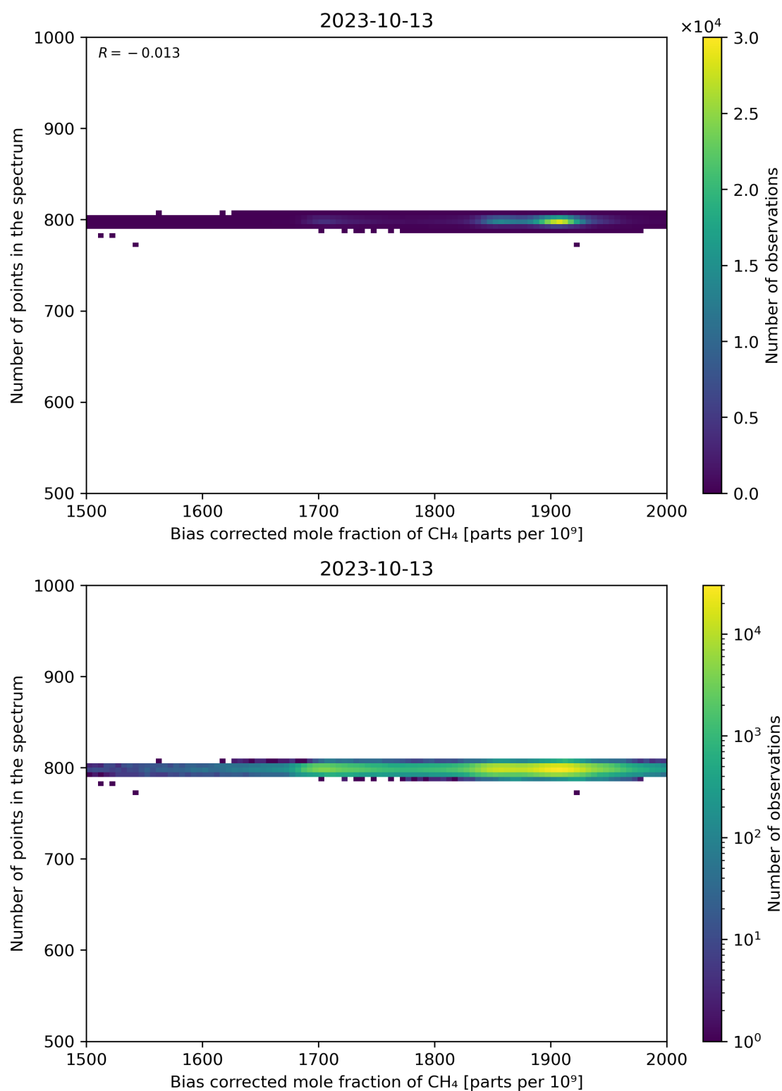
Figure 68: Scatter density plot of “Bias corrected mole fraction of CH 4 ” against “Number of points in the spectrum” for 2023-10-12 to 2023-10-14.
