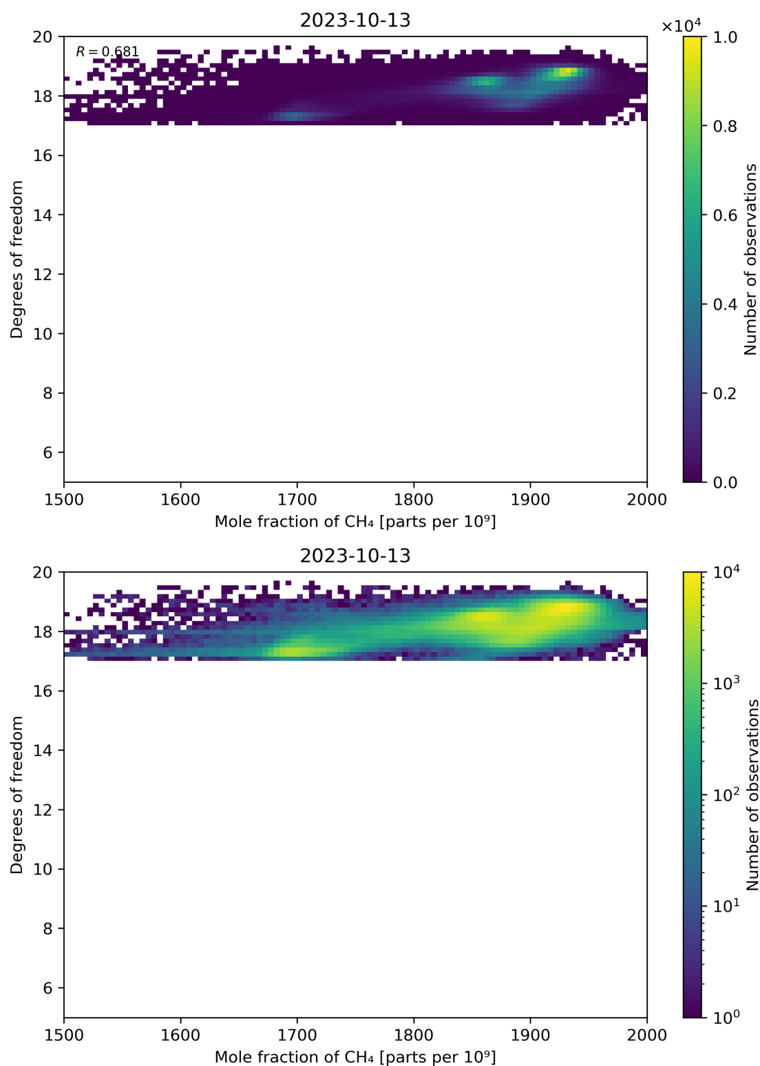
Figure 72: Scatter density plot of “Mole fraction of CH 4 ” against “Degrees of freedom” for 2023-10-12 to 2023-10-14.
