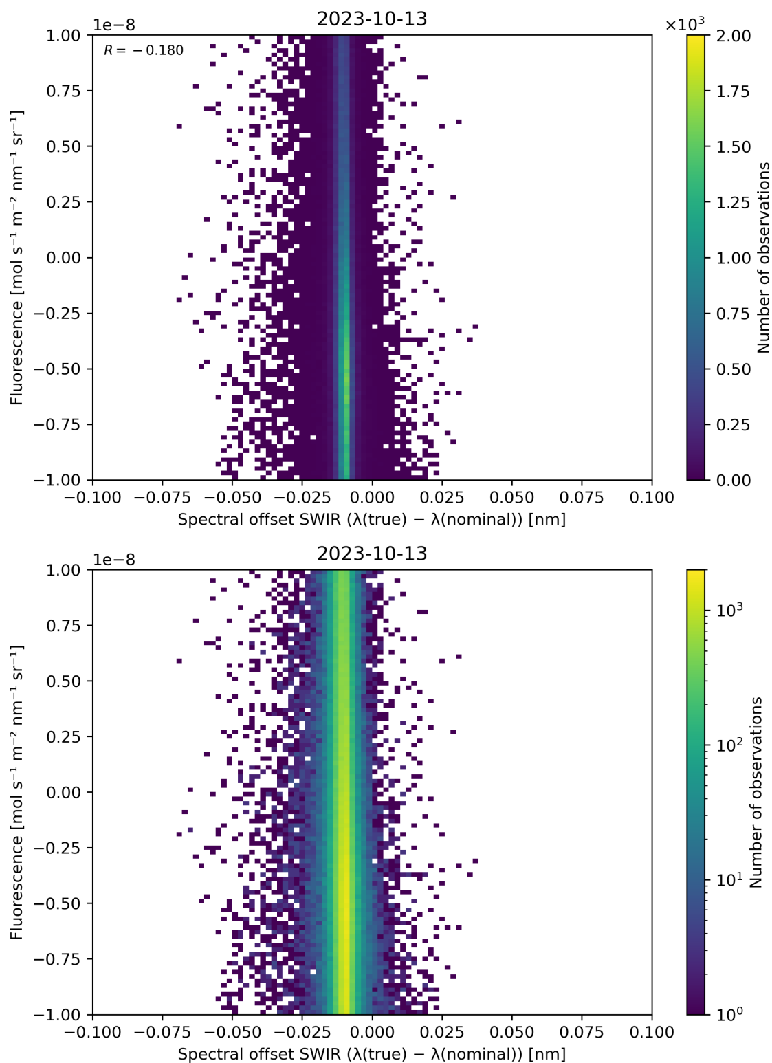
Figure 120: Scatter density plot of “Spectral offset SWIR ( \lambda(\text{true}) - \lambda(\text{nominal}) )” against “Fluorescence” for 2023-10-12 to 2023-10-14.
