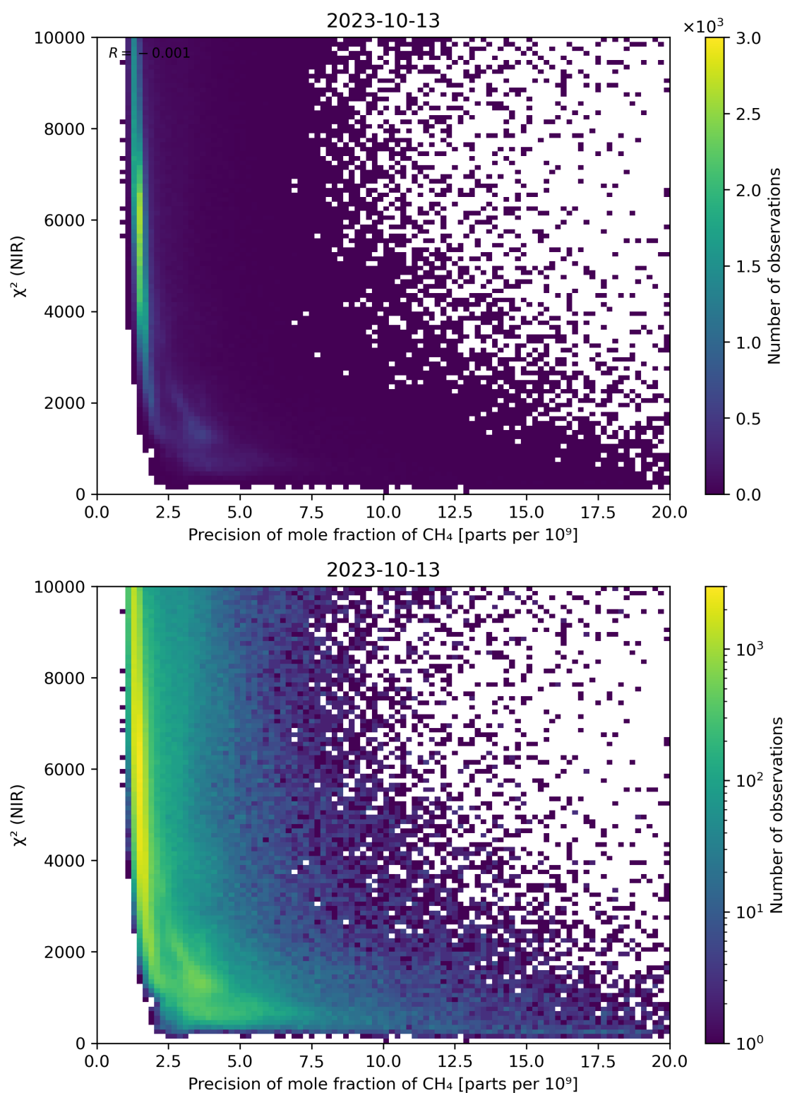
Figure 78: Scatter density plot of “Precision of mole fraction of CH 4 ” against “ \chi^2 (NIR)” for 2023-10-12 to 2023-10-14.
