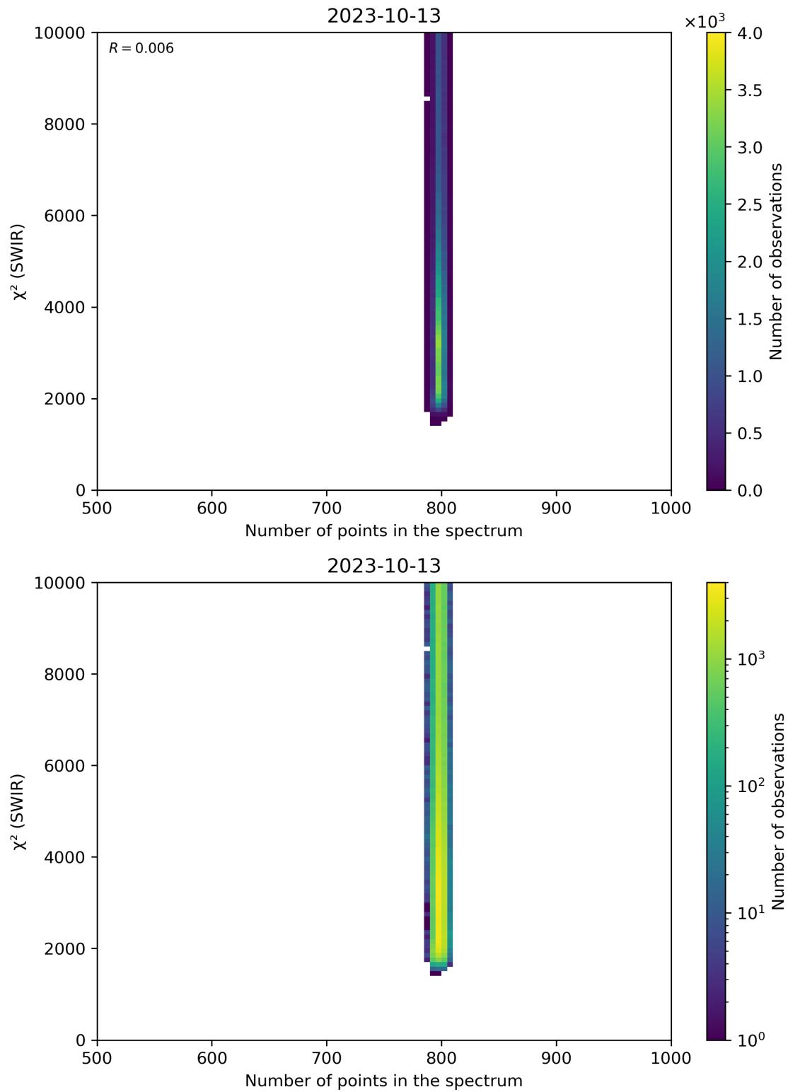
Figure 89: Scatter density plot of “Number of points in the spectrum” against “ \chi^2 (SWIR)” for 2023-10-12 to 2023-10-14.
