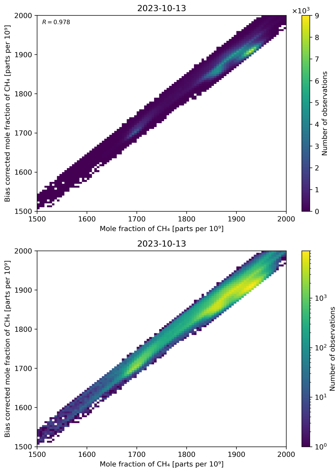
Figure 74: Scatter density plot of “Mole fraction of CH 4 ” against “Bias corrected mole fraction of CH 4 ” for 2023-10-12 to 2023-10-14.
