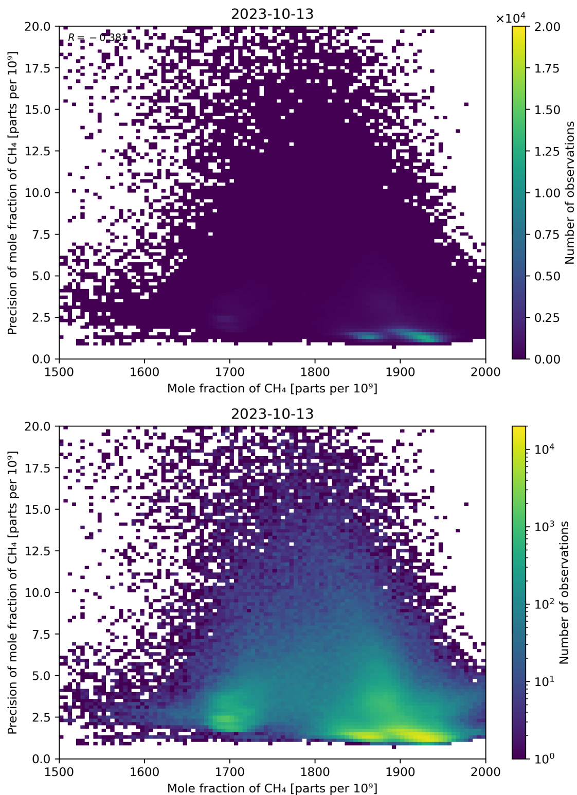
Figure 75: Scatter density plot of “Mole fraction of CH 4 ” against “Precision of mole fraction of CH 4 ” for 2023-10-12 to 2023-10-14.
