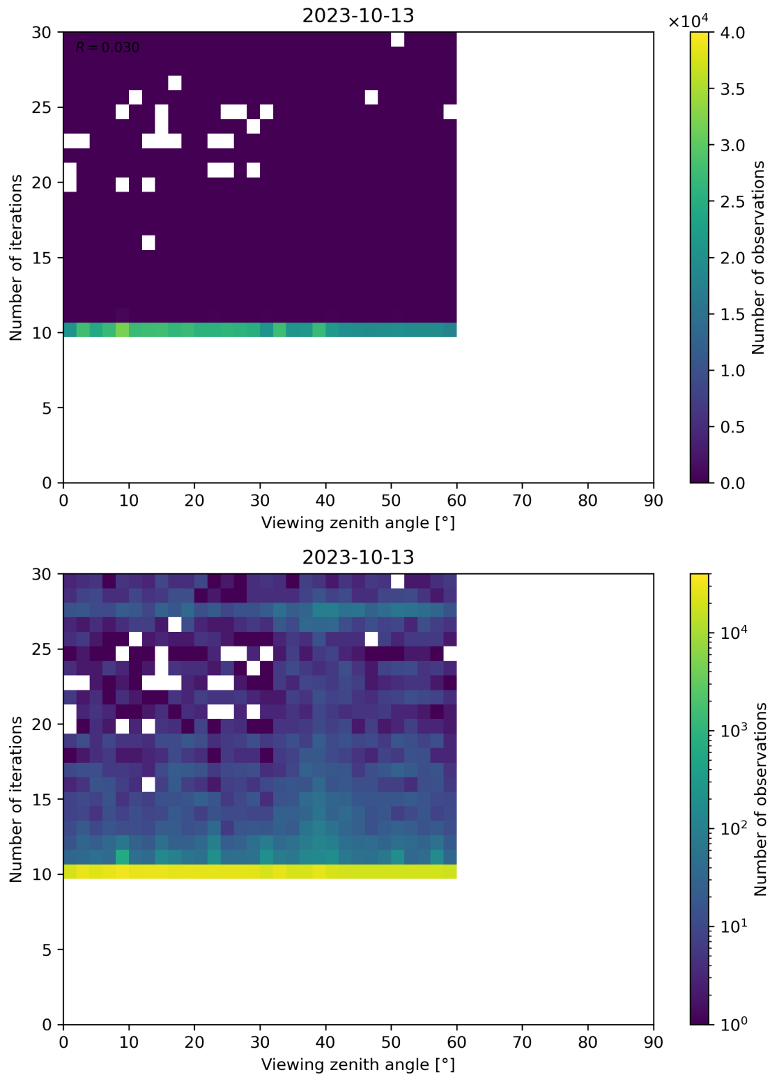
Figure 113: Scatter density plot of “Viewing zenith angle” against “Number of iterations” for 2023-10-12 to 2023-10-14.
