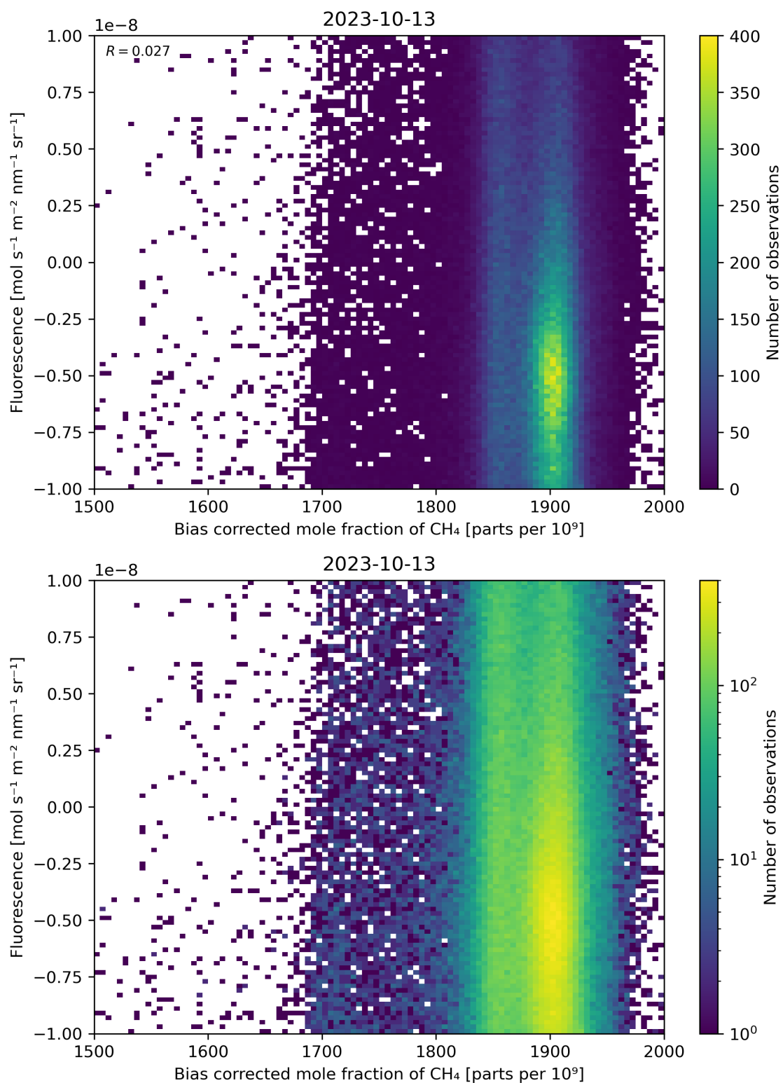
Figure 66: Scatter density plot of “Bias corrected mole fraction of \text{CH}_4 ” against “Fluorescence” for 2023-10-12 to 2023-10-14.
