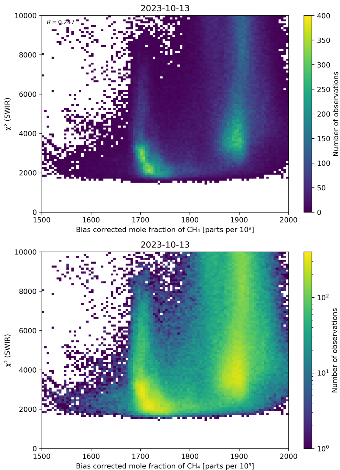
Figure 64: Scatter density plot of “Bias corrected mole fraction of CH 4 ” against “ \chi^2 (SWIR)” for 2023-10-12 to 2023-10-14.
