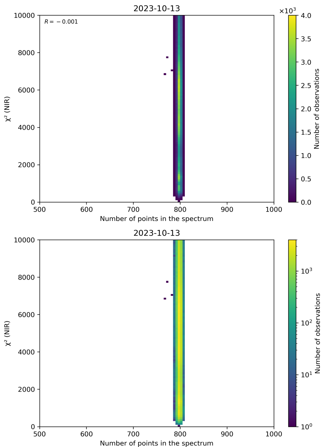
Figure 88: Scatter density plot of “Number of points in the spectrum” against “ \chi^2 (NIR)” for 2023-10-12 to 2023-10-14.
