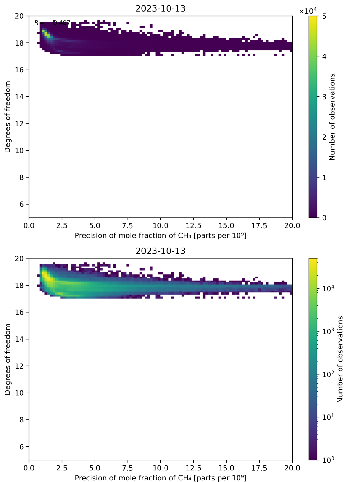
Figure 80: Scatter density plot of “Precision of mole fraction of CH 4 ” against “Degrees of freedom” for 2023-10-12 to 2023-10-14.
