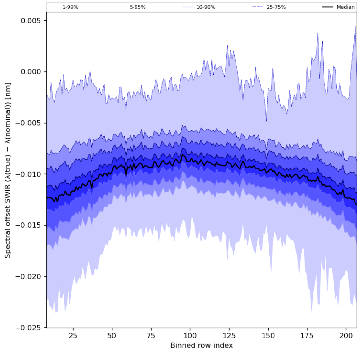
Figure 38: Along track statistics of “Spectral offset SWIR ( \lambda(\text{true}) - \lambda(\text{nominal}) )” for 2023-10-13 to 2023-10-15
