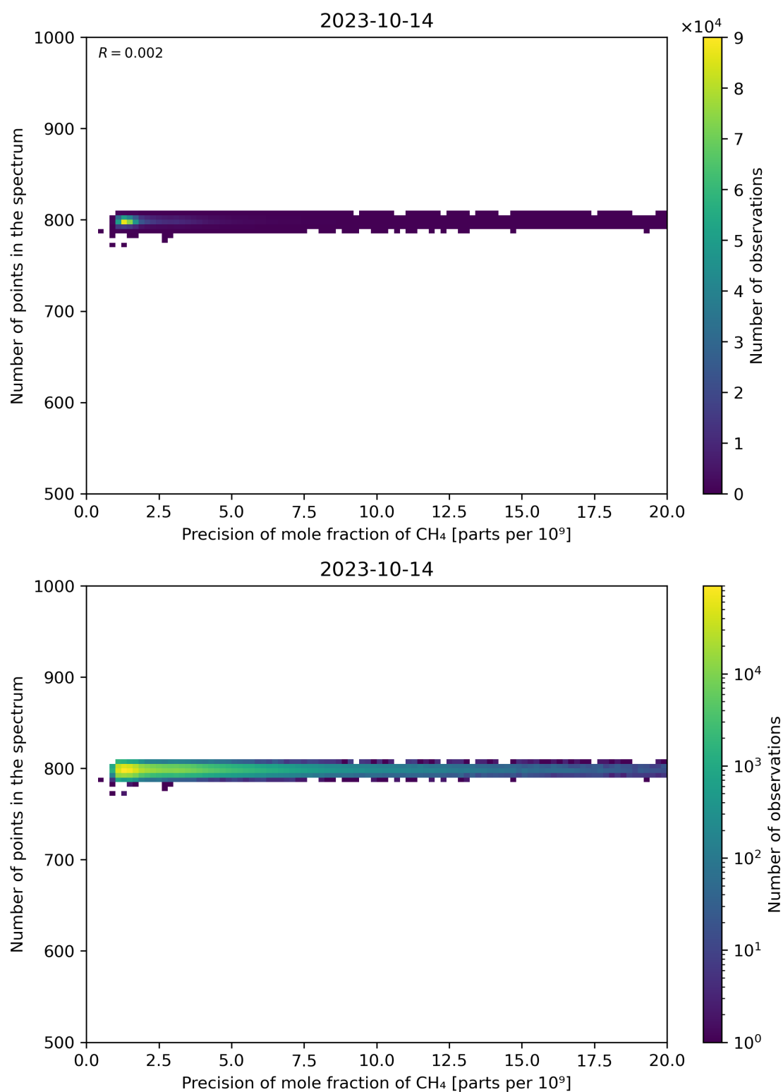
Figure 84: Scatter density plot of “Precision of mole fraction of CH 4 ” against “Number of points in the spectrum” for 2023-10-13 to 2023-10-15.
