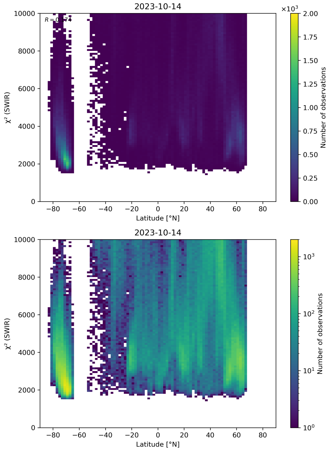
Figure 54: Scatter density plot of “Latitude” against “ \chi^2 (SWIR)” for 2023-10-13 to 2023-10-15.
