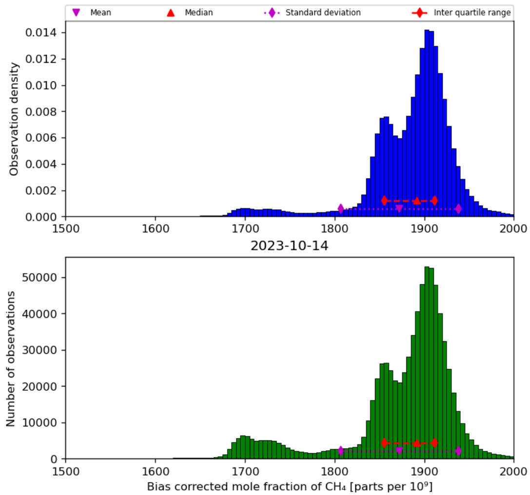
Figure 25: Histogram of “Bias corrected mole fraction of CH 4 ” for 2023-10-13 to 2023-10-15
