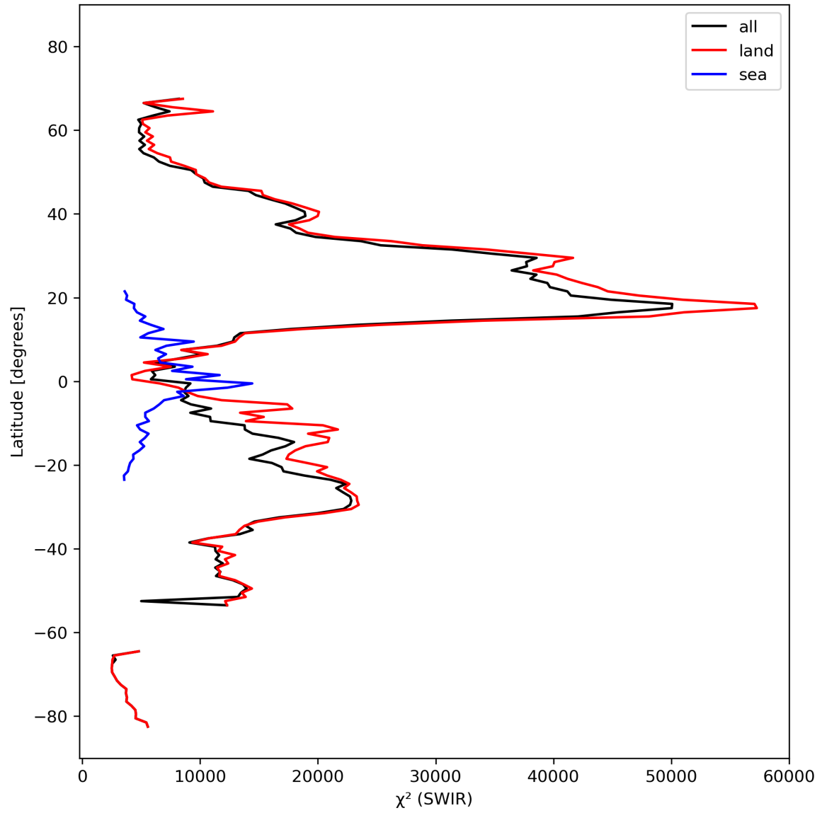
Figure 17: Zonal average of “ \chi^2 (SWIR)” for 2023-10-13 to 2023-10-15.
