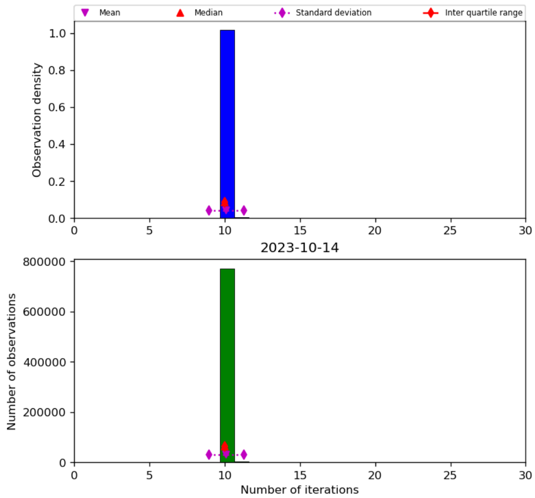
Figure 31: Histogram of “Number of iterations” for 2023-10-13 to 2023-10-15
