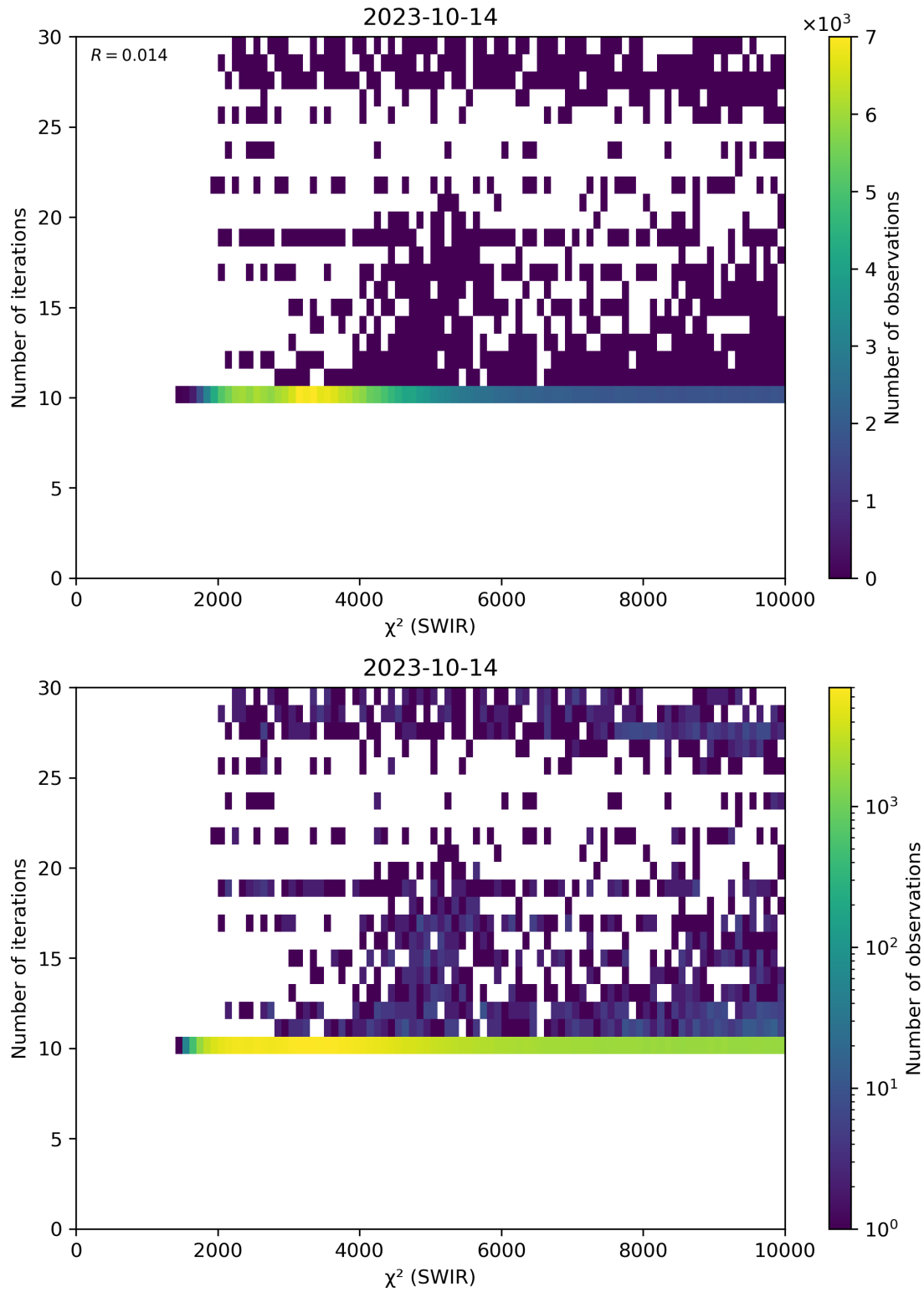
Figure 50: Scatter density plot of “ \chi^2 (SWIR)” against “Number of iterations” for 2023-10-13 to 2023-10-15.
