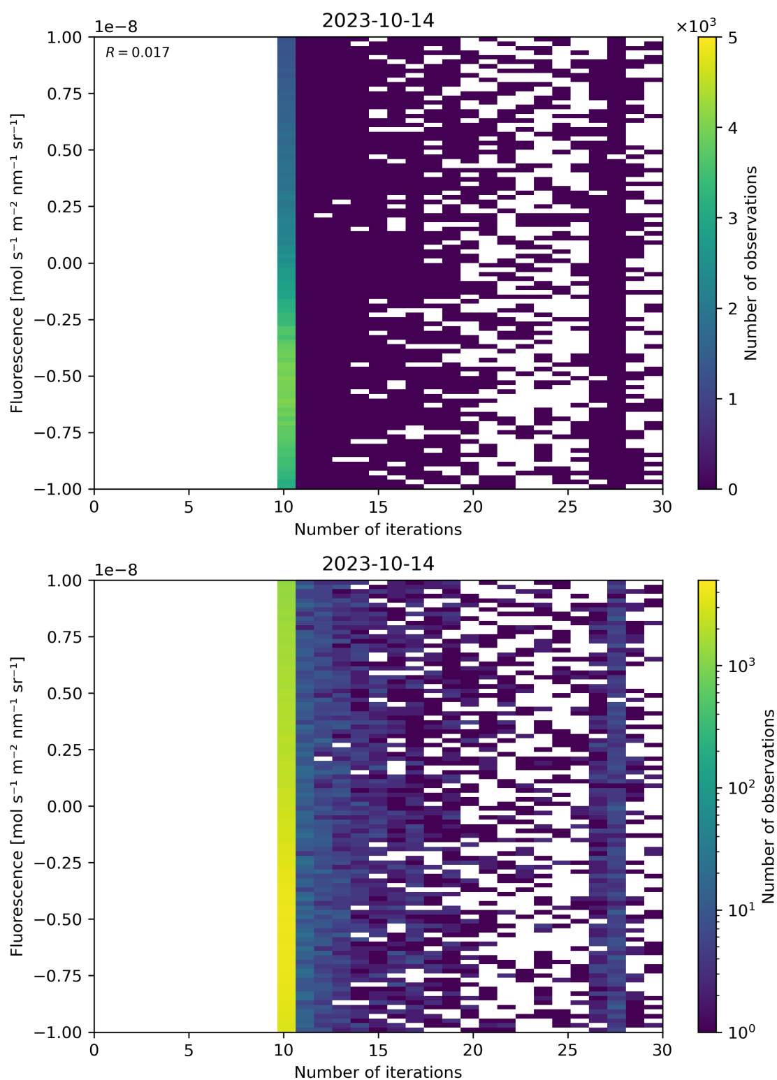
Figure 87: Scatter density plot of “Number of iterations” against “Fluorescence” for 2023-10-13 to 2023-10-15.
