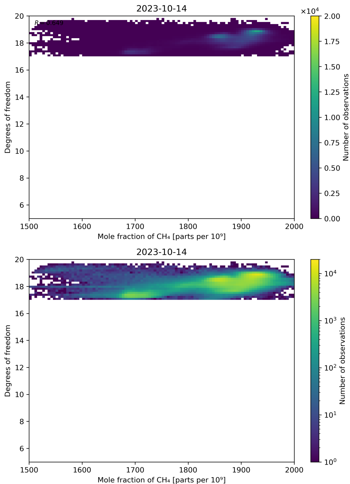
Figure 72: Scatter density plot of “Mole fraction of CH 4 ” against “Degrees of freedom” for 2023-10-13 to 2023-10-15.
