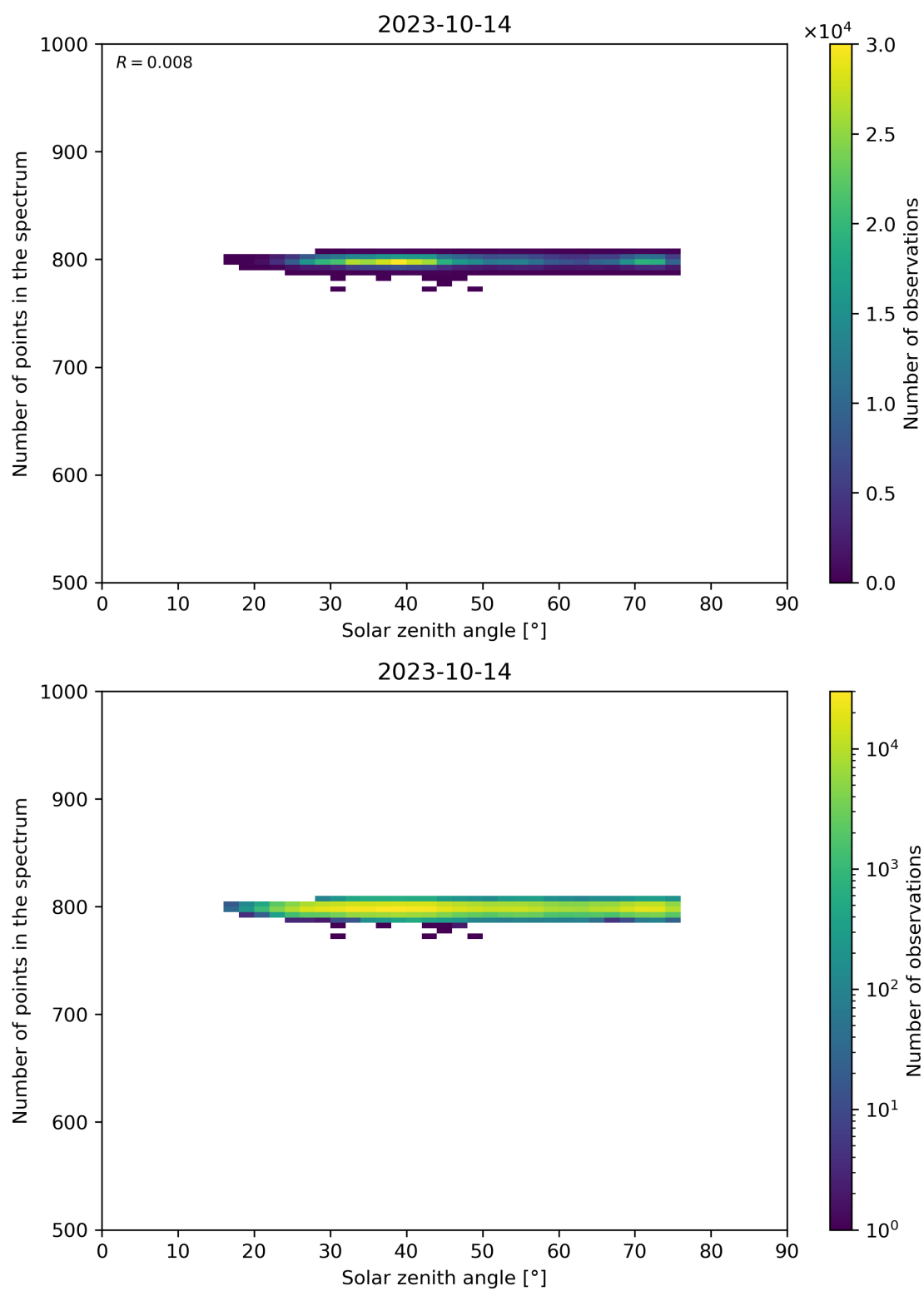
Figure 103: Scatter density plot of “Solar zenith angle” against “Number of points in the spectrum” for 2023-10-13 to 2023-10-15.
