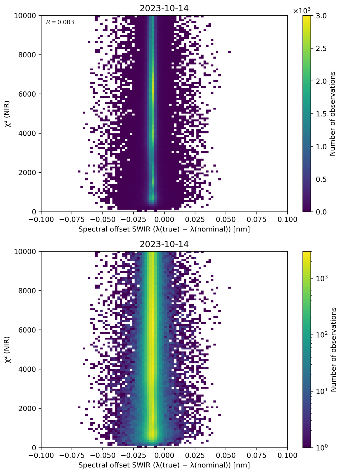
Figure 117: Scatter density plot of “Spectral offset SWIR ( \lambda(\text{true}) - \lambda(\text{nominal}) )” against “ \chi^2 (NIR)” for 2023-10-13 to 2023-10-15.
