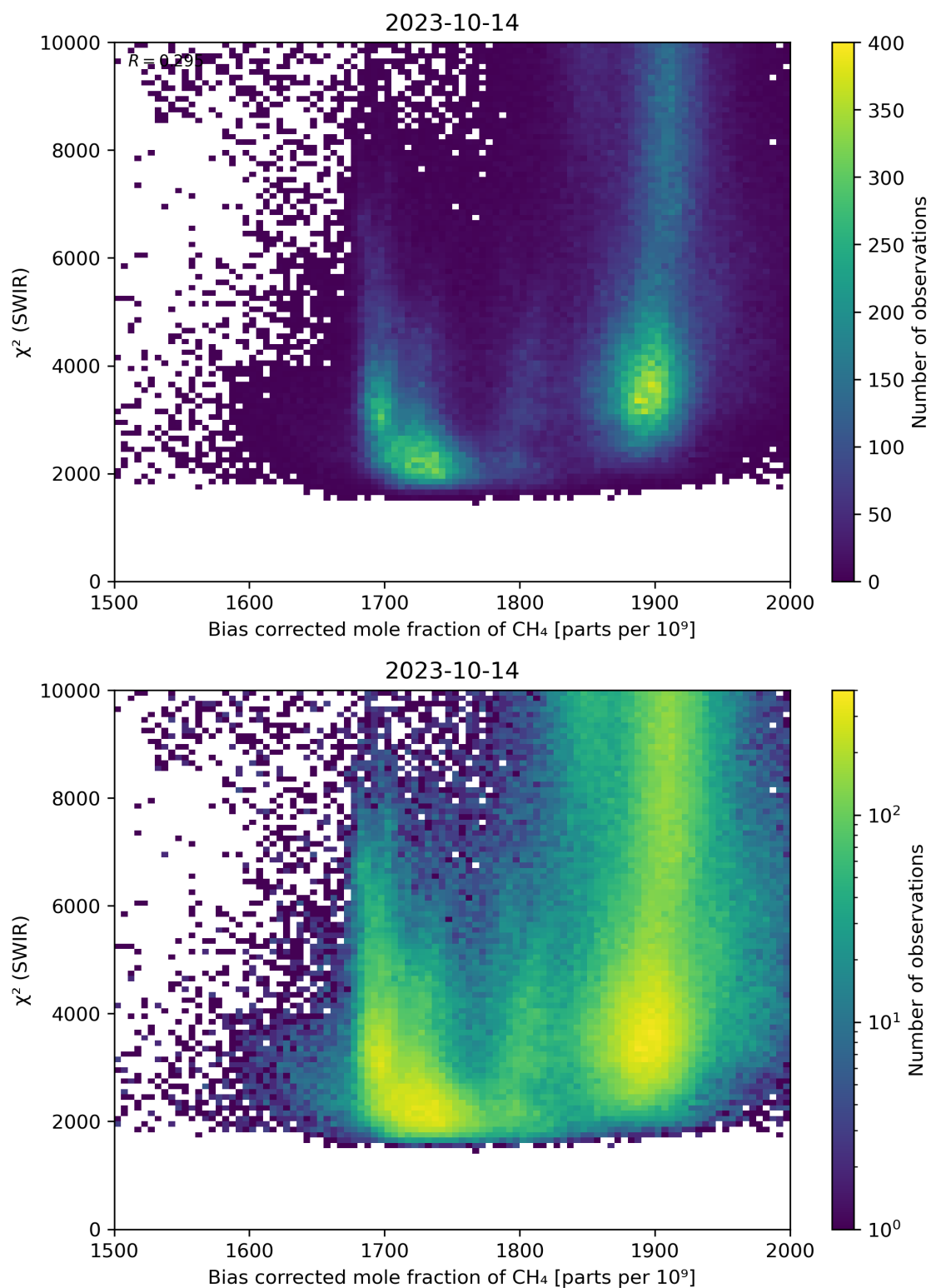
Figure 64: Scatter density plot of “Bias corrected mole fraction of CH 4 ” against “ \chi^2 (SWIR)” for 2023-10-13 to 2023-10-15.
