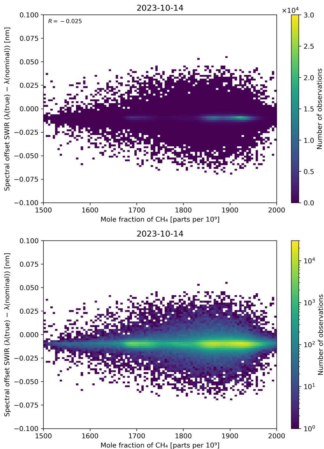
Figure 86: Scatter density plot of “Mole fraction of CH 4 ” against “Spectral offset SWIR ( \lambda(\text{true}) - \lambda(\text{nominal}) )” for 2023-10-13 to 2023-10-15.
