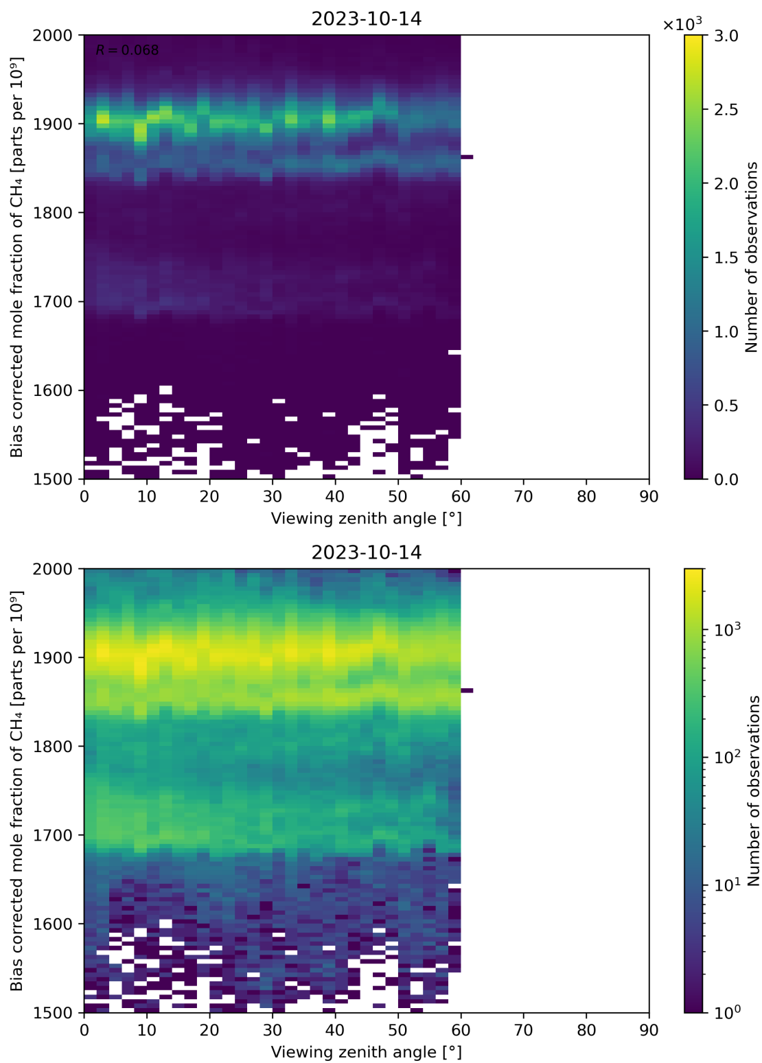
Figure 111: Scatter density plot of “Viewing zenith angle” against “Bias corrected mole fraction of CH 4 ” for 2023-10-13 to 2023-10-15.
