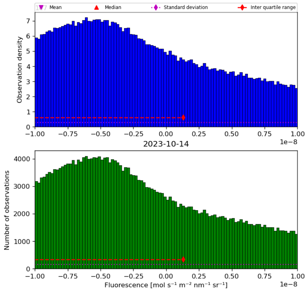
Figure 32: Histogram of “Fluorescence” for 2023-10-13 to 2023-10-15
