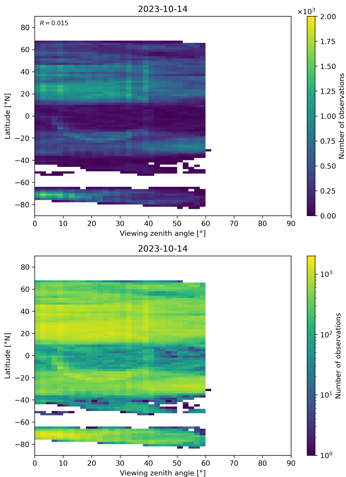
Figure 109: Scatter density plot of “Viewing zenith angle” against “Latitude” for 2023-10-13 to 2023-10-15.
