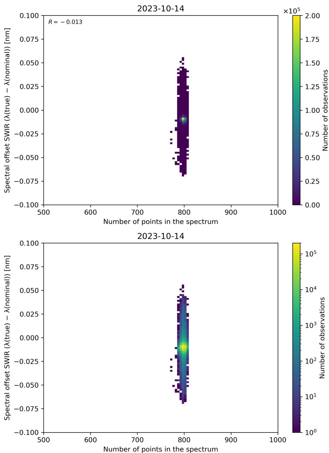
Figure 93: Scatter density plot of “Number of points in the spectrum” against “Spectral offset SWIR ( \lambda(\text{true}) - \lambda(\text{nominal}) )” for 2023-10-13 to 2023-10-15.
