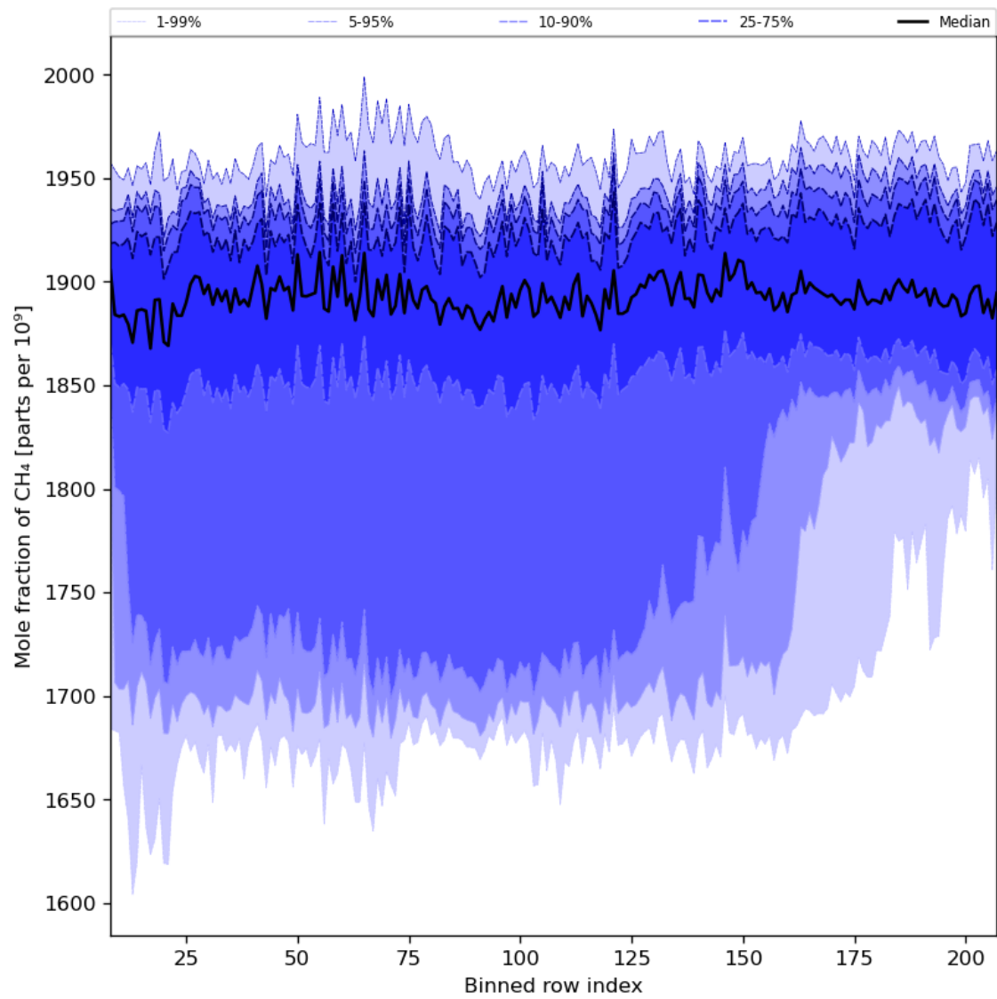
Figure 34: Along track statistics of “Mole fraction of CH 4 ” for 2023-10-13 to 2023-10-15
