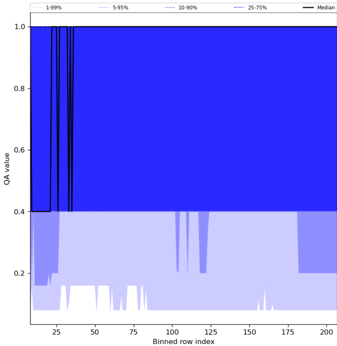
Figure 33: Along track statistics of “QA value” for 2023-10-13 to 2023-10-15
