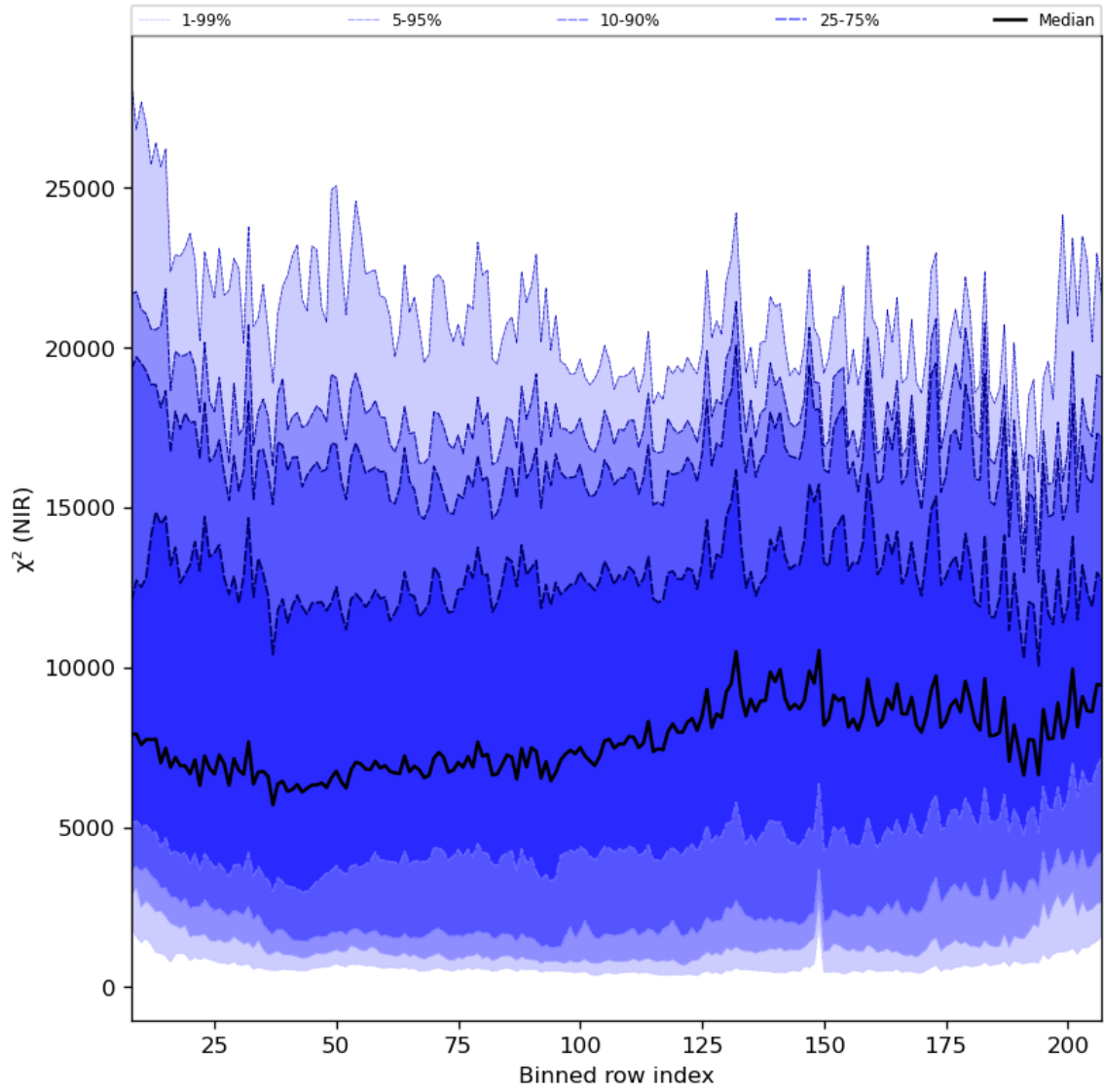
Figure 40: Along track statistics of “ \chi^2 (NIR)” for 2023-10-13 to 2023-10-15
