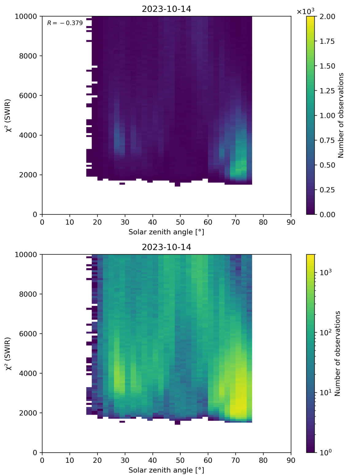
Figure 95: Scatter density plot of “Solar zenith angle” against “ \chi^2 (SWIR)” for 2023-10-13 to 2023-10-15.
