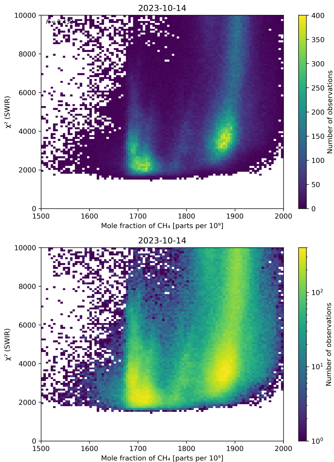
Figure 71: Scatter density plot of “Mole fraction of CH 4 ” against “ \chi^2 (SWIR)” for 2023-10-13 to 2023-10-15.
