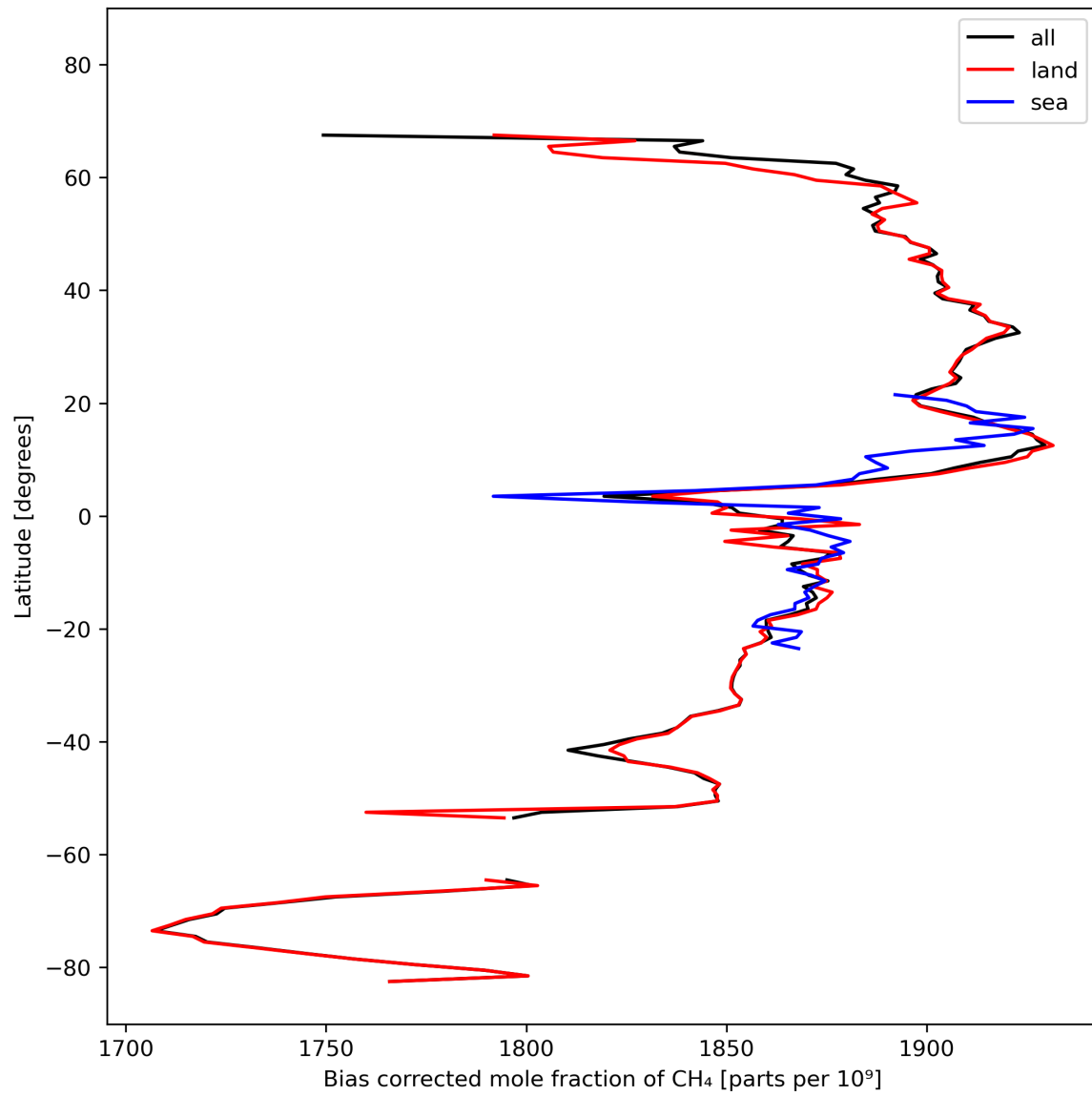
Figure 14: Zonal average of “Bias corrected mole fraction of CH 4 ” for 2023-10-13 to 2023-10-15.
