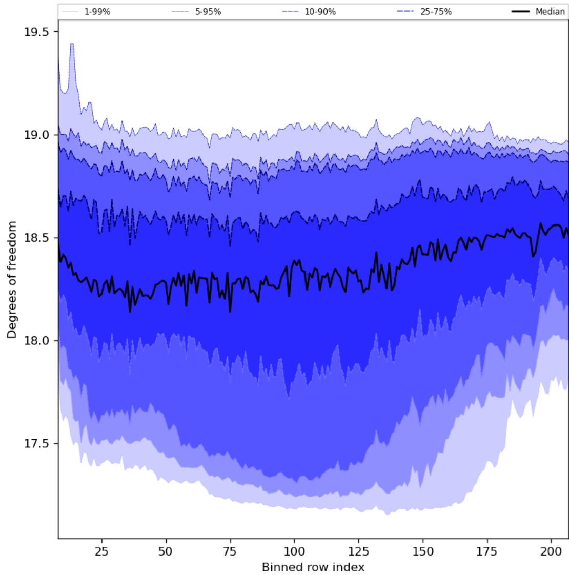
Figure 41: Along track statistics of “Degrees of freedom” for 2023-10-13 to 2023-10-15
