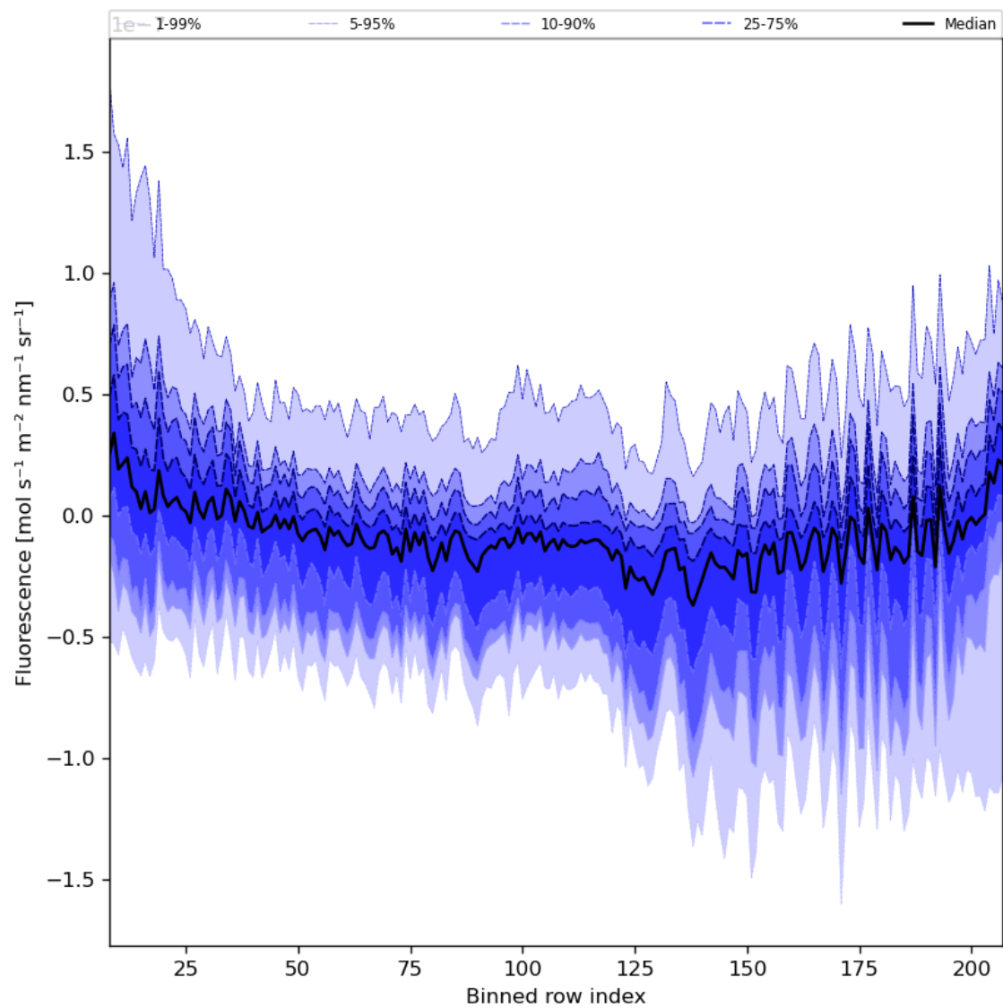
Figure 43: Along track statistics of “Fluorescence” for 2023-10-13 to 2023-10-15
