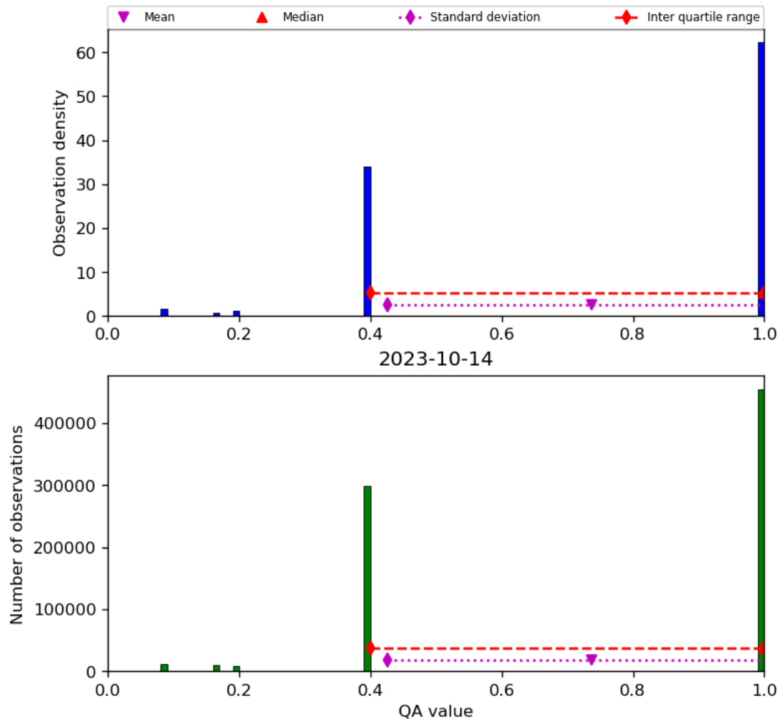
Figure 22: Histogram of “QA value” for 2023-10-13 to 2023-10-15
