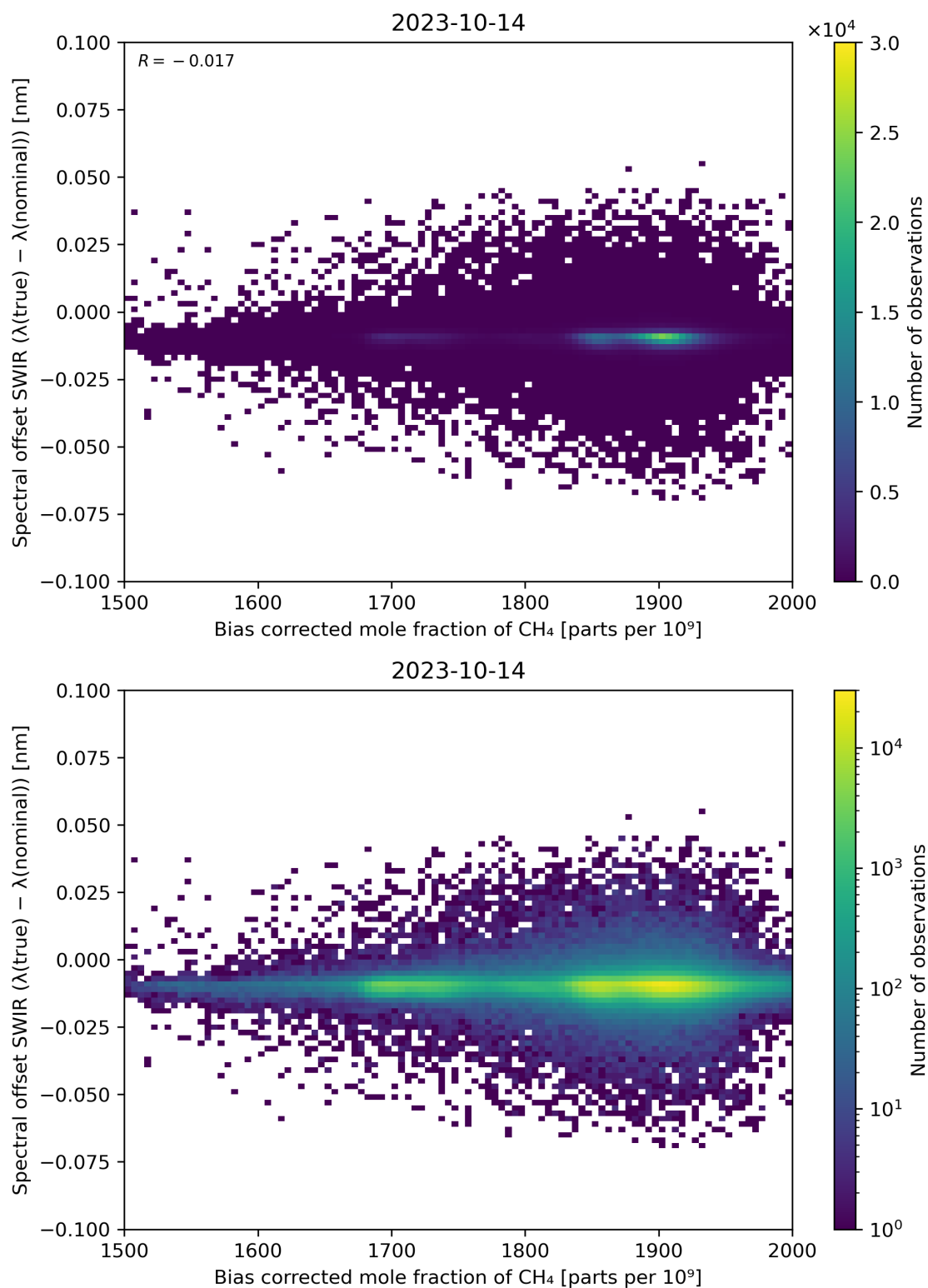
Figure 69: Scatter density plot of “Bias corrected mole fraction of \text{CH}_4 ” against “Spectral offset SWIR ( \lambda(\text{true}) - \lambda(\text{nominal}) )” for 2023-10-13 to 2023-10-15.
