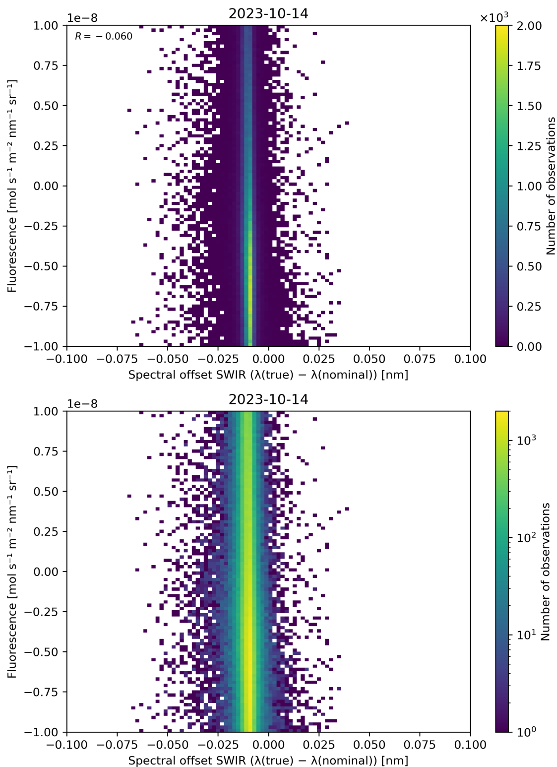
Figure 120: Scatter density plot of “Spectral offset SWIR ( \lambda(\text{true}) - \lambda(\text{nominal}) )” against “Fluorescence” for 2023-10-13 to 2023-10-15.
