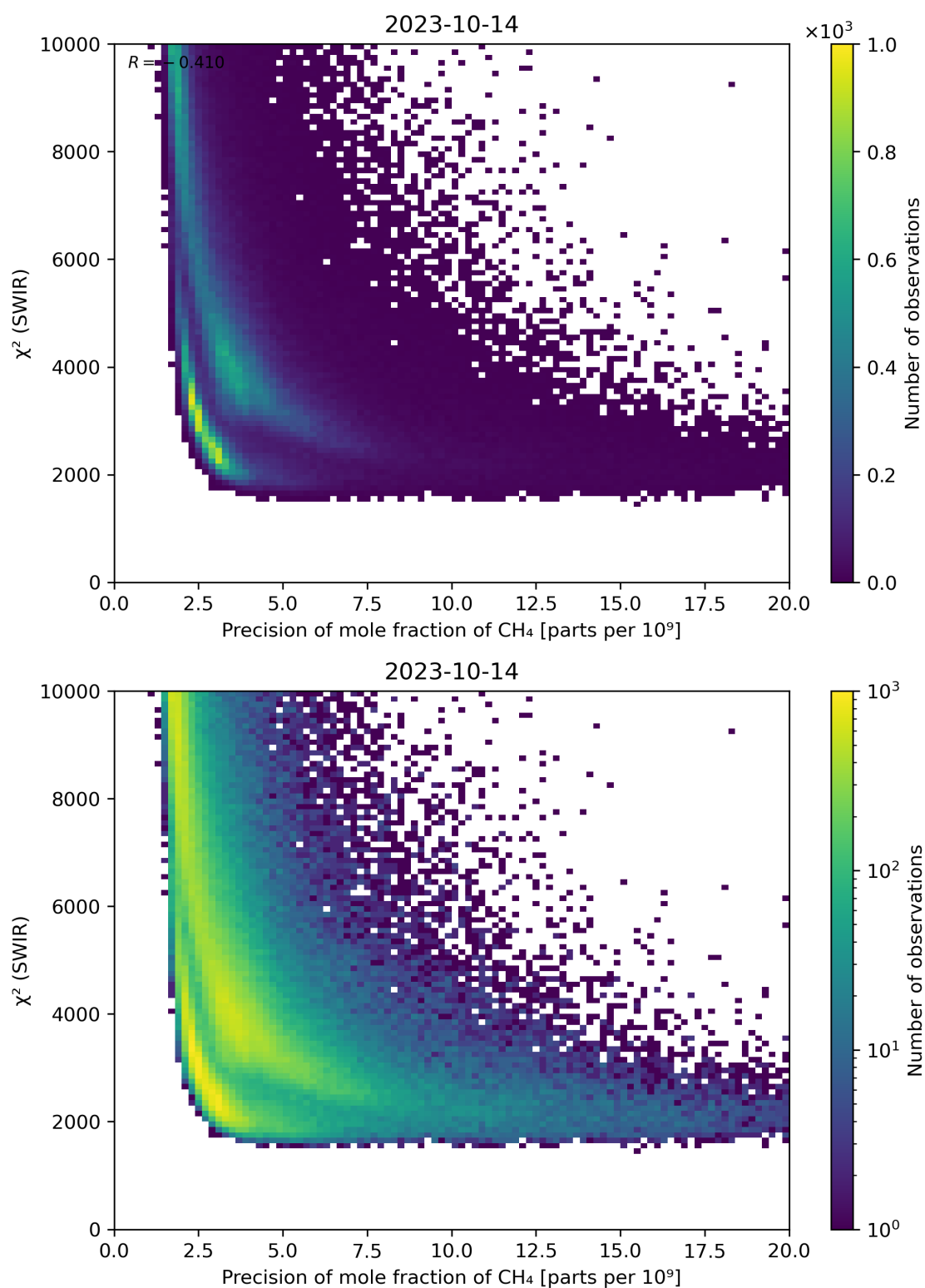
Figure 79: Scatter density plot of “Precision of mole fraction of \text{CH}_4 ” against “ \chi^2 (SWIR)” for 2023-10-13 to 2023-10-15.
