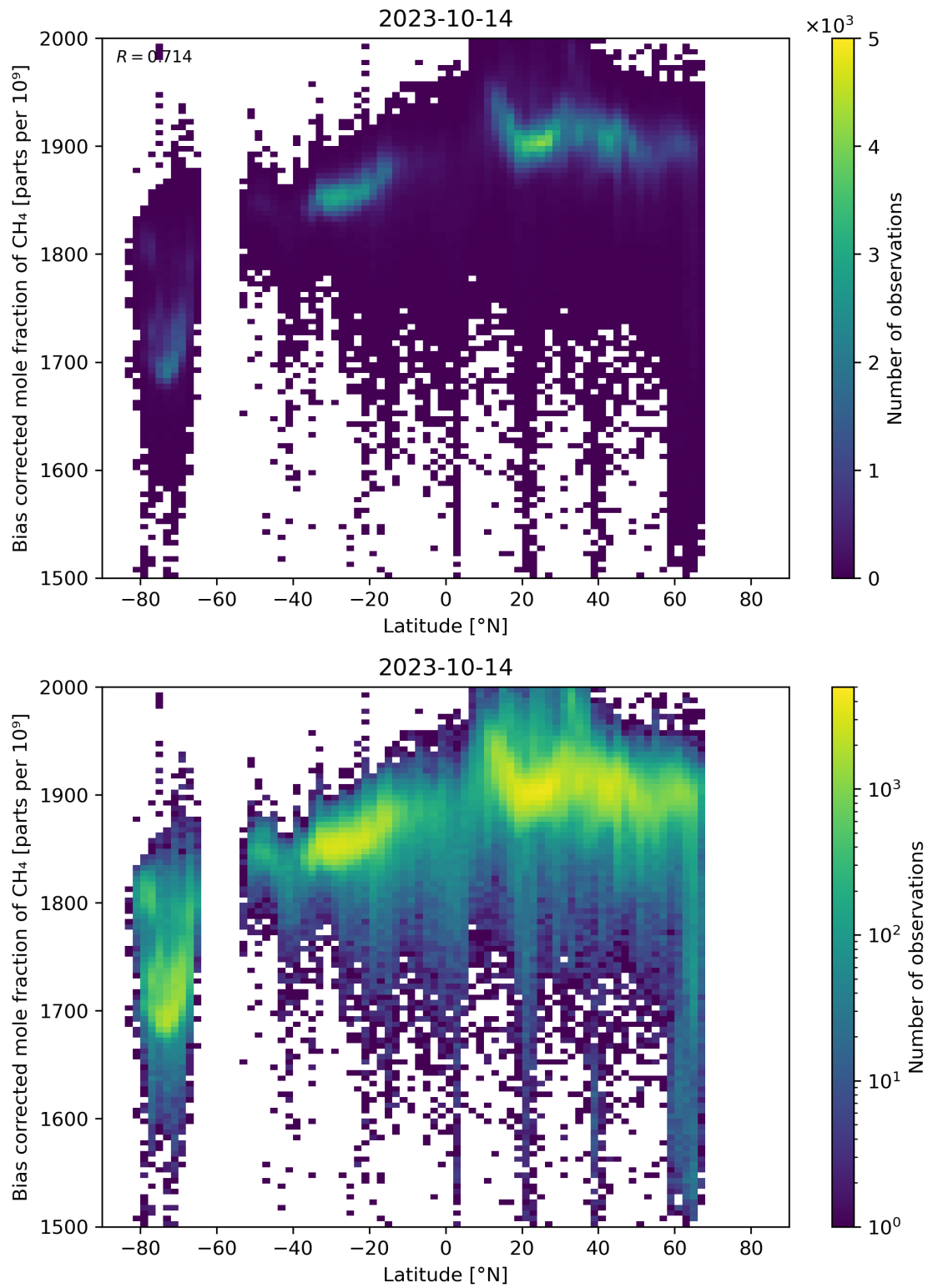
Figure 58: Scatter density plot of “Latitude” against “Bias corrected mole fraction of CH 4 ” for 2023-10-13 to 2023-10-15.
