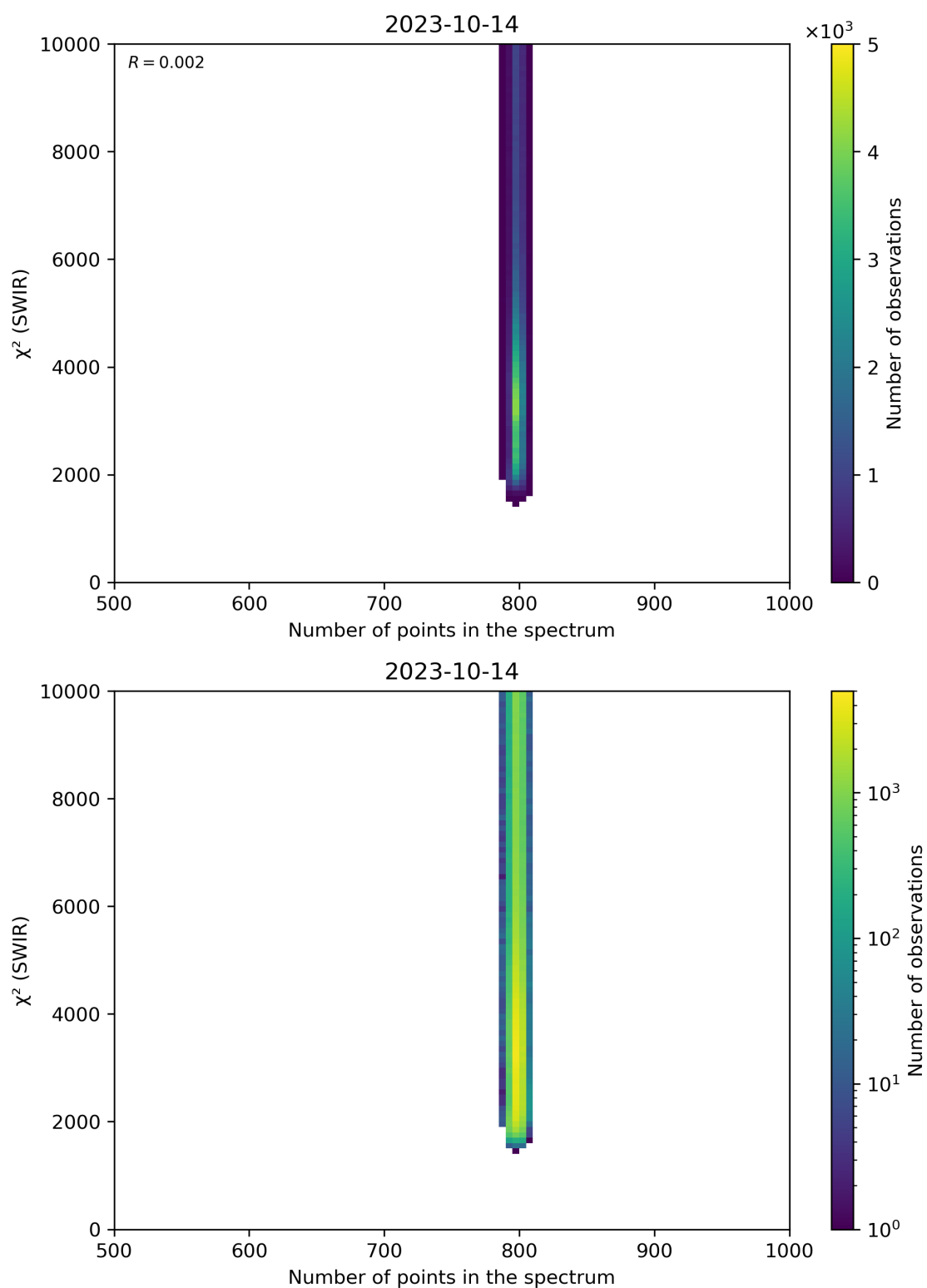
Figure 89: Scatter density plot of “Number of points in the spectrum” against “ \chi^2 (SWIR)” for 2023-10-13 to 2023-10-15.
