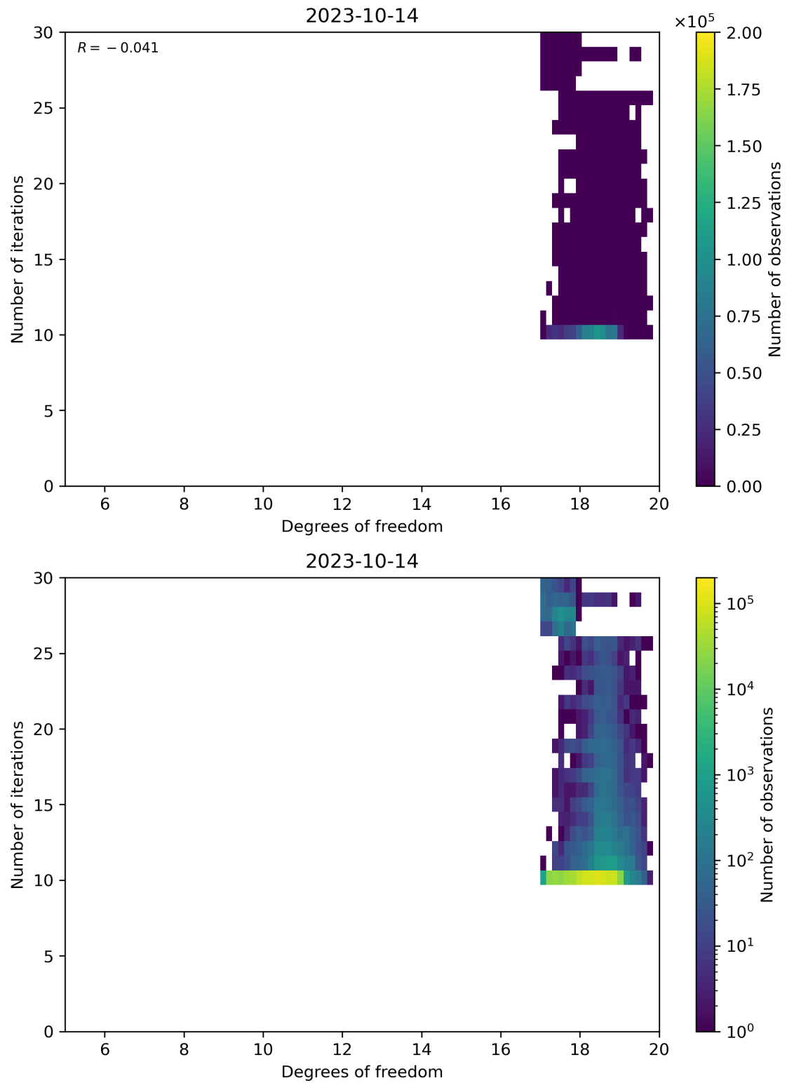
Figure 52: Scatter density plot of “Degrees of freedom” against “Number of iterations” for 2023-10-13 to 2023-10-15.
