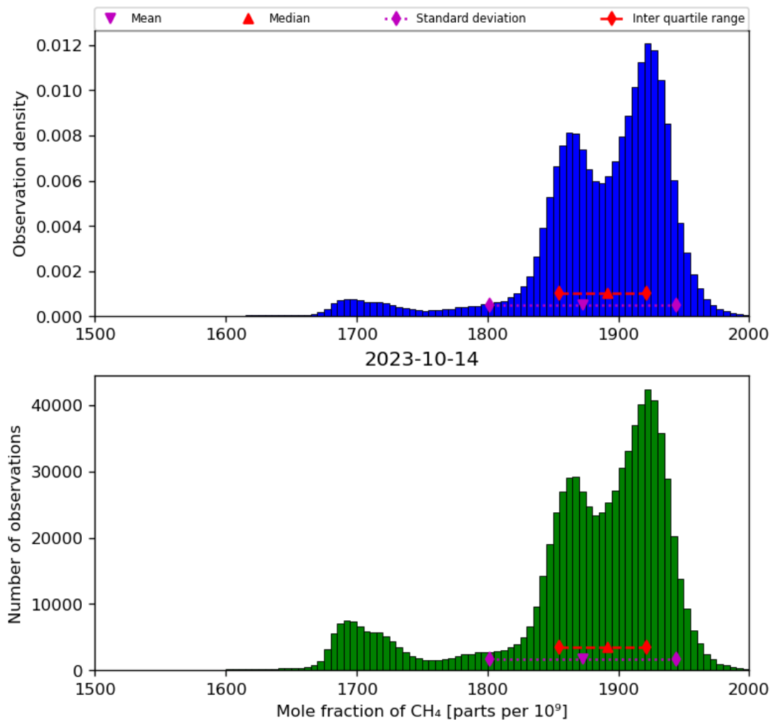
Figure 23: Histogram of “Mole fraction of CH 4 ” for 2023-10-13 to 2023-10-15
