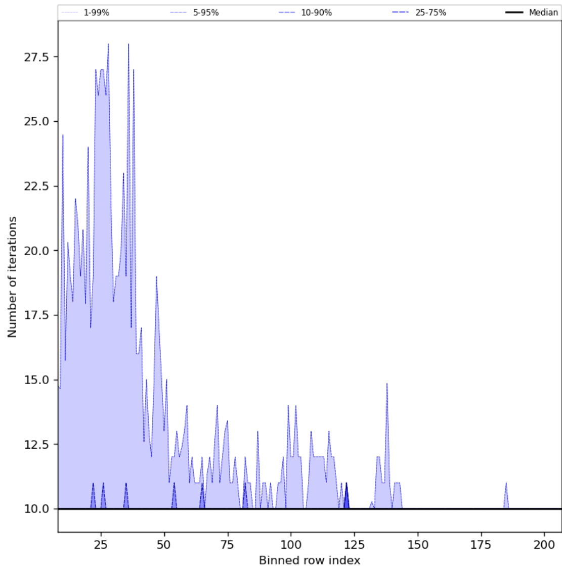
Figure 42: Along track statistics of “Number of iterations” for 2023-10-13 to 2023-10-15
