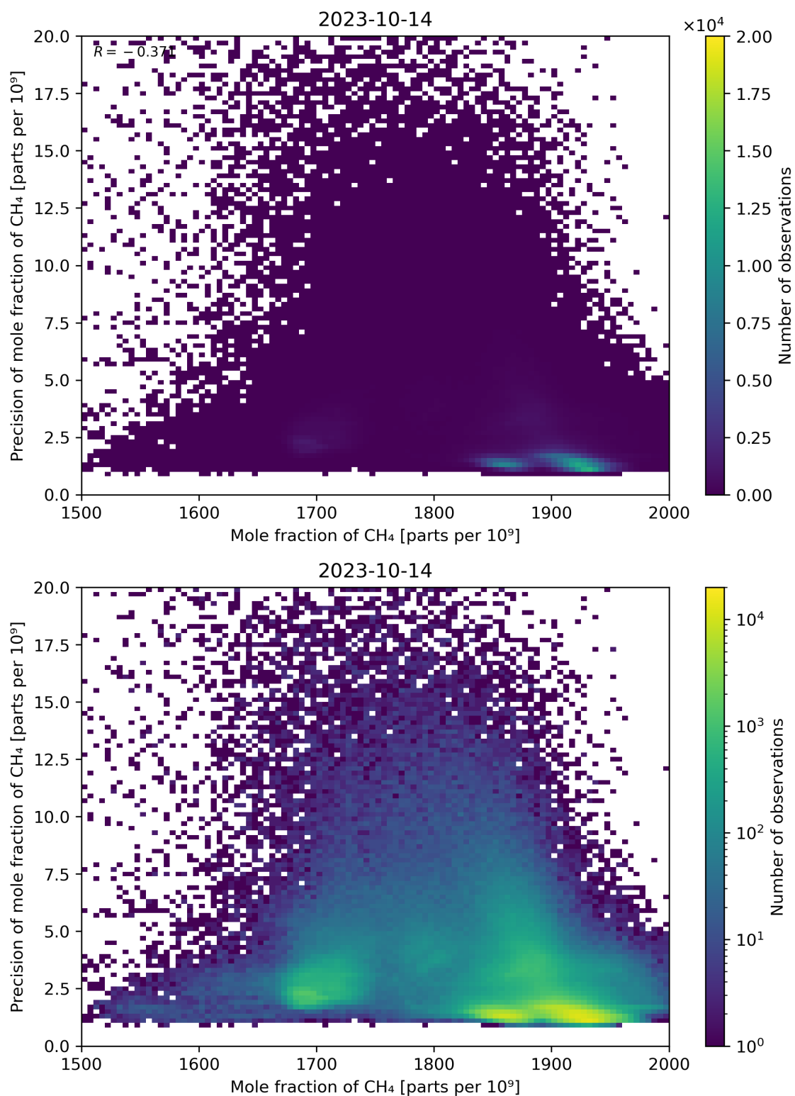
Figure 75: Scatter density plot of “Mole fraction of CH 4 ” against “Precision of mole fraction of CH 4 ” for 2023-10-13 to 2023-10-15.
