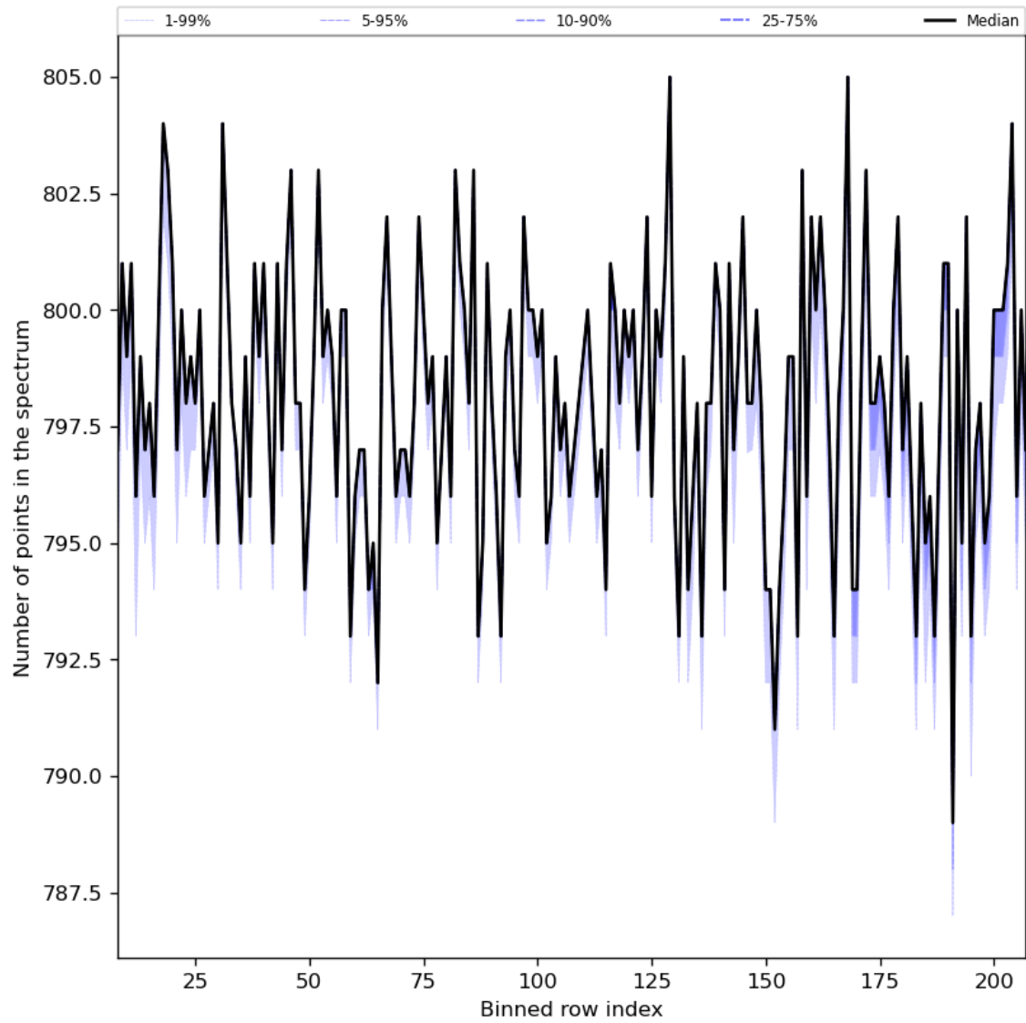
Figure 37: Along track statistics of “Number of points in the spectrum” for 2023-10-13 to 2023-10-15
