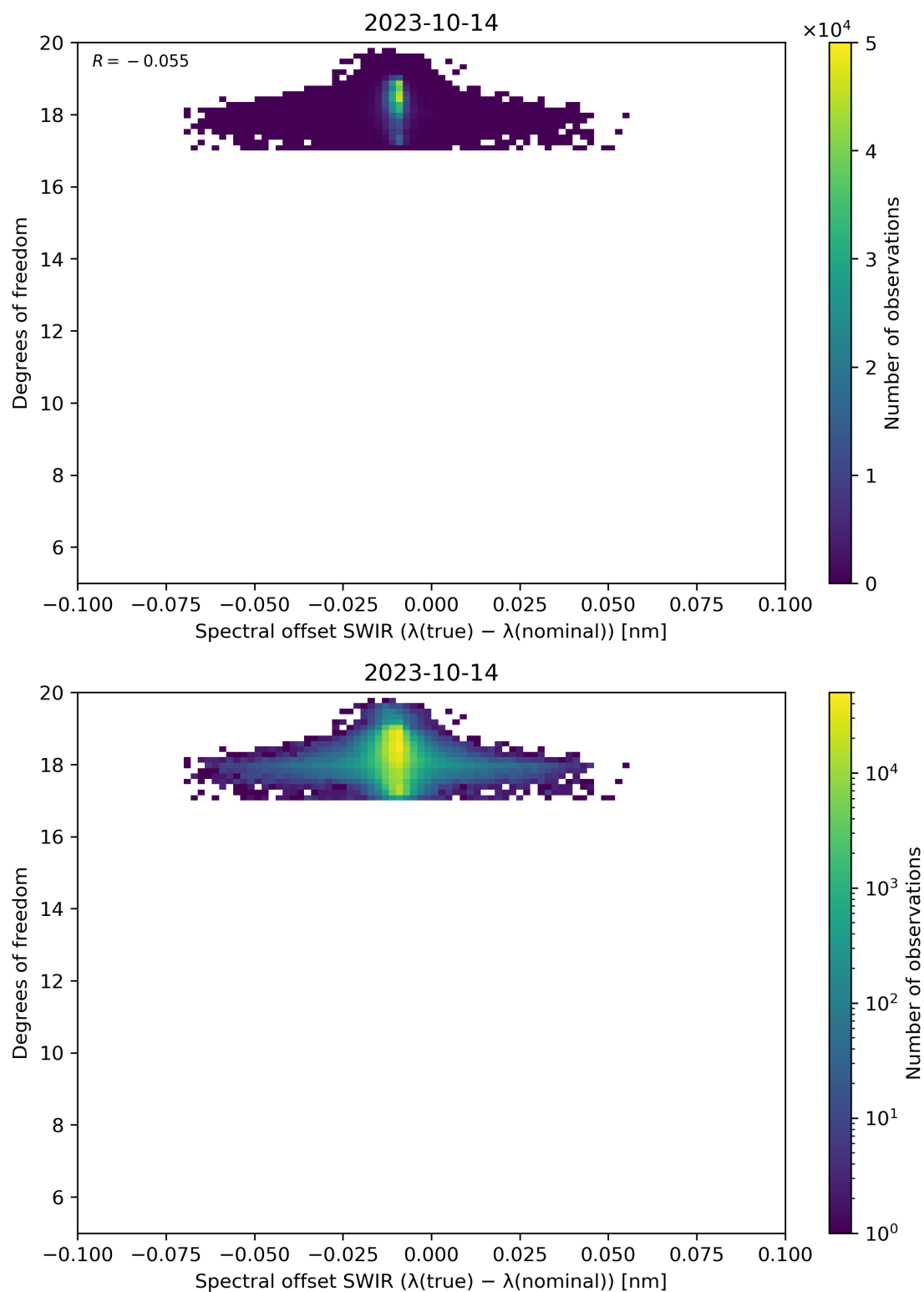
Figure 119: Scatter density plot of “Spectral offset SWIR ( \lambda(\text{true}) - \lambda(\text{nominal}) )” against “Degrees of freedom” for 2023-10-13 to 2023-10-15.
