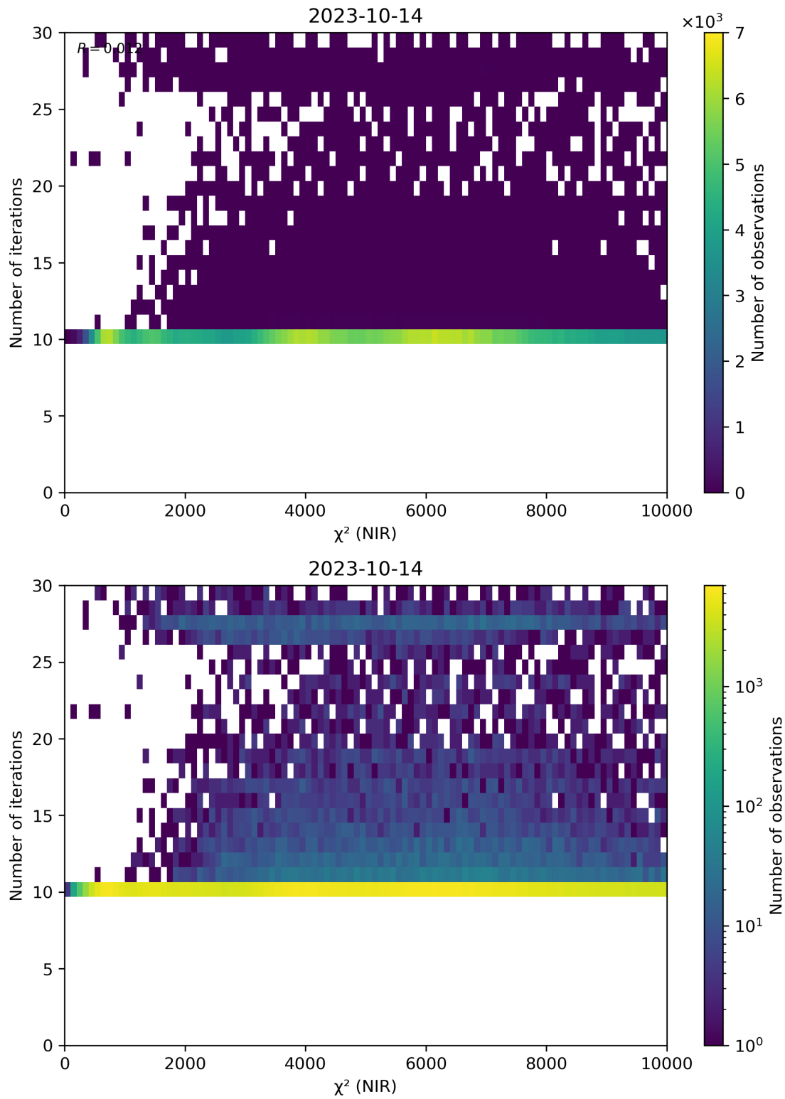
Figure 46: Scatter density plot of “ \chi^2 (NIR)” against “Number of iterations” for 2023-10-13 to 2023-10-15.
