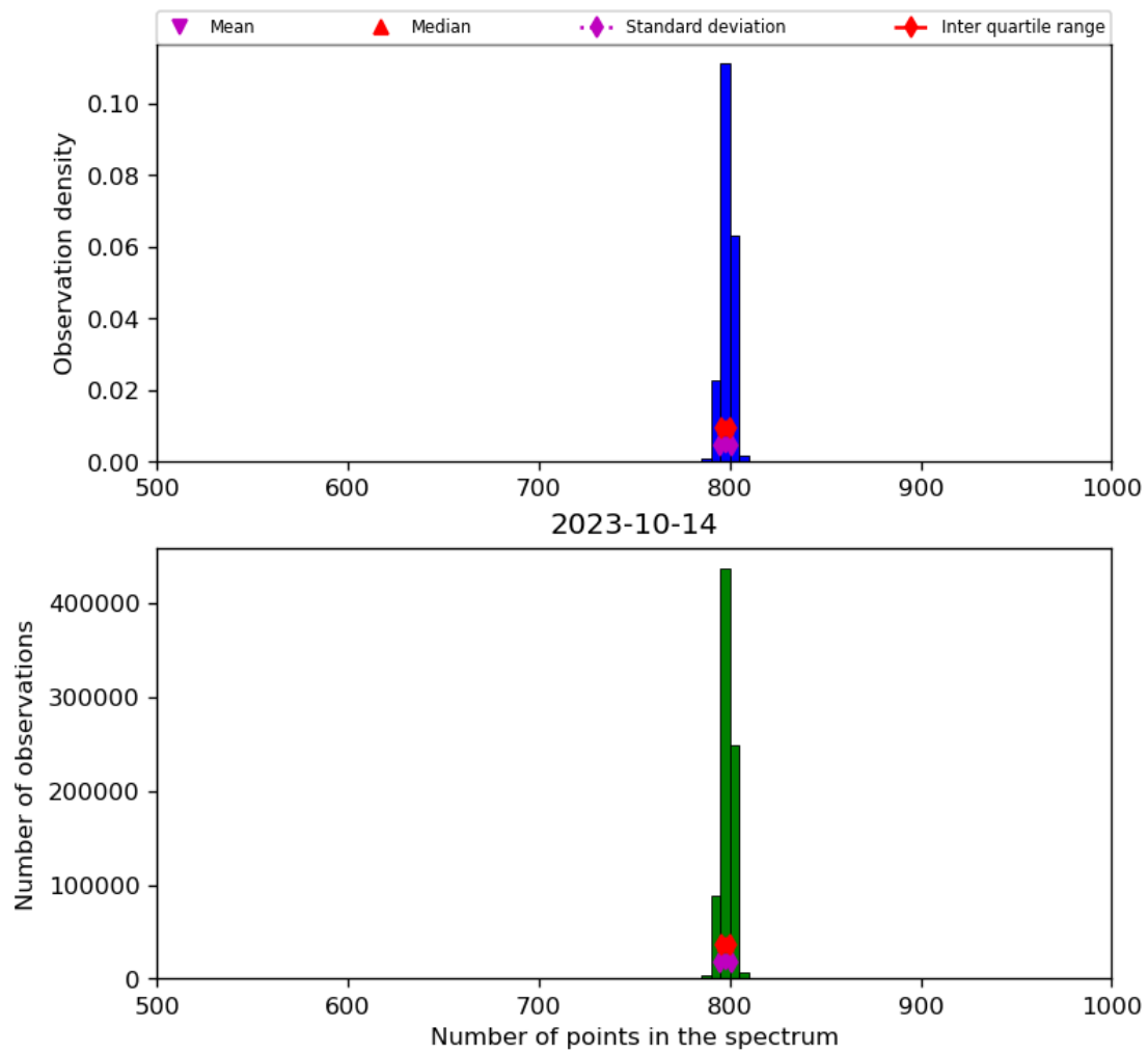
Figure 26: Histogram of “Number of points in the spectrum” for 2023-10-13 to 2023-10-15
