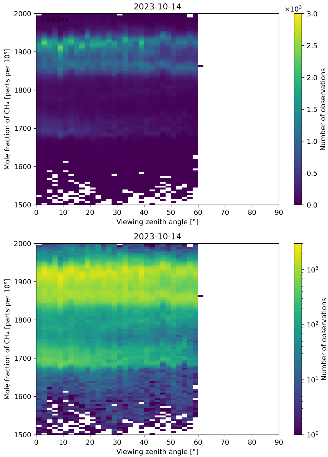
Figure 110: Scatter density plot of “Viewing zenith angle” against “Mole fraction of CH 4 ” for 2023-10-13 to 2023-10-15.
