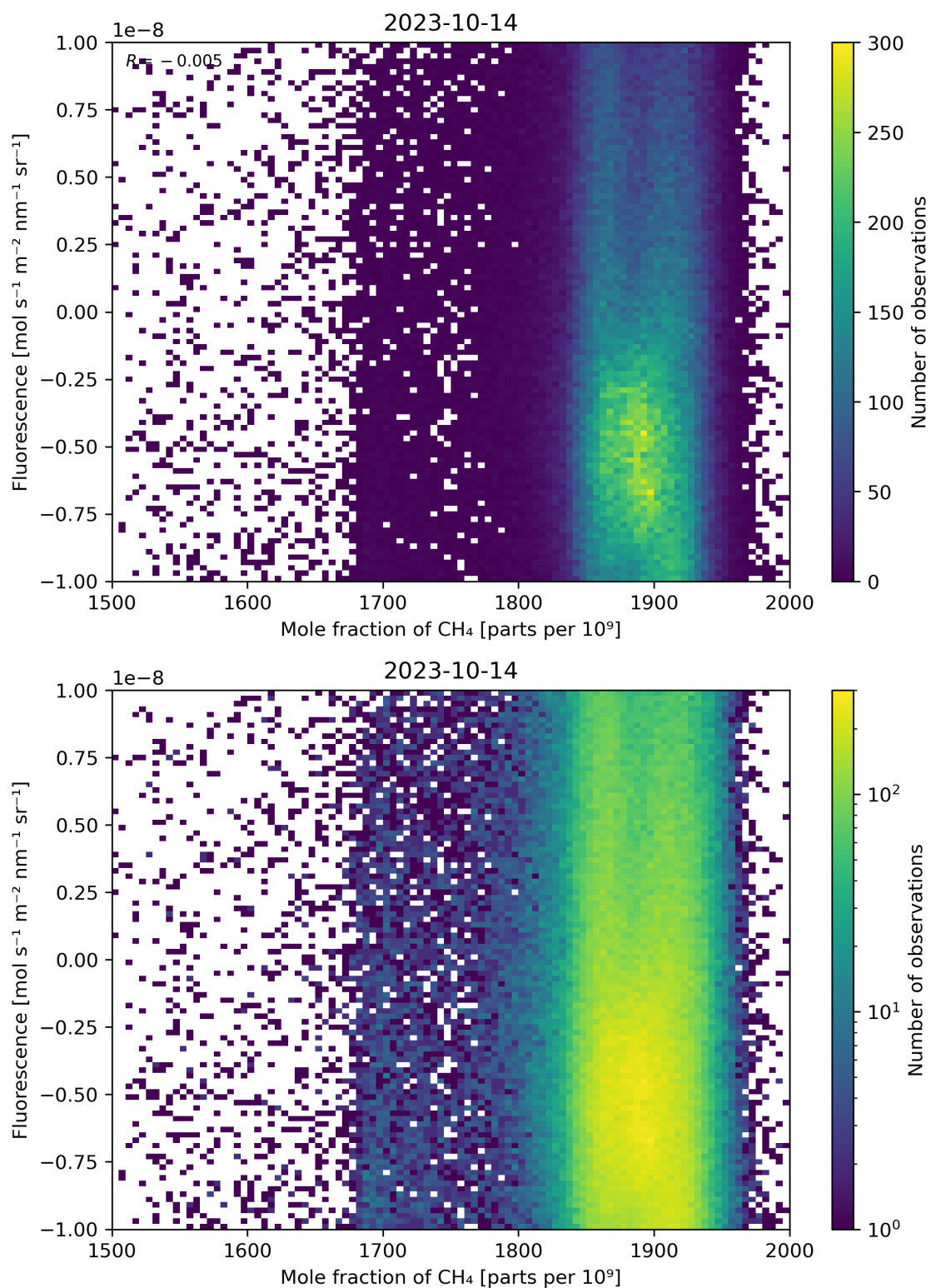
Figure 73: Scatter density plot of “Mole fraction of \text{CH}_4 ” against “Fluorescence” for 2023-10-13 to 2023-10-15.
