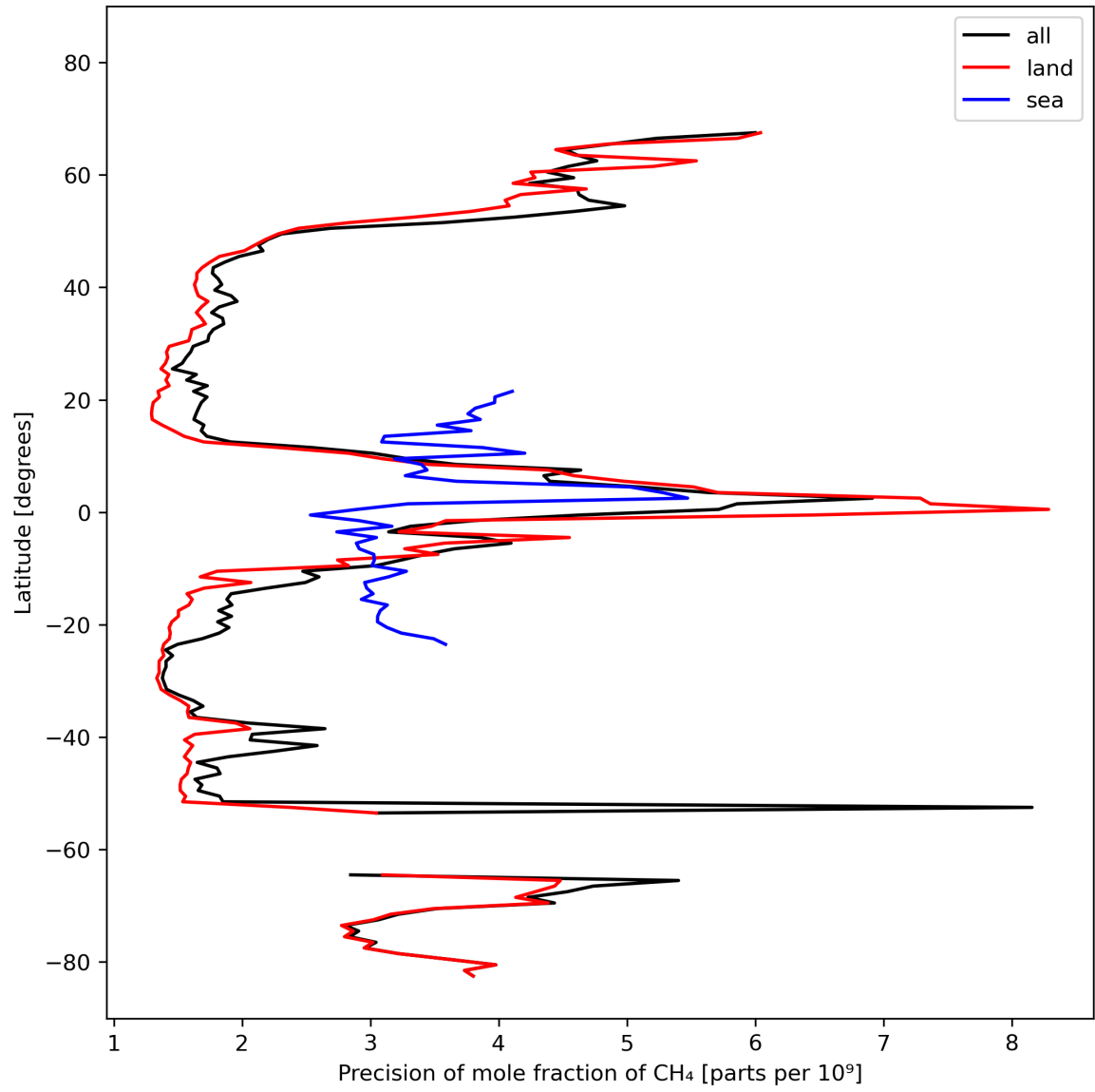
Figure 13: Zonal average of “Precision of mole fraction of CH 4 ” for 2023-10-13 to 2023-10-15.
