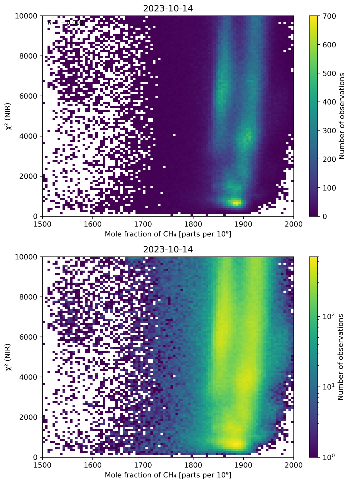
Figure 70: Scatter density plot of “Mole fraction of CH 4 ” against “ \chi^2 (NIR)” for 2023-10-13 to 2023-10-15.
