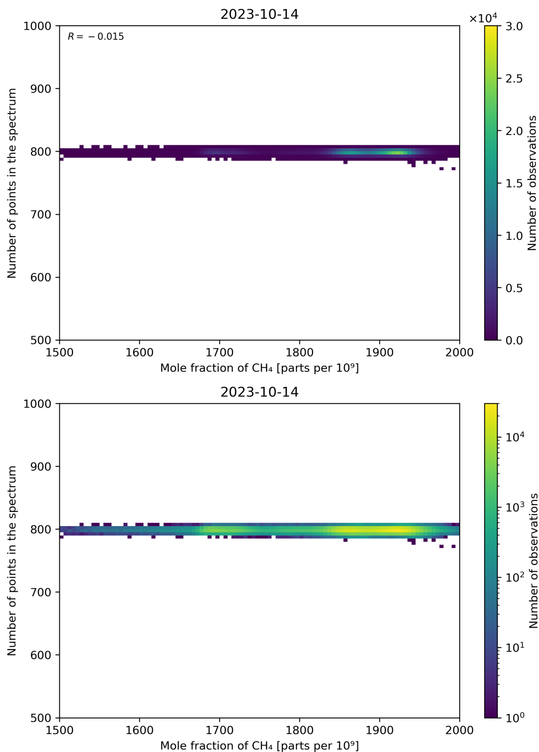
Figure 77: Scatter density plot of “Mole fraction of CH 4 ” against “Number of points in the spectrum” for 2023-10-13 to 2023-10-15.
