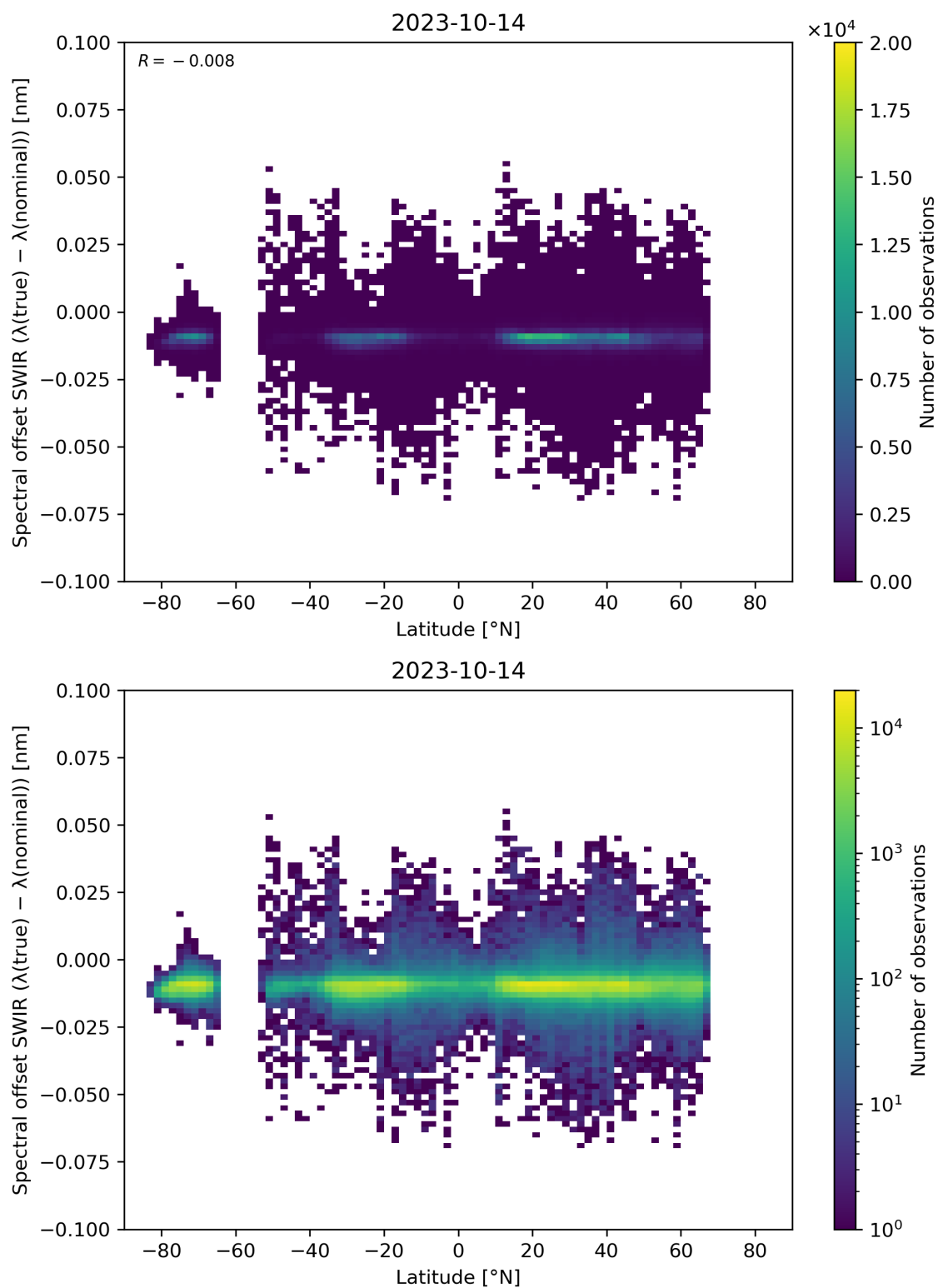
Figure 62: Scatter density plot of “Latitude” against “Spectral offset SWIR ( \lambda(\text{true}) - \lambda(\text{nominal}) )” for 2023-10-13 to 2023-10-15.
