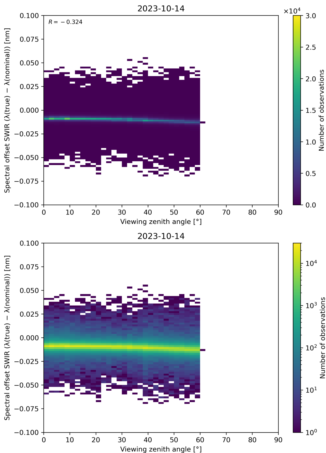
Figure 116: Scatter density plot of “Viewing zenith angle” against “Spectral offset SWIR ( \lambda(\text{true}) - \lambda(\text{nominal}) )” for 2023-10-13 to 2023-10-15.
