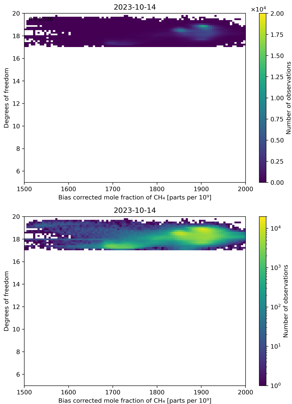
Figure 65: Scatter density plot of “Bias corrected mole fraction of CH 4 ” against “Degrees of freedom” for 2023-10-13 to 2023-10-15.
