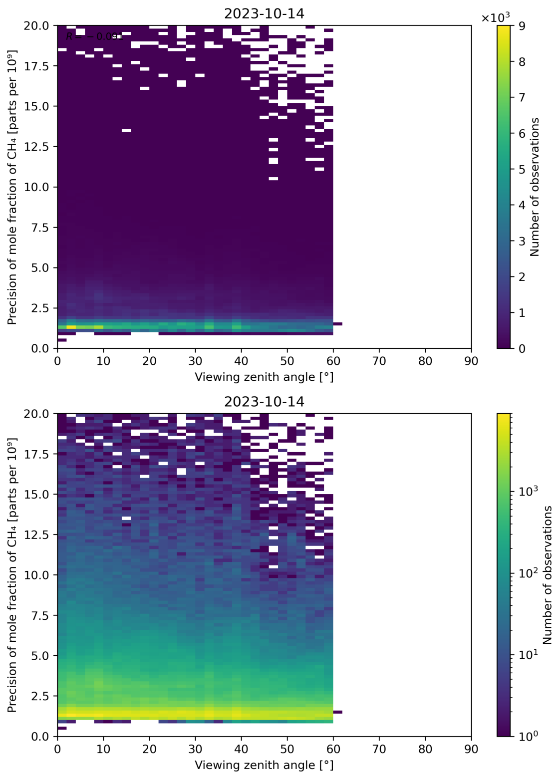
Figure 112: Scatter density plot of “Viewing zenith angle” against “Precision of mole fraction of CH 4 ” for 2023-10-13 to 2023-10-15.
