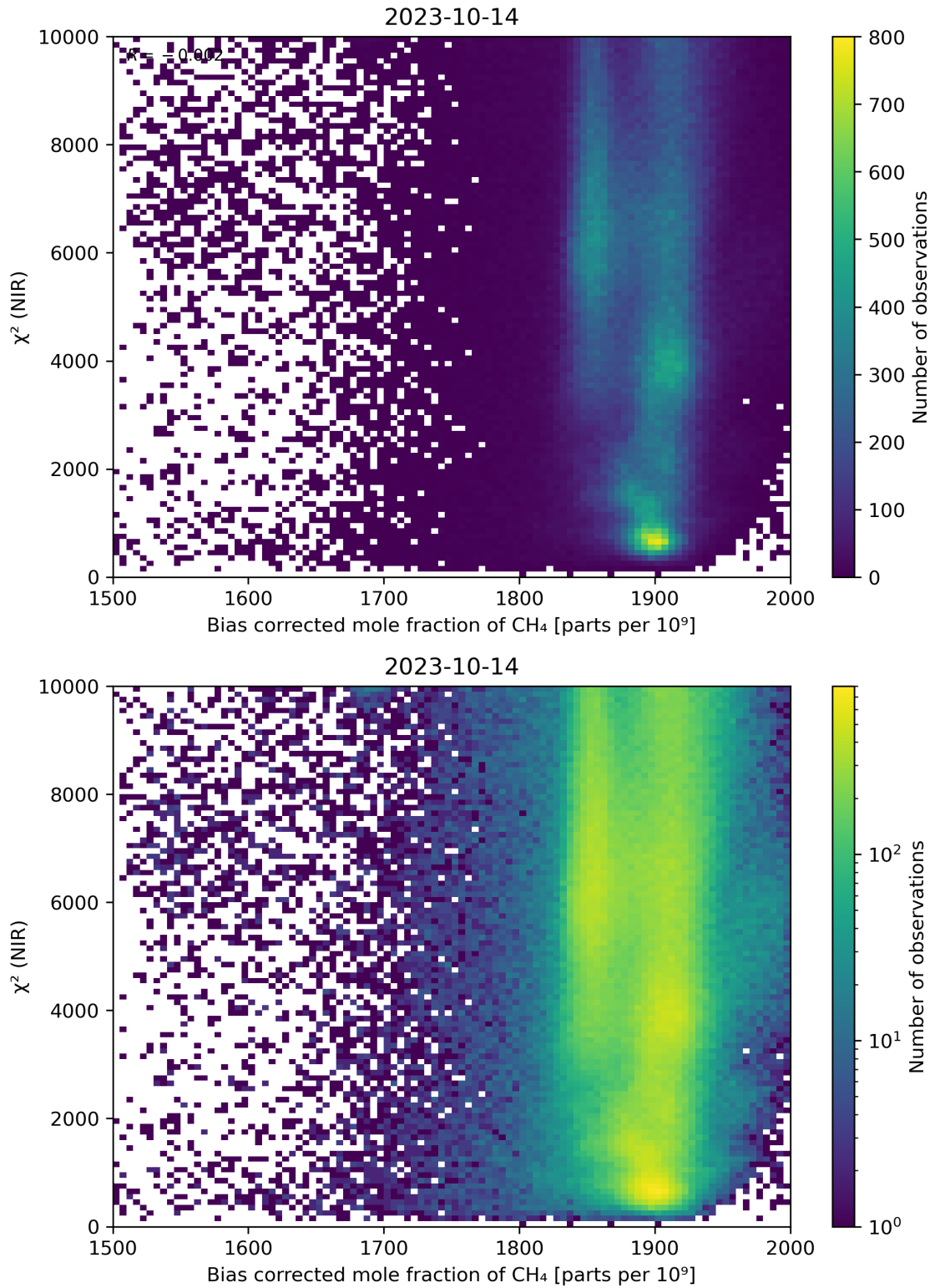
Figure 63: Scatter density plot of “Bias corrected mole fraction of \text{CH}_4 ” against “ \chi^2 (NIR)” for 2023-10-13 to 2023-10-15.
