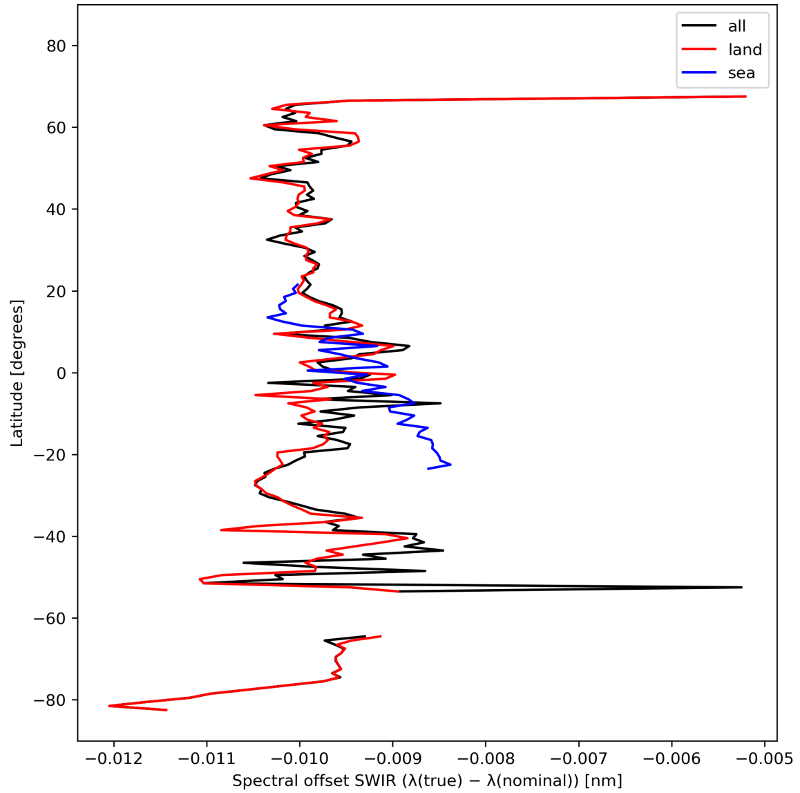
Figure 16: Zonal average of “Spectral offset SWIR ( \lambda(\text{true}) - \lambda(\text{nominal}) )” for 2023-10-13 to 2023-10-15.
