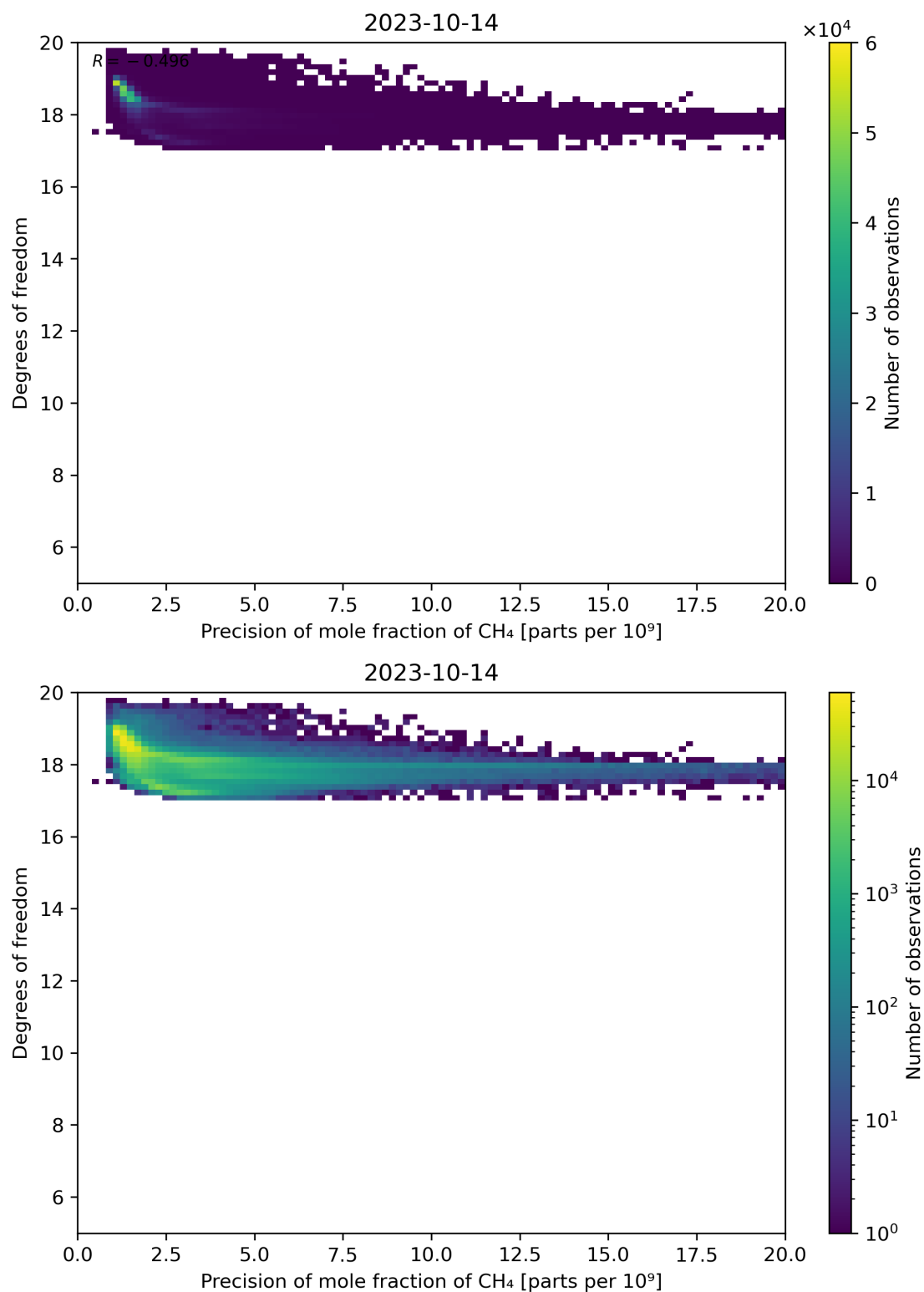
Figure 80: Scatter density plot of “Precision of mole fraction of CH 4 ” against “Degrees of freedom” for 2023-10-13 to 2023-10-15.
