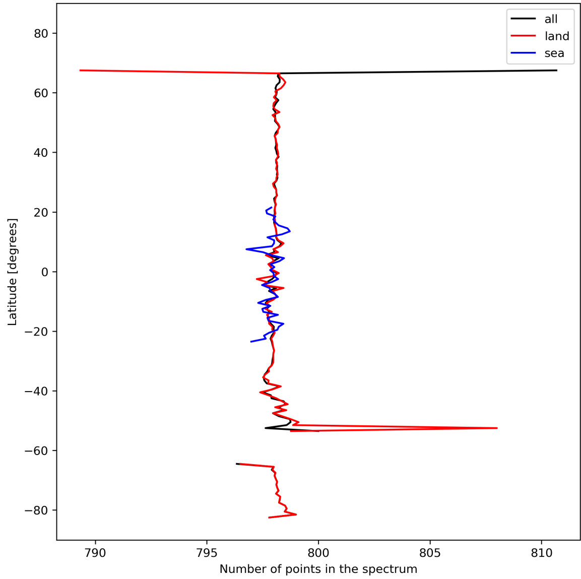
Figure 15: Zonal average of “Number of points in the spectrum” for 2023-10-13 to 2023-10-15.
