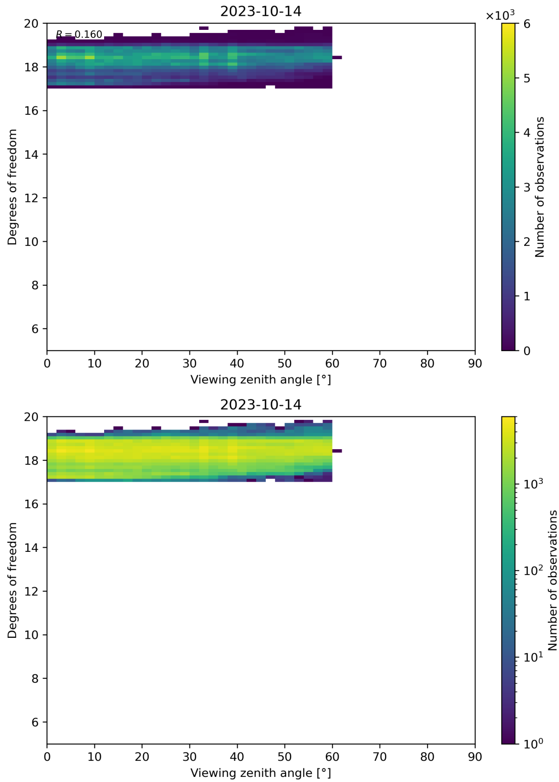
Figure 107: Scatter density plot of “Viewing zenith angle” against “Degrees of freedom” for 2023-10-13 to 2023-10-15.
