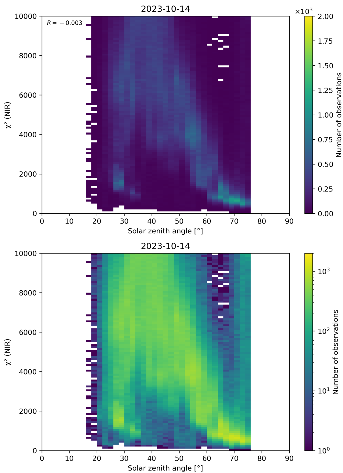
Figure 94: Scatter density plot of “Solar zenith angle” against “ \chi^2 (NIR)” for 2023-10-13 to 2023-10-15.
