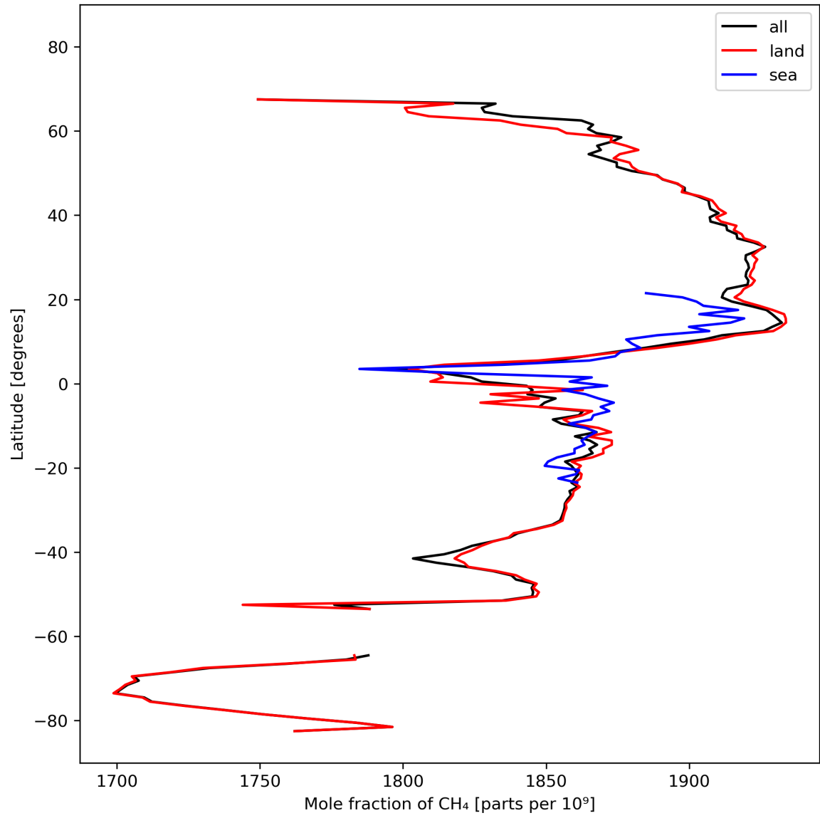
Figure 12: Zonal average of “Mole fraction of \text{CH}_4 ” for 2023-10-13 to 2023-10-15.
