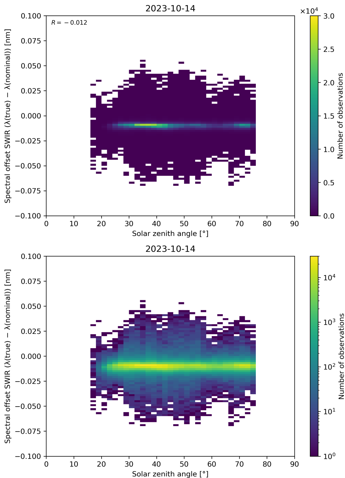
Figure 104: Scatter density plot of “Solar zenith angle” against “Spectral offset SWIR ( \lambda(\text{true}) - \lambda(\text{nominal}) )” for 2023-10-13 to 2023-10-15.
