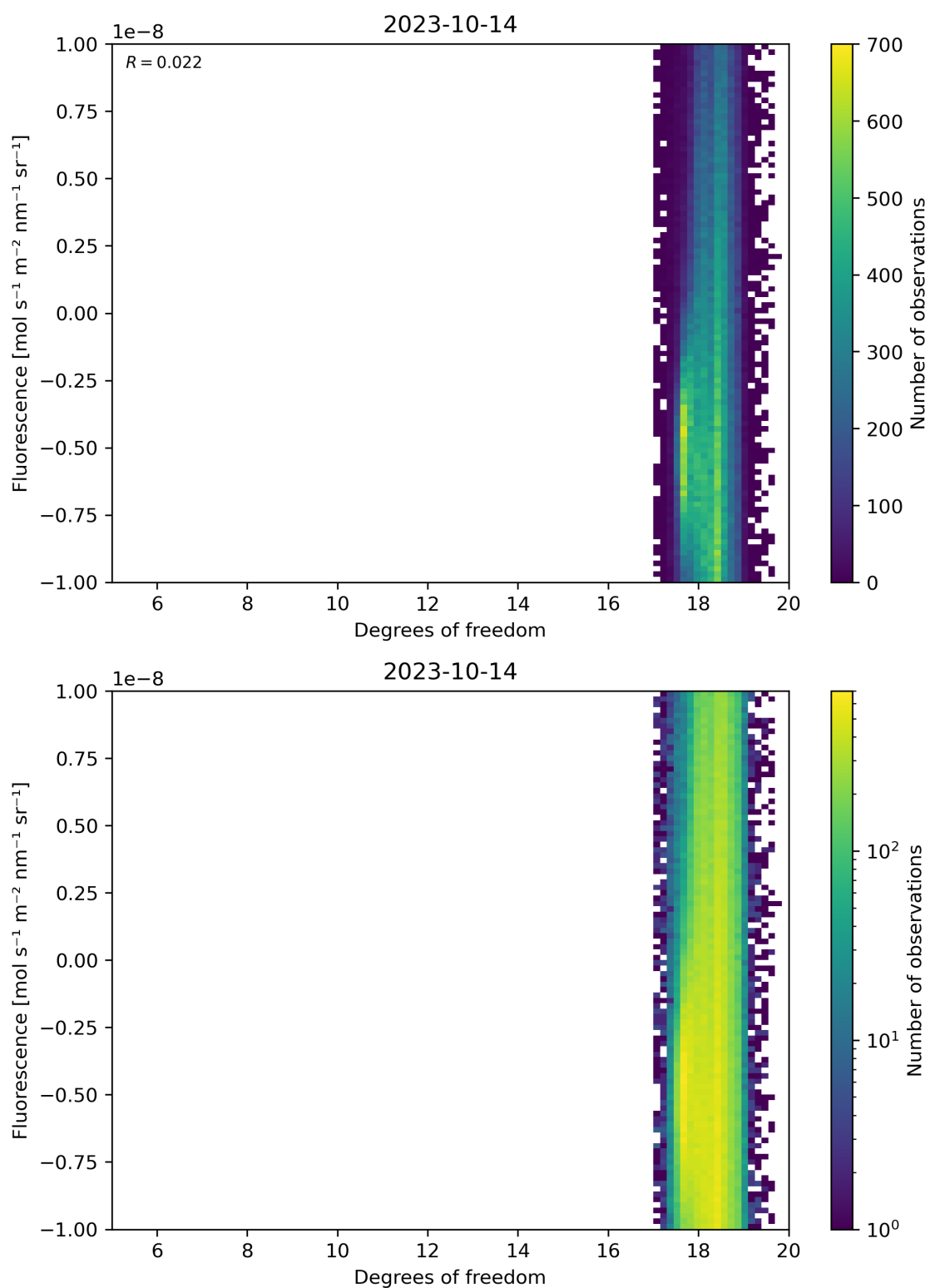
Figure 51: Scatter density plot of “Degrees of freedom” against “Fluorescence” for 2023-10-13 to 2023-10-15.
