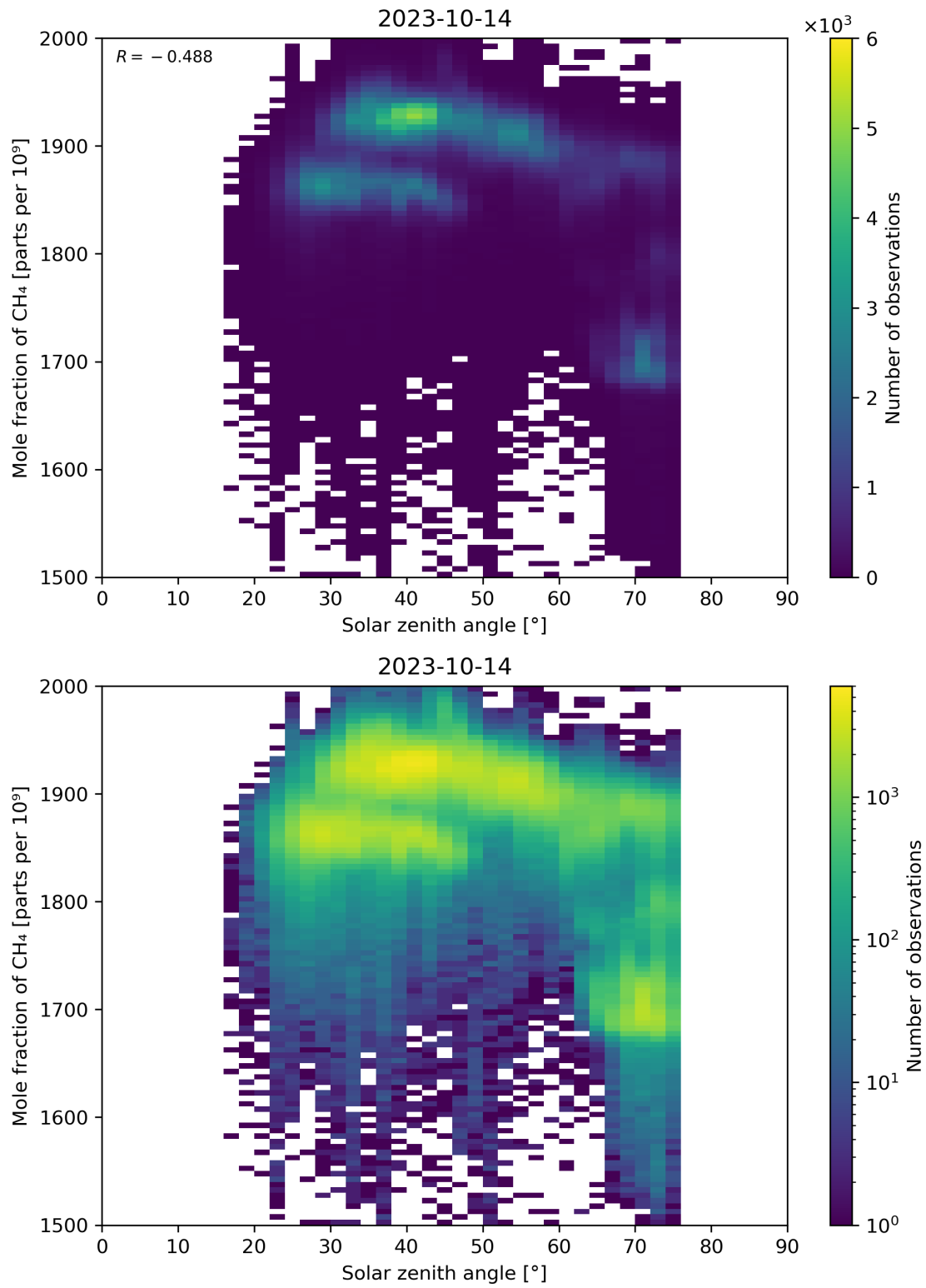
Figure 99: Scatter density plot of “Solar zenith angle” against “Mole fraction of CH 4 ” for 2023-10-13 to 2023-10-15.
