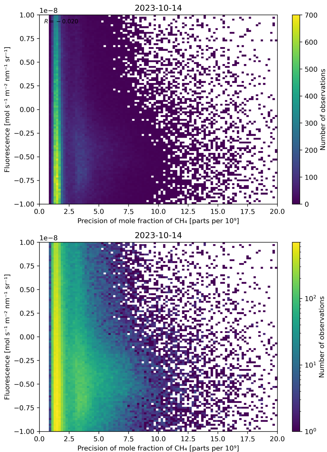
Figure 81: Scatter density plot of “Precision of mole fraction of CH 4 ” against “Fluorescence” for 2023-10-13 to 2023-10-15.
