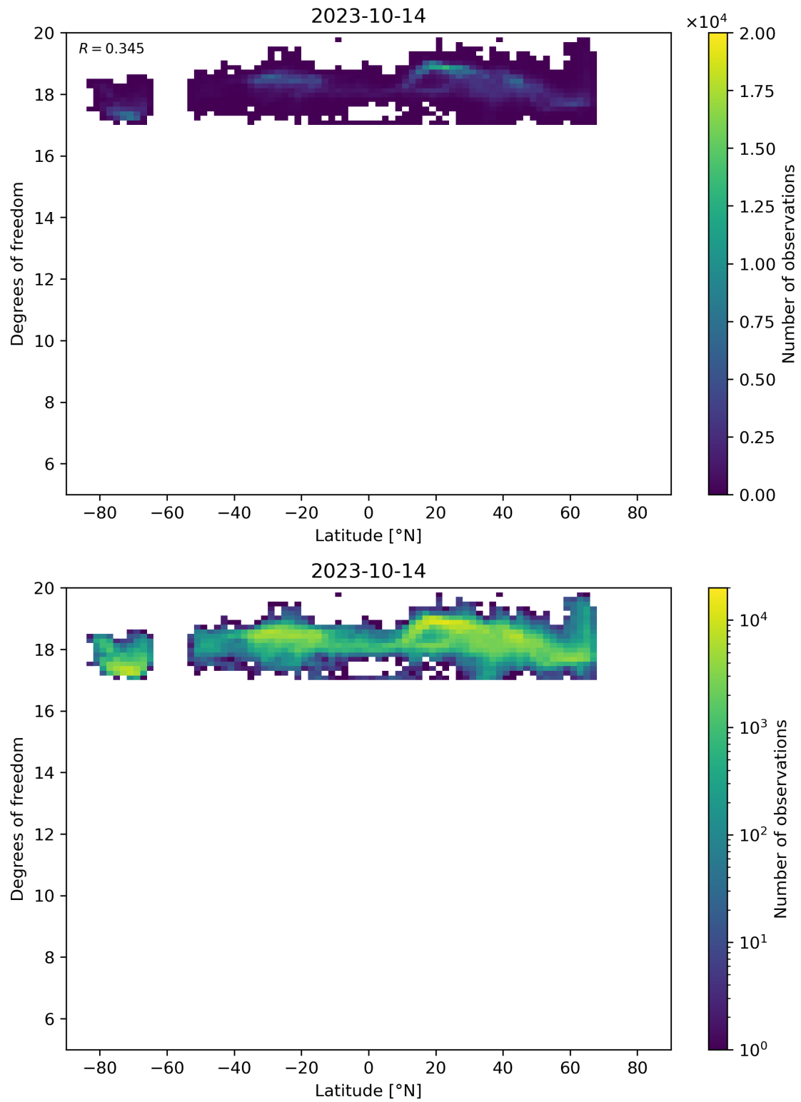
Figure 55: Scatter density plot of “Latitude” against “Degrees of freedom” for 2023-10-13 to 2023-10-15.
