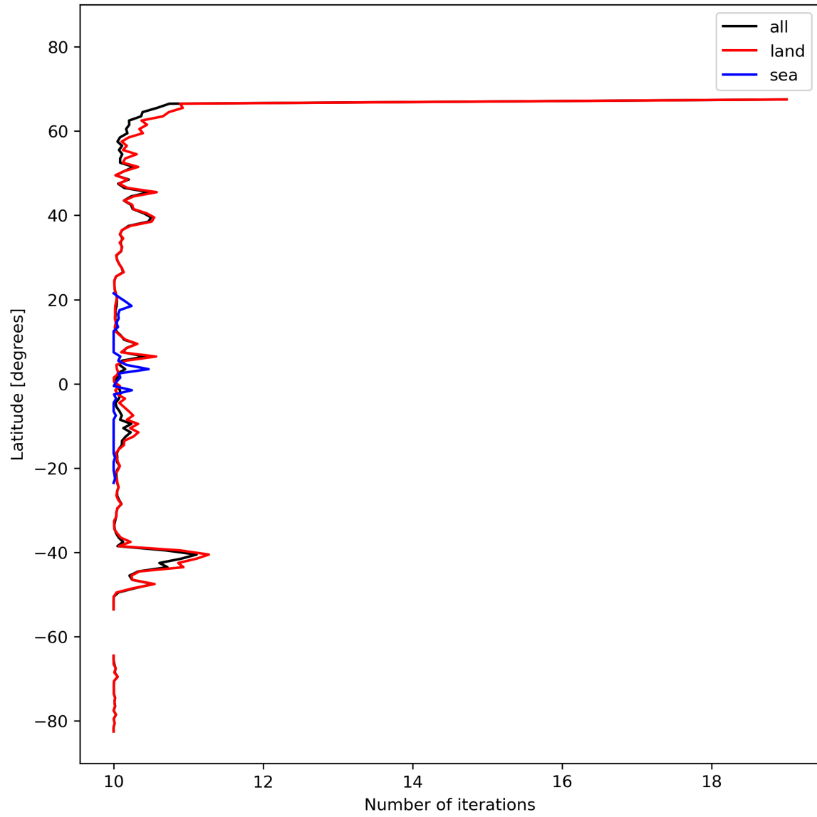
Figure 20: Zonal average of “Number of iterations” for 2023-10-13 to 2023-10-15.
