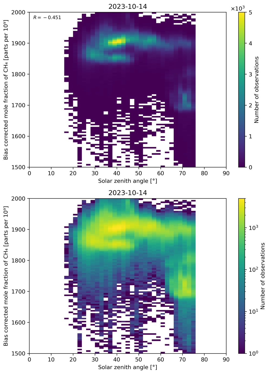
Figure 100: Scatter density plot of “Solar zenith angle” against “Bias corrected mole fraction of CH 4 ” for 2023-10-13 to 2023-10-15.
