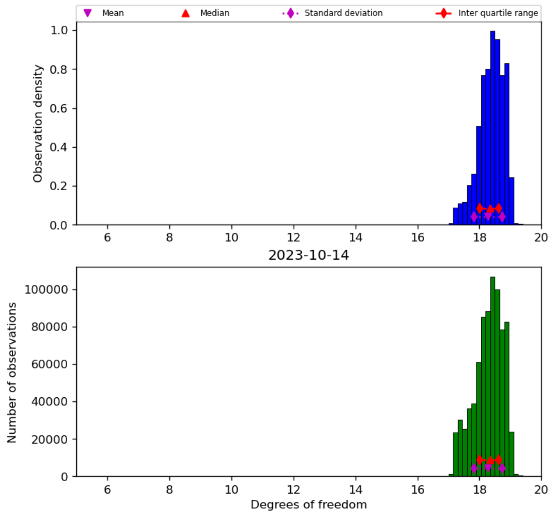
Figure 30: Histogram of “Degrees of freedom” for 2023-10-13 to 2023-10-15
