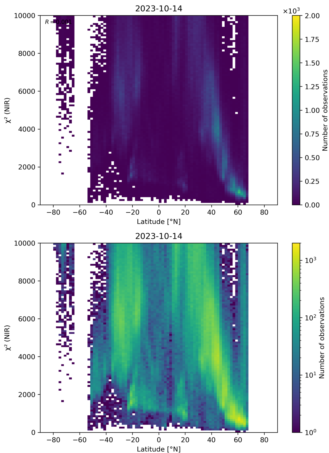
Figure 53: Scatter density plot of “Latitude” against “ \chi^2 (NIR)” for 2023-10-13 to 2023-10-15.
