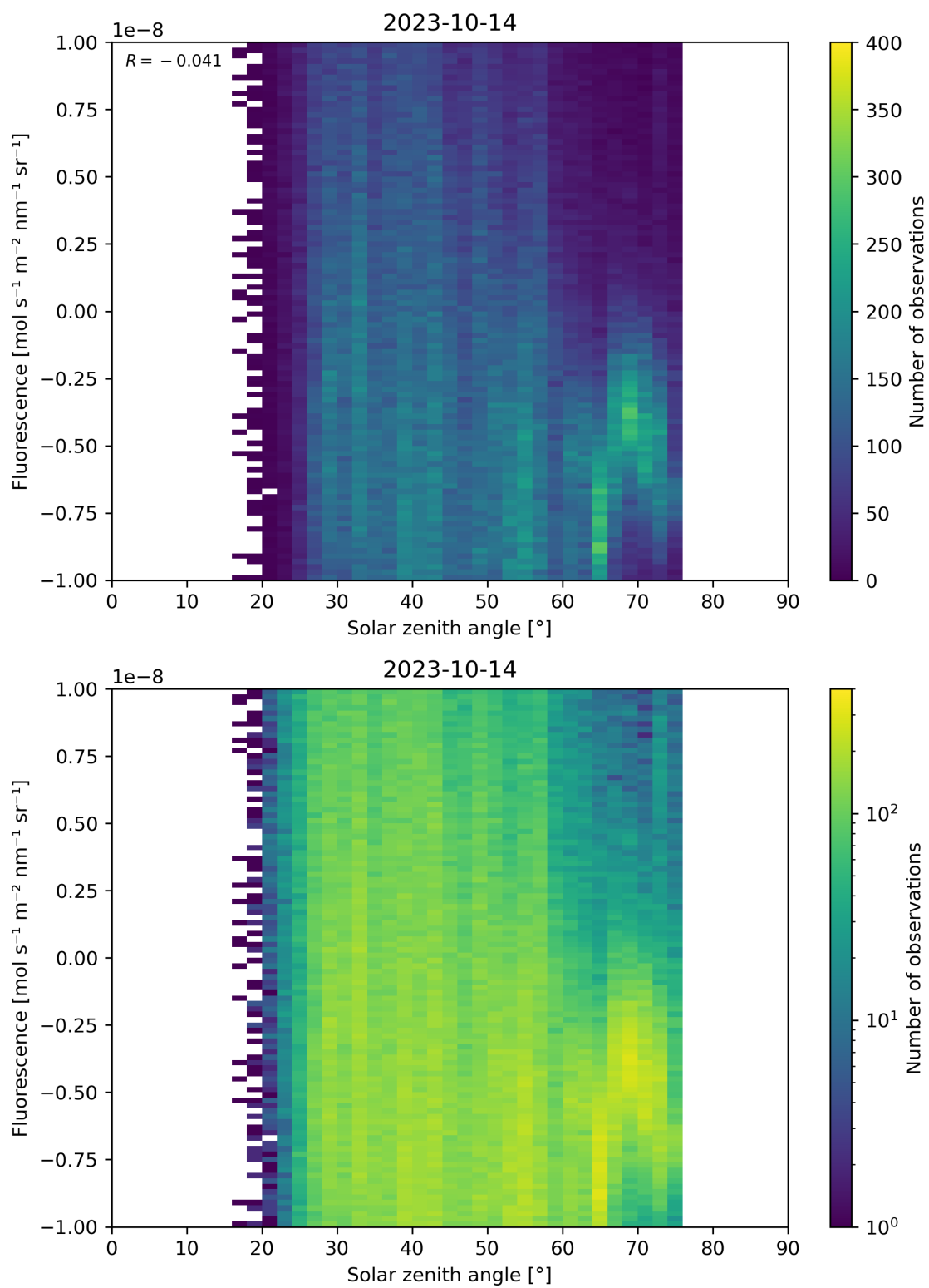
Figure 97: Scatter density plot of “Solar zenith angle” against “Fluorescence” for 2023-10-13 to 2023-10-15.
