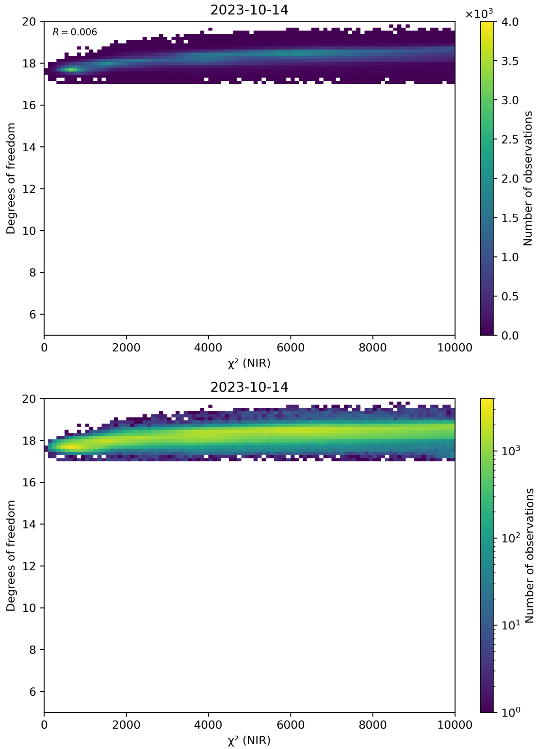
Figure 44: Scatter density plot of “ \chi^2 (NIR)” against “Degrees of freedom” for 2023-10-13 to 2023-10-15.
