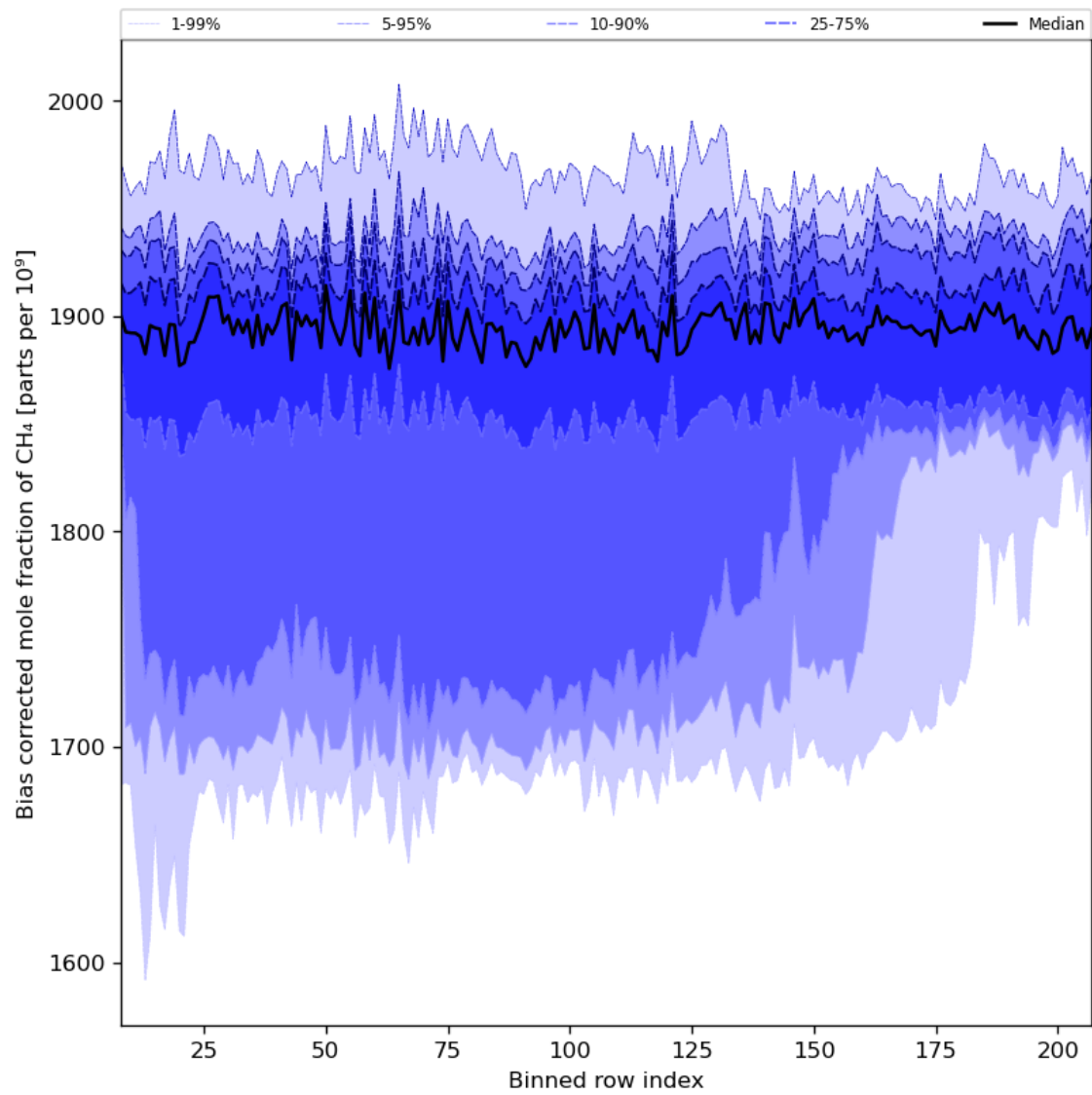
Figure 36: Along track statistics of “Bias corrected mole fraction of CH 4 ” for 2023-10-13 to 2023-10-15
