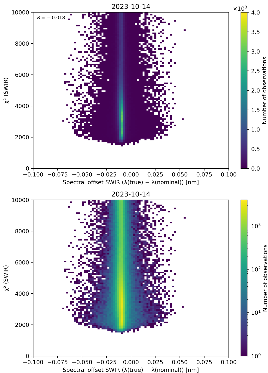
Figure 118: Scatter density plot of “Spectral offset SWIR ( \lambda(\text{true}) - \lambda(\text{nominal}) )” against “ \chi^2 (SWIR)” for 2023-10-13 to 2023-10-15.
