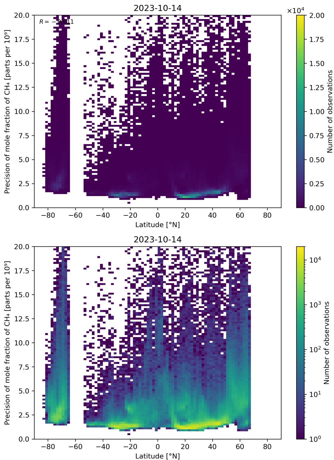
Figure 59: Scatter density plot of “Latitude” against “Precision of mole fraction of CH 4 ” for 2023-10-13 to 2023-10-15.
