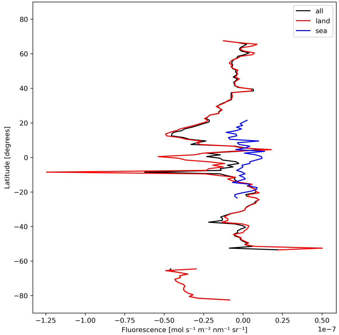
Figure 21: Zonal average of “Fluorescence” for 2023-10-13 to 2023-10-15.
