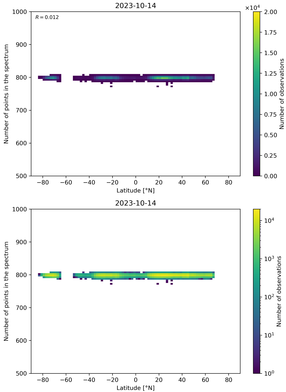
Figure 61: Scatter density plot of “Latitude” against “Number of points in the spectrum” for 2023-10-13 to 2023-10-15.
