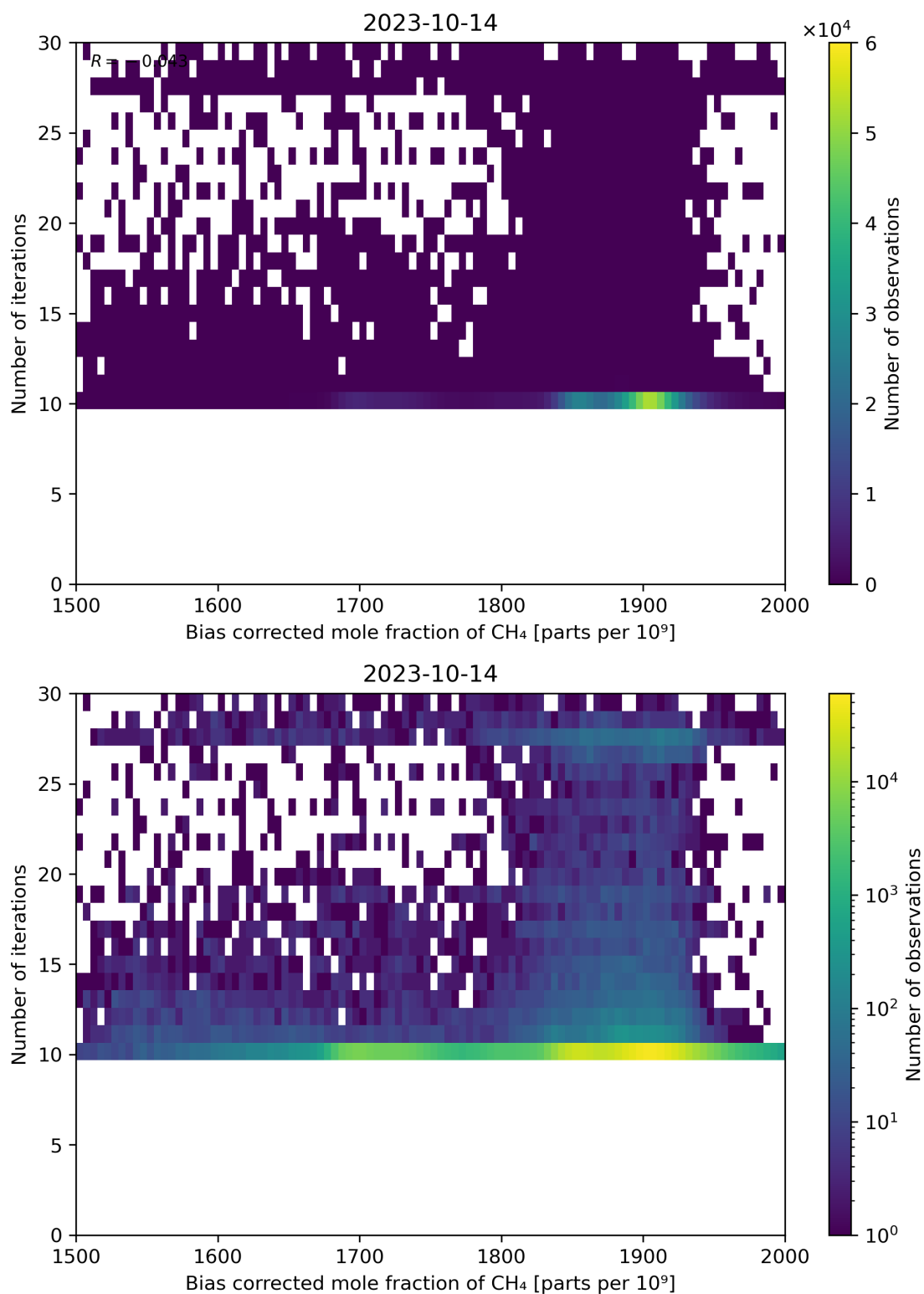
Figure 67: Scatter density plot of “Bias corrected mole fraction of \text{CH}_4 ” against “Number of iterations” for 2023-10-13 to 2023-10-15.
