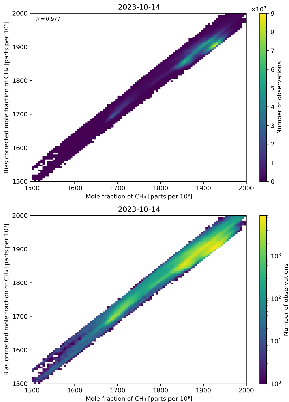
Figure 74: Scatter density plot of “Mole fraction of CH 4 ” against “Bias corrected mole fraction of CH 4 ” for 2023-10-13 to 2023-10-15.
