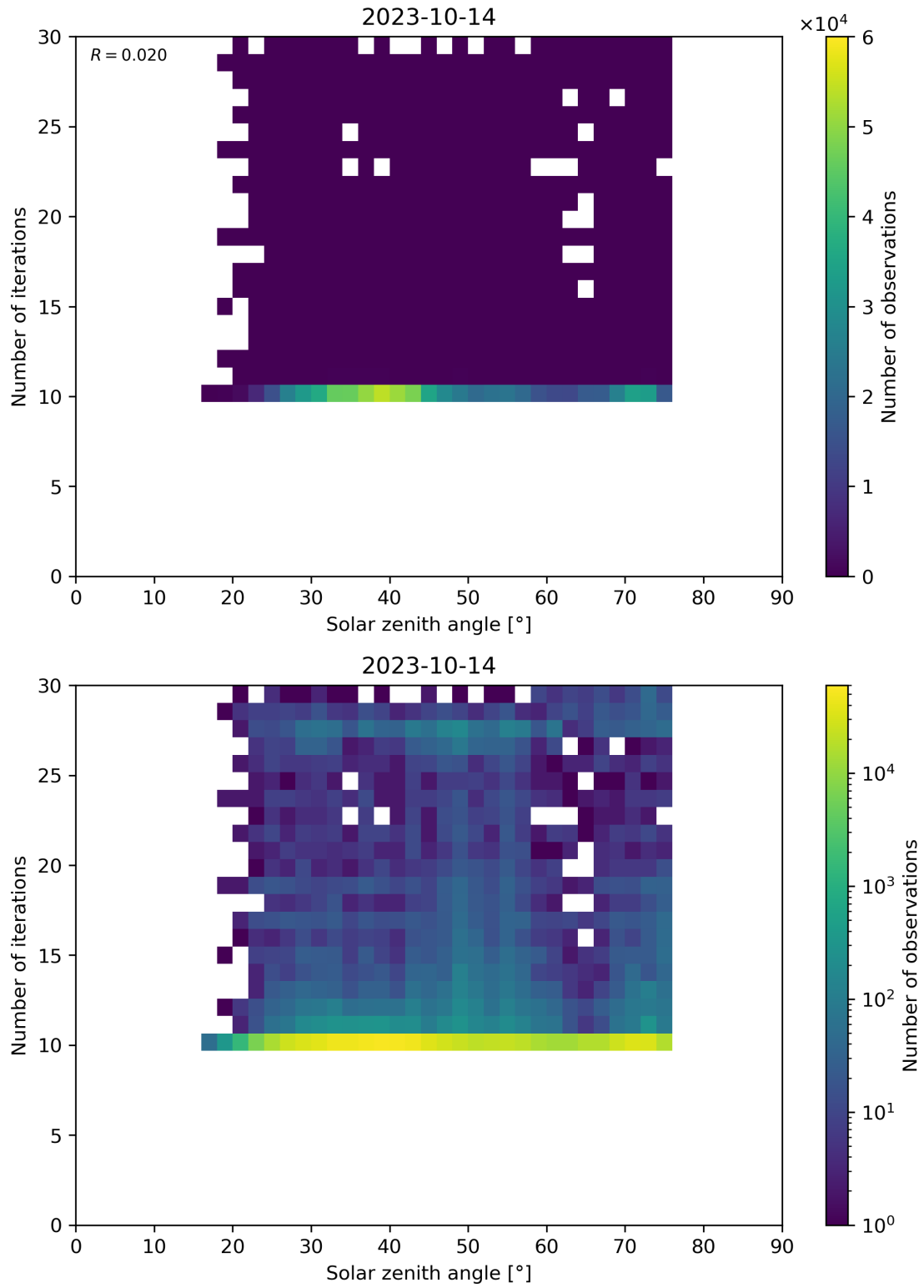
Figure 102: Scatter density plot of “Solar zenith angle” against “Number of iterations” for 2023-10-13 to 2023-10-15.
