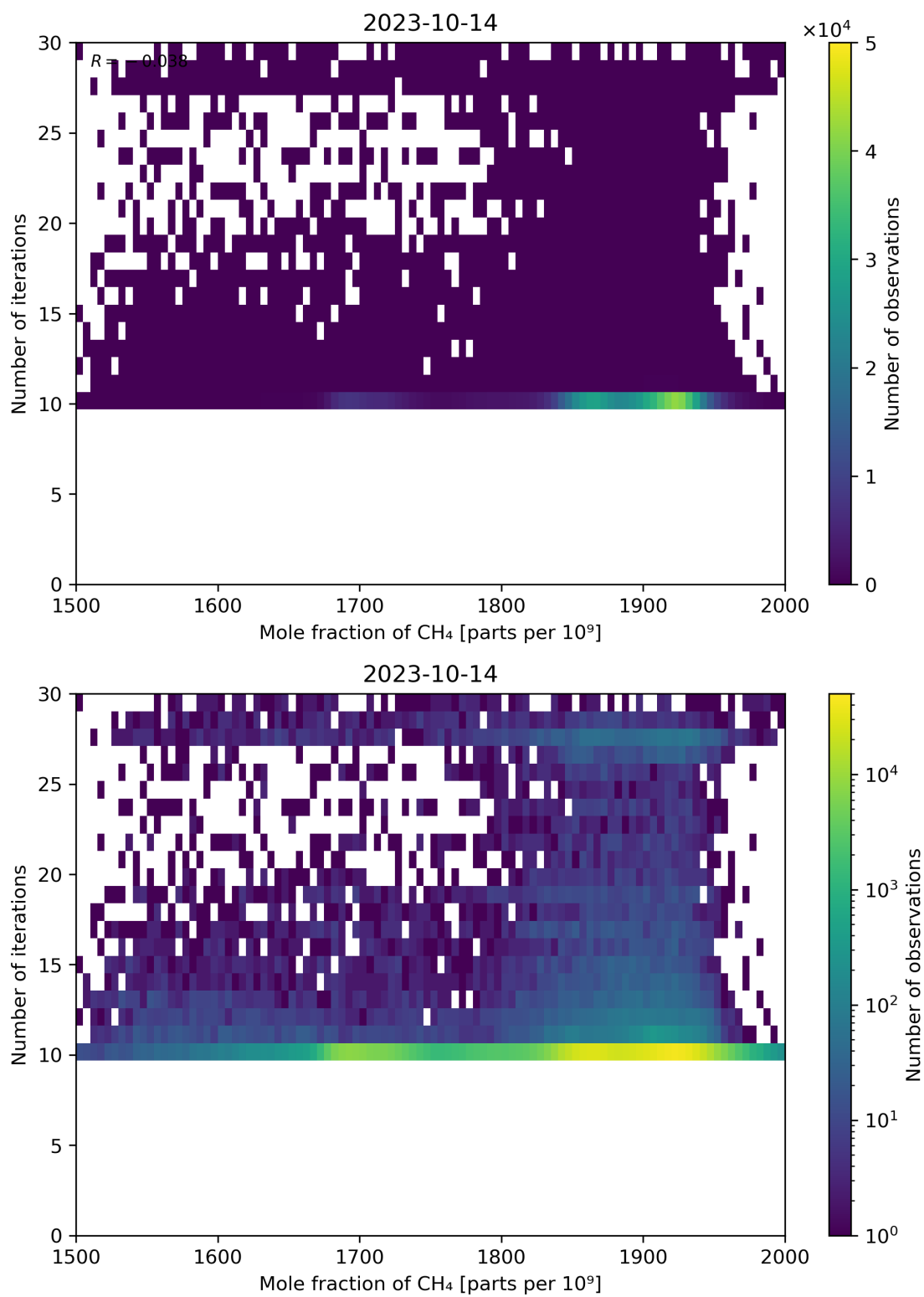
Figure 76: Scatter density plot of “Mole fraction of CH 4 ” against “Number of iterations” for 2023-10-13 to 2023-10-15.
