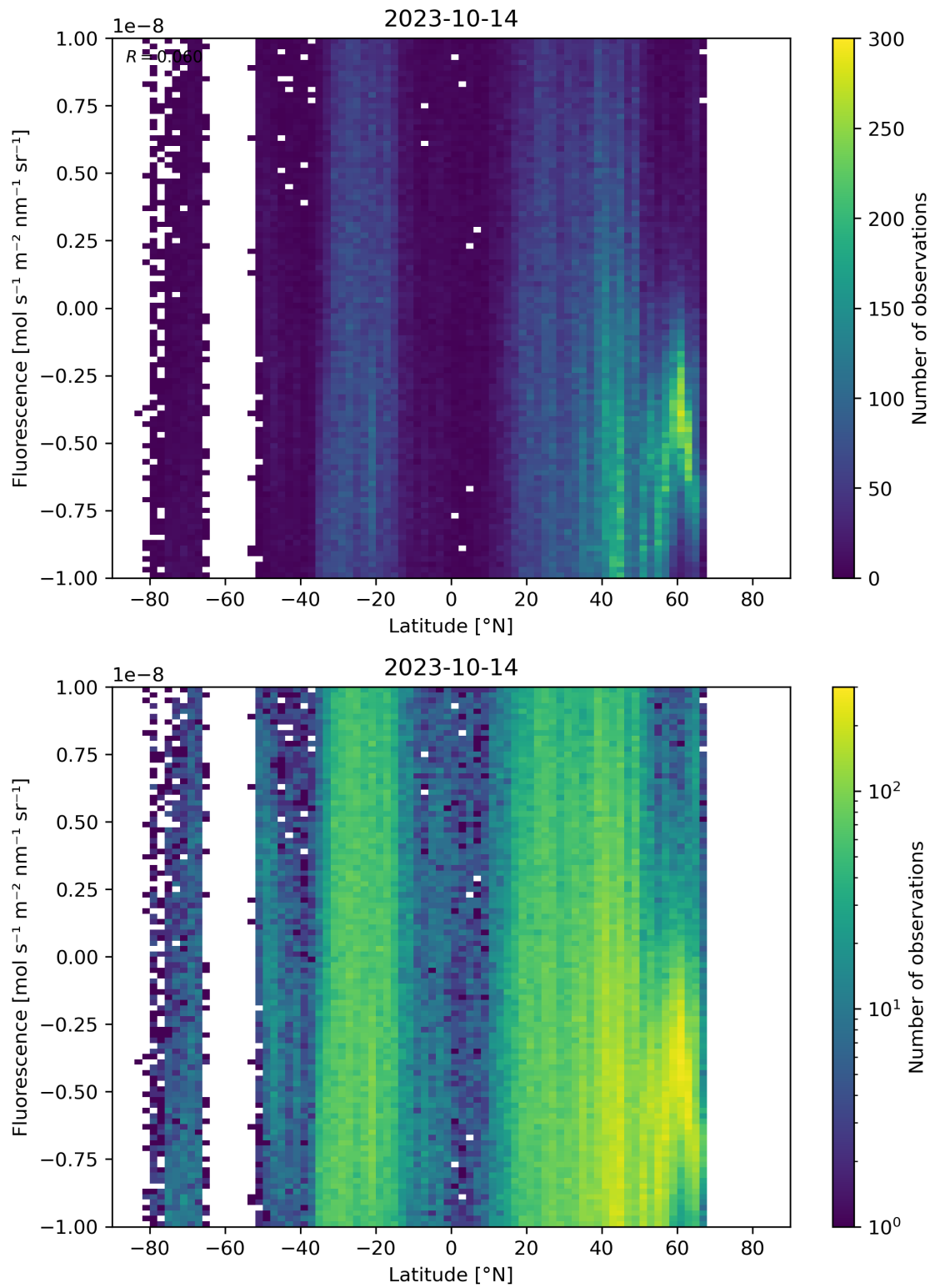
Figure 56: Scatter density plot of “Latitude” against “Fluorescence” for 2023-10-13 to 2023-10-15.
