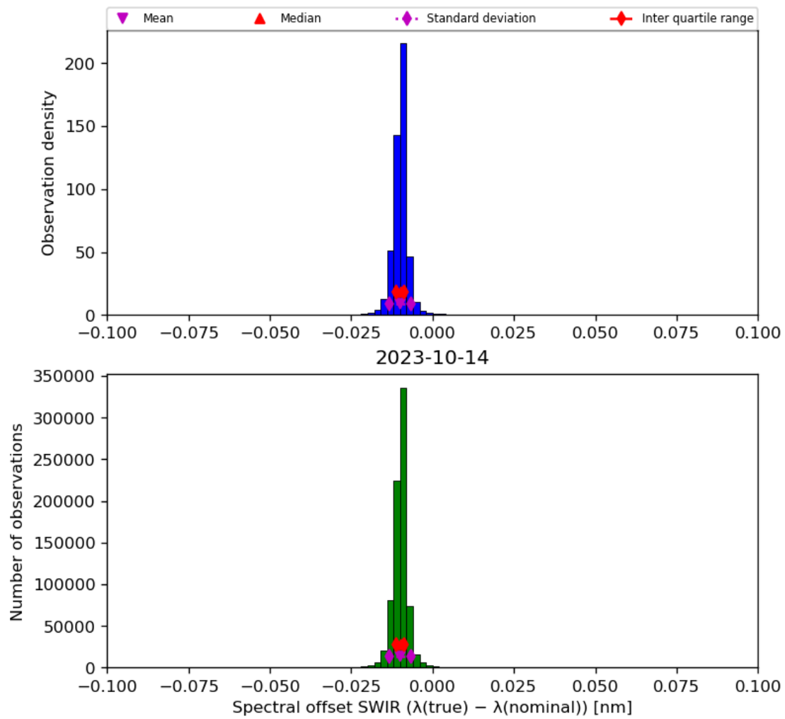
Figure 27: Histogram of “Spectral offset SWIR ( \lambda(\text{true}) - \lambda(\text{nominal}) )” for 2023-10-13 to 2023-10-15
