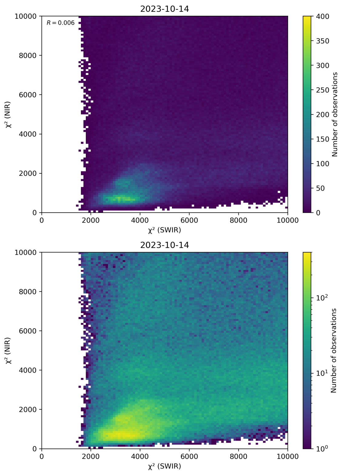
Figure 47: Scatter density plot of “ \chi^2 (SWIR)” against “ \chi^2 (NIR)” for 2023-10-13 to 2023-10-15.
