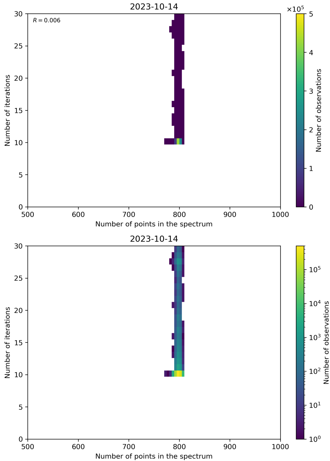
Figure 92: Scatter density plot of “Number of points in the spectrum” against “Number of iterations” for 2023-10-13 to 2023-10-15.
