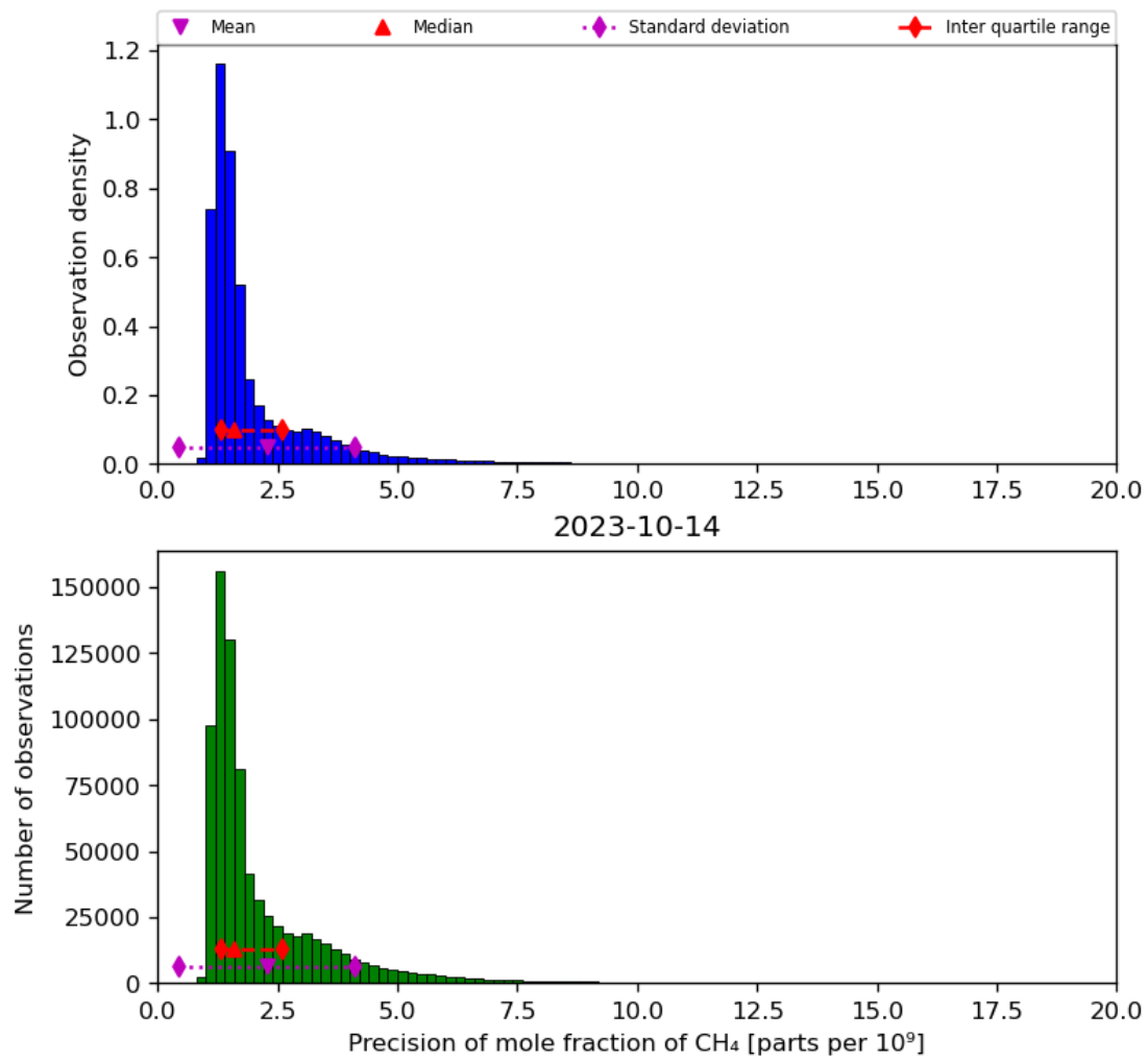
Figure 24: Histogram of “Precision of mole fraction of CH 4 ” for 2023-10-13 to 2023-10-15
