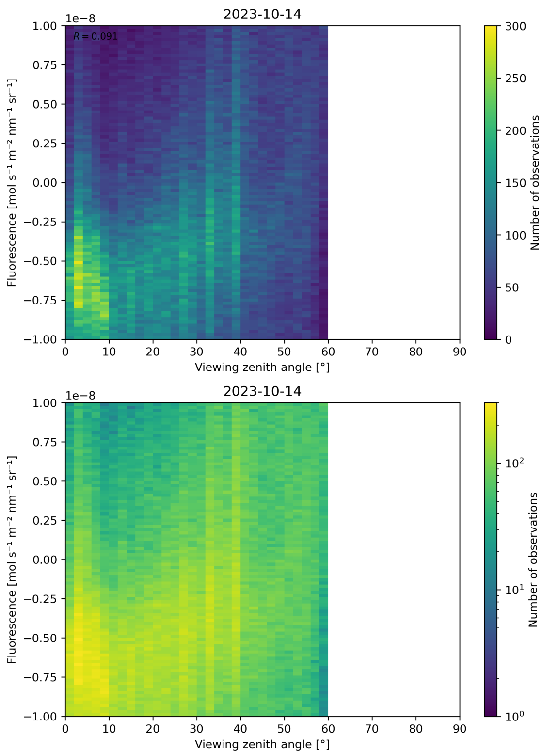
Figure 108: Scatter density plot of “Viewing zenith angle” against “Fluorescence” for 2023-10-13 to 2023-10-15.
