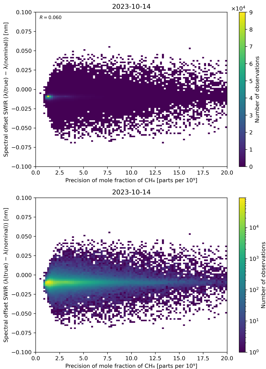
Figure 85: Scatter density plot of “Precision of mole fraction of CH 4 ” against “Spectral offset SWIR ( \lambda(\text{true}) - \lambda(\text{nominal}) )” for 2023-10-13 to 2023-10-15.
