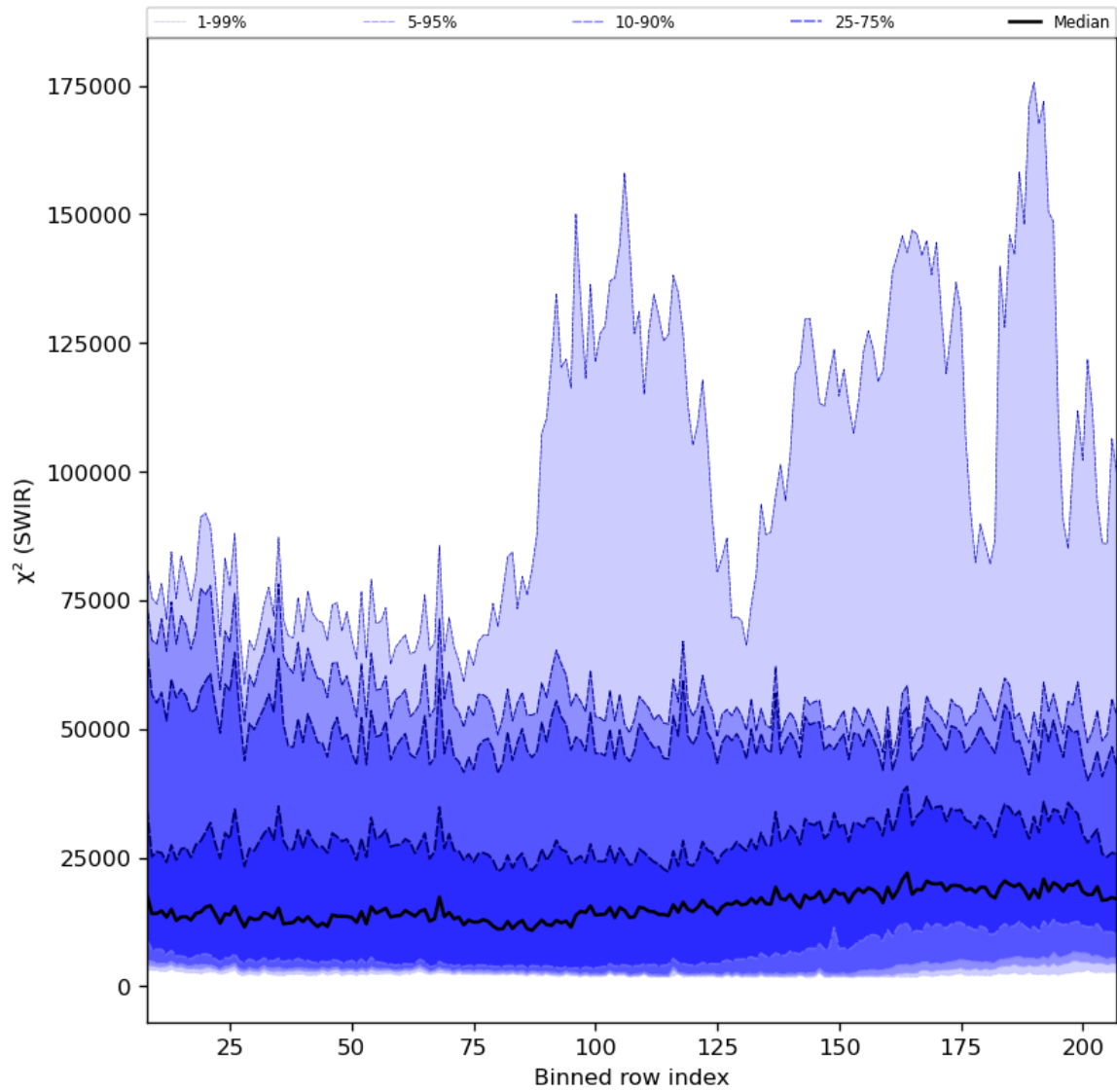
Figure 39: Along track statistics of " \chi^2 (SWIR)" for 2023-10-13 to 2023-10-15
