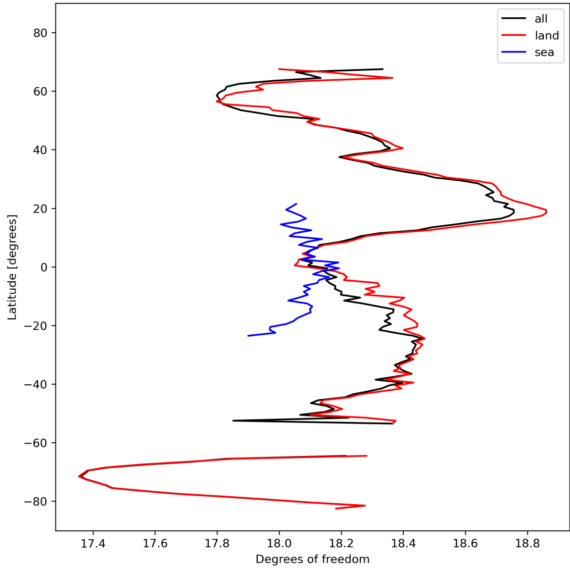
Figure 19: Zonal average of “Degrees of freedom” for 2023-10-13 to 2023-10-15.
