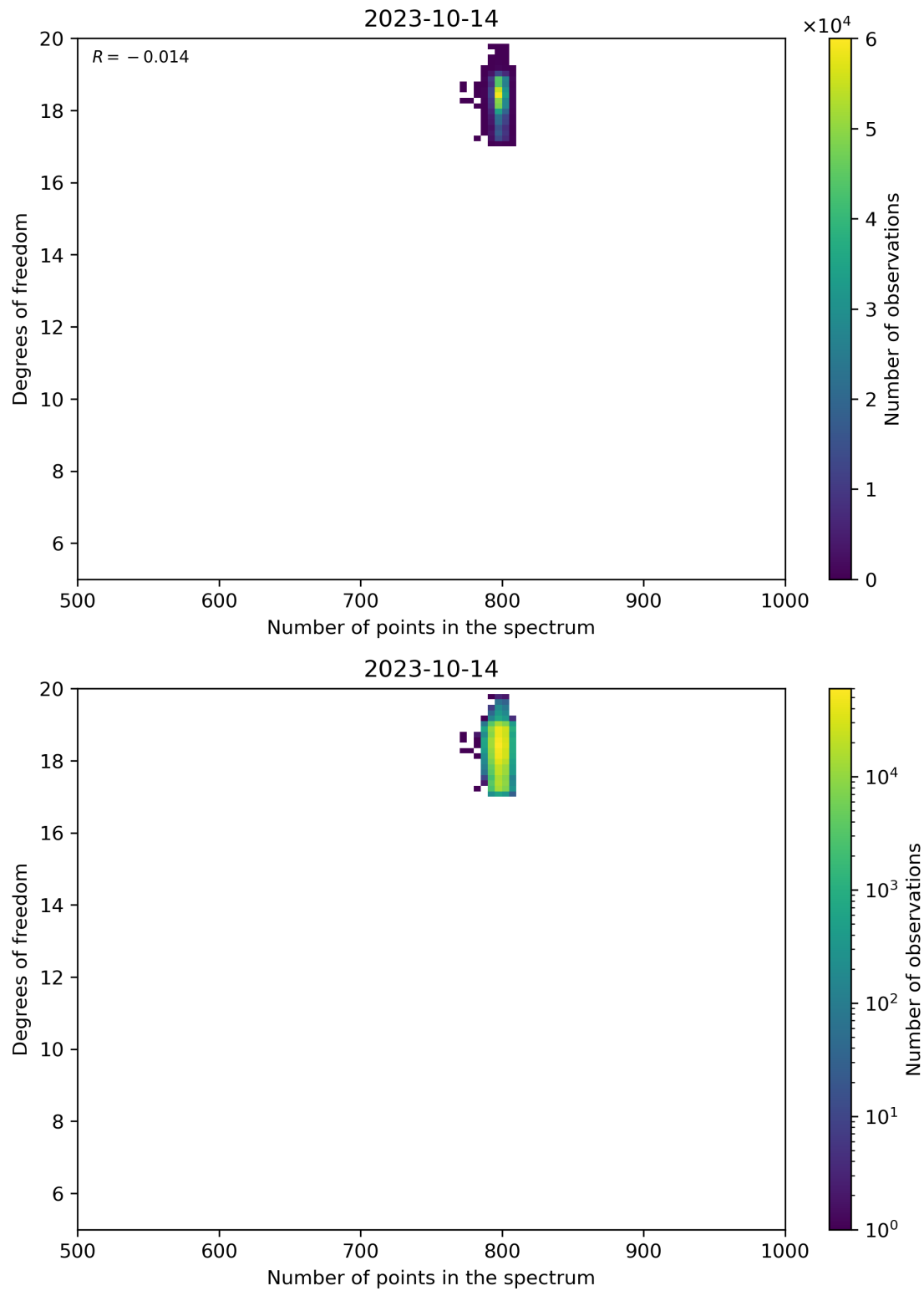
Figure 90: Scatter density plot of “Number of points in the spectrum” against “Degrees of freedom” for 2023-10-13 to 2023-10-15.
