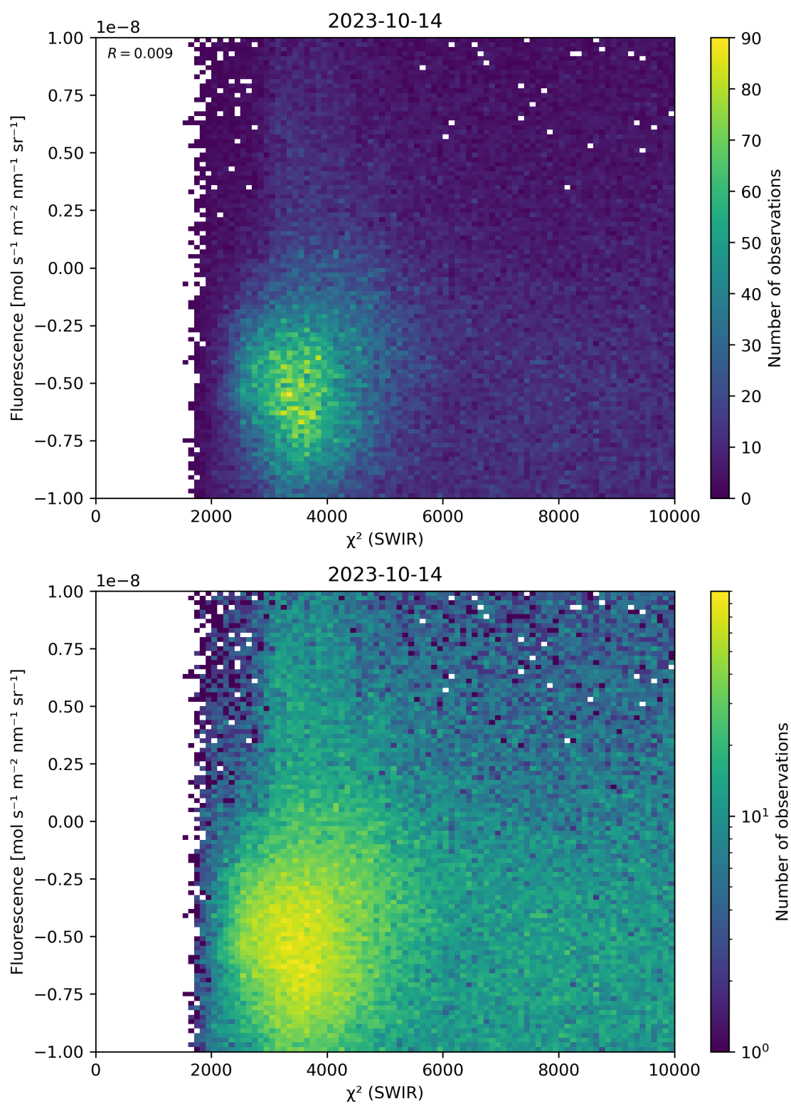
Figure 49: Scatter density plot of “ \chi^2 (SWIR)” against “Fluorescence” for 2023-10-13 to 2023-10-15.
