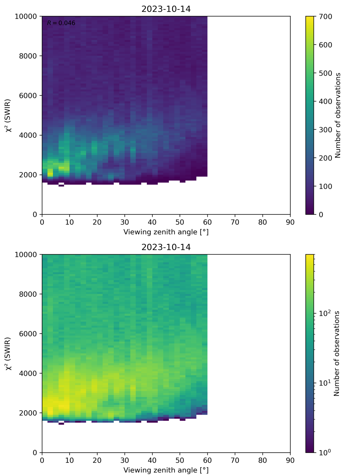
Figure 106: Scatter density plot of “Viewing zenith angle” against “ \chi^2 (SWIR)” for 2023-10-13 to 2023-10-15.
