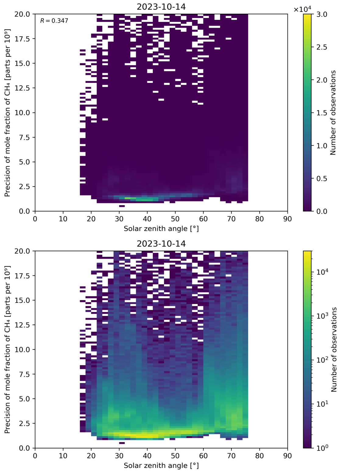
Figure 101: Scatter density plot of “Solar zenith angle” against “Precision of mole fraction of CH 4 ” for 2023-10-13 to 2023-10-15.
