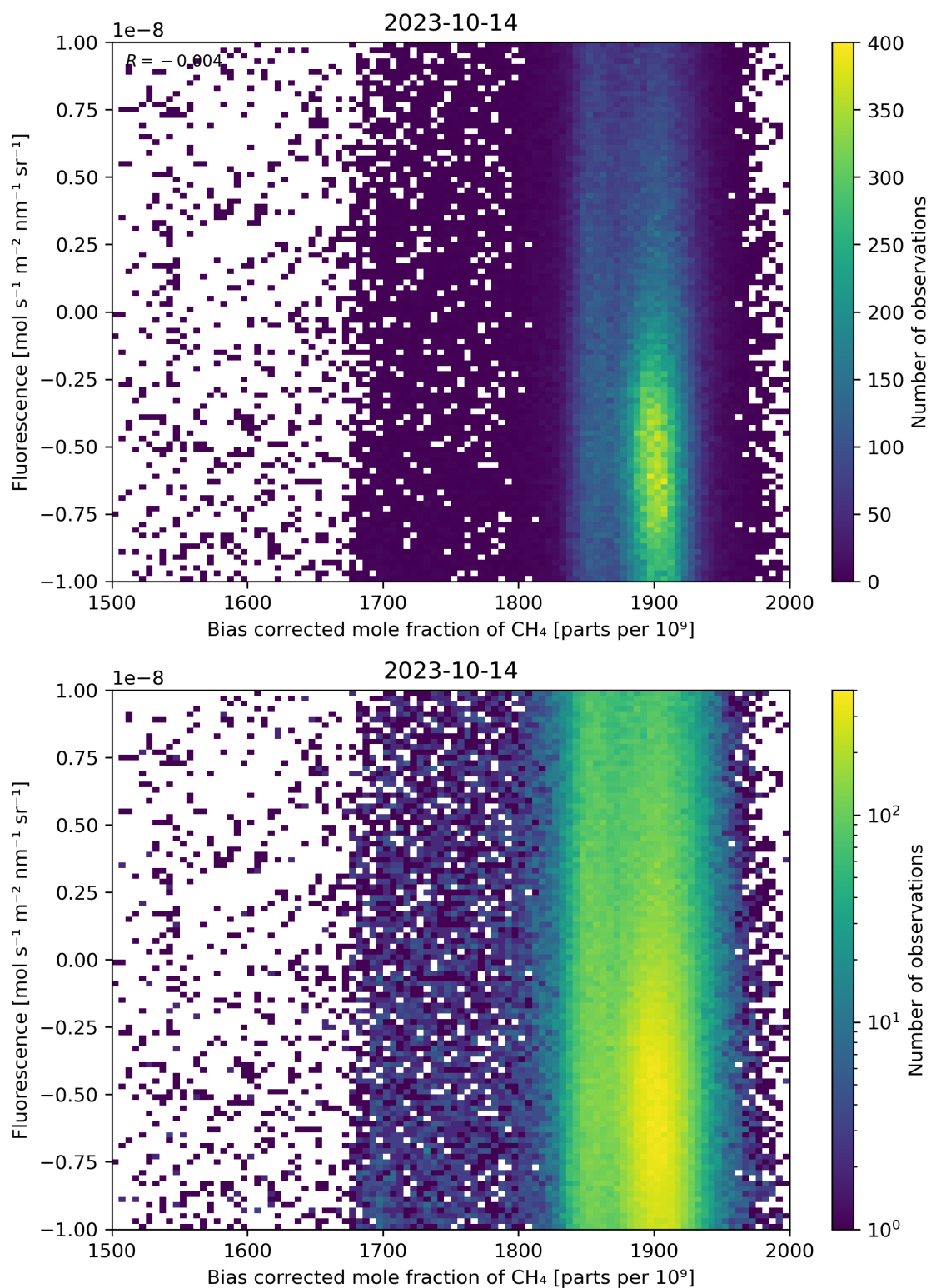
Figure 66: Scatter density plot of “Bias corrected mole fraction of \text{CH}_4 ” against “Fluorescence” for 2023-10-13 to 2023-10-15.
