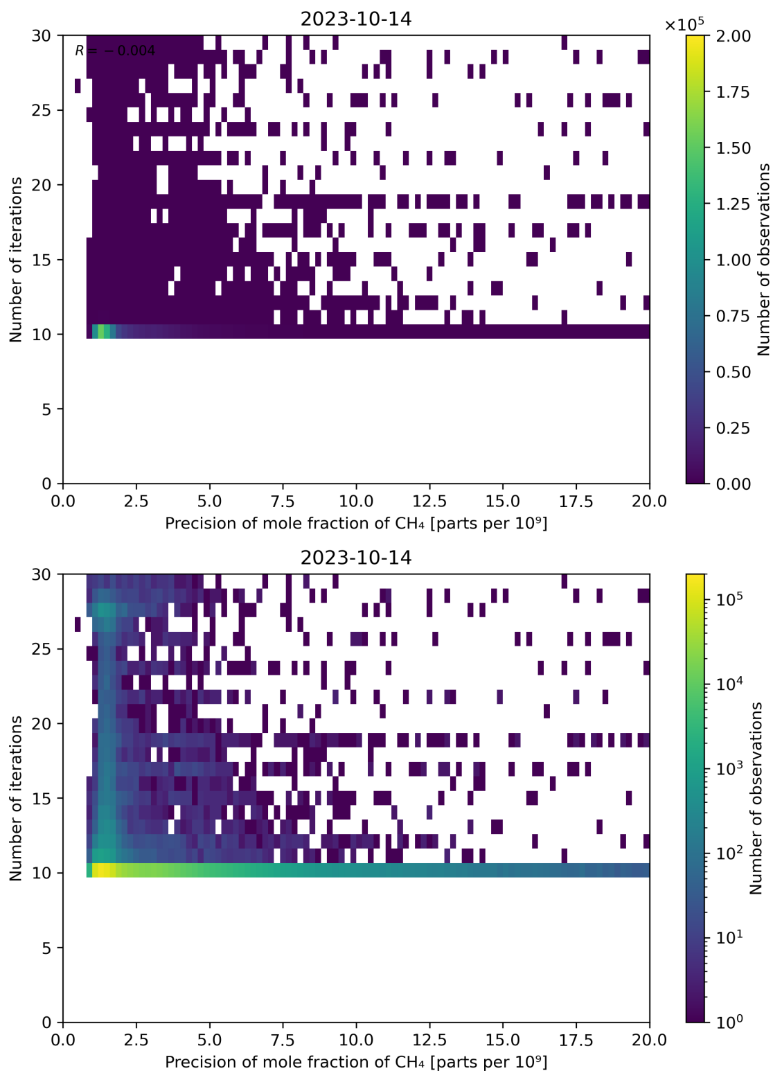
Figure 83: Scatter density plot of “Precision of mole fraction of CH 4 ” against “Number of iterations” for 2023-10-13 to 2023-10-15.
