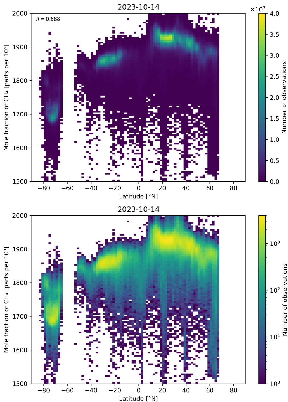
Figure 57: Scatter density plot of “Latitude” against “Mole fraction of \text{CH}_4 ” for 2023-10-13 to 2023-10-15.
