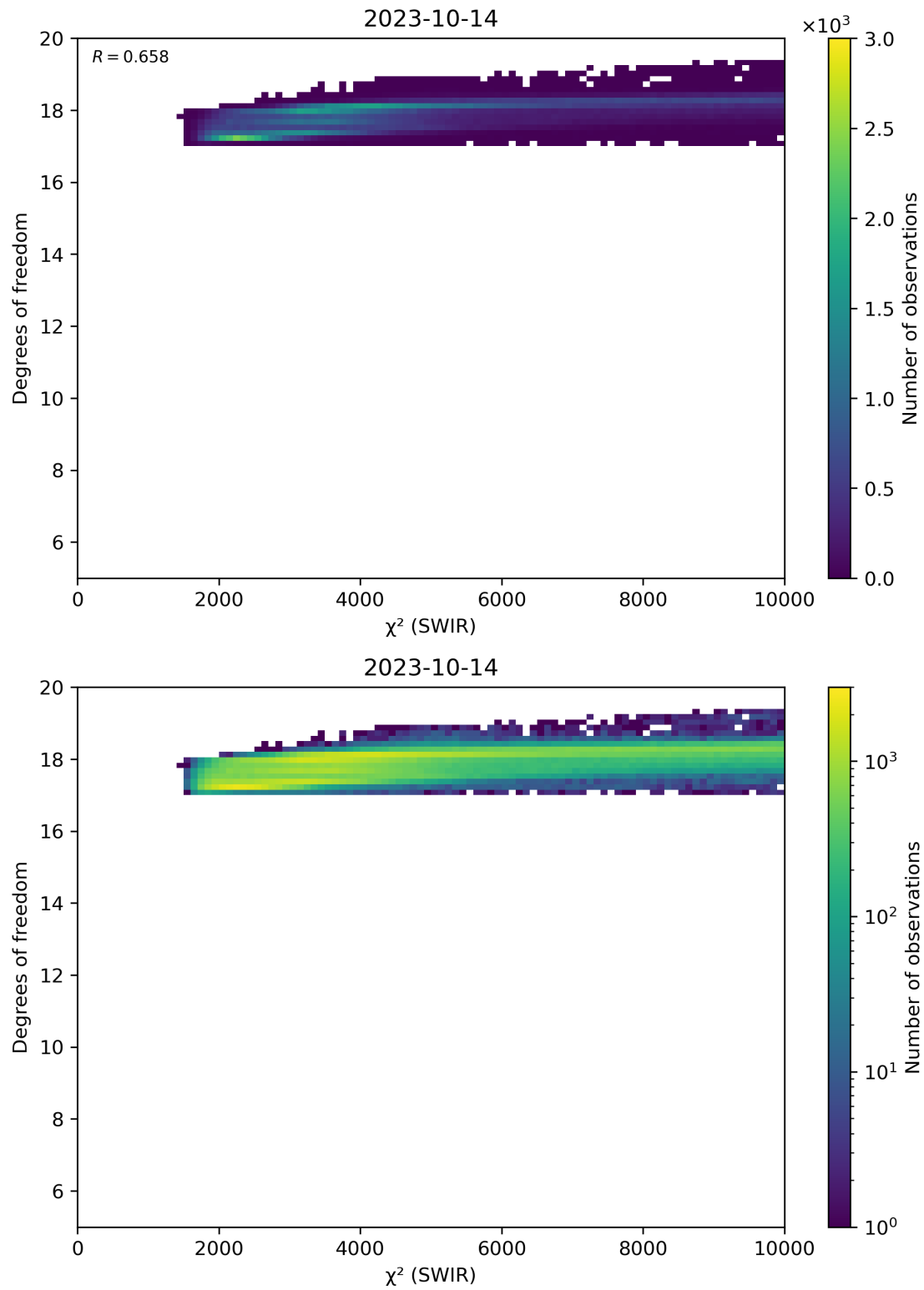
Figure 48: Scatter density plot of “ \chi^2 (SWIR)” against “Degrees of freedom” for 2023-10-13 to 2023-10-15.
