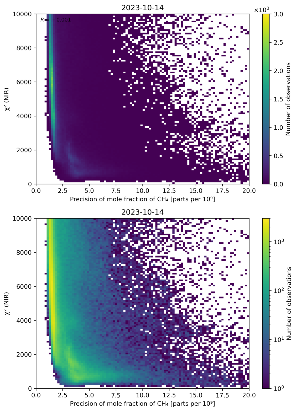
Figure 78: Scatter density plot of “Precision of mole fraction of CH 4 ” against “ \chi^2 (NIR)” for 2023-10-13 to 2023-10-15.
