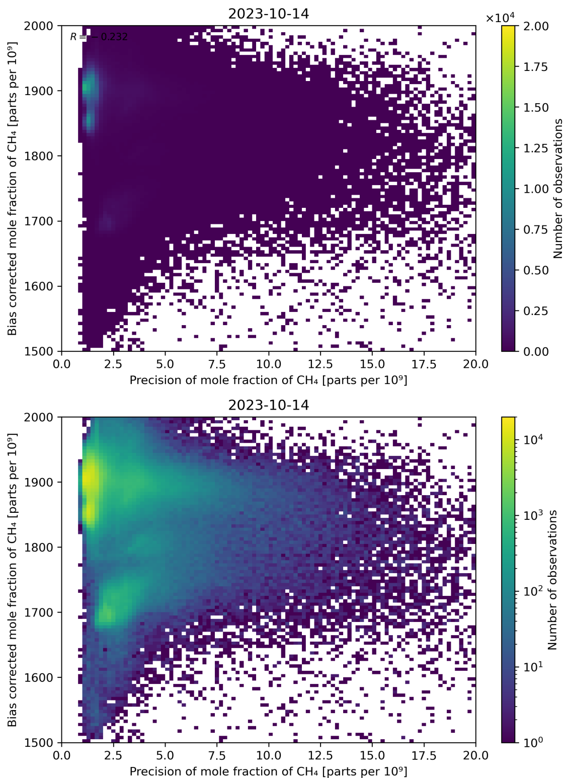
Figure 82: Scatter density plot of “Precision of mole fraction of CH 4 ” against “Bias corrected mole fraction of CH 4 ” for 2023-10-13 to 2023-10-15.
