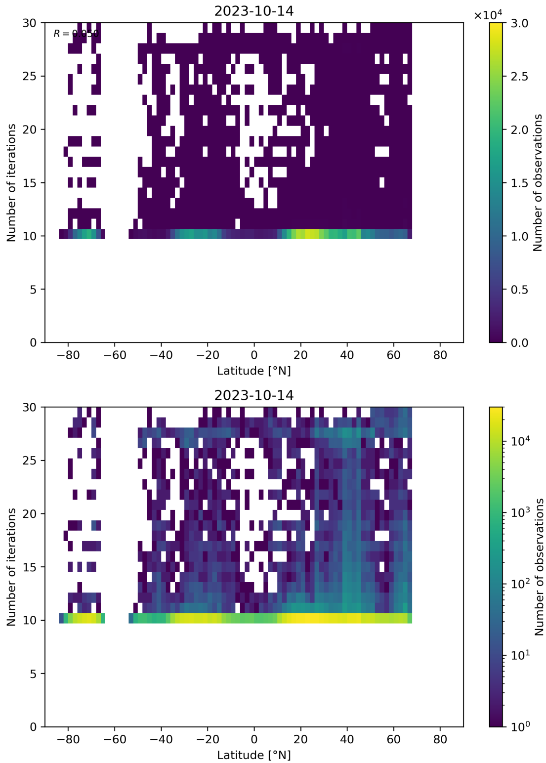
Figure 60: Scatter density plot of “Latitude” against “Number of iterations” for 2023-10-13 to 2023-10-15.
