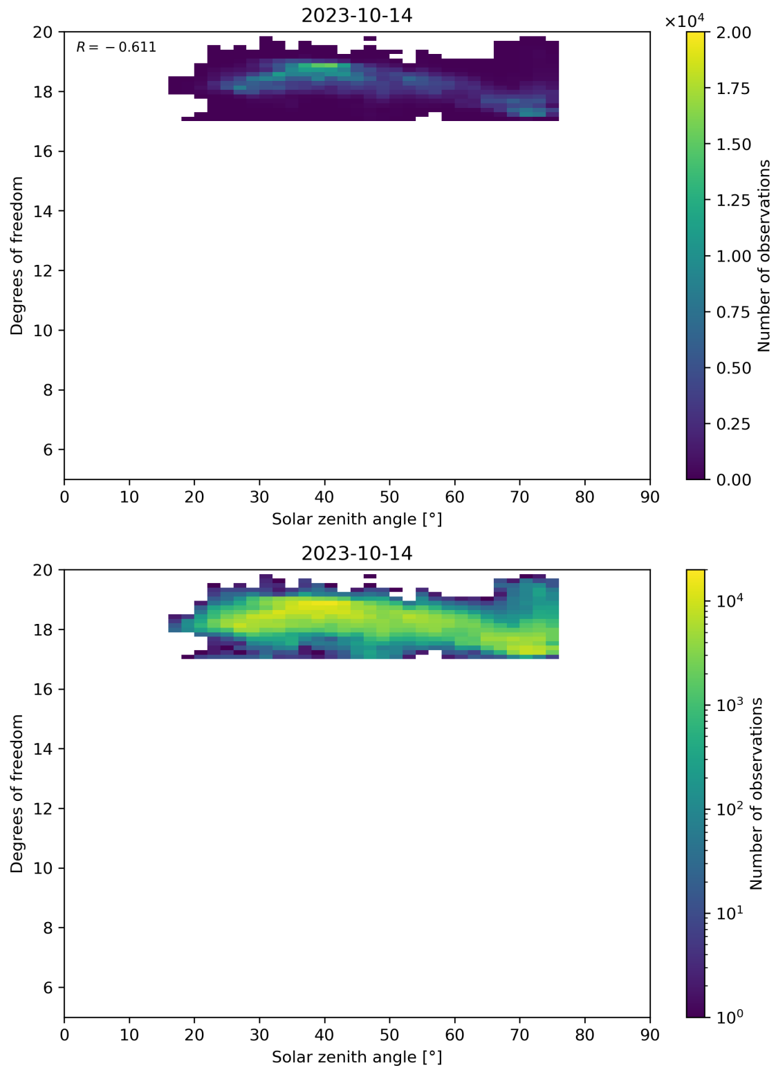
Figure 96: Scatter density plot of “Solar zenith angle” against “Degrees of freedom” for 2023-10-13 to 2023-10-15.
