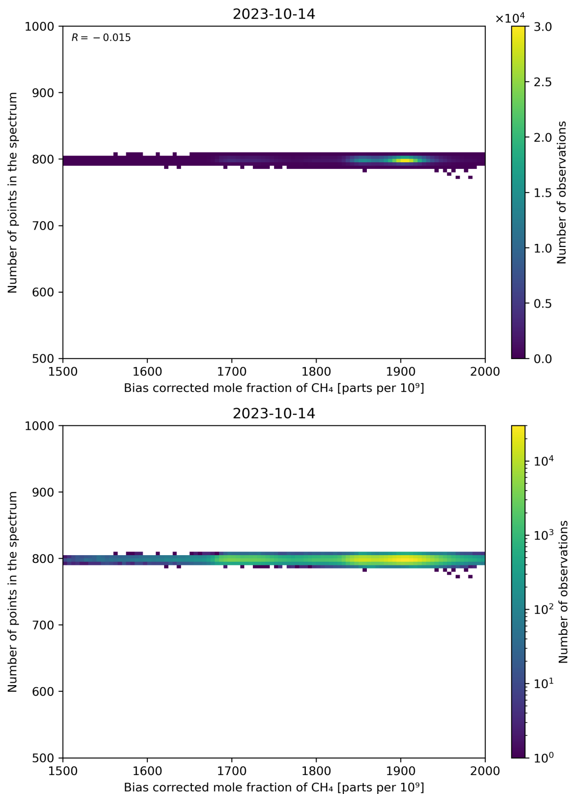
Figure 68: Scatter density plot of “Bias corrected mole fraction of CH 4 ” against “Number of points in the spectrum” for 2023-10-13 to 2023-10-15.
