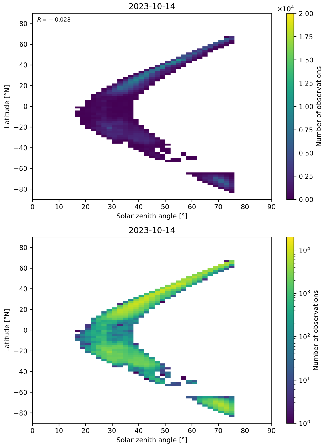
Figure 98: Scatter density plot of “Solar zenith angle” against “Latitude” for 2023-10-13 to 2023-10-15.
