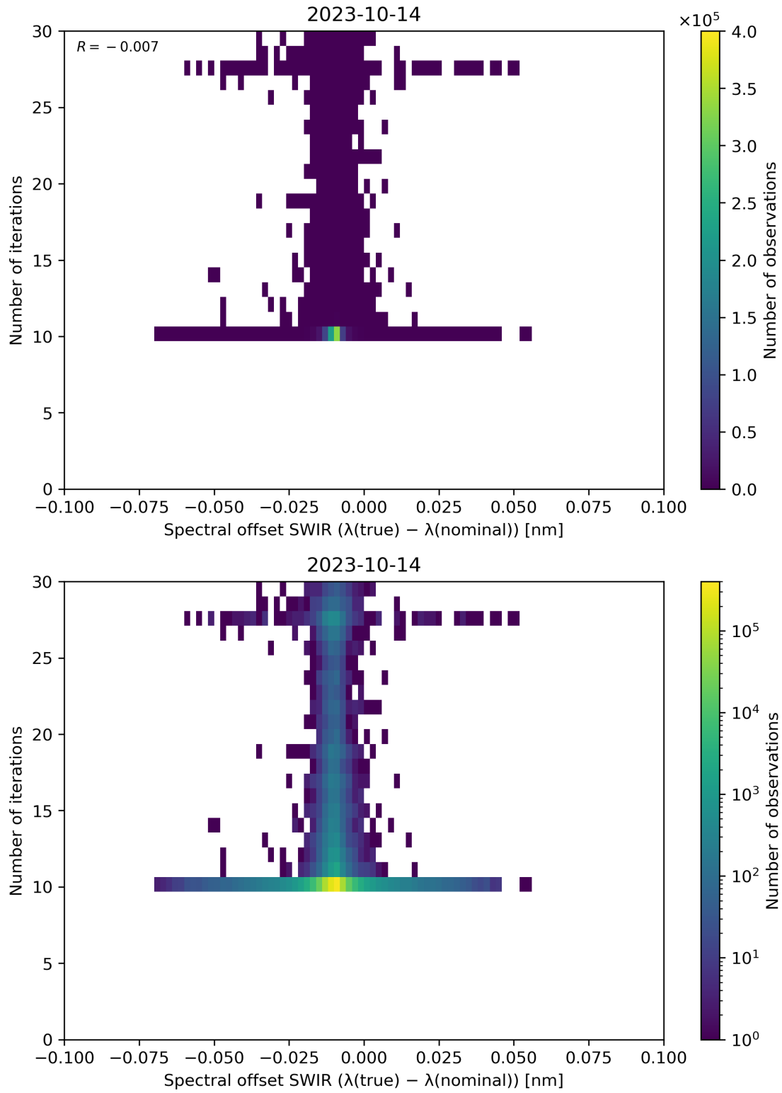
Figure 121: Scatter density plot of “Spectral offset SWIR ( \lambda(\text{true}) - \lambda(\text{nominal}) )” against “Number of iterations” for 2023-10-13 to 2023-10-15.
