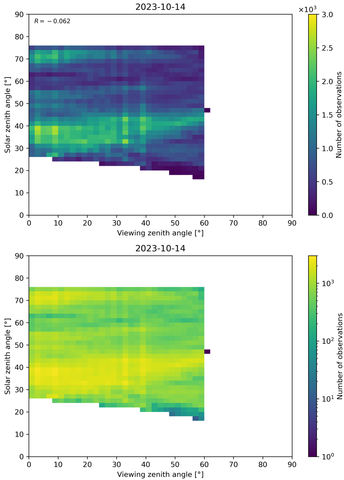
Figure 115: Scatter density plot of “Viewing zenith angle” against “Solar zenith angle” for 2023-10-13 to 2023-10-15.
