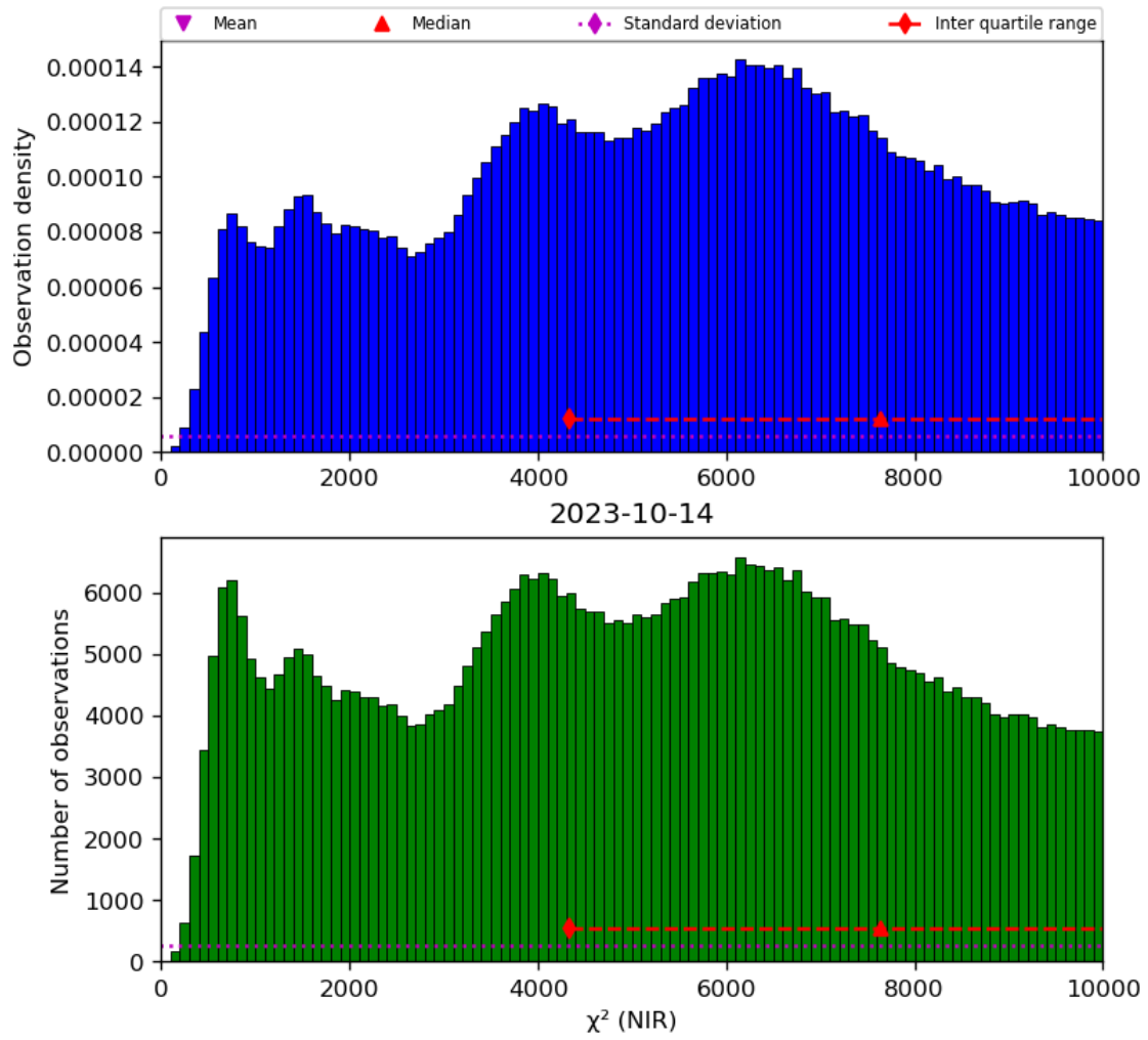
Figure 29: Histogram of “ \chi^2 (NIR)” for 2023-10-13 to 2023-10-15
