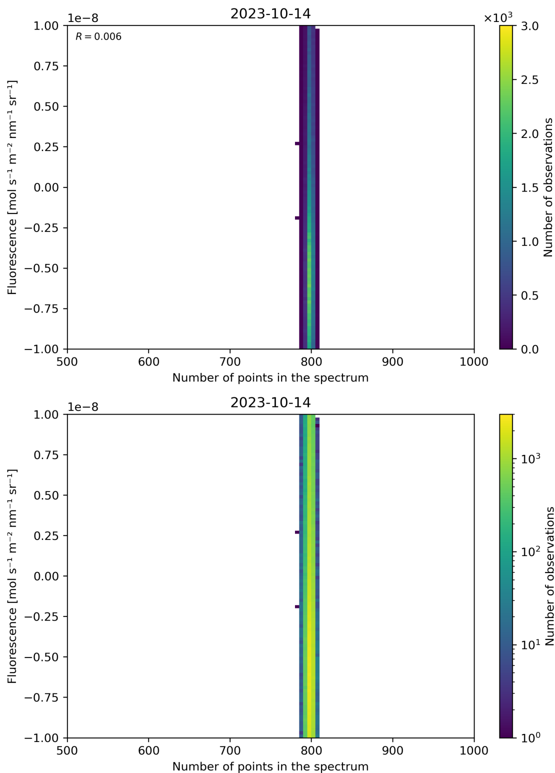
Figure 91: Scatter density plot of “Number of points in the spectrum” against “Fluorescence” for 2023-10-13 to 2023-10-15.
