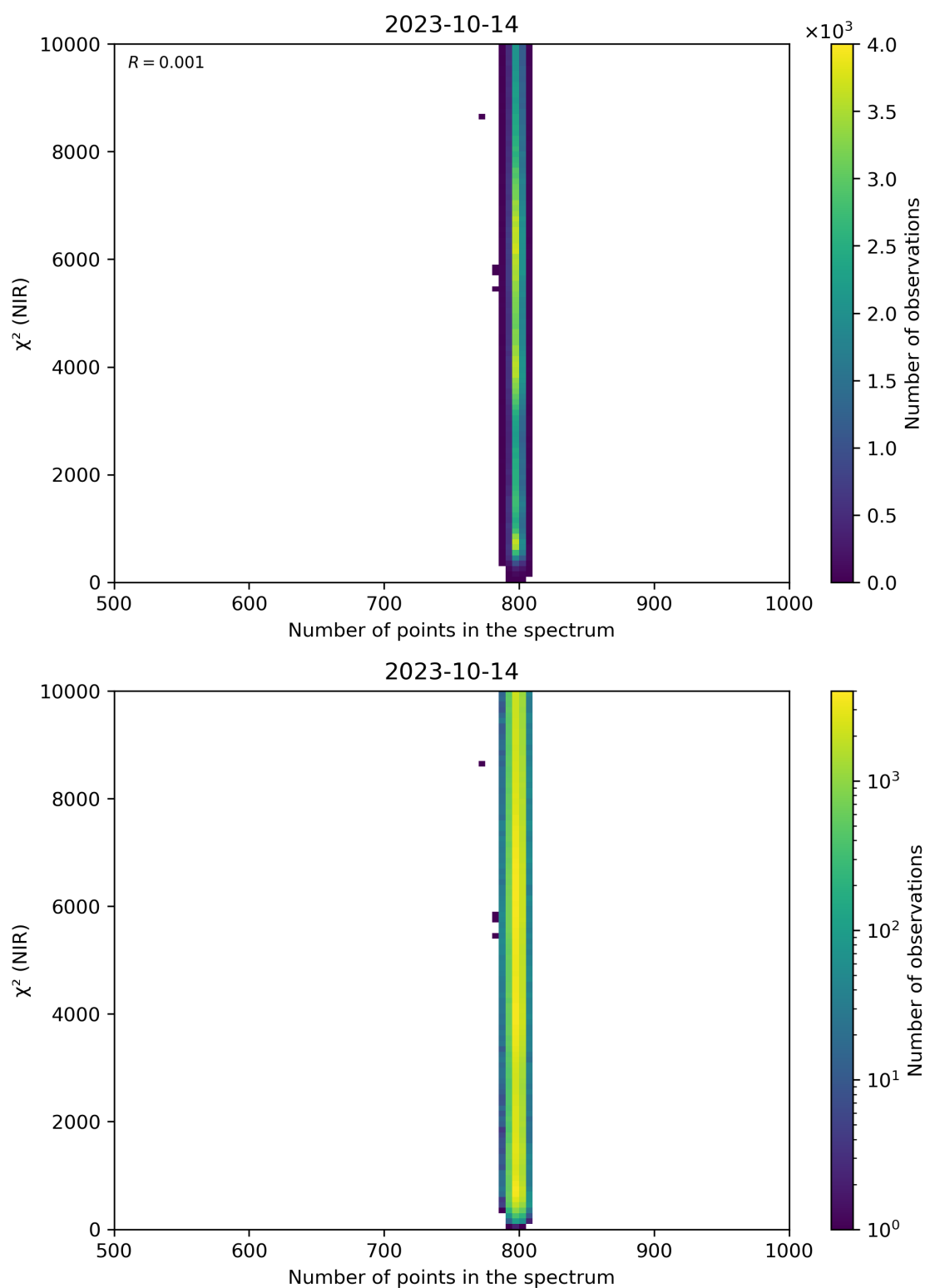
Figure 88: Scatter density plot of “Number of points in the spectrum” against “ \chi^2 (NIR)” for 2023-10-13 to 2023-10-15.
