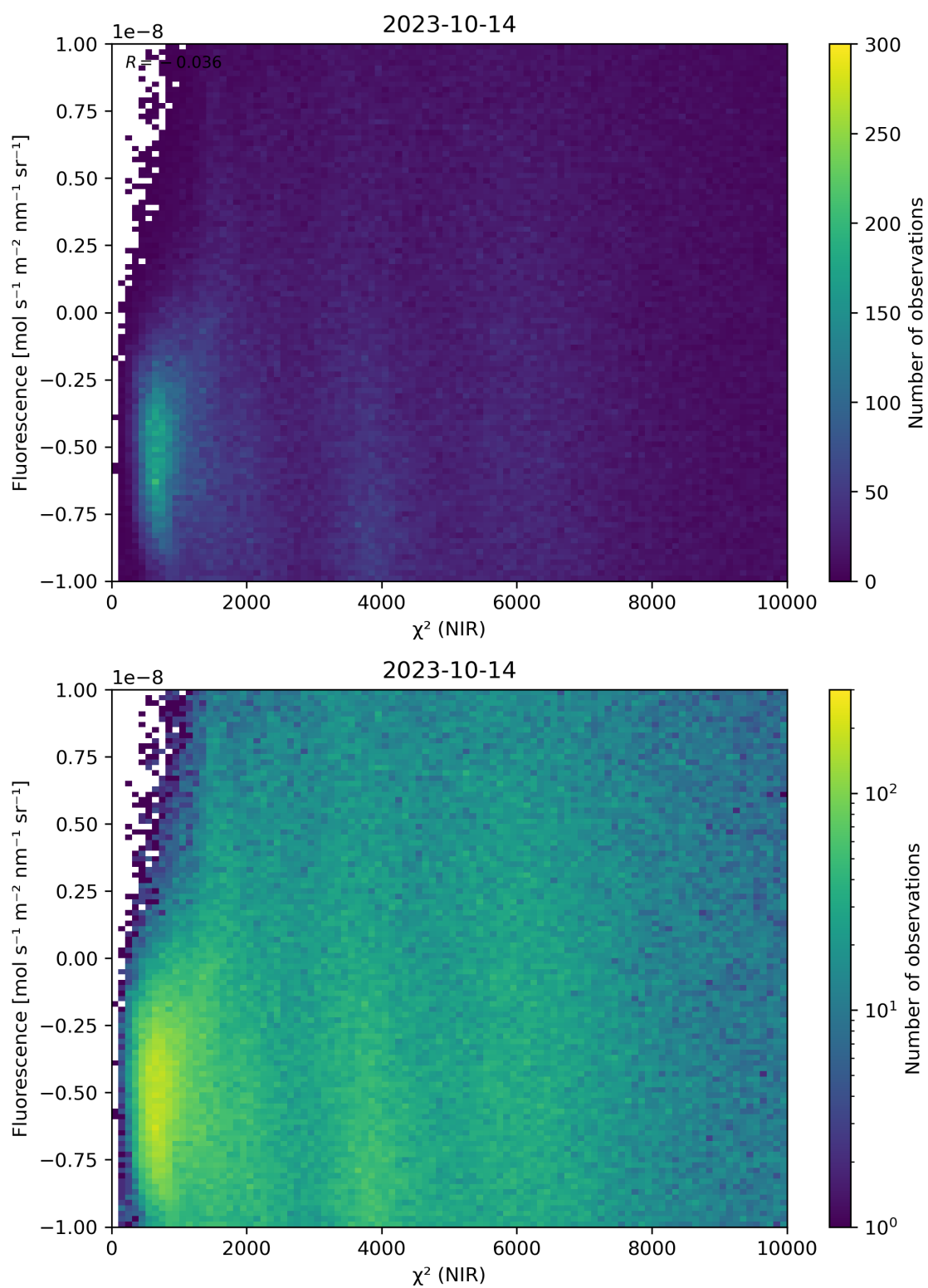
Figure 45: Scatter density plot of “ \chi^2 (NIR)” against “Fluorescence” for 2023-10-13 to 2023-10-15.
