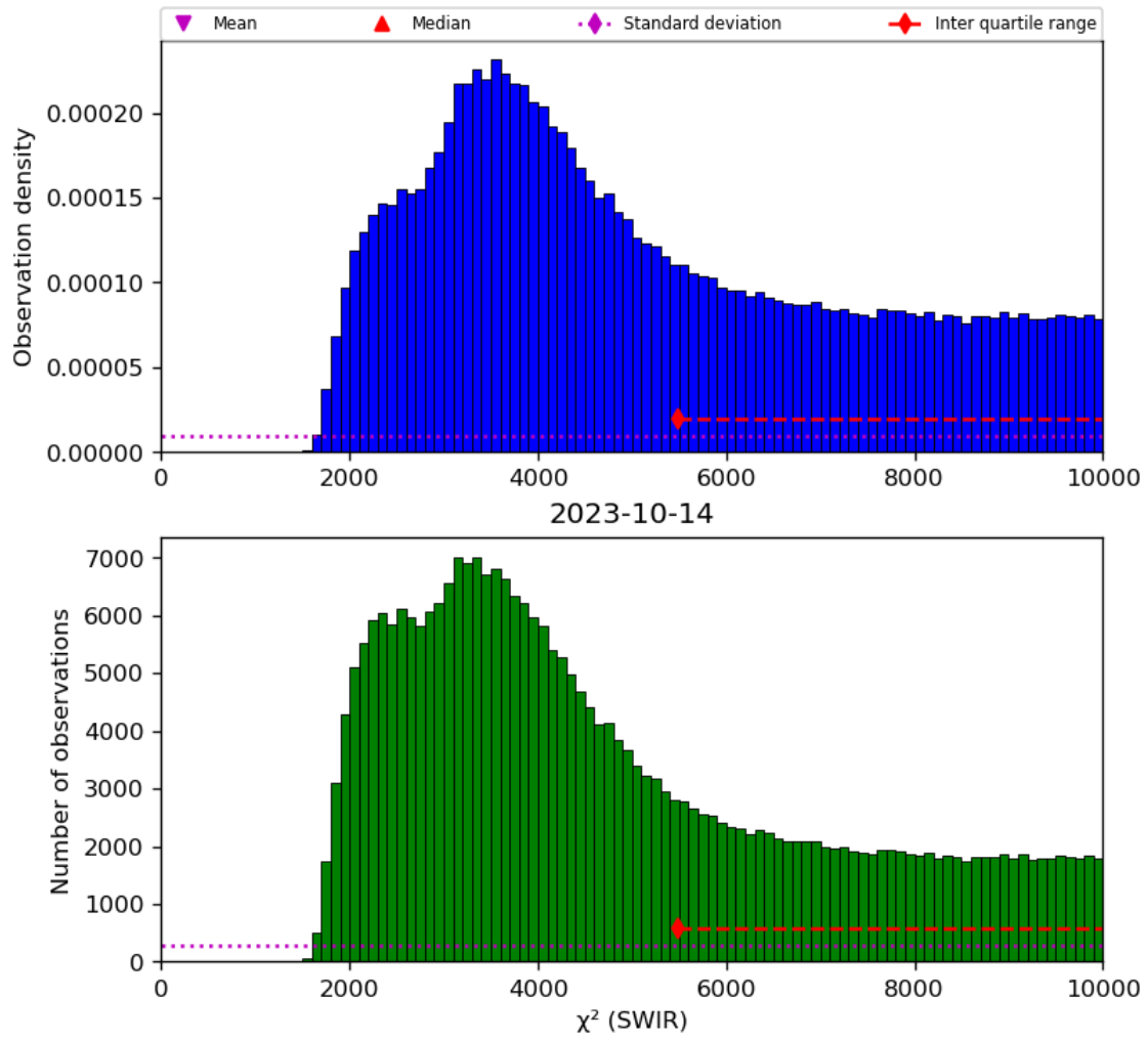
Figure 28: Histogram of “ \chi^2 (SWIR)” for 2023-10-13 to 2023-10-15
