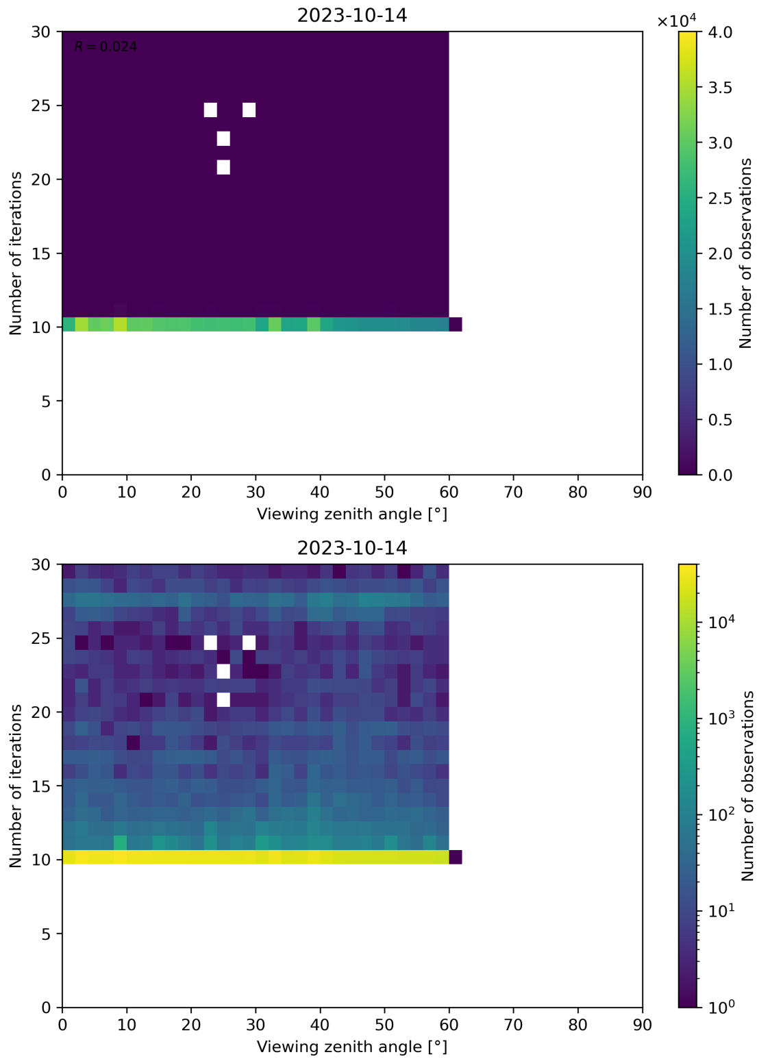
Figure 113: Scatter density plot of “Viewing zenith angle” against “Number of iterations” for 2023-10-13 to 2023-10-15.
