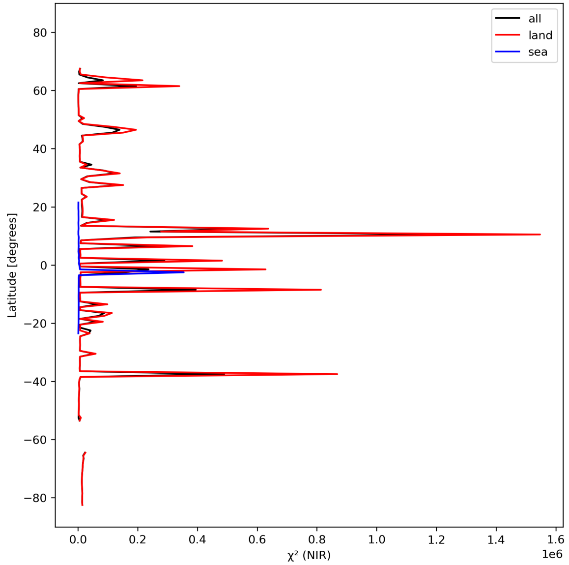
Figure 18: Zonal average of “ \chi^2 (NIR)” for 2023-10-13 to 2023-10-15.
