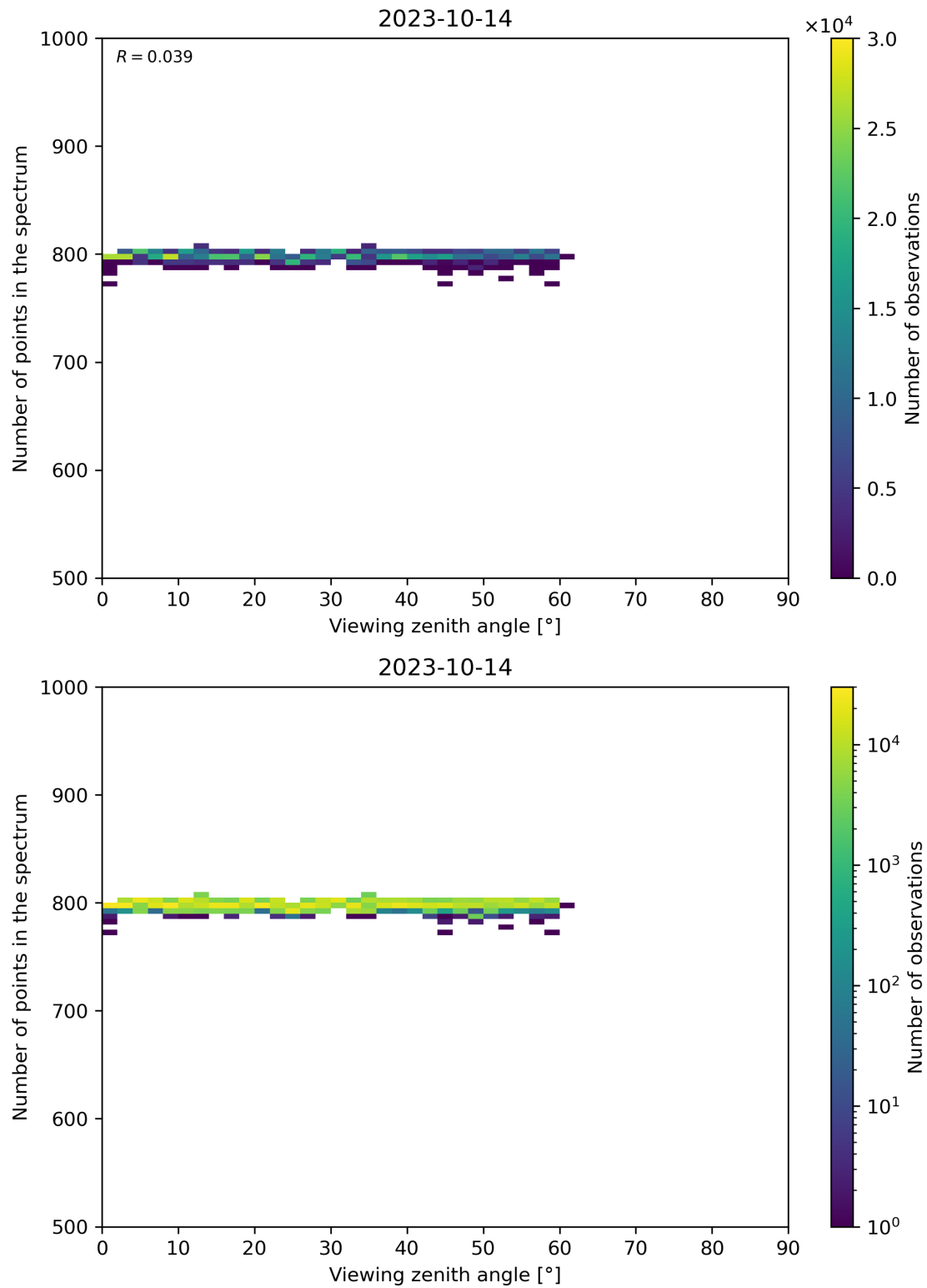
Figure 114: Scatter density plot of “Viewing zenith angle” against “Number of points in the spectrum” for 2023-10-13 to 2023-10-15.
