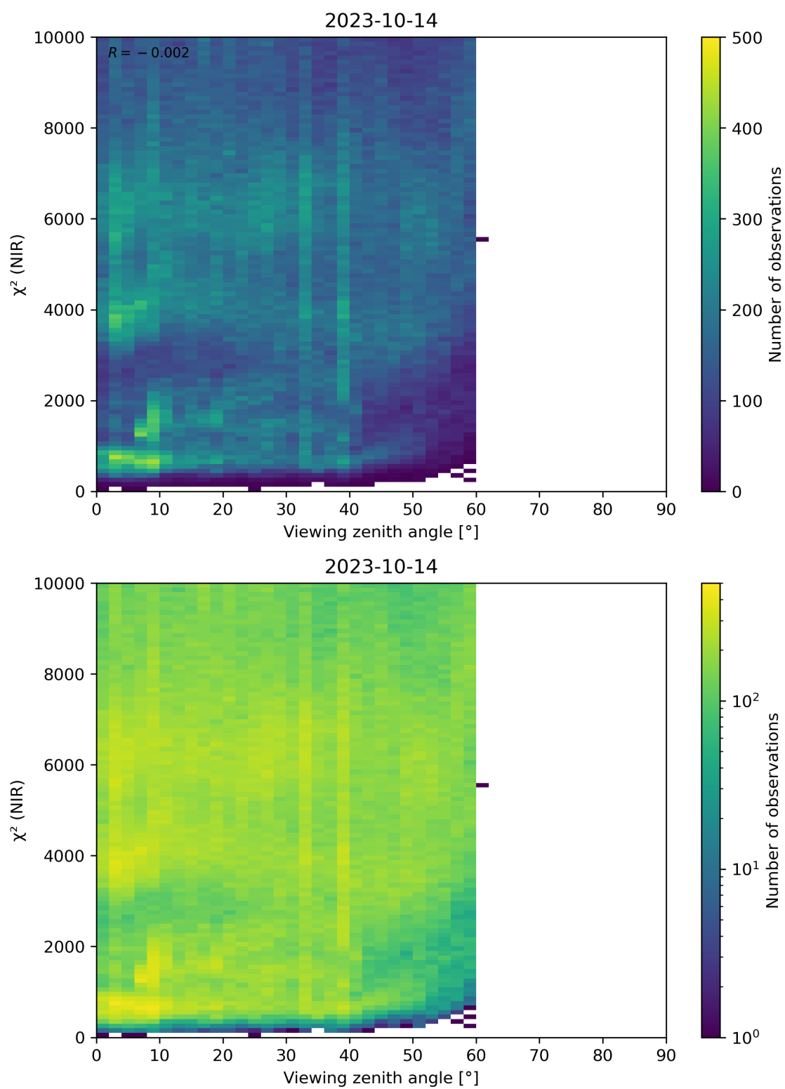
Figure 105: Scatter density plot of “Viewing zenith angle” against “ \chi^2 (NIR)” for 2023-10-13 to 2023-10-15.
