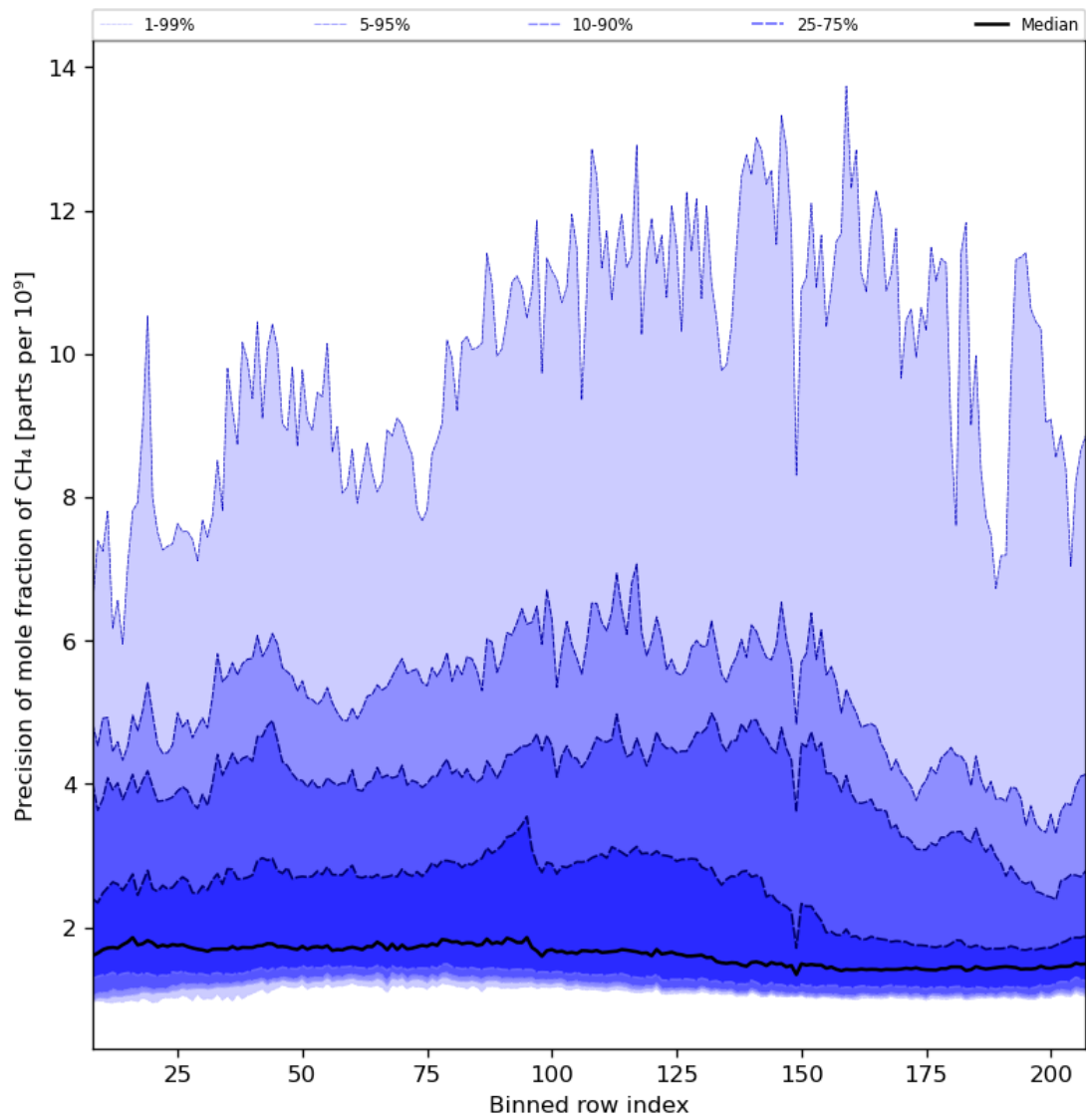
Figure 35: Along track statistics of “Precision of mole fraction of CH 4 ” for 2023-10-13 to 2023-10-15
