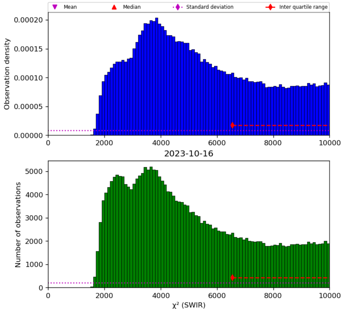
Figure 28: Histogram of “ \chi^2 (SWIR)” for 2023-10-15 to 2023-10-17
