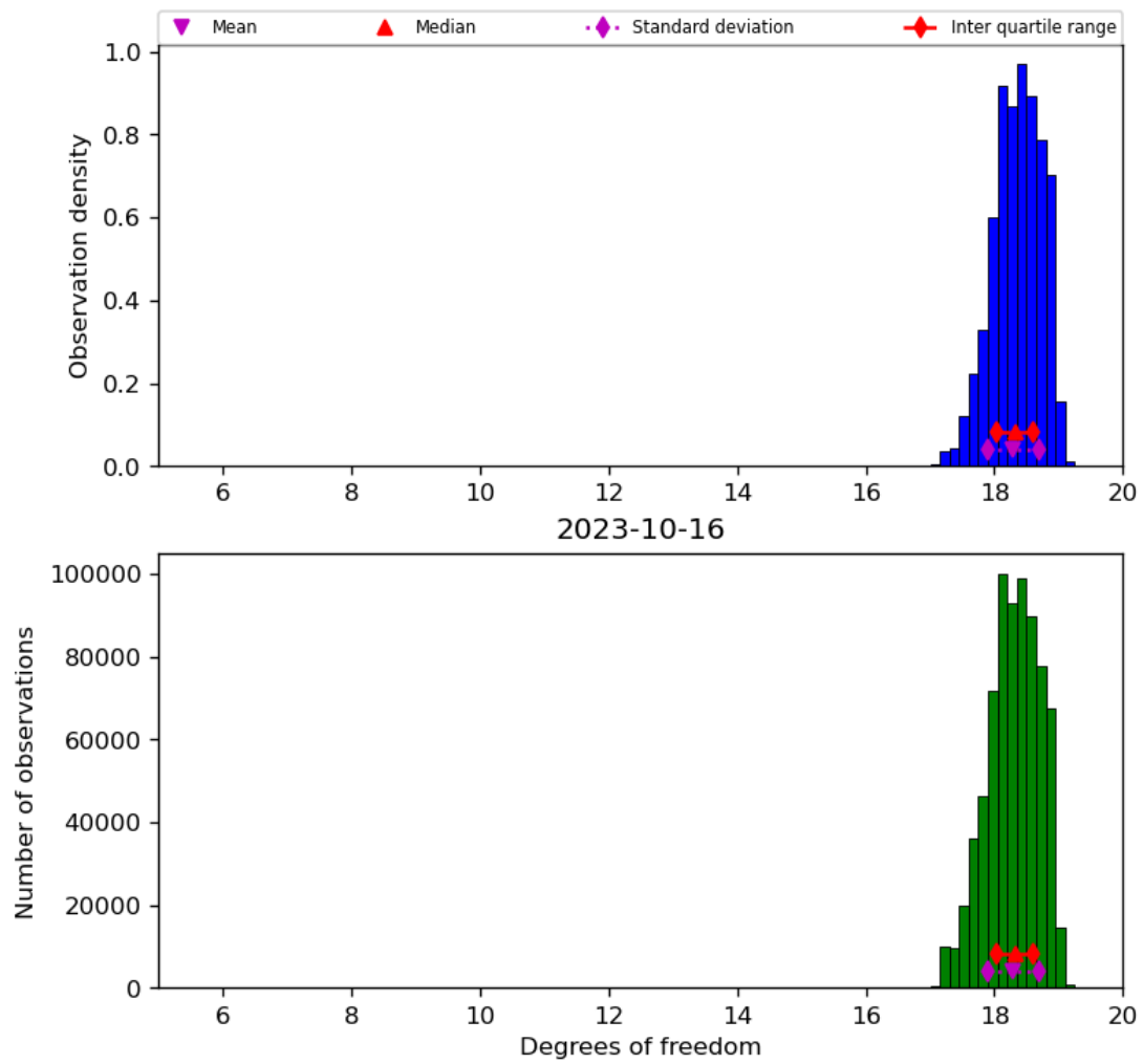
Figure 30: Histogram of “Degrees of freedom” for 2023-10-15 to 2023-10-17
