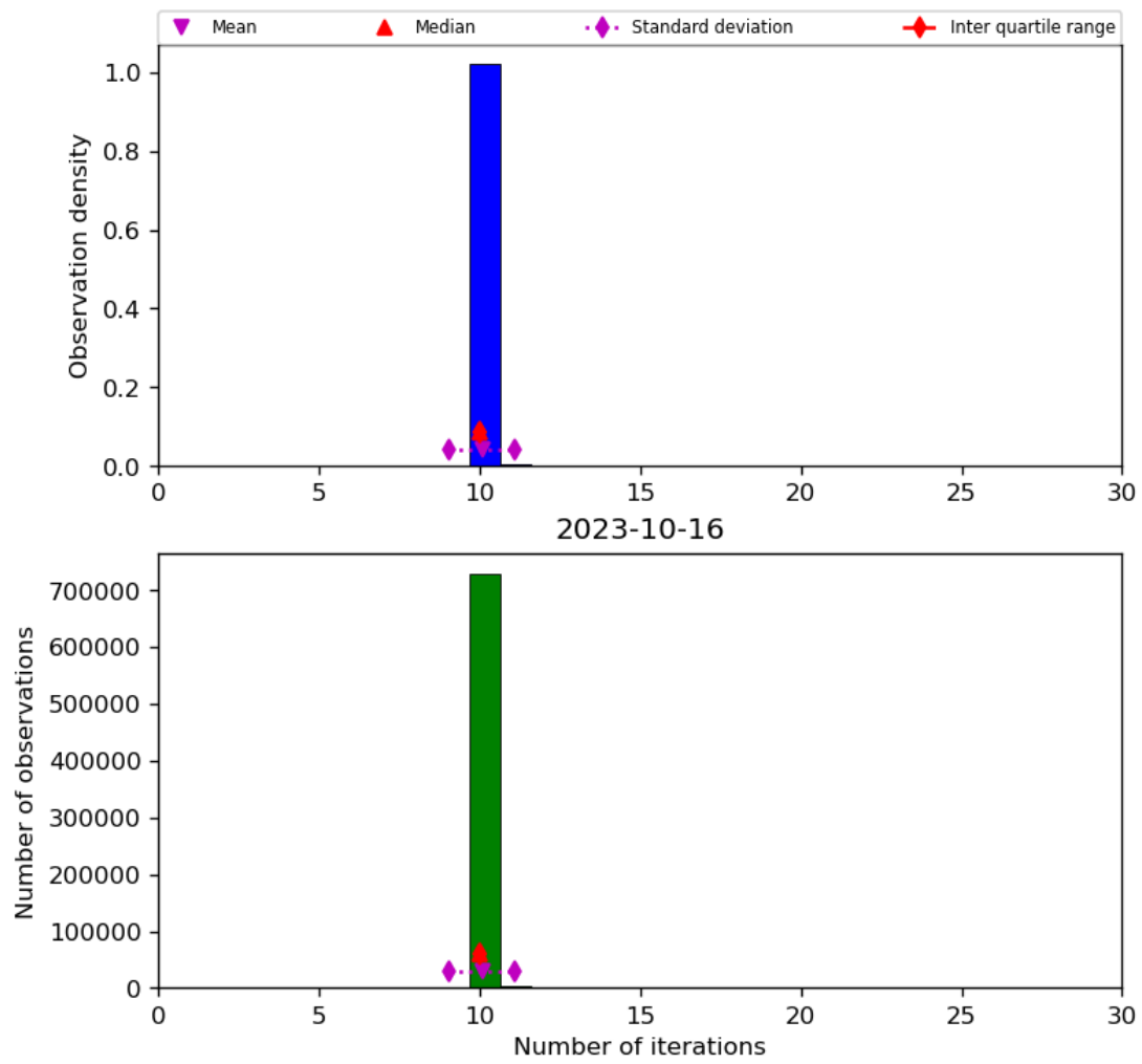
Figure 31: Histogram of “Number of iterations” for 2023-10-15 to 2023-10-17
