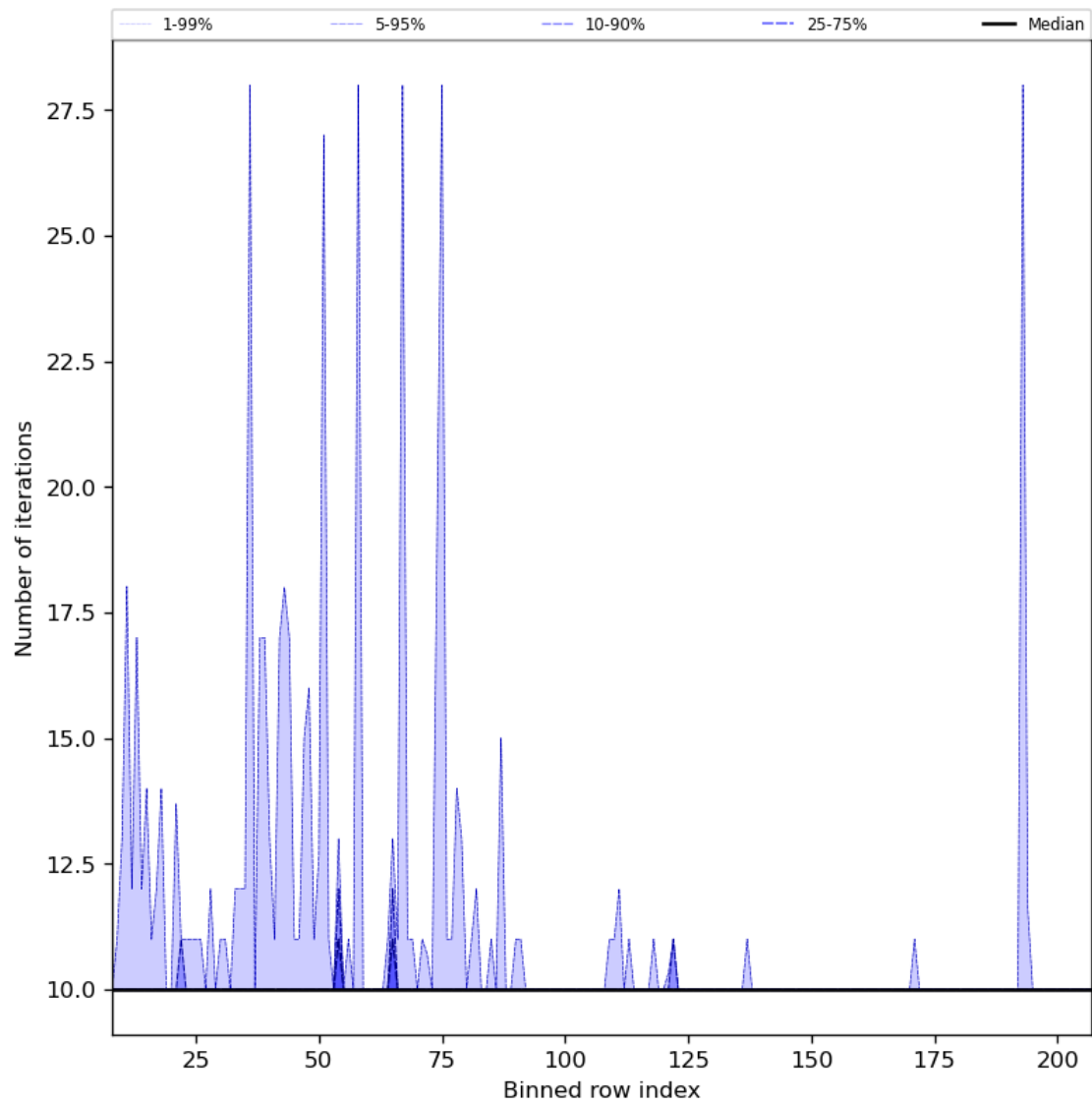
Figure 42: Along track statistics of “Number of iterations” for 2023-10-15 to 2023-10-17
