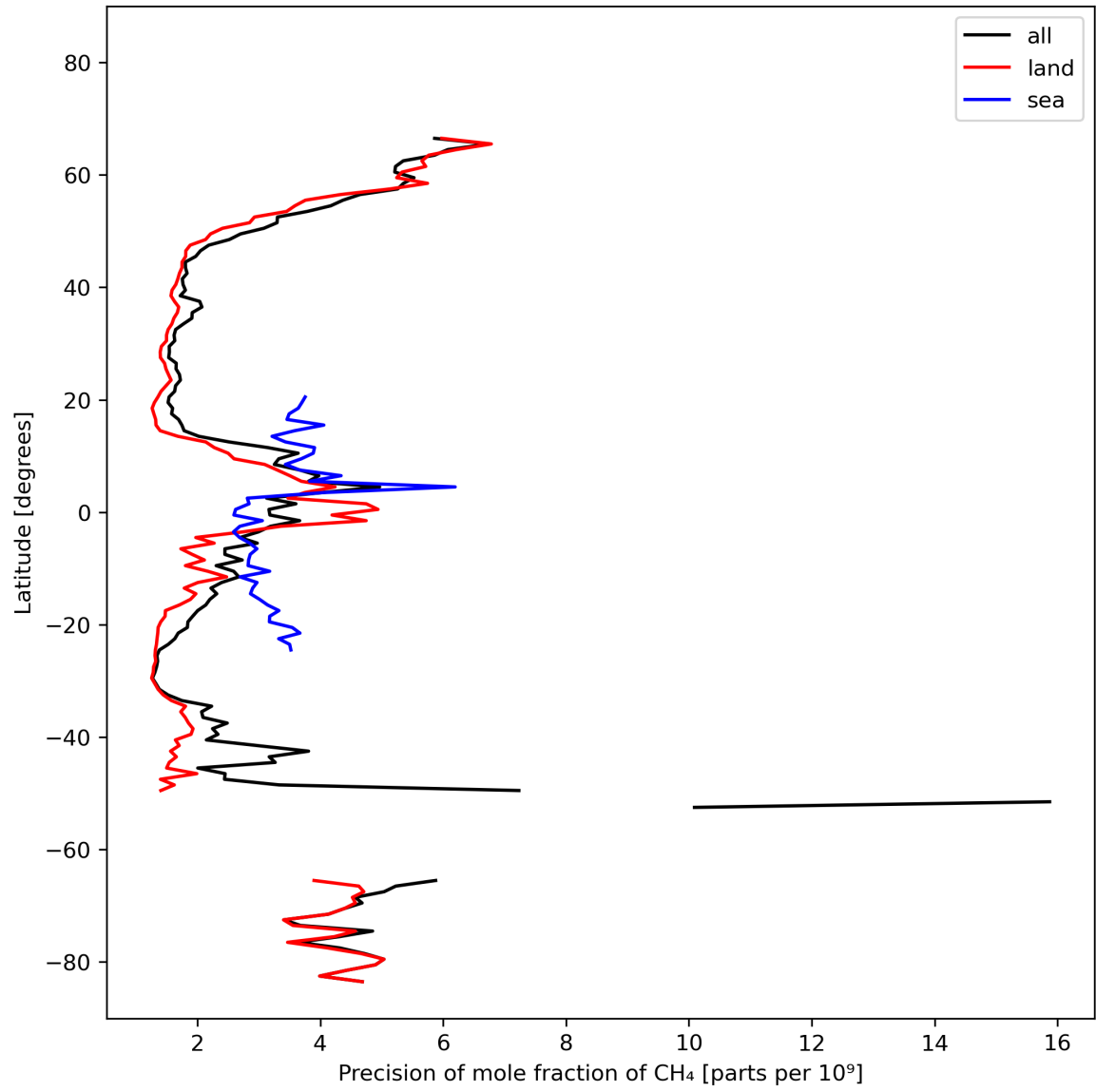
Figure 13: Zonal average of “Precision of mole fraction of \text{CH}_4 ” for 2023-10-15 to 2023-10-17.
