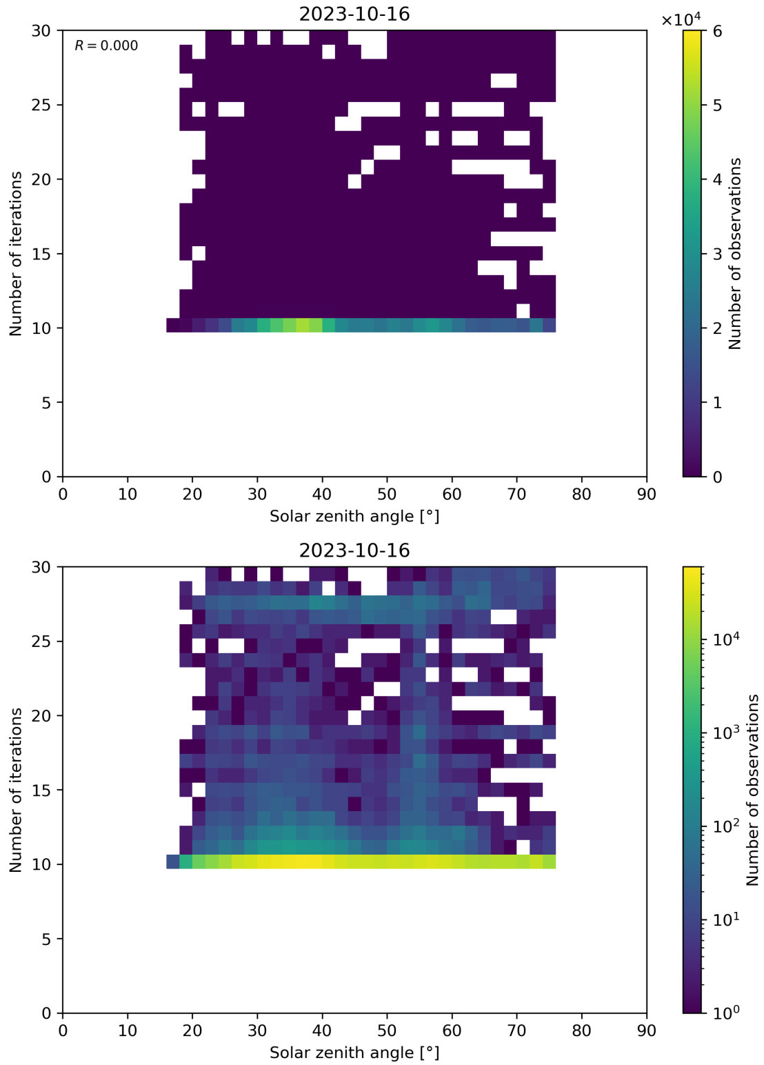
Figure 102: Scatter density plot of “Solar zenith angle” against “Number of iterations” for 2023-10-15 to 2023-10-17.
