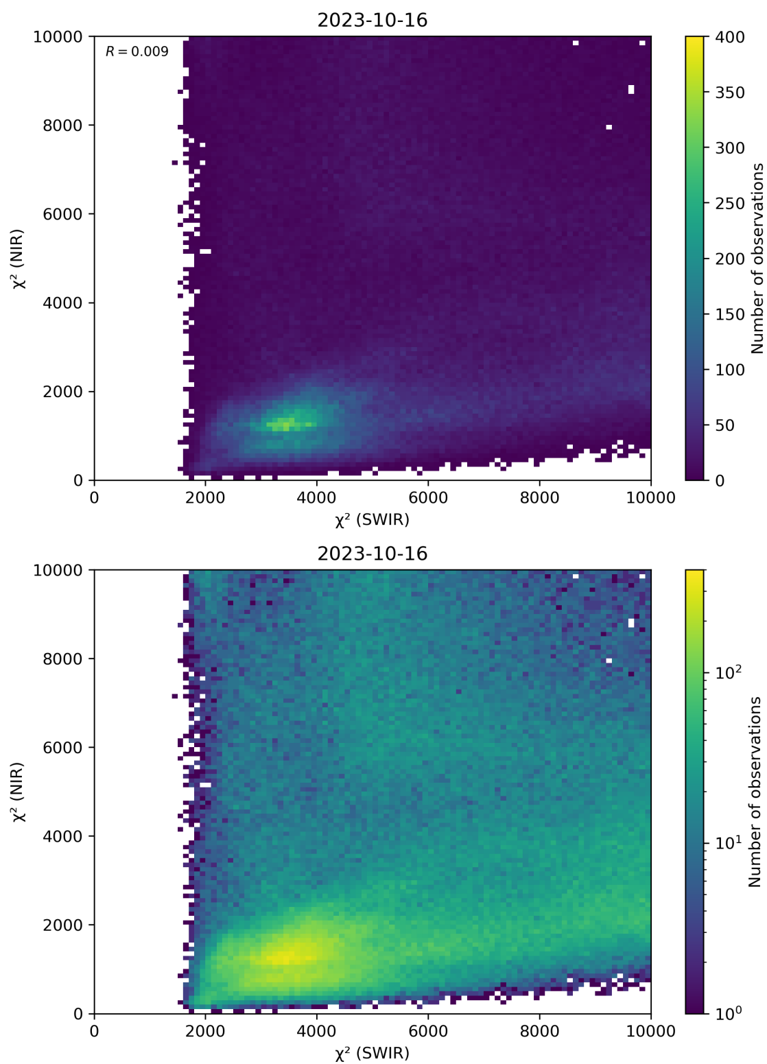
Figure 47: Scatter density plot of “ \chi^2 (SWIR)” against “ \chi^2 (NIR)” for 2023-10-15 to 2023-10-17.
