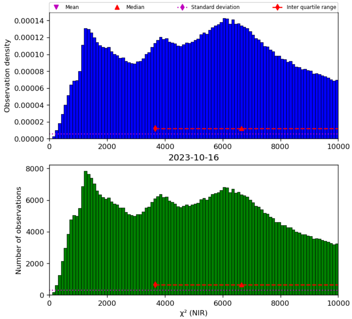
Figure 29: Histogram of “ \chi^2 (NIR)” for 2023-10-15 to 2023-10-17
