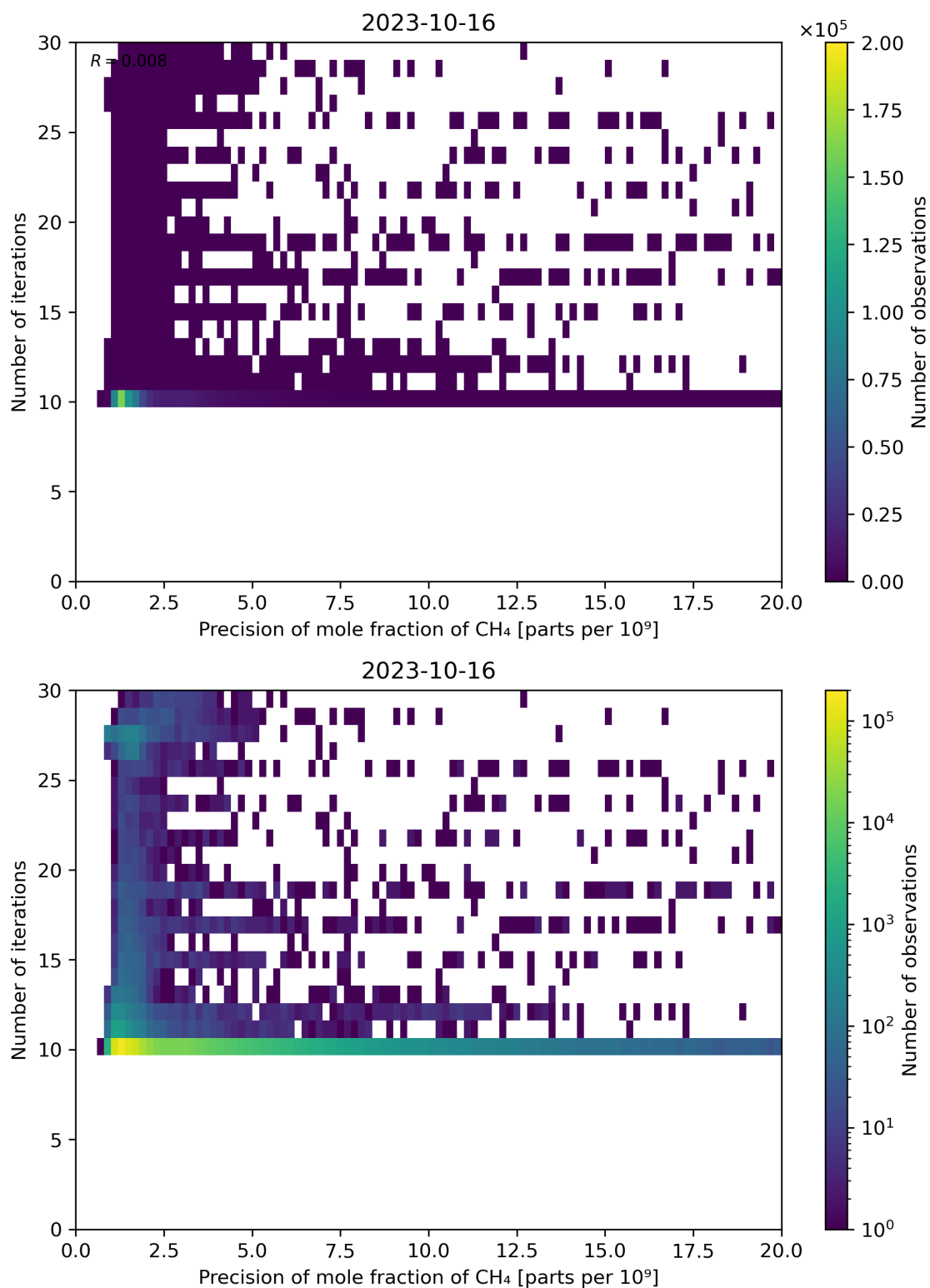
Figure 83: Scatter density plot of “Precision of mole fraction of CH 4 ” against “Number of iterations” for 2023-10-15 to 2023-10-17.
