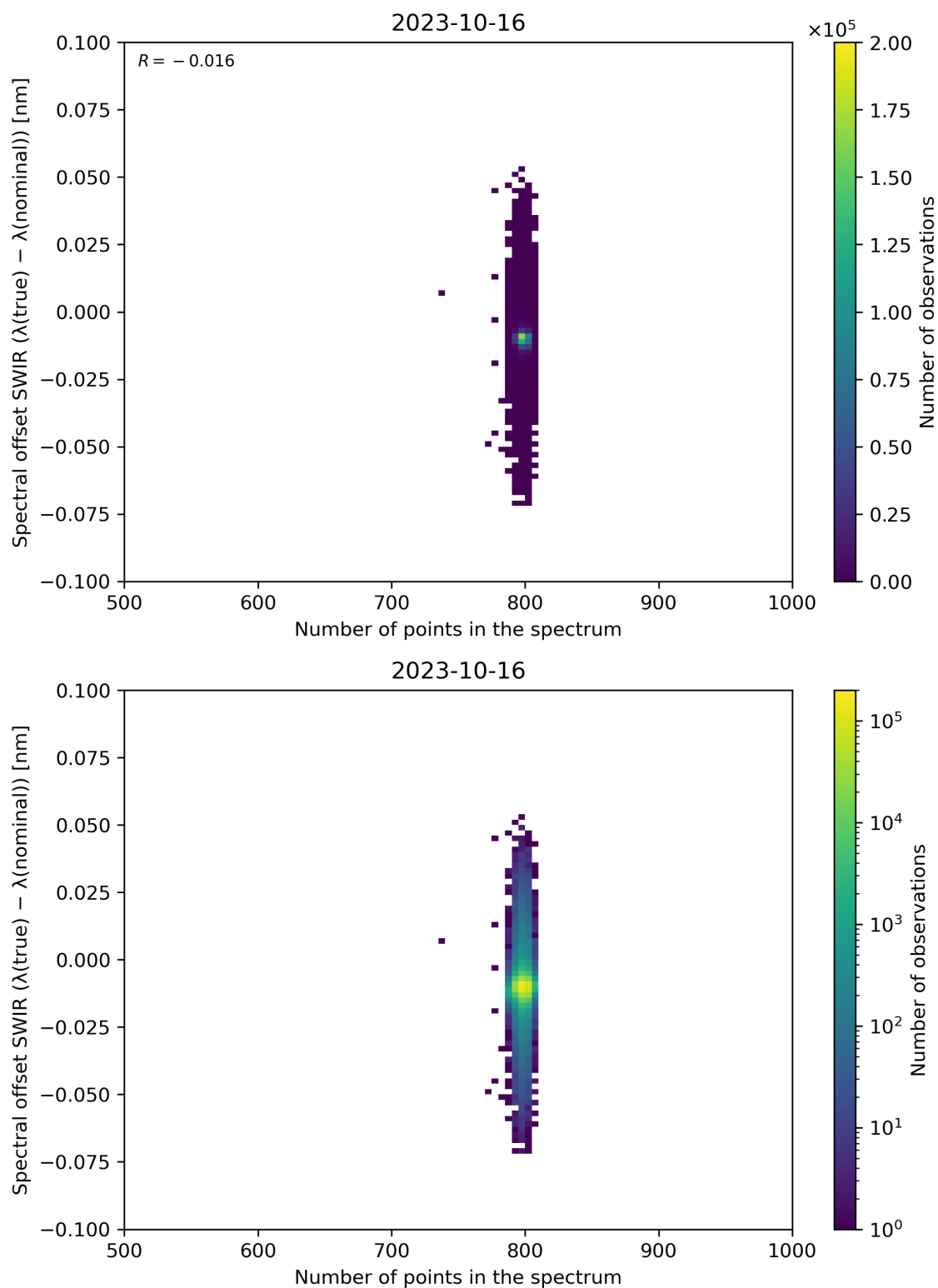
Figure 93: Scatter density plot of “Number of points in the spectrum” against “Spectral offset SWIR ( \lambda(\text{true}) - \lambda(\text{nominal}) )” for 2023-10-15 to 2023-10-17.
