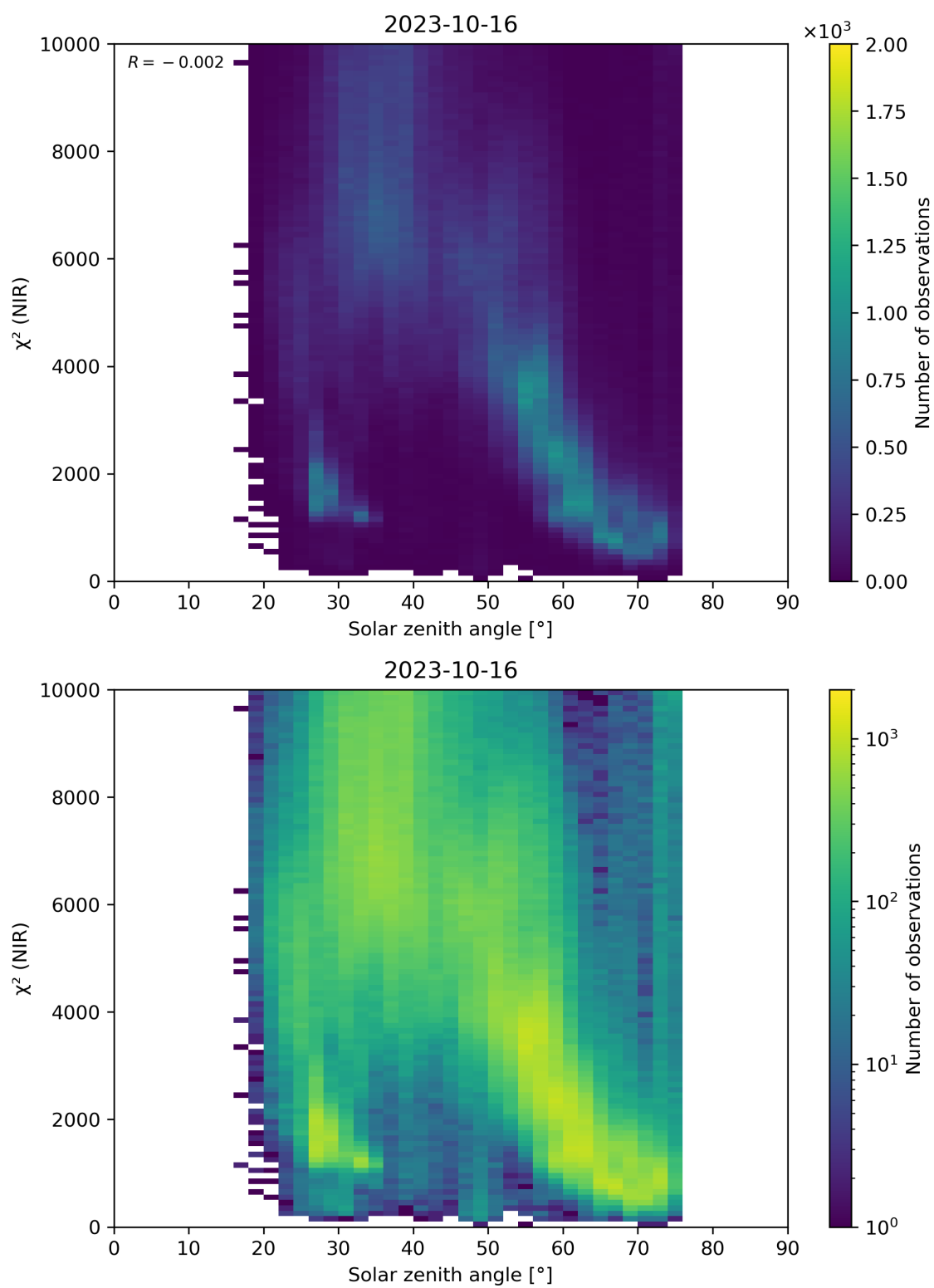
Figure 94: Scatter density plot of “Solar zenith angle” against “ \chi^2 (NIR)” for 2023-10-15 to 2023-10-17.
