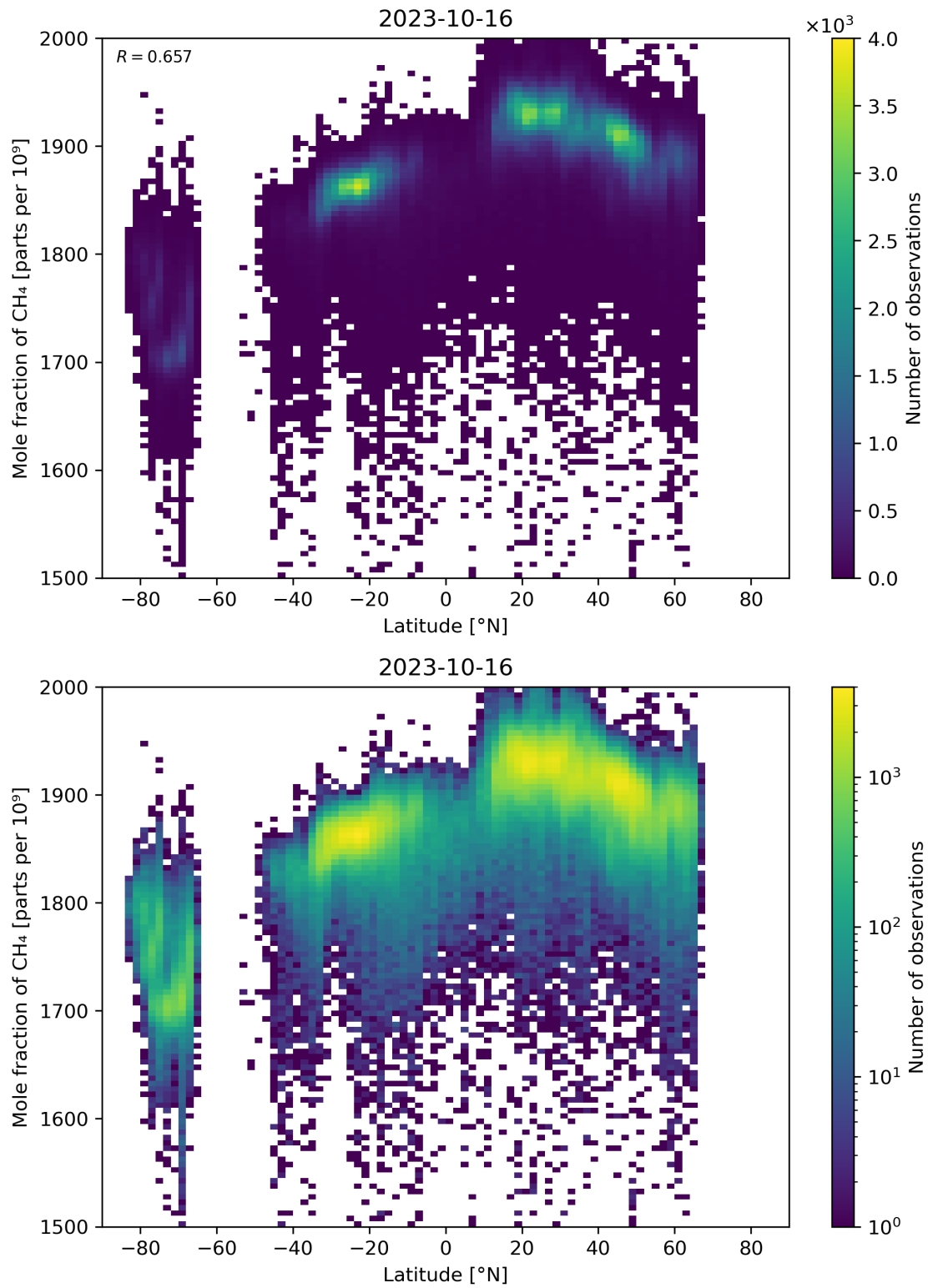
Figure 57: Scatter density plot of “Latitude” against “Mole fraction of \text{CH}_4 ” for 2023-10-15 to 2023-10-17.
