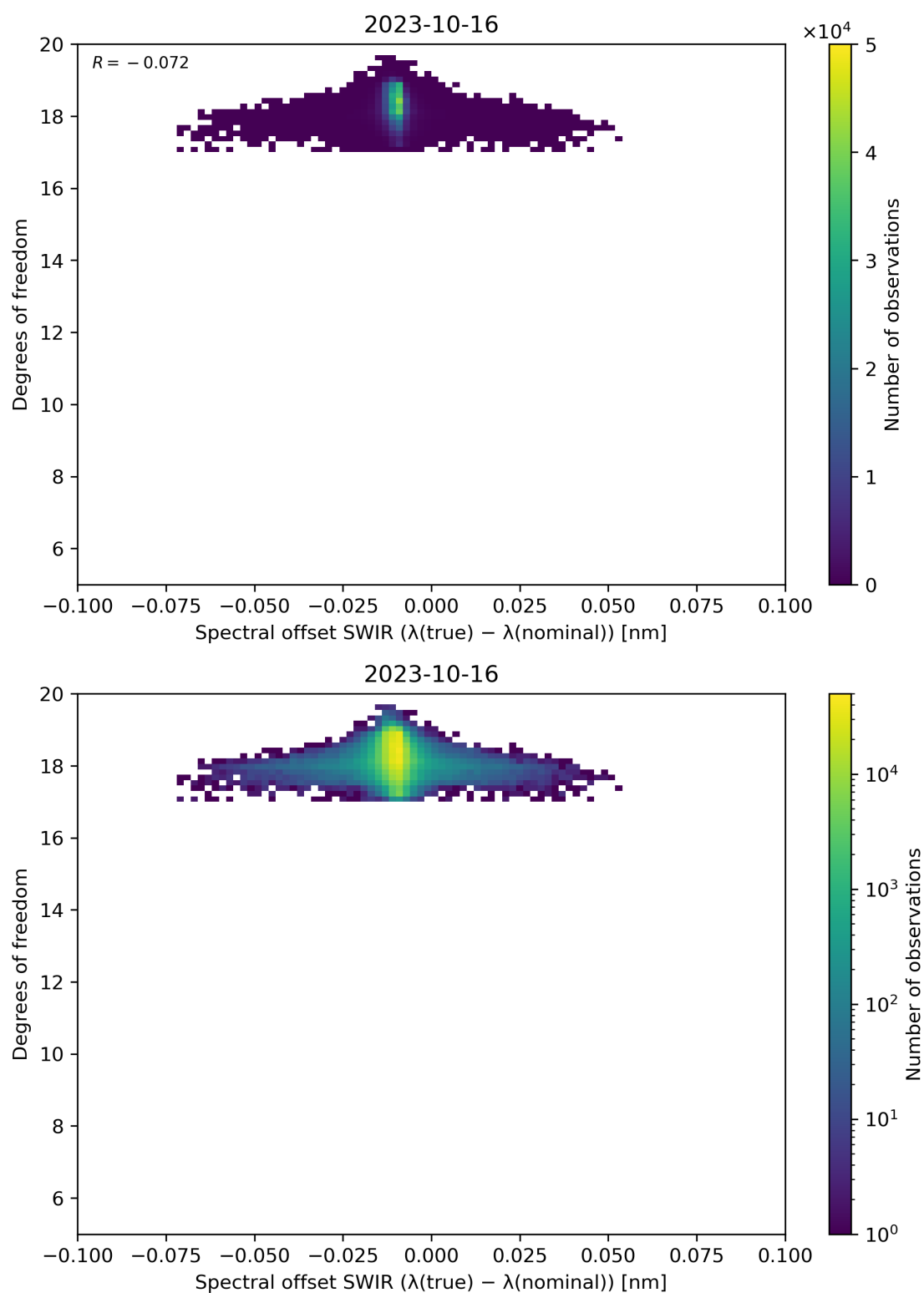
Figure 119: Scatter density plot of “Spectral offset SWIR ( \lambda(\text{true}) - \lambda(\text{nominal}) )” against “Degrees of freedom” for 2023-10-15 to 2023-10-17.
