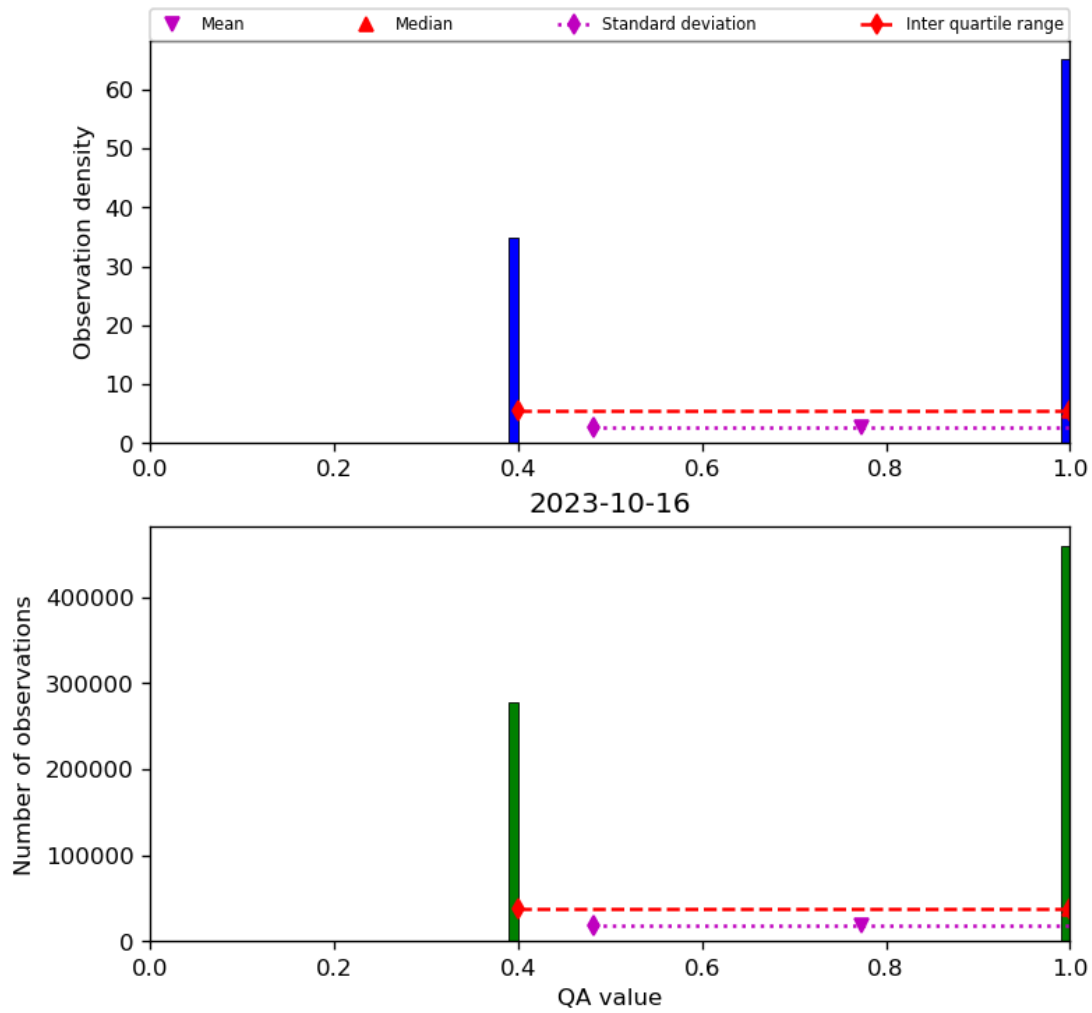
Figure 22: Histogram of “QA value” for 2023-10-15 to 2023-10-17
