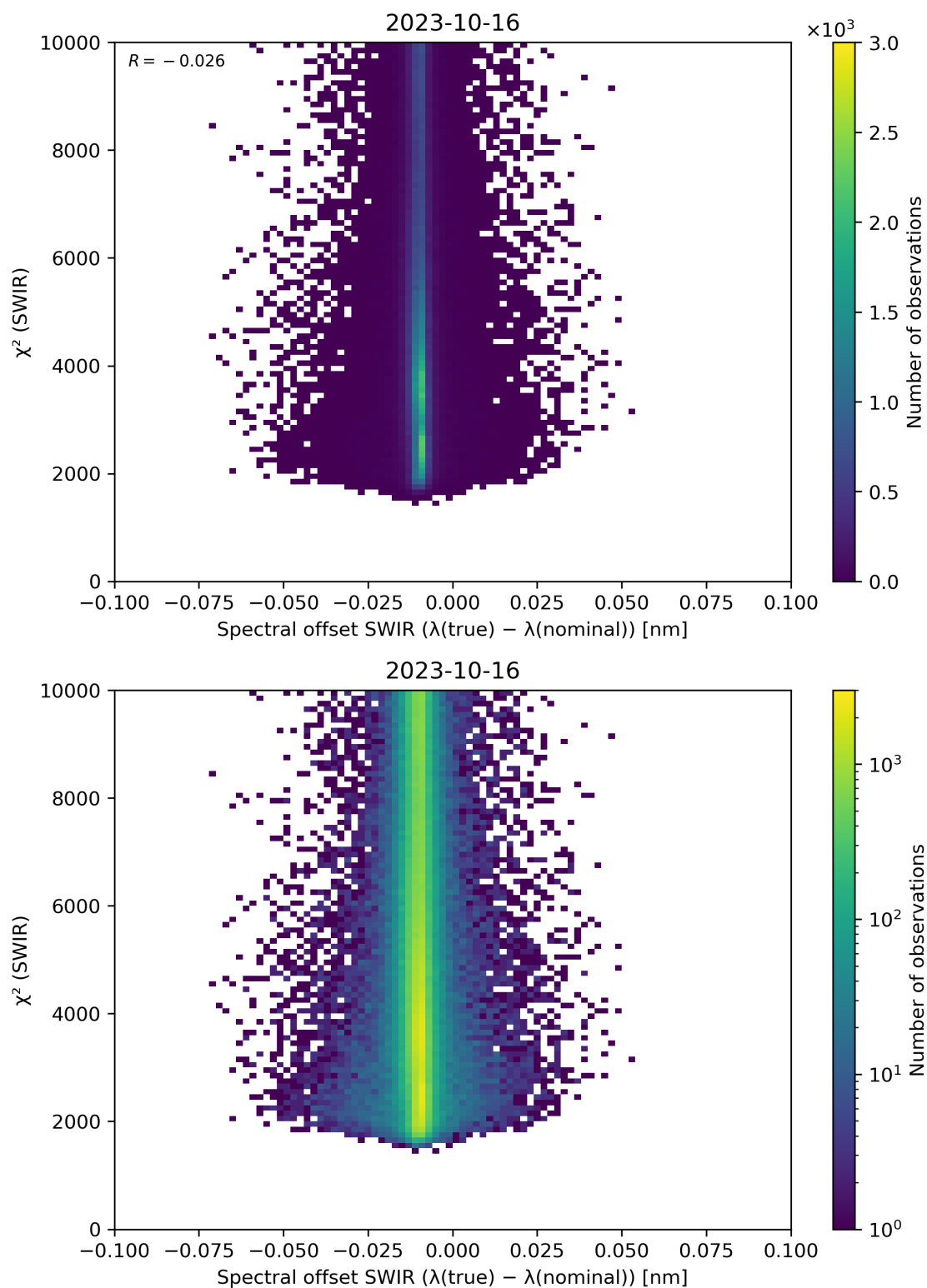
Figure 118: Scatter density plot of “Spectral offset SWIR ( \lambda(\text{true}) - \lambda(\text{nominal}) )” against “ \chi^2 (SWIR)” for 2023-10-15 to 2023-10-17.
