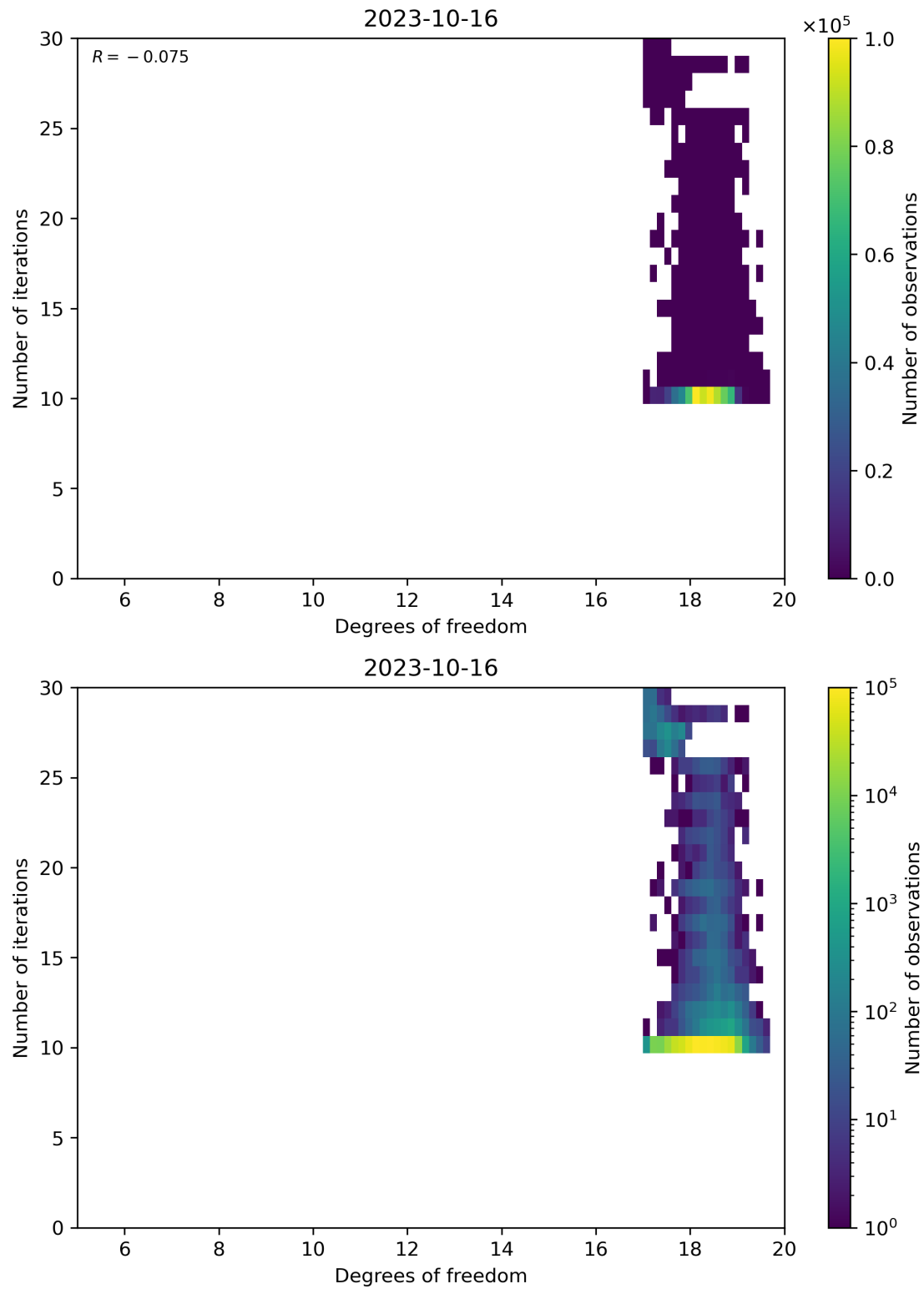
Figure 52: Scatter density plot of “Degrees of freedom” against “Number of iterations” for 2023-10-15 to 2023-10-17.
