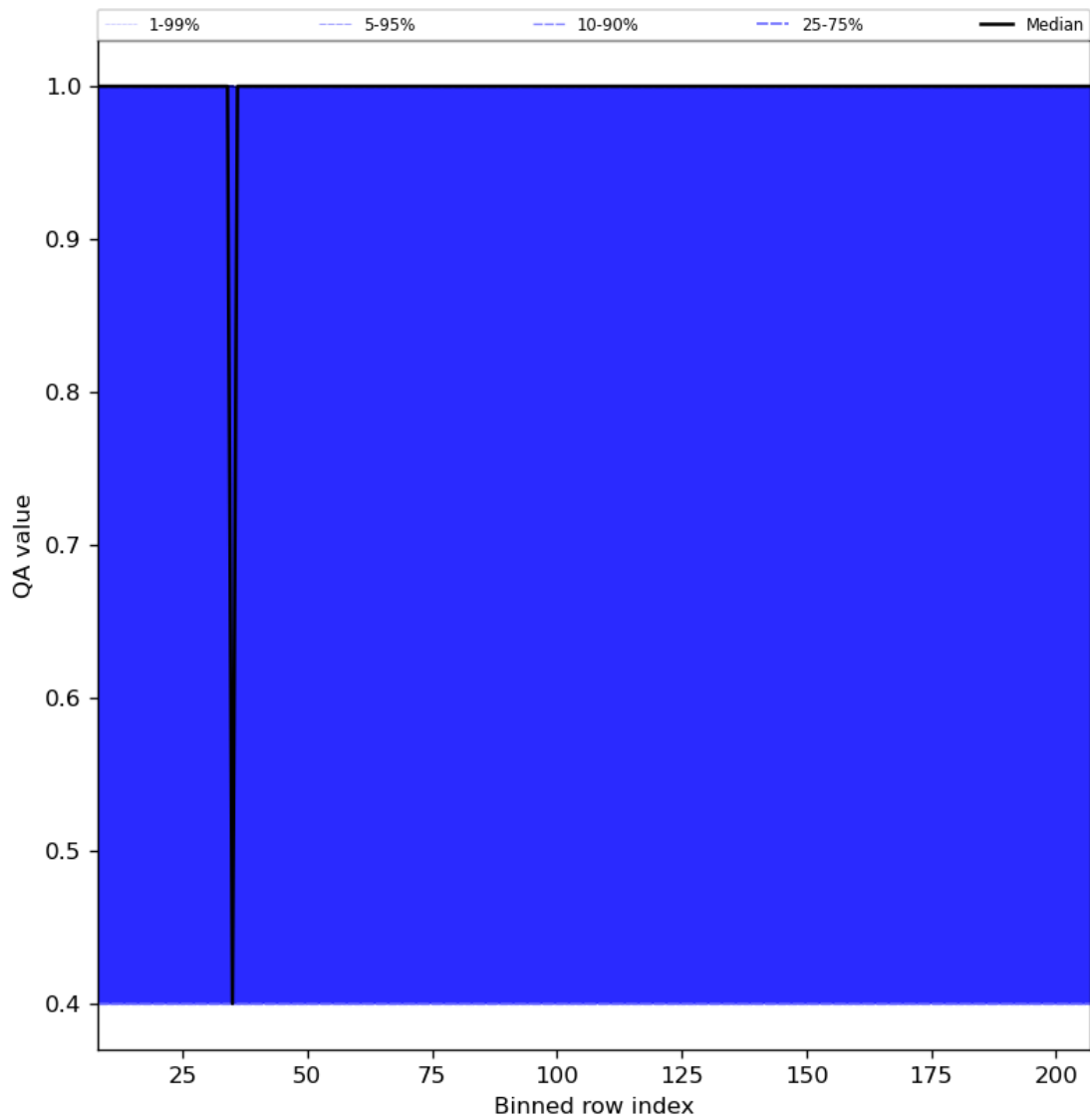
Figure 33: Along track statistics of “QA value” for 2023-10-15 to 2023-10-17
