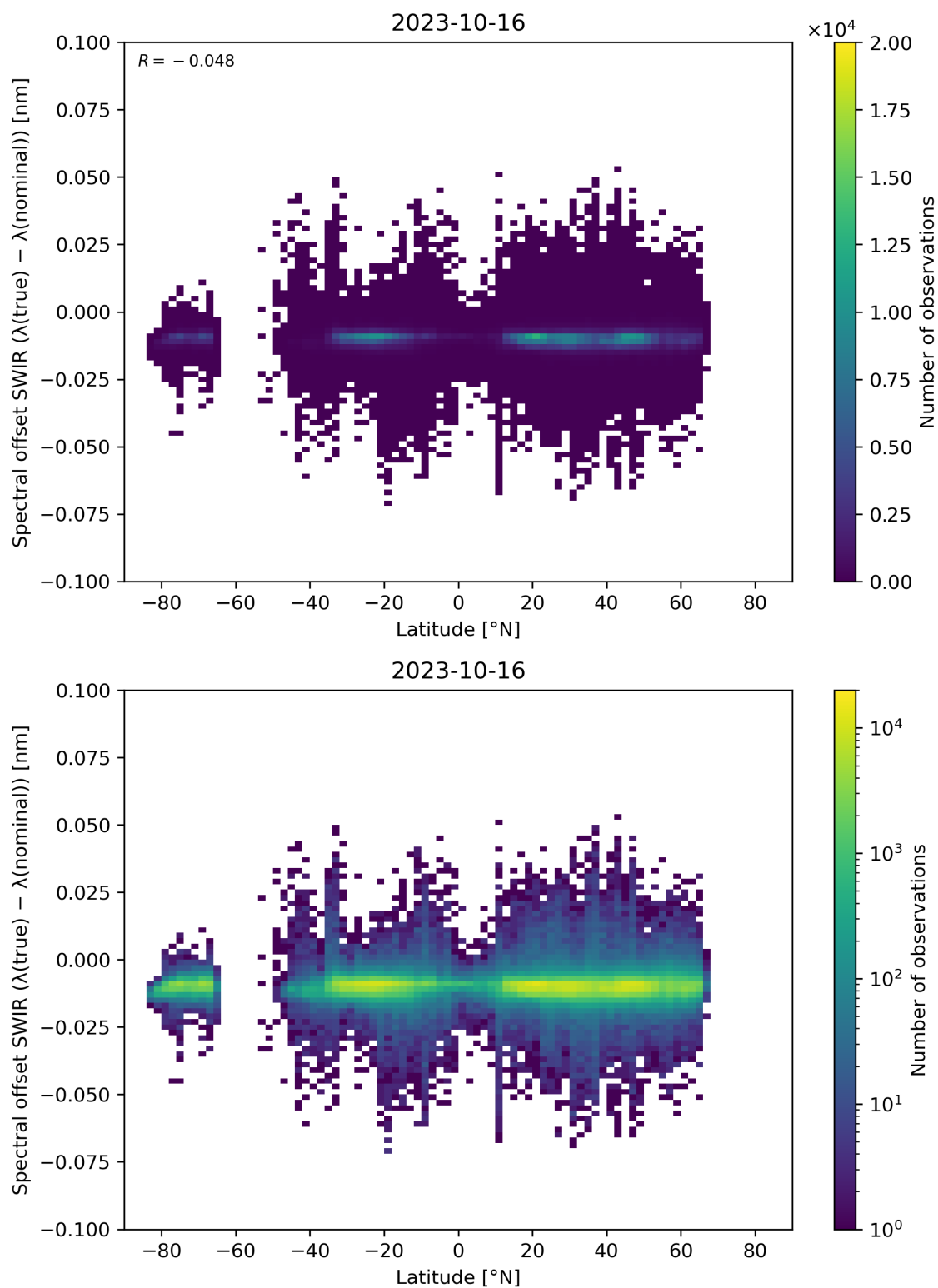
Figure 62: Scatter density plot of “Latitude” against “Spectral offset SWIR ( \lambda(\text{true}) - \lambda(\text{nominal}) )” for 2023-10-15 to 2023-10-17.
