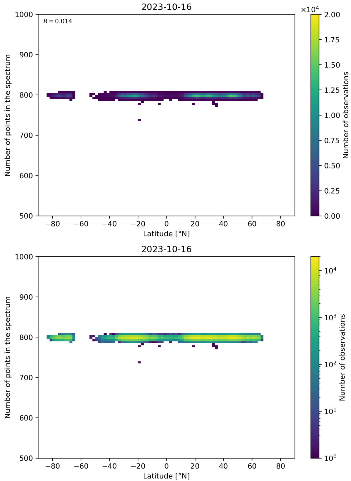
Figure 61: Scatter density plot of “Latitude” against “Number of points in the spectrum” for 2023-10-15 to 2023-10-17.
