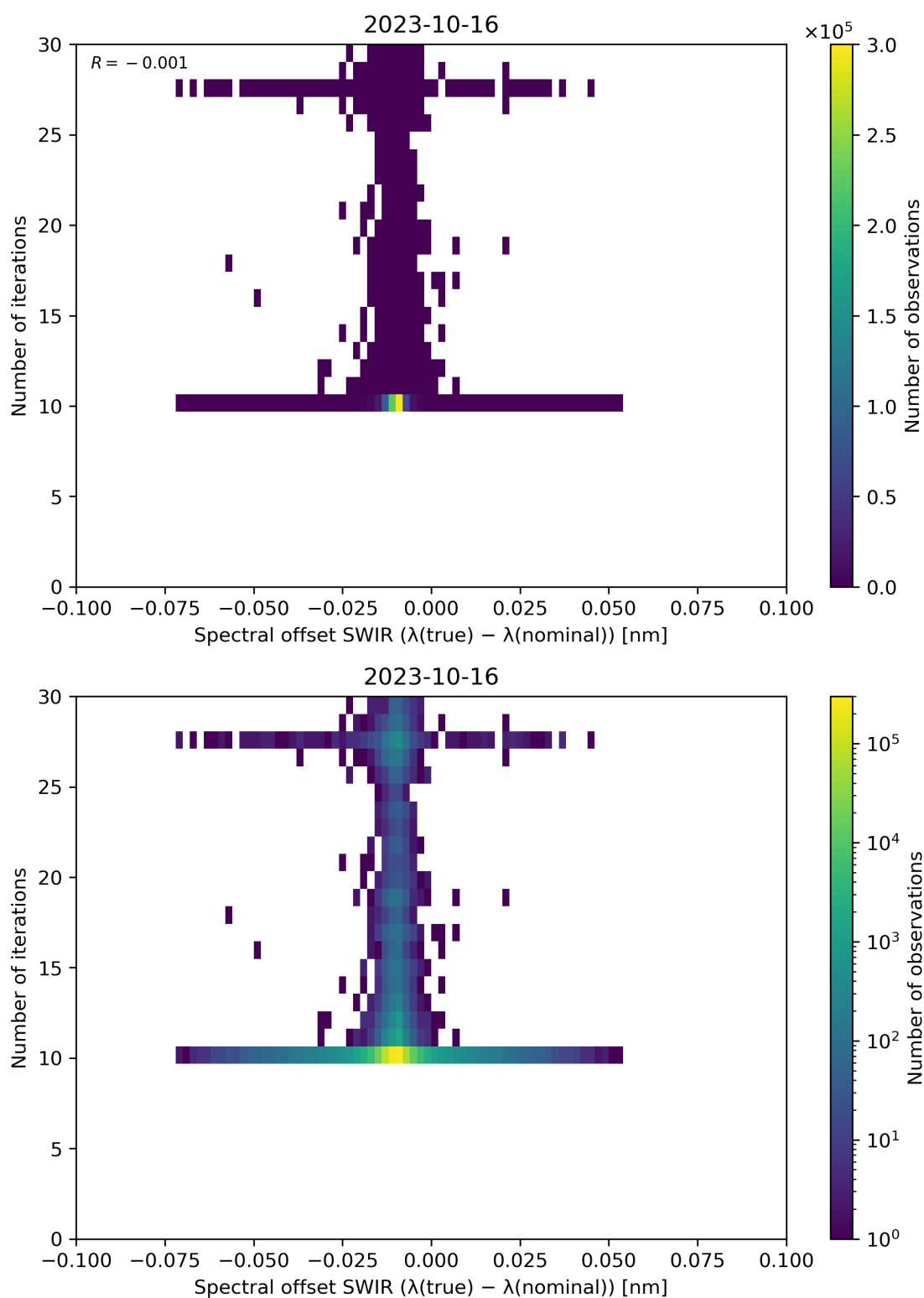
Figure 121: Scatter density plot of “Spectral offset SWIR ( \lambda(\text{true}) - \lambda(\text{nominal}) )” against “Number of iterations” for 2023-10-15 to 2023-10-17.
