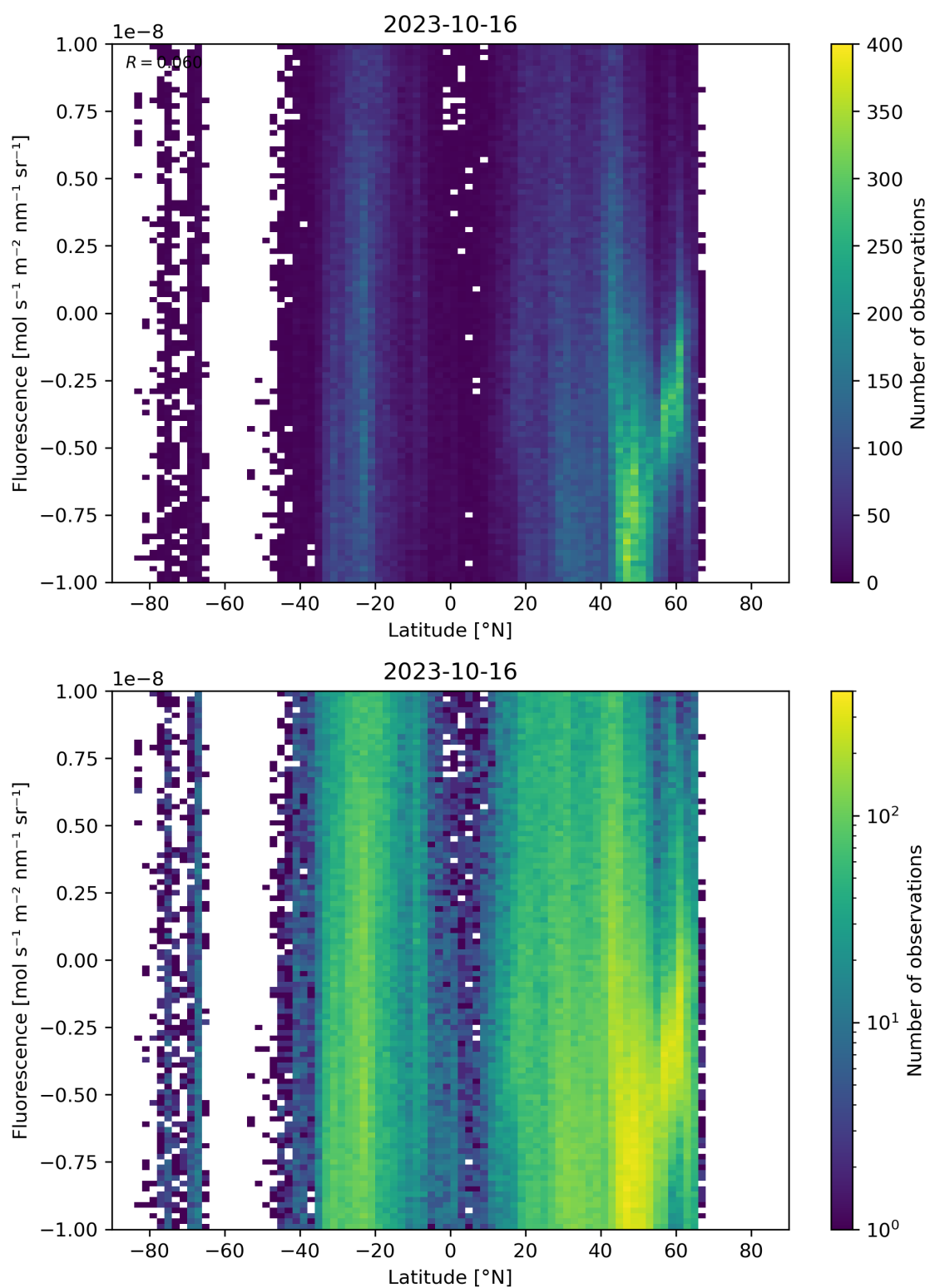
Figure 56: Scatter density plot of “Latitude” against “Fluorescence” for 2023-10-15 to 2023-10-17.
