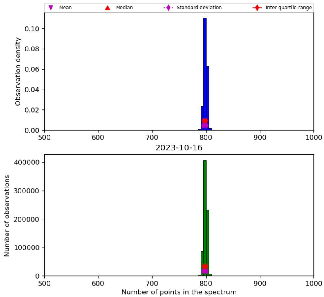
Figure 26: Histogram of “Number of points in the spectrum” for 2023-10-15 to 2023-10-17
