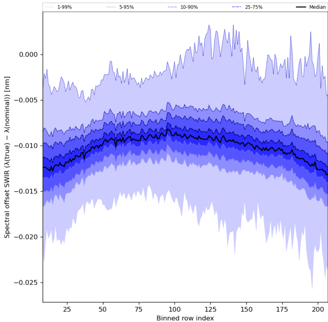
Figure 38: Along track statistics of “Spectral offset SWIR ( \lambda(\text{true}) - \lambda(\text{nominal}) )” for 2023-10-15 to 2023-10-17
