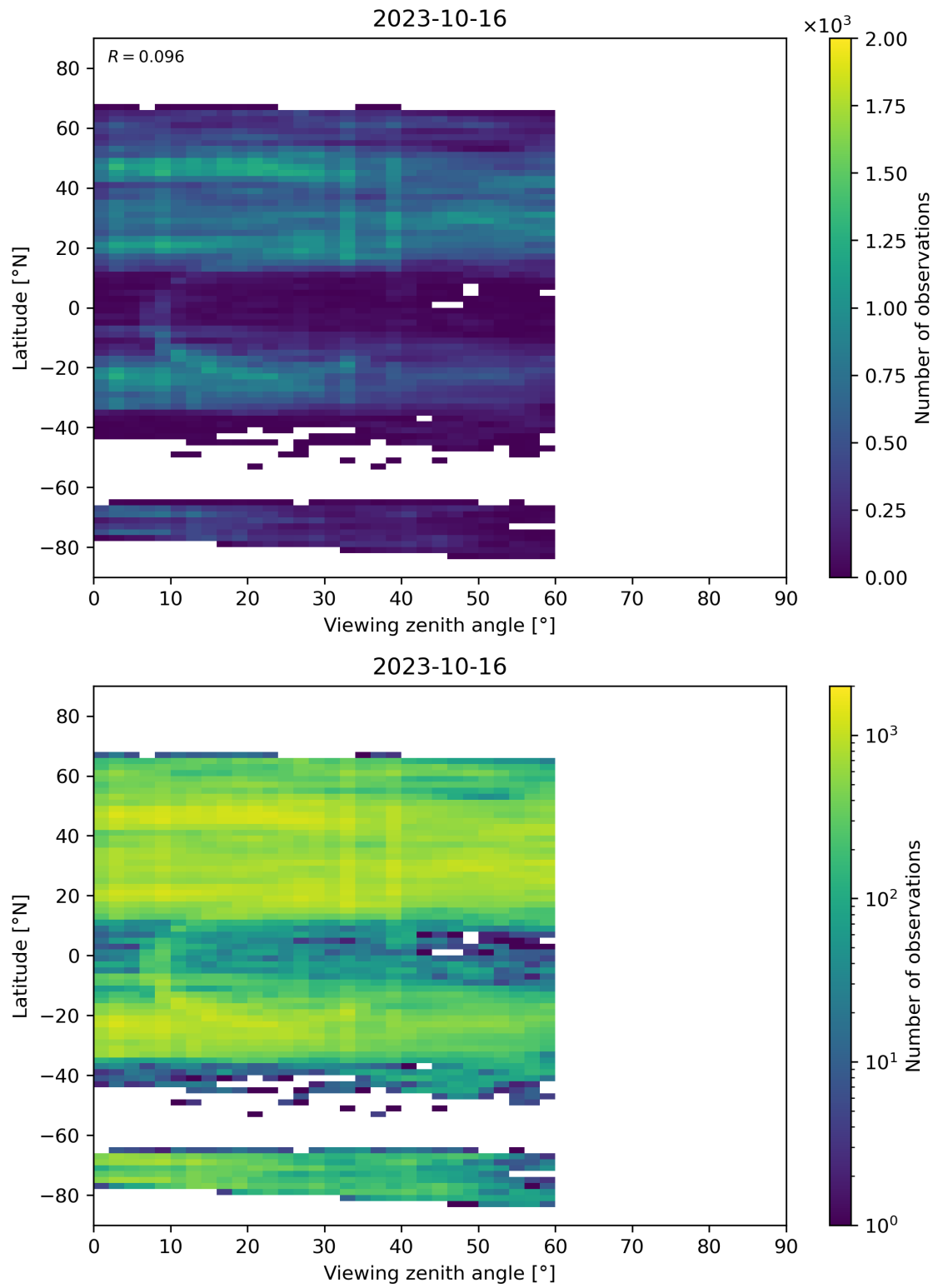
Figure 109: Scatter density plot of “Viewing zenith angle” against “Latitude” for 2023-10-15 to 2023-10-17.
