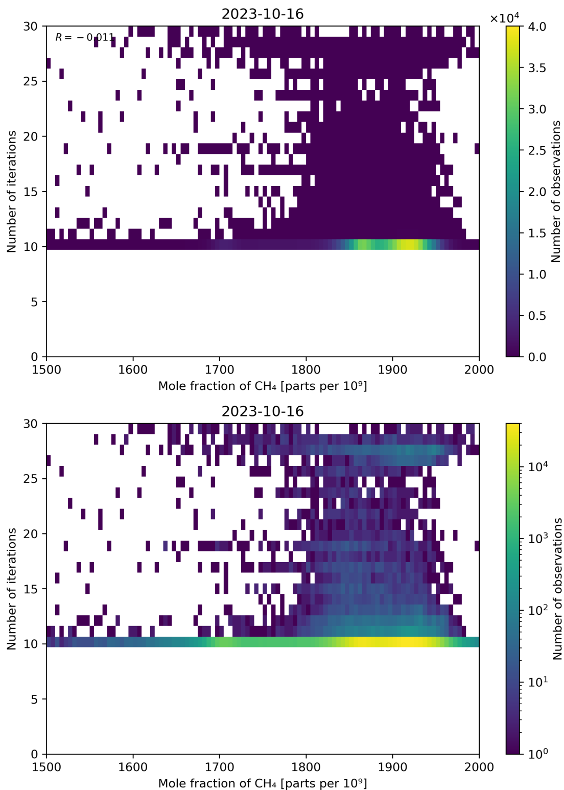
Figure 76: Scatter density plot of “Mole fraction of CH 4 ” against “Number of iterations” for 2023-10-15 to 2023-10-17.
