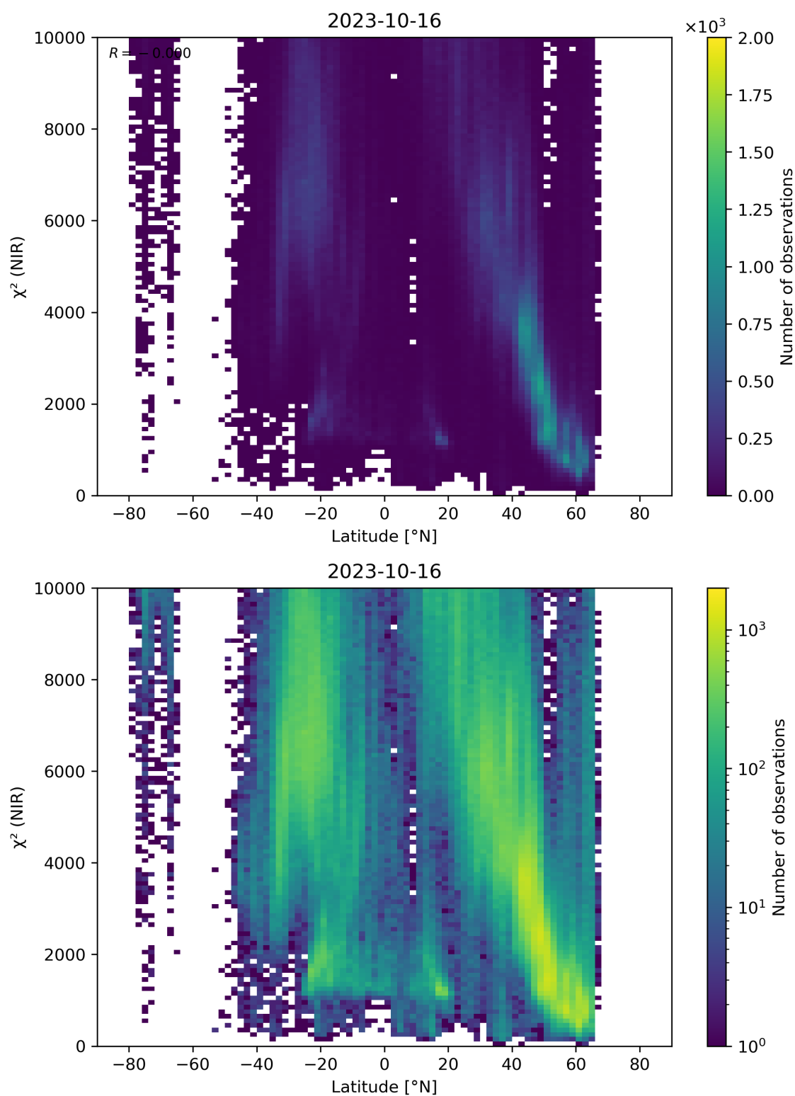
Figure 53: Scatter density plot of “Latitude” against “ \chi^2 (NIR)” for 2023-10-15 to 2023-10-17.
