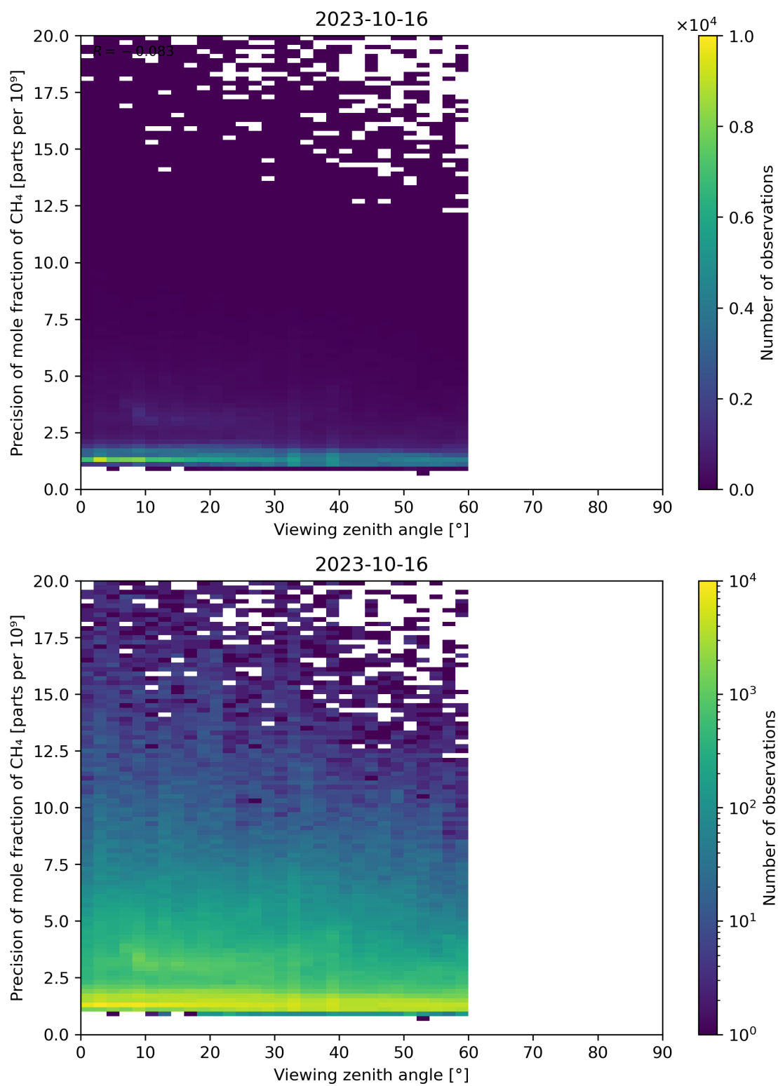
Figure 112: Scatter density plot of “Viewing zenith angle” against “Precision of mole fraction of CH 4 ” for 2023-10-15 to 2023-10-17.
