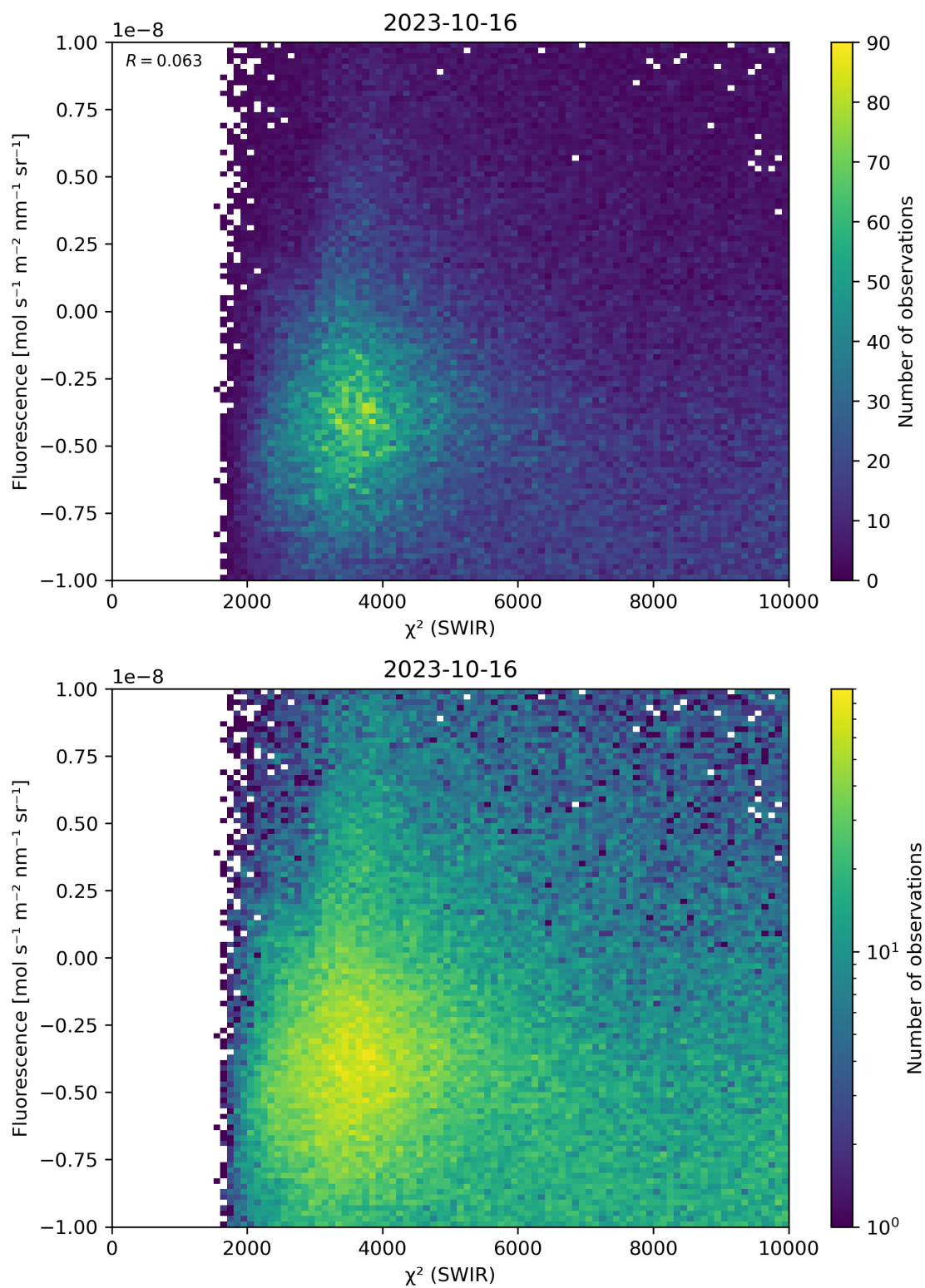
Figure 49: Scatter density plot of “ \chi^2 (SWIR)” against “Fluorescence” for 2023-10-15 to 2023-10-17.
