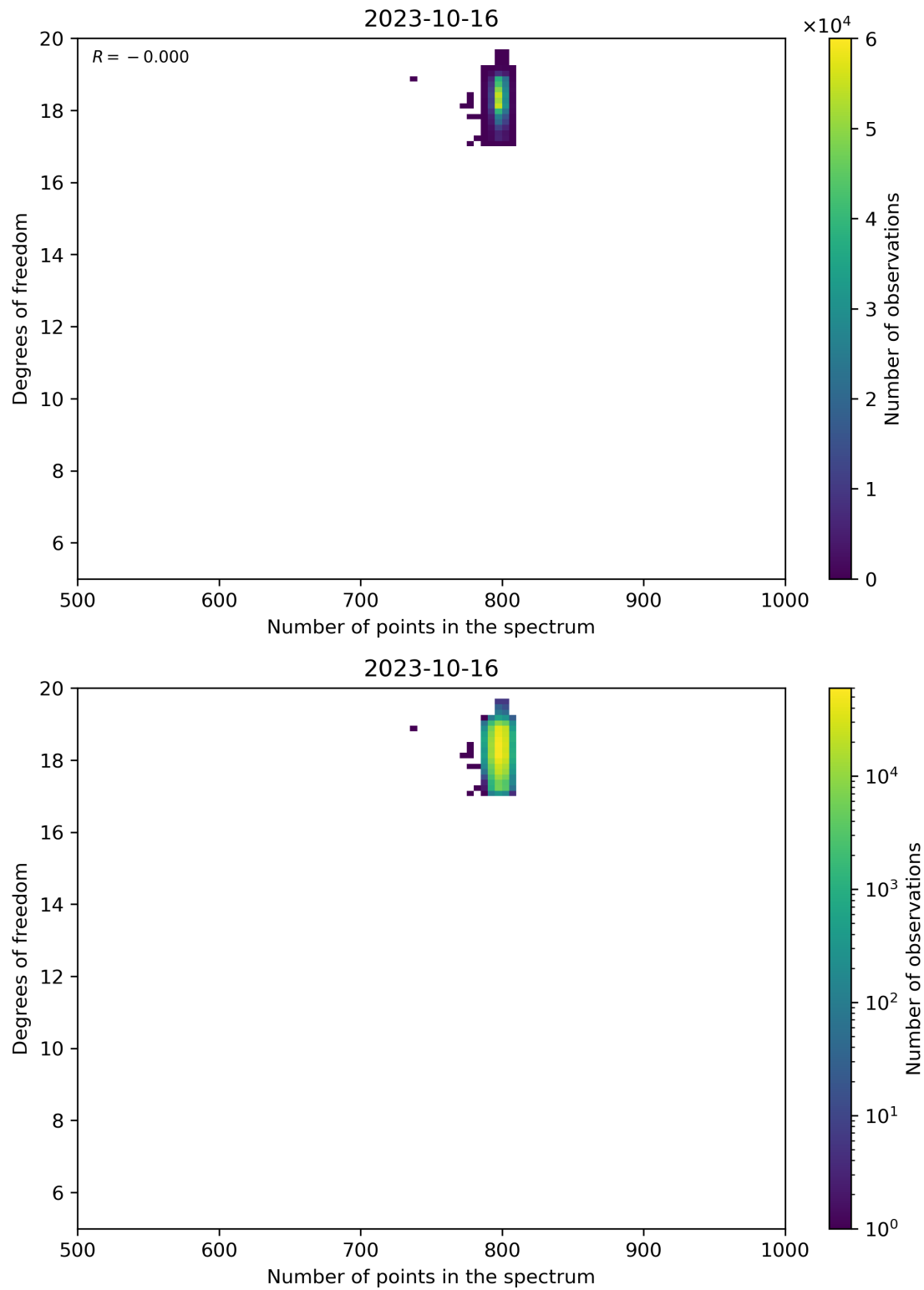
Figure 90: Scatter density plot of “Number of points in the spectrum” against “Degrees of freedom” for 2023-10-15 to 2023-10-17.
