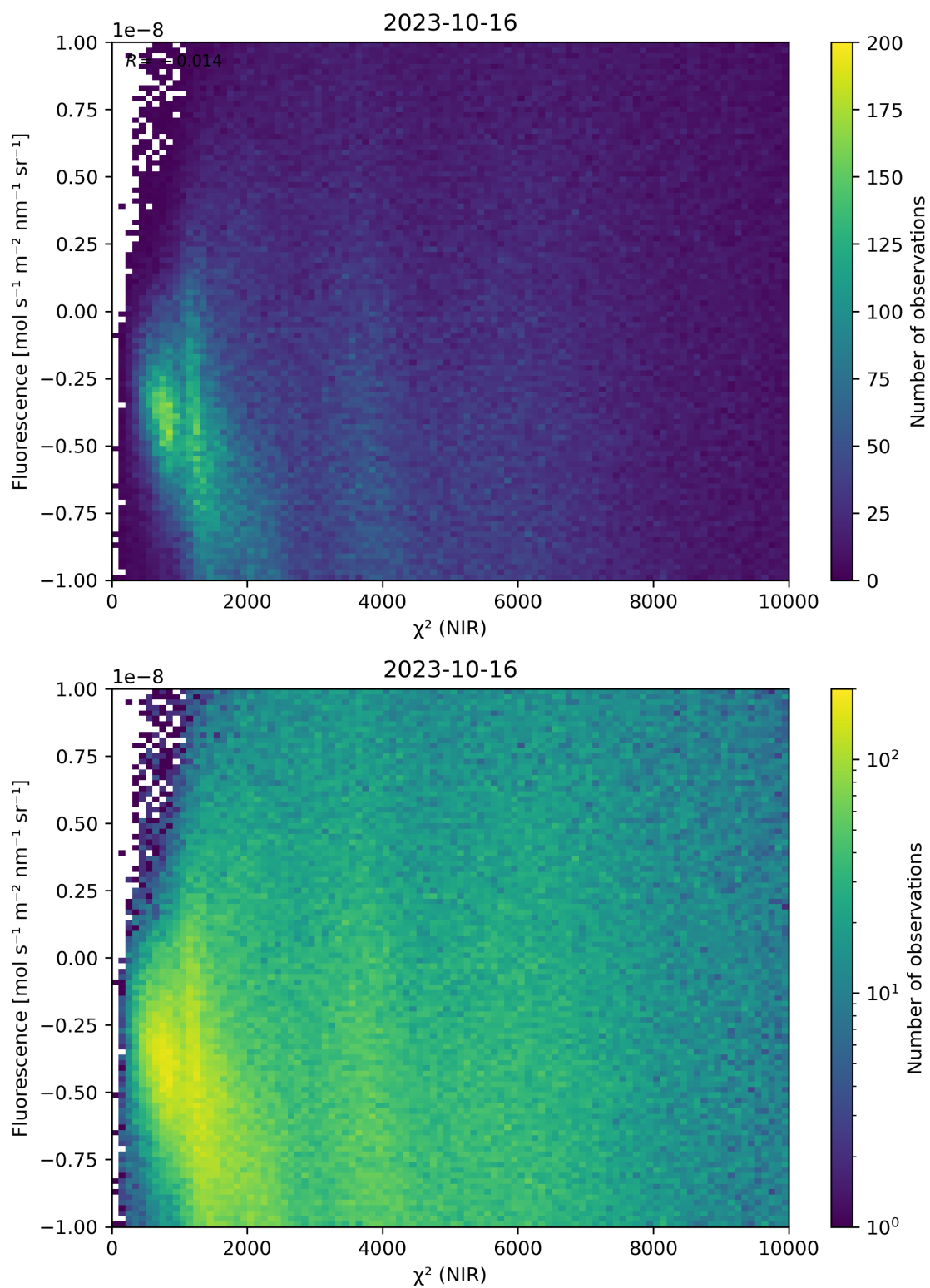
Figure 45: Scatter density plot of “ \chi^2 (NIR)” against “Fluorescence” for 2023-10-15 to 2023-10-17.
