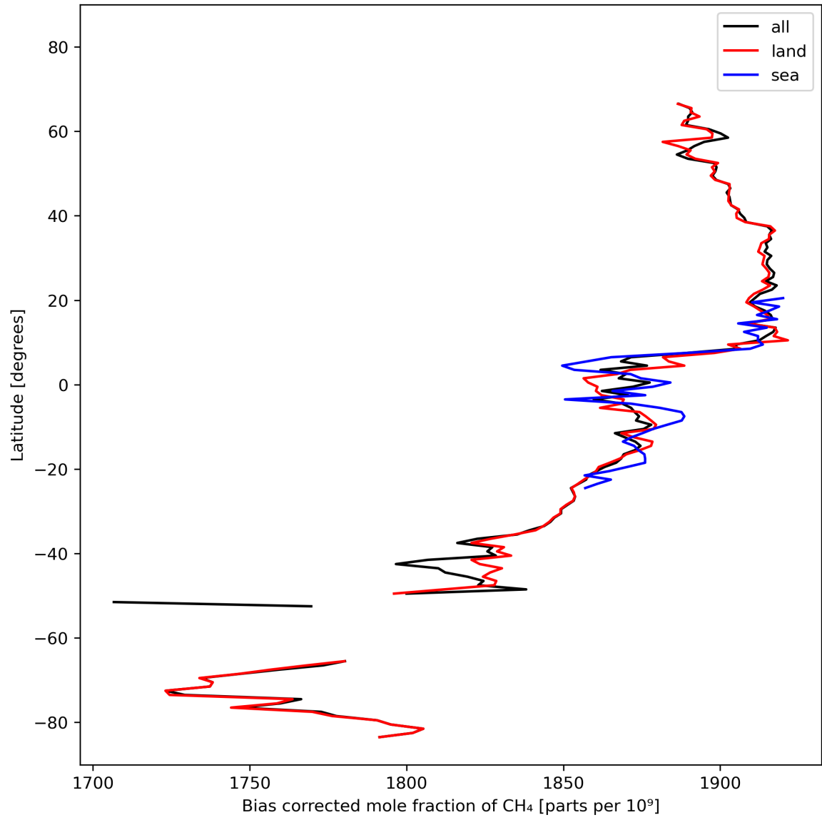
Figure 14: Zonal average of “Bias corrected mole fraction of CH 4 ” for 2023-10-15 to 2023-10-17.
