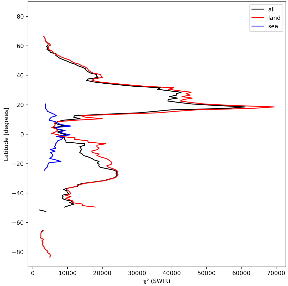
Figure 17: Zonal average of “ \chi^2 (SWIR)” for 2023-10-15 to 2023-10-17.
