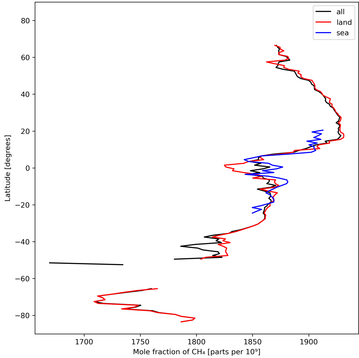
Figure 12: Zonal average of “Mole fraction of \text{CH}_4 ” for 2023-10-15 to 2023-10-17.
