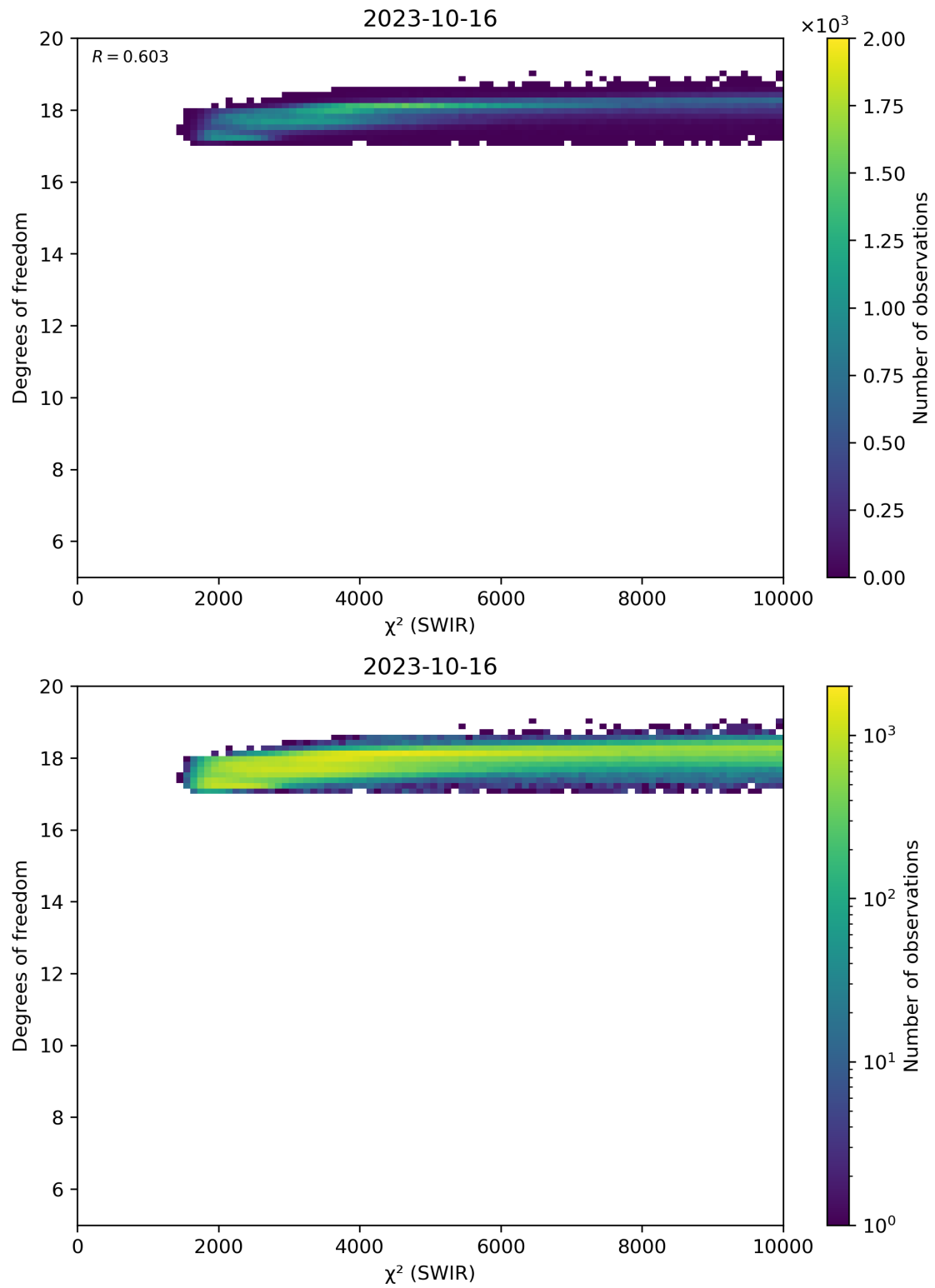
Figure 48: Scatter density plot of “ \chi^2 (SWIR)” against “Degrees of freedom” for 2023-10-15 to 2023-10-17.
