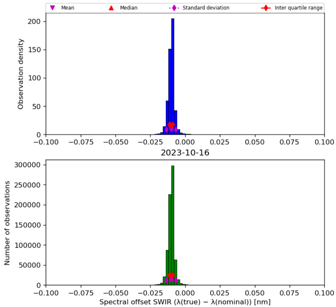
Figure 27: Histogram of “Spectral offset SWIR ( \lambda(\text{true}) - \lambda(\text{nominal}) )” for 2023-10-15 to 2023-10-17
