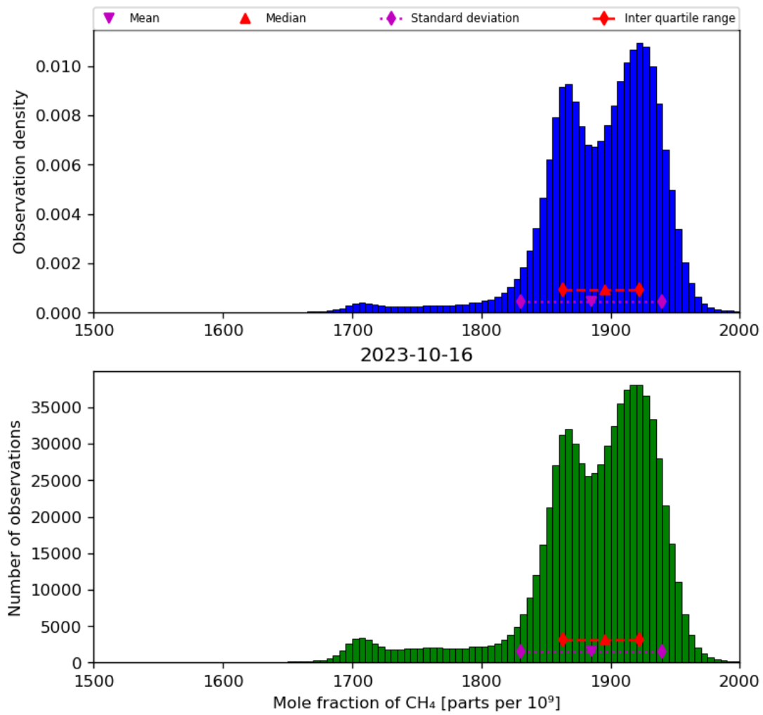
Figure 23: Histogram of "Mole fraction of CH 4 " for 2023-10-15 to 2023-10-17
