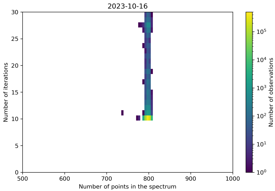
Figure 92: Scatter density plot of “Number of points in the spectrum” against “Number of iterations” for 2023-10-15 to 2023-10-17.
