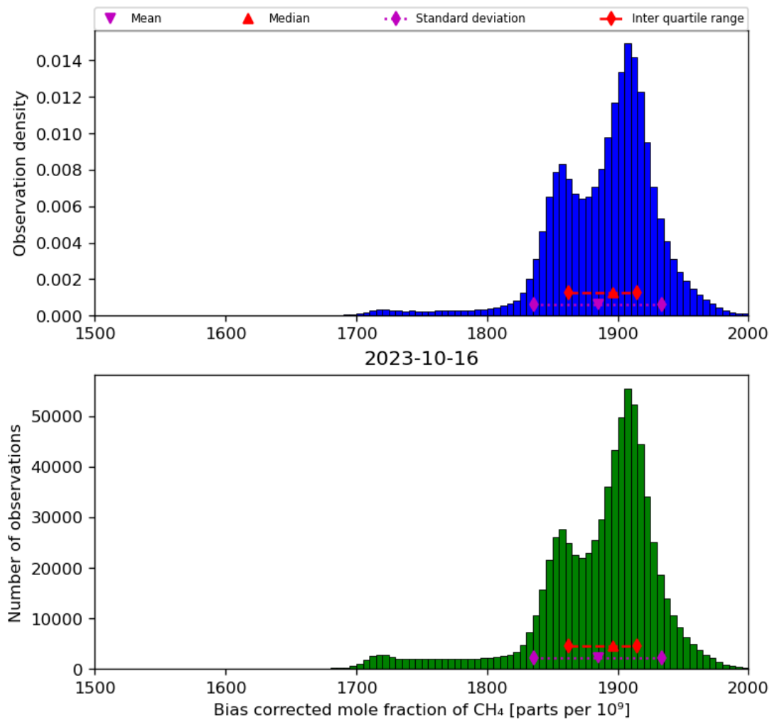
Figure 25: Histogram of “Bias corrected mole fraction of CH 4 ” for 2023-10-15 to 2023-10-17
