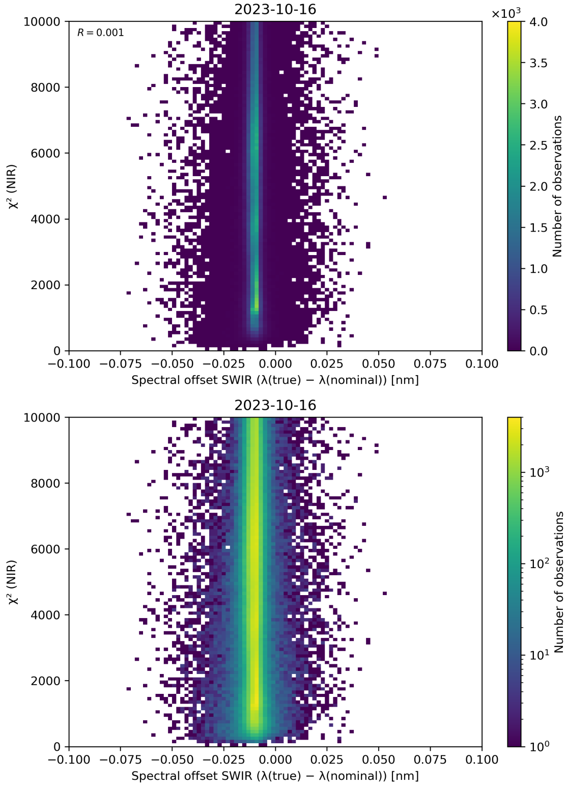
Figure 117: Scatter density plot of “Spectral offset SWIR ( \lambda(\text{true}) - \lambda(\text{nominal}) )” against “ \chi^2 (NIR)” for 2023-10-15 to 2023-10-17.
