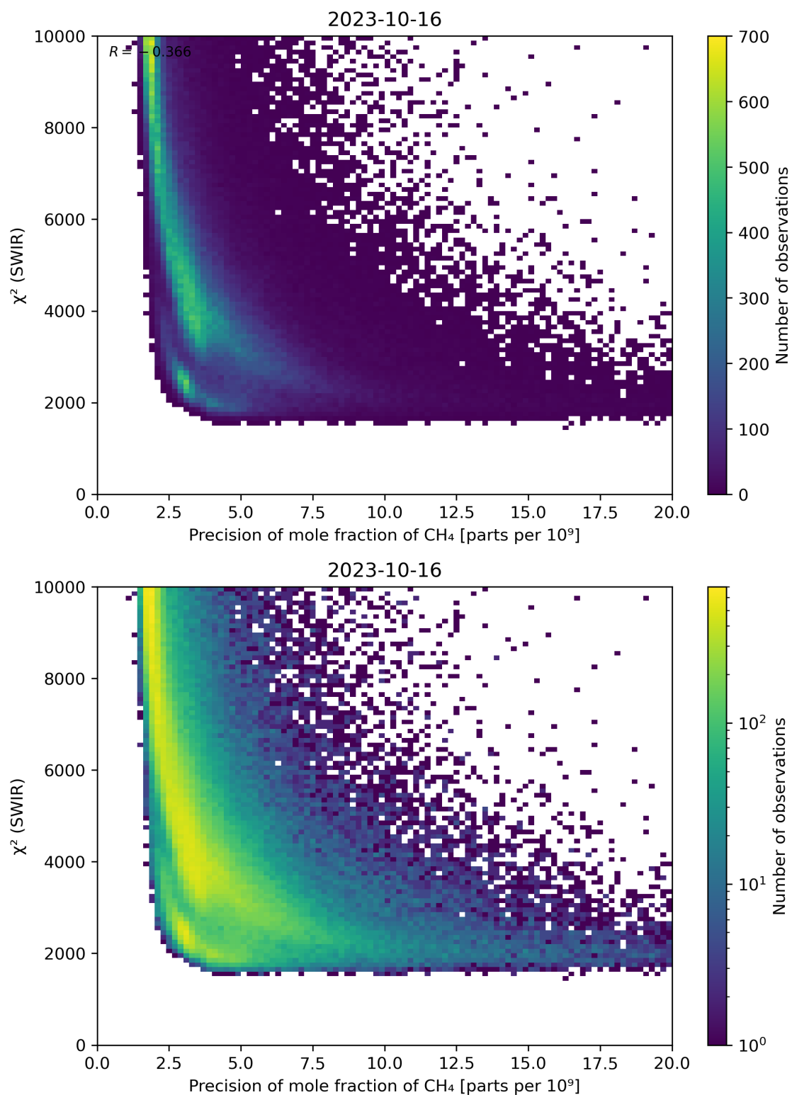
Figure 79: Scatter density plot of “Precision of mole fraction of \text{CH}_4 ” against “ \chi^2 (SWIR)” for 2023-10-15 to 2023-10-17.
