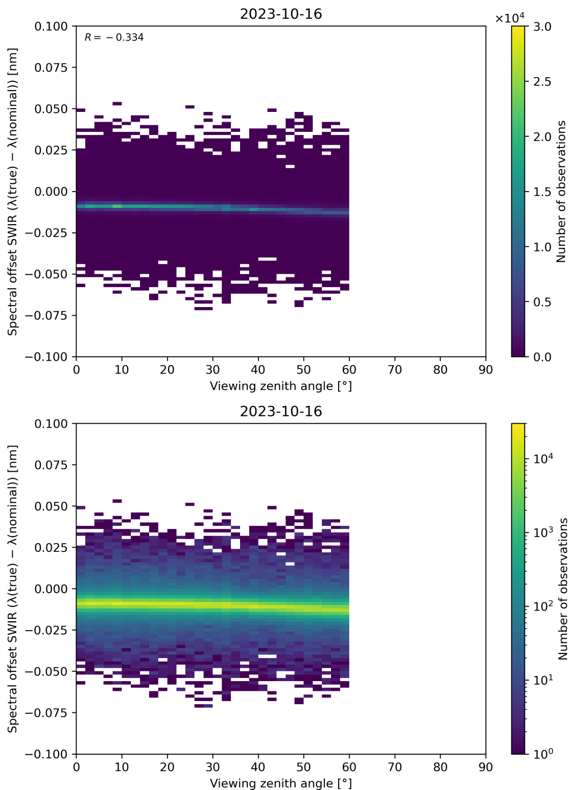
Figure 116: Scatter density plot of “Viewing zenith angle” against “Spectral offset SWIR ( \lambda(\text{true}) - \lambda(\text{nominal}) )” for 2023-10-15 to 2023-10-17.
