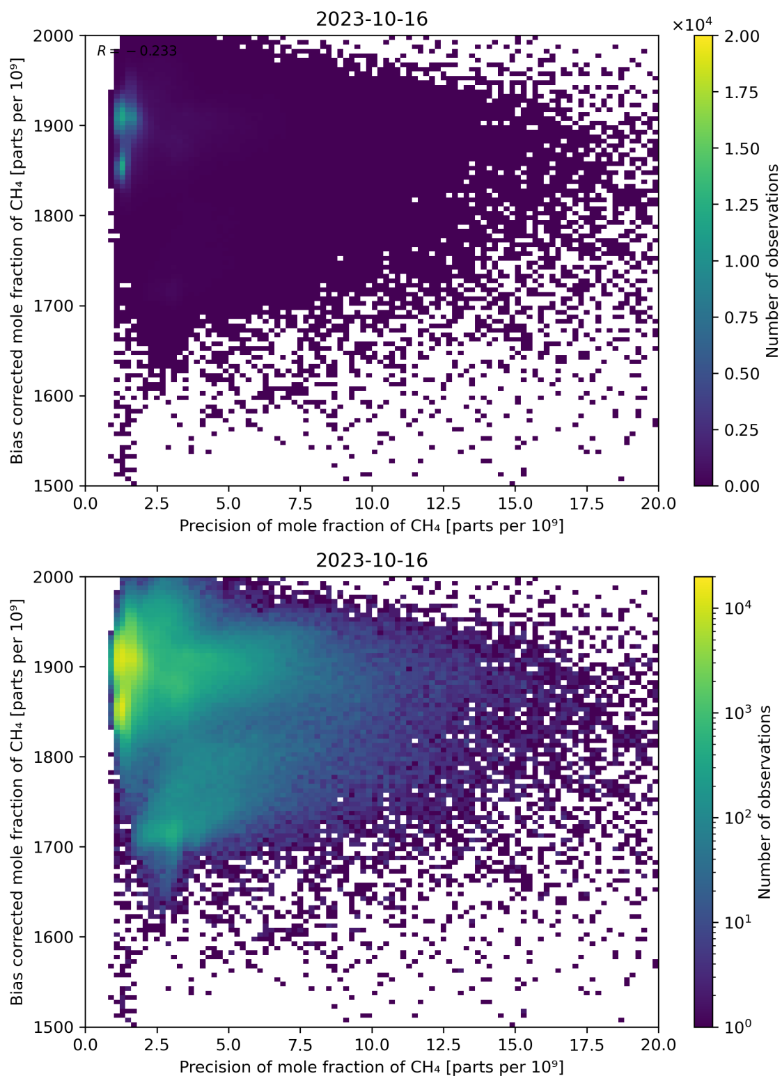
Figure 82: Scatter density plot of “Precision of mole fraction of CH 4 ” against “Bias corrected mole fraction of CH 4 ” for 2023-10-15 to 2023-10-17.
