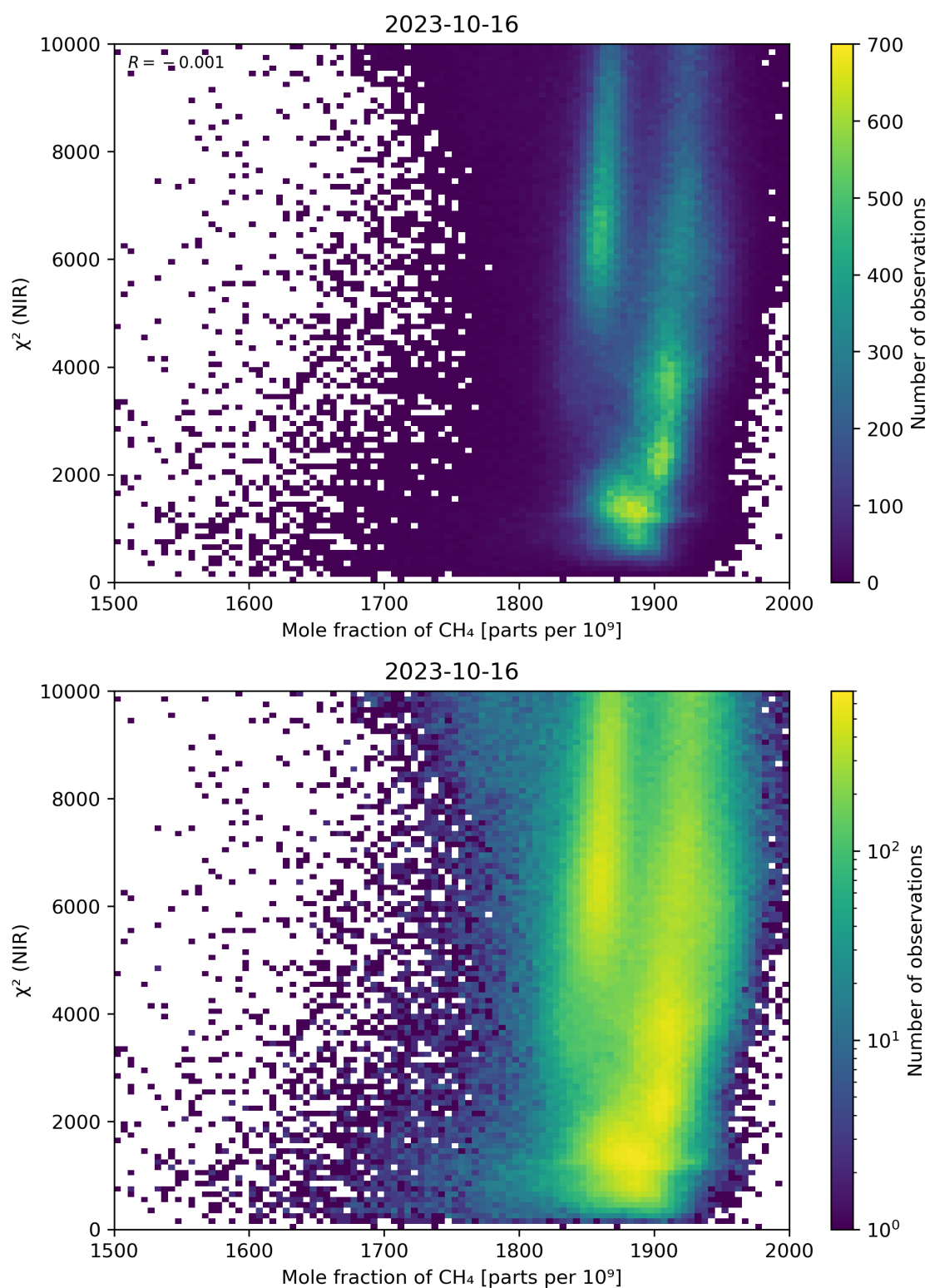
Figure 70: Scatter density plot of “Mole fraction of CH 4 ” against “ \chi^2 (NIR)” for 2023-10-15 to 2023-10-17.
