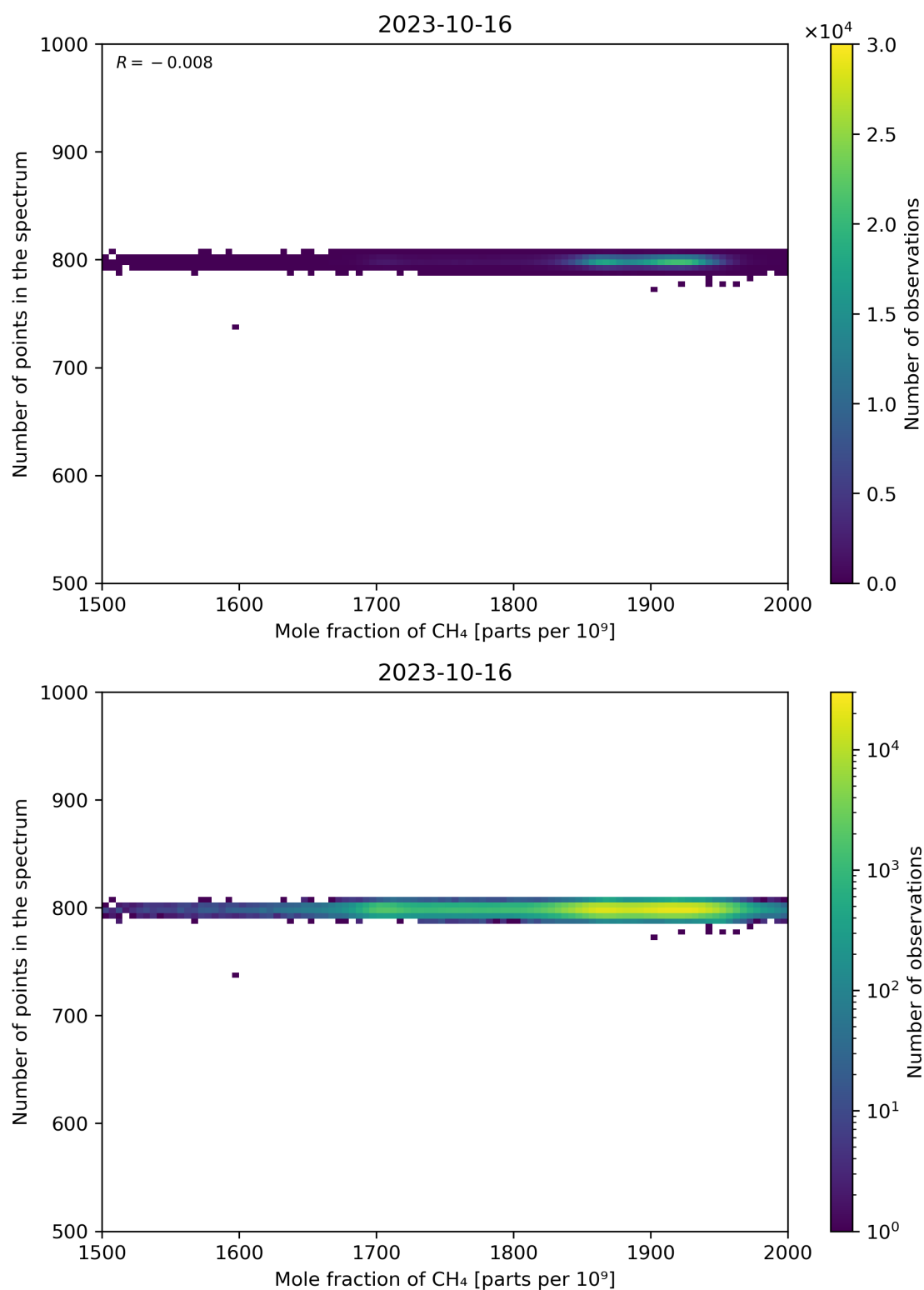
Figure 77: Scatter density plot of “Mole fraction of CH 4 ” against “Number of points in the spectrum” for 2023-10-15 to 2023-10-17.
