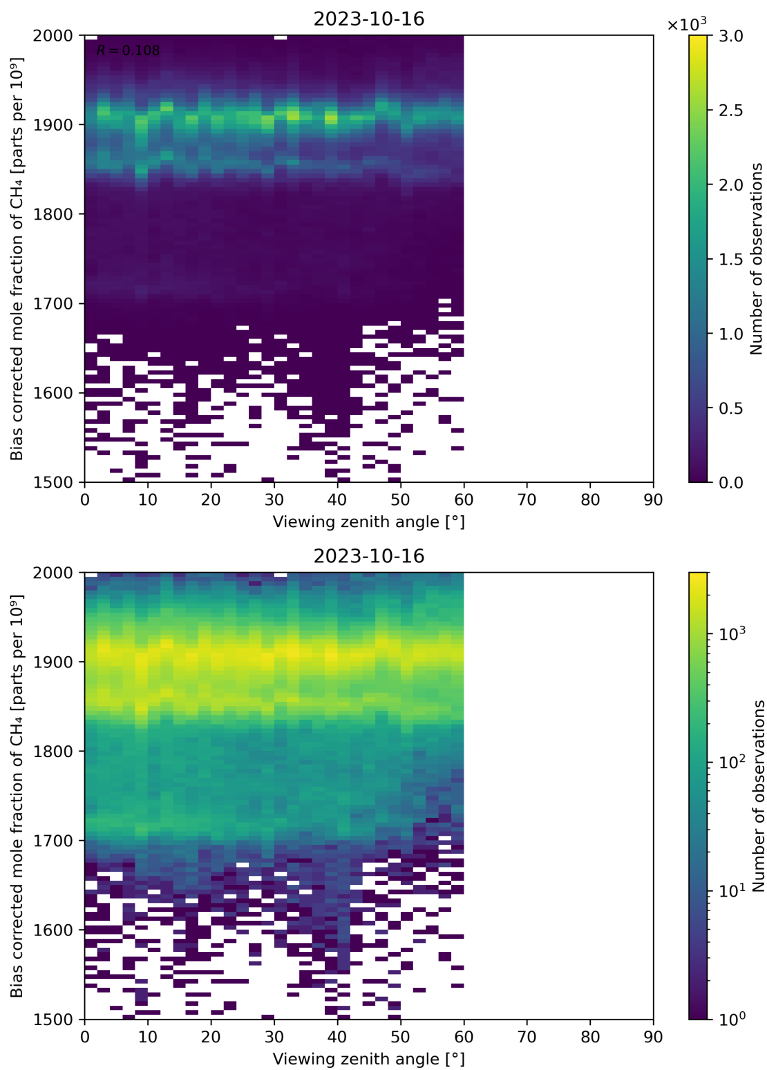
Figure 111: Scatter density plot of “Viewing zenith angle” against “Bias corrected mole fraction of CH 4 ” for 2023-10-15 to 2023-10-17.
