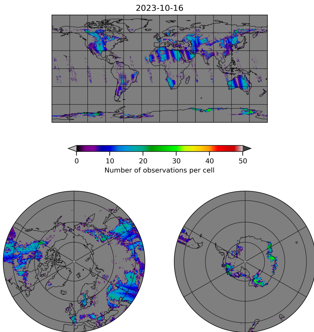
Figure 10: Map of the number of observations for 2023-10-15 to 2023-10-17
