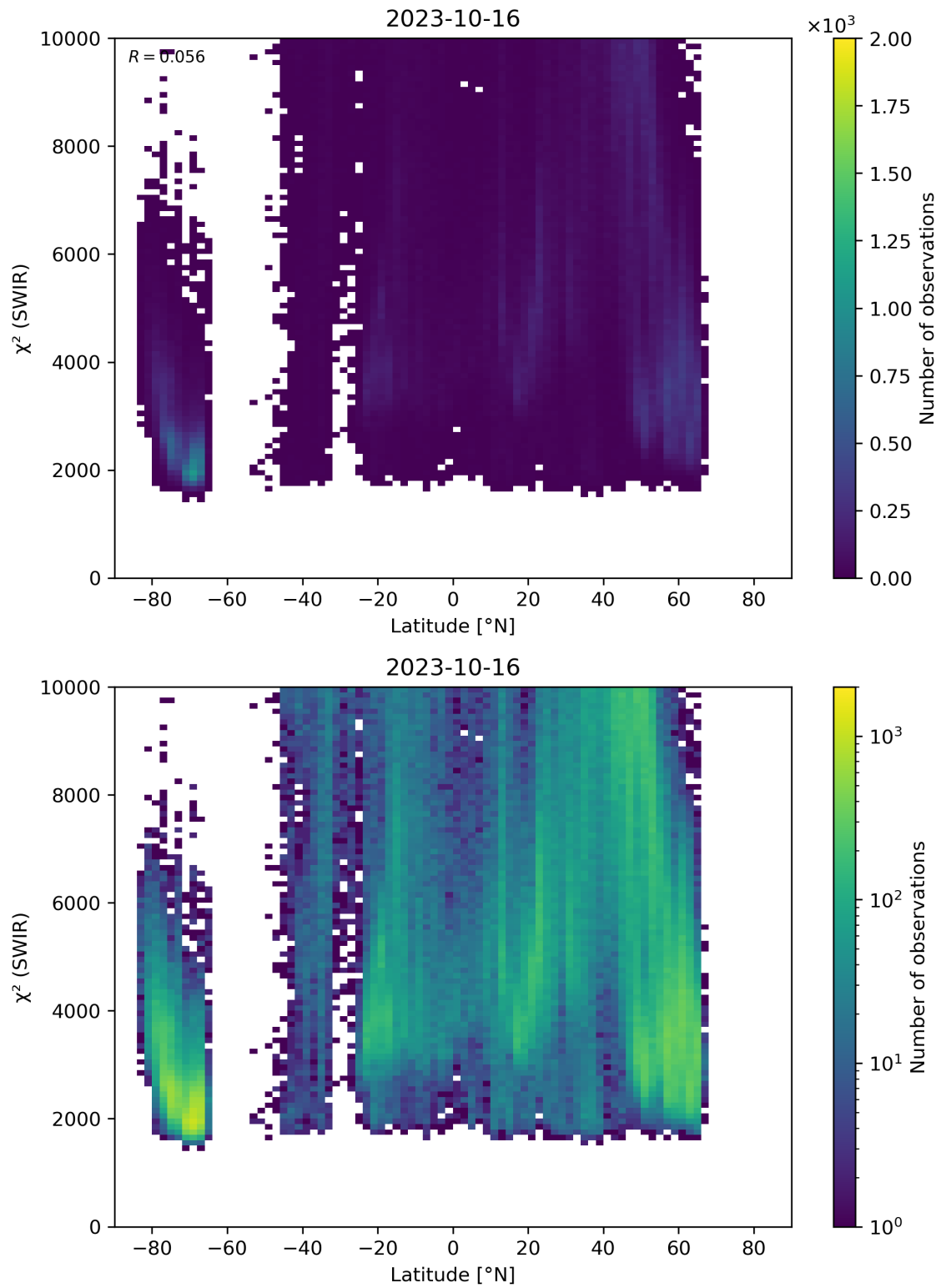
Figure 54: Scatter density plot of “Latitude” against “ \chi^2 (SWIR)” for 2023-10-15 to 2023-10-17.
