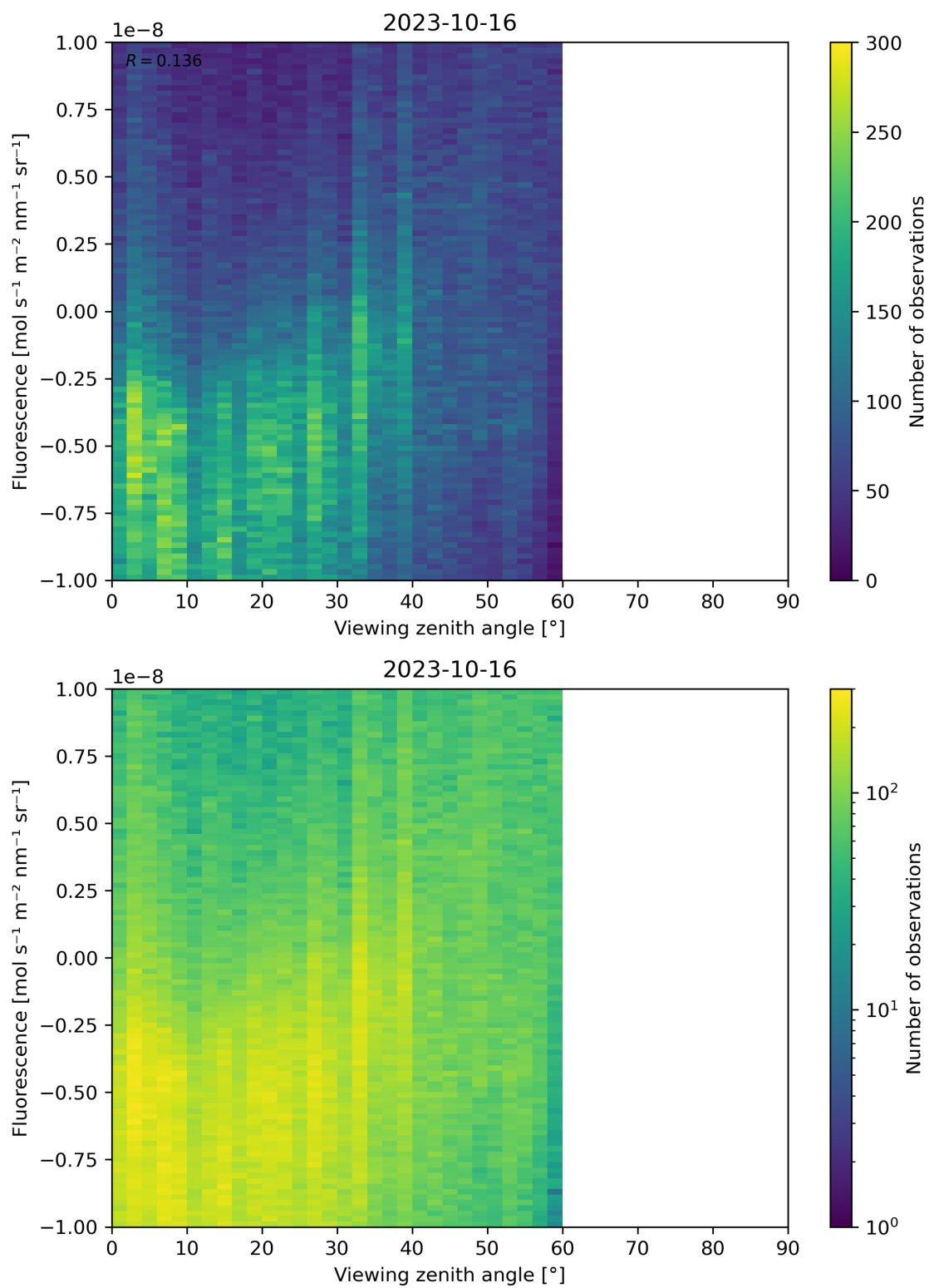
Figure 108: Scatter density plot of “Viewing zenith angle” against “Fluorescence” for 2023-10-15 to 2023-10-17.
