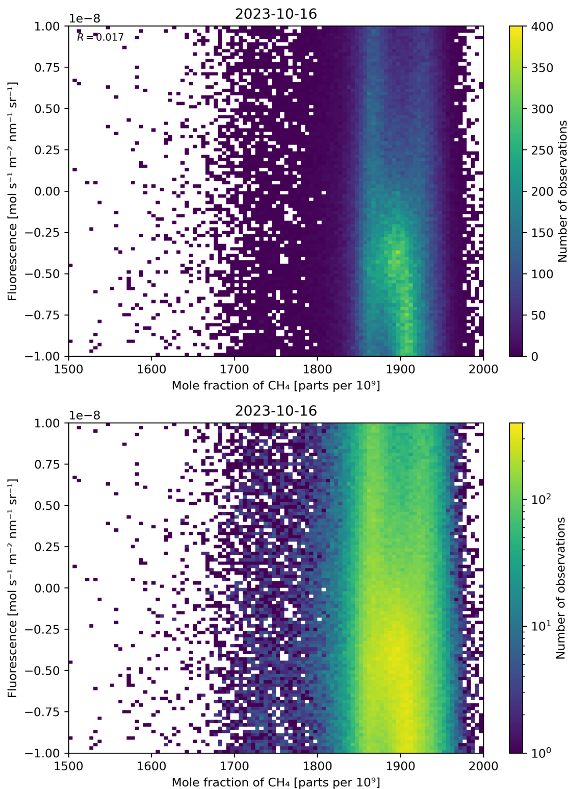
Figure 73: Scatter density plot of “Mole fraction of \text{CH}_4 ” against “Fluorescence” for 2023-10-15 to 2023-10-17.
