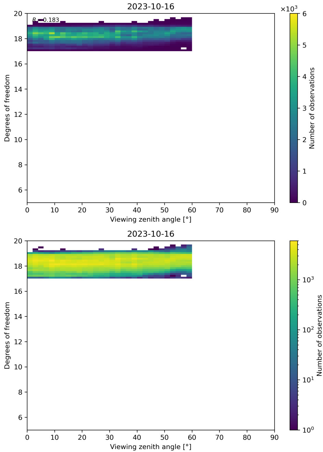
Figure 107: Scatter density plot of “Viewing zenith angle” against “Degrees of freedom” for 2023-10-15 to 2023-10-17.
