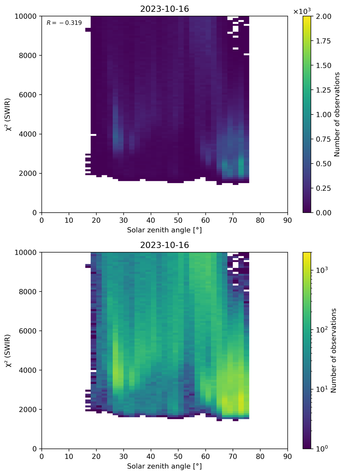
Figure 95: Scatter density plot of “Solar zenith angle” against “ \chi^2 (SWIR)” for 2023-10-15 to 2023-10-17.
