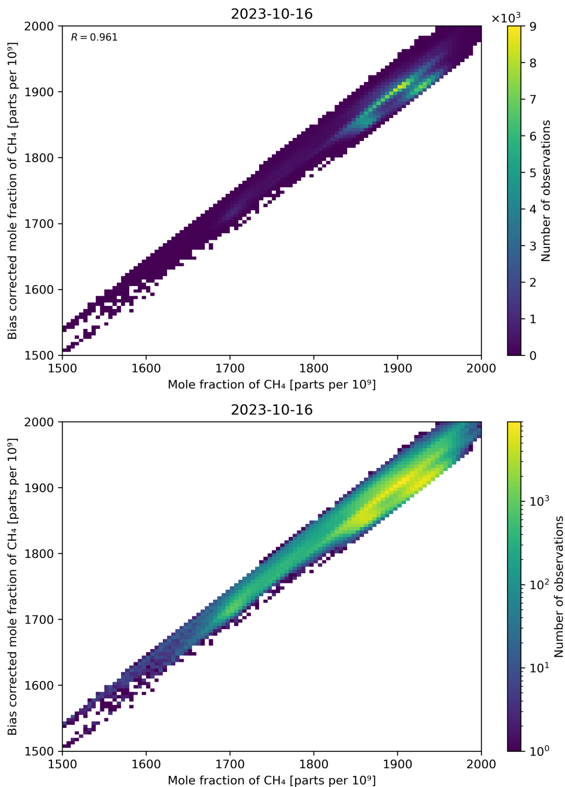
Figure 74: Scatter density plot of “Mole fraction of CH 4 ” against “Bias corrected mole fraction of CH 4 ” for 2023-10-15 to 2023-10-17.
