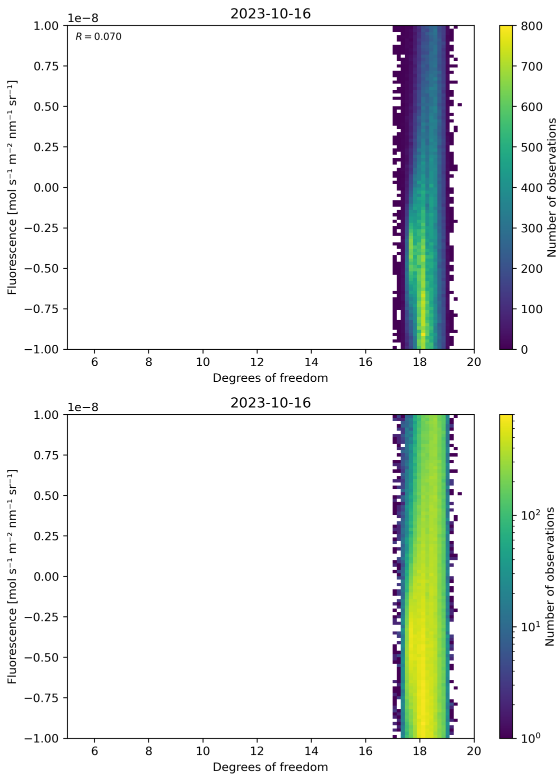
Figure 51: Scatter density plot of “Degrees of freedom” against “Fluorescence” for 2023-10-15 to 2023-10-17.
