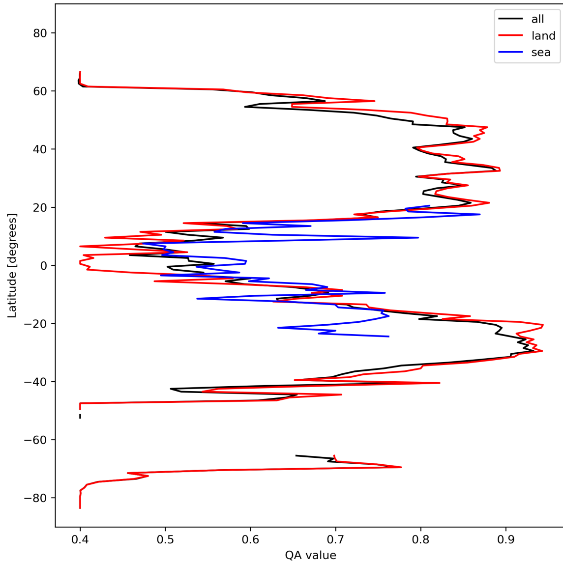
Figure 11: Zonal average of “QA value” for 2023-10-15 to 2023-10-17.
