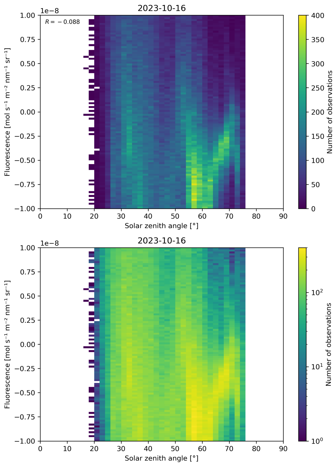
Figure 97: Scatter density plot of “Solar zenith angle” against “Fluorescence” for 2023-10-15 to 2023-10-17.
