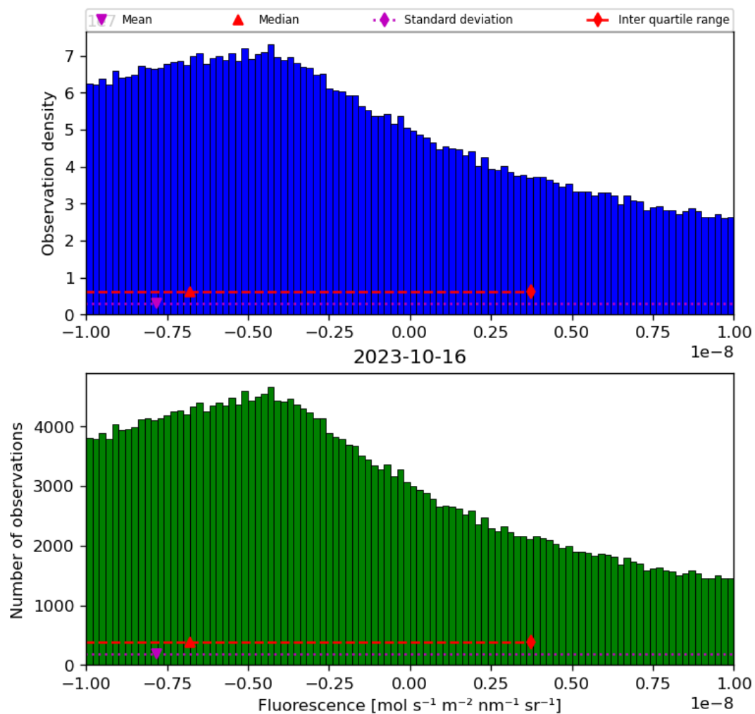
Figure 32: Histogram of “Fluorescence” for 2023-10-15 to 2023-10-17
