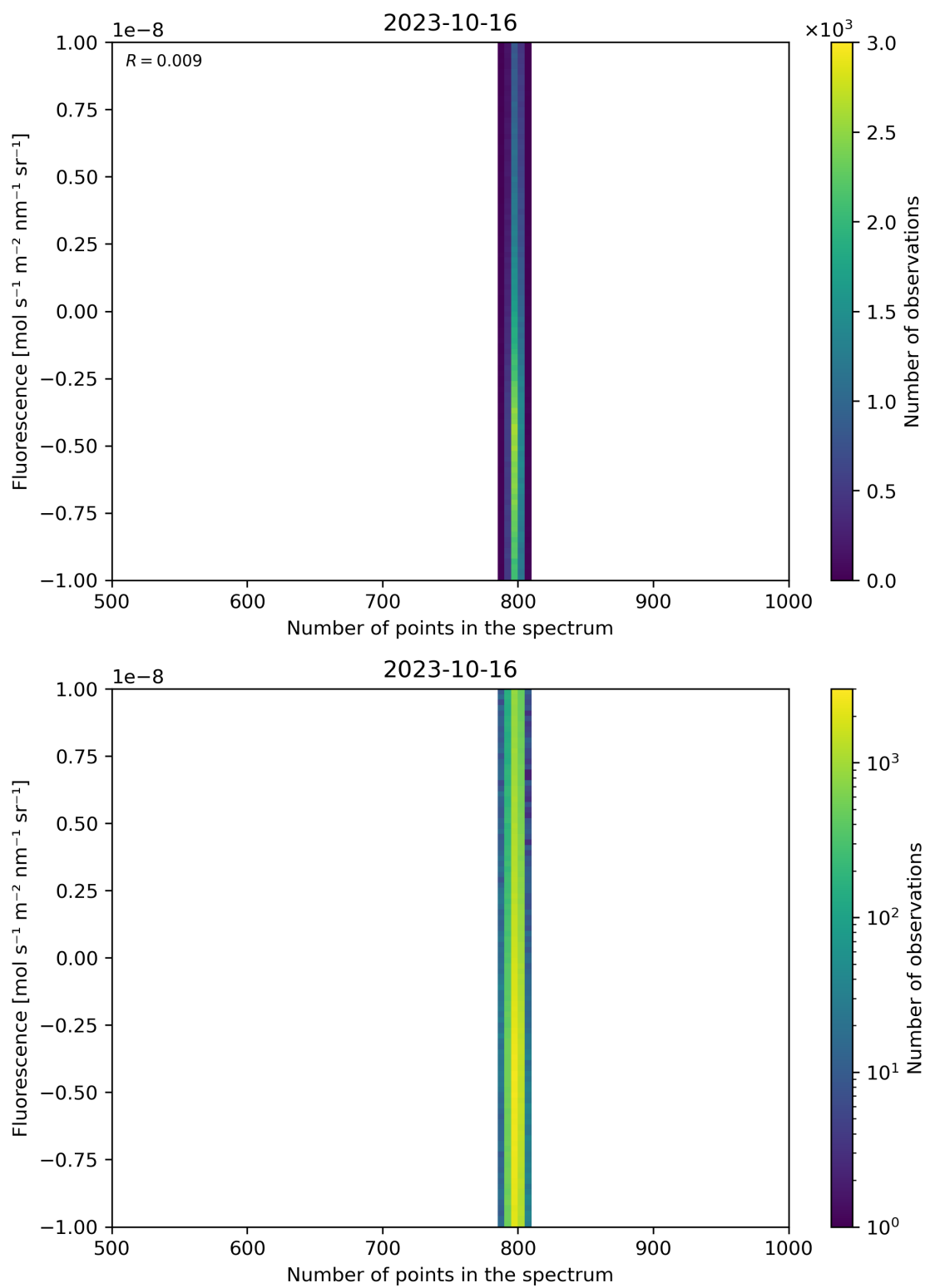
Figure 91: Scatter density plot of “Number of points in the spectrum” against “Fluorescence” for 2023-10-15 to 2023-10-17.
