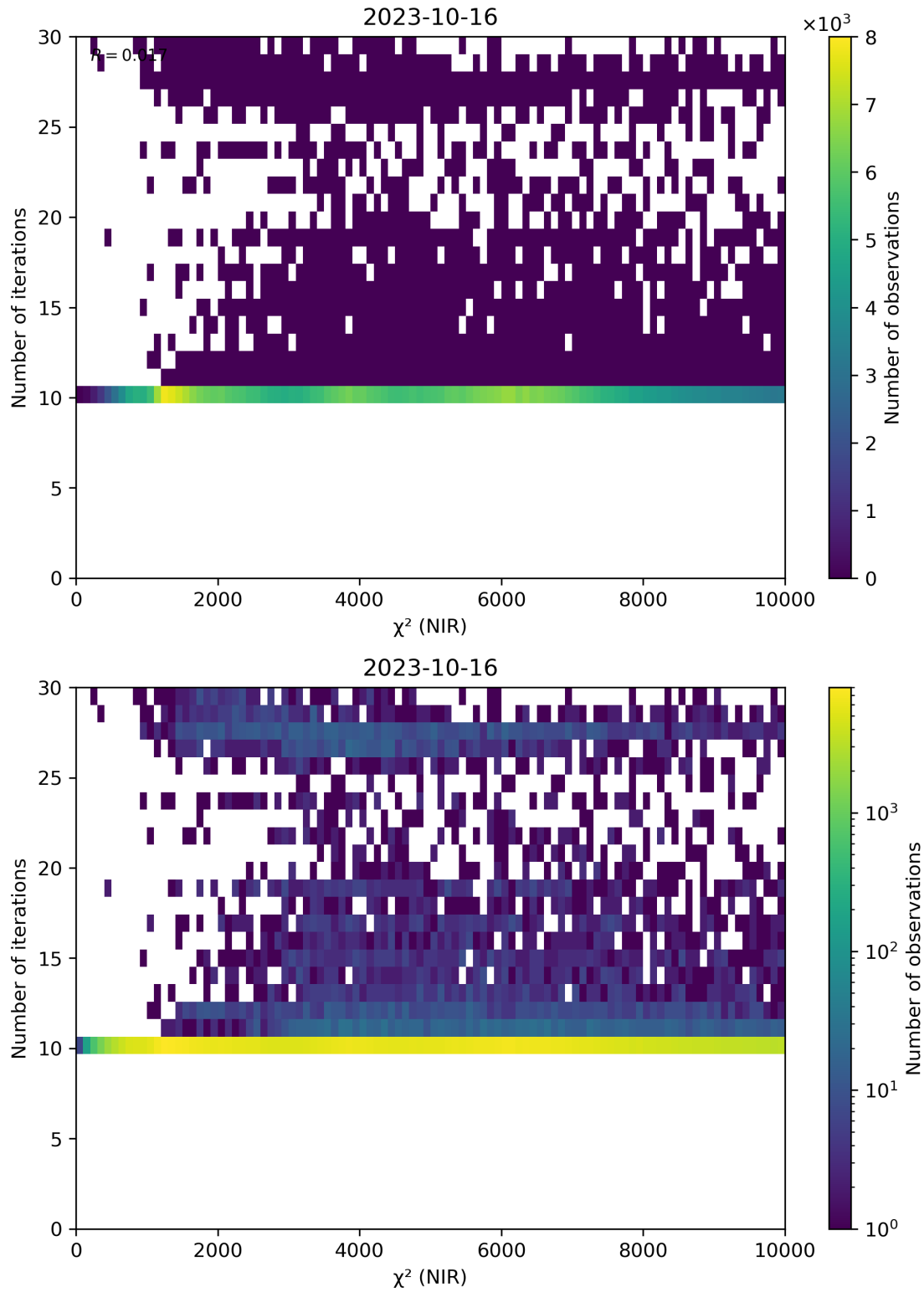
Figure 46: Scatter density plot of “ \chi^2 (NIR)” against “Number of iterations” for 2023-10-15 to 2023-10-17.
