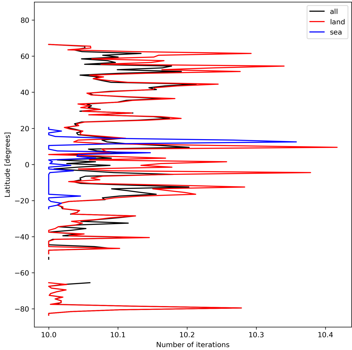
Figure 20: Zonal average of “Number of iterations” for 2023-10-15 to 2023-10-17.
