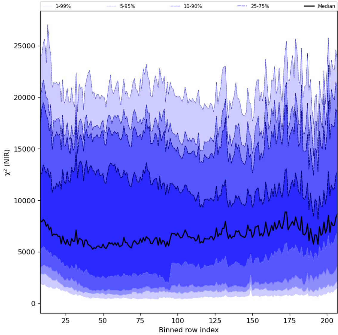
Figure 40: Along track statistics of " \chi^2 (NIR)" for 2023-10-15 to 2023-10-17
