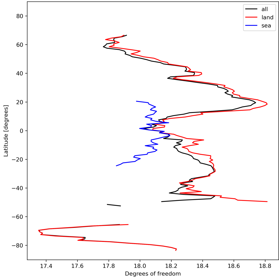
Figure 19: Zonal average of “Degrees of freedom” for 2023-10-15 to 2023-10-17.
