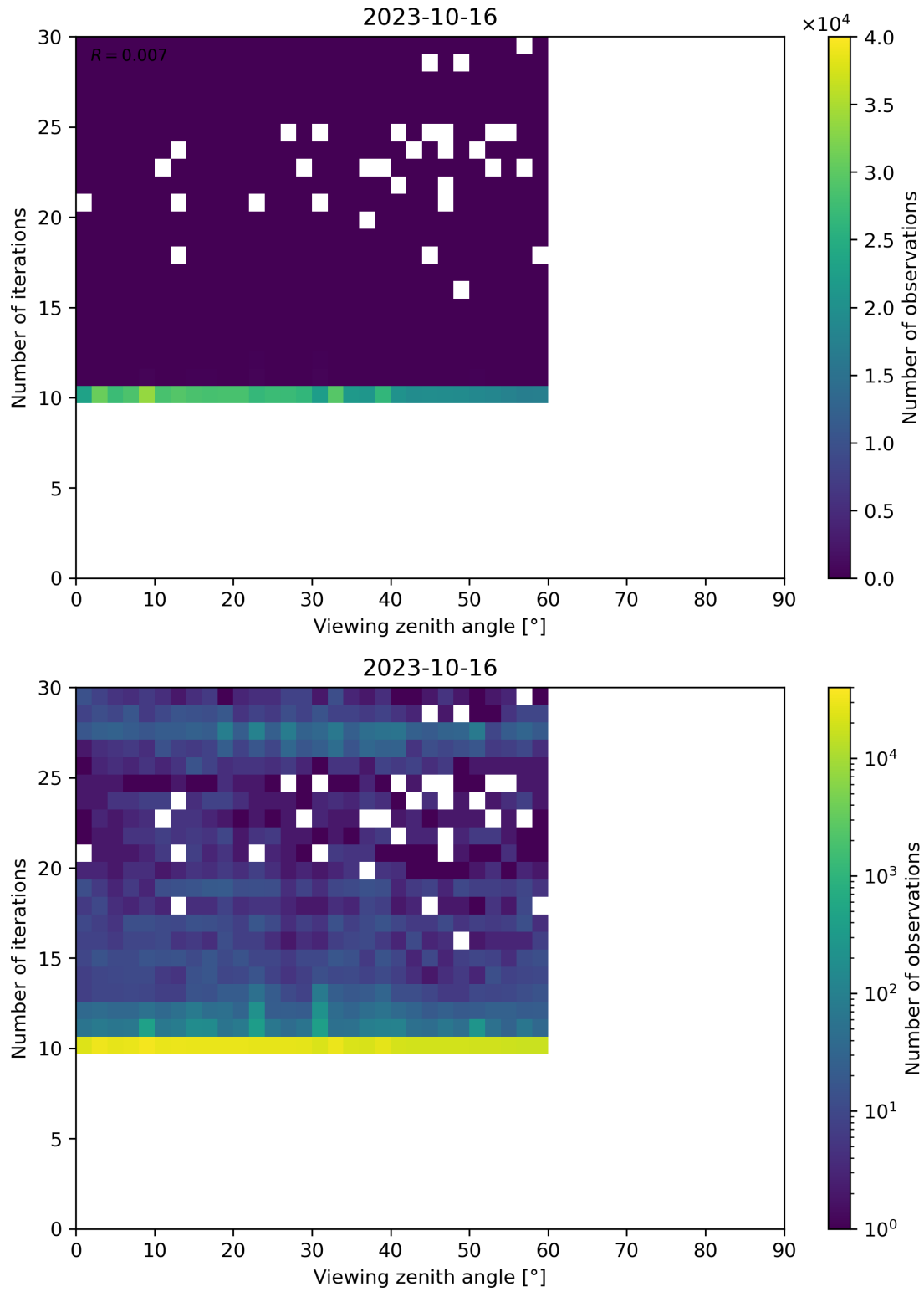
Figure 113: Scatter density plot of “Viewing zenith angle” against “Number of iterations” for 2023-10-15 to 2023-10-17.
