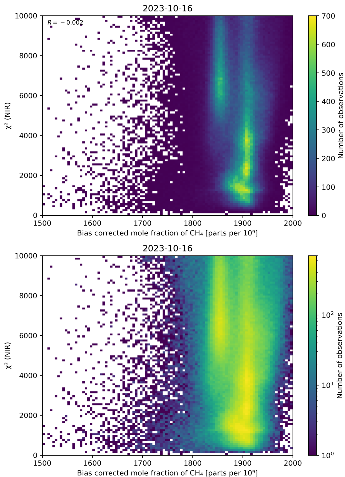
Figure 63: Scatter density plot of “Bias corrected mole fraction of CH 4 ” against “ \chi^2 (NIR)” for 2023-10-15 to 2023-10-17.
