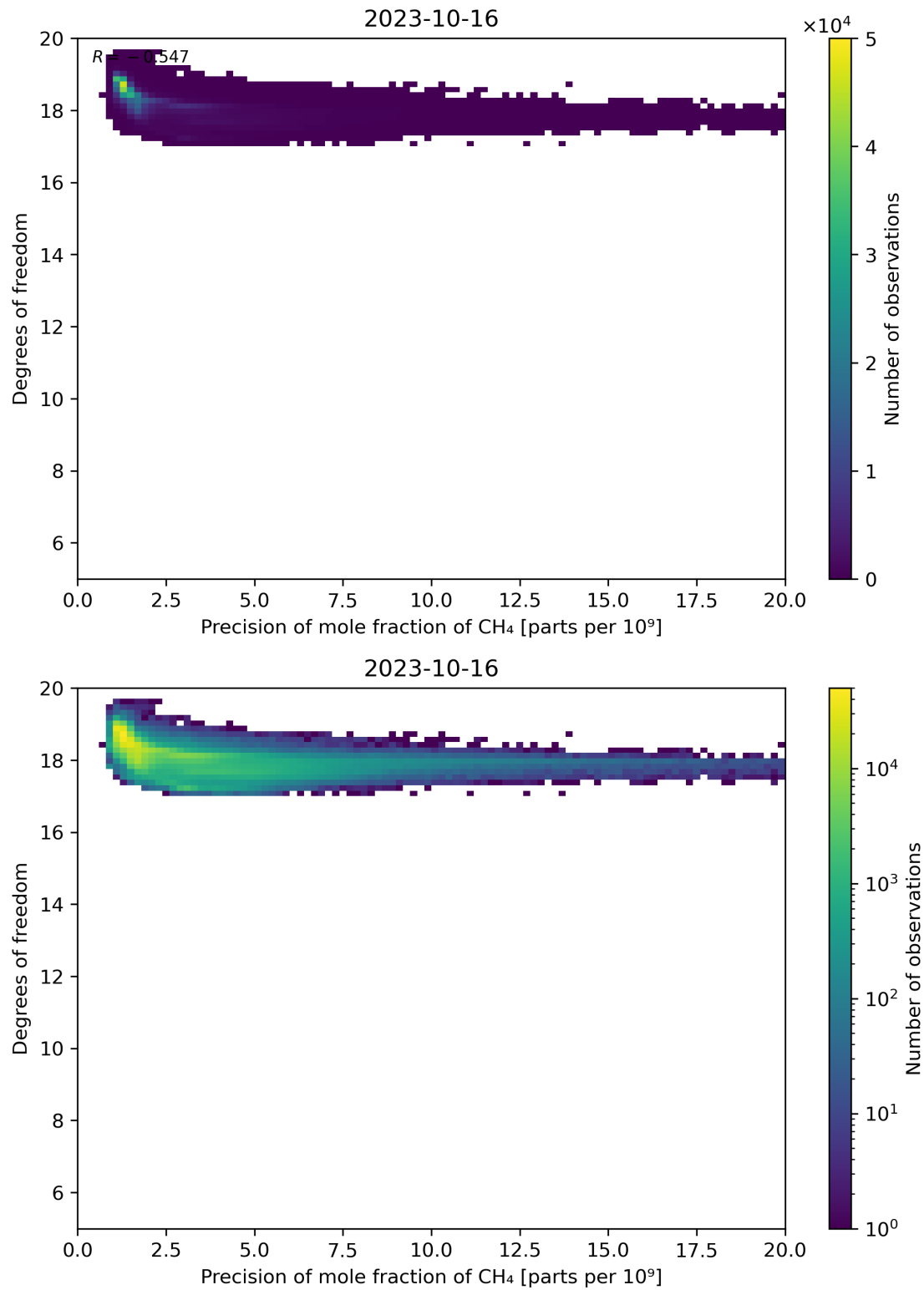
Figure 80: Scatter density plot of “Precision of mole fraction of CH 4 ” against “Degrees of freedom” for 2023-10-15 to 2023-10-17.
