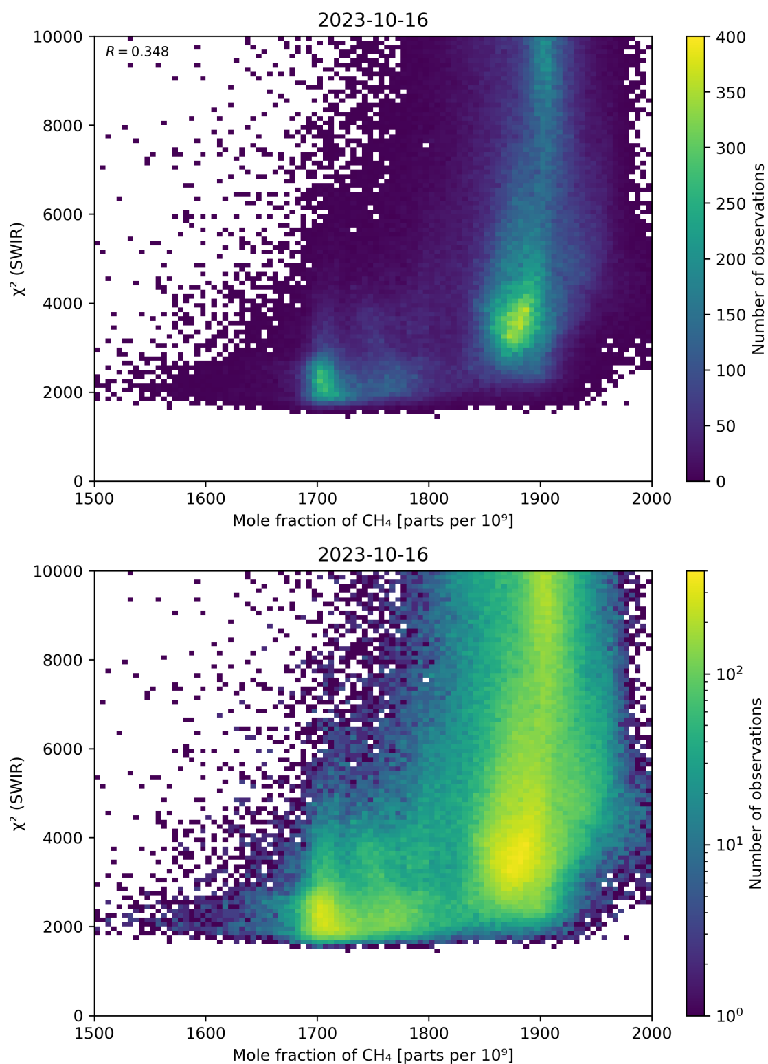
Figure 71: Scatter density plot of “Mole fraction of \text{CH}_4 ” against “ \chi^2 (SWIR)” for 2023-10-15 to 2023-10-17.
