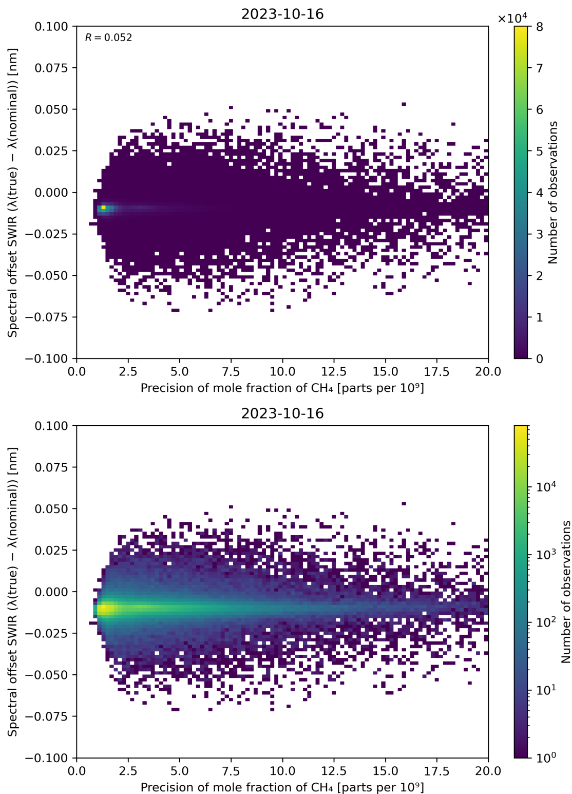
Figure 85: Scatter density plot of “Precision of mole fraction of \text{CH}_4 ” against “Spectral offset SWIR ( \lambda(\text{true}) - \lambda(\text{nominal}) )” for 2023-10-15 to 2023-10-17.
