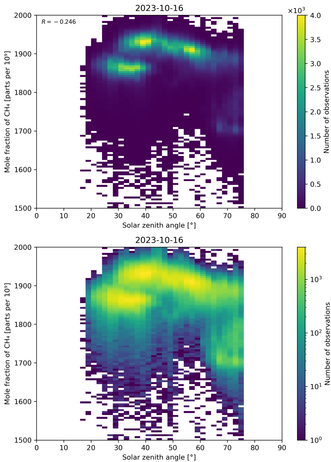
Figure 99: Scatter density plot of “Solar zenith angle” against “Mole fraction of CH 4 ” for 2023-10-15 to 2023-10-17.
