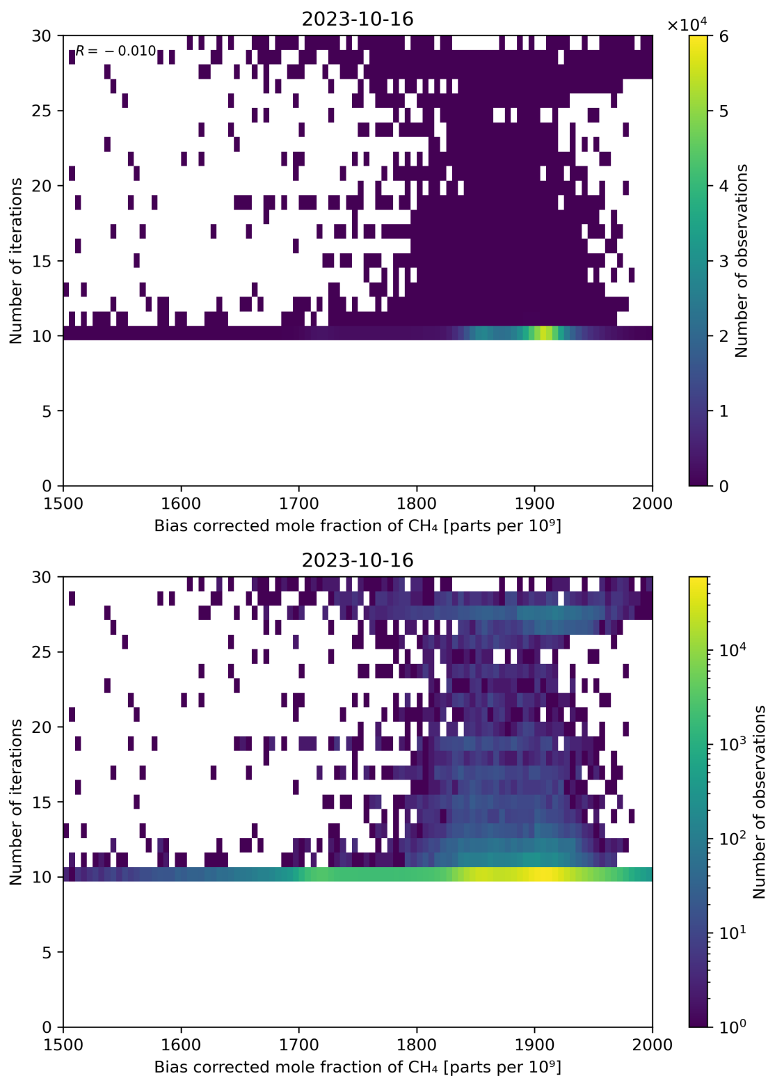
Figure 67: Scatter density plot of “Bias corrected mole fraction of CH 4 ” against “Number of iterations” for 2023-10-15 to 2023-10-17.
