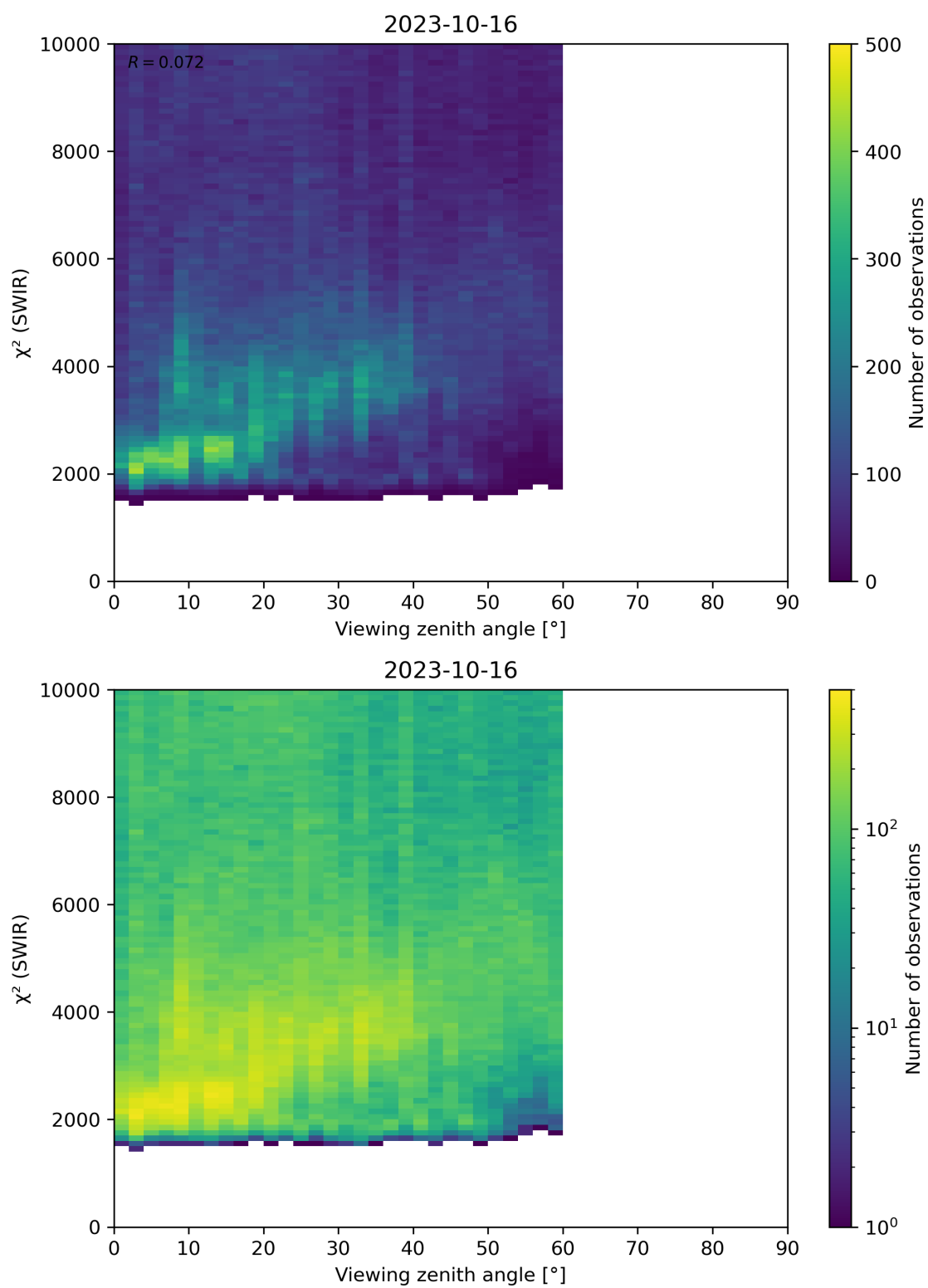
Figure 106: Scatter density plot of “Viewing zenith angle” against “ \chi^2 (SWIR)” for 2023-10-15 to 2023-10-17.
