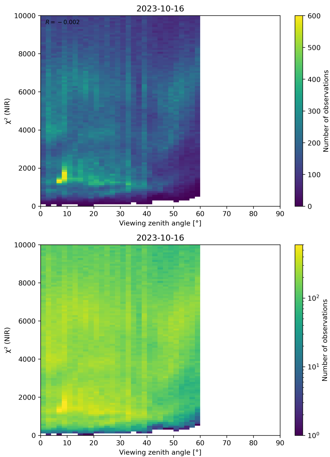
Figure 105: Scatter density plot of “Viewing zenith angle” against “ \chi^2 (NIR)” for 2023-10-15 to 2023-10-17.
