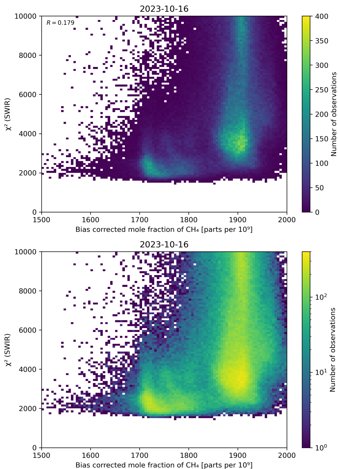
Figure 64: Scatter density plot of “Bias corrected mole fraction of CH 4 ” against “ \chi^2 (SWIR)” for 2023-10-15 to 2023-10-17.
