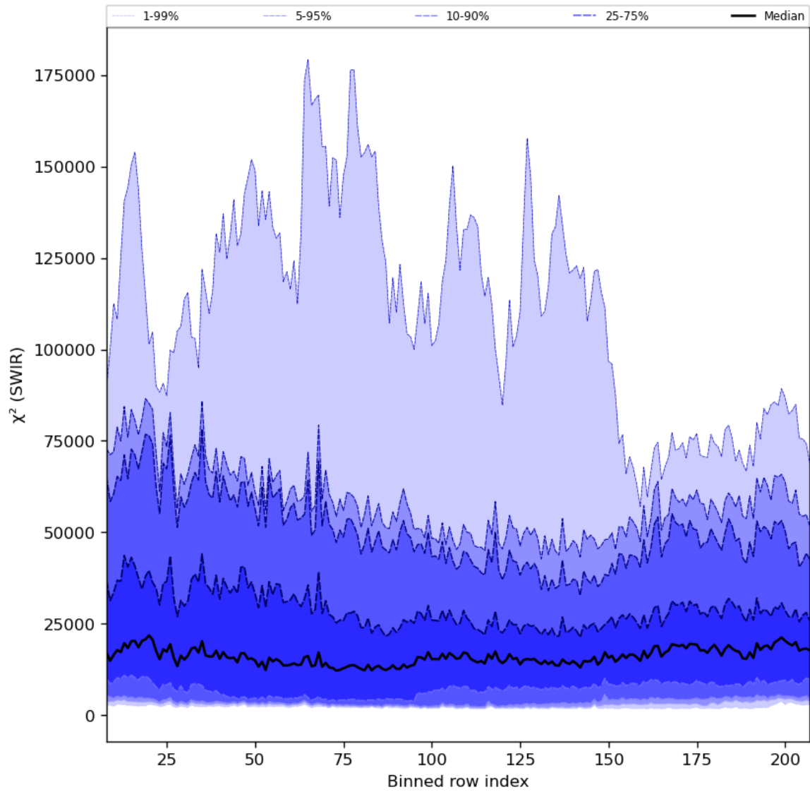
Figure 39: Along track statistics of “ \chi^2 (SWIR)” for 2023-10-15 to 2023-10-17
