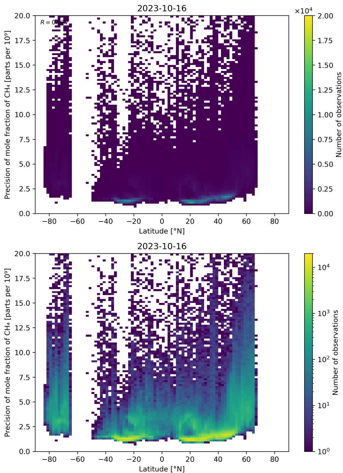
Figure 59: Scatter density plot of “Latitude” against “Precision of mole fraction of CH 4 ” for 2023-10-15 to 2023-10-17.
