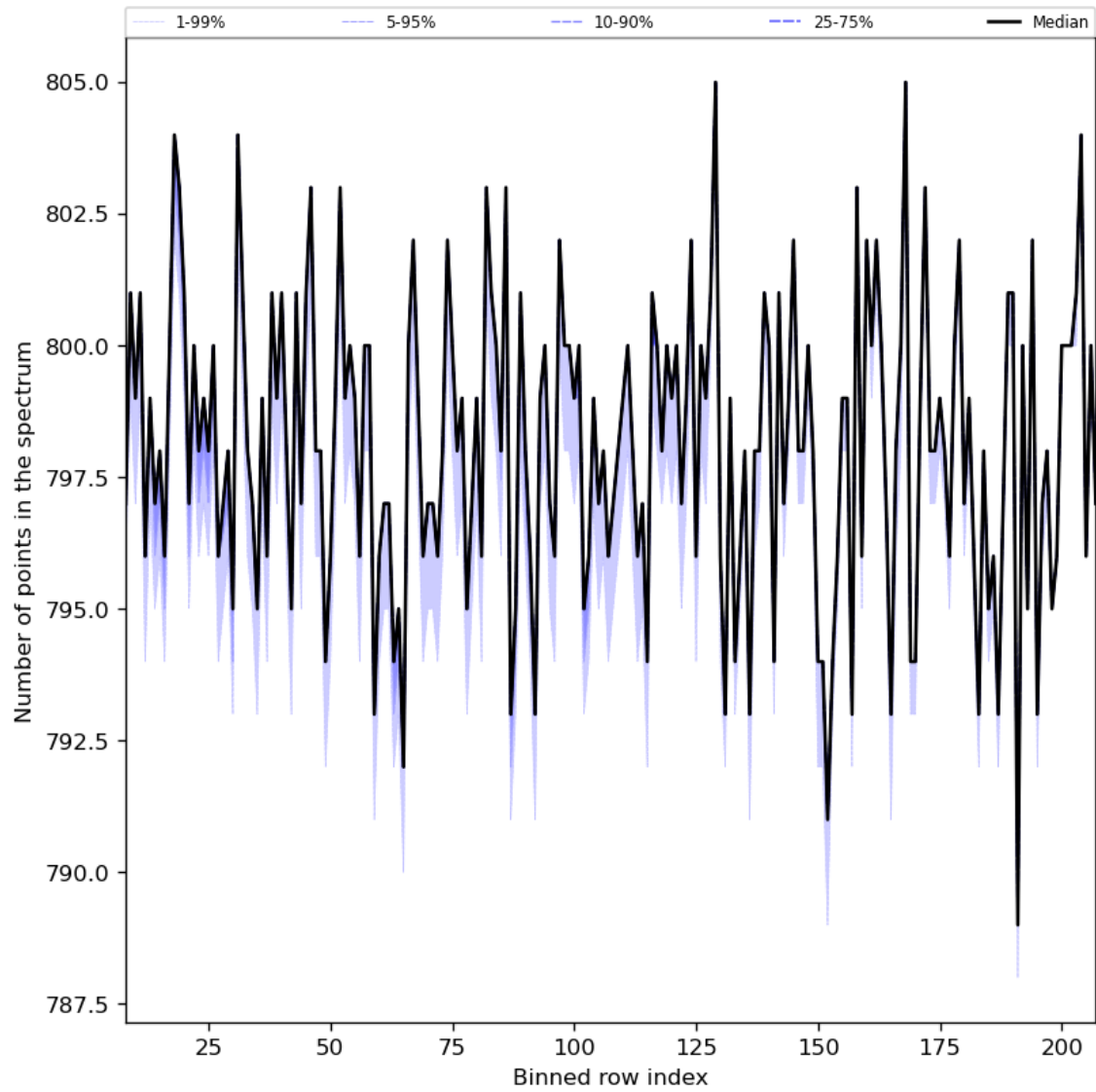
Figure 37: Along track statistics of “Number of points in the spectrum” for 2023-10-15 to 2023-10-17
