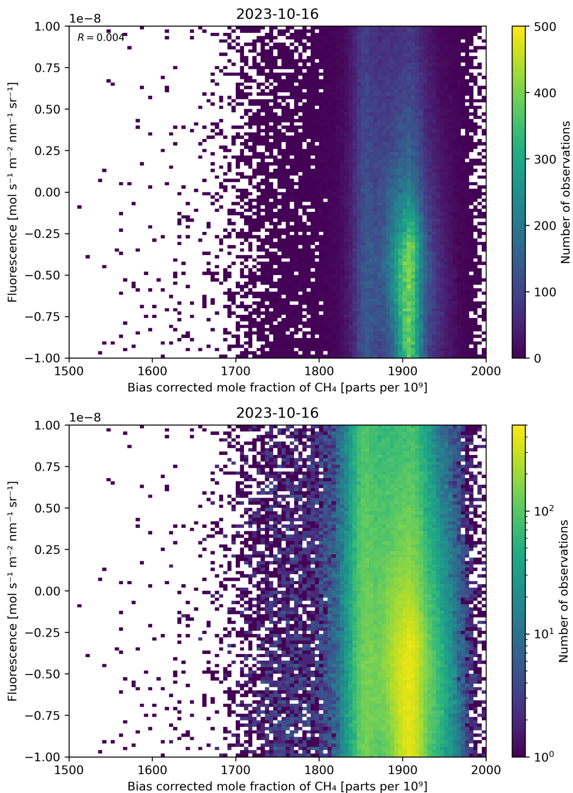
Figure 66: Scatter density plot of “Bias corrected mole fraction of \text{CH}_4 ” against “Fluorescence” for 2023-10-15 to 2023-10-17.
