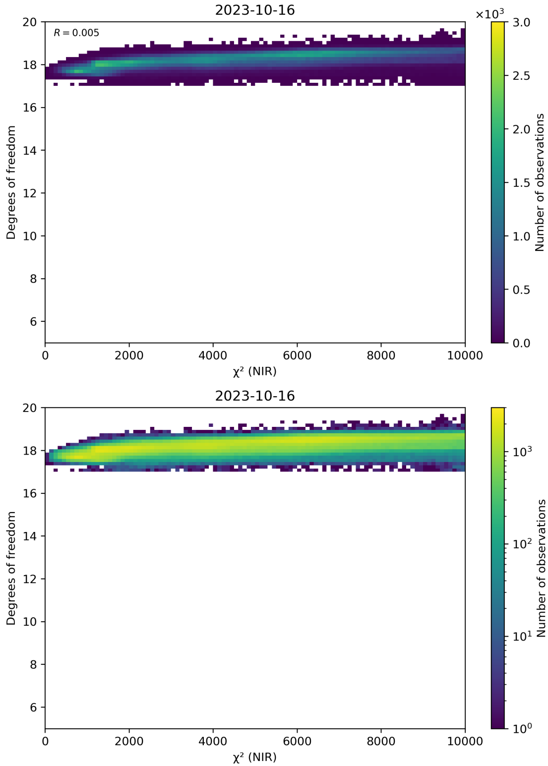
Figure 44: Scatter density plot of “ \chi^2 (NIR)” against “Degrees of freedom” for 2023-10-15 to 2023-10-17.
