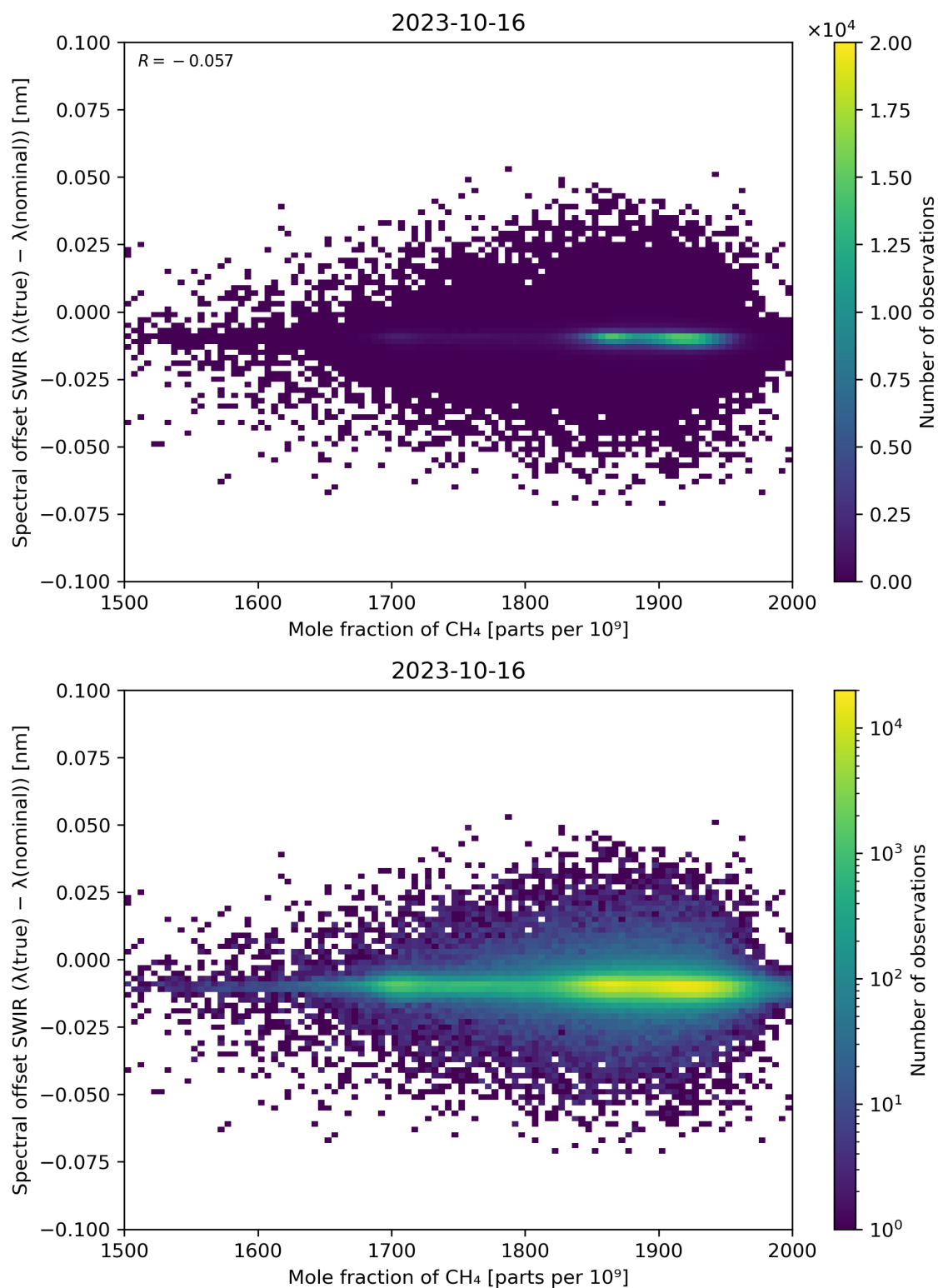
Figure 86: Scatter density plot of “Mole fraction of CH 4 ” against “Spectral offset SWIR ( \lambda(\text{true}) - \lambda(\text{nominal}) )” for 2023-10-15 to 2023-10-17.
