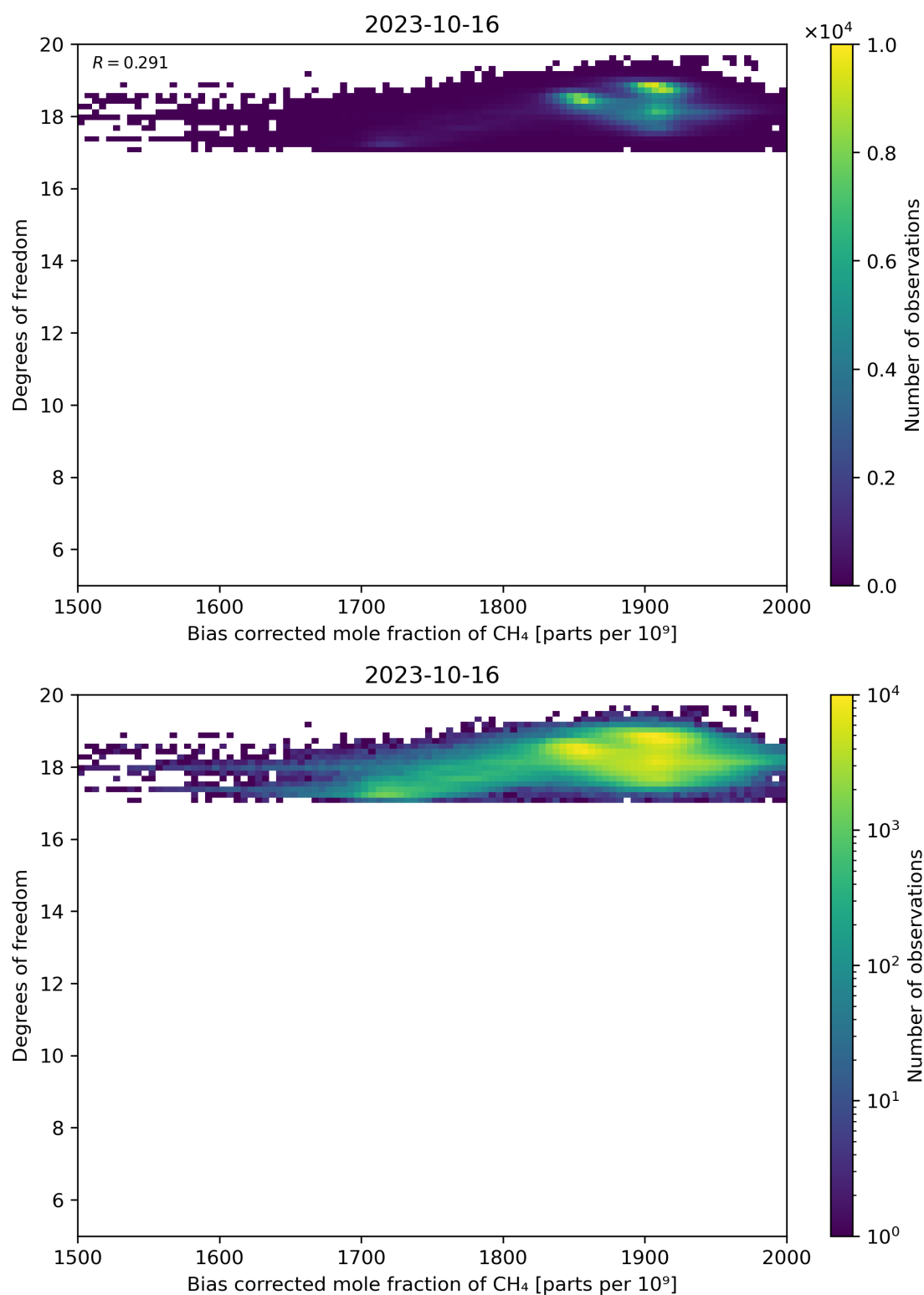
Figure 65: Scatter density plot of “Bias corrected mole fraction of \text{CH}_4 ” against “Degrees of freedom” for 2023-10-15 to 2023-10-17.
