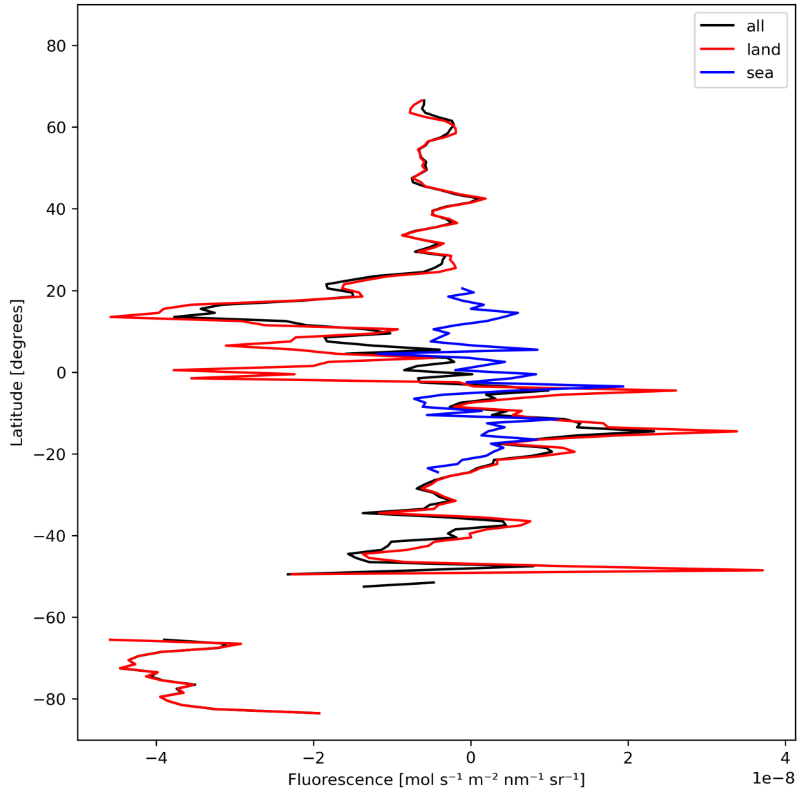
Figure 21: Zonal average of “Fluorescence” for 2023-10-15 to 2023-10-17.
