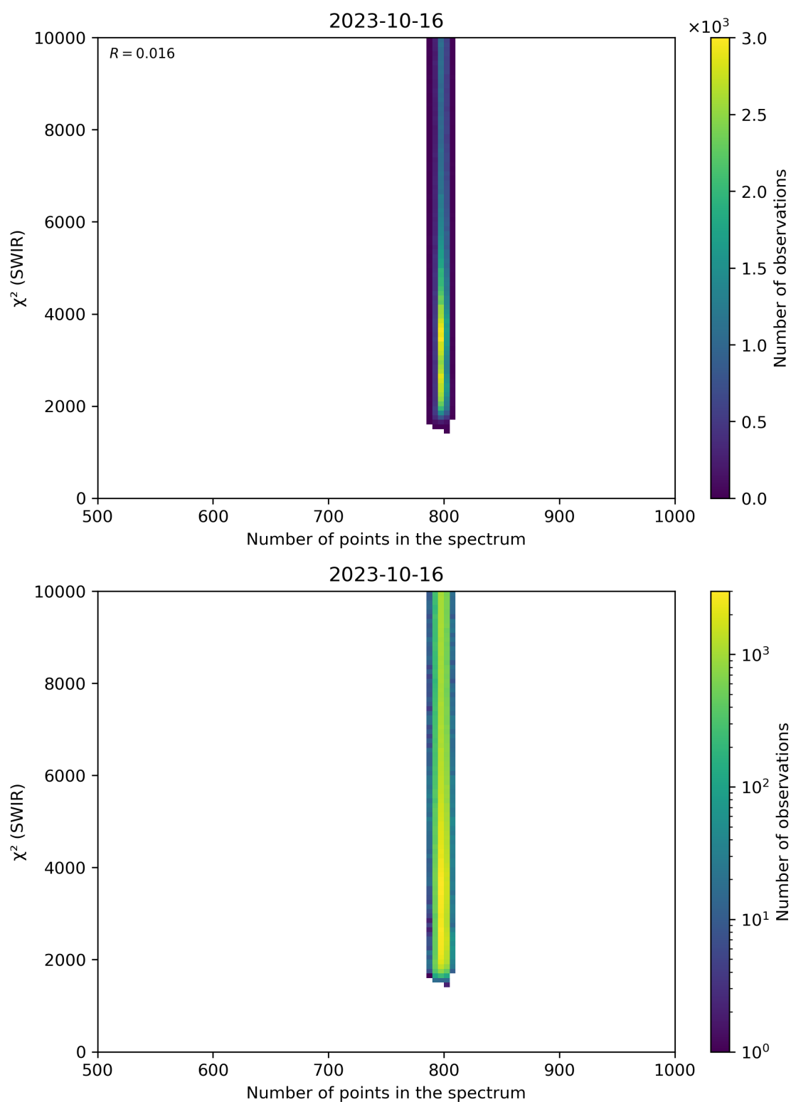
Figure 89: Scatter density plot of “Number of points in the spectrum” against “ \chi^2 (SWIR)” for 2023-10-15 to 2023-10-17.
