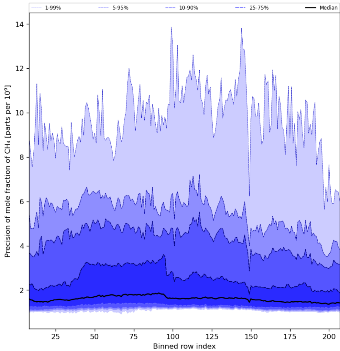
Figure 35: Along track statistics of “Precision of mole fraction of CH 4 ” for 2023-10-15 to 2023-10-17
