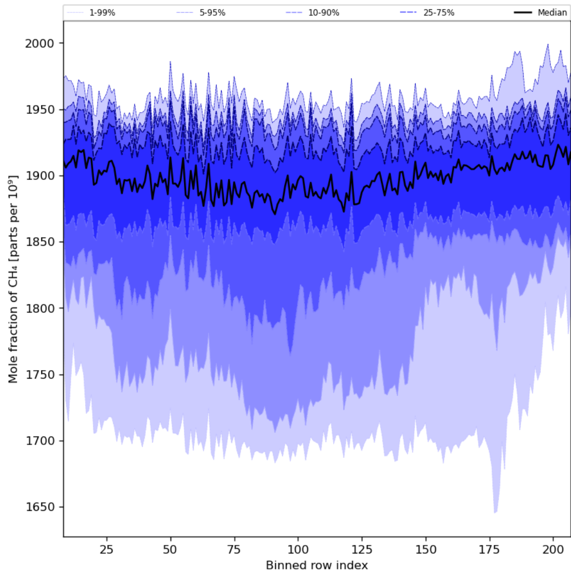
Figure 34: Along track statistics of “Mole fraction of CH 4 ” for 2023-10-15 to 2023-10-17
