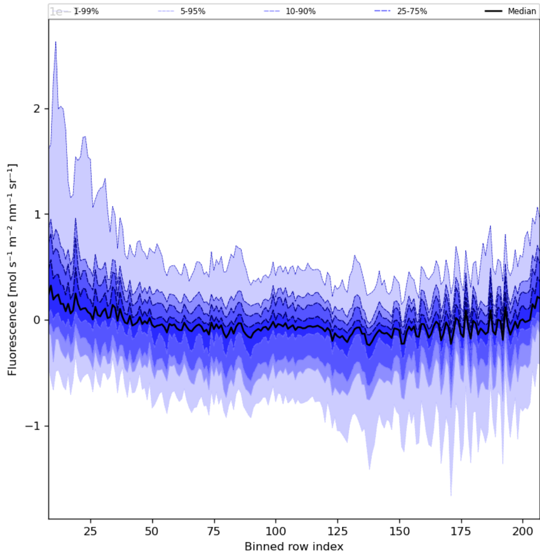
Figure 43: Along track statistics of “Fluorescence” for 2023-10-15 to 2023-10-17
