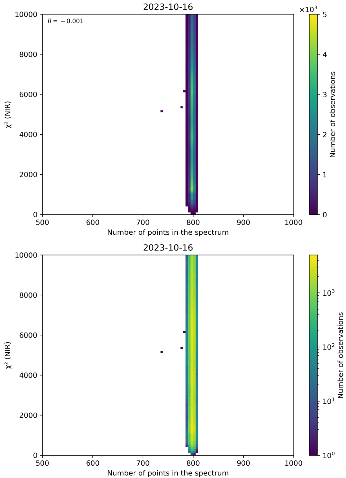
Figure 88: Scatter density plot of “Number of points in the spectrum” against “ \chi^2 (NIR)” for 2023-10-15 to 2023-10-17.
