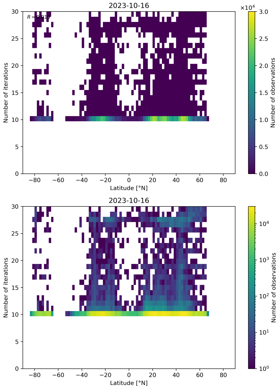
Figure 60: Scatter density plot of “Latitude” against “Number of iterations” for 2023-10-15 to 2023-10-17.
