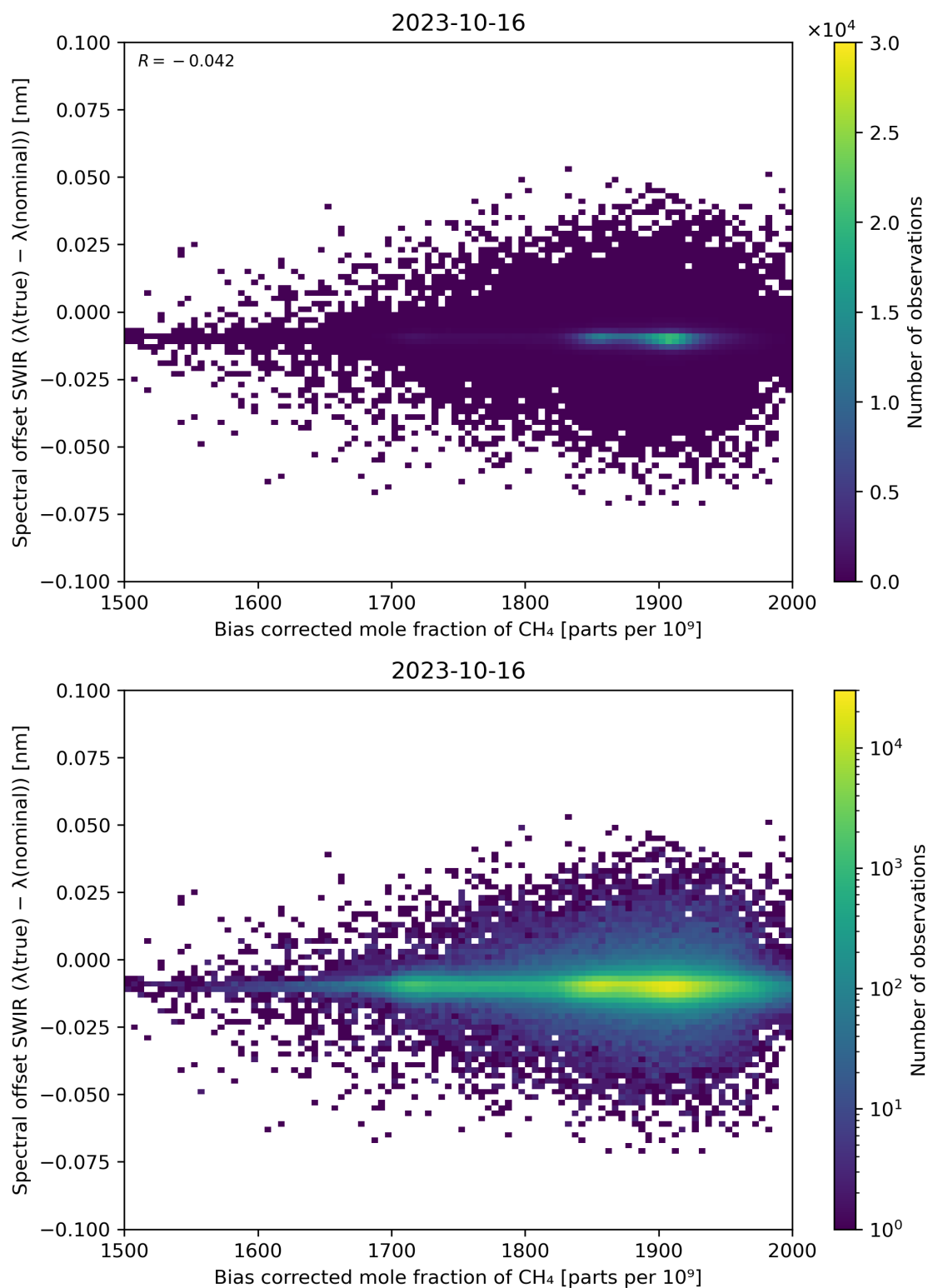
Figure 69: Scatter density plot of “Bias corrected mole fraction of \text{CH}_4 ” against “Spectral offset SWIR ( \lambda(\text{true}) - \lambda(\text{nominal}) )” for 2023-10-15 to 2023-10-17.
