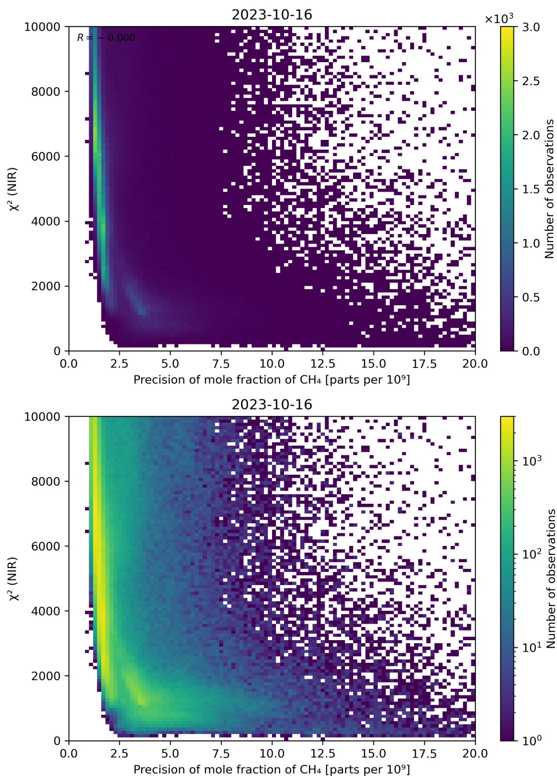
Figure 78: Scatter density plot of “Precision of mole fraction of CH 4 ” against “ \chi^2 (NIR)” for 2023-10-15 to 2023-10-17.
