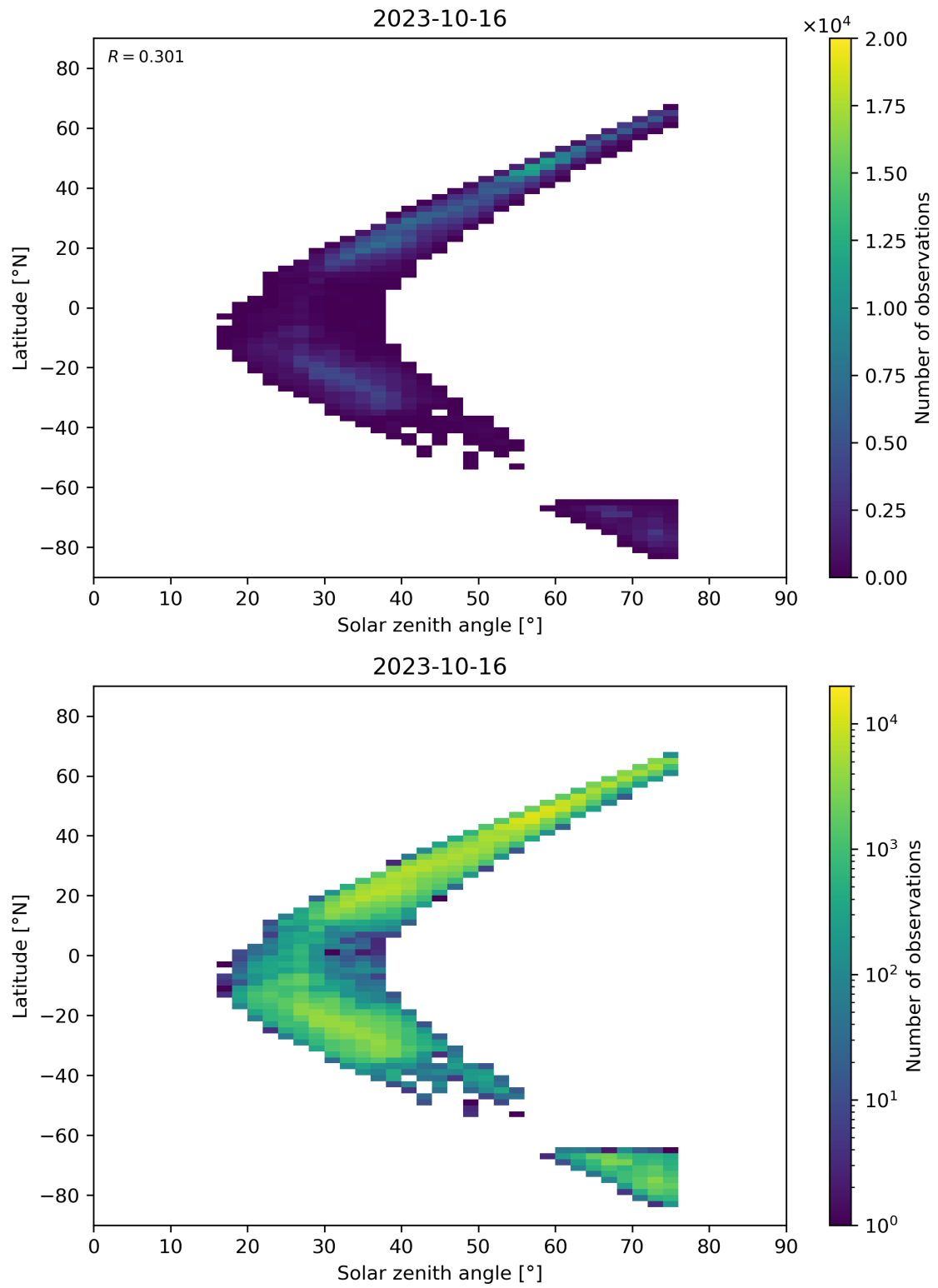
Figure 98: Scatter density plot of “Solar zenith angle” against “Latitude” for 2023-10-15 to 2023-10-17.
