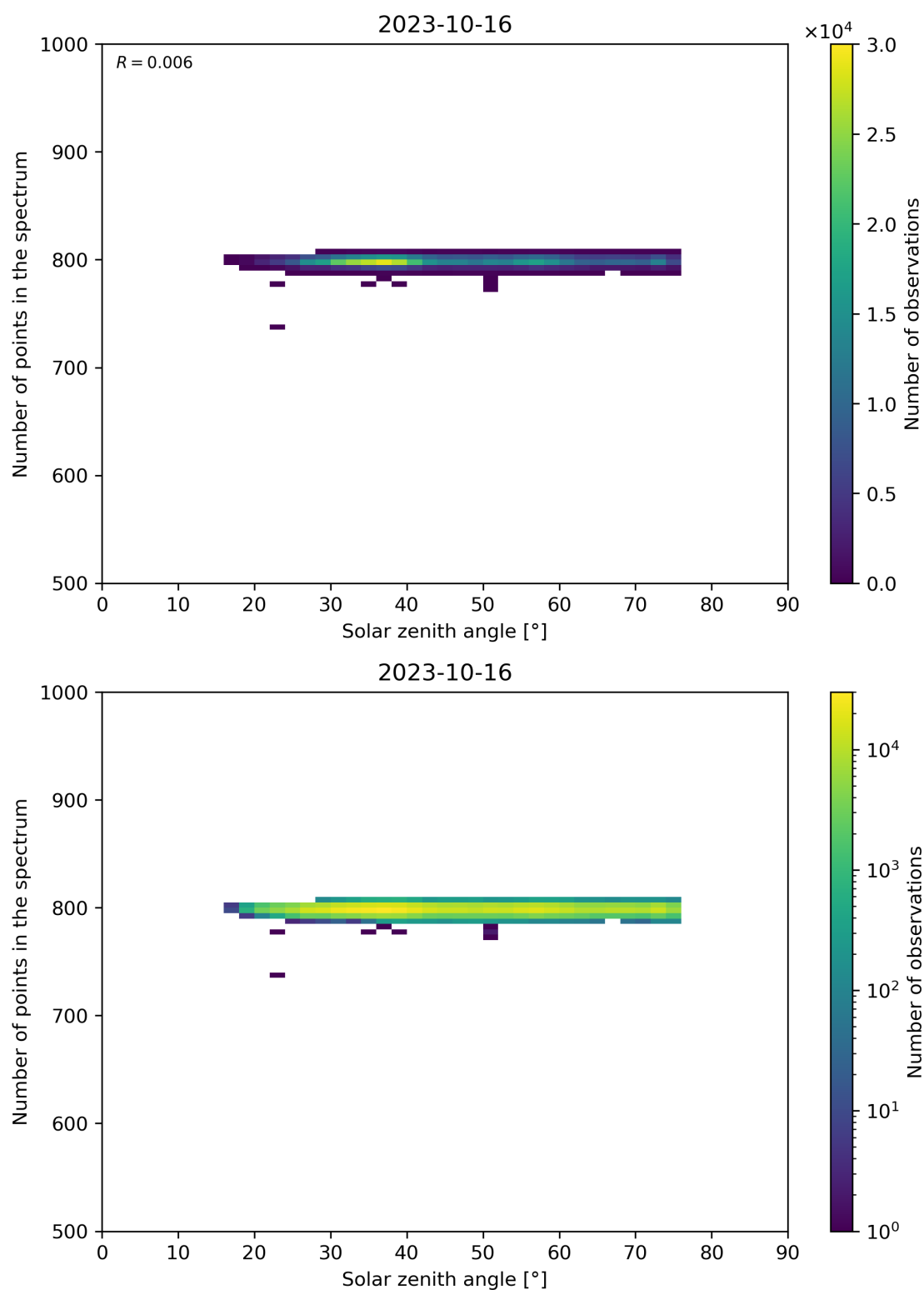
Figure 103: Scatter density plot of “Solar zenith angle” against “Number of points in the spectrum” for 2023-10-15 to 2023-10-17.
