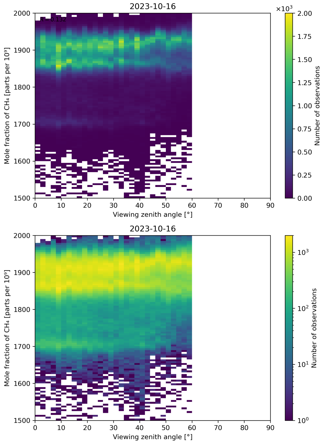
Figure 110: Scatter density plot of “Viewing zenith angle” against “Mole fraction of CH 4 ” for 2023-10-15 to 2023-10-17.
