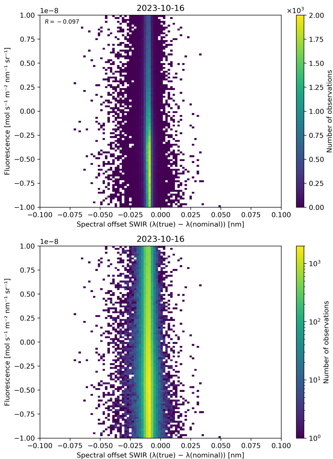
Figure 120: Scatter density plot of “Spectral offset SWIR ( \lambda(\text{true}) - \lambda(\text{nominal}) )” against “Fluorescence” for 2023-10-15 to 2023-10-17.
