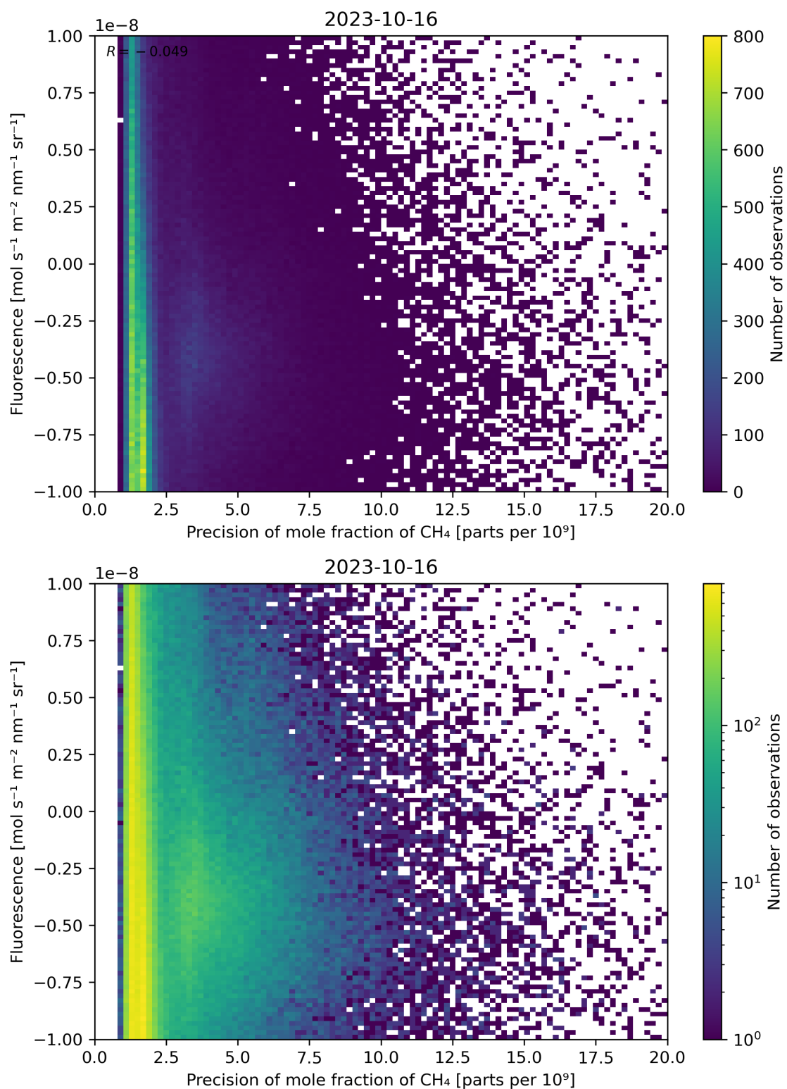
Figure 81: Scatter density plot of “Precision of mole fraction of \text{CH}_4 ” against “Fluorescence” for 2023-10-15 to 2023-10-17.
