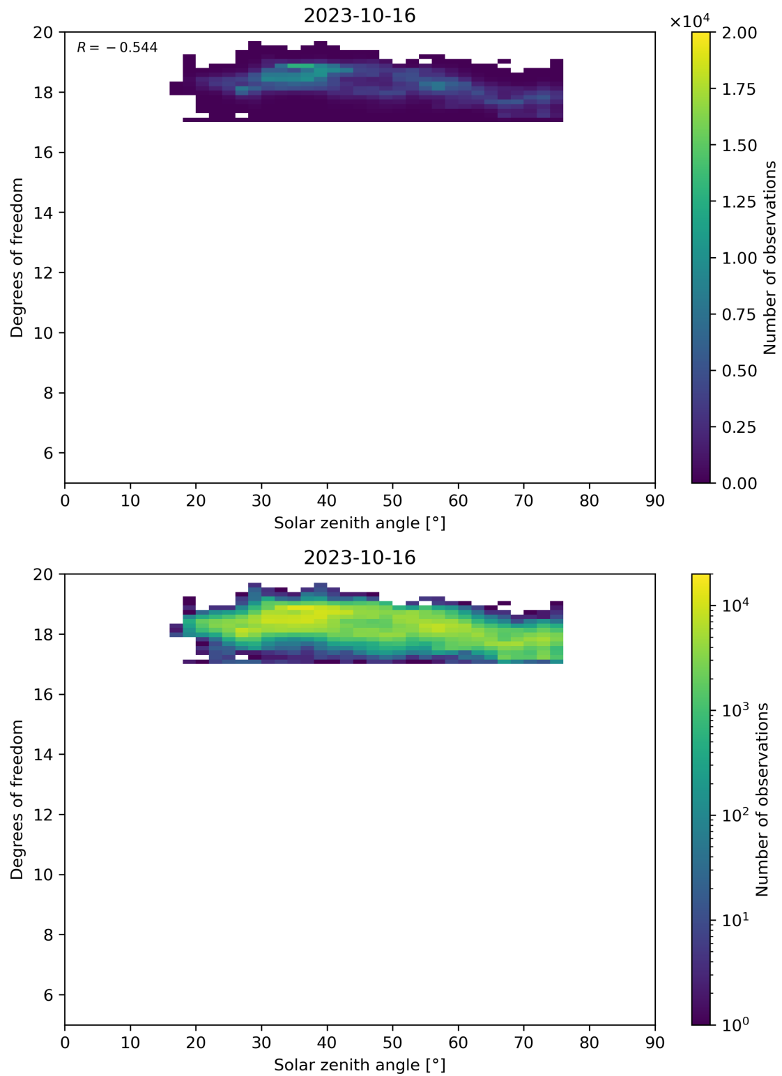
Figure 96: Scatter density plot of “Solar zenith angle” against “Degrees of freedom” for 2023-10-15 to 2023-10-17.
