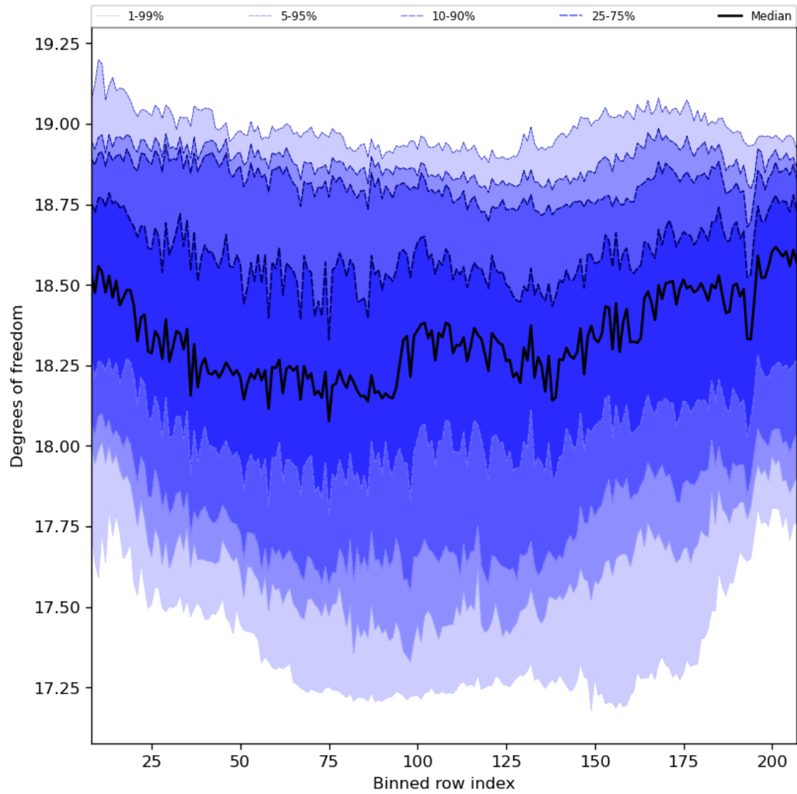
Figure 41: Along track statistics of “Degrees of freedom” for 2023-10-15 to 2023-10-17
