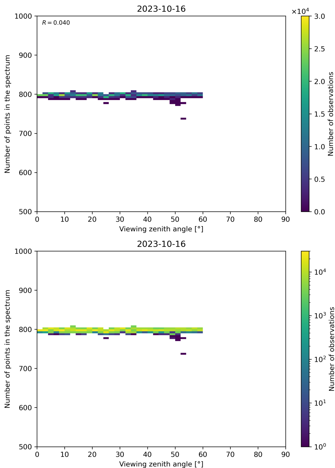
Figure 114: Scatter density plot of “Viewing zenith angle” against “Number of points in the spectrum” for 2023-10-15 to 2023-10-17.
