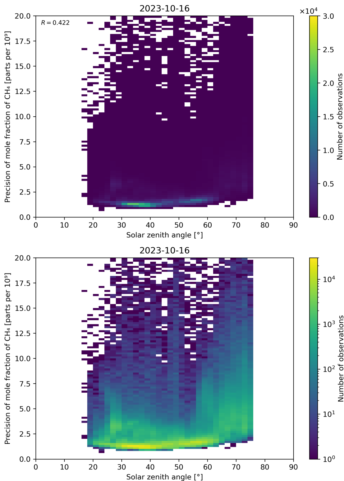
Figure 101: Scatter density plot of “Solar zenith angle” against “Precision of mole fraction of CH 4 ” for 2023-10-15 to 2023-10-17.
