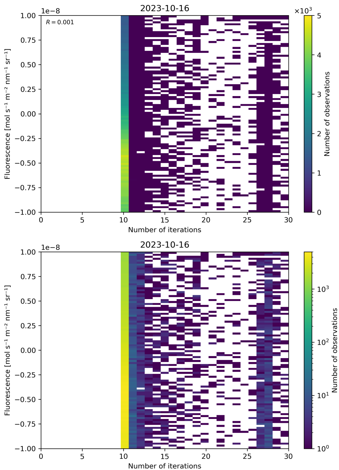
Figure 87: Scatter density plot of “Number of iterations” against “Fluorescence” for 2023-10-15 to 2023-10-17.
