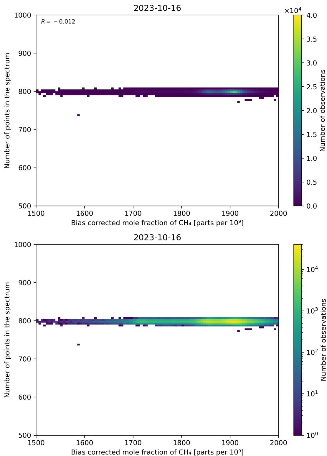
Figure 68: Scatter density plot of “Bias corrected mole fraction of CH 4 ” against “Number of points in the spectrum” for 2023-10-15 to 2023-10-17.
