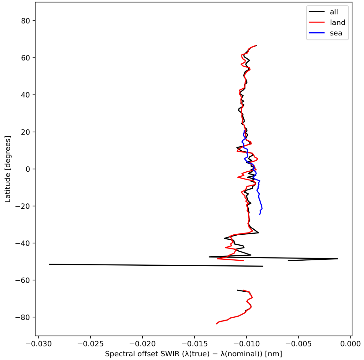
Figure 16: Zonal average of “Spectral offset SWIR ( \lambda(\text{true}) - \lambda(\text{nominal}) )” for 2023-10-15 to 2023-10-17.
