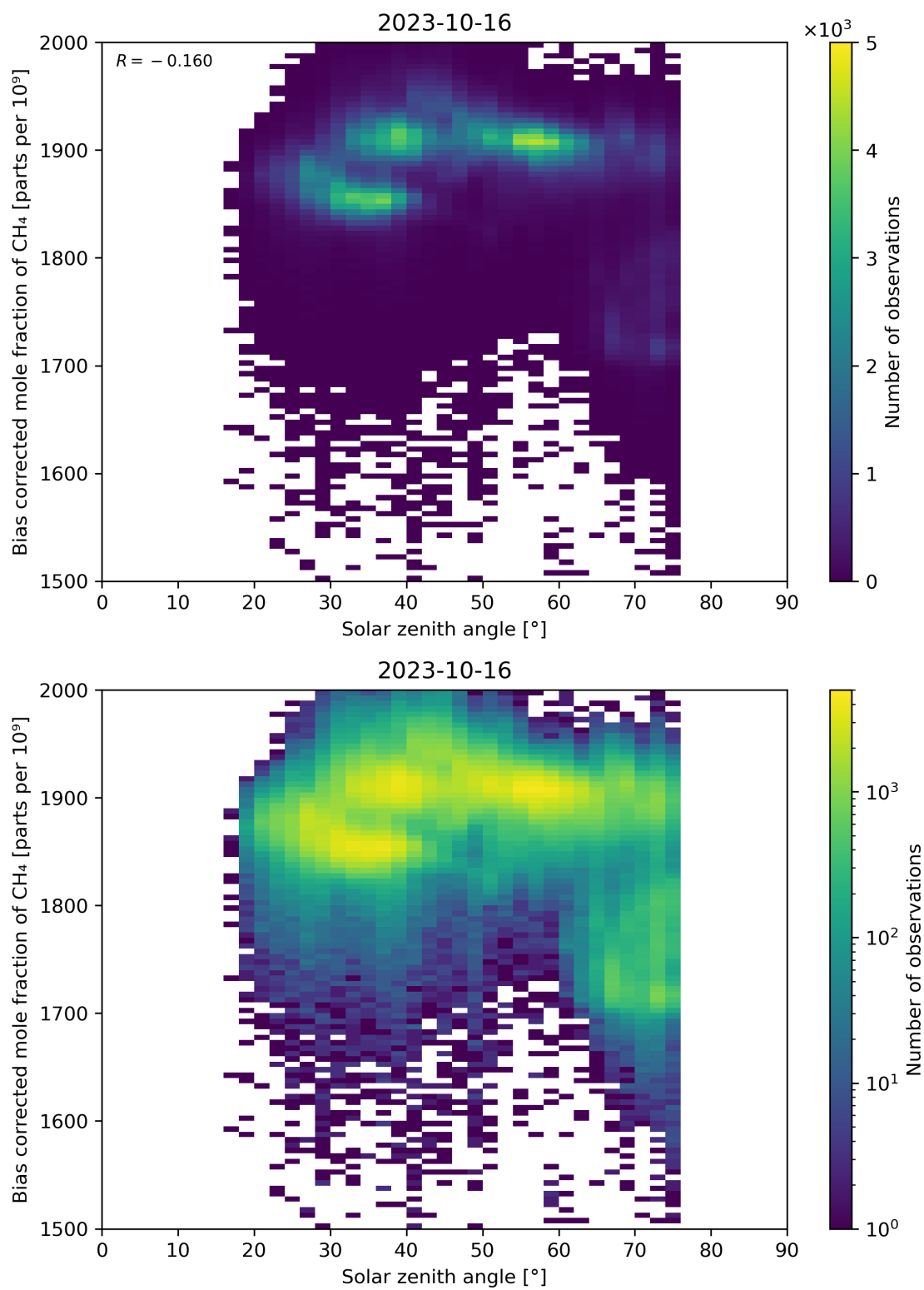
Figure 100: Scatter density plot of “Solar zenith angle” against “Bias corrected mole fraction of \text{CH}_4 ” for 2023-10-15 to 2023-10-17.
