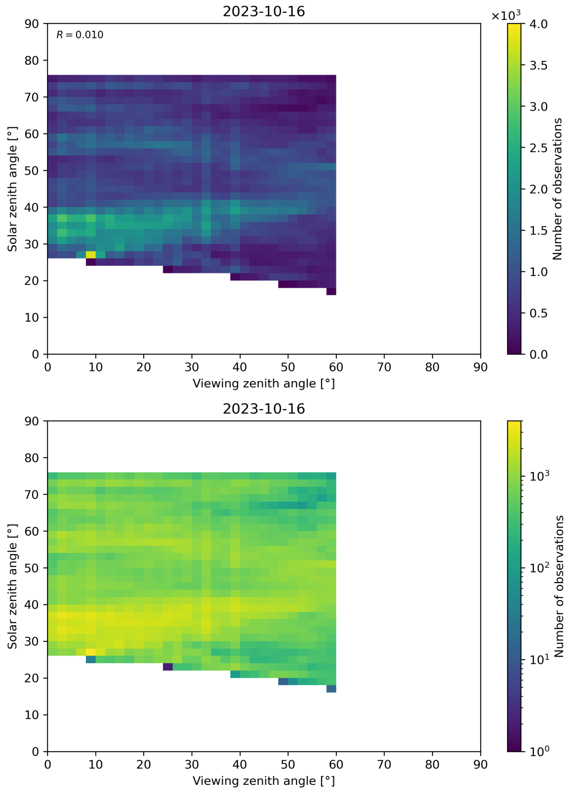
Figure 115: Scatter density plot of “Viewing zenith angle” against “Solar zenith angle” for 2023-10-15 to 2023-10-17.
