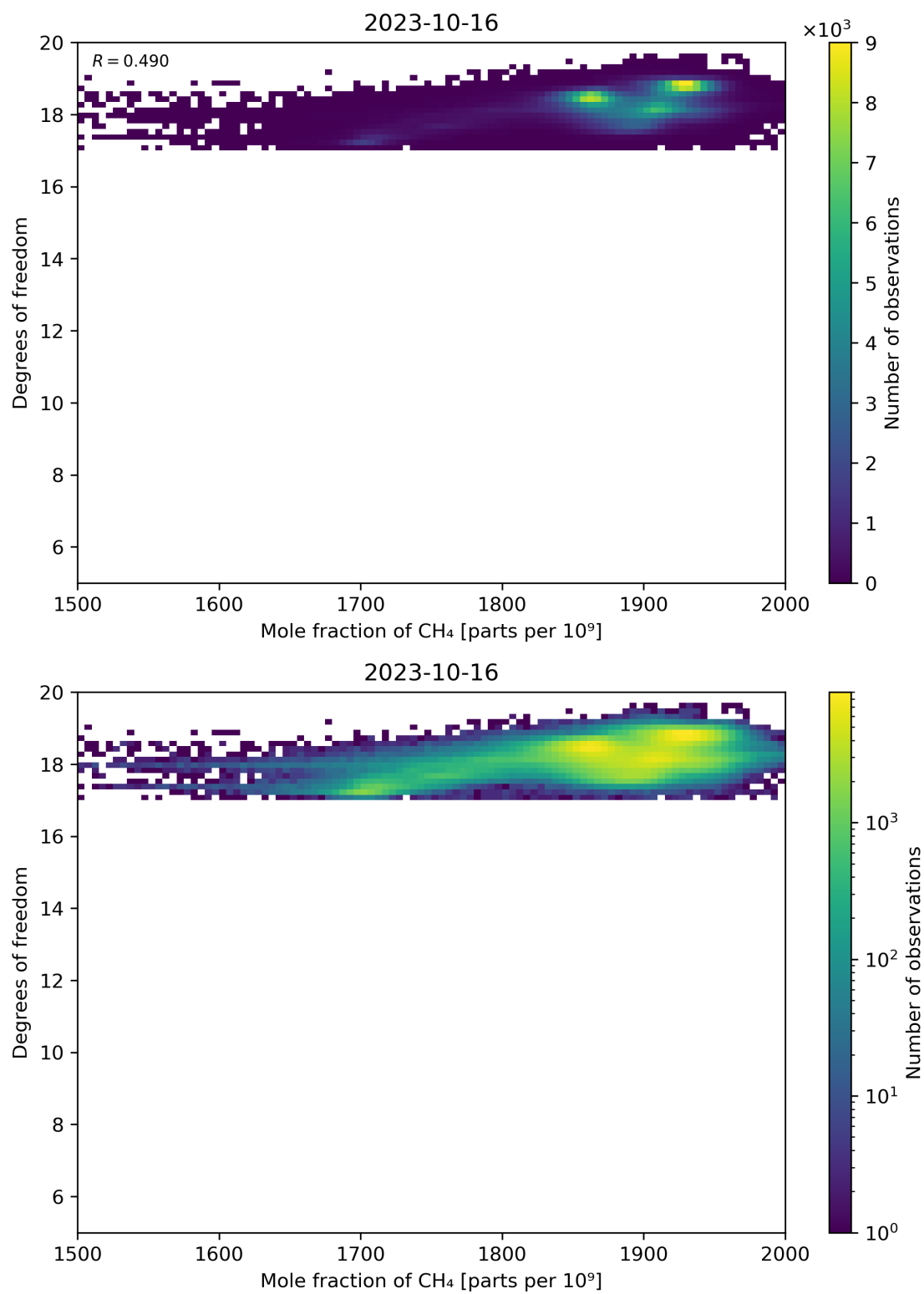
Figure 72: Scatter density plot of “Mole fraction of CH 4 ” against “Degrees of freedom” for 2023-10-15 to 2023-10-17.
