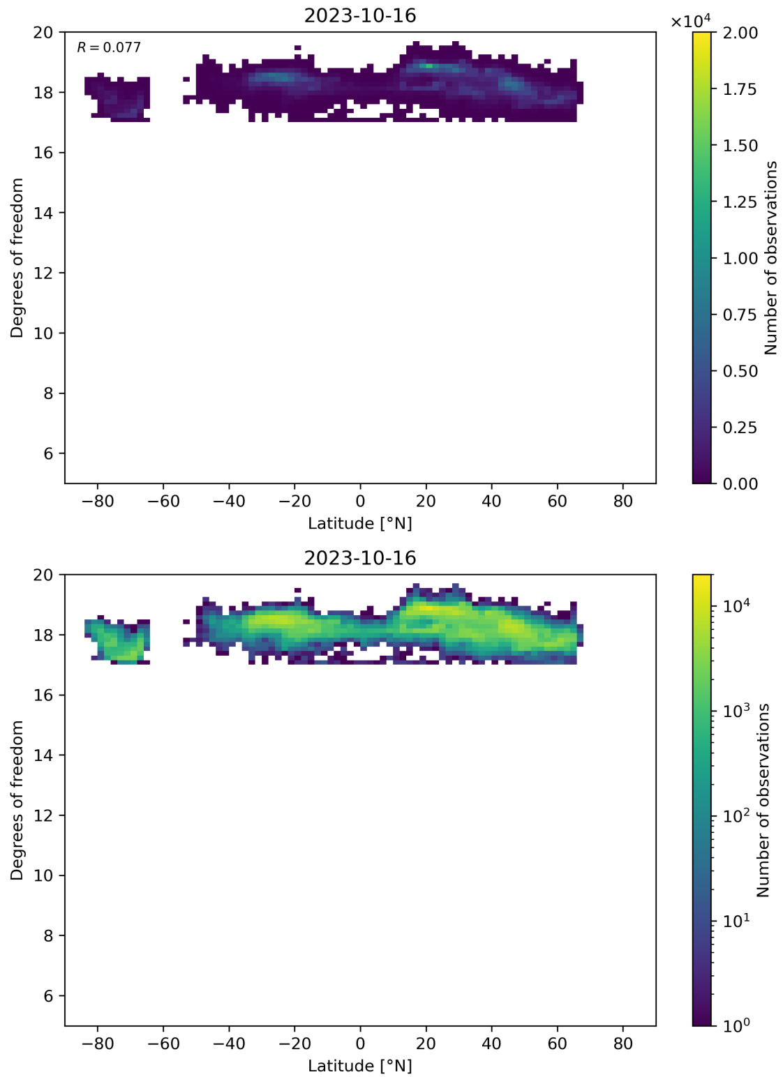
Figure 55: Scatter density plot of “Latitude” against “Degrees of freedom” for 2023-10-15 to 2023-10-17.
