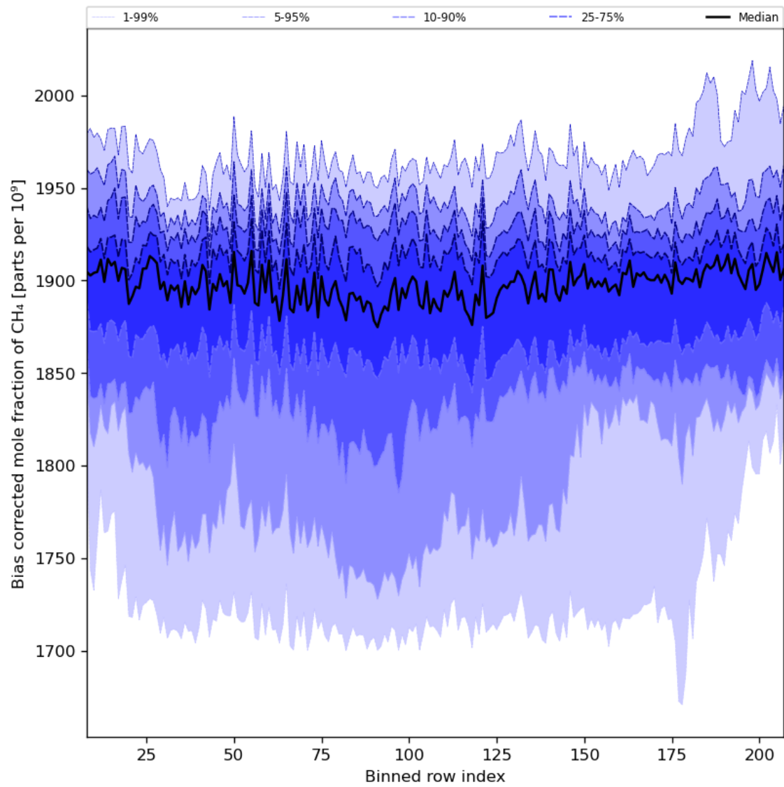
Figure 36: Along track statistics of “Bias corrected mole fraction of CH 4 ” for 2023-10-15 to 2023-10-17
