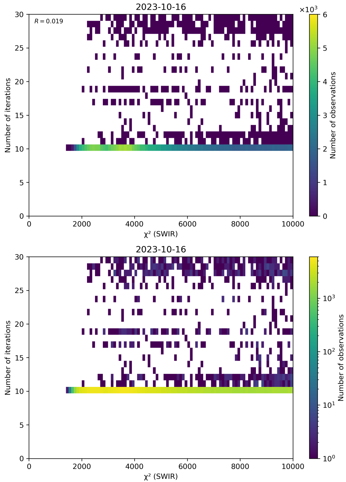
Figure 50: Scatter density plot of “ \chi^2 (SWIR)” against “Number of iterations” for 2023-10-15 to 2023-10-17.
