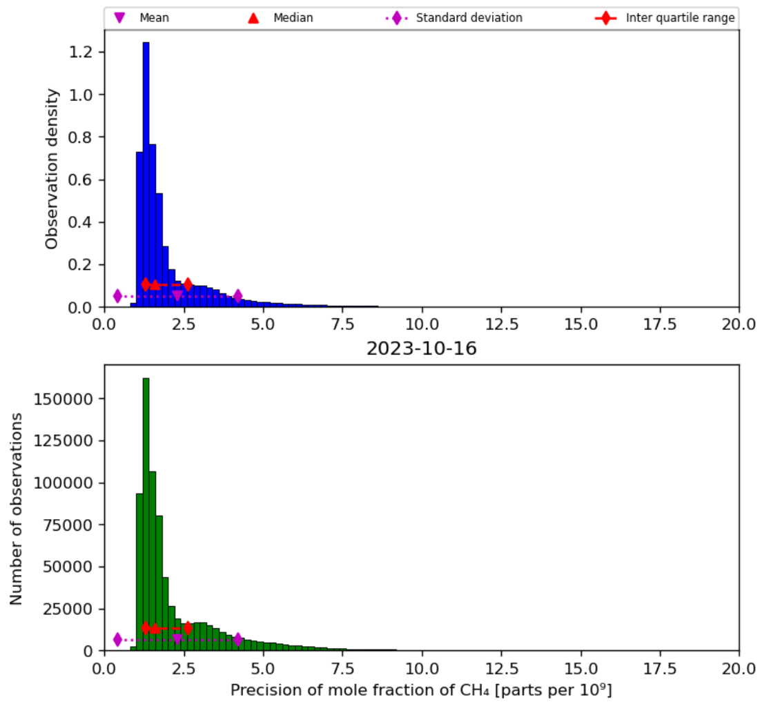
Figure 24: Histogram of “Precision of mole fraction of CH 4 ” for 2023-10-15 to 2023-10-17
