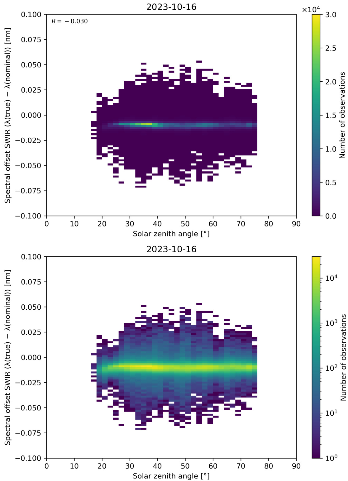
Figure 104: Scatter density plot of “Solar zenith angle” against “Spectral offset SWIR ( \lambda(\text{true}) - \lambda(\text{nominal}) )” for 2023-10-15 to 2023-10-17.
