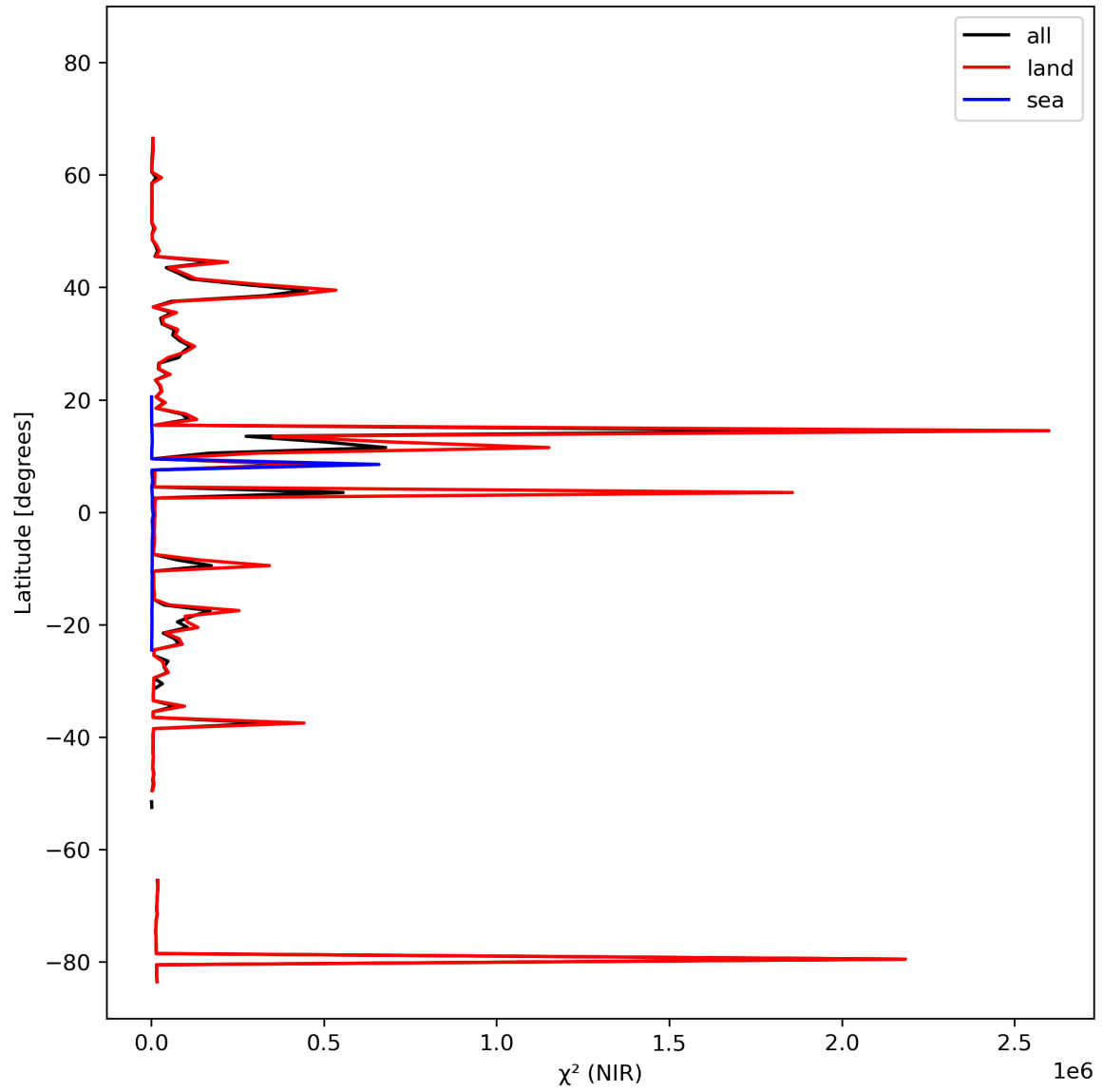
Figure 18: Zonal average of “ \chi^2 (NIR)” for 2023-10-15 to 2023-10-17.
