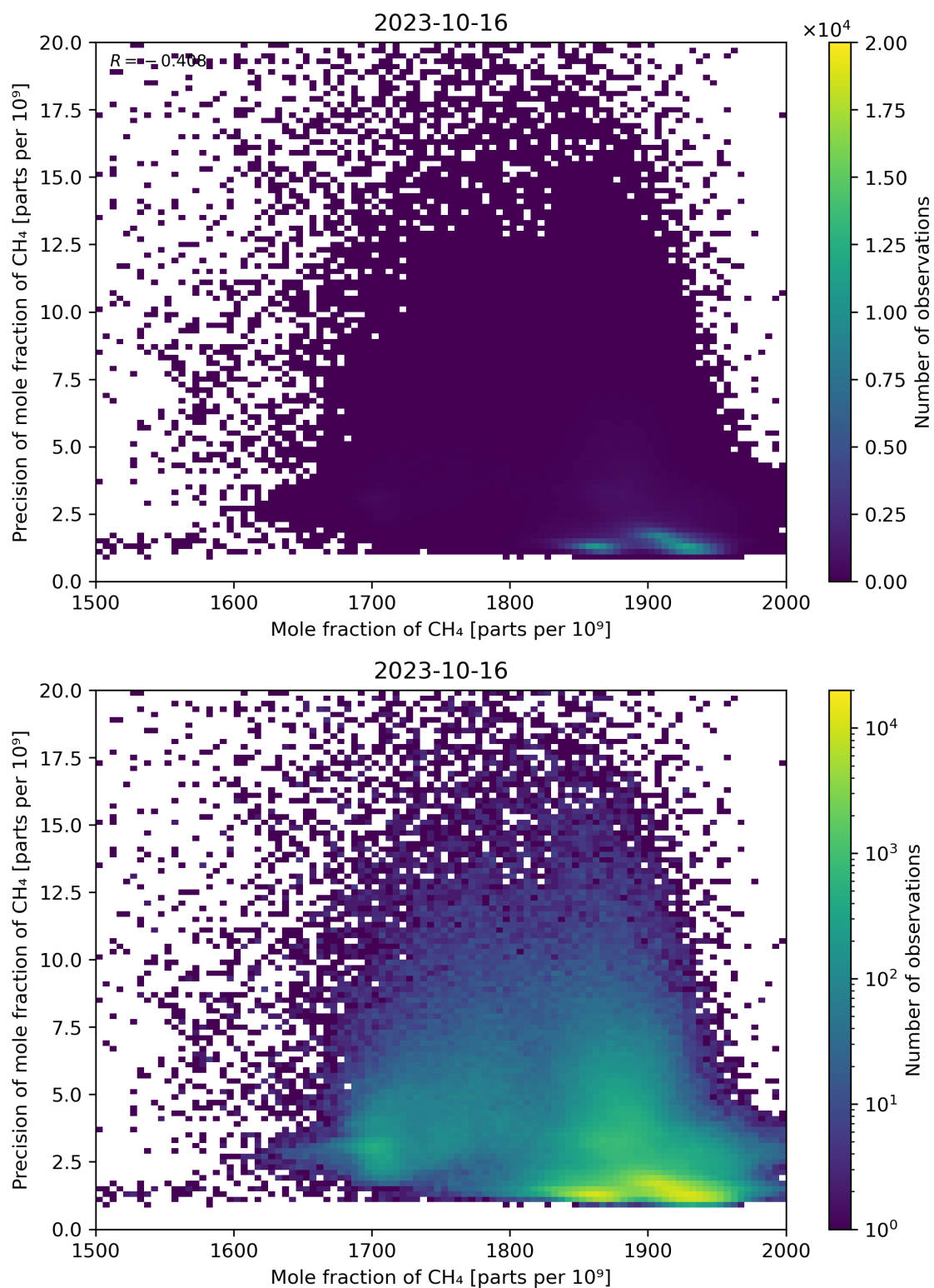
Figure 75: Scatter density plot of “Mole fraction of CH 4 ” against “Precision of mole fraction of CH 4 ” for 2023-10-15 to 2023-10-17.
