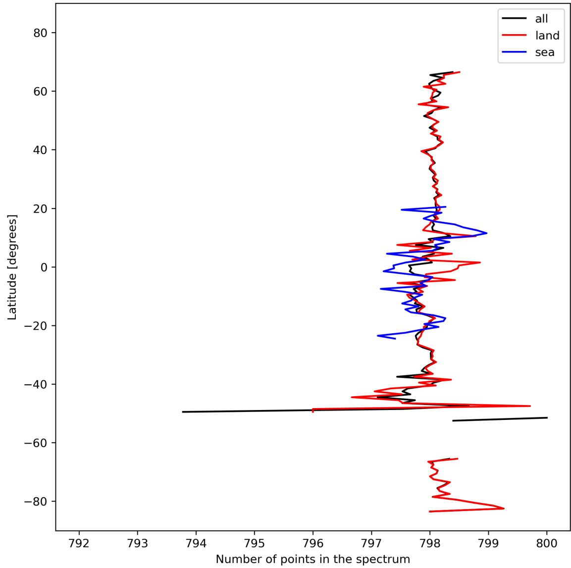
Figure 15: Zonal average of “Number of points in the spectrum” for 2023-10-15 to 2023-10-17.
