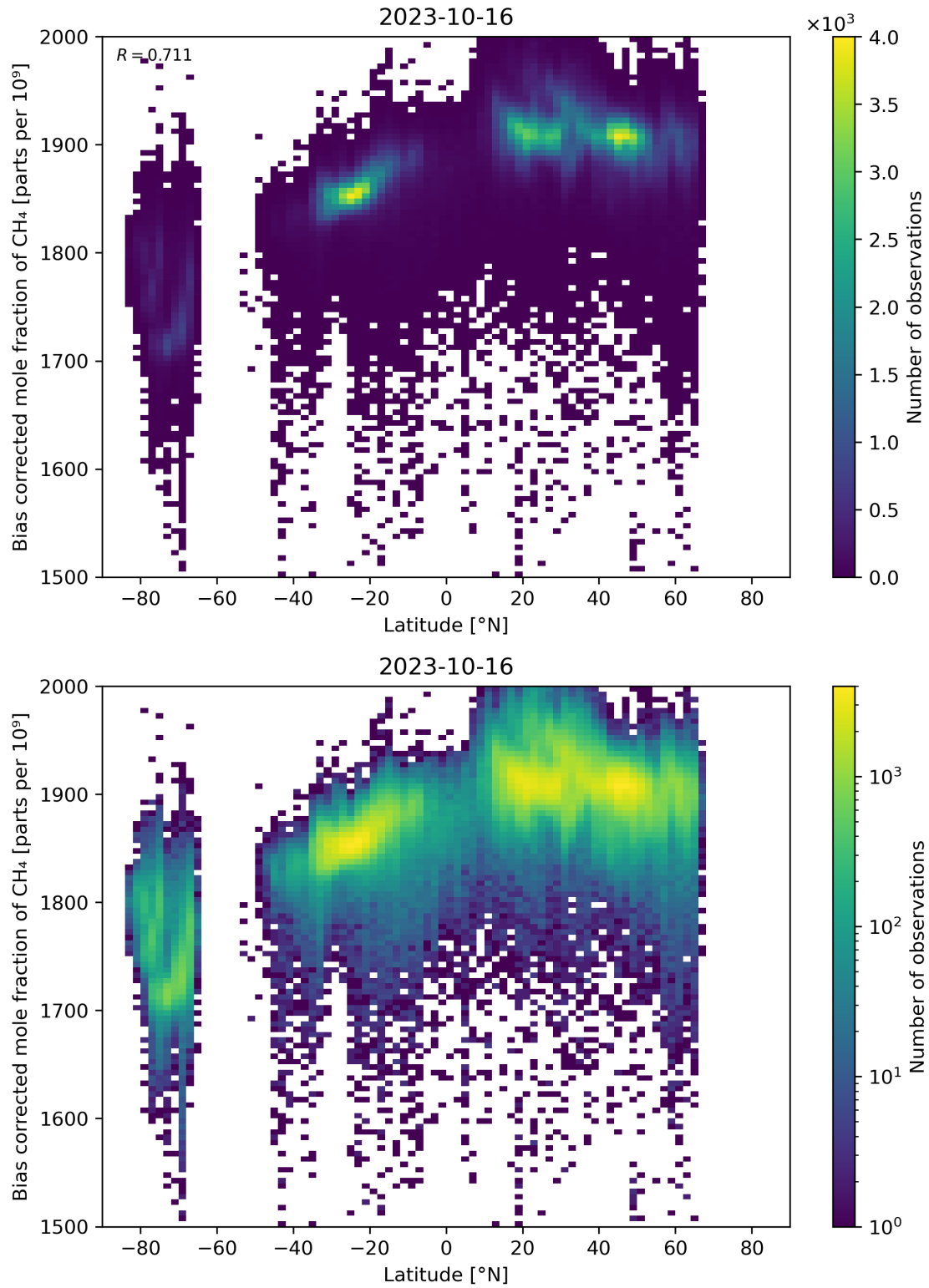
Figure 58: Scatter density plot of “Latitude” against “Bias corrected mole fraction of \text{CH}_4 ” for 2023-10-15 to 2023-10-17.
