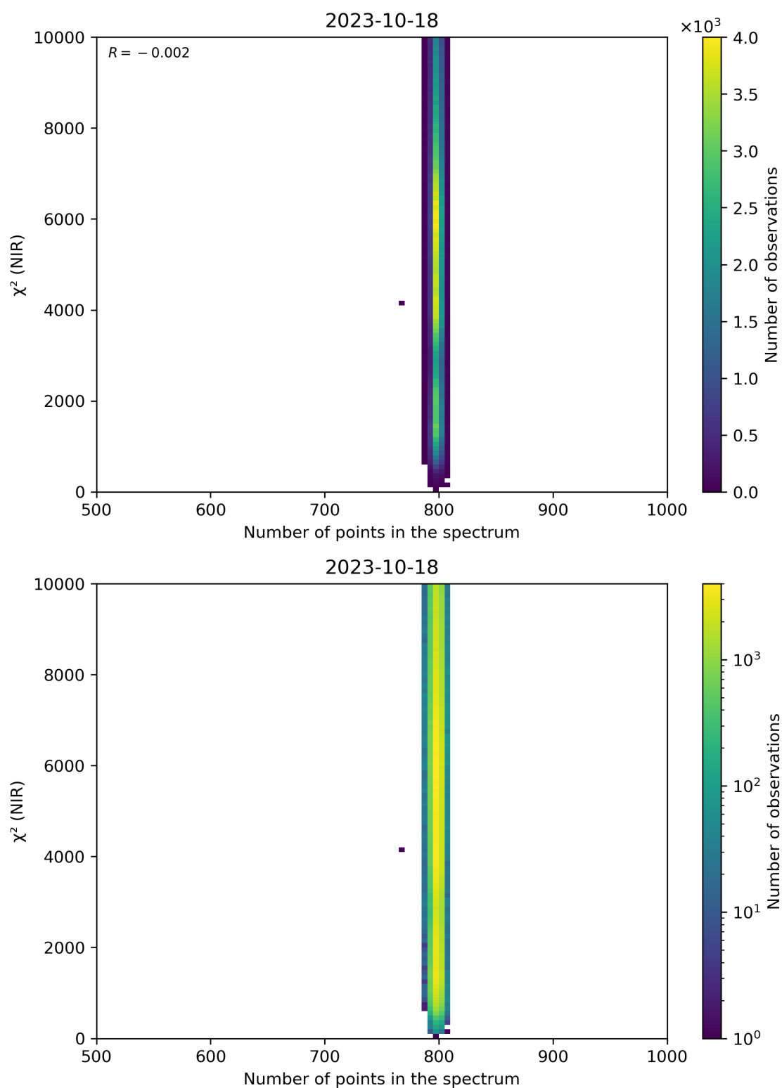
Figure 88: Scatter density plot of “Number of points in the spectrum” against “ \chi^2 (NIR)” for 2023-10-17 to 2023-10-19.
