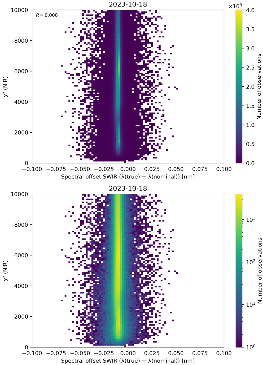
Figure 117: Scatter density plot of “Spectral offset SWIR ( \lambda(\text{true}) - \lambda(\text{nominal}) )” against “ \chi^2 (NIR)” for 2023-10-17 to 2023-10-19.
