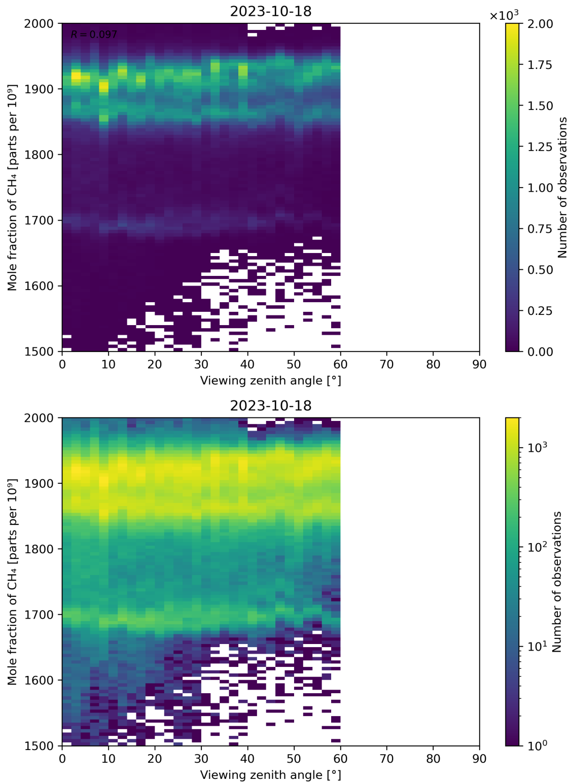
Figure 110: Scatter density plot of “Viewing zenith angle” against “Mole fraction of \text{CH}_4 ” for 2023-10-17 to 2023-10-19.
