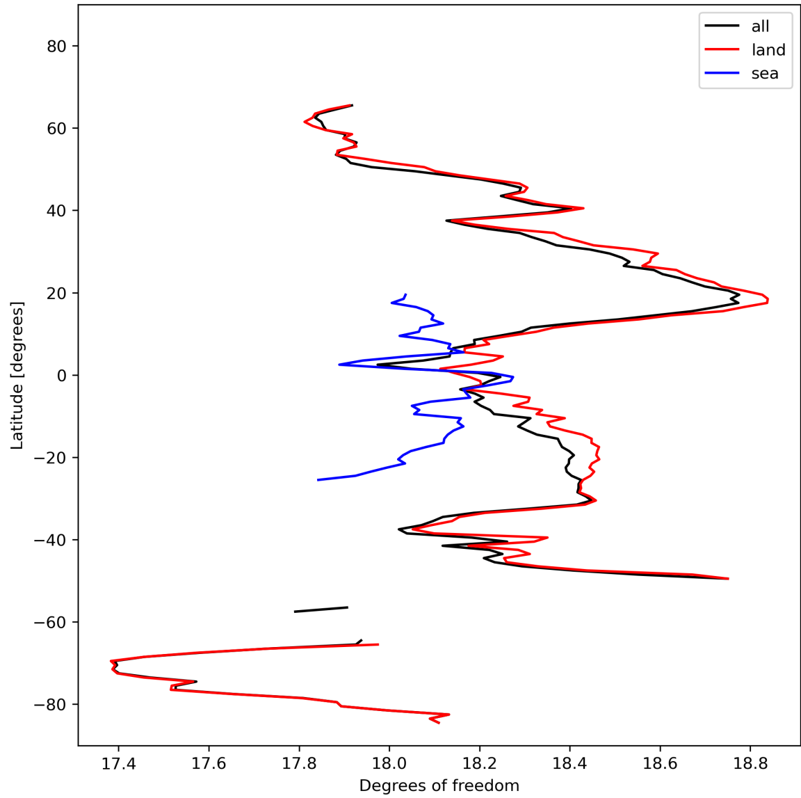
Figure 19: Zonal average of “Degrees of freedom” for 2023-10-17 to 2023-10-19.
