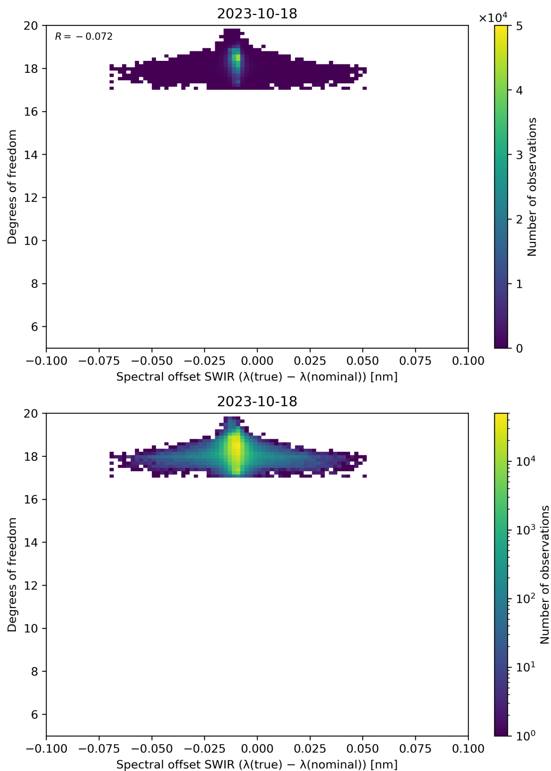
Figure 119: Scatter density plot of “Spectral offset SWIR ( \lambda(\text{true}) - \lambda(\text{nominal}) )” against “Degrees of freedom” for 2023-10-17 to 2023-10-19.
