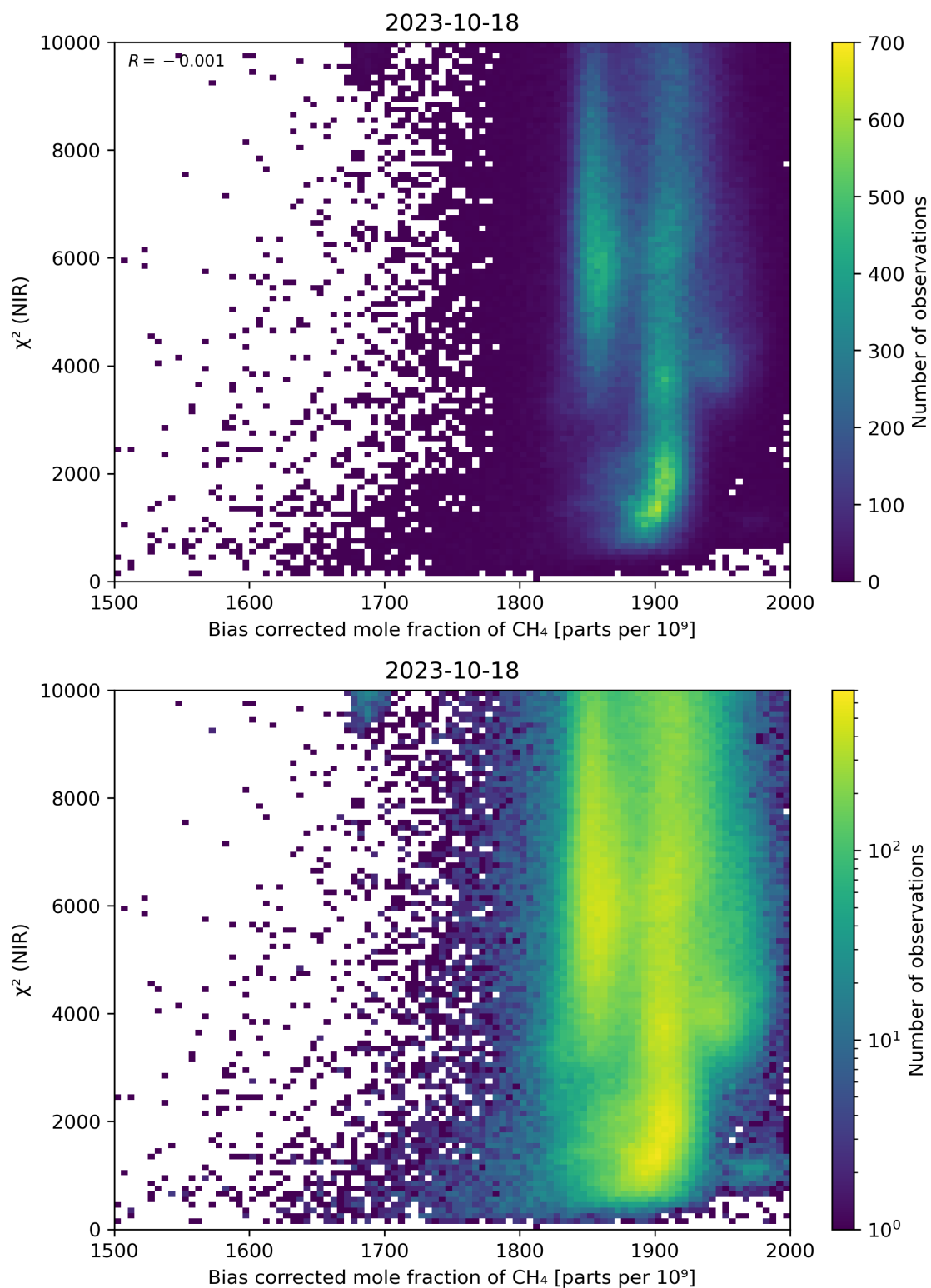
Figure 63: Scatter density plot of “Bias corrected mole fraction of CH 4 ” against “ \chi^2 (NIR)” for 2023-10-17 to 2023-10-19.
