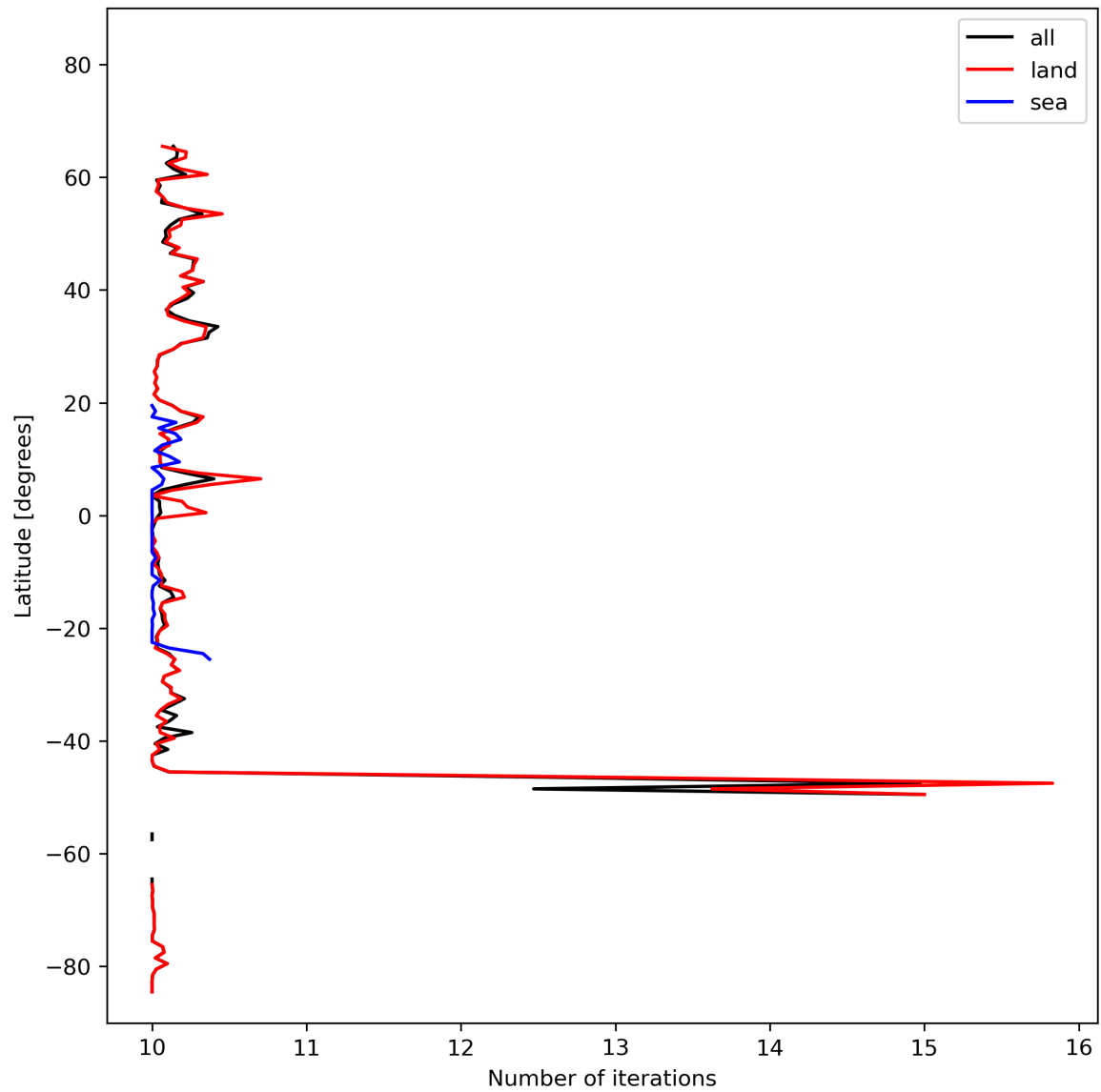
Figure 20: Zonal average of “Number of iterations” for 2023-10-17 to 2023-10-19.
