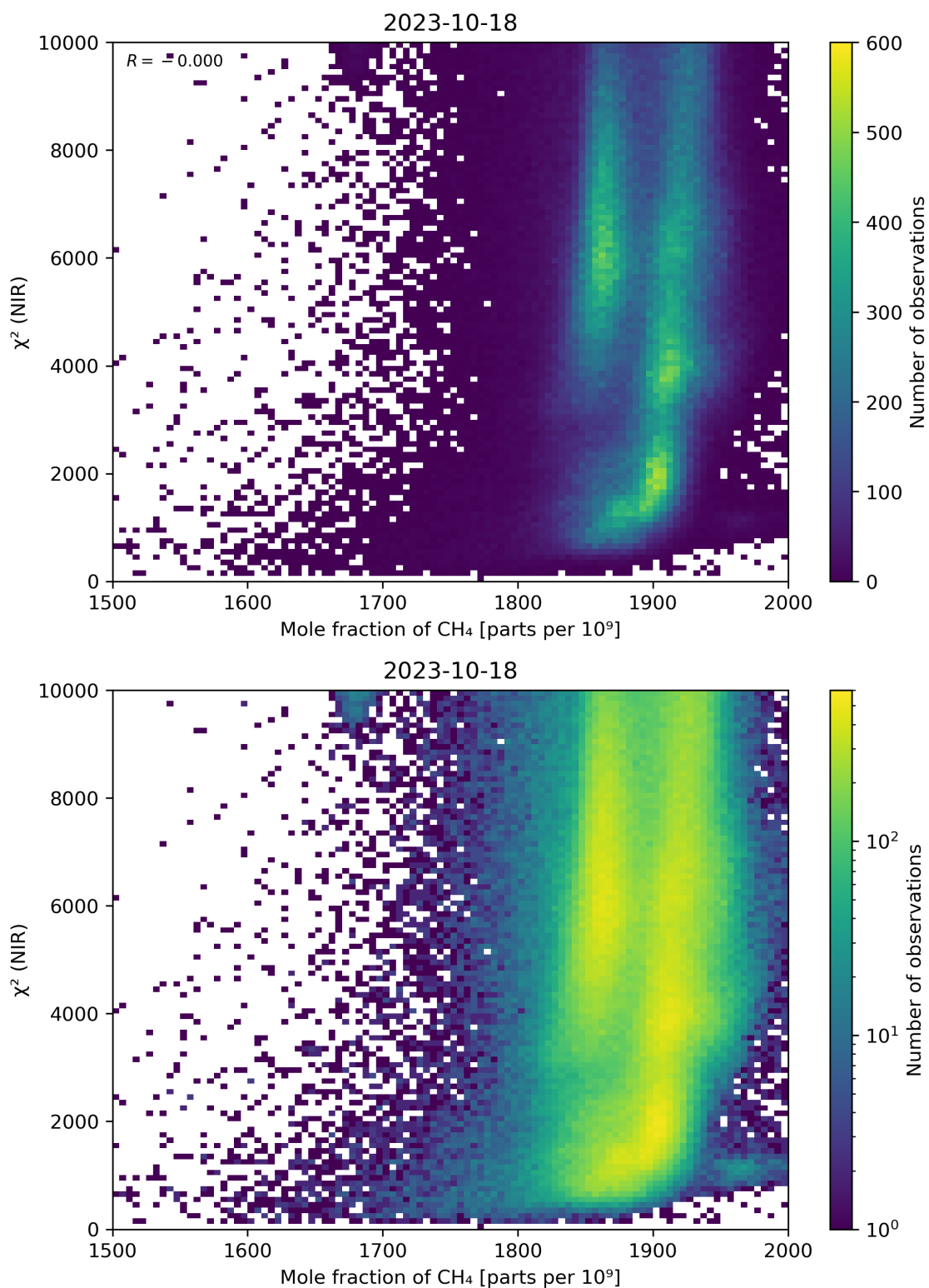
Figure 70: Scatter density plot of “Mole fraction of CH 4 ” against “ \chi^2 (NIR)” for 2023-10-17 to 2023-10-19.
