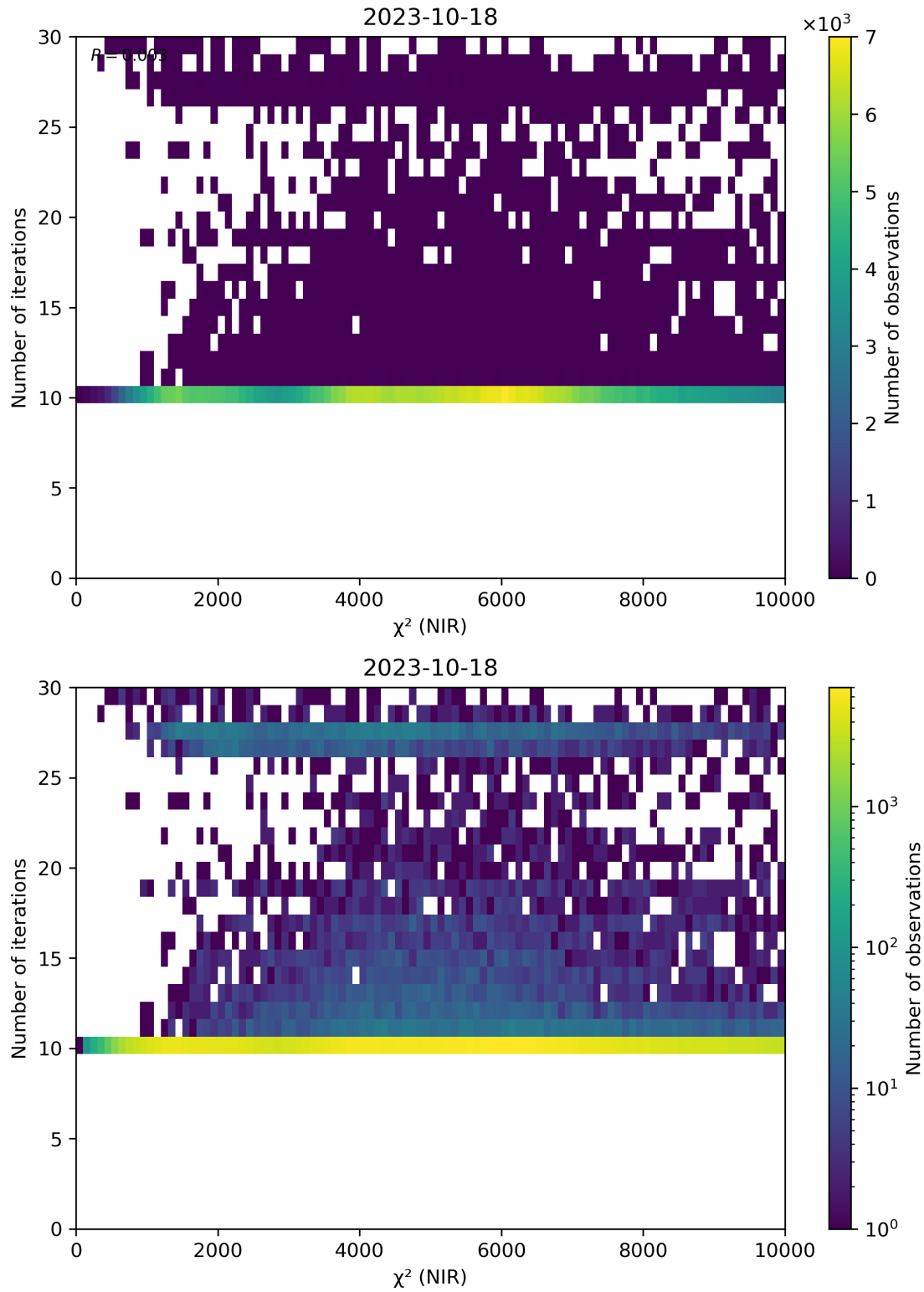
Figure 46: Scatter density plot of “ \chi^2 (NIR)” against “Number of iterations” for 2023-10-17 to 2023-10-19.
