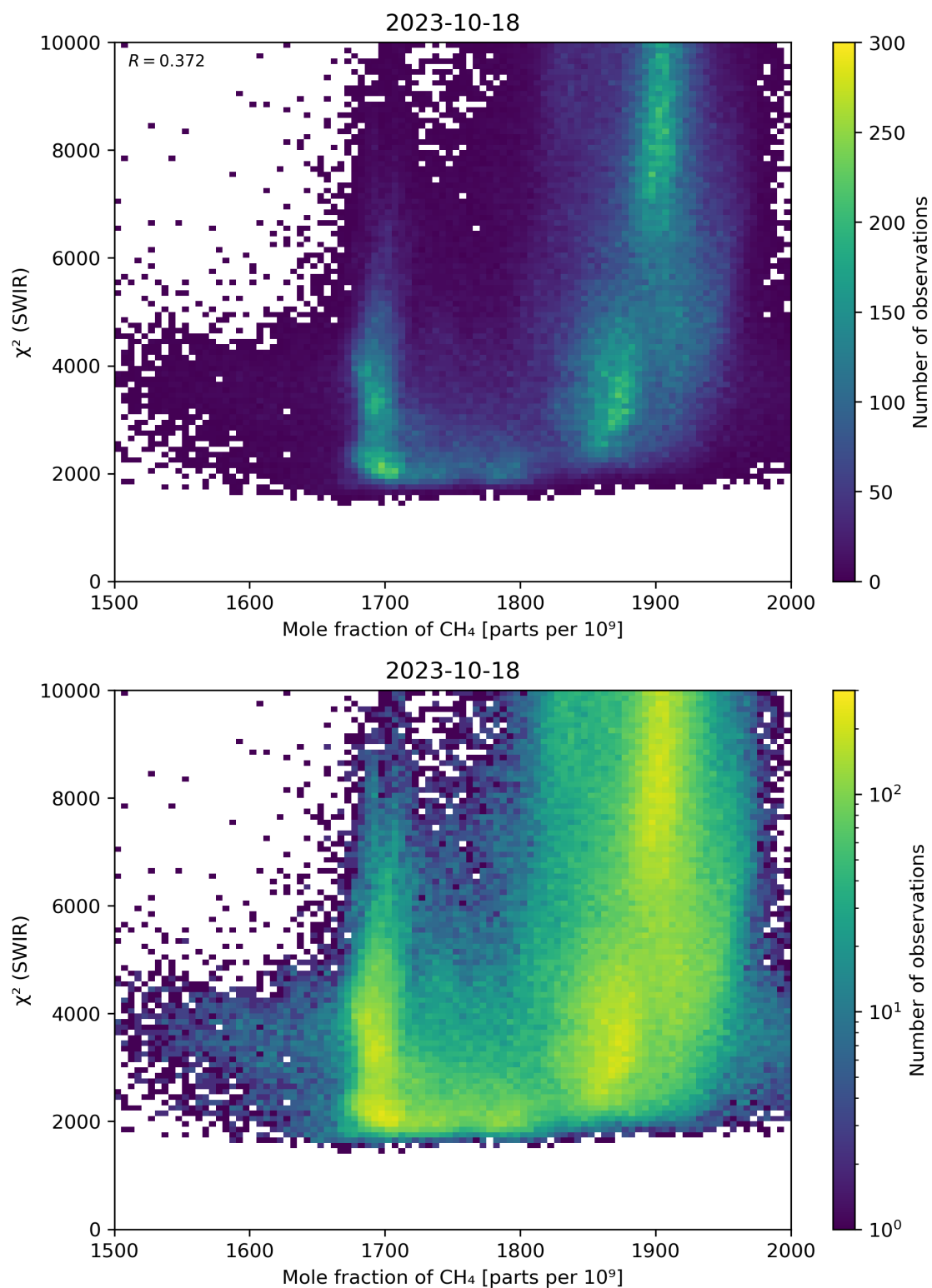
Figure 71: Scatter density plot of “Mole fraction of \text{CH}_4 ” against “ \chi^2 (SWIR)” for 2023-10-17 to 2023-10-19.
