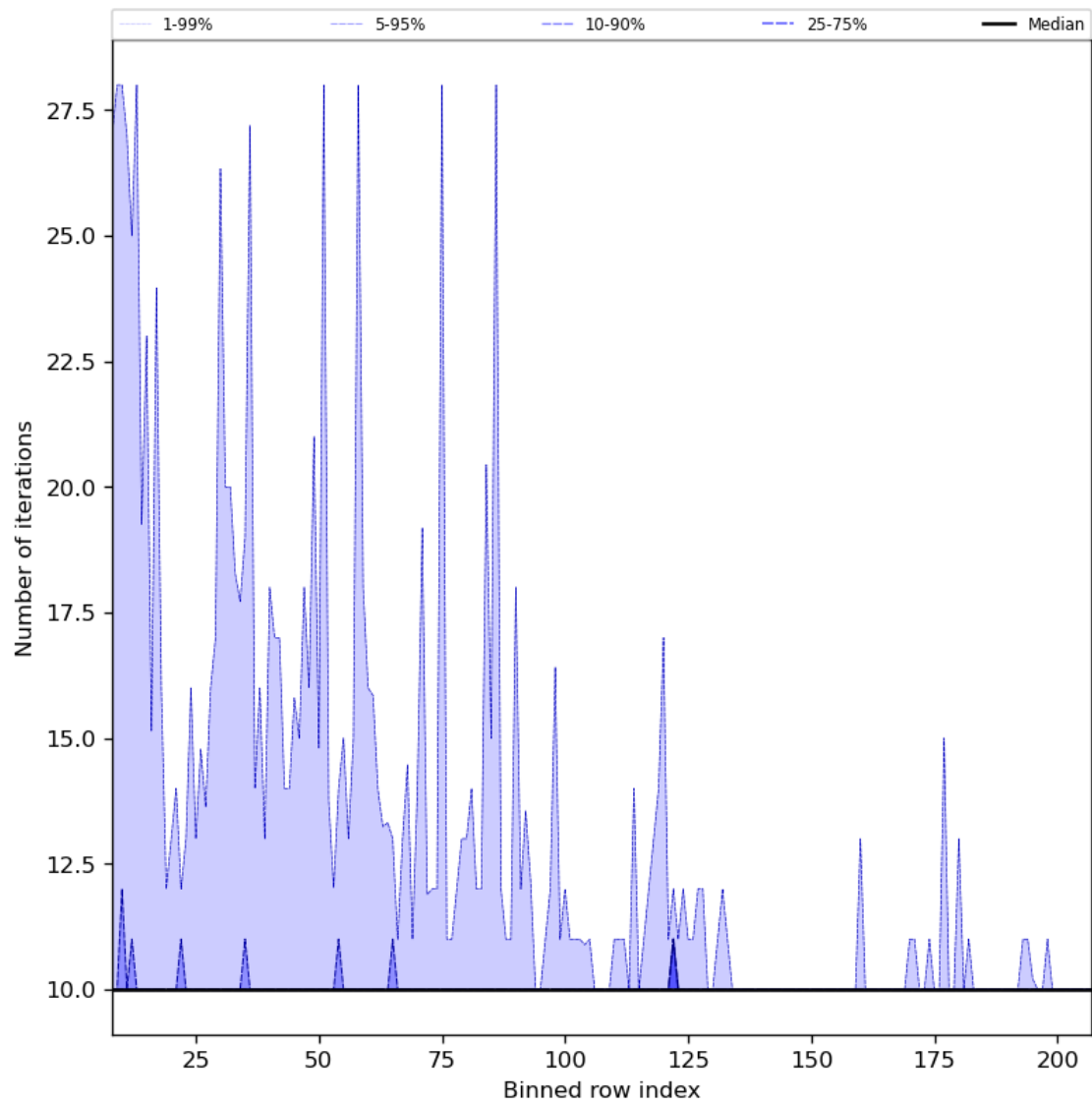
Figure 42: Along track statistics of “Number of iterations” for 2023-10-17 to 2023-10-19
