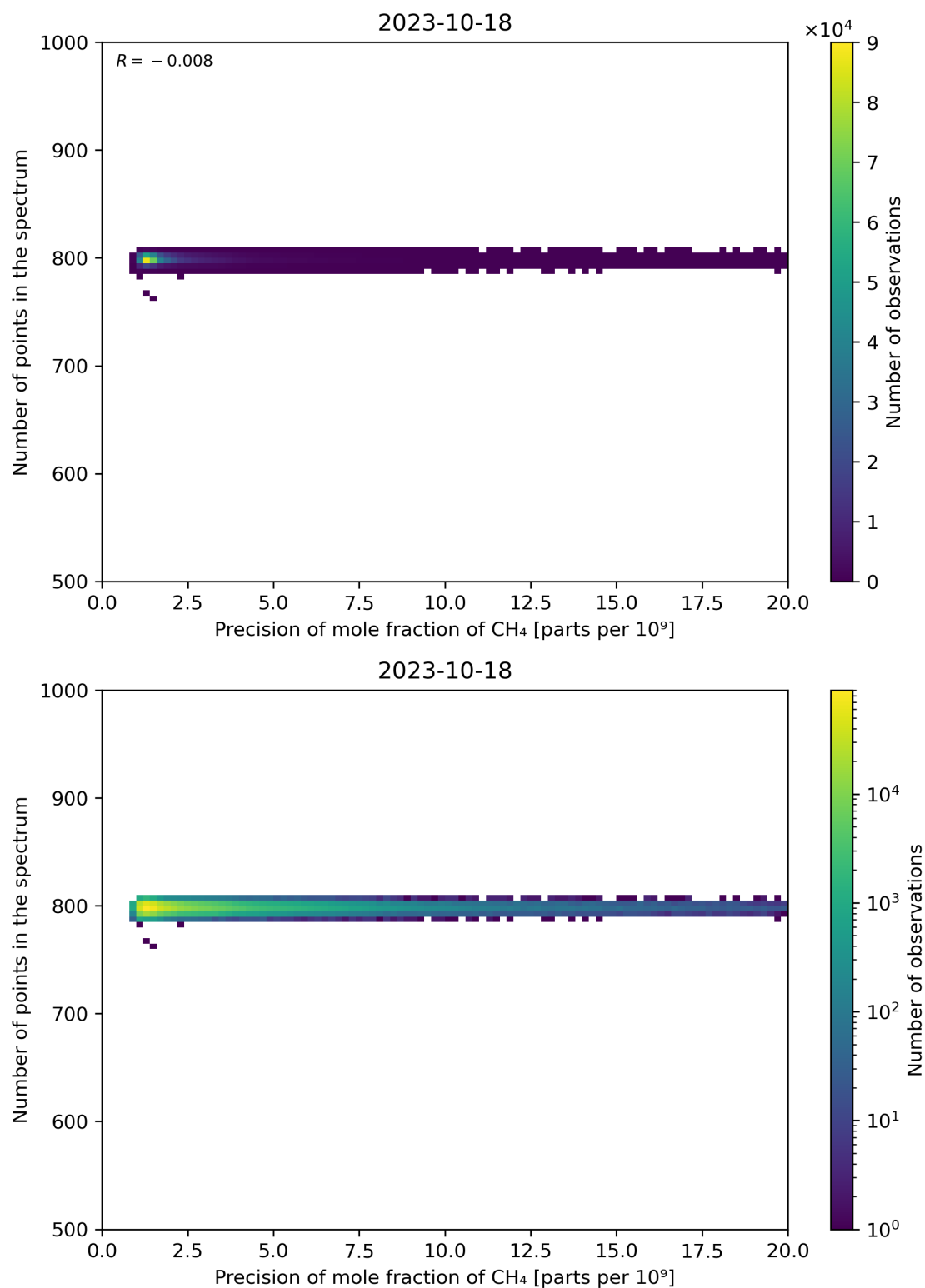
Figure 84: Scatter density plot of “Precision of mole fraction of CH 4 ” against “Number of points in the spectrum” for 2023-10-17 to 2023-10-19.
