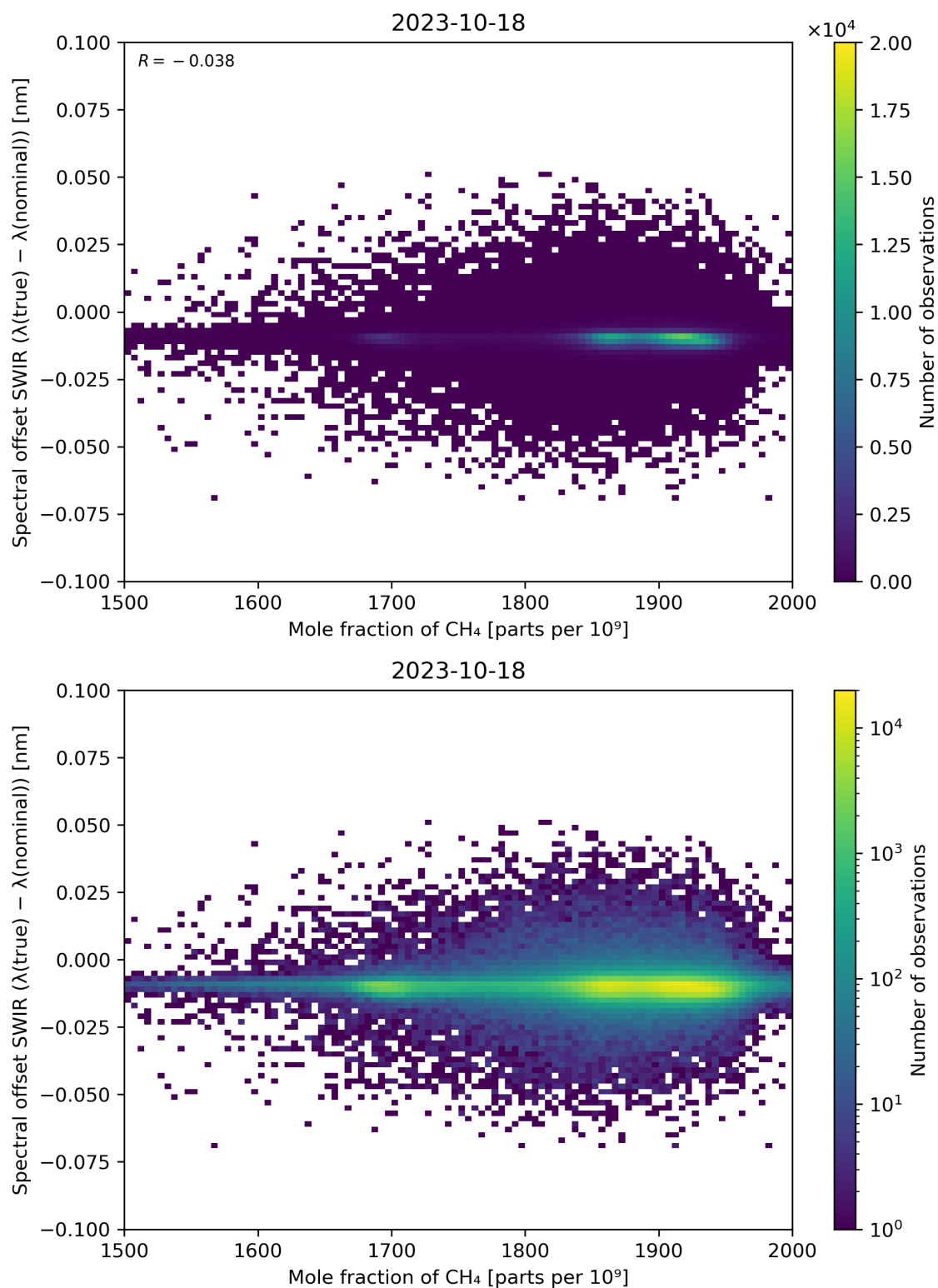
Figure 86: Scatter density plot of “Mole fraction of CH 4 ” against “Spectral offset SWIR ( \lambda(\text{true}) - \lambda(\text{nominal}) )” for 2023-10-17 to 2023-10-19.
