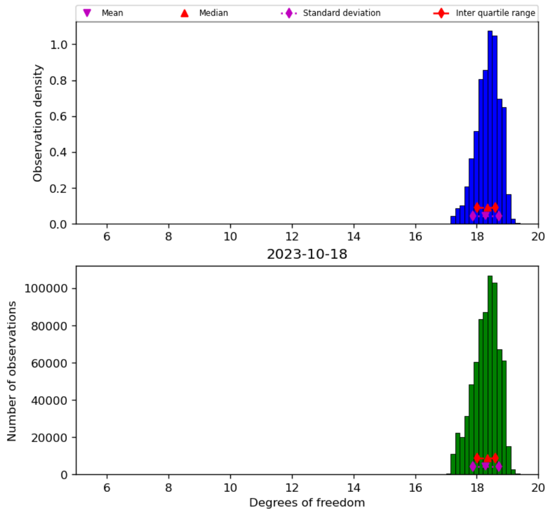
Figure 30: Histogram of “Degrees of freedom” for 2023-10-17 to 2023-10-19
