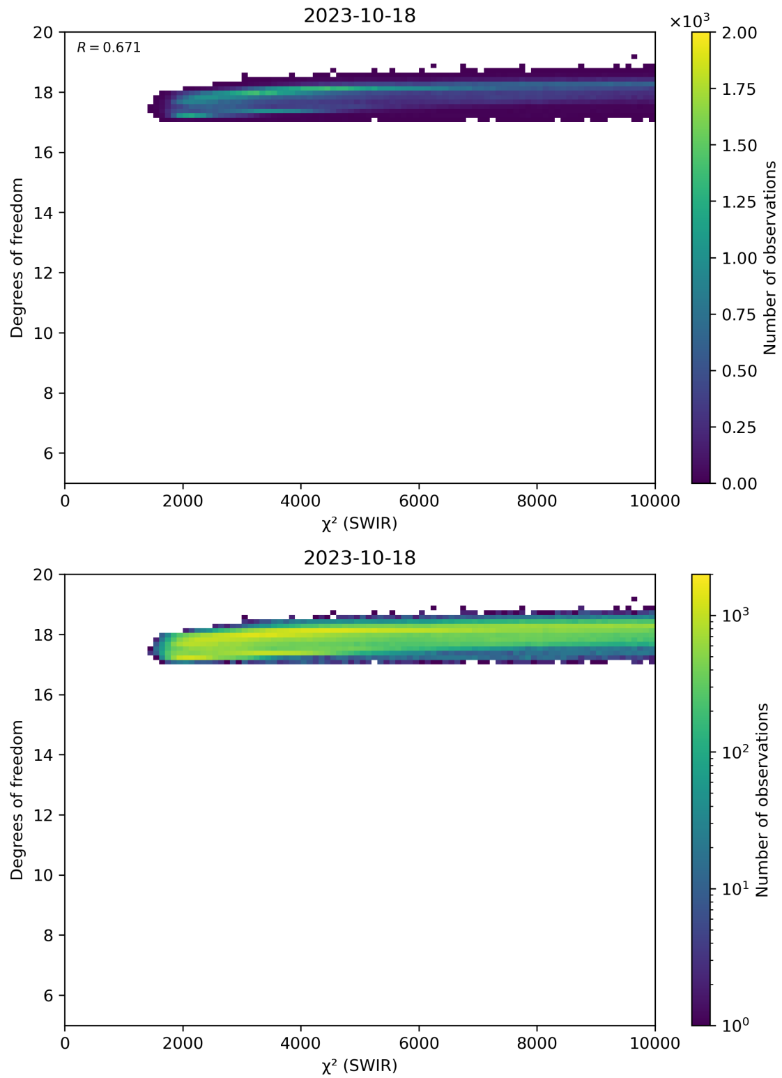
Figure 48: Scatter density plot of “ \chi^2 (SWIR)” against “Degrees of freedom” for 2023-10-17 to 2023-10-19.
