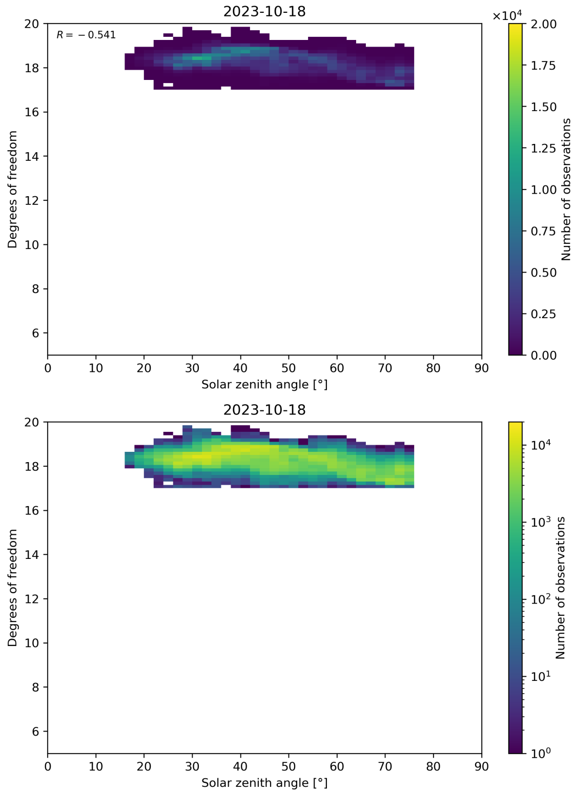
Figure 96: Scatter density plot of “Solar zenith angle” against “Degrees of freedom” for 2023-10-17 to 2023-10-19.
