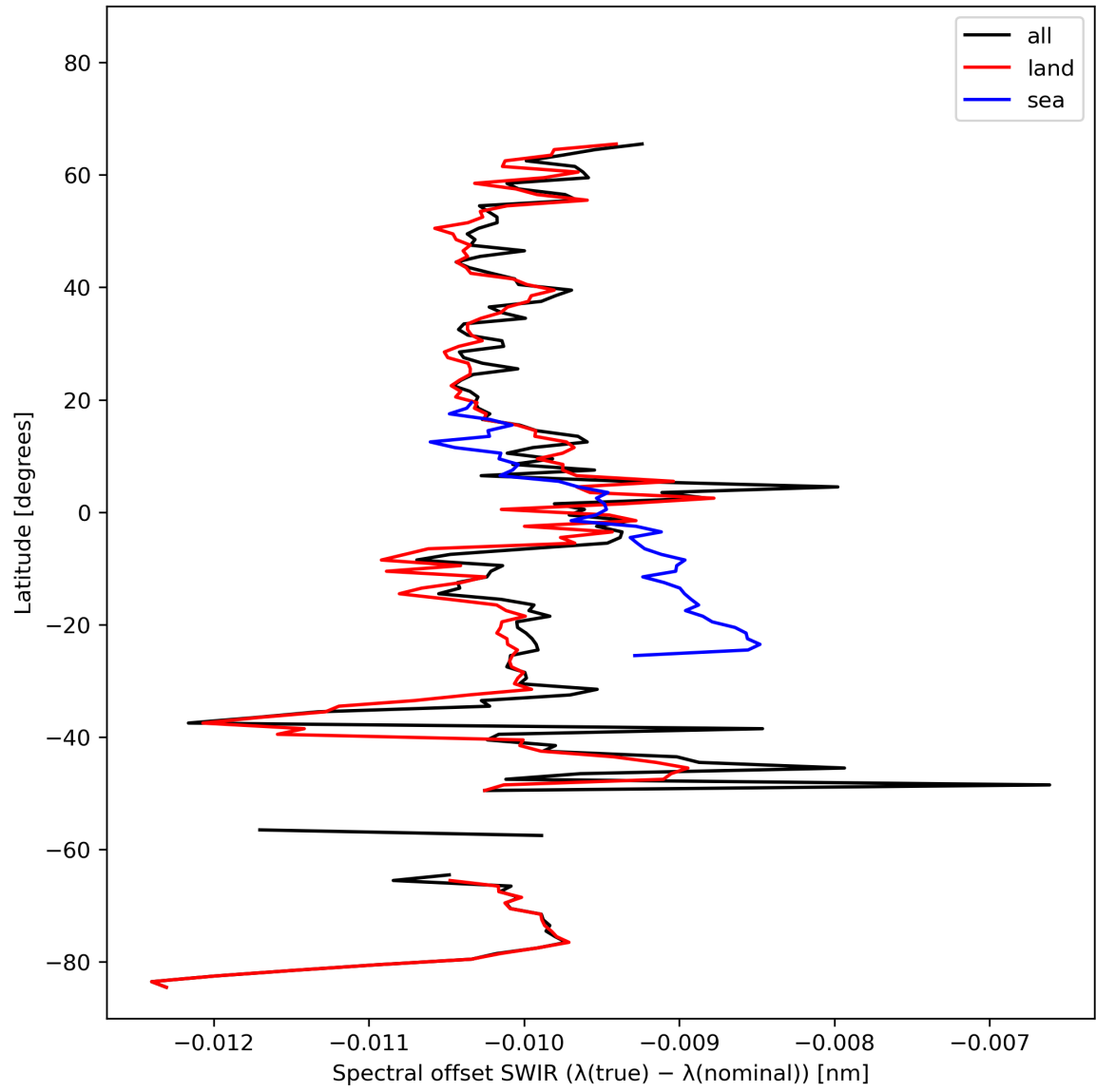
Figure 16: Zonal average of “Spectral offset SWIR ( \lambda(\text{true}) - \lambda(\text{nominal}) )” for 2023-10-17 to 2023-10-19.
