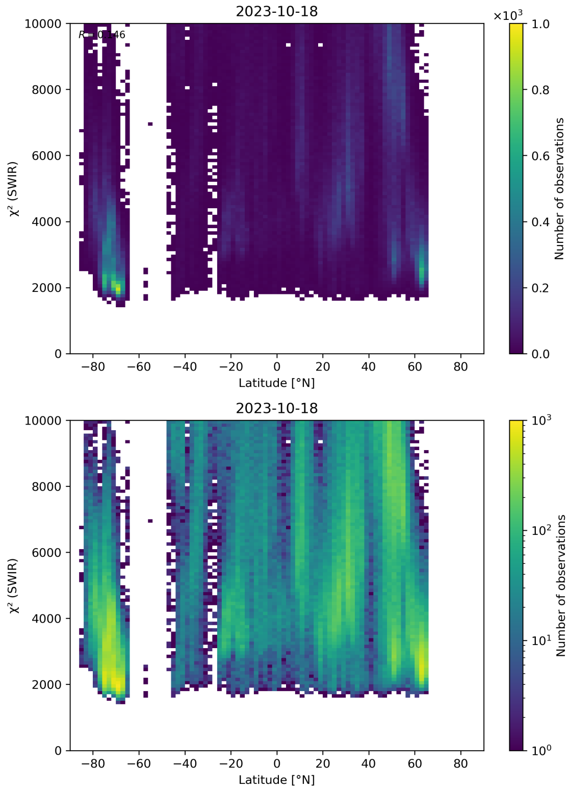
Figure 54: Scatter density plot of “Latitude” against “ \chi^2 (SWIR)” for 2023-10-17 to 2023-10-19.
