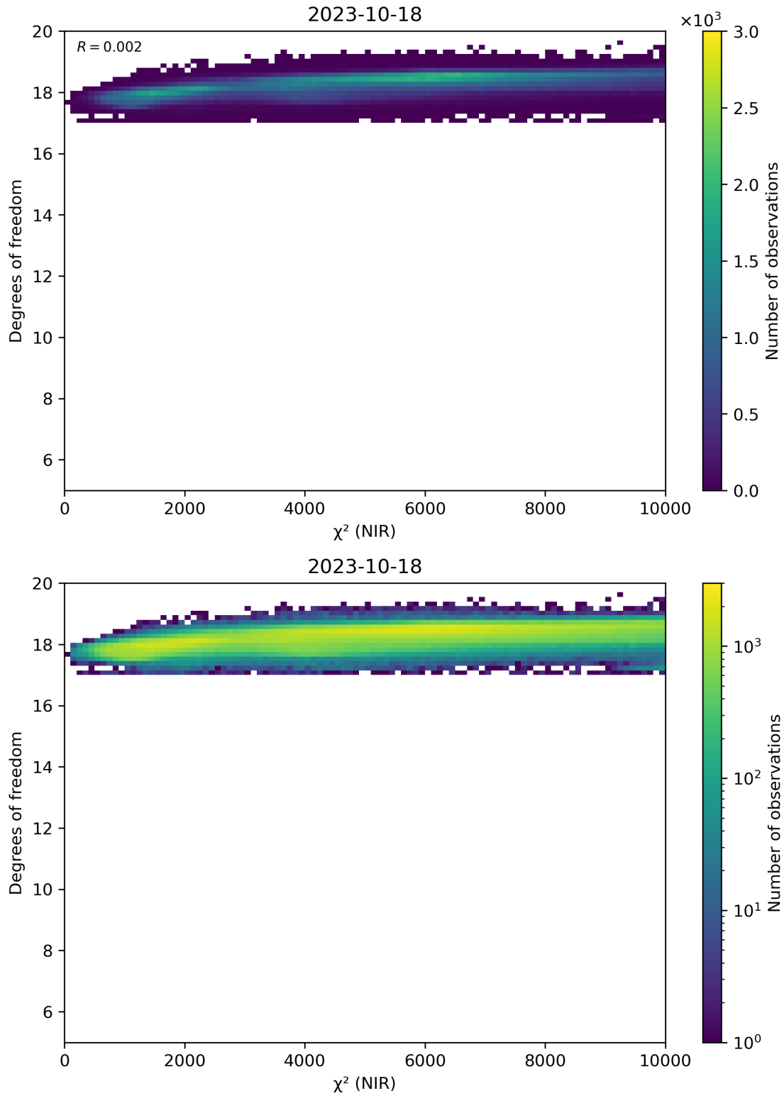
Figure 44: Scatter density plot of “ \chi^2 (NIR)” against “Degrees of freedom” for 2023-10-17 to 2023-10-19.
