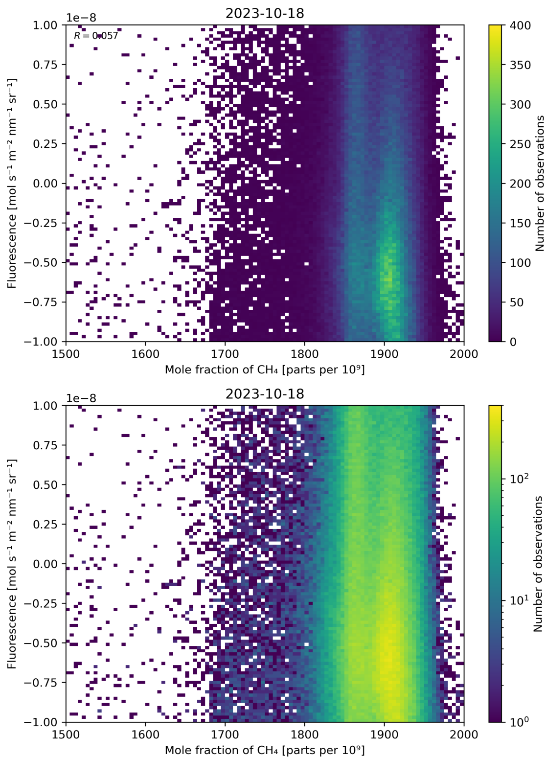
Figure 73: Scatter density plot of “Mole fraction of \text{CH}_4 ” against “Fluorescence” for 2023-10-17 to 2023-10-19.
