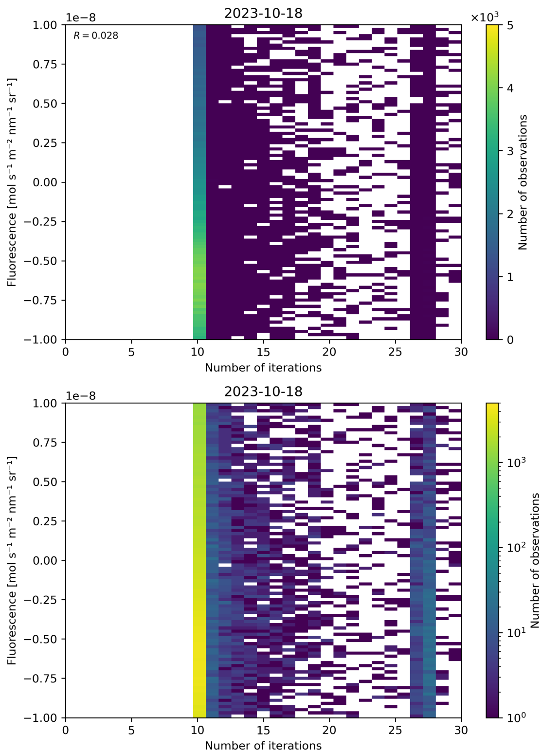
Figure 87: Scatter density plot of “Number of iterations” against “Fluorescence” for 2023-10-17 to 2023-10-19.
