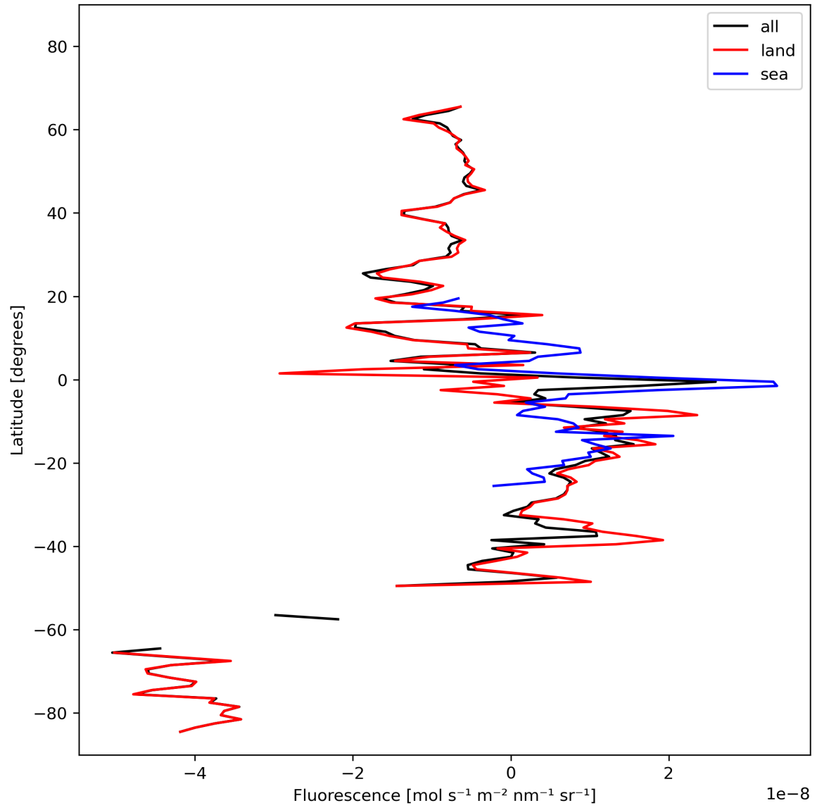
Figure 21: Zonal average of “Fluorescence” for 2023-10-17 to 2023-10-19.
