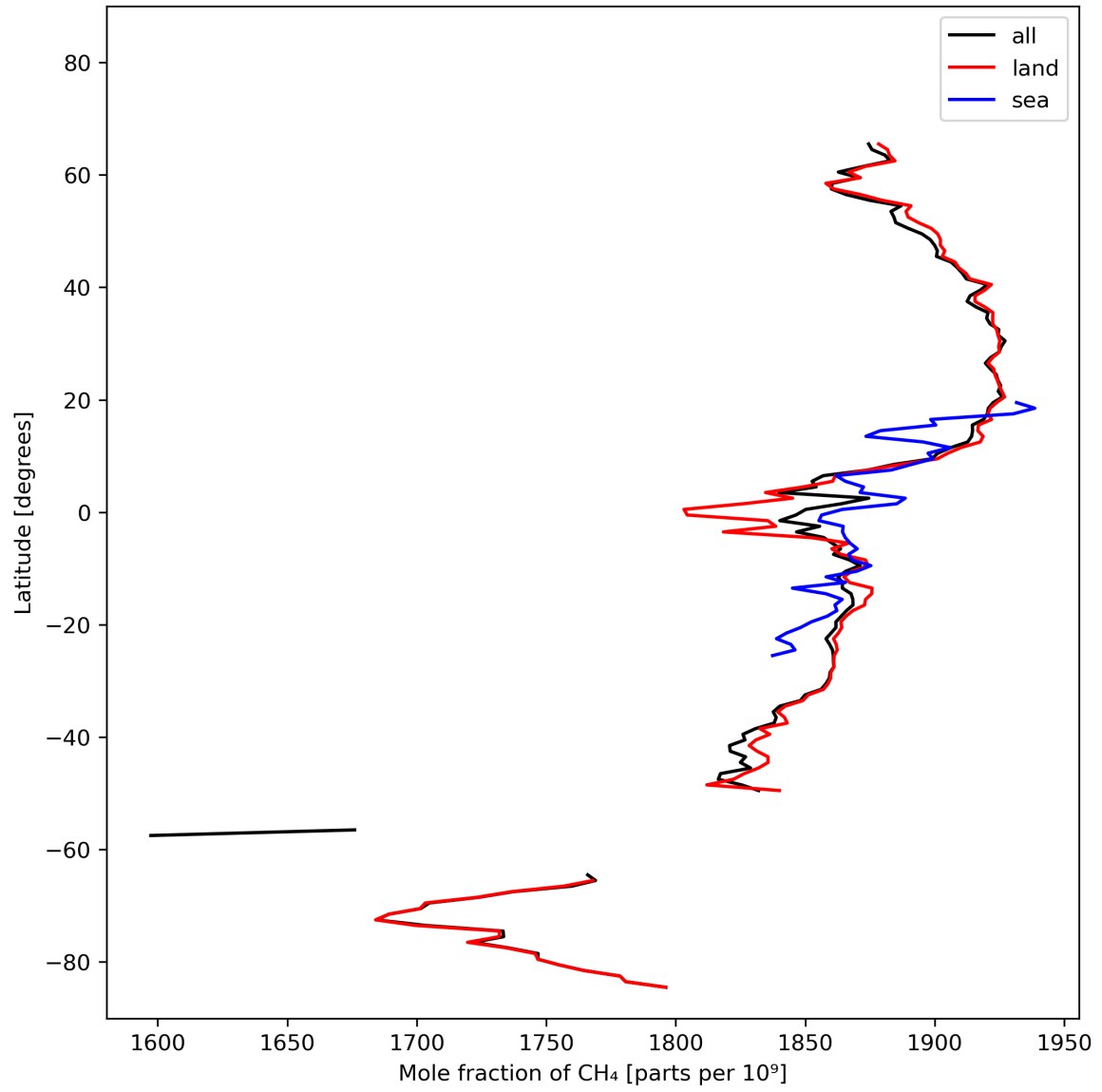
Figure 12: Zonal average of “Mole fraction of \text{CH}_4 ” for 2023-10-17 to 2023-10-19.
