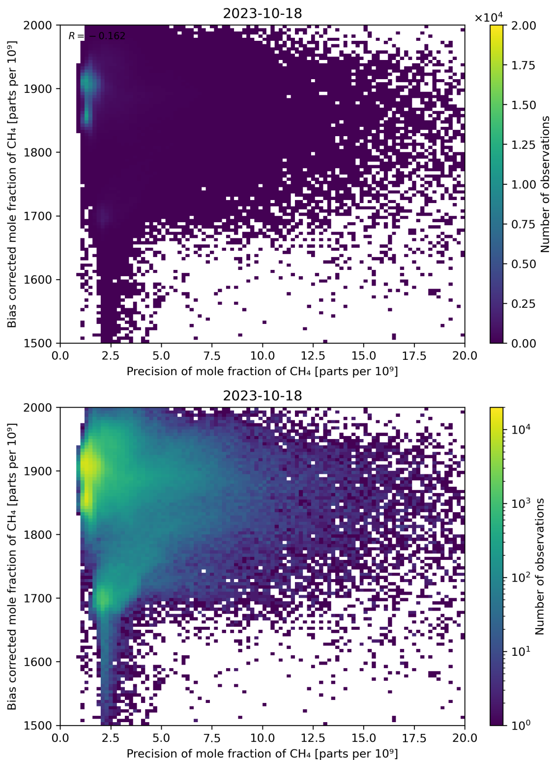
Figure 82: Scatter density plot of “Precision of mole fraction of CH 4 ” against “Bias corrected mole fraction of CH 4 ” for 2023-10-17 to 2023-10-19.
