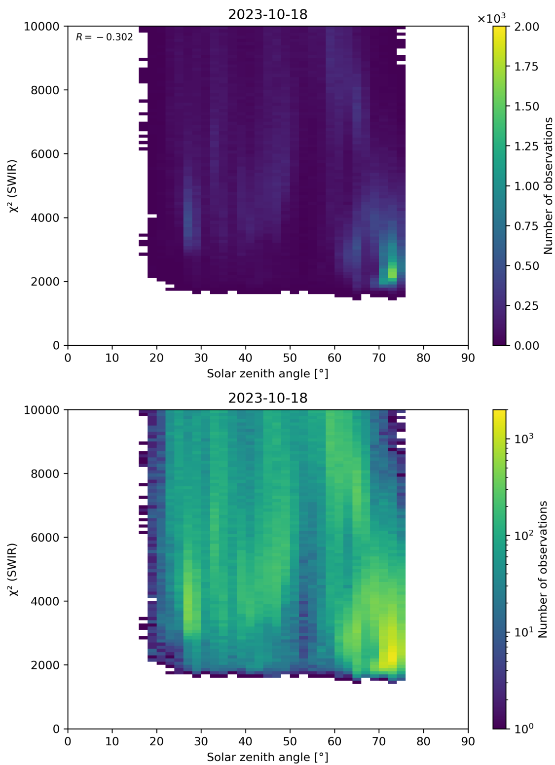
Figure 95: Scatter density plot of “Solar zenith angle” against “ \chi^2 (SWIR)” for 2023-10-17 to 2023-10-19.
