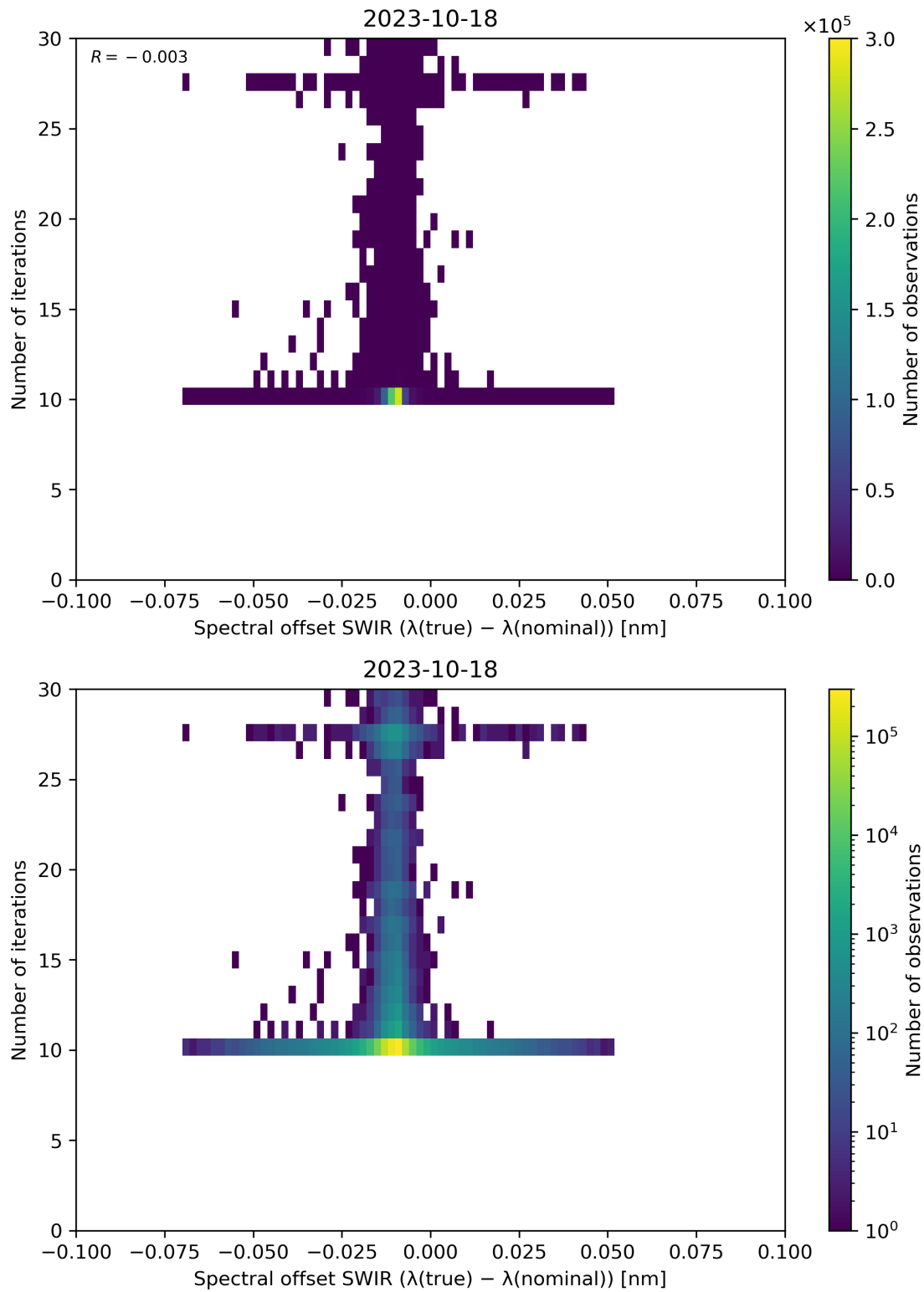
Figure 121: Scatter density plot of “Spectral offset SWIR ( \lambda(\text{true}) - \lambda(\text{nominal}) )” against “Number of iterations” for 2023-10-17 to 2023-10-19.
