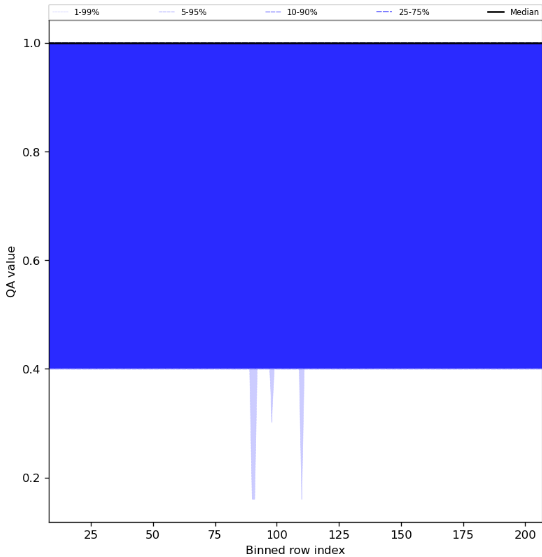
Figure 33: Along track statistics of “QA value” for 2023-10-17 to 2023-10-19
