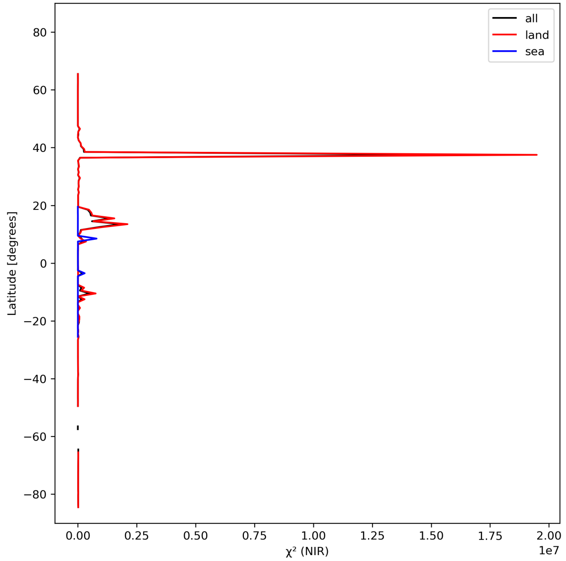
Figure 18: Zonal average of “ \chi^2 (NIR)” for 2023-10-17 to 2023-10-19.
