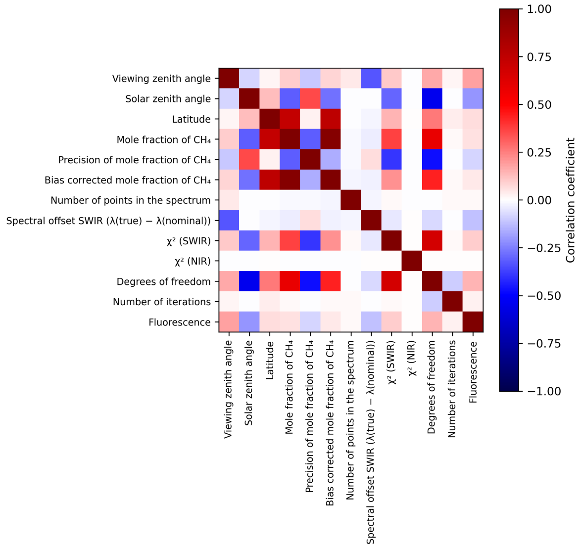
Figure 2: Map of correlation matrix for 2023-10-17 to 2023-10-19.
