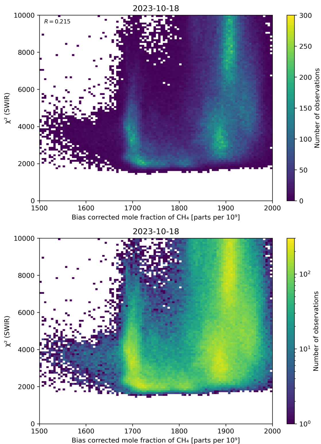
Figure 64: Scatter density plot of “Bias corrected mole fraction of \text{CH}_4 ” against “ \chi^2 (SWIR)” for 2023-10-17 to 2023-10-19.
