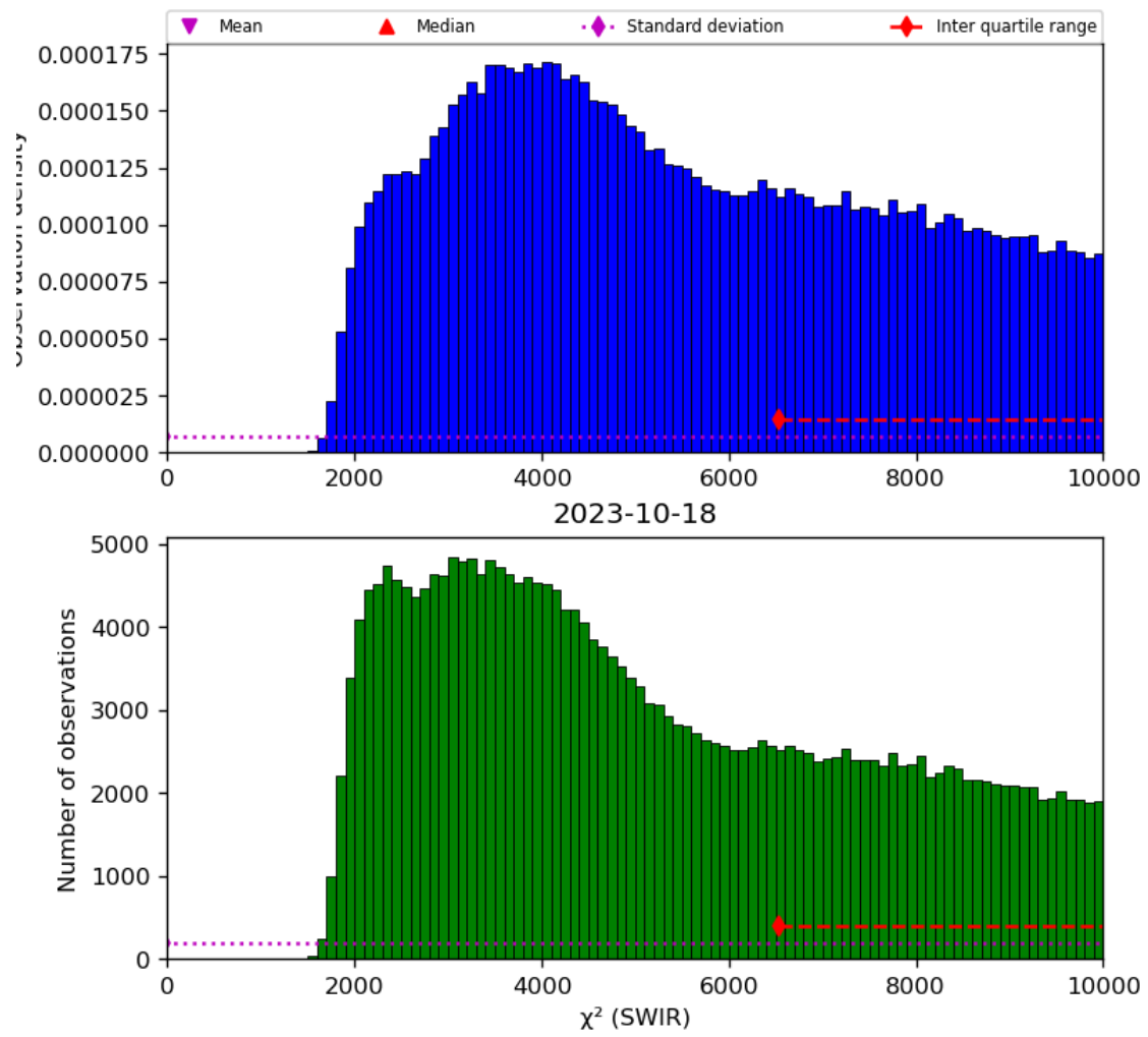
Figure 28: Histogram of “ \chi^2 (SWIR)” for 2023-10-17 to 2023-10-19
