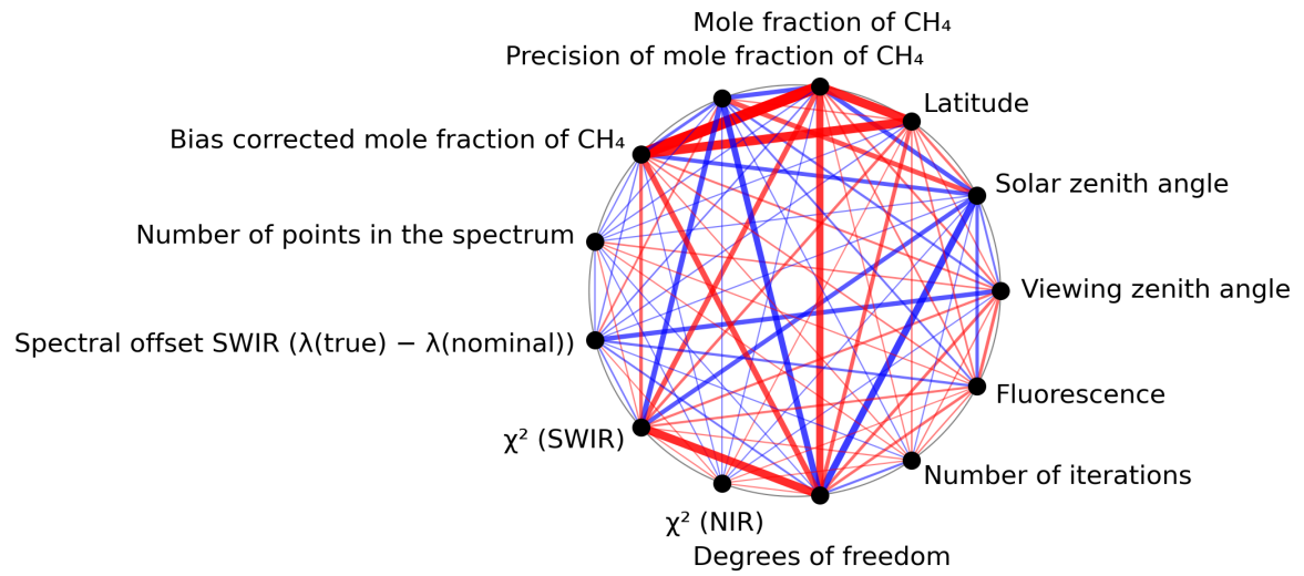
Figure 1: Map of correlation graph for 2023-10-17 to 2023-10-19.
