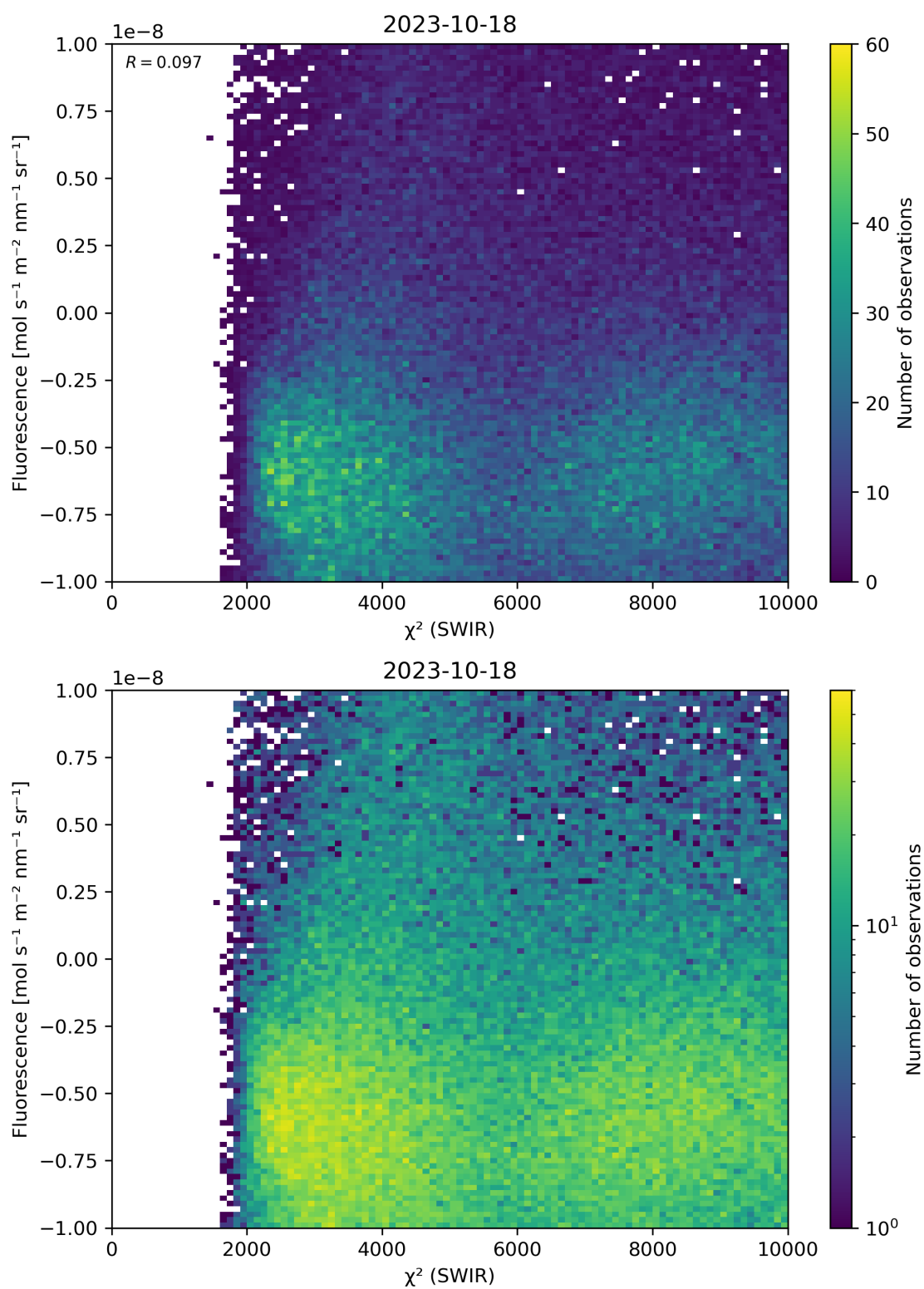
Figure 49: Scatter density plot of “ \chi^2 (SWIR)” against “Fluorescence” for 2023-10-17 to 2023-10-19.
