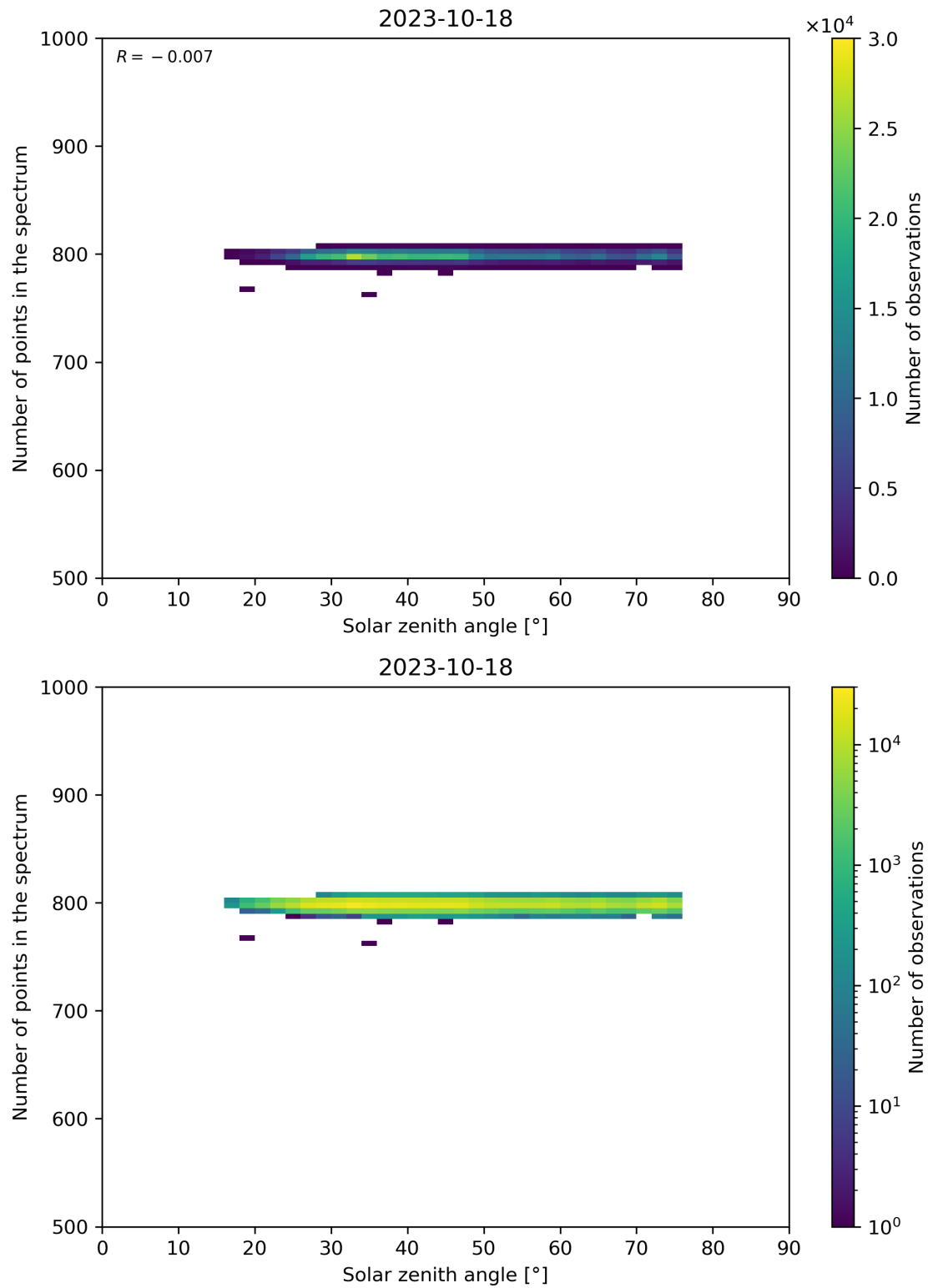
Figure 103: Scatter density plot of “Solar zenith angle” against “Number of points in the spectrum” for 2023-10-17 to 2023-10-19.
