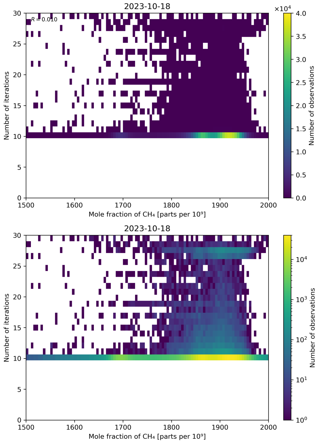
Figure 76: Scatter density plot of “Mole fraction of CH 4 ” against “Number of iterations” for 2023-10-17 to 2023-10-19.
