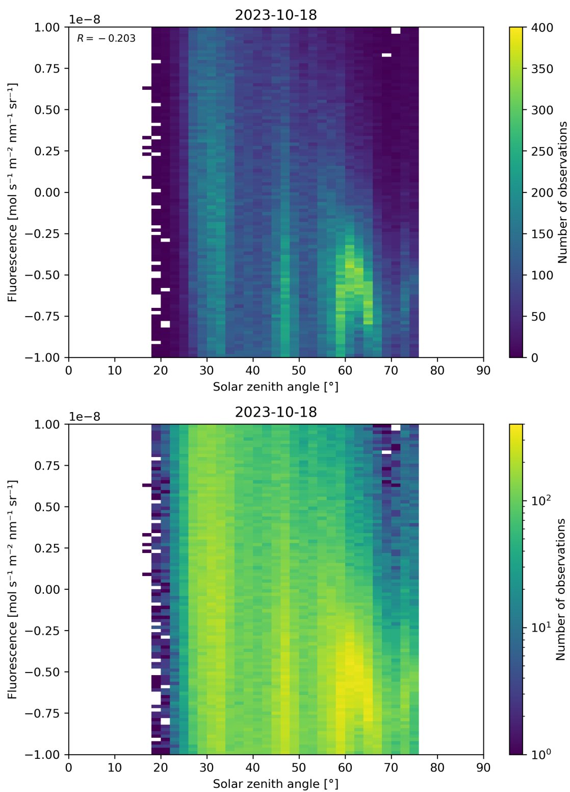
Figure 97: Scatter density plot of “Solar zenith angle” against “Fluorescence” for 2023-10-17 to 2023-10-19.
