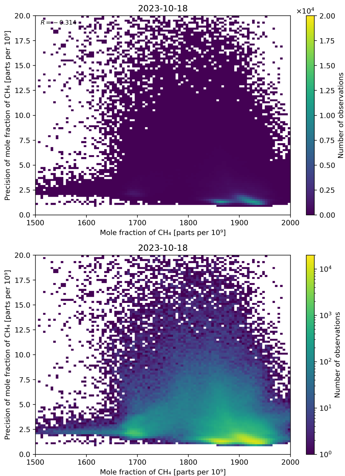
Figure 75: Scatter density plot of “Mole fraction of CH 4 ” against “Precision of mole fraction of CH 4 ” for 2023-10-17 to 2023-10-19.
