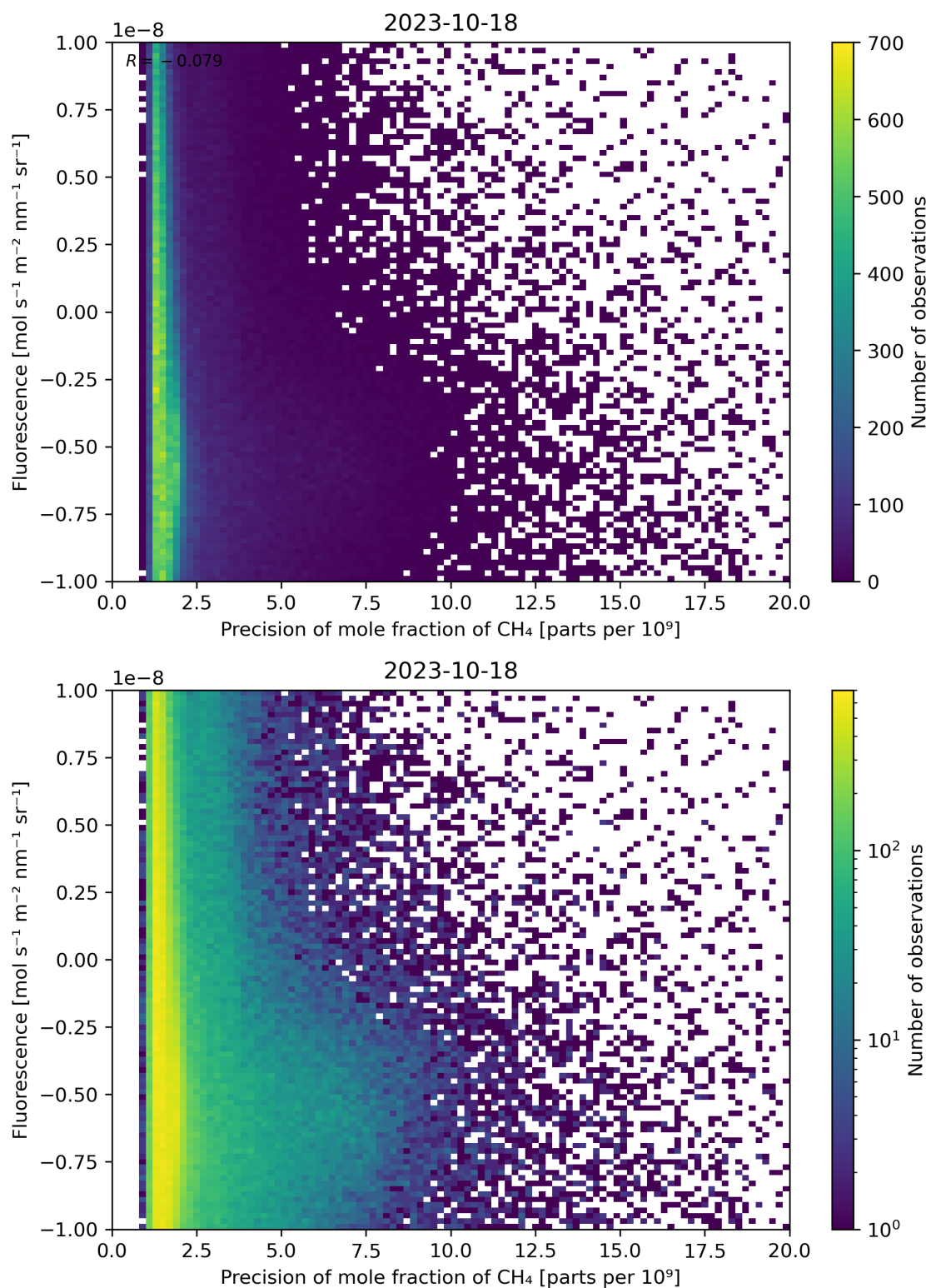
Figure 81: Scatter density plot of “Precision of mole fraction of \text{CH}_4 ” against “Fluorescence” for 2023-10-17 to 2023-10-19.
