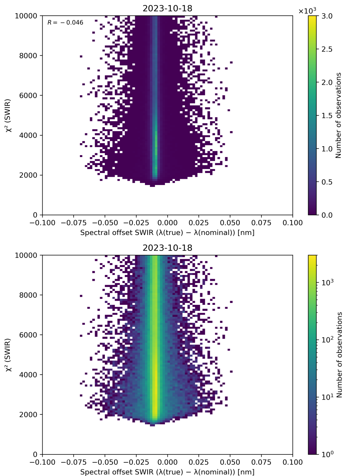
Figure 118: Scatter density plot of “Spectral offset SWIR ( \lambda(\text{true}) - \lambda(\text{nominal}) )” against “ \chi^2 (SWIR)” for 2023-10-17 to 2023-10-19.
