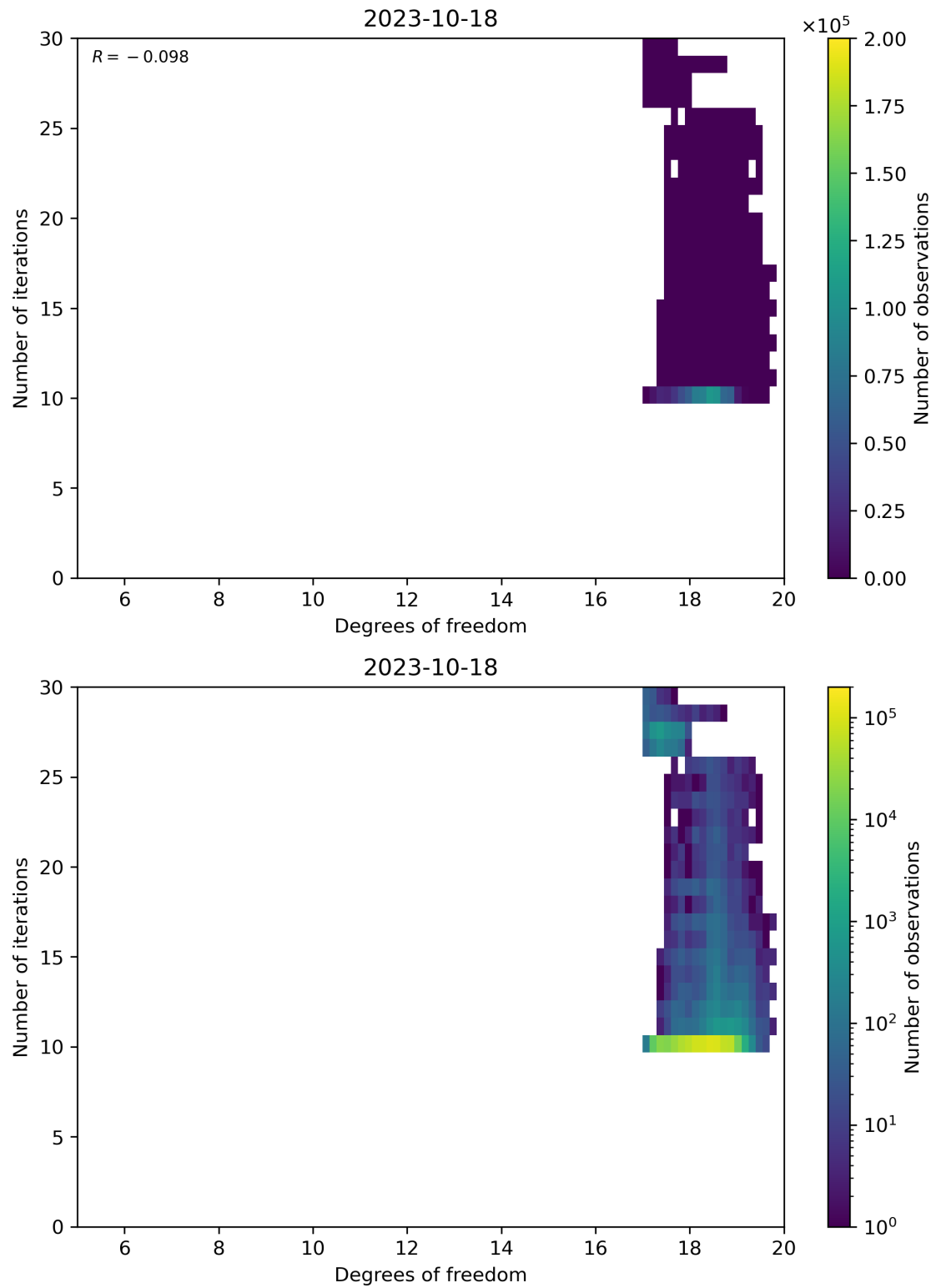
Figure 52: Scatter density plot of “Degrees of freedom” against “Number of iterations” for 2023-10-17 to 2023-10-19.
