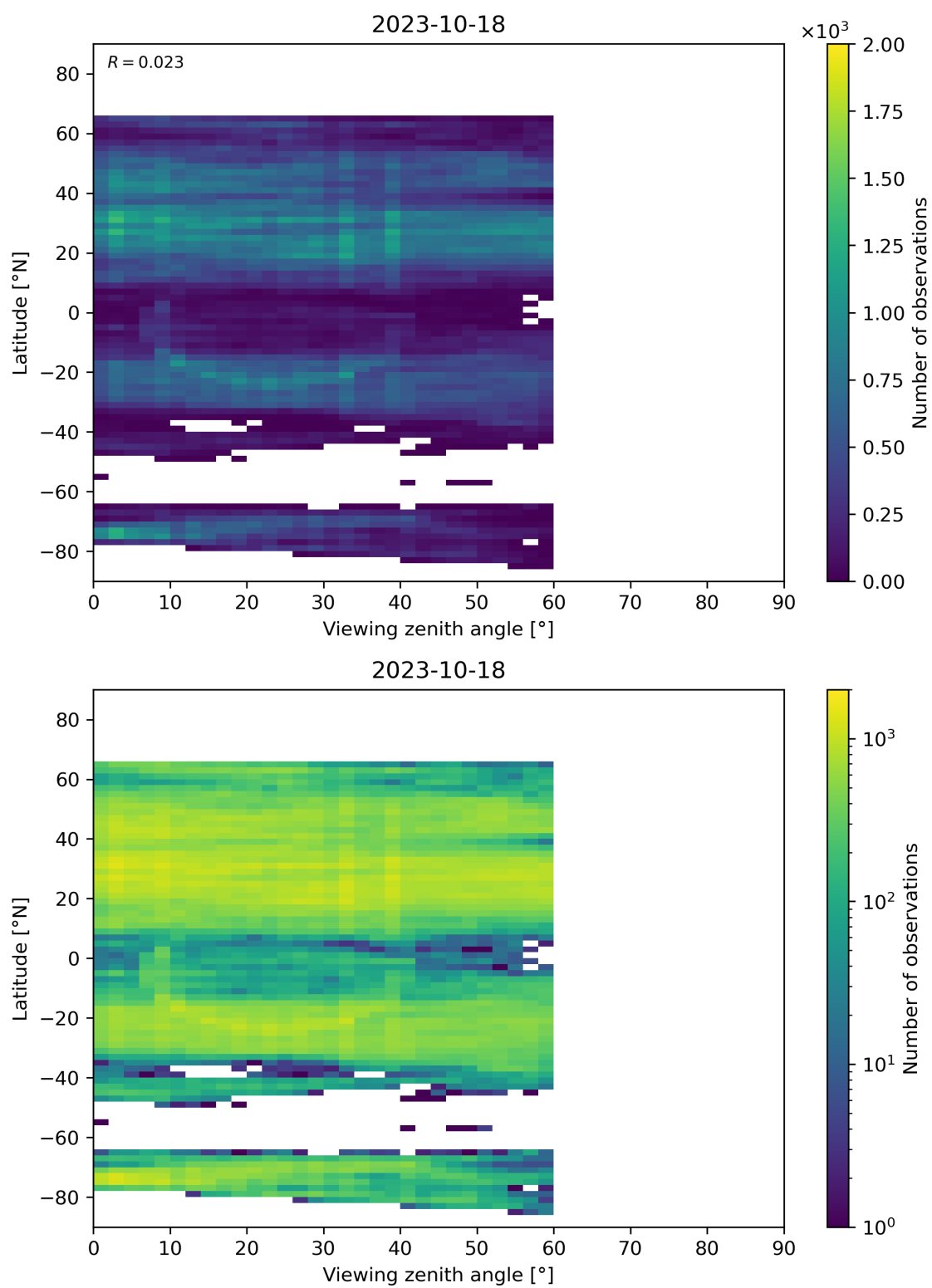
Figure 109: Scatter density plot of “Viewing zenith angle” against “Latitude” for 2023-10-17 to 2023-10-19.
