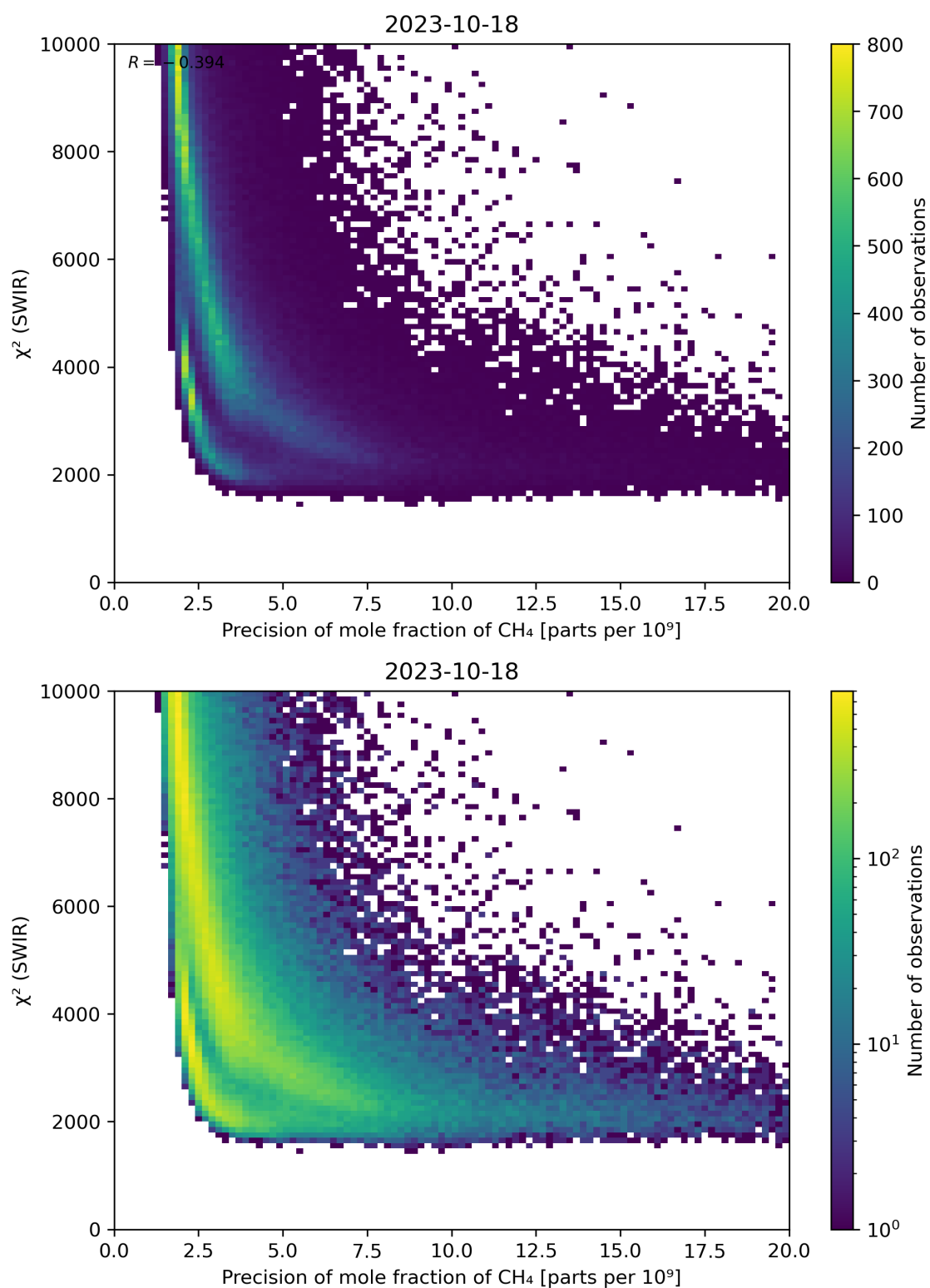
Figure 79: Scatter density plot of “Precision of mole fraction of CH 4 ” against “ \chi^2 (SWIR)” for 2023-10-17 to 2023-10-19.
