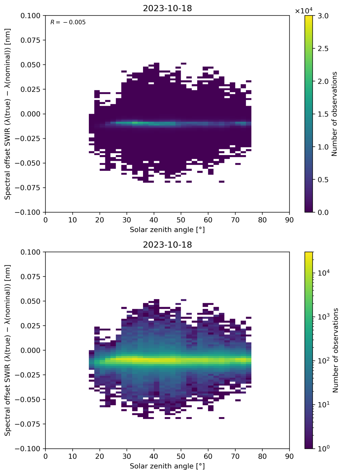
Figure 104: Scatter density plot of “Solar zenith angle” against “Spectral offset SWIR ( \lambda(\text{true}) - \lambda(\text{nominal}) )” for 2023-10-17 to 2023-10-19.
