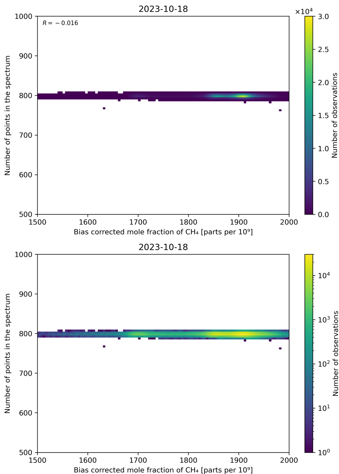
Figure 68: Scatter density plot of “Bias corrected mole fraction of CH 4 ” against “Number of points in the spectrum” for 2023-10-17 to 2023-10-19.
