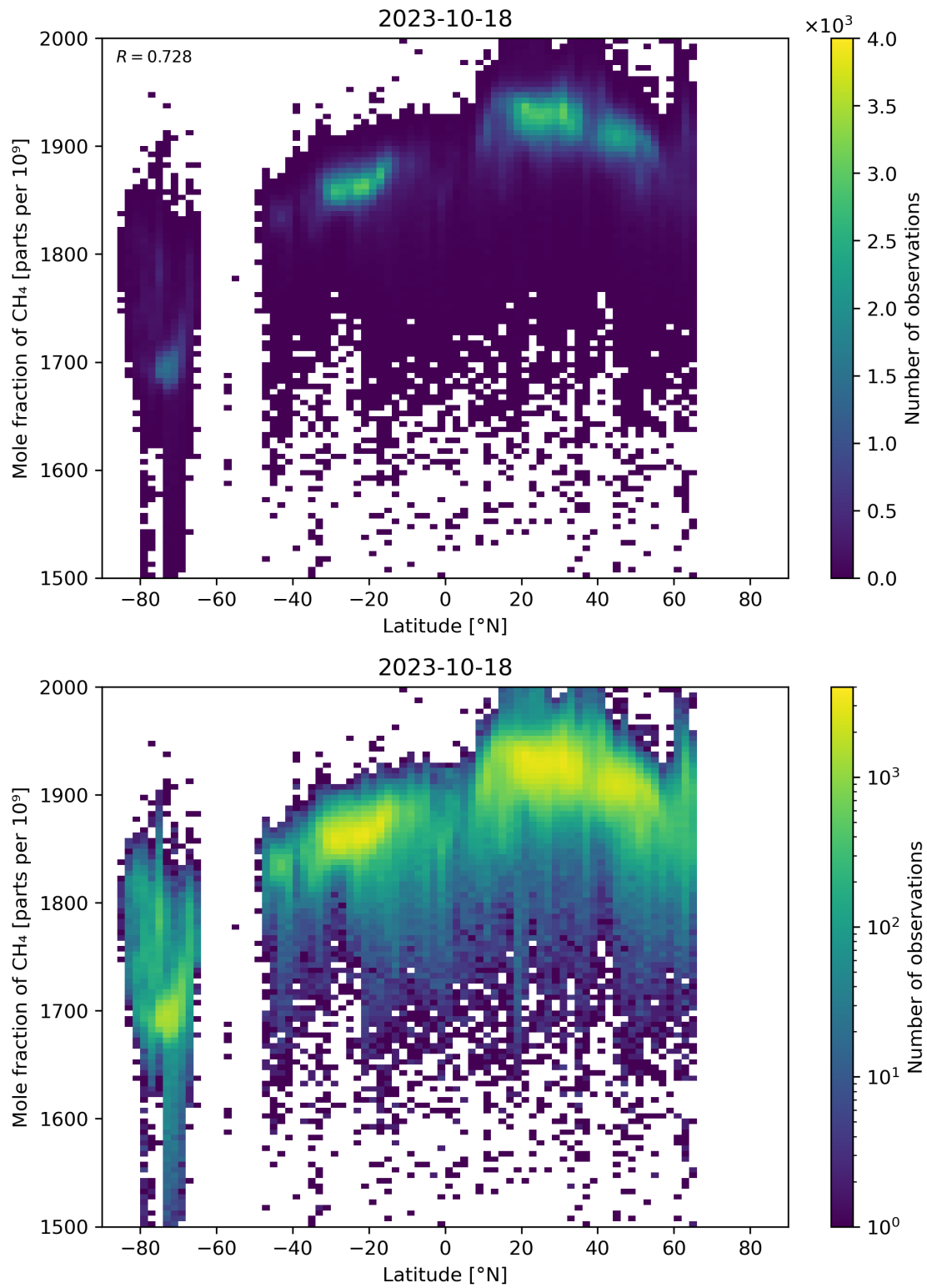
Figure 57: Scatter density plot of “Latitude” against “Mole fraction of CH 4 ” for 2023-10-17 to 2023-10-19.
