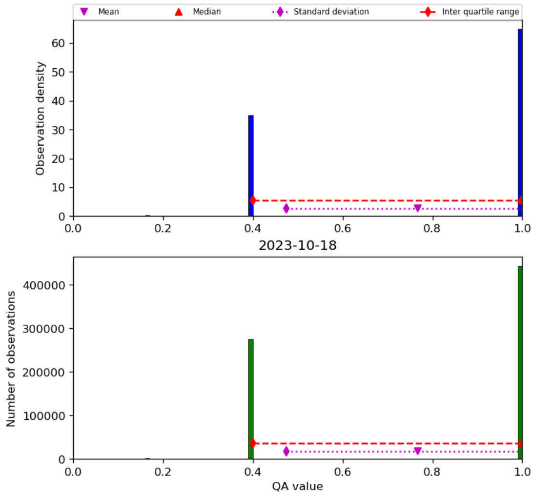
Figure 22: Histogram of “QA value” for 2023-10-17 to 2023-10-19
