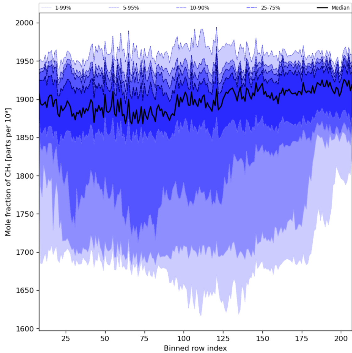
Figure 34: Along track statistics of “Mole fraction of CH 4 ” for 2023-10-17 to 2023-10-19
