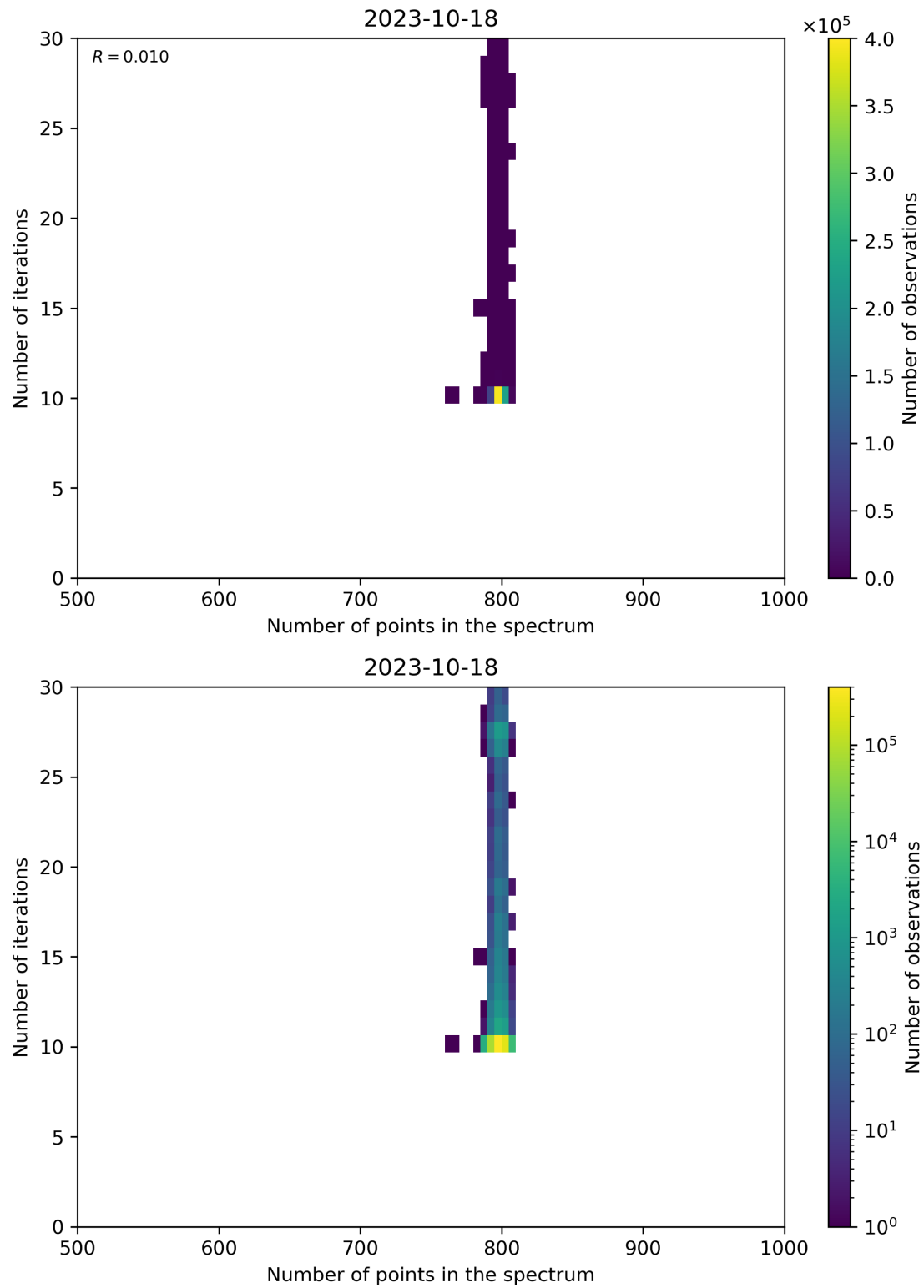
Figure 92: Scatter density plot of “Number of points in the spectrum” against “Number of iterations” for 2023-10-17 to 2023-10-19.
