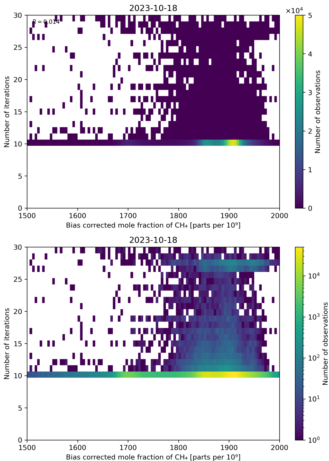
Figure 67: Scatter density plot of “Bias corrected mole fraction of \text{CH}_4 ” against “Number of iterations” for 2023-10-17 to 2023-10-19.
