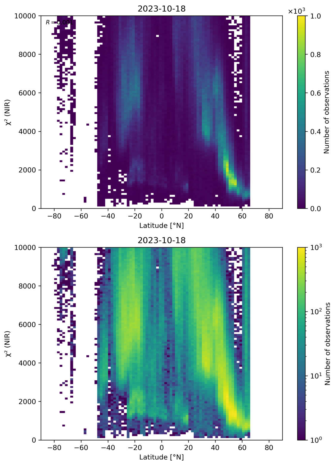
Figure 53: Scatter density plot of “Latitude” against “ \chi^2 (NIR)” for 2023-10-17 to 2023-10-19.
