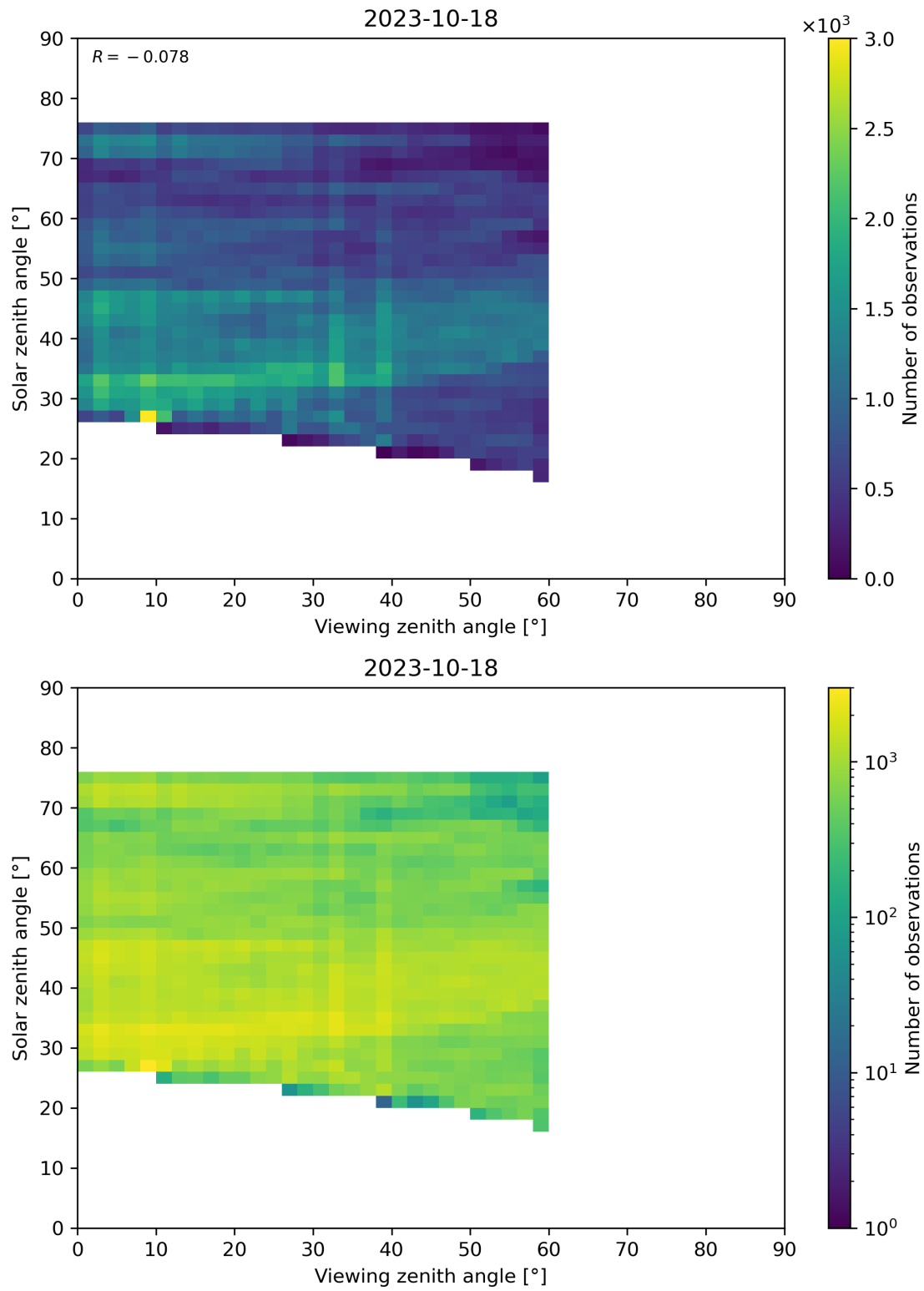
Figure 115: Scatter density plot of “Viewing zenith angle” against “Solar zenith angle” for 2023-10-17 to 2023-10-19.
