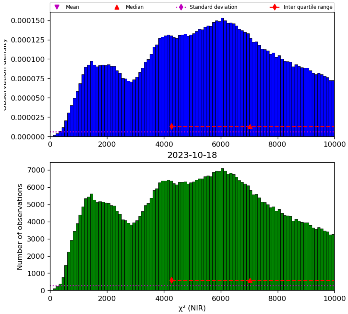
Figure 29: Histogram of “ \chi^2 (NIR)” for 2023-10-17 to 2023-10-19
