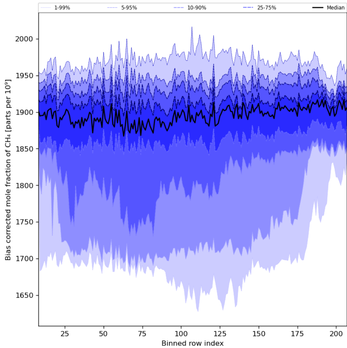
Figure 36: Along track statistics of “Bias corrected mole fraction of CH 4 ” for 2023-10-17 to 2023-10-19
