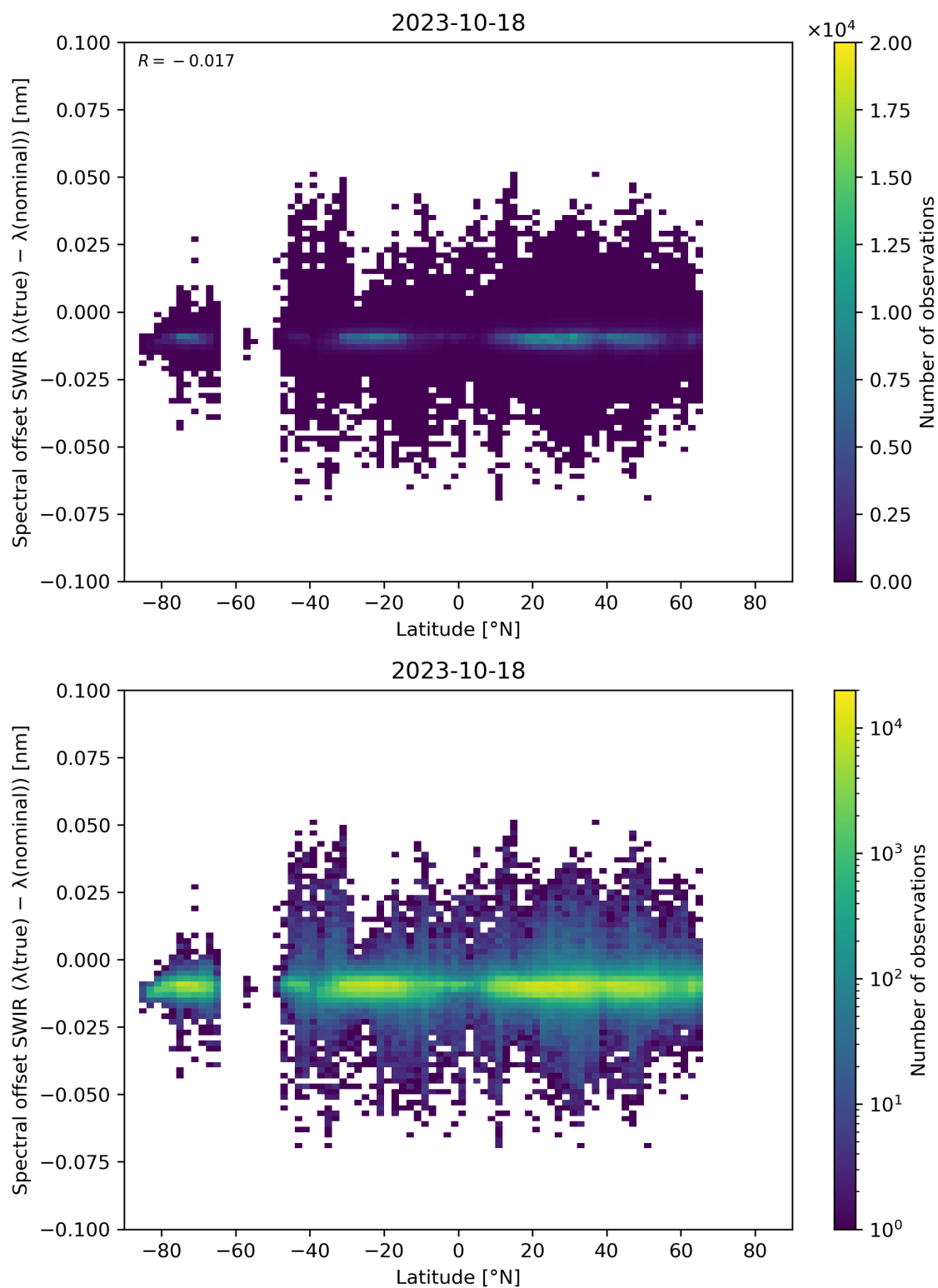
Figure 62: Scatter density plot of “Latitude” against “Spectral offset SWIR ( \lambda(\text{true}) - \lambda(\text{nominal}) )” for 2023-10-17 to 2023-10-19.
