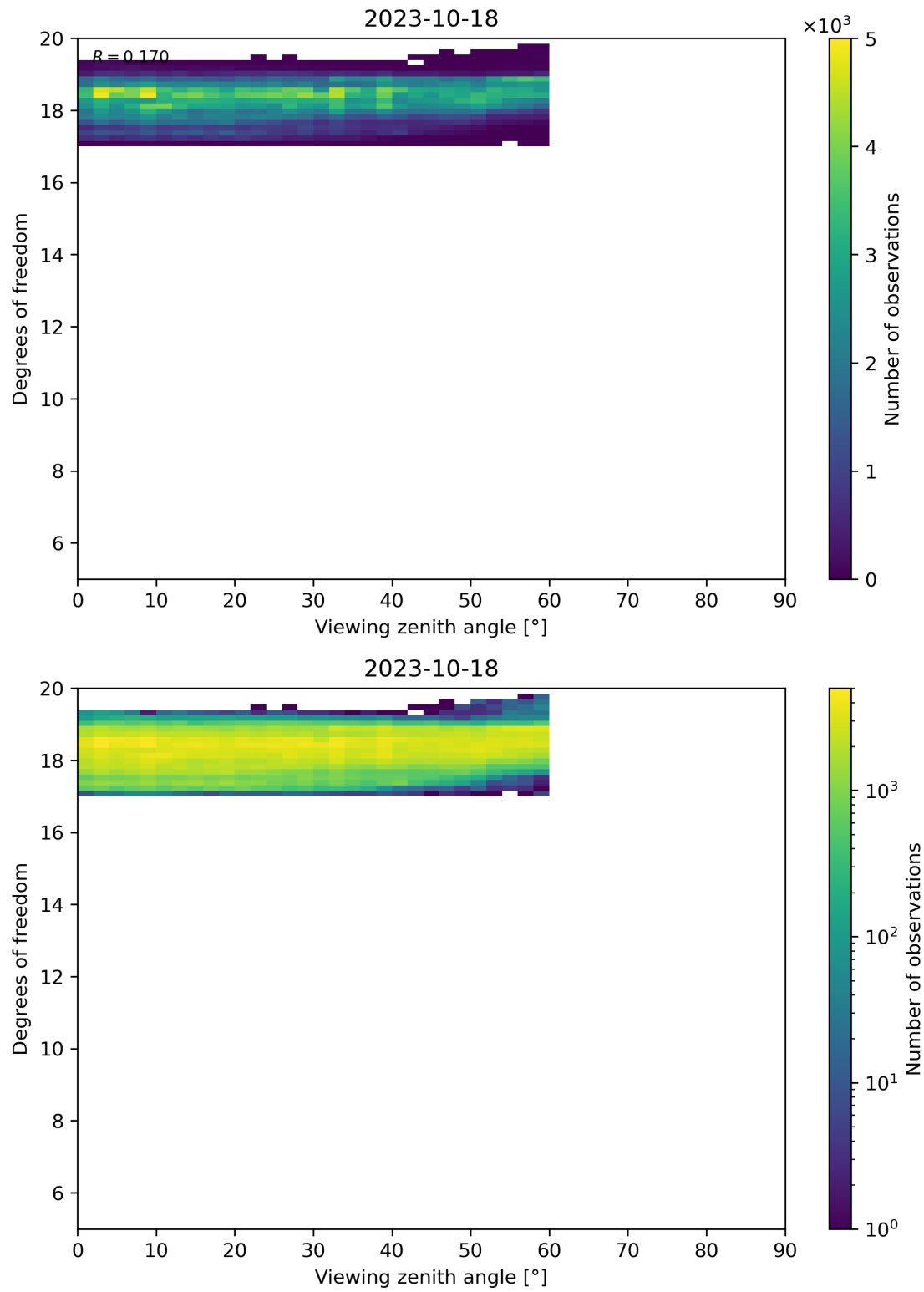
Figure 107: Scatter density plot of “Viewing zenith angle” against “Degrees of freedom” for 2023-10-17 to 2023-10-19.
