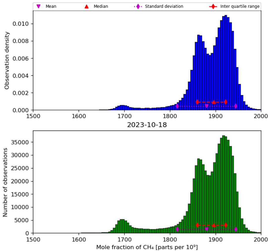
Figure 23: Histogram of "Mole fraction of CH 4 " for 2023-10-17 to 2023-10-19
