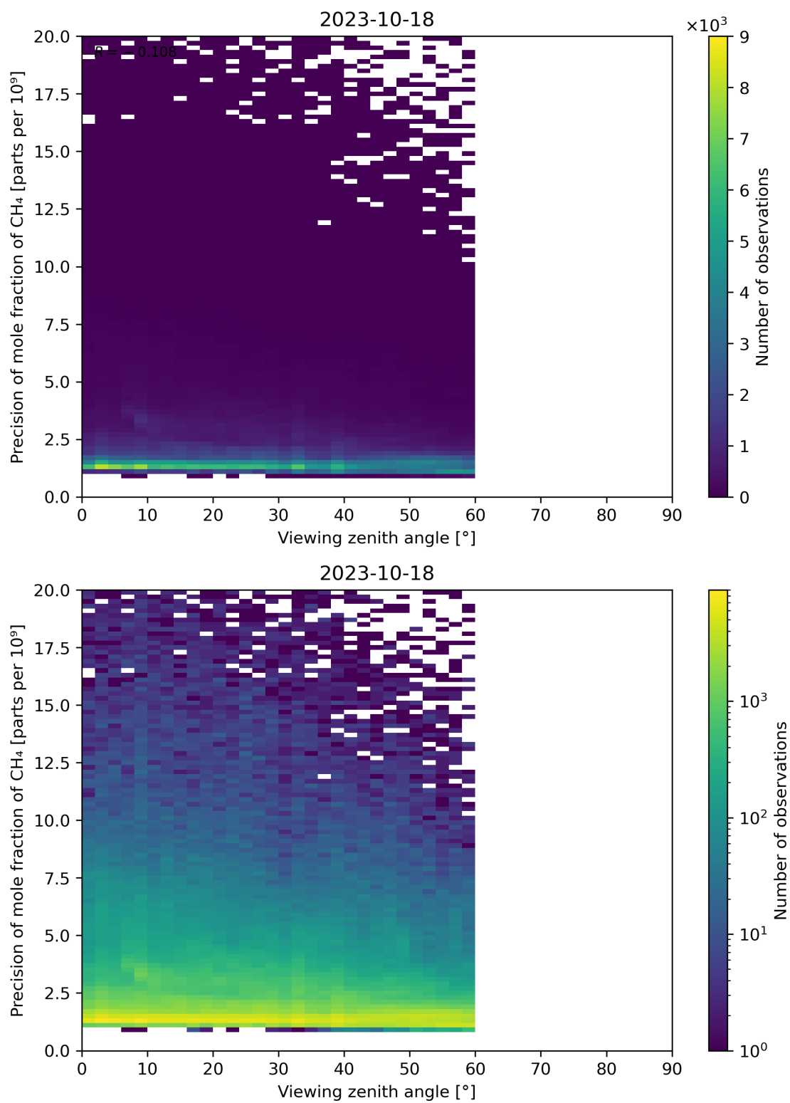
Figure 112: Scatter density plot of “Viewing zenith angle” against “Precision of mole fraction of CH 4 ” for 2023-10-17 to 2023-10-19.
