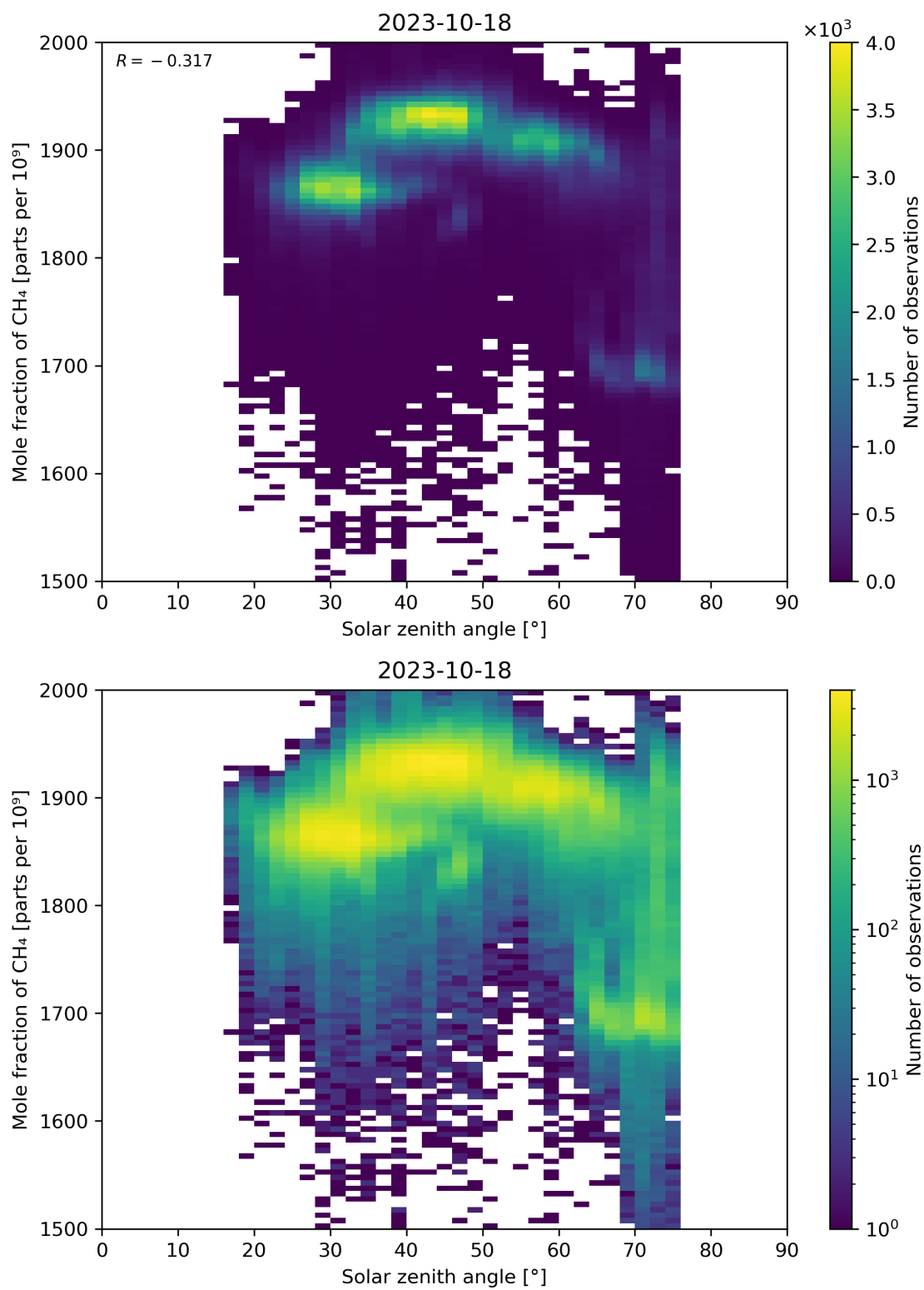
Figure 99: Scatter density plot of “Solar zenith angle” against “Mole fraction of CH 4 ” for 2023-10-17 to 2023-10-19.
