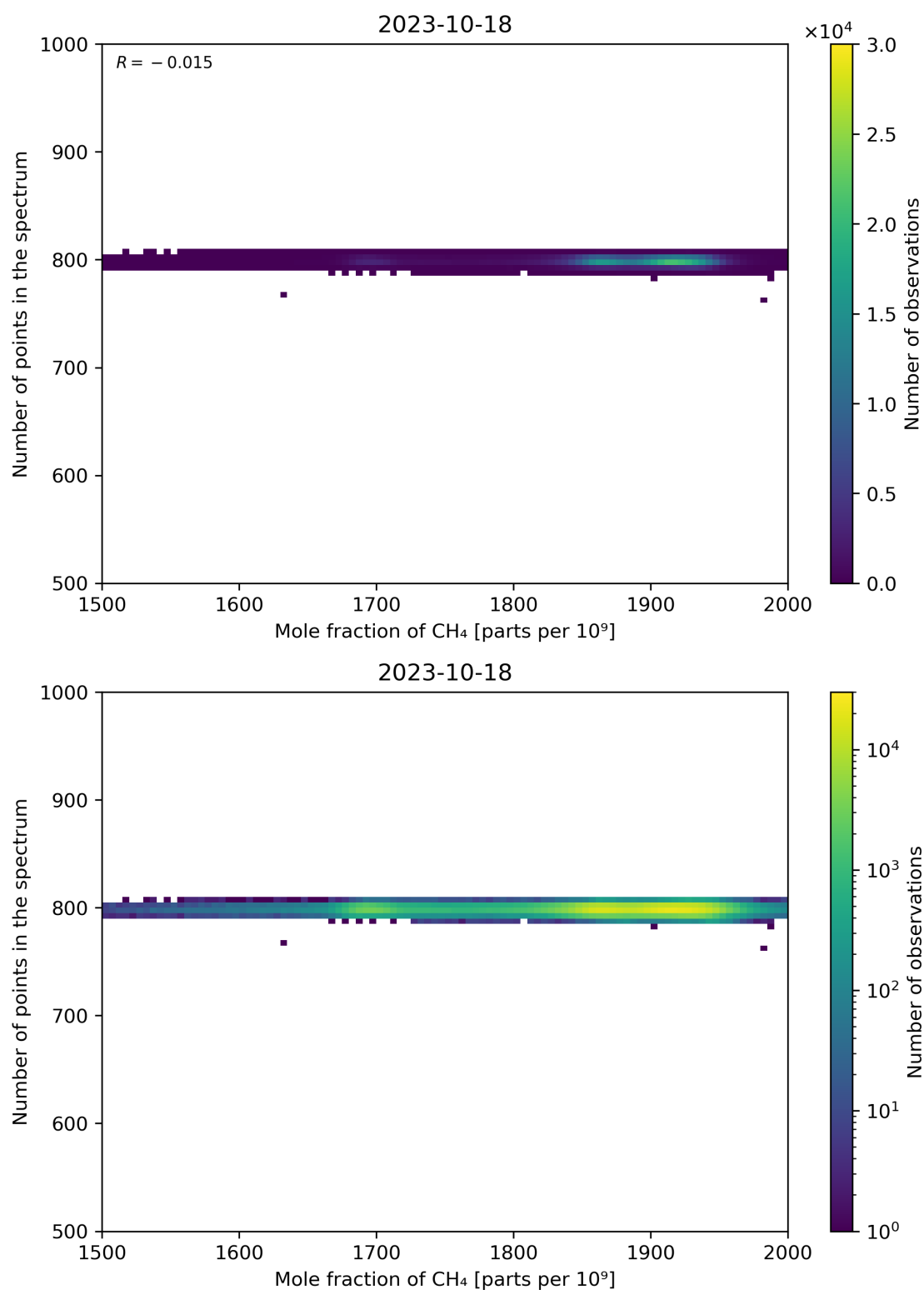
Figure 77: Scatter density plot of “Mole fraction of CH 4 ” against “Number of points in the spectrum” for 2023-10-17 to 2023-10-19.
