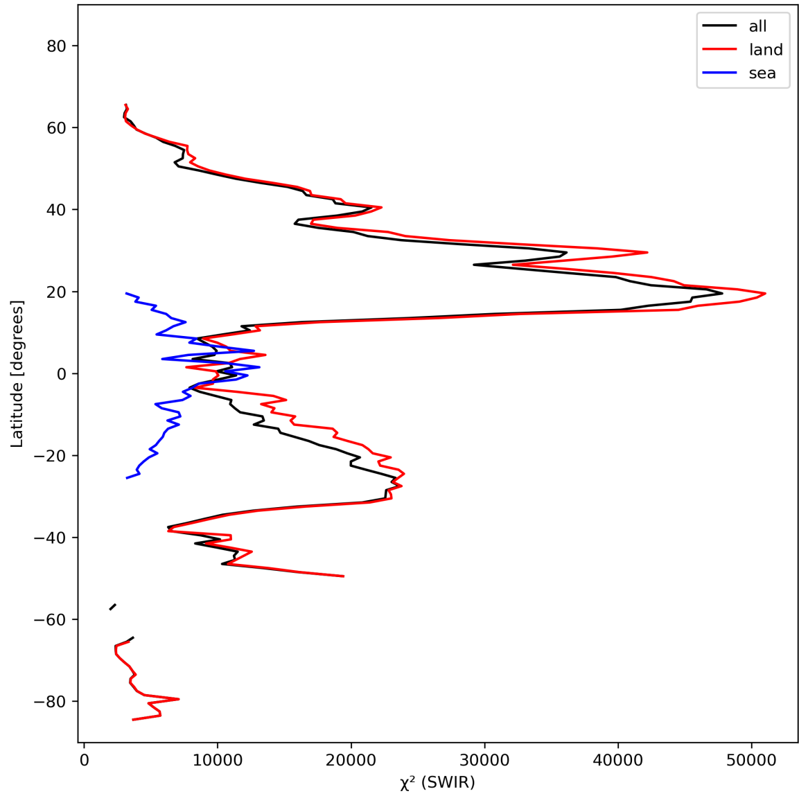
Figure 17: Zonal average of “ \chi^2 (SWIR)” for 2023-10-17 to 2023-10-19.
