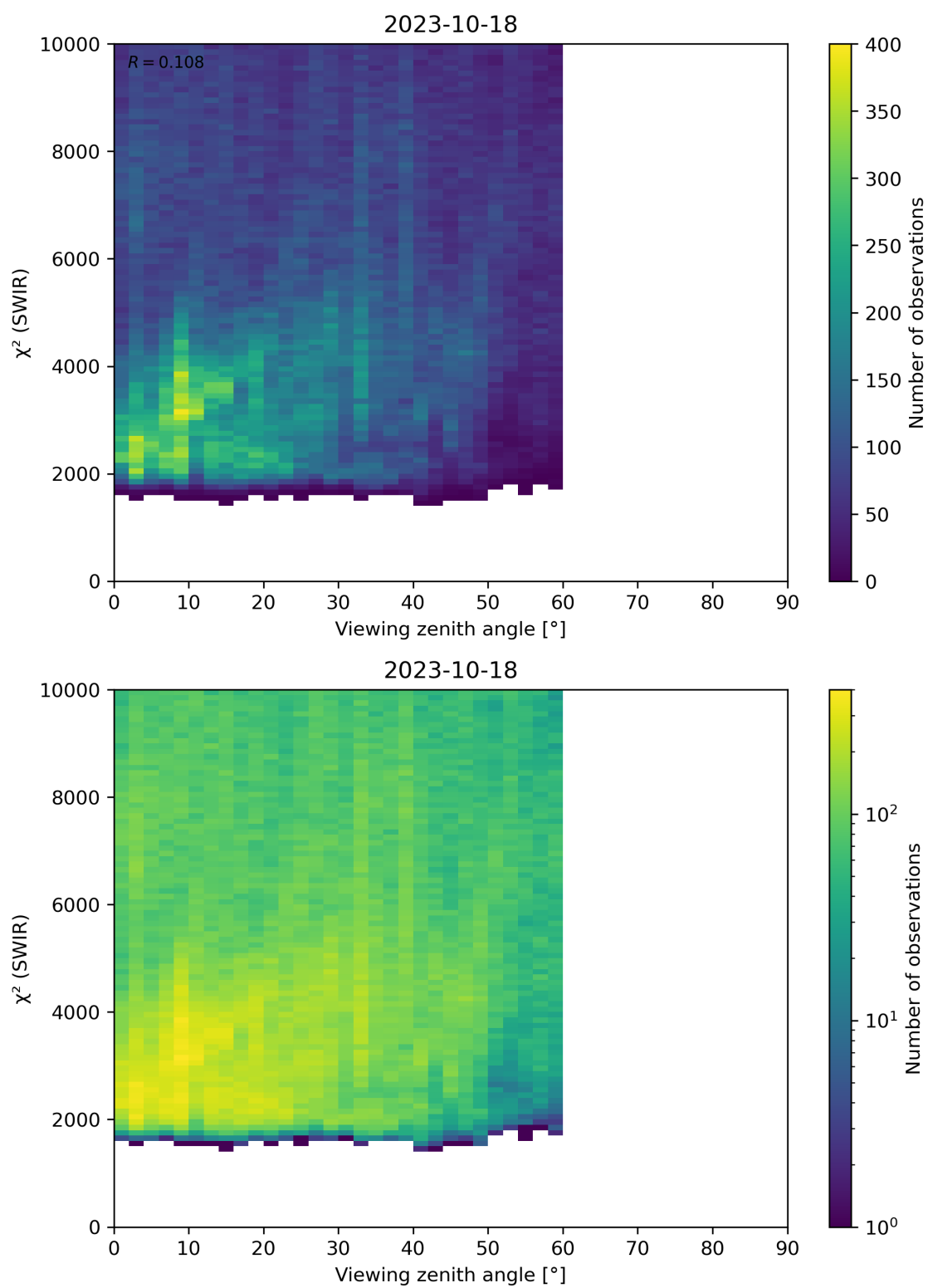
Figure 106: Scatter density plot of “Viewing zenith angle” against “ \chi^2 (SWIR)” for 2023-10-17 to 2023-10-19.
