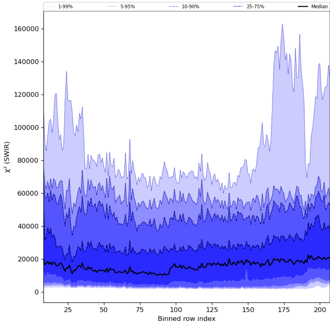
Figure 39: Along track statistics of “ \chi^2 (SWIR)” for 2023-10-17 to 2023-10-19
