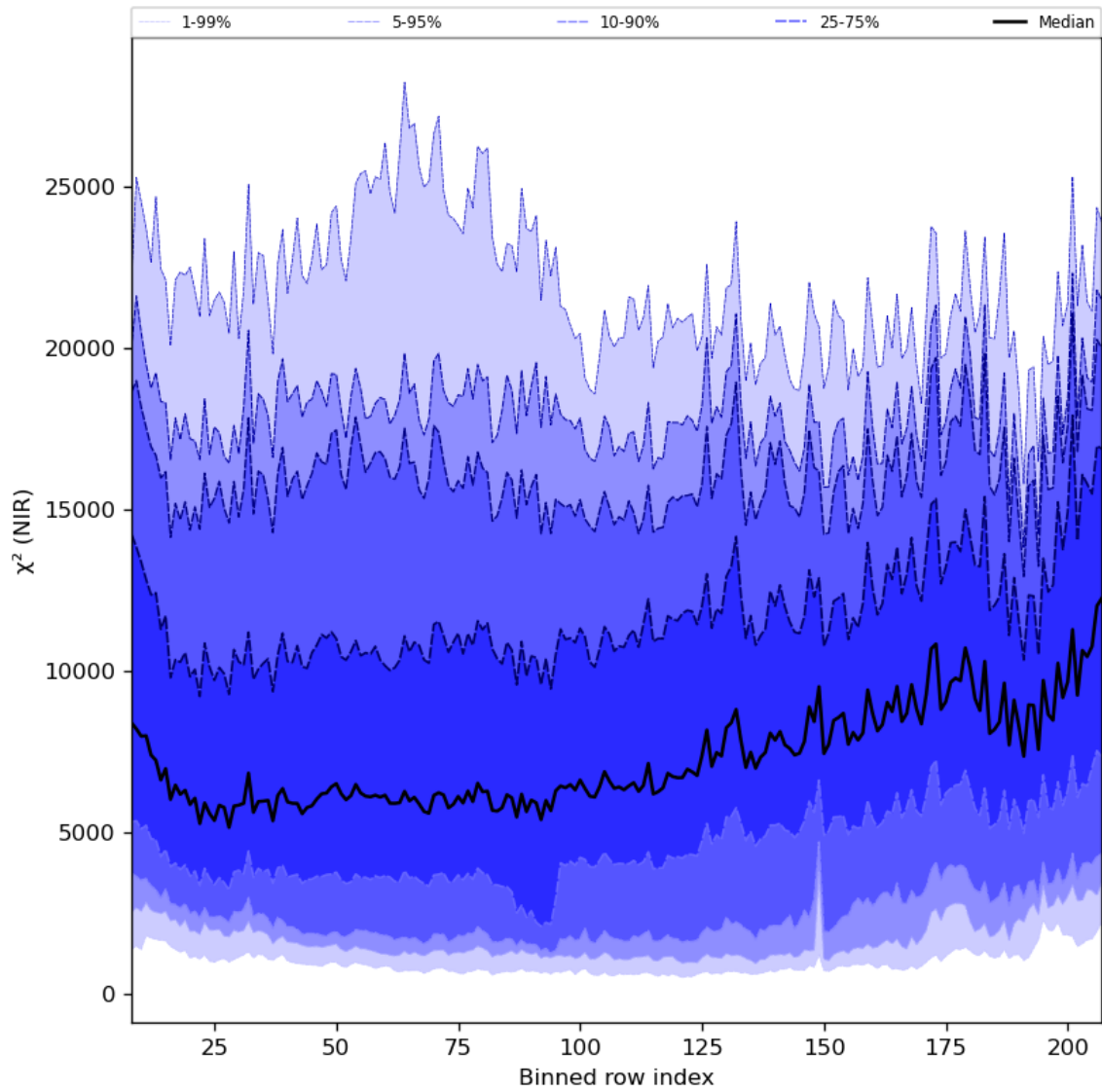
Figure 40: Along track statistics of “ \chi^2 (NIR)” for 2023-10-17 to 2023-10-19
