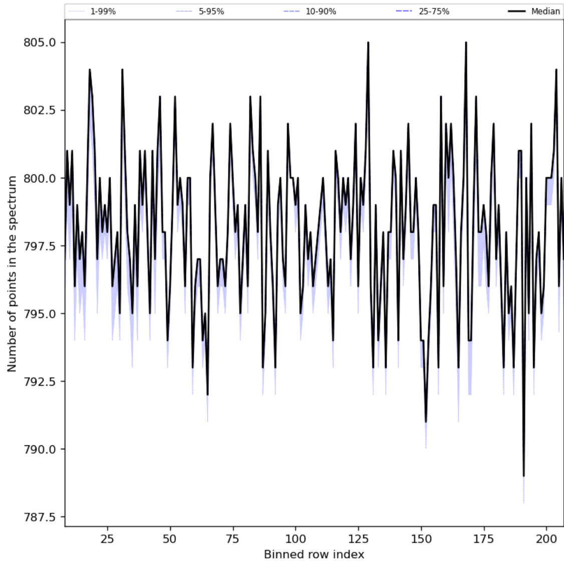
Figure 37: Along track statistics of “Number of points in the spectrum” for 2023-10-17 to 2023-10-19
