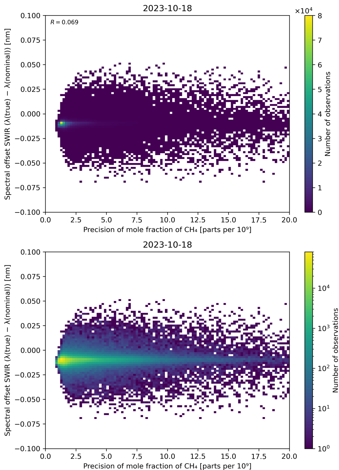
Figure 85: Scatter density plot of “Precision of mole fraction of \text{CH}_4 ” against “Spectral offset SWIR ( \lambda(\text{true}) - \lambda(\text{nominal}) )” for 2023-10-17 to 2023-10-19.
