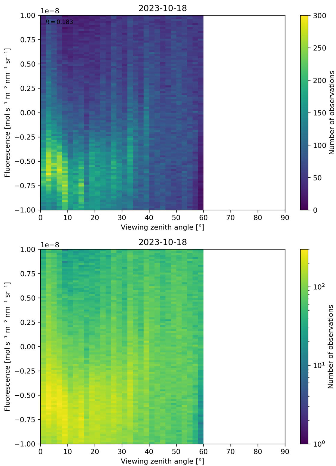
Figure 108: Scatter density plot of “Viewing zenith angle” against “Fluorescence” for 2023-10-17 to 2023-10-19.
