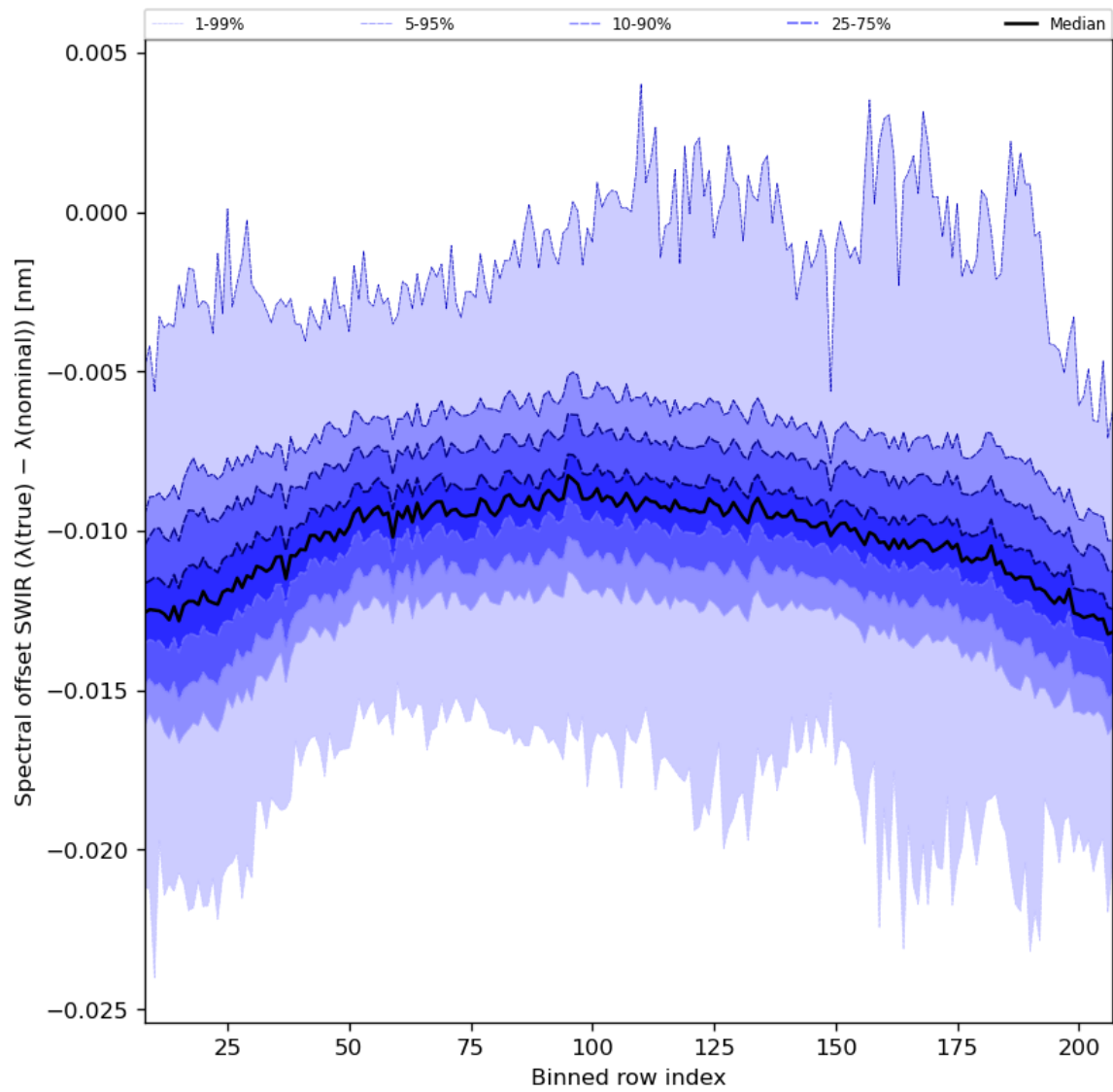
Figure 38: Along track statistics of “Spectral offset SWIR ( \lambda(\text{true}) - \lambda(\text{nominal}) )” for 2023-10-17 to 2023-10-19
