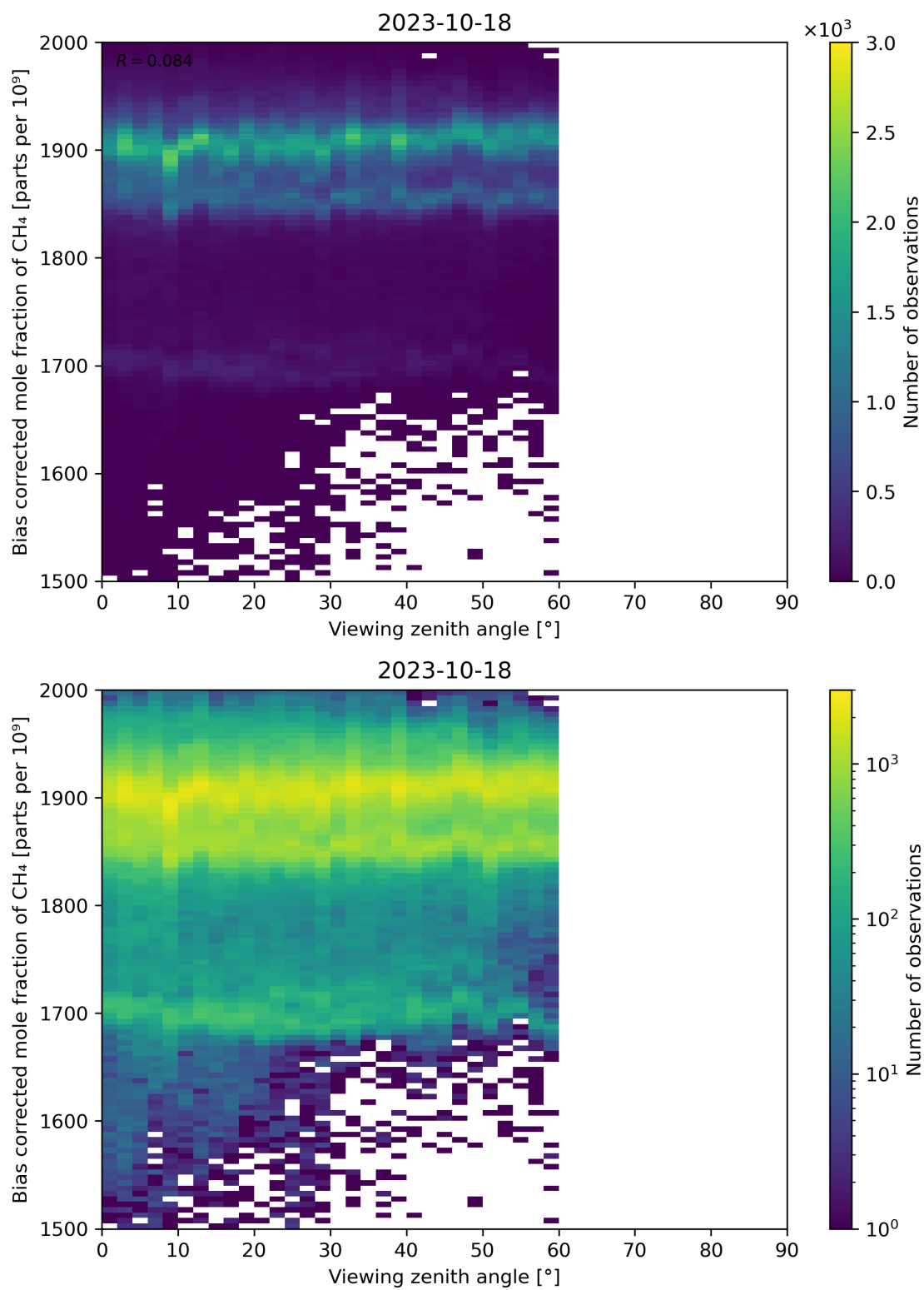
Figure 111: Scatter density plot of “Viewing zenith angle” against “Bias corrected mole fraction of CH 4 ” for 2023-10-17 to 2023-10-19.
