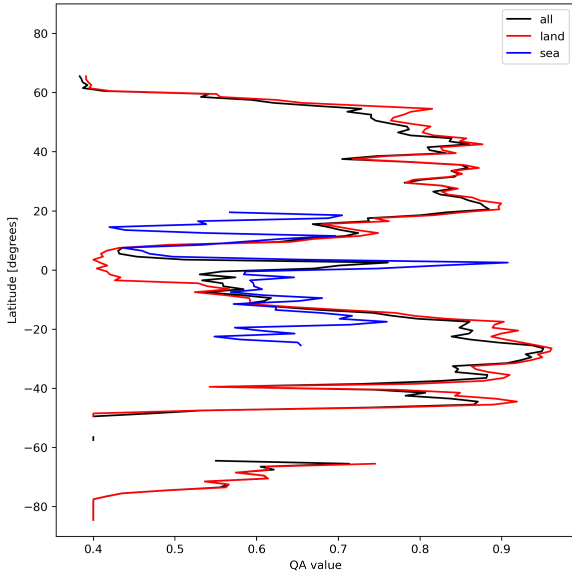
Figure 11: Zonal average of “QA value” for 2023-10-17 to 2023-10-19.
