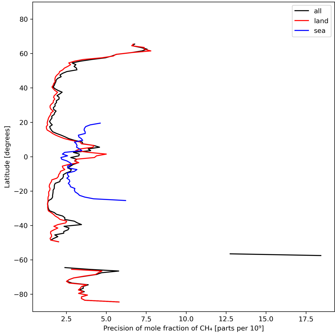
Figure 13: Zonal average of “Precision of mole fraction of CH 4 ” for 2023-10-17 to 2023-10-19.
