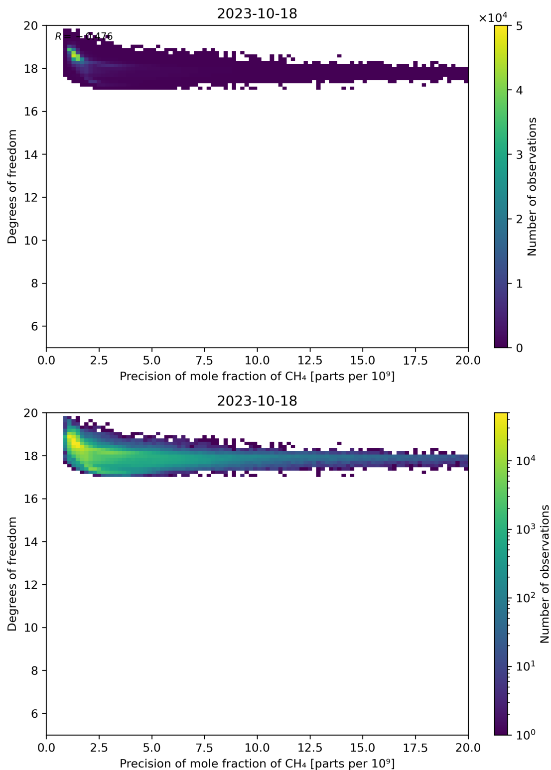
Figure 80: Scatter density plot of “Precision of mole fraction of CH 4 ” against “Degrees of freedom” for 2023-10-17 to 2023-10-19.
