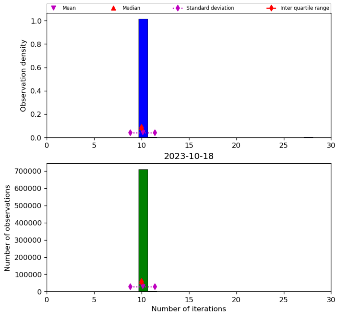
Figure 31: Histogram of “Number of iterations” for 2023-10-17 to 2023-10-19
