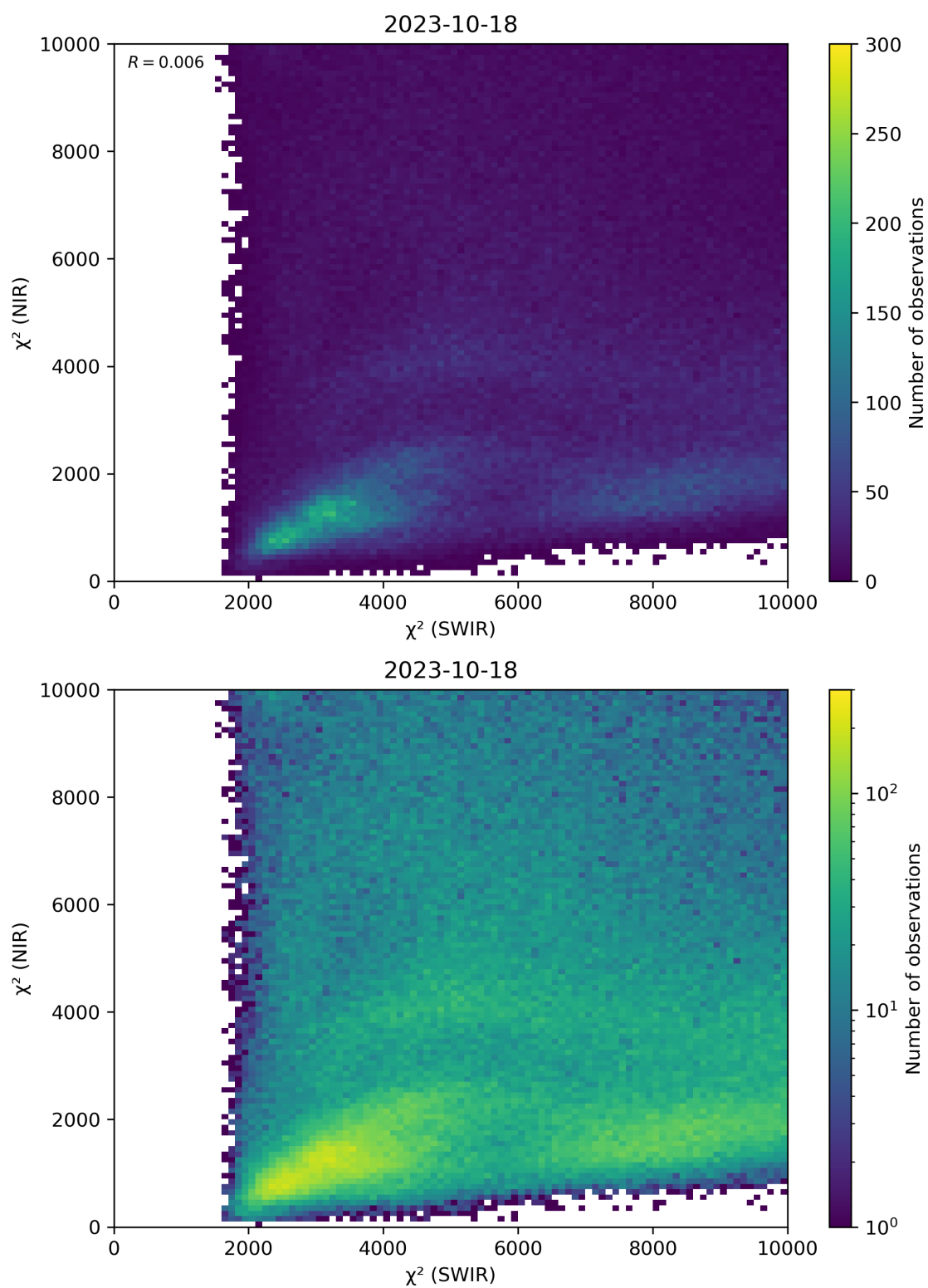
Figure 47: Scatter density plot of “ \chi^2 (SWIR)” against “ \chi^2 (NIR)” for 2023-10-17 to 2023-10-19.
