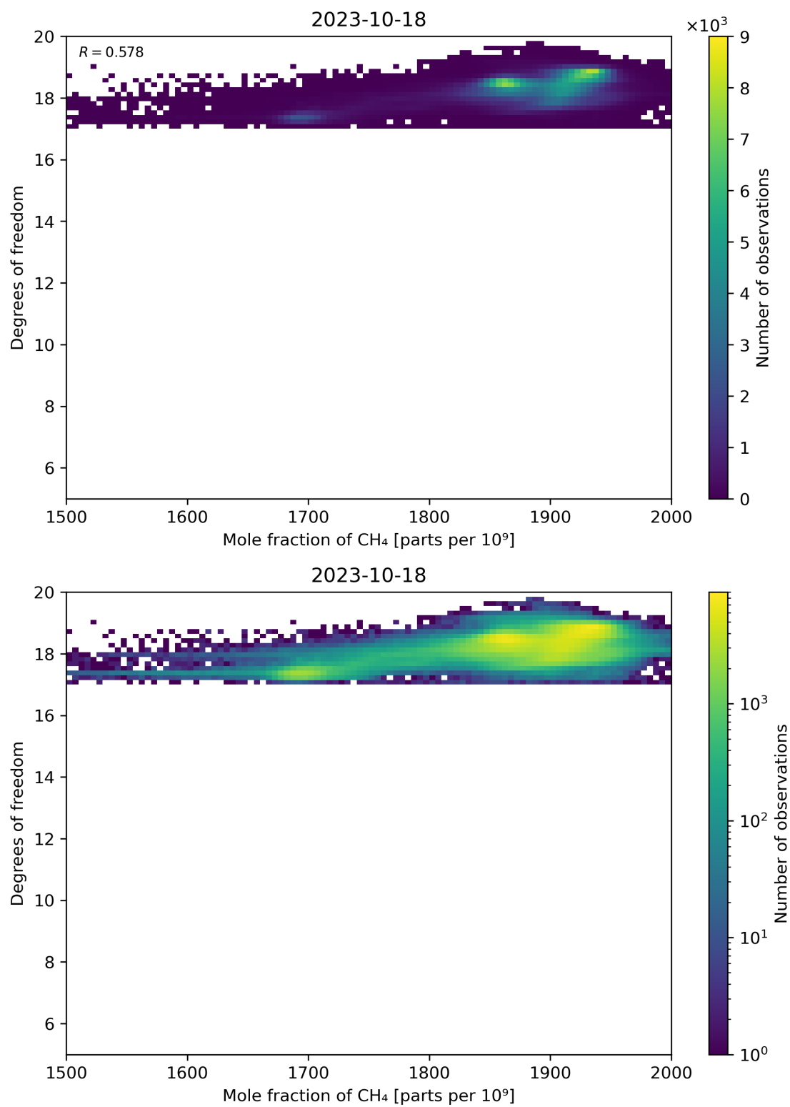
Figure 72: Scatter density plot of “Mole fraction of CH 4 ” against “Degrees of freedom” for 2023-10-17 to 2023-10-19.
