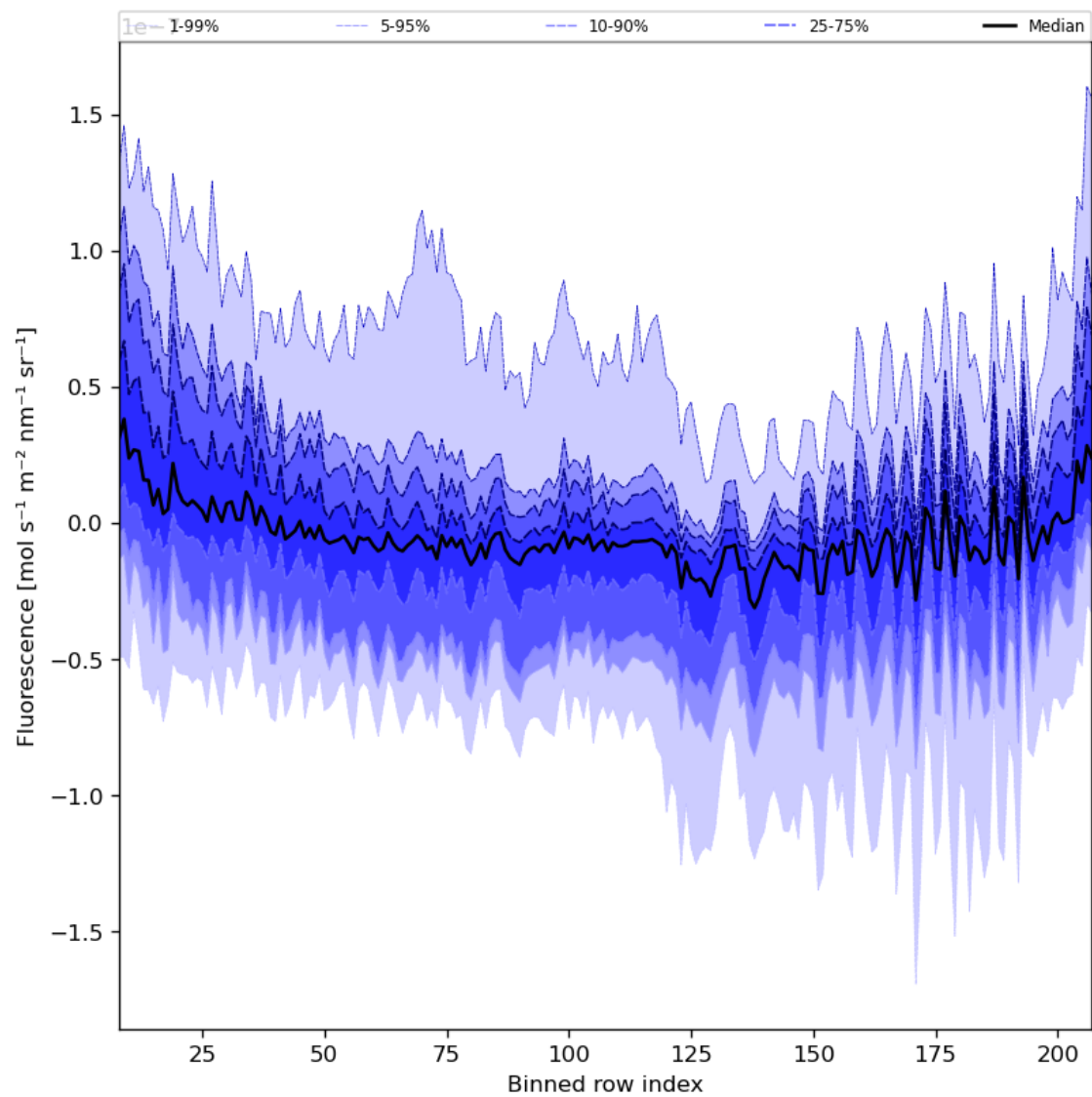
Figure 43: Along track statistics of “Fluorescence” for 2023-10-17 to 2023-10-19
