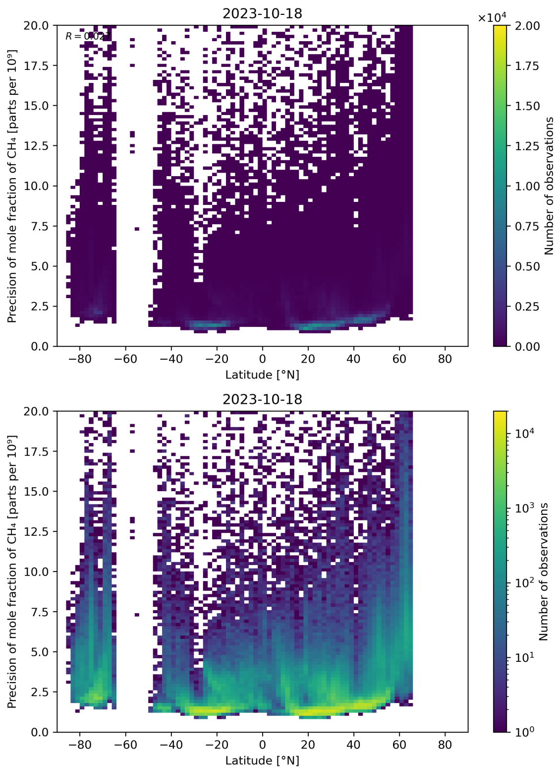
Figure 59: Scatter density plot of “Latitude” against “Precision of mole fraction of CH 4 ” for 2023-10-17 to 2023-10-19.
