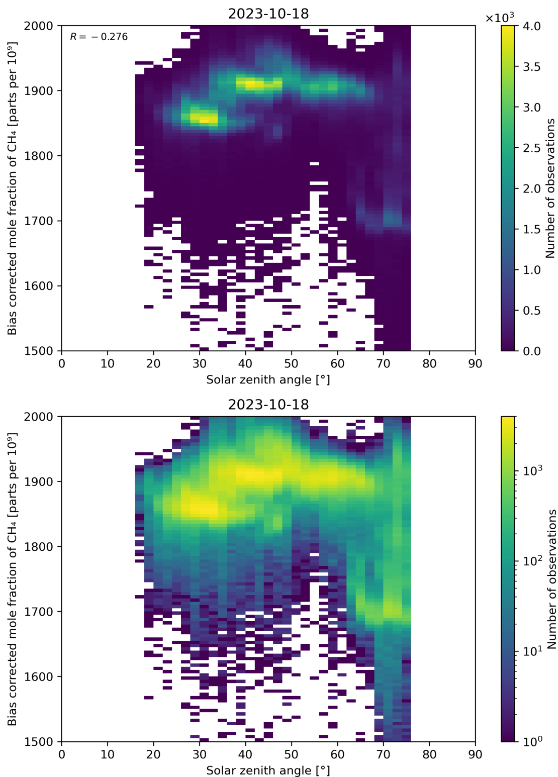
Figure 100: Scatter density plot of “Solar zenith angle” against “Bias corrected mole fraction of \text{CH}_4 ” for 2023-10-17 to 2023-10-19.
