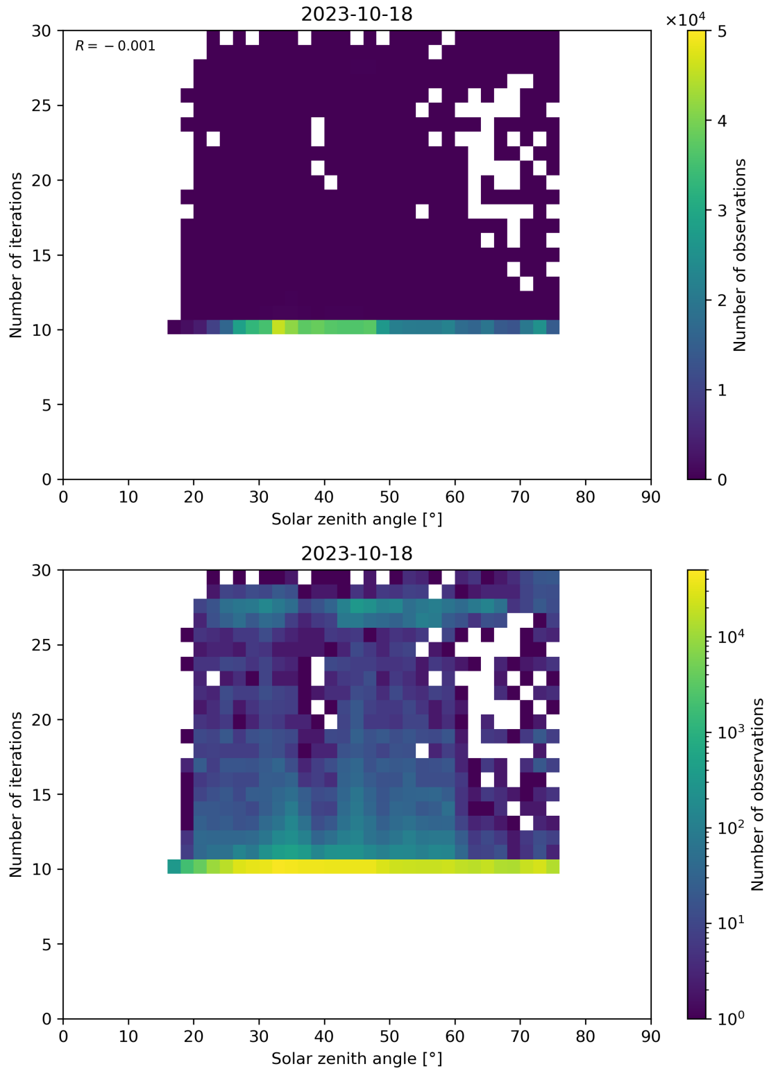
Figure 102: Scatter density plot of “Solar zenith angle” against “Number of iterations” for 2023-10-17 to 2023-10-19.
