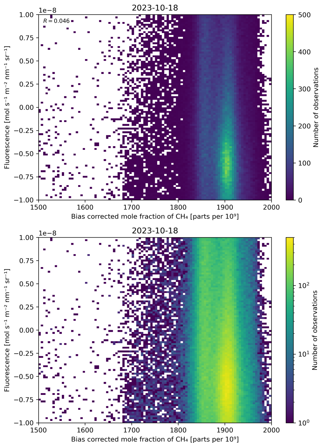
Figure 66: Scatter density plot of “Bias corrected mole fraction of \text{CH}_4 ” against “Fluorescence” for 2023-10-17 to 2023-10-19.
