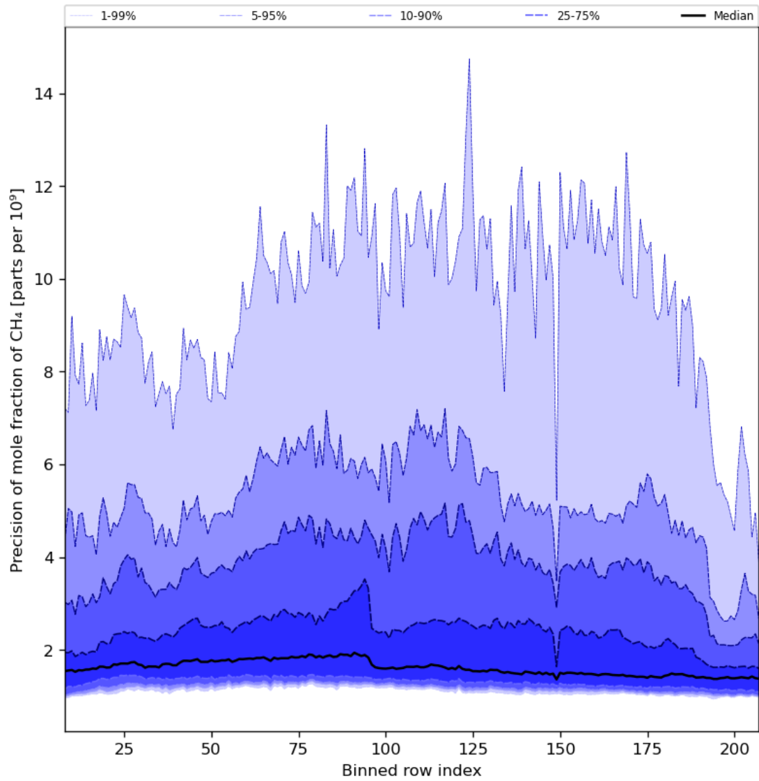
Figure 35: Along track statistics of “Precision of mole fraction of CH 4 ” for 2023-10-17 to 2023-10-19
