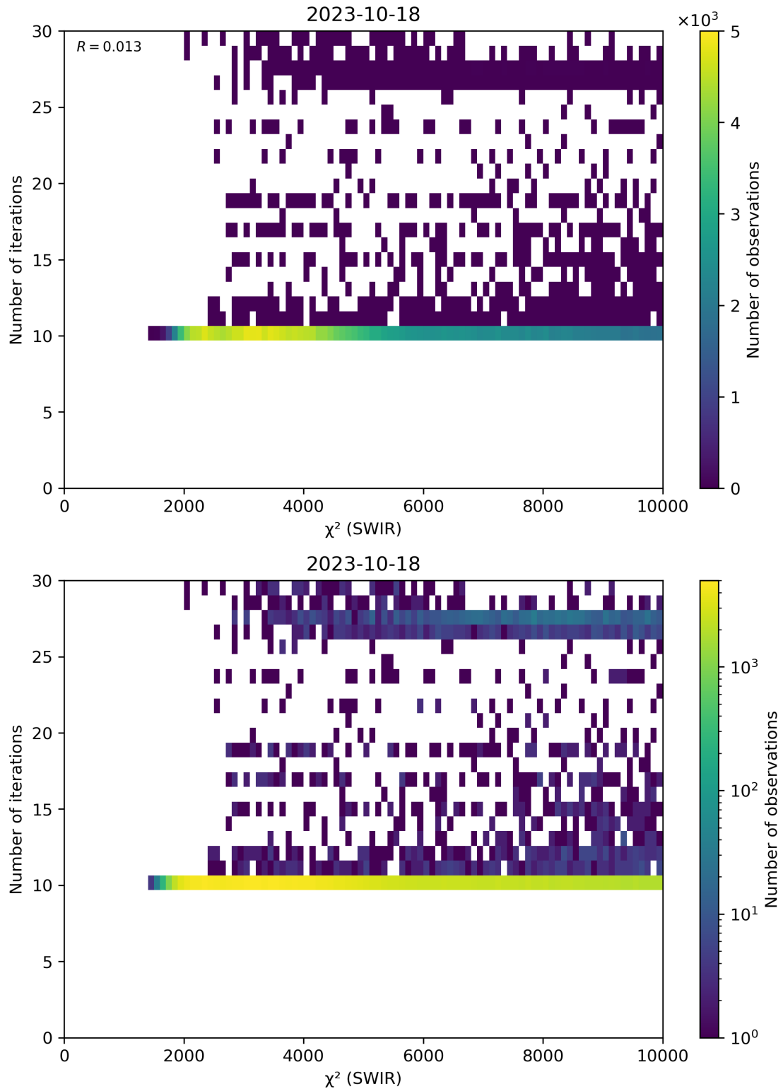
Figure 50: Scatter density plot of “ \chi^2 (SWIR)” against “Number of iterations” for 2023-10-17 to 2023-10-19.
