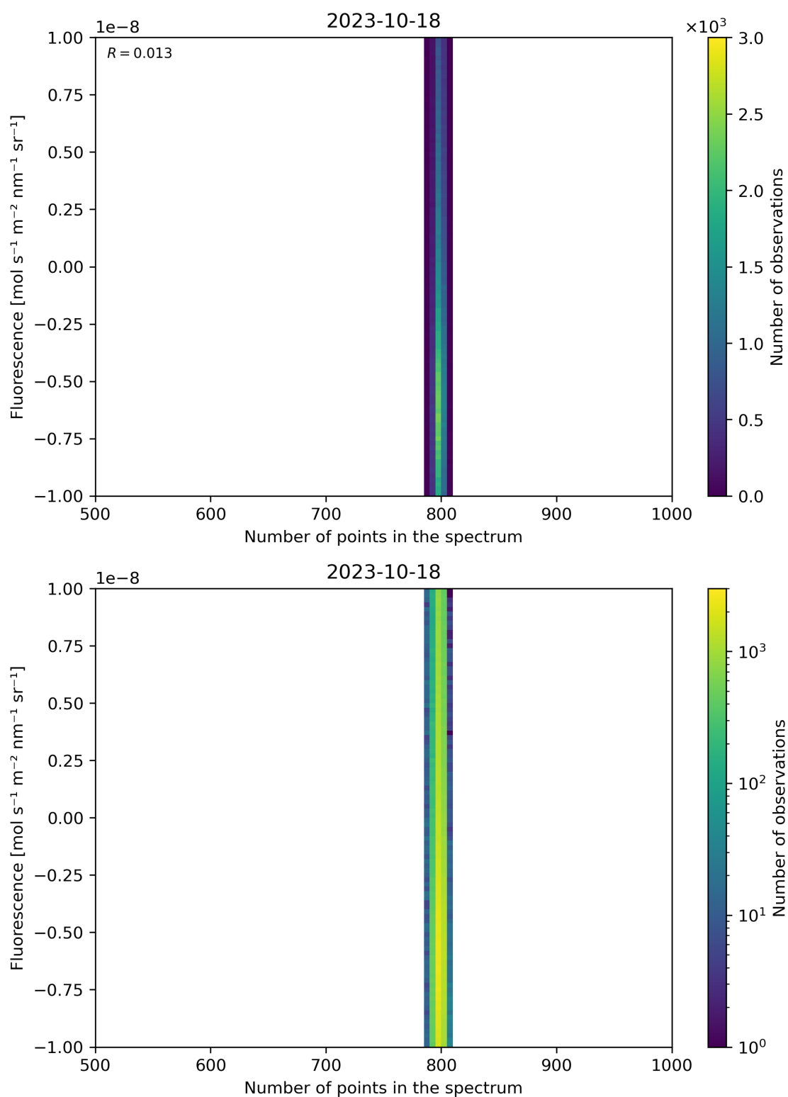
Figure 91: Scatter density plot of “Number of points in the spectrum” against “Fluorescence” for 2023-10-17 to 2023-10-19.
