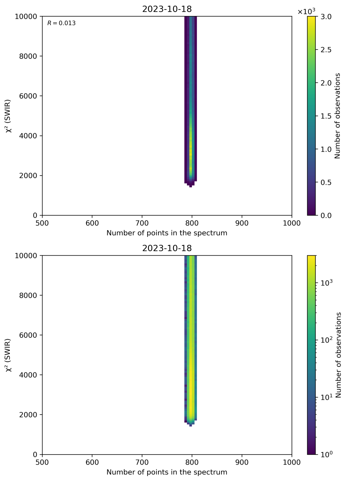
Figure 89: Scatter density plot of “Number of points in the spectrum” against “ \chi^2 (SWIR)” for 2023-10-17 to 2023-10-19.
