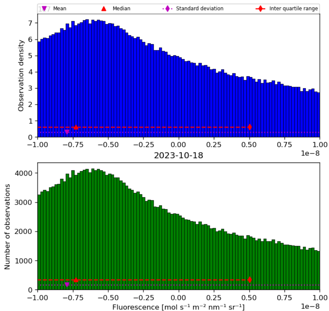
Figure 32: Histogram of “Fluorescence” for 2023-10-17 to 2023-10-19
