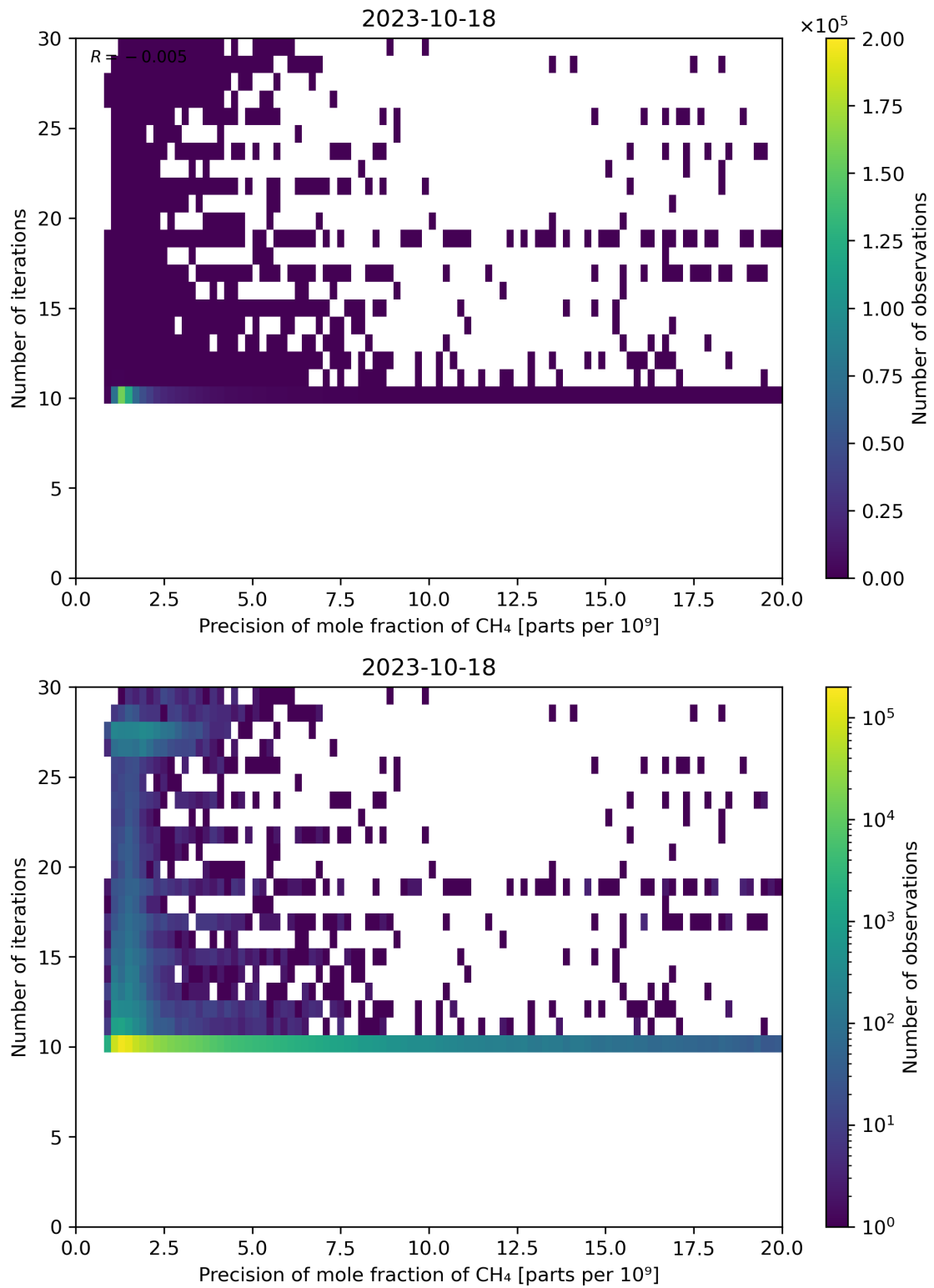
Figure 83: Scatter density plot of “Precision of mole fraction of CH 4 ” against “Number of iterations” for 2023-10-17 to 2023-10-19.
