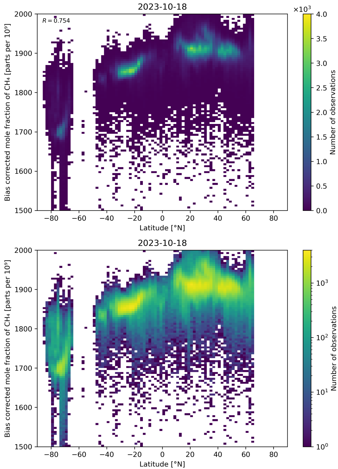
Figure 58: Scatter density plot of “Latitude” against “Bias corrected mole fraction of CH 4 ” for 2023-10-17 to 2023-10-19.
