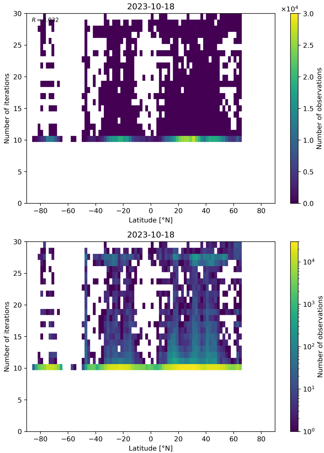
Figure 60: Scatter density plot of “Latitude” against “Number of iterations” for 2023-10-17 to 2023-10-19.
