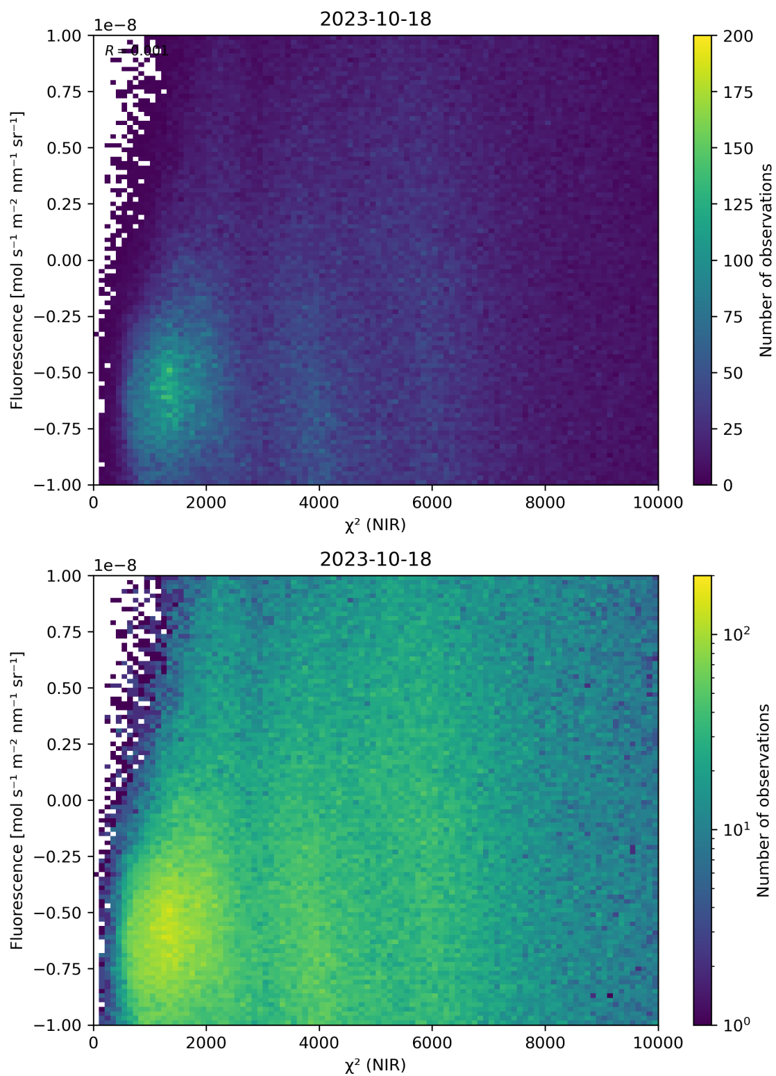
Figure 45: Scatter density plot of “ \chi^2 (NIR)” against “Fluorescence” for 2023-10-17 to 2023-10-19.
