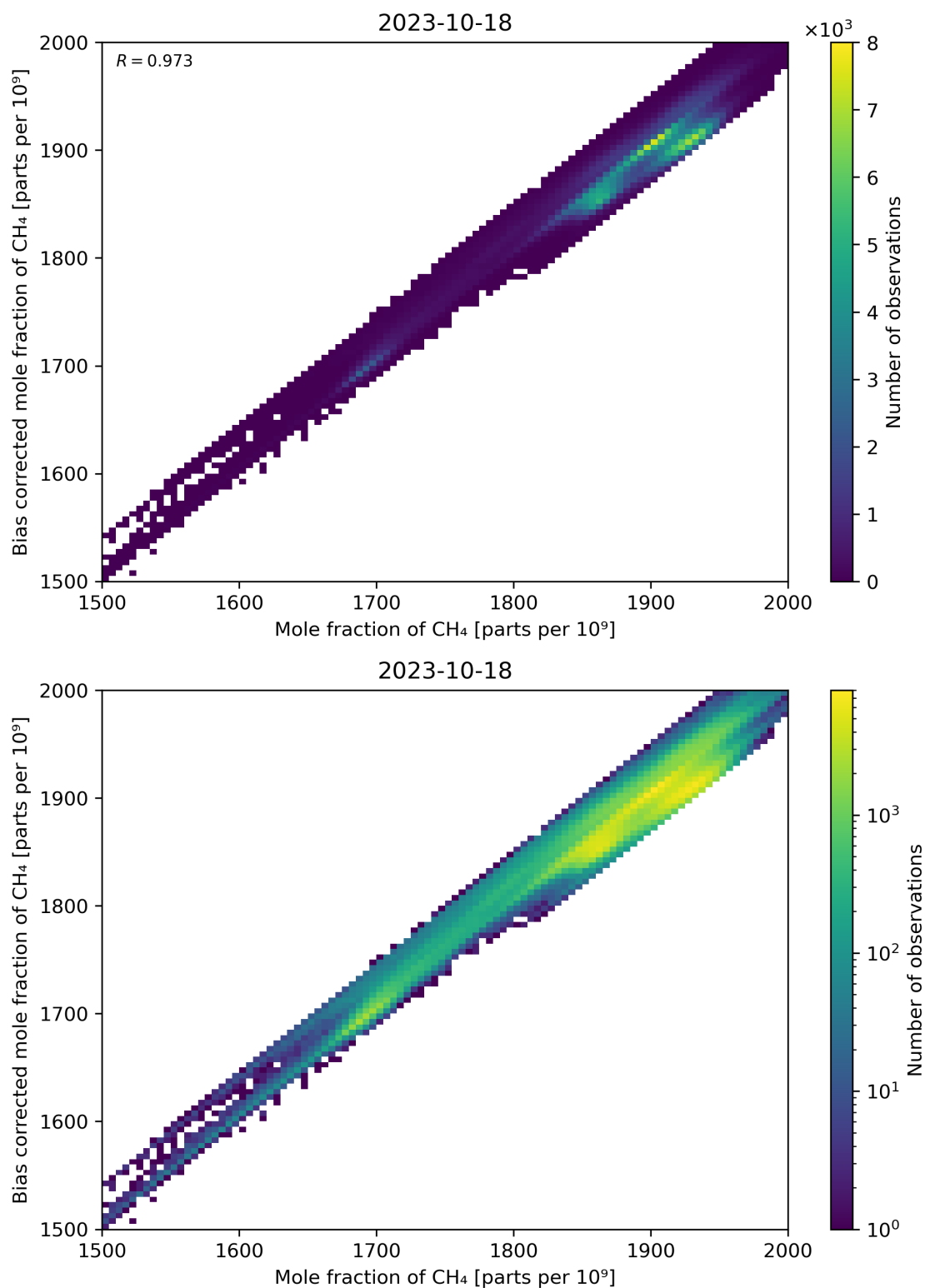
Figure 74: Scatter density plot of “Mole fraction of CH 4 ” against “Bias corrected mole fraction of CH 4 ” for 2023-10-17 to 2023-10-19.
