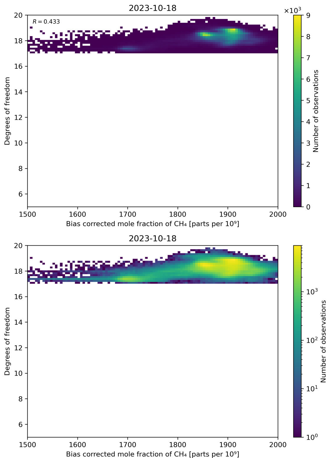
Figure 65: Scatter density plot of “Bias corrected mole fraction of CH 4 ” against “Degrees of freedom” for 2023-10-17 to 2023-10-19.
