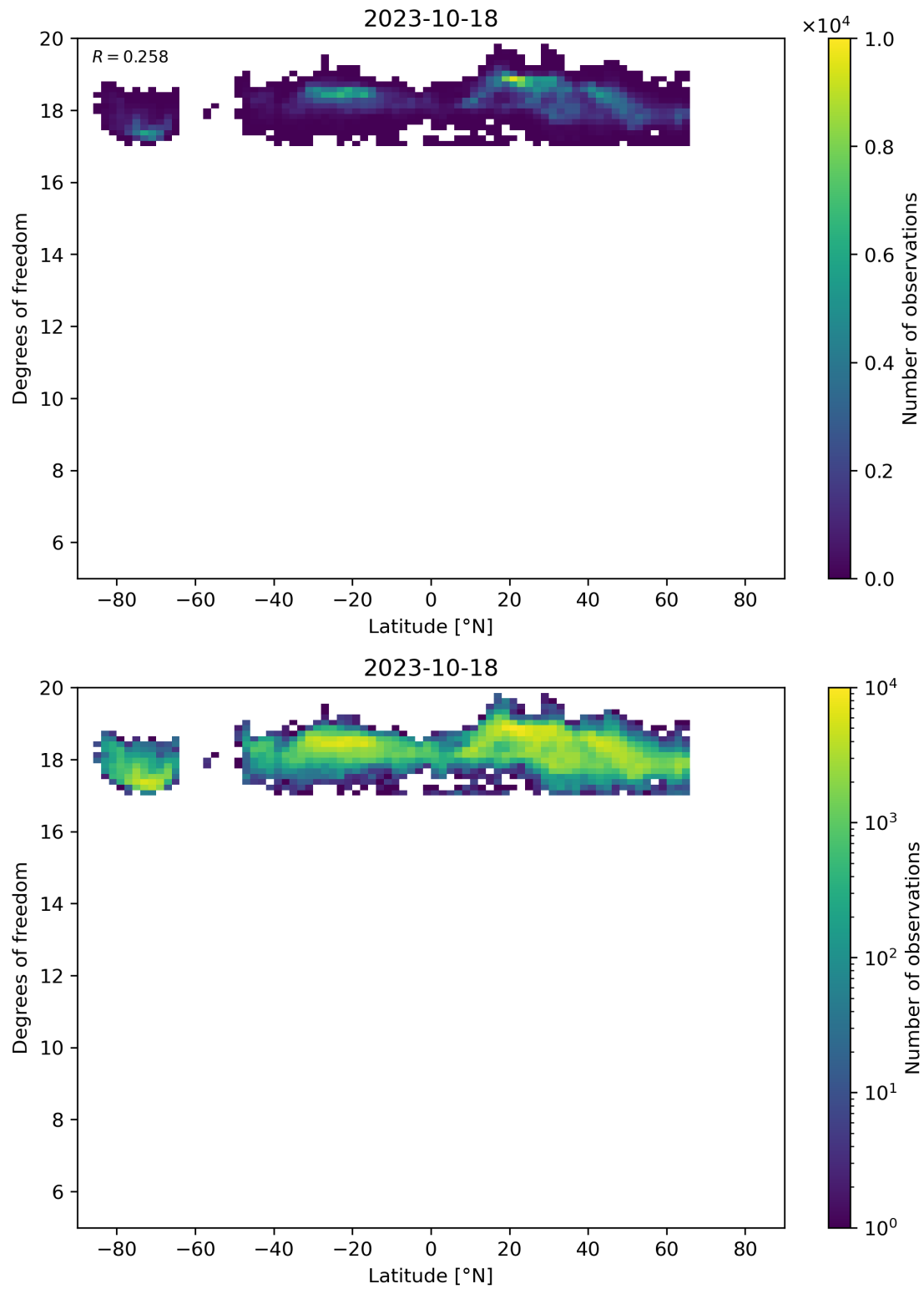
Figure 55: Scatter density plot of “Latitude” against “Degrees of freedom” for 2023-10-17 to 2023-10-19.
