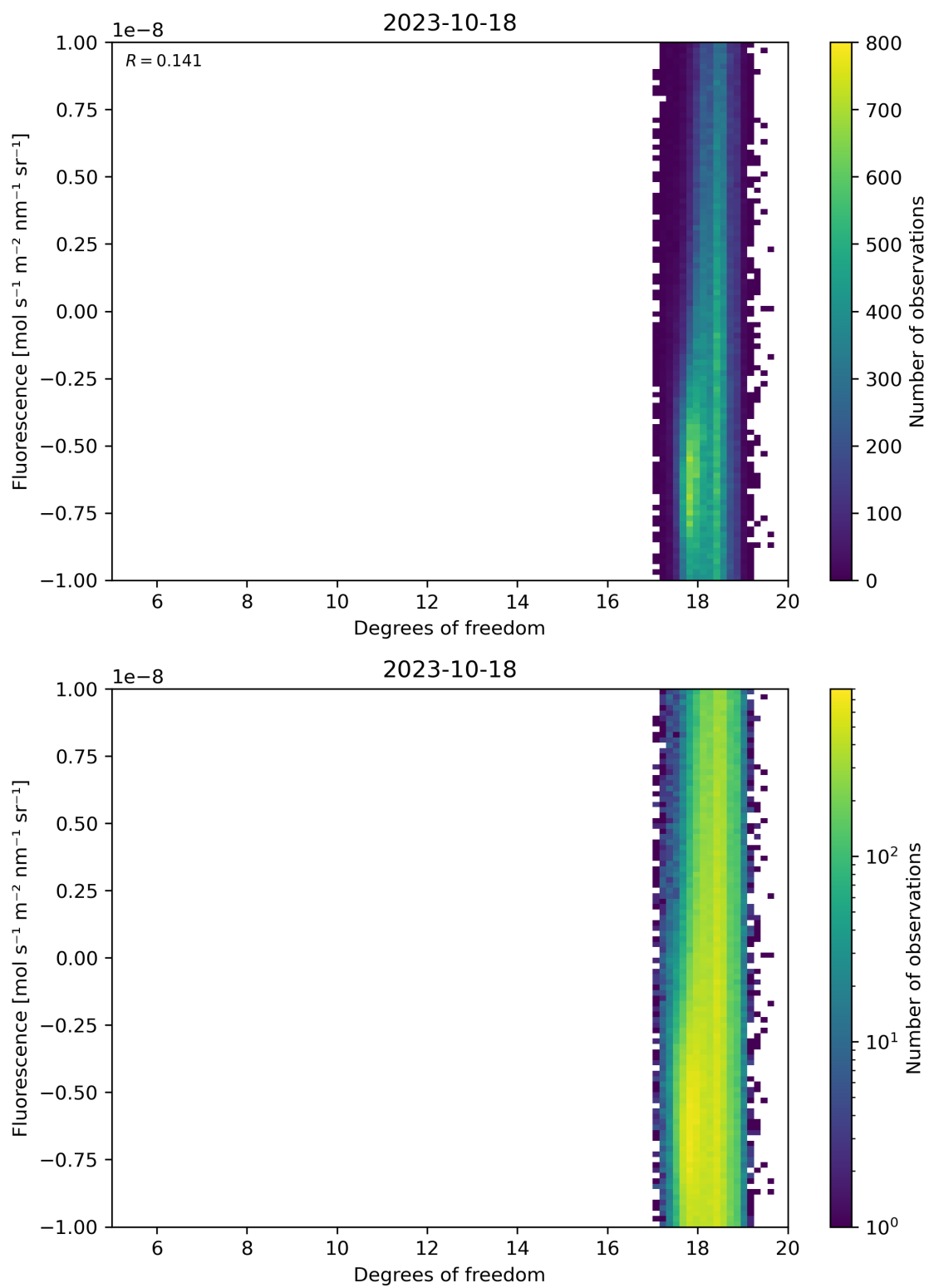
Figure 51: Scatter density plot of “Degrees of freedom” against “Fluorescence” for 2023-10-17 to 2023-10-19.
