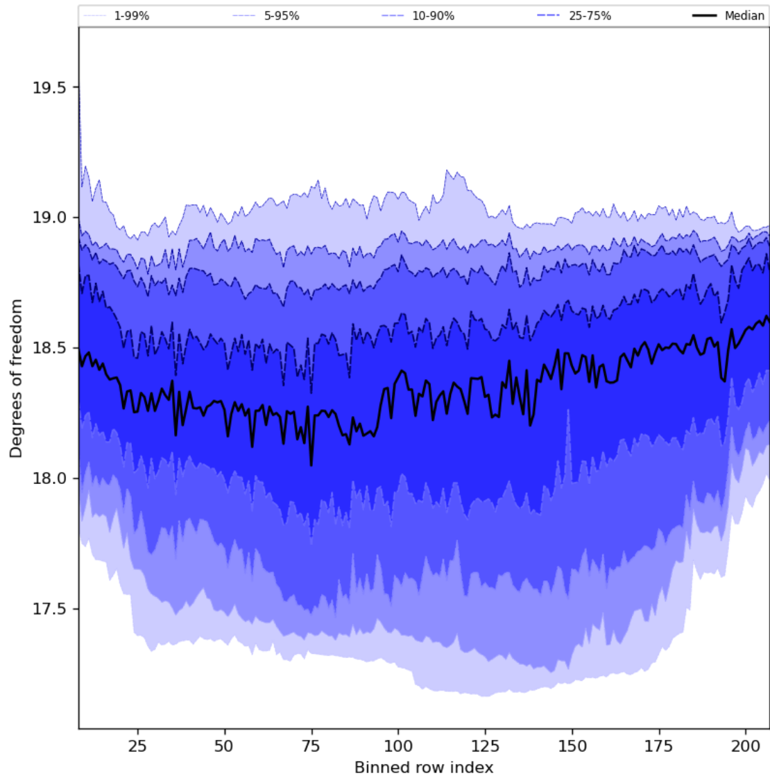
Figure 41: Along track statistics of “Degrees of freedom” for 2023-10-17 to 2023-10-19
