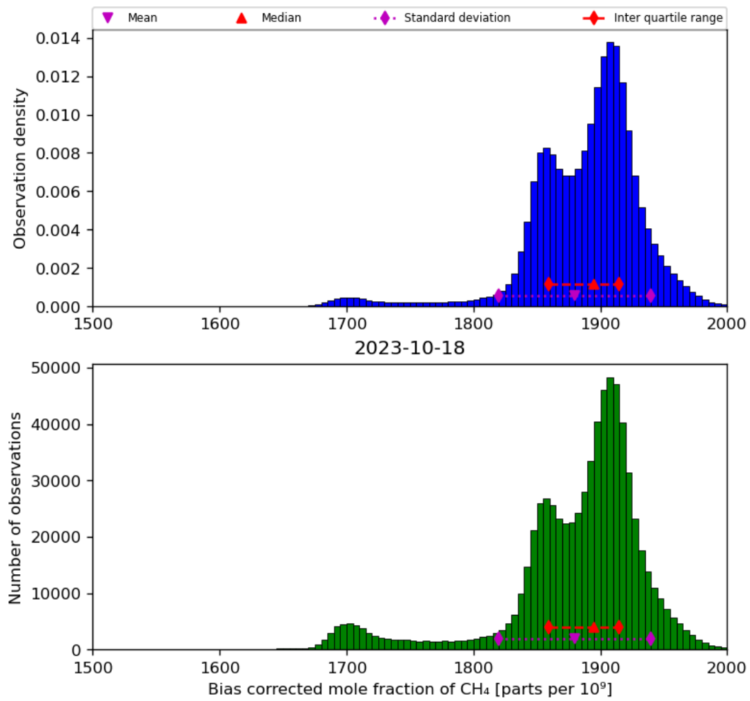
Figure 25: Histogram of “Bias corrected mole fraction of CH 4 ” for 2023-10-17 to 2023-10-19
