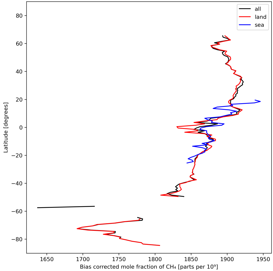
Figure 14: Zonal average of “Bias corrected mole fraction of CH 4 ” for 2023-10-17 to 2023-10-19.
