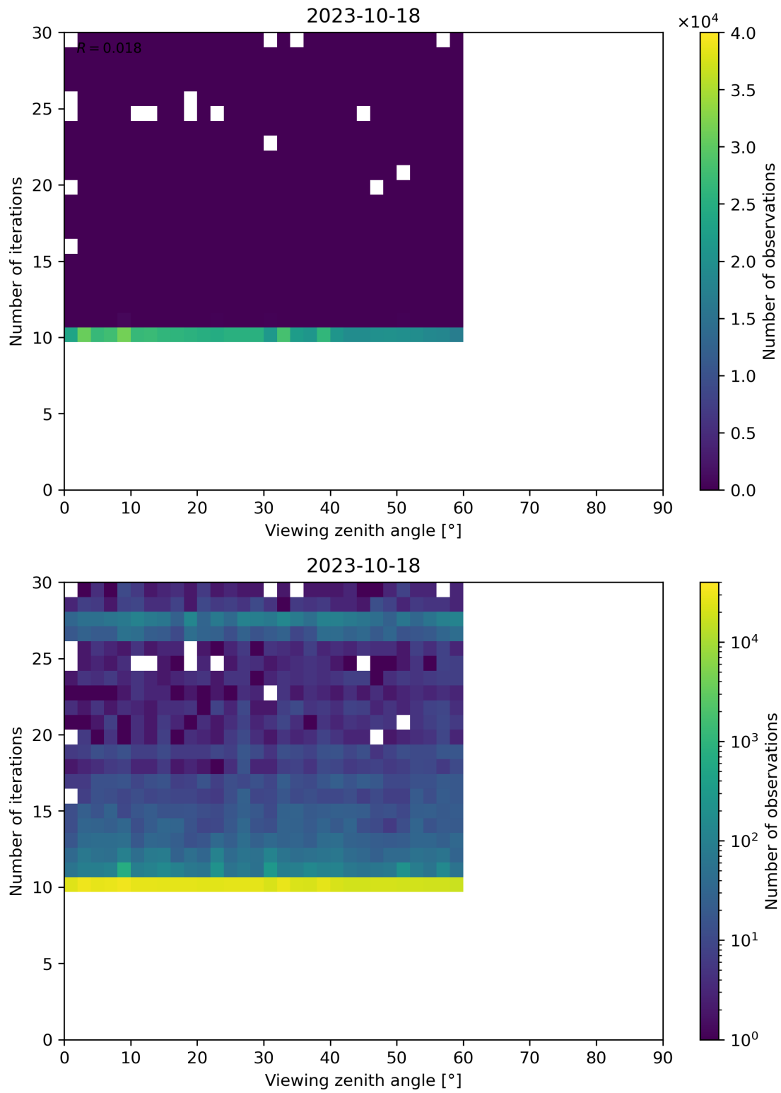
Figure 113: Scatter density plot of “Viewing zenith angle” against “Number of iterations” for 2023-10-17 to 2023-10-19.
