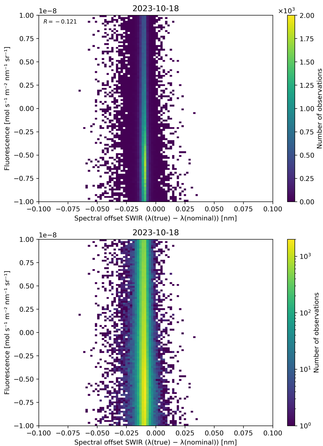
Figure 120: Scatter density plot of “Spectral offset SWIR ( \lambda(\text{true}) - \lambda(\text{nominal}) )” against “Fluorescence” for 2023-10-17 to 2023-10-19.
