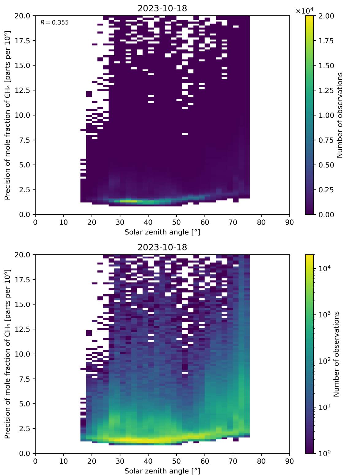
Figure 101: Scatter density plot of “Solar zenith angle” against “Precision of mole fraction of \text{CH}_4 ” for 2023-10-17 to 2023-10-19.
