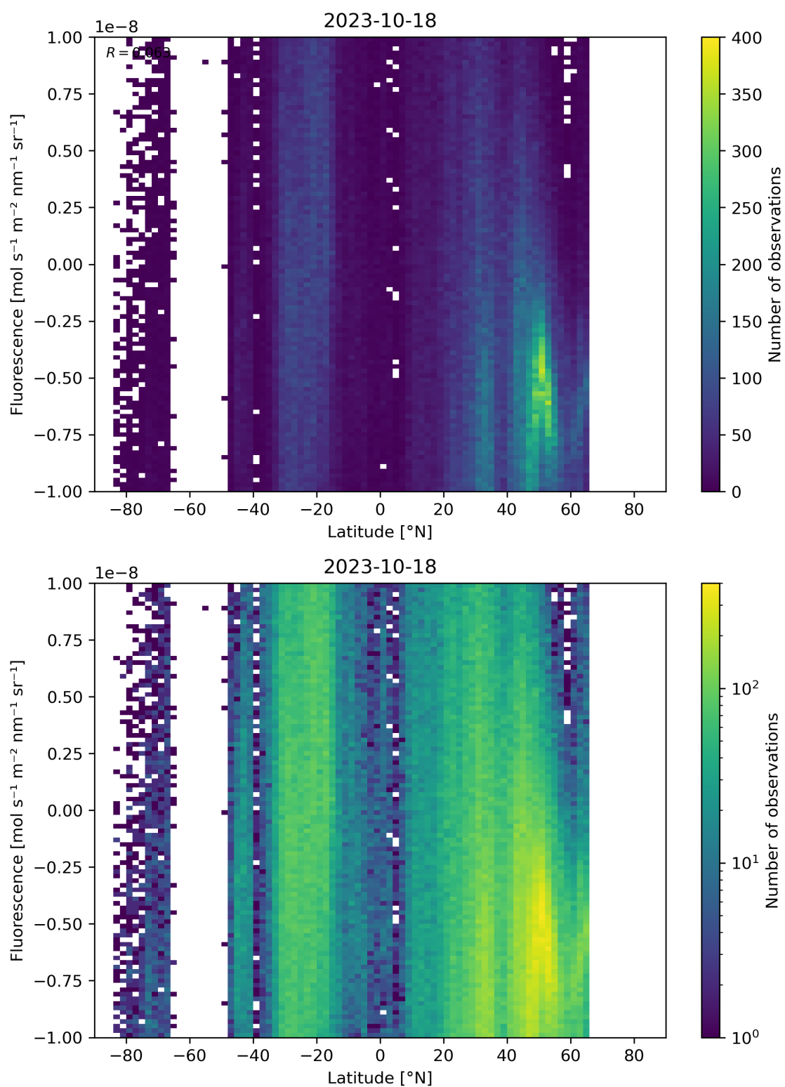
Figure 56: Scatter density plot of “Latitude” against “Fluorescence” for 2023-10-17 to 2023-10-19.
