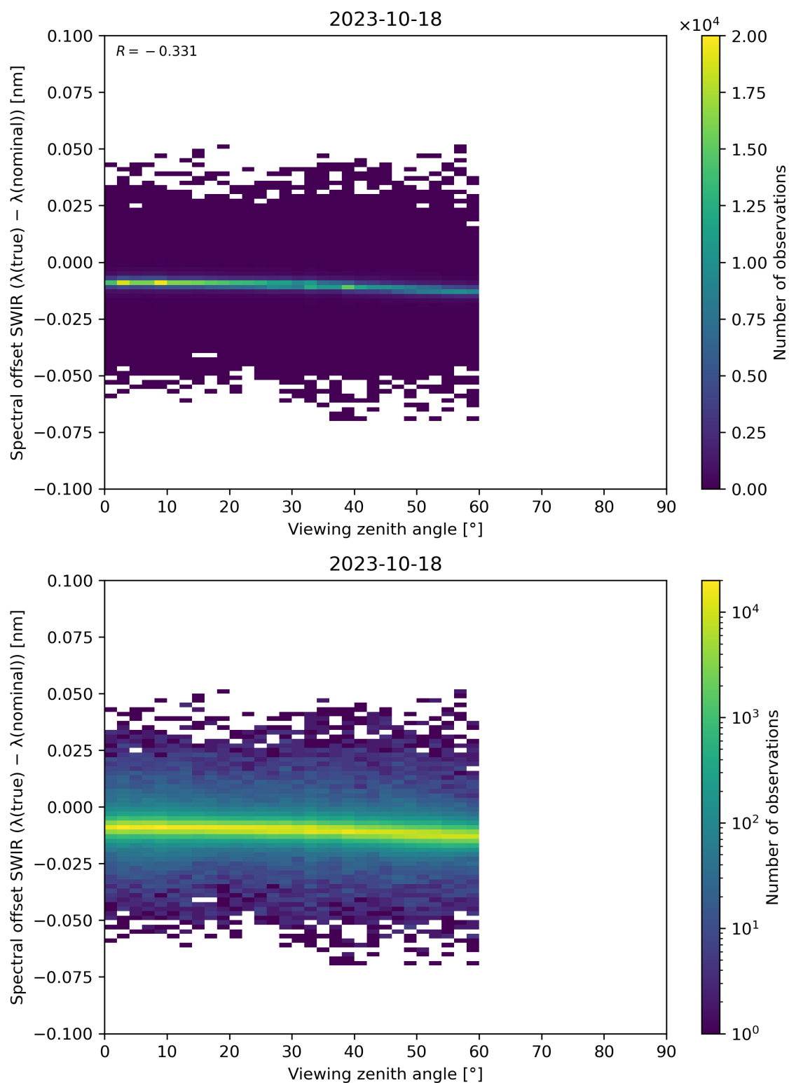
Figure 116: Scatter density plot of “Viewing zenith angle” against “Spectral offset SWIR ( \lambda(\text{true}) - \lambda(\text{nominal}) )” for 2023-10-17 to 2023-10-19.
