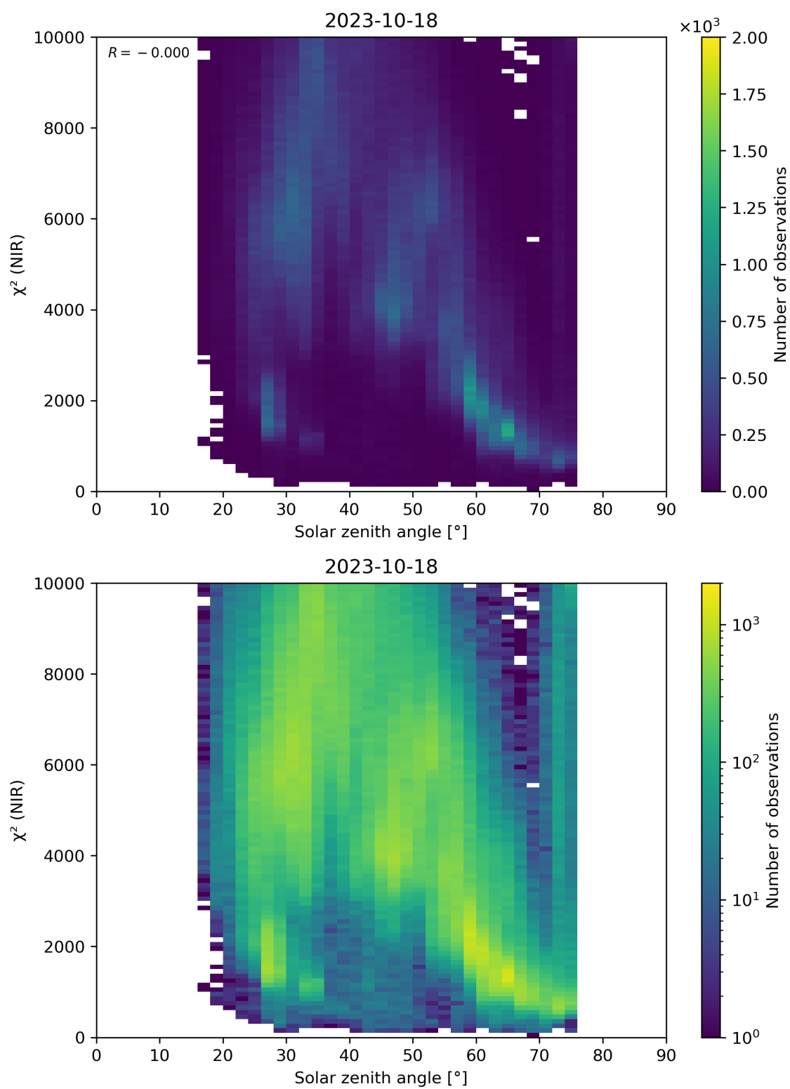
Figure 94: Scatter density plot of “Solar zenith angle” against “ \chi^2 (NIR)” for 2023-10-17 to 2023-10-19.
