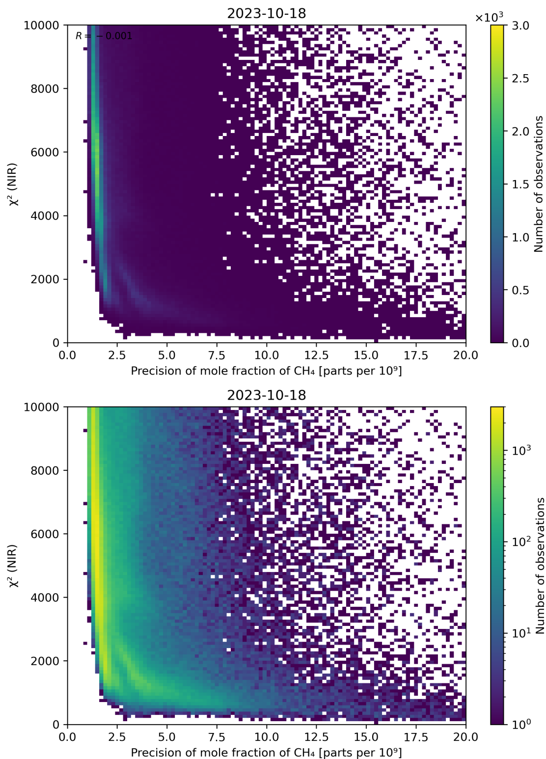
Figure 78: Scatter density plot of “Precision of mole fraction of CH 4 ” against “ \chi^2 (NIR)” for 2023-10-17 to 2023-10-19.
