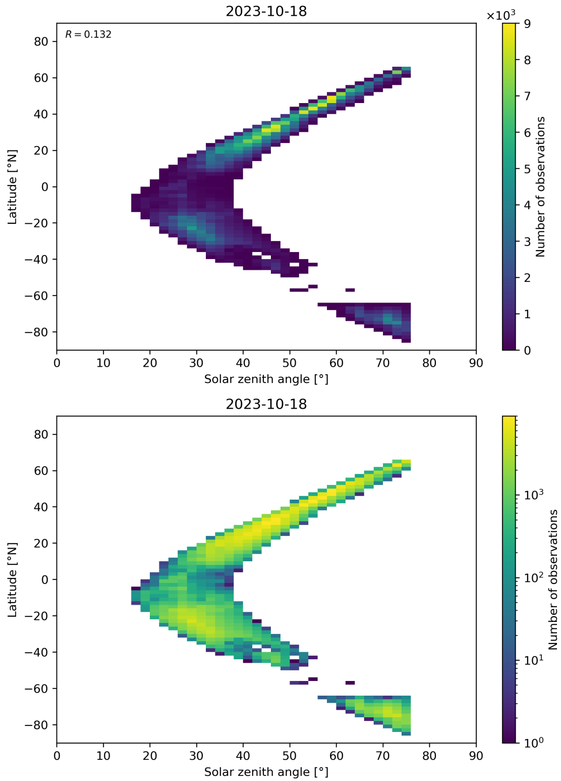
Figure 98: Scatter density plot of “Solar zenith angle” against “Latitude” for 2023-10-17 to 2023-10-19.
