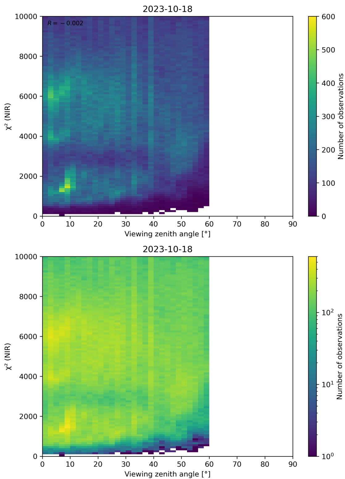
Figure 105: Scatter density plot of “Viewing zenith angle” against “ \chi^2 (NIR)” for 2023-10-17 to 2023-10-19.
