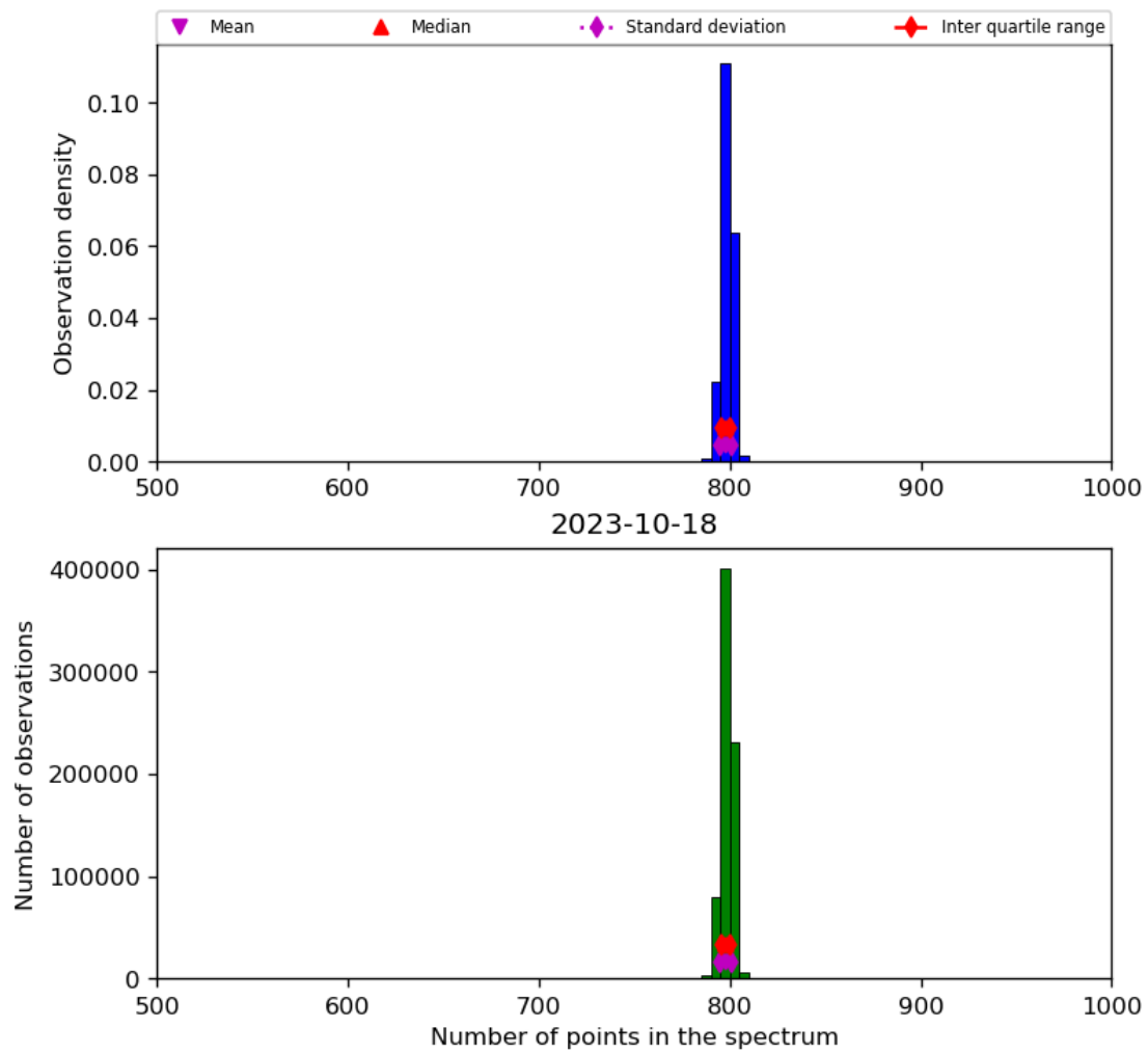
Figure 26: Histogram of “Number of points in the spectrum” for 2023-10-17 to 2023-10-19
