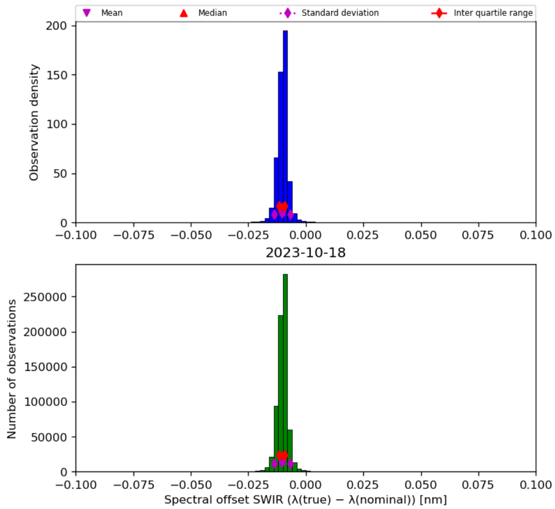
Figure 27: Histogram of “Spectral offset SWIR ( \lambda(\text{true}) - \lambda(\text{nominal}) )” for 2023-10-17 to 2023-10-19
