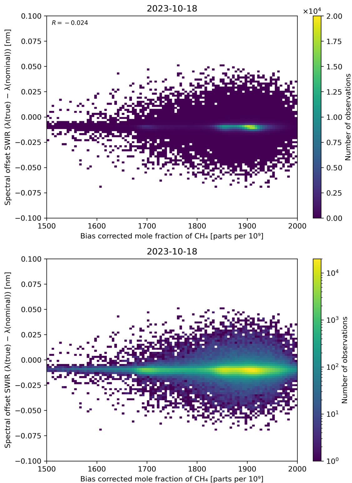
Figure 69: Scatter density plot of “Bias corrected mole fraction of \text{CH}_4 ” against “Spectral offset SWIR ( \lambda(\text{true}) - \lambda(\text{nominal}) )” for 2023-10-17 to 2023-10-19.
