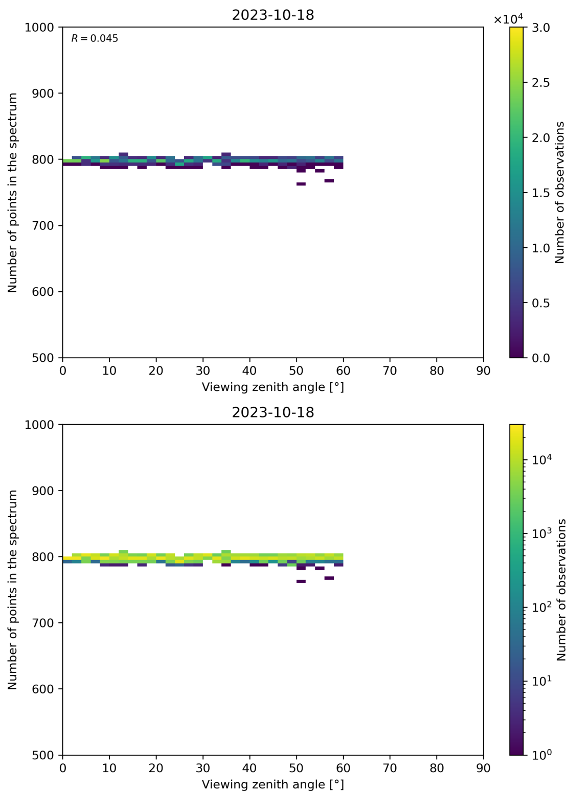
Figure 114: Scatter density plot of “Viewing zenith angle” against “Number of points in the spectrum” for 2023-10-17 to 2023-10-19.
