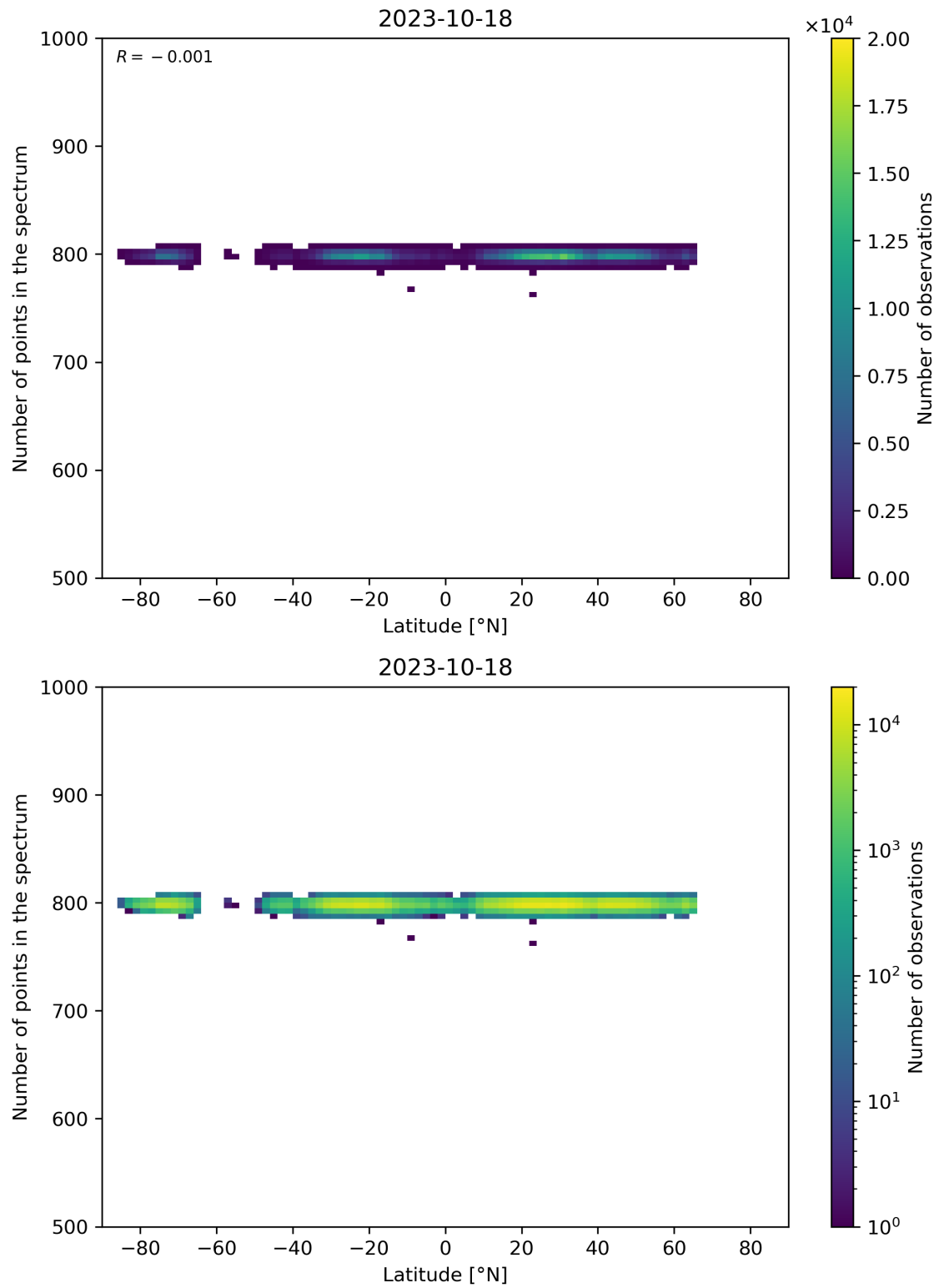
Figure 61: Scatter density plot of “Latitude” against “Number of points in the spectrum” for 2023-10-17 to 2023-10-19.
