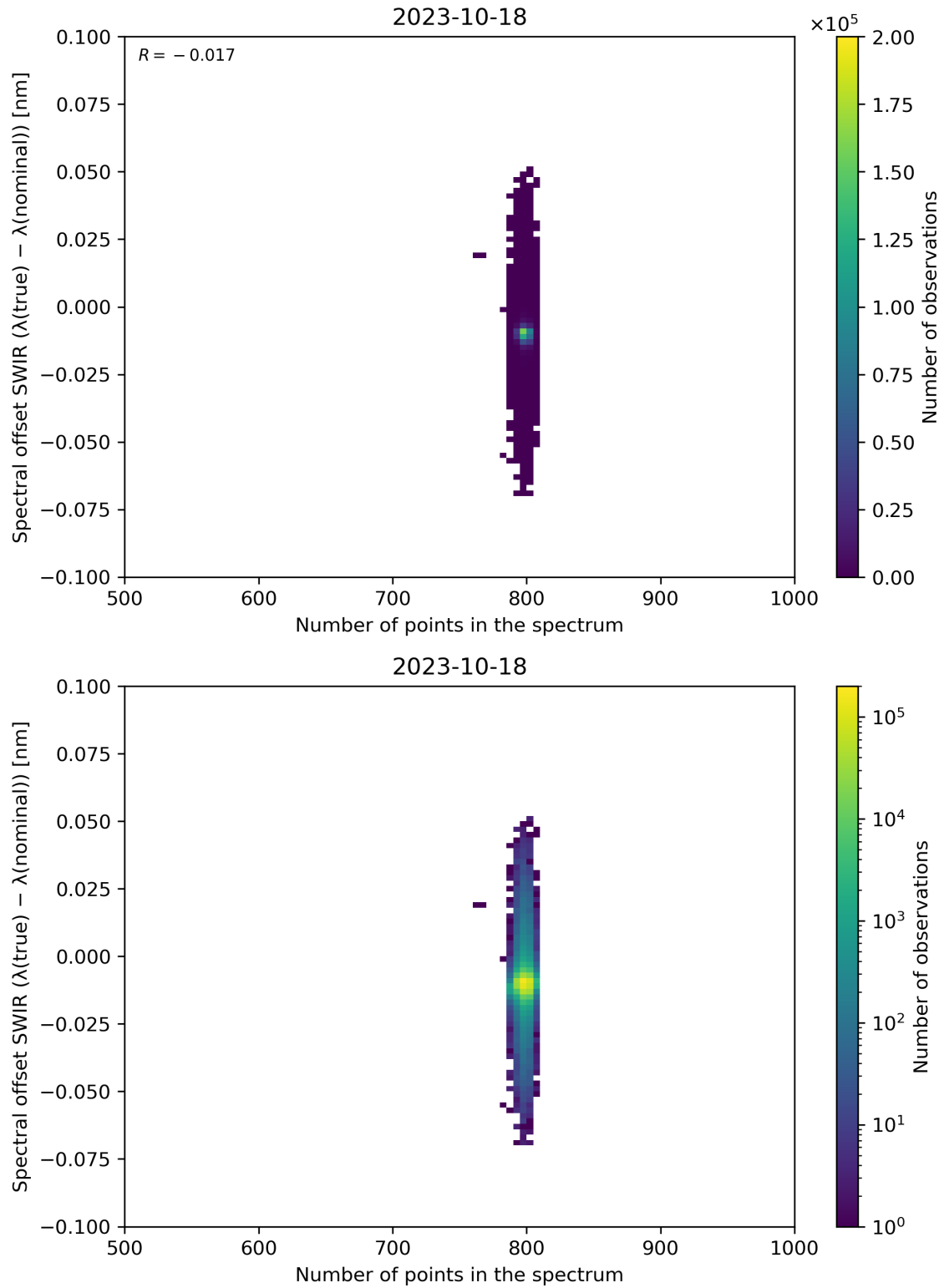
Figure 93: Scatter density plot of “Number of points in the spectrum” against “Spectral offset SWIR ( \lambda(\text{true}) - \lambda(\text{nominal}) )” for 2023-10-17 to 2023-10-19.
