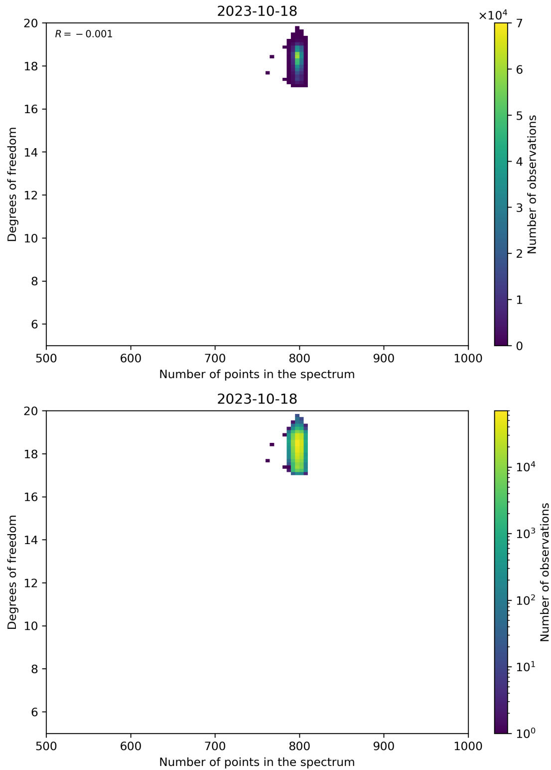
Figure 90: Scatter density plot of “Number of points in the spectrum” against “Degrees of freedom” for 2023-10-17 to 2023-10-19.
