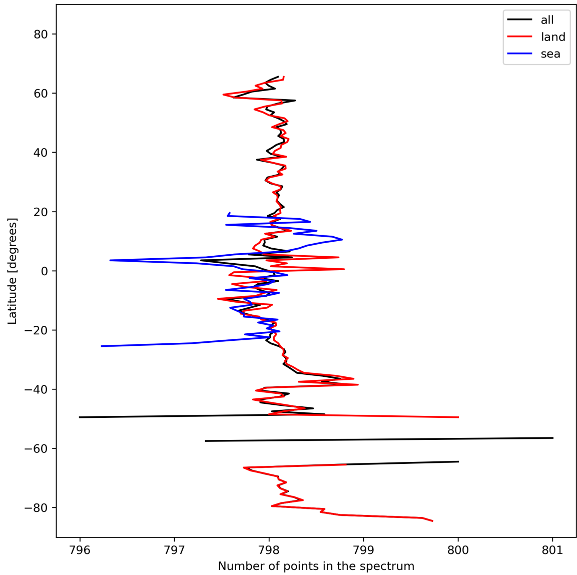
Figure 15: Zonal average of “Number of points in the spectrum” for 2023-10-17 to 2023-10-19.
