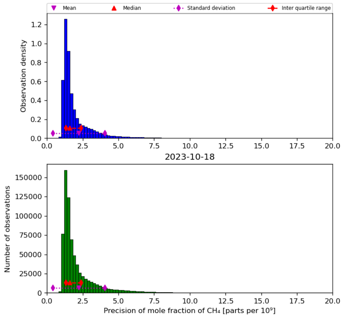
Figure 24: Histogram of “Precision of mole fraction of CH 4 ” for 2023-10-17 to 2023-10-19
