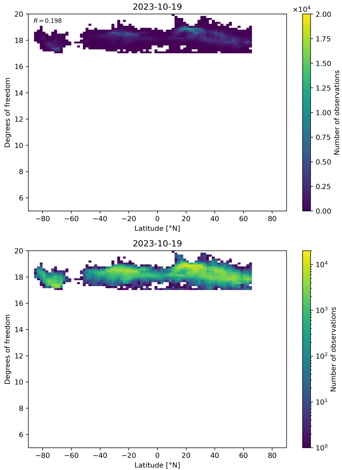
Figure 55: Scatter density plot of “Latitude” against “Degrees of freedom” for 2023-10-18 to 2023-10-20.
