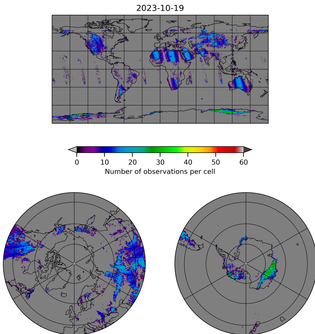
Figure 10: Map of the number of observations for 2023-10-18 to 2023-10-20
