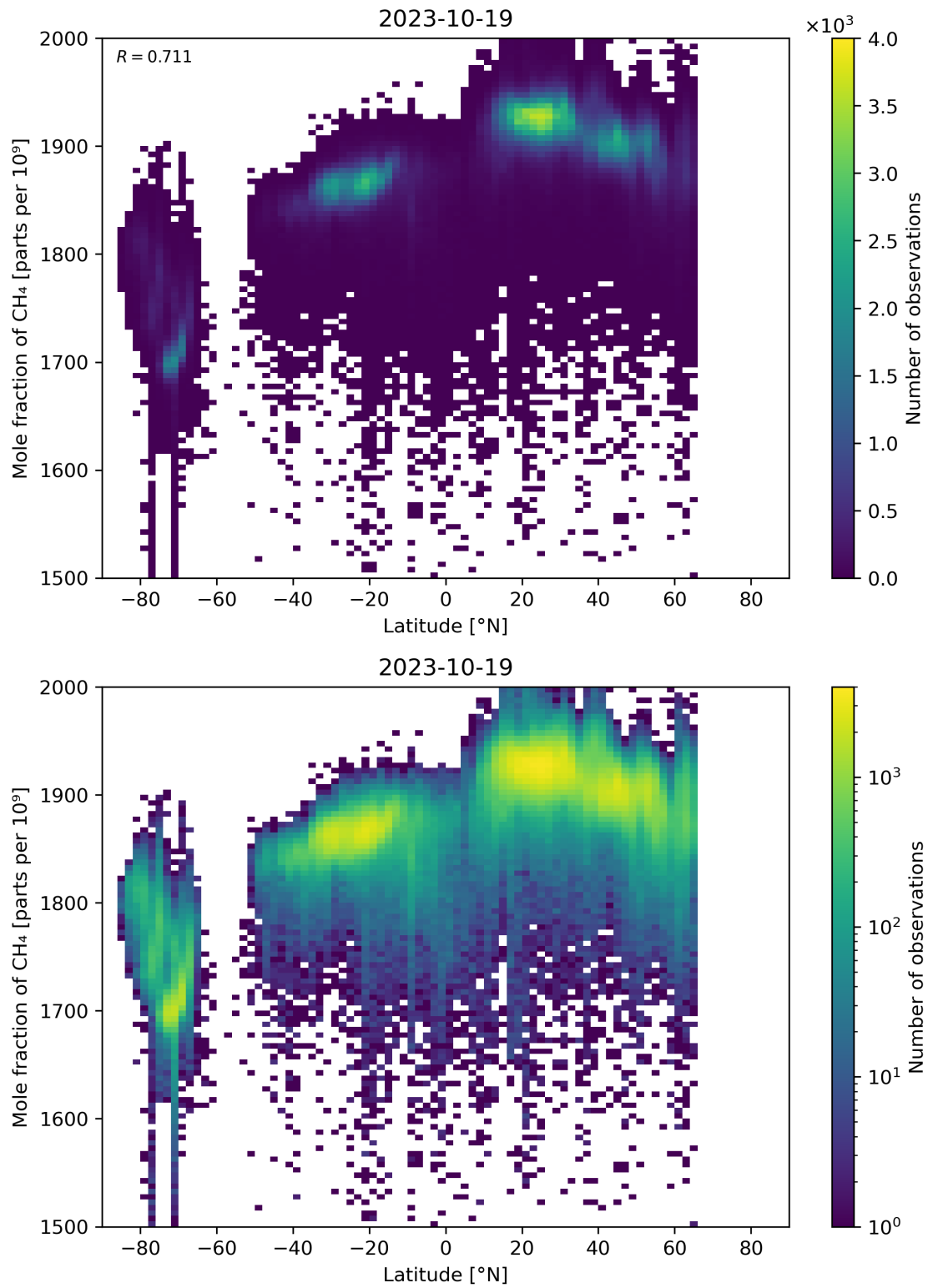
Figure 57: Scatter density plot of “Latitude” against “Mole fraction of \text{CH}_4 ” for 2023-10-18 to 2023-10-20.
