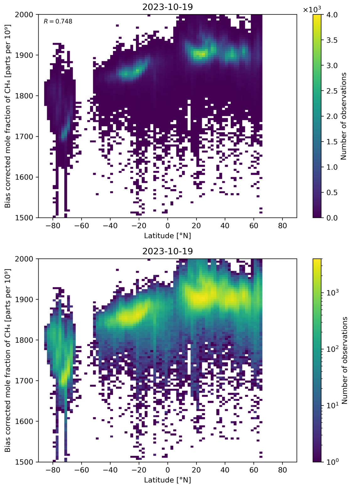
Figure 58: Scatter density plot of “Latitude” against “Bias corrected mole fraction of CH 4 ” for 2023-10-18 to 2023-10-20.
