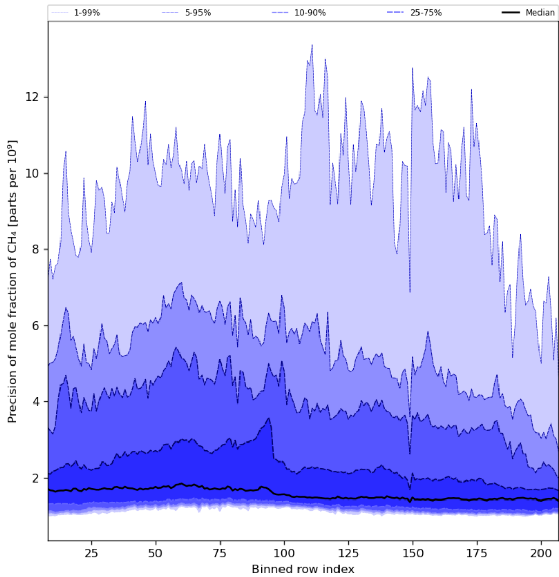
Figure 35: Along track statistics of “Precision of mole fraction of \text{CH}_4 ” for 2023-10-18 to 2023-10-20
