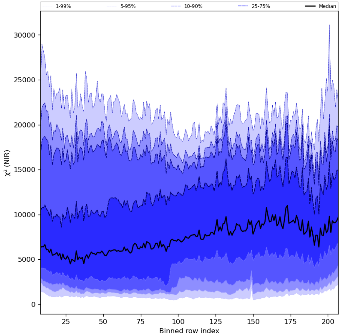
Figure 40: Along track statistics of “ \chi^2 (NIR)” for 2023-10-18 to 2023-10-20
