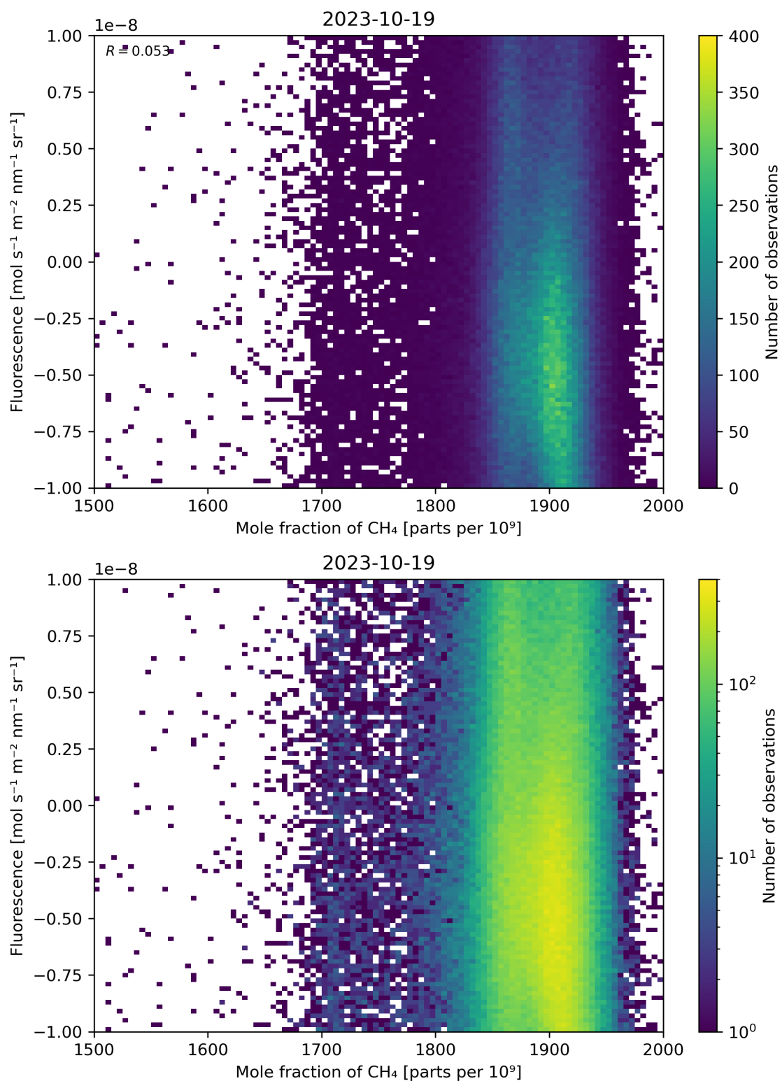
Figure 73: Scatter density plot of “Mole fraction of CH 4 ” against “Fluorescence” for 2023-10-18 to 2023-10-20.
