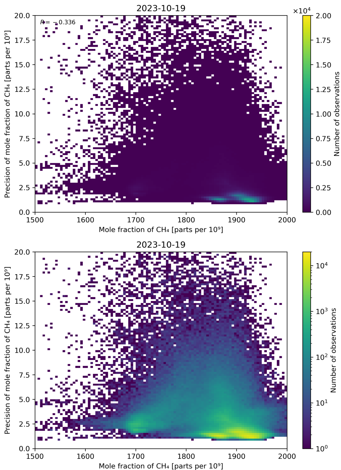
Figure 75: Scatter density plot of “Mole fraction of CH 4 ” against “Precision of mole fraction of CH 4 ” for 2023-10-18 to 2023-10-20.
