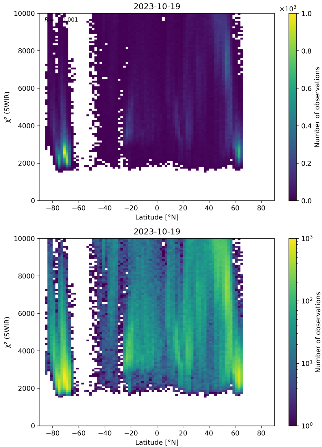
Figure 54: Scatter density plot of “Latitude” against “ \chi^2 (SWIR)” for 2023-10-18 to 2023-10-20.
