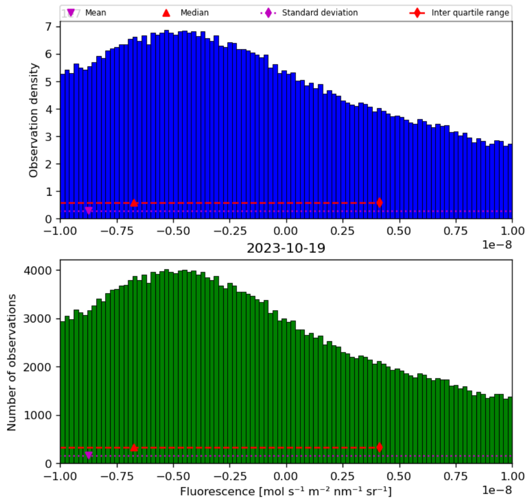
Figure 32: Histogram of “Fluorescence” for 2023-10-18 to 2023-10-20
