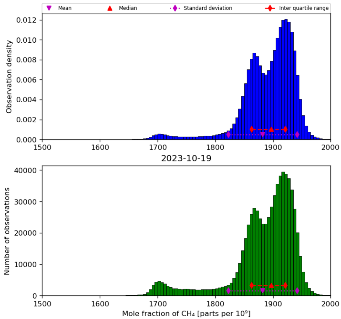
Figure 23: Histogram of “Mole fraction of CH 4 ” for 2023-10-18 to 2023-10-20
