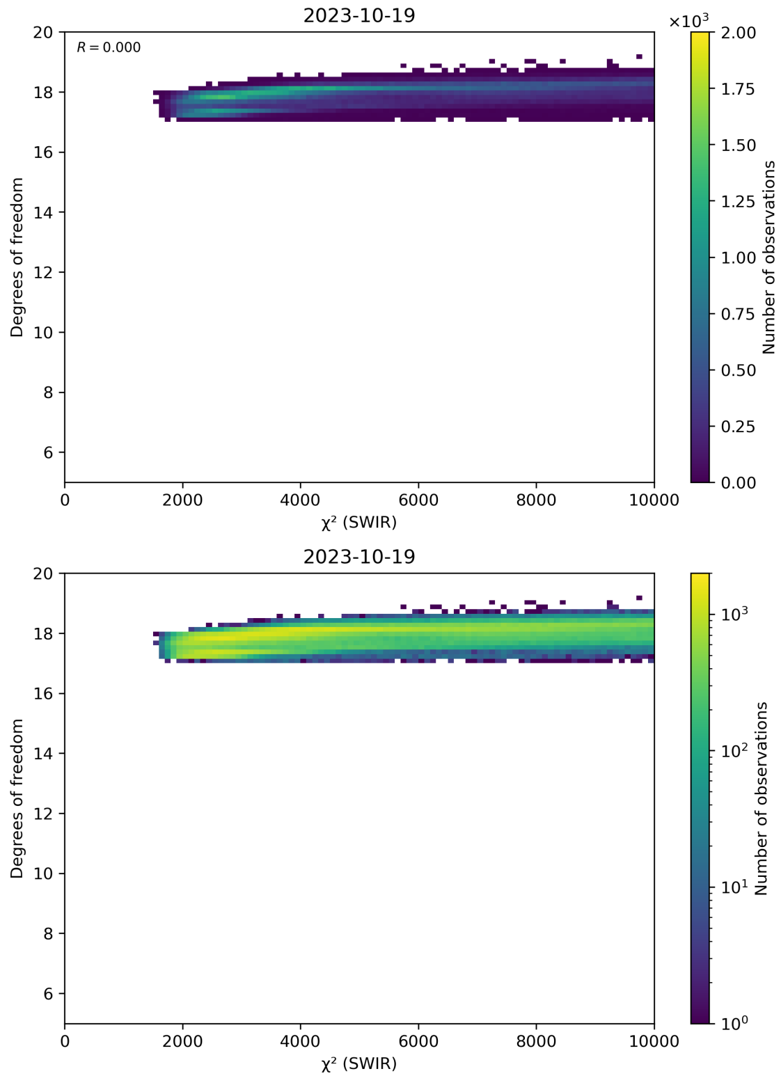
Figure 48: Scatter density plot of “ \chi^2 (SWIR)” against “Degrees of freedom” for 2023-10-18 to 2023-10-20.
