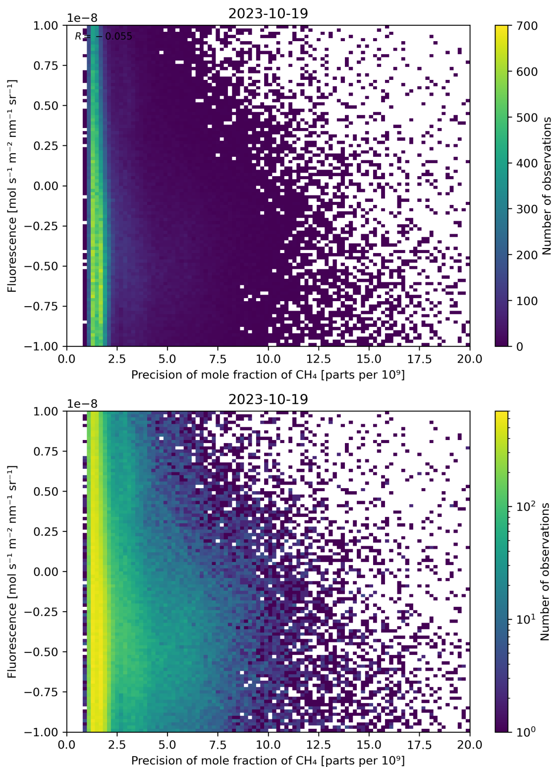
Figure 81: Scatter density plot of “Precision of mole fraction of CH 4 ” against “Fluorescence” for 2023-10-18 to 2023-10-20.
