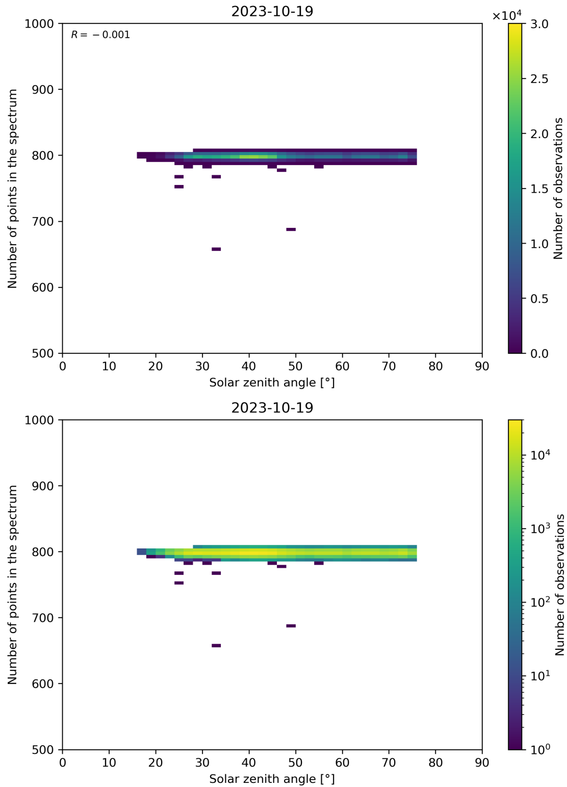
Figure 103: Scatter density plot of “Solar zenith angle” against “Number of points in the spectrum” for 2023-10-18 to 2023-10-20.
