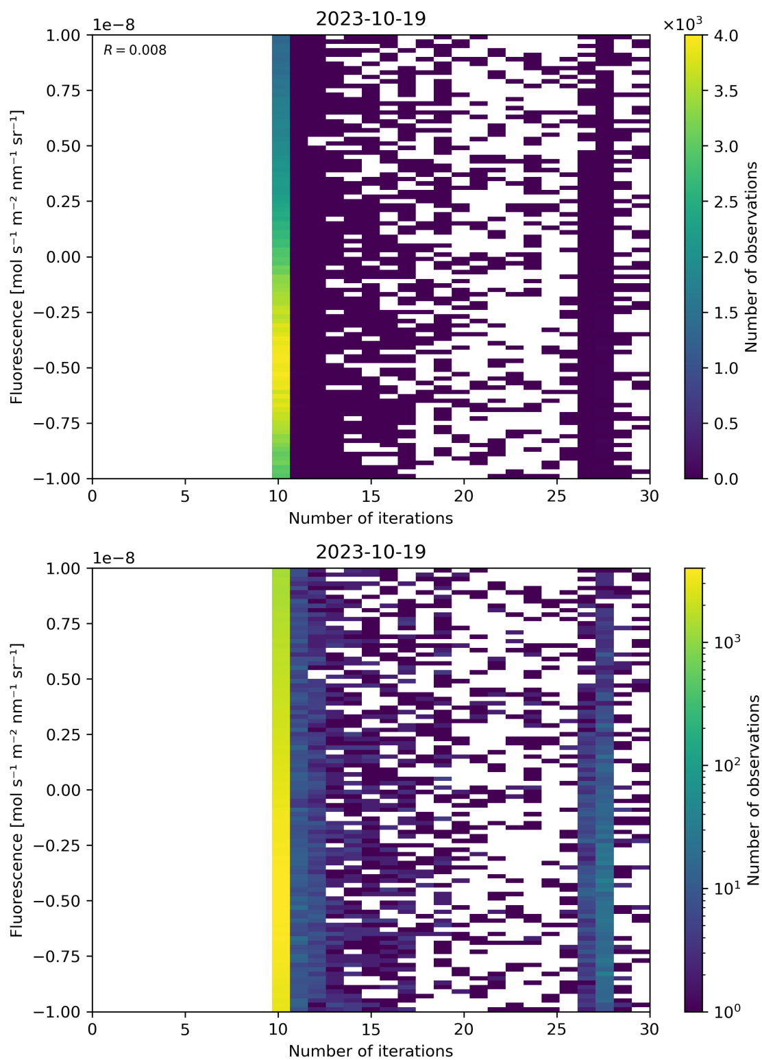
Figure 87: Scatter density plot of “Number of iterations” against “Fluorescence” for 2023-10-18 to 2023-10-20.
