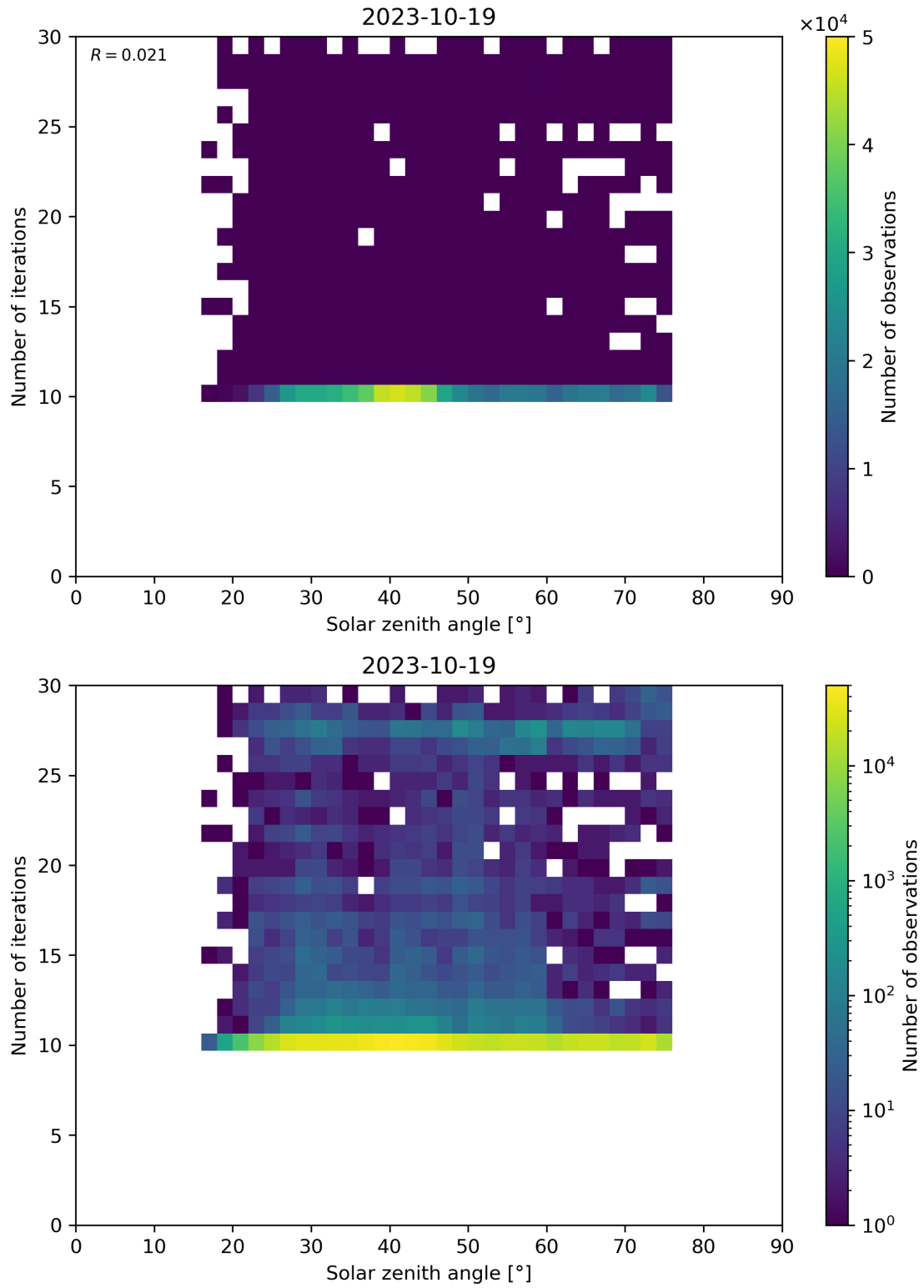
Figure 102: Scatter density plot of “Solar zenith angle” against “Number of iterations” for 2023-10-18 to 2023-10-20.
