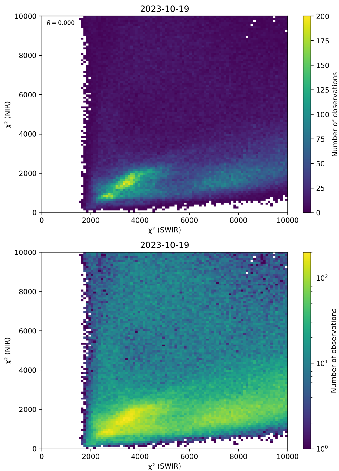
Figure 47: Scatter density plot of “ \chi^2 (SWIR)” against “ \chi^2 (NIR)” for 2023-10-18 to 2023-10-20.
