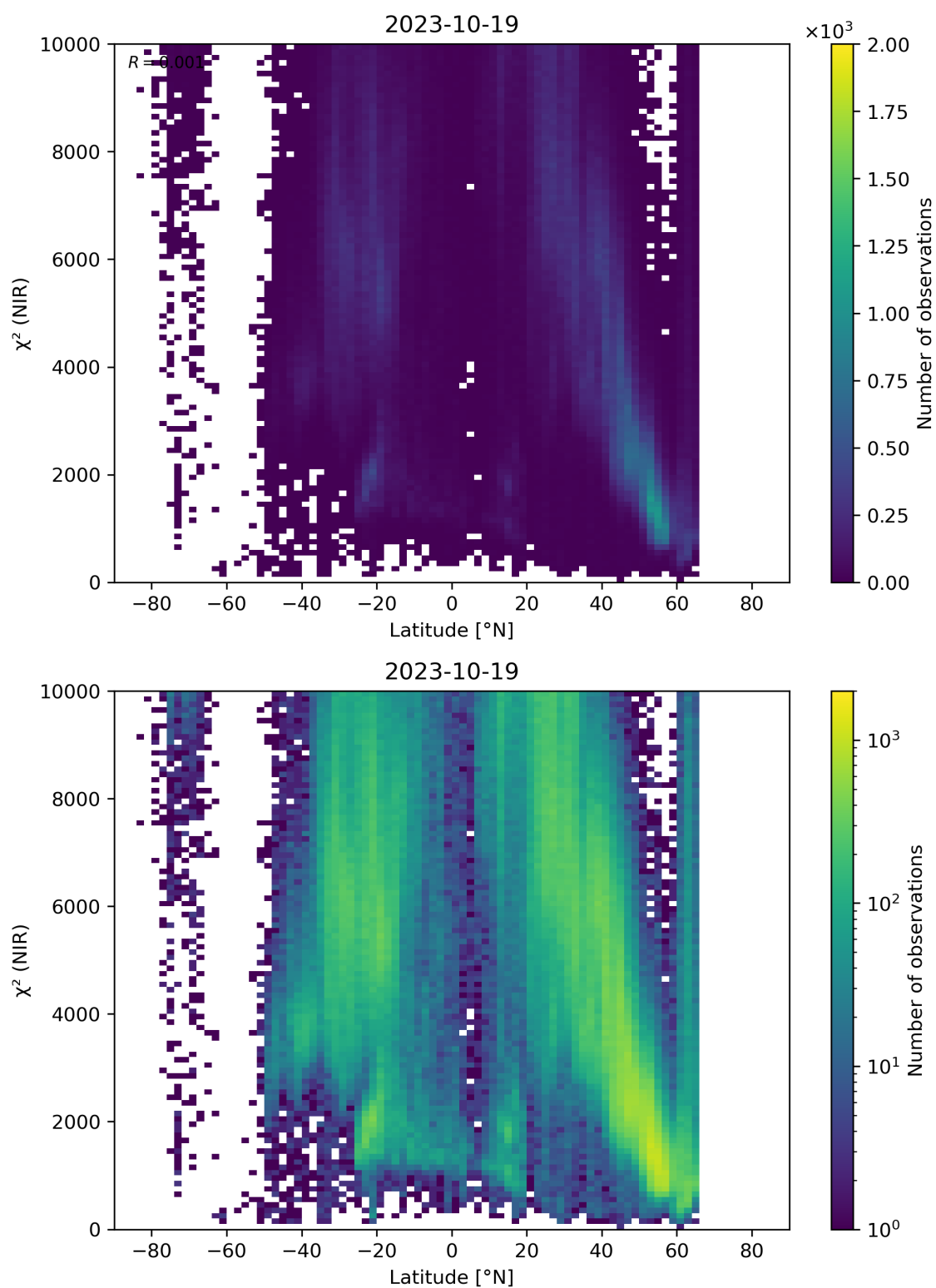
Figure 53: Scatter density plot of “Latitude” against “ \chi^2 (NIR)” for 2023-10-18 to 2023-10-20.
