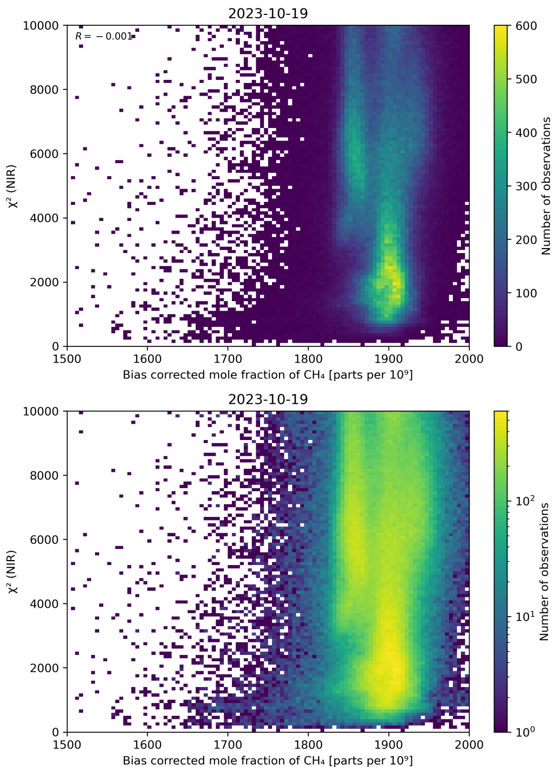
Figure 63: Scatter density plot of “Bias corrected mole fraction of CH 4 ” against “ \chi^2 (NIR)” for 2023-10-18 to 2023-10-20.
