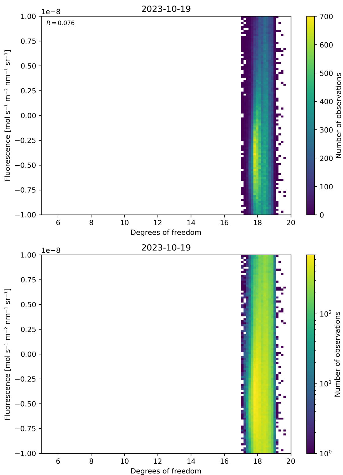
Figure 51: Scatter density plot of “Degrees of freedom” against “Fluorescence” for 2023-10-18 to 2023-10-20.
