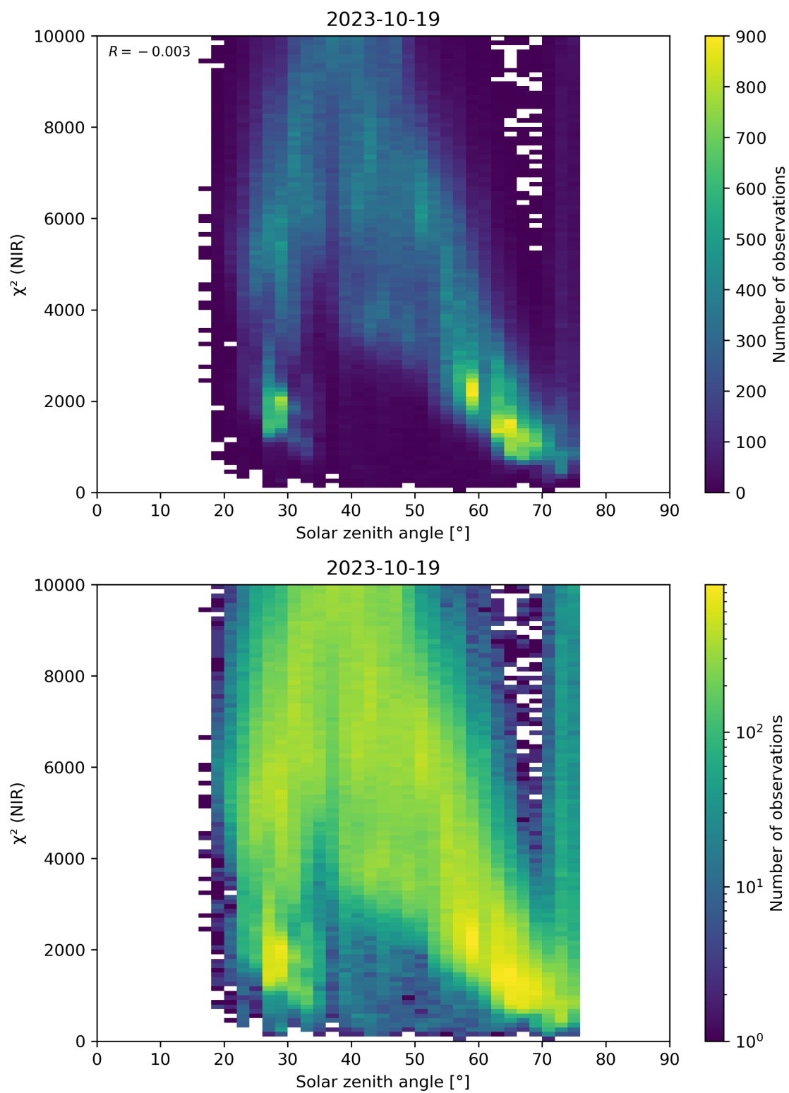
Figure 94: Scatter density plot of “Solar zenith angle” against “ \chi^2 (NIR)” for 2023-10-18 to 2023-10-20.
