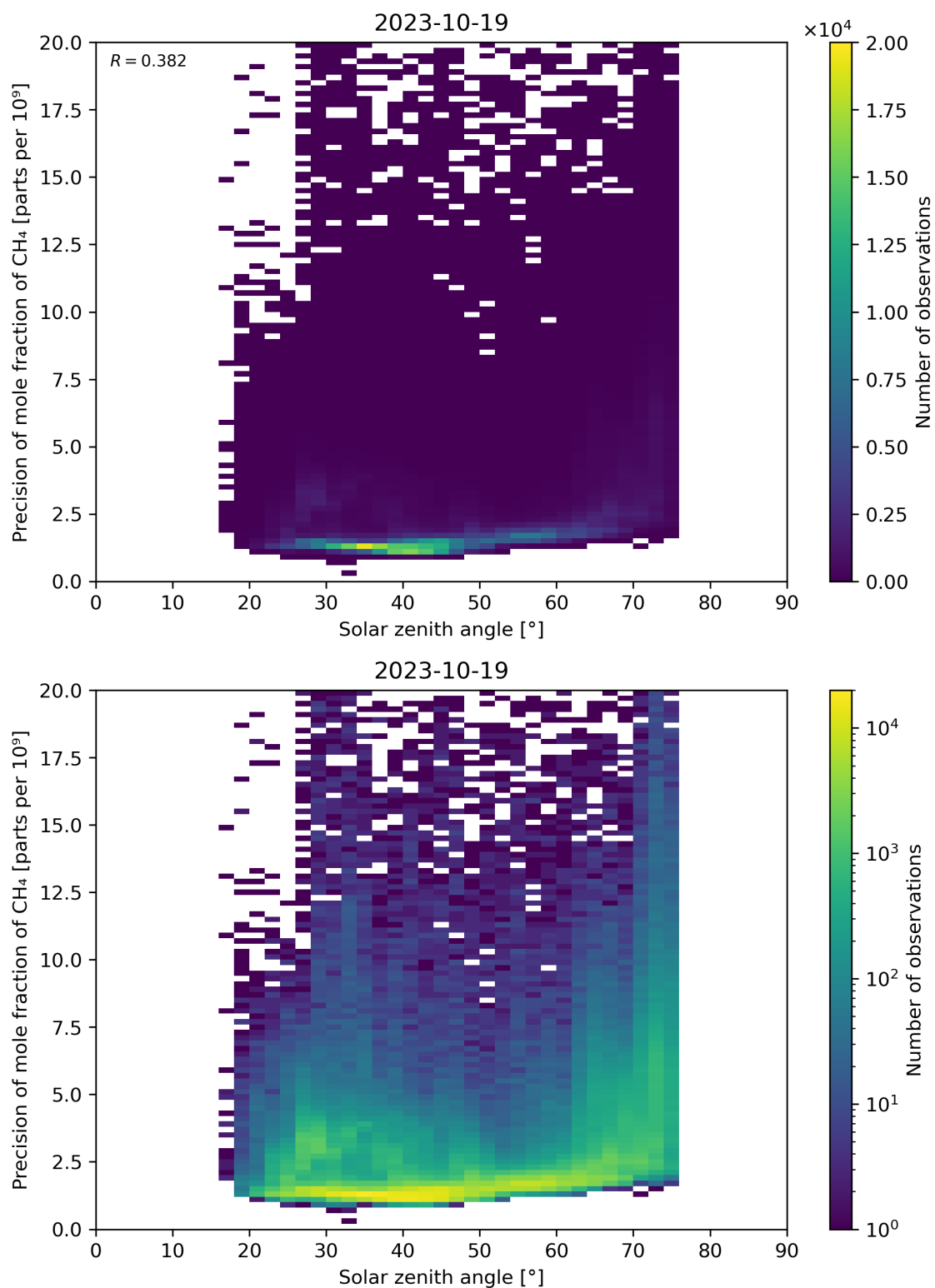
Figure 101: Scatter density plot of “Solar zenith angle” against “Precision of mole fraction of CH 4 ” for 2023-10-18 to 2023-10-20.
