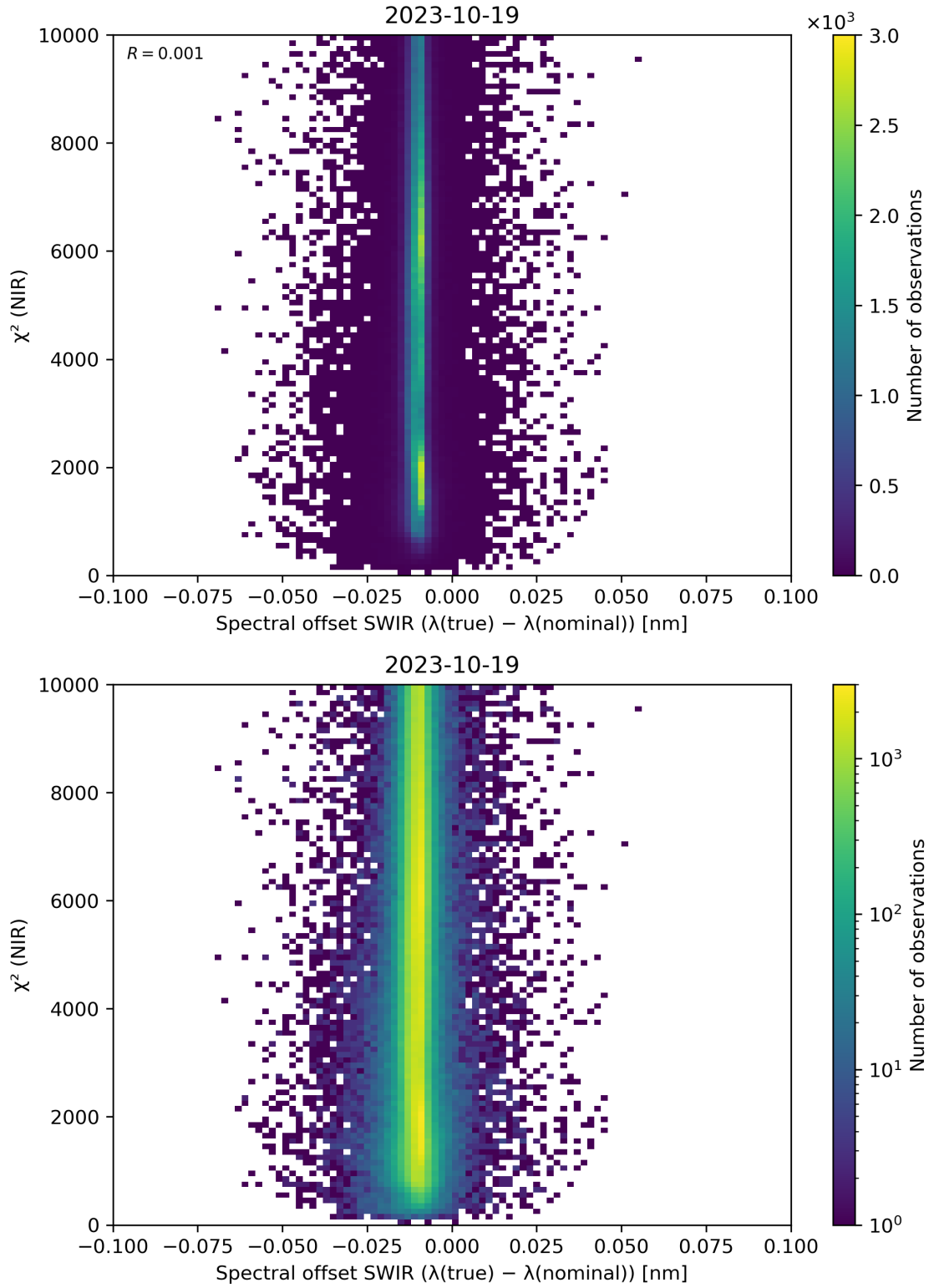
Figure 117: Scatter density plot of “Spectral offset SWIR ( \lambda(\text{true}) - \lambda(\text{nominal}) )” against “ \chi^2 (NIR)” for 2023-10-18 to 2023-10-20.
