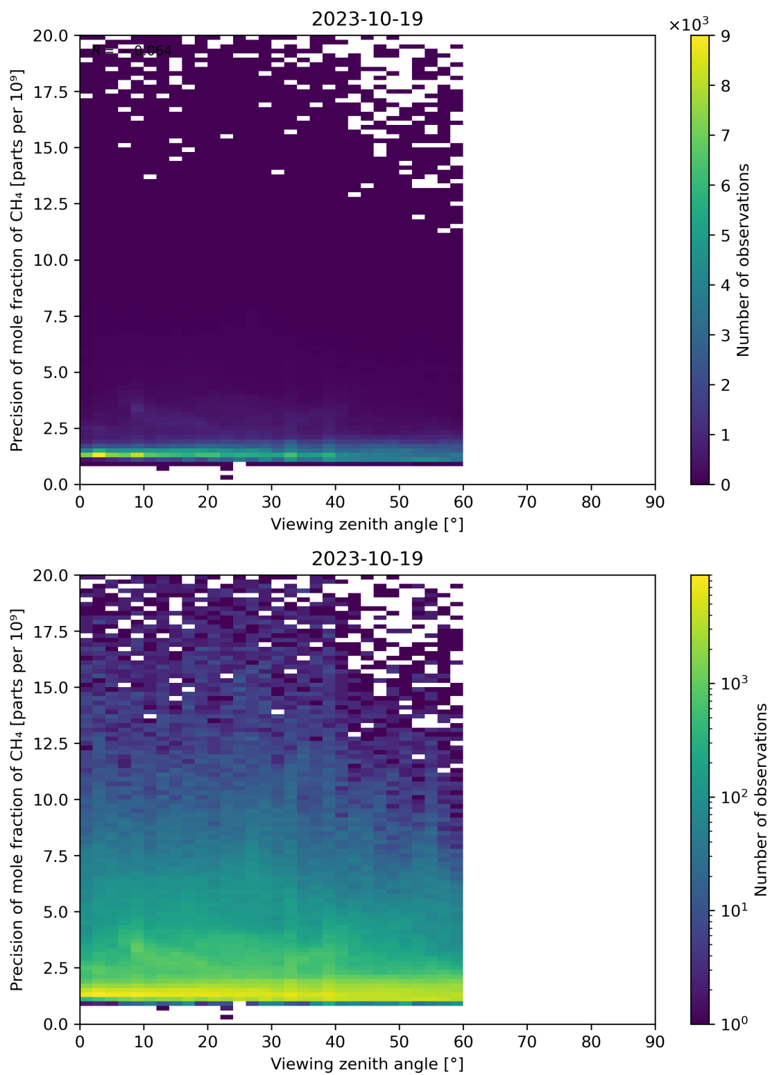
Figure 112: Scatter density plot of “Viewing zenith angle” against “Precision of mole fraction of CH 4 ” for 2023-10-18 to 2023-10-20.
