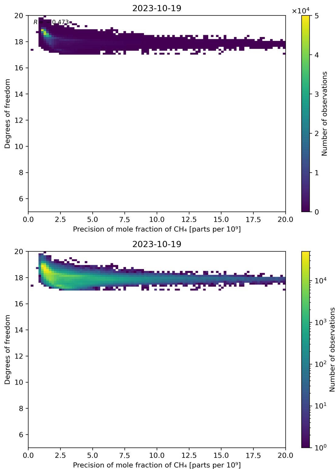
Figure 80: Scatter density plot of “Precision of mole fraction of CH 4 ” against “Degrees of freedom” for 2023-10-18 to 2023-10-20.
