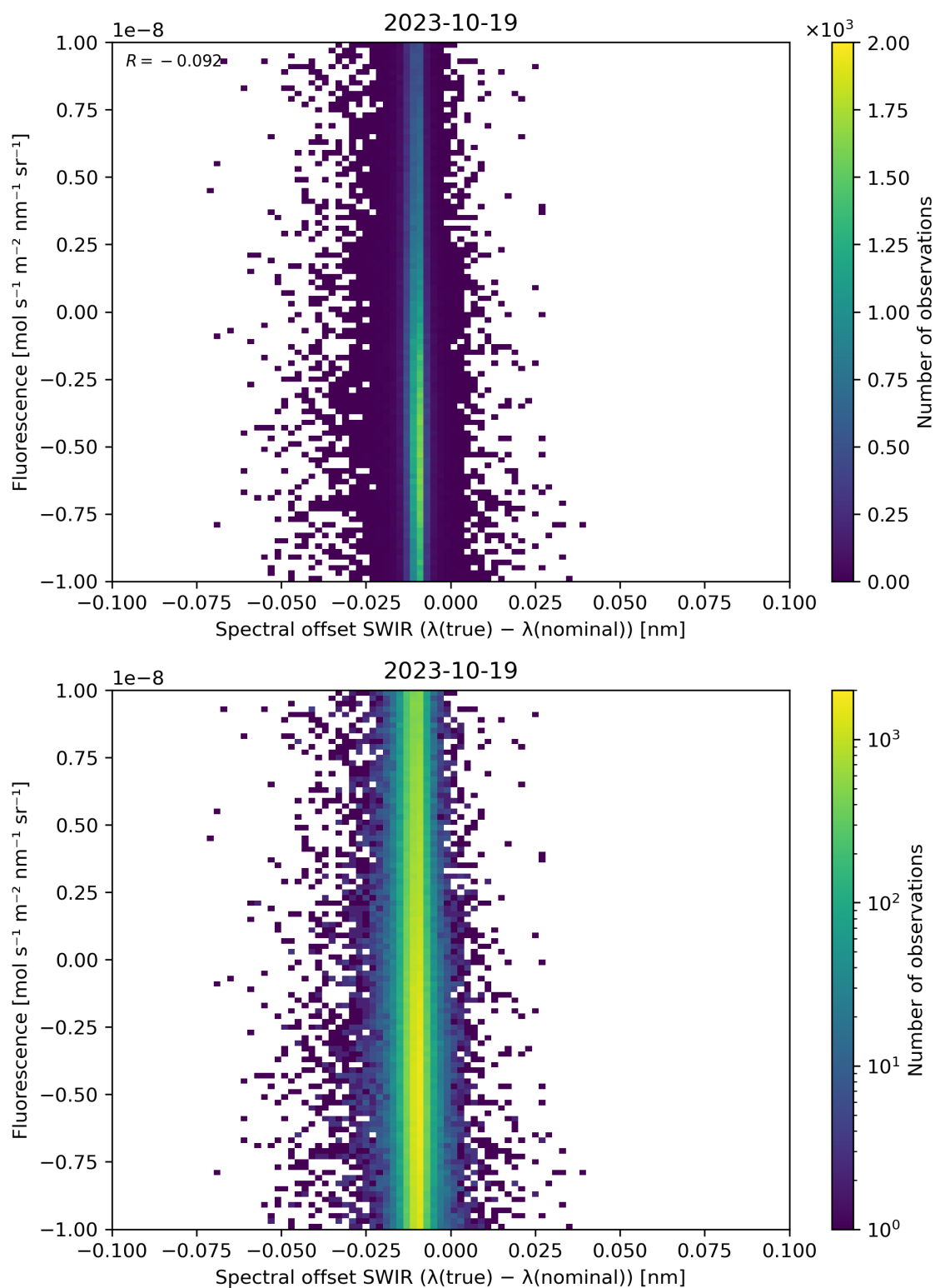
Figure 120: Scatter density plot of “Spectral offset SWIR ( \lambda(\text{true}) - \lambda(\text{nominal}) )” against “Fluorescence” for 2023-10-18 to 2023-10-20.
