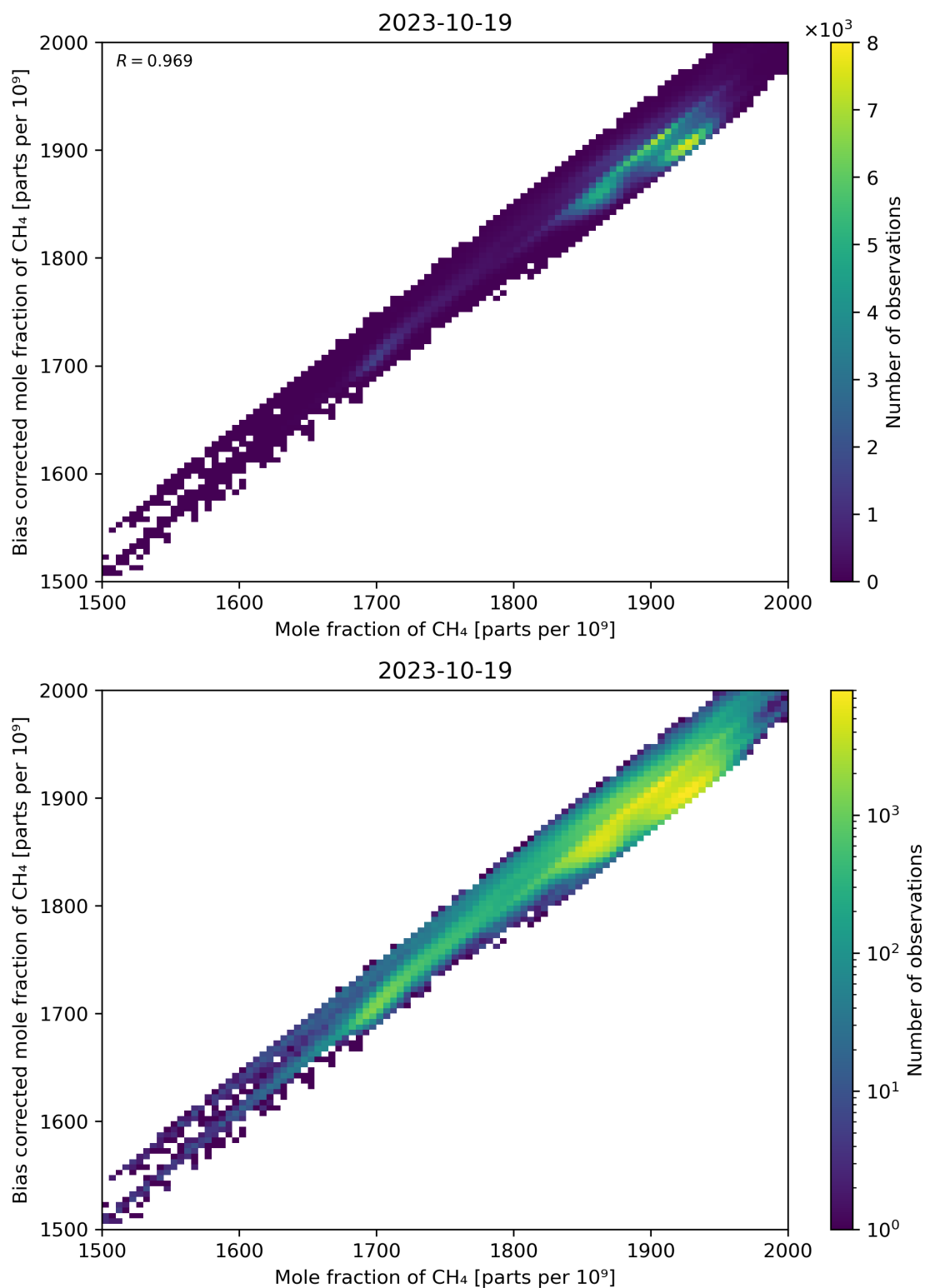
Figure 74: Scatter density plot of “Mole fraction of CH 4 ” against “Bias corrected mole fraction of CH 4 ” for 2023-10-18 to 2023-10-20.
