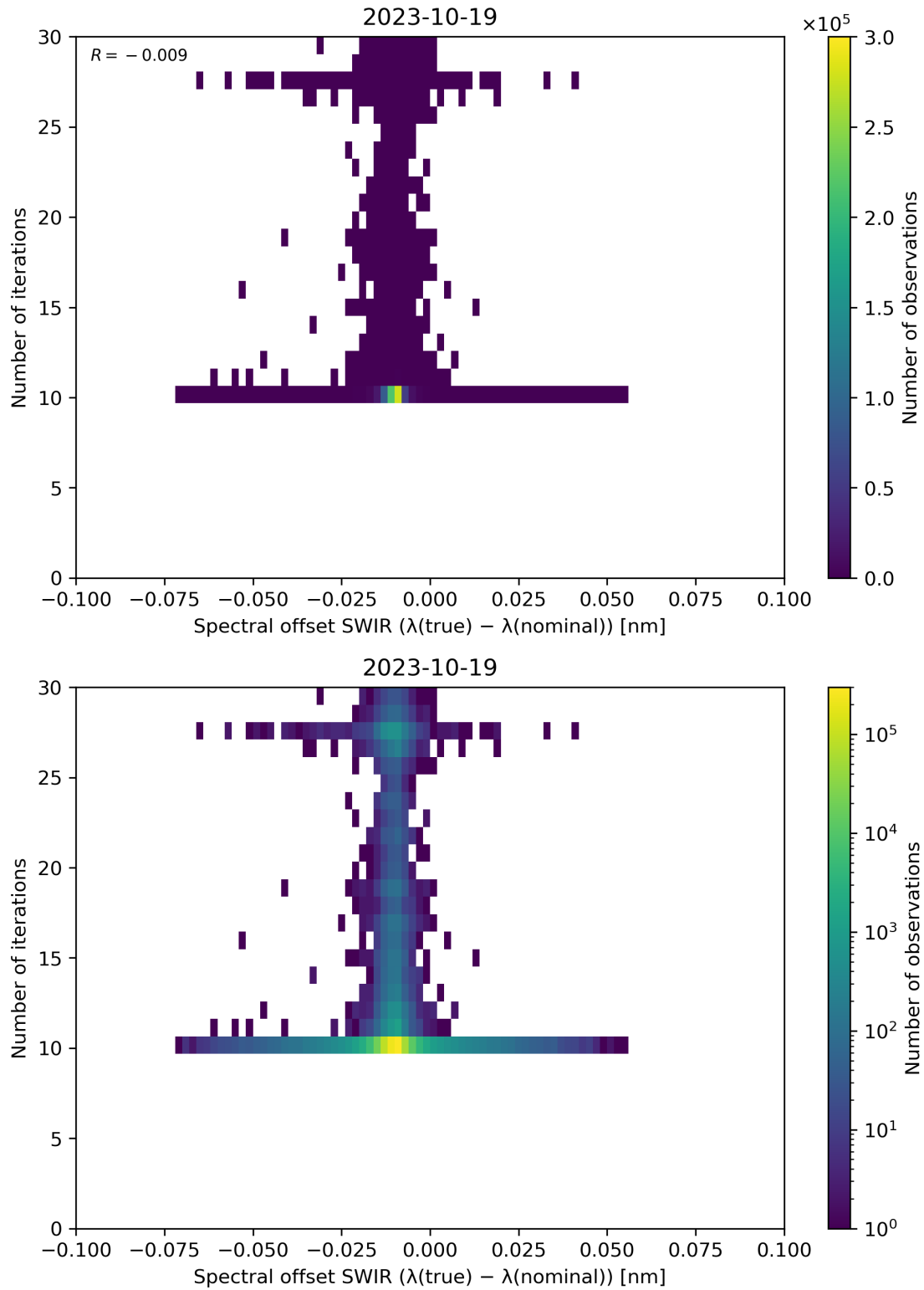
Figure 121: Scatter density plot of “Spectral offset SWIR ( \lambda(\text{true}) - \lambda(\text{nominal}) )” against “Number of iterations” for 2023-10-18 to 2023-10-20.
