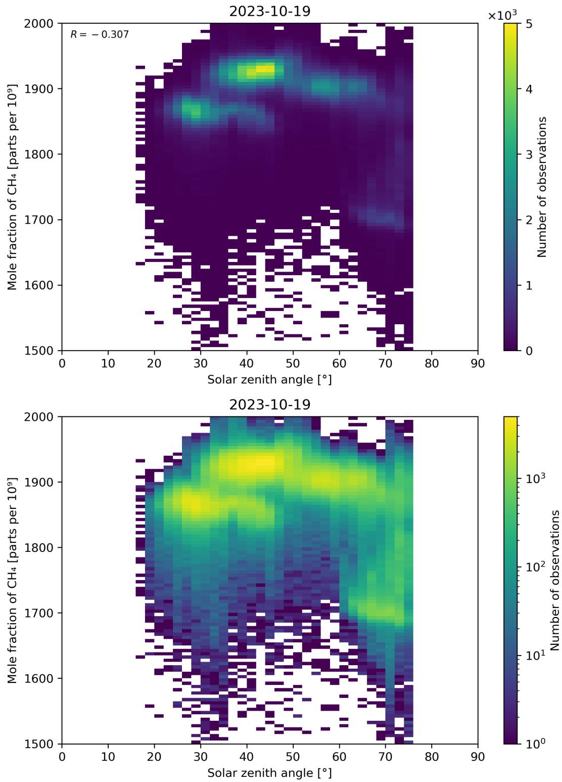
Figure 99: Scatter density plot of “Solar zenith angle” against “Mole fraction of CH 4 ” for 2023-10-18 to 2023-10-20.
