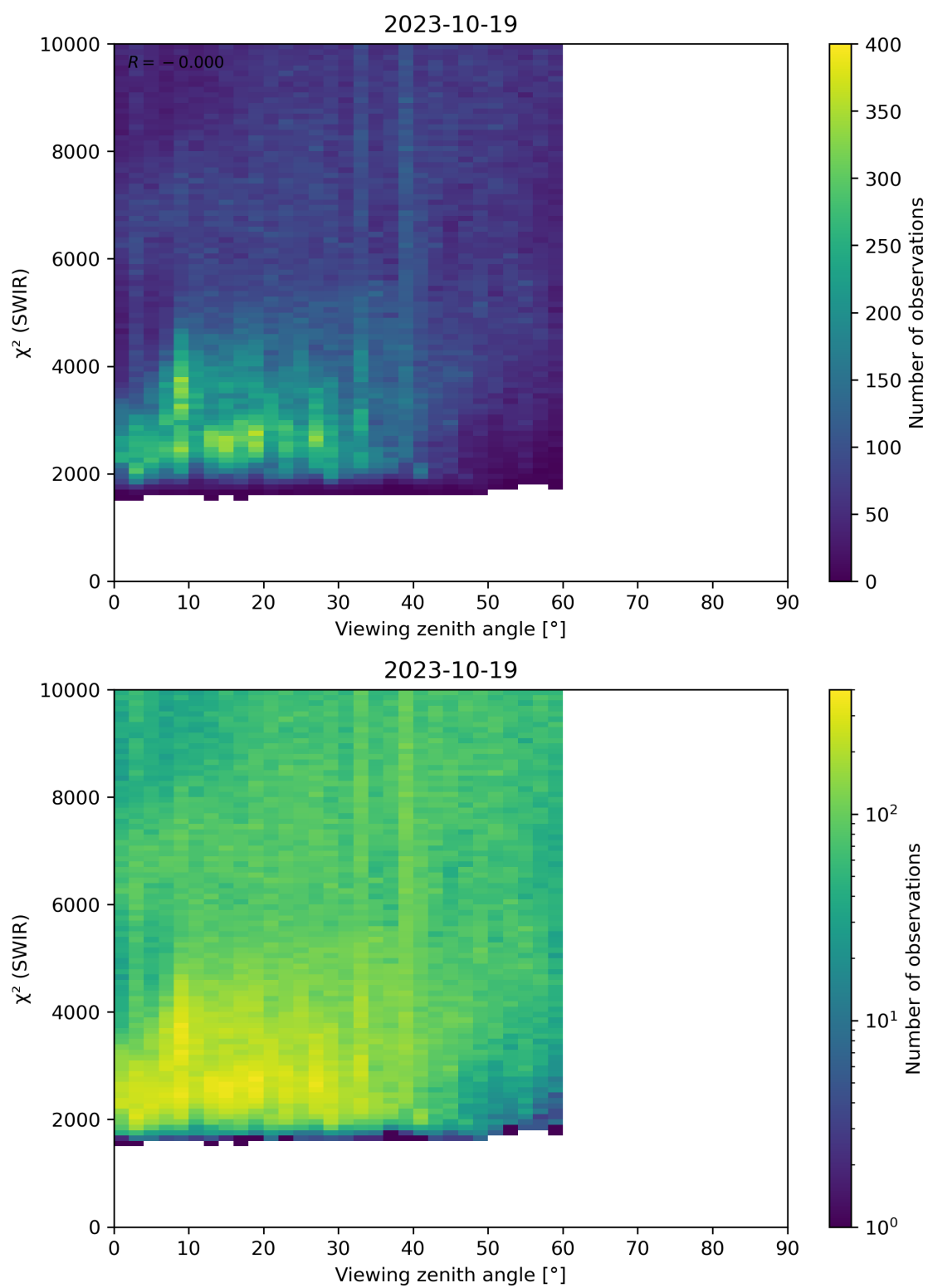
Figure 106: Scatter density plot of “Viewing zenith angle” against “ \chi^2 (SWIR)” for 2023-10-18 to 2023-10-20.
