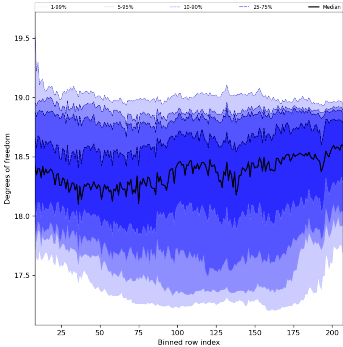
Figure 41: Along track statistics of “Degrees of freedom” for 2023-10-18 to 2023-10-20
