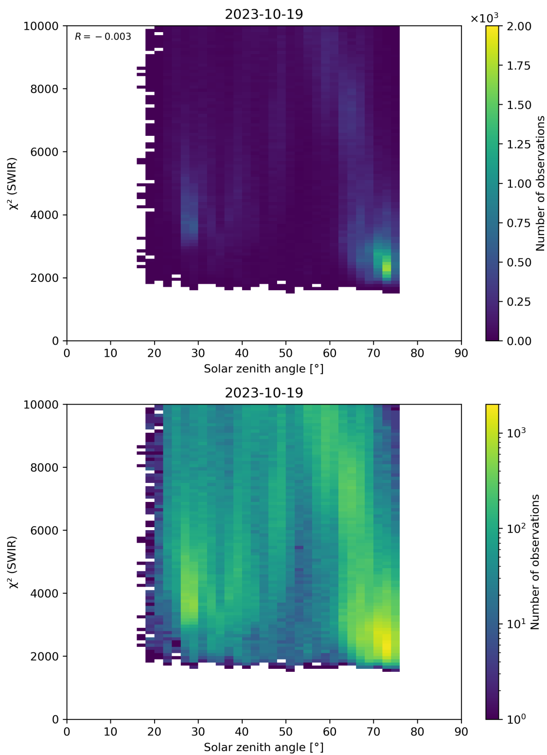
Figure 95: Scatter density plot of “Solar zenith angle” against “ \chi^2 (SWIR)” for 2023-10-18 to 2023-10-20.
