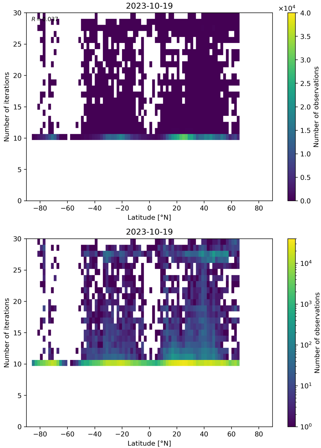
Figure 60: Scatter density plot of “Latitude” against “Number of iterations” for 2023-10-18 to 2023-10-20.
