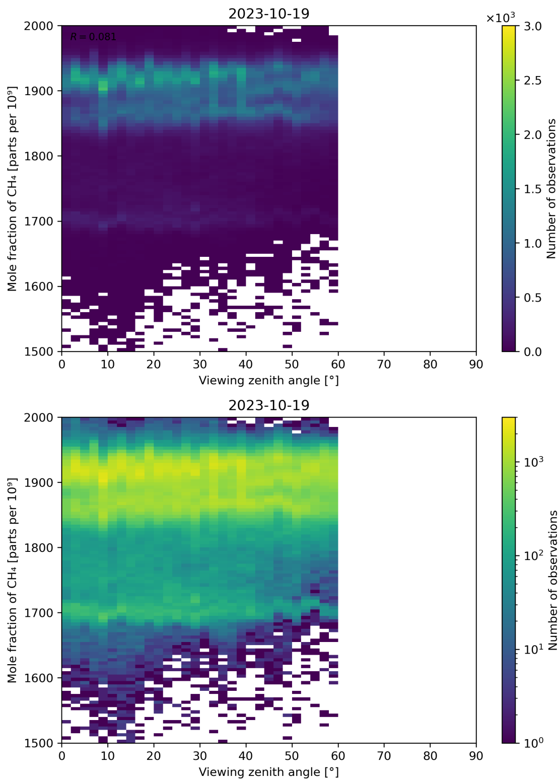
Figure 110: Scatter density plot of “Viewing zenith angle” against “Mole fraction of CH 4 ” for 2023-10-18 to 2023-10-20.
