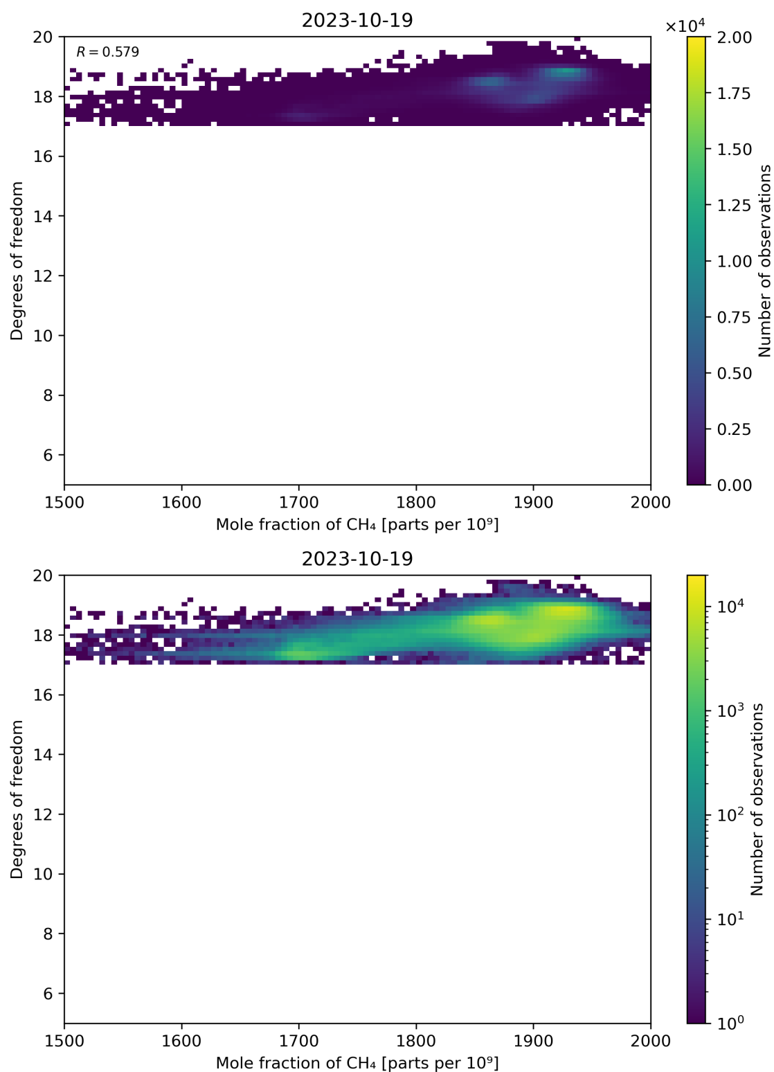
Figure 72: Scatter density plot of “Mole fraction of CH 4 ” against “Degrees of freedom” for 2023-10-18 to 2023-10-20.
