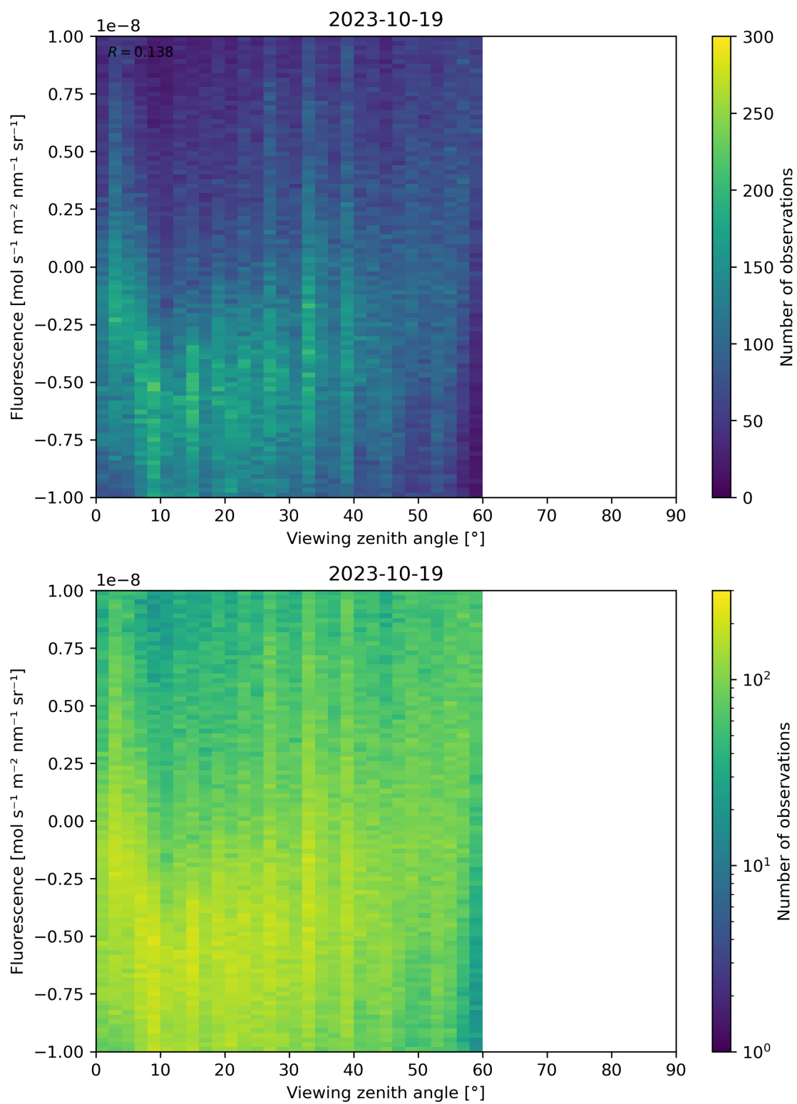
Figure 108: Scatter density plot of “Viewing zenith angle” against “Fluorescence” for 2023-10-18 to 2023-10-20.
