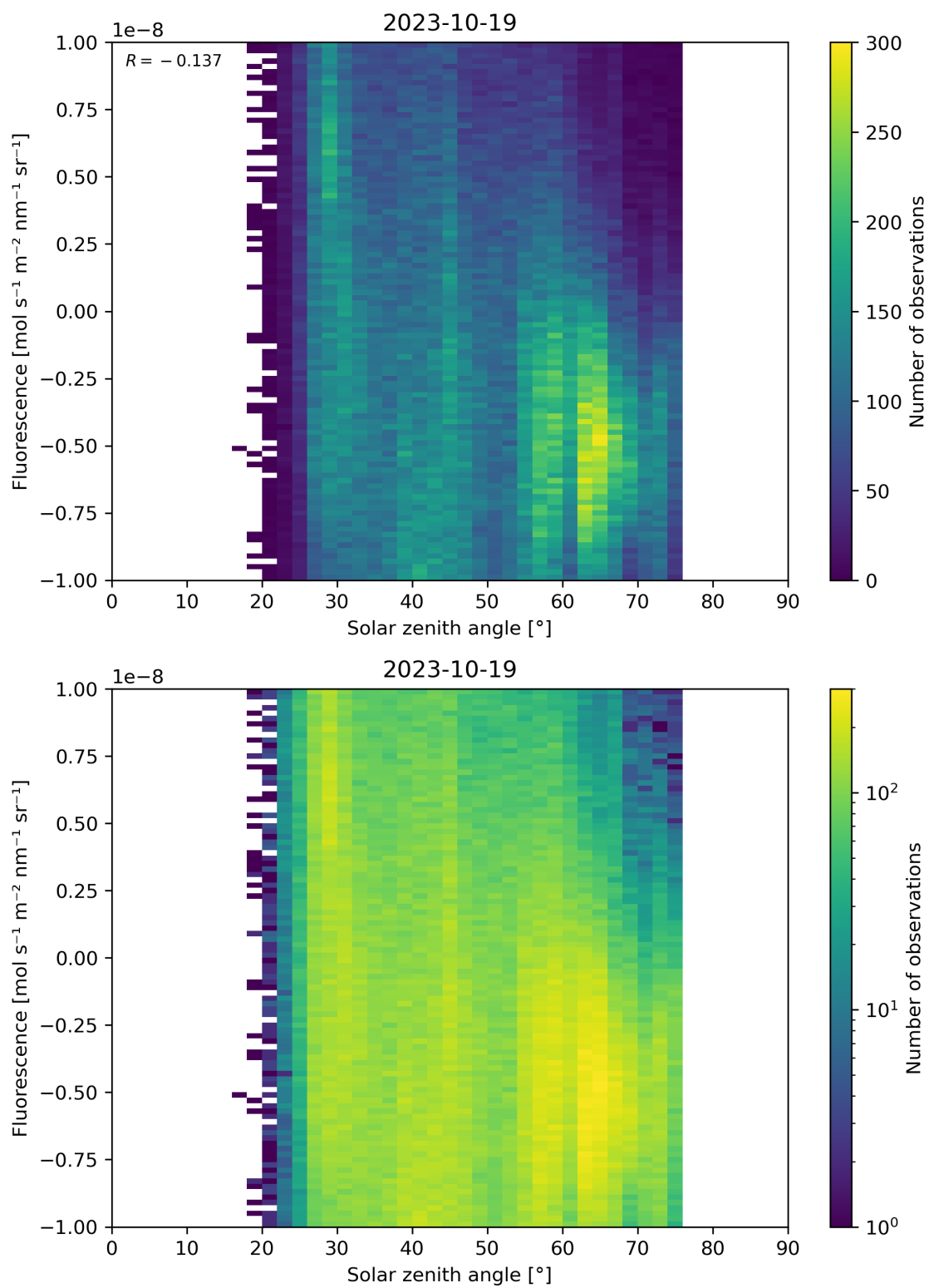
Figure 97: Scatter density plot of “Solar zenith angle” against “Fluorescence” for 2023-10-18 to 2023-10-20.
