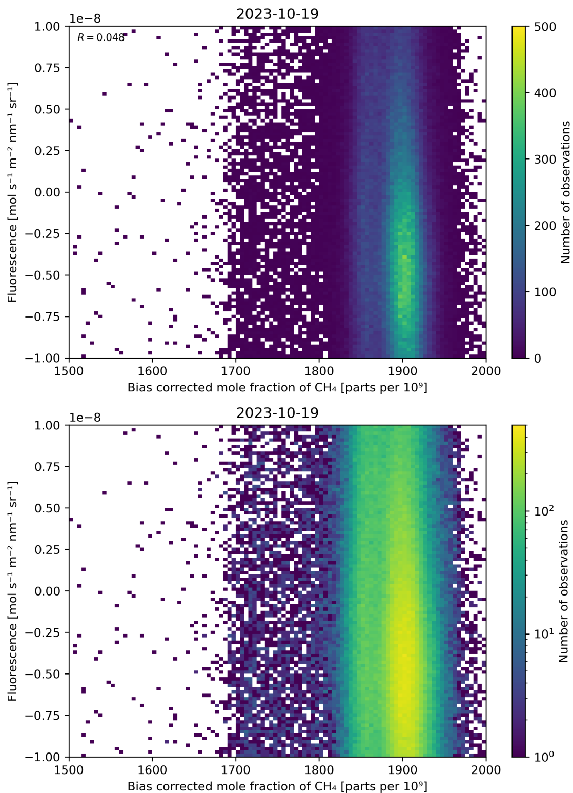
Figure 66: Scatter density plot of “Bias corrected mole fraction of \text{CH}_4 ” against “Fluorescence” for 2023-10-18 to 2023-10-20.
