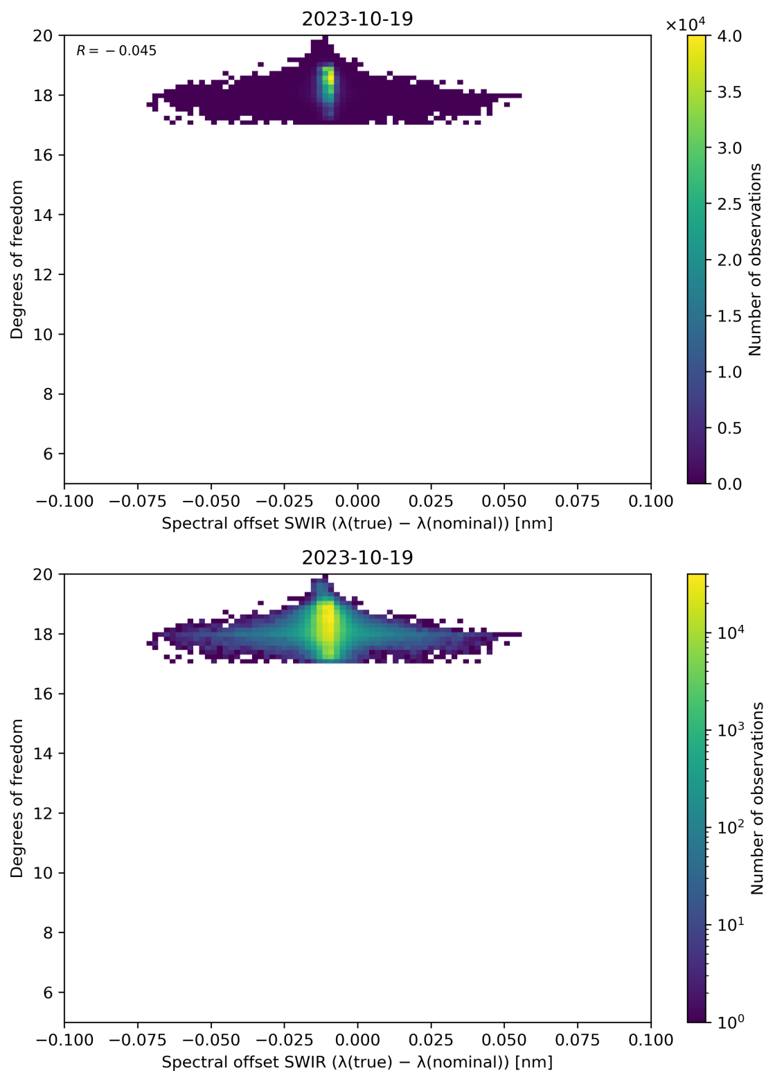
Figure 119: Scatter density plot of “Spectral offset SWIR ( \lambda(\text{true}) - \lambda(\text{nominal}) )” against “Degrees of freedom” for 2023-10-18 to 2023-10-20.
