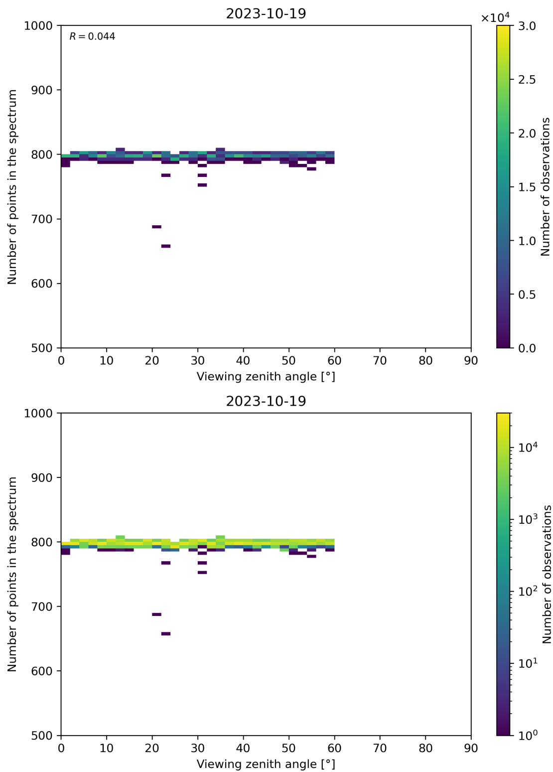
Figure 114: Scatter density plot of “Viewing zenith angle” against “Number of points in the spectrum” for 2023-10-18 to 2023-10-20.
