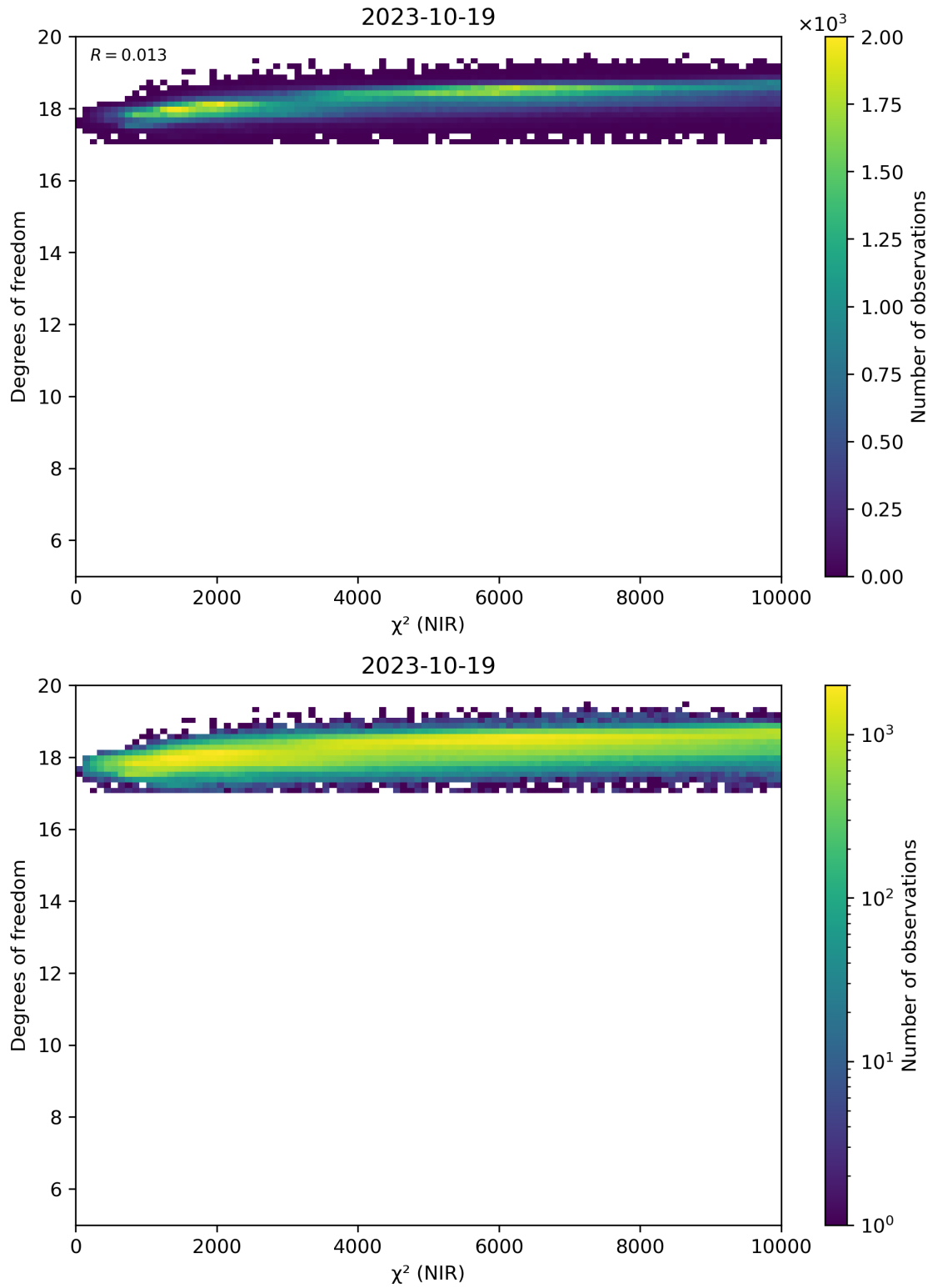
Figure 44: Scatter density plot of “ \chi^2 (NIR)” against “Degrees of freedom” for 2023-10-18 to 2023-10-20.
