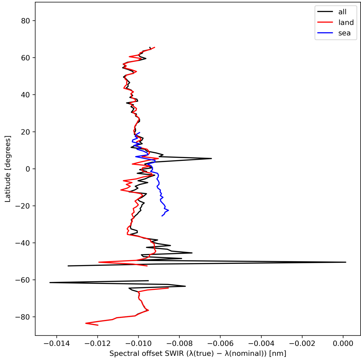
Figure 16: Zonal average of “Spectral offset SWIR ( \lambda(\text{true}) - \lambda(\text{nominal}) )” for 2023-10-18 to 2023-10-20.
