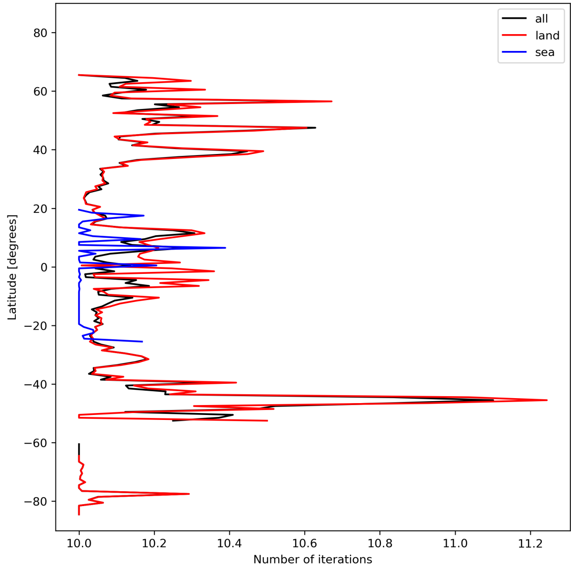
Figure 20: Zonal average of “Number of iterations” for 2023-10-18 to 2023-10-20.
