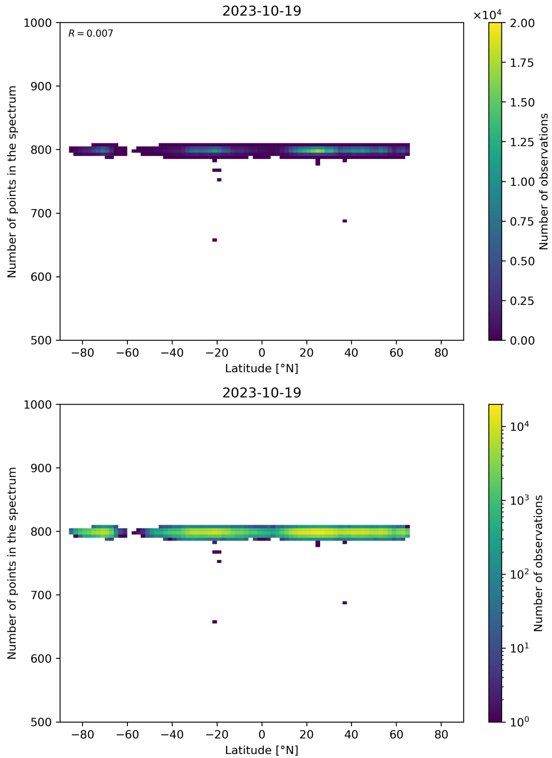
Figure 61: Scatter density plot of “Latitude” against “Number of points in the spectrum” for 2023-10-18 to 2023-10-20.
