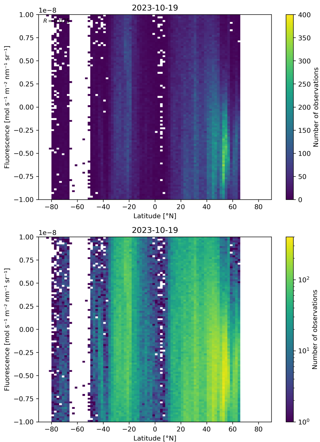
Figure 56: Scatter density plot of “Latitude” against “Fluorescence” for 2023-10-18 to 2023-10-20.
