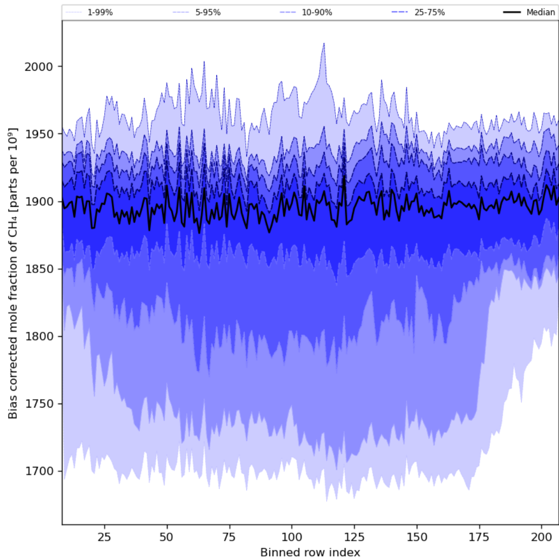
Figure 36: Along track statistics of “Bias corrected mole fraction of CH 4 ” for 2023-10-18 to 2023-10-20
