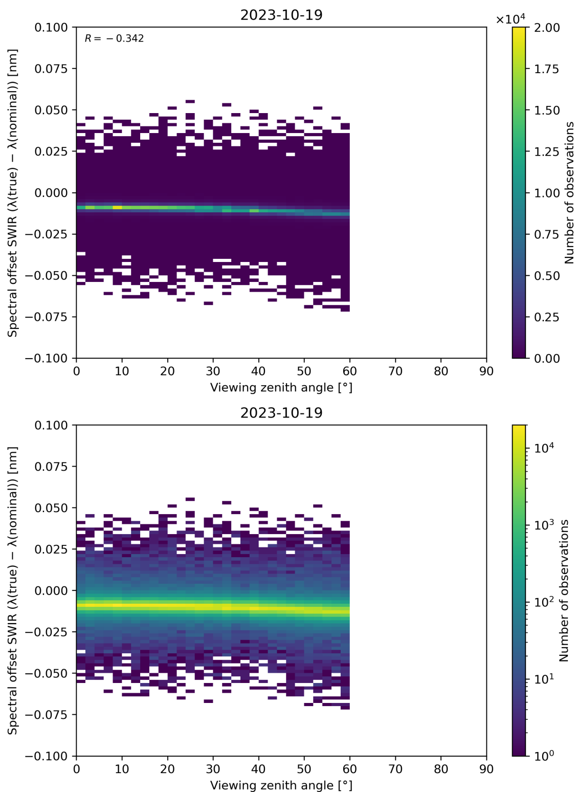
Figure 116: Scatter density plot of “Viewing zenith angle” against “Spectral offset SWIR ( \lambda(\text{true}) - \lambda(\text{nominal}) )” for 2023-10-18 to 2023-10-20.
