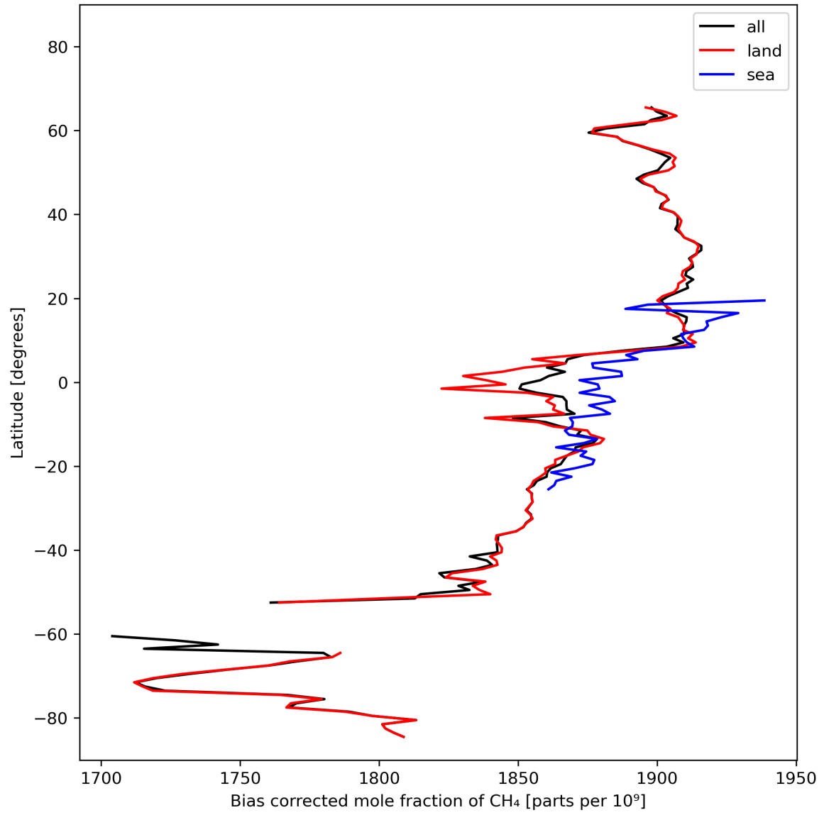
Figure 14: Zonal average of “Bias corrected mole fraction of CH 4 ” for 2023-10-18 to 2023-10-20.
