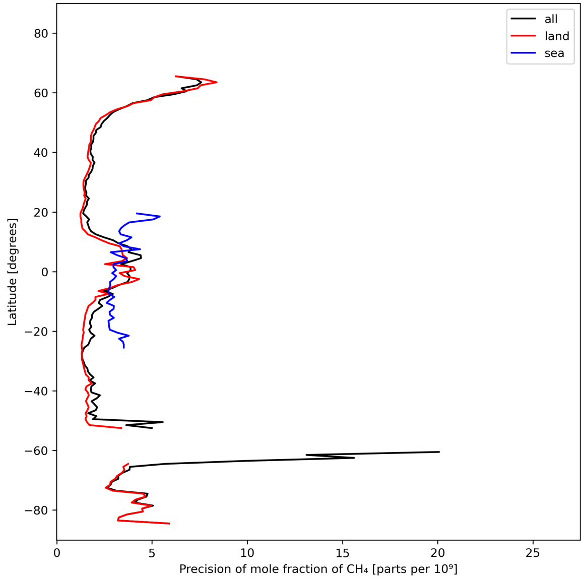
Figure 13: Zonal average of “Precision of mole fraction of CH 4 ” for 2023-10-18 to 2023-10-20.
