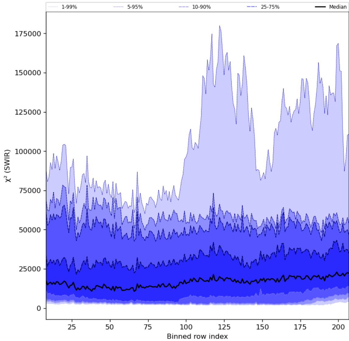
Figure 39: Along track statistics of “ \chi^2 (SWIR)” for 2023-10-18 to 2023-10-20
