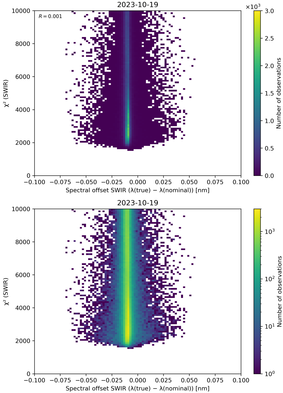
Figure 118: Scatter density plot of “Spectral offset SWIR ( \lambda(\text{true}) - \lambda(\text{nominal}) )” against “ \chi^2 (SWIR)” for 2023-10-18 to 2023-10-20.
