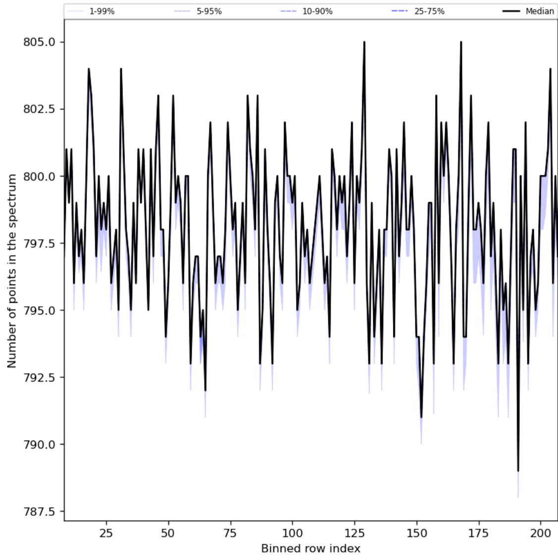
Figure 37: Along track statistics of “Number of points in the spectrum” for 2023-10-18 to 2023-10-20
