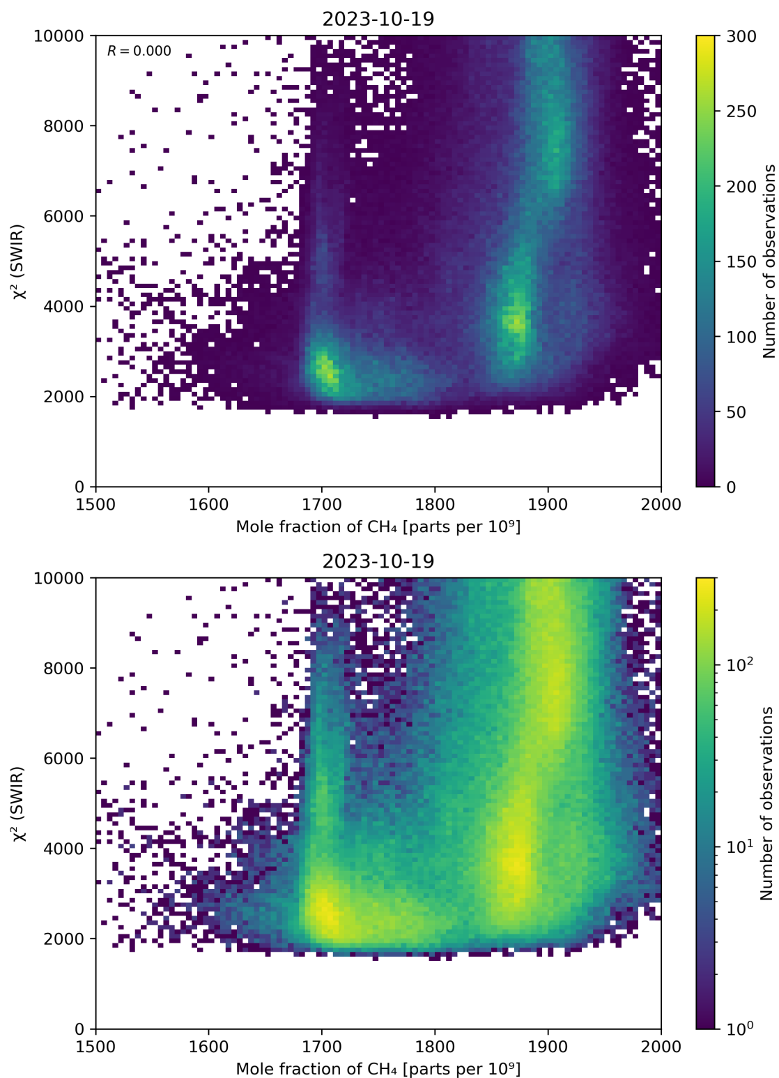
Figure 71: Scatter density plot of “Mole fraction of \text{CH}_4 ” against “ \chi^2 (SWIR)” for 2023-10-18 to 2023-10-20.
