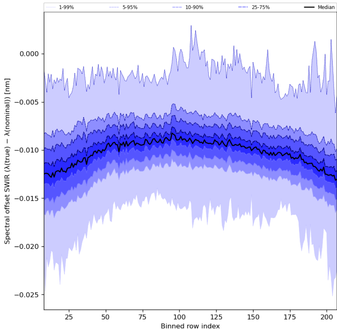
Figure 38: Along track statistics of “Spectral offset SWIR ( \lambda(\text{true}) - \lambda(\text{nominal}) )” for 2023-10-18 to 2023-10-20
