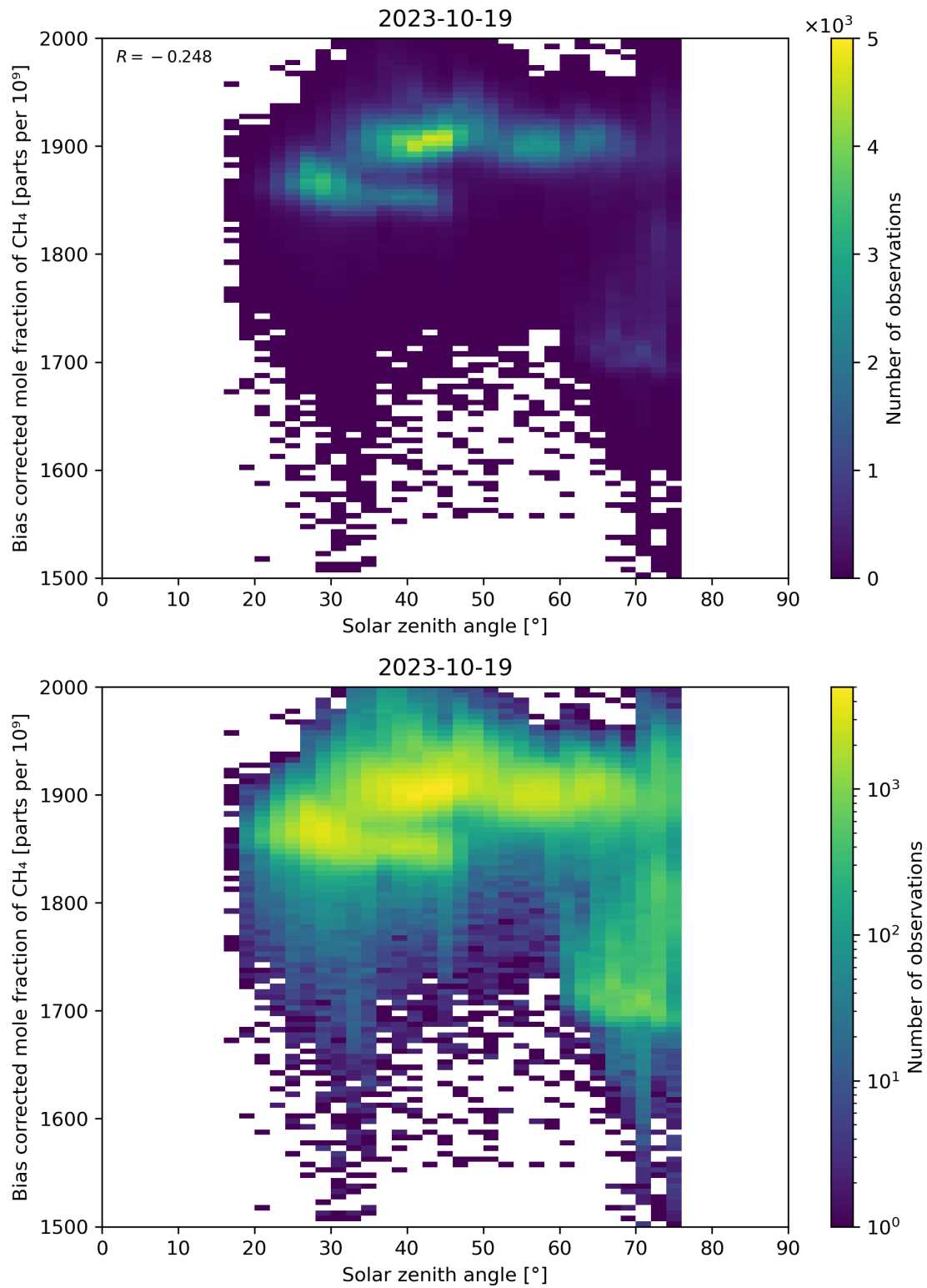
Figure 100: Scatter density plot of “Solar zenith angle” against “Bias corrected mole fraction of CH 4 ” for 2023-10-18 to 2023-10-20.
