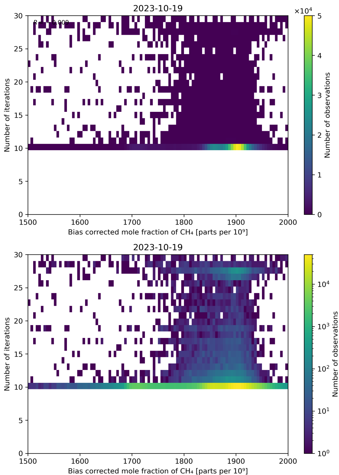
Figure 67: Scatter density plot of “Bias corrected mole fraction of CH 4 ” against “Number of iterations” for 2023-10-18 to 2023-10-20.
