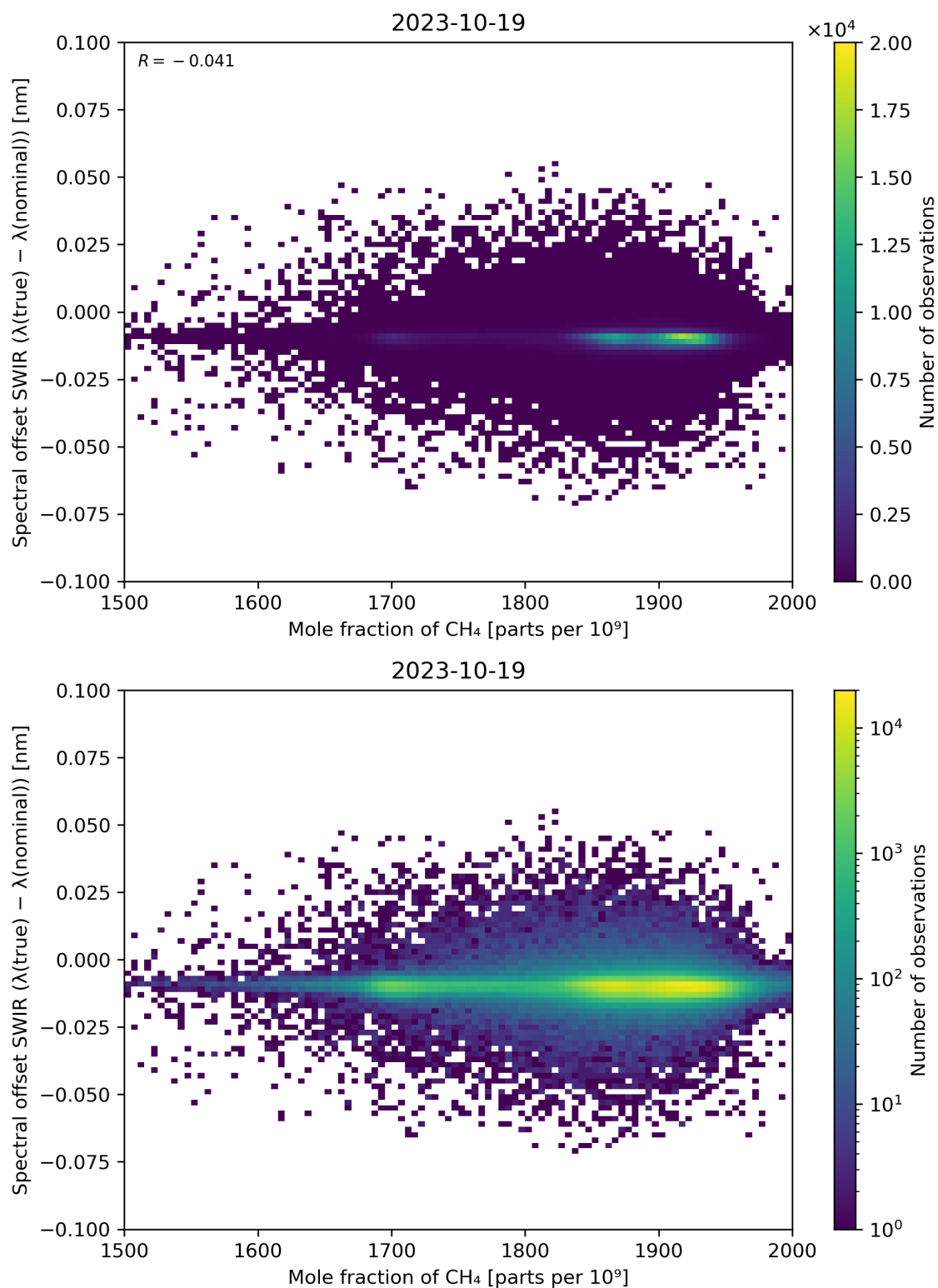
Figure 86: Scatter density plot of “Mole fraction of CH 4 ” against “Spectral offset SWIR ( \lambda(\text{true}) - \lambda(\text{nominal}) )” for 2023-10-18 to 2023-10-20.
