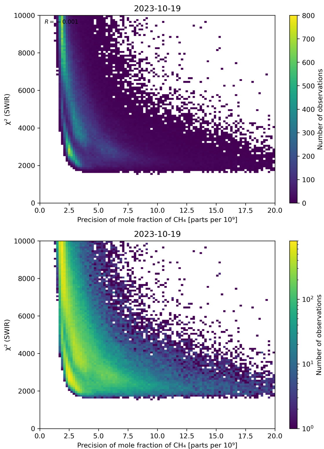
Figure 79: Scatter density plot of “Precision of mole fraction of \text{CH}_4 ” against “ \chi^2 (SWIR)” for 2023-10-18 to 2023-10-20.
