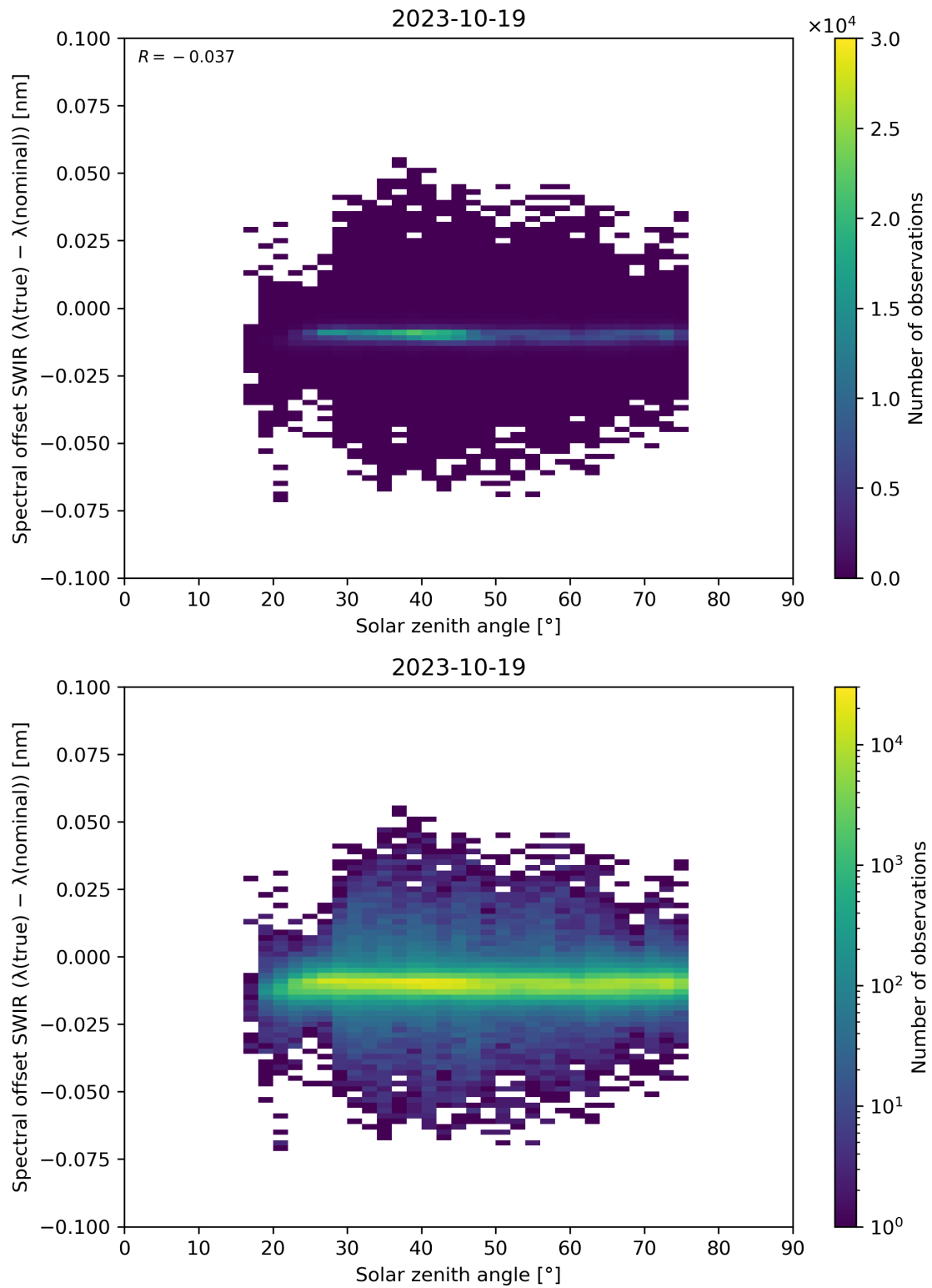
Figure 104: Scatter density plot of “Solar zenith angle” against “Spectral offset SWIR ( \lambda(\text{true}) - \lambda(\text{nominal}) )” for 2023-10-18 to 2023-10-20.
