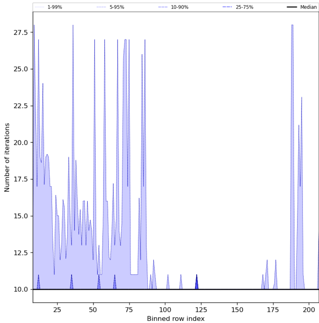
Figure 42: Along track statistics of “Number of iterations” for 2023-10-18 to 2023-10-20
