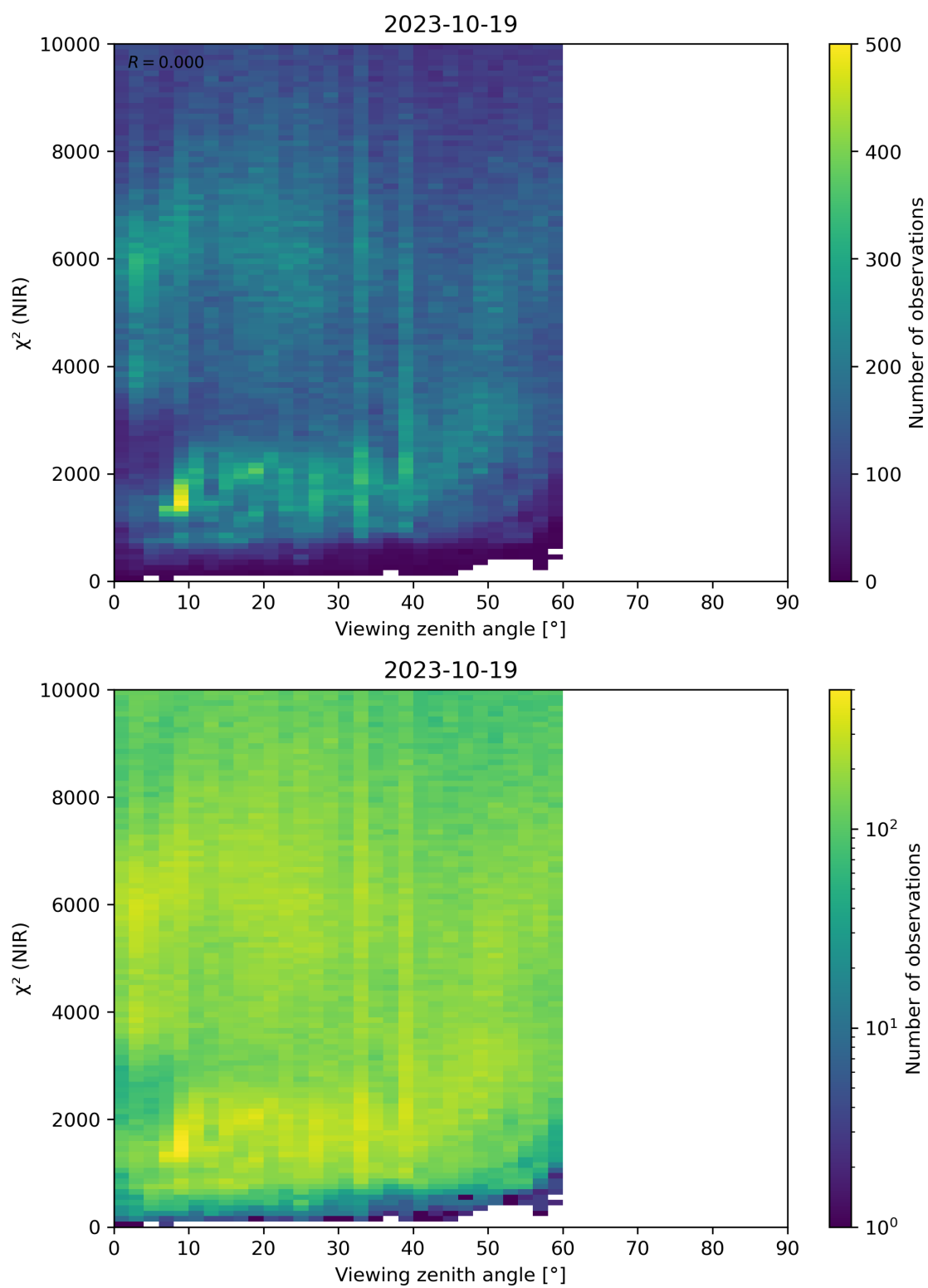
Figure 105: Scatter density plot of “Viewing zenith angle” against “ \chi^2 (NIR)” for 2023-10-18 to 2023-10-20.
