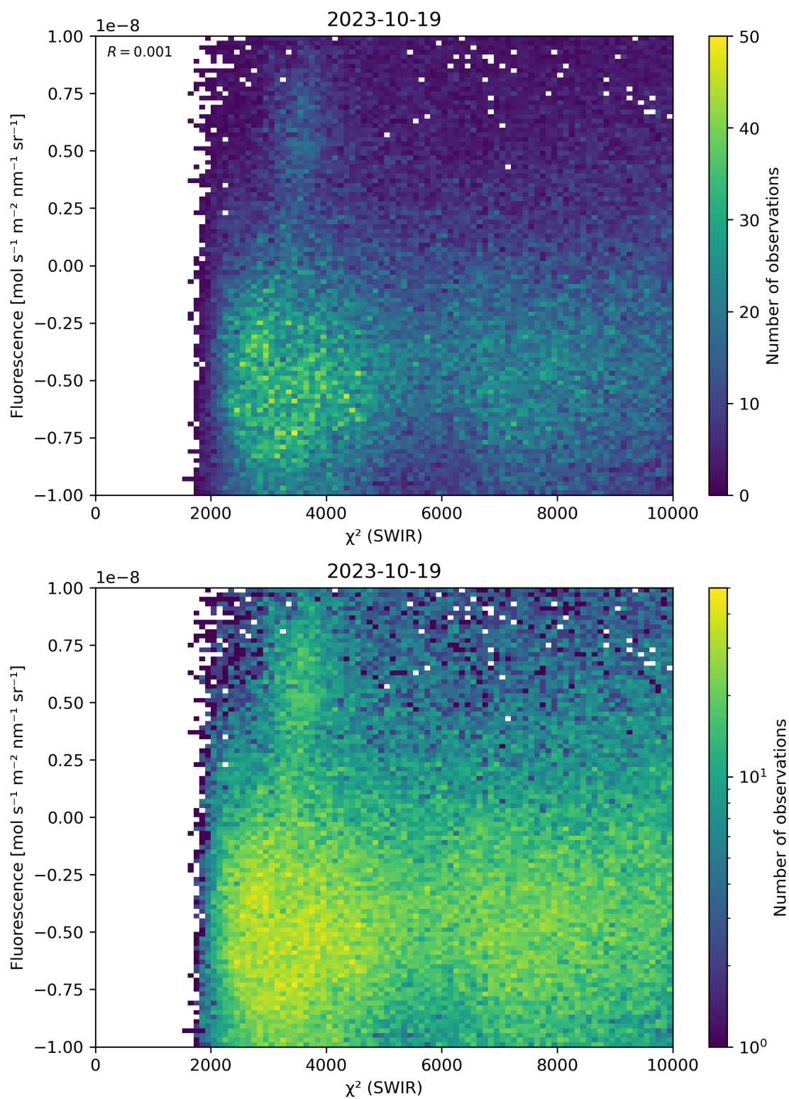
Figure 49: Scatter density plot of “ \chi^2 (SWIR)” against “Fluorescence” for 2023-10-18 to 2023-10-20.
