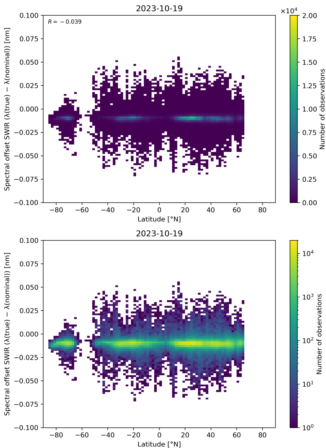
Figure 62: Scatter density plot of “Latitude” against “Spectral offset SWIR ( \lambda(\text{true}) - \lambda(\text{nominal}) )” for 2023-10-18 to 2023-10-20.
