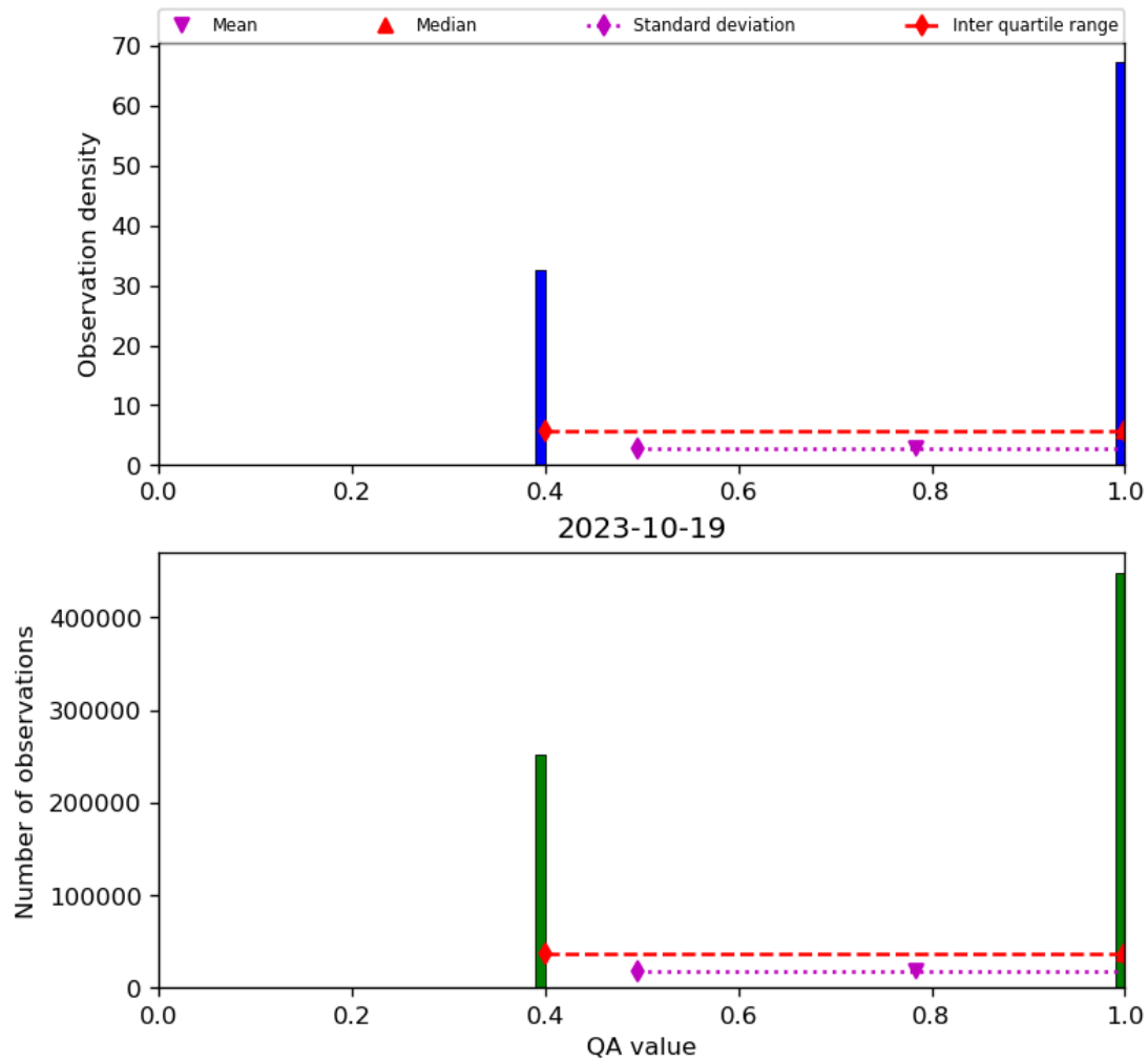
Figure 22: Histogram of “QA value” for 2023-10-18 to 2023-10-20
