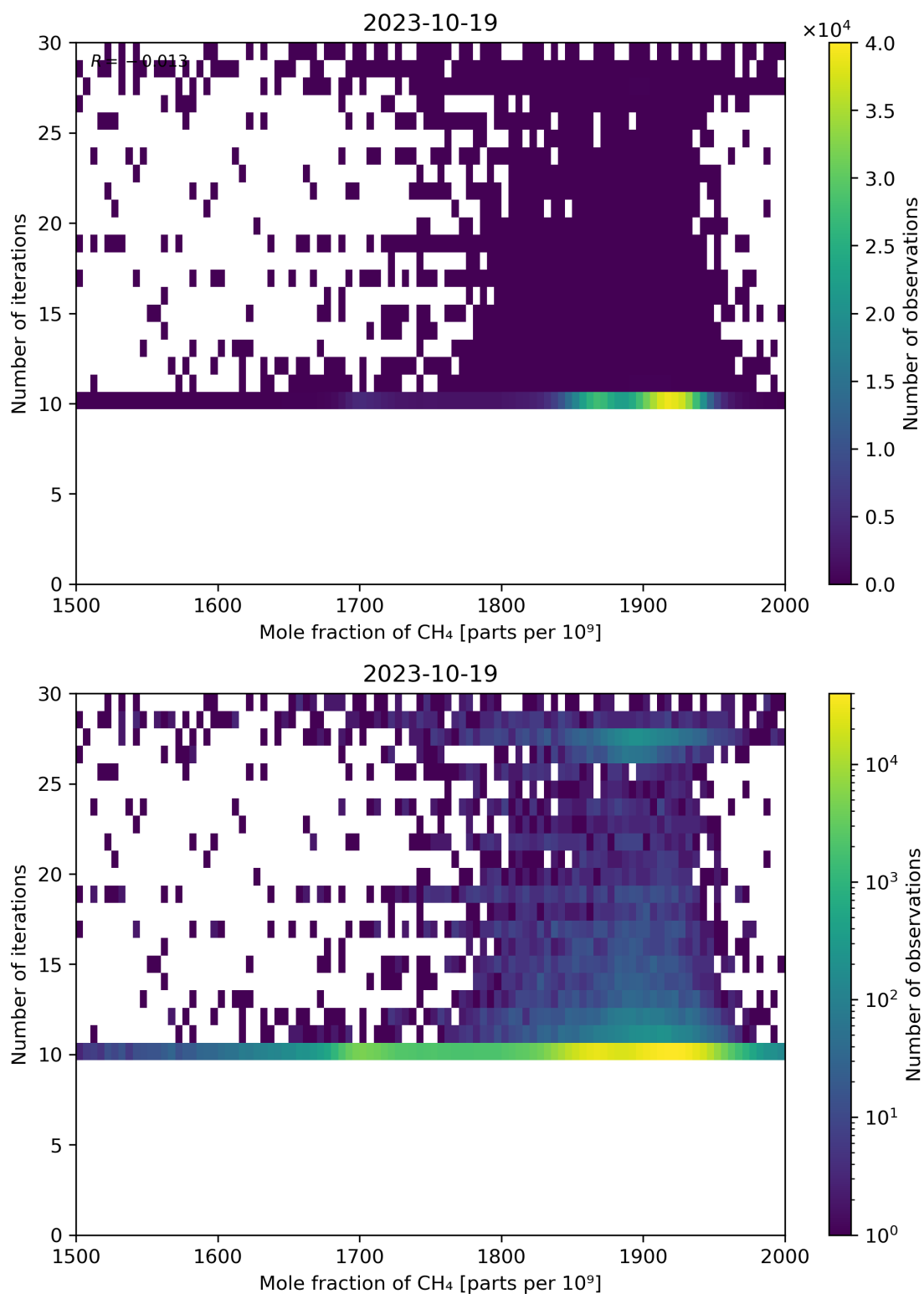
Figure 76: Scatter density plot of “Mole fraction of CH 4 ” against “Number of iterations” for 2023-10-18 to 2023-10-20.
