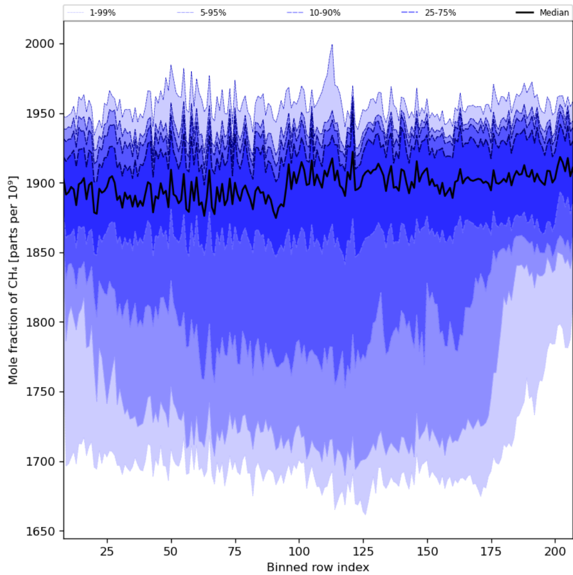
Figure 34: Along track statistics of “Mole fraction of CH 4 ” for 2023-10-18 to 2023-10-20
