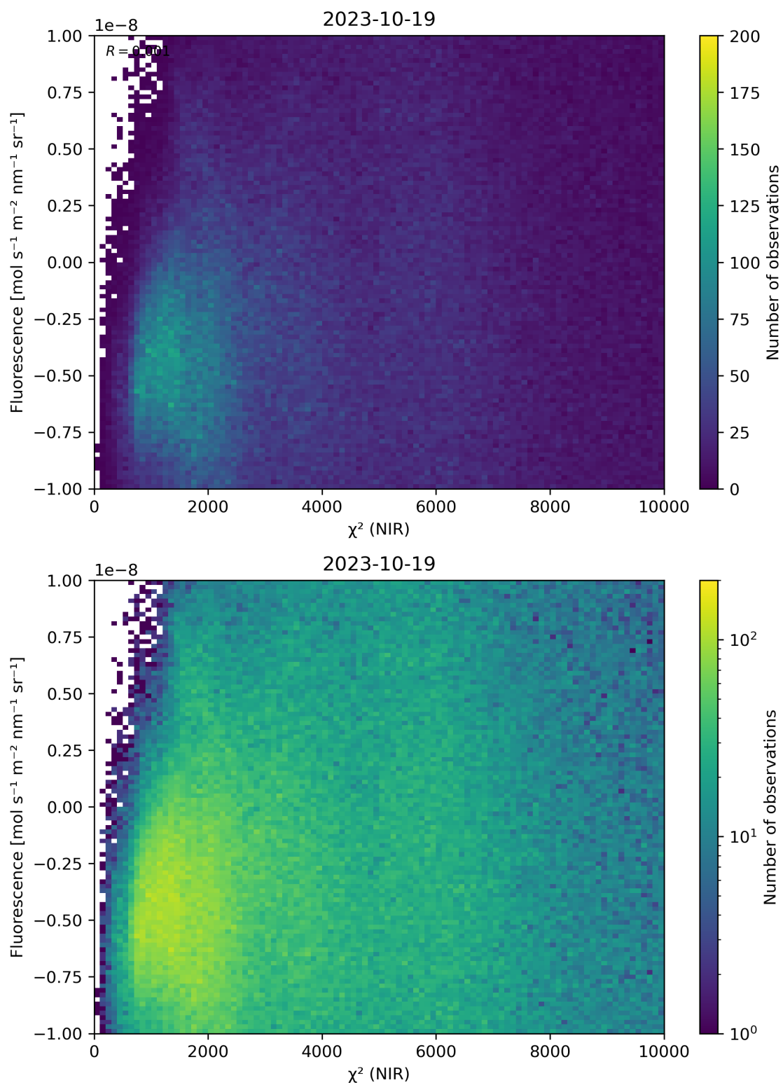
Figure 45: Scatter density plot of “ \chi^2 (NIR)” against “Fluorescence” for 2023-10-18 to 2023-10-20.
