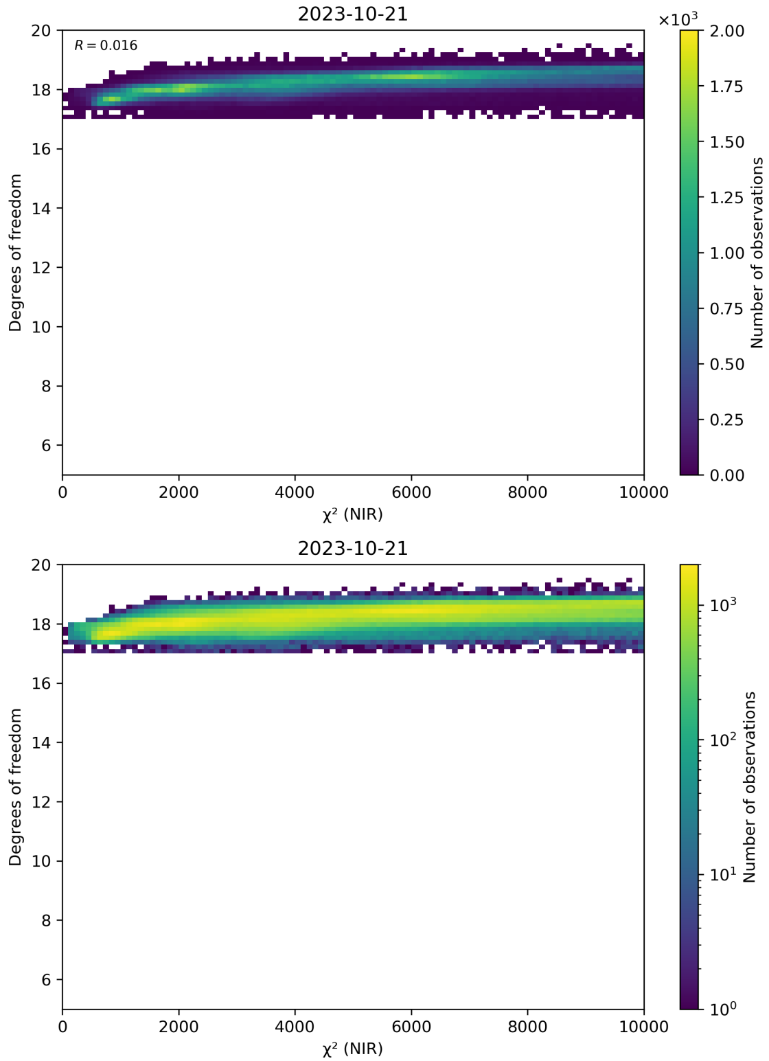
Figure 44: Scatter density plot of “ \chi^2 (NIR)” against “Degrees of freedom” for 2023-10-20 to 2023-10-22.
