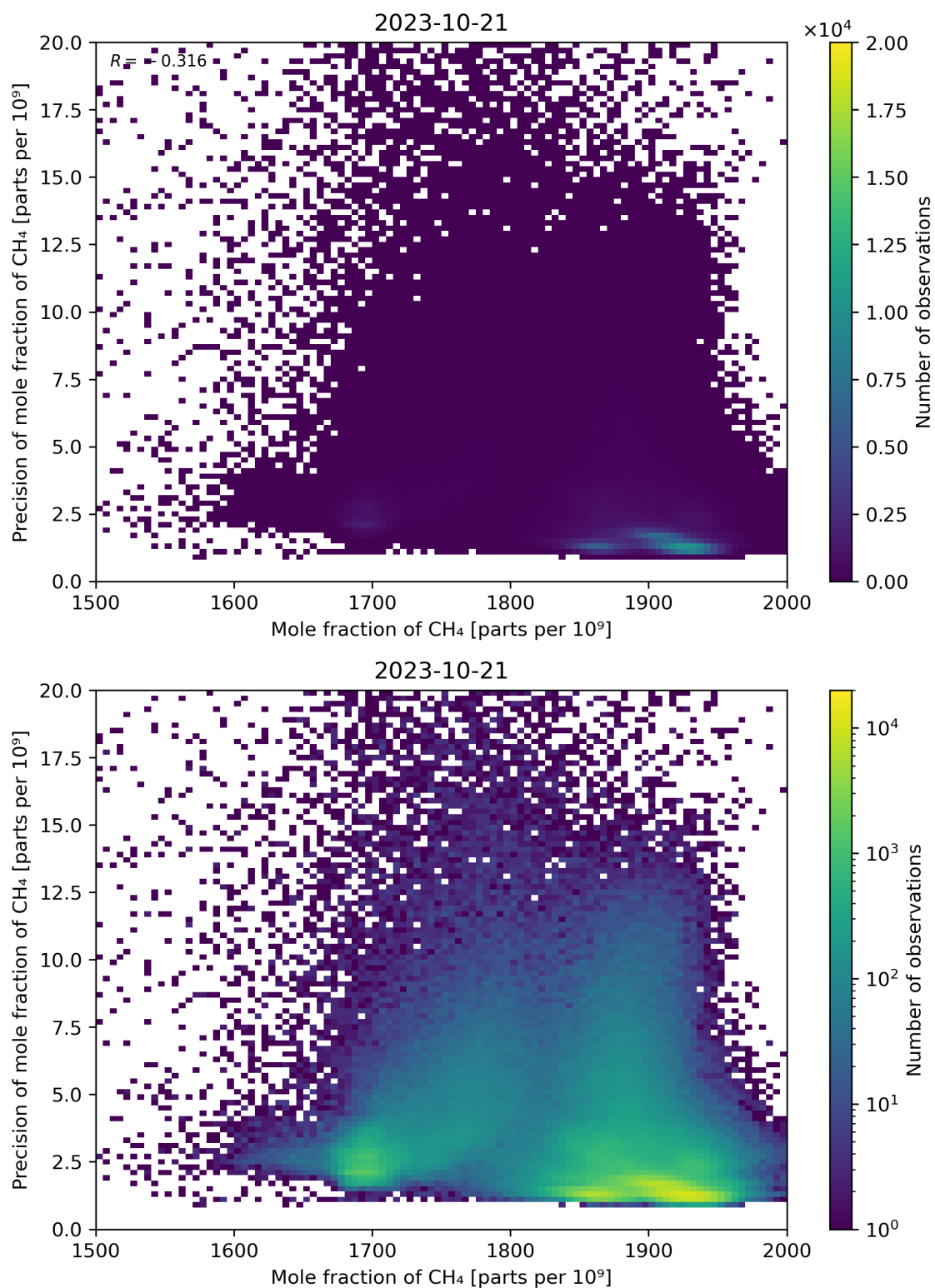
Figure 75: Scatter density plot of “Mole fraction of CH 4 ” against “Precision of mole fraction of CH 4 ” for 2023-10-20 to 2023-10-22.
