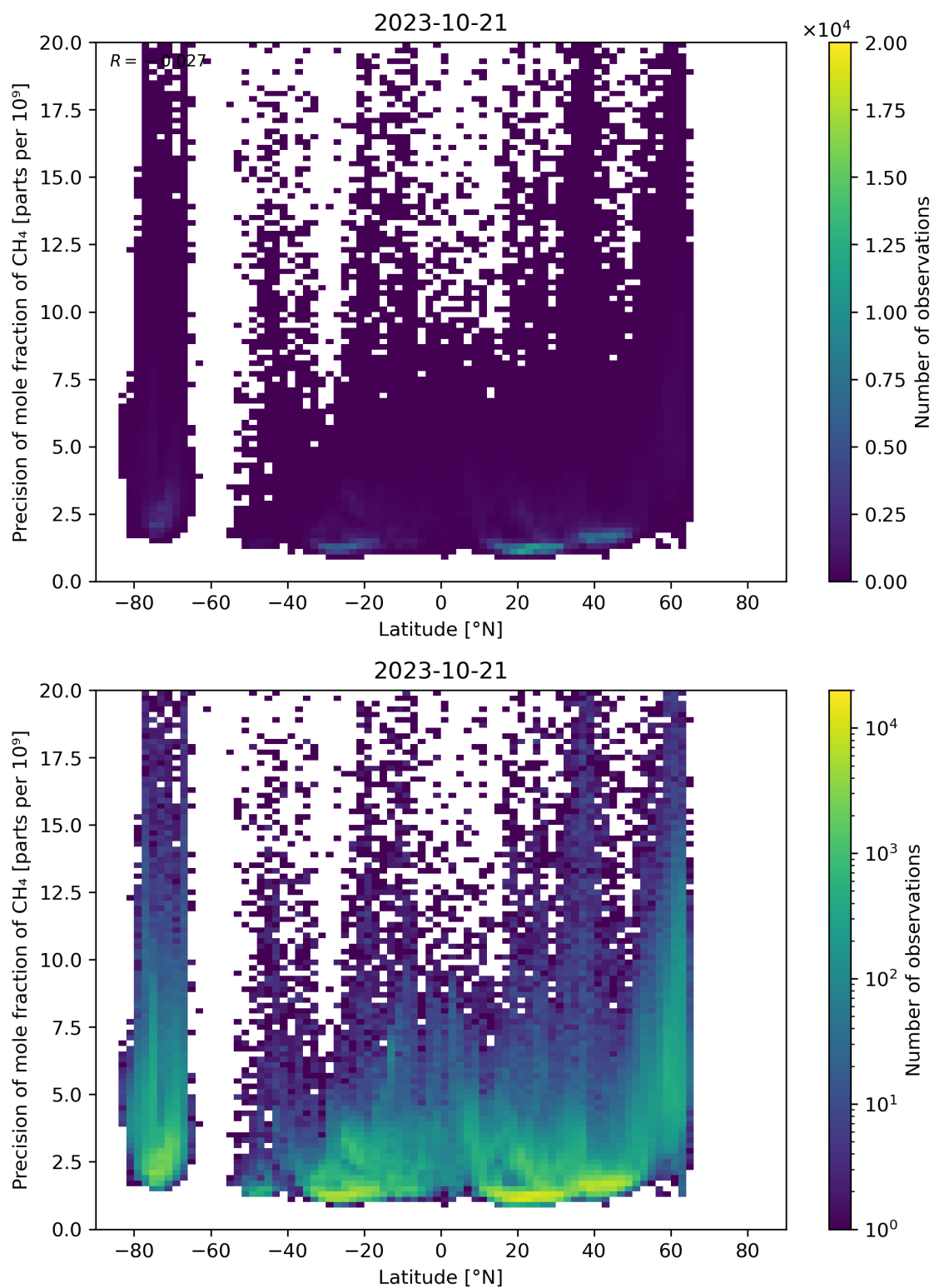
Figure 59: Scatter density plot of “Latitude” against “Precision of mole fraction of CH 4 ” for 2023-10-20 to 2023-10-22.
