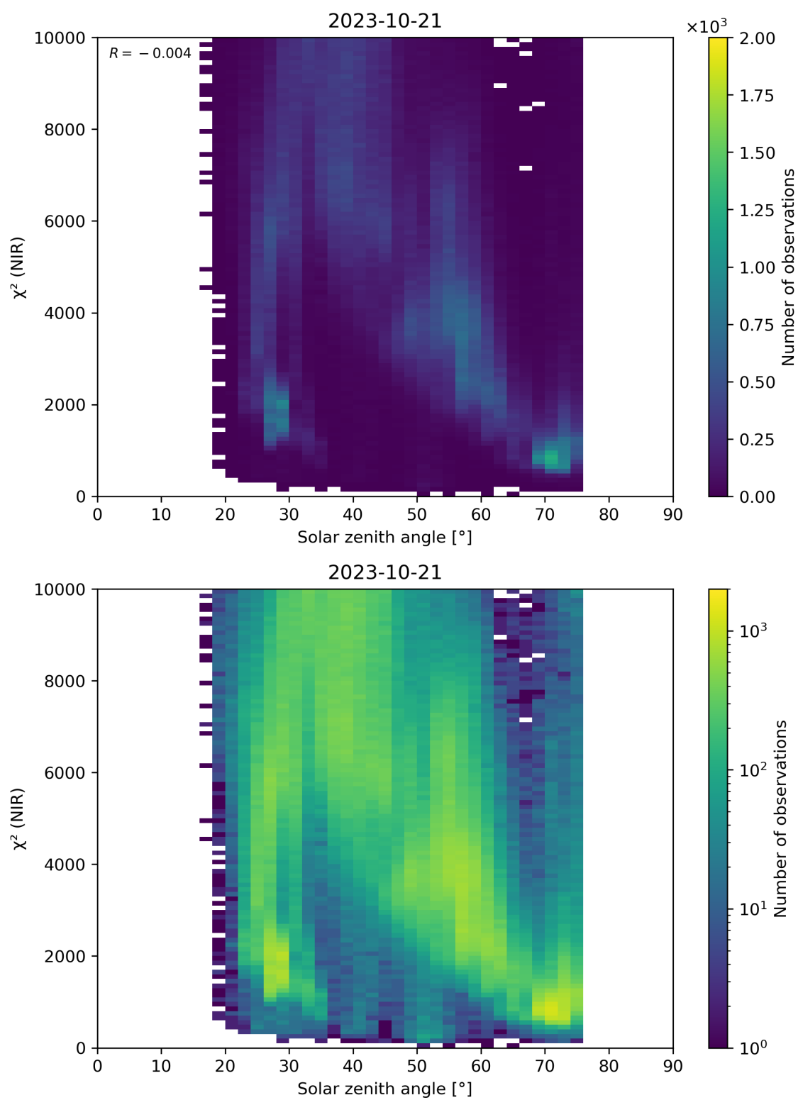
Figure 94: Scatter density plot of “Solar zenith angle” against “ \chi^2 (NIR)” for 2023-10-20 to 2023-10-22.
