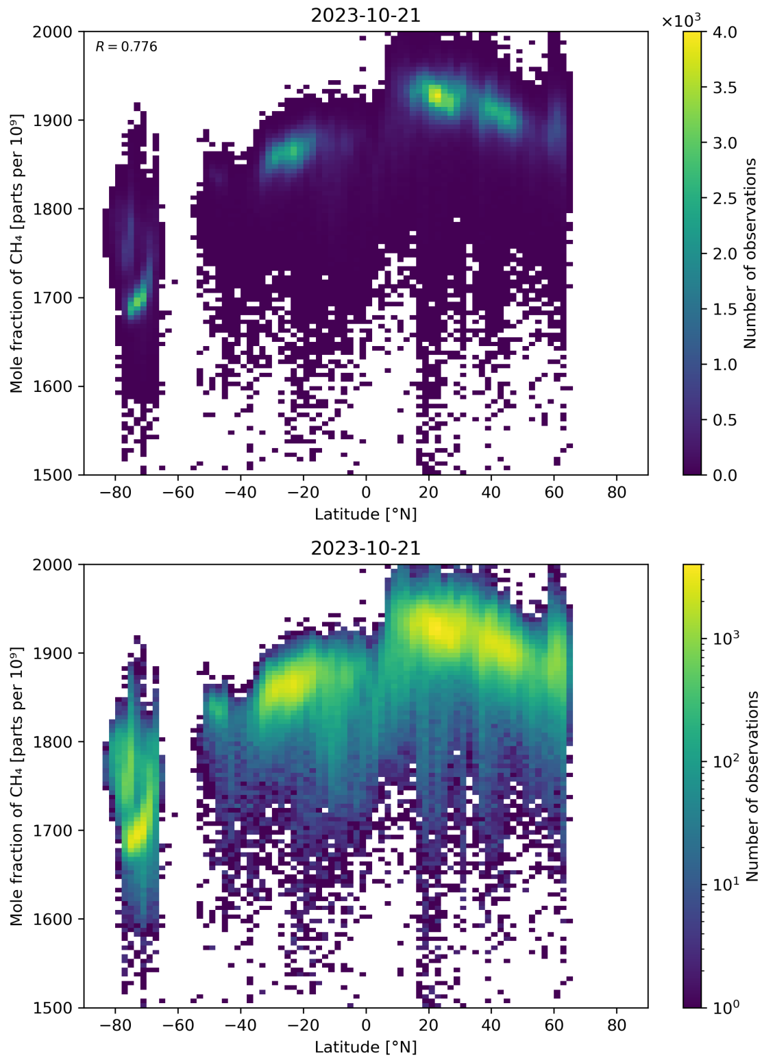
Figure 57: Scatter density plot of “Latitude” against “Mole fraction of \text{CH}_4 ” for 2023-10-20 to 2023-10-22.
