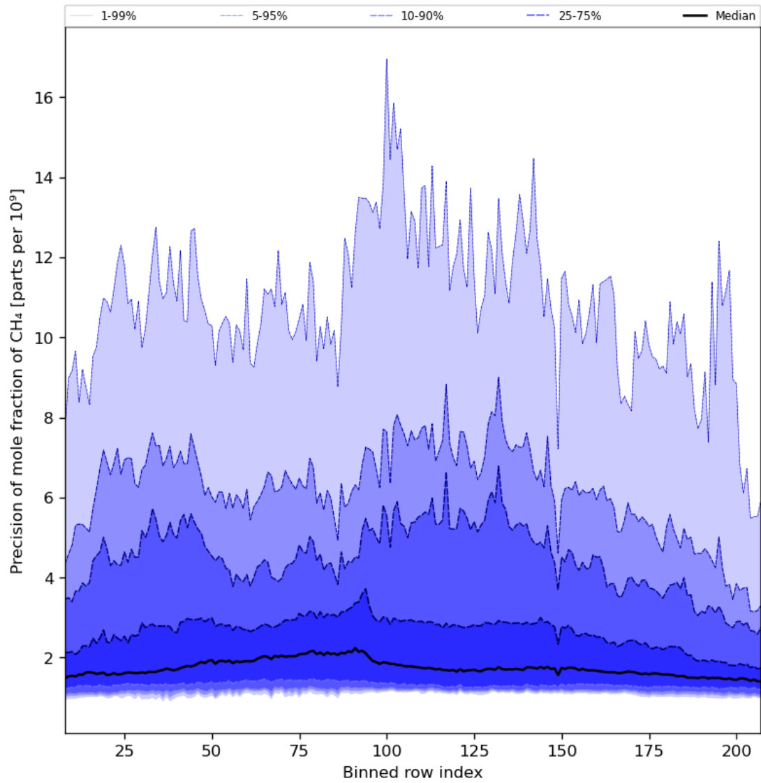
Figure 35: Along track statistics of “Precision of mole fraction of \text{CH}_4 ” for 2023-10-20 to 2023-10-22
