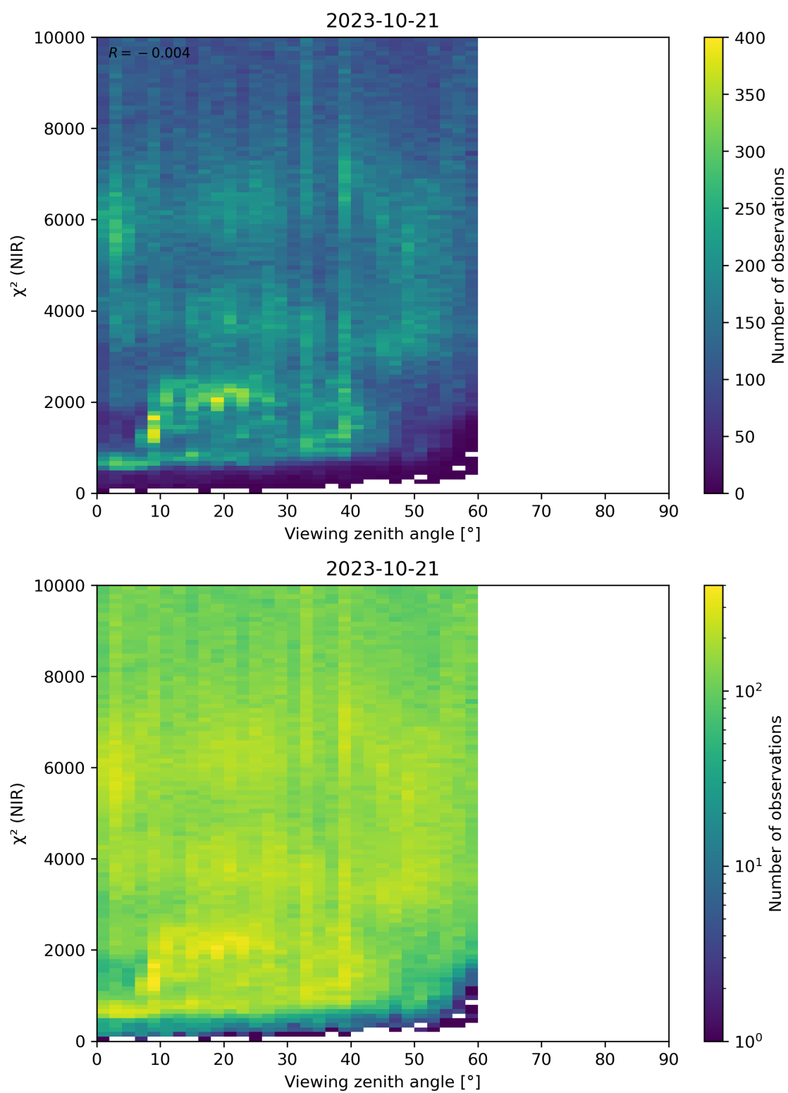
Figure 105: Scatter density plot of “Viewing zenith angle” against “ \chi^2 (NIR)” for 2023-10-20 to 2023-10-22.
