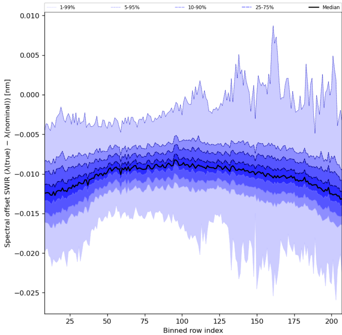
Figure 38: Along track statistics of “Spectral offset SWIR ( \lambda(\text{true}) - \lambda(\text{nominal}) )” for 2023-10-20 to 2023-10-22
