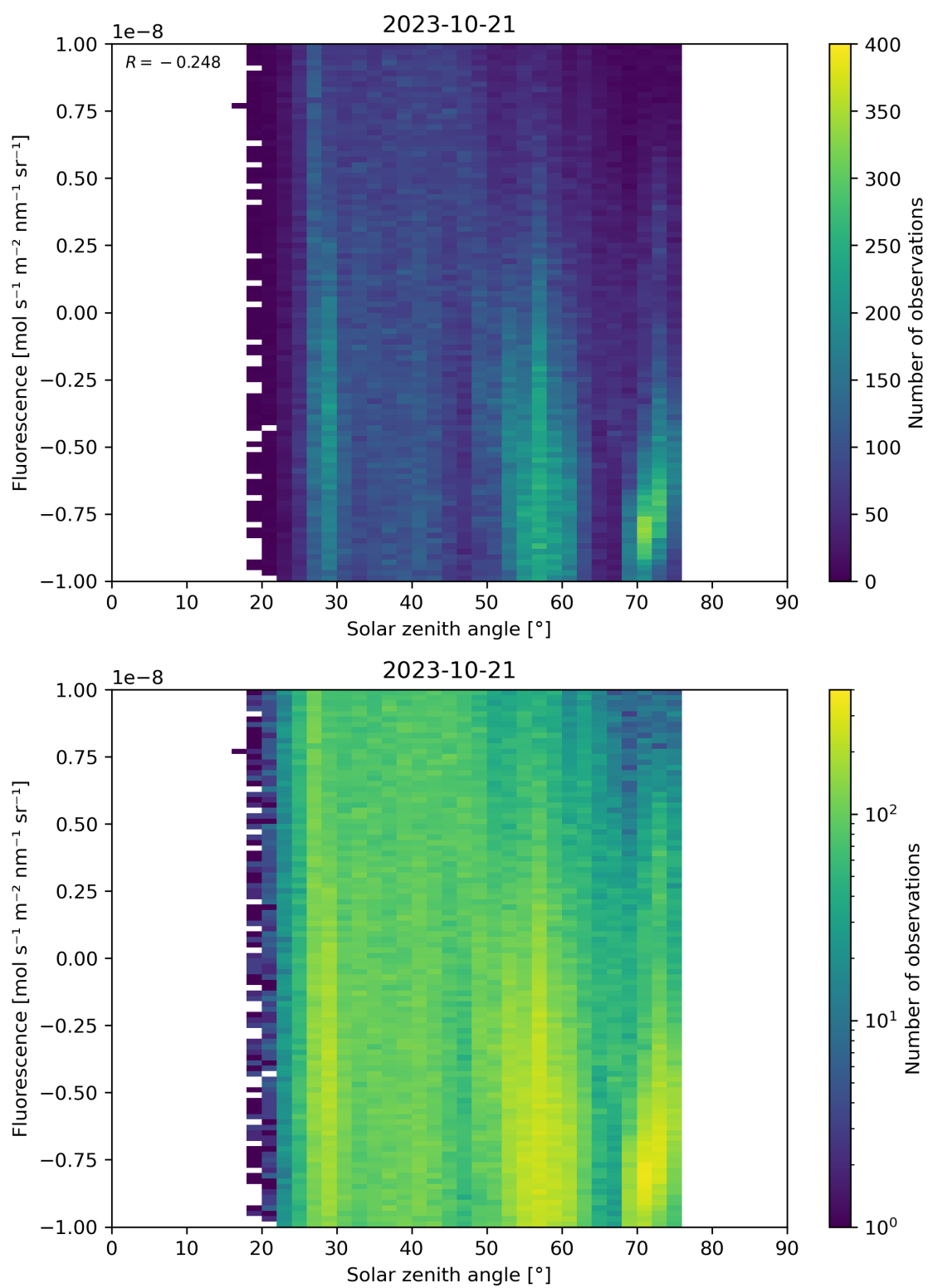
Figure 97: Scatter density plot of “Solar zenith angle” against “Fluorescence” for 2023-10-20 to 2023-10-22.
