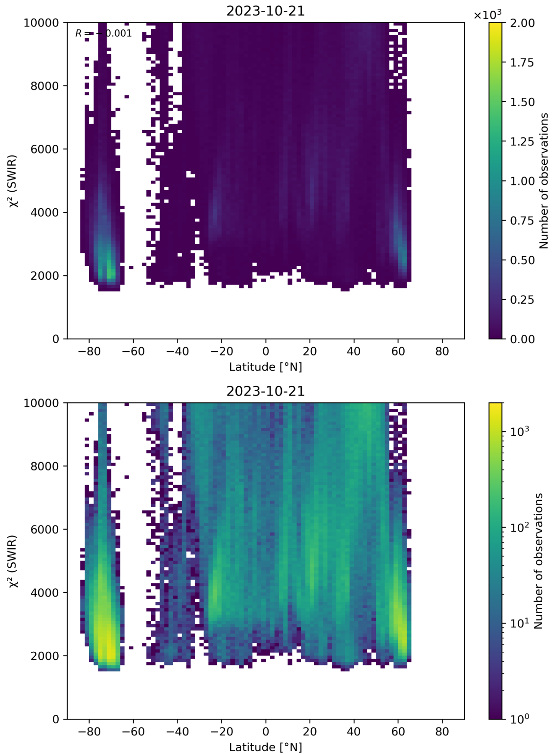
Figure 54: Scatter density plot of “Latitude” against “ \chi^2 (SWIR)” for 2023-10-20 to 2023-10-22.
