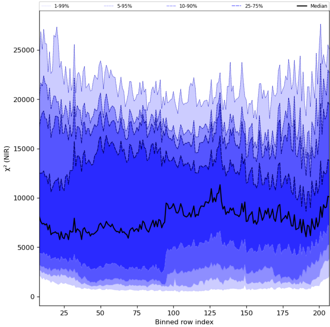
Figure 40: Along track statistics of " \chi^2 (NIR)" for 2023-10-20 to 2023-10-22
