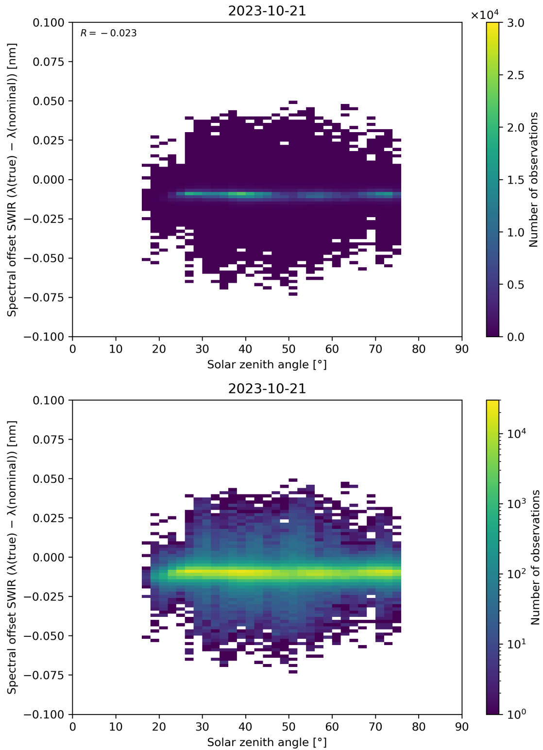
Figure 104: Scatter density plot of “Solar zenith angle” against “Spectral offset SWIR ( \lambda(\text{true}) - \lambda(\text{nominal}) )” for 2023-10-20 to 2023-10-22.
