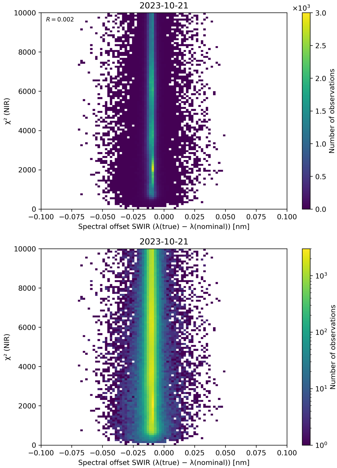
Figure 117: Scatter density plot of “Spectral offset SWIR ( \lambda(\text{true}) - \lambda(\text{nominal}) )” against “ \chi^2 (NIR)” for 2023-10-20 to 2023-10-22.
