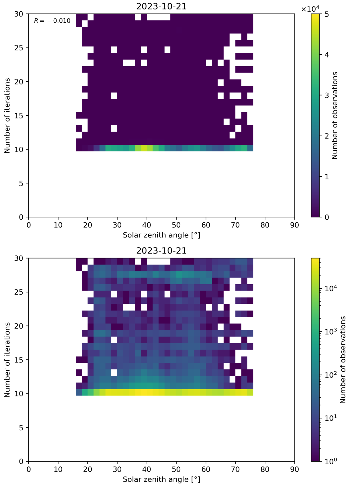
Figure 102: Scatter density plot of “Solar zenith angle” against “Number of iterations” for 2023-10-20 to 2023-10-22.
