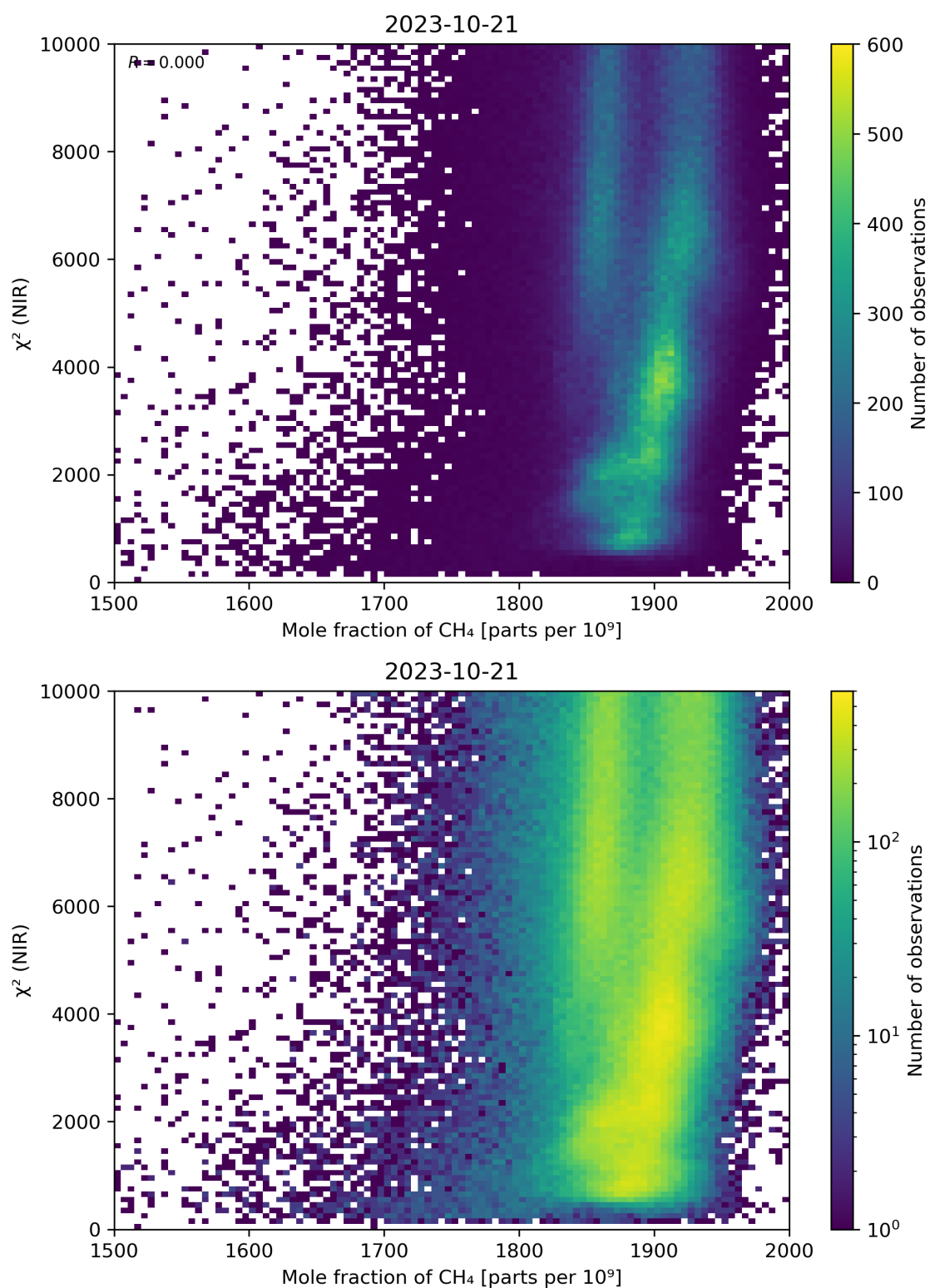
Figure 70: Scatter density plot of “Mole fraction of \text{CH}_4 ” against “ \chi^2 (NIR)” for 2023-10-20 to 2023-10-22.
