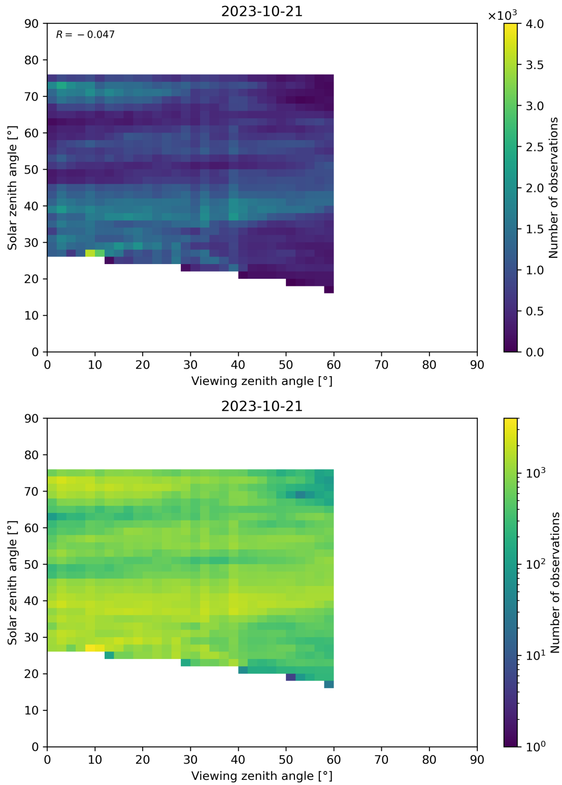
Figure 115: Scatter density plot of “Viewing zenith angle” against “Solar zenith angle” for 2023-10-20 to 2023-10-22.
