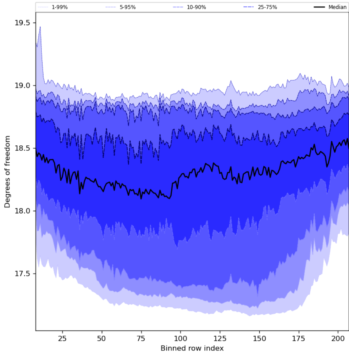
Figure 41: Along track statistics of “Degrees of freedom” for 2023-10-20 to 2023-10-22
