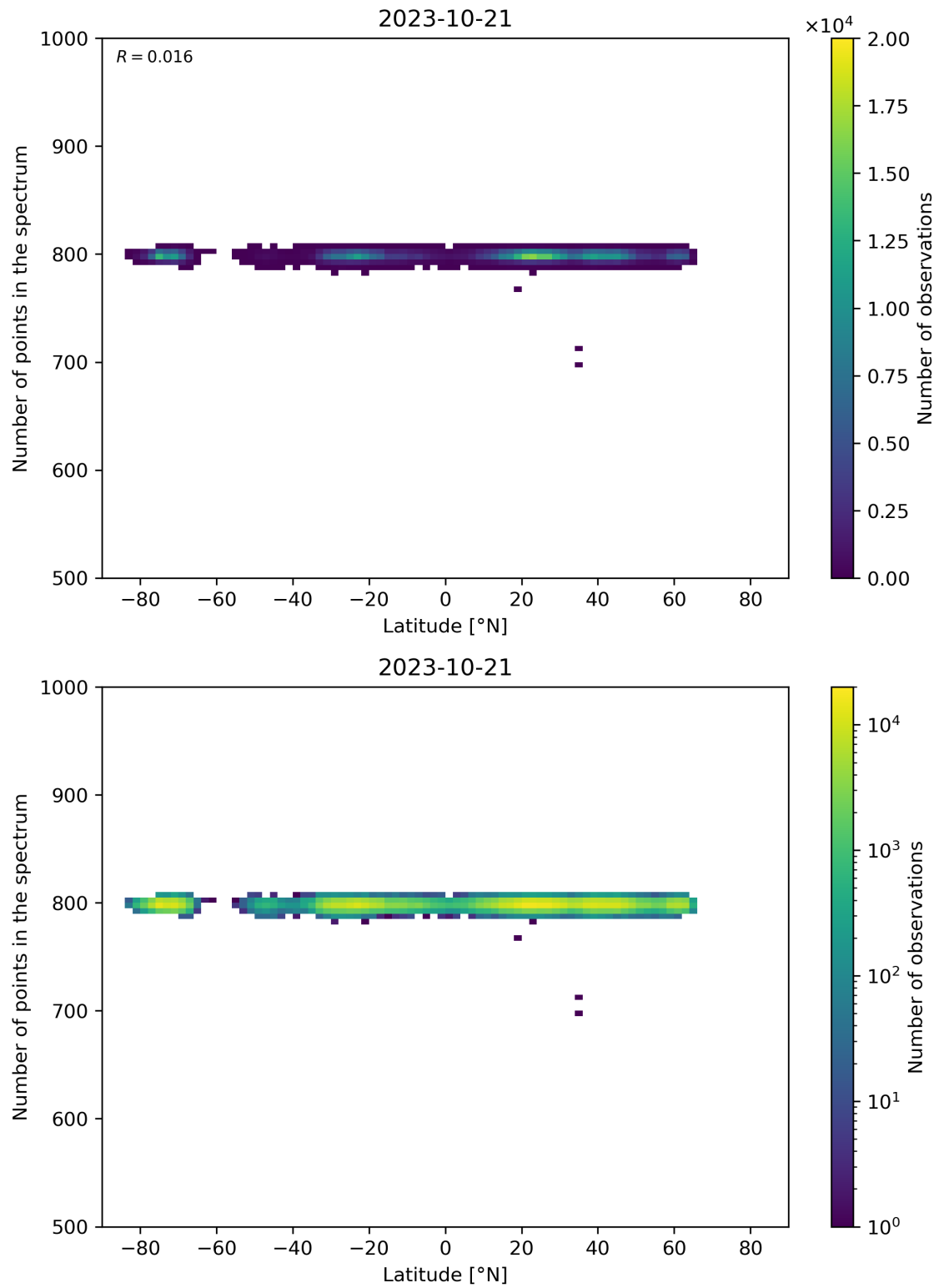
Figure 61: Scatter density plot of “Latitude” against “Number of points in the spectrum” for 2023-10-20 to 2023-10-22.
