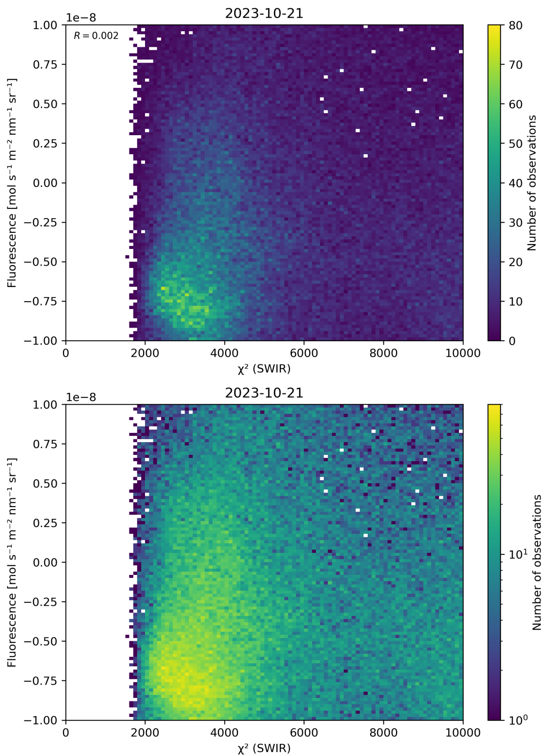
Figure 49: Scatter density plot of “ \chi^2 (SWIR)” against “Fluorescence” for 2023-10-20 to 2023-10-22.
