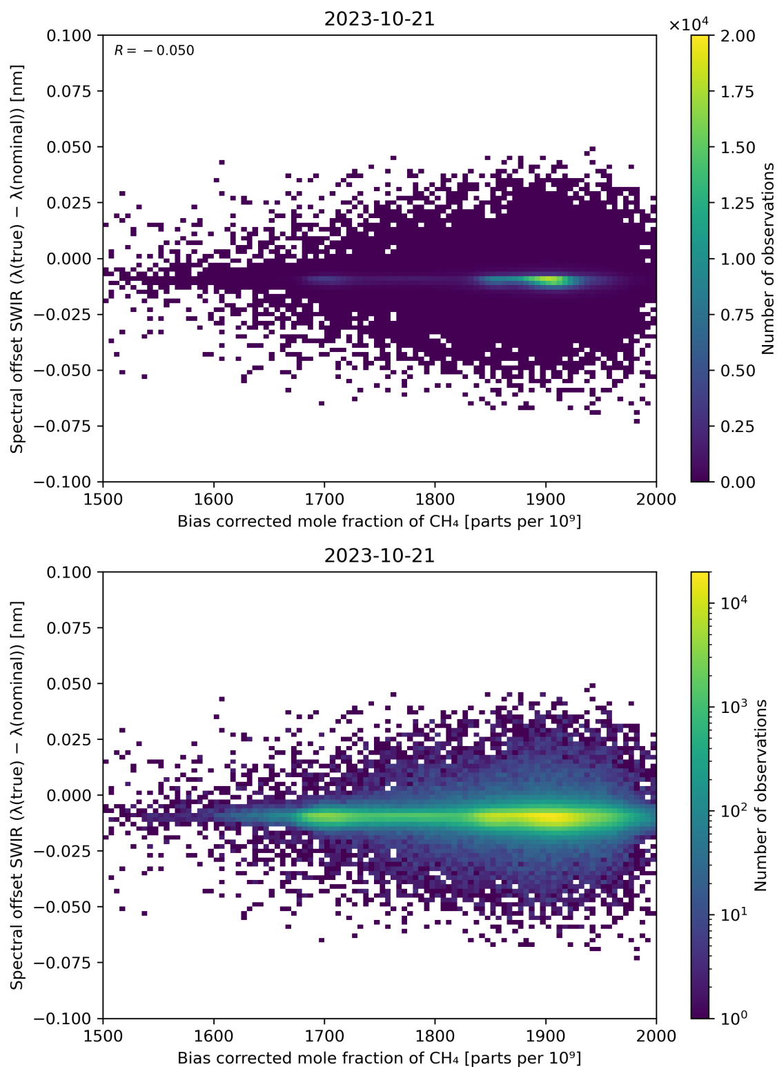
Figure 69: Scatter density plot of “Bias corrected mole fraction of \text{CH}_4 ” against “Spectral offset SWIR ( \lambda(\text{true}) - \lambda(\text{nominal}) )” for 2023-10-20 to 2023-10-22.
