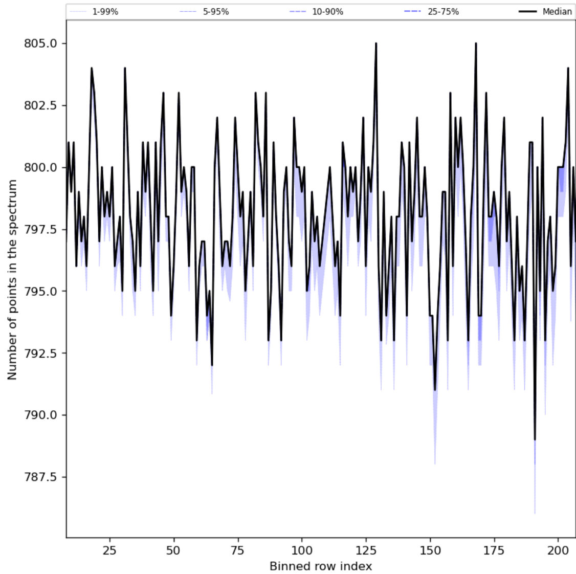
Figure 37: Along track statistics of “Number of points in the spectrum” for 2023-10-20 to 2023-10-22
