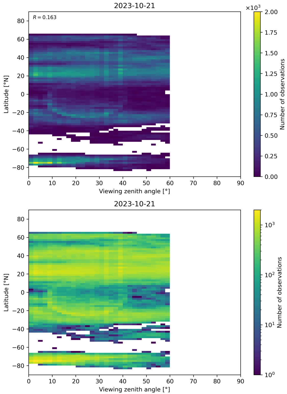
Figure 109: Scatter density plot of “Viewing zenith angle” against “Latitude” for 2023-10-20 to 2023-10-22.
