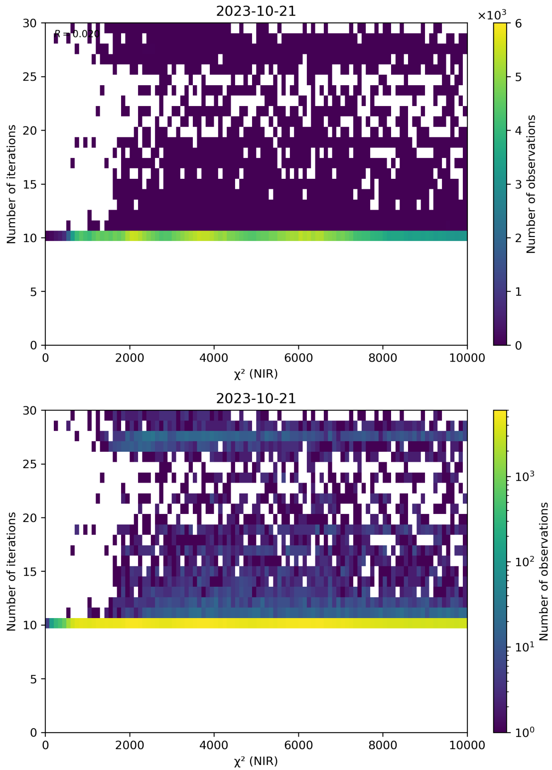
Figure 46: Scatter density plot of “ \chi^2 (NIR)” against “Number of iterations” for 2023-10-20 to 2023-10-22.
