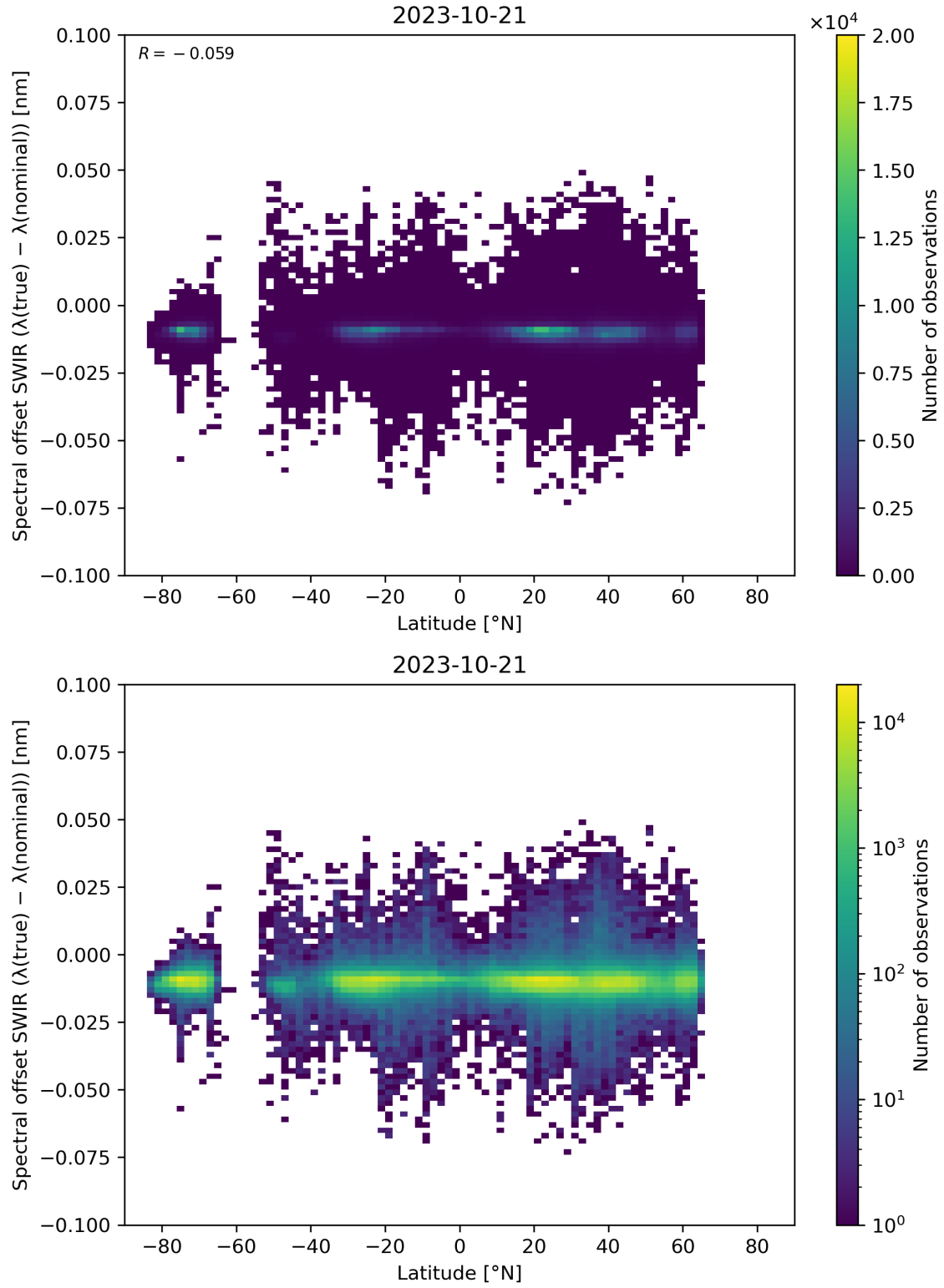
Figure 62: Scatter density plot of “Latitude” against “Spectral offset SWIR ( \lambda(\text{true}) - \lambda(\text{nominal}) )” for 2023-10-20 to 2023-10-22.
