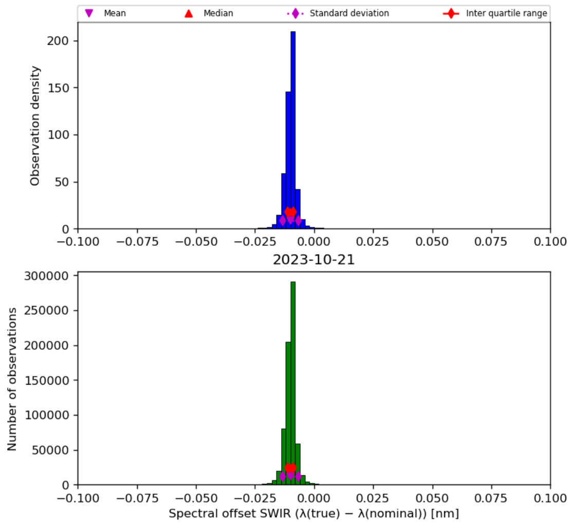
Figure 27: Histogram of “Spectral offset SWIR ( \lambda(\text{true}) - \lambda(\text{nominal}) )” for 2023-10-20 to 2023-10-22
