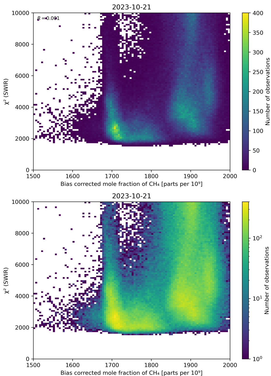
Figure 64: Scatter density plot of “Bias corrected mole fraction of CH 4 ” against “ \chi^2 (SWIR)” for 2023-10-20 to 2023-10-22.
