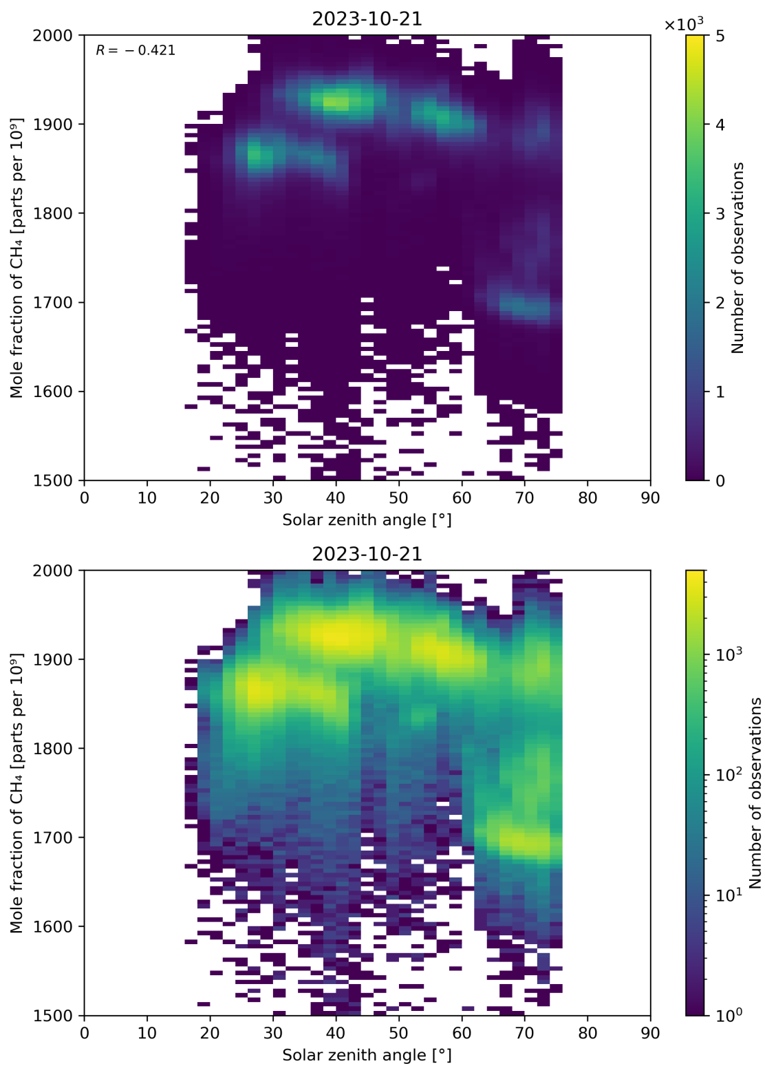
Figure 99: Scatter density plot of “Solar zenith angle” against “Mole fraction of CH 4 ” for 2023-10-20 to 2023-10-22.
