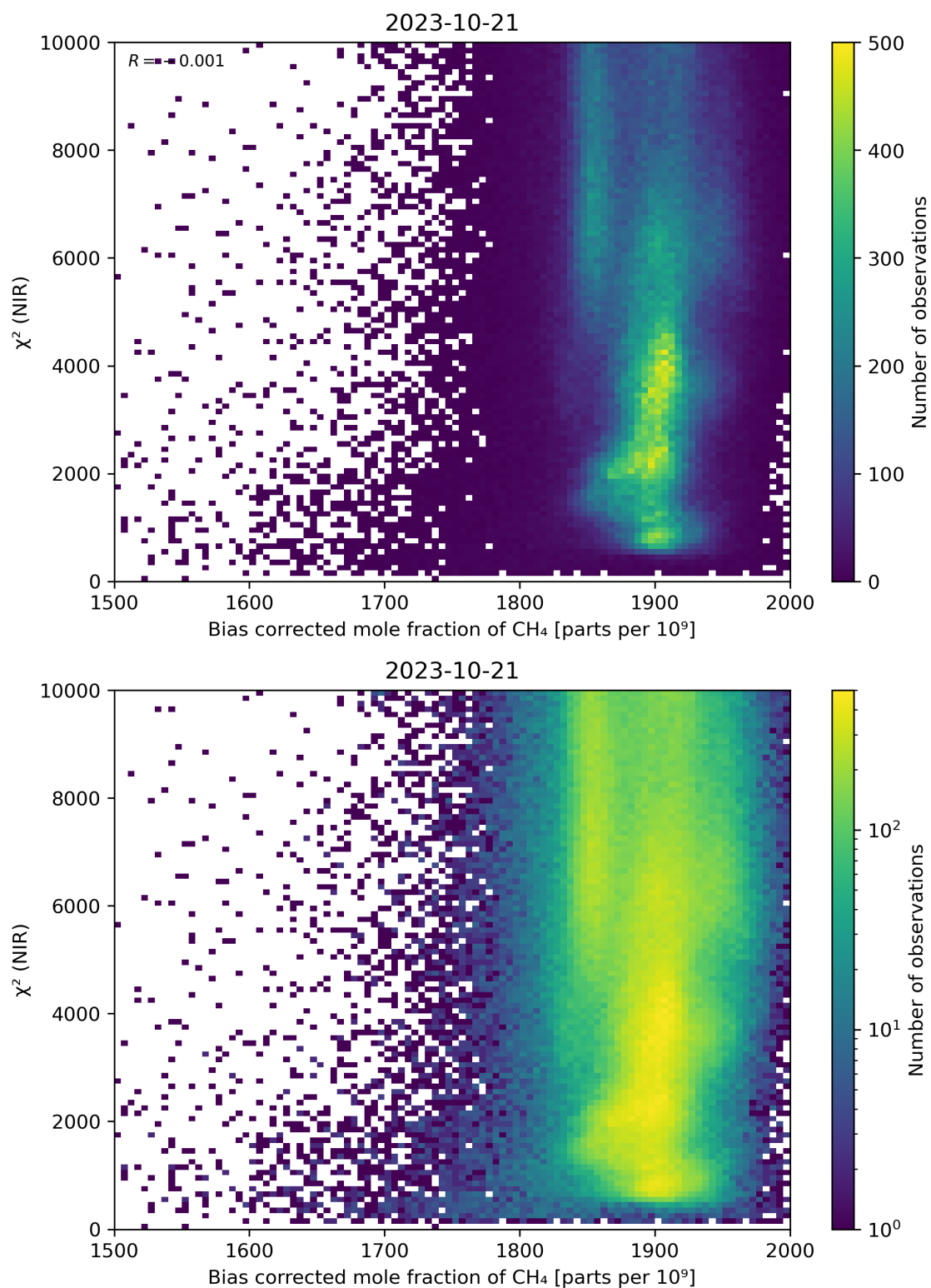
Figure 63: Scatter density plot of “Bias corrected mole fraction of CH 4 ” against “ \chi^2 (NIR)” for 2023-10-20 to 2023-10-22.
