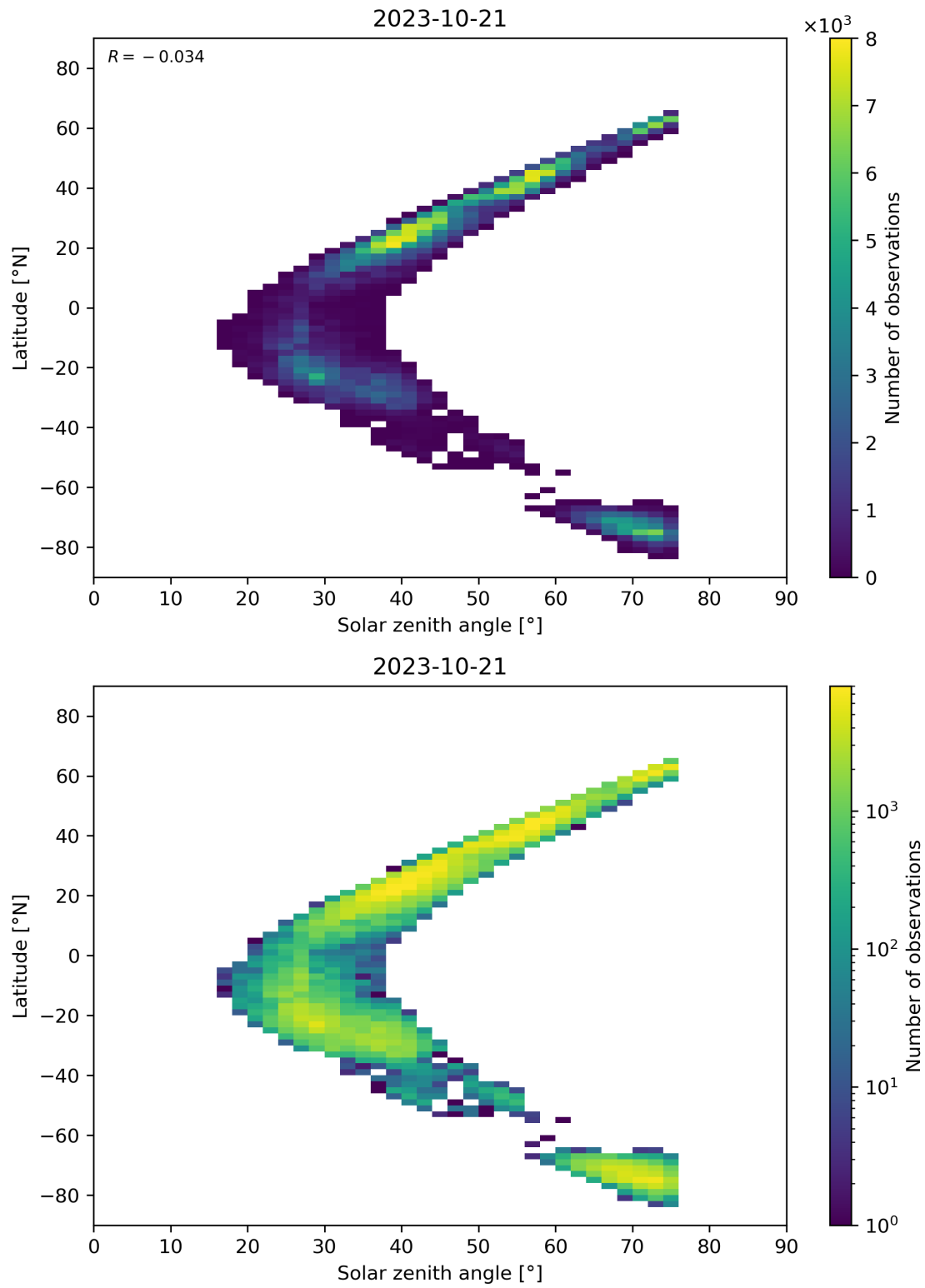
Figure 98: Scatter density plot of “Solar zenith angle” against “Latitude” for 2023-10-20 to 2023-10-22.
