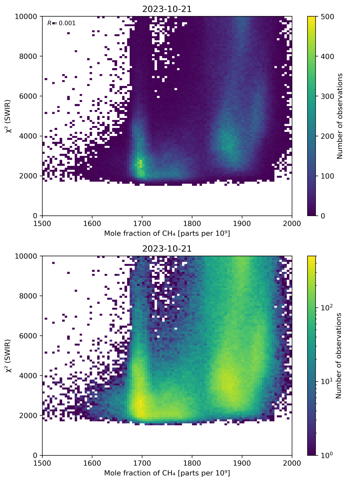
Figure 71: Scatter density plot of “Mole fraction of CH 4 ” against “ \chi^2 (SWIR)” for 2023-10-20 to 2023-10-22.
