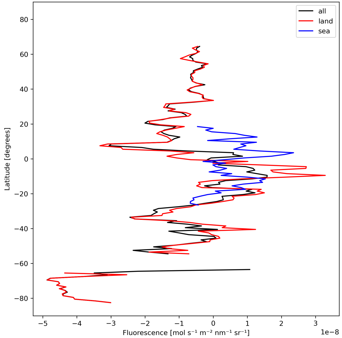
Figure 21: Zonal average of “Fluorescence” for 2023-10-20 to 2023-10-22.
