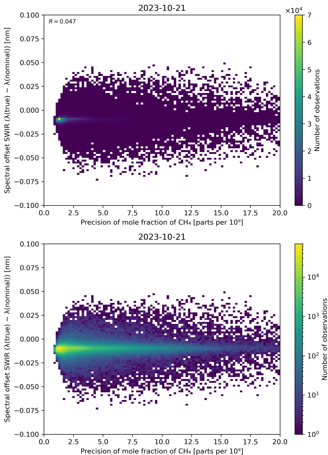
Figure 85: Scatter density plot of “Precision of mole fraction of CH 4 ” against “Spectral offset SWIR ( \lambda(\text{true}) - \lambda(\text{nominal}) )” for 2023-10-20 to 2023-10-22.
