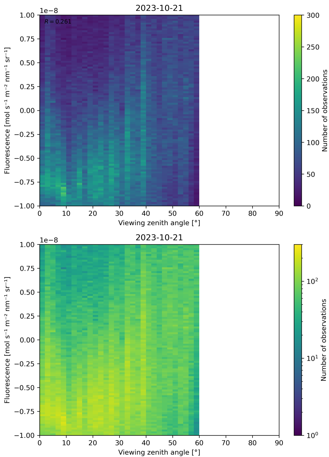
Figure 108: Scatter density plot of “Viewing zenith angle” against “Fluorescence” for 2023-10-20 to 2023-10-22.
