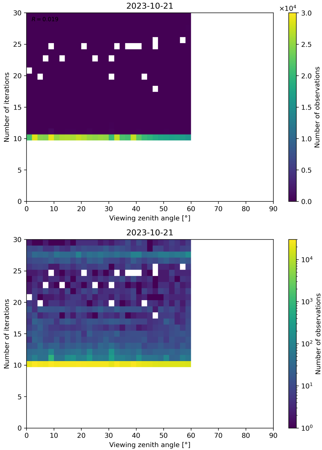
Figure 113: Scatter density plot of “Viewing zenith angle” against “Number of iterations” for 2023-10-20 to 2023-10-22.
