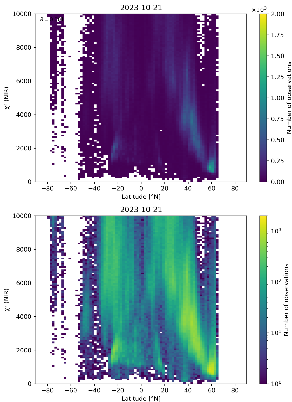
Figure 53: Scatter density plot of “Latitude” against “ \chi^2 (NIR)” for 2023-10-20 to 2023-10-22.
