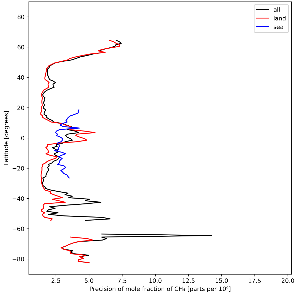
Figure 13: Zonal average of “Precision of mole fraction of CH 4 ” for 2023-10-20 to 2023-10-22.
