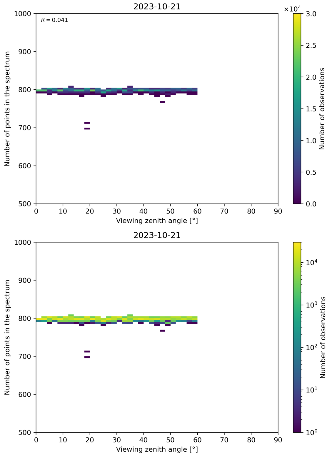
Figure 114: Scatter density plot of “Viewing zenith angle” against “Number of points in the spectrum” for 2023-10-20 to 2023-10-22.
