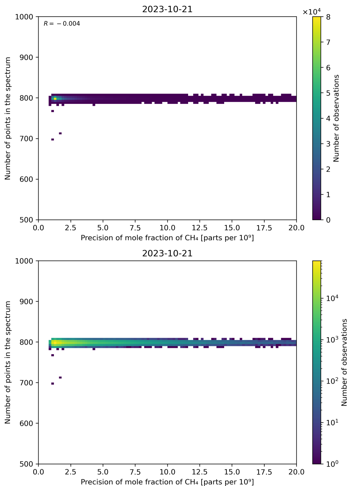
Figure 84: Scatter density plot of “Precision of mole fraction of CH 4 ” against “Number of points in the spectrum” for 2023-10-20 to 2023-10-22.
