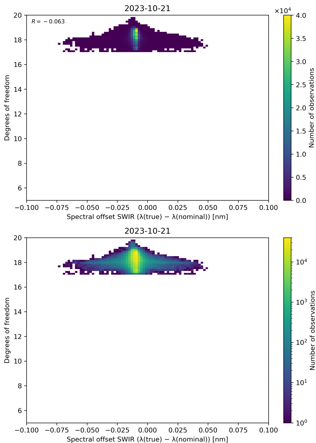
Figure 119: Scatter density plot of “Spectral offset SWIR ( \lambda(\text{true}) - \lambda(\text{nominal}) )” against “Degrees of freedom” for 2023-10-20 to 2023-10-22.
