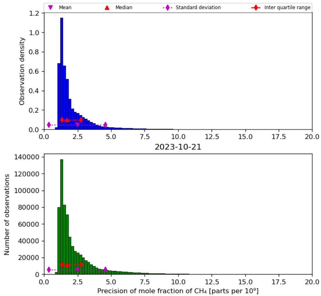
Figure 24: Histogram of “Precision of mole fraction of CH 4 ” for 2023-10-20 to 2023-10-22
