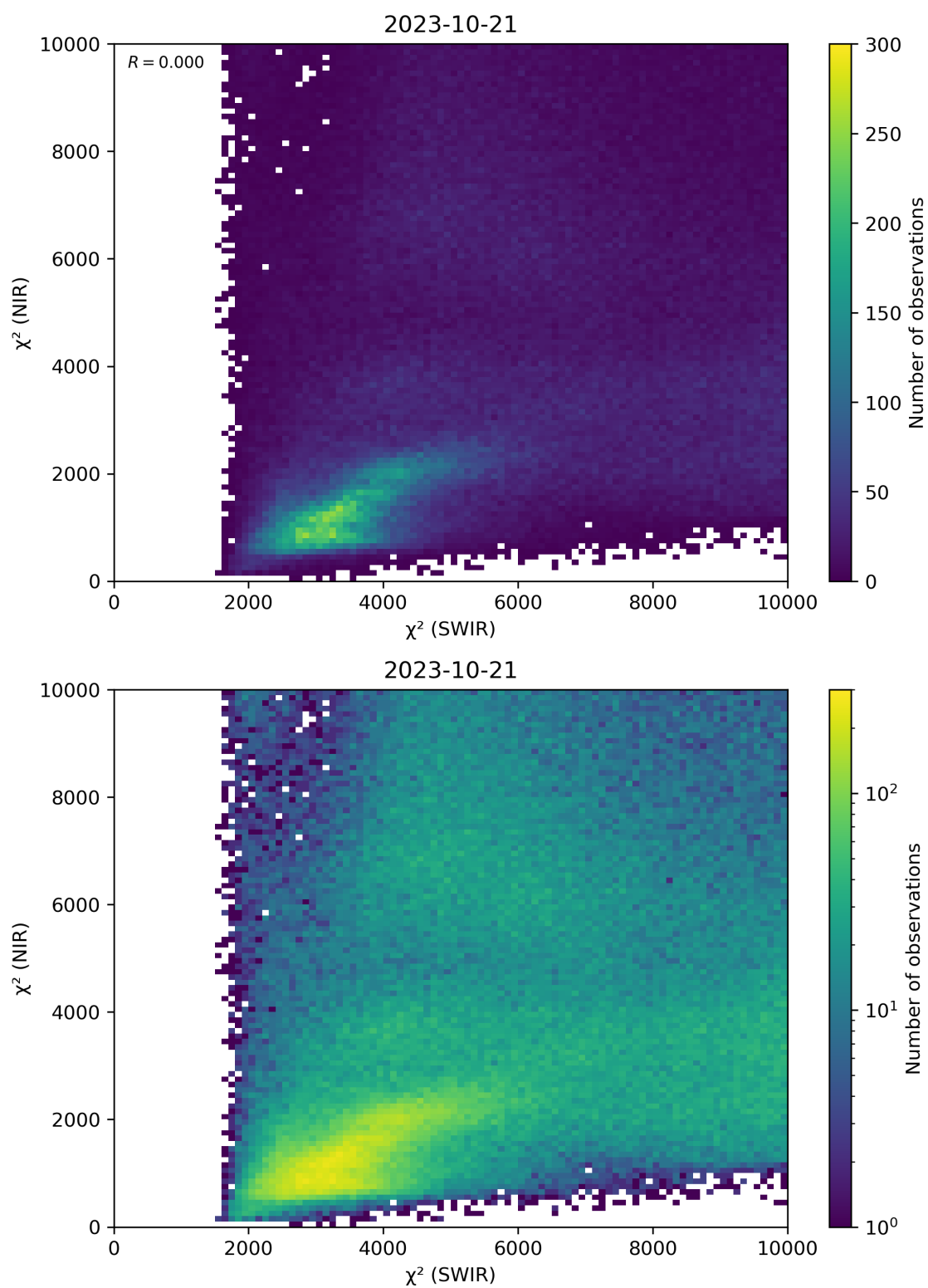
Figure 47: Scatter density plot of “ \chi^2 (SWIR)” against “ \chi^2 (NIR)” for 2023-10-20 to 2023-10-22.
