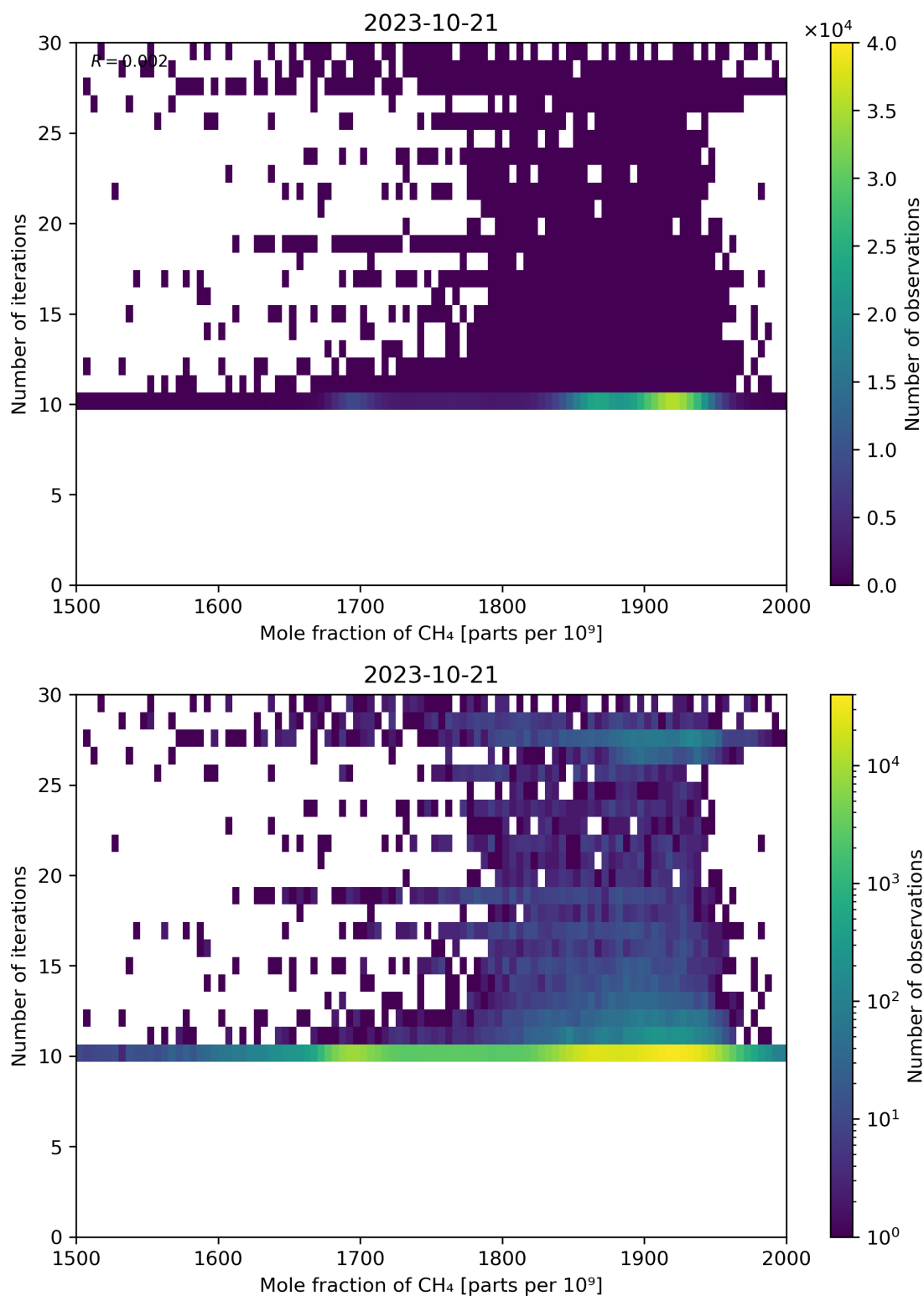
Figure 76: Scatter density plot of “Mole fraction of CH 4 ” against “Number of iterations” for 2023-10-20 to 2023-10-22.
