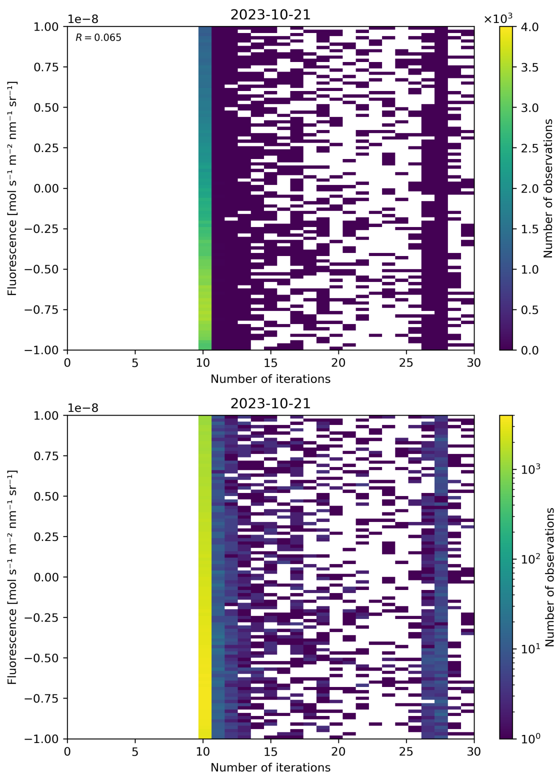
Figure 87: Scatter density plot of “Number of iterations” against “Fluorescence” for 2023-10-20 to 2023-10-22.
