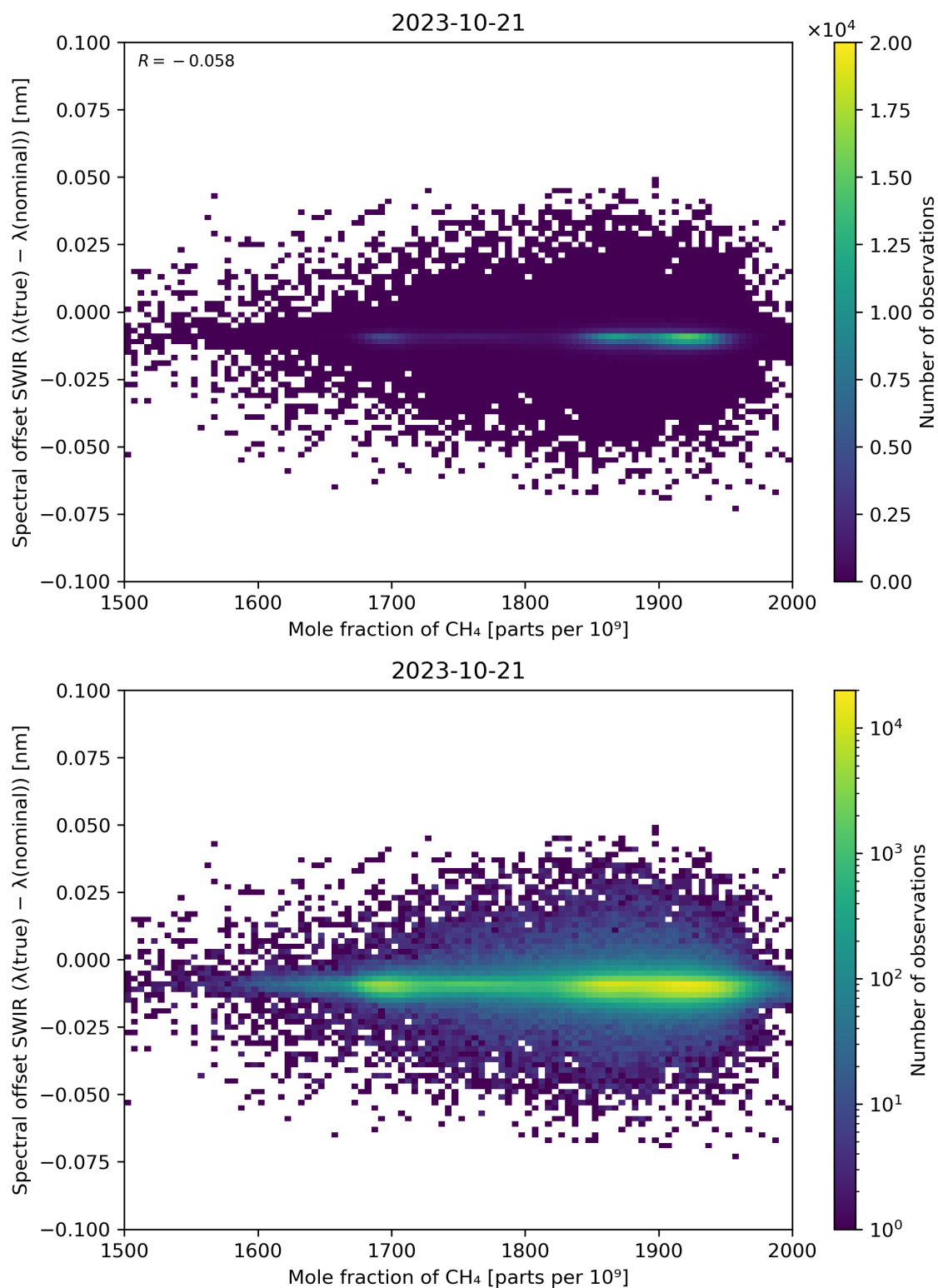
Figure 86: Scatter density plot of “Mole fraction of CH 4 ” against “Spectral offset SWIR ( \lambda(\text{true}) - \lambda(\text{nominal}) )” for 2023-10-20 to 2023-10-22.
