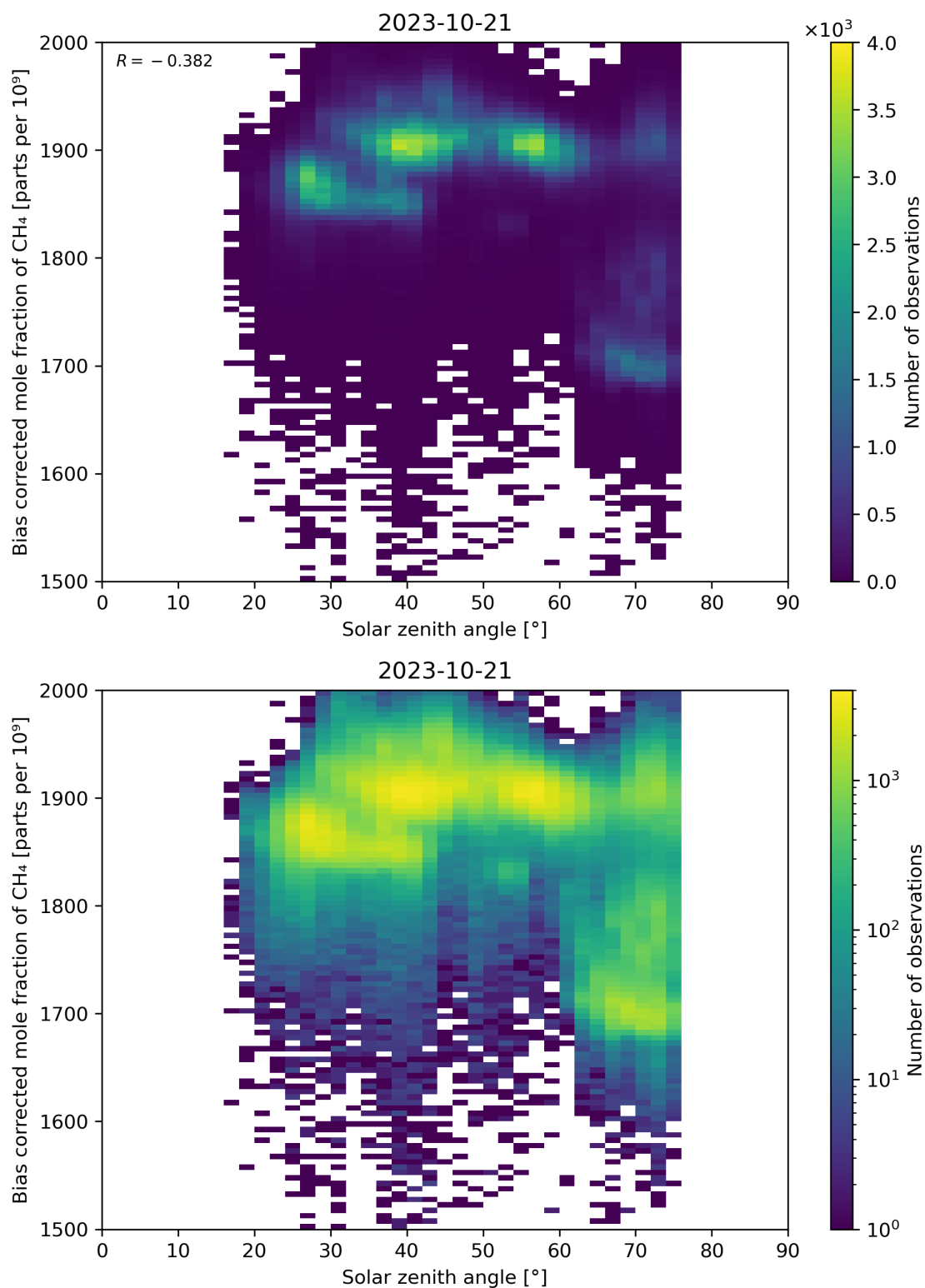
Figure 100: Scatter density plot of “Solar zenith angle” against “Bias corrected mole fraction of CH 4 ” for 2023-10-20 to 2023-10-22.
