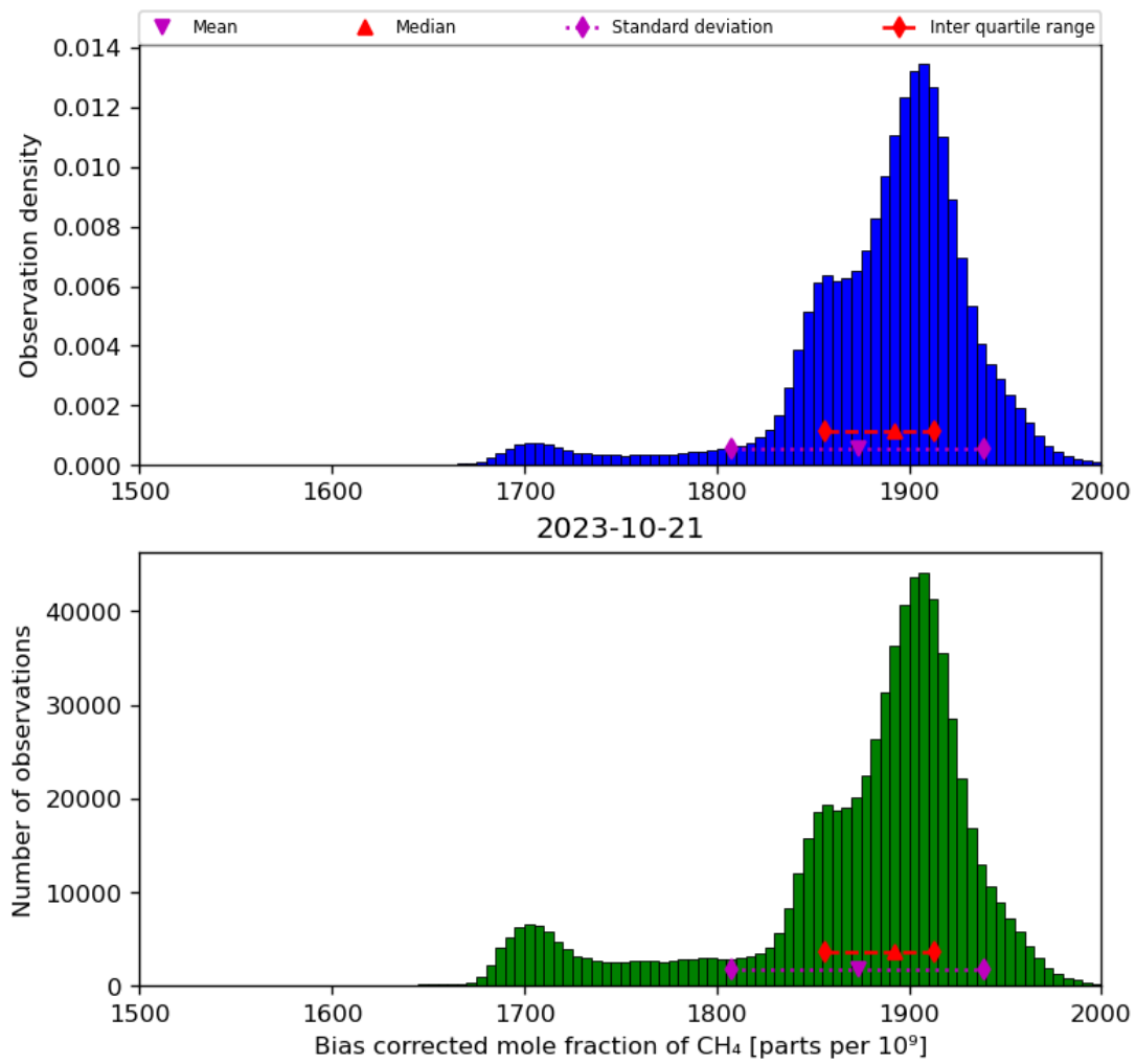
Figure 25: Histogram of “Bias corrected mole fraction of CH 4 ” for 2023-10-20 to 2023-10-22
