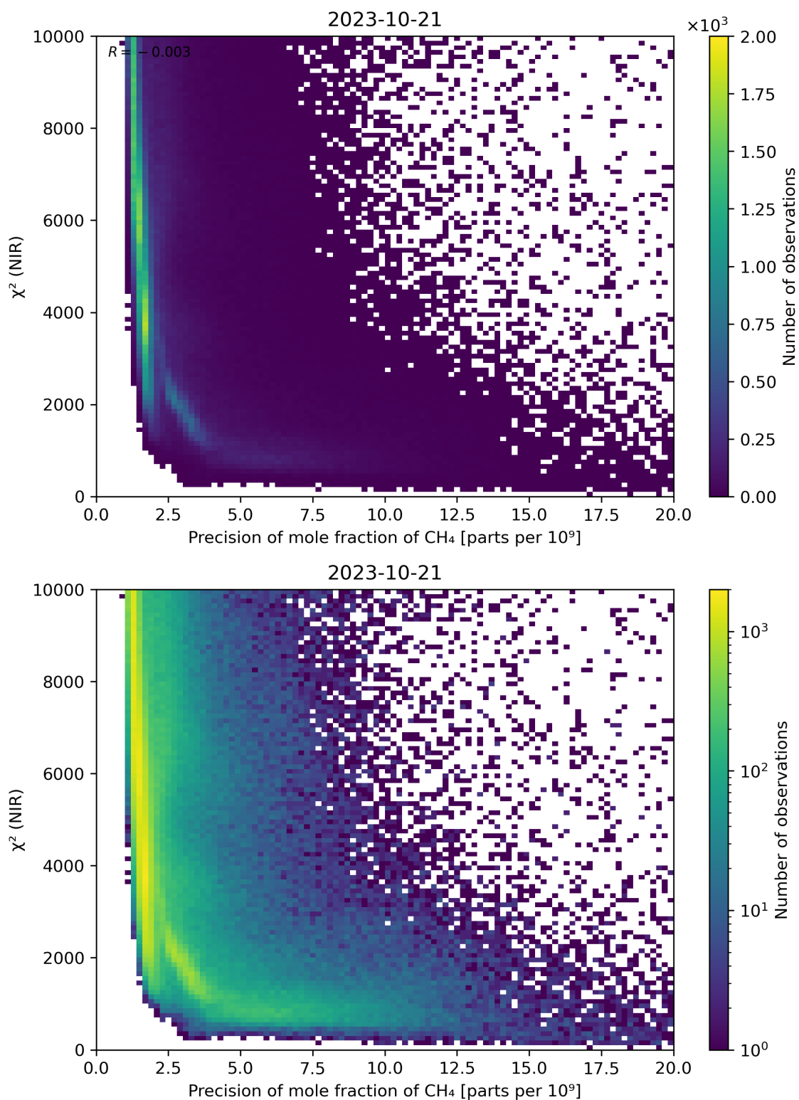
Figure 78: Scatter density plot of “Precision of mole fraction of CH 4 ” against “ \chi^2 (NIR)” for 2023-10-20 to 2023-10-22.
