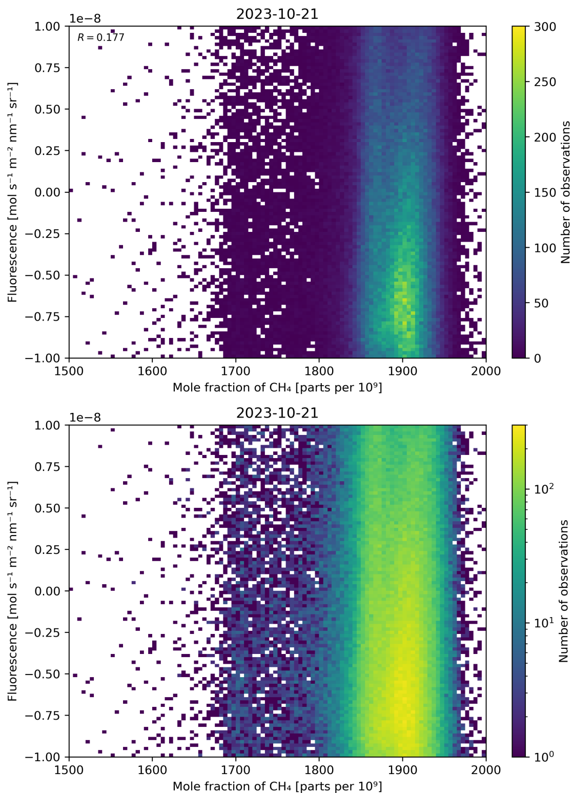
Figure 73: Scatter density plot of “Mole fraction of \text{CH}_4 ” against “Fluorescence” for 2023-10-20 to 2023-10-22.
