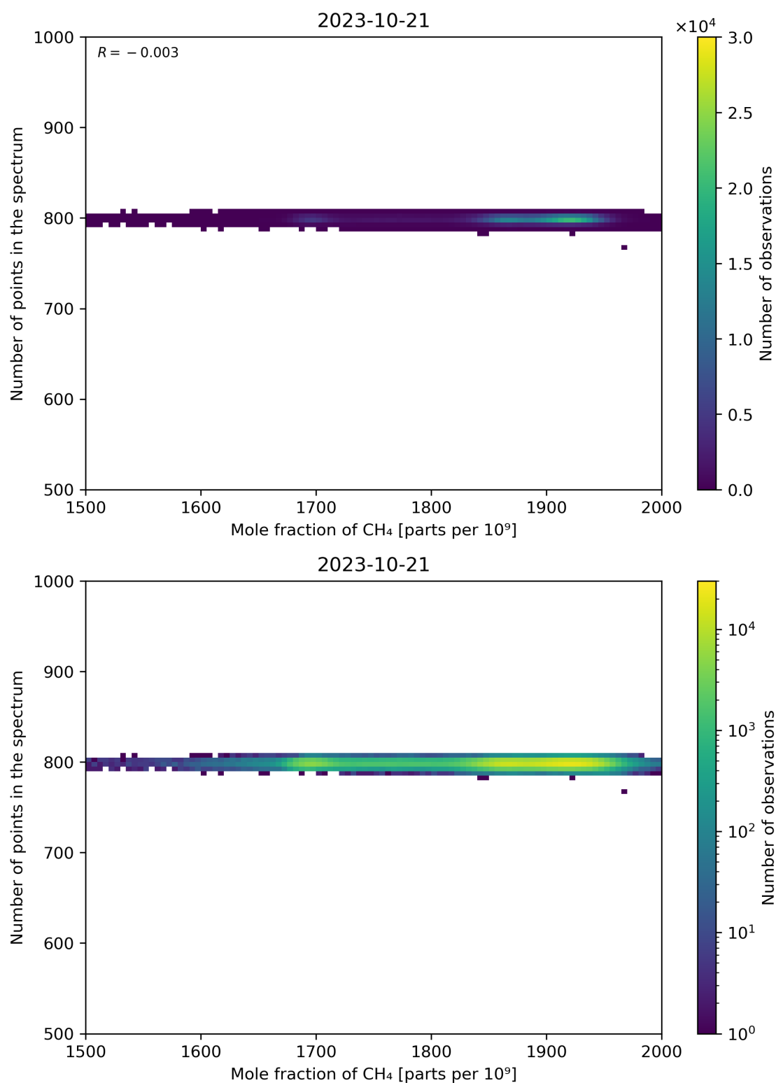
Figure 77: Scatter density plot of “Mole fraction of CH 4 ” against “Number of points in the spectrum” for 2023-10-20 to 2023-10-22.
