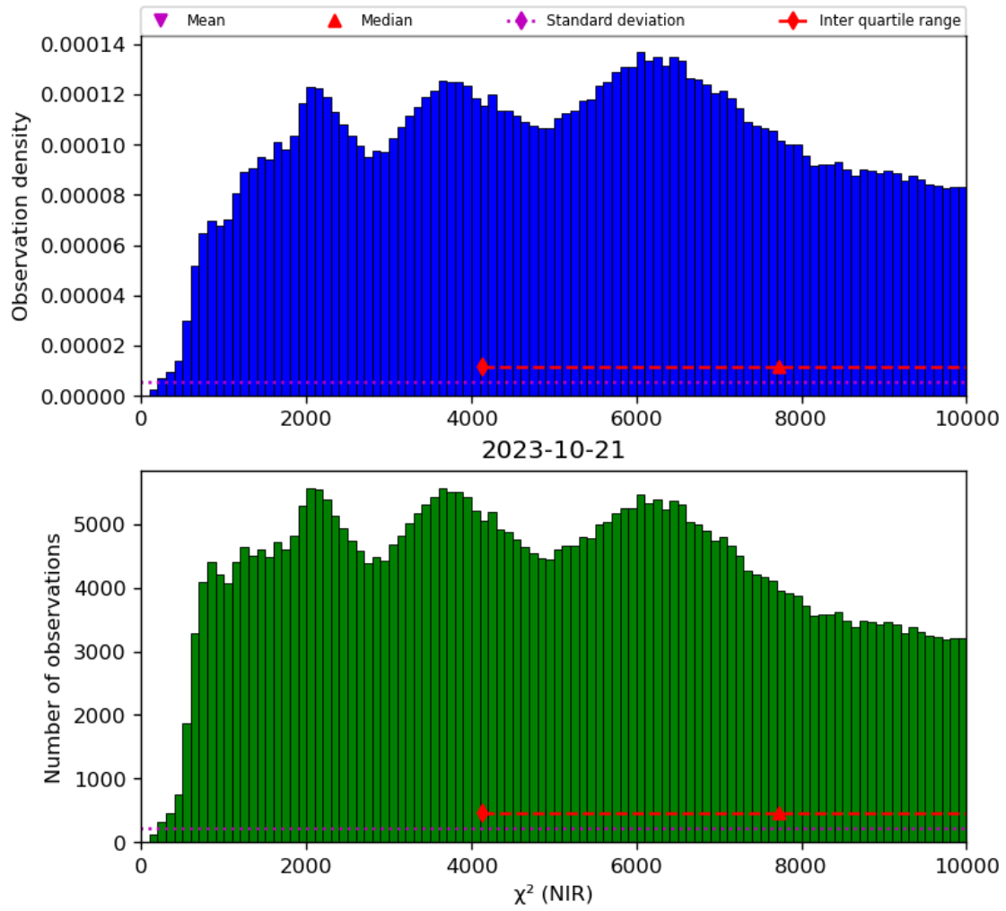
Figure 29: Histogram of “ \chi^2 (NIR)” for 2023-10-20 to 2023-10-22
