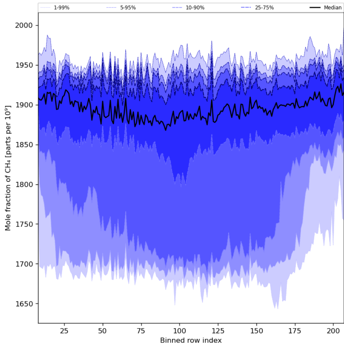
Figure 34: Along track statistics of “Mole fraction of CH 4 ” for 2023-10-20 to 2023-10-22
