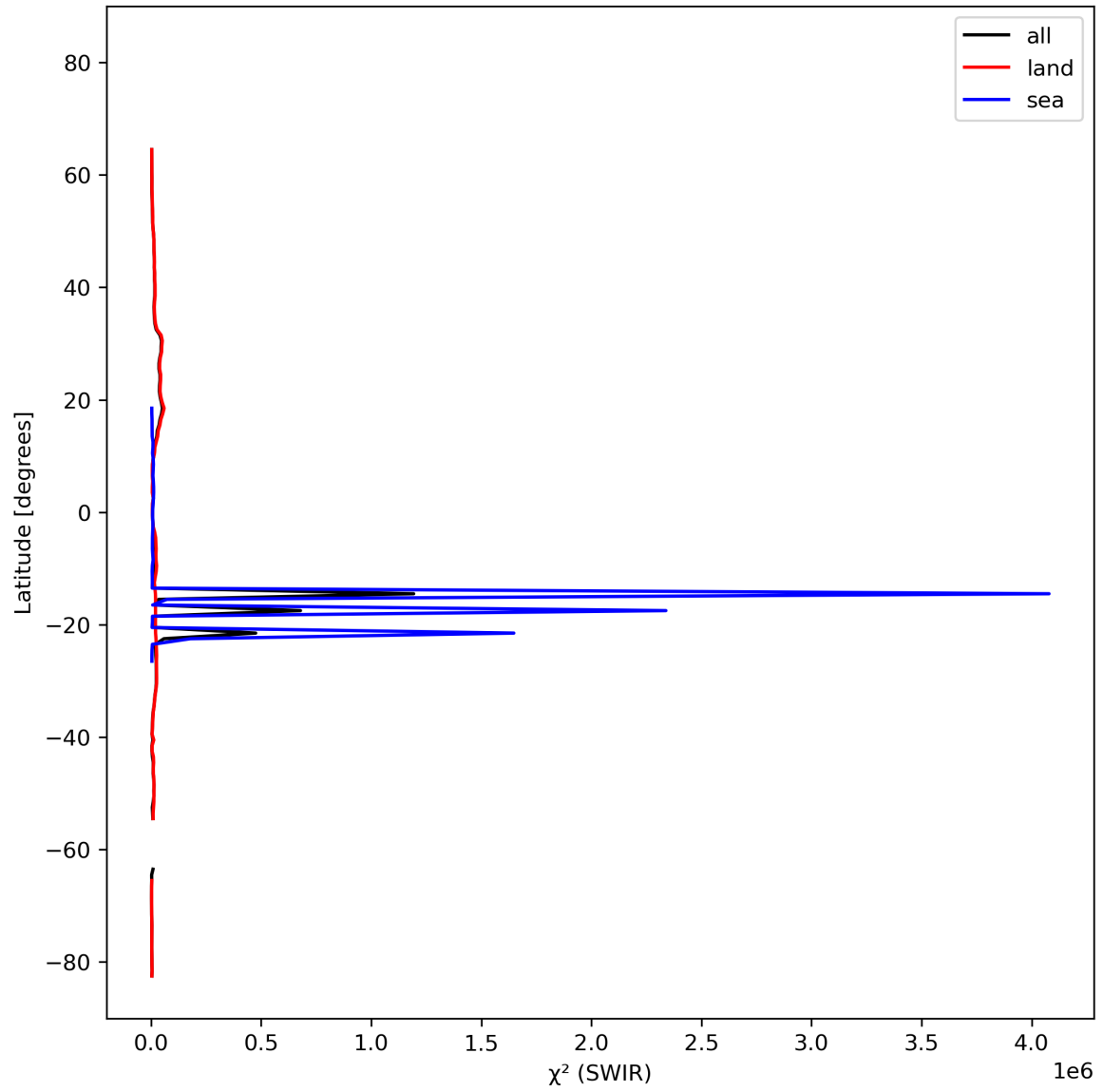
Figure 17: Zonal average of “ \chi^2 (SWIR)” for 2023-10-20 to 2023-10-22.
