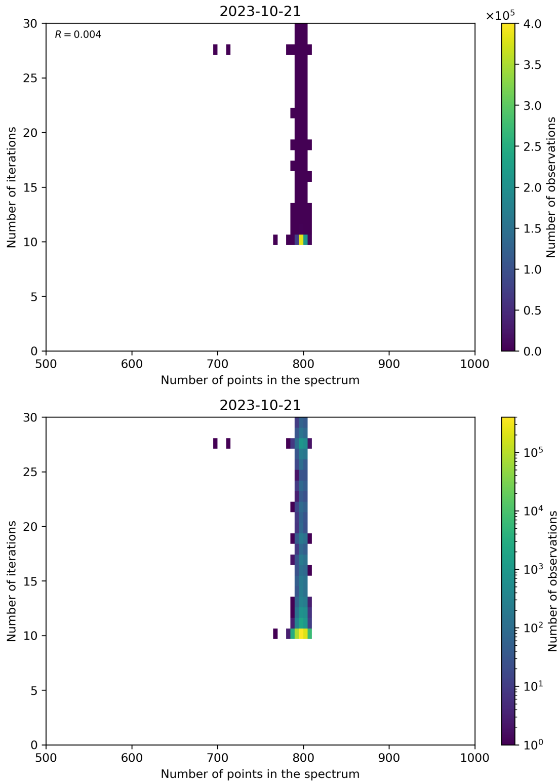
Figure 92: Scatter density plot of “Number of points in the spectrum” against “Number of iterations” for 2023-10-20 to 2023-10-22.
