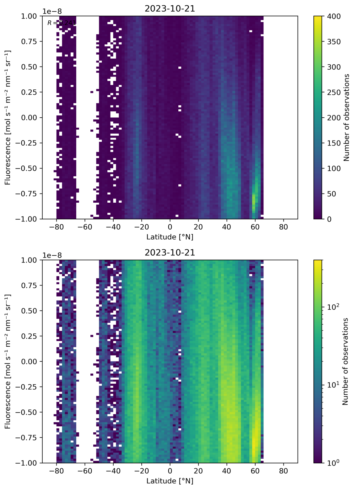
Figure 56: Scatter density plot of “Latitude” against “Fluorescence” for 2023-10-20 to 2023-10-22.
