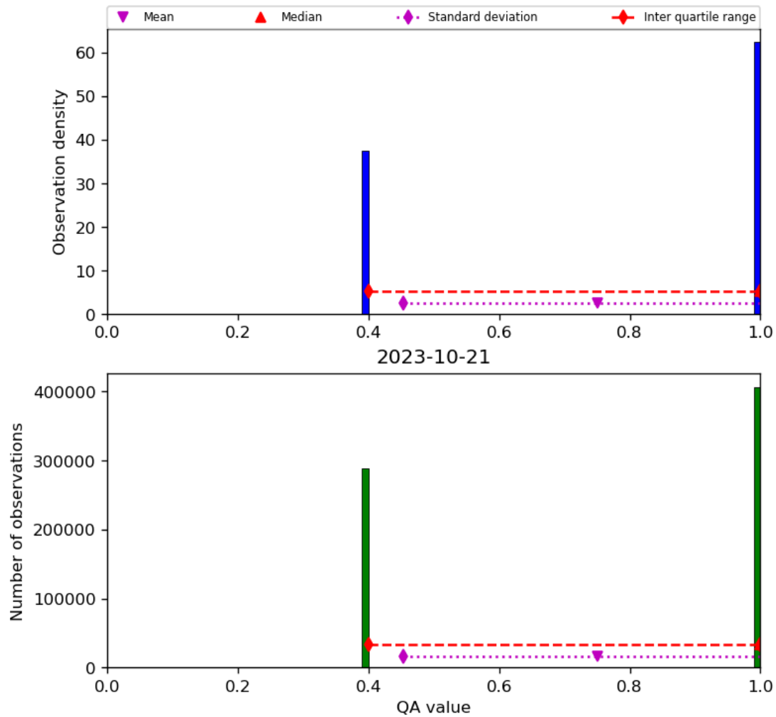
Figure 22: Histogram of “QA value” for 2023-10-20 to 2023-10-22
