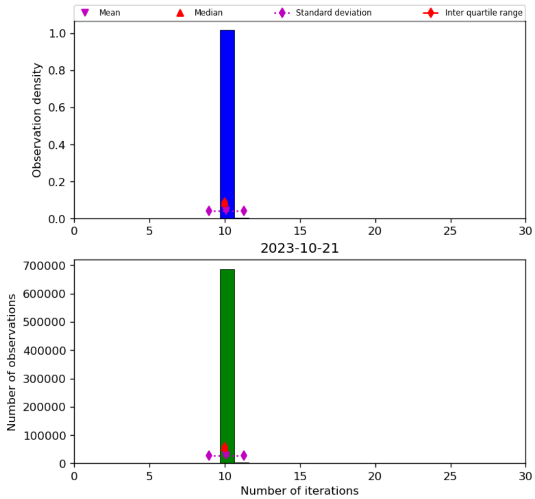
Figure 31: Histogram of “Number of iterations” for 2023-10-20 to 2023-10-22
