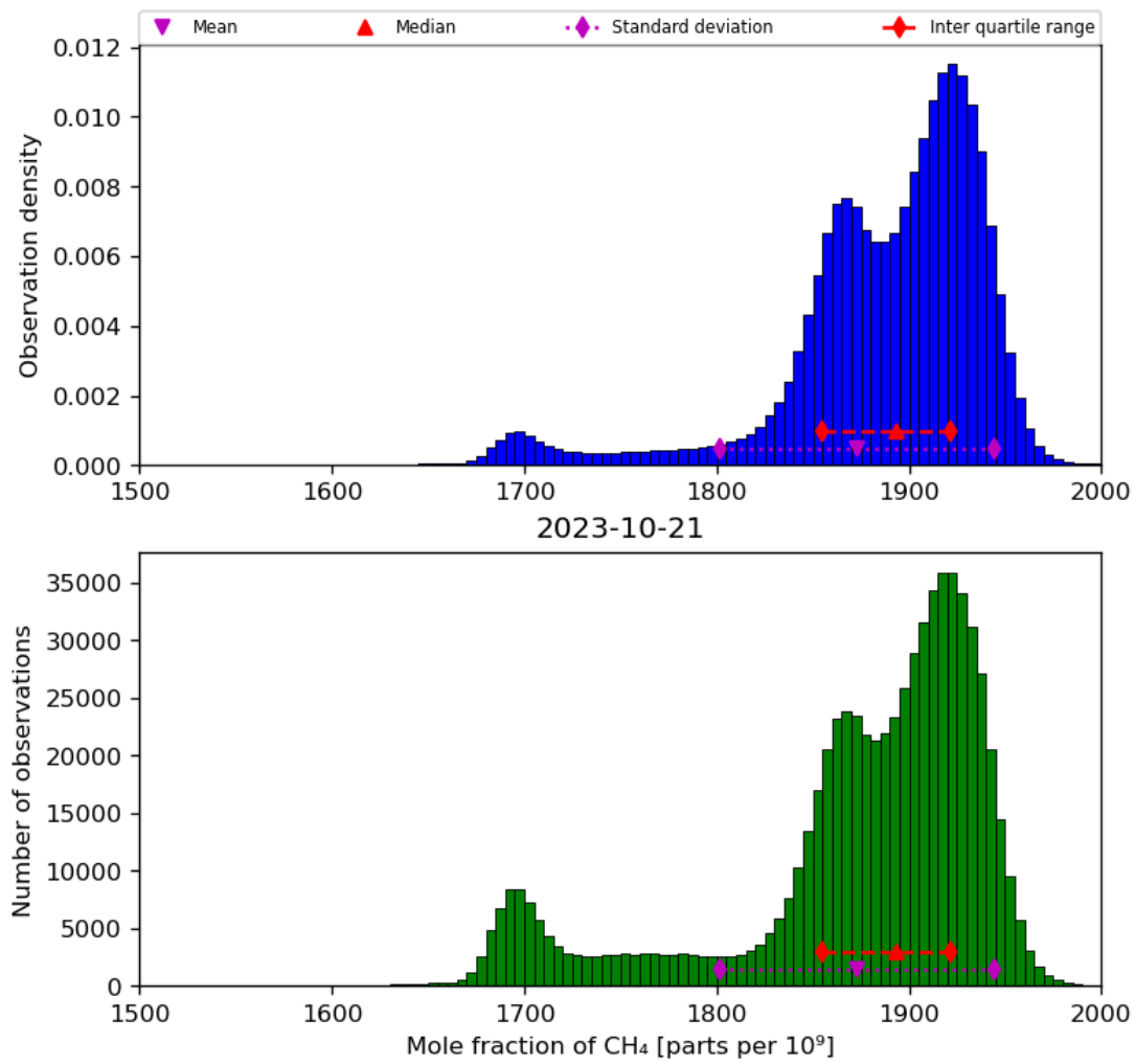
Figure 23: Histogram of “Mole fraction of CH 4 ” for 2023-10-20 to 2023-10-22
