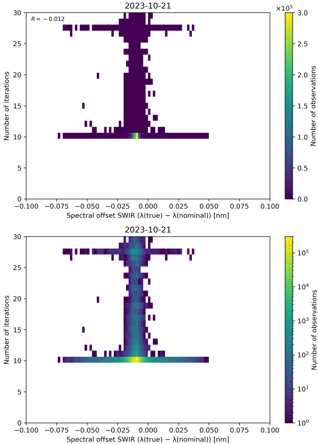
Figure 121: Scatter density plot of “Spectral offset SWIR ( \lambda(\text{true}) - \lambda(\text{nominal}) )” against “Number of iterations” for 2023-10-20 to 2023-10-22.
