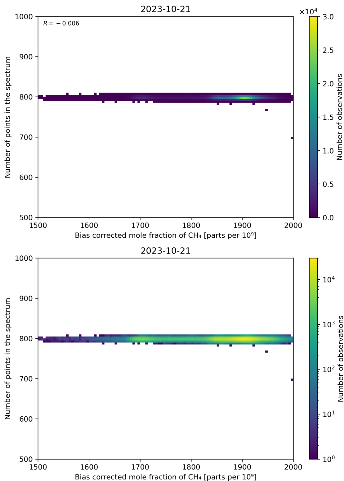
Figure 68: Scatter density plot of “Bias corrected mole fraction of CH 4 ” against “Number of points in the spectrum” for 2023-10-20 to 2023-10-22.
