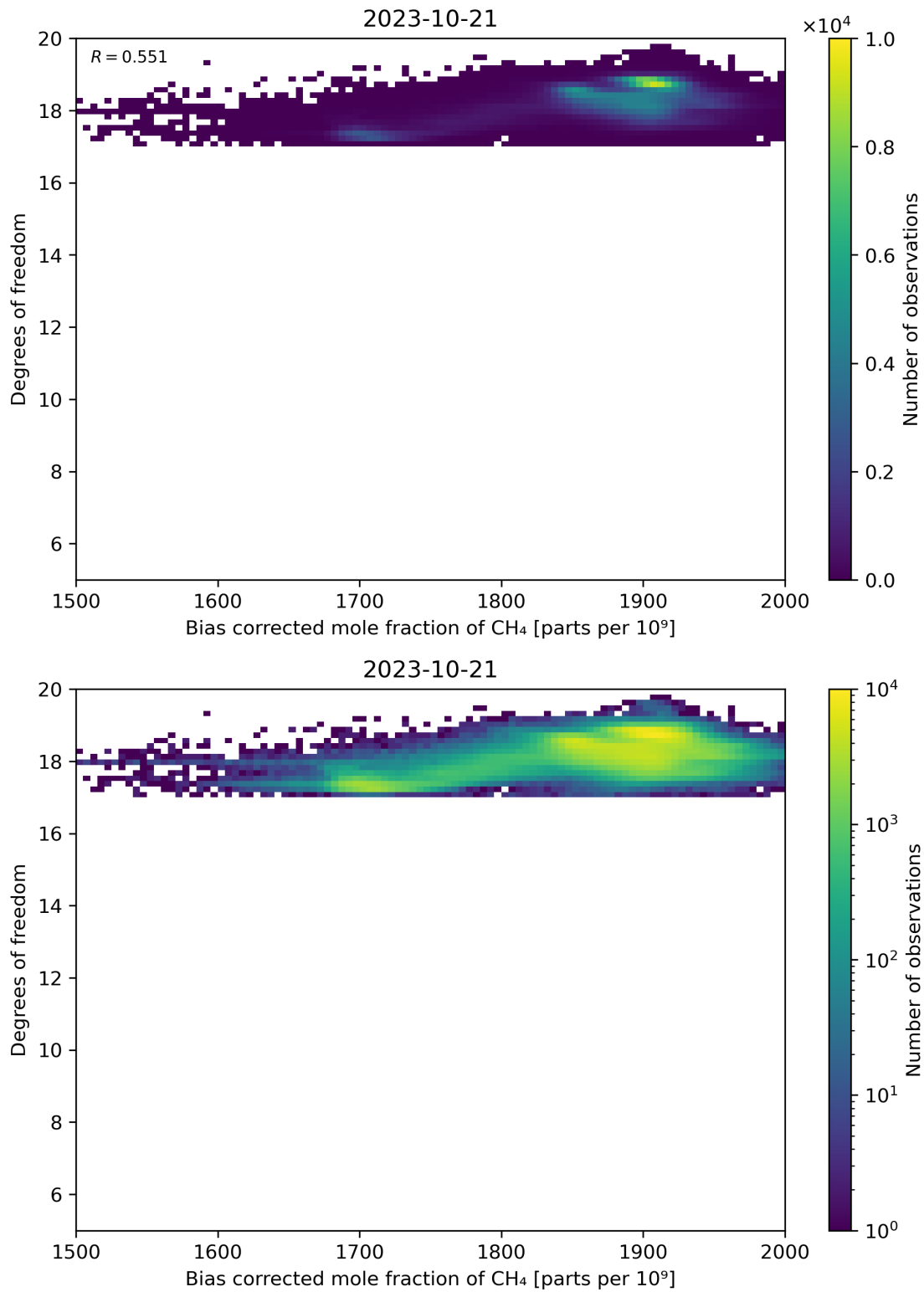
Figure 65: Scatter density plot of “Bias corrected mole fraction of CH 4 ” against “Degrees of freedom” for 2023-10-20 to 2023-10-22.
