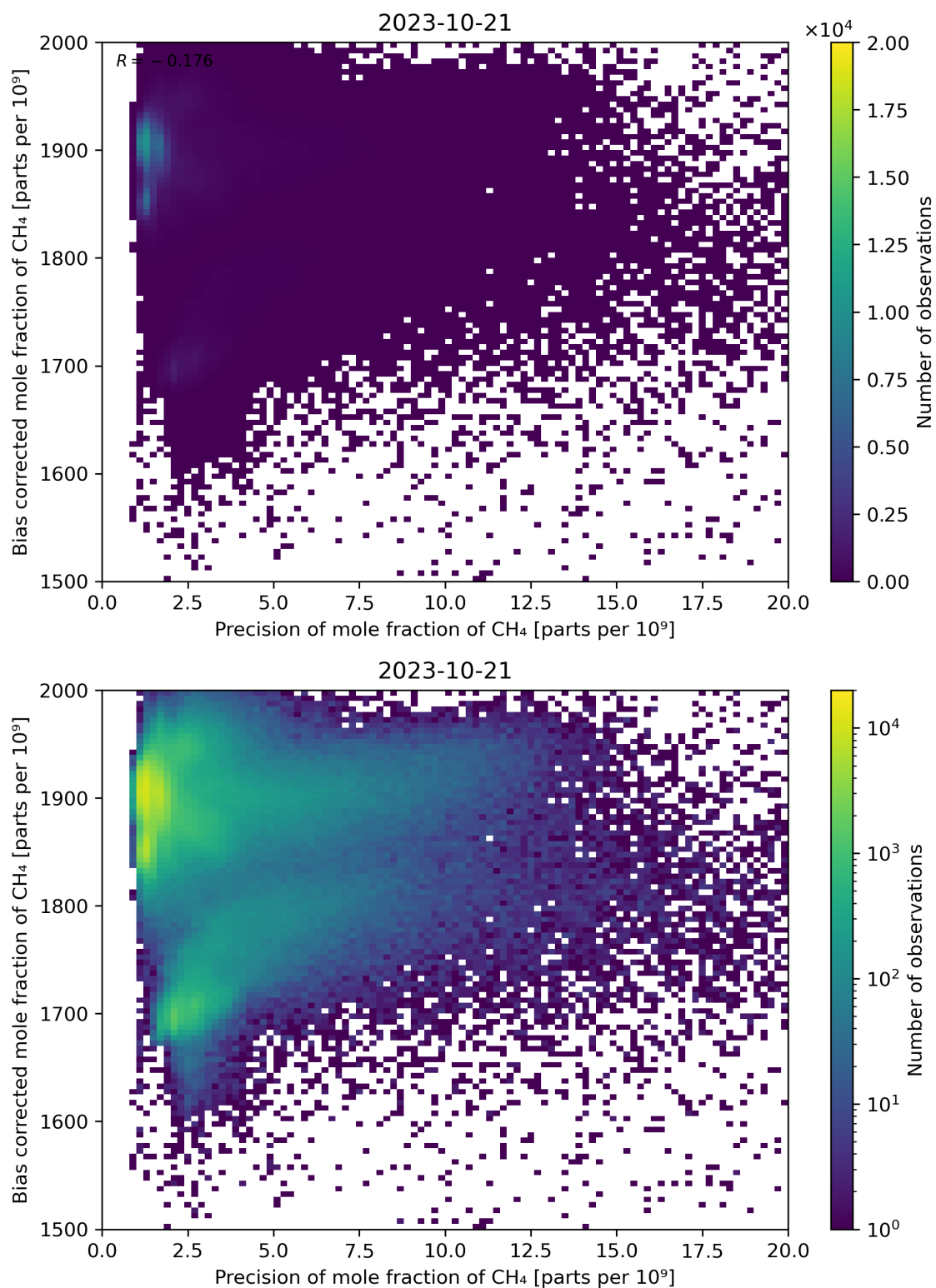
Figure 82: Scatter density plot of “Precision of mole fraction of CH 4 ” against “Bias corrected mole fraction of CH 4 ” for 2023-10-20 to 2023-10-22.
