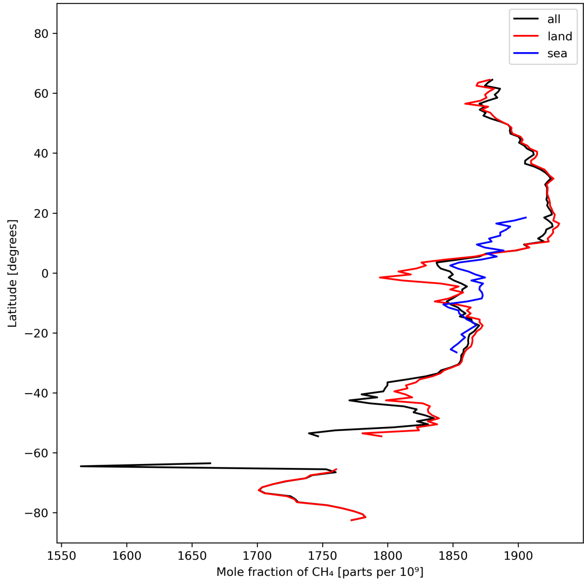
Figure 12: Zonal average of “Mole fraction of CH 4 ” for 2023-10-20 to 2023-10-22.
