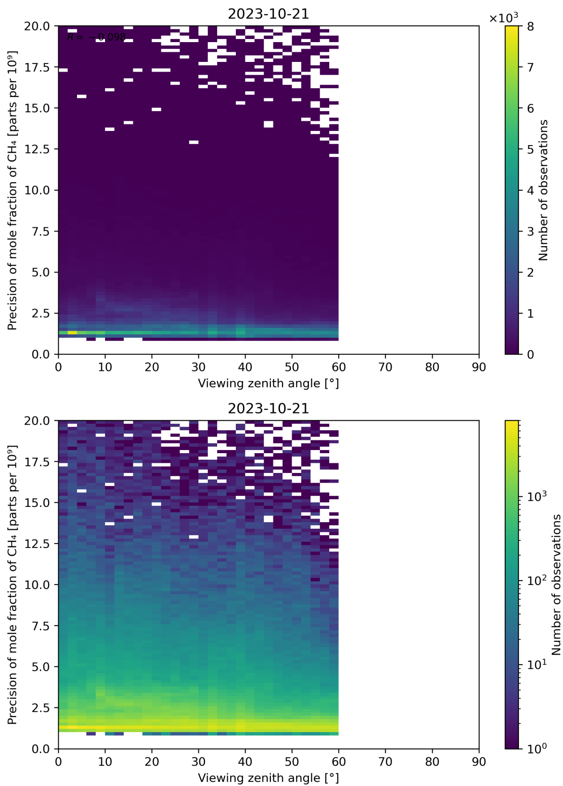
Figure 112: Scatter density plot of “Viewing zenith angle” against “Precision of mole fraction of CH 4 ” for 2023-10-20 to 2023-10-22.
