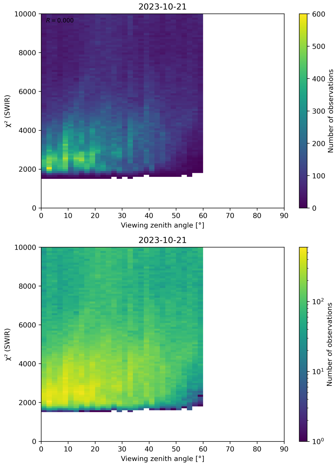
Figure 106: Scatter density plot of “Viewing zenith angle” against “ \chi^2 (SWIR)” for 2023-10-20 to 2023-10-22.
