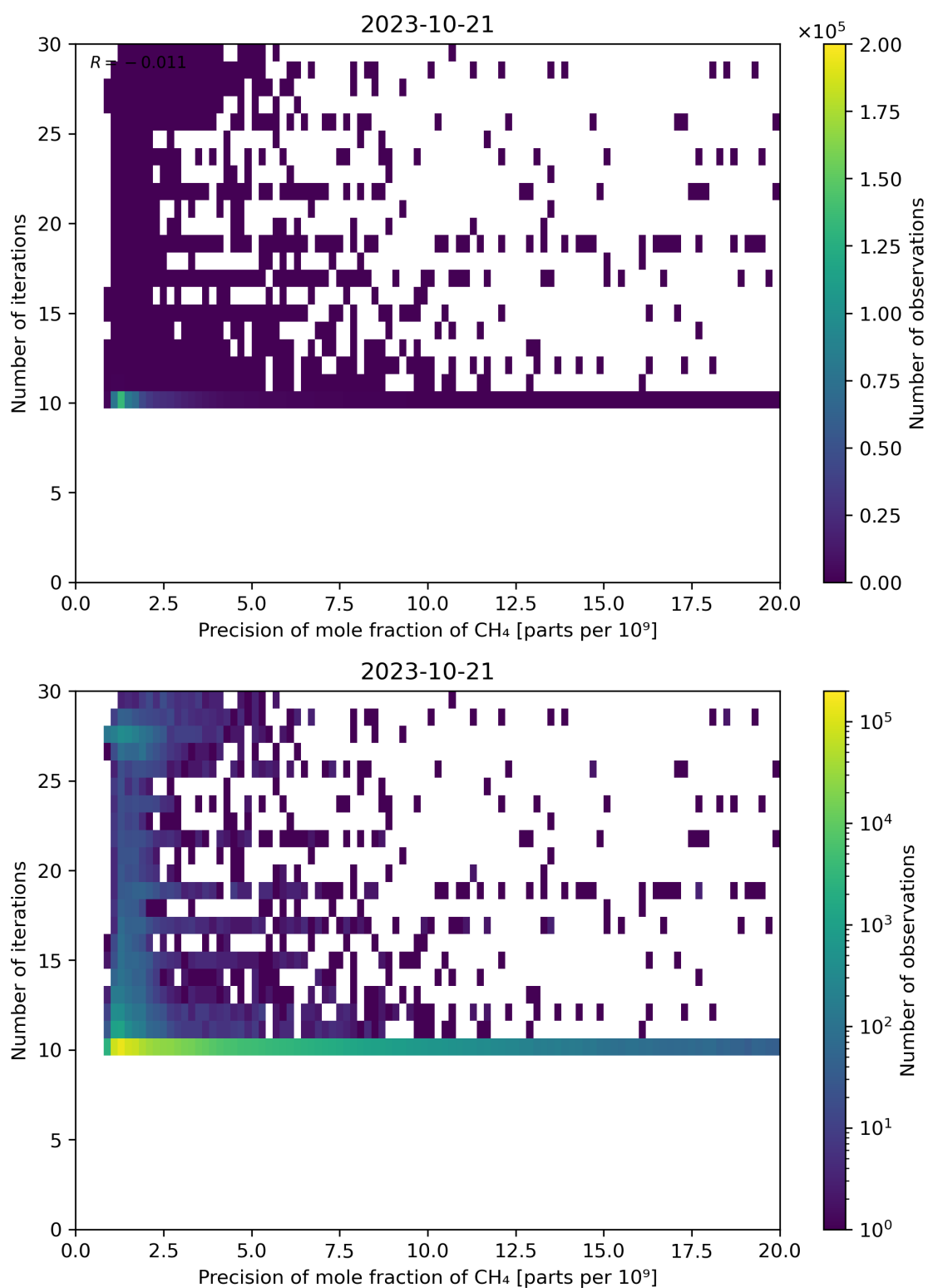
Figure 83: Scatter density plot of “Precision of mole fraction of CH 4 ” against “Number of iterations” for 2023-10-20 to 2023-10-22.
