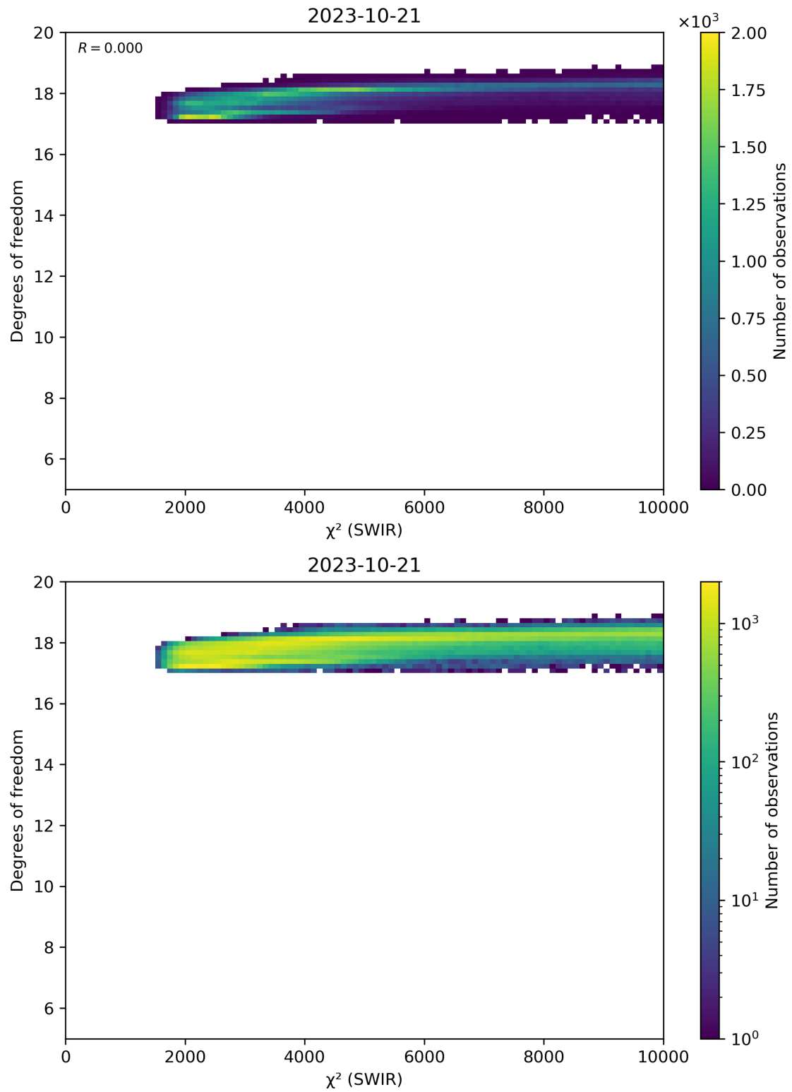
Figure 48: Scatter density plot of “ \chi^2 (SWIR)” against “Degrees of freedom” for 2023-10-20 to 2023-10-22.
