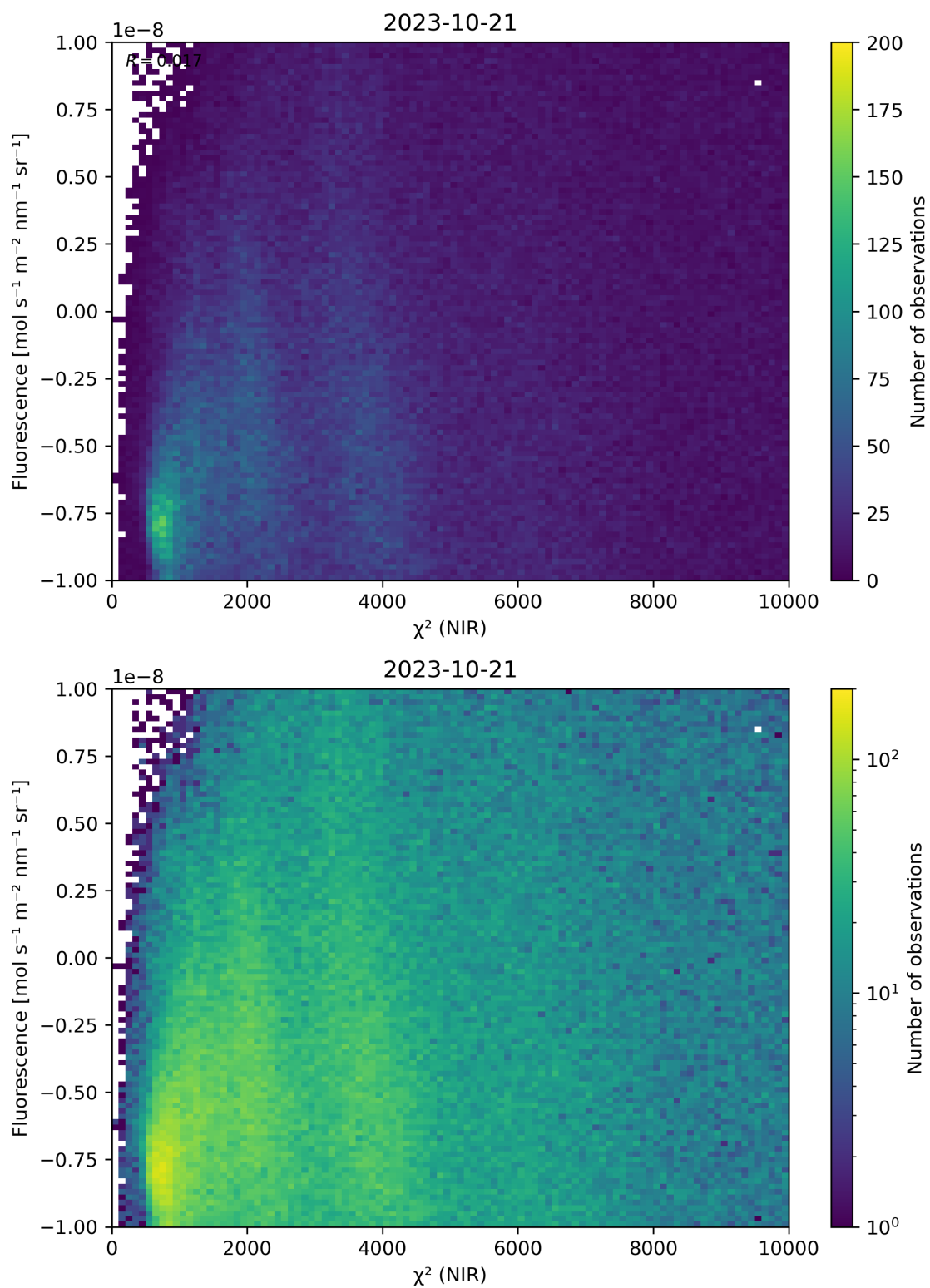
Figure 45: Scatter density plot of “ \chi^2 (NIR)” against “Fluorescence” for 2023-10-20 to 2023-10-22.
