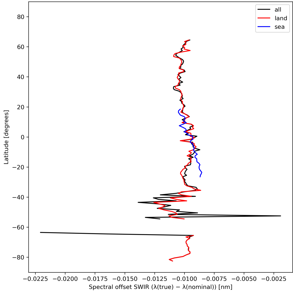
Figure 16: Zonal average of “Spectral offset SWIR ( \lambda(\text{true}) - \lambda(\text{nominal}) )” for 2023-10-20 to 2023-10-22.
