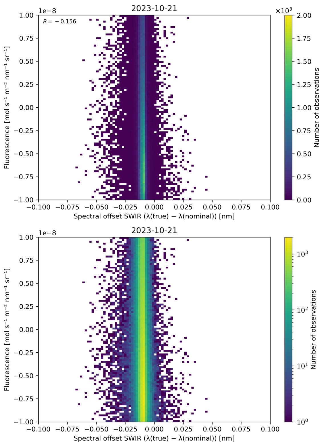
Figure 120: Scatter density plot of “Spectral offset SWIR ( \lambda(\text{true}) - \lambda(\text{nominal}) )” against “Fluorescence” for 2023-10-20 to 2023-10-22.
