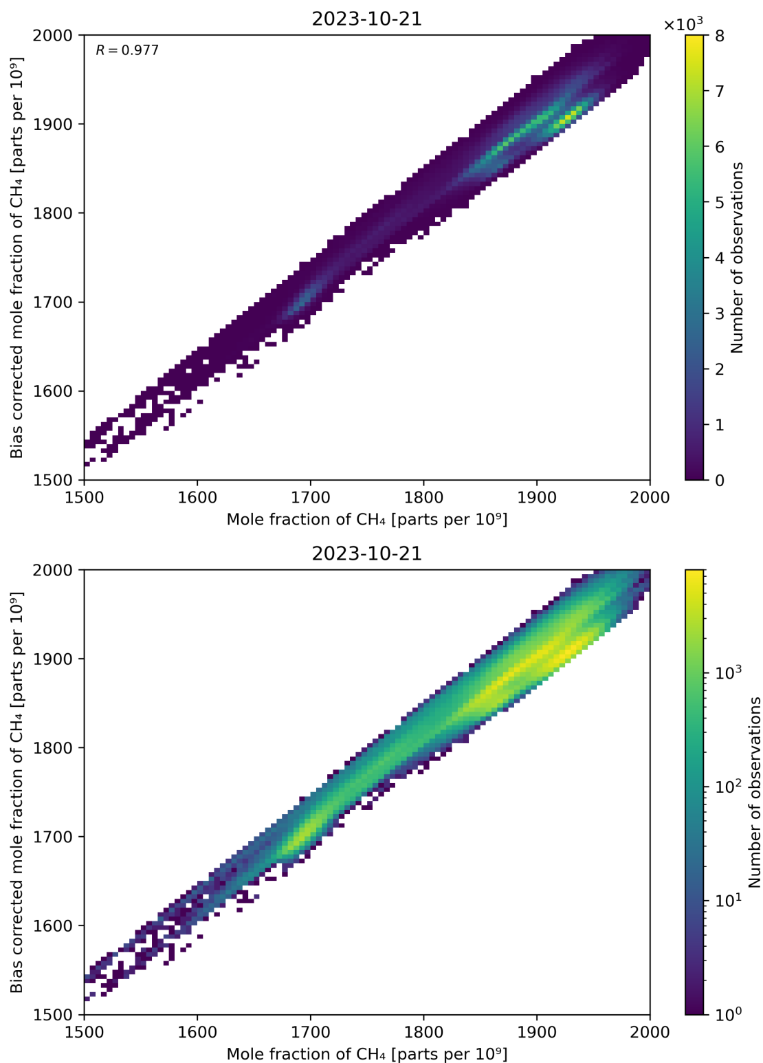
Figure 74: Scatter density plot of “Mole fraction of CH 4 ” against “Bias corrected mole fraction of CH 4 ” for 2023-10-20 to 2023-10-22.
