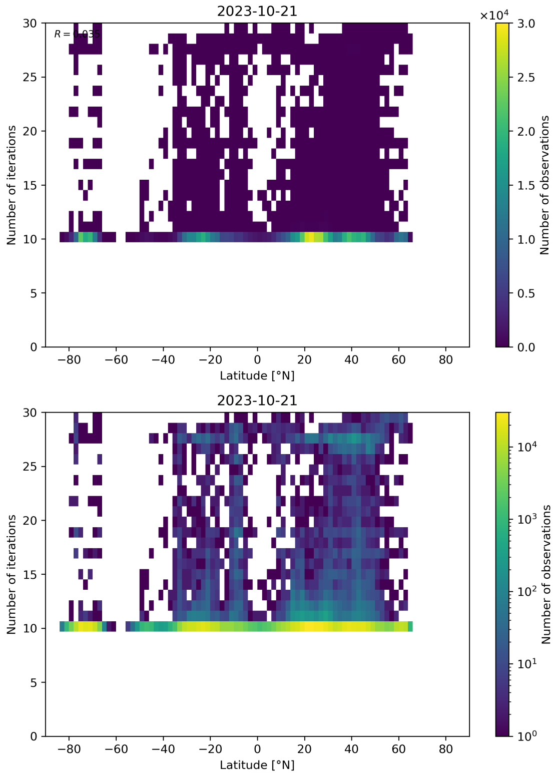
Figure 60: Scatter density plot of “Latitude” against “Number of iterations” for 2023-10-20 to 2023-10-22.
