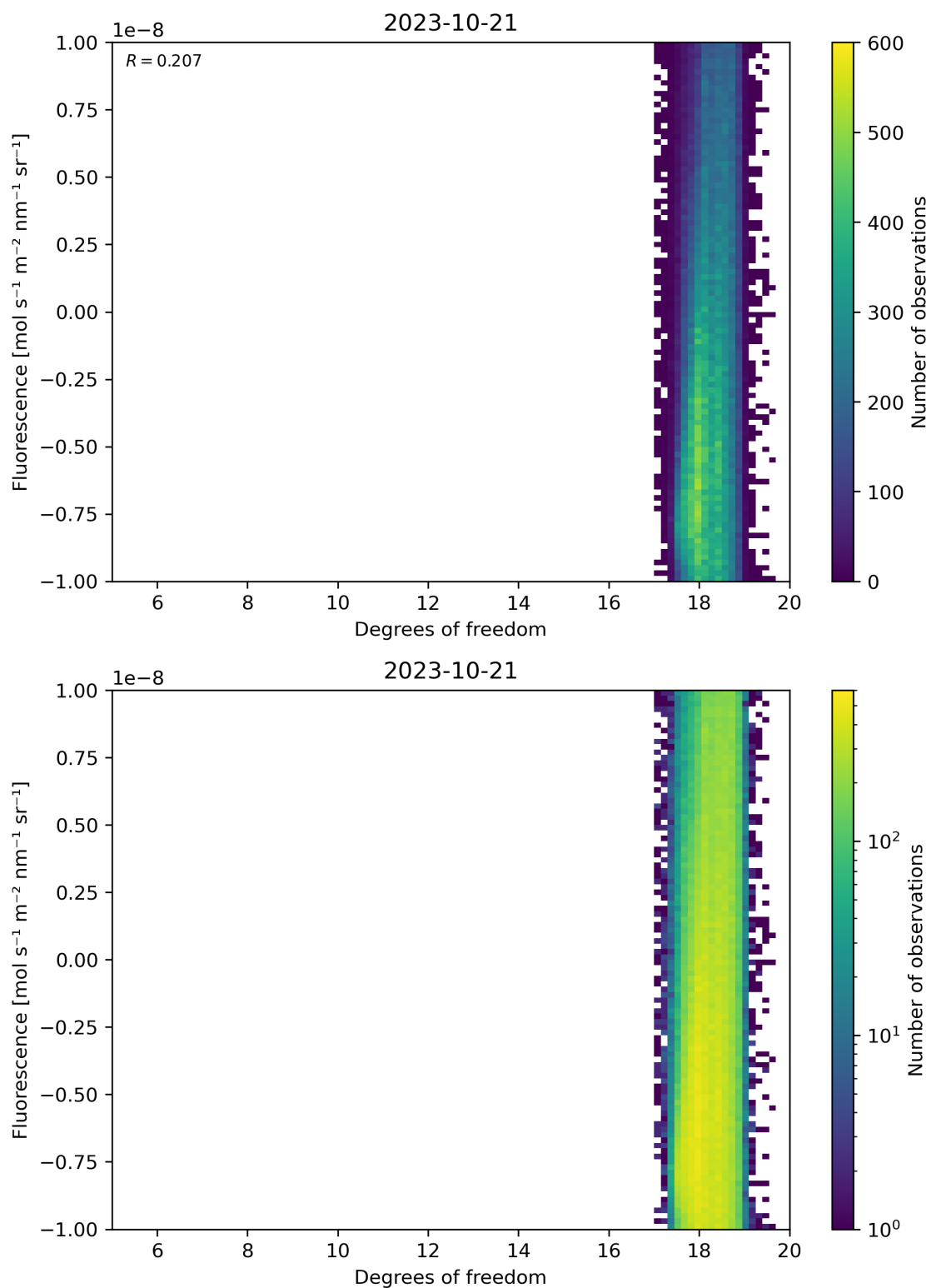
Figure 51: Scatter density plot of “Degrees of freedom” against “Fluorescence” for 2023-10-20 to 2023-10-22.
