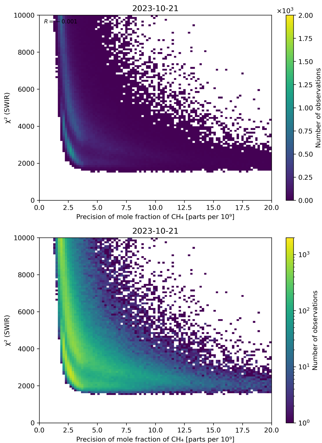
Figure 79: Scatter density plot of “Precision of mole fraction of \text{CH}_4 ” against “ \chi^2 (SWIR)” for 2023-10-20 to 2023-10-22.
