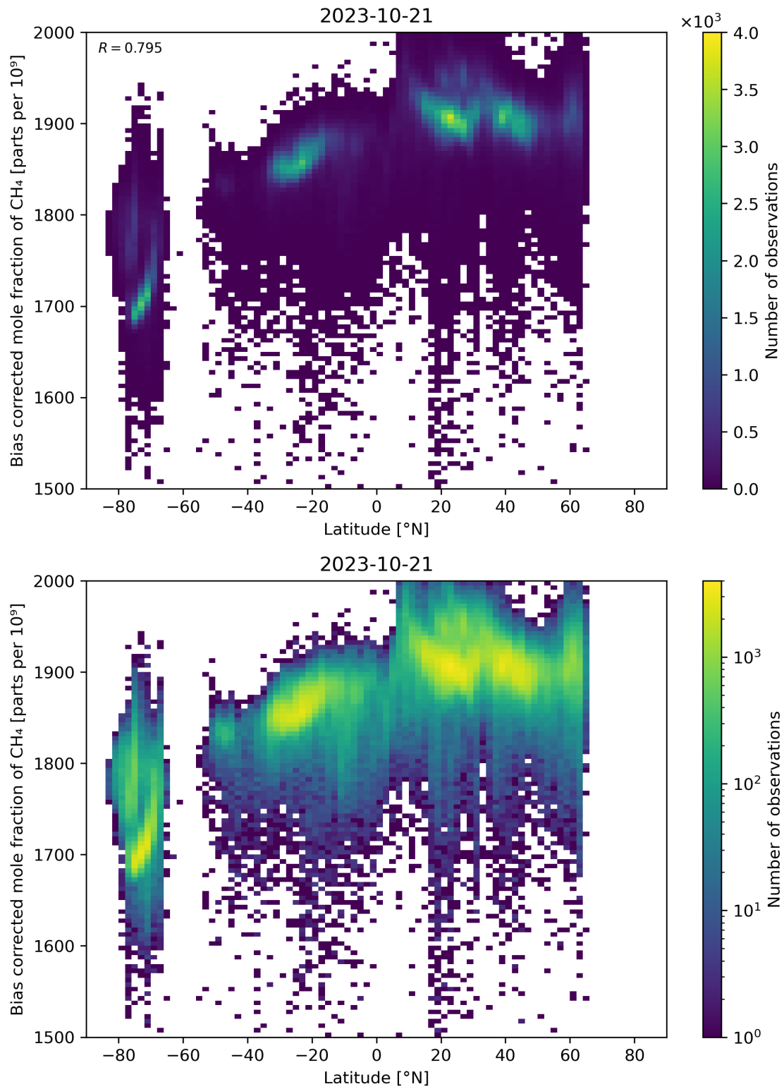
Figure 58: Scatter density plot of “Latitude” against “Bias corrected mole fraction of \text{CH}_4 ” for 2023-10-20 to 2023-10-22.
