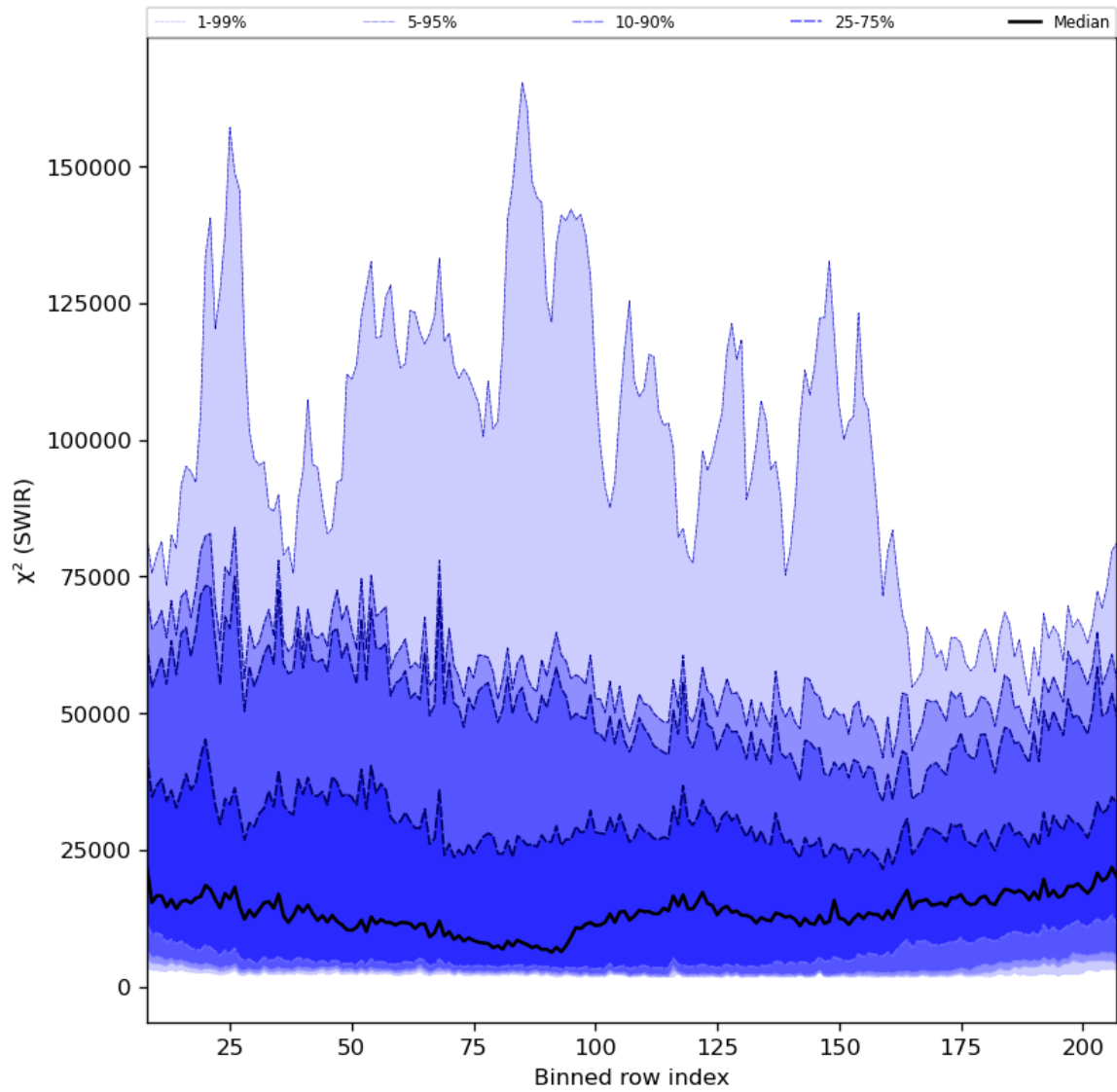
Figure 39: Along track statistics of " \chi^2 (SWIR)" for 2023-10-20 to 2023-10-22
