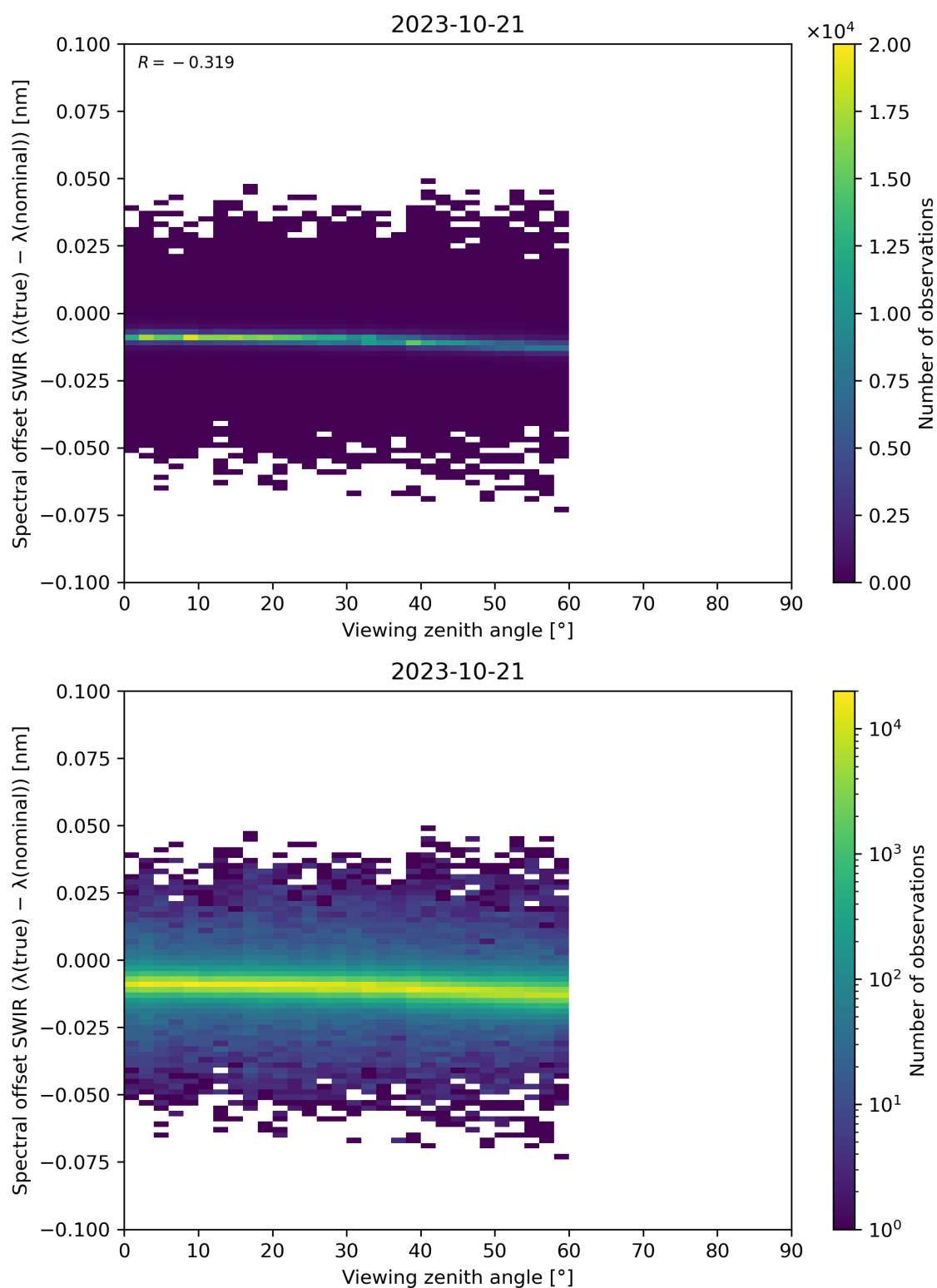
Figure 116: Scatter density plot of “Viewing zenith angle” against “Spectral offset SWIR ( \lambda(\text{true}) - \lambda(\text{nominal}) )” for 2023-10-20 to 2023-10-22.
