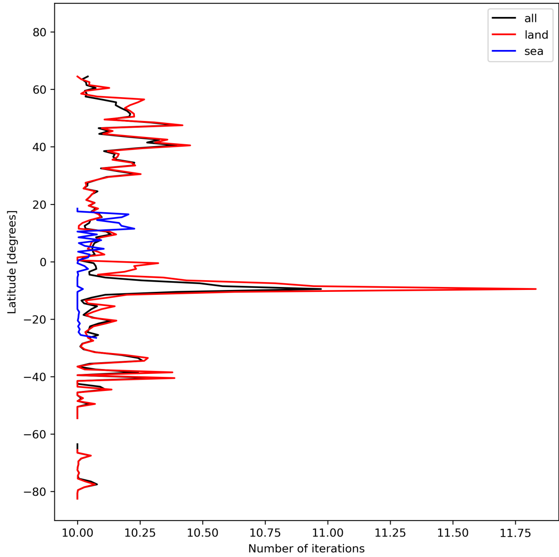
Figure 20: Zonal average of “Number of iterations” for 2023-10-20 to 2023-10-22.
