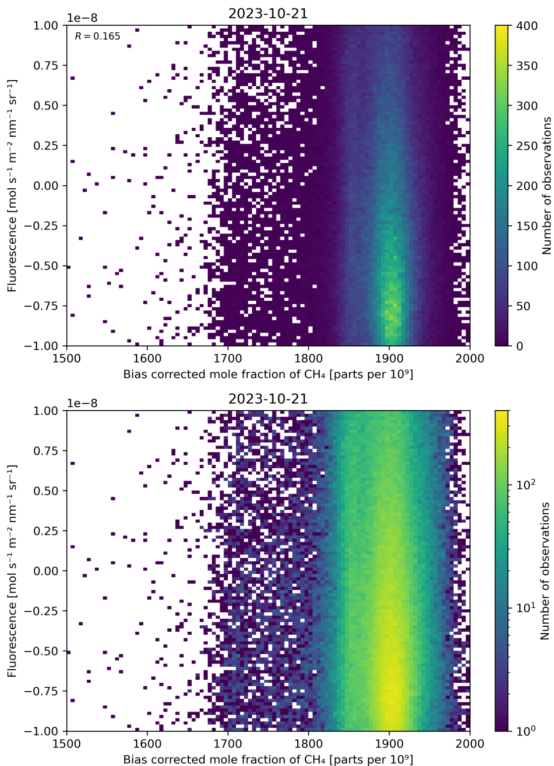
Figure 66: Scatter density plot of “Bias corrected mole fraction of \text{CH}_4 ” against “Fluorescence” for 2023-10-20 to 2023-10-22.
