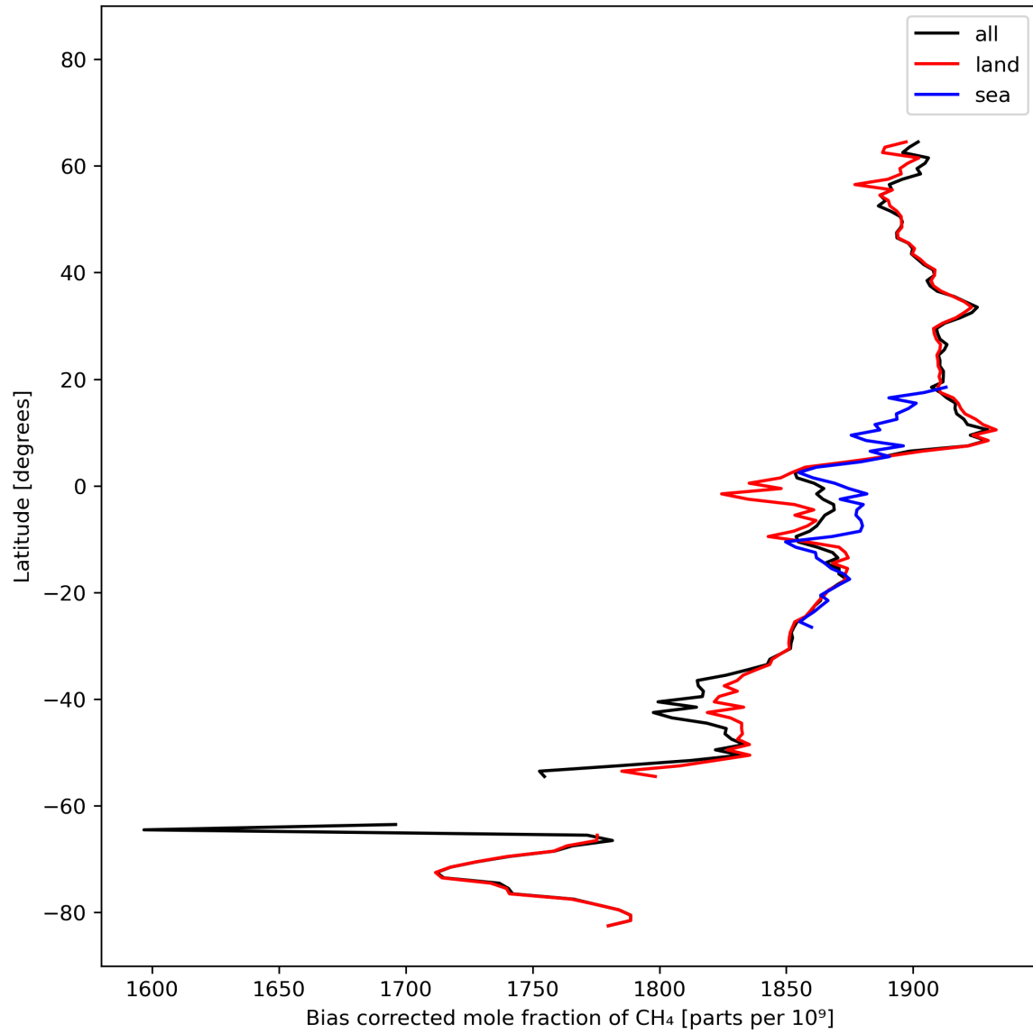
Figure 14: Zonal average of “Bias corrected mole fraction of CH 4 ” for 2023-10-20 to 2023-10-22.
