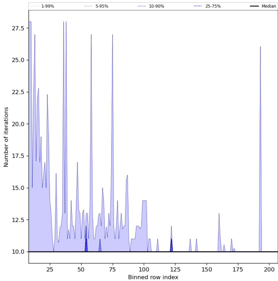
Figure 42: Along track statistics of “Number of iterations” for 2023-10-20 to 2023-10-22
