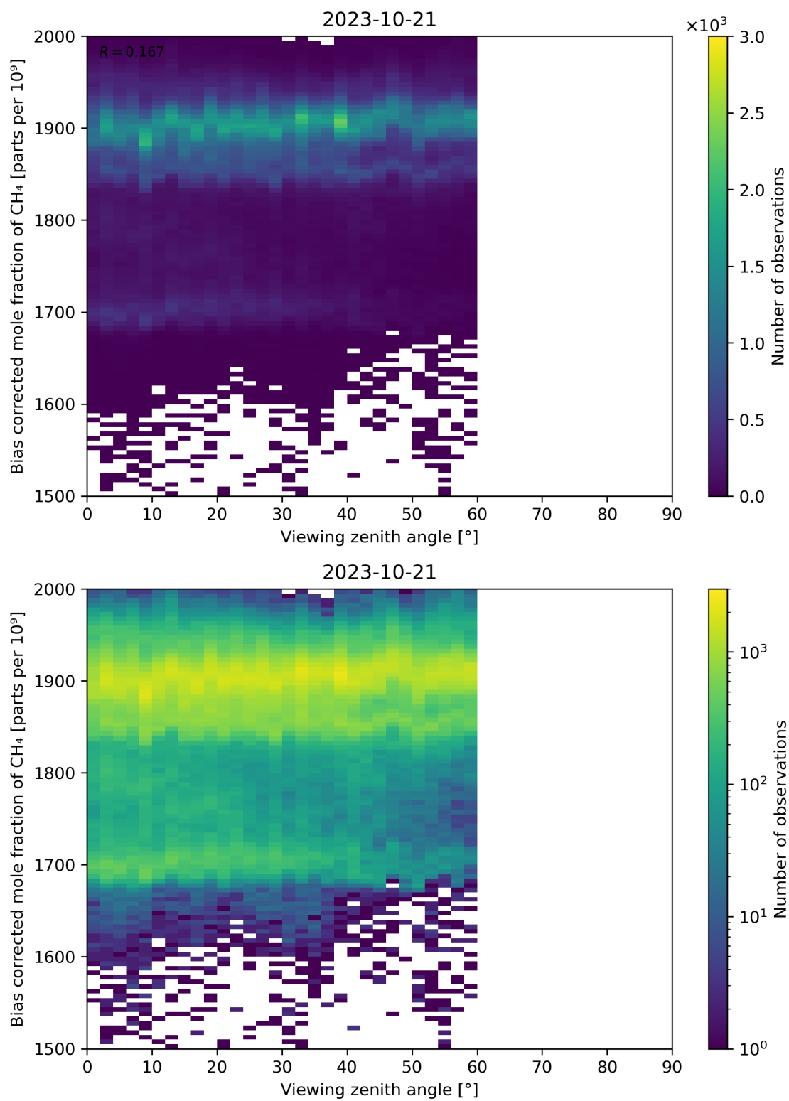
Figure 111: Scatter density plot of “Viewing zenith angle” against “Bias corrected mole fraction of CH 4 ” for 2023-10-20 to 2023-10-22.
