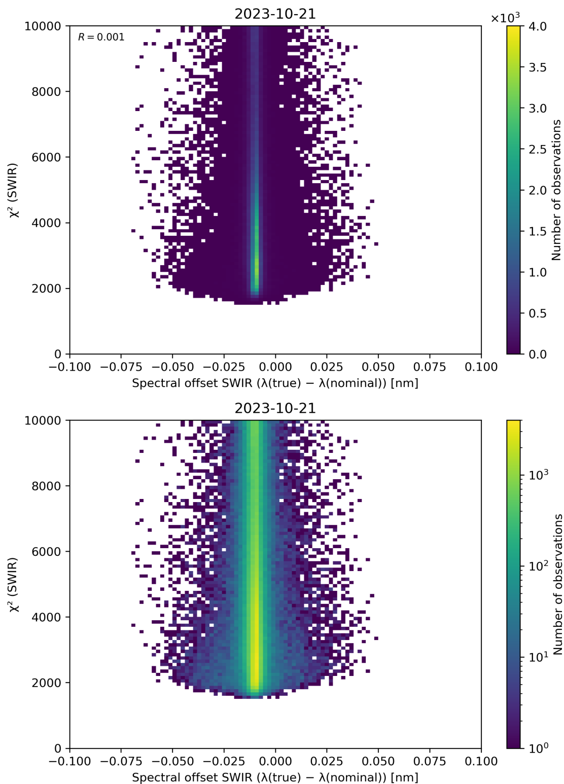
Figure 118: Scatter density plot of “Spectral offset SWIR ( \lambda(\text{true}) - \lambda(\text{nominal}) )” against “ \chi^2 (SWIR)” for 2023-10-20 to 2023-10-22.
