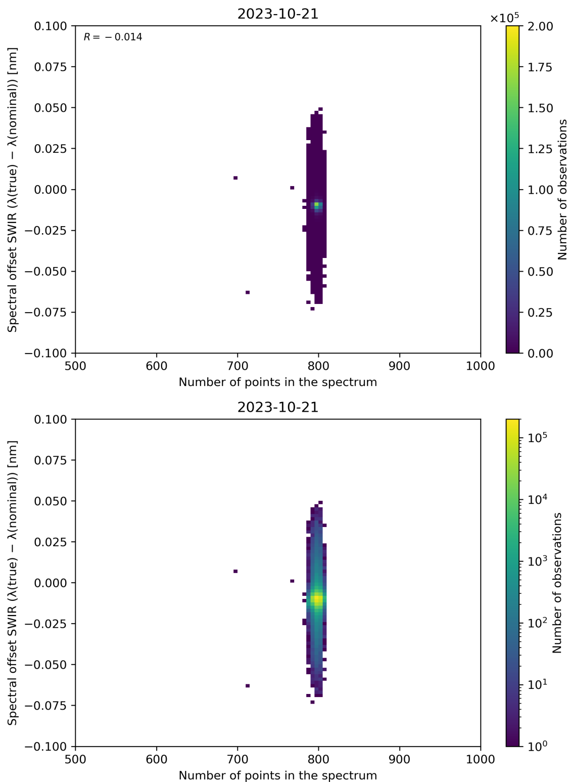
Figure 93: Scatter density plot of “Number of points in the spectrum” against “Spectral offset SWIR ( \lambda(\text{true}) - \lambda(\text{nominal}) )” for 2023-10-20 to 2023-10-22.
