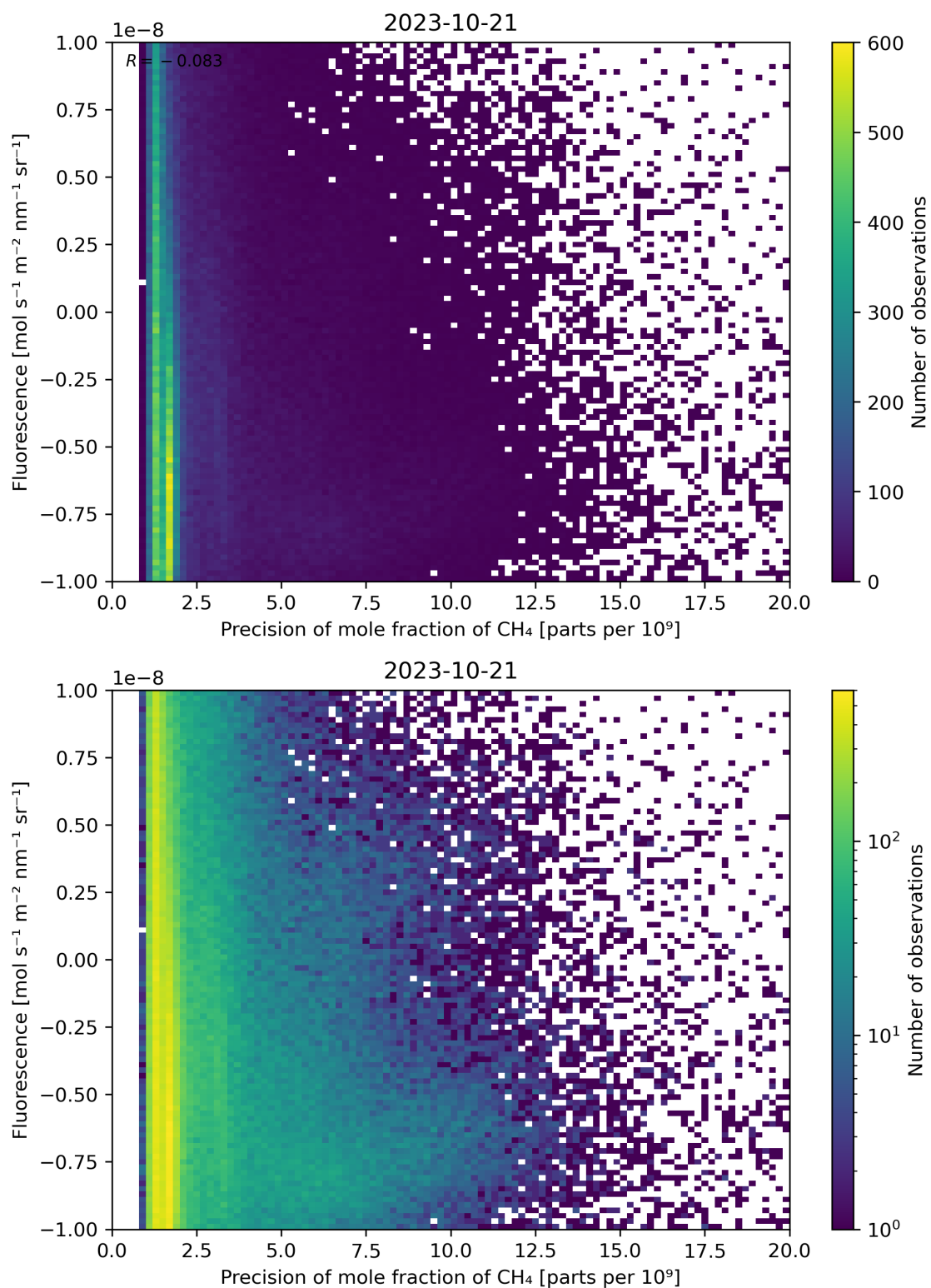
Figure 81: Scatter density plot of “Precision of mole fraction of \text{CH}_4 ” against “Fluorescence” for 2023-10-20 to 2023-10-22.
