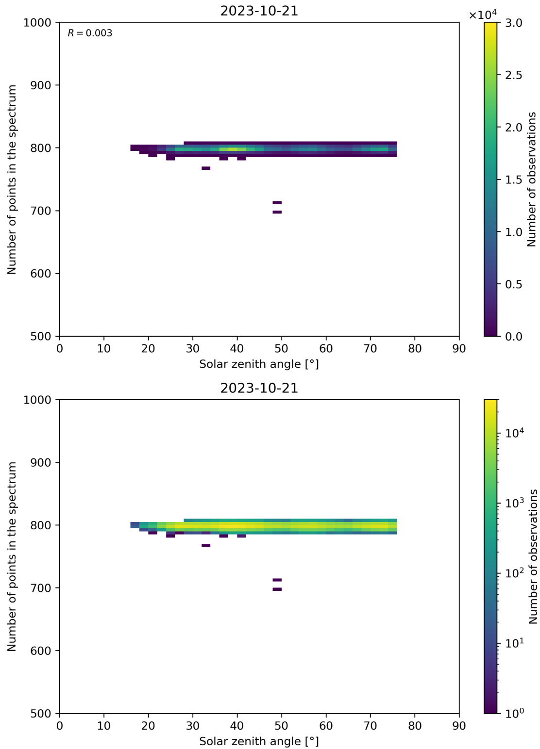
Figure 103: Scatter density plot of “Solar zenith angle” against “Number of points in the spectrum” for 2023-10-20 to 2023-10-22.
