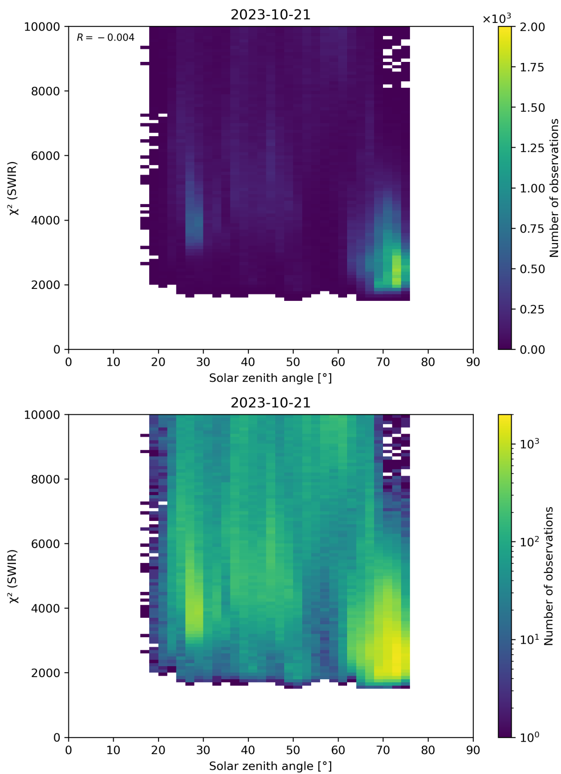
Figure 95: Scatter density plot of “Solar zenith angle” against “ \chi^2 (SWIR)” for 2023-10-20 to 2023-10-22.
