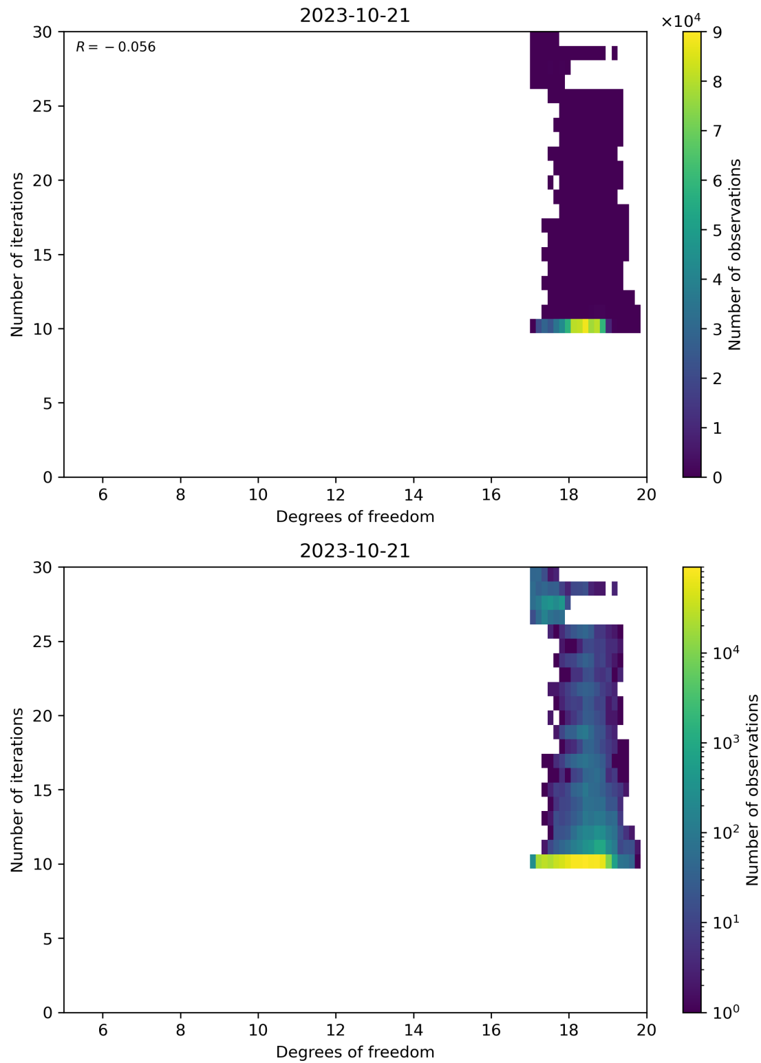
Figure 52: Scatter density plot of “Degrees of freedom” against “Number of iterations” for 2023-10-20 to 2023-10-22.
