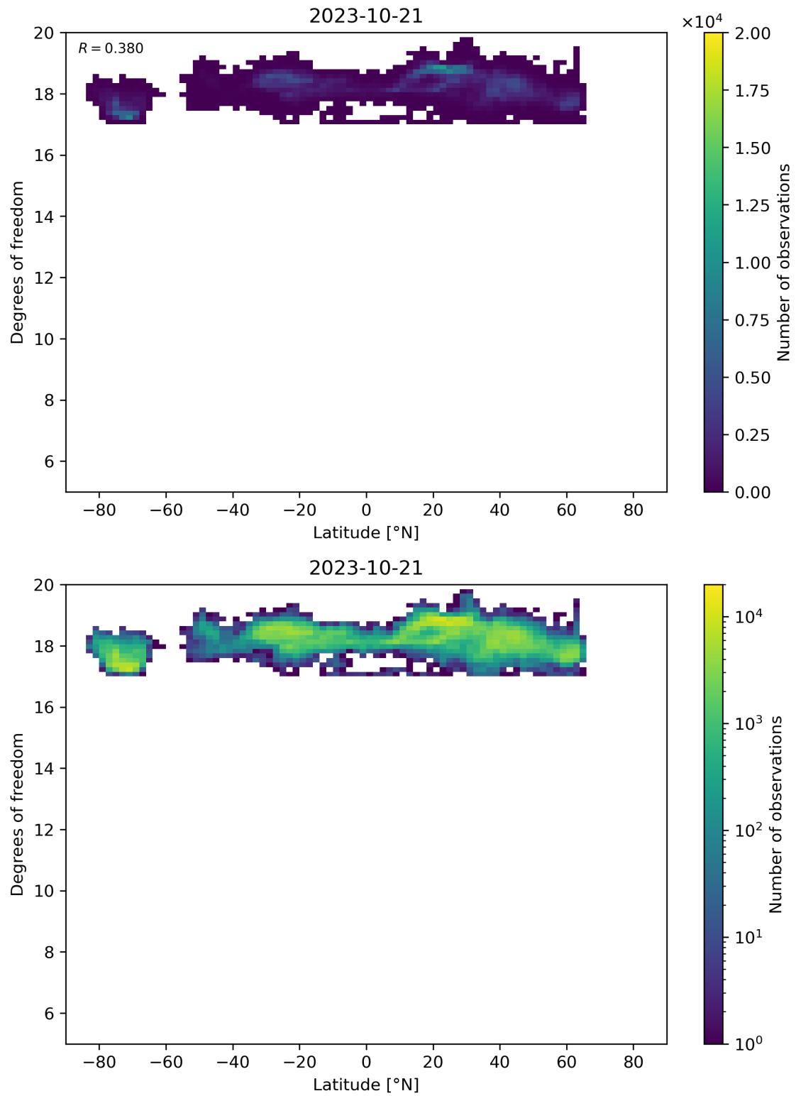
Figure 55: Scatter density plot of “Latitude” against “Degrees of freedom” for 2023-10-20 to 2023-10-22.
