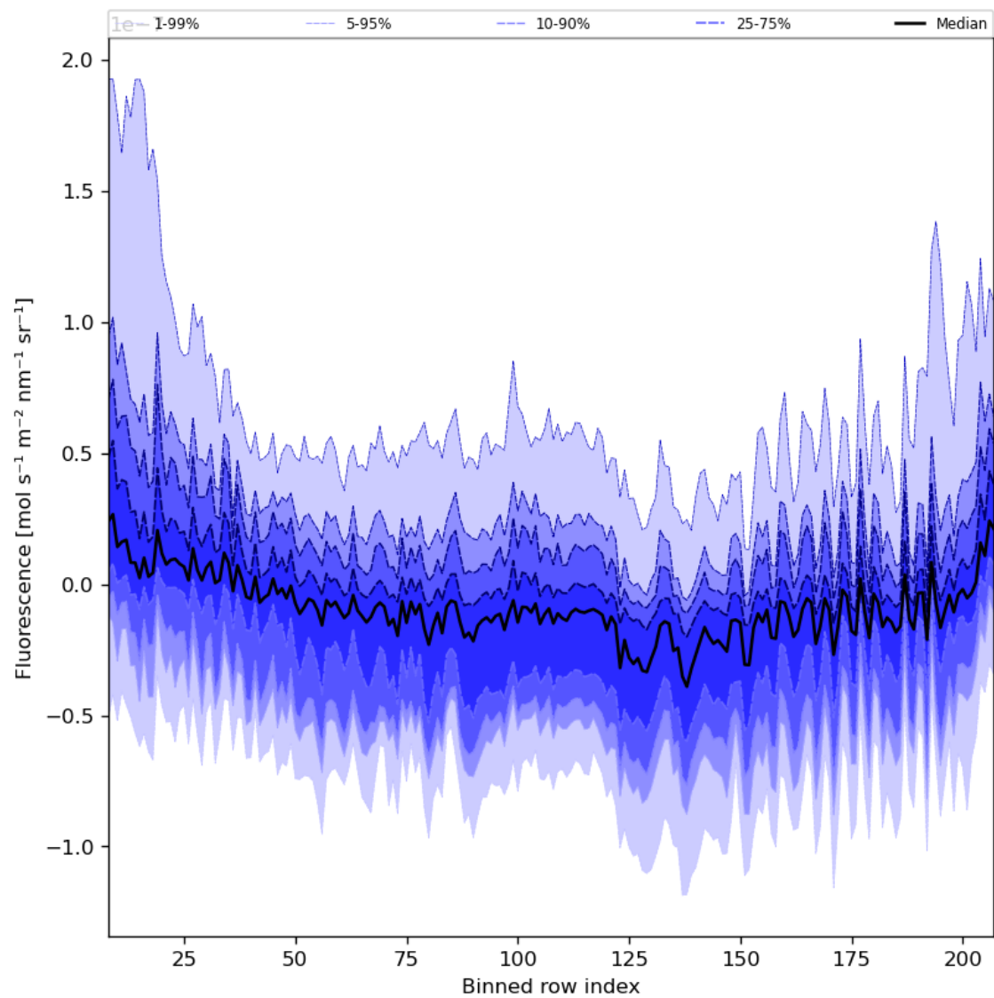
Figure 43: Along track statistics of “Fluorescence” for 2023-10-20 to 2023-10-22
