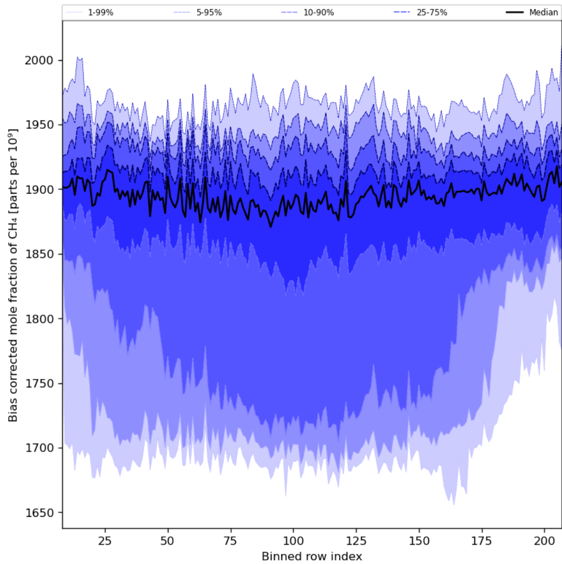
Figure 36: Along track statistics of “Bias corrected mole fraction of CH 4 ” for 2023-10-20 to 2023-10-22
