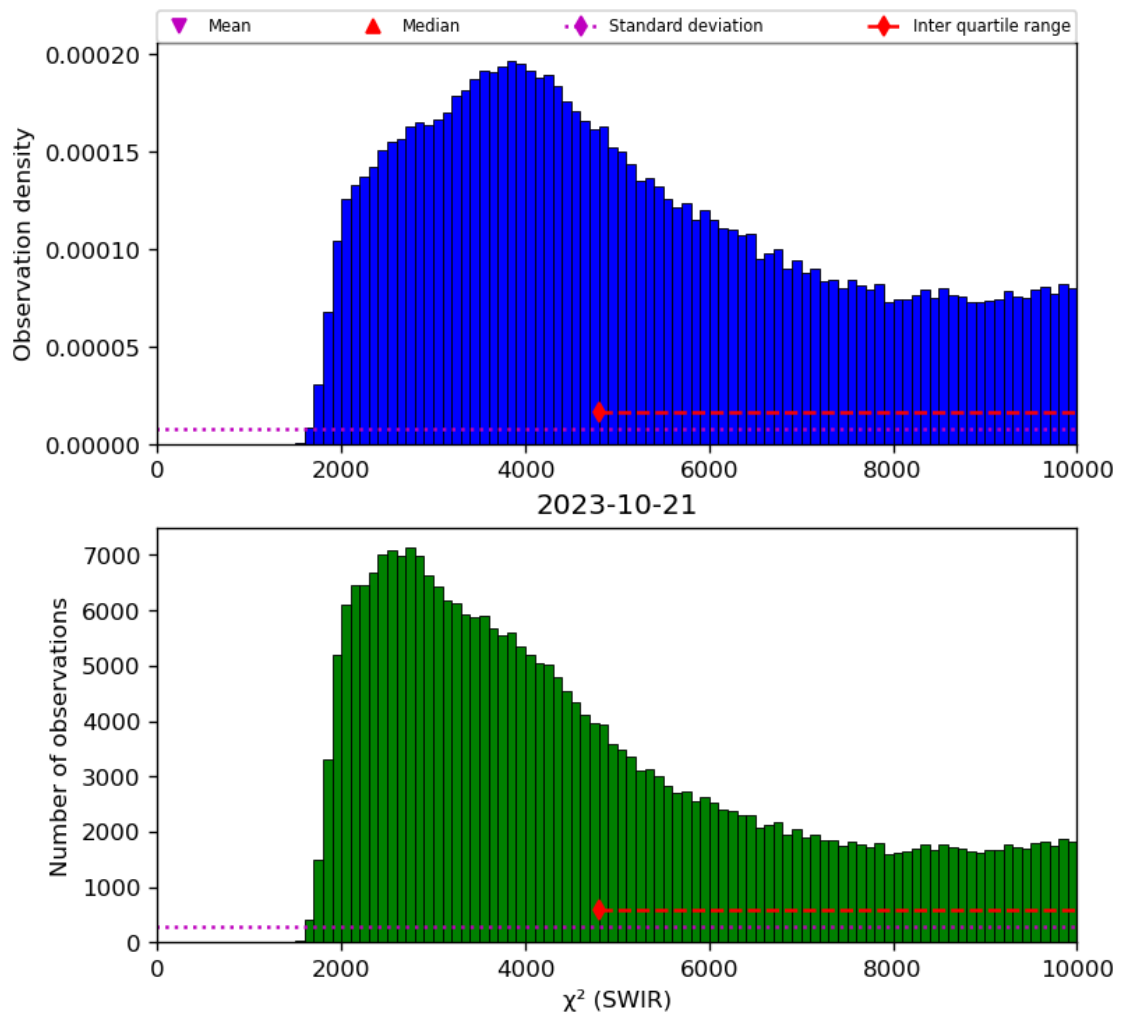
Figure 28: Histogram of “ \chi^2 (SWIR)” for 2023-10-20 to 2023-10-22
