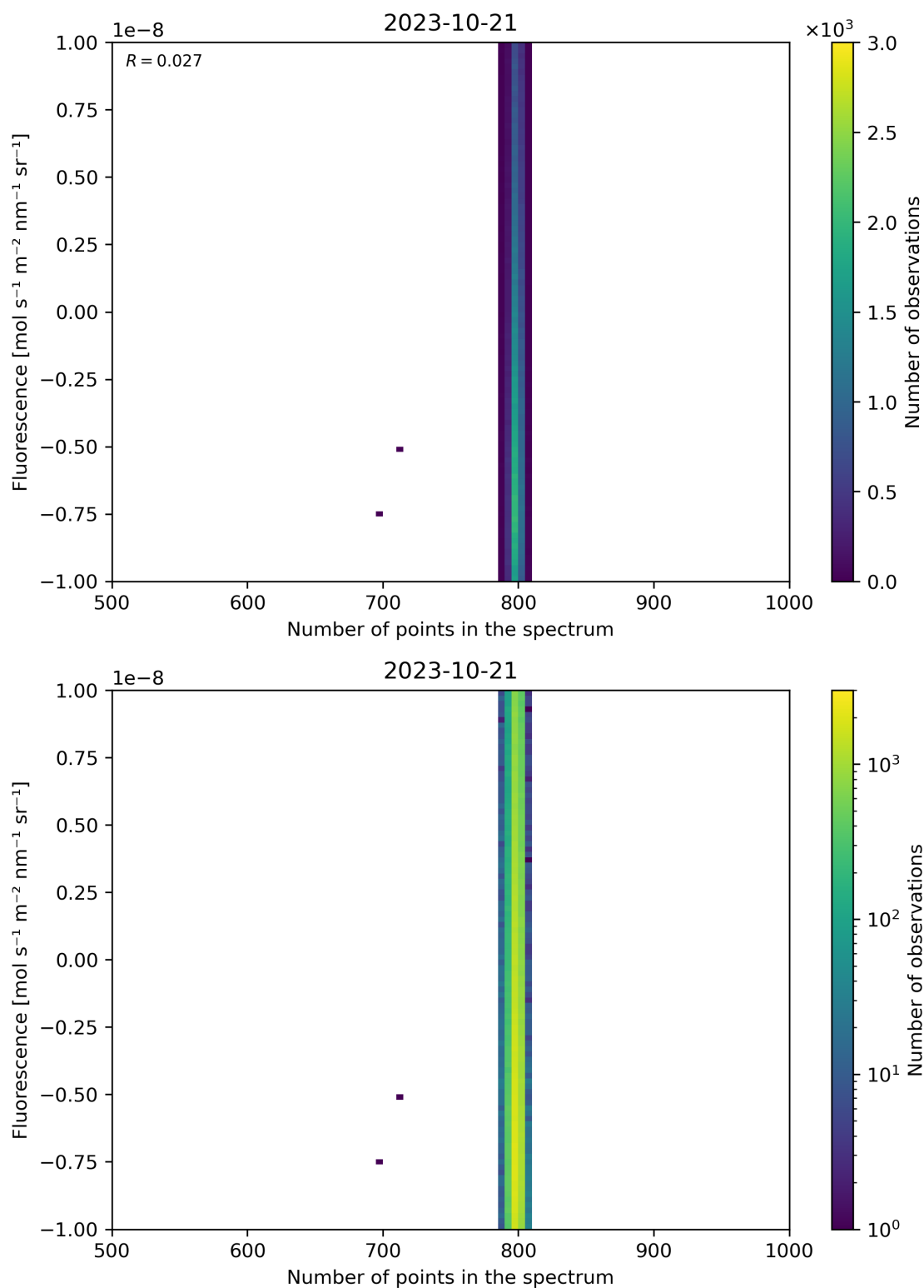
Figure 91: Scatter density plot of “Number of points in the spectrum” against “Fluorescence” for 2023-10-20 to 2023-10-22.
