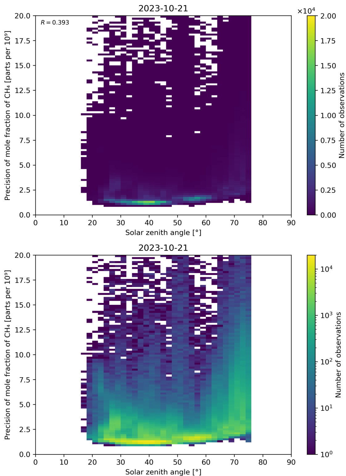
Figure 101: Scatter density plot of “Solar zenith angle” against “Precision of mole fraction of \text{CH}_4 ” for 2023-10-20 to 2023-10-22.
