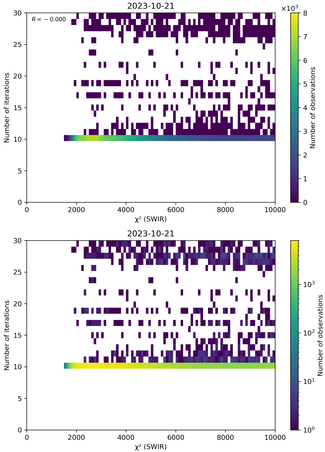
Figure 50: Scatter density plot of “ \chi^2 (SWIR)” against “Number of iterations” for 2023-10-20 to 2023-10-22.
