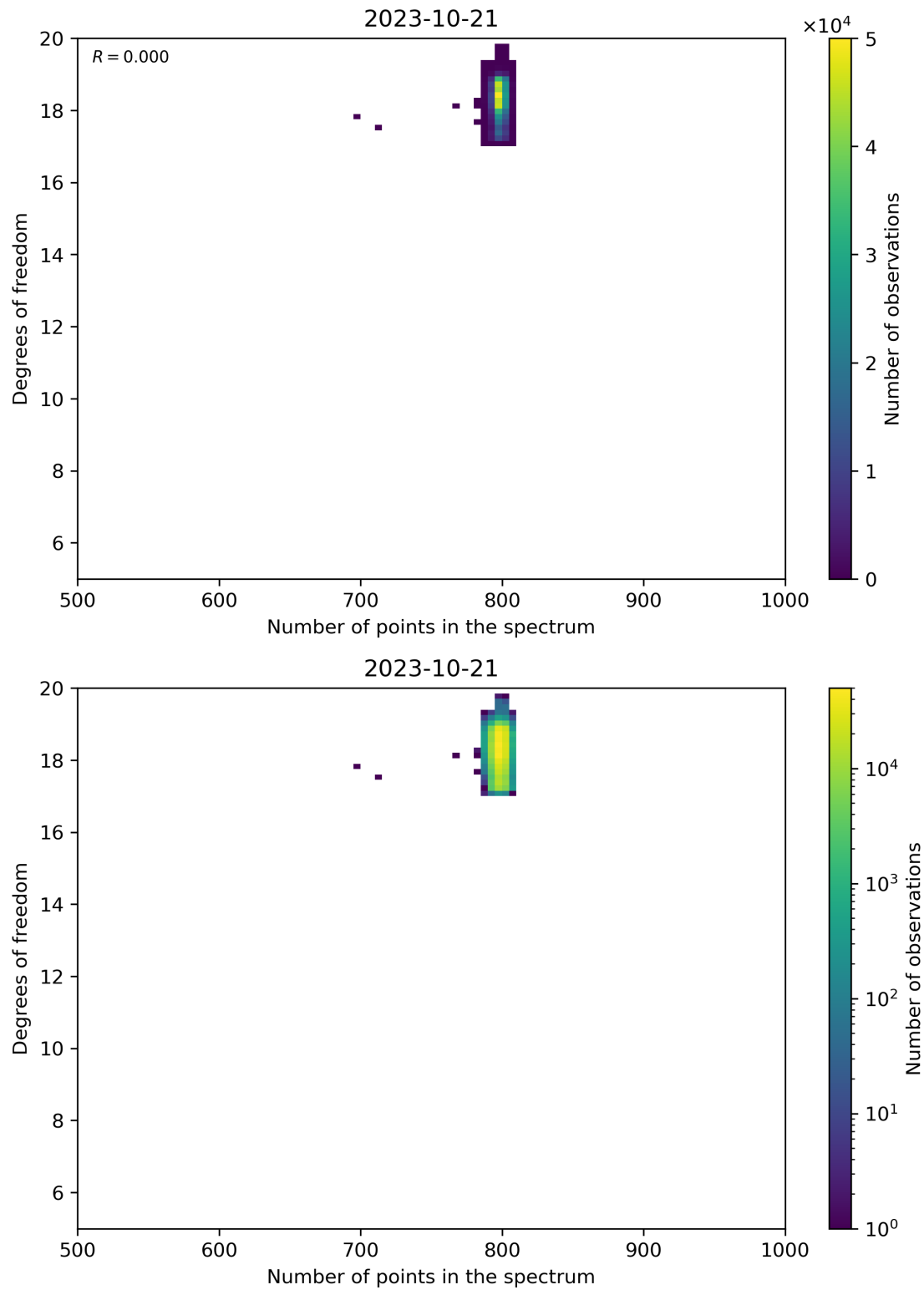
Figure 90: Scatter density plot of “Number of points in the spectrum” against “Degrees of freedom” for 2023-10-20 to 2023-10-22.
