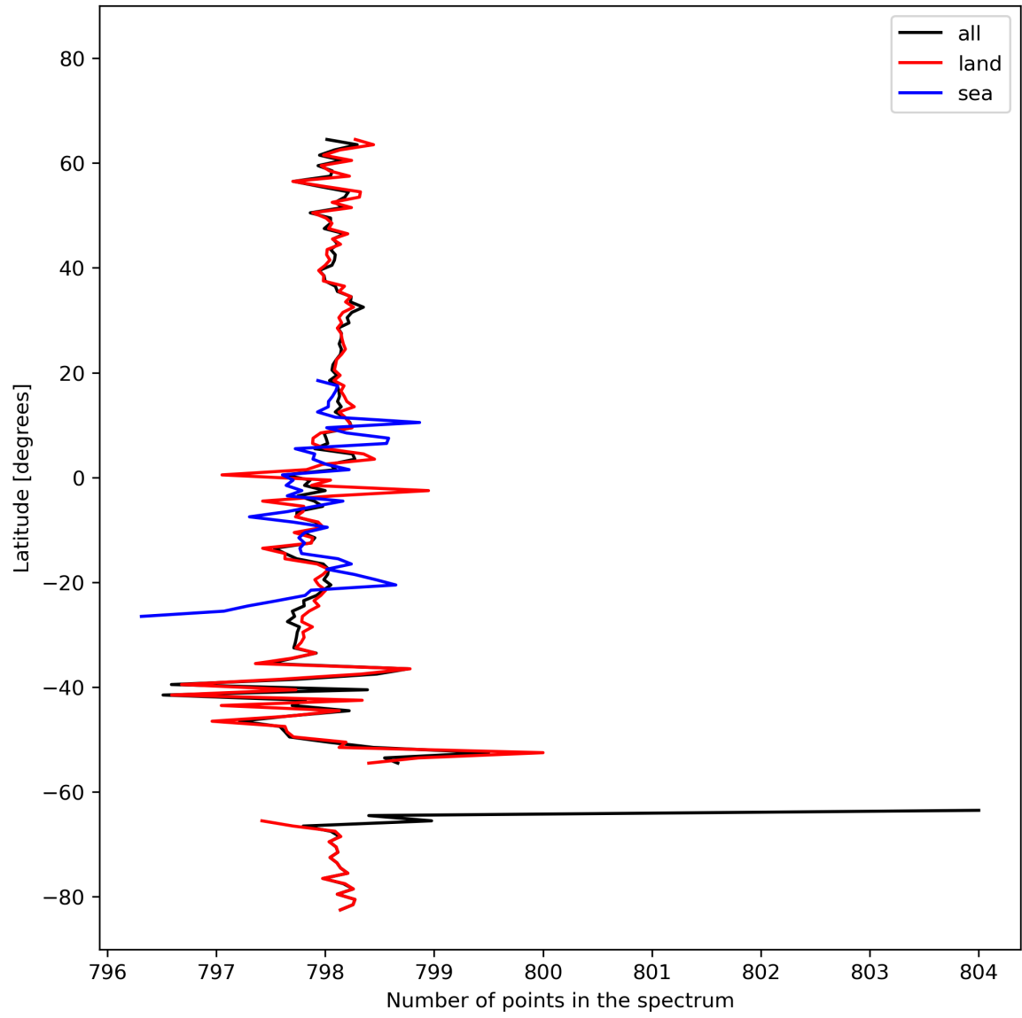
Figure 15: Zonal average of “Number of points in the spectrum” for 2023-10-20 to 2023-10-22.
