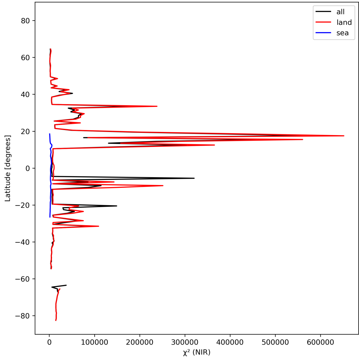
Figure 18: Zonal average of “ \chi^2 (NIR)” for 2023-10-20 to 2023-10-22.
