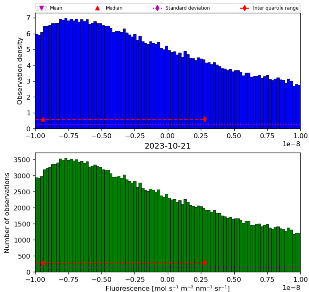
Figure 32: Histogram of “Fluorescence” for 2023-10-20 to 2023-10-22
