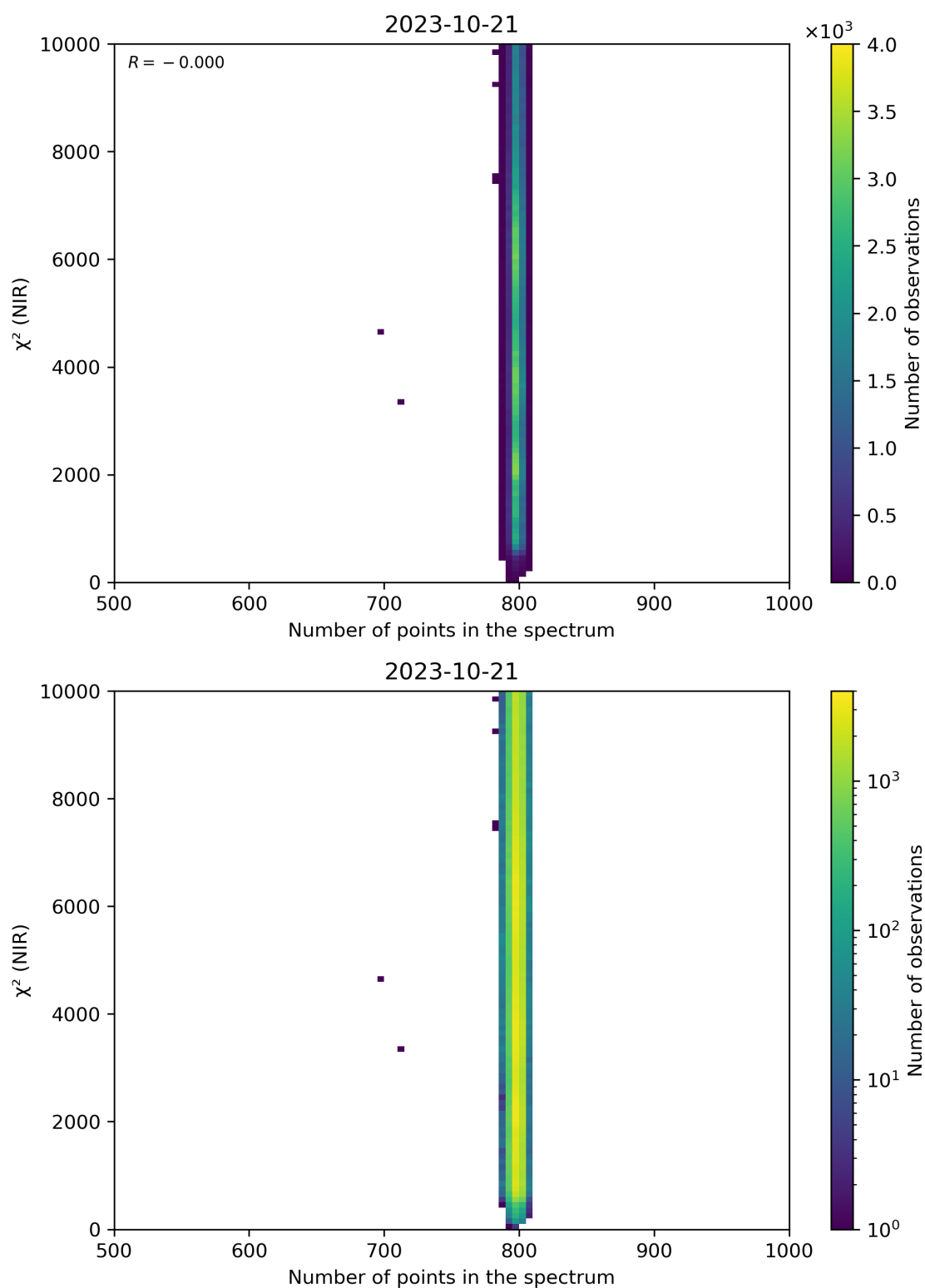
Figure 88: Scatter density plot of “Number of points in the spectrum” against “ \chi^2 (NIR)” for 2023-10-20 to 2023-10-22.
