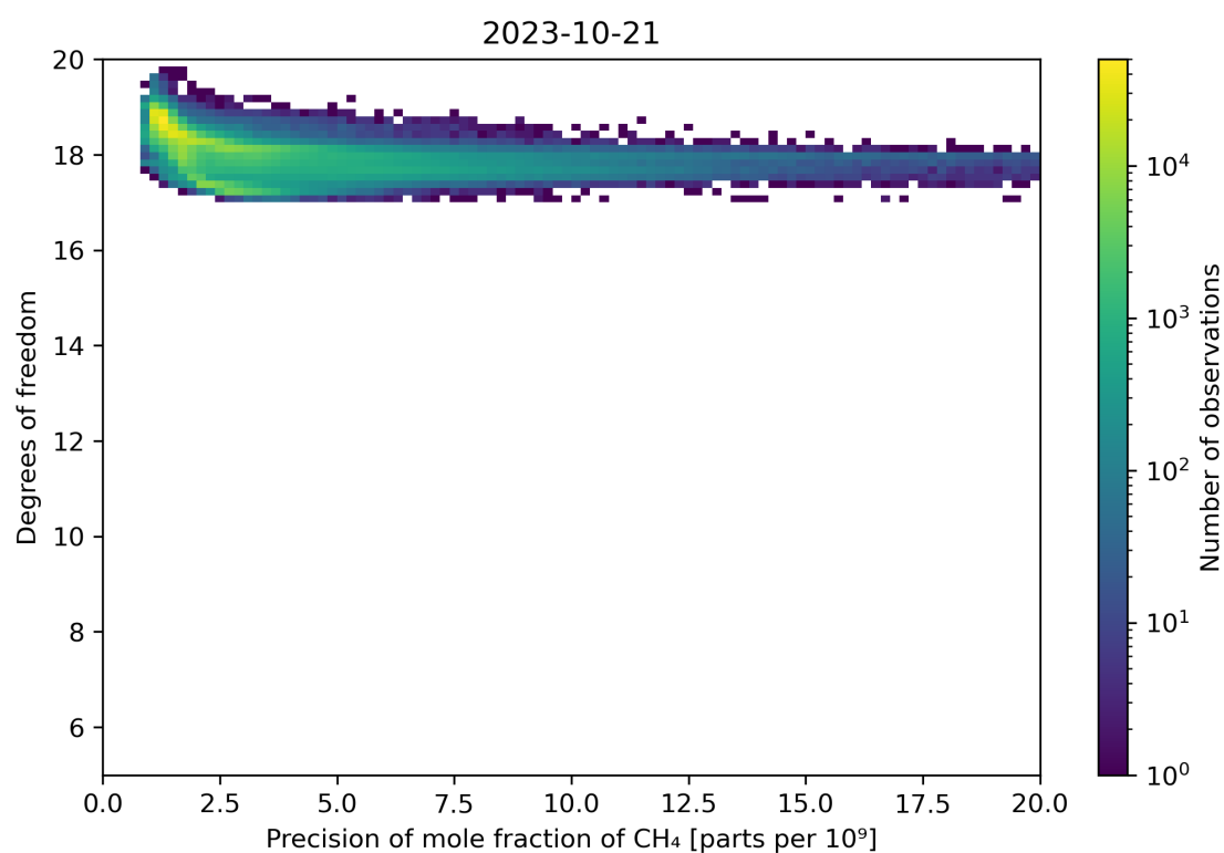
Figure 80: Scatter density plot of “Precision of mole fraction of \text{CH}_4 ” against “Degrees of freedom” for 2023-10-20 to 2023-10-22.
