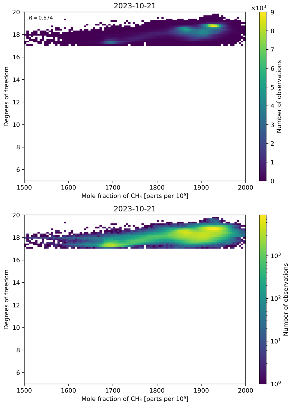
Figure 72: Scatter density plot of “Mole fraction of CH 4 ” against “Degrees of freedom” for 2023-10-20 to 2023-10-22.
