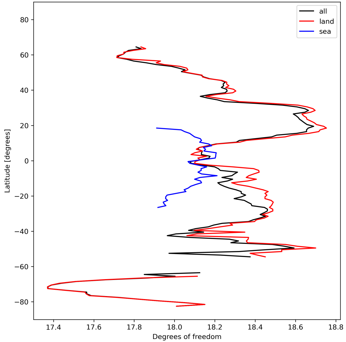
Figure 19: Zonal average of “Degrees of freedom” for 2023-10-20 to 2023-10-22.
