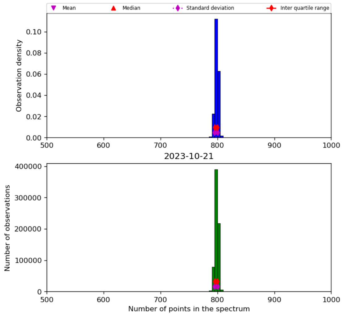
Figure 26: Histogram of “Number of points in the spectrum” for 2023-10-20 to 2023-10-22
