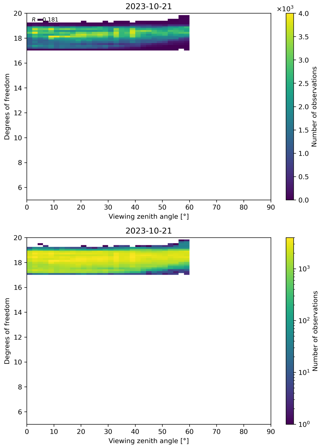
Figure 107: Scatter density plot of “Viewing zenith angle” against “Degrees of freedom” for 2023-10-20 to 2023-10-22.
