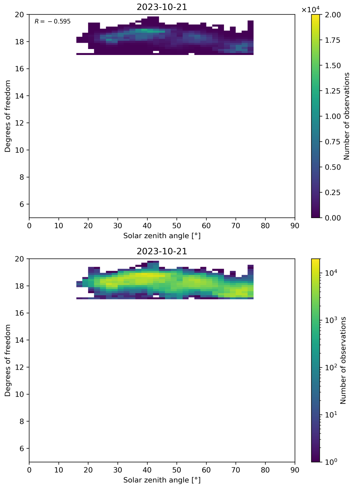
Figure 96: Scatter density plot of “Solar zenith angle” against “Degrees of freedom” for 2023-10-20 to 2023-10-22.
