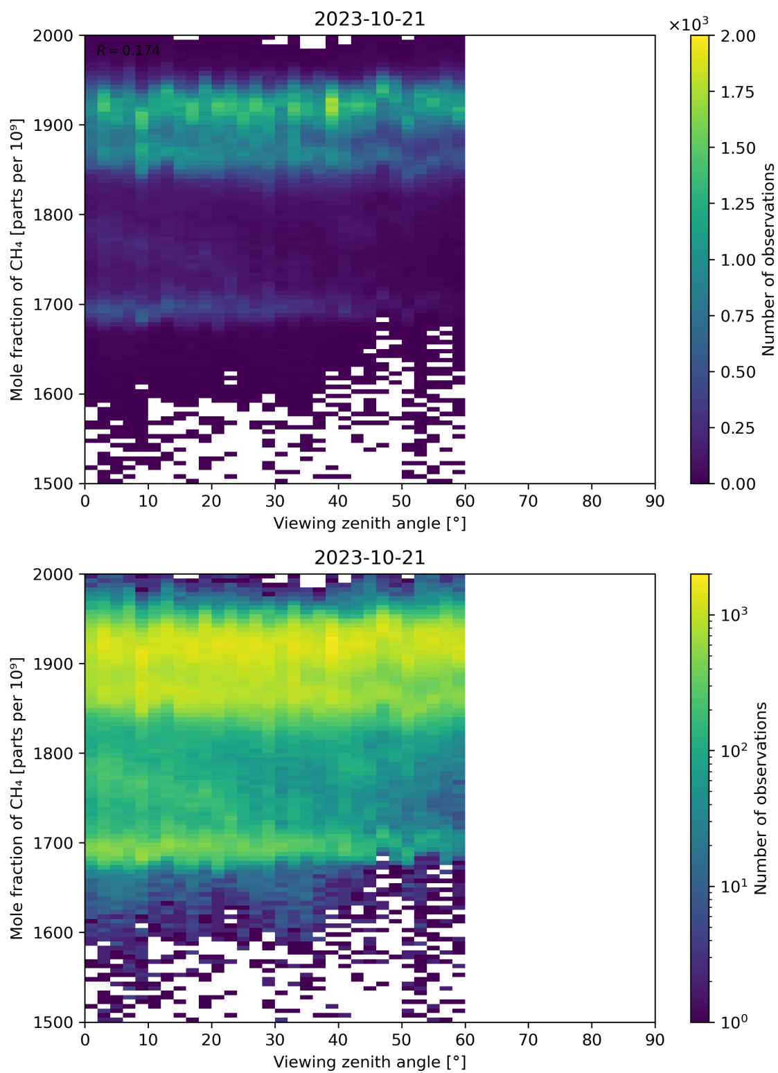
Figure 110: Scatter density plot of “Viewing zenith angle” against “Mole fraction of CH 4 ” for 2023-10-20 to 2023-10-22.
