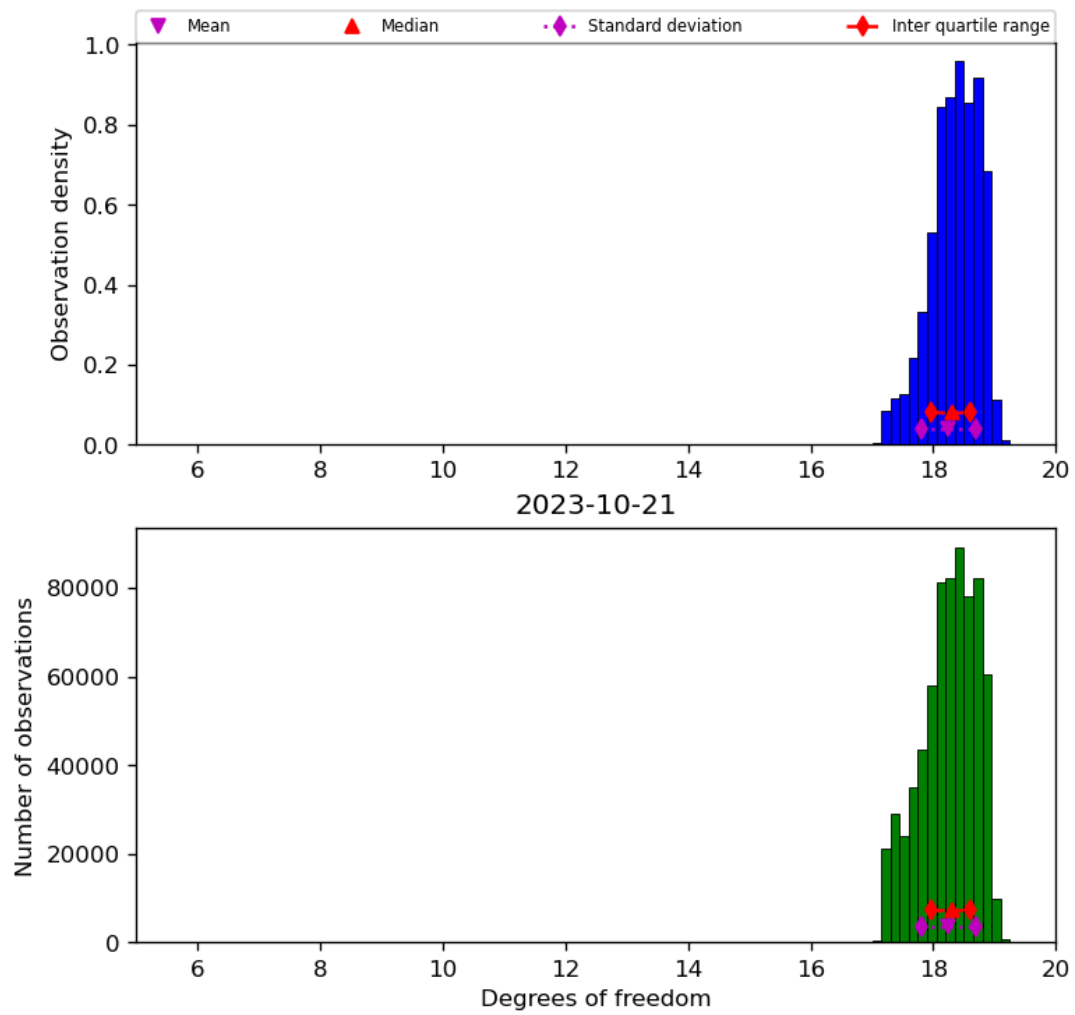
Figure 30: Histogram of “Degrees of freedom” for 2023-10-20 to 2023-10-22
