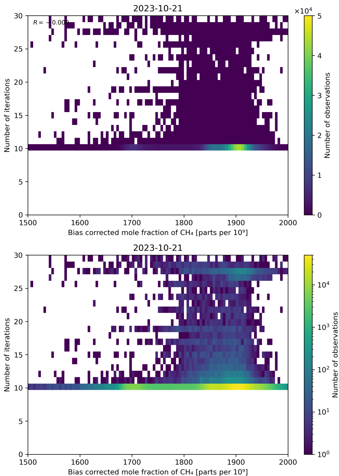
Figure 67: Scatter density plot of “Bias corrected mole fraction of CH 4 ” against “Number of iterations” for 2023-10-20 to 2023-10-22.
