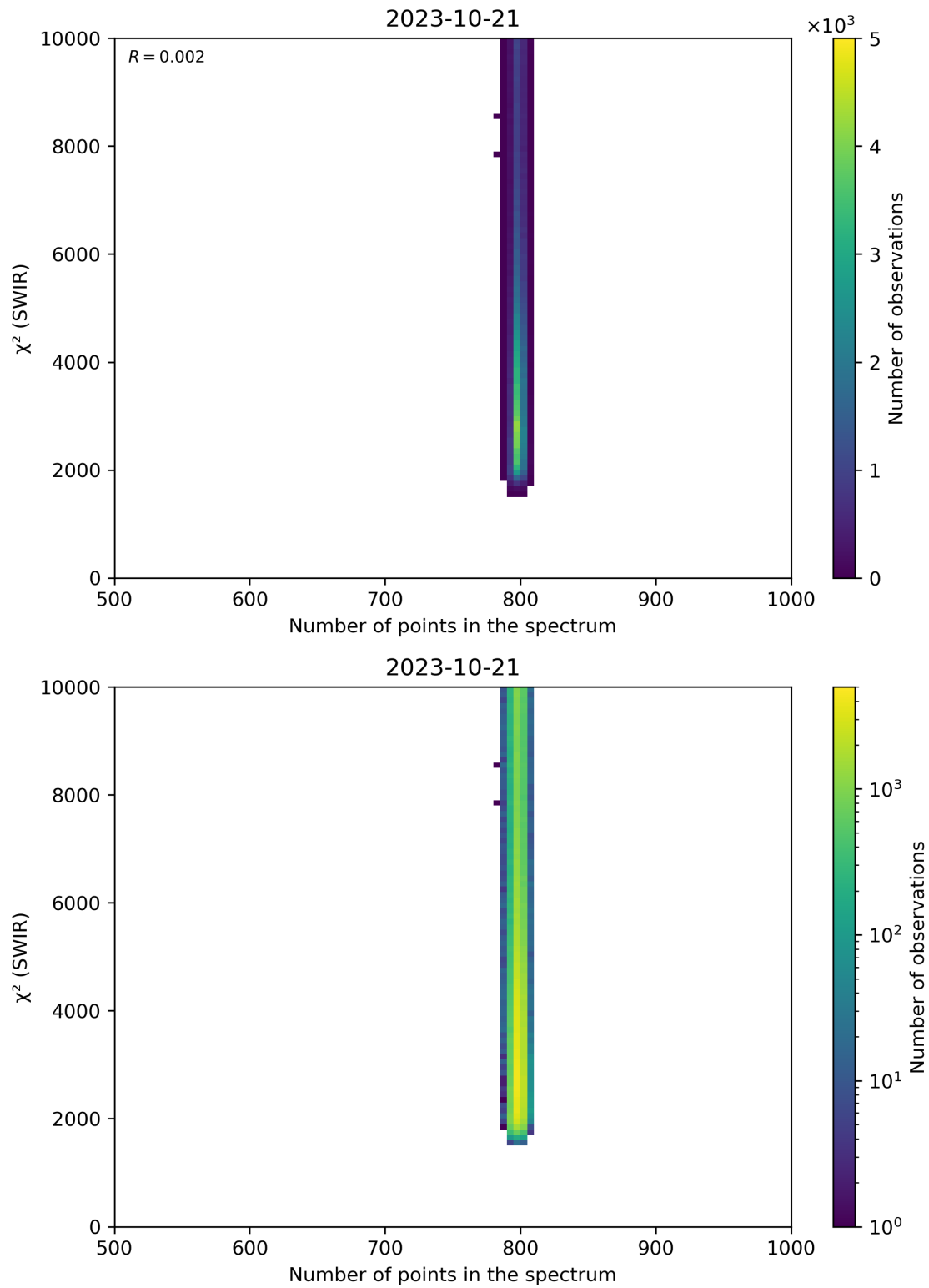
Figure 89: Scatter density plot of “Number of points in the spectrum” against “ \chi^2 (SWIR)” for 2023-10-20 to 2023-10-22.
