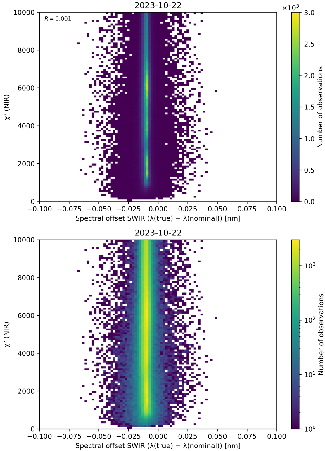
Figure 117: Scatter density plot of “Spectral offset SWIR ( \lambda(\text{true}) - \lambda(\text{nominal}) )” against “ \chi^2 (NIR)” for 2023-10-22 to 2023-10-23.
