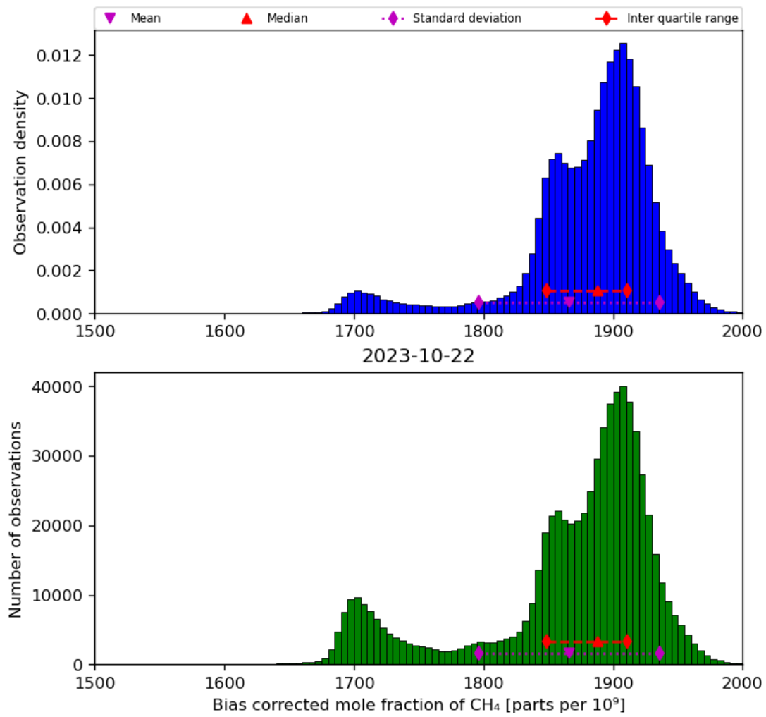
Figure 25: Histogram of “Bias corrected mole fraction of CH 4 ” for 2023-10-22 to 2023-10-23
