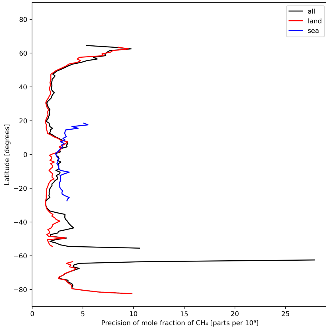
Figure 13: Zonal average of “Precision of mole fraction of CH 4 ” for 2023-10-22 to 2023-10-23.
