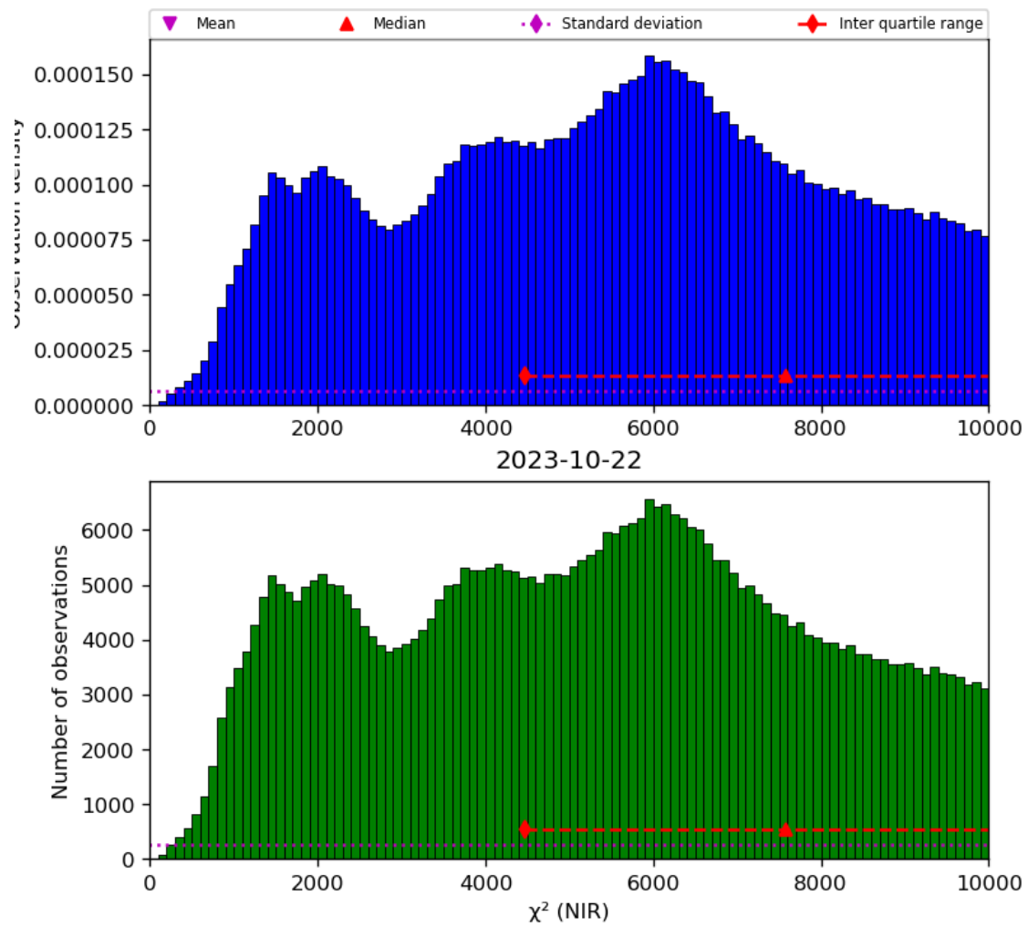
Figure 29: Histogram of “ \chi^2 (NIR)” for 2023-10-22 to 2023-10-23
