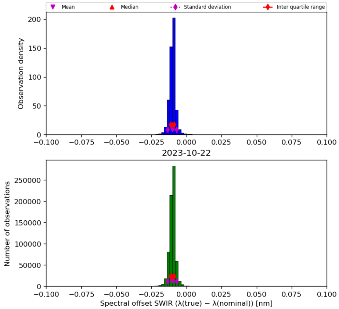
Figure 27: Histogram of “Spectral offset SWIR ( \lambda(\text{true}) - \lambda(\text{nominal}) )” for 2023-10-22 to 2023-10-23
