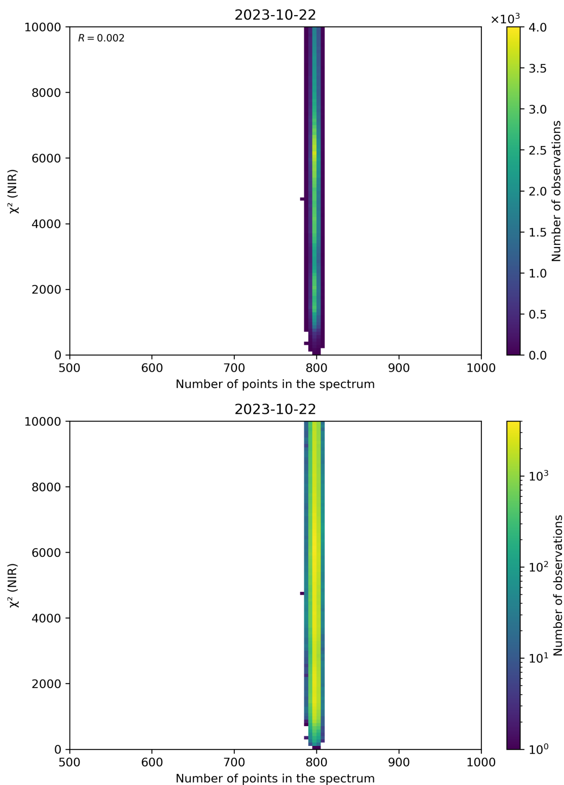
Figure 88: Scatter density plot of “Number of points in the spectrum” against “ \chi^2 (NIR)” for 2023-10-22 to 2023-10-23.
