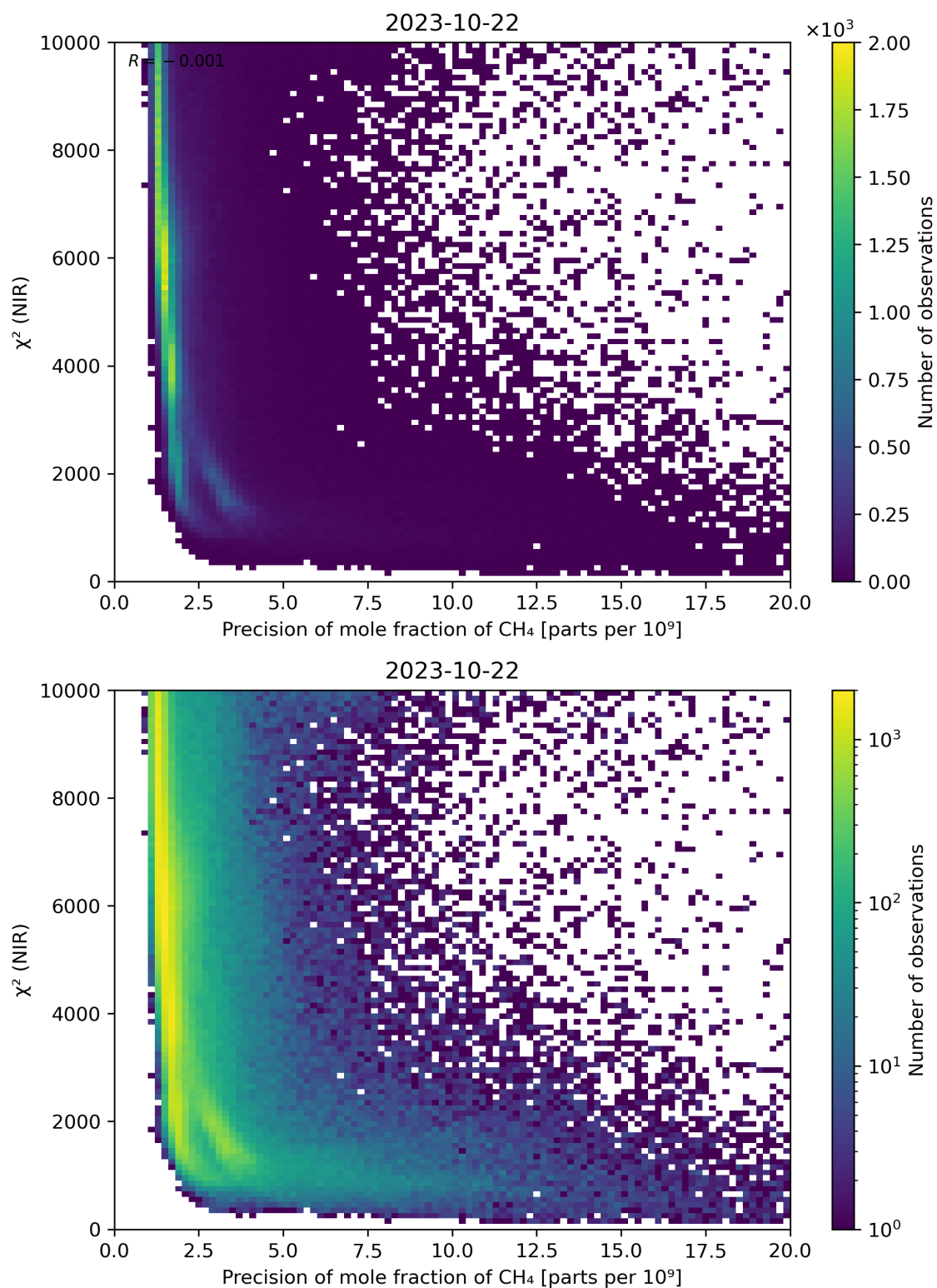
Figure 78: Scatter density plot of “Precision of mole fraction of \text{CH}_4 ” against “ \chi^2 (NIR)” for 2023-10-22 to 2023-10-23.
