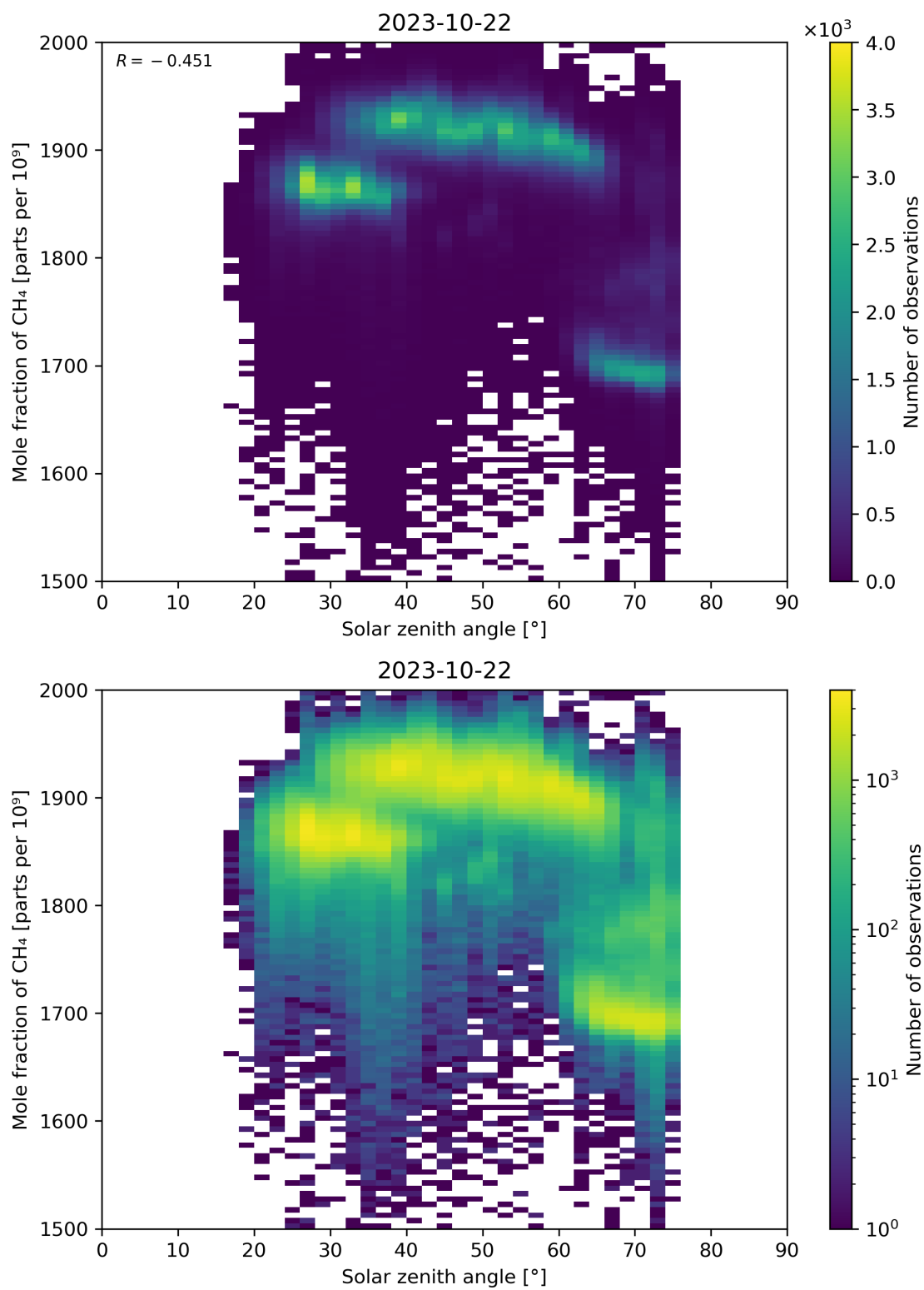
Figure 99: Scatter density plot of “Solar zenith angle” against “Mole fraction of \text{CH}_4 ” for 2023-10-22 to 2023-10-23.
