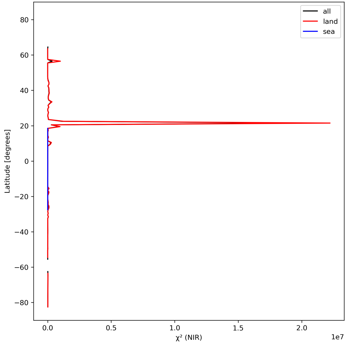
Figure 18: Zonal average of “ \chi^2 (NIR)” for 2023-10-22 to 2023-10-23.
