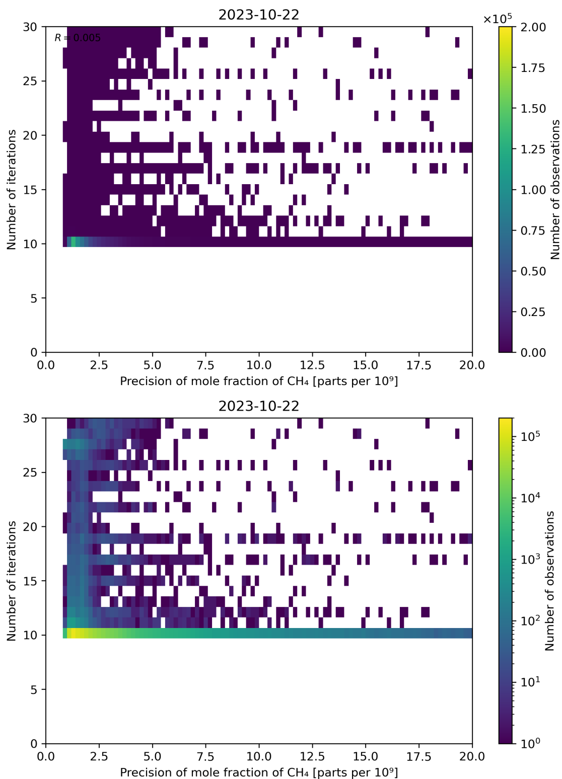
Figure 83: Scatter density plot of “Precision of mole fraction of CH 4 ” against “Number of iterations” for 2023-10-22 to 2023-10-23.
