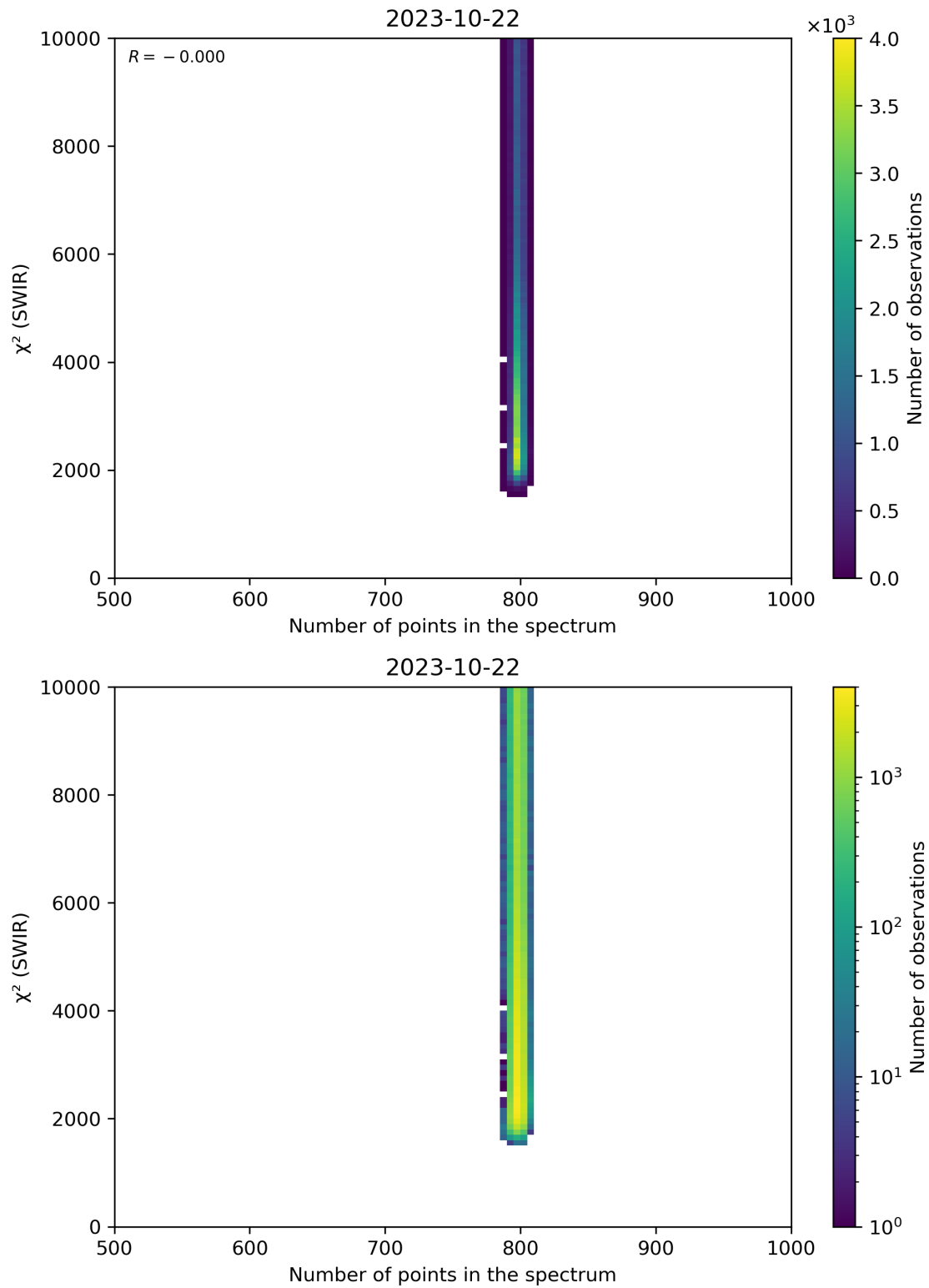
Figure 89: Scatter density plot of “Number of points in the spectrum” against “ \chi^2 (SWIR)” for 2023-10-22 to 2023-10-23.
