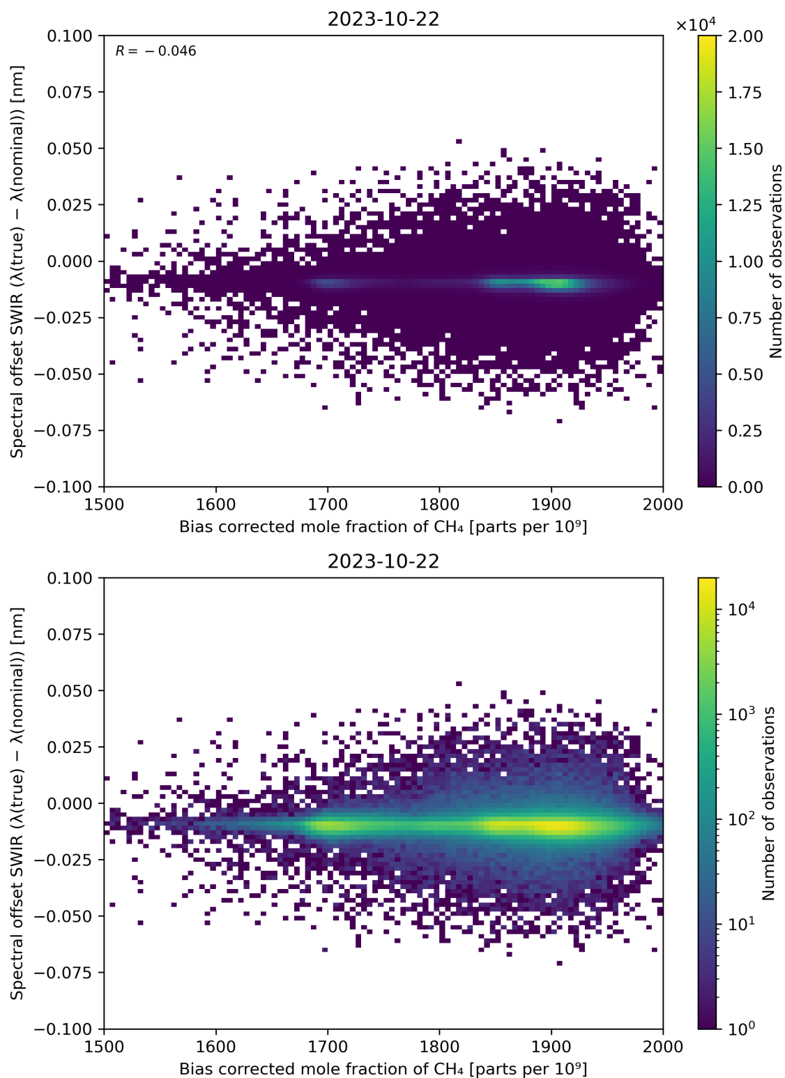
Figure 69: Scatter density plot of “Bias corrected mole fraction of \text{CH}_4 ” against “Spectral offset SWIR ( \lambda(\text{true}) - \lambda(\text{nominal}) )” for 2023-10-22 to 2023-10-23.
