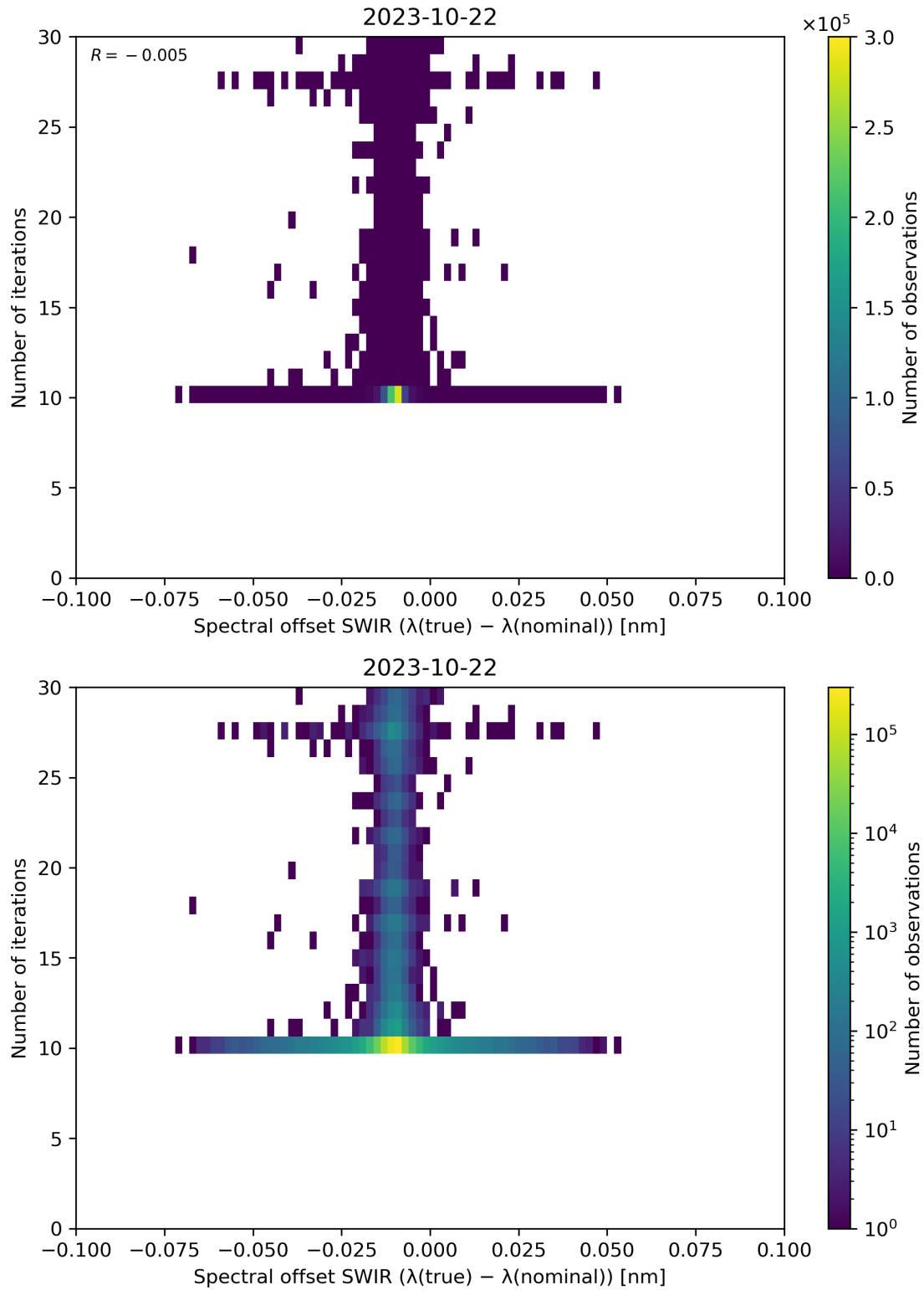
Figure 121: Scatter density plot of “Spectral offset SWIR ( \lambda(\text{true}) - \lambda(\text{nominal}) )” against “Number of iterations” for 2023-10-22 to 2023-10-23.
