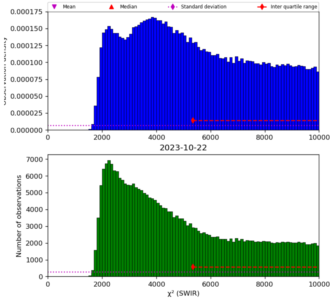
Figure 28: Histogram of “ \chi^2 (SWIR)” for 2023-10-22 to 2023-10-23
