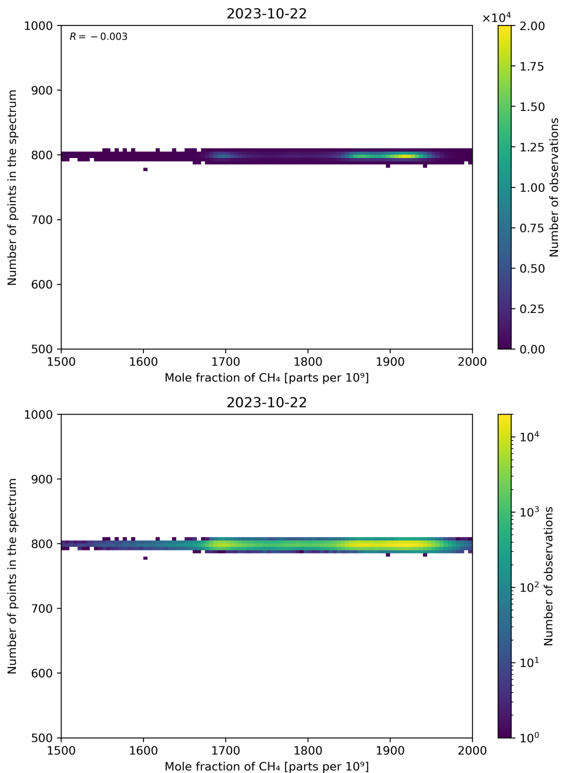
Figure 77: Scatter density plot of “Mole fraction of CH 4 ” against “Number of points in the spectrum” for 2023-10-22 to 2023-10-23.
