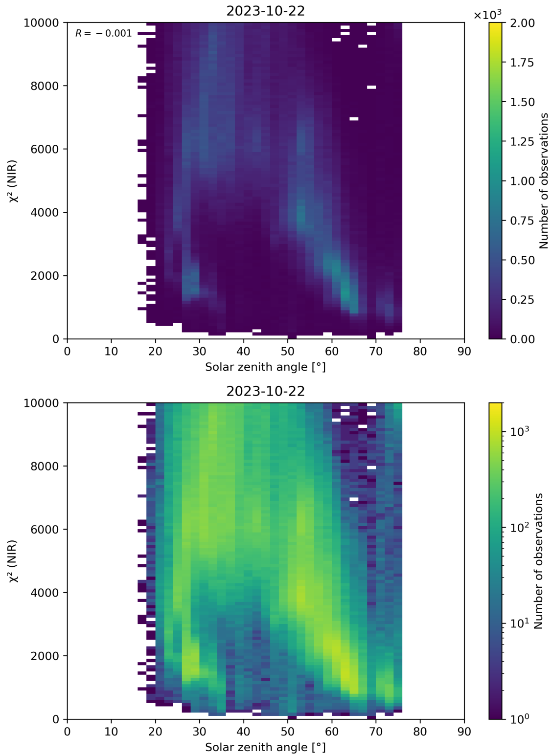
Figure 94: Scatter density plot of “Solar zenith angle” against “ \chi^2 (NIR)” for 2023-10-22 to 2023-10-23.
