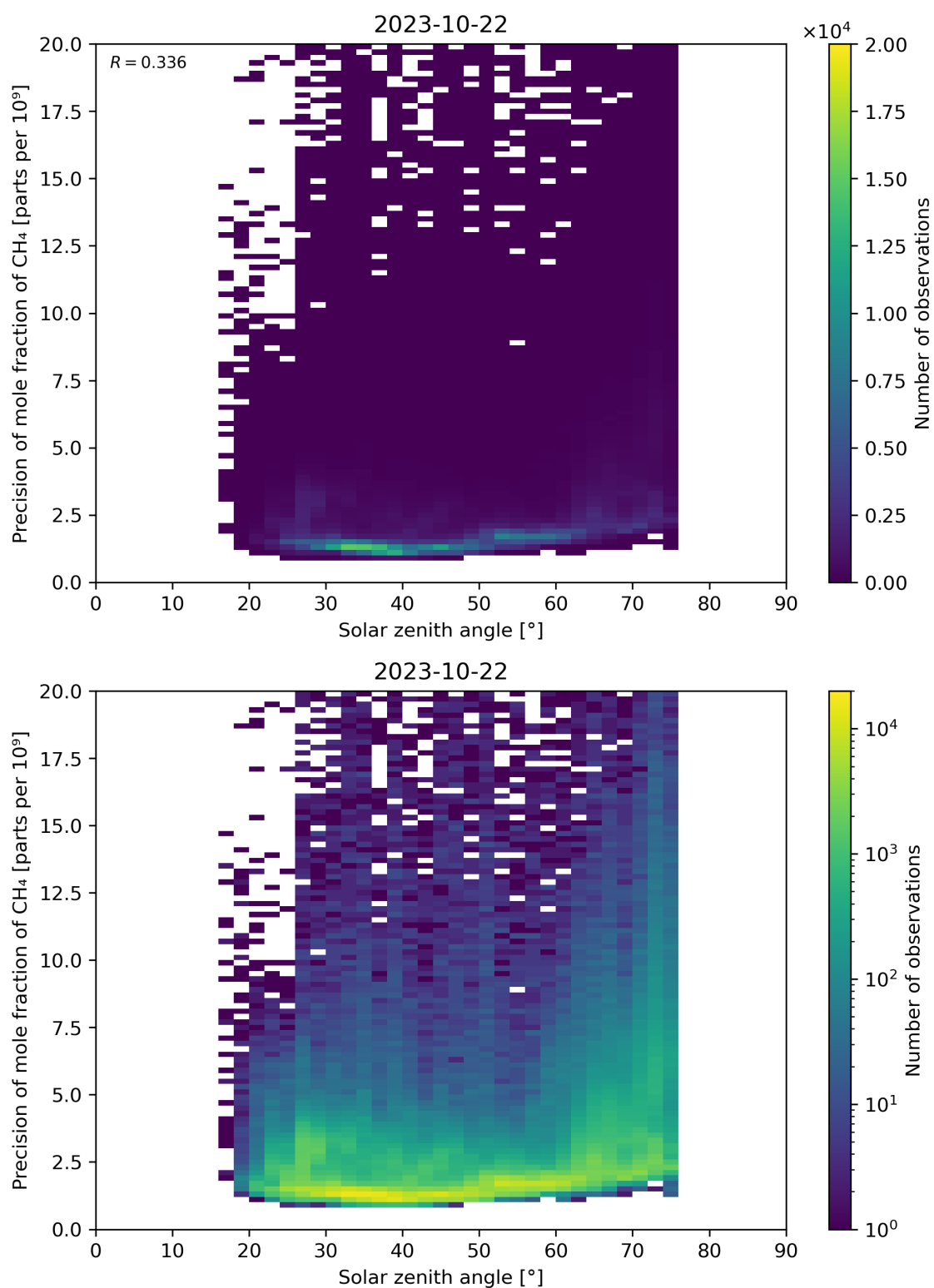
Figure 101: Scatter density plot of “Solar zenith angle” against “Precision of mole fraction of CH 4 ” for 2023-10-22 to 2023-10-23.
