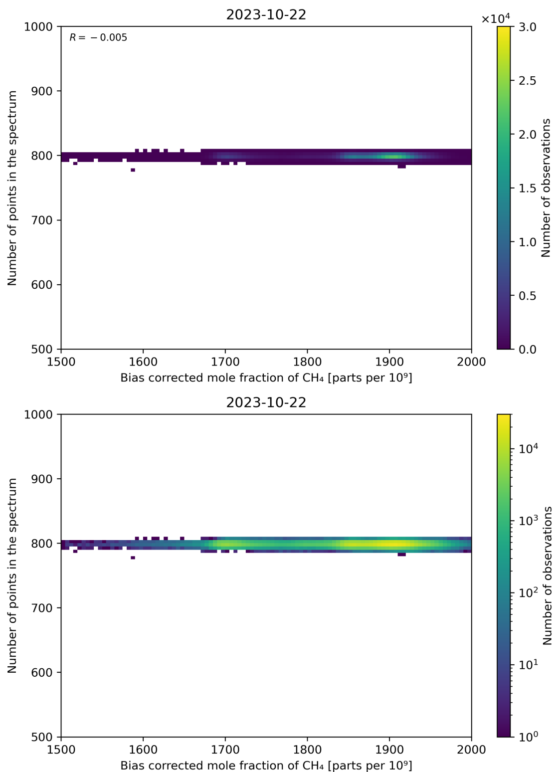
Figure 68: Scatter density plot of “Bias corrected mole fraction of CH 4 ” against “Number of points in the spectrum” for 2023-10-22 to 2023-10-23.
