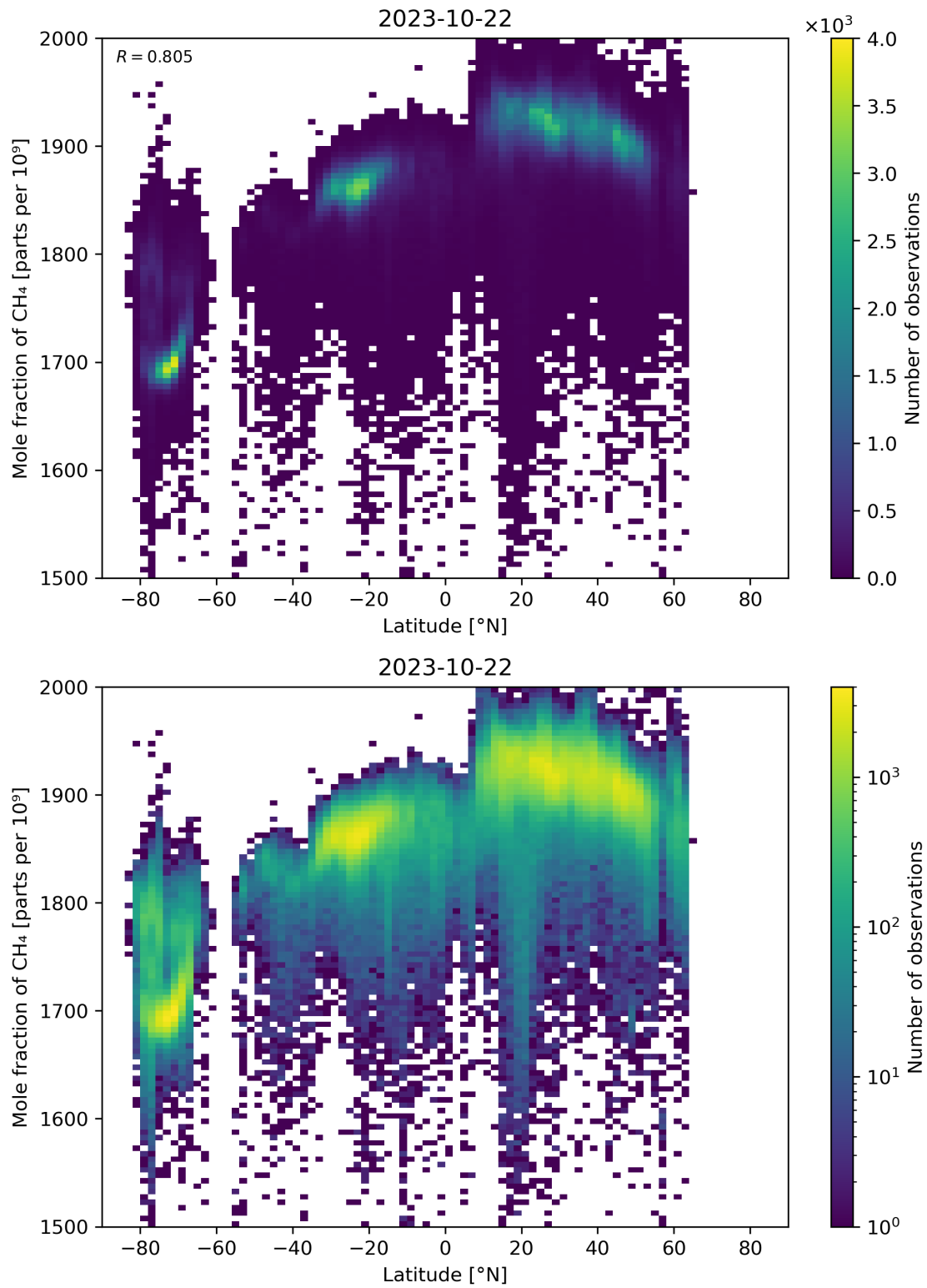
Figure 57: Scatter density plot of “Latitude” against “Mole fraction of \text{CH}_4 ” for 2023-10-22 to 2023-10-23.
