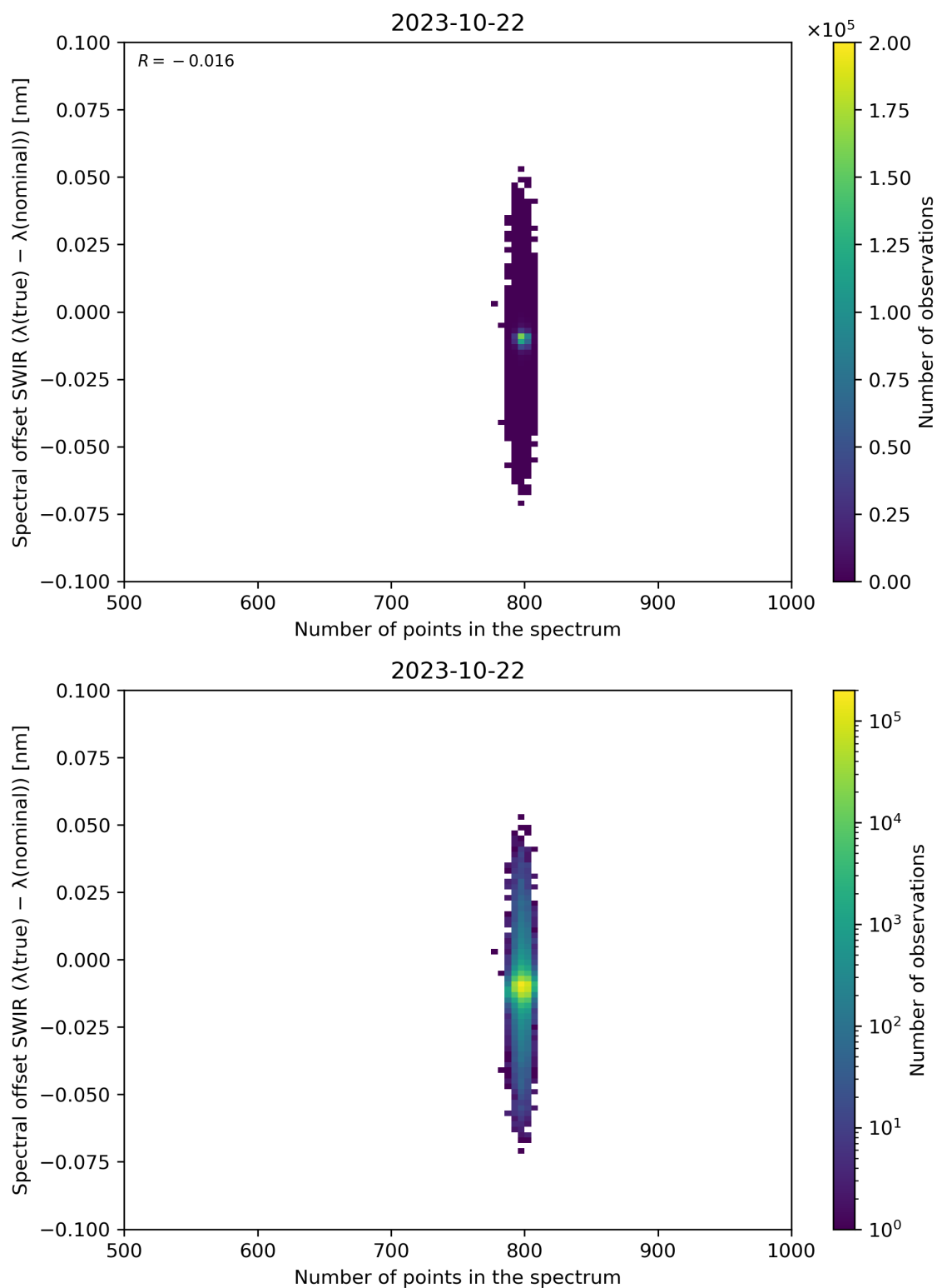
Figure 93: Scatter density plot of “Number of points in the spectrum” against “Spectral offset SWIR ( \lambda(\text{true}) - \lambda(\text{nominal}) )” for 2023-10-22 to 2023-10-23.
