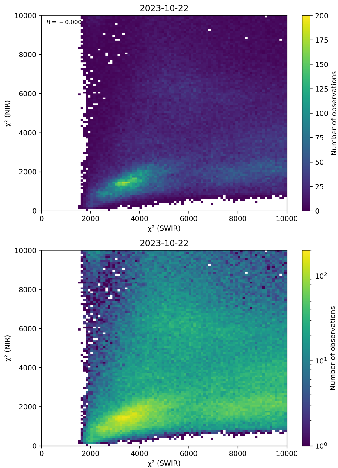
Figure 47: Scatter density plot of “ \chi^2 (SWIR)” against “ \chi^2 (NIR)” for 2023-10-22 to 2023-10-23.
