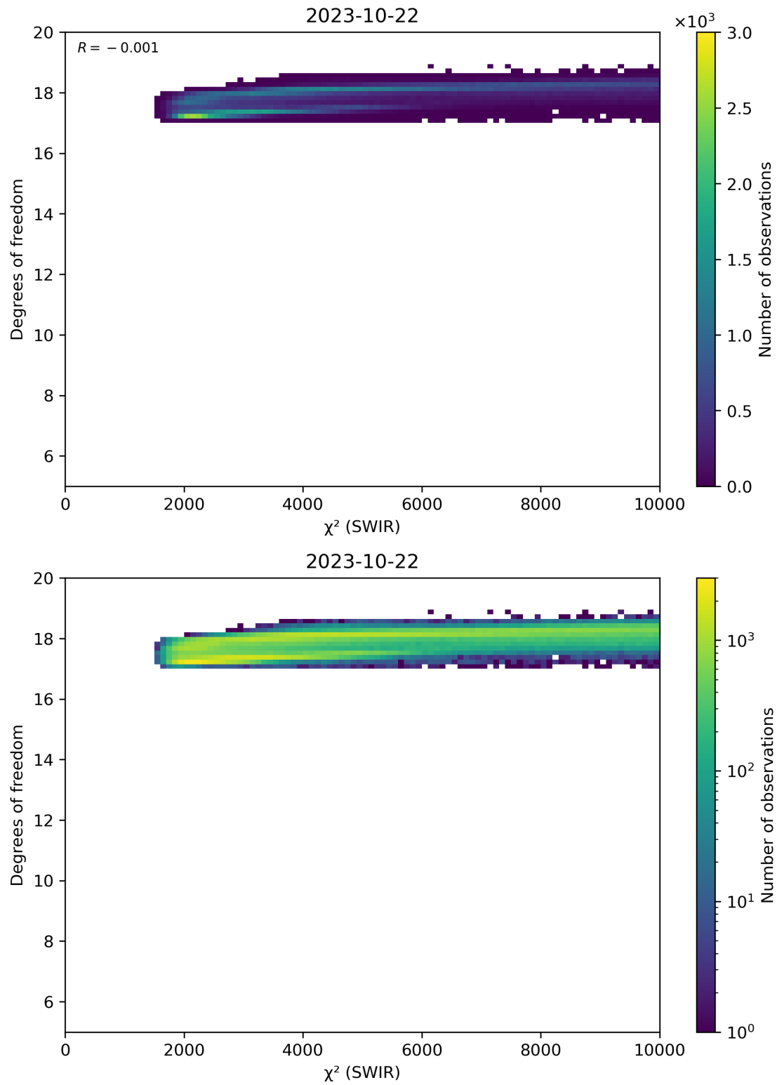
Figure 48: Scatter density plot of “ \chi^2 (SWIR)” against “Degrees of freedom” for 2023-10-22 to 2023-10-23.
