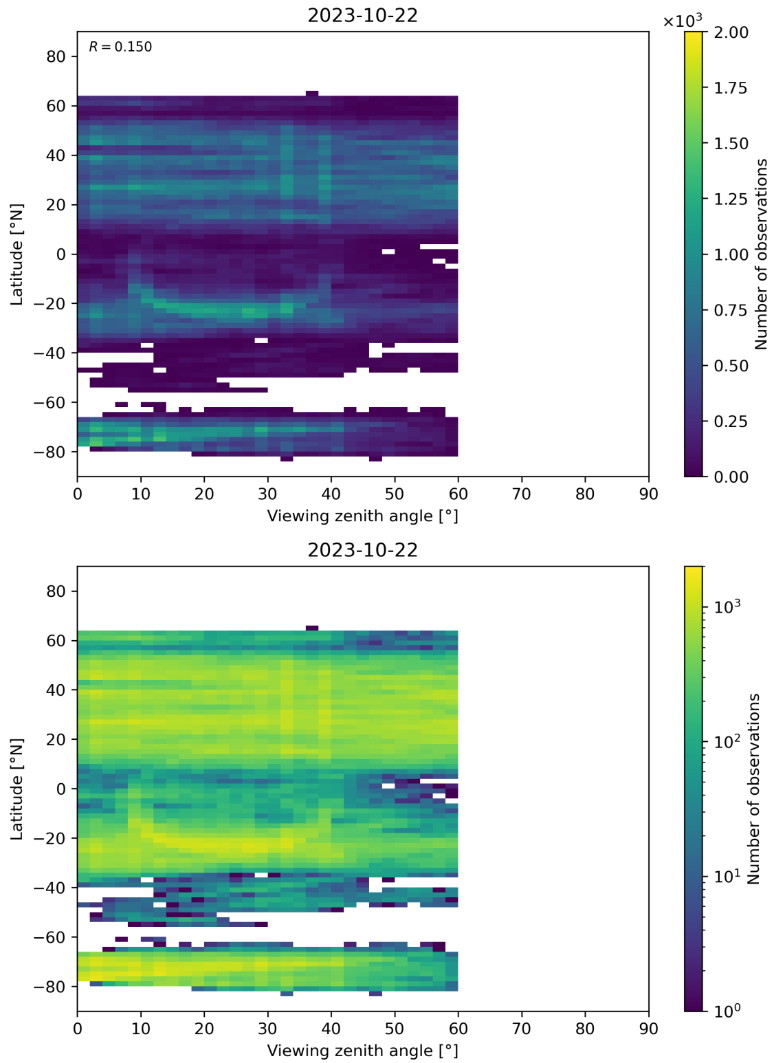
Figure 109: Scatter density plot of “Viewing zenith angle” against “Latitude” for 2023-10-22 to 2023-10-23.
