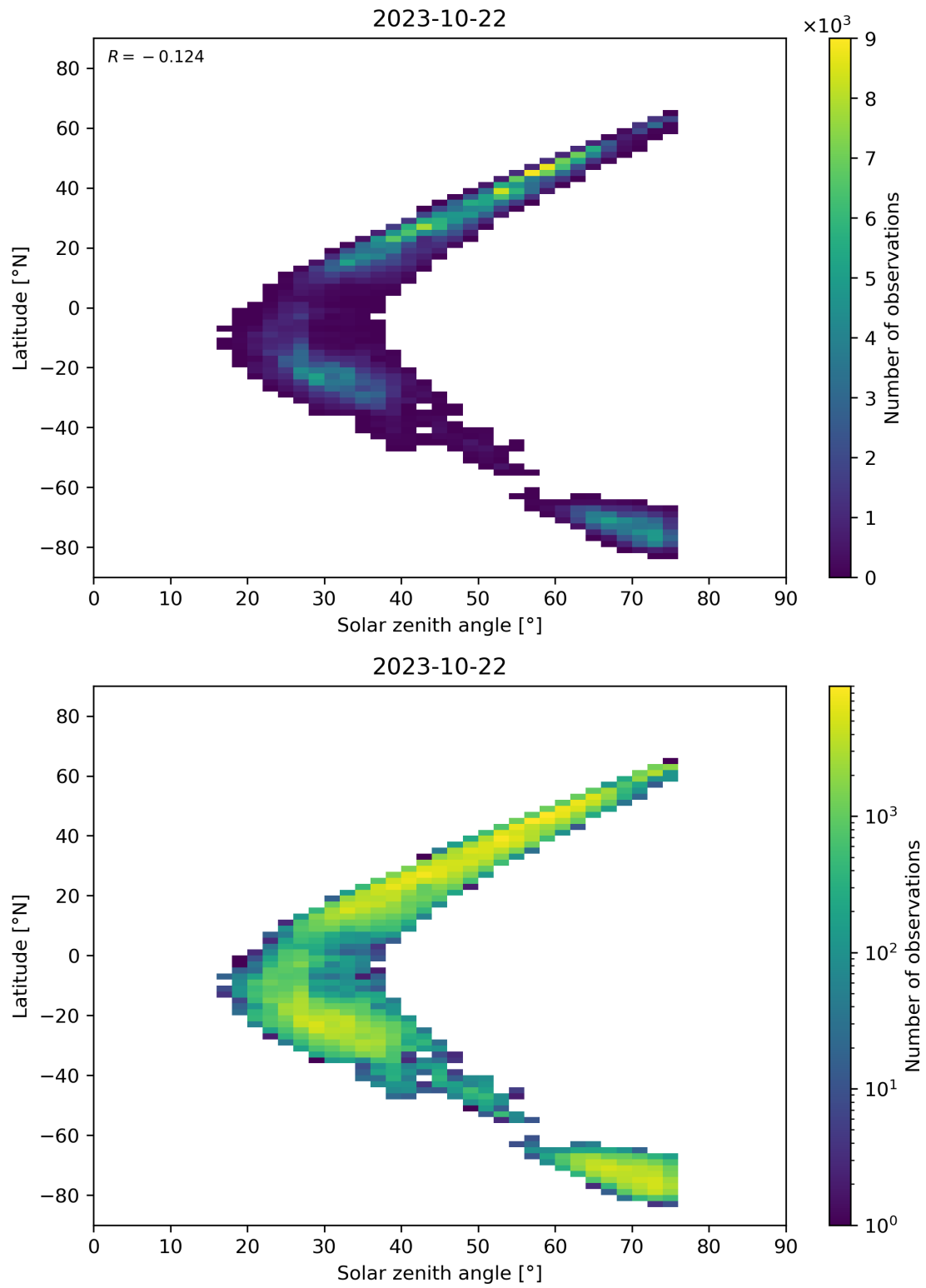
Figure 98: Scatter density plot of “Solar zenith angle” against “Latitude” for 2023-10-22 to 2023-10-23.
