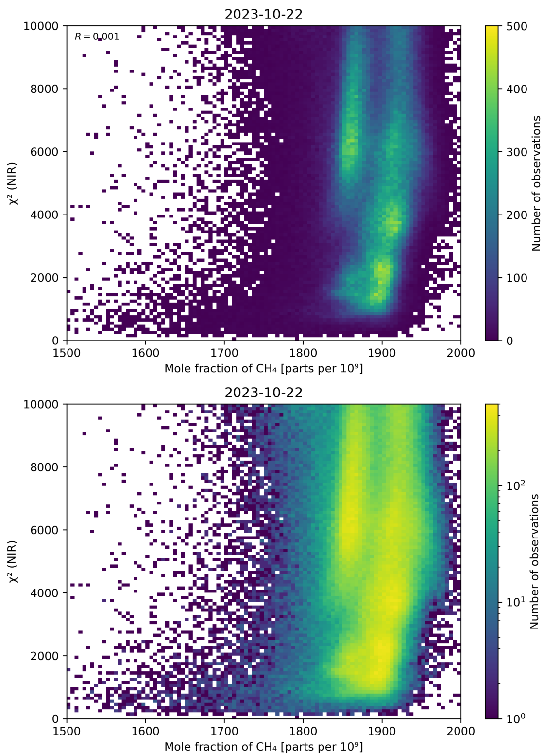
Figure 70: Scatter density plot of “Mole fraction of CH 4 ” against “ \chi^2 (NIR)” for 2023-10-22 to 2023-10-23.
