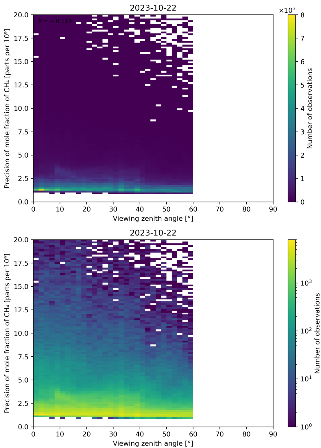
Figure 112: Scatter density plot of “Viewing zenith angle” against “Precision of mole fraction of CH 4 ” for 2023-10-22 to 2023-10-23.
