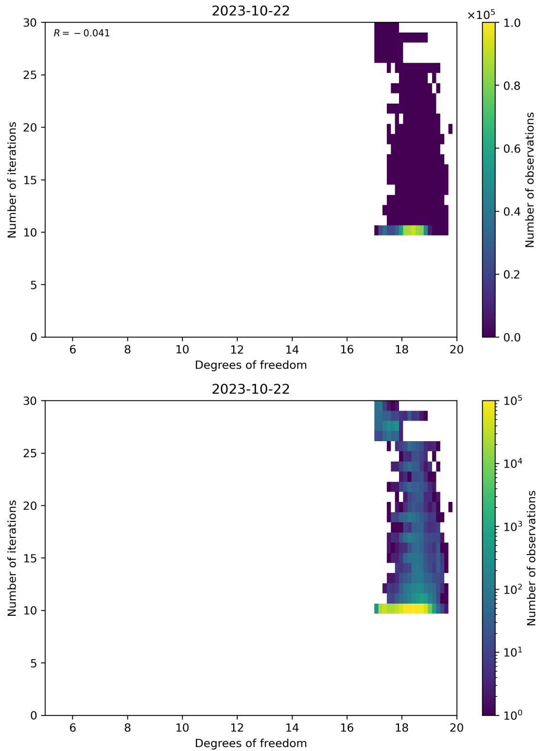
Figure 52: Scatter density plot of “Degrees of freedom” against “Number of iterations” for 2023-10-22 to 2023-10-23.
