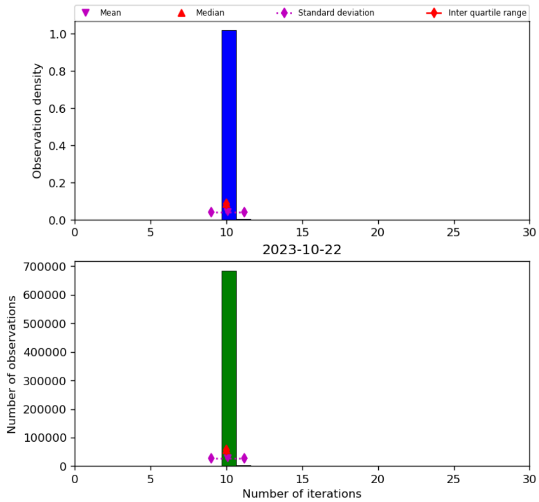
Figure 31: Histogram of “Number of iterations” for 2023-10-22 to 2023-10-23
