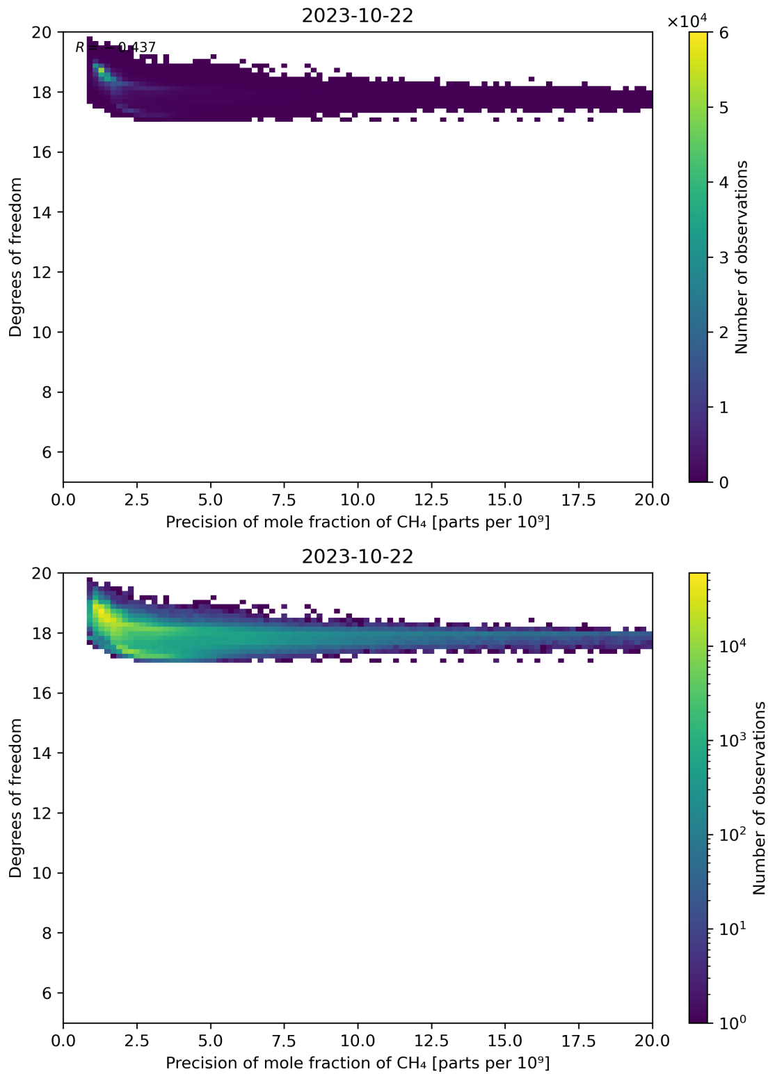
Figure 80: Scatter density plot of “Precision of mole fraction of CH 4 ” against “Degrees of freedom” for 2023-10-22 to 2023-10-23.
