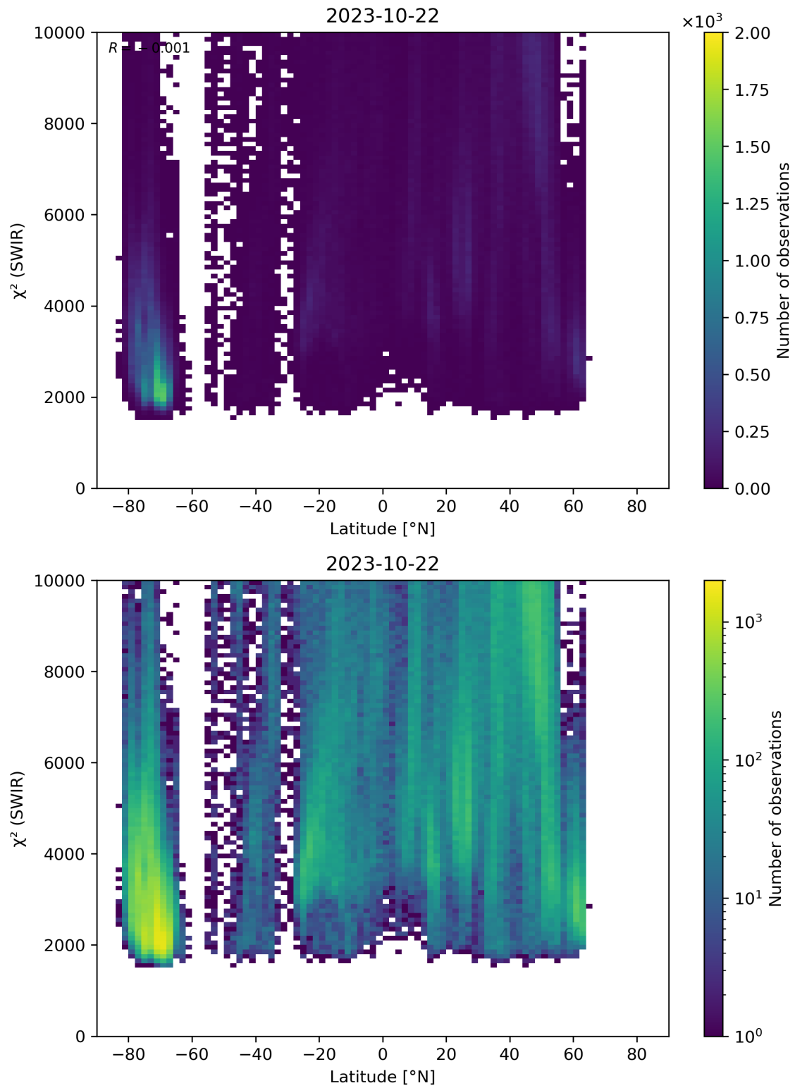
Figure 54: Scatter density plot of “Latitude” against “ \chi^2 (SWIR)” for 2023-10-22 to 2023-10-23.
