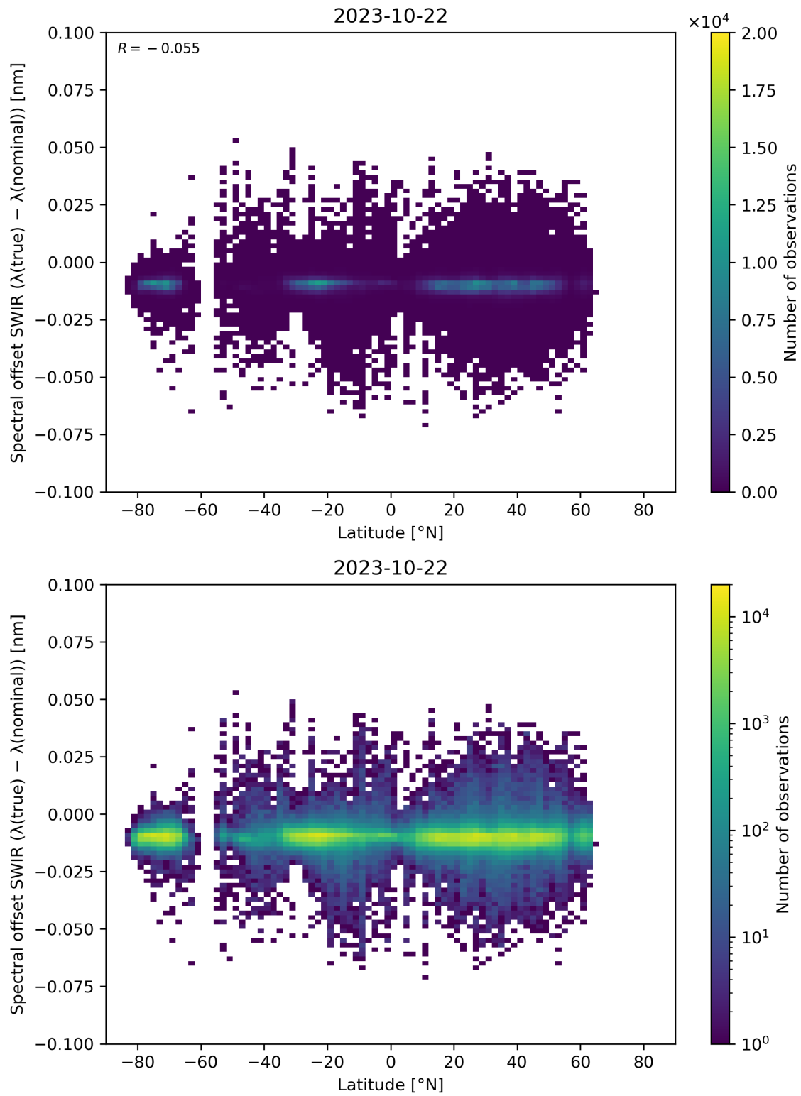
Figure 62: Scatter density plot of “Latitude” against “Spectral offset SWIR ( \lambda(\text{true}) - \lambda(\text{nominal}) )” for 2023-10-22 to 2023-10-23.
