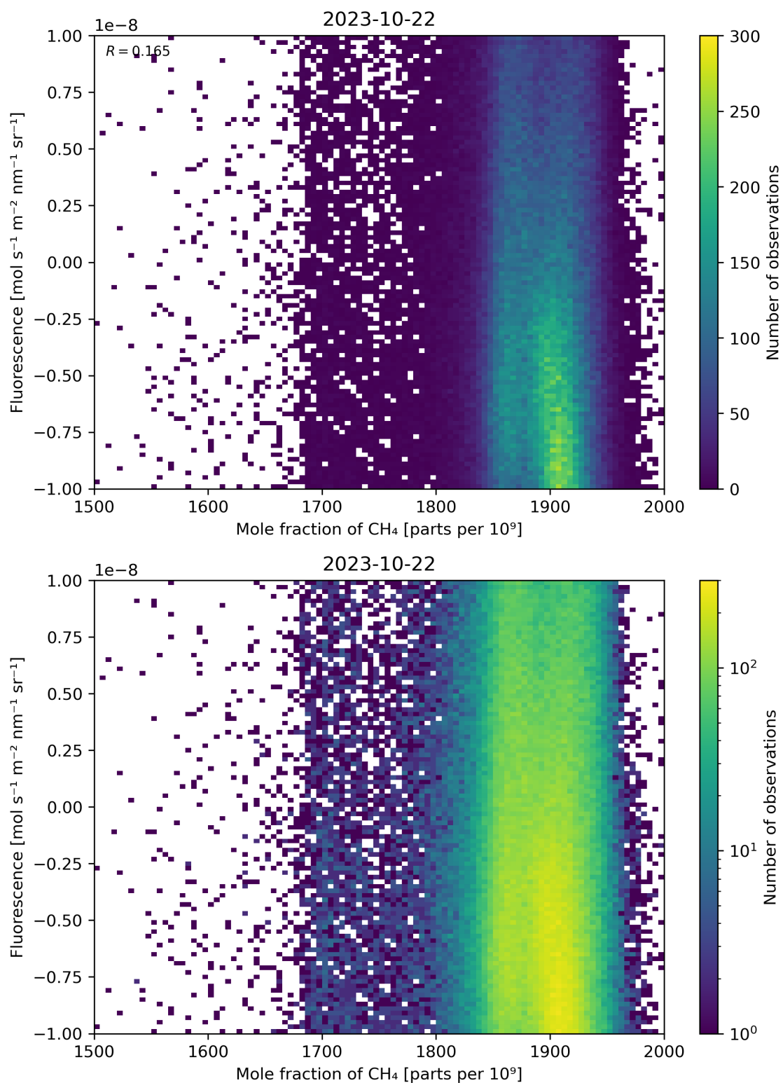
Figure 73: Scatter density plot of “Mole fraction of \text{CH}_4 ” against “Fluorescence” for 2023-10-22 to 2023-10-23.
