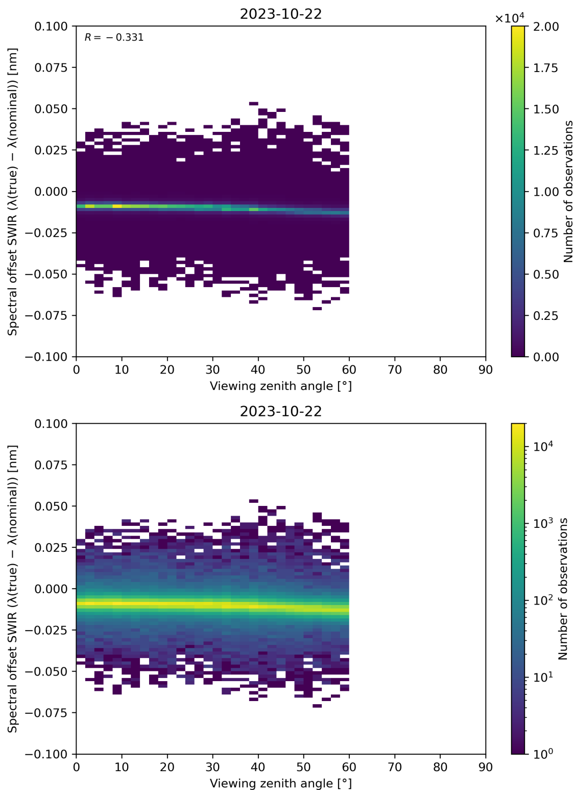
Figure 116: Scatter density plot of “Viewing zenith angle” against “Spectral offset SWIR ( \lambda(\text{true}) - \lambda(\text{nominal}) )” for 2023-10-22 to 2023-10-23.
