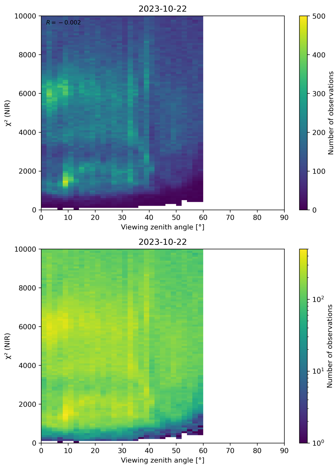
Figure 105: Scatter density plot of “Viewing zenith angle” against “ \chi^2 (NIR)” for 2023-10-22 to 2023-10-23.
