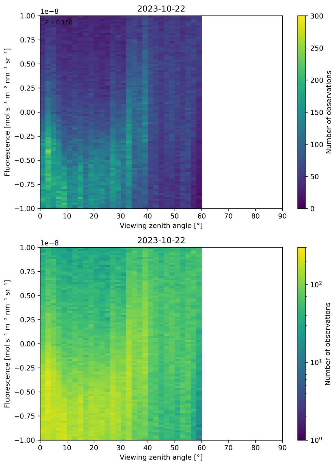
Figure 108: Scatter density plot of “Viewing zenith angle” against “Fluorescence” for 2023-10-22 to 2023-10-23.
