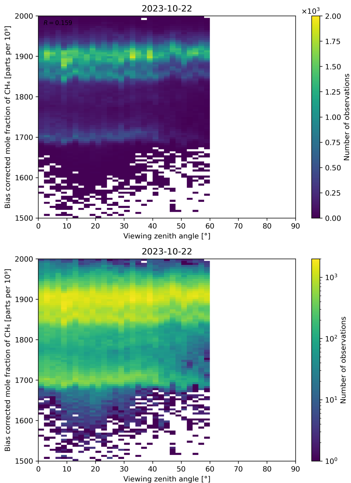
Figure 111: Scatter density plot of “Viewing zenith angle” against “Bias corrected mole fraction of CH 4 ” for 2023-10-22 to 2023-10-23.
