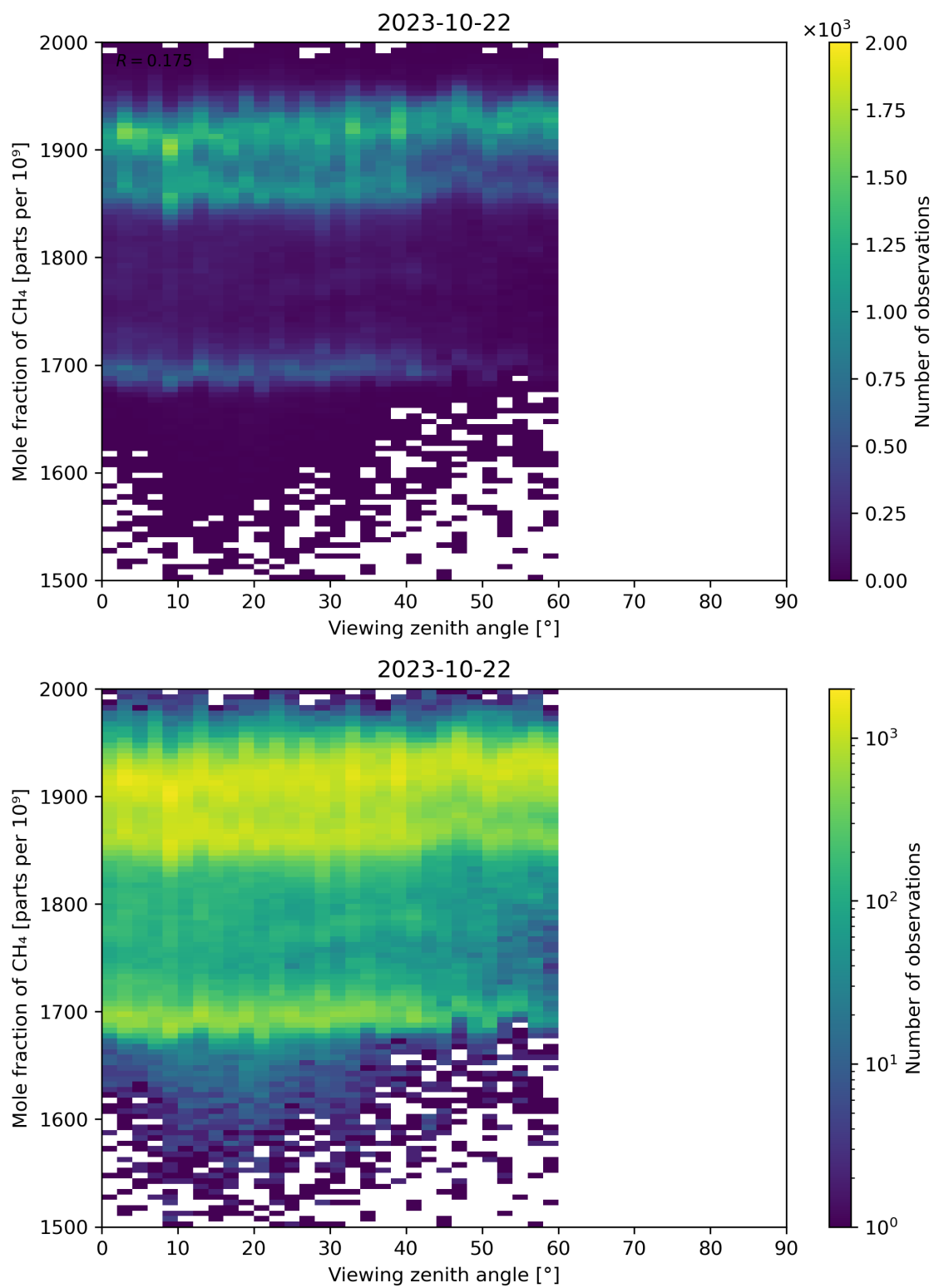
Figure 110: Scatter density plot of “Viewing zenith angle” against “Mole fraction of CH 4 ” for 2023-10-22 to 2023-10-23.
