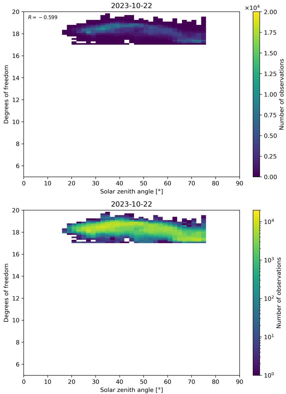
Figure 96: Scatter density plot of “Solar zenith angle” against “Degrees of freedom” for 2023-10-22 to 2023-10-23.
