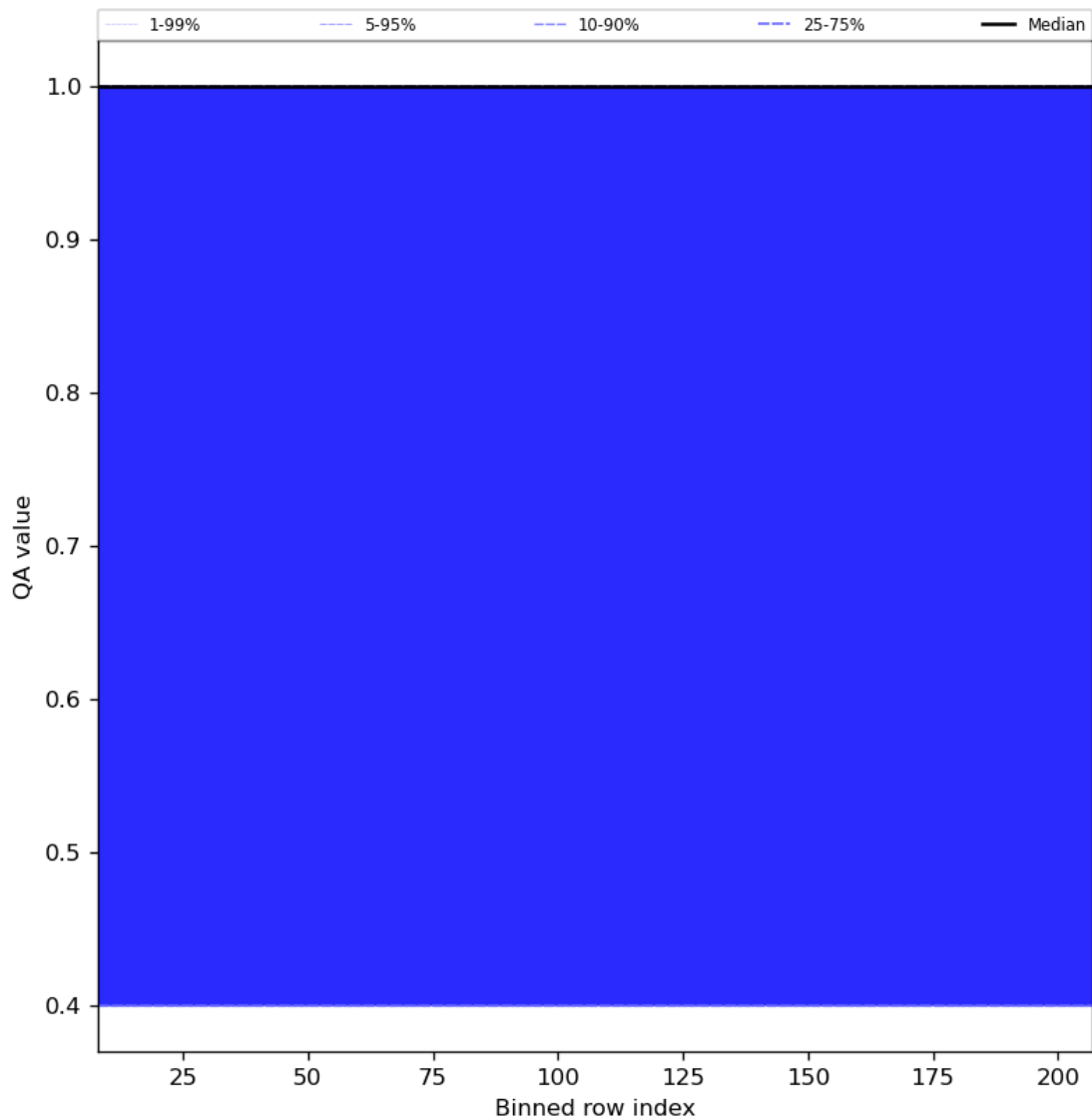
Figure 33: Along track statistics of “QA value” for 2023-10-22 to 2023-10-23
