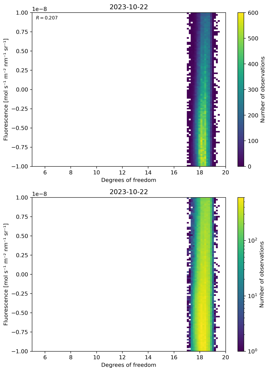
Figure 51: Scatter density plot of “Degrees of freedom” against “Fluorescence” for 2023-10-22 to 2023-10-23.
