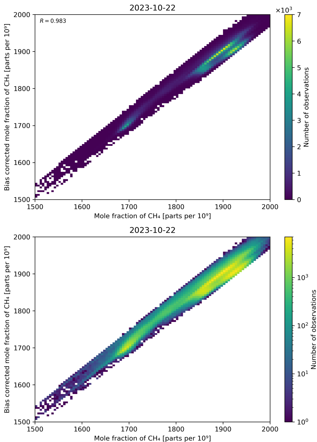
Figure 74: Scatter density plot of “Mole fraction of CH 4 ” against “Bias corrected mole fraction of CH 4 ” for 2023-10-22 to 2023-10-23.
