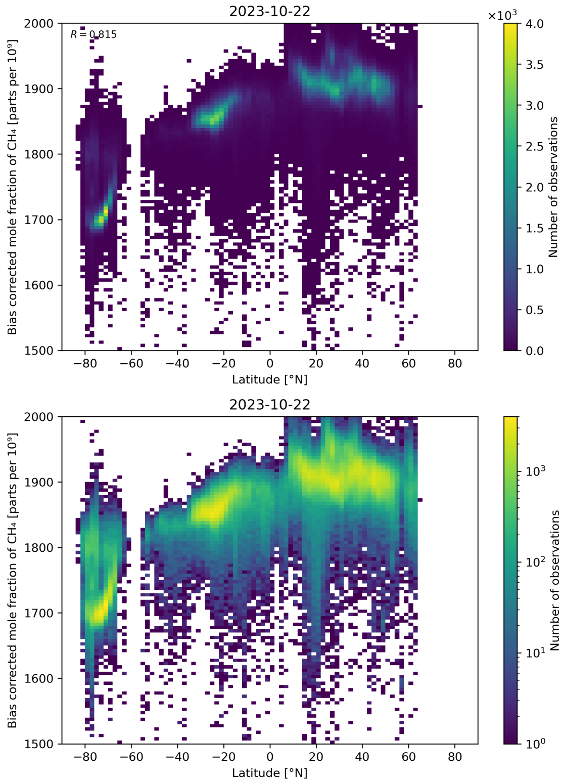
Figure 58: Scatter density plot of “Latitude” against “Bias corrected mole fraction of CH 4 ” for 2023-10-22 to 2023-10-23.
