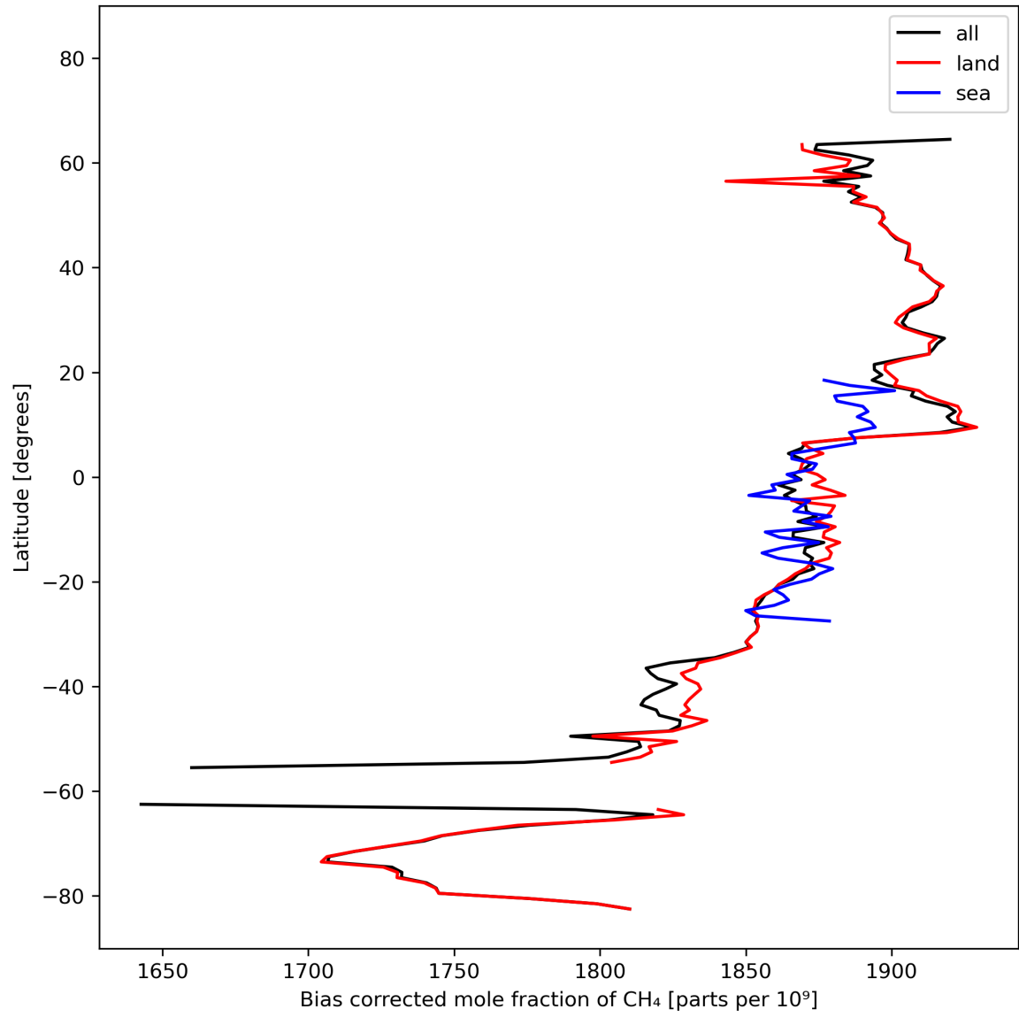
Figure 14: Zonal average of “Bias corrected mole fraction of CH 4 ” for 2023-10-22 to 2023-10-23.
