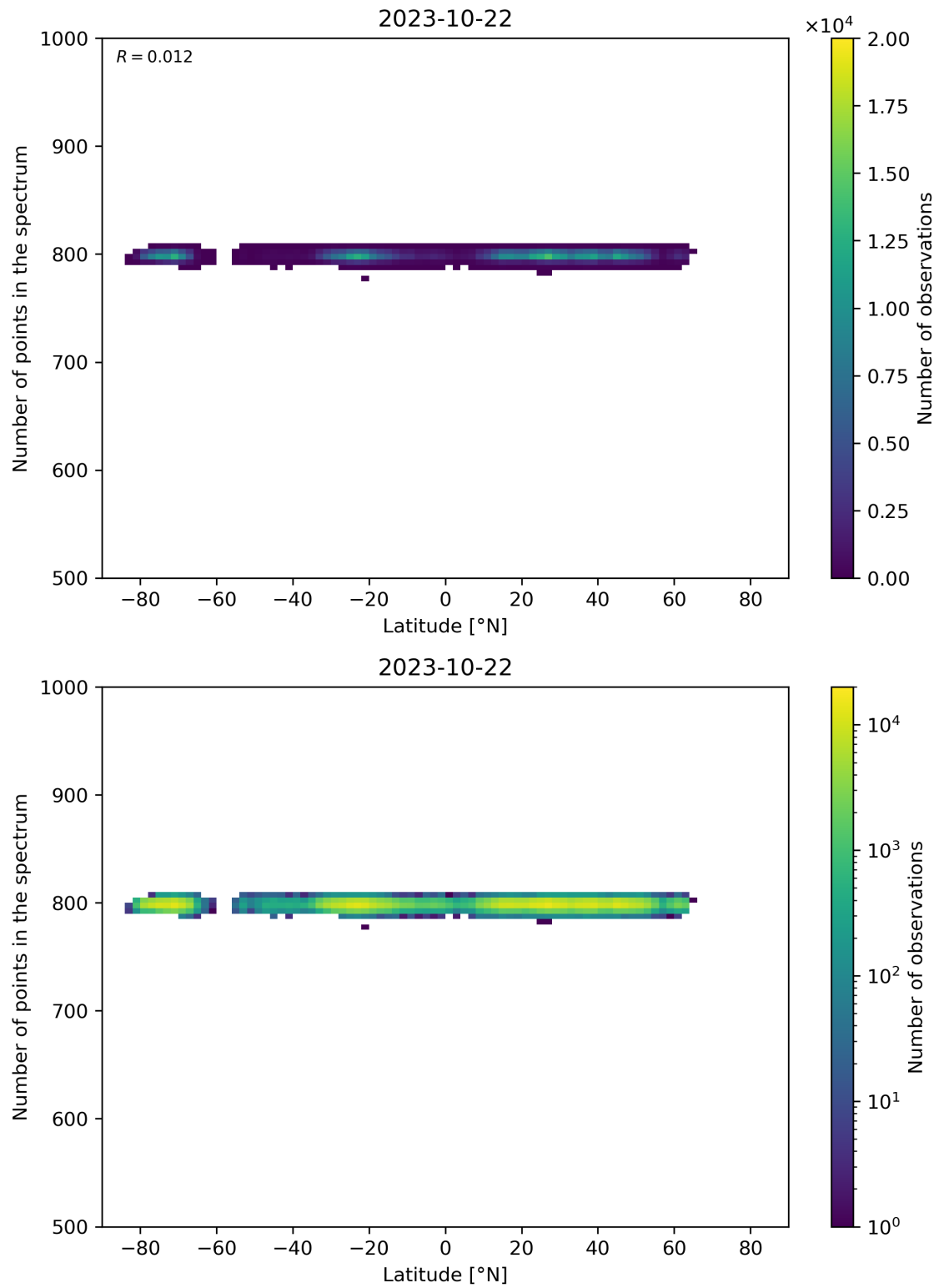
Figure 61: Scatter density plot of “Latitude” against “Number of points in the spectrum” for 2023-10-22 to 2023-10-23.
