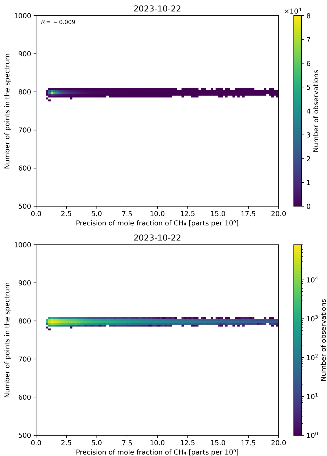
Figure 84: Scatter density plot of “Precision of mole fraction of CH 4 ” against “Number of points in the spectrum” for 2023-10-22 to 2023-10-23.
