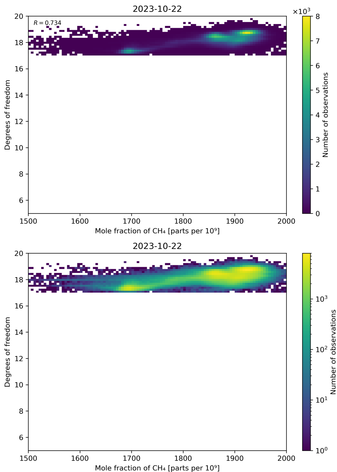
Figure 72: Scatter density plot of “Mole fraction of CH 4 ” against “Degrees of freedom” for 2023-10-22 to 2023-10-23.
