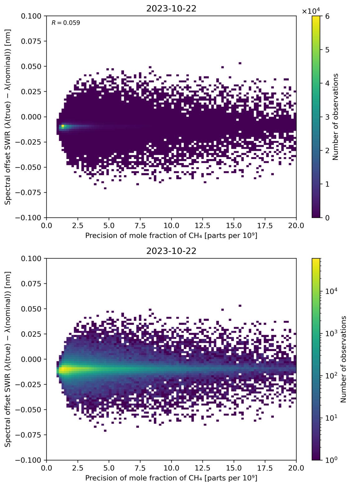
Figure 85: Scatter density plot of “Precision of mole fraction of \text{CH}_4 ” against “Spectral offset SWIR ( \lambda(\text{true}) - \lambda(\text{nominal}) )” for 2023-10-22 to 2023-10-23.
