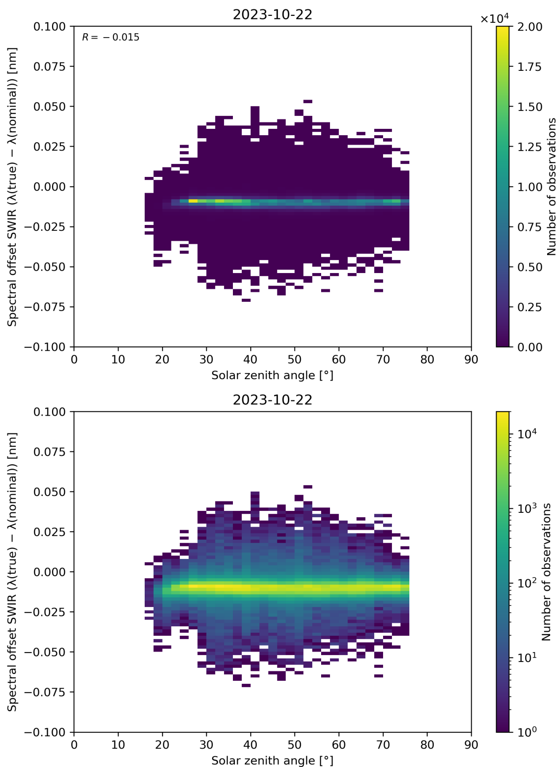
Figure 104: Scatter density plot of “Solar zenith angle” against “Spectral offset SWIR ( \lambda(\text{true}) - \lambda(\text{nominal}) )” for 2023-10-22 to 2023-10-23.
