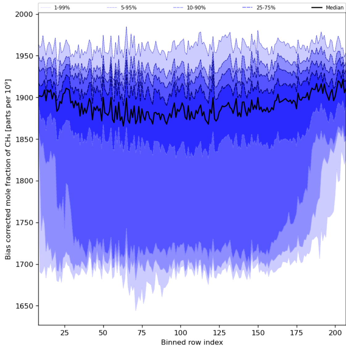
Figure 36: Along track statistics of “Bias corrected mole fraction of CH 4 ” for 2023-10-22 to 2023-10-23
