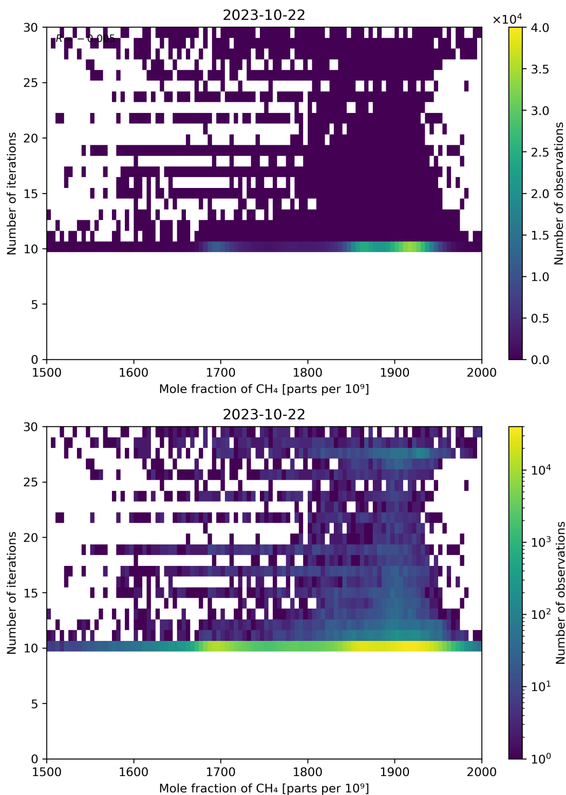
Figure 76: Scatter density plot of “Mole fraction of CH 4 ” against “Number of iterations” for 2023-10-22 to 2023-10-23.
