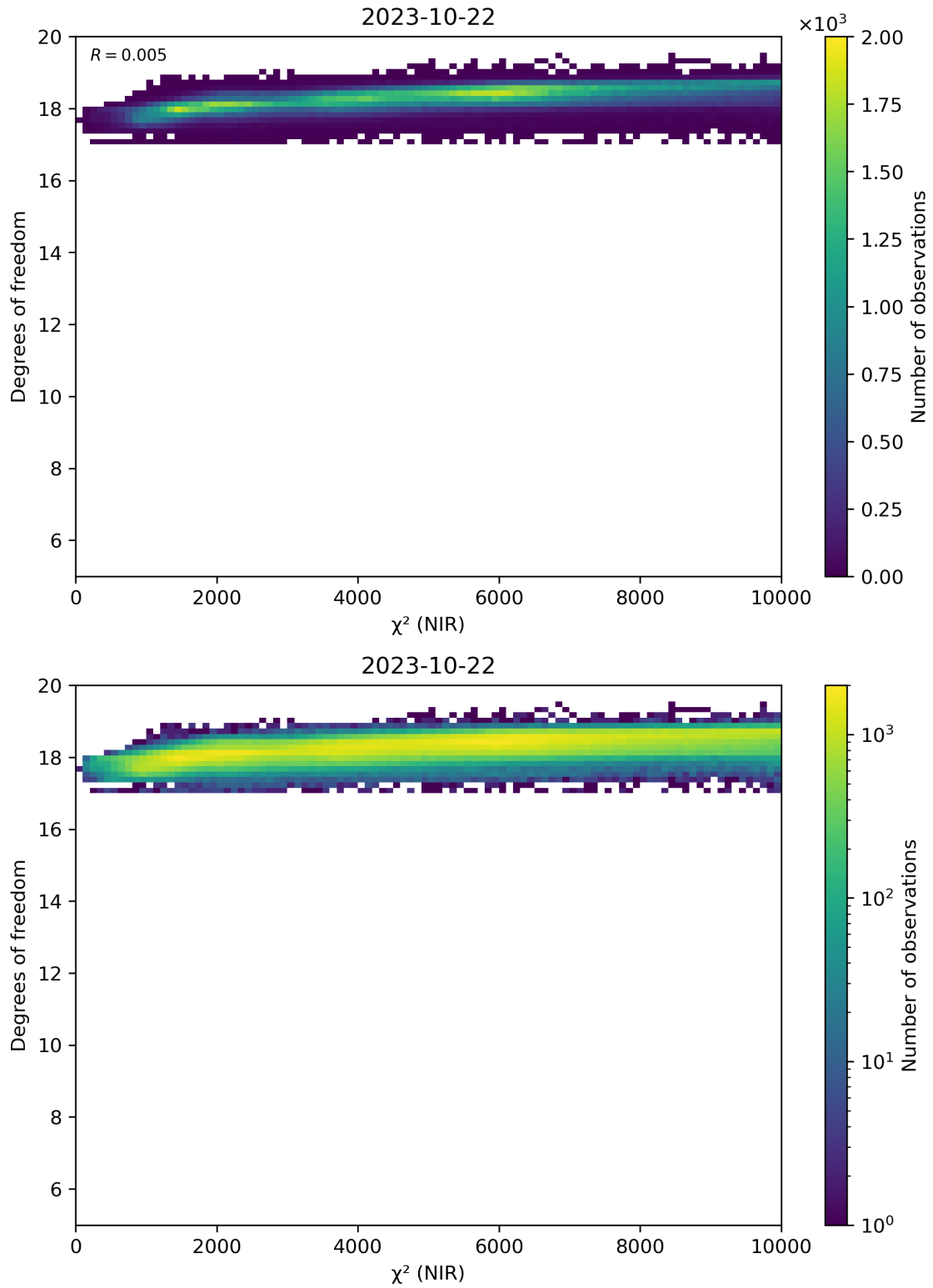
Figure 44: Scatter density plot of “ \chi^2 (NIR)” against “Degrees of freedom” for 2023-10-22 to 2023-10-23.
