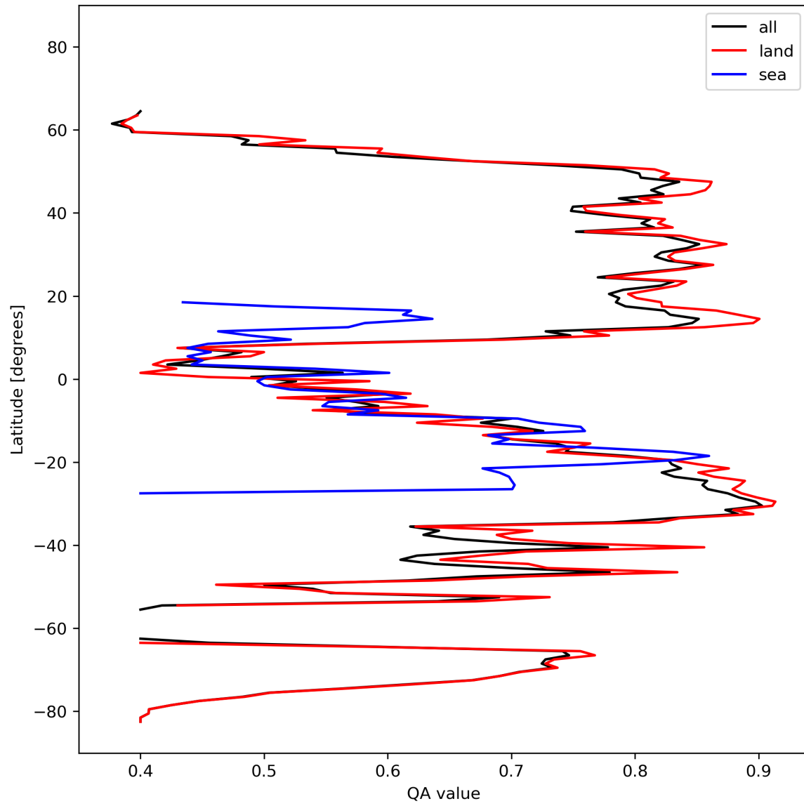
Figure 11: Zonal average of “QA value” for 2023-10-22 to 2023-10-23.
