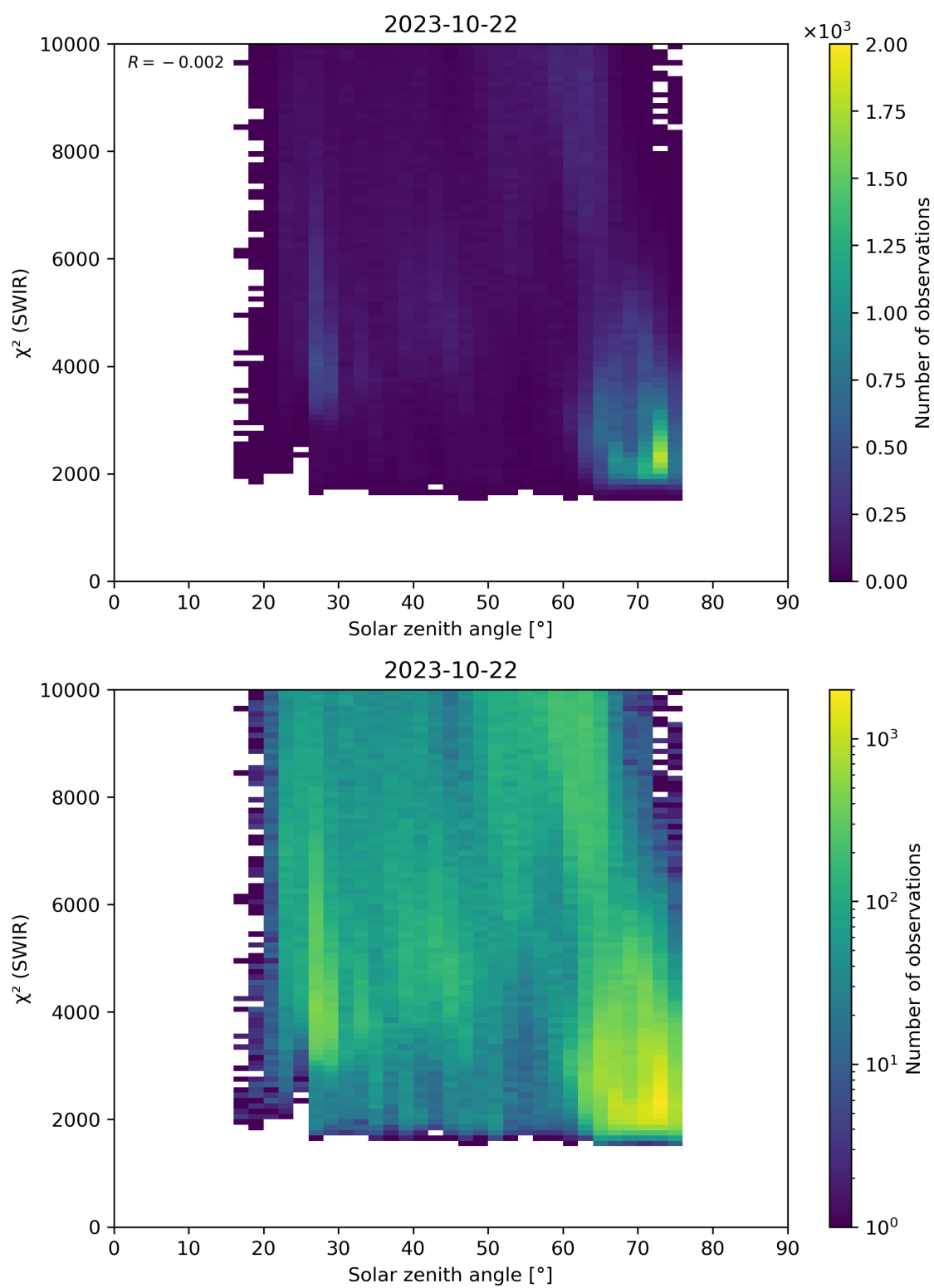
Figure 95: Scatter density plot of “Solar zenith angle” against “ \chi^2 (SWIR)” for 2023-10-22 to 2023-10-23.
