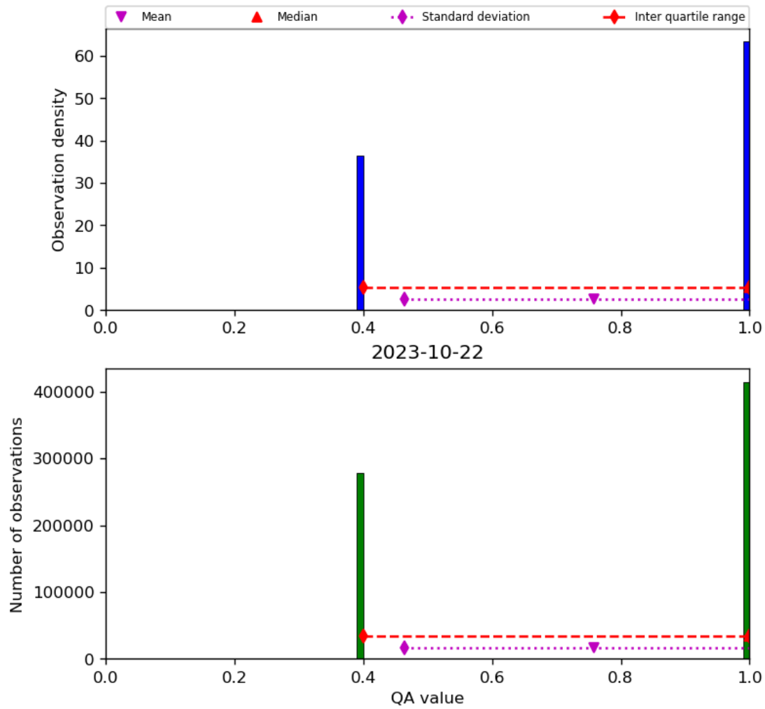
Figure 22: Histogram of “QA value” for 2023-10-22 to 2023-10-23
