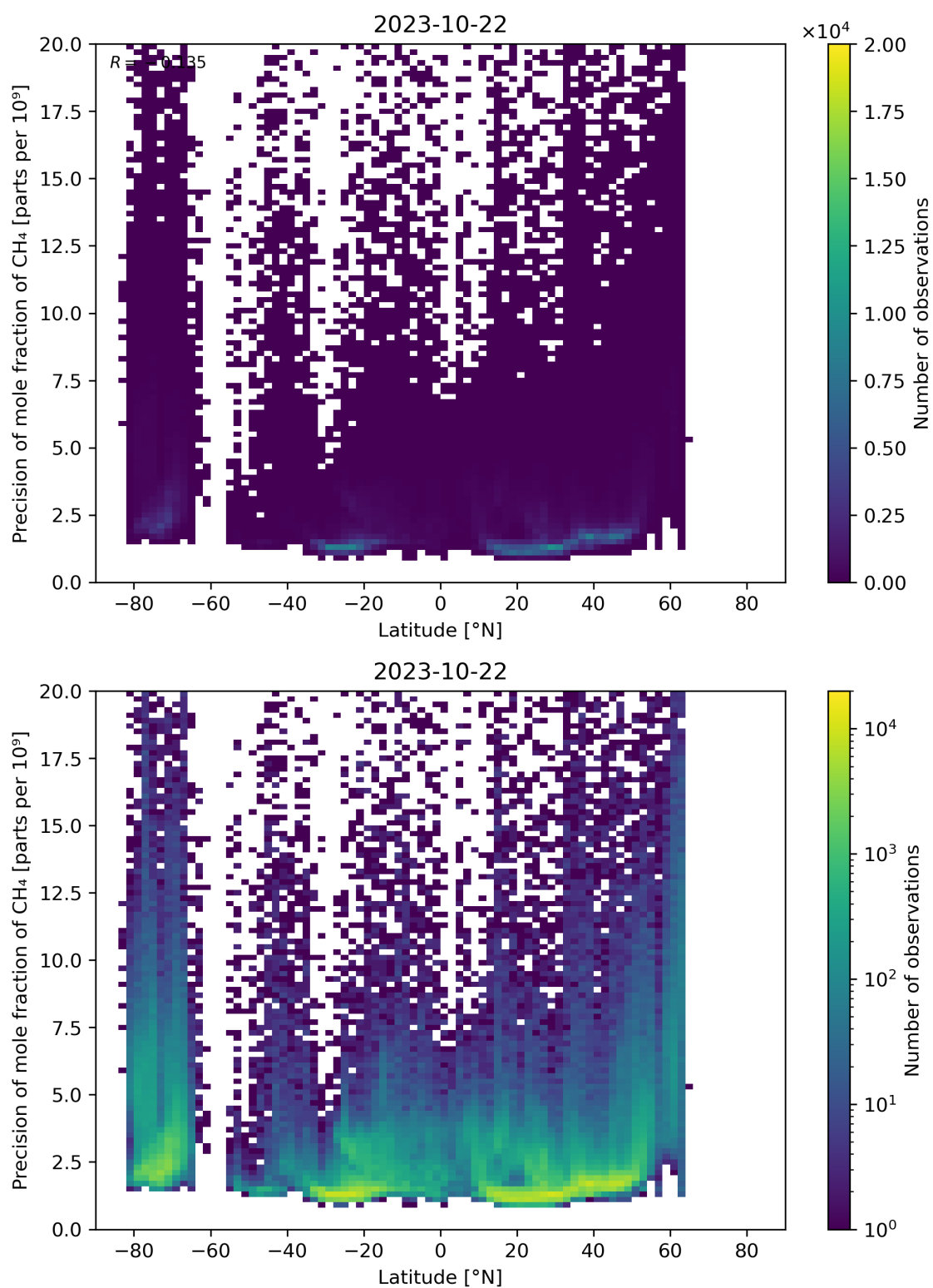
Figure 59: Scatter density plot of “Latitude” against “Precision of mole fraction of CH 4 ” for 2023-10-22 to 2023-10-23.
