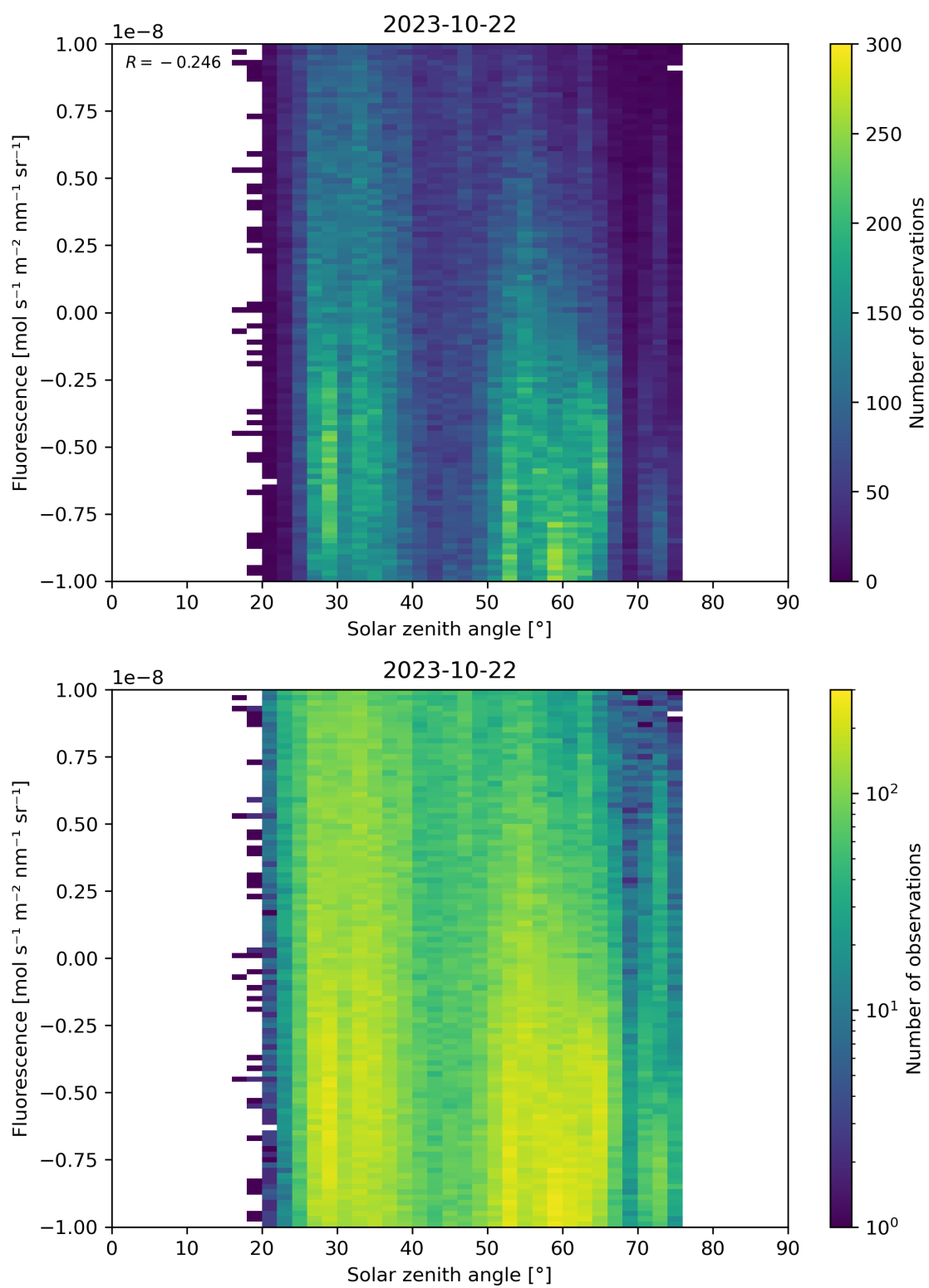
Figure 97: Scatter density plot of “Solar zenith angle” against “Fluorescence” for 2023-10-22 to 2023-10-23.
