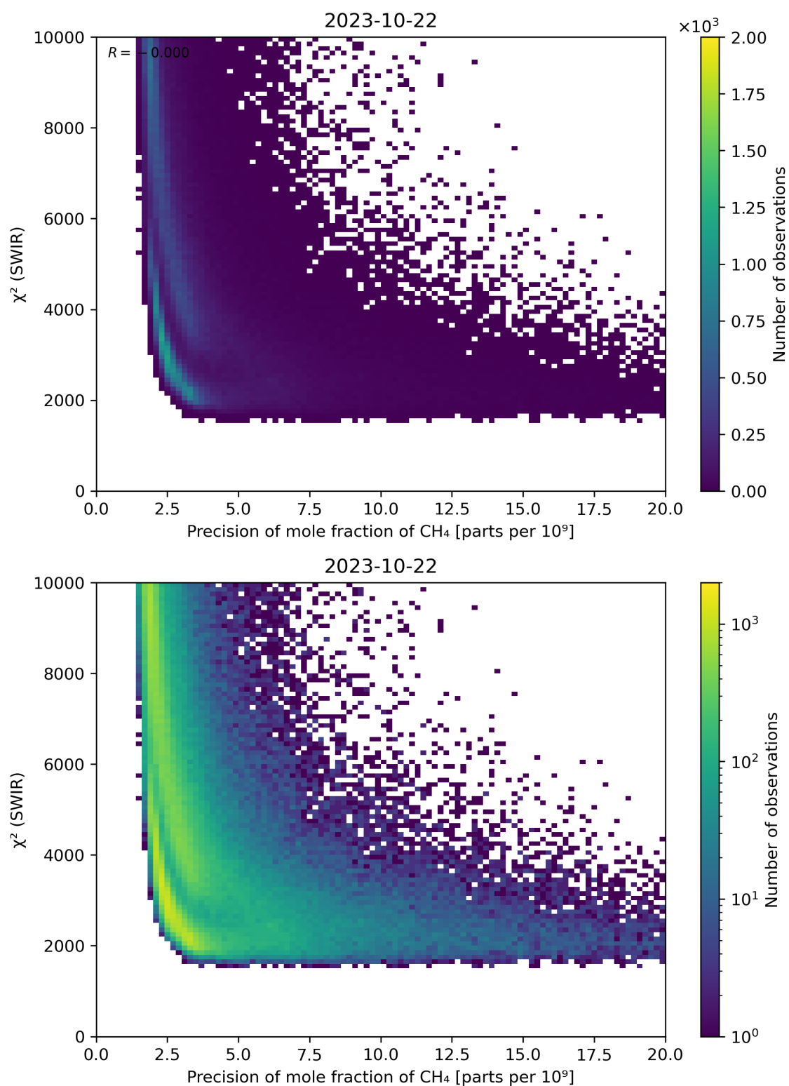
Figure 79: Scatter density plot of “Precision of mole fraction of CH 4 ” against “ \chi^2 (SWIR)” for 2023-10-22 to 2023-10-23.
