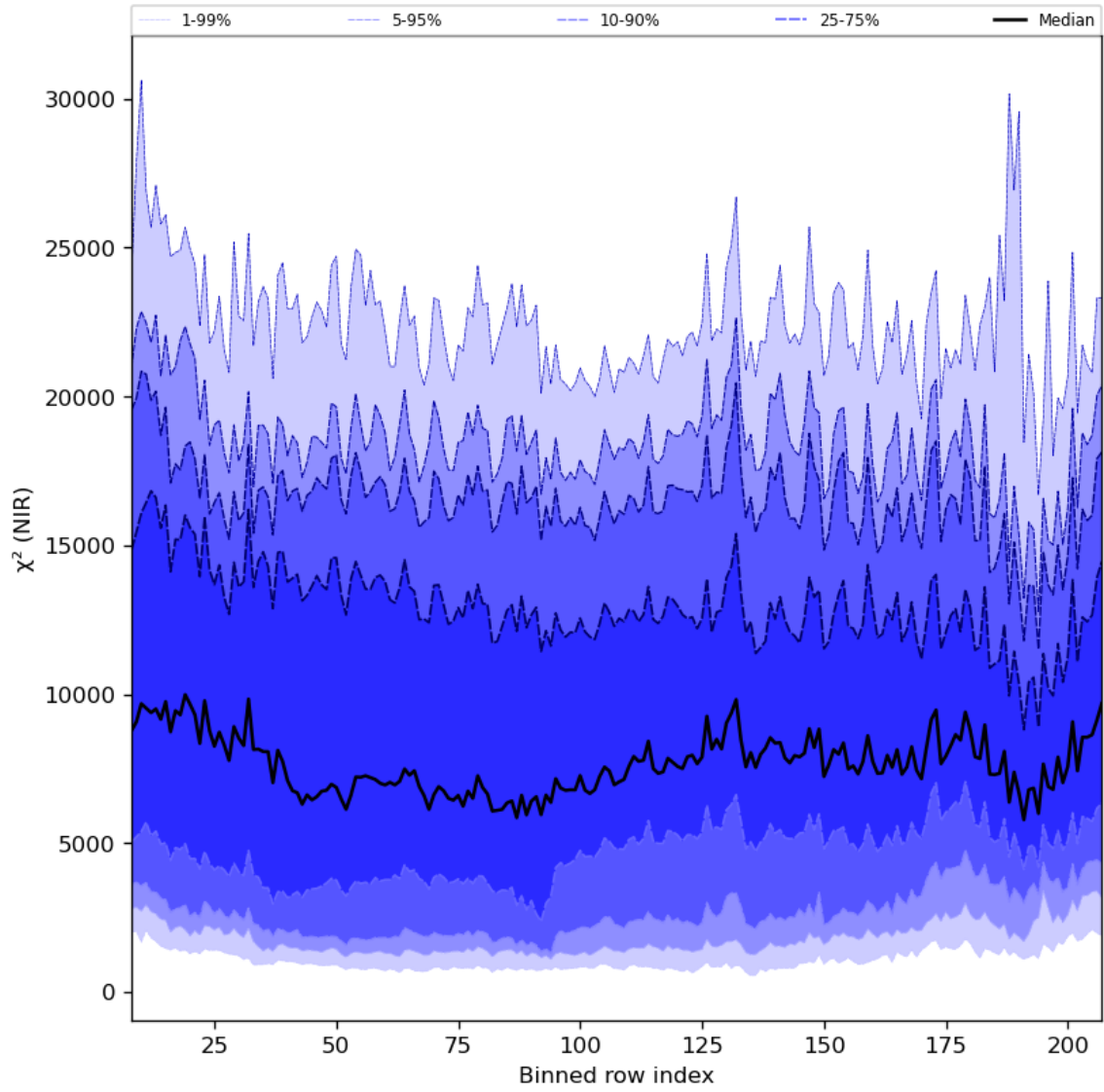
Figure 40: Along track statistics of “ \chi^2 (NIR)” for 2023-10-22 to 2023-10-23
