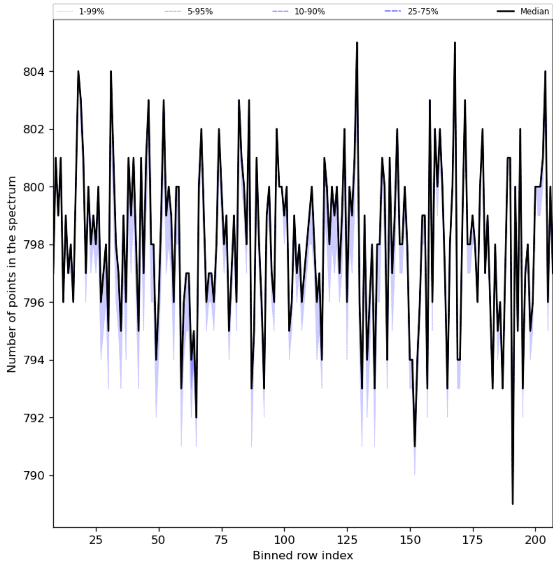
Figure 37: Along track statistics of “Number of points in the spectrum” for 2023-10-22 to 2023-10-23
