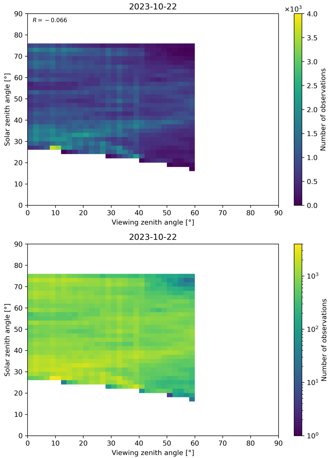
Figure 115: Scatter density plot of “Viewing zenith angle” against “Solar zenith angle” for 2023-10-22 to 2023-10-23.
