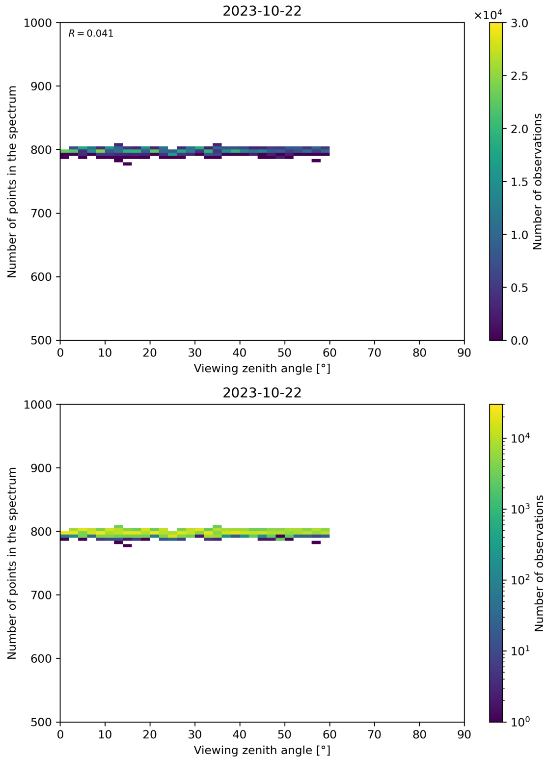
Figure 114: Scatter density plot of “Viewing zenith angle” against “Number of points in the spectrum” for 2023-10-22 to 2023-10-23.
