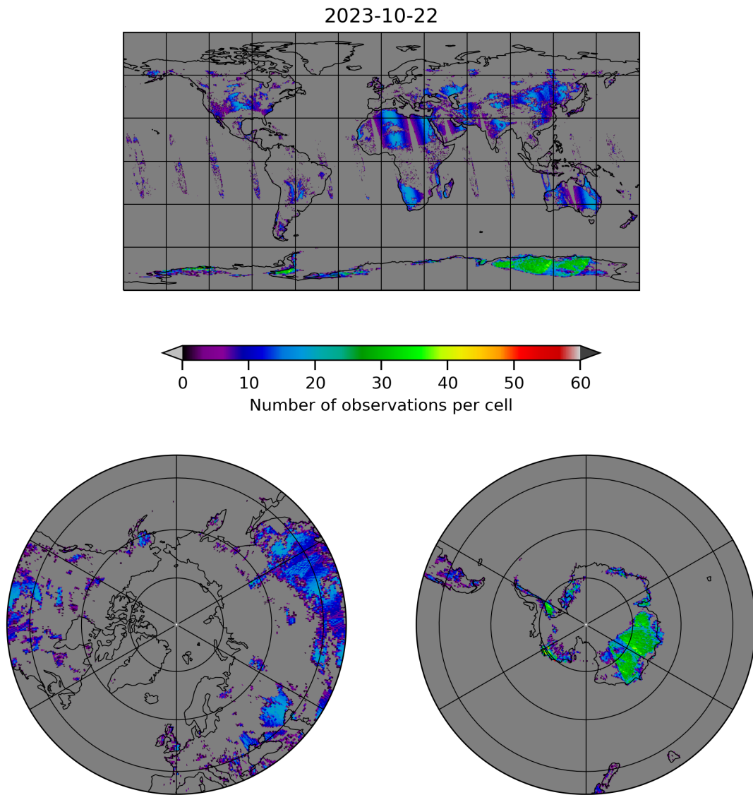
Figure 10: Map of the number of observations for 2023-10-22 to 2023-10-23
