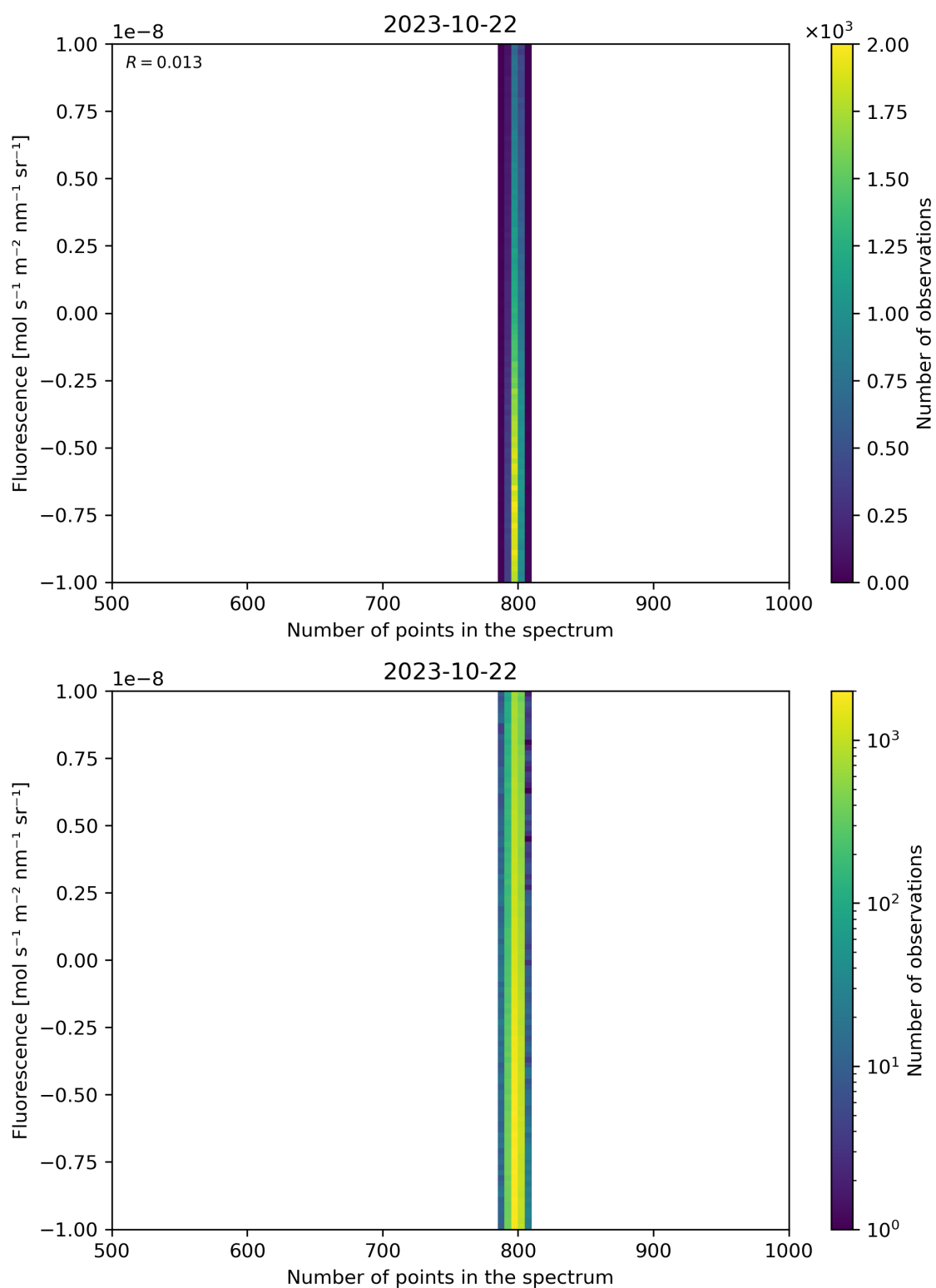
Figure 91: Scatter density plot of “Number of points in the spectrum” against “Fluorescence” for 2023-10-22 to 2023-10-23.
