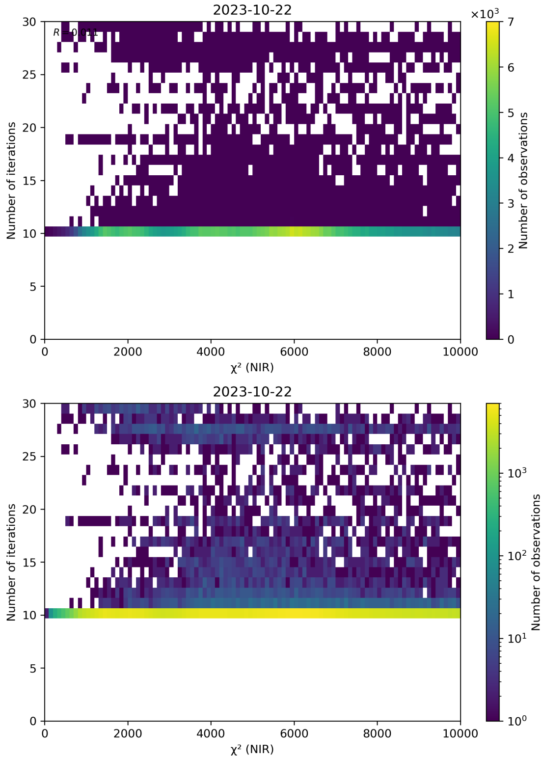
Figure 46: Scatter density plot of “ \chi^2 (NIR)” against “Number of iterations” for 2023-10-22 to 2023-10-23.
