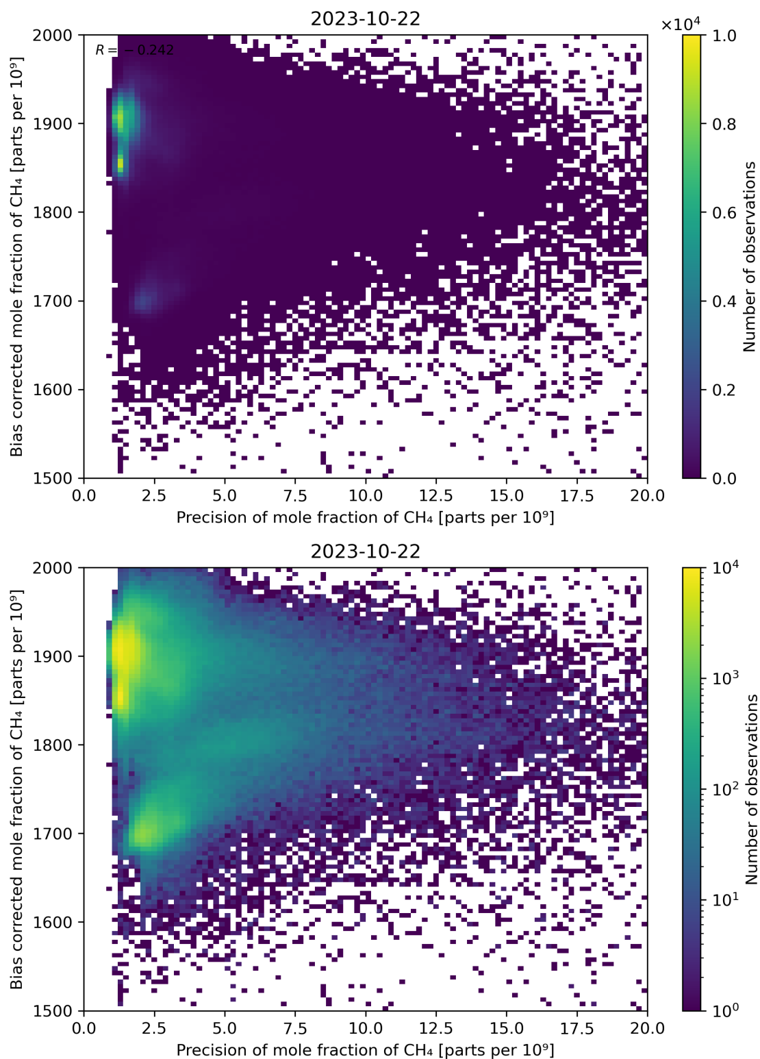
Figure 82: Scatter density plot of “Precision of mole fraction of \text{CH}_4 ” against “Bias corrected mole fraction of \text{CH}_4 ” for 2023-10-22 to 2023-10-23.
