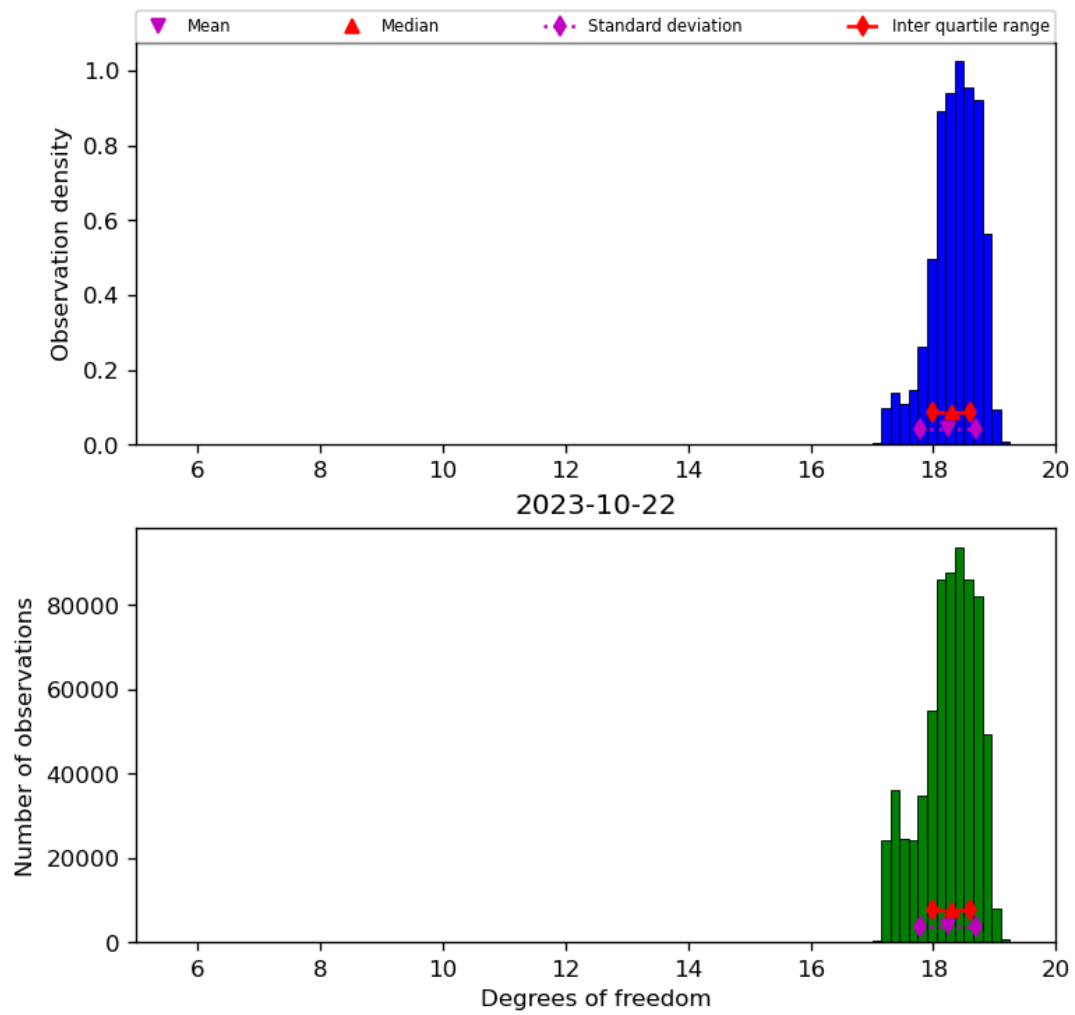
Figure 30: Histogram of “Degrees of freedom” for 2023-10-22 to 2023-10-23
