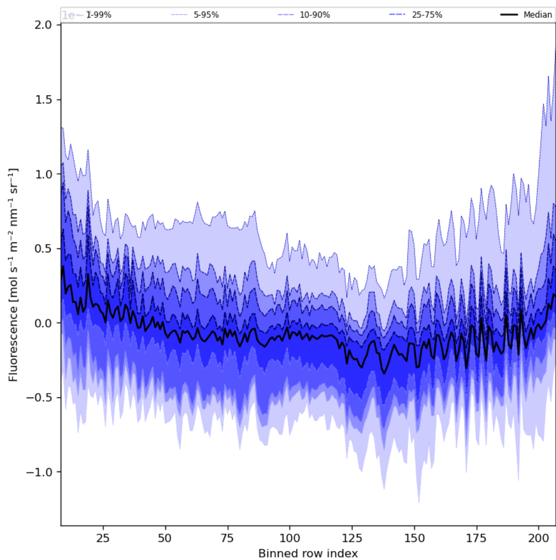
Figure 43: Along track statistics of “Fluorescence” for 2023-10-22 to 2023-10-23
