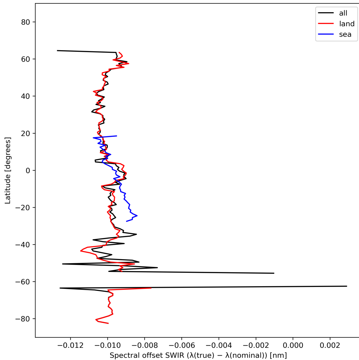
Figure 16: Zonal average of “Spectral offset SWIR ( \lambda(\text{true}) - \lambda(\text{nominal}) )” for 2023-10-22 to 2023-10-23.
