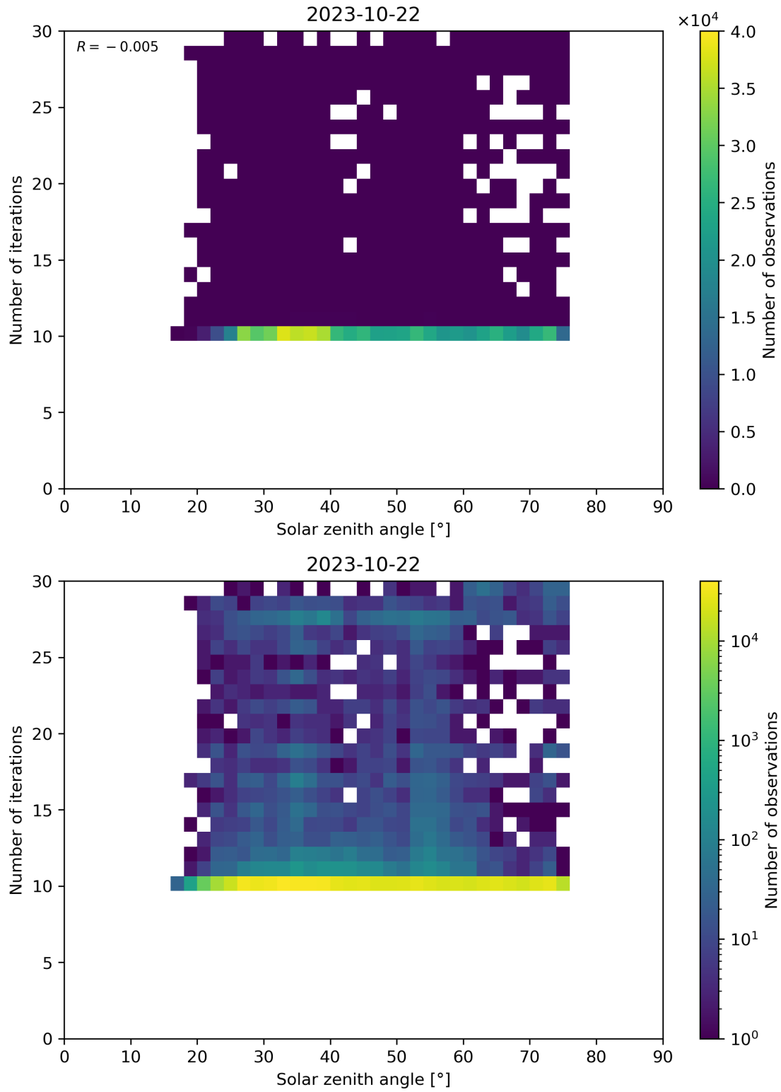
Figure 102: Scatter density plot of “Solar zenith angle” against “Number of iterations” for 2023-10-22 to 2023-10-23.
