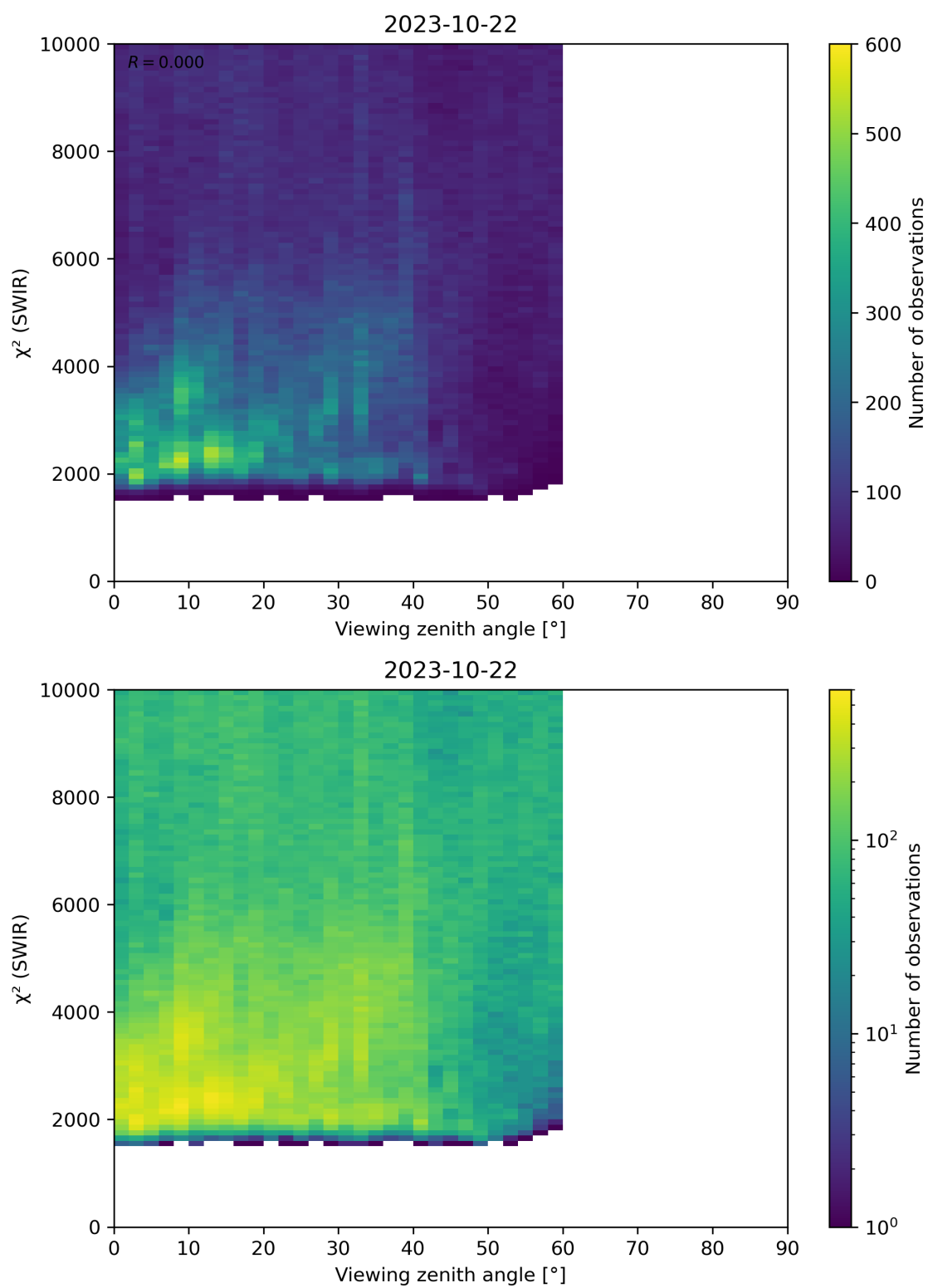
Figure 106: Scatter density plot of “Viewing zenith angle” against “ \chi^2 (SWIR)” for 2023-10-22 to 2023-10-23.
