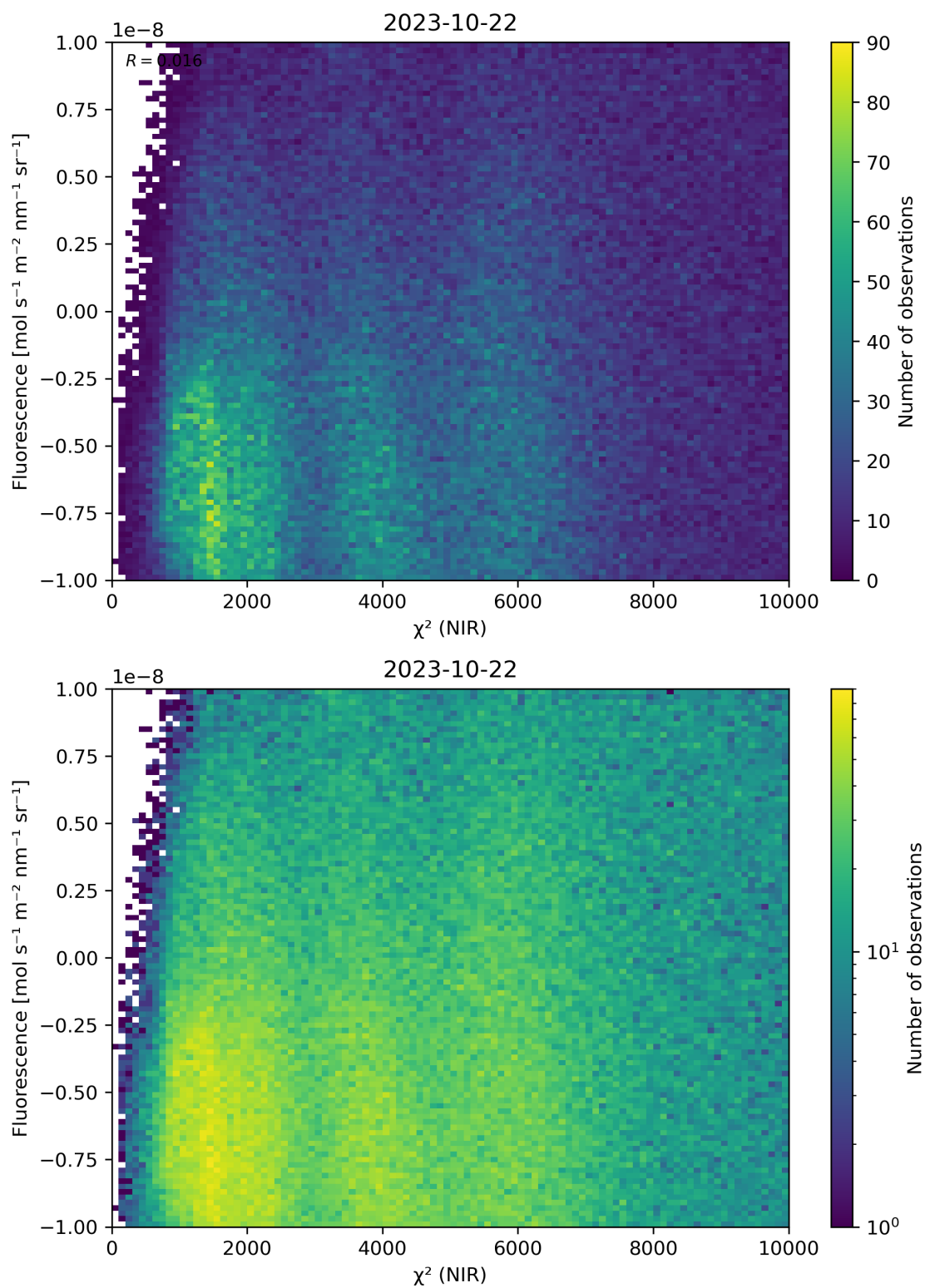
Figure 45: Scatter density plot of “ \chi^2 (NIR)” against “Fluorescence” for 2023-10-22 to 2023-10-23.
