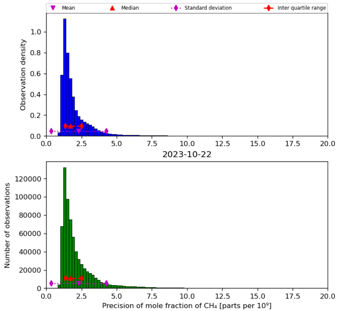
Figure 24: Histogram of “Precision of mole fraction of CH 4 ” for 2023-10-22 to 2023-10-23
