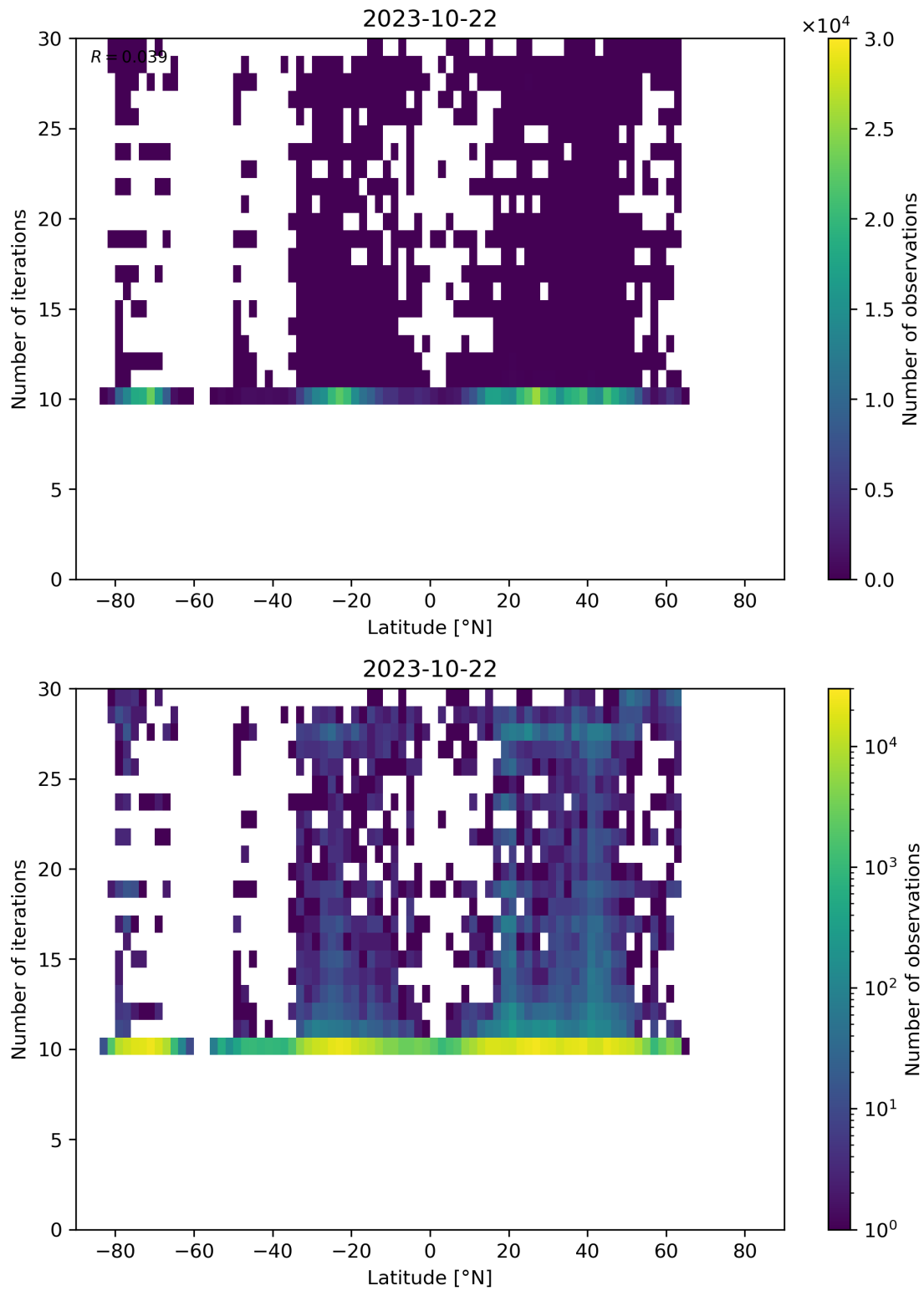
Figure 60: Scatter density plot of “Latitude” against “Number of iterations” for 2023-10-22 to 2023-10-23.
