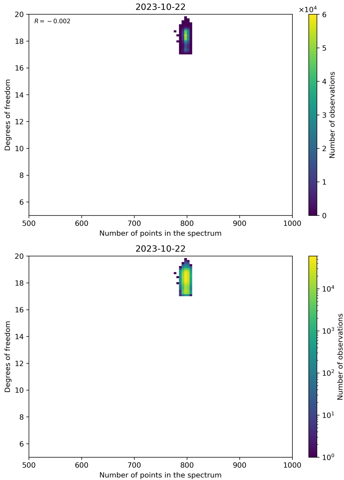
Figure 90: Scatter density plot of “Number of points in the spectrum” against “Degrees of freedom” for 2023-10-22 to 2023-10-23.
