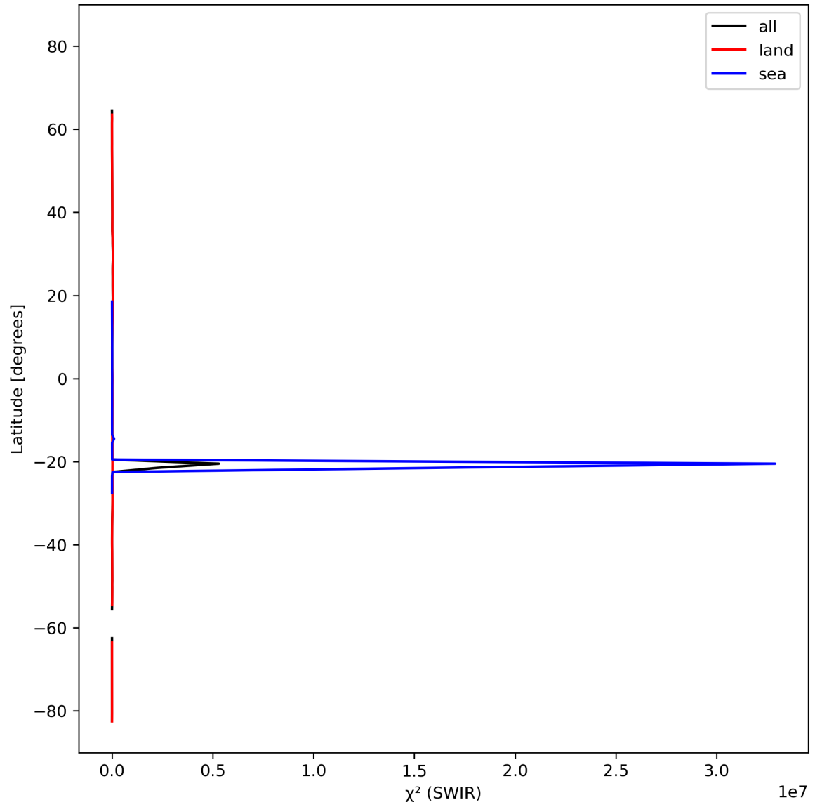
Figure 17: Zonal average of “ \chi^2 (SWIR)” for 2023-10-22 to 2023-10-23.
