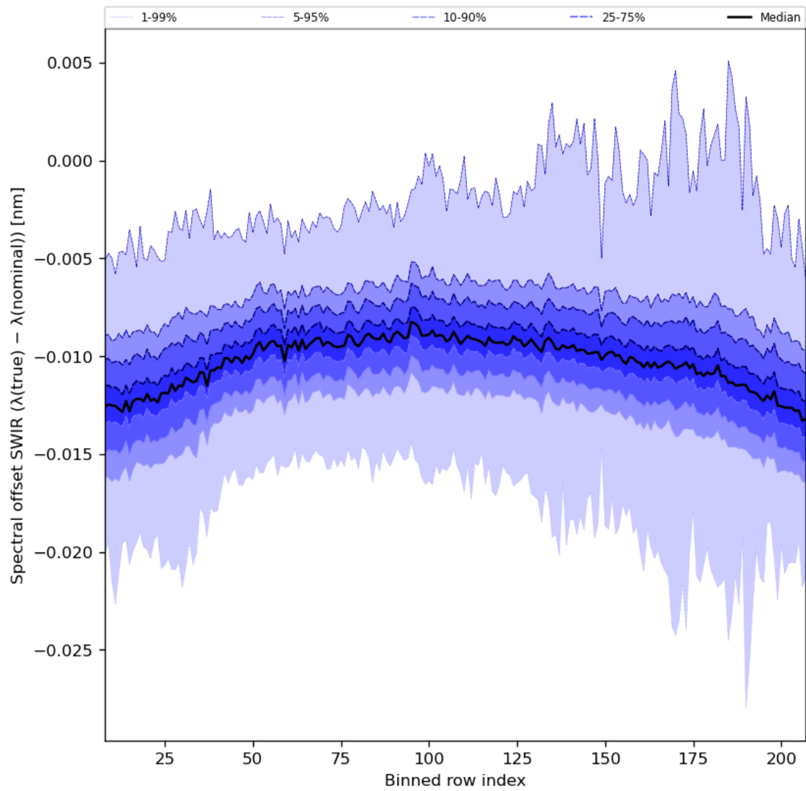
Figure 38: Along track statistics of “Spectral offset SWIR ( \lambda(\text{true}) - \lambda(\text{nominal}) )” for 2023-10-22 to 2023-10-23
