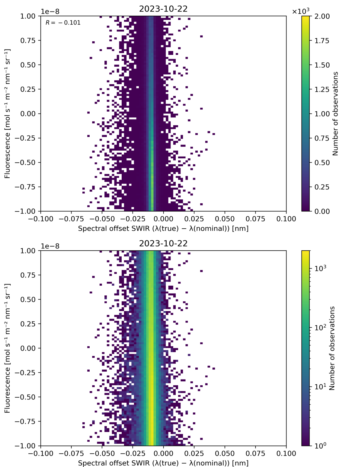
Figure 120: Scatter density plot of “Spectral offset SWIR ( \lambda(\text{true}) - \lambda(\text{nominal}) )” against “Fluorescence” for 2023-10-22 to 2023-10-23.
