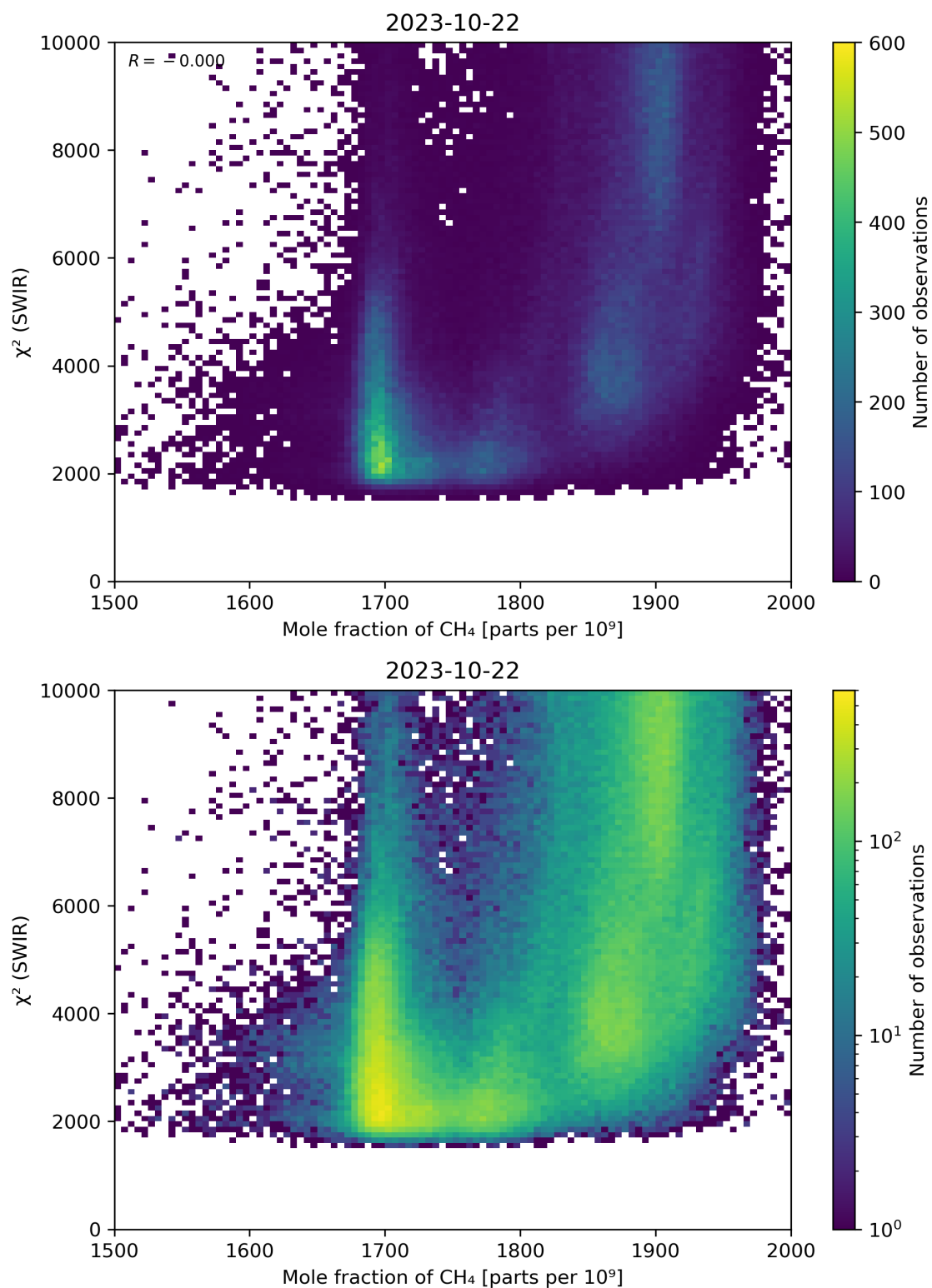
Figure 71: Scatter density plot of “Mole fraction of CH 4 ” against “ \chi^2 (SWIR)” for 2023-10-22 to 2023-10-23.
