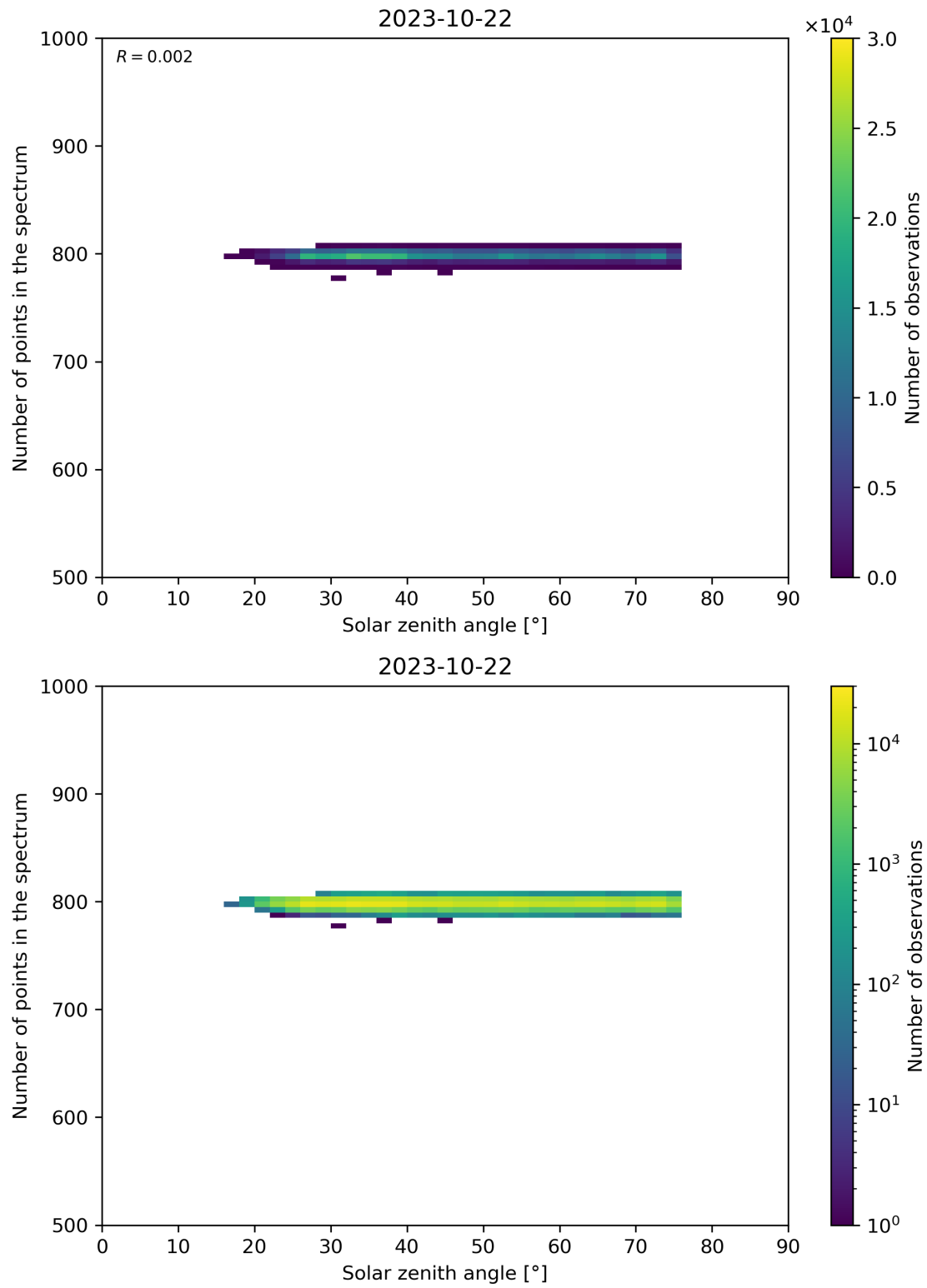
Figure 103: Scatter density plot of “Solar zenith angle” against “Number of points in the spectrum” for 2023-10-22 to 2023-10-23.
