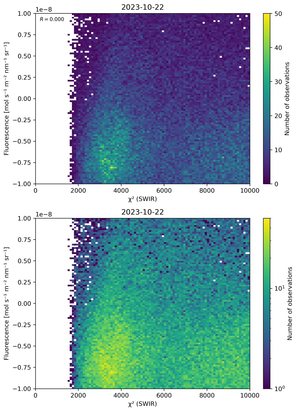
Figure 49: Scatter density plot of “ \chi^2 (SWIR)” against “Fluorescence” for 2023-10-22 to 2023-10-23.
