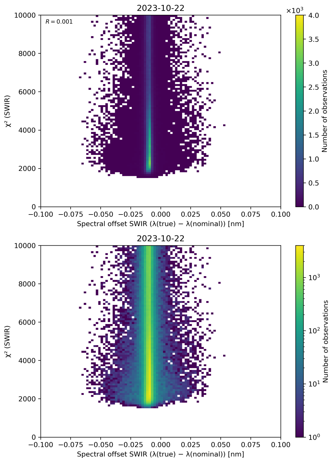
Figure 118: Scatter density plot of “Spectral offset SWIR ( \lambda(\text{true}) - \lambda(\text{nominal}) )” against “ \chi^2 (SWIR)” for 2023-10-22 to 2023-10-23.
