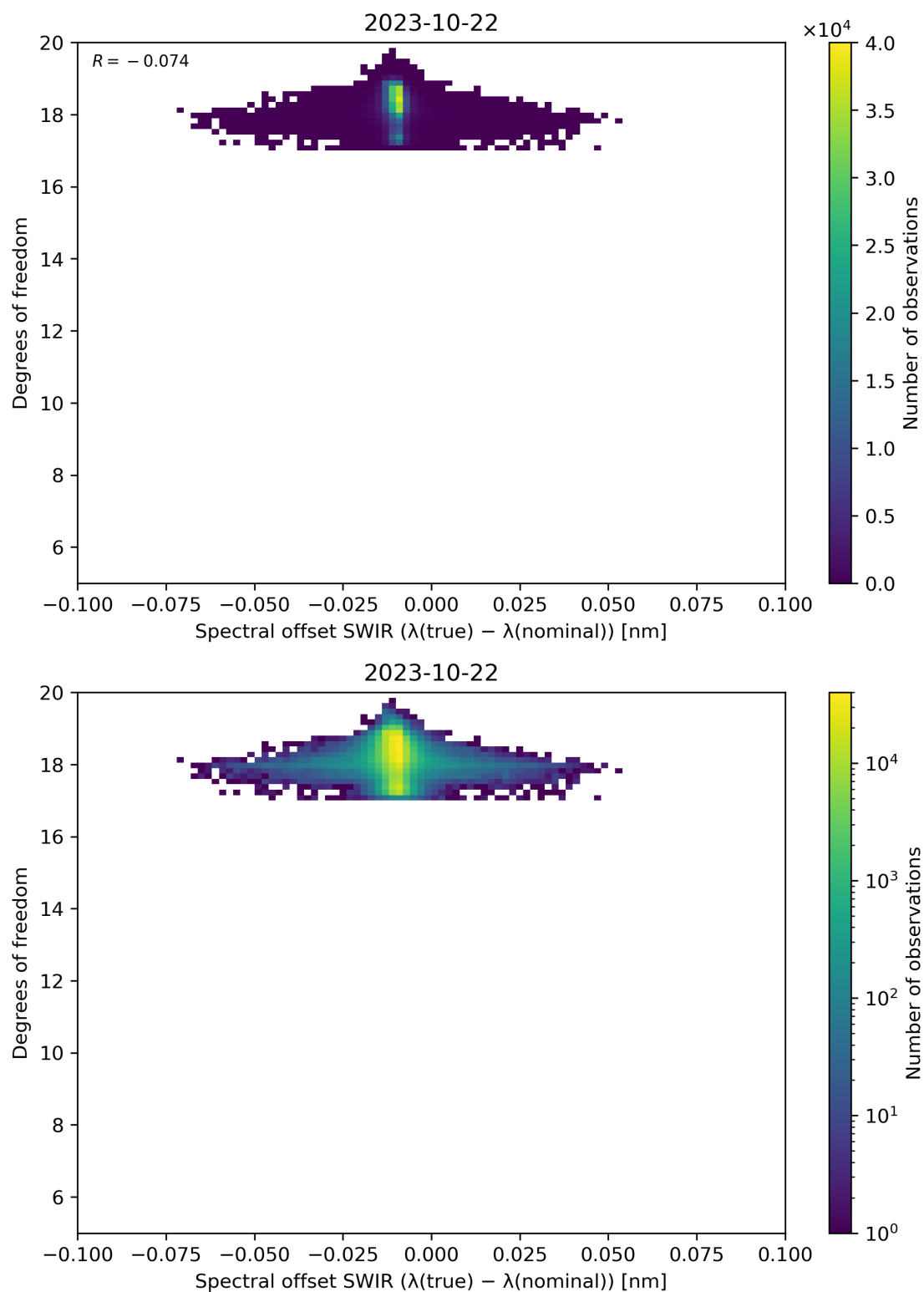
Figure 119: Scatter density plot of “Spectral offset SWIR ( \lambda(\text{true}) - \lambda(\text{nominal}) )” against “Degrees of freedom” for 2023-10-22 to 2023-10-23.
