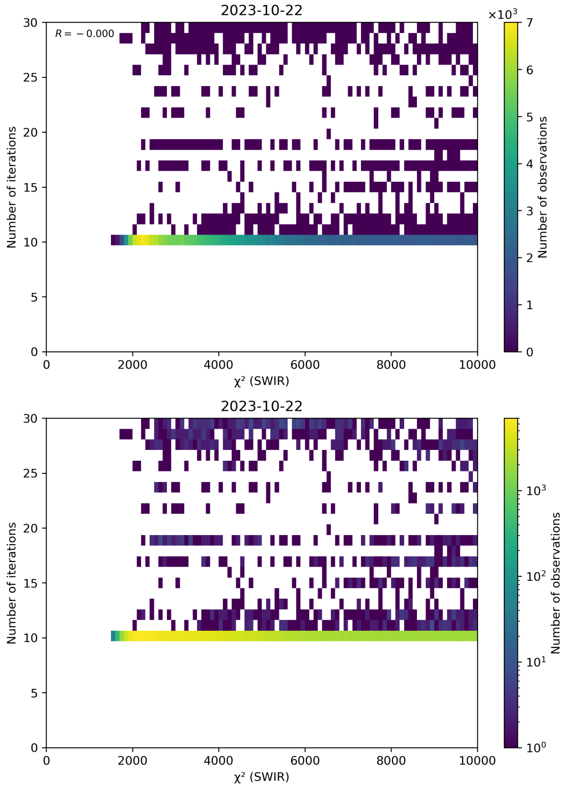
Figure 50: Scatter density plot of “ \chi^2 (SWIR)” against “Number of iterations” for 2023-10-22 to 2023-10-23.
