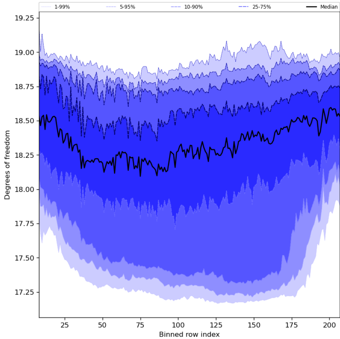
Figure 41: Along track statistics of “Degrees of freedom” for 2023-10-22 to 2023-10-23
