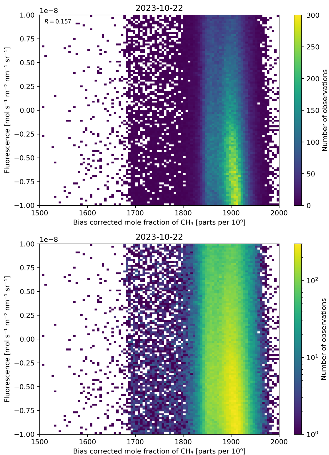
Figure 66: Scatter density plot of “Bias corrected mole fraction of \text{CH}_4 ” against “Fluorescence” for 2023-10-22 to 2023-10-23.
