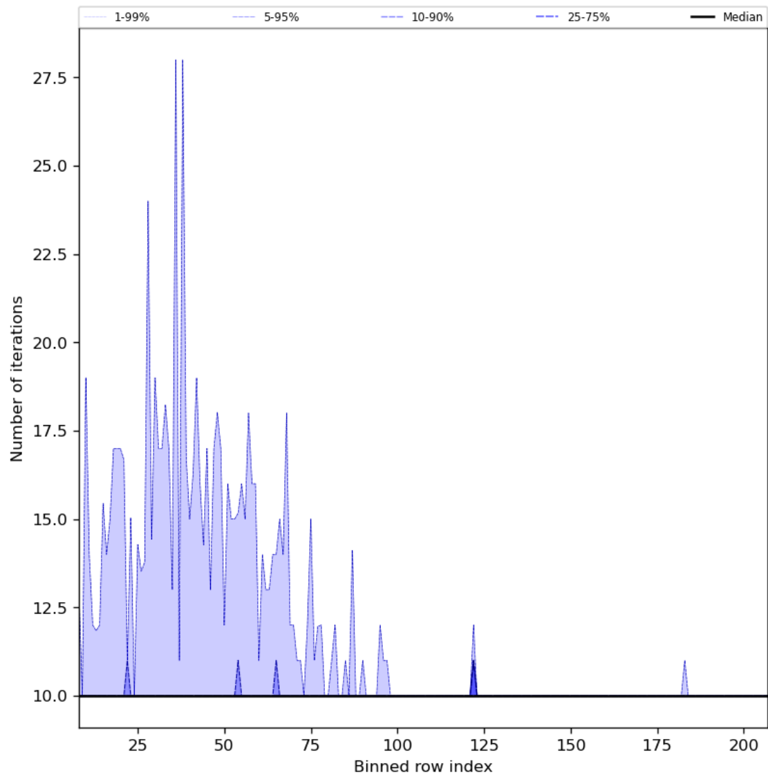
Figure 42: Along track statistics of “Number of iterations” for 2023-10-22 to 2023-10-23
