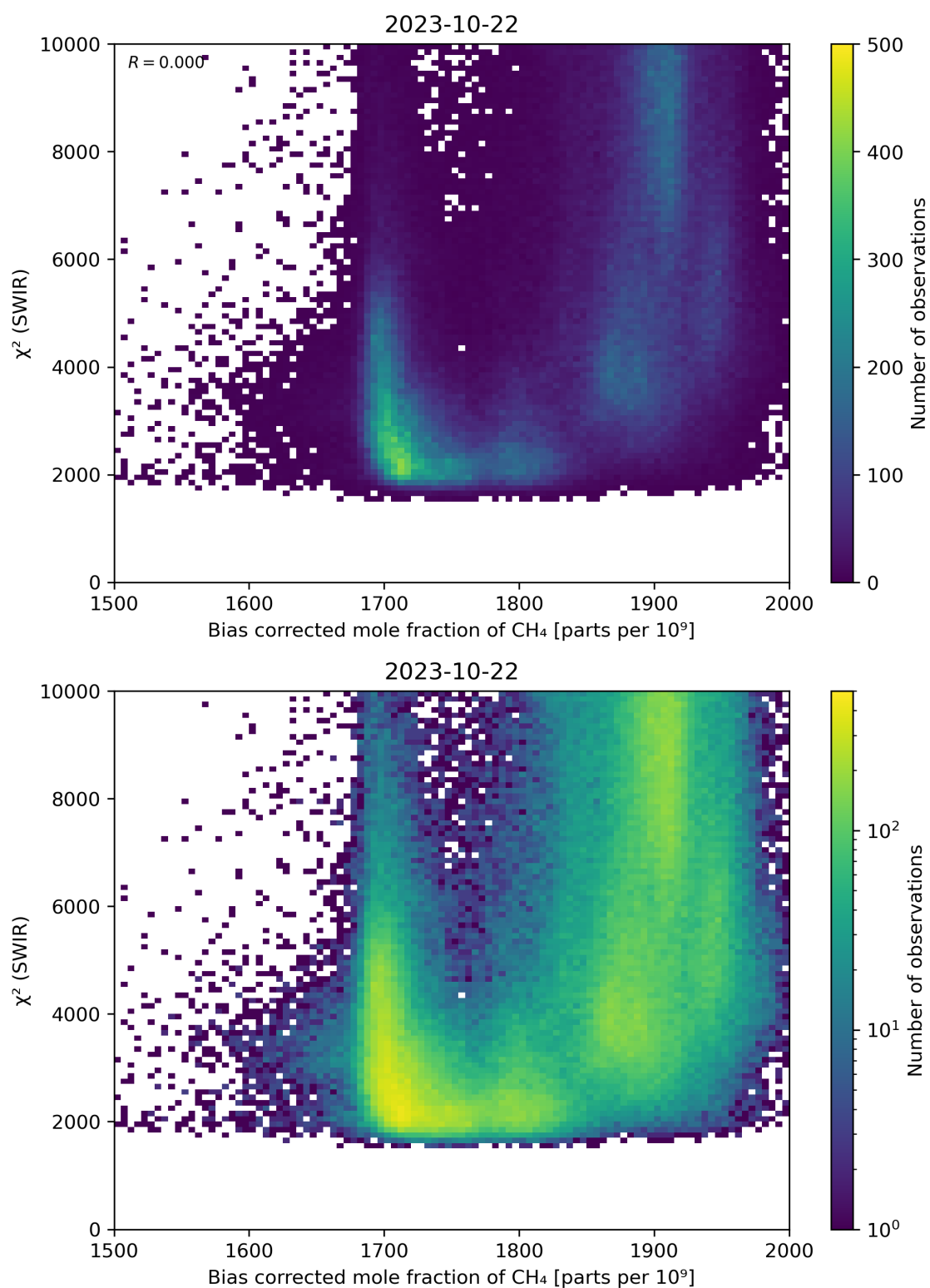
Figure 64: Scatter density plot of “Bias corrected mole fraction of CH 4 ” against “ \chi^2 (SWIR)” for 2023-10-22 to 2023-10-23.
