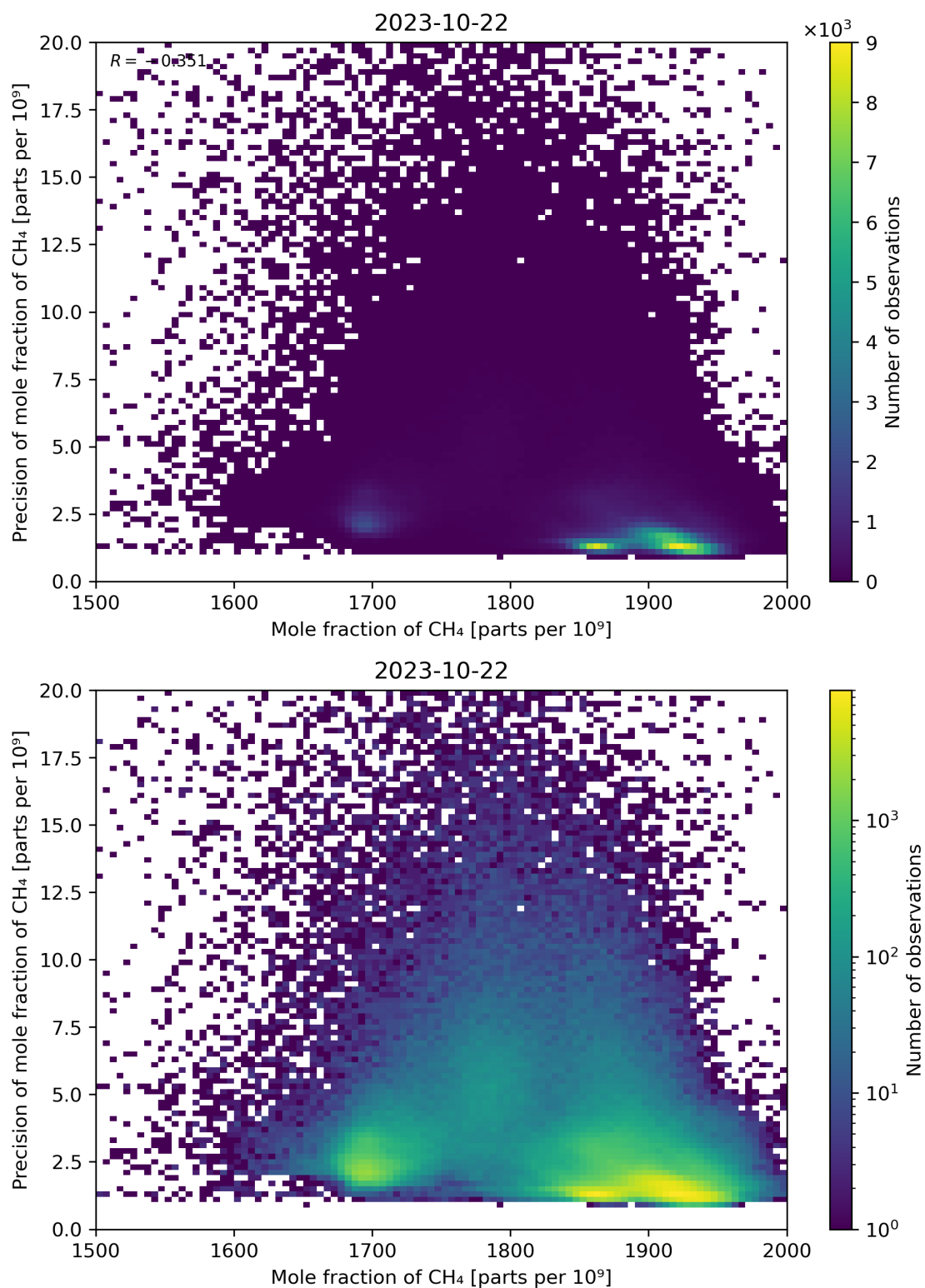
Figure 75: Scatter density plot of “Mole fraction of CH 4 ” against “Precision of mole fraction of CH 4 ” for 2023-10-22 to 2023-10-23.
