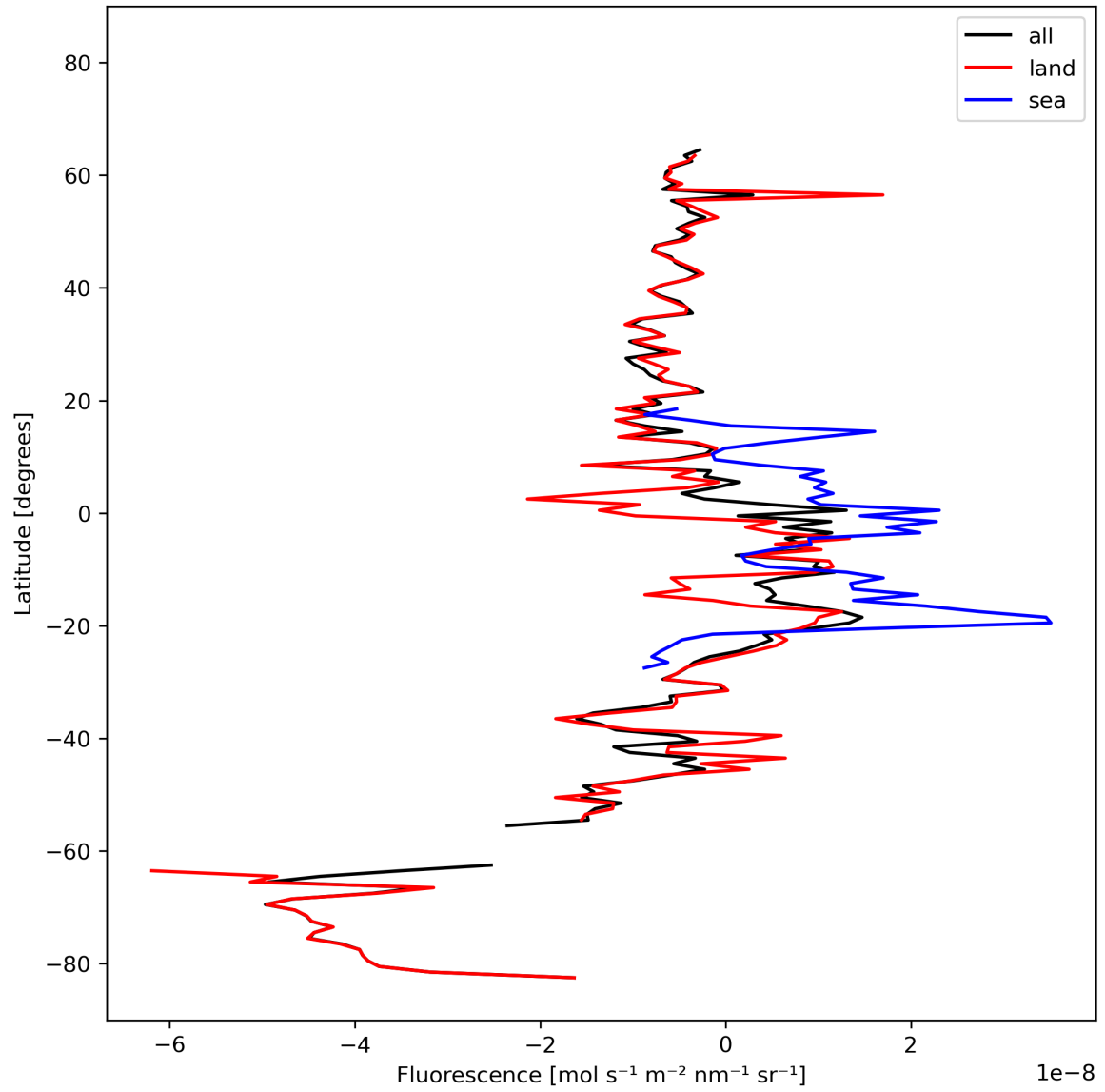
Figure 21: Zonal average of “Fluorescence” for 2023-10-22 to 2023-10-23.
