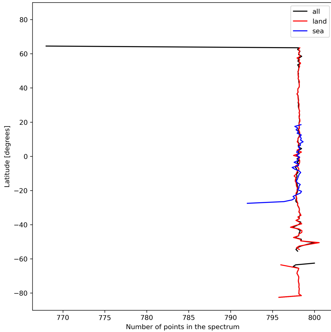
Figure 15: Zonal average of “Number of points in the spectrum” for 2023-10-22 to 2023-10-23.
