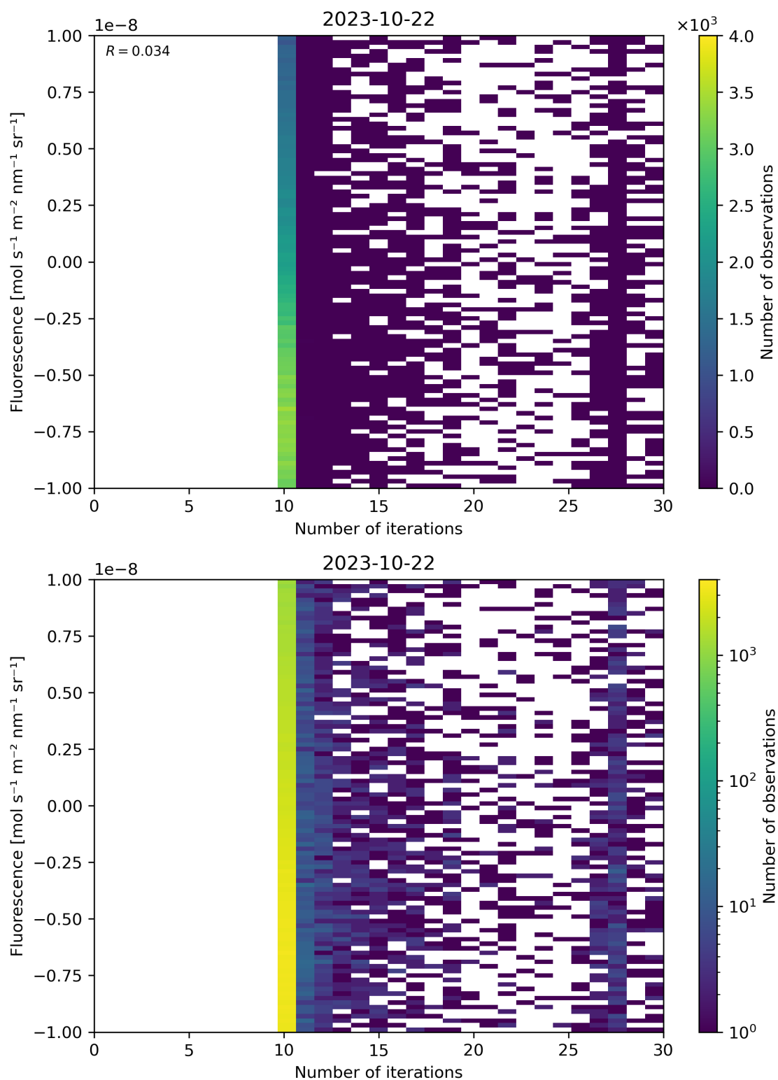
Figure 87: Scatter density plot of “Number of iterations” against “Fluorescence” for 2023-10-22 to 2023-10-23.
