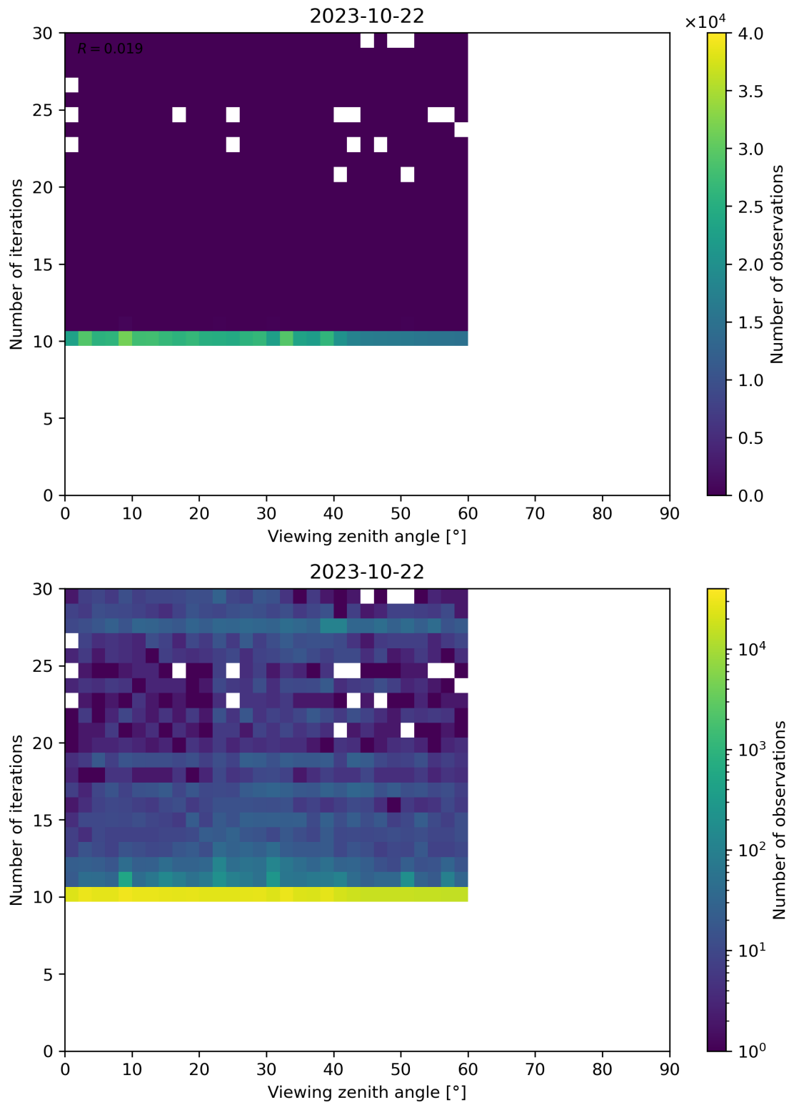
Figure 113: Scatter density plot of “Viewing zenith angle” against “Number of iterations” for 2023-10-22 to 2023-10-23.
