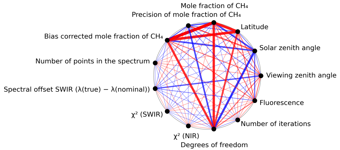
Figure 1: Map of correlation graph for 2023-10-22 to 2023-10-23.
