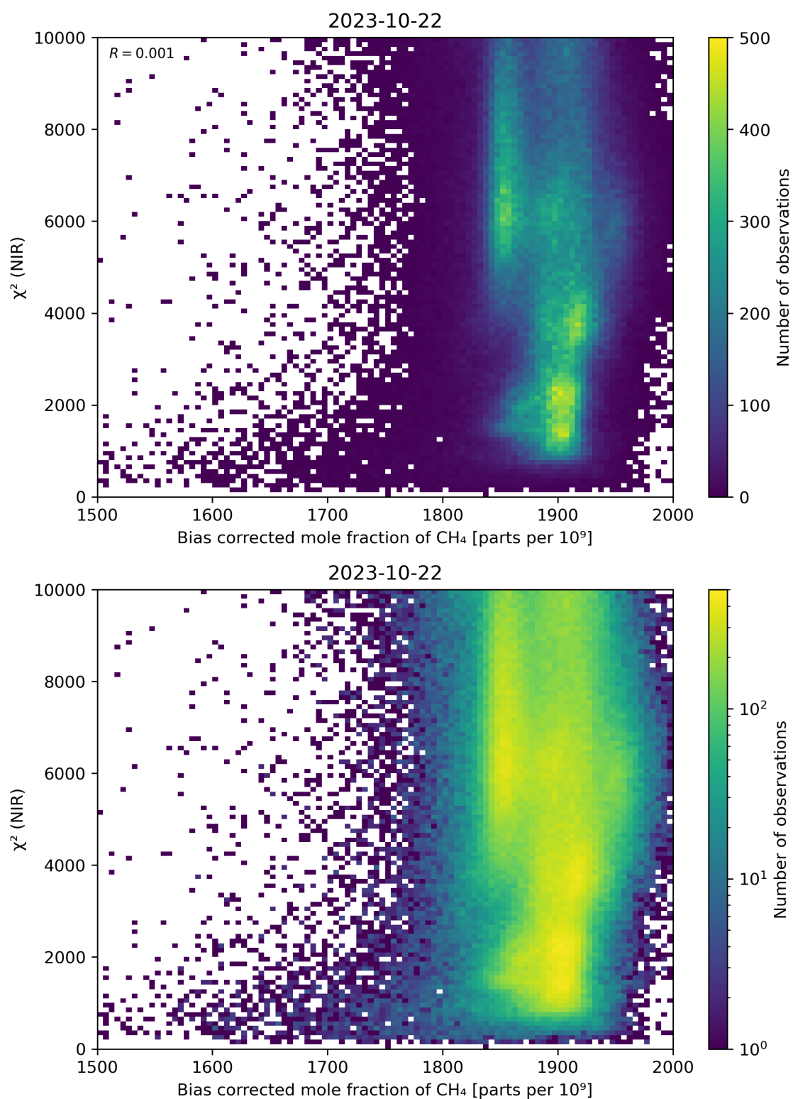
Figure 63: Scatter density plot of “Bias corrected mole fraction of CH 4 ” against “ \chi^2 (NIR)” for 2023-10-22 to 2023-10-23.
