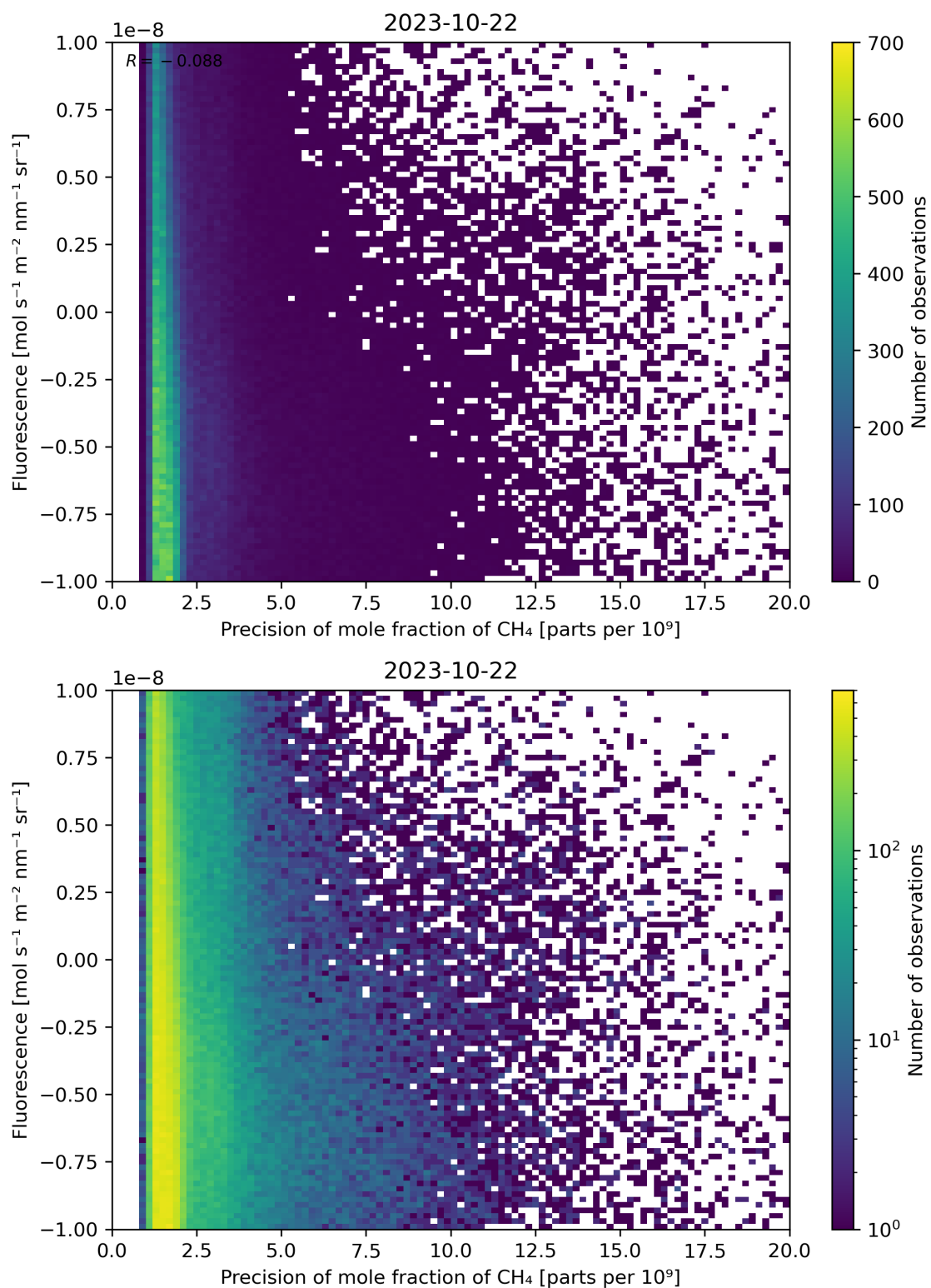
Figure 81: Scatter density plot of “Precision of mole fraction of CH 4 ” against “Fluorescence” for 2023-10-22 to 2023-10-23.
