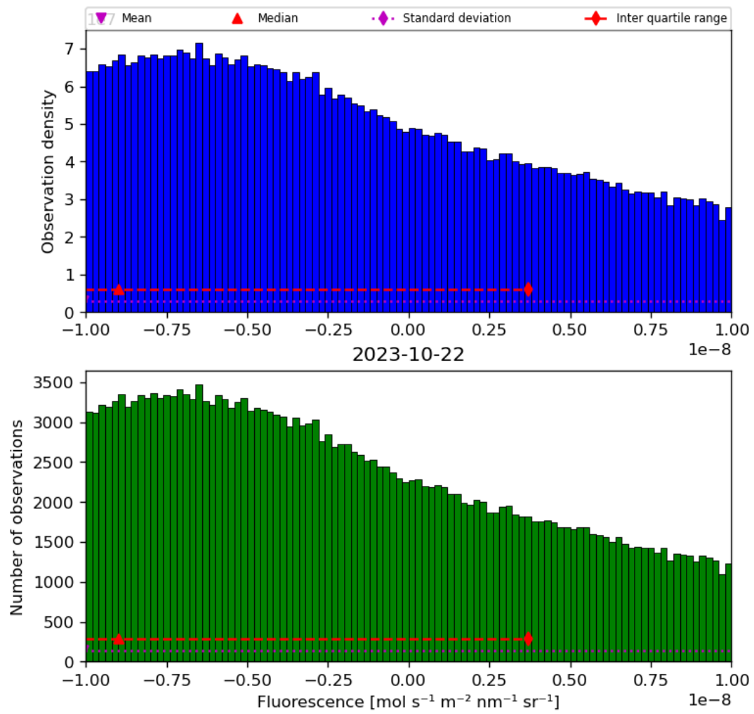
Figure 32: Histogram of “Fluorescence” for 2023-10-22 to 2023-10-23
