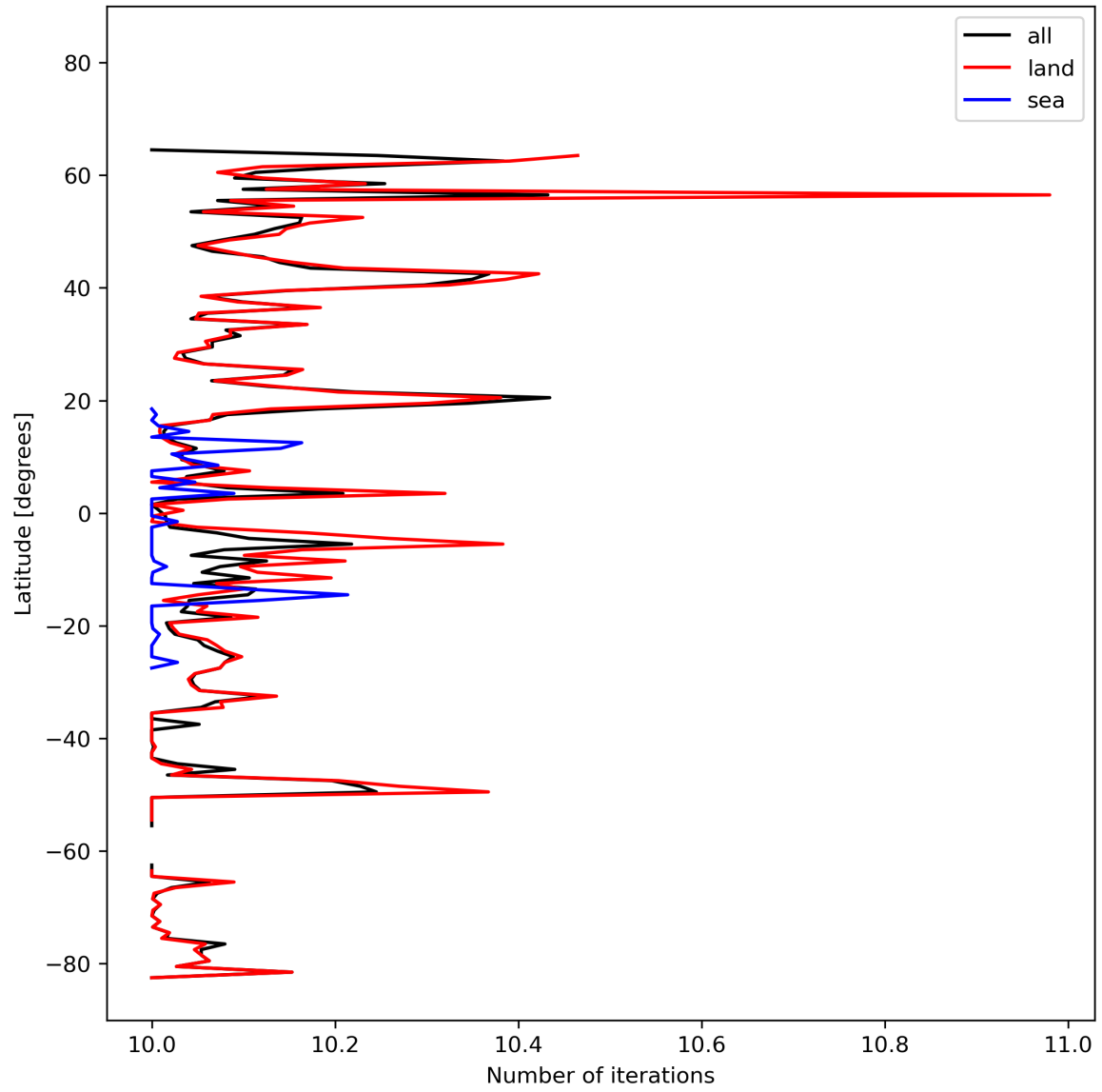
Figure 20: Zonal average of “Number of iterations” for 2023-10-22 to 2023-10-23.
