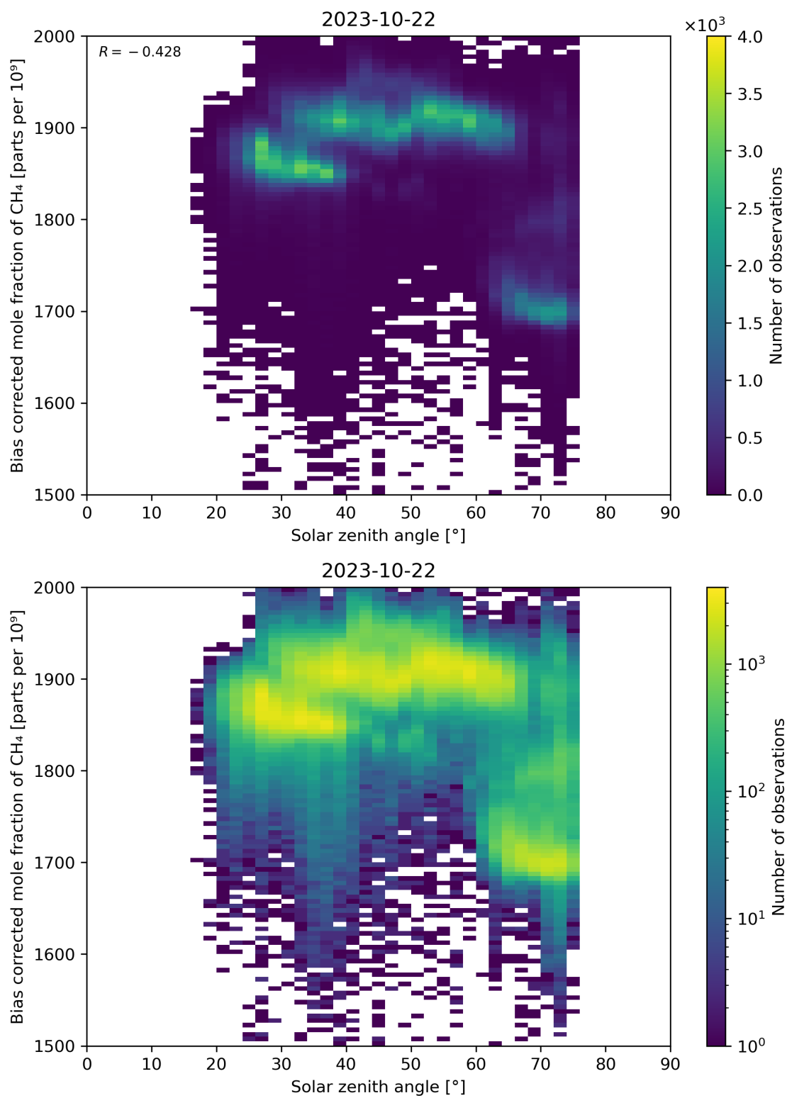
Figure 100: Scatter density plot of “Solar zenith angle” against “Bias corrected mole fraction of CH 4 ” for 2023-10-22 to 2023-10-23.
