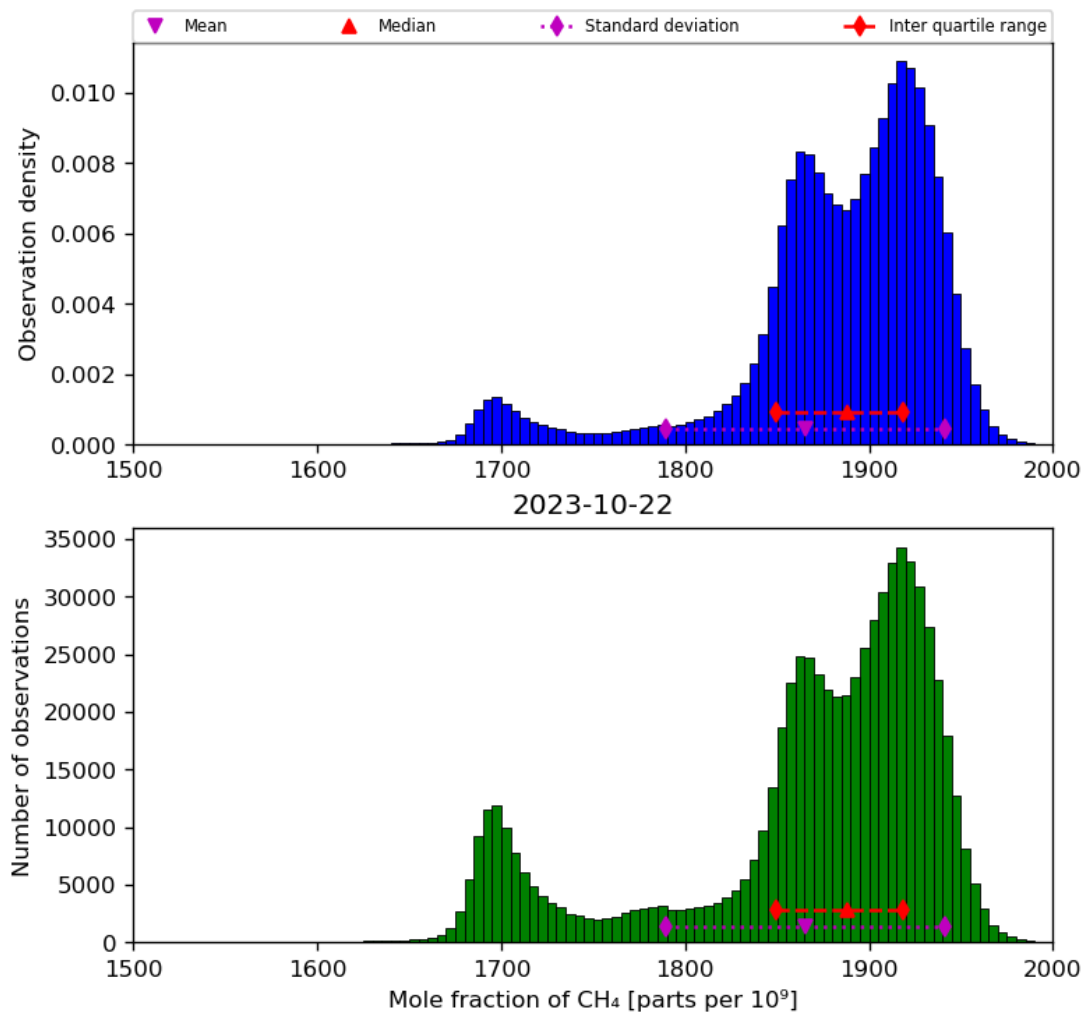
Figure 23: Histogram of “Mole fraction of CH 4 ” for 2023-10-22 to 2023-10-23
