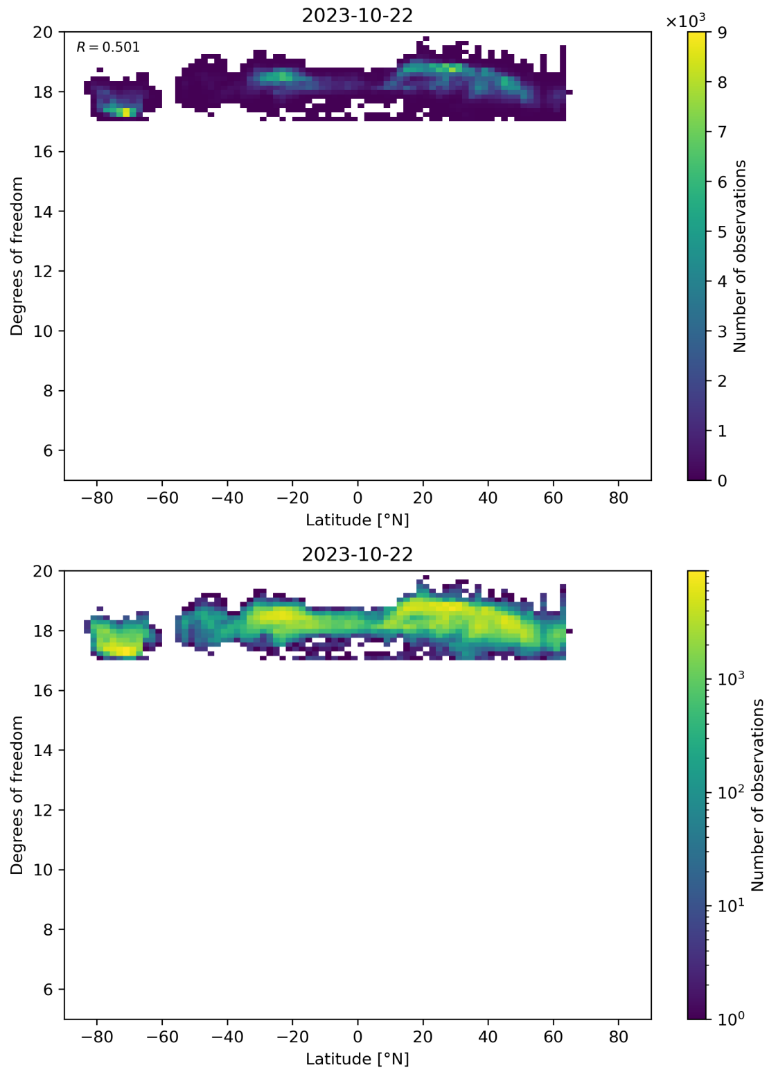
Figure 55: Scatter density plot of “Latitude” against “Degrees of freedom” for 2023-10-22 to 2023-10-23.
