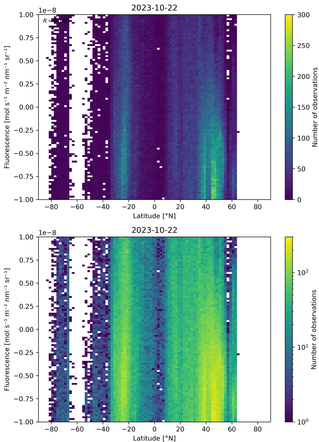
Figure 56: Scatter density plot of “Latitude” against “Fluorescence” for 2023-10-22 to 2023-10-23.
