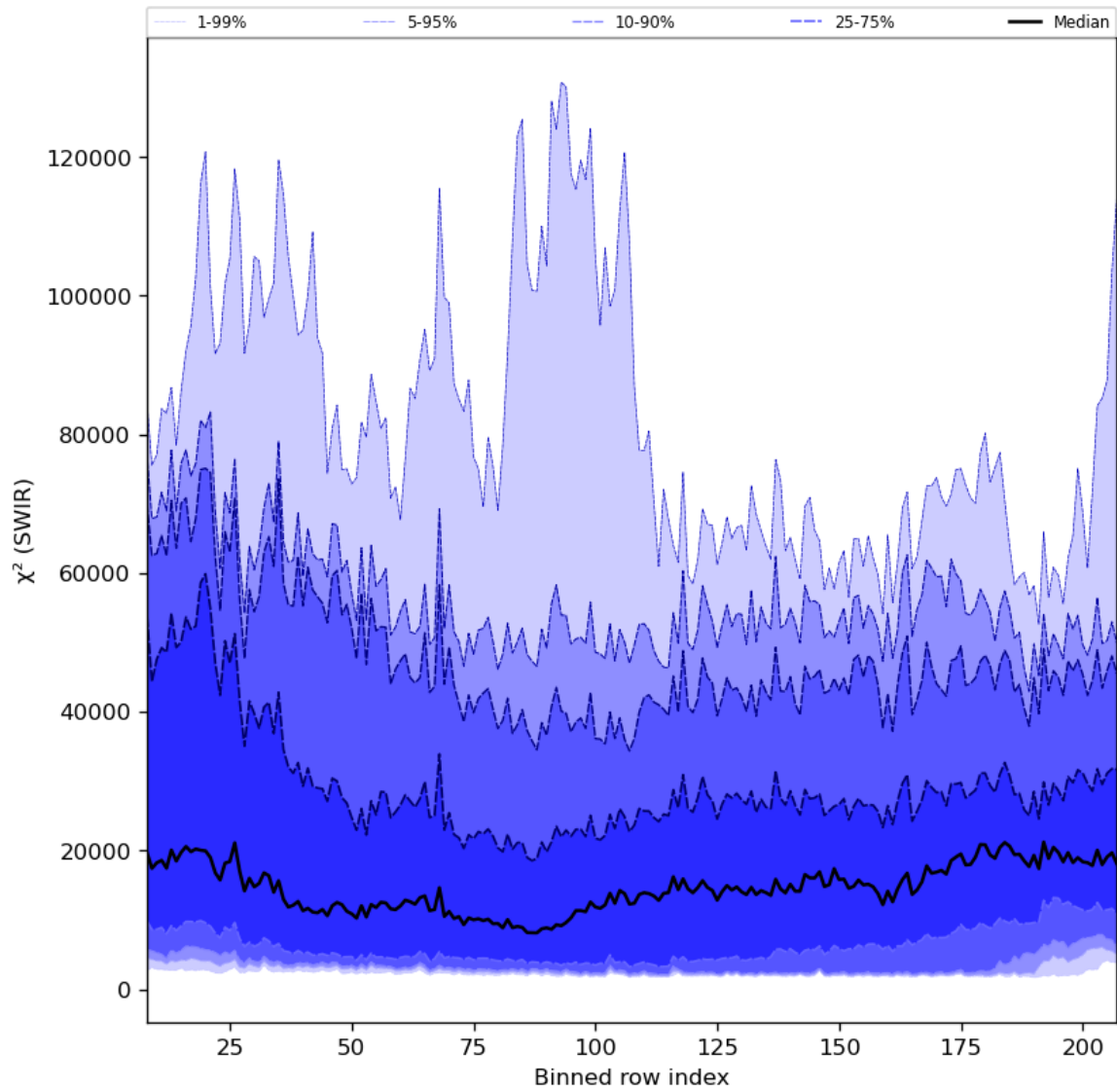
Figure 39: Along track statistics of “ \chi^2 (SWIR)” for 2023-10-22 to 2023-10-23
