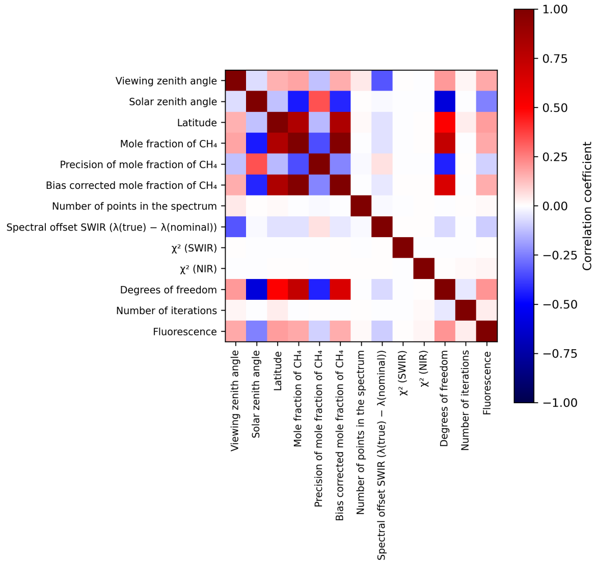
Figure 2: Map of correlation matrix for 2023-10-22 to 2023-10-23.
