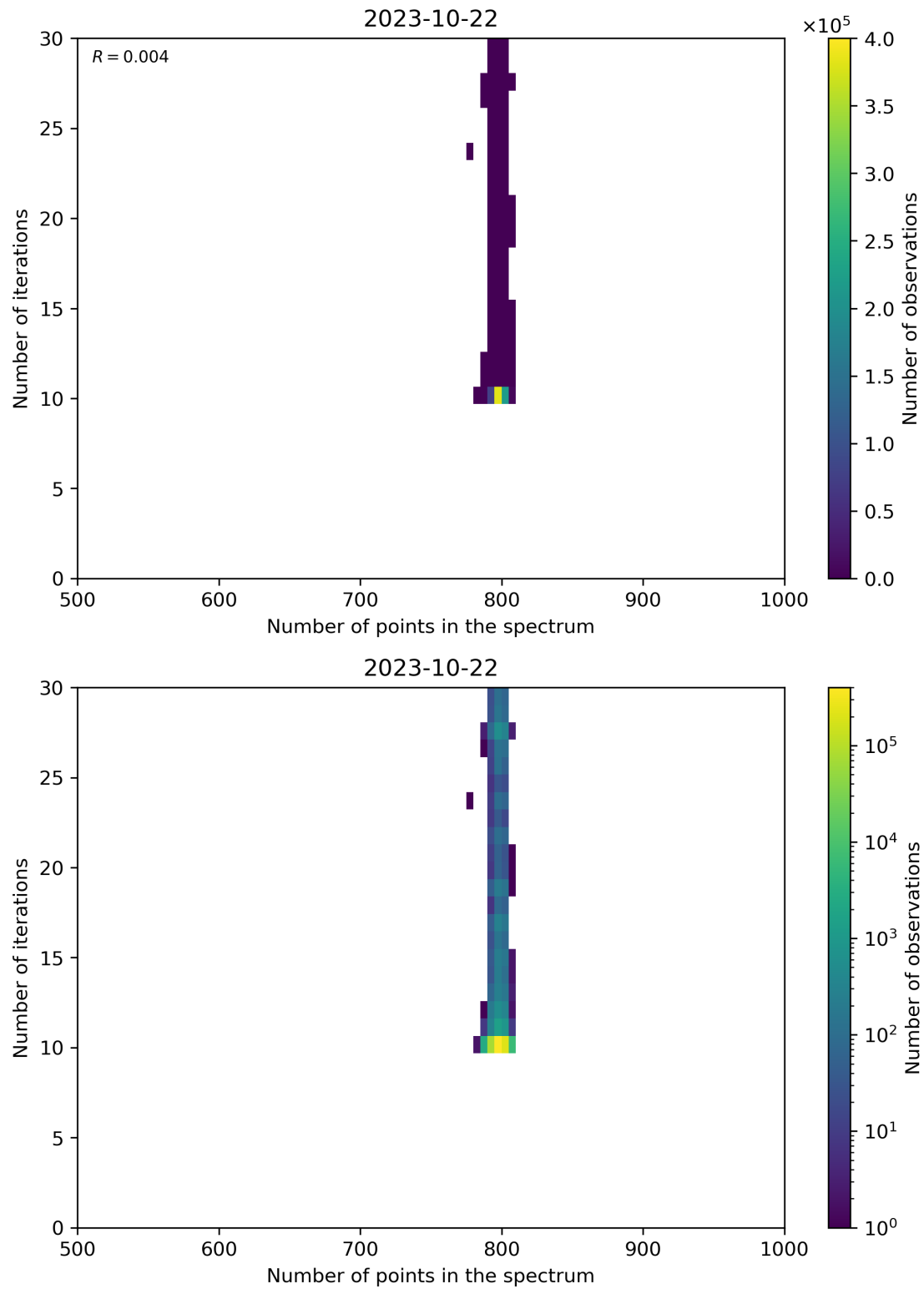
Figure 92: Scatter density plot of “Number of points in the spectrum” against “Number of iterations” for 2023-10-22 to 2023-10-23.
