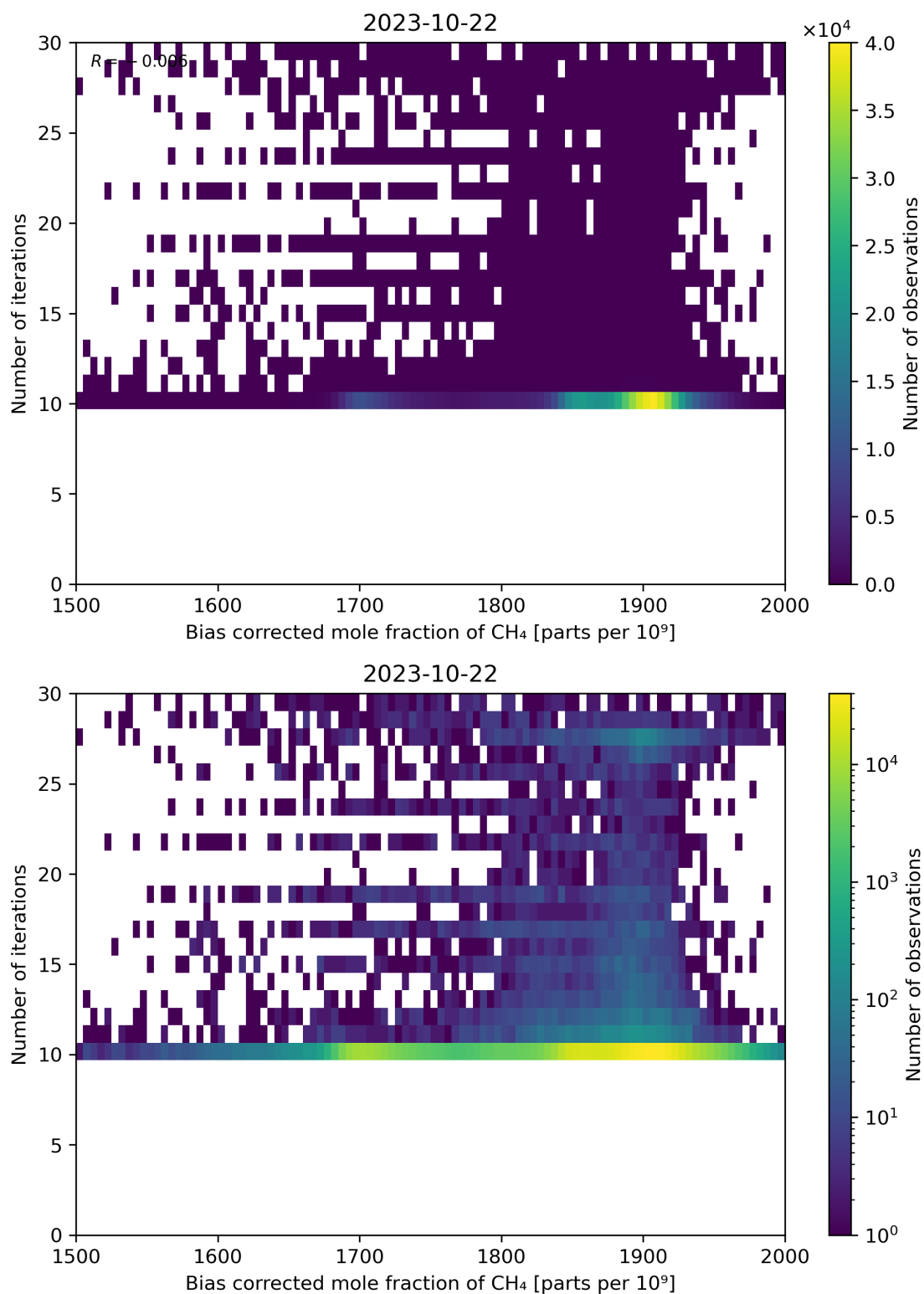
Figure 67: Scatter density plot of “Bias corrected mole fraction of CH 4 ” against “Number of iterations” for 2023-10-22 to 2023-10-23.
