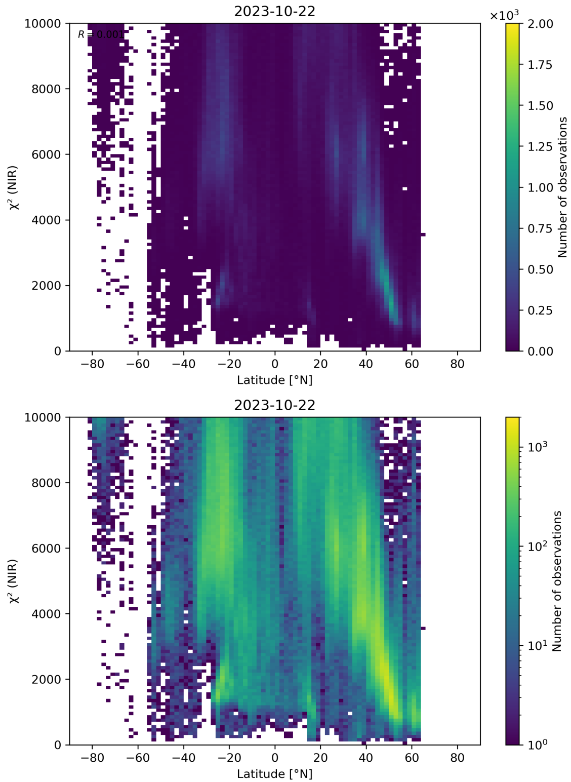
Figure 53: Scatter density plot of “Latitude” against “ \chi^2 (NIR)” for 2023-10-22 to 2023-10-23.
