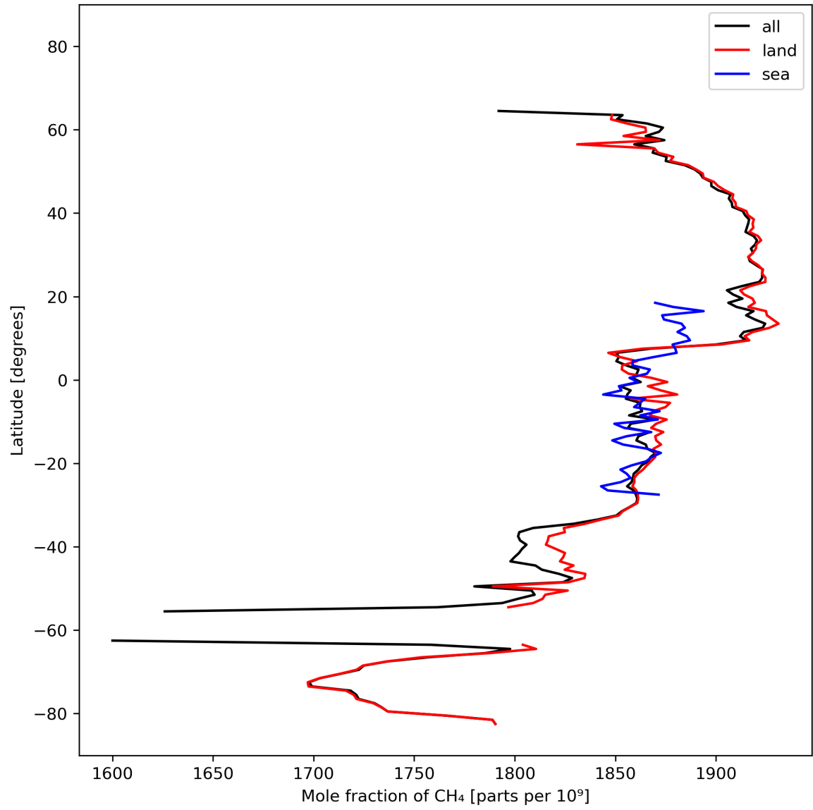
Figure 12: Zonal average of “Mole fraction of \text{CH}_4 ” for 2023-10-22 to 2023-10-23.
