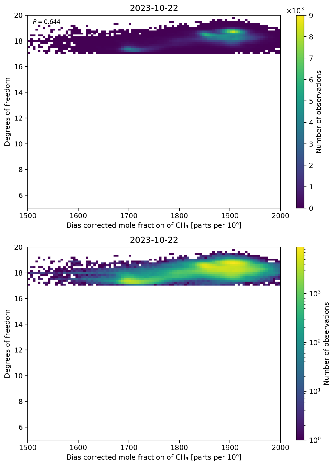
Figure 65: Scatter density plot of “Bias corrected mole fraction of CH 4 ” against “Degrees of freedom” for 2023-10-22 to 2023-10-23.
