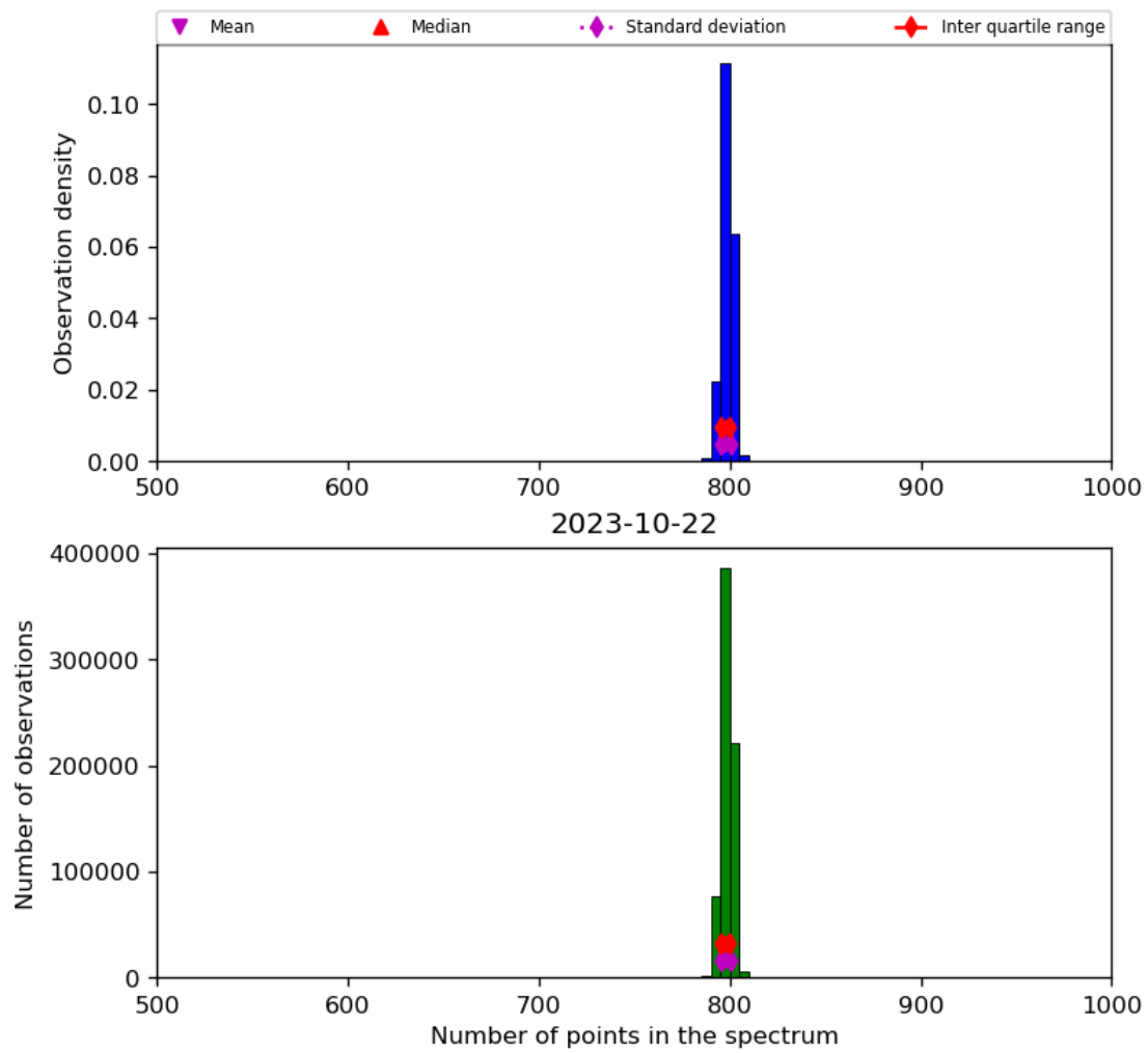
Figure 26: Histogram of “Number of points in the spectrum” for 2023-10-22 to 2023-10-23
