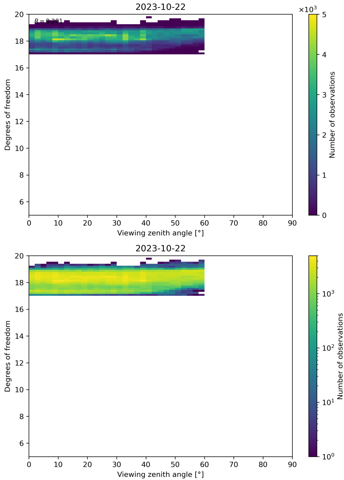
Figure 107: Scatter density plot of “Viewing zenith angle” against “Degrees of freedom” for 2023-10-22 to 2023-10-23.
