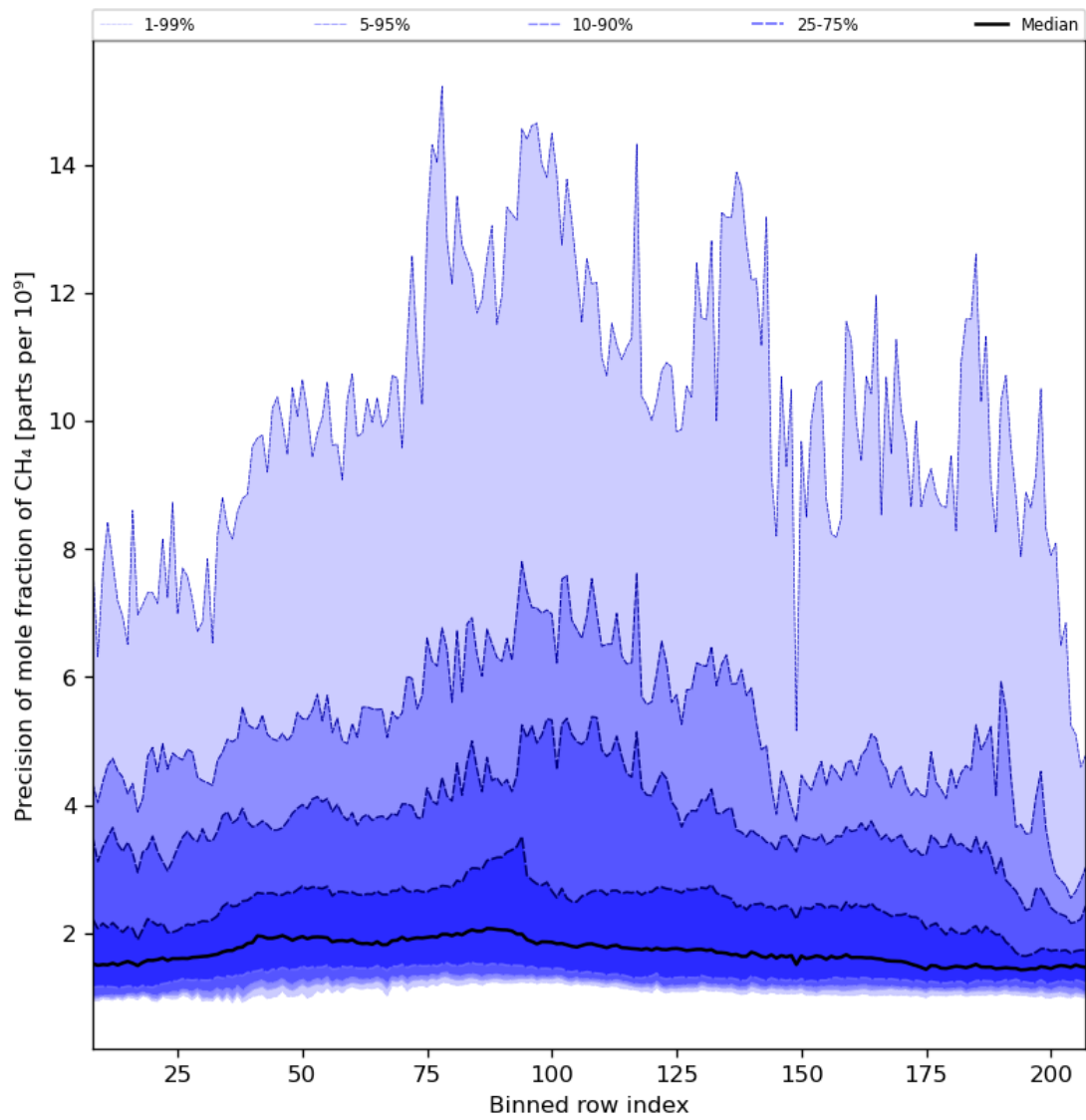
Figure 35: Along track statistics of “Precision of mole fraction of CH 4 ” for 2023-10-22 to 2023-10-23
