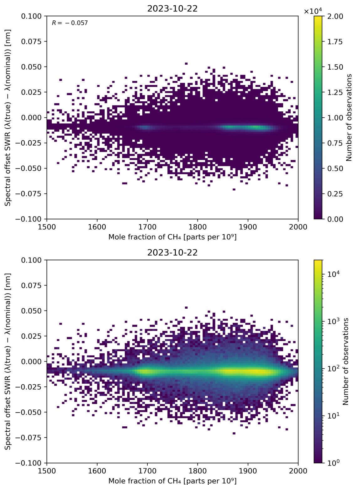
Figure 86: Scatter density plot of “Mole fraction of CH 4 ” against “Spectral offset SWIR ( \lambda(\text{true}) - \lambda(\text{nominal}) )” for 2023-10-22 to 2023-10-23.
