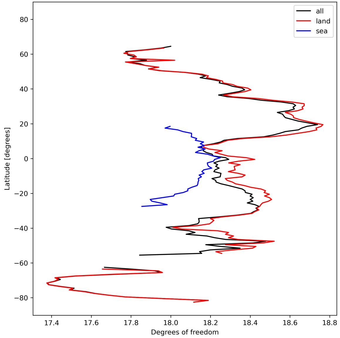
Figure 19: Zonal average of “Degrees of freedom” for 2023-10-22 to 2023-10-23.
