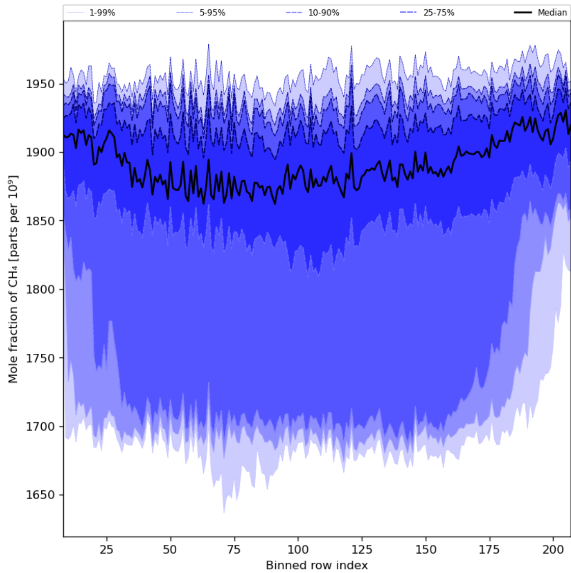
Figure 34: Along track statistics of “Mole fraction of CH 4 ” for 2023-10-22 to 2023-10-23
