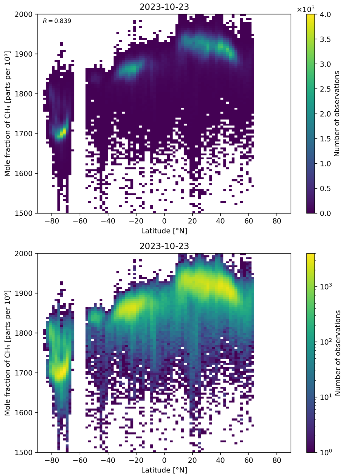
Figure 57: Scatter density plot of “Latitude” against “Mole fraction of CH 4 ” for 2023-10-22 to 2023-10-24.
