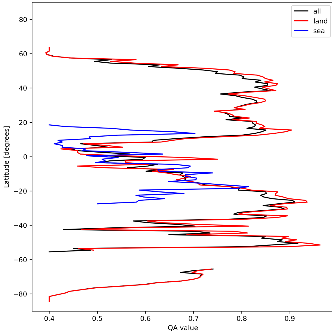
Figure 11: Zonal average of “QA value” for 2023-10-22 to 2023-10-24.
