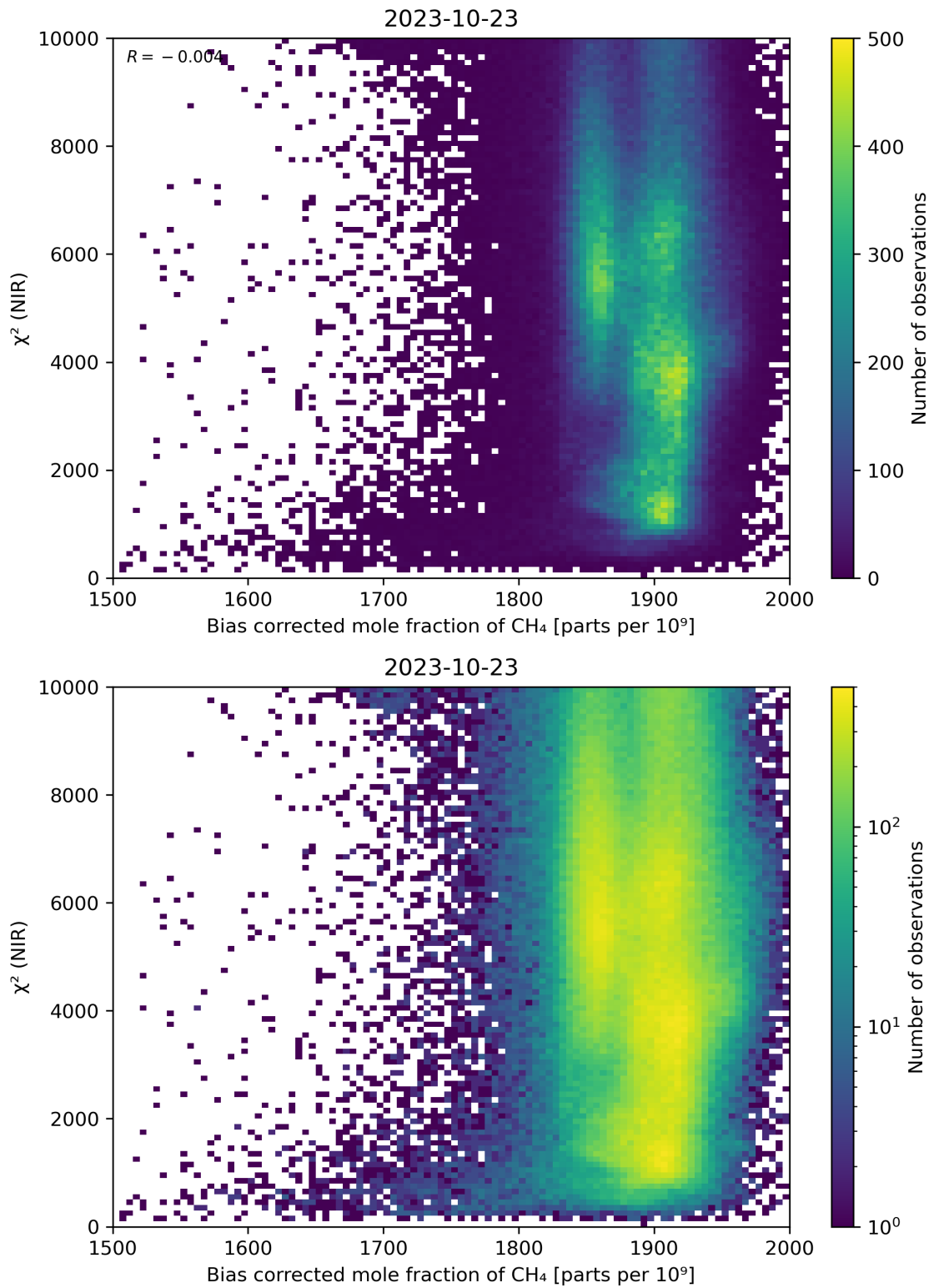
Figure 63: Scatter density plot of “Bias corrected mole fraction of CH 4 ” against “ \chi^2 (NIR)” for 2023-10-22 to 2023-10-24.
