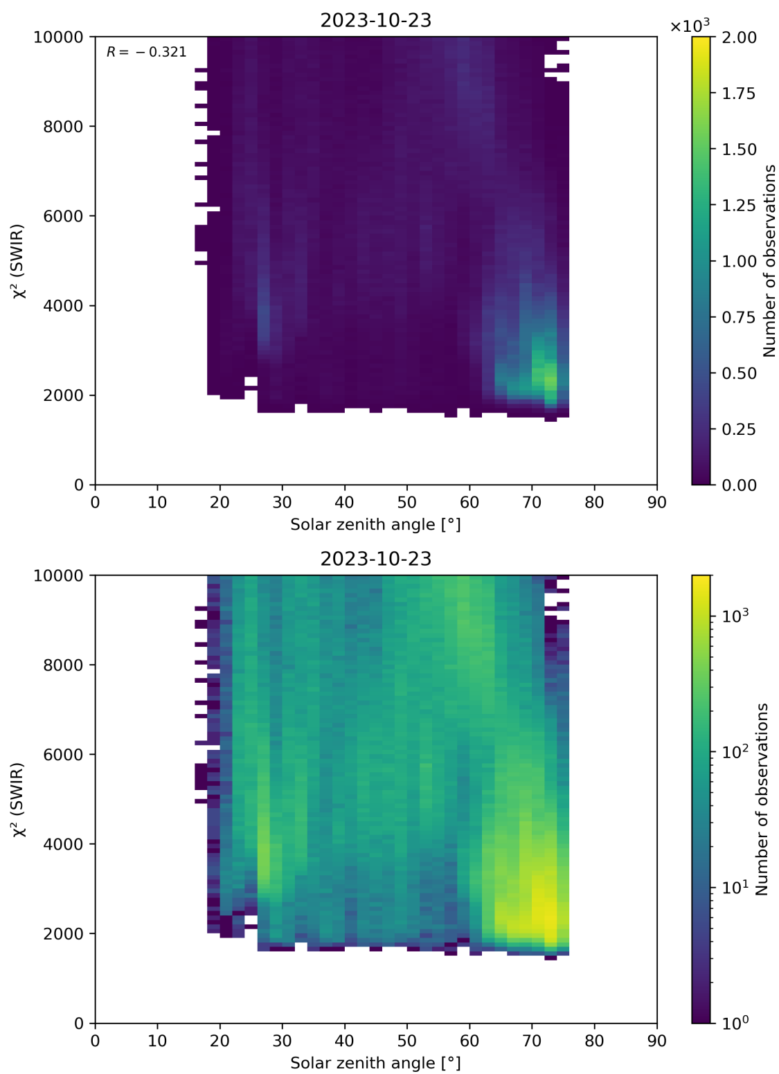
Figure 95: Scatter density plot of “Solar zenith angle” against “ \chi^2 (SWIR)” for 2023-10-22 to 2023-10-24.
