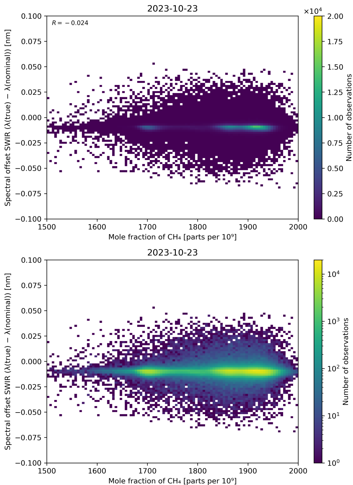
Figure 86: Scatter density plot of “Mole fraction of CH 4 ” against “Spectral offset SWIR ( \lambda(\text{true}) - \lambda(\text{nominal}) )” for 2023-10-22 to 2023-10-24.
