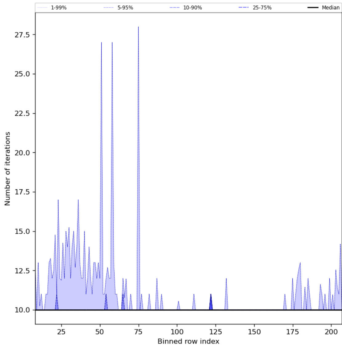
Figure 42: Along track statistics of “Number of iterations” for 2023-10-22 to 2023-10-24
