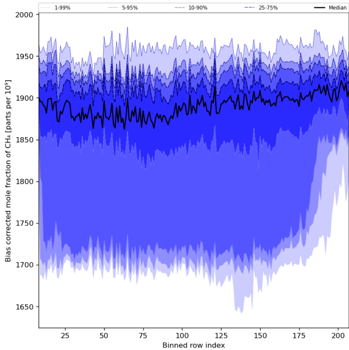
Figure 36: Along track statistics of “Bias corrected mole fraction of CH 4 ” for 2023-10-22 to 2023-10-24
