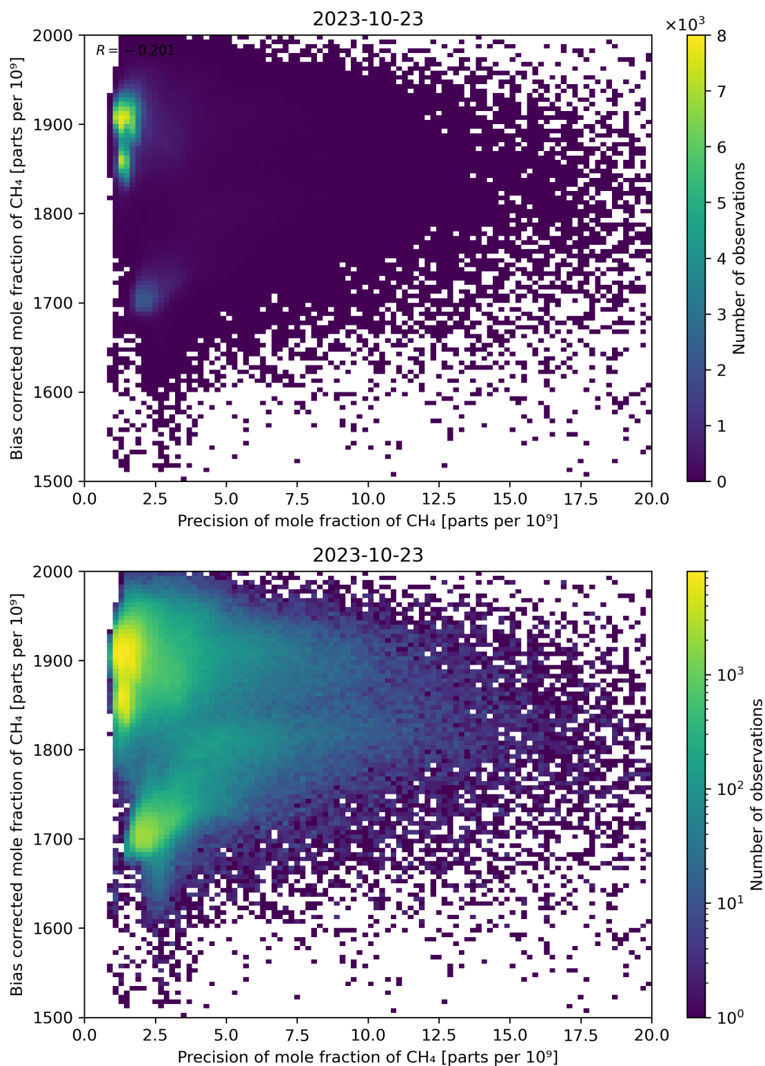
Figure 82: Scatter density plot of “Precision of mole fraction of CH 4 ” against “Bias corrected mole fraction of CH 4 ” for 2023-10-22 to 2023-10-24.
