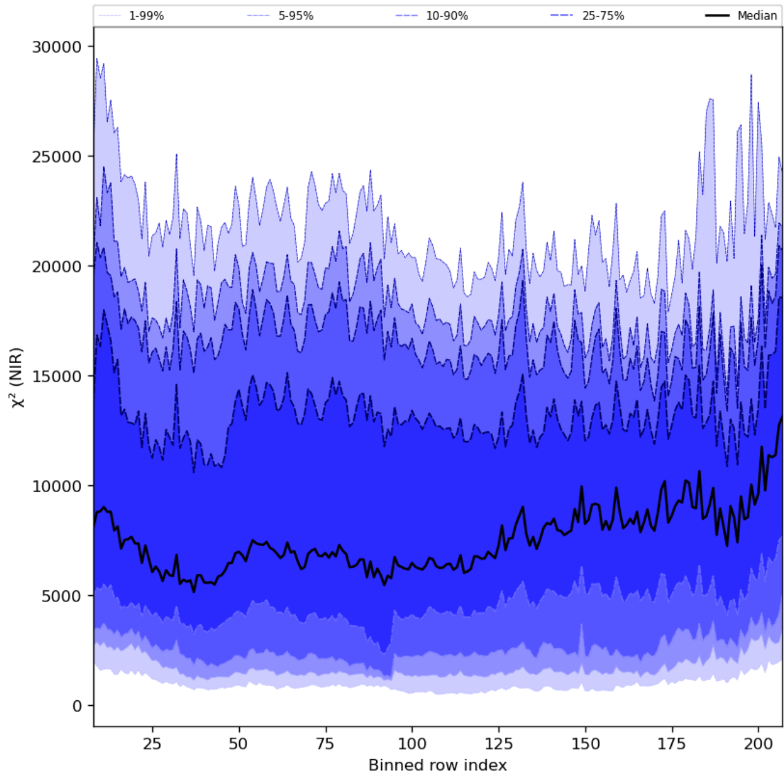
Figure 40: Along track statistics of “ \chi^2 (NIR)” for 2023-10-22 to 2023-10-24
