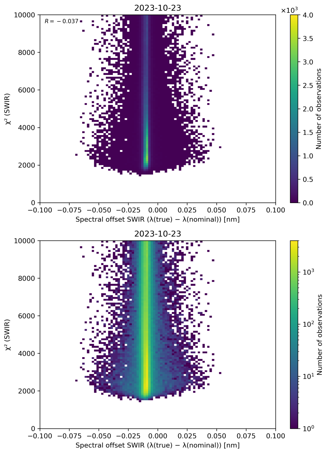
Figure 118: Scatter density plot of “Spectral offset SWIR ( \lambda(\text{true}) - \lambda(\text{nominal}) )” against “ \chi^2 (SWIR)” for 2023-10-22 to 2023-10-24.
