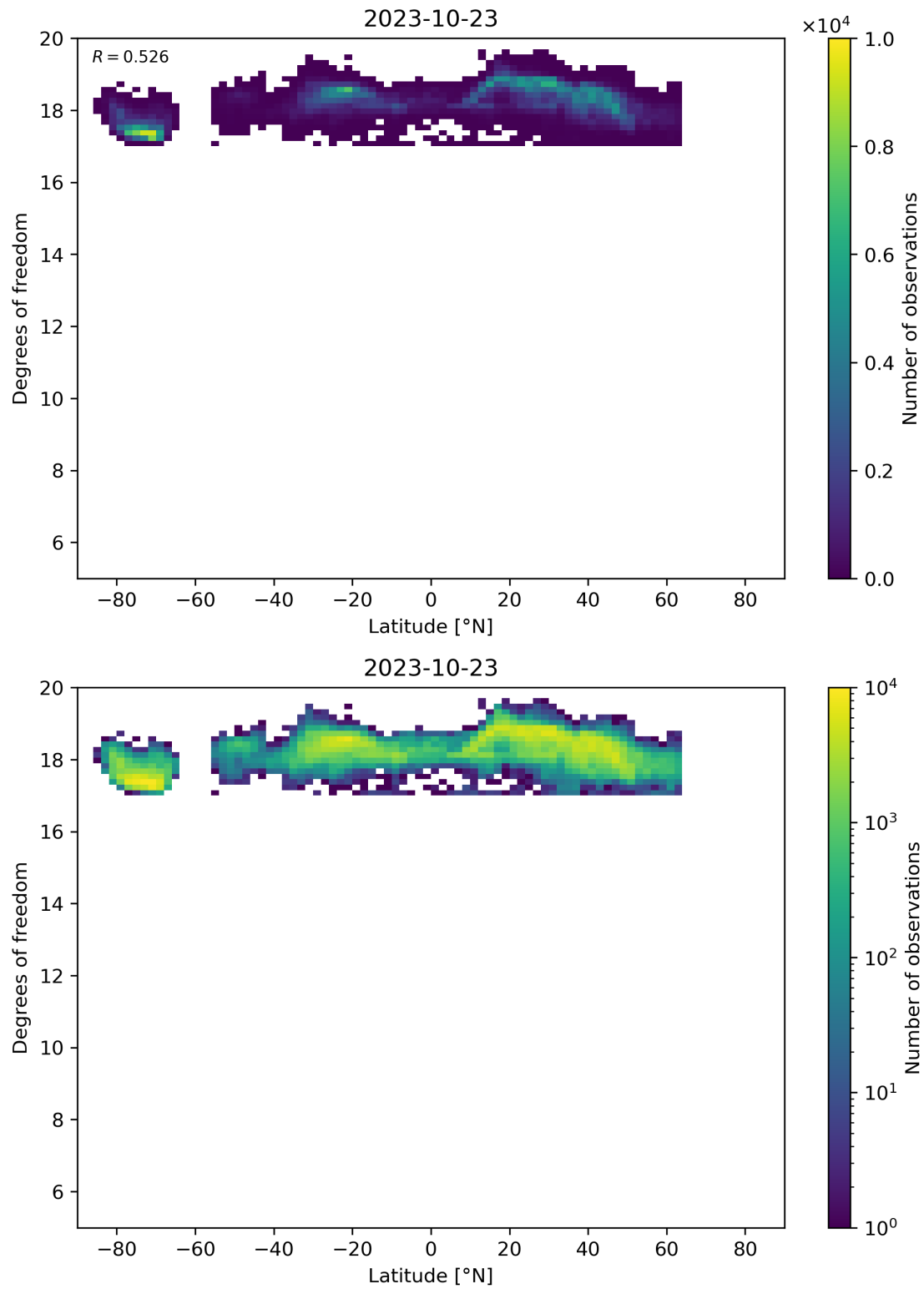
Figure 55: Scatter density plot of “Latitude” against “Degrees of freedom” for 2023-10-22 to 2023-10-24.
