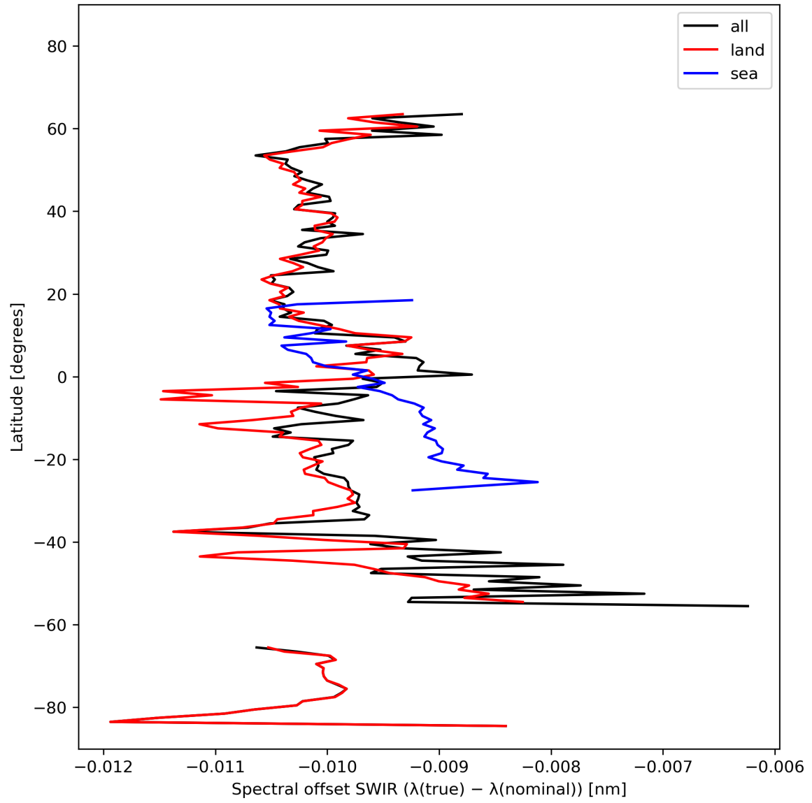
Figure 16: Zonal average of “Spectral offset SWIR ( \lambda(\text{true}) - \lambda(\text{nominal}) )” for 2023-10-22 to 2023-10-24.
