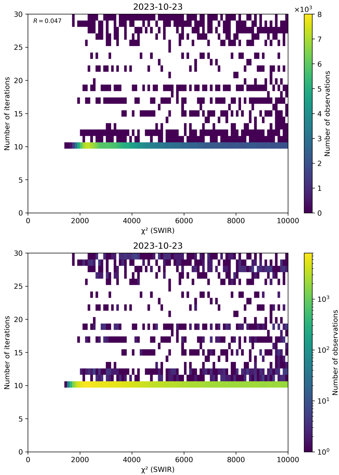
Figure 50: Scatter density plot of “ \chi^2 (SWIR)” against “Number of iterations” for 2023-10-22 to 2023-10-24.
