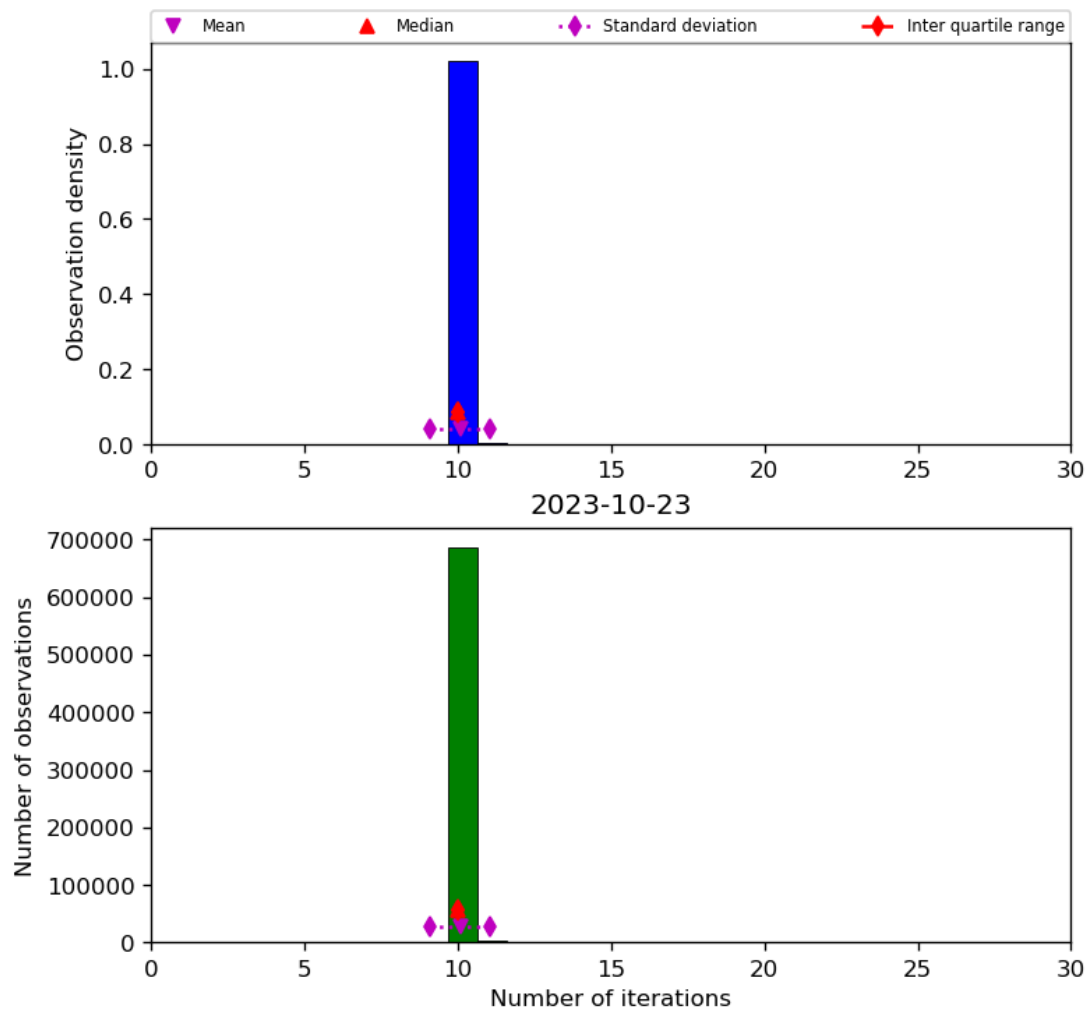
Figure 31: Histogram of “Number of iterations” for 2023-10-22 to 2023-10-24
