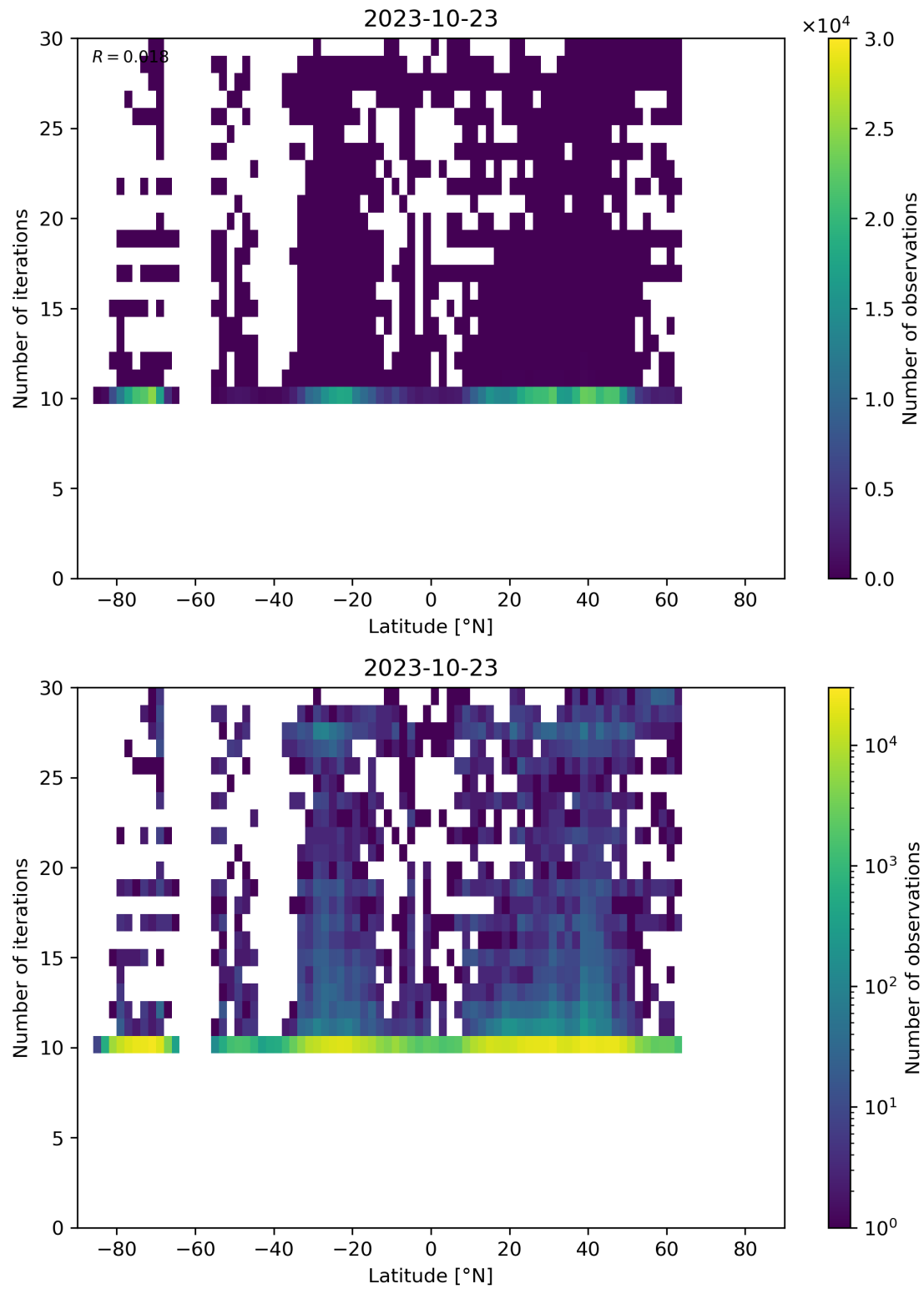
Figure 60: Scatter density plot of “Latitude” against “Number of iterations” for 2023-10-22 to 2023-10-24.
