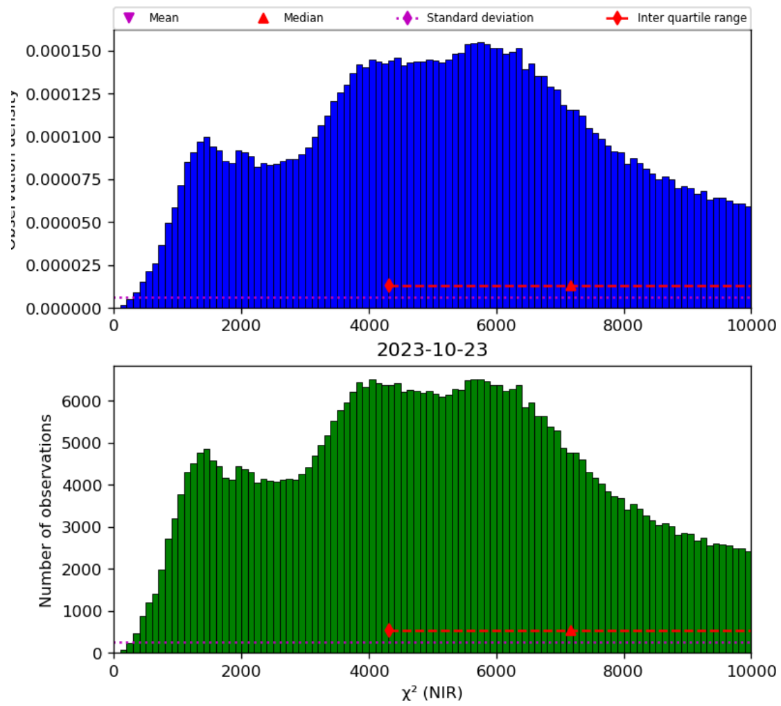
Figure 29: Histogram of “ \chi^2 (NIR)” for 2023-10-22 to 2023-10-24
