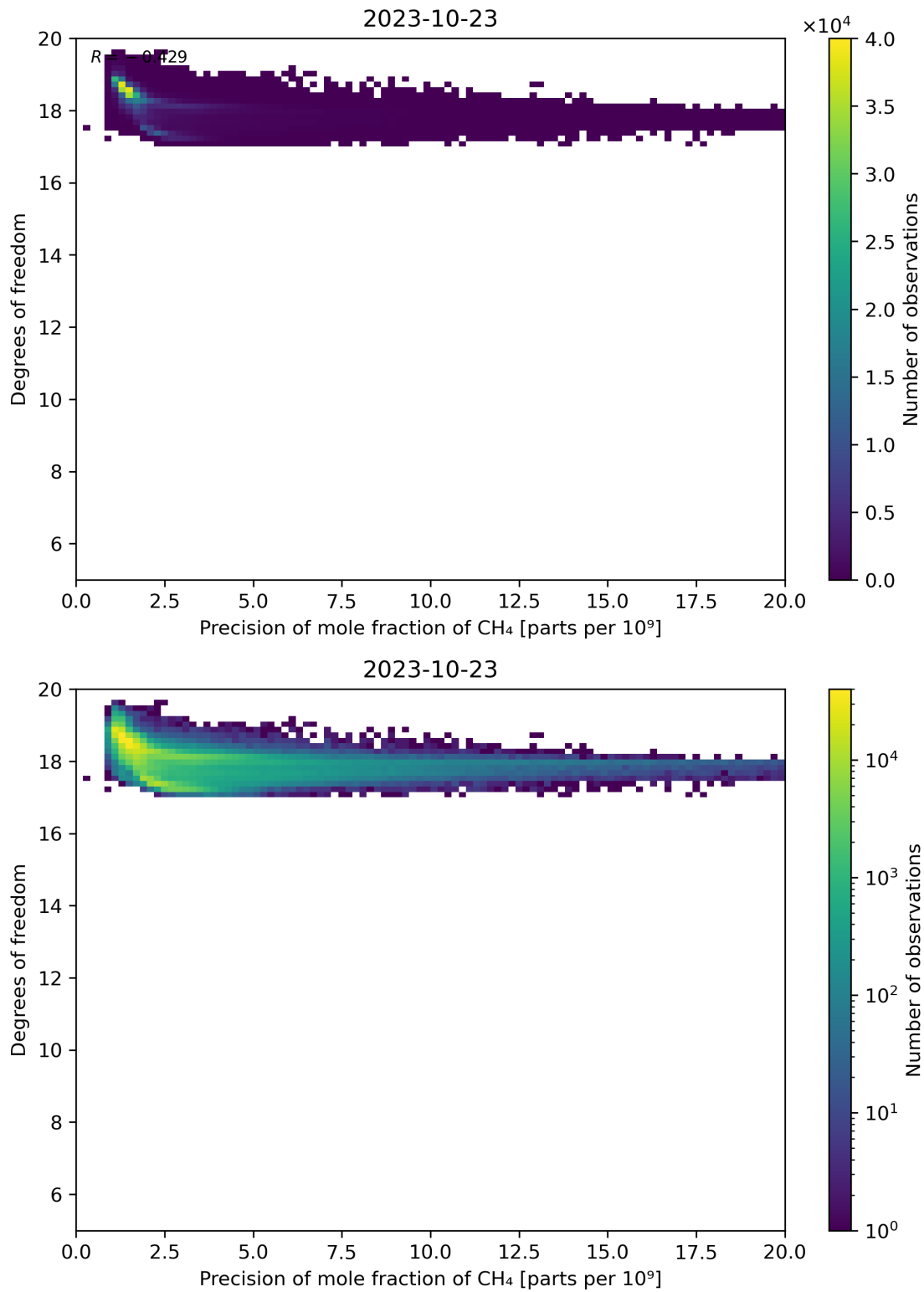
Figure 80: Scatter density plot of “Precision of mole fraction of CH 4 ” against “Degrees of freedom” for 2023-10-22 to 2023-10-24.
