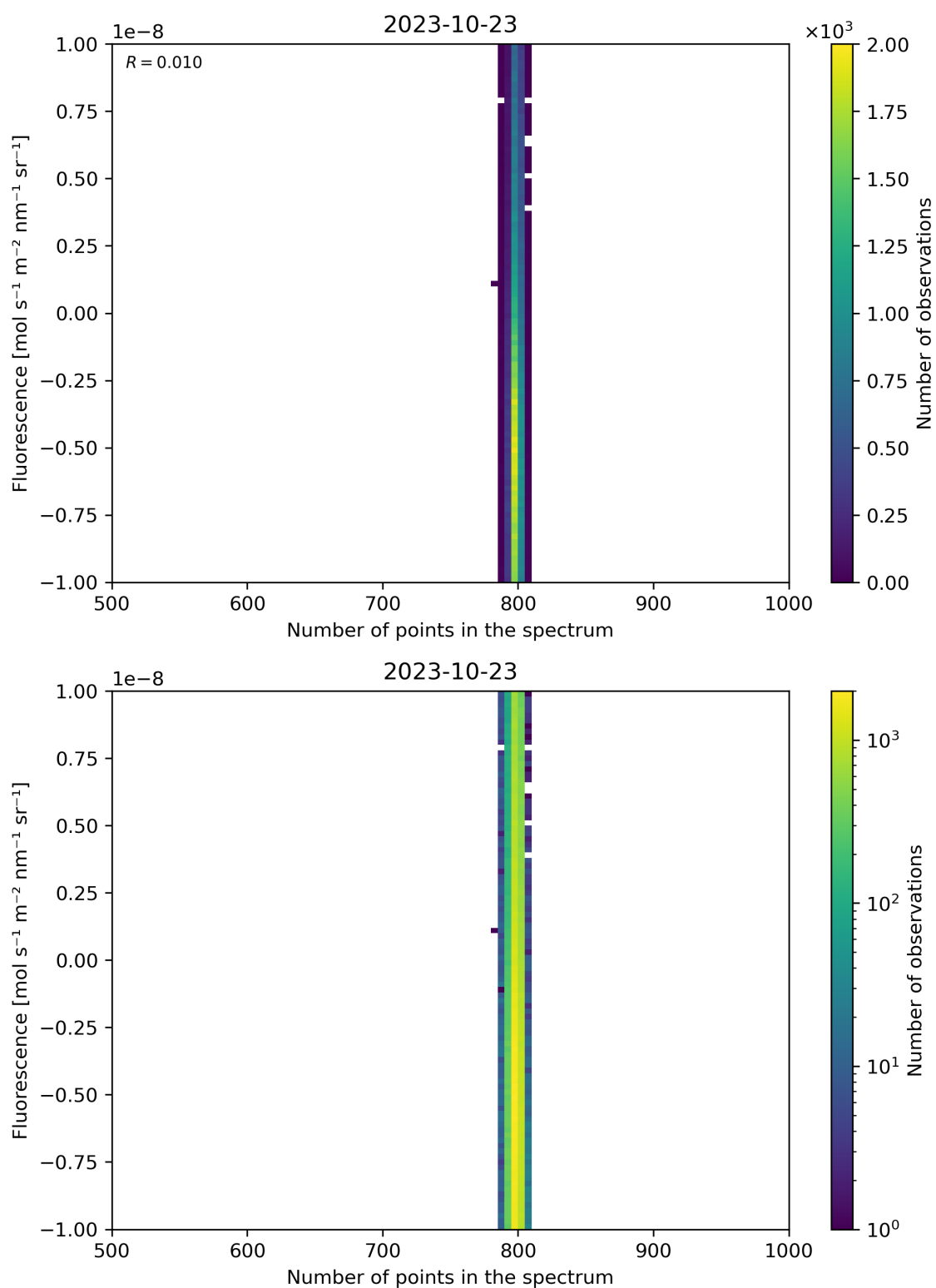
Figure 91: Scatter density plot of “Number of points in the spectrum” against “Fluorescence” for 2023-10-22 to 2023-10-24.
