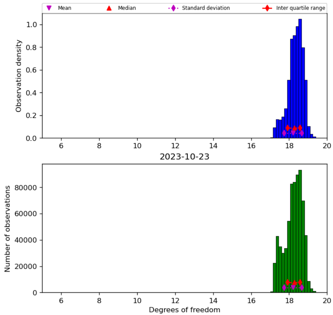
Figure 30: Histogram of “Degrees of freedom” for 2023-10-22 to 2023-10-24
