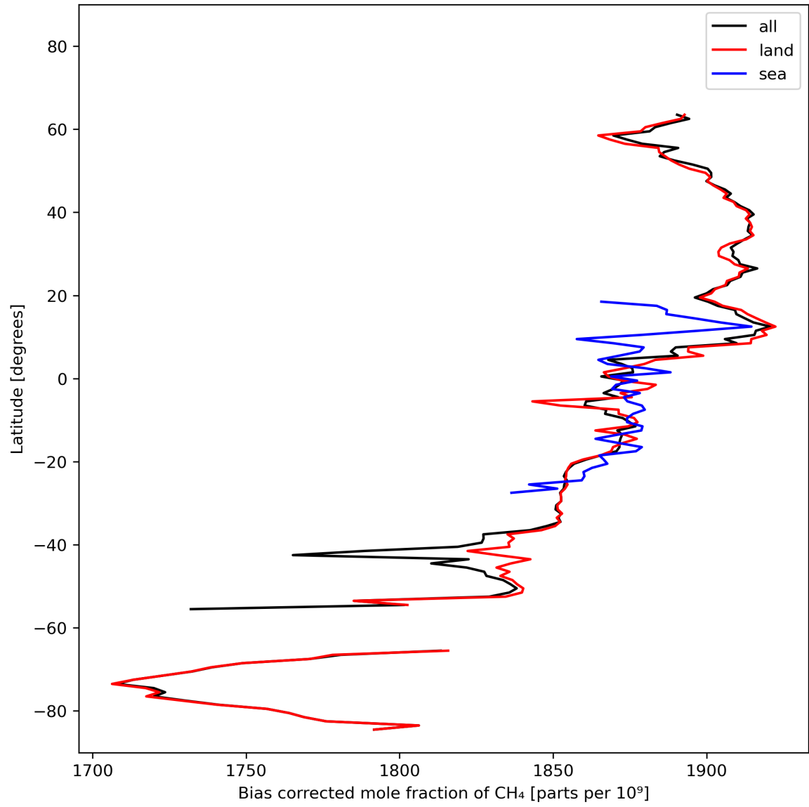
Figure 14: Zonal average of “Bias corrected mole fraction of CH 4 ” for 2023-10-22 to 2023-10-24.
