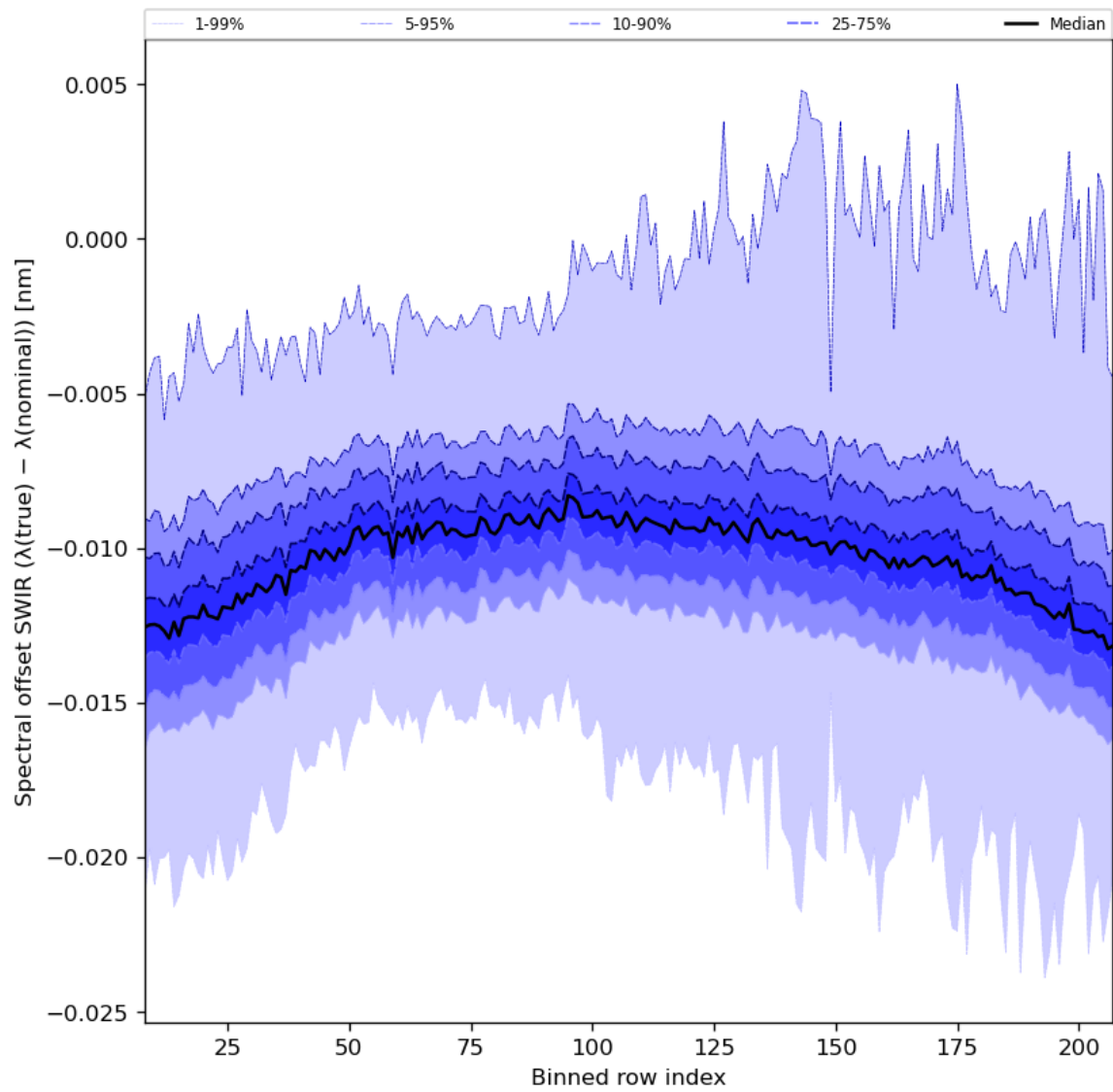
Figure 38: Along track statistics of “Spectral offset SWIR ( \lambda(\text{true}) - \lambda(\text{nominal}) )” for 2023-10-22 to 2023-10-24
