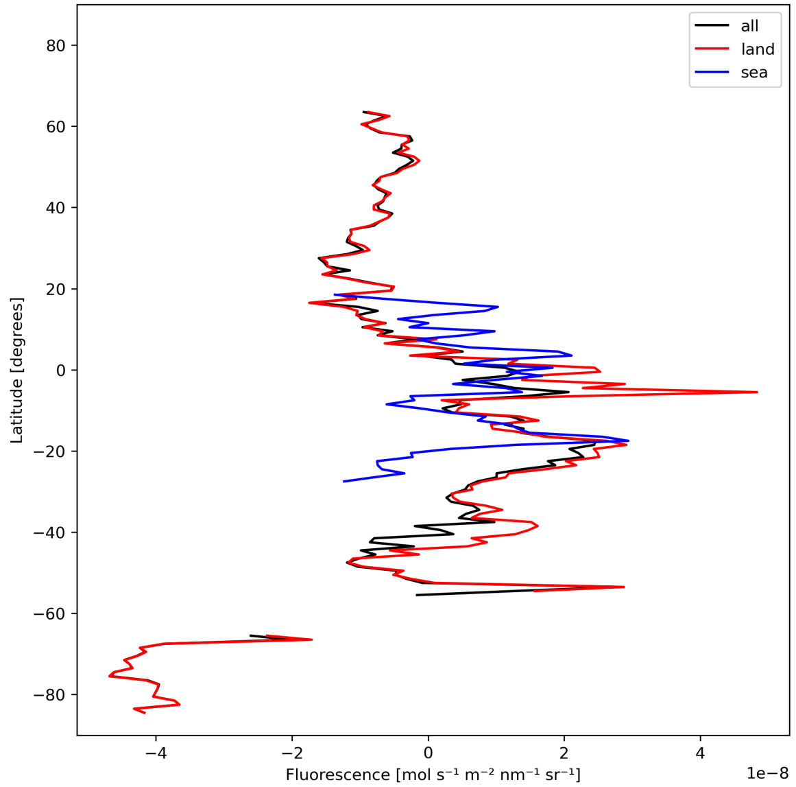
Figure 21: Zonal average of “Fluorescence” for 2023-10-22 to 2023-10-24.
