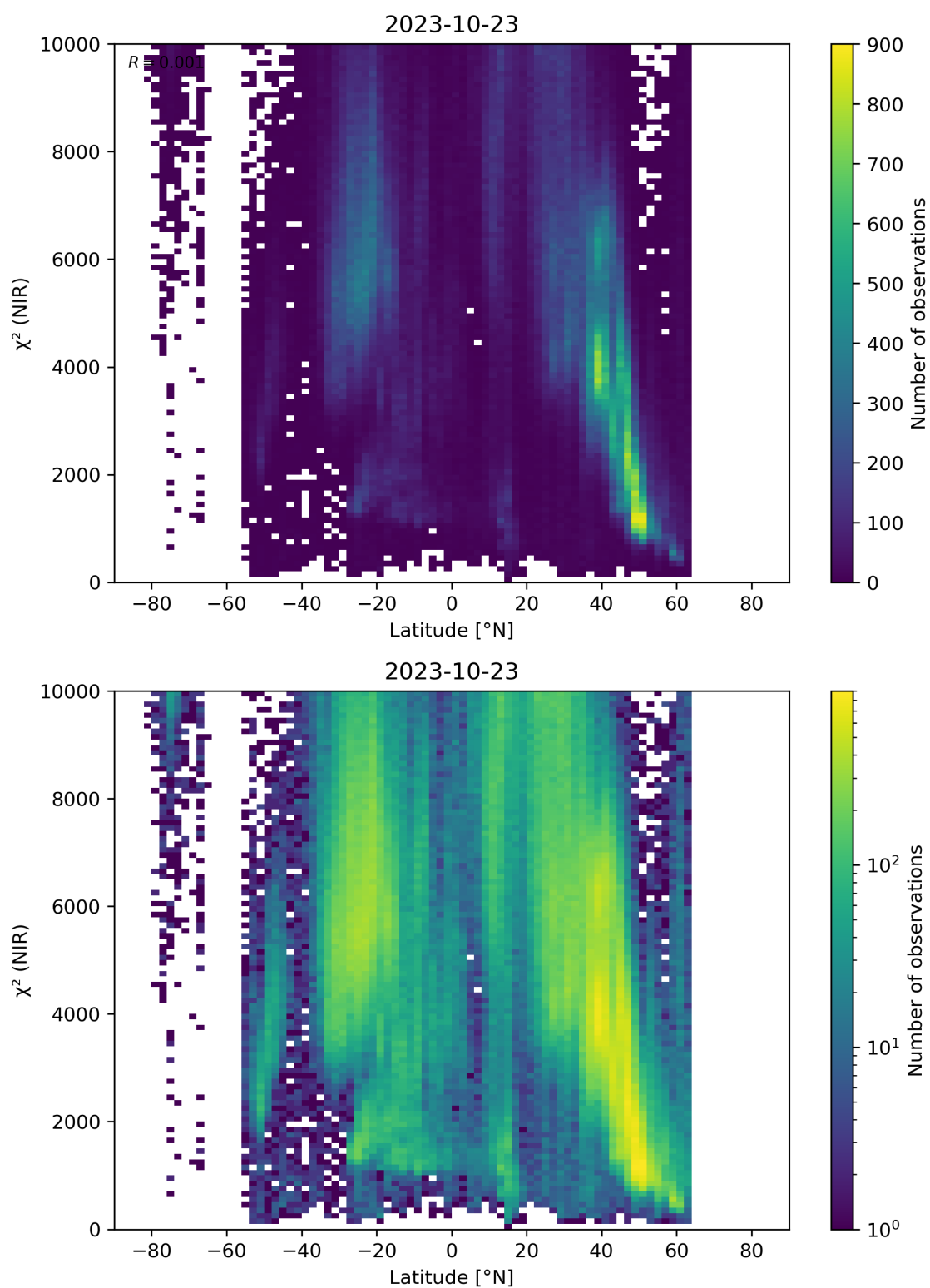
Figure 53: Scatter density plot of “Latitude” against “ \chi^2 (NIR)” for 2023-10-22 to 2023-10-24.
