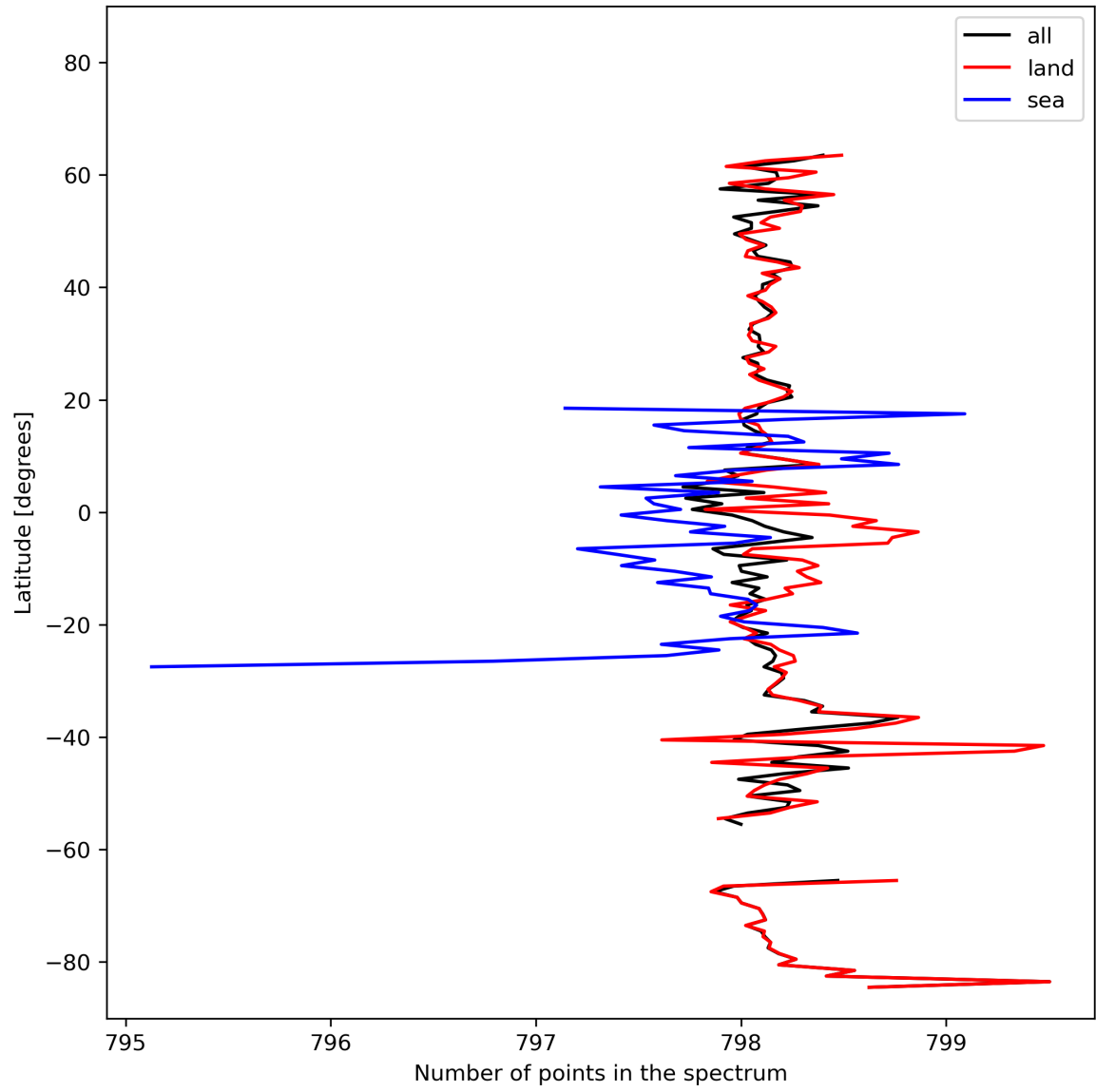
Figure 15: Zonal average of “Number of points in the spectrum” for 2023-10-22 to 2023-10-24.
