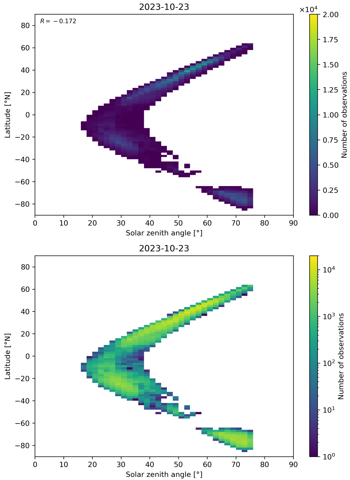
Figure 98: Scatter density plot of “Solar zenith angle” against “Latitude” for 2023-10-22 to 2023-10-24.
