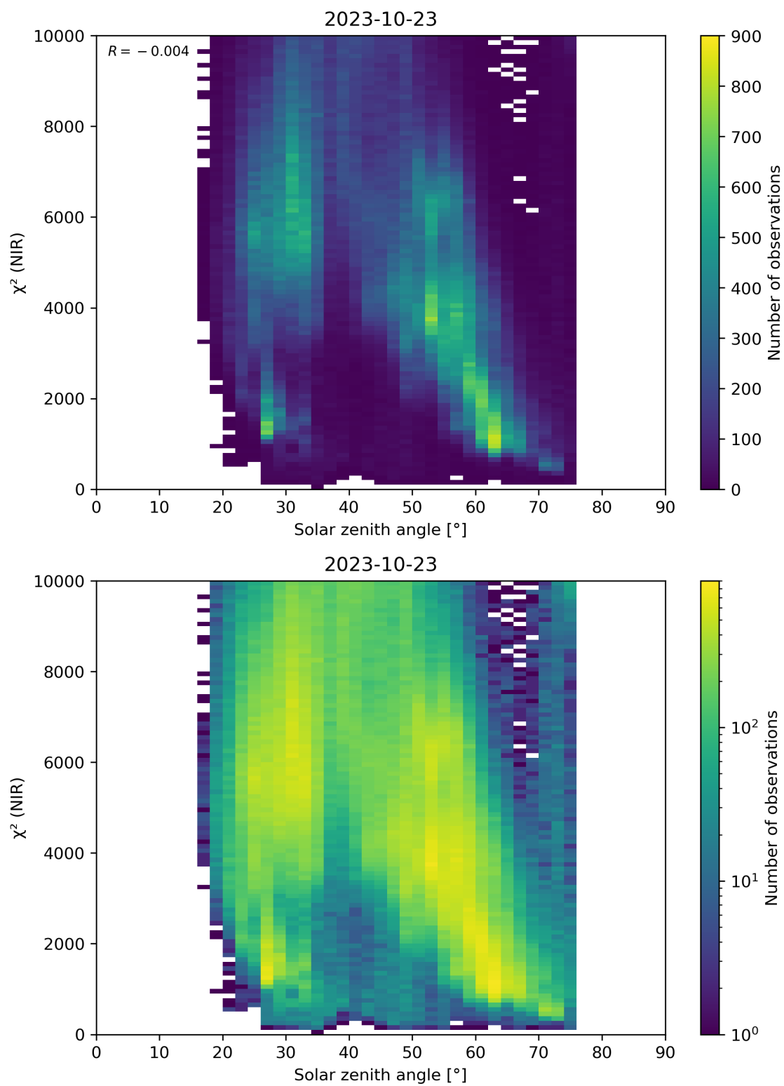
Figure 94: Scatter density plot of “Solar zenith angle” against “ \chi^2 (NIR)” for 2023-10-22 to 2023-10-24.
