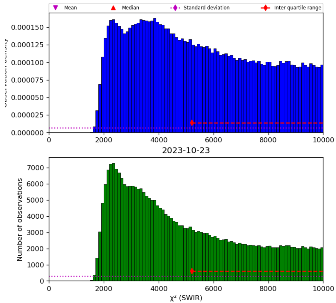
Figure 28: Histogram of “ \chi^2 (SWIR)” for 2023-10-22 to 2023-10-24
