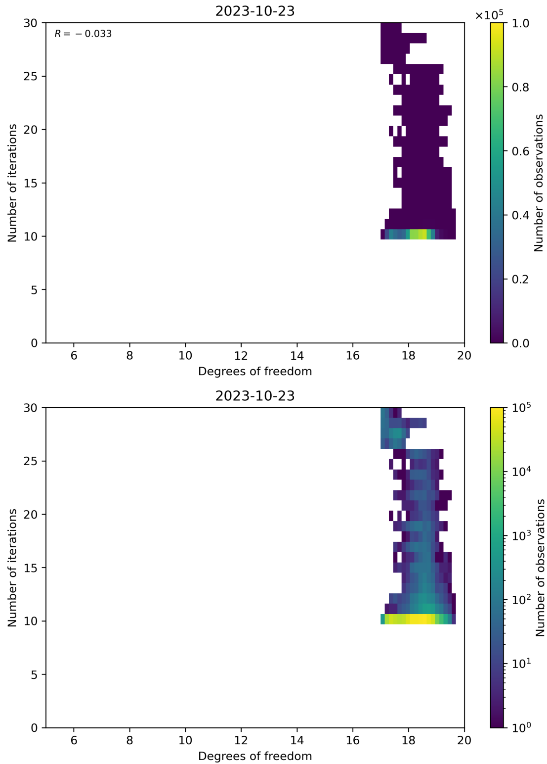
Figure 52: Scatter density plot of “Degrees of freedom” against “Number of iterations” for 2023-10-22 to 2023-10-24.
