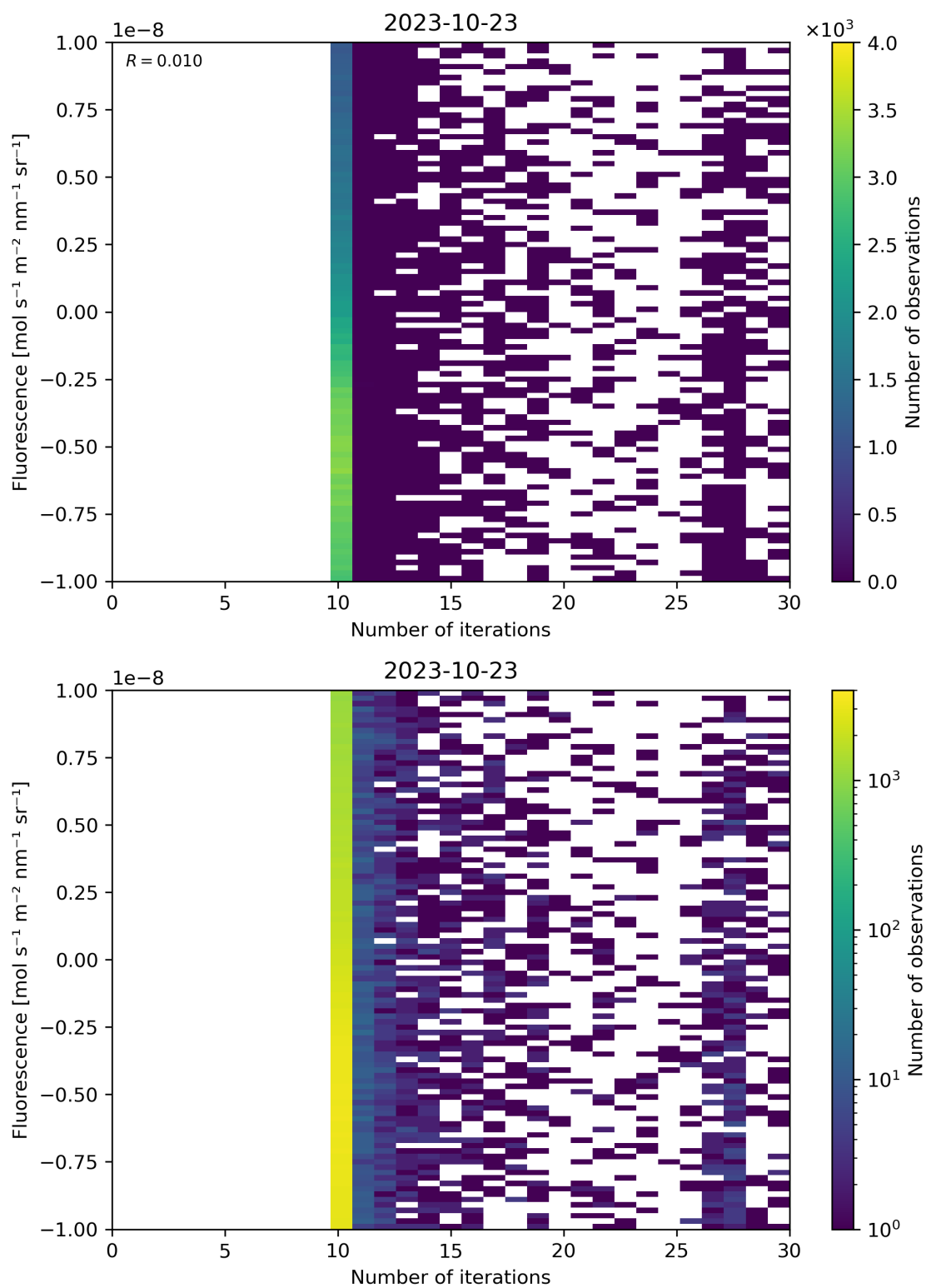
Figure 87: Scatter density plot of “Number of iterations” against “Fluorescence” for 2023-10-22 to 2023-10-24.
