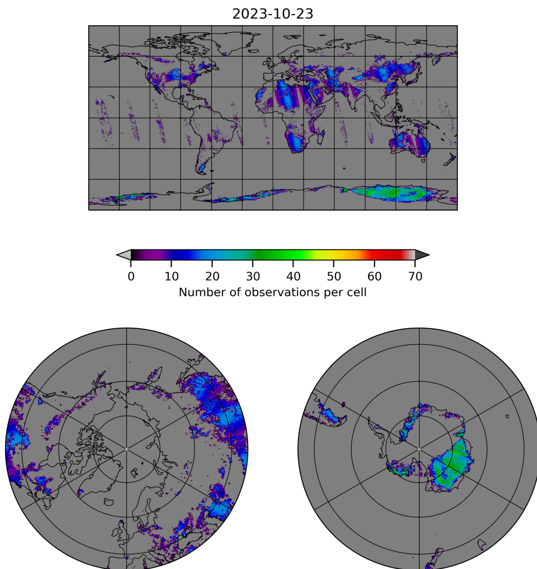
Figure 10: Map of the number of observations for 2023-10-22 to 2023-10-24
