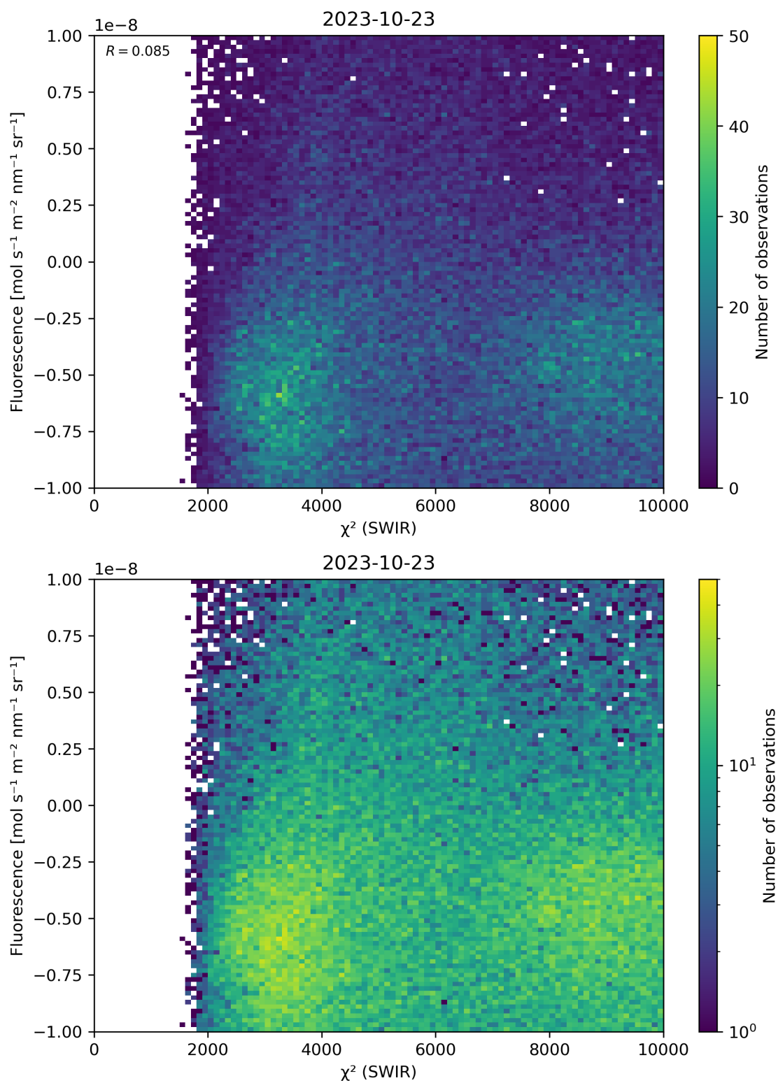
Figure 49: Scatter density plot of “ \chi^2 (SWIR)” against “Fluorescence” for 2023-10-22 to 2023-10-24.
