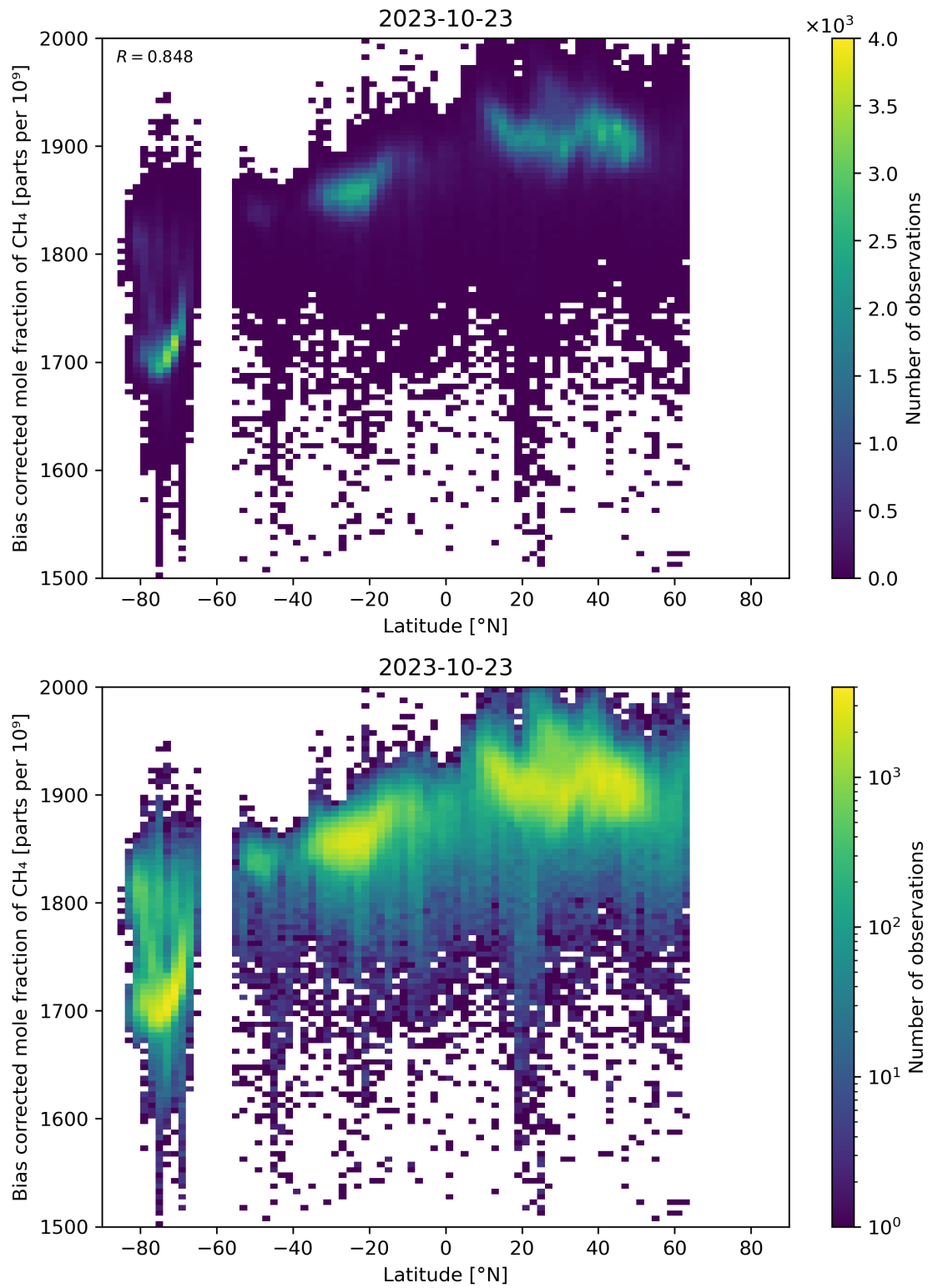
Figure 58: Scatter density plot of “Latitude” against “Bias corrected mole fraction of \text{CH}_4 ” for 2023-10-22 to 2023-10-24.
