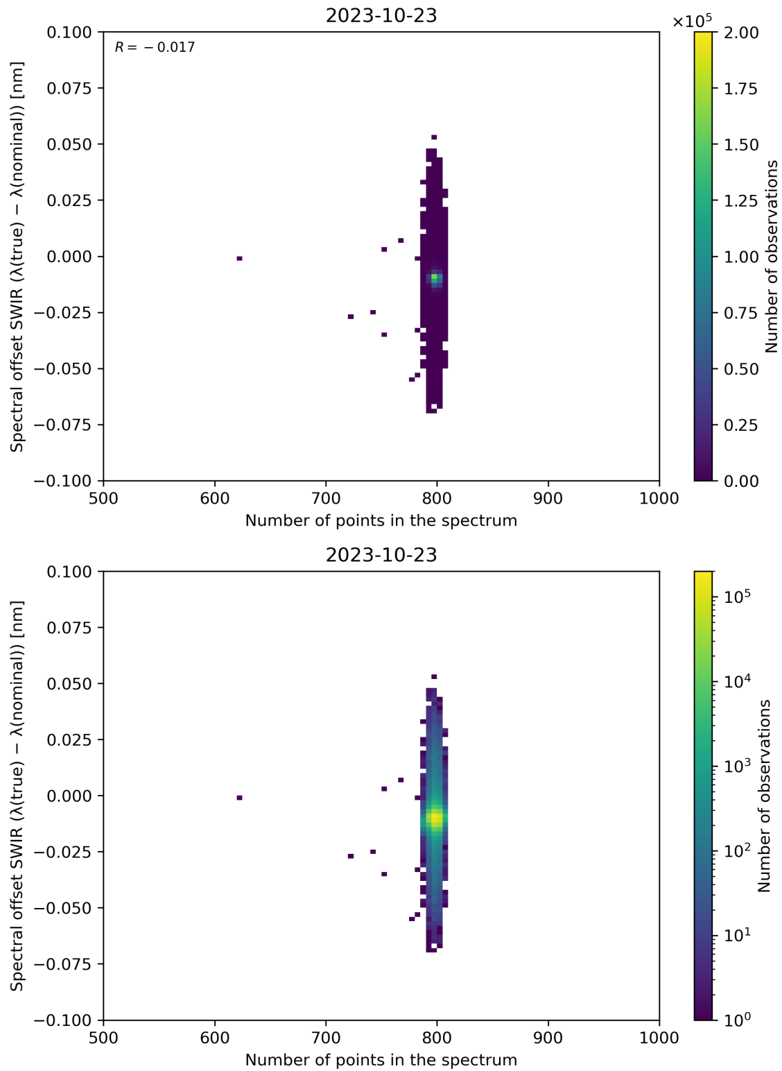
Figure 93: Scatter density plot of “Number of points in the spectrum” against “Spectral offset SWIR ( \lambda(\text{true}) - \lambda(\text{nominal}) )” for 2023-10-22 to 2023-10-24.
