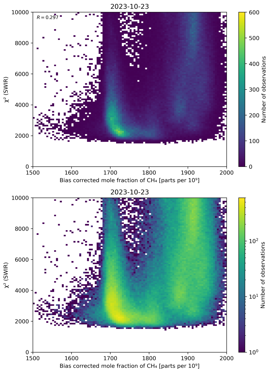
Figure 64: Scatter density plot of “Bias corrected mole fraction of CH 4 ” against “ \chi^2 (SWIR)” for 2023-10-22 to 2023-10-24.
