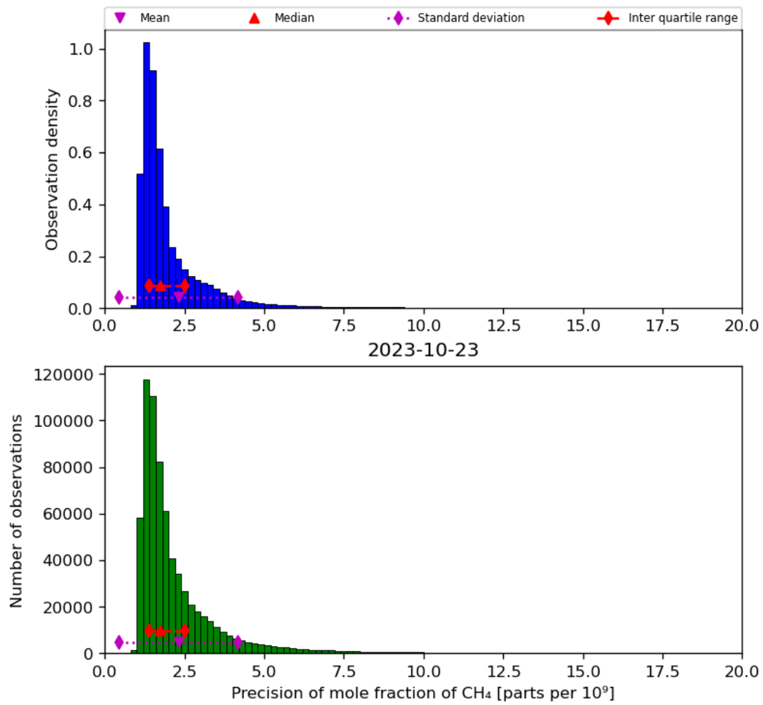
Figure 24: Histogram of “Precision of mole fraction of CH 4 ” for 2023-10-22 to 2023-10-24
