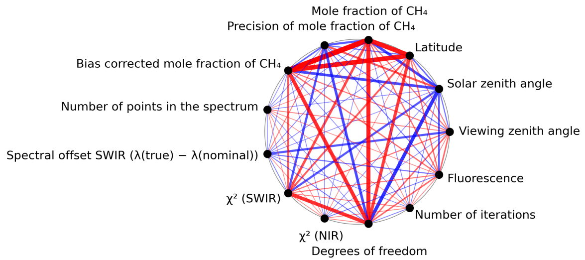
Figure 1: Map of correlation graph for 2023-10-22 to 2023-10-24.
