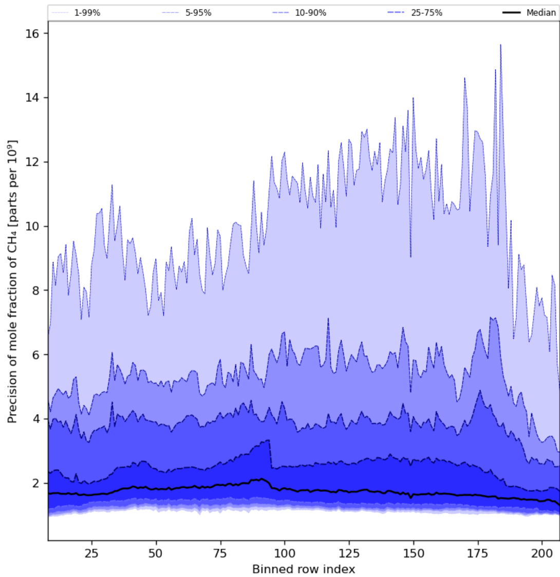
Figure 35: Along track statistics of “Precision of mole fraction of CH 4 ” for 2023-10-22 to 2023-10-24
