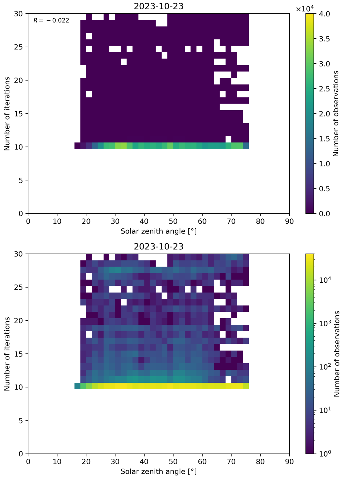
Figure 102: Scatter density plot of “Solar zenith angle” against “Number of iterations” for 2023-10-22 to 2023-10-24.
