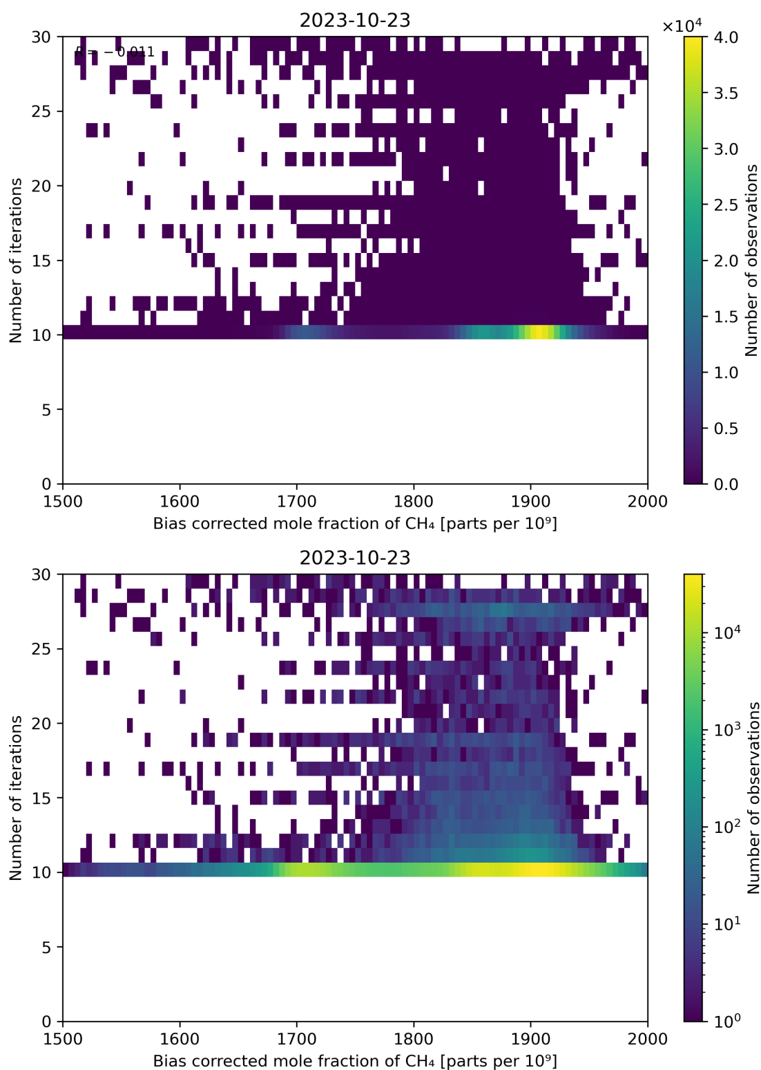
Figure 67: Scatter density plot of “Bias corrected mole fraction of CH 4 ” against “Number of iterations” for 2023-10-22 to 2023-10-24.
