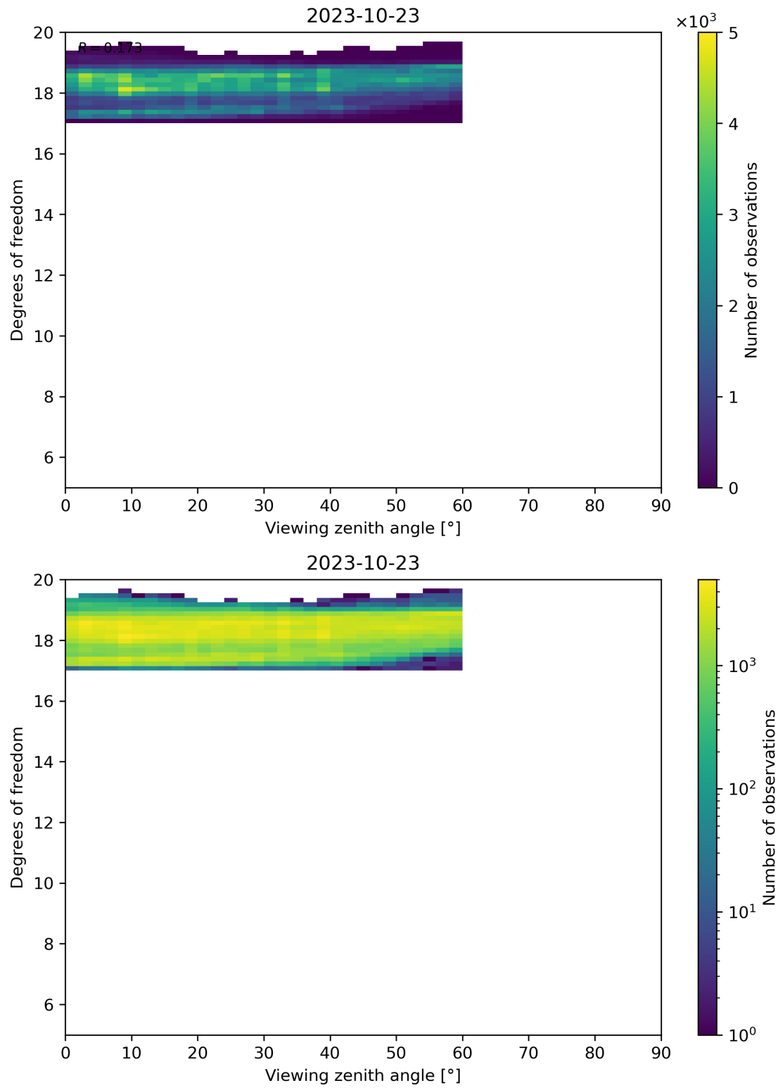
Figure 107: Scatter density plot of “Viewing zenith angle” against “Degrees of freedom” for 2023-10-22 to 2023-10-24.
