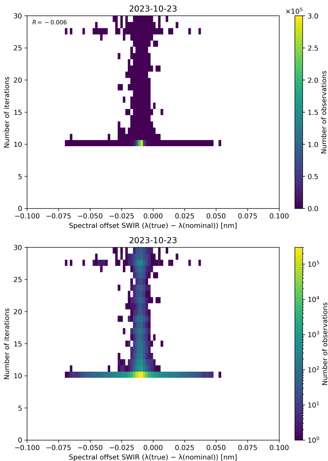
Figure 121: Scatter density plot of “Spectral offset SWIR ( \lambda(\text{true}) - \lambda(\text{nominal}) )” against “Number of iterations” for 2023-10-22 to 2023-10-24.
