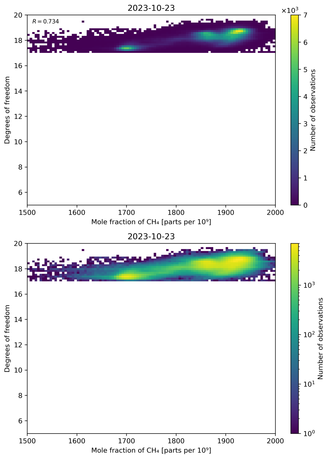
Figure 72: Scatter density plot of “Mole fraction of CH 4 ” against “Degrees of freedom” for 2023-10-22 to 2023-10-24.
