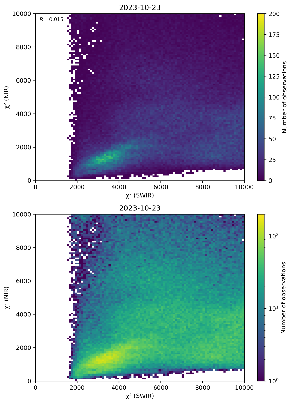
Figure 47: Scatter density plot of “ \chi^2 (SWIR)” against “ \chi^2 (NIR)” for 2023-10-22 to 2023-10-24.
