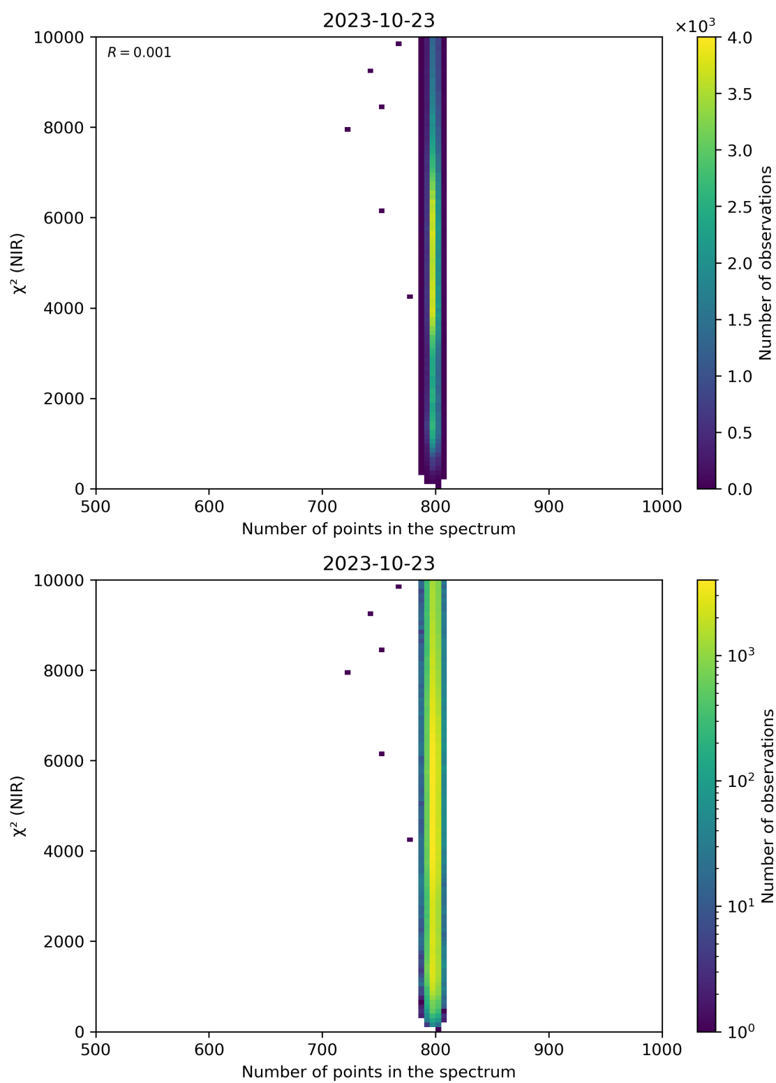
Figure 88: Scatter density plot of “Number of points in the spectrum” against “ \chi^2 (NIR)” for 2023-10-22 to 2023-10-24.
