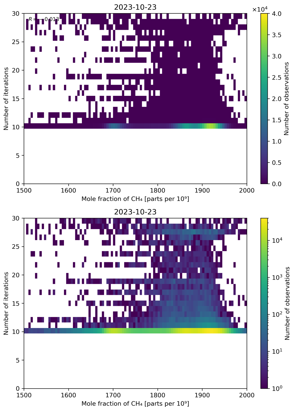
Figure 76: Scatter density plot of “Mole fraction of CH 4 ” against “Number of iterations” for 2023-10-22 to 2023-10-24.
