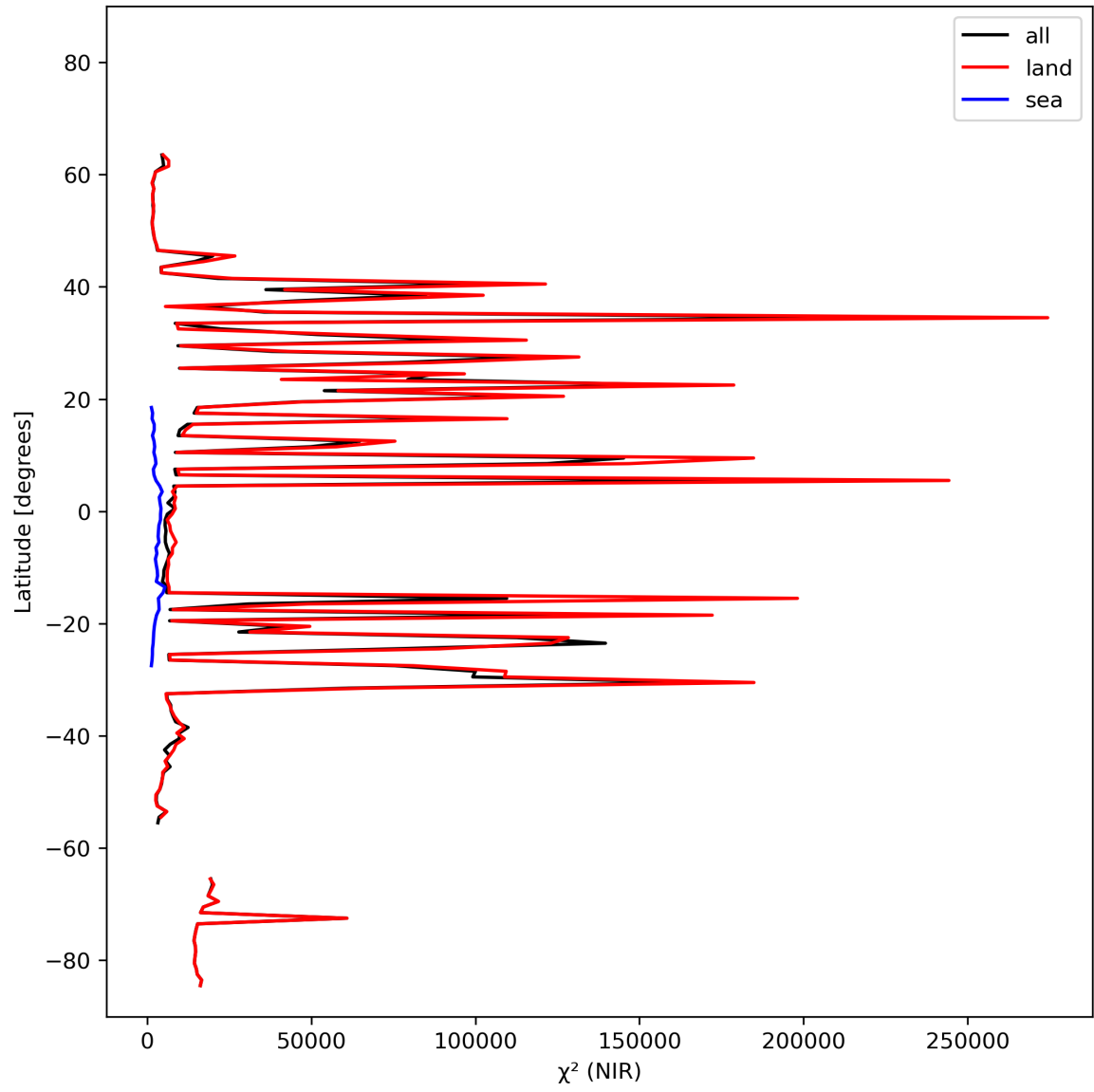
Figure 18: Zonal average of “ \chi^2 (NIR)” for 2023-10-22 to 2023-10-24.
