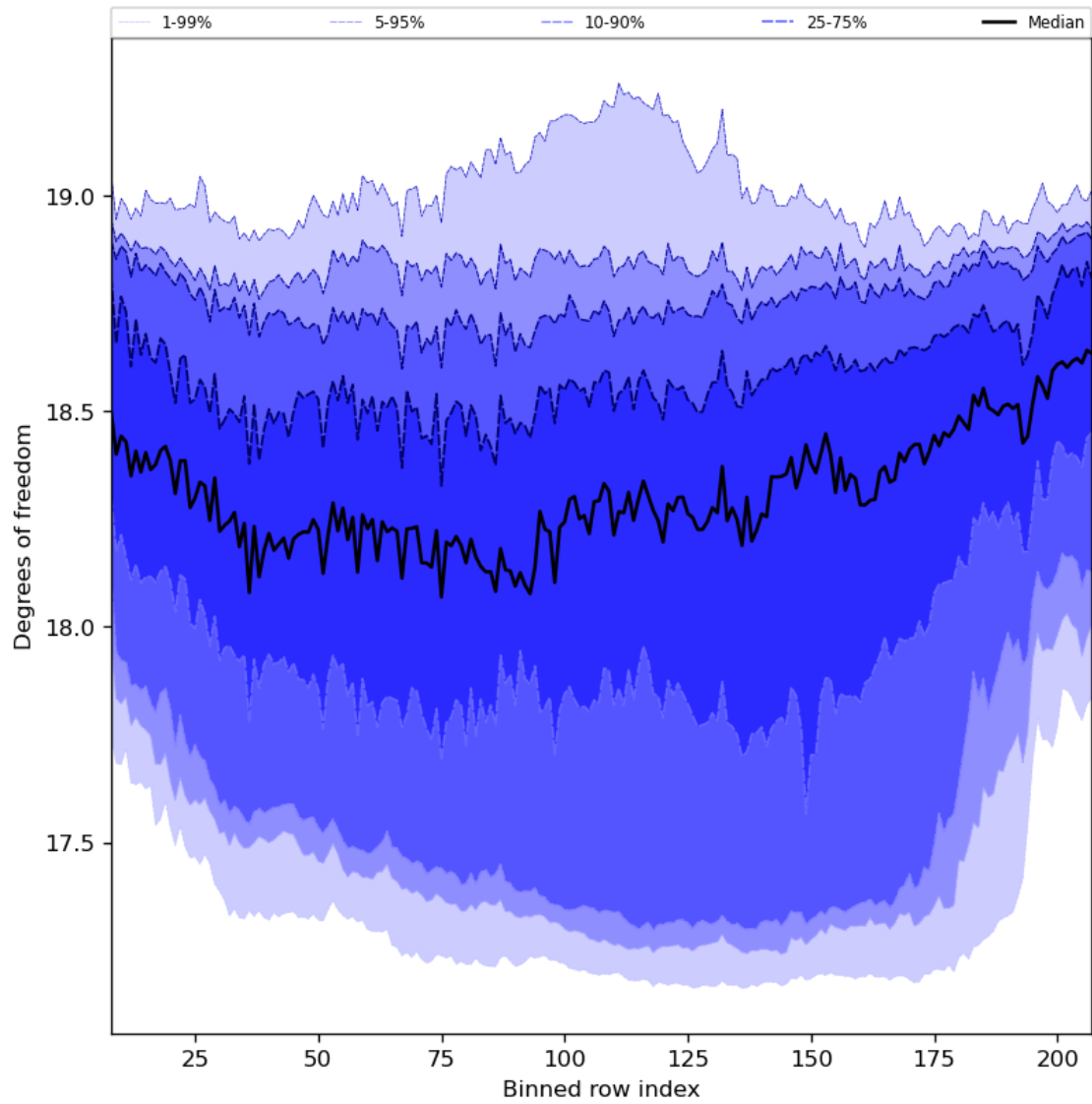
Figure 41: Along track statistics of “Degrees of freedom” for 2023-10-22 to 2023-10-24
