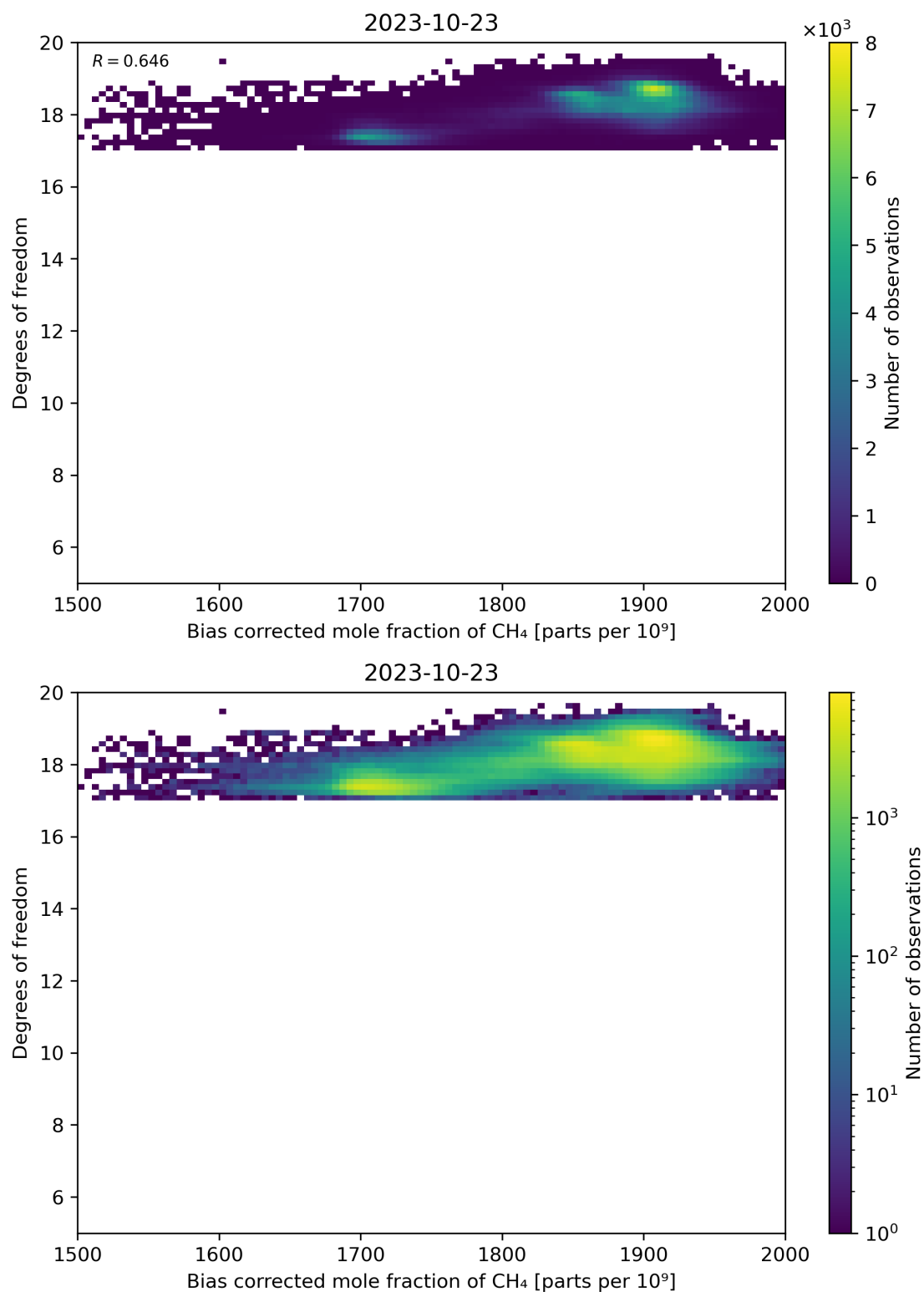
Figure 65: Scatter density plot of “Bias corrected mole fraction of CH 4 ” against “Degrees of freedom” for 2023-10-22 to 2023-10-24.
