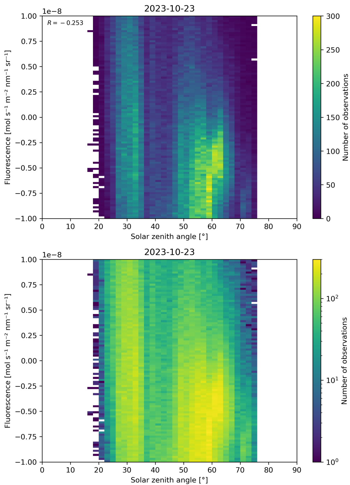
Figure 97: Scatter density plot of “Solar zenith angle” against “Fluorescence” for 2023-10-22 to 2023-10-24.
