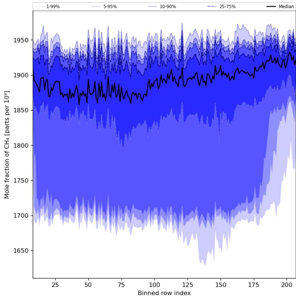
Figure 34: Along track statistics of “Mole fraction of CH 4 ” for 2023-10-22 to 2023-10-24
