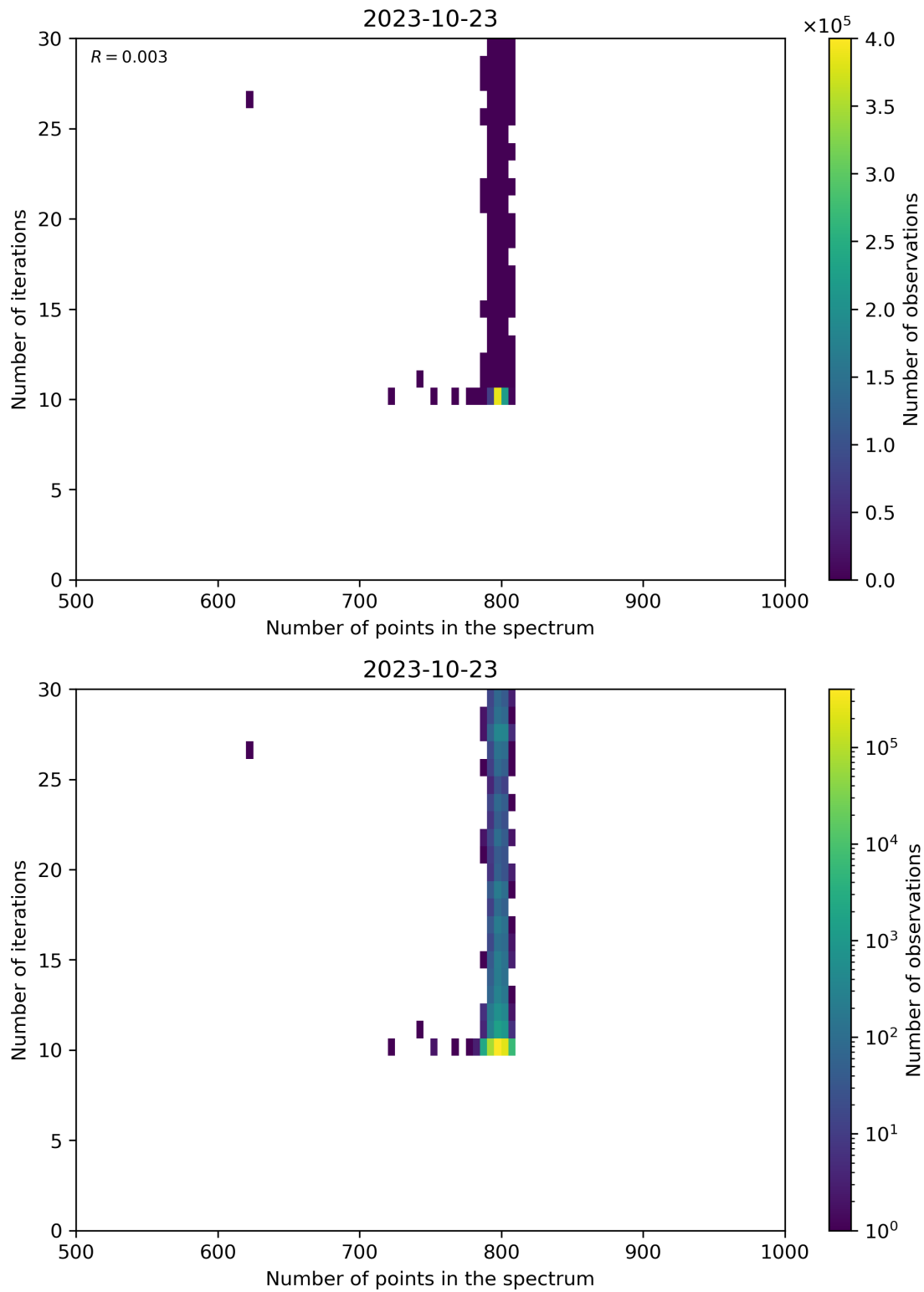
Figure 92: Scatter density plot of “Number of points in the spectrum” against “Number of iterations” for 2023-10-22 to 2023-10-24.
