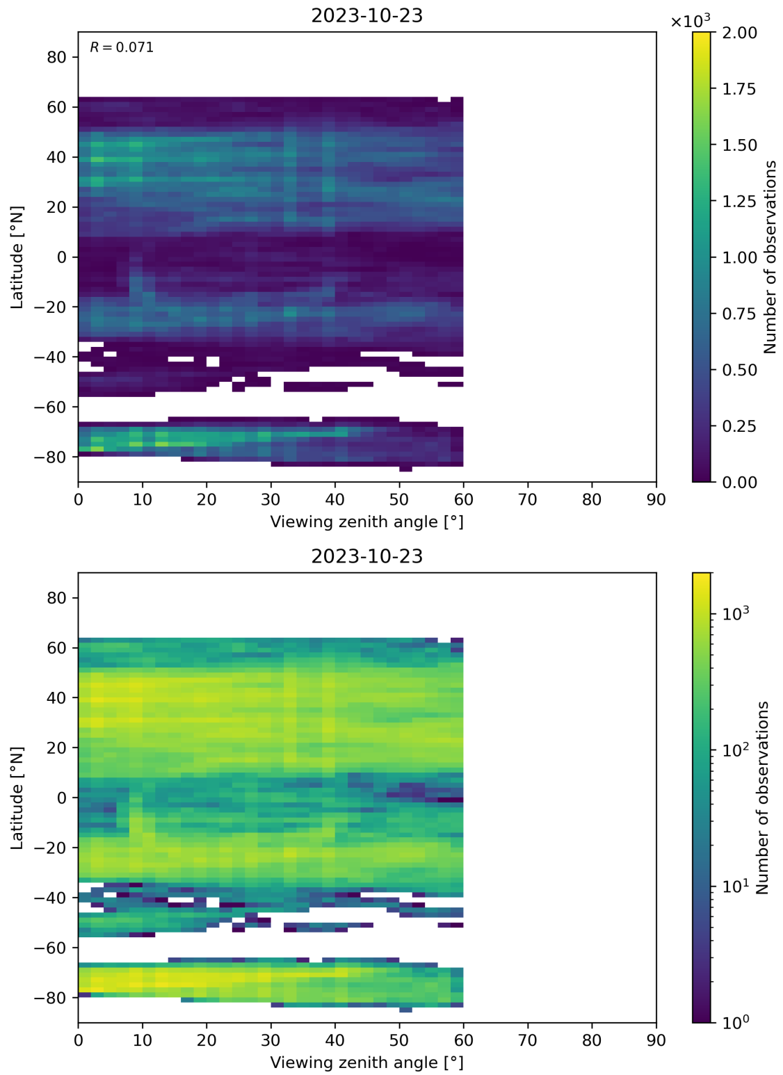
Figure 109: Scatter density plot of “Viewing zenith angle” against “Latitude” for 2023-10-22 to 2023-10-24.
