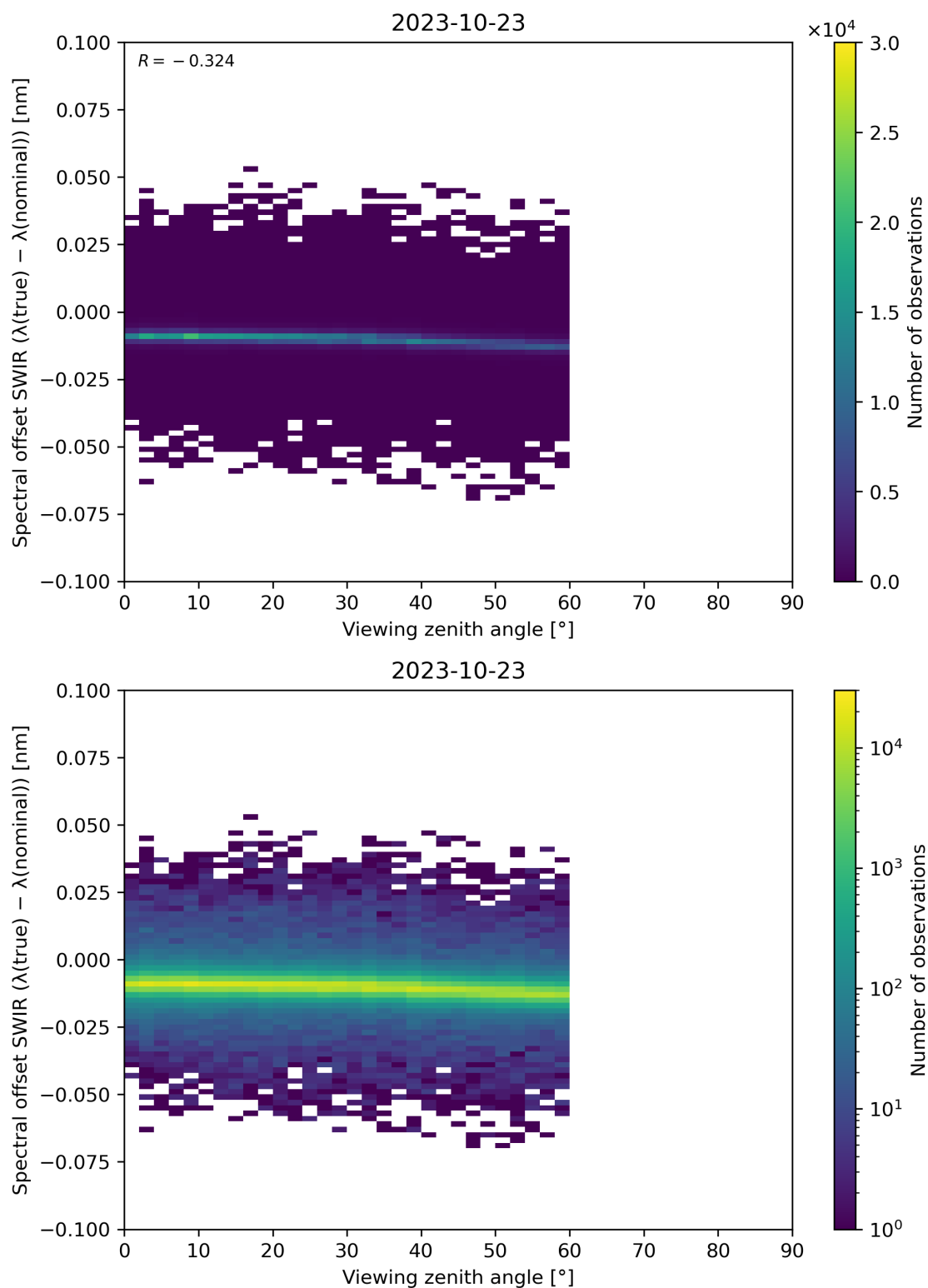
Figure 116: Scatter density plot of “Viewing zenith angle” against “Spectral offset SWIR ( \lambda(\text{true}) - \lambda(\text{nominal}) )” for 2023-10-22 to 2023-10-24.
