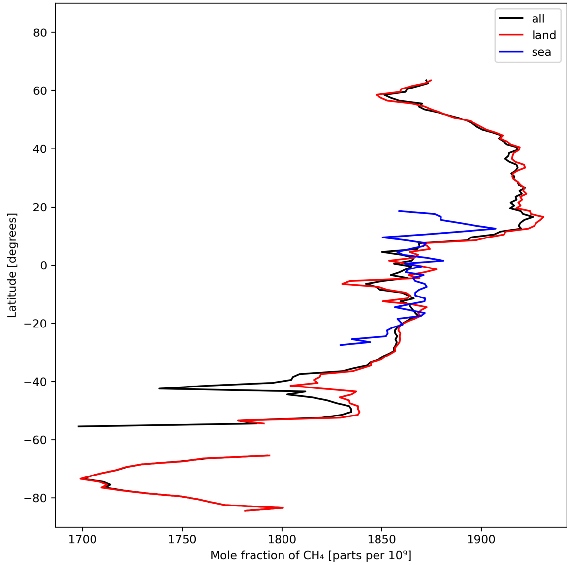
Figure 12: Zonal average of “Mole fraction of CH 4 ” for 2023-10-22 to 2023-10-24.
