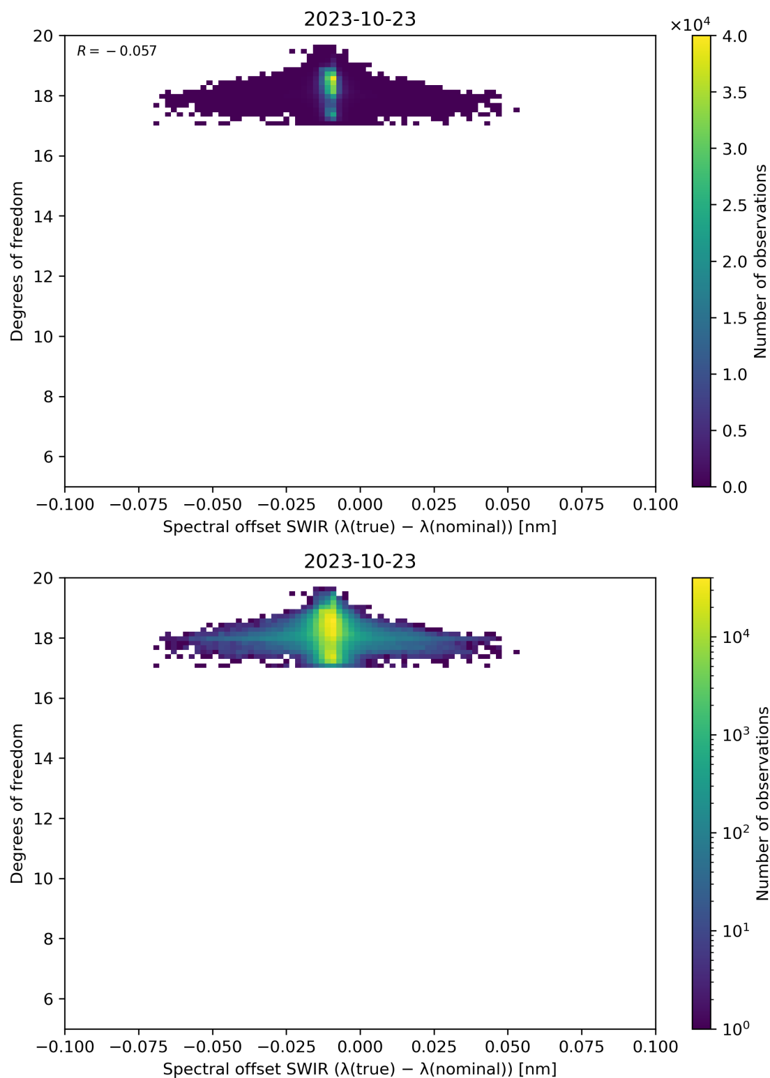
Figure 119: Scatter density plot of “Spectral offset SWIR ( \lambda(\text{true}) - \lambda(\text{nominal}) )” against “Degrees of freedom” for 2023-10-22 to 2023-10-24.
