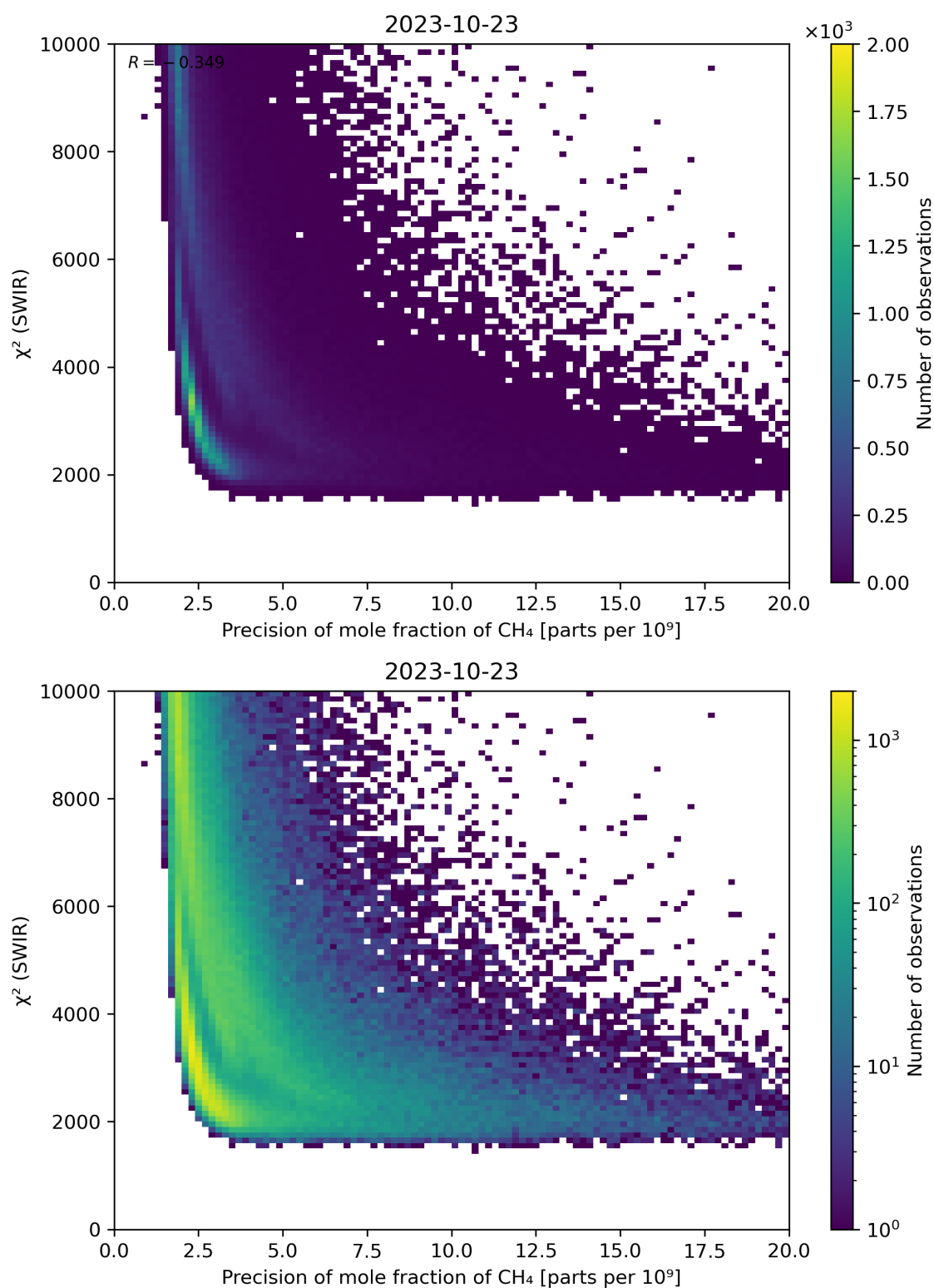
Figure 79: Scatter density plot of “Precision of mole fraction of CH 4 ” against “ \chi^2 (SWIR)” for 2023-10-22 to 2023-10-24.
