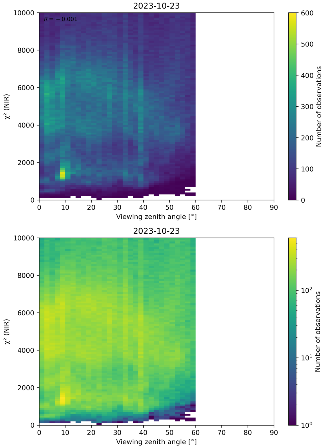
Figure 105: Scatter density plot of “Viewing zenith angle” against “ \chi^2 (NIR)” for 2023-10-22 to 2023-10-24.
