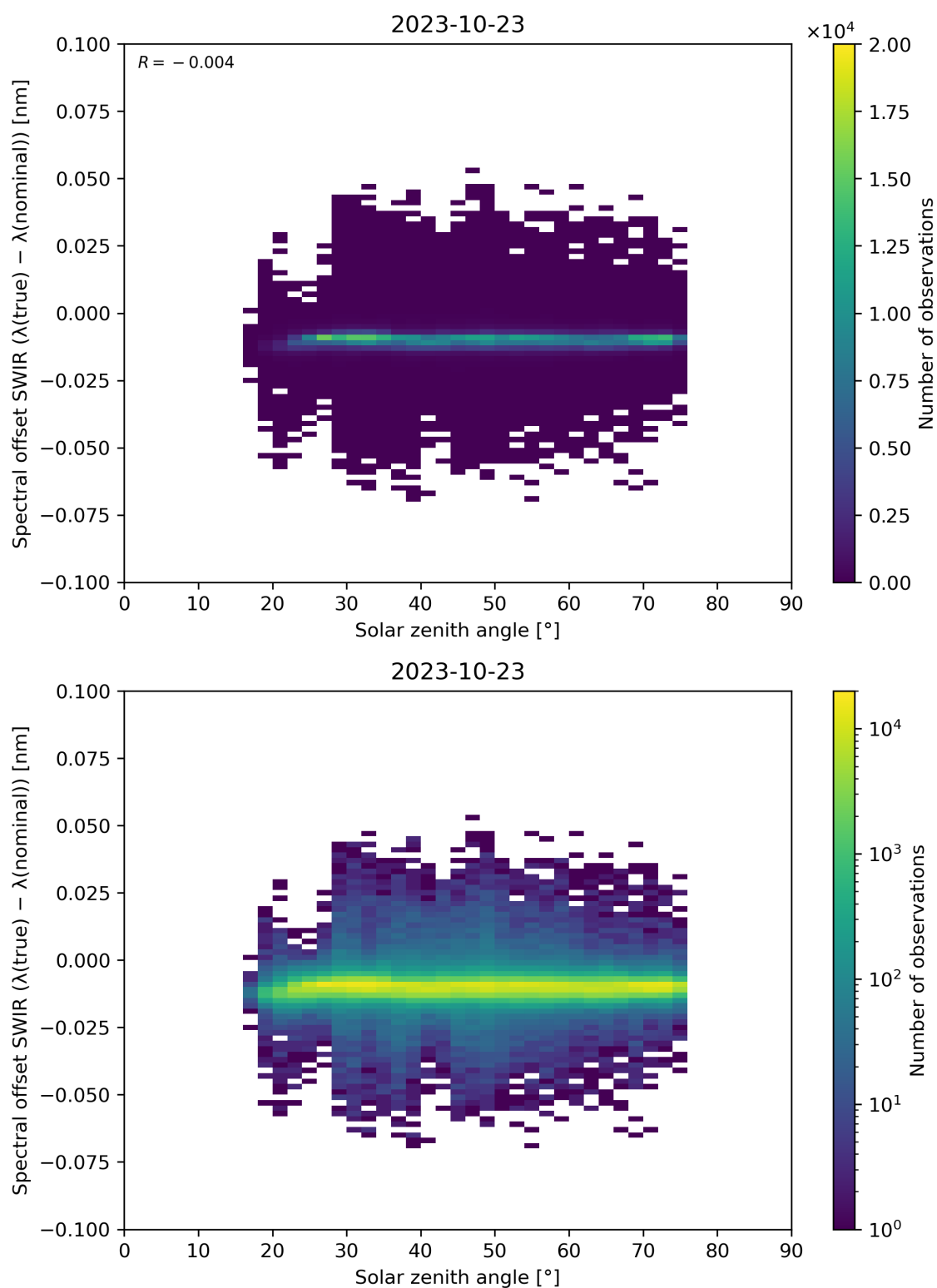
Figure 104: Scatter density plot of “Solar zenith angle” against “Spectral offset SWIR ( \lambda(\text{true}) - \lambda(\text{nominal}) )” for 2023-10-22 to 2023-10-24.
