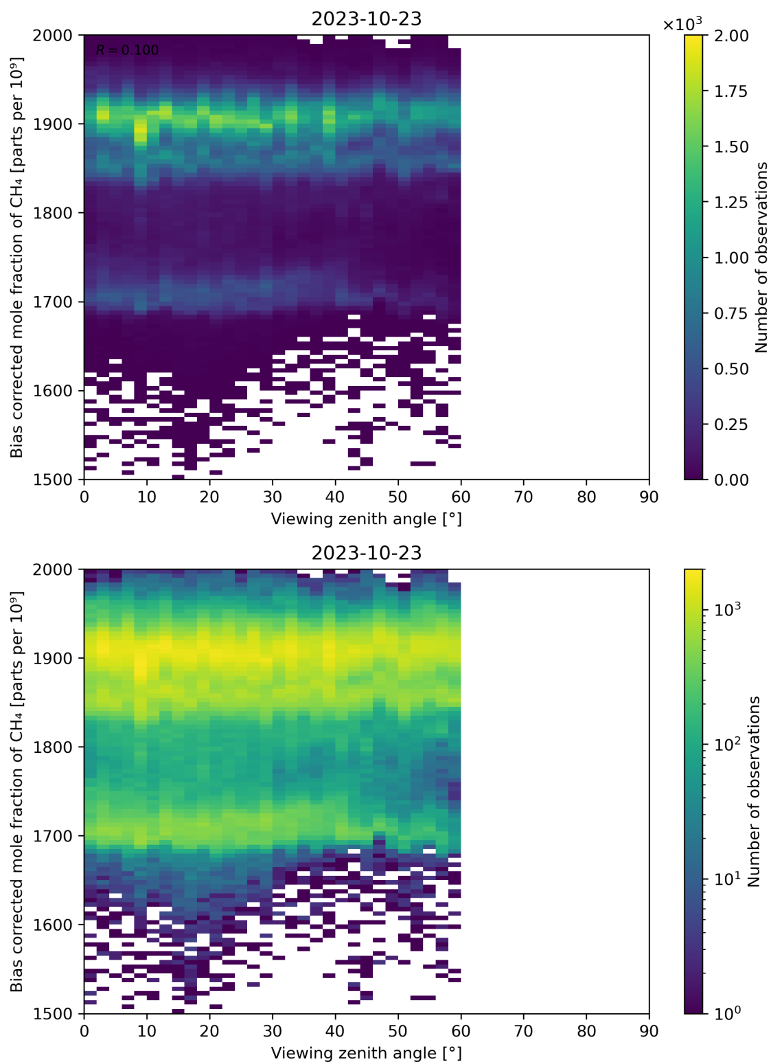
Figure 111: Scatter density plot of “Viewing zenith angle” against “Bias corrected mole fraction of CH 4 ” for 2023-10-22 to 2023-10-24.
