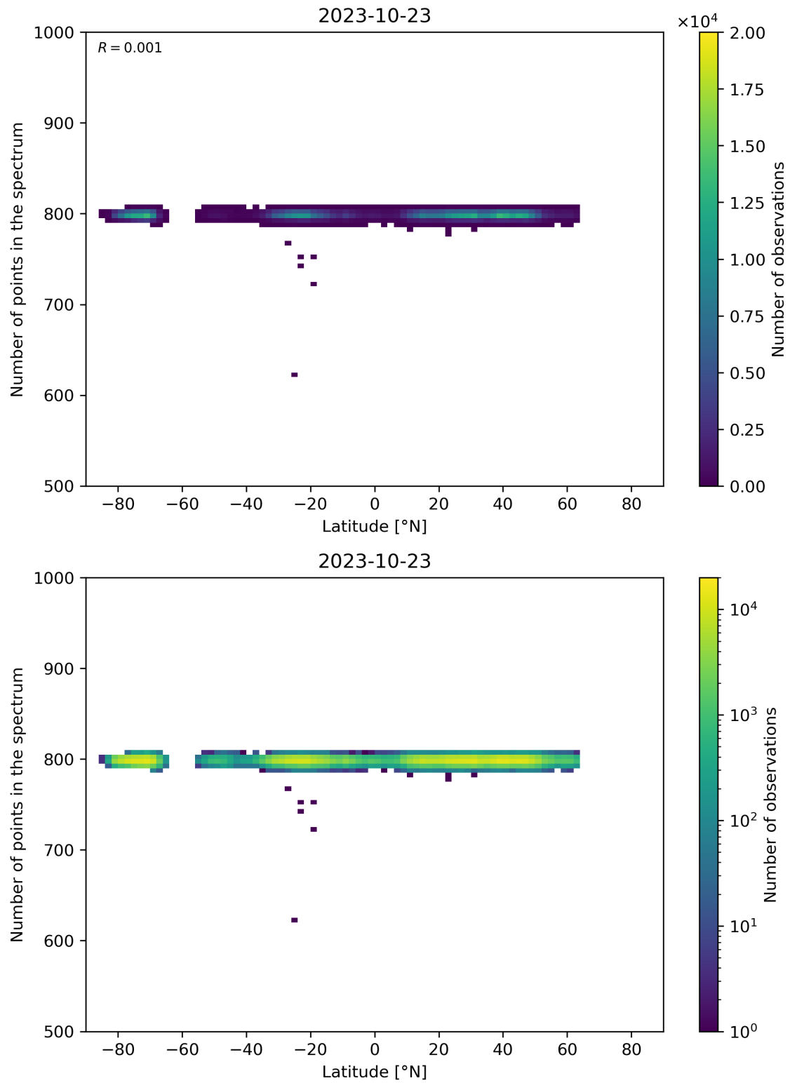
Figure 61: Scatter density plot of “Latitude” against “Number of points in the spectrum” for 2023-10-22 to 2023-10-24.
