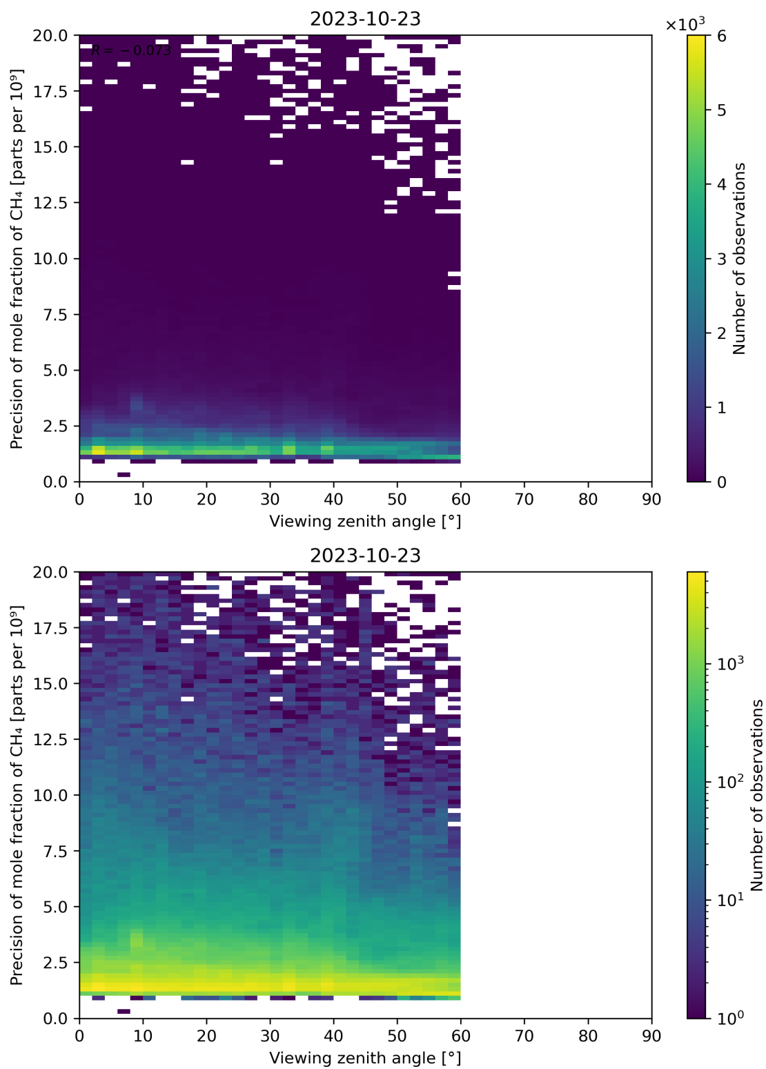
Figure 112: Scatter density plot of “Viewing zenith angle” against “Precision of mole fraction of CH 4 ” for 2023-10-22 to 2023-10-24.
