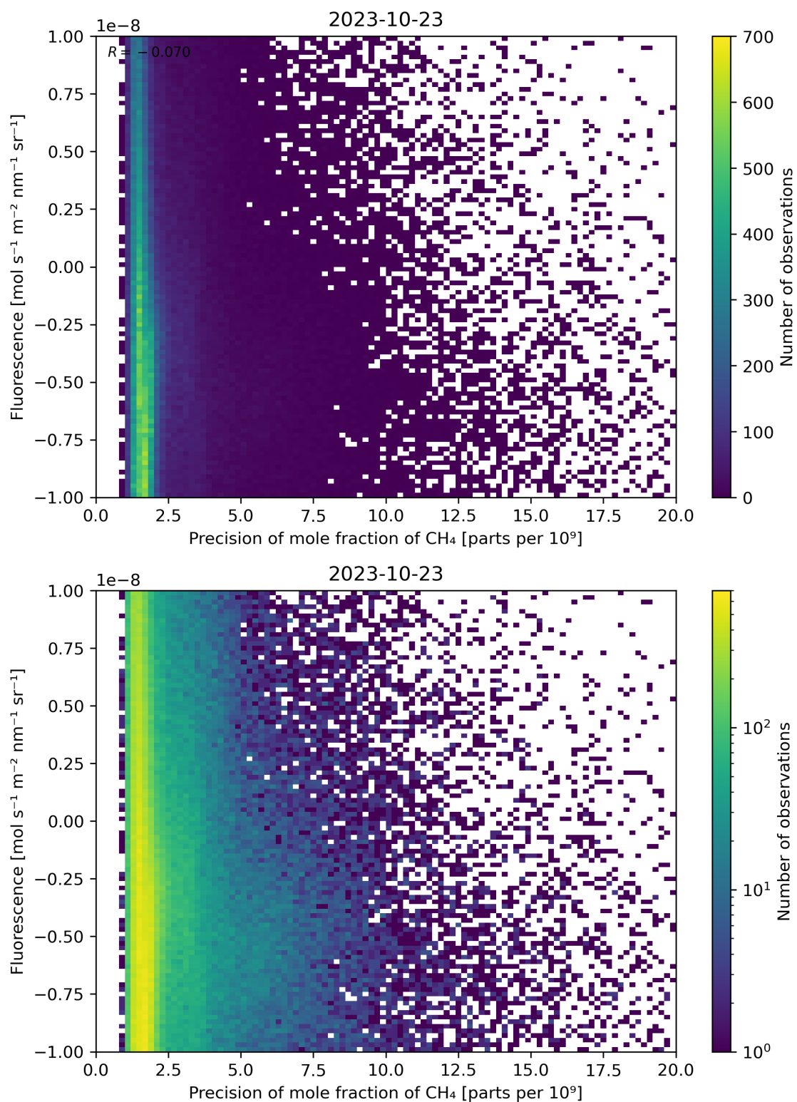
Figure 81: Scatter density plot of “Precision of mole fraction of \text{CH}_4 ” against “Fluorescence” for 2023-10-22 to 2023-10-24.
