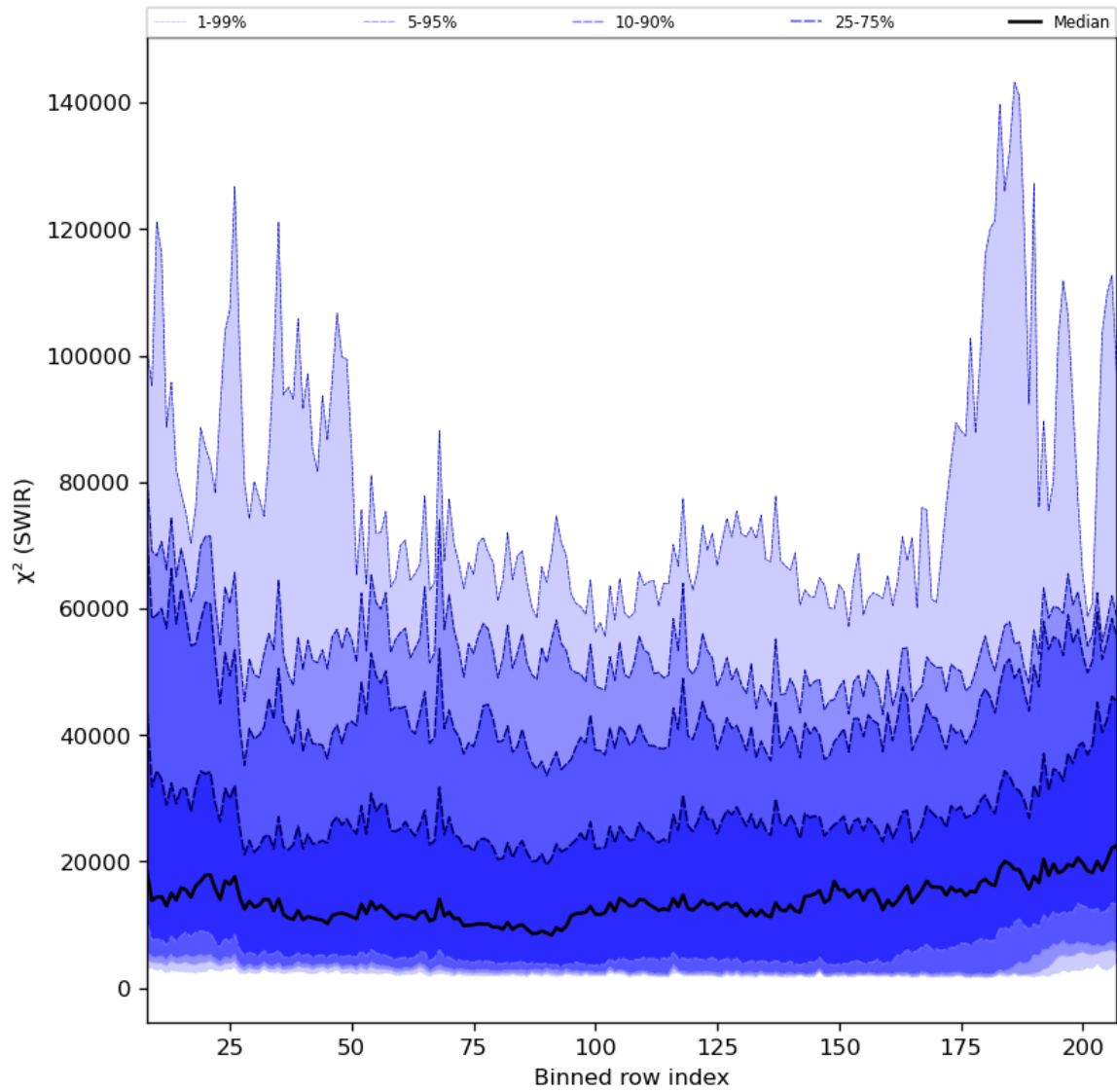
Figure 39: Along track statistics of “ \chi^2 (SWIR)” for 2023-10-22 to 2023-10-24
