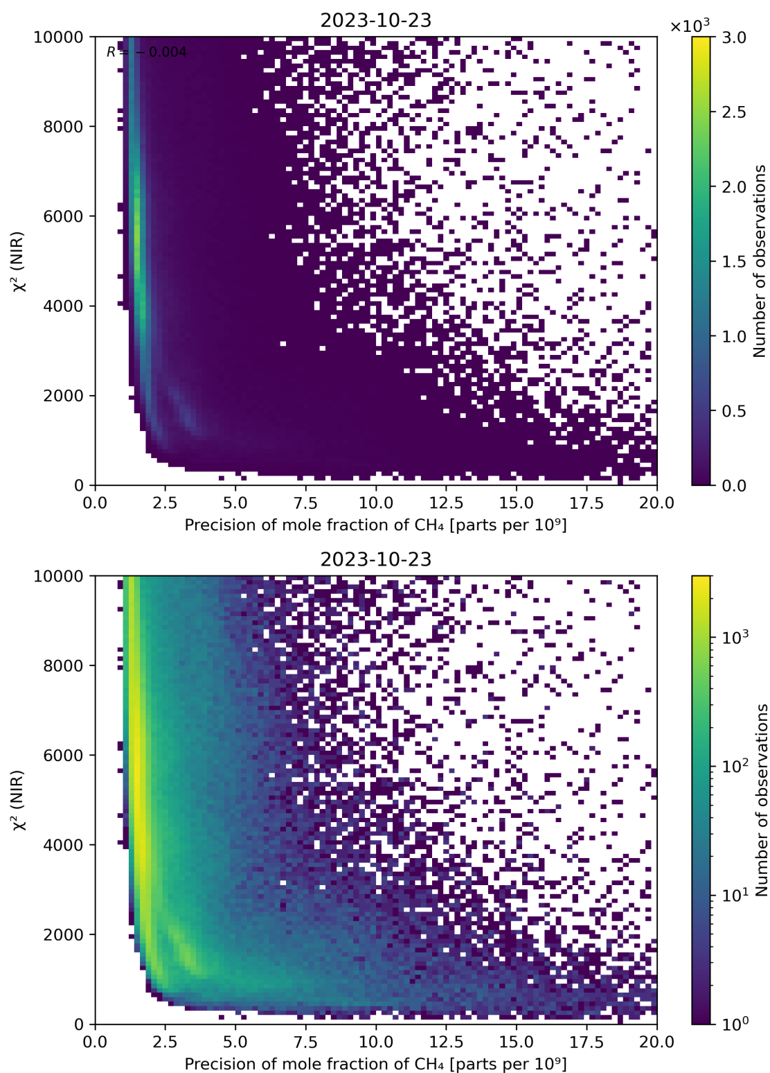
Figure 78: Scatter density plot of “Precision of mole fraction of CH 4 ” against “ \chi^2 (NIR)” for 2023-10-22 to 2023-10-24.
