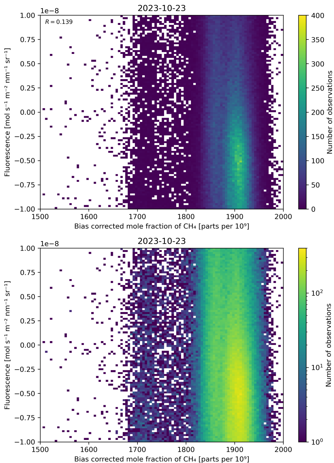
Figure 66: Scatter density plot of “Bias corrected mole fraction of \text{CH}_4 ” against “Fluorescence” for 2023-10-22 to 2023-10-24.
