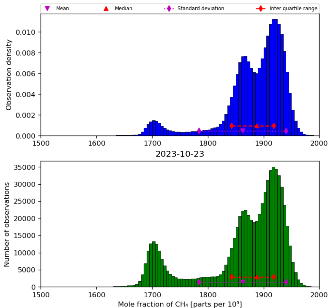
Figure 23: Histogram of “Mole fraction of CH 4 ” for 2023-10-22 to 2023-10-24
