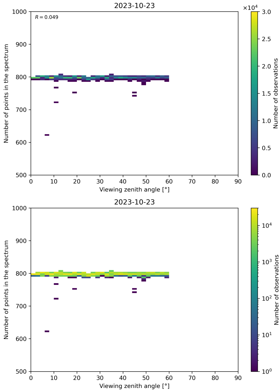
Figure 114: Scatter density plot of “Viewing zenith angle” against “Number of points in the spectrum” for 2023-10-22 to 2023-10-24.
