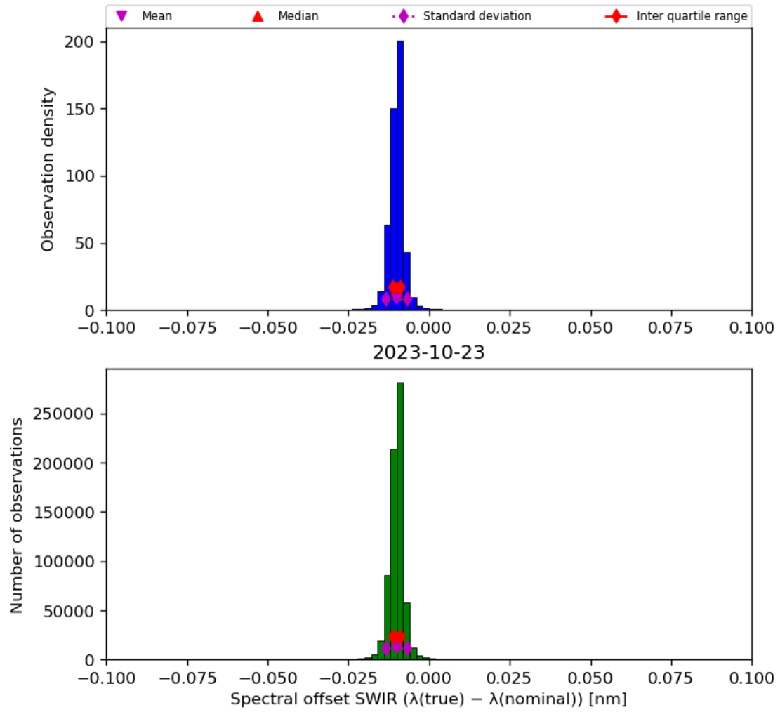
Figure 27: Histogram of “Spectral offset SWIR ( \lambda(\text{true}) - \lambda(\text{nominal}) )” for 2023-10-22 to 2023-10-24
