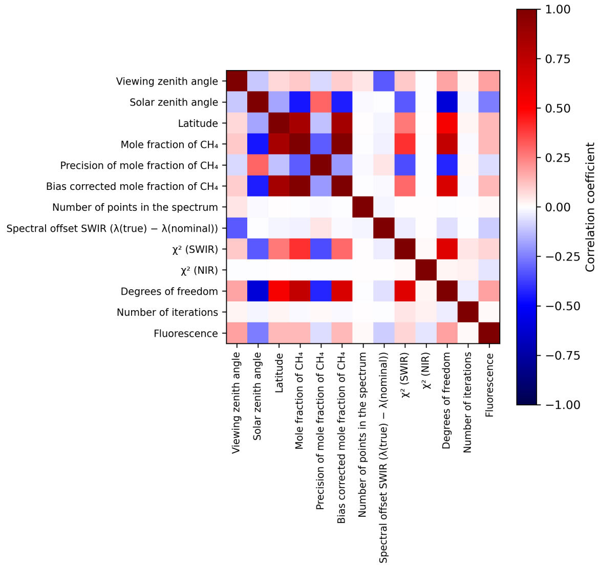
Figure 2: Map of correlation matrix for 2023-10-22 to 2023-10-24.
