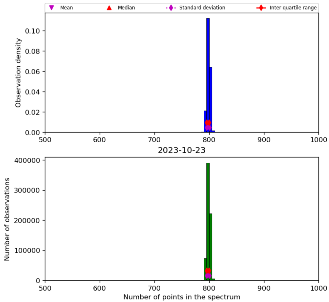
Figure 26: Histogram of “Number of points in the spectrum” for 2023-10-22 to 2023-10-24
