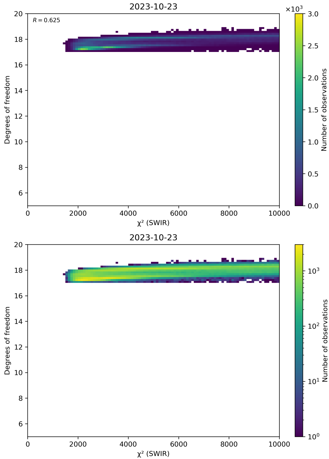
Figure 48: Scatter density plot of “ \chi^2 (SWIR)” against “Degrees of freedom” for 2023-10-22 to 2023-10-24.
