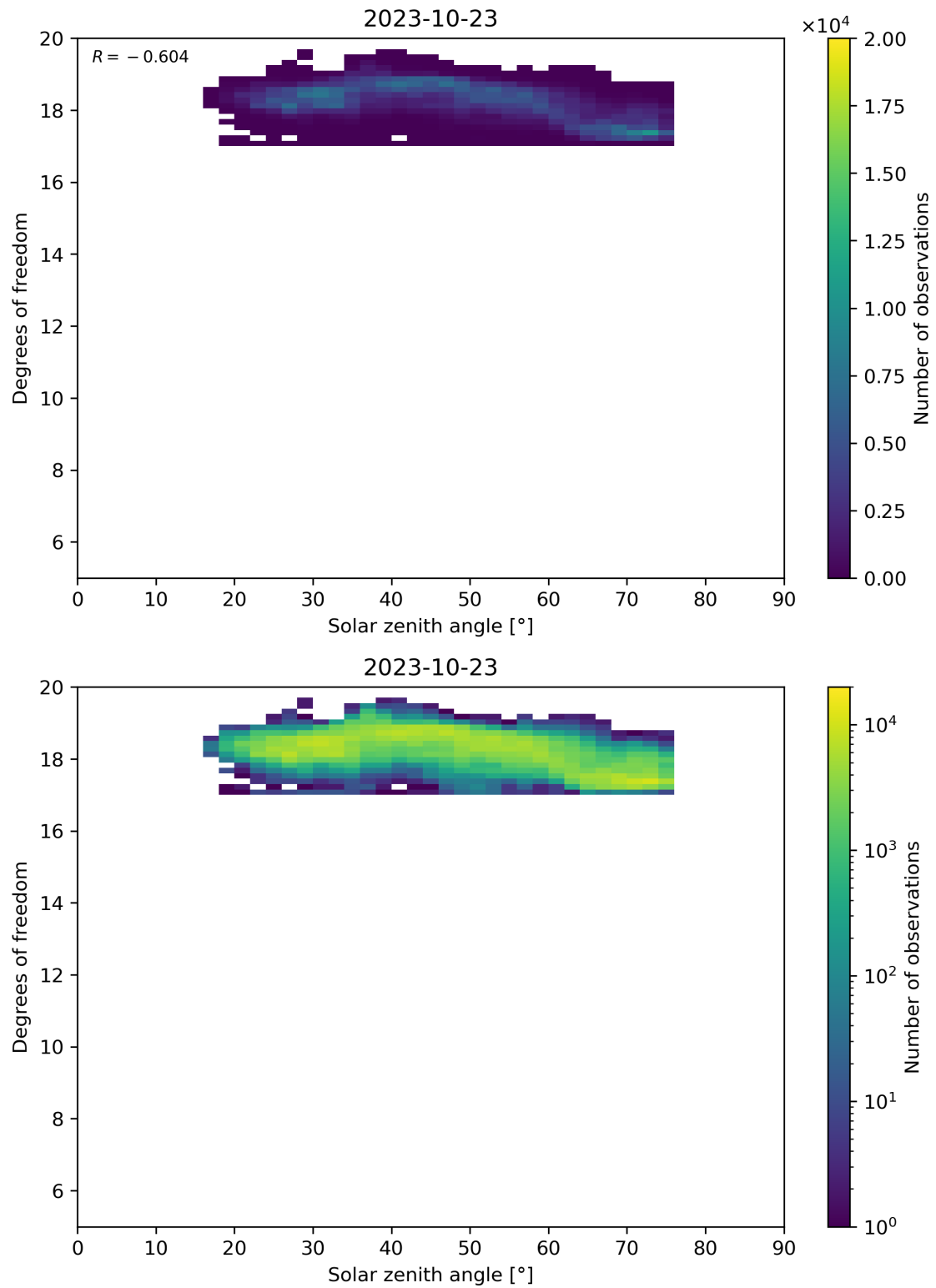
Figure 96: Scatter density plot of “Solar zenith angle” against “Degrees of freedom” for 2023-10-22 to 2023-10-24.
