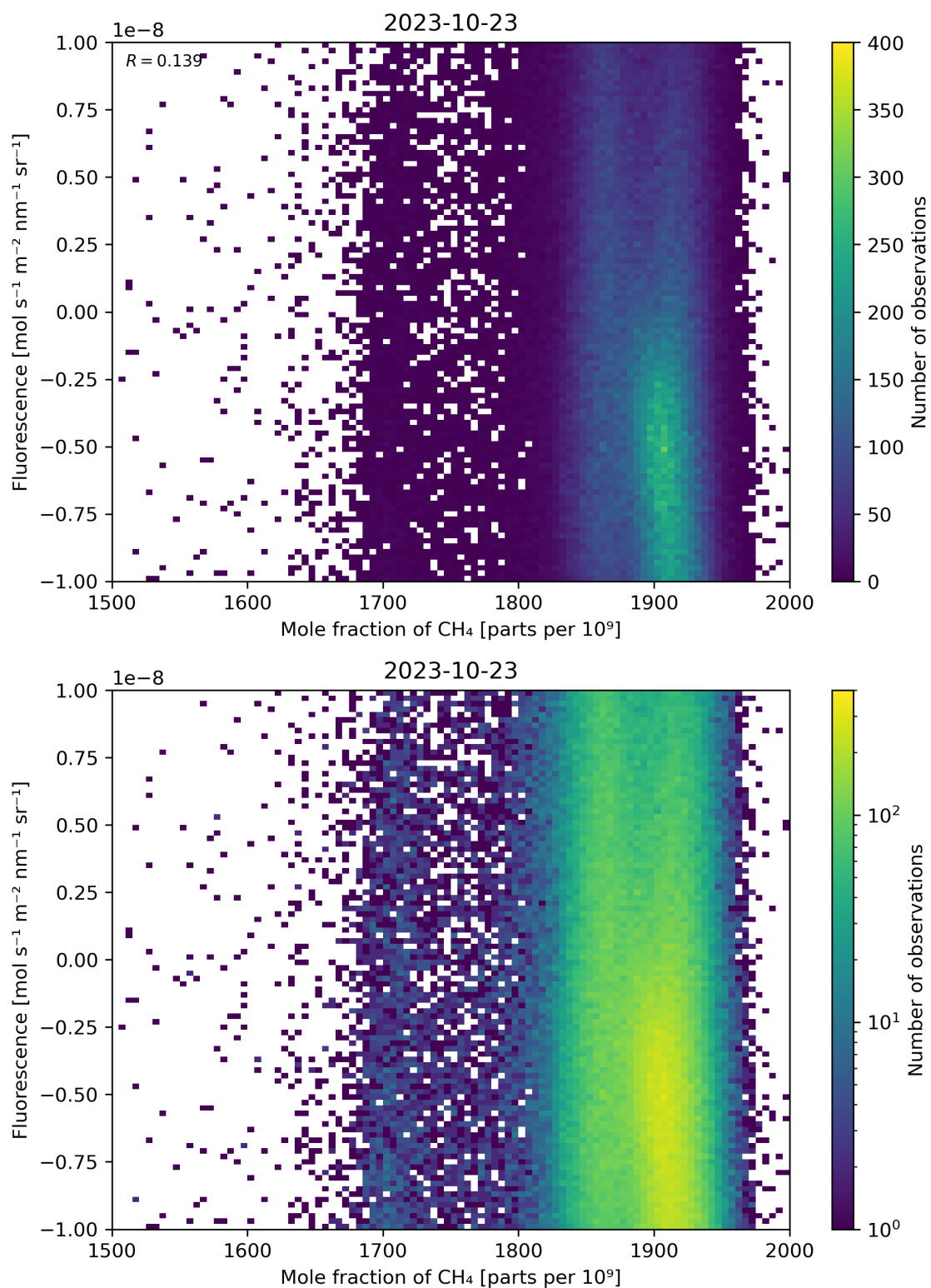
Figure 73: Scatter density plot of “Mole fraction of CH 4 ” against “Fluorescence” for 2023-10-22 to 2023-10-24.
