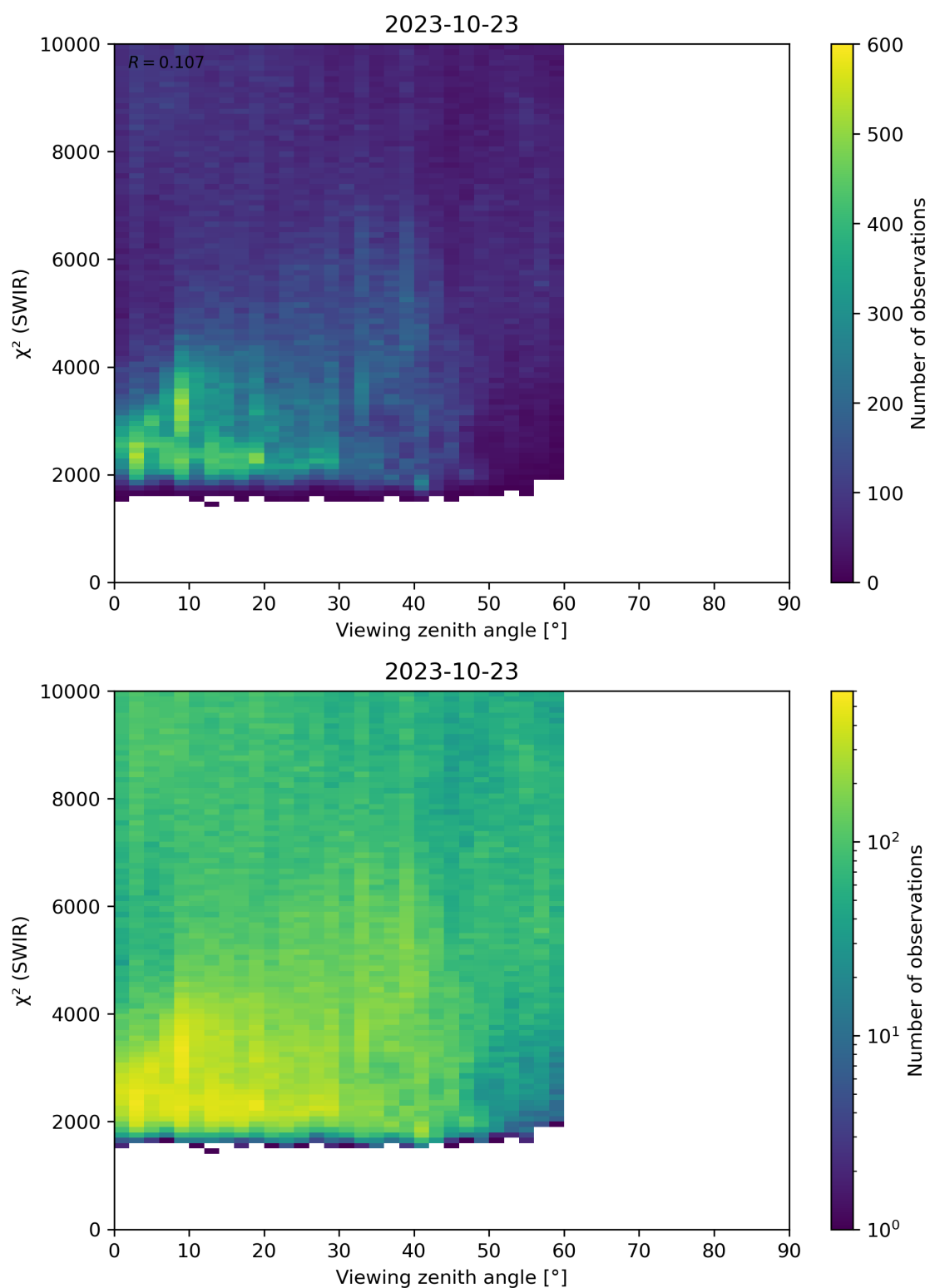
Figure 106: Scatter density plot of “Viewing zenith angle” against “ \chi^2 (SWIR)” for 2023-10-22 to 2023-10-24.
