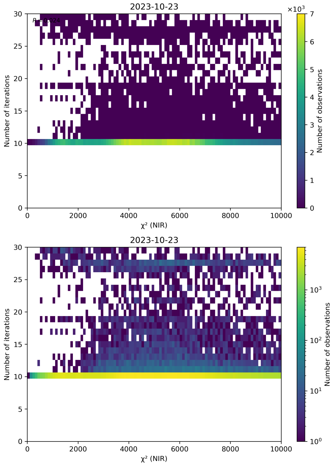
Figure 46: Scatter density plot of “ \chi^2 (NIR)” against “Number of iterations” for 2023-10-22 to 2023-10-24.
