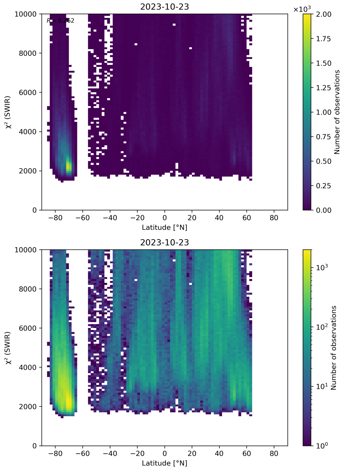
Figure 54: Scatter density plot of “Latitude” against “ \chi^2 (SWIR)” for 2023-10-22 to 2023-10-24.
