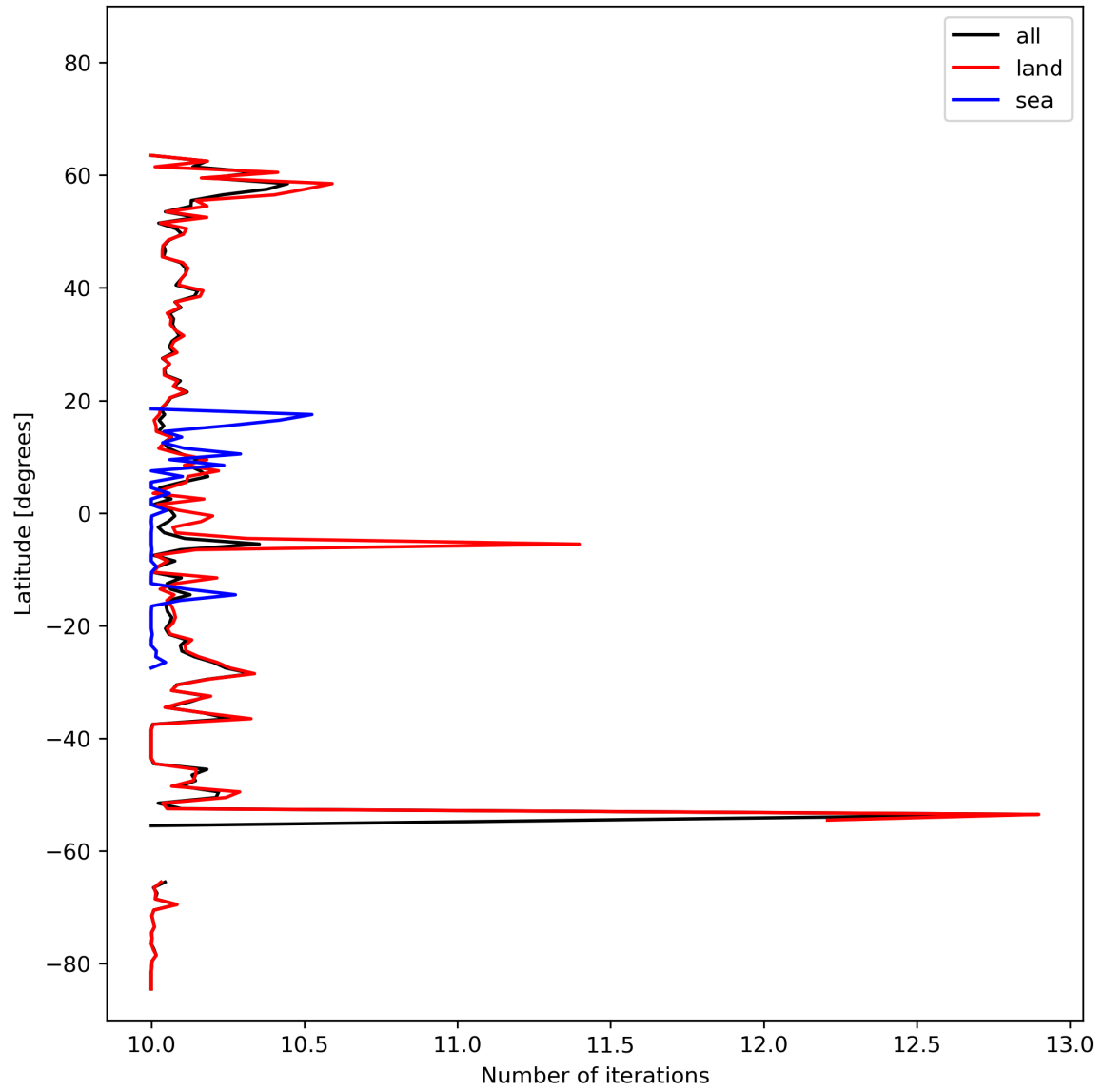
Figure 20: Zonal average of “Number of iterations” for 2023-10-22 to 2023-10-24.
