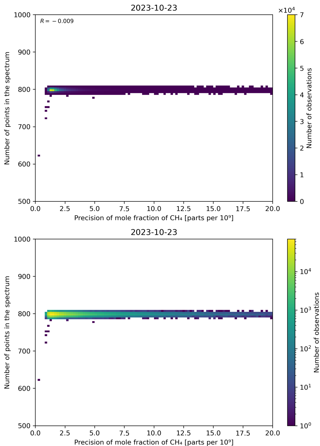
Figure 84: Scatter density plot of “Precision of mole fraction of CH 4 ” against “Number of points in the spectrum” for 2023-10-22 to 2023-10-24.
