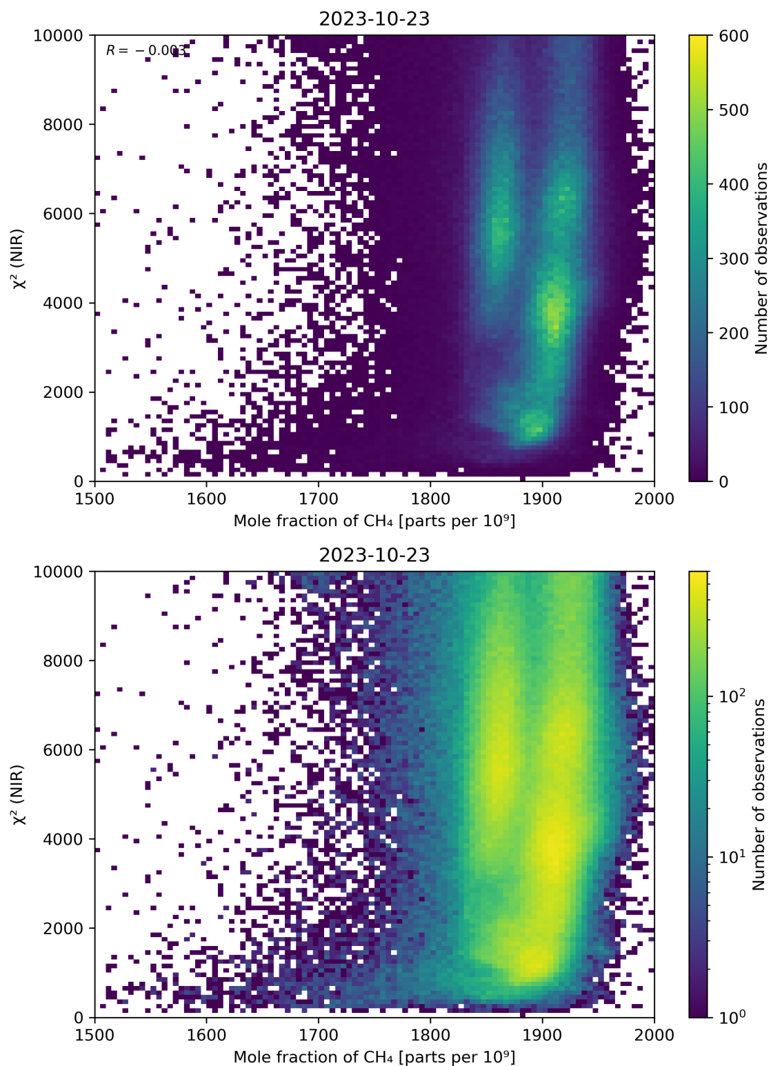
Figure 70: Scatter density plot of “Mole fraction of CH 4 ” against “ \chi^2 (NIR)” for 2023-10-22 to 2023-10-24.
