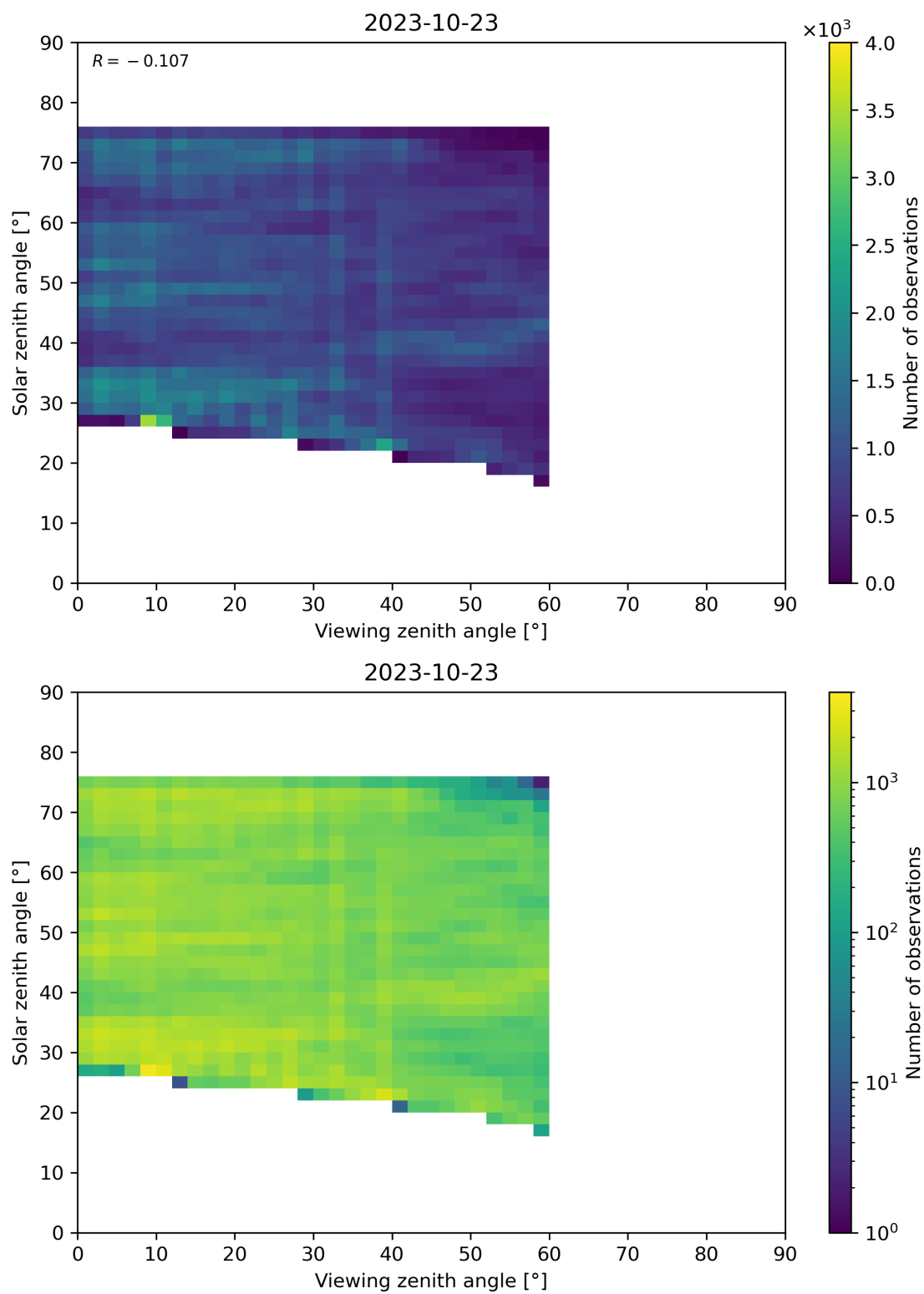
Figure 115: Scatter density plot of “Viewing zenith angle” against “Solar zenith angle” for 2023-10-22 to 2023-10-24.
