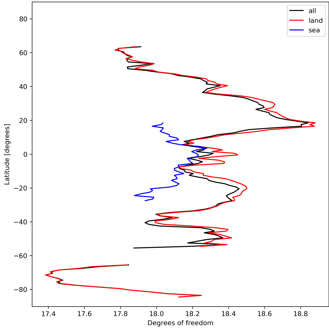
Figure 19: Zonal average of “Degrees of freedom” for 2023-10-22 to 2023-10-24.
