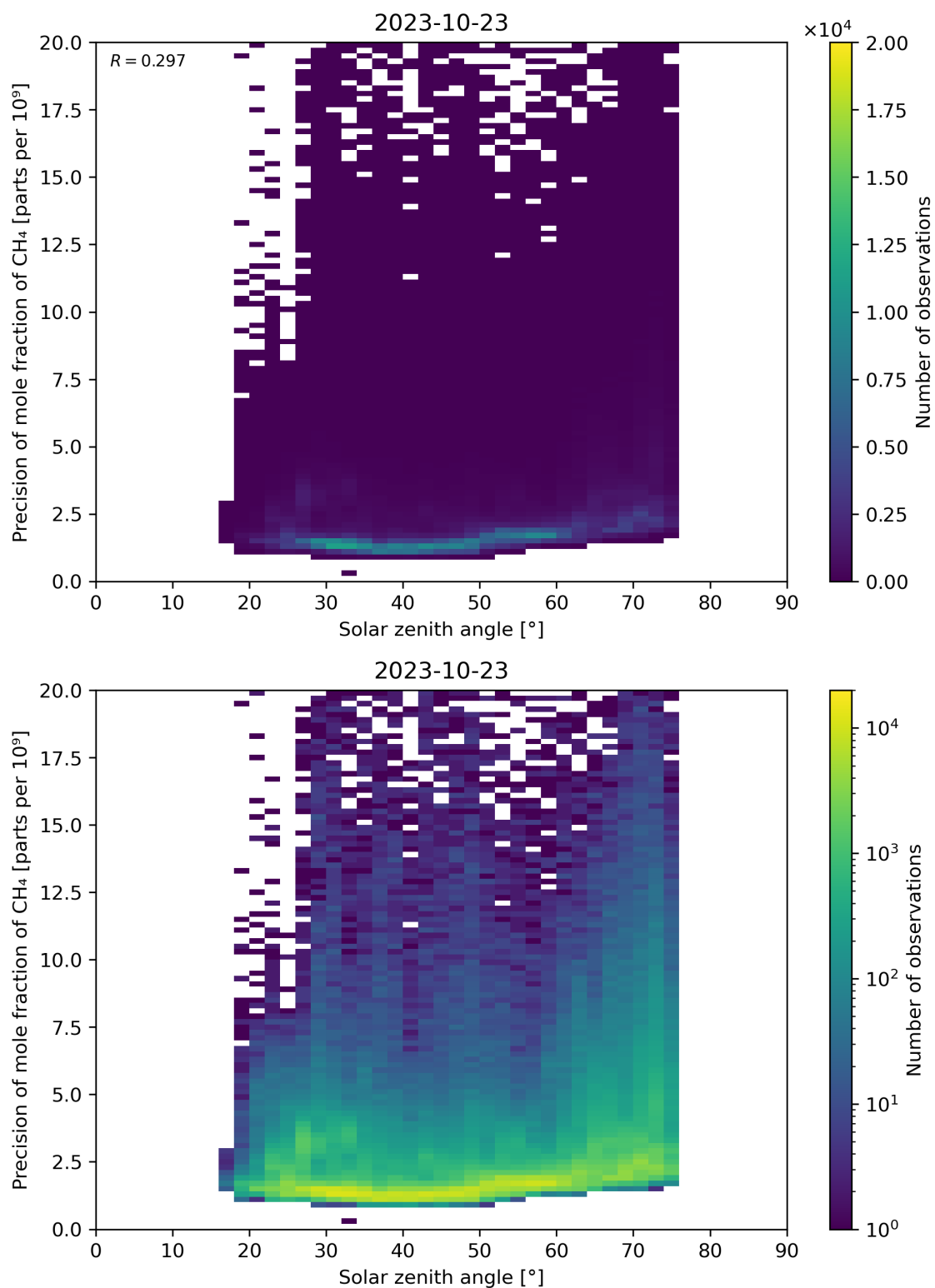
Figure 101: Scatter density plot of “Solar zenith angle” against “Precision of mole fraction of CH 4 ” for 2023-10-22 to 2023-10-24.
