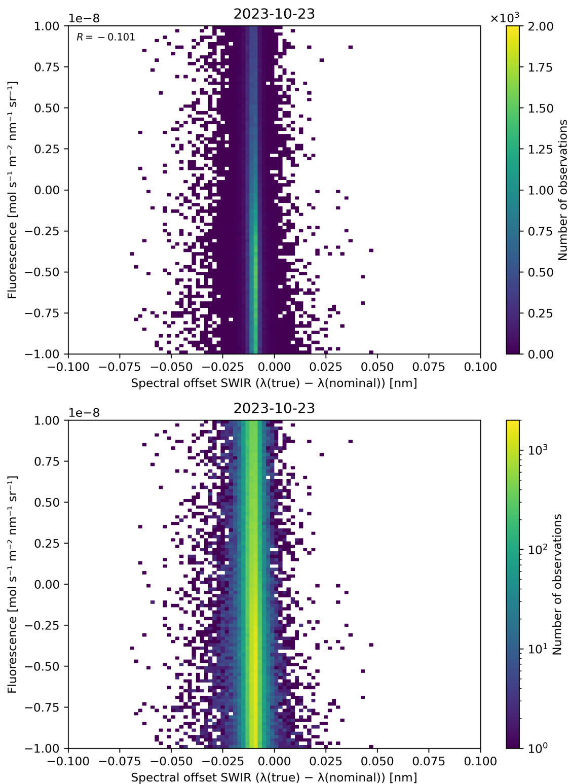
Figure 120: Scatter density plot of “Spectral offset SWIR ( \lambda(\text{true}) - \lambda(\text{nominal}) )” against “Fluorescence” for 2023-10-22 to 2023-10-24.
