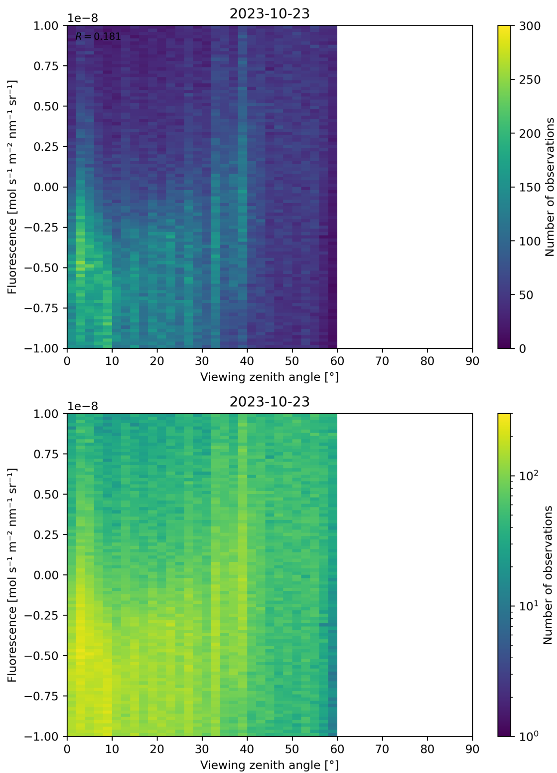
Figure 108: Scatter density plot of “Viewing zenith angle” against “Fluorescence” for 2023-10-22 to 2023-10-24.
