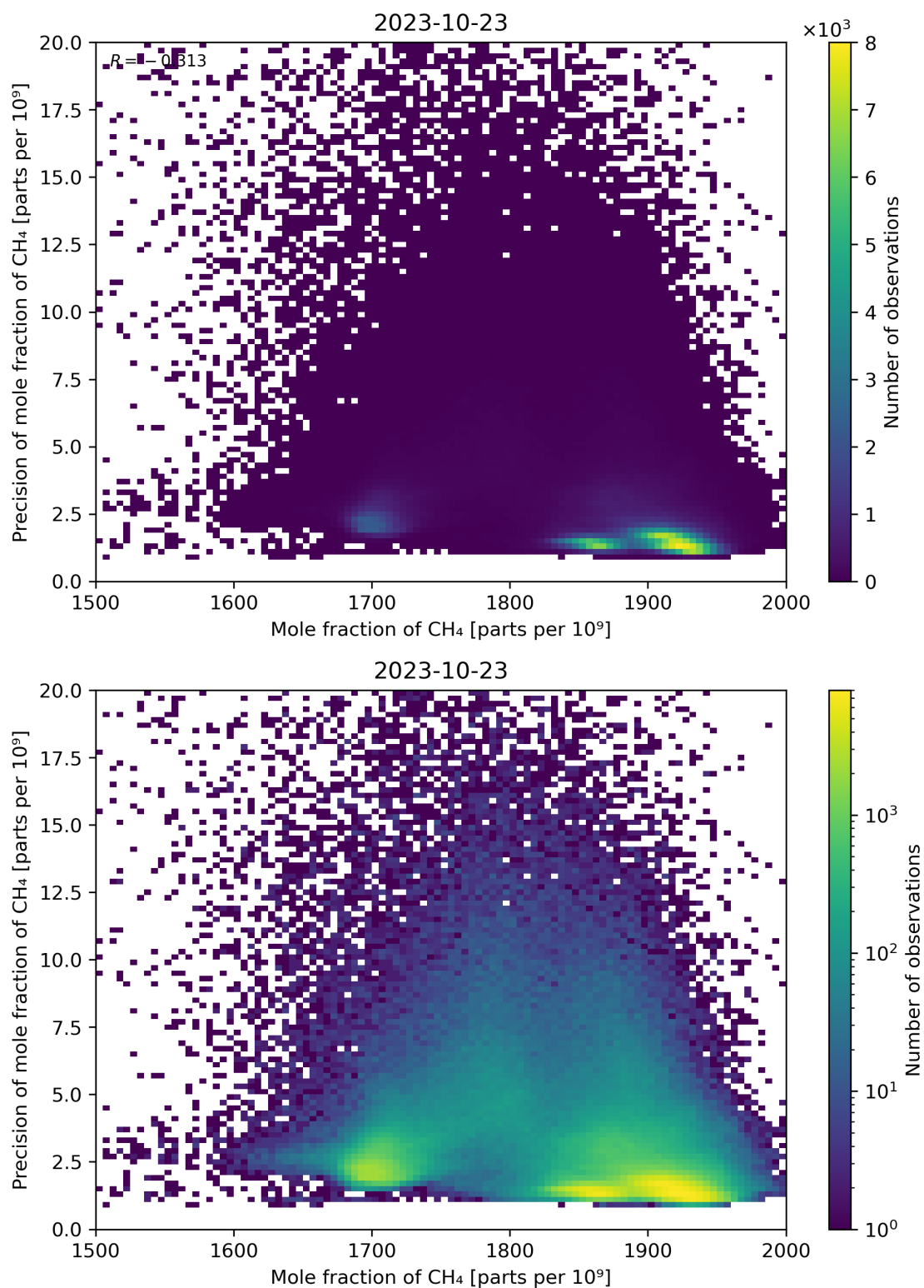
Figure 75: Scatter density plot of “Mole fraction of CH 4 ” against “Precision of mole fraction of CH 4 ” for 2023-10-22 to 2023-10-24.
