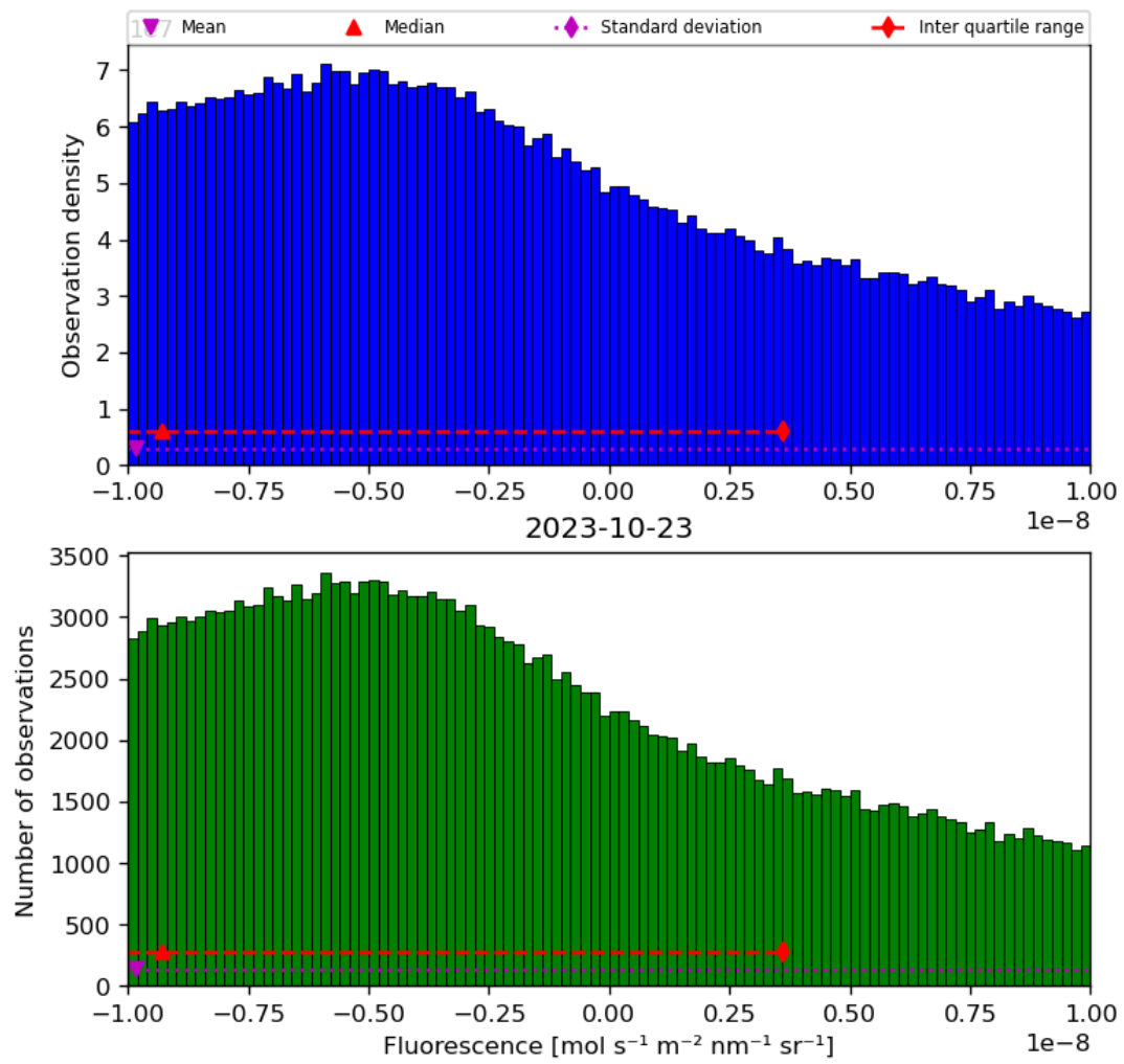
Figure 32: Histogram of “Fluorescence” for 2023-10-22 to 2023-10-24
