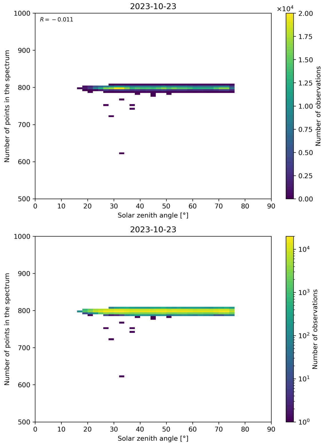
Figure 103: Scatter density plot of “Solar zenith angle” against “Number of points in the spectrum” for 2023-10-22 to 2023-10-24.
