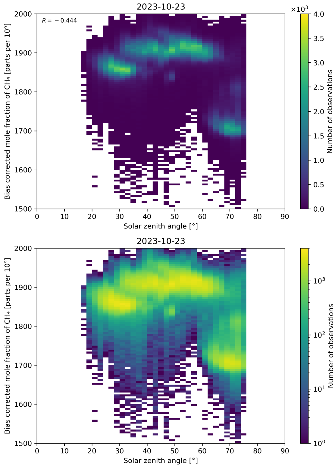
Figure 100: Scatter density plot of “Solar zenith angle” against “Bias corrected mole fraction of \text{CH}_4 ” for 2023-10-22 to 2023-10-24.
