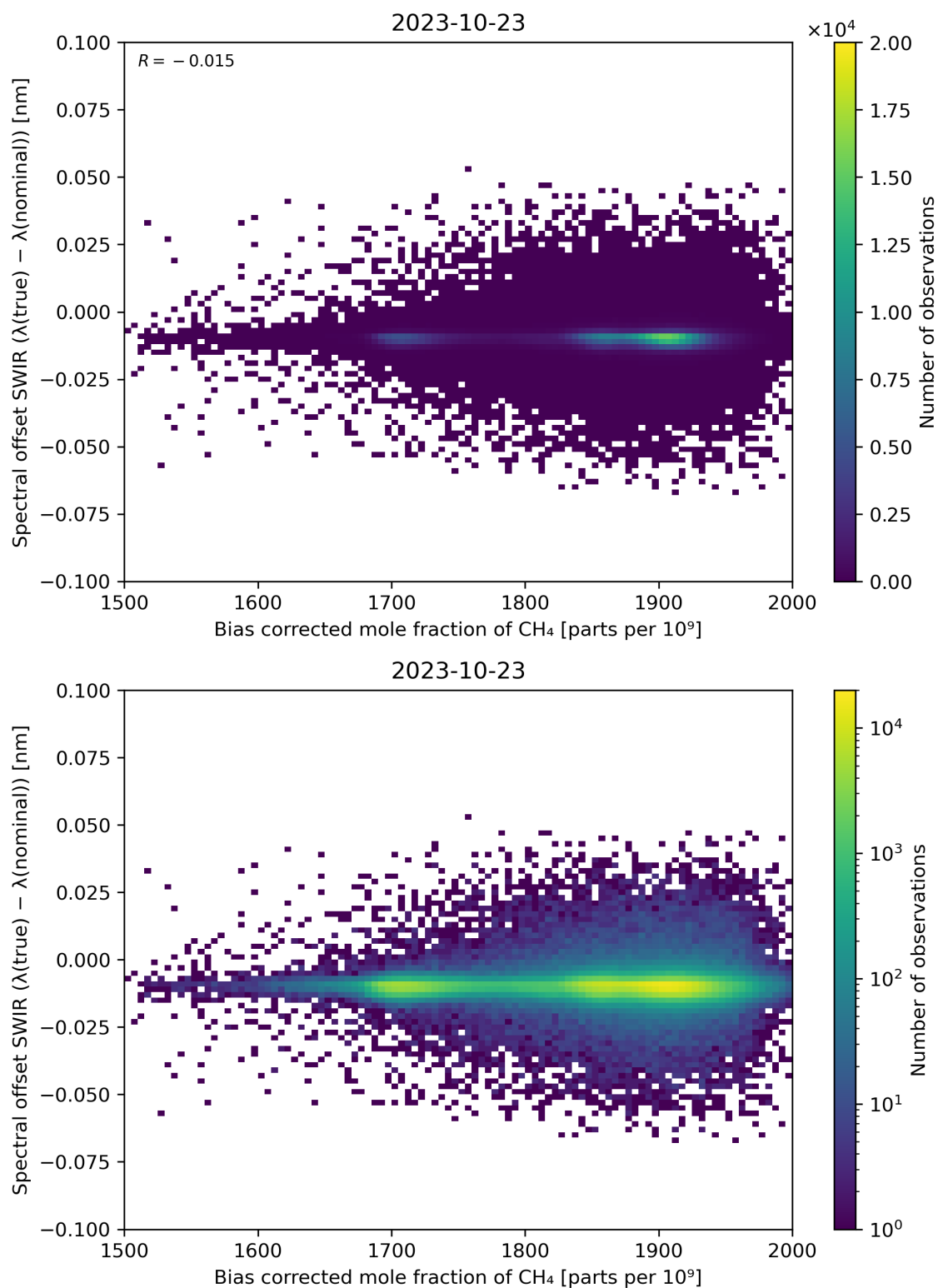
Figure 69: Scatter density plot of “Bias corrected mole fraction of \text{CH}_4 ” against “Spectral offset SWIR ( \lambda(\text{true}) - \lambda(\text{nominal}) )” for 2023-10-22 to 2023-10-24.
