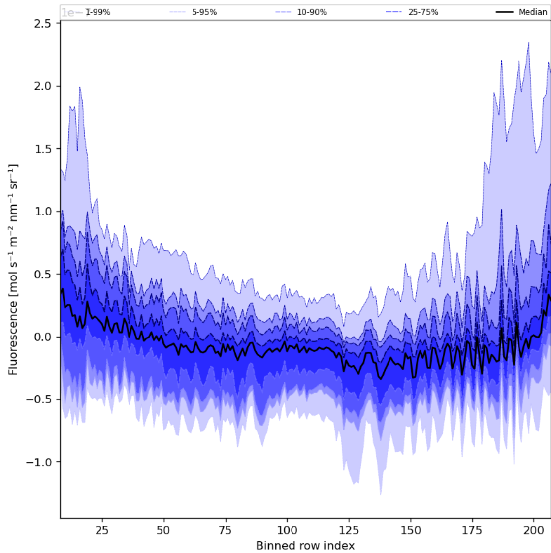
Figure 43: Along track statistics of “Fluorescence” for 2023-10-22 to 2023-10-24
