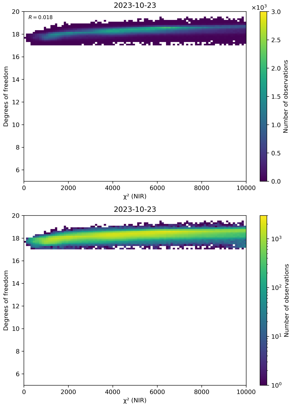
Figure 44: Scatter density plot of “ \chi^2 (NIR)” against “Degrees of freedom” for 2023-10-22 to 2023-10-24.
