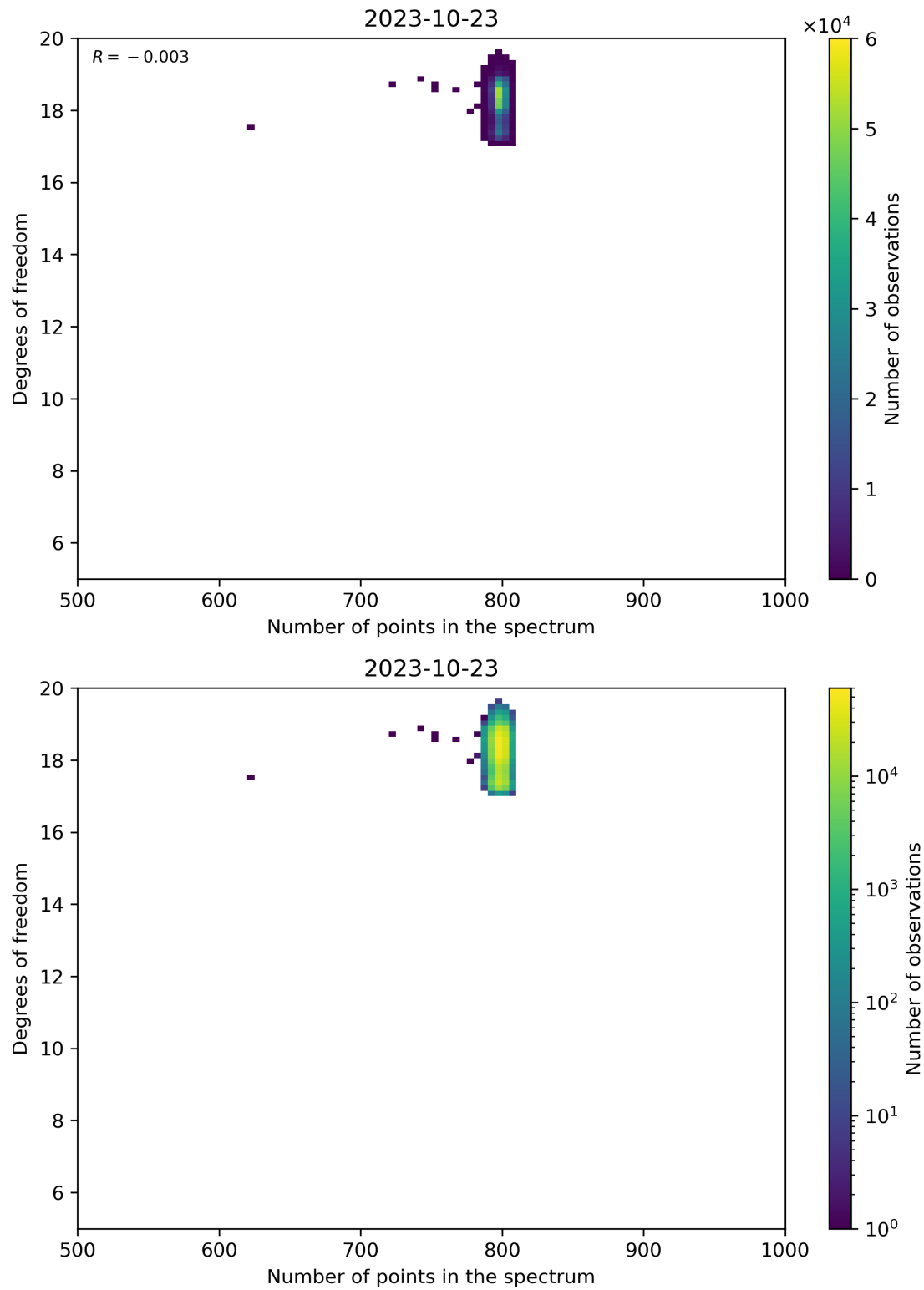
Figure 90: Scatter density plot of “Number of points in the spectrum” against “Degrees of freedom” for 2023-10-22 to 2023-10-24.
