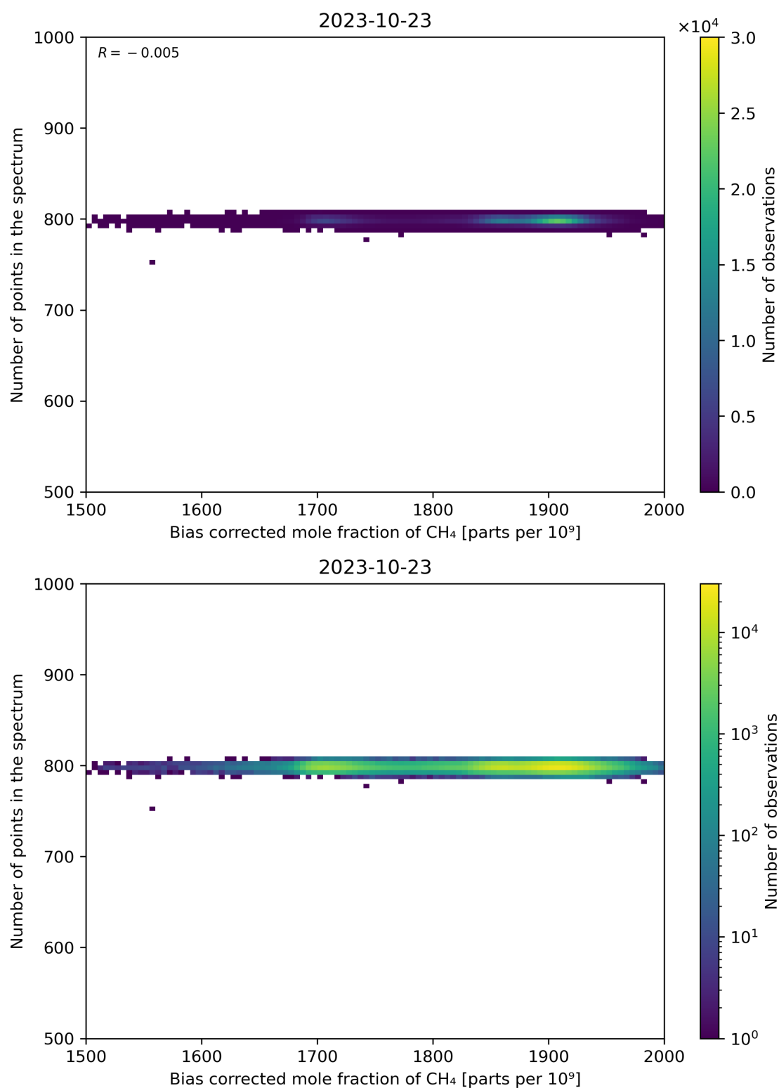
Figure 68: Scatter density plot of “Bias corrected mole fraction of CH 4 ” against “Number of points in the spectrum” for 2023-10-22 to 2023-10-24.
