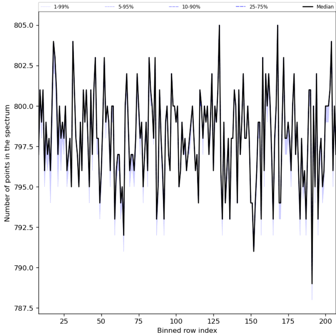
Figure 37: Along track statistics of “Number of points in the spectrum” for 2023-10-22 to 2023-10-24
