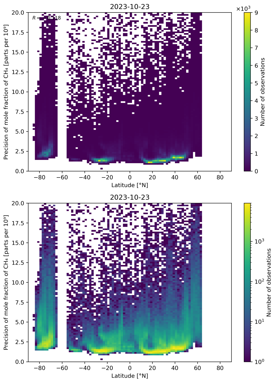
Figure 59: Scatter density plot of “Latitude” against “Precision of mole fraction of CH 4 ” for 2023-10-22 to 2023-10-24.
