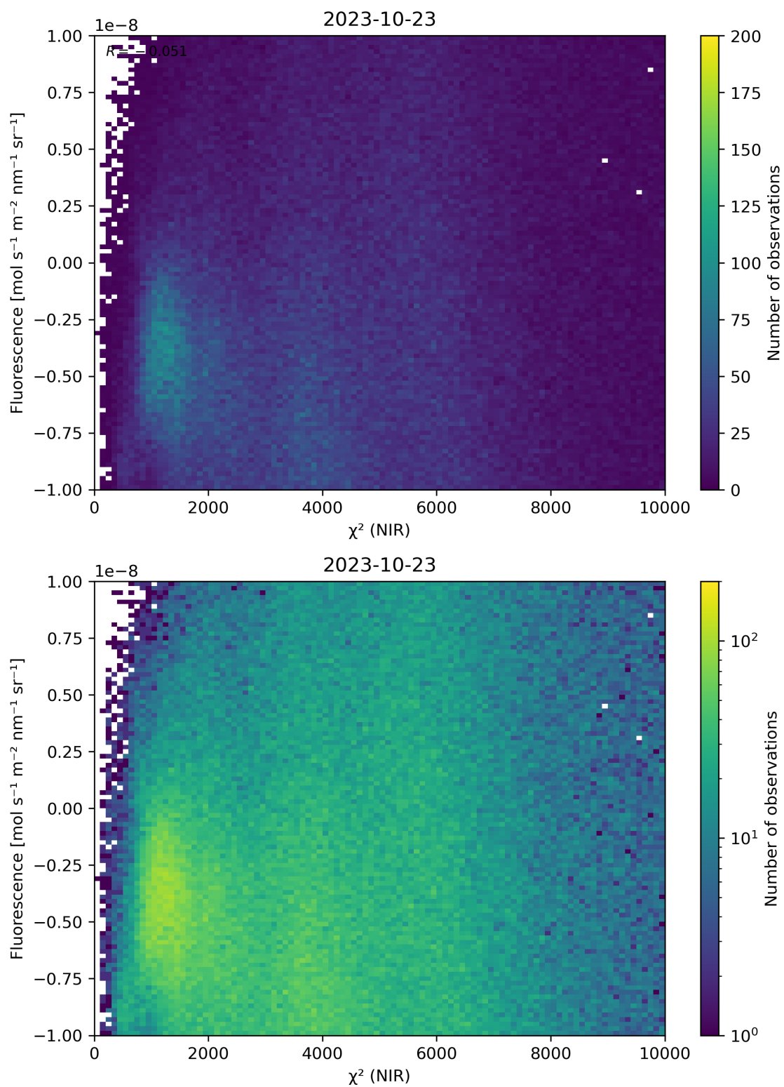
Figure 45: Scatter density plot of “ \chi^2 (NIR)” against “Fluorescence” for 2023-10-22 to 2023-10-24.
