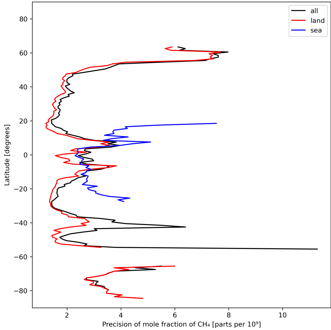
Figure 13: Zonal average of “Precision of mole fraction of CH 4 ” for 2023-10-22 to 2023-10-24.
