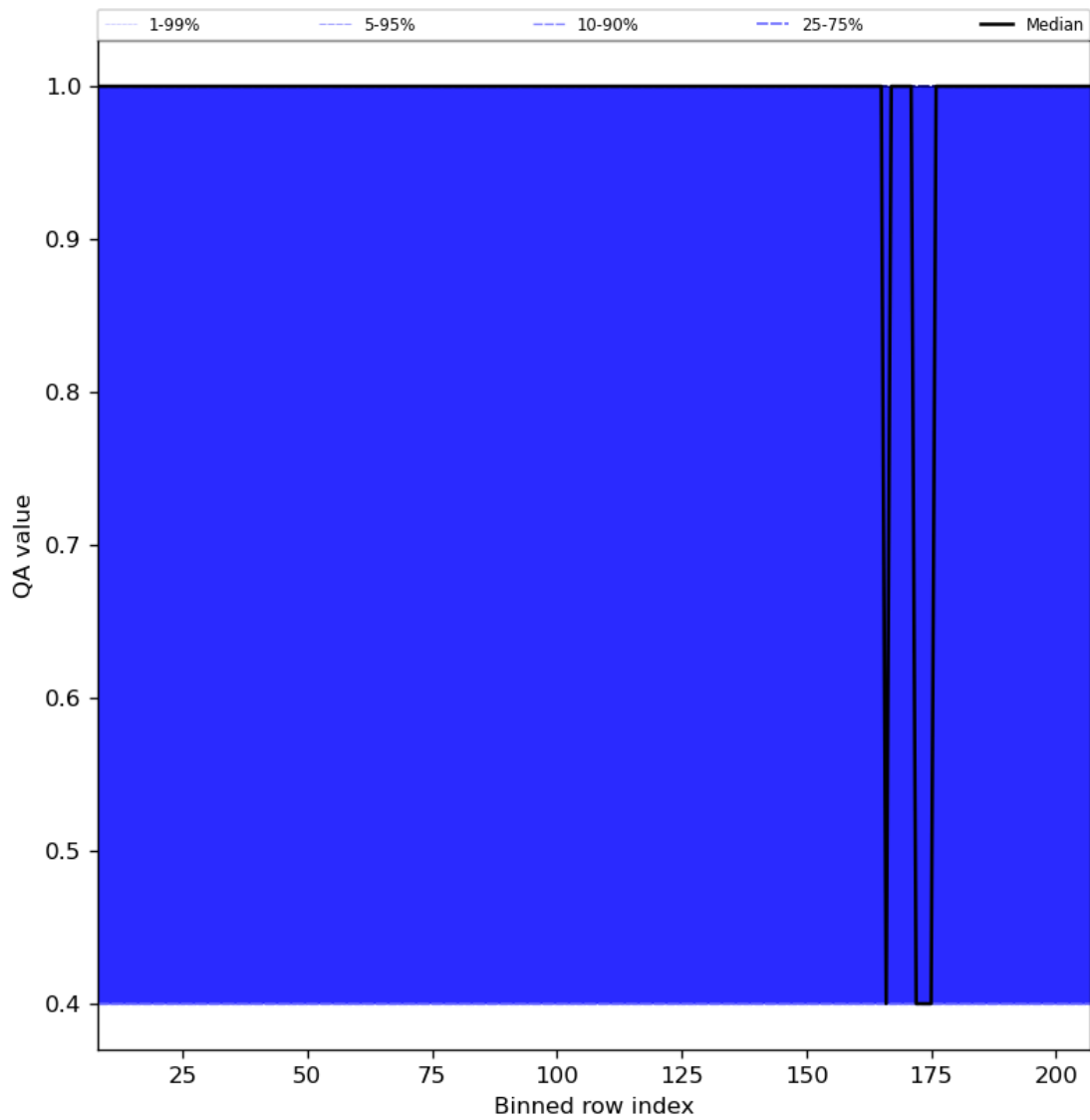
Figure 33: Along track statistics of “QA value” for 2023-10-22 to 2023-10-24
