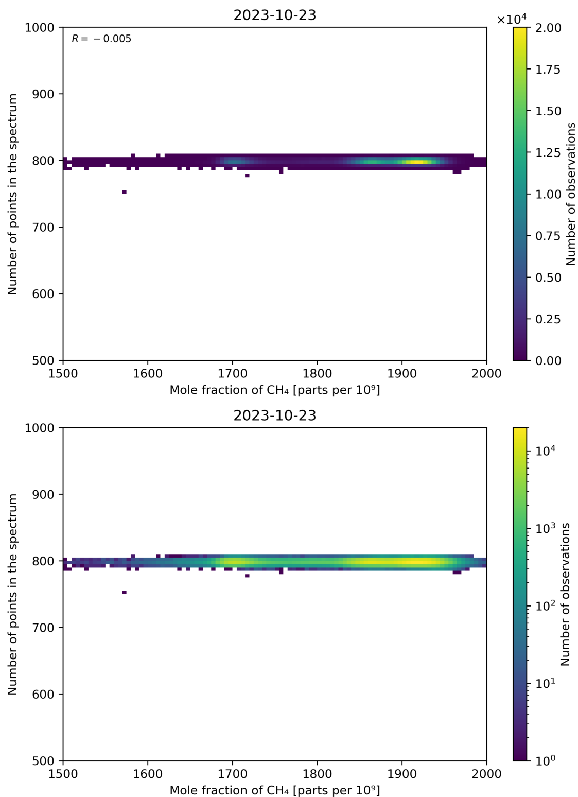
Figure 77: Scatter density plot of “Mole fraction of CH 4 ” against “Number of points in the spectrum” for 2023-10-22 to 2023-10-24.
