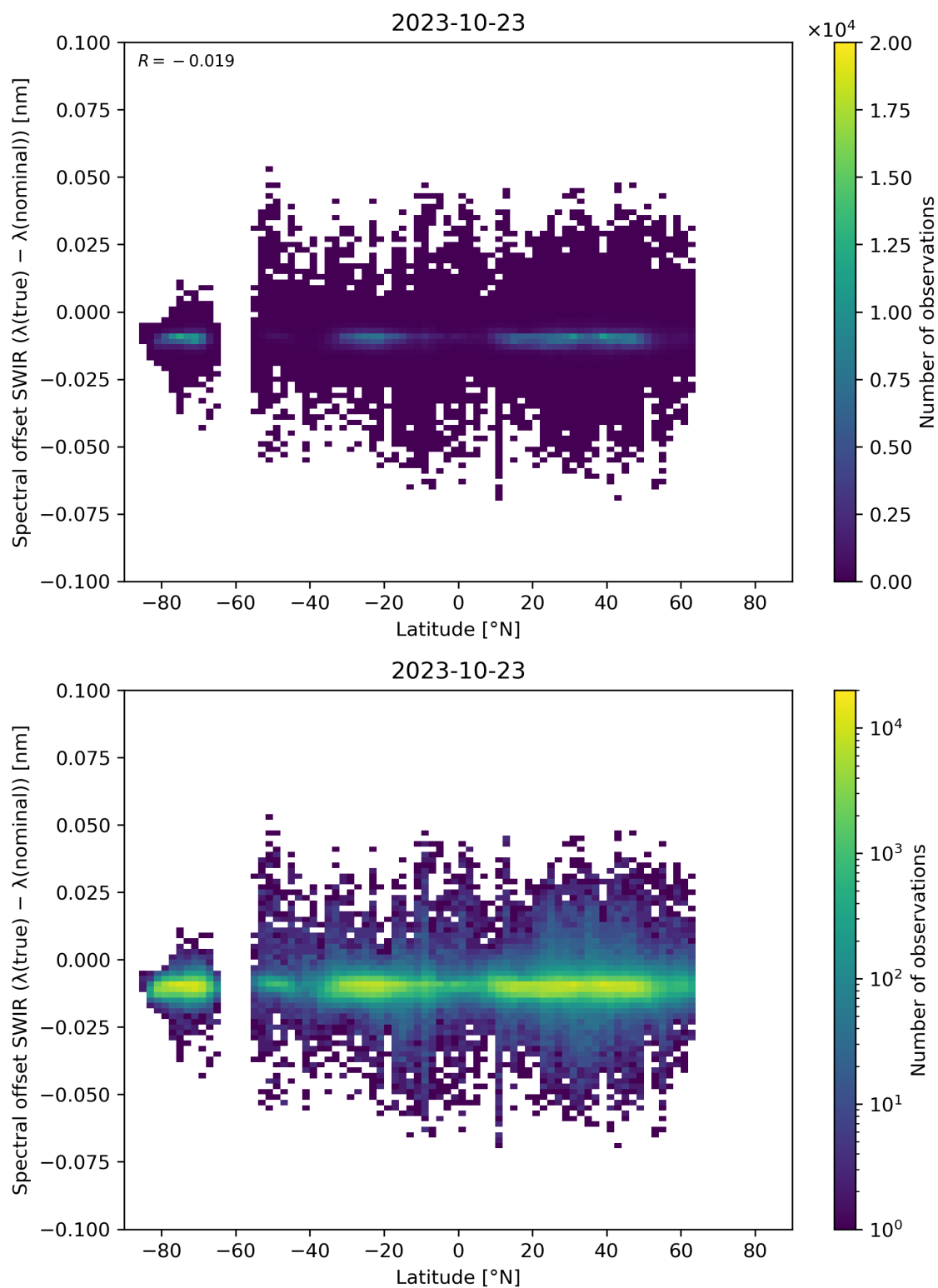
Figure 62: Scatter density plot of “Latitude” against “Spectral offset SWIR ( \lambda(\text{true}) - \lambda(\text{nominal}) )” for 2023-10-22 to 2023-10-24.
