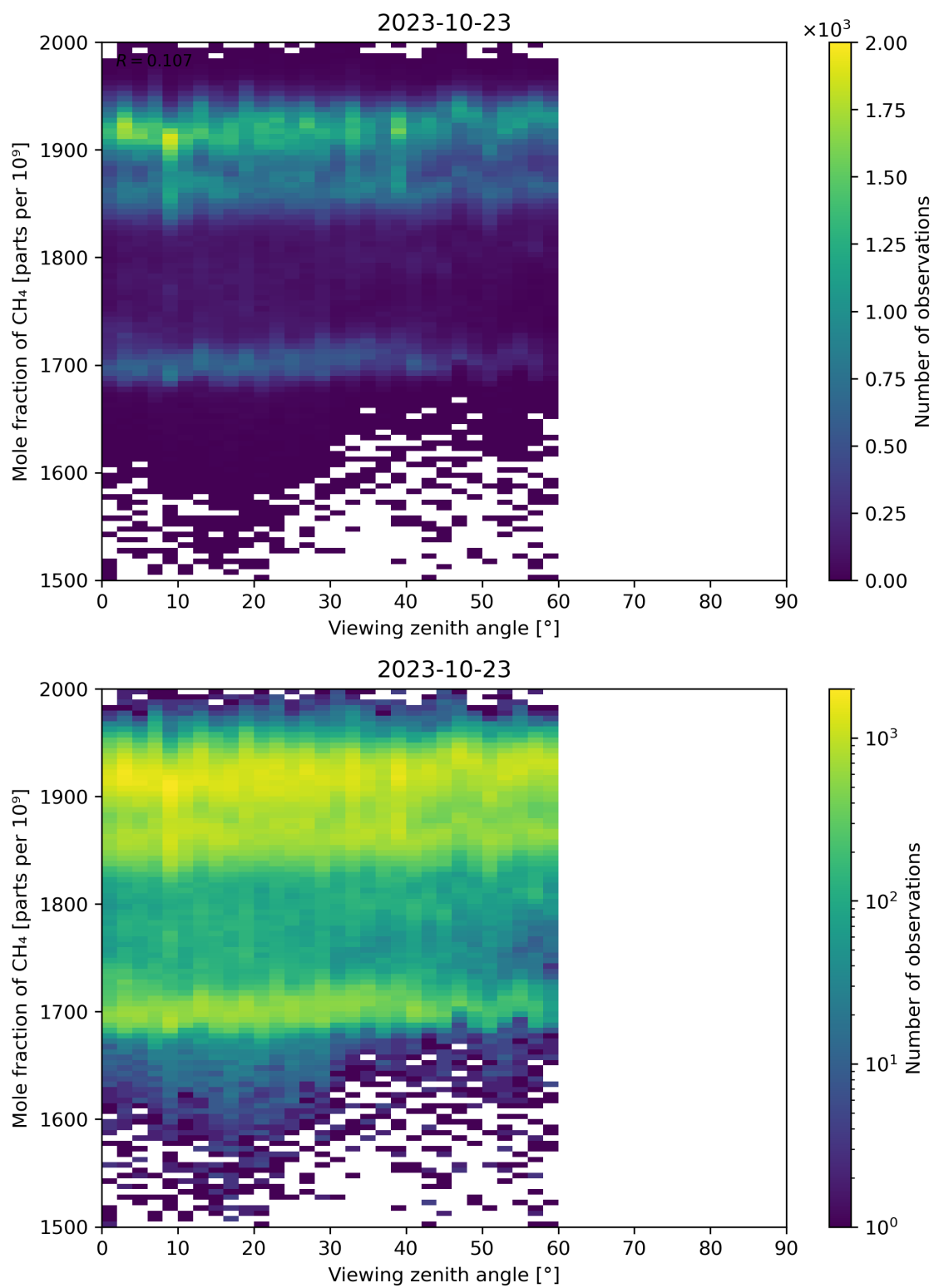
Figure 110: Scatter density plot of “Viewing zenith angle” against “Mole fraction of CH 4 ” for 2023-10-22 to 2023-10-24.
