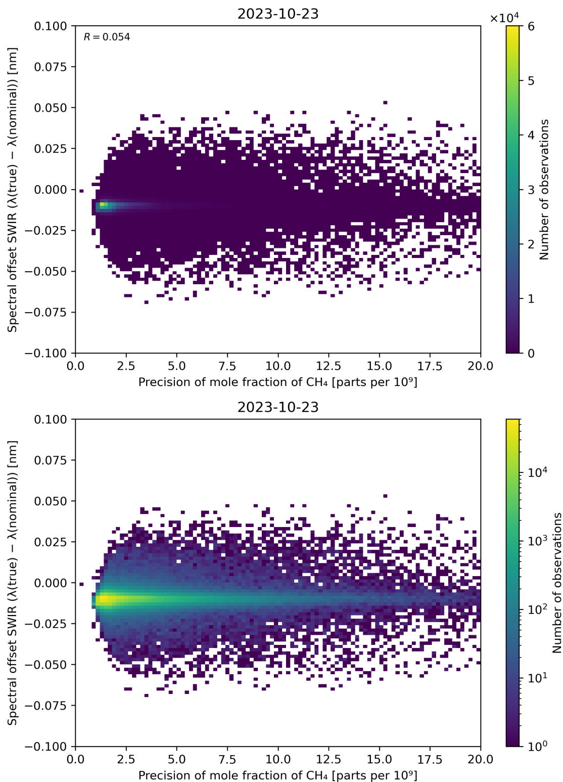
Figure 85: Scatter density plot of “Precision of mole fraction of \text{CH}_4 ” against “Spectral offset SWIR ( \lambda(\text{true}) - \lambda(\text{nominal}) )” for 2023-10-22 to 2023-10-24.
