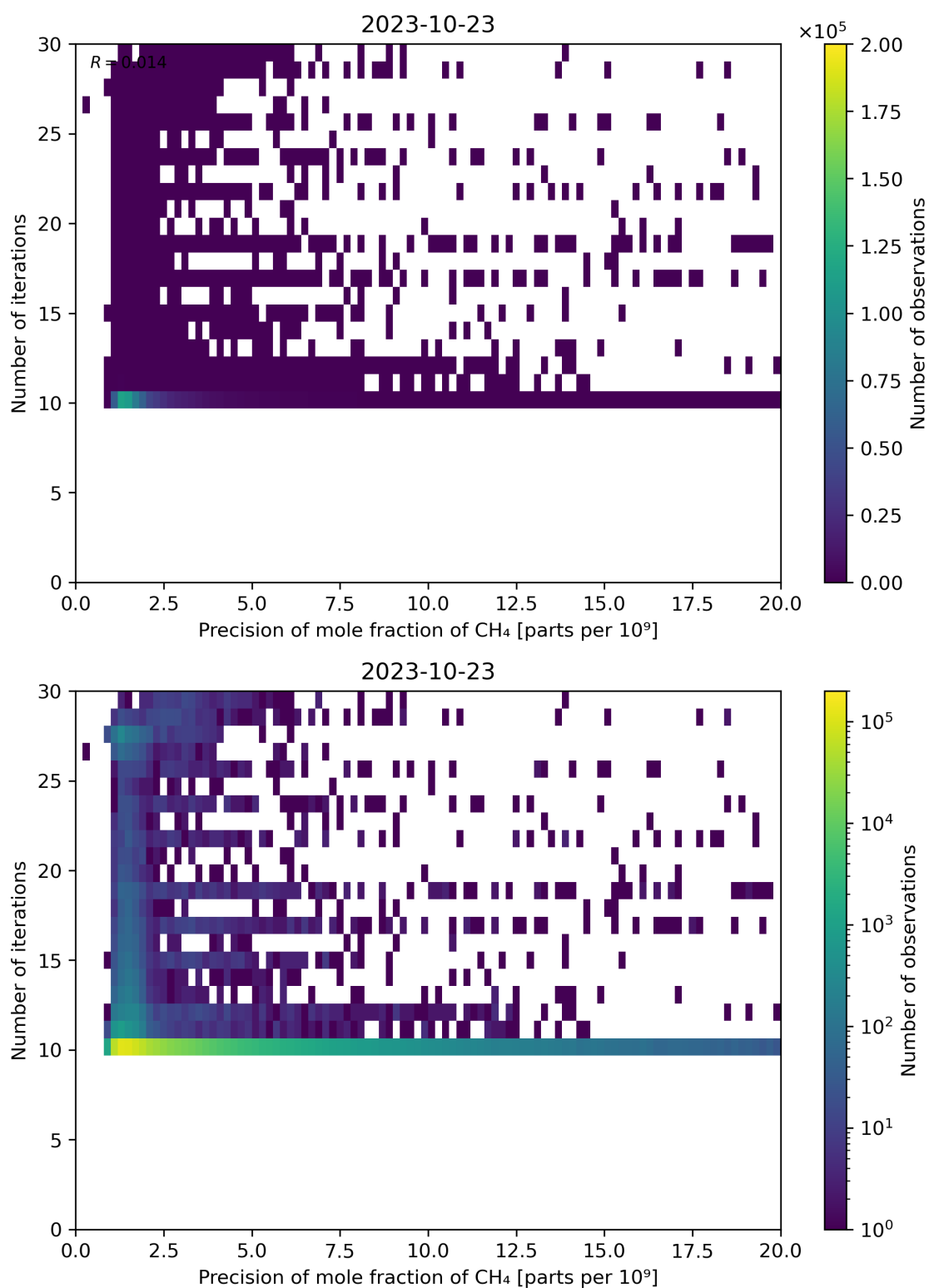
Figure 83: Scatter density plot of “Precision of mole fraction of CH 4 ” against “Number of iterations” for 2023-10-22 to 2023-10-24.
