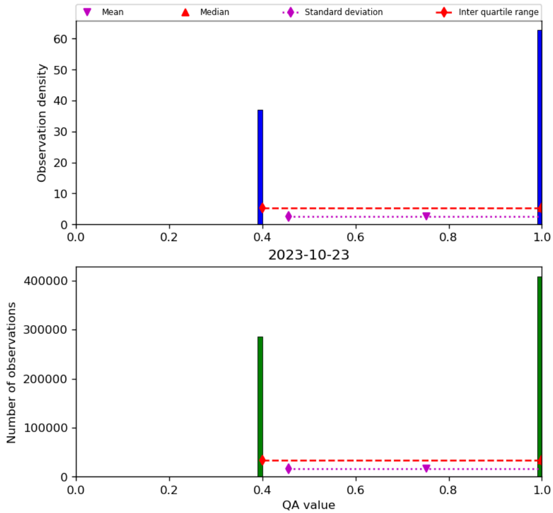
Figure 22: Histogram of “QA value” for 2023-10-22 to 2023-10-24
