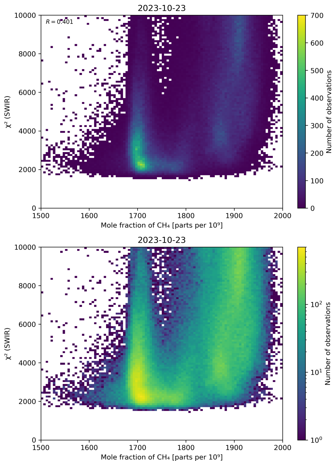
Figure 71: Scatter density plot of “Mole fraction of CH 4 ” against “ \chi^2 (SWIR)” for 2023-10-22 to 2023-10-24.
