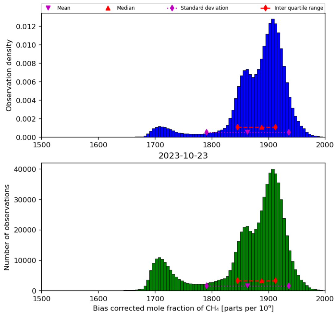
Figure 25: Histogram of “Bias corrected mole fraction of CH 4 ” for 2023-10-22 to 2023-10-24
