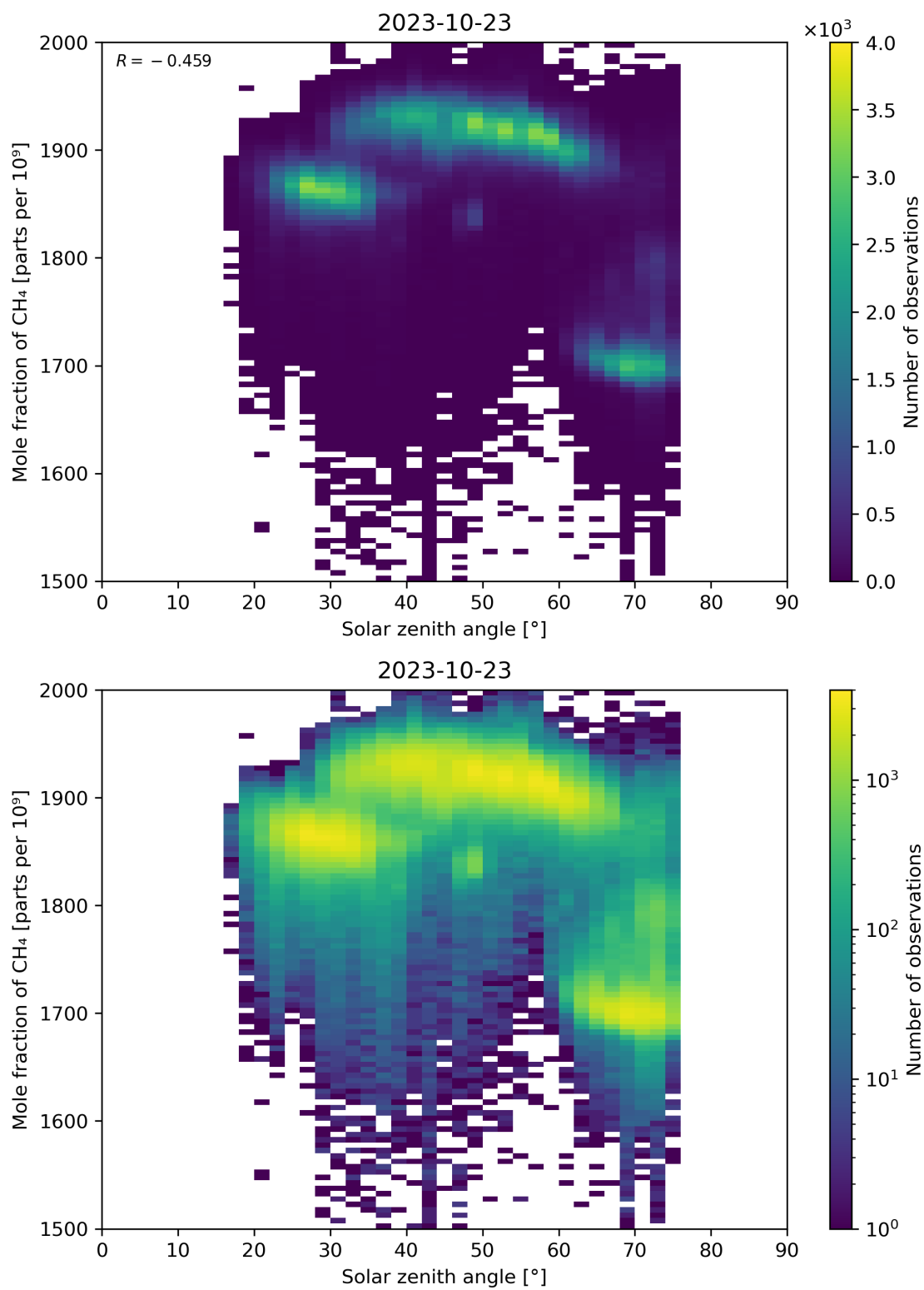
Figure 99: Scatter density plot of “Solar zenith angle” against “Mole fraction of \text{CH}_4 ” for 2023-10-22 to 2023-10-24.
