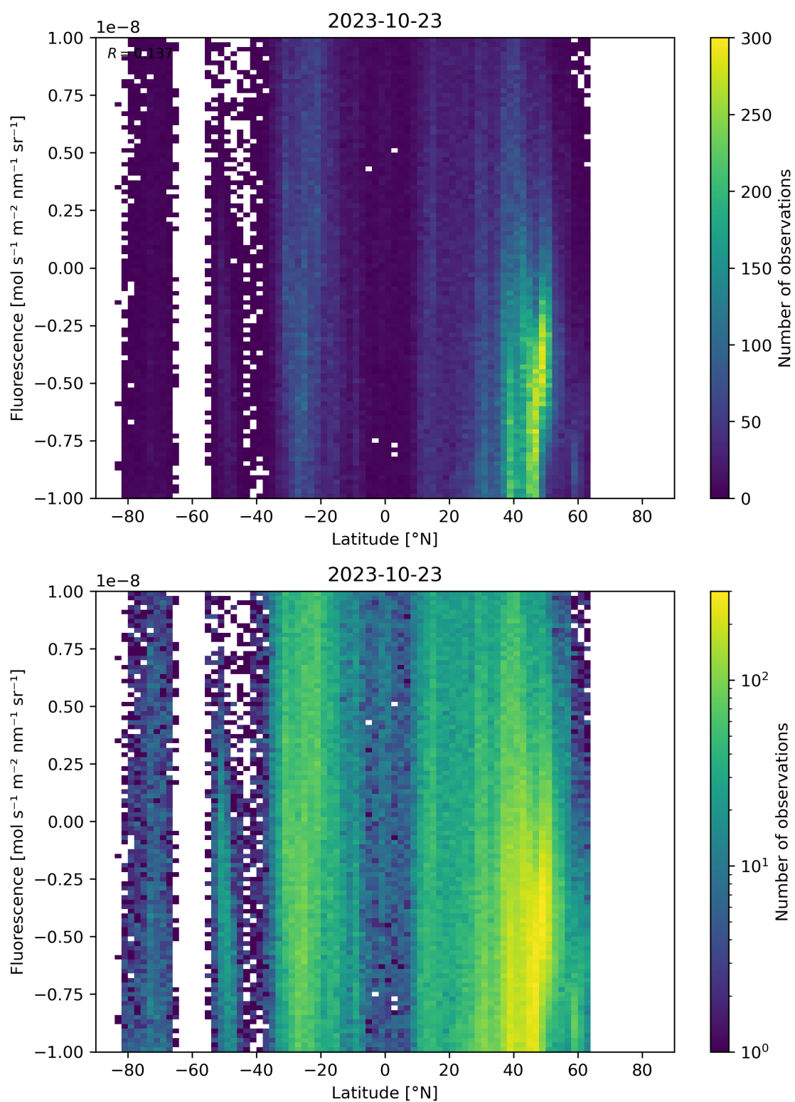
Figure 56: Scatter density plot of “Latitude” against “Fluorescence” for 2023-10-22 to 2023-10-24.
