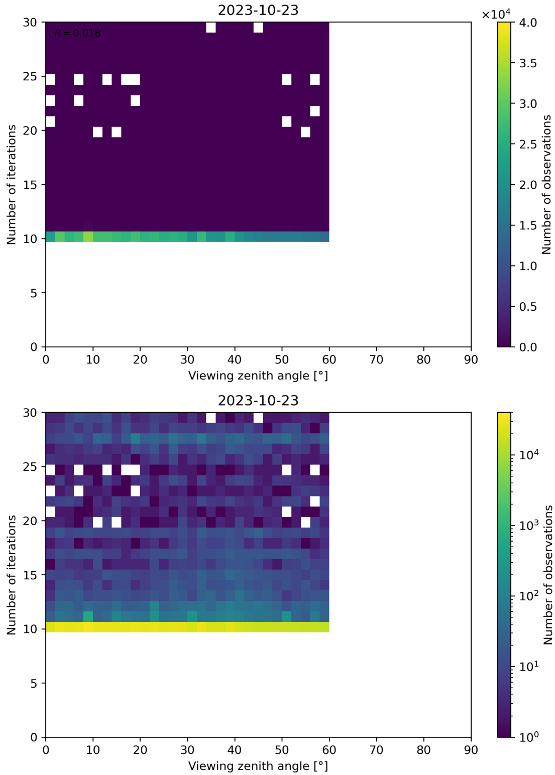
Figure 113: Scatter density plot of “Viewing zenith angle” against “Number of iterations” for 2023-10-22 to 2023-10-24.
