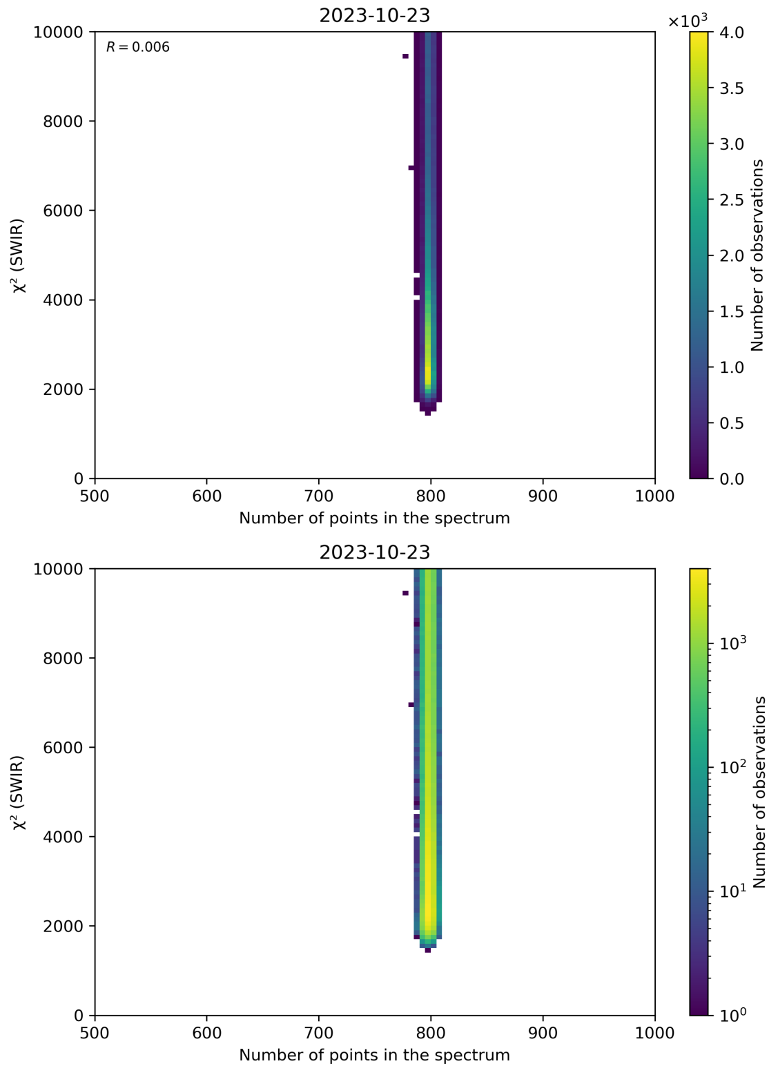
Figure 89: Scatter density plot of “Number of points in the spectrum” against “ \chi^2 (SWIR)” for 2023-10-22 to 2023-10-24.
