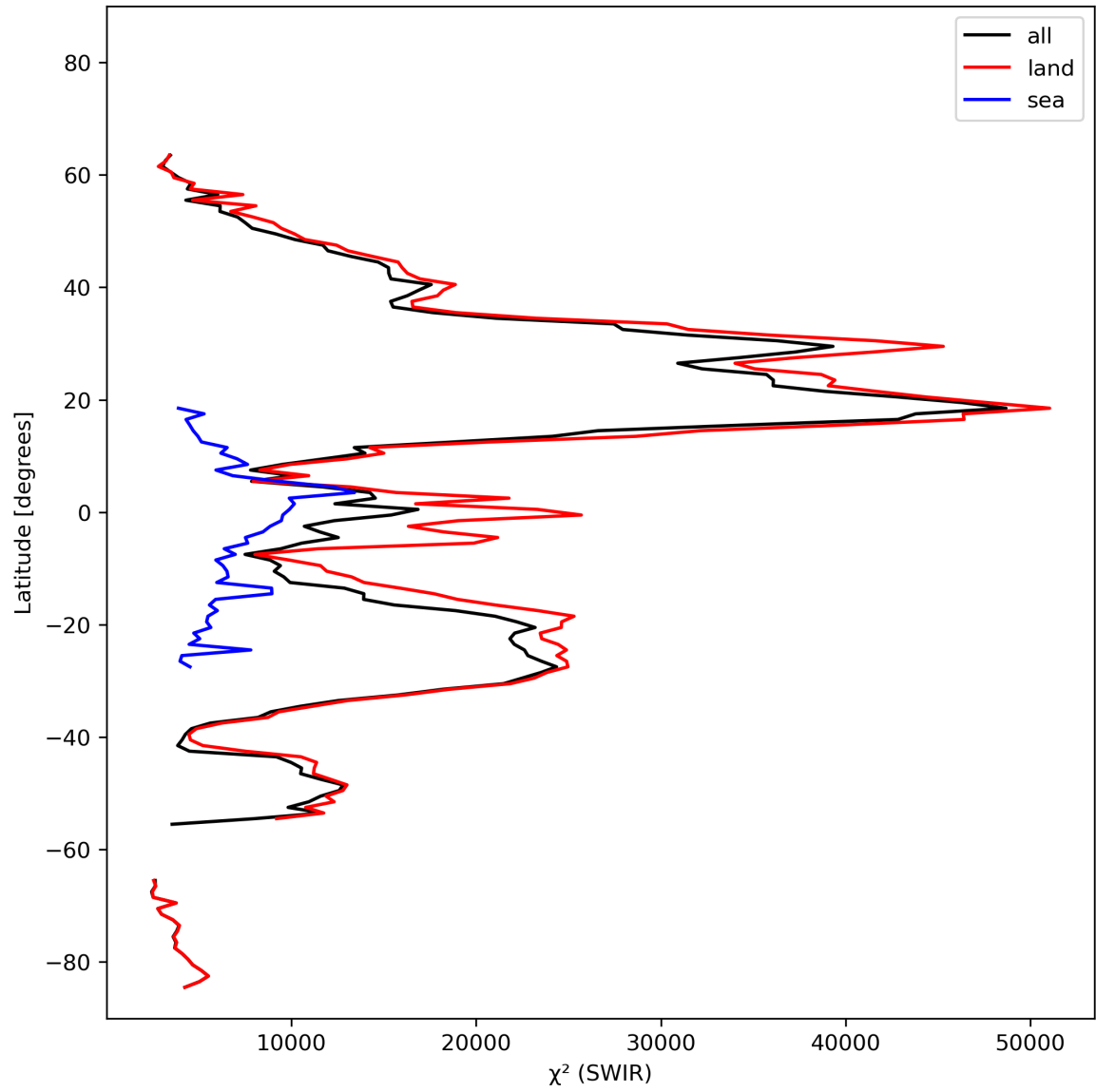
Figure 17: Zonal average of “ \chi^2 (SWIR)” for 2023-10-22 to 2023-10-24.
