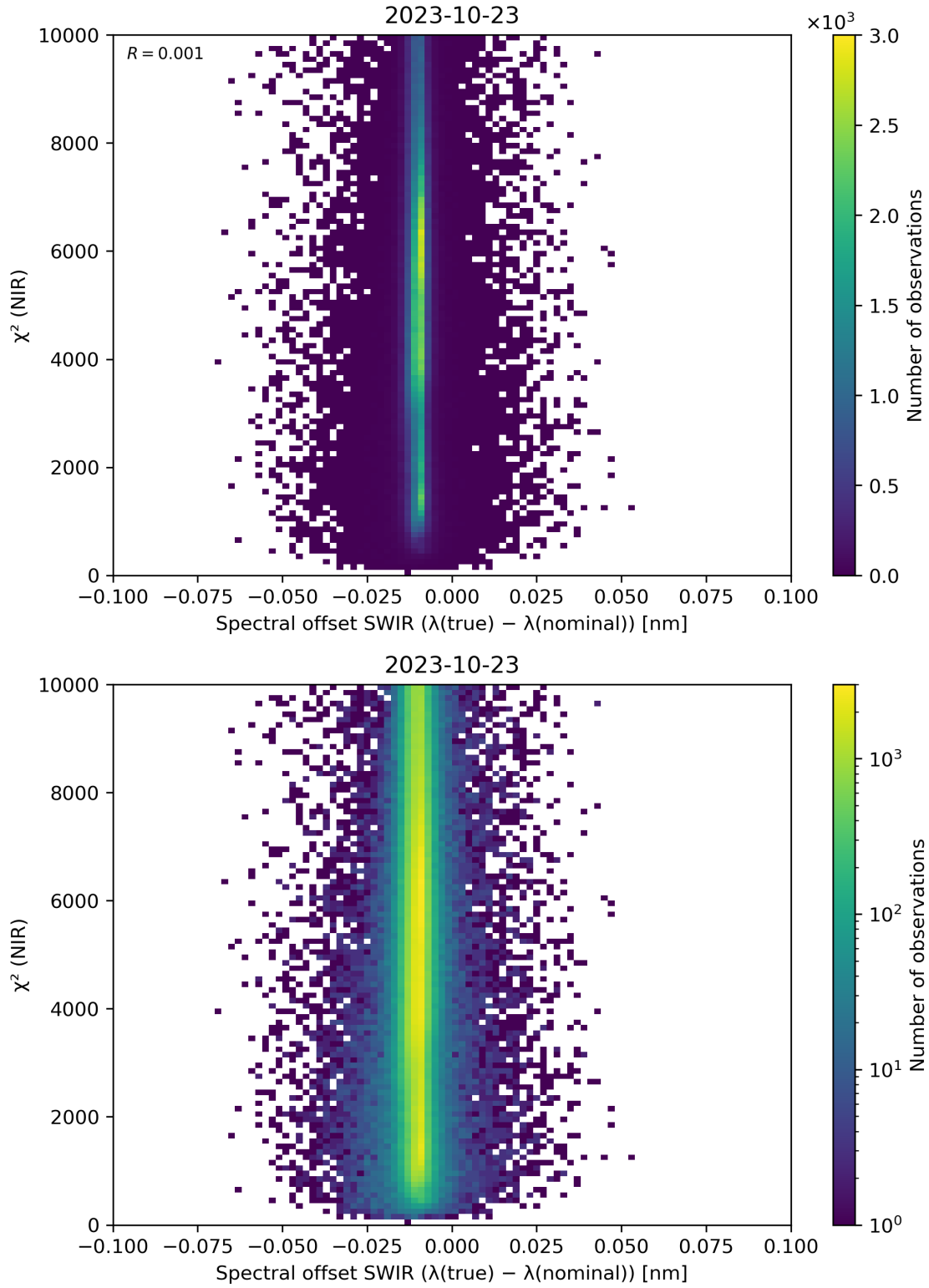
Figure 117: Scatter density plot of “Spectral offset SWIR ( \lambda(\text{true}) - \lambda(\text{nominal}) )” against “ \chi^2 (NIR)” for 2023-10-22 to 2023-10-24.
