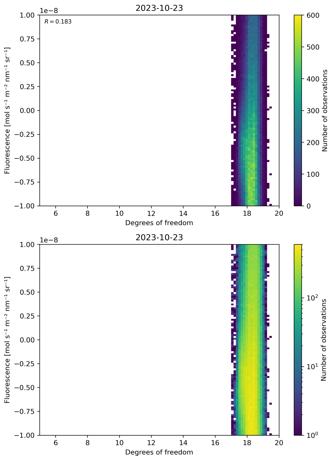
Figure 51: Scatter density plot of “Degrees of freedom” against “Fluorescence” for 2023-10-22 to 2023-10-24.
