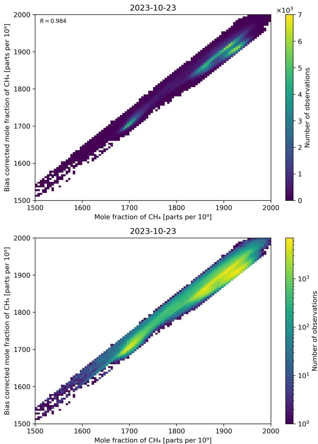
Figure 74: Scatter density plot of “Mole fraction of CH 4 ” against “Bias corrected mole fraction of CH 4 ” for 2023-10-22 to 2023-10-24.
