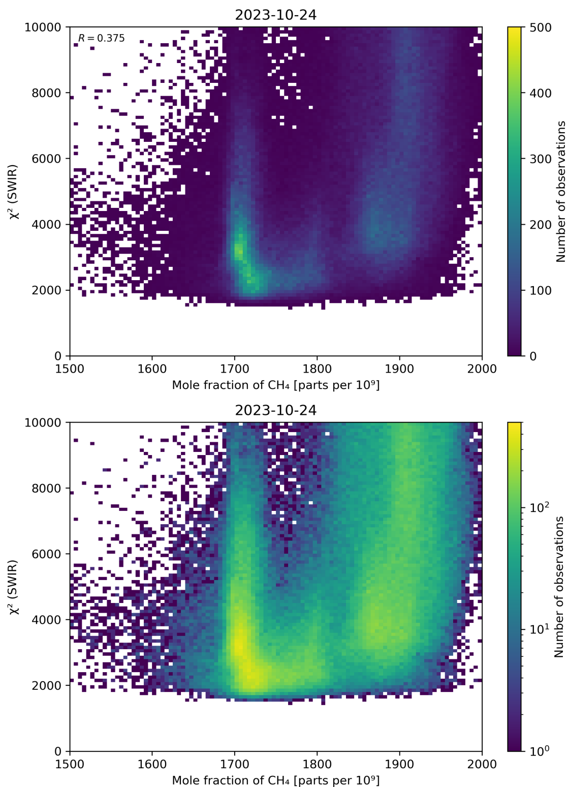
Figure 71: Scatter density plot of “Mole fraction of \text{CH}_4 ” against “ \chi^2 (SWIR)” for 2023-10-23 to 2023-10-25.
