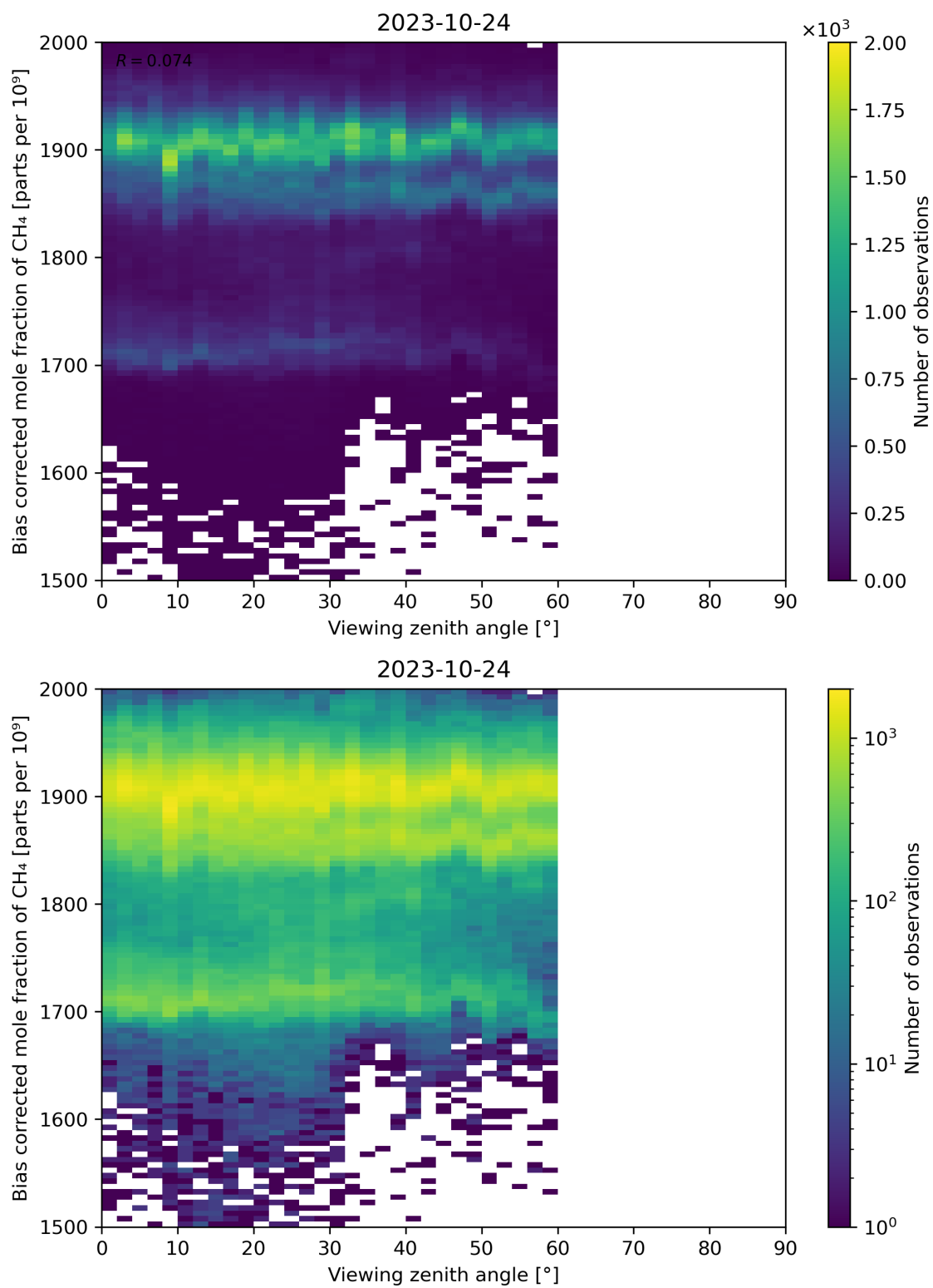
Figure 111: Scatter density plot of “Viewing zenith angle” against “Bias corrected mole fraction of CH 4 ” for 2023-10-23 to 2023-10-25.
