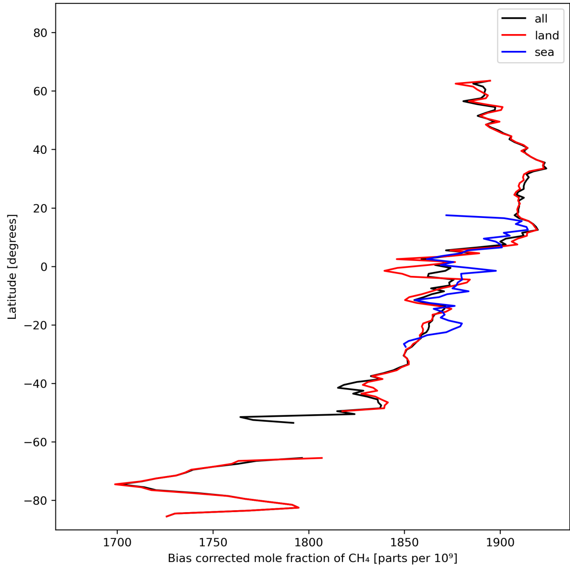
Figure 14: Zonal average of “Bias corrected mole fraction of CH 4 ” for 2023-10-23 to 2023-10-25.
