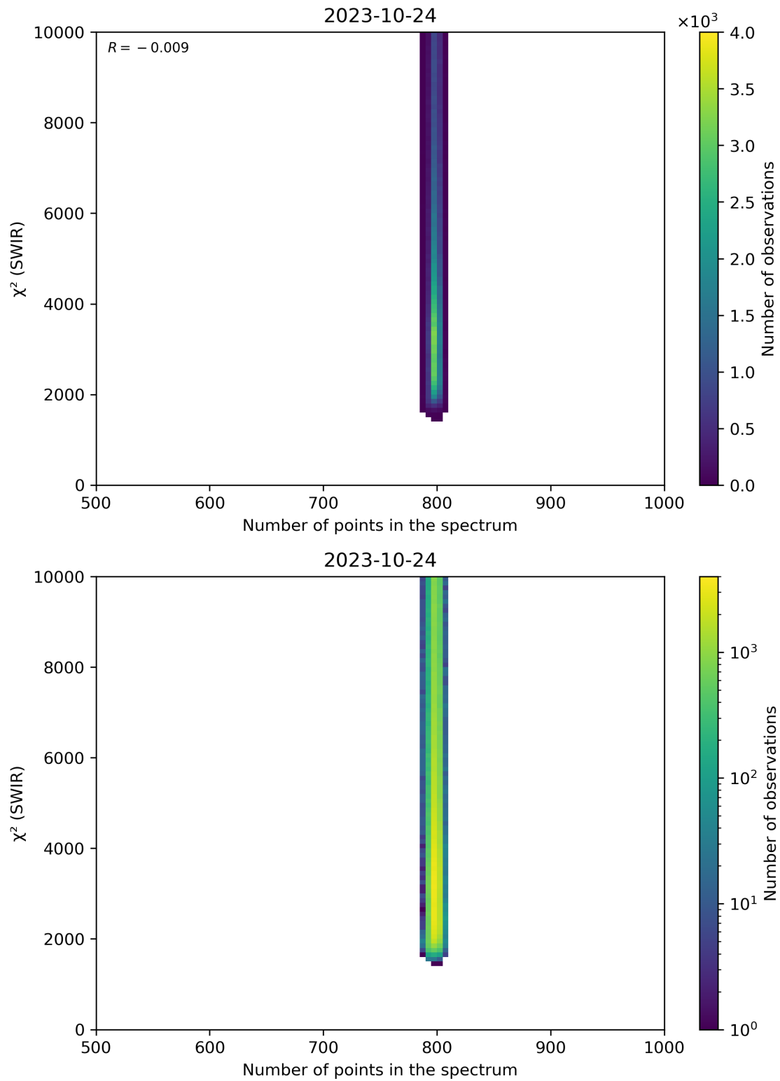
Figure 89: Scatter density plot of “Number of points in the spectrum” against “ \chi^2 (SWIR)” for 2023-10-23 to 2023-10-25.
