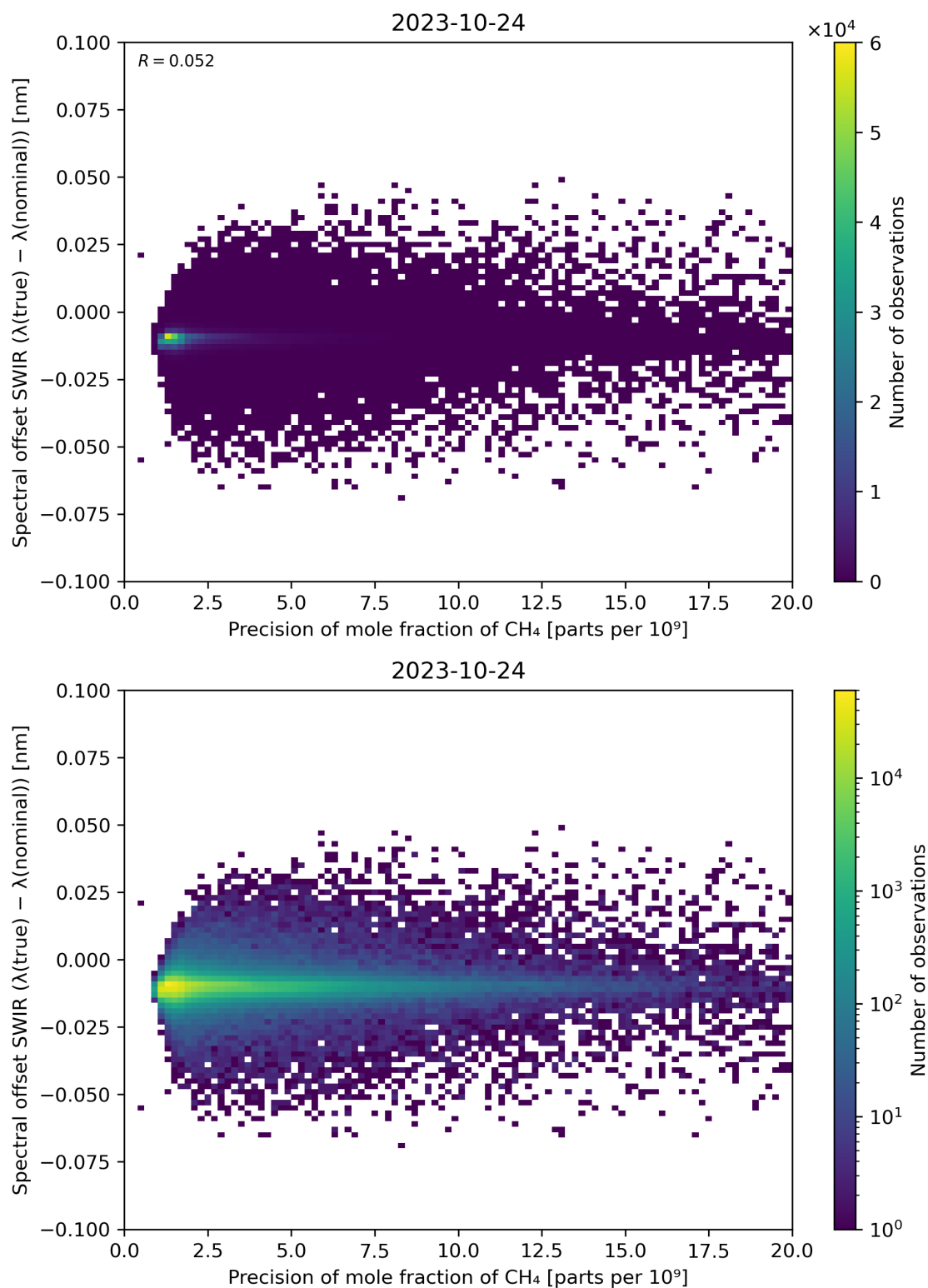
Figure 85: Scatter density plot of “Precision of mole fraction of \text{CH}_4 ” against “Spectral offset SWIR ( \lambda(\text{true}) - \lambda(\text{nominal}) )” for 2023-10-23 to 2023-10-25.
