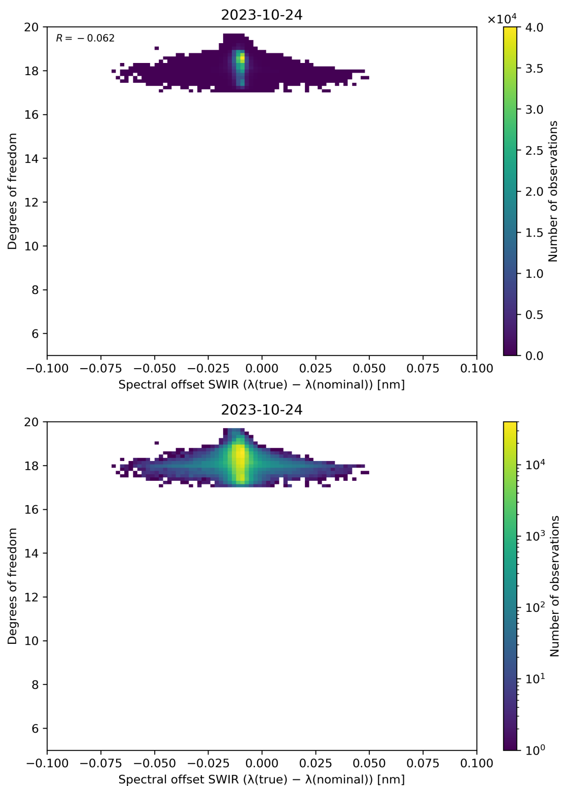
Figure 119: Scatter density plot of “Spectral offset SWIR ( \lambda(\text{true}) - \lambda(\text{nominal}) )” against “Degrees of freedom” for 2023-10-23 to 2023-10-25.
