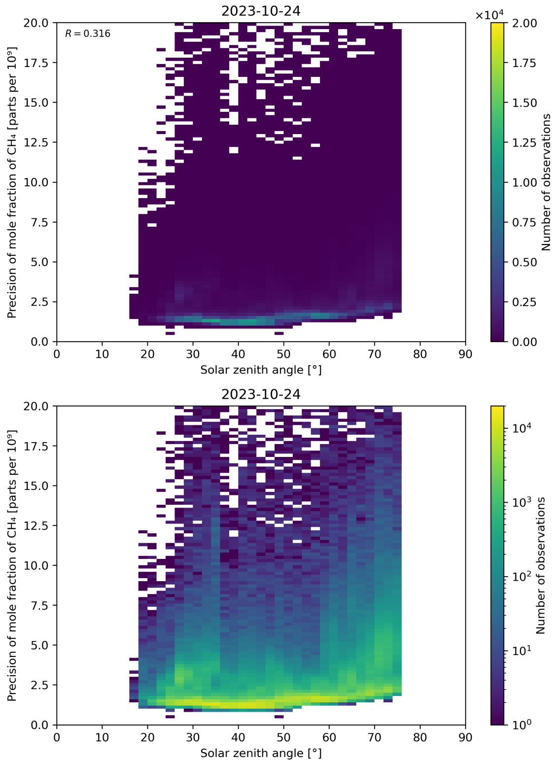
Figure 101: Scatter density plot of “Solar zenith angle” against “Precision of mole fraction of CH 4 ” for 2023-10-23 to 2023-10-25.
