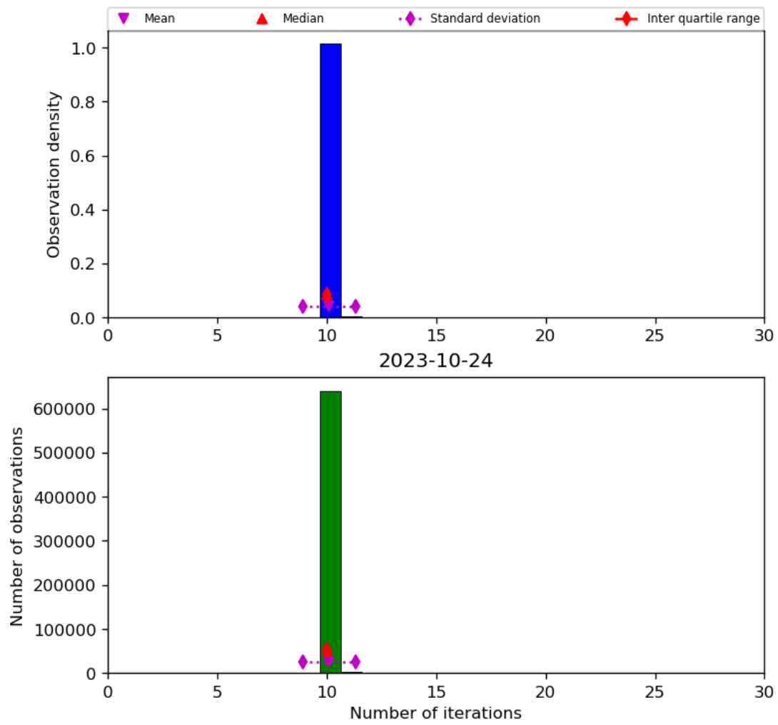
Figure 31: Histogram of “Number of iterations” for 2023-10-23 to 2023-10-25
