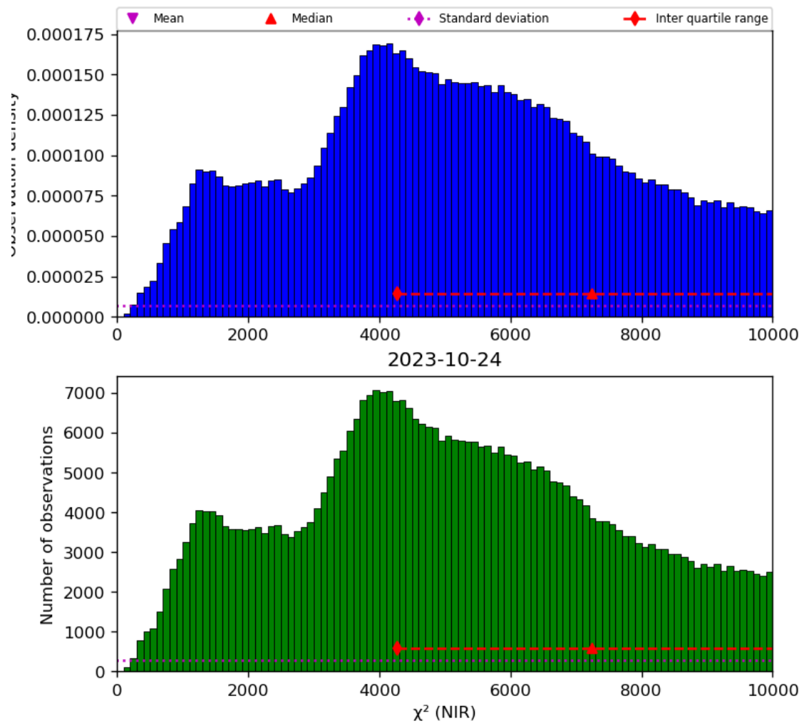
Figure 29: Histogram of “ \chi^2 (NIR)” for 2023-10-23 to 2023-10-25
