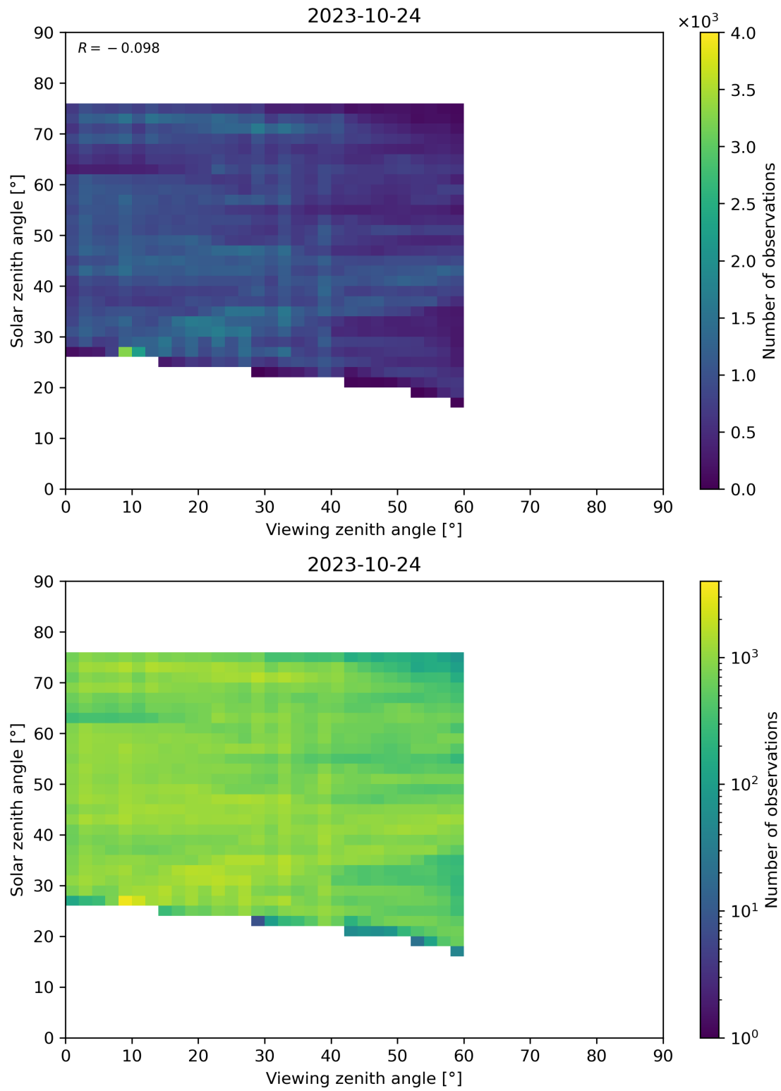
Figure 115: Scatter density plot of “Viewing zenith angle” against “Solar zenith angle” for 2023-10-23 to 2023-10-25.
