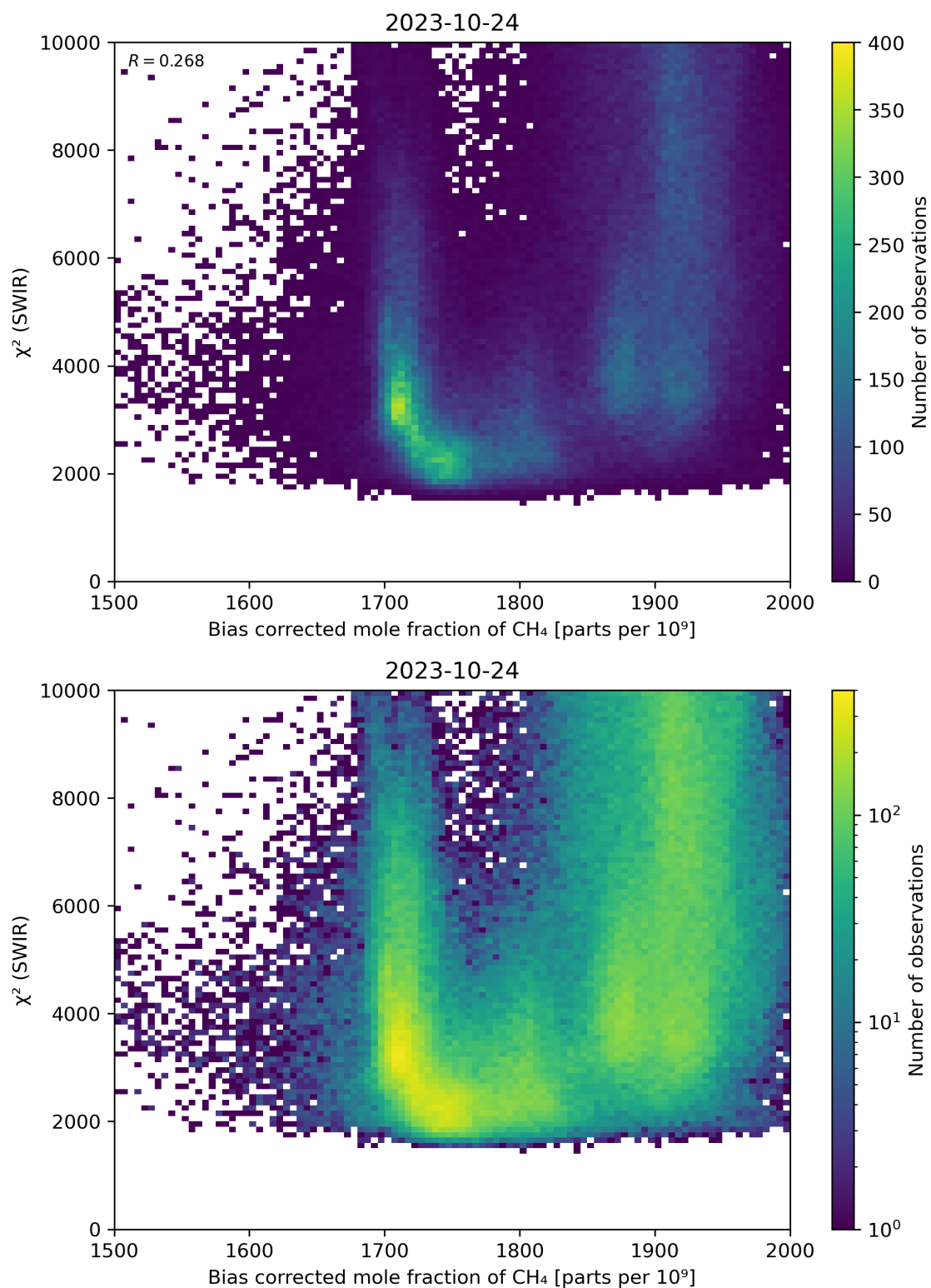
Figure 64: Scatter density plot of “Bias corrected mole fraction of CH 4 ” against “ \chi^2 (SWIR)” for 2023-10-23 to 2023-10-25.
