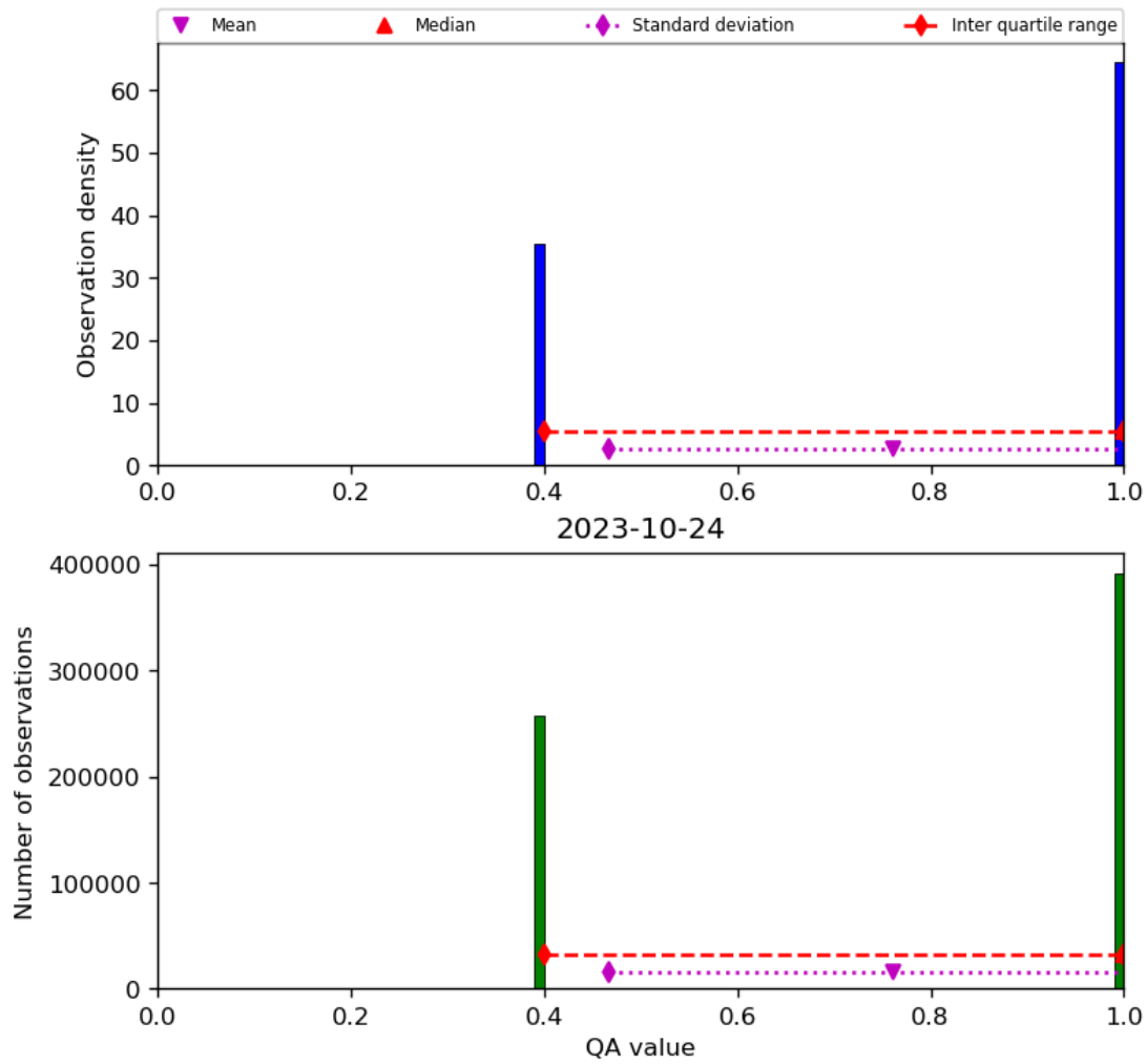
Figure 22: Histogram of “QA value” for 2023-10-23 to 2023-10-25
