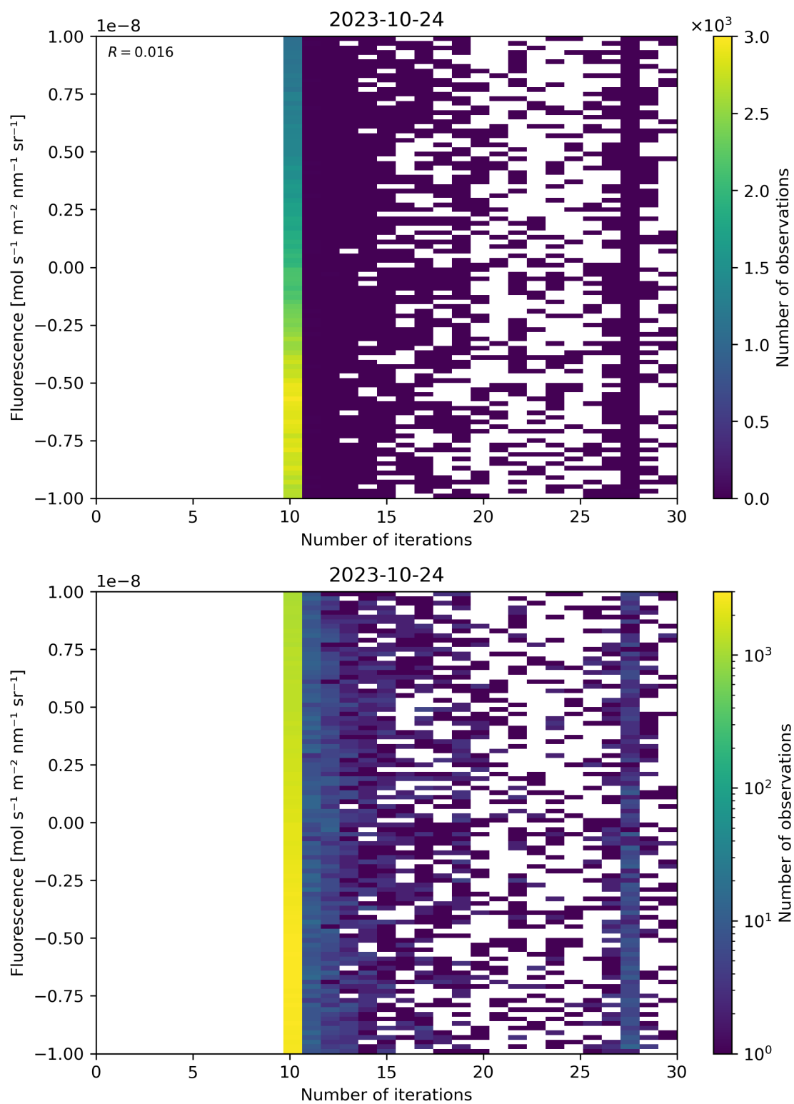
Figure 87: Scatter density plot of “Number of iterations” against “Fluorescence” for 2023-10-23 to 2023-10-25.
