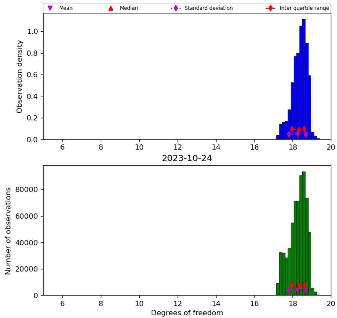
Figure 30: Histogram of “Degrees of freedom” for 2023-10-23 to 2023-10-25
