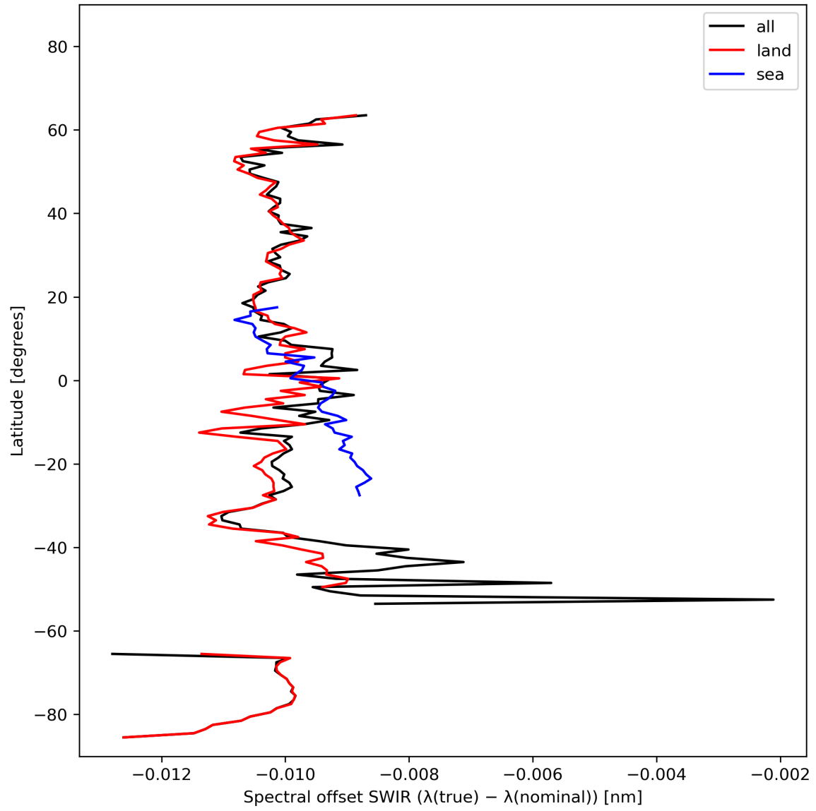
Figure 16: Zonal average of “Spectral offset SWIR ( \lambda(\text{true}) - \lambda(\text{nominal}) )” for 2023-10-23 to 2023-10-25.
