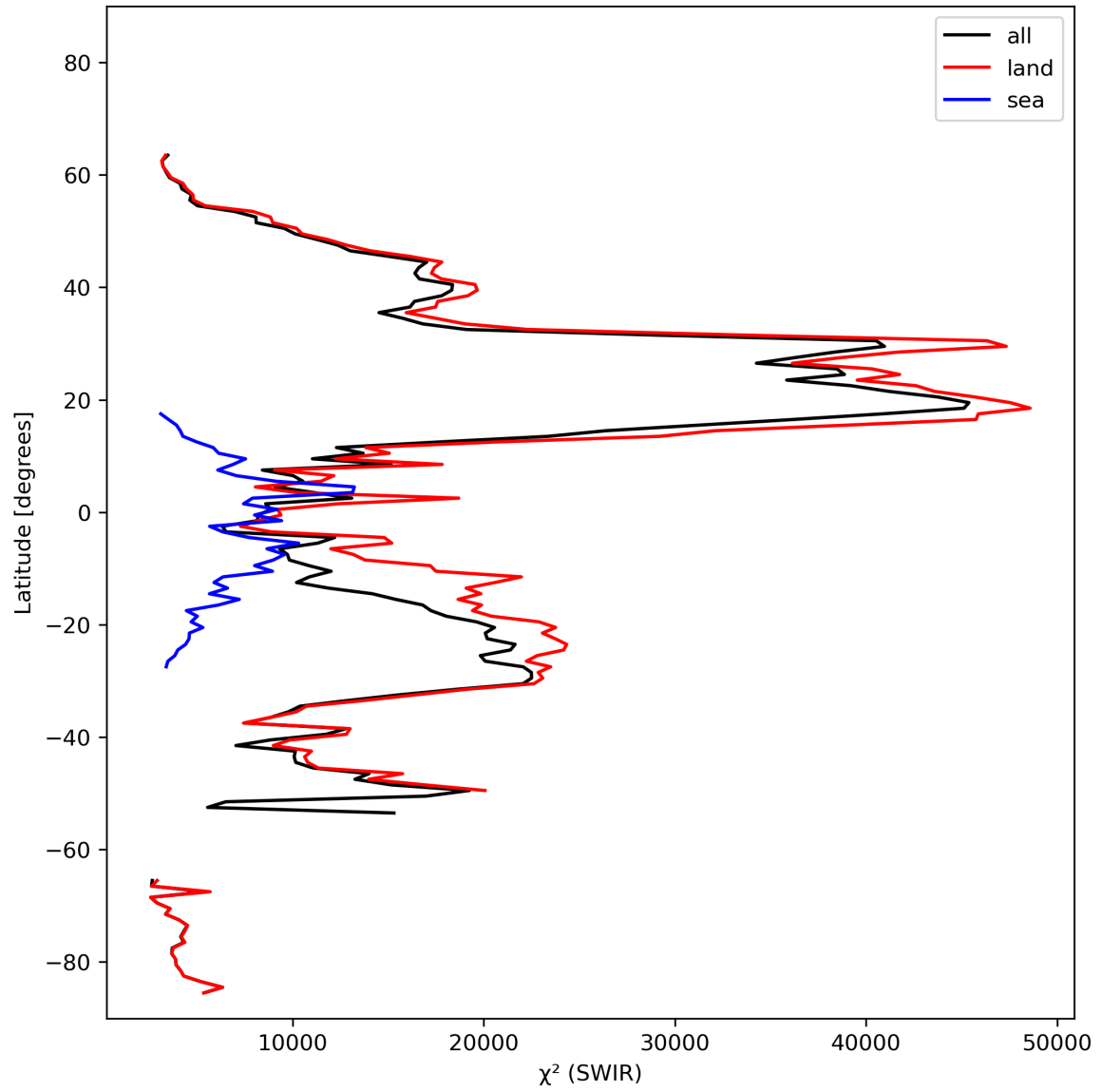
Figure 17: Zonal average of “ \chi^2 (SWIR)” for 2023-10-23 to 2023-10-25.
