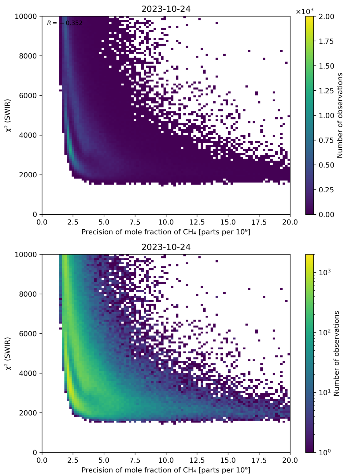
Figure 79: Scatter density plot of “Precision of mole fraction of \text{CH}_4 ” against “ \chi^2 (SWIR)” for 2023-10-23 to 2023-10-25.
