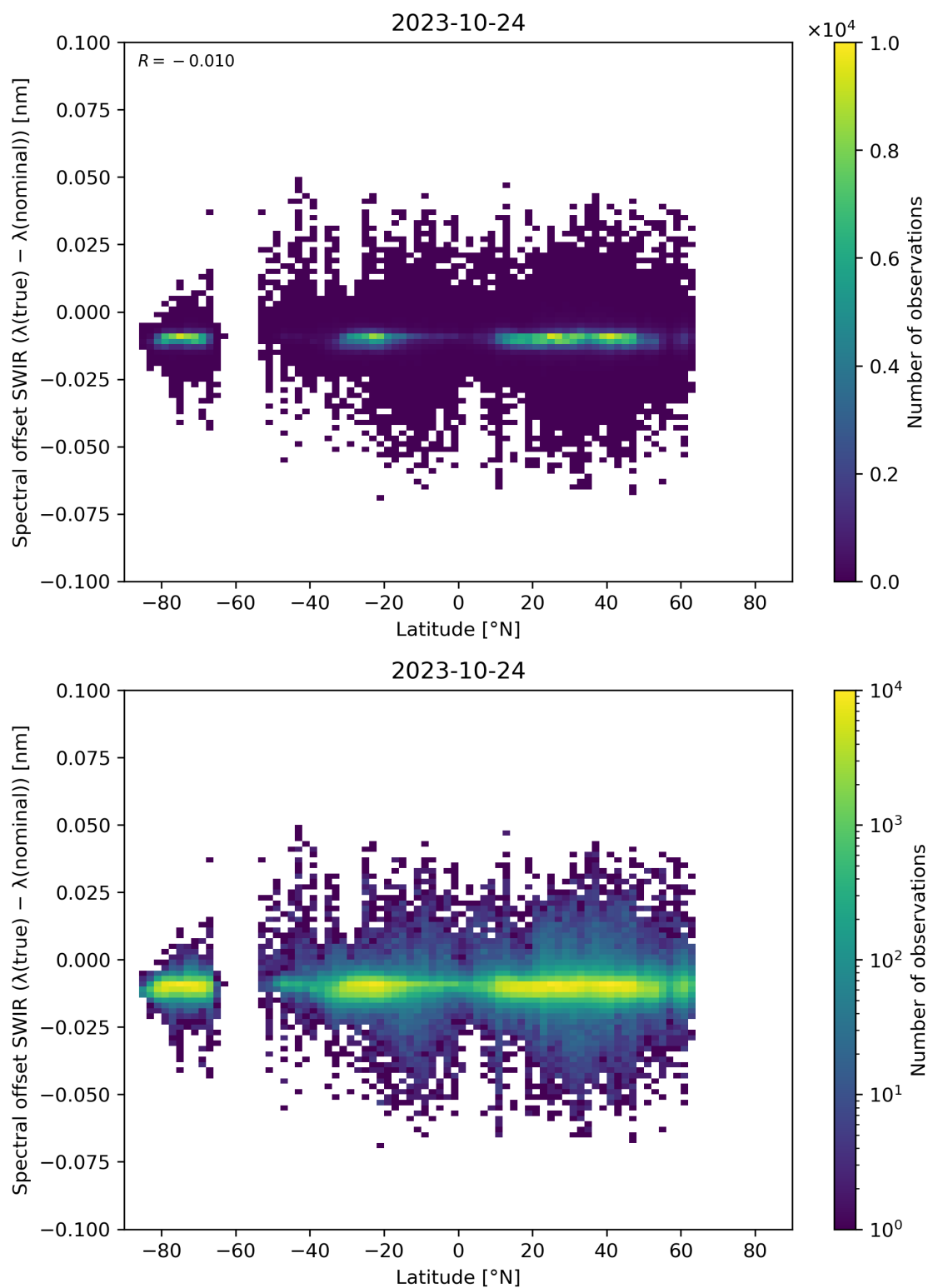
Figure 62: Scatter density plot of “Latitude” against “Spectral offset SWIR ( \lambda(\text{true}) - \lambda(\text{nominal}) )” for 2023-10-23 to 2023-10-25.
