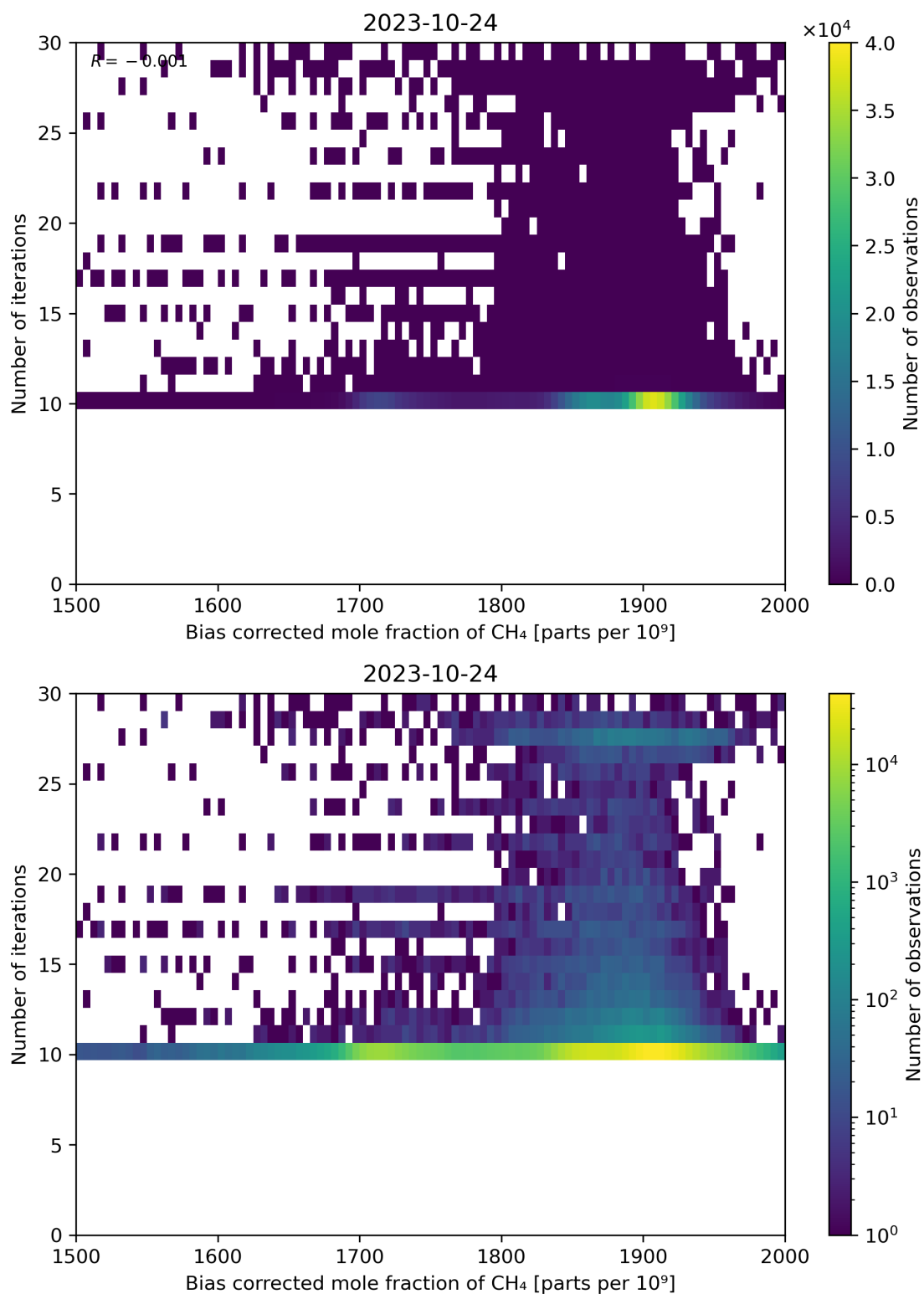
Figure 67: Scatter density plot of “Bias corrected mole fraction of CH 4 ” against “Number of iterations” for 2023-10-23 to 2023-10-25.
