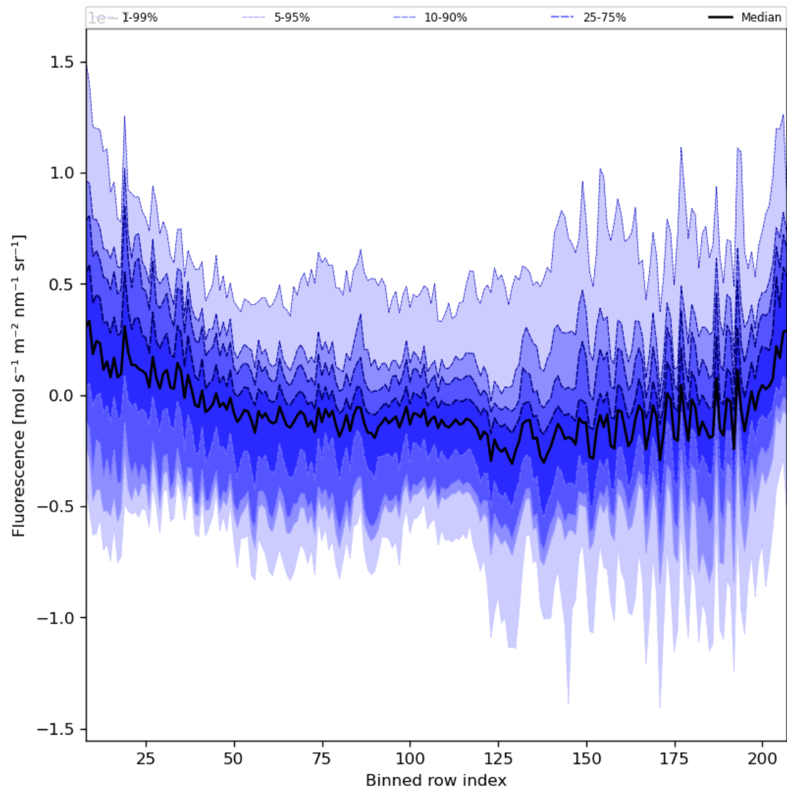
Figure 43: Along track statistics of “Fluorescence” for 2023-10-23 to 2023-10-25
