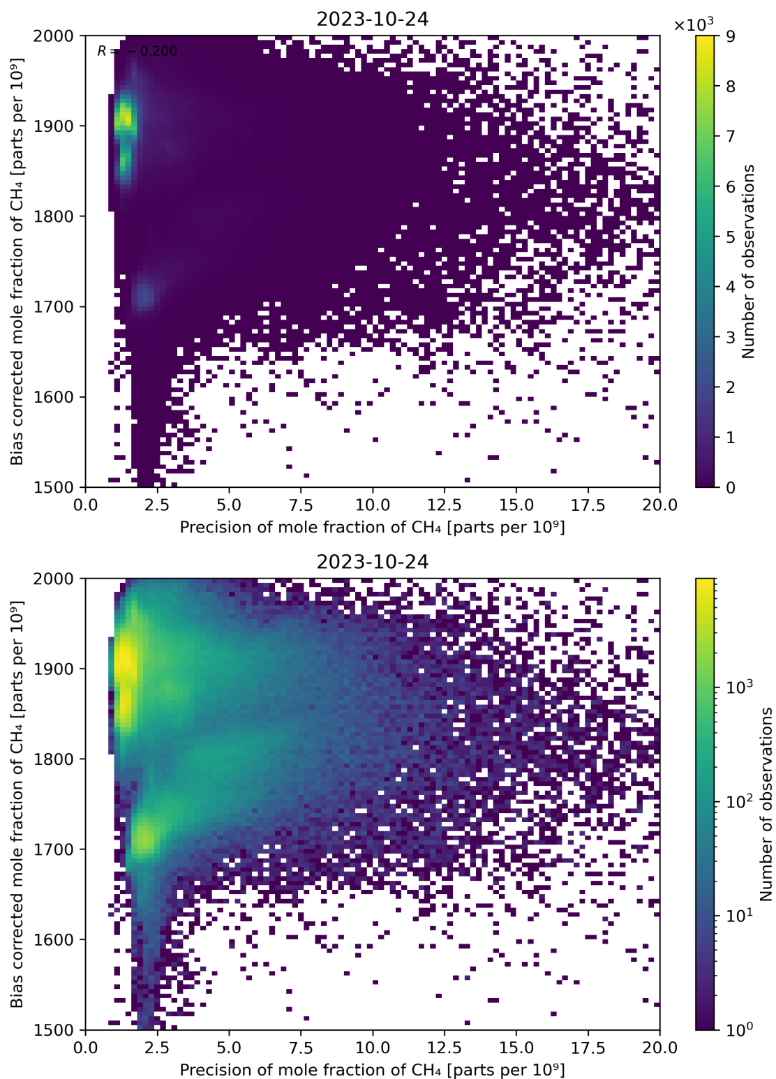
Figure 82: Scatter density plot of “Precision of mole fraction of \text{CH}_4 ” against “Bias corrected mole fraction of \text{CH}_4 ” for 2023-10-23 to 2023-10-25.
