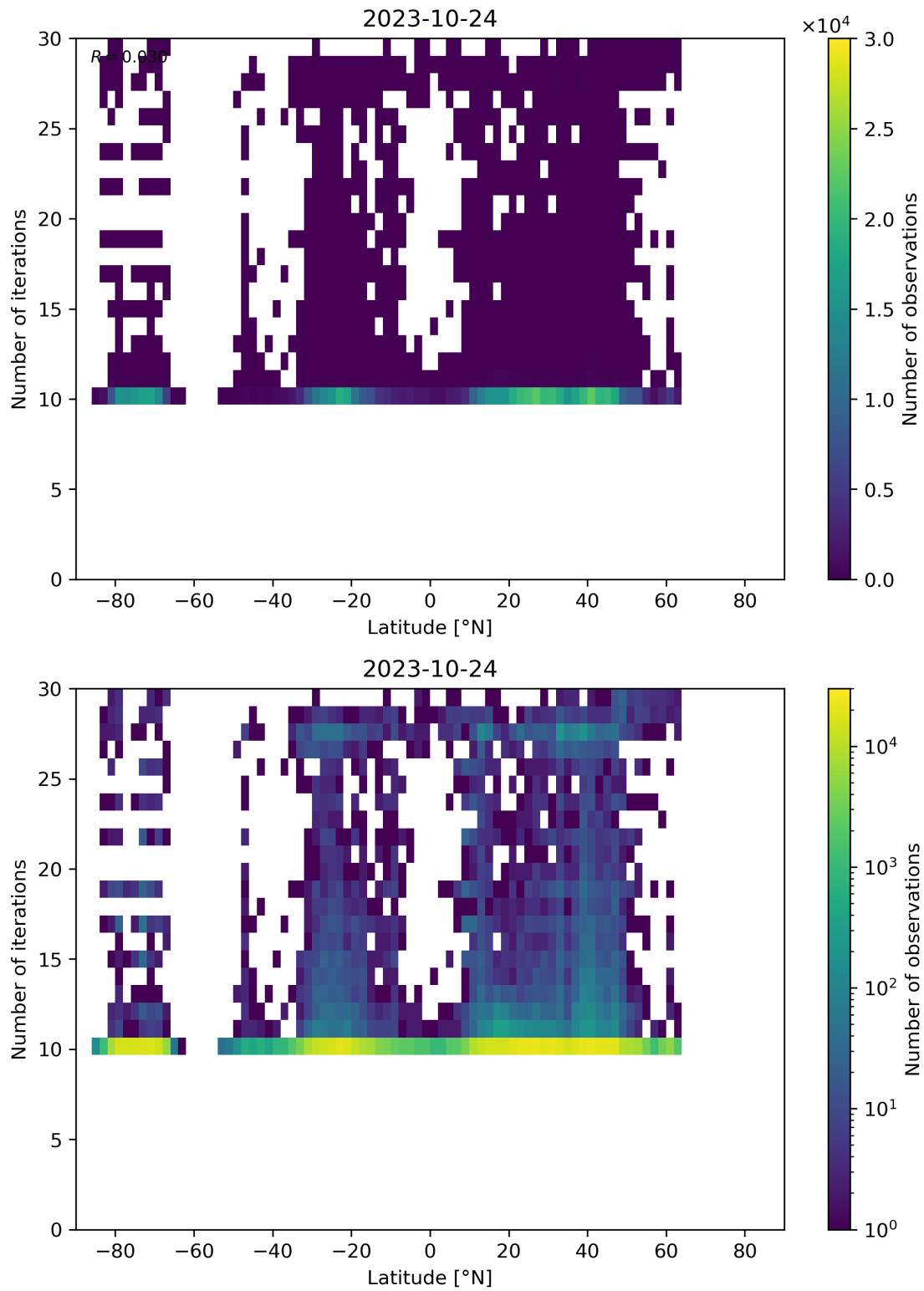
Figure 60: Scatter density plot of “Latitude” against “Number of iterations” for 2023-10-23 to 2023-10-25.
