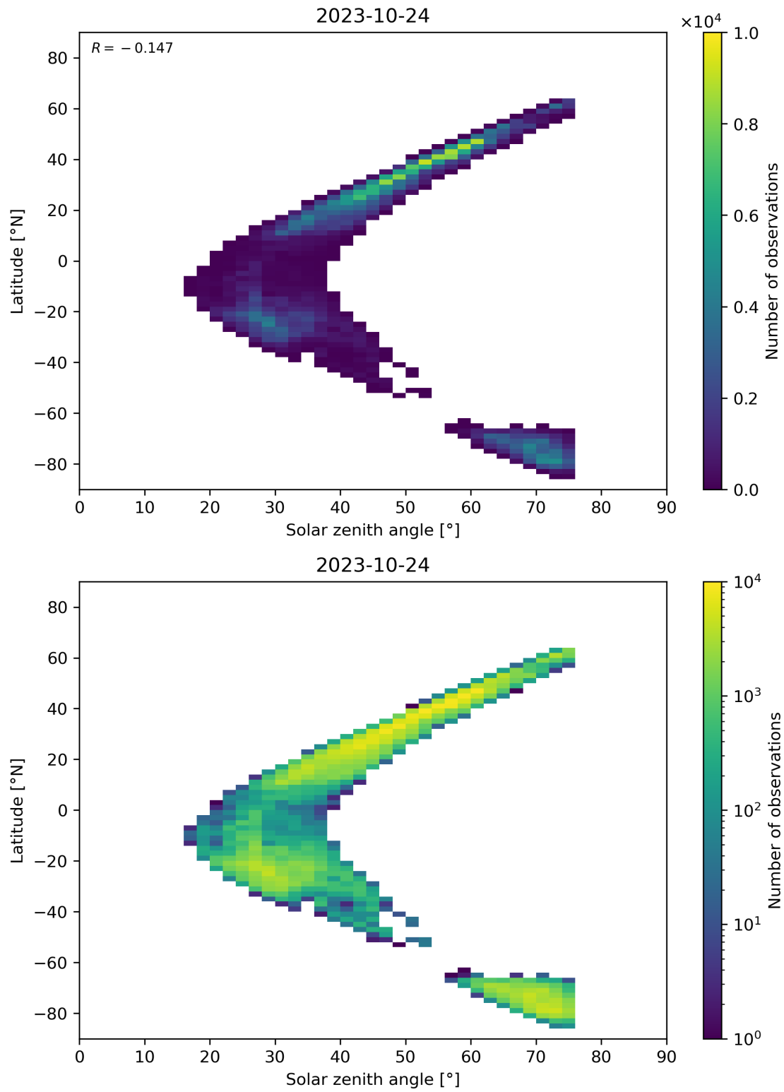
Figure 98: Scatter density plot of “Solar zenith angle” against “Latitude” for 2023-10-23 to 2023-10-25.
