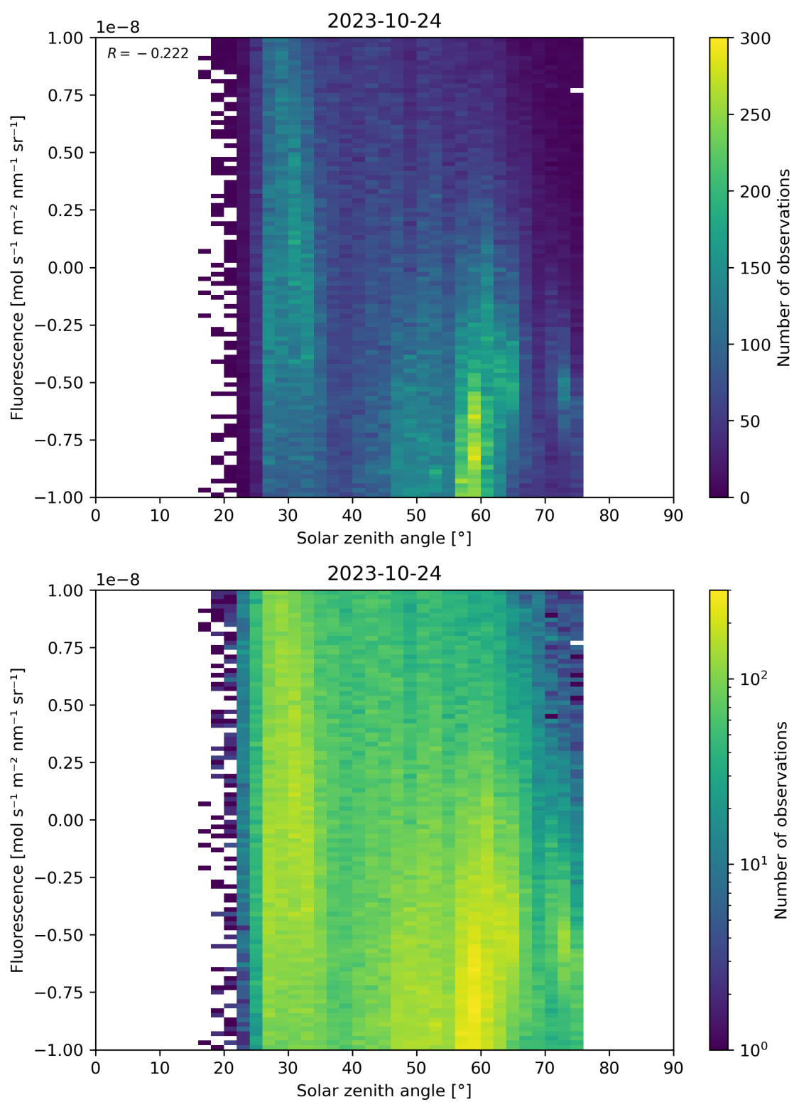
Figure 97: Scatter density plot of “Solar zenith angle” against “Fluorescence” for 2023-10-23 to 2023-10-25.
