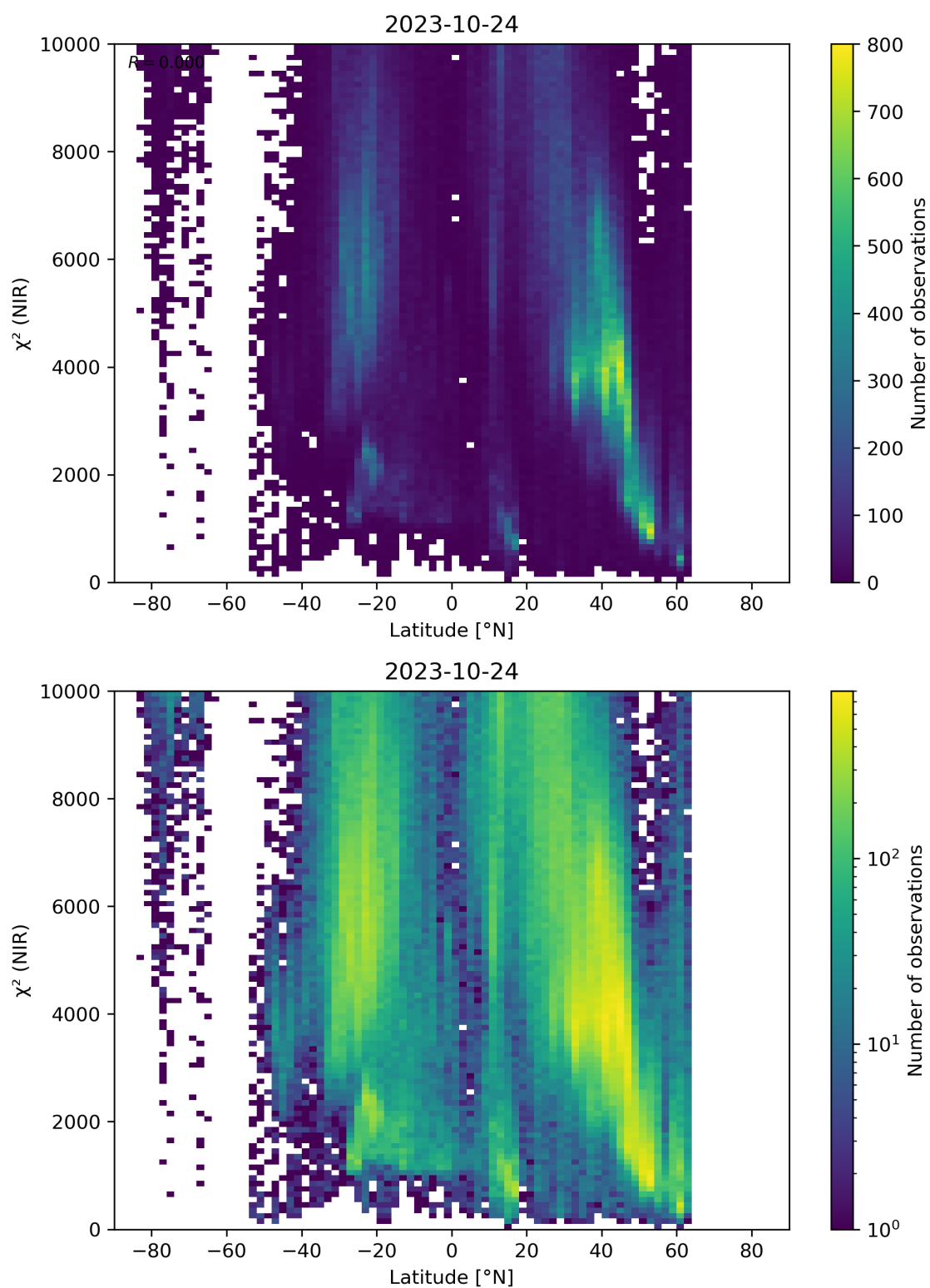
Figure 53: Scatter density plot of “Latitude” against “ \chi^2 (NIR)” for 2023-10-23 to 2023-10-25.
