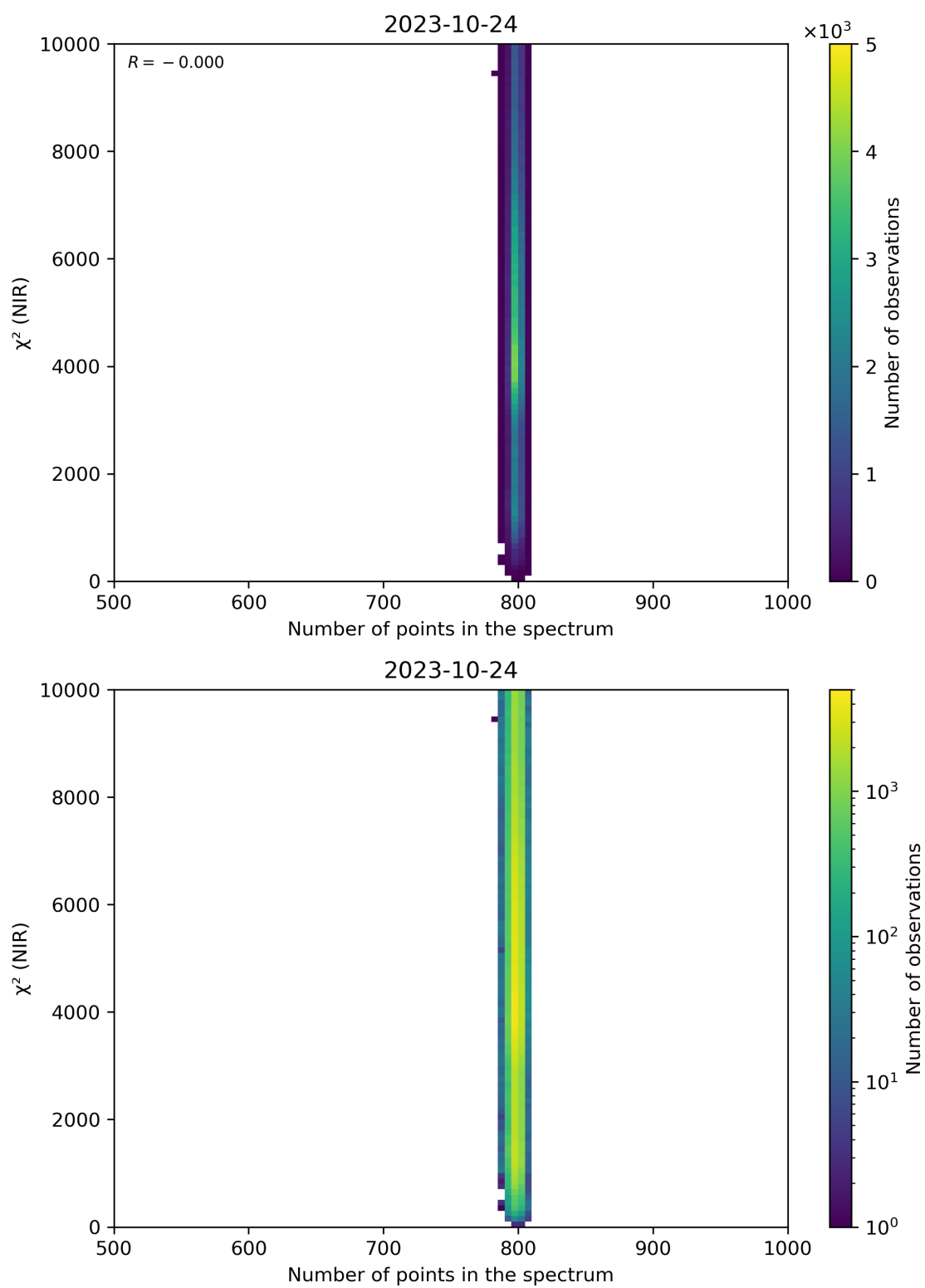
Figure 88: Scatter density plot of “Number of points in the spectrum” against “ \chi^2 (NIR)” for 2023-10-23 to 2023-10-25.
