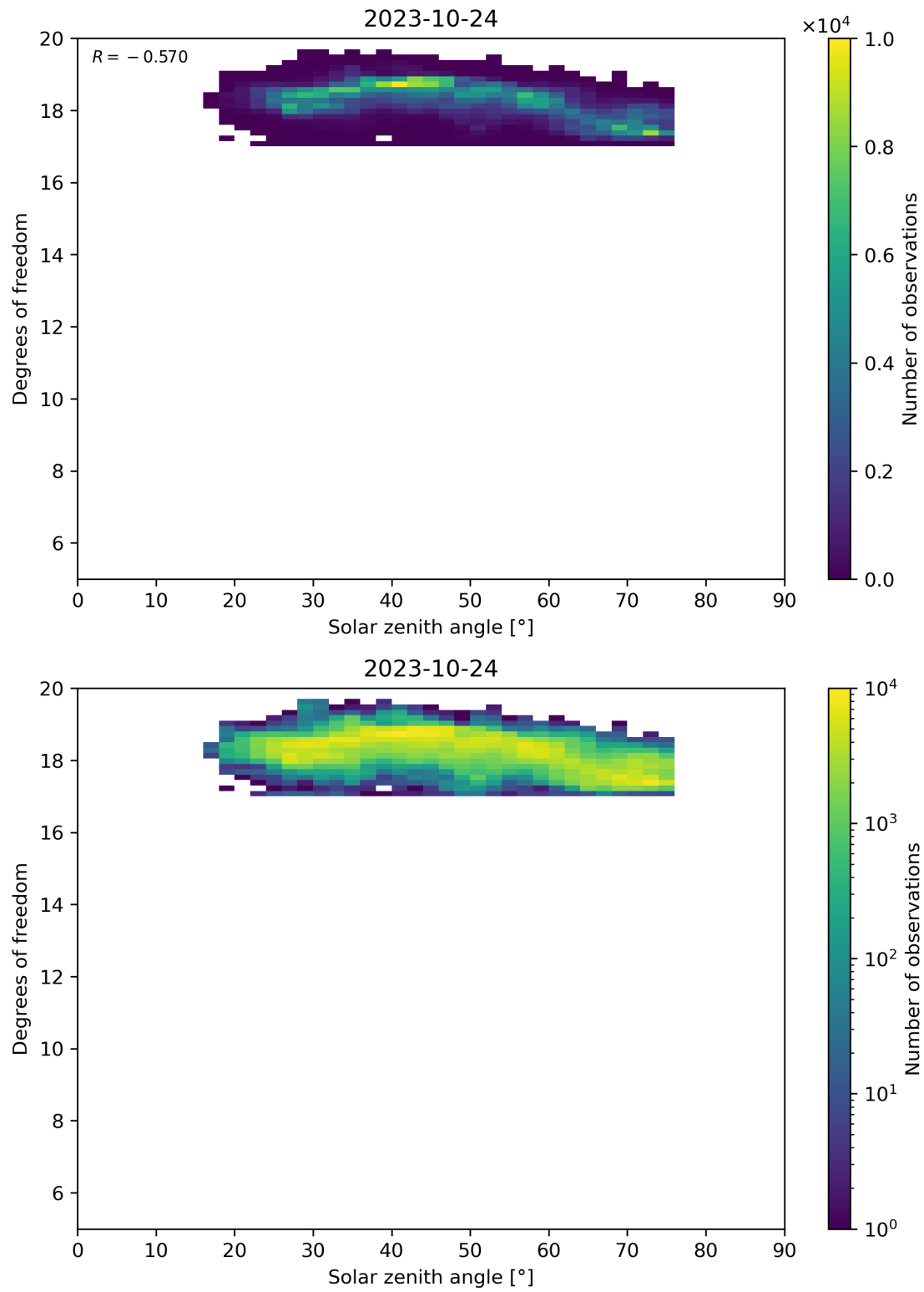
Figure 96: Scatter density plot of “Solar zenith angle” against “Degrees of freedom” for 2023-10-23 to 2023-10-25.
