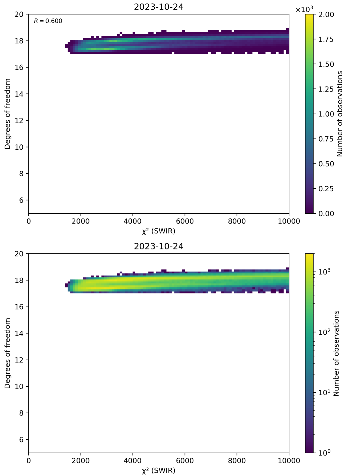
Figure 48: Scatter density plot of “ \chi^2 (SWIR)” against “Degrees of freedom” for 2023-10-23 to 2023-10-25.
