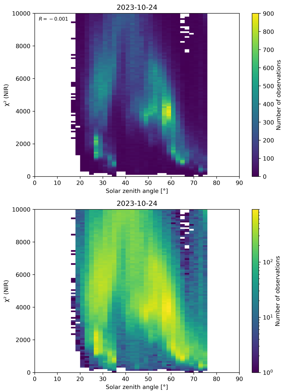
Figure 94: Scatter density plot of “Solar zenith angle” against “ \chi^2 (NIR)” for 2023-10-23 to 2023-10-25.
