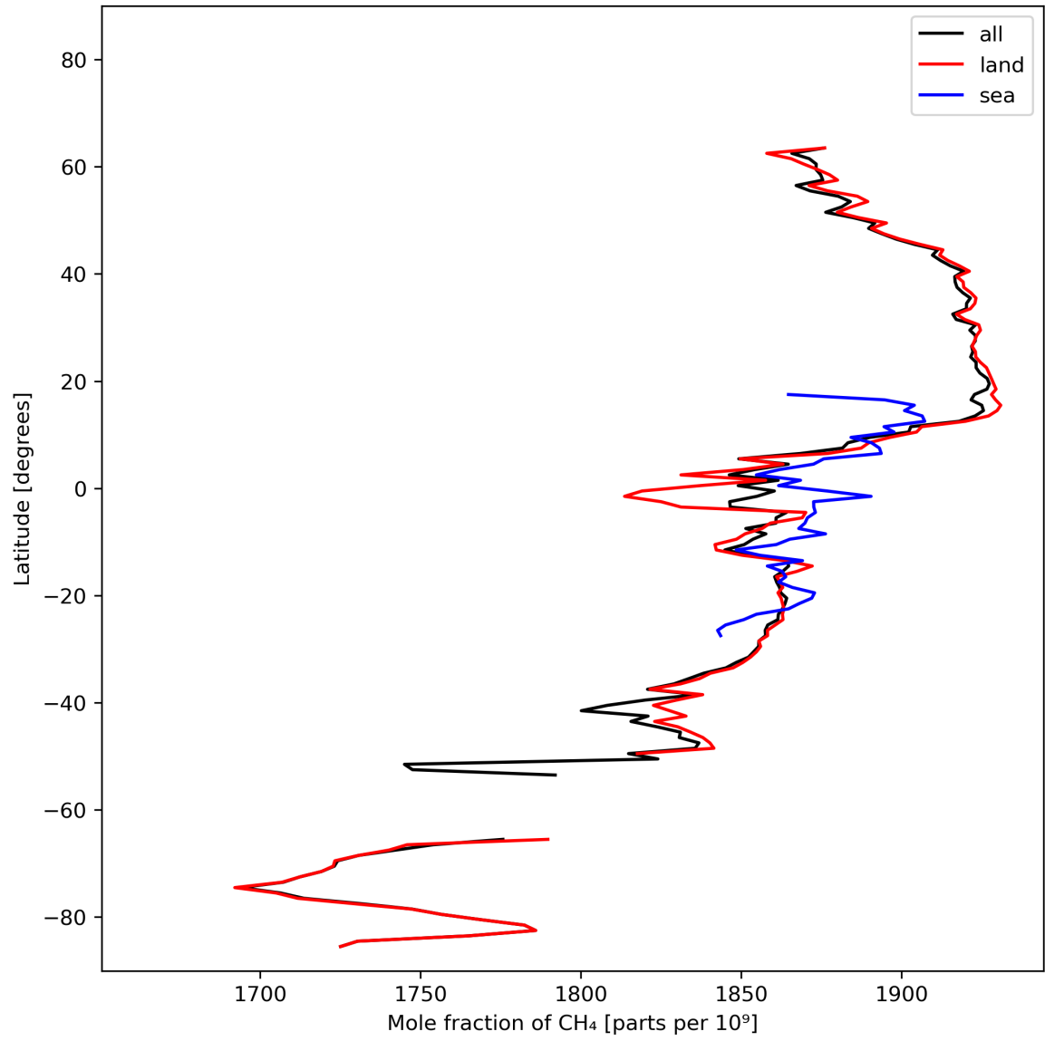
Figure 12: Zonal average of “Mole fraction of CH 4 ” for 2023-10-23 to 2023-10-25.
