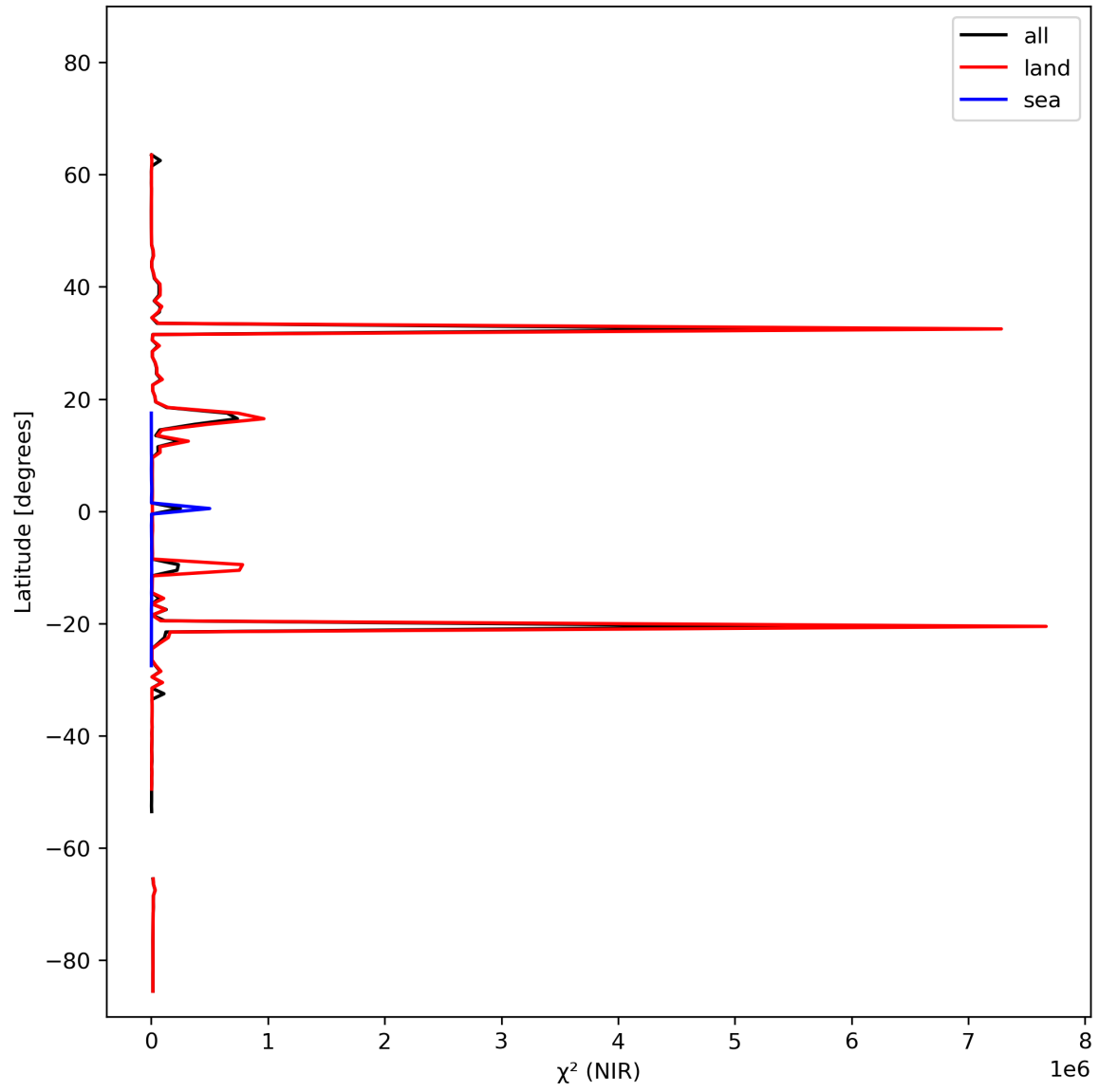
Figure 18: Zonal average of “ \chi^2 (NIR)” for 2023-10-23 to 2023-10-25.
