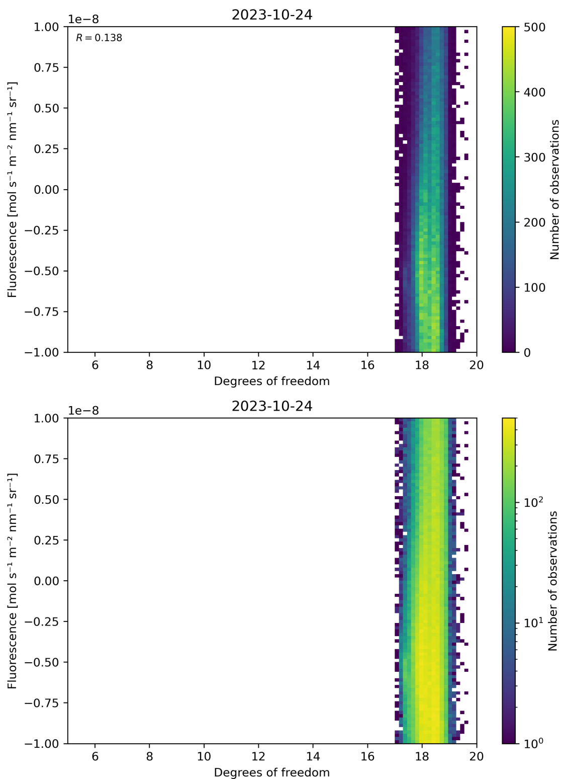
Figure 51: Scatter density plot of “Degrees of freedom” against “Fluorescence” for 2023-10-23 to 2023-10-25.
