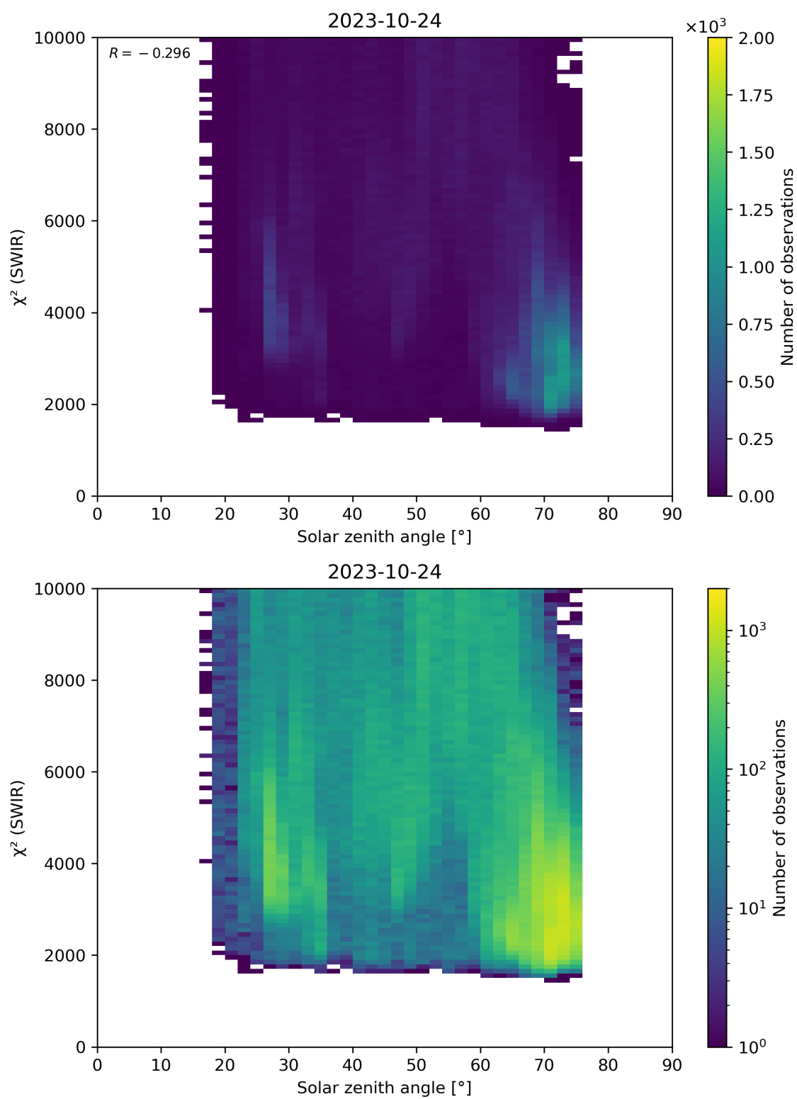
Figure 95: Scatter density plot of “Solar zenith angle” against “ \chi^2 (SWIR)” for 2023-10-23 to 2023-10-25.
