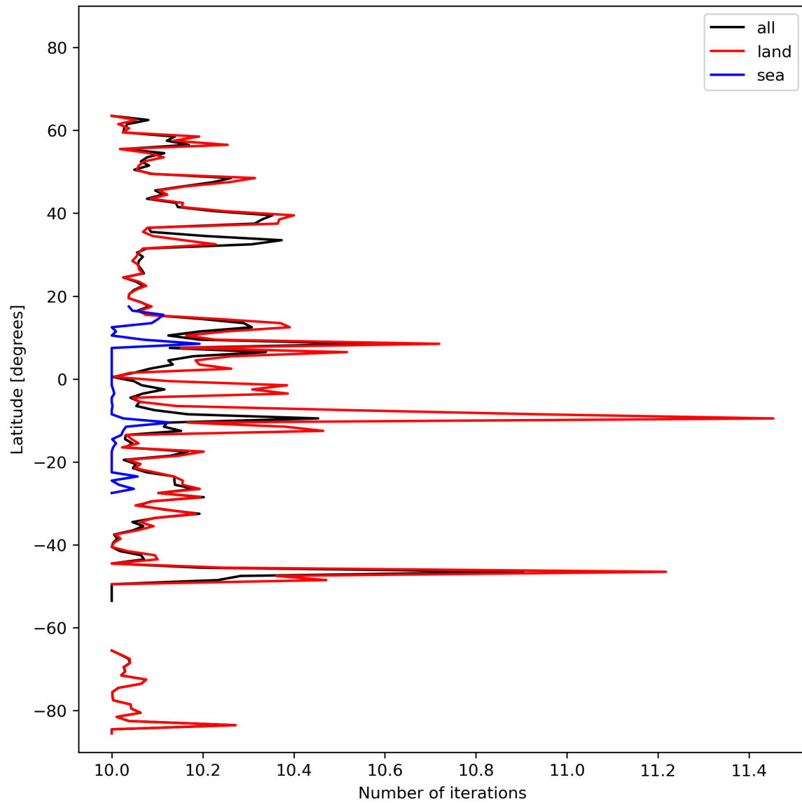
Figure 20: Zonal average of “Number of iterations” for 2023-10-23 to 2023-10-25.
