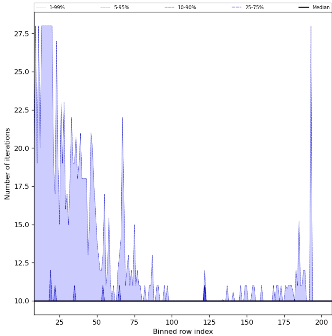
Figure 42: Along track statistics of “Number of iterations” for 2023-10-23 to 2023-10-25
