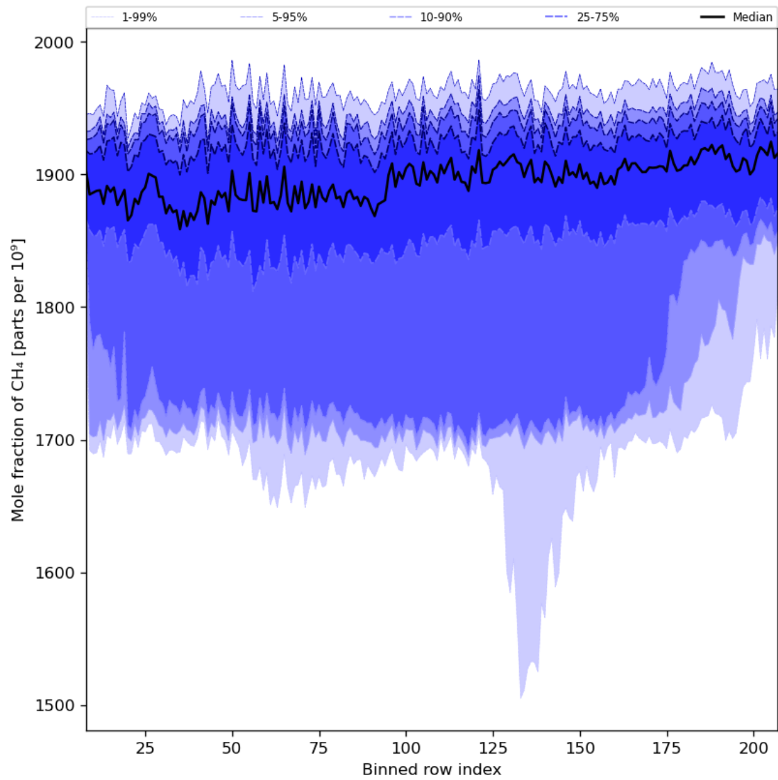
Figure 34: Along track statistics of “Mole fraction of CH 4 ” for 2023-10-23 to 2023-10-25
