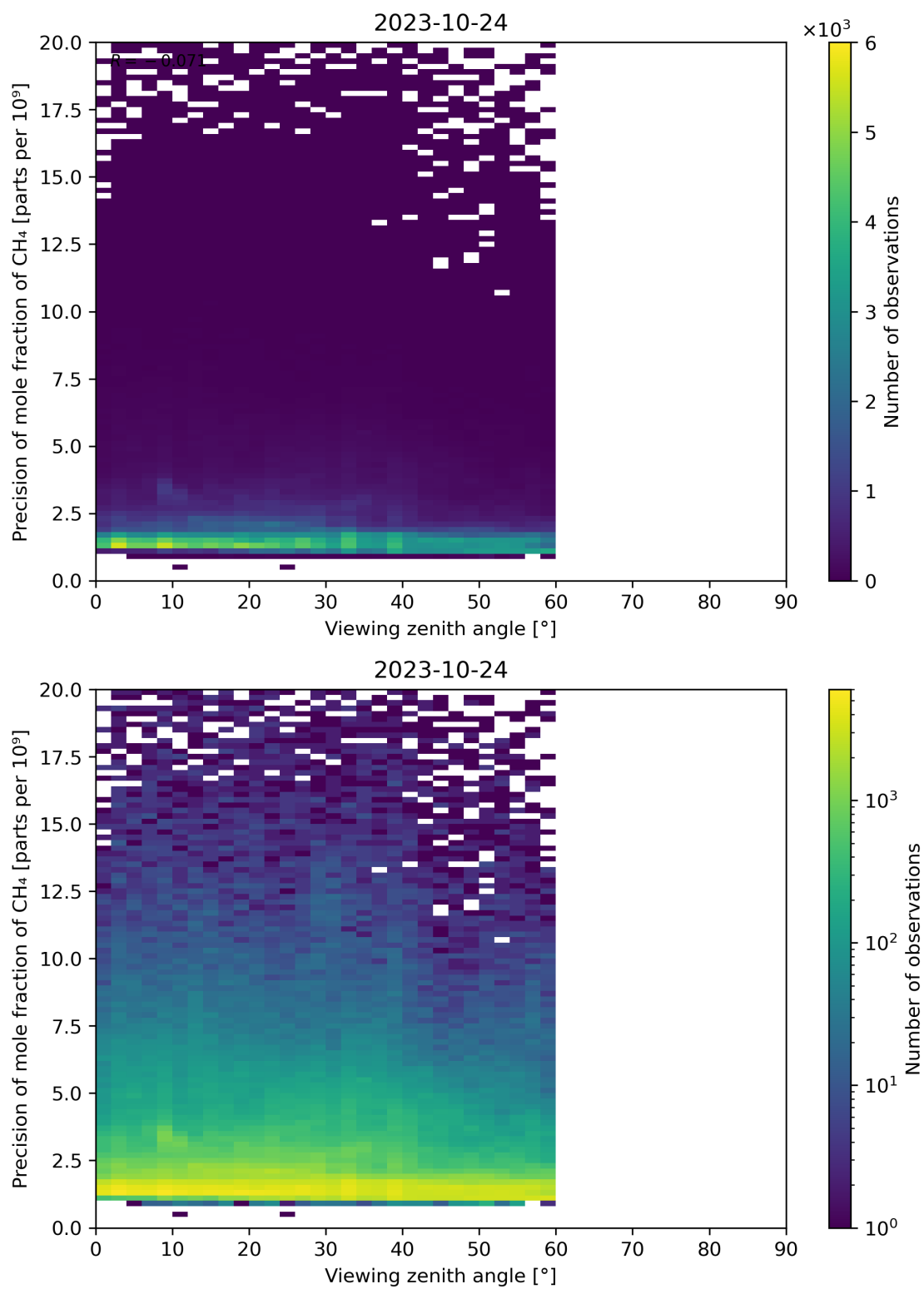
Figure 112: Scatter density plot of “Viewing zenith angle” against “Precision of mole fraction of CH 4 ” for 2023-10-23 to 2023-10-25.
