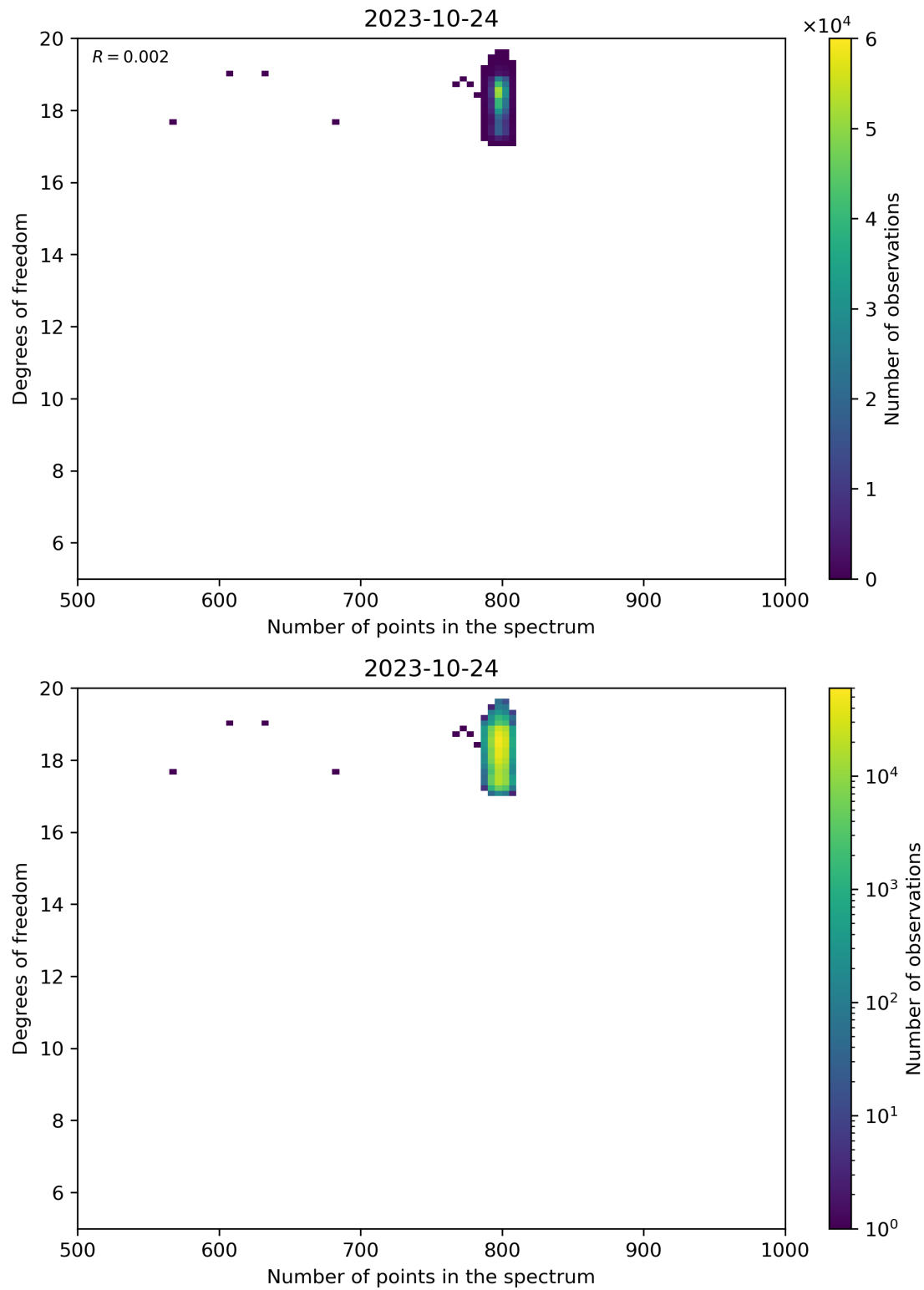
Figure 90: Scatter density plot of “Number of points in the spectrum” against “Degrees of freedom” for 2023-10-23 to 2023-10-25.
