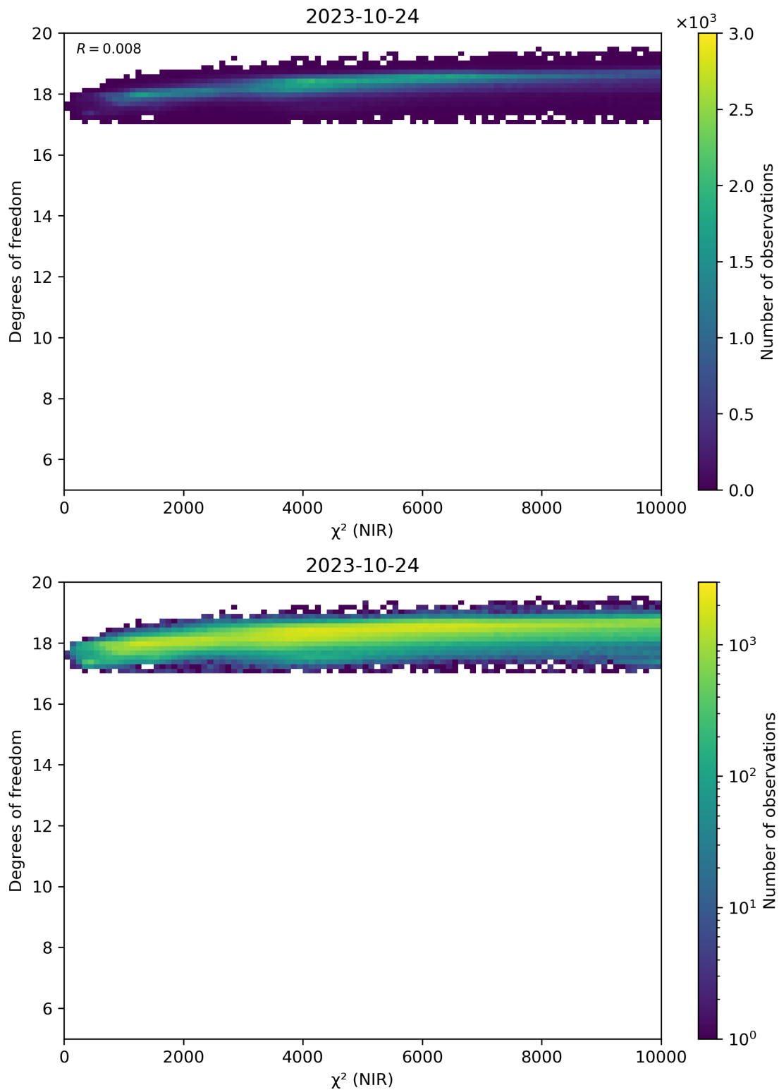
Figure 44: Scatter density plot of “ \chi^2 (NIR)” against “Degrees of freedom” for 2023-10-23 to 2023-10-25.
