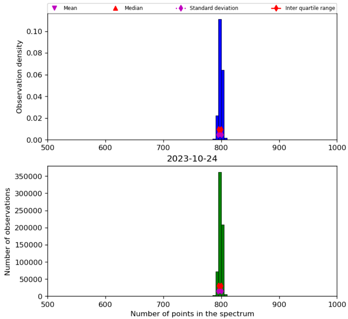
Figure 26: Histogram of “Number of points in the spectrum” for 2023-10-23 to 2023-10-25
