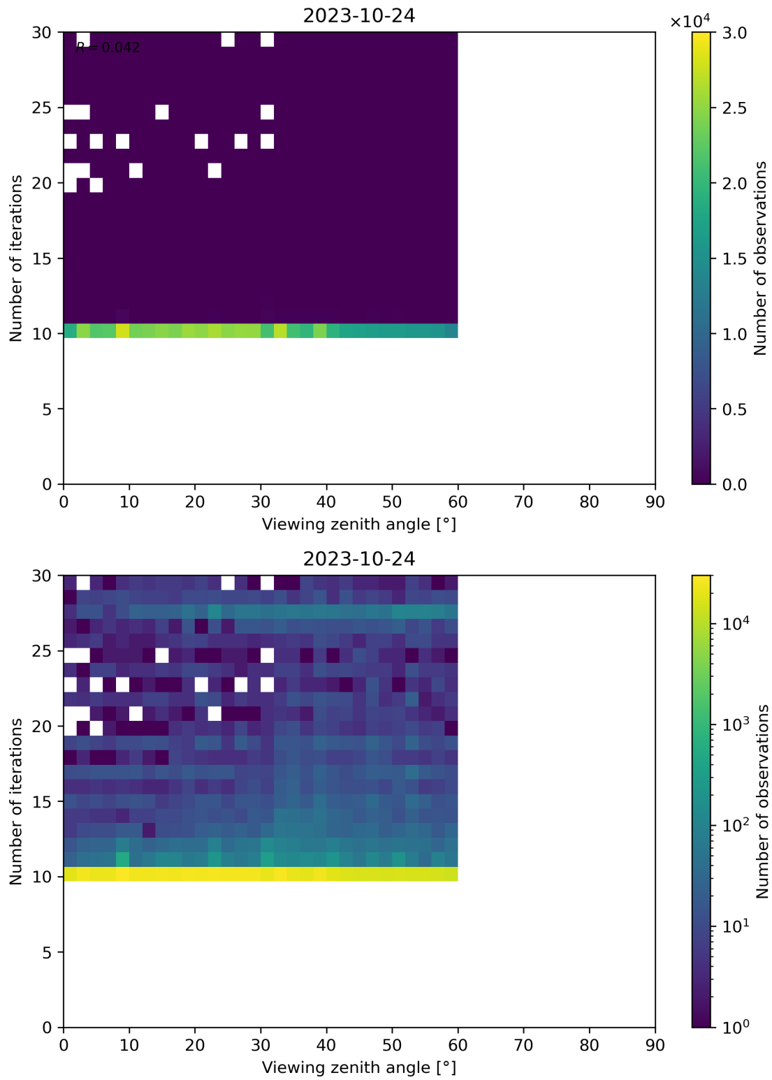
Figure 113: Scatter density plot of “Viewing zenith angle” against “Number of iterations” for 2023-10-23 to 2023-10-25.
