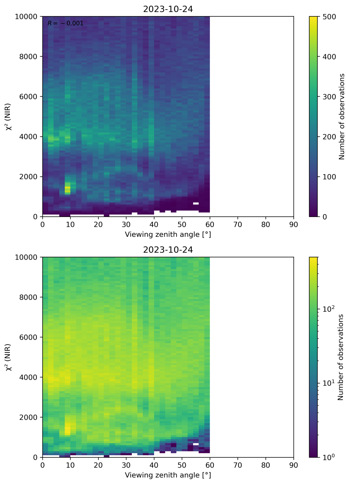
Figure 105: Scatter density plot of “Viewing zenith angle” against “ \chi^2 (NIR)” for 2023-10-23 to 2023-10-25.
