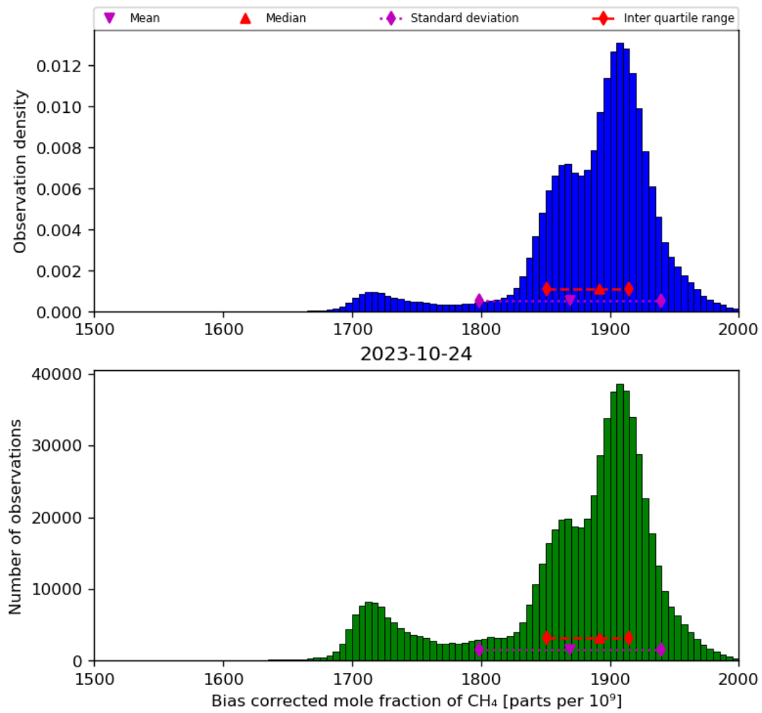
Figure 25: Histogram of “Bias corrected mole fraction of CH 4 ” for 2023-10-23 to 2023-10-25
