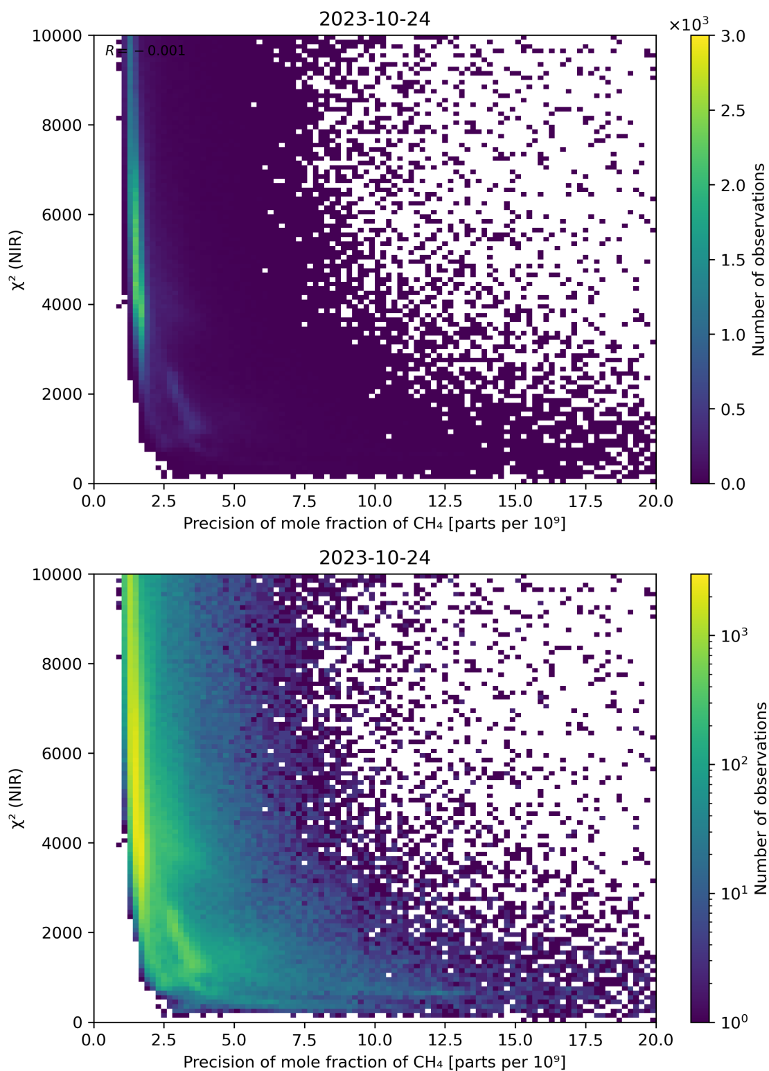
Figure 78: Scatter density plot of “Precision of mole fraction of CH 4 ” against “ \chi^2 (NIR)” for 2023-10-23 to 2023-10-25.
