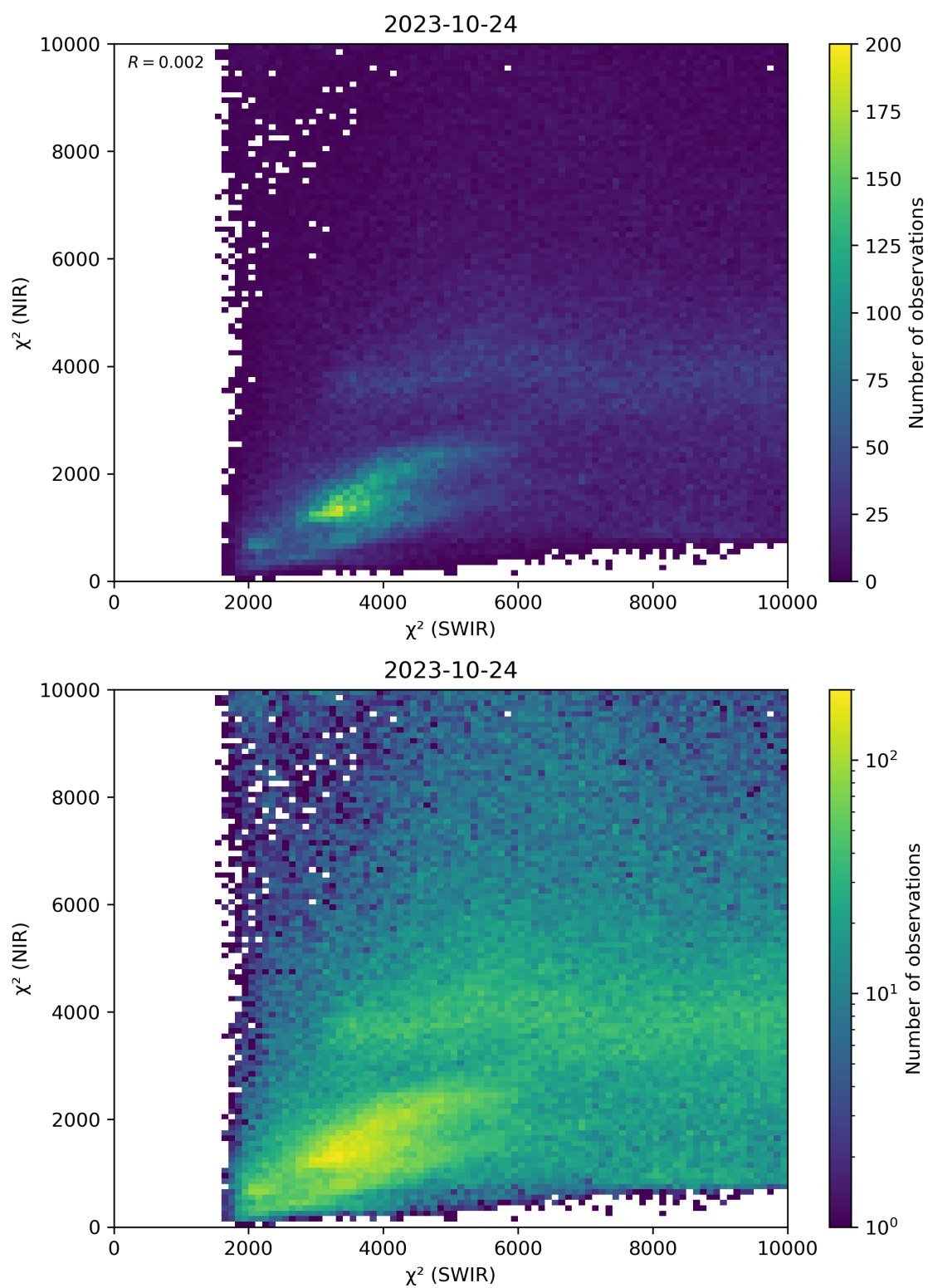
Figure 47: Scatter density plot of “ \chi^2 (SWIR)” against “ \chi^2 (NIR)” for 2023-10-23 to 2023-10-25.
