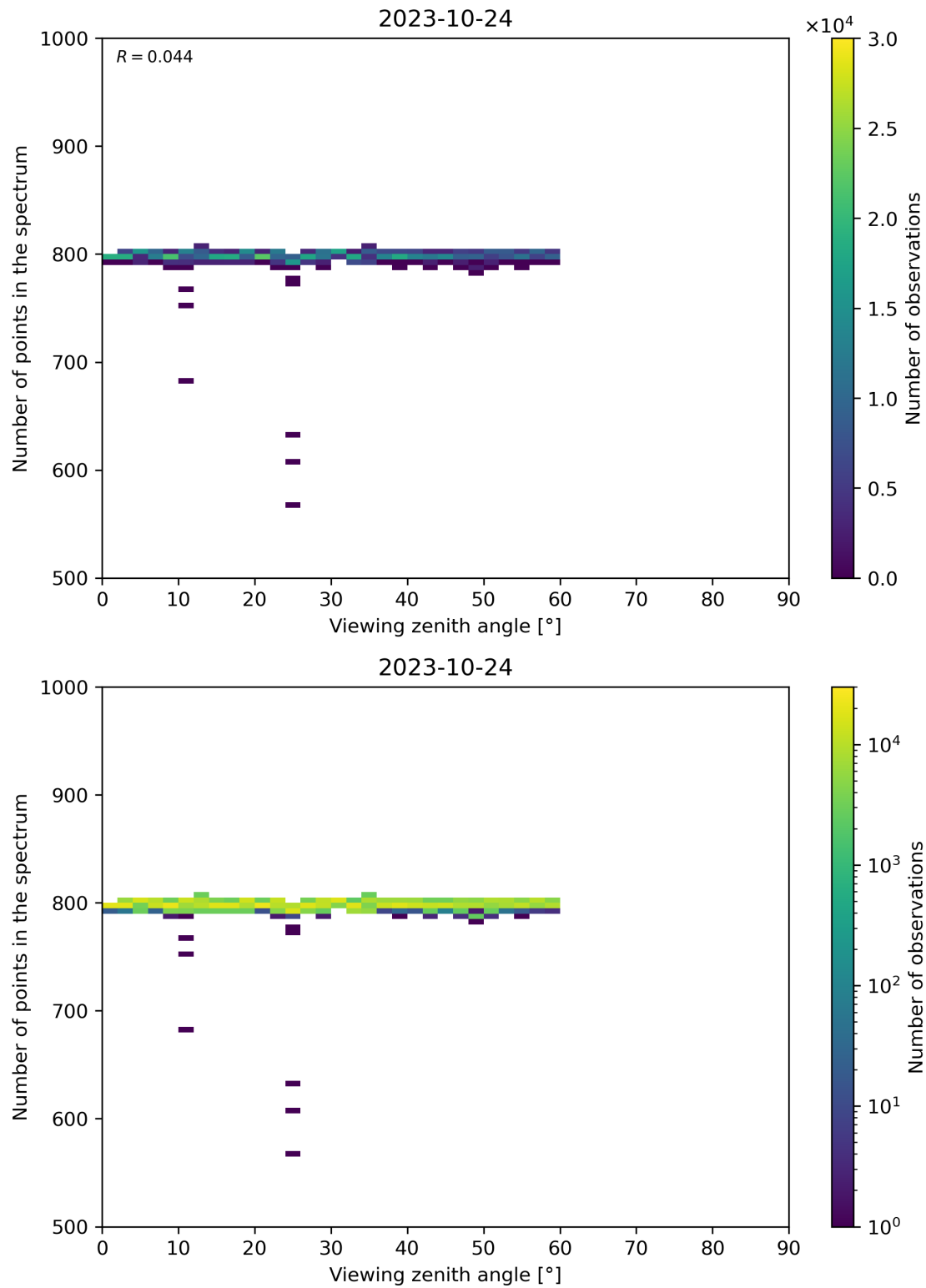
Figure 114: Scatter density plot of “Viewing zenith angle” against “Number of points in the spectrum” for 2023-10-23 to 2023-10-25.
