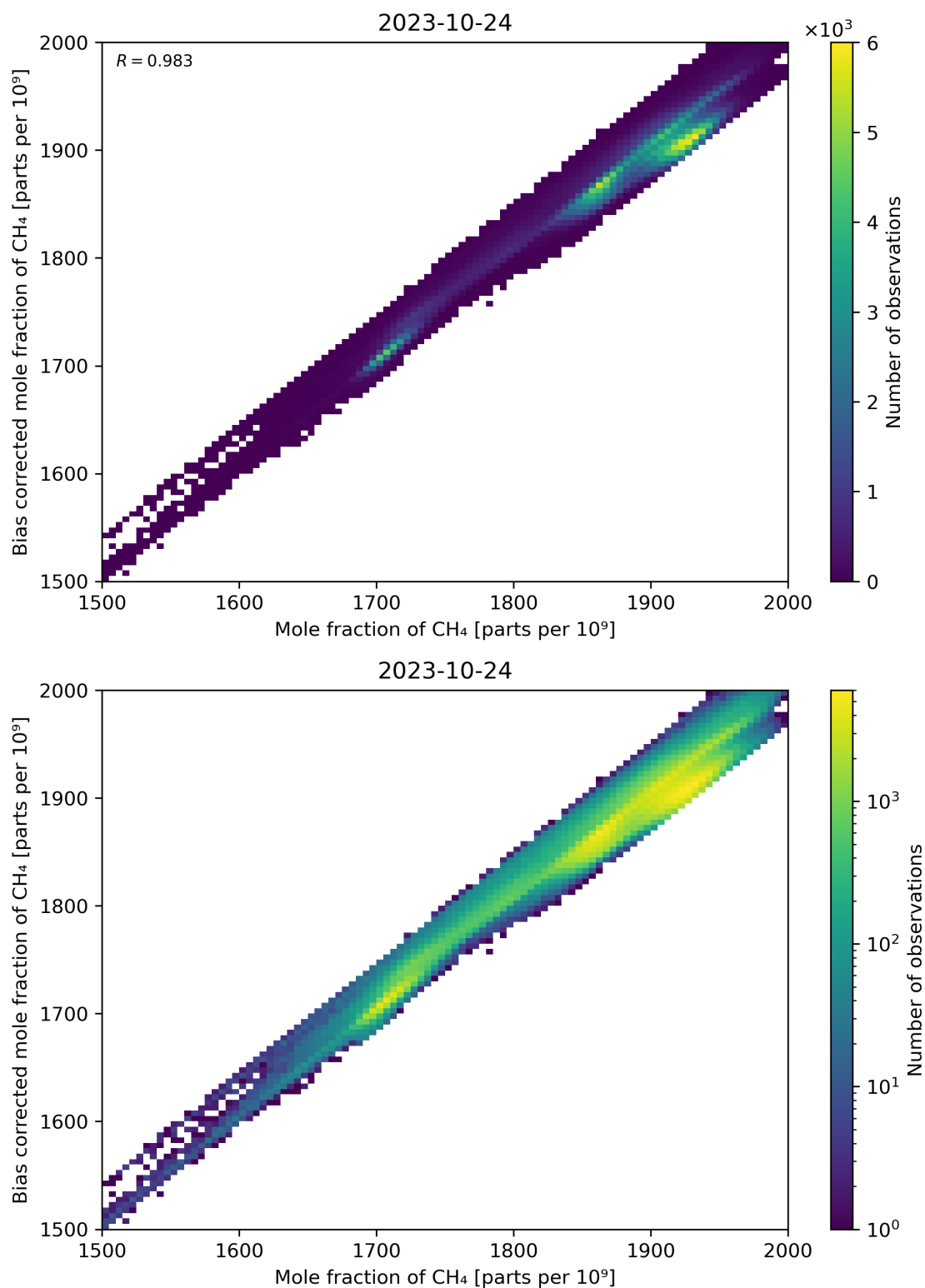
Figure 74: Scatter density plot of “Mole fraction of CH 4 ” against “Bias corrected mole fraction of CH 4 ” for 2023-10-23 to 2023-10-25.
