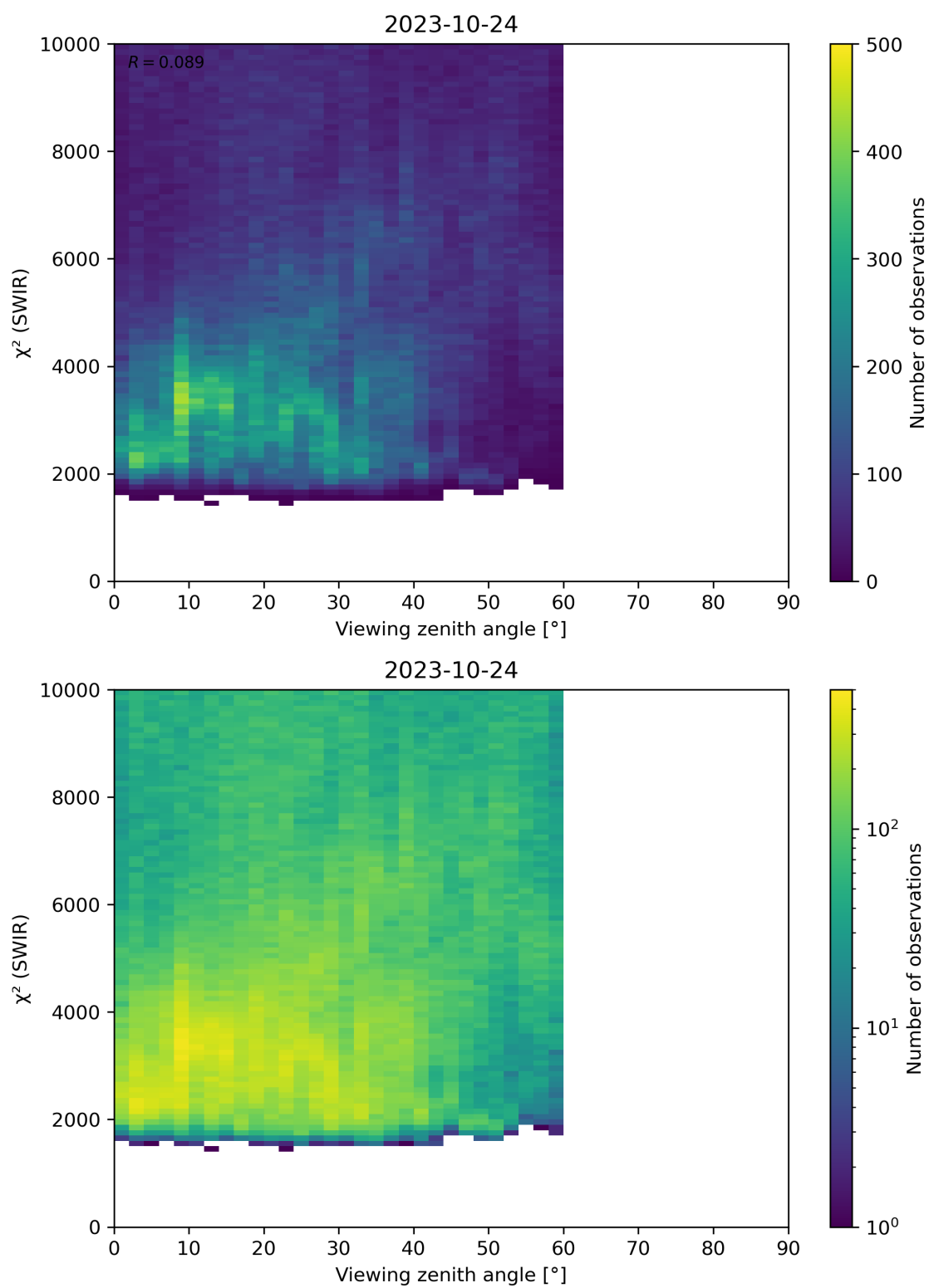
Figure 106: Scatter density plot of “Viewing zenith angle” against “ \chi^2 (SWIR)” for 2023-10-23 to 2023-10-25.
