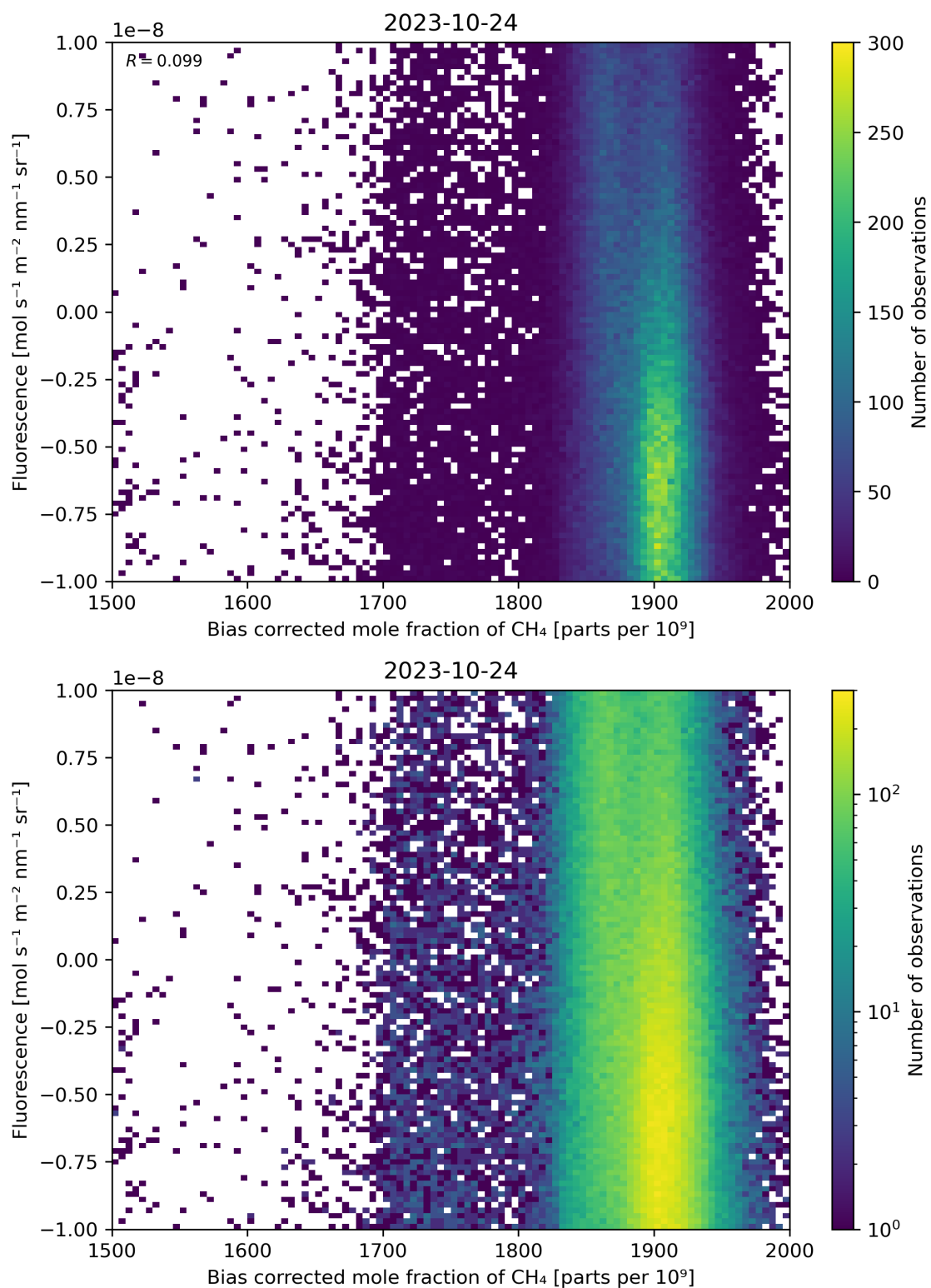
Figure 66: Scatter density plot of “Bias corrected mole fraction of \text{CH}_4 ” against “Fluorescence” for 2023-10-23 to 2023-10-25.
