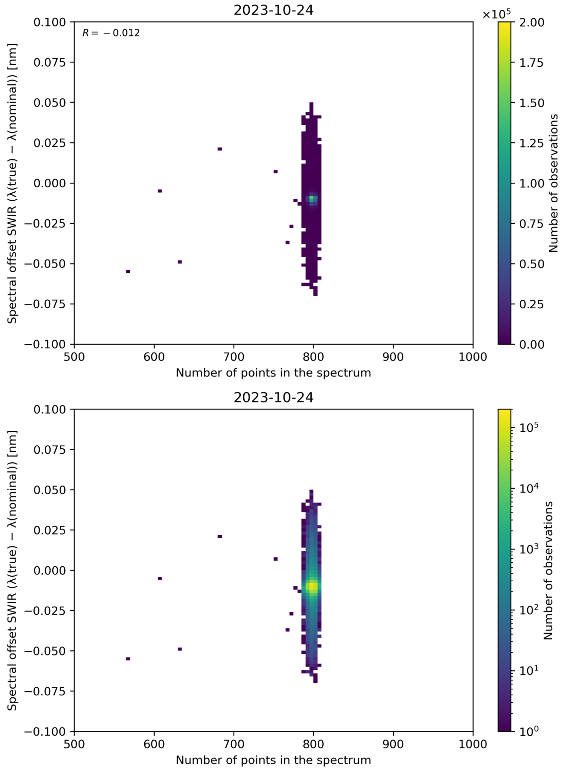
Figure 93: Scatter density plot of “Number of points in the spectrum” against “Spectral offset SWIR ( \lambda(\text{true}) - \lambda(\text{nominal}) )” for 2023-10-23 to 2023-10-25.
