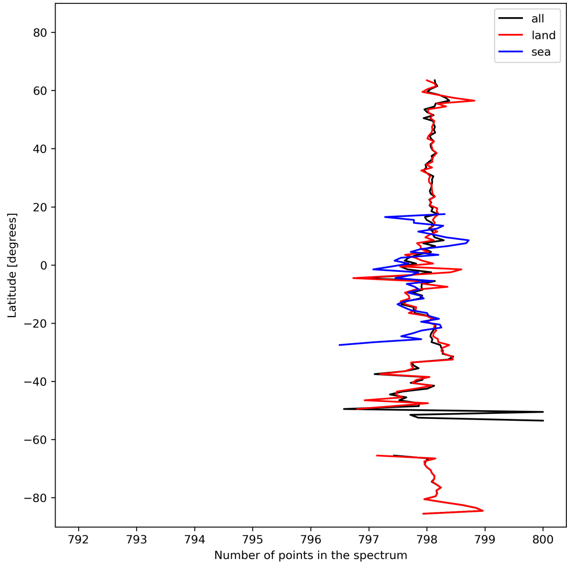
Figure 15: Zonal average of “Number of points in the spectrum” for 2023-10-23 to 2023-10-25.
