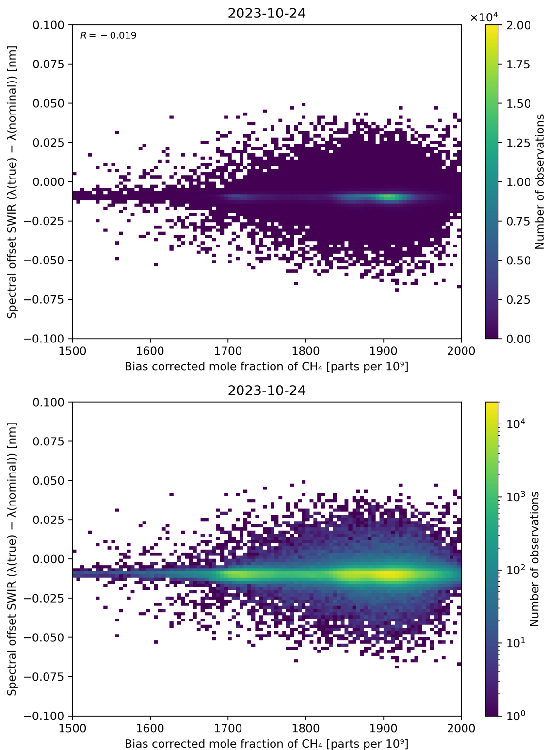
Figure 69: Scatter density plot of “Bias corrected mole fraction of \text{CH}_4 ” against “Spectral offset SWIR ( \lambda(\text{true}) - \lambda(\text{nominal}) )” for 2023-10-23 to 2023-10-25.
