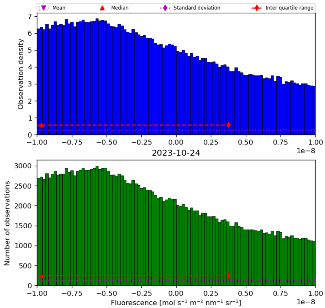
Figure 32: Histogram of “Fluorescence” for 2023-10-23 to 2023-10-25
