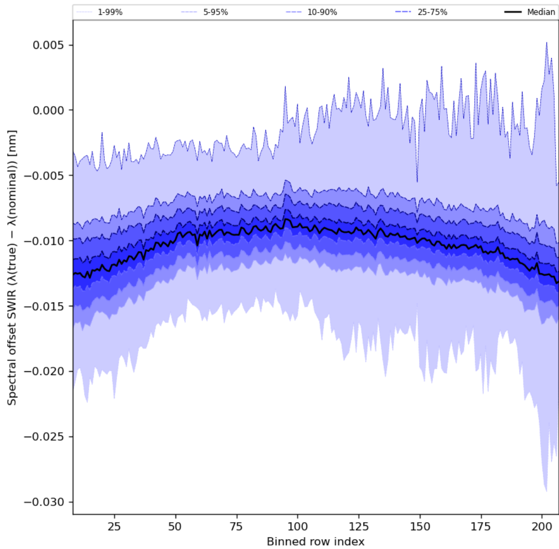
Figure 38: Along track statistics of “Spectral offset SWIR ( \lambda(\text{true}) - \lambda(\text{nominal}) )” for 2023-10-23 to 2023-10-25
