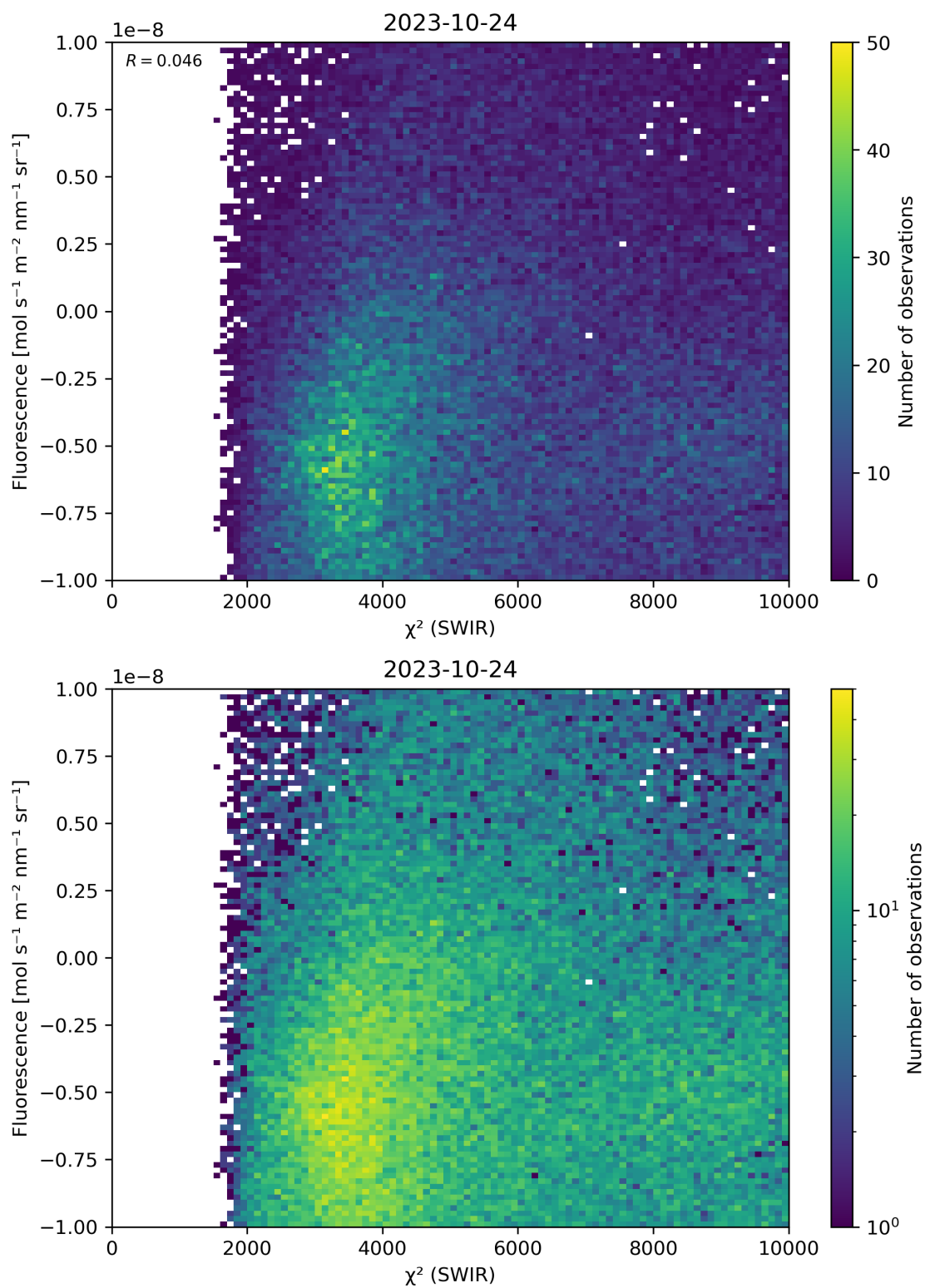
Figure 49: Scatter density plot of “ \chi^2 (SWIR)” against “Fluorescence” for 2023-10-23 to 2023-10-25.
