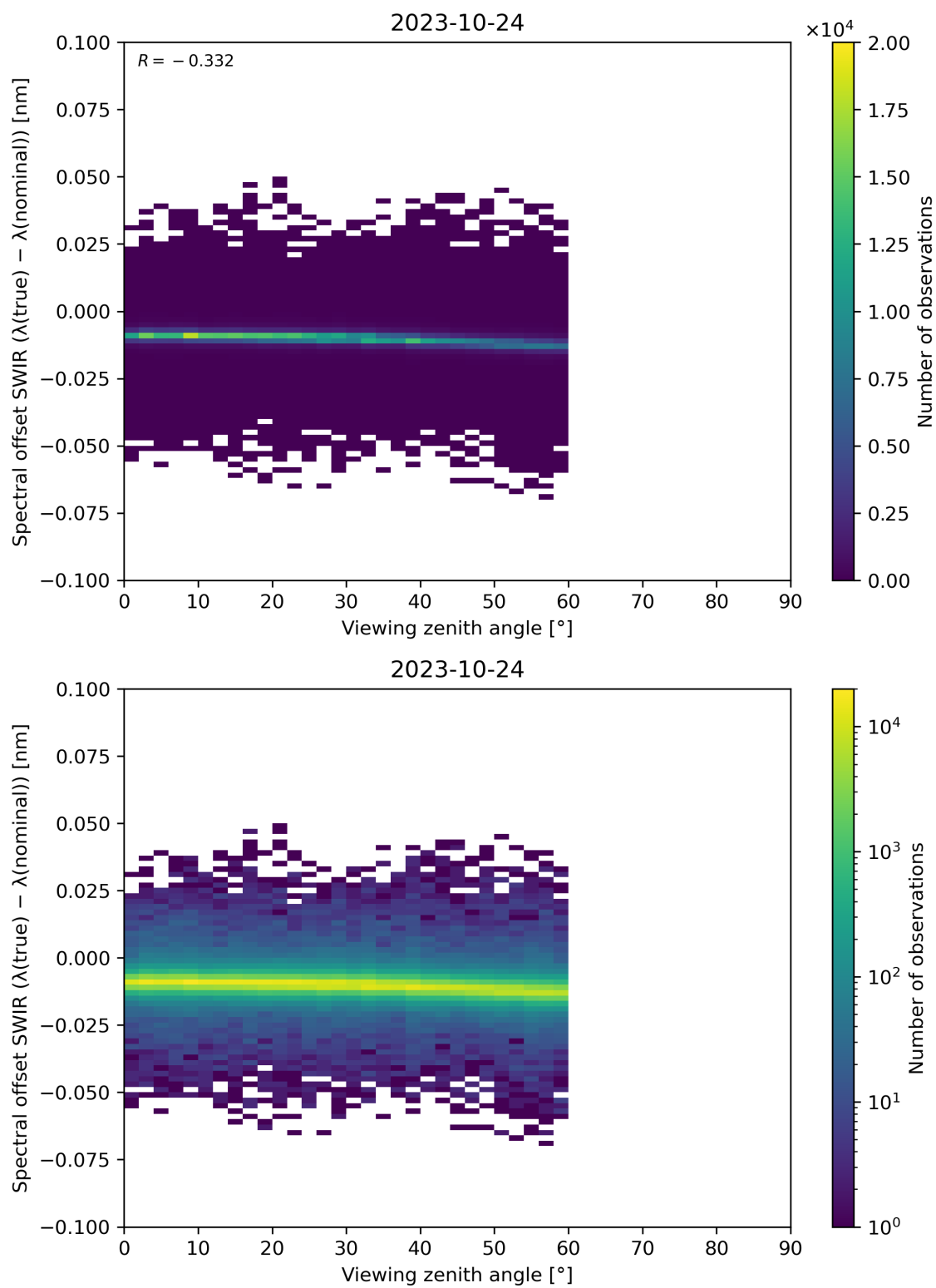
Figure 116: Scatter density plot of “Viewing zenith angle” against “Spectral offset SWIR ( \lambda(\text{true}) - \lambda(\text{nominal}) )” for 2023-10-23 to 2023-10-25.
