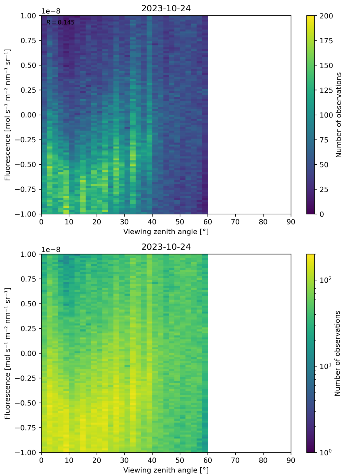
Figure 108: Scatter density plot of “Viewing zenith angle” against “Fluorescence” for 2023-10-23 to 2023-10-25.
