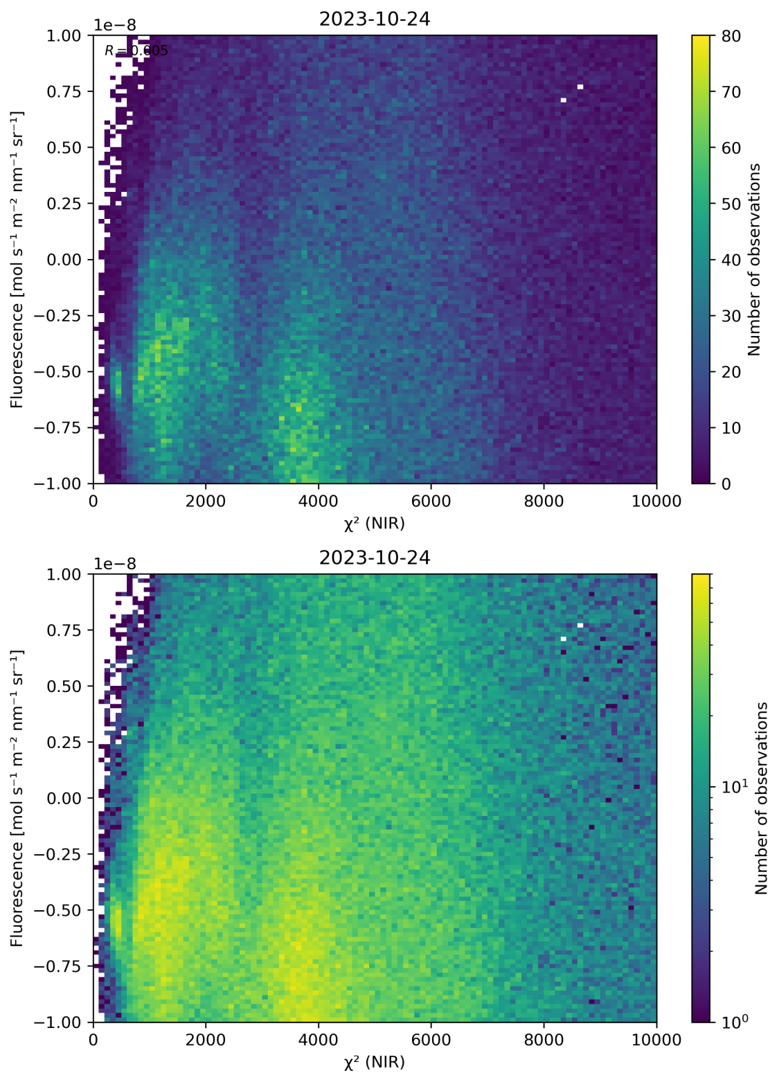
Figure 45: Scatter density plot of “ \chi^2 (NIR)” against “Fluorescence” for 2023-10-23 to 2023-10-25.
