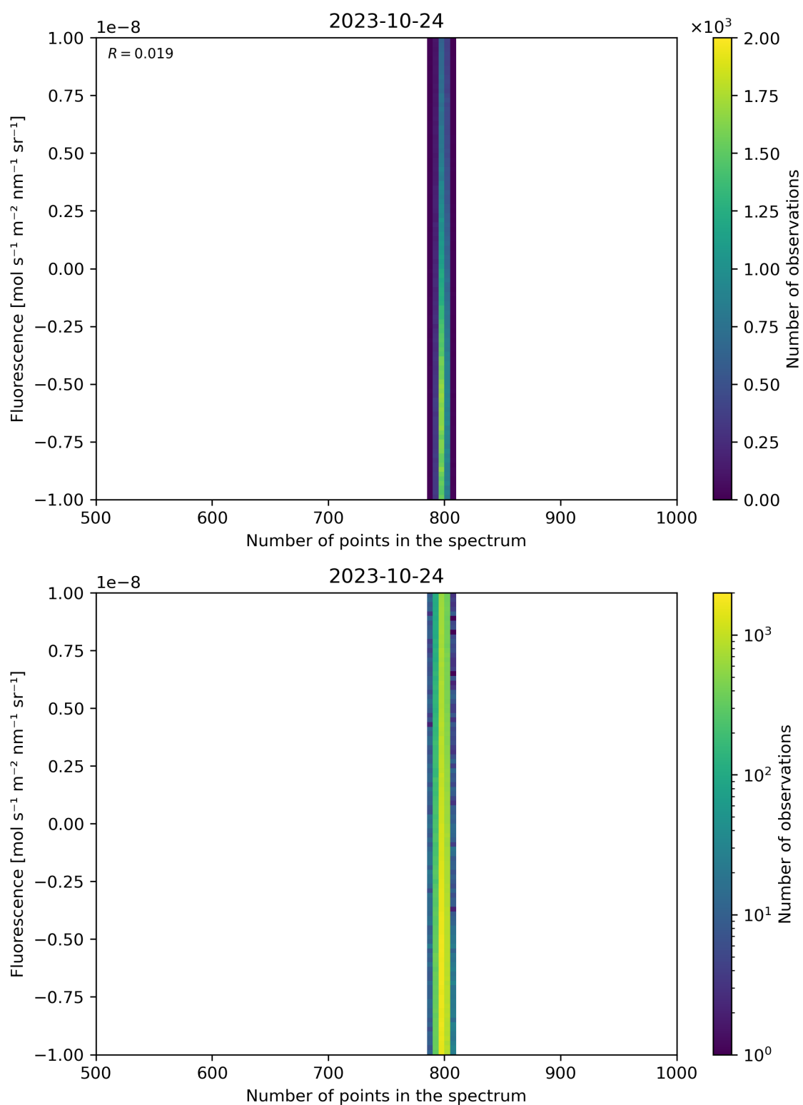
Figure 91: Scatter density plot of “Number of points in the spectrum” against “Fluorescence” for 2023-10-23 to 2023-10-25.
