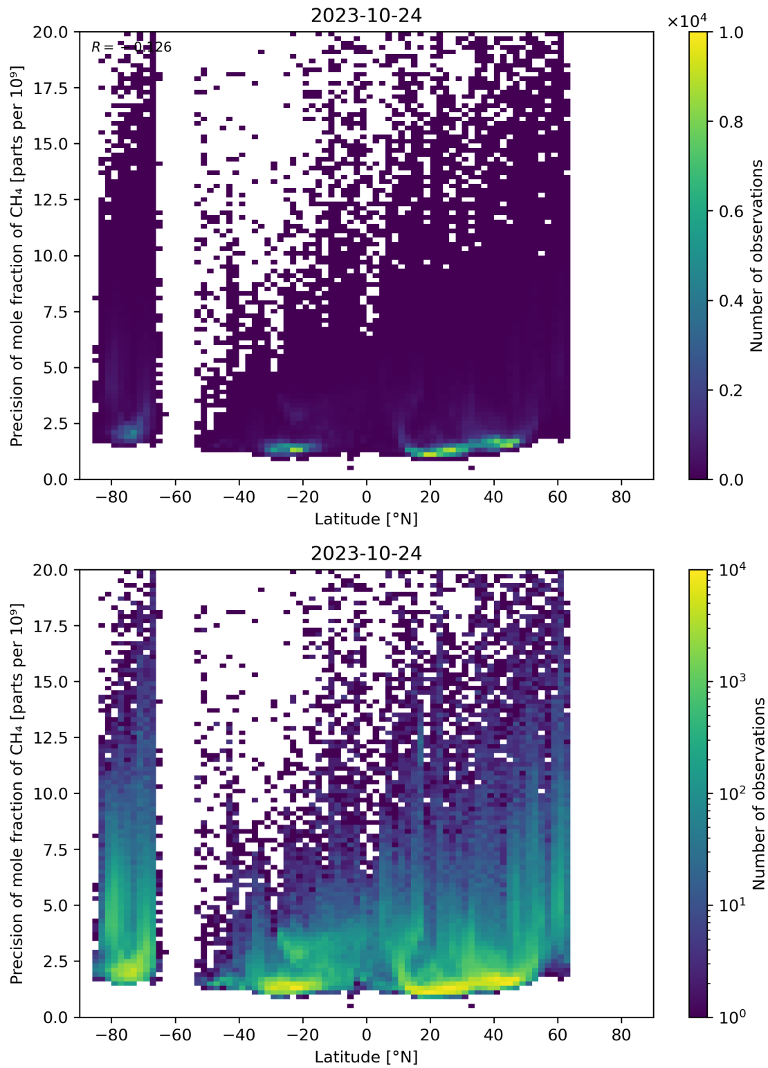
Figure 59: Scatter density plot of “Latitude” against “Precision of mole fraction of CH 4 ” for 2023-10-23 to 2023-10-25.
