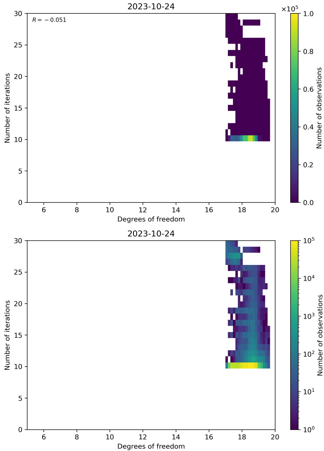
Figure 52: Scatter density plot of “Degrees of freedom” against “Number of iterations” for 2023-10-23 to 2023-10-25.
