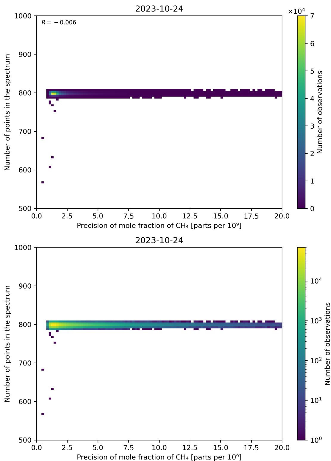
Figure 84: Scatter density plot of “Precision of mole fraction of CH 4 ” against “Number of points in the spectrum” for 2023-10-23 to 2023-10-25.
