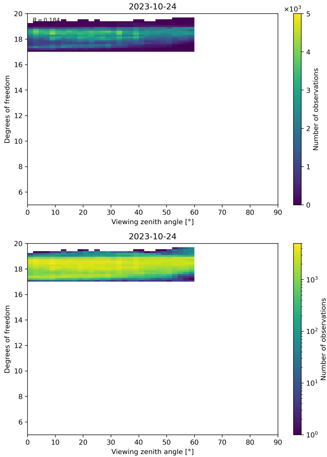
Figure 107: Scatter density plot of “Viewing zenith angle” against “Degrees of freedom” for 2023-10-23 to 2023-10-25.
