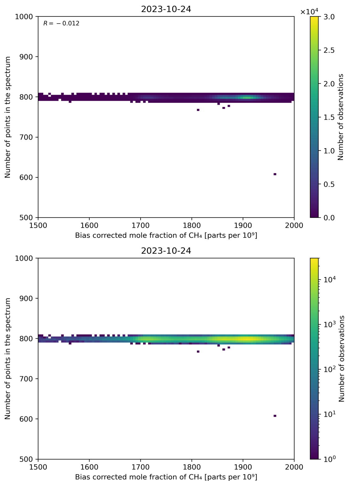
Figure 68: Scatter density plot of “Bias corrected mole fraction of CH 4 ” against “Number of points in the spectrum” for 2023-10-23 to 2023-10-25.
