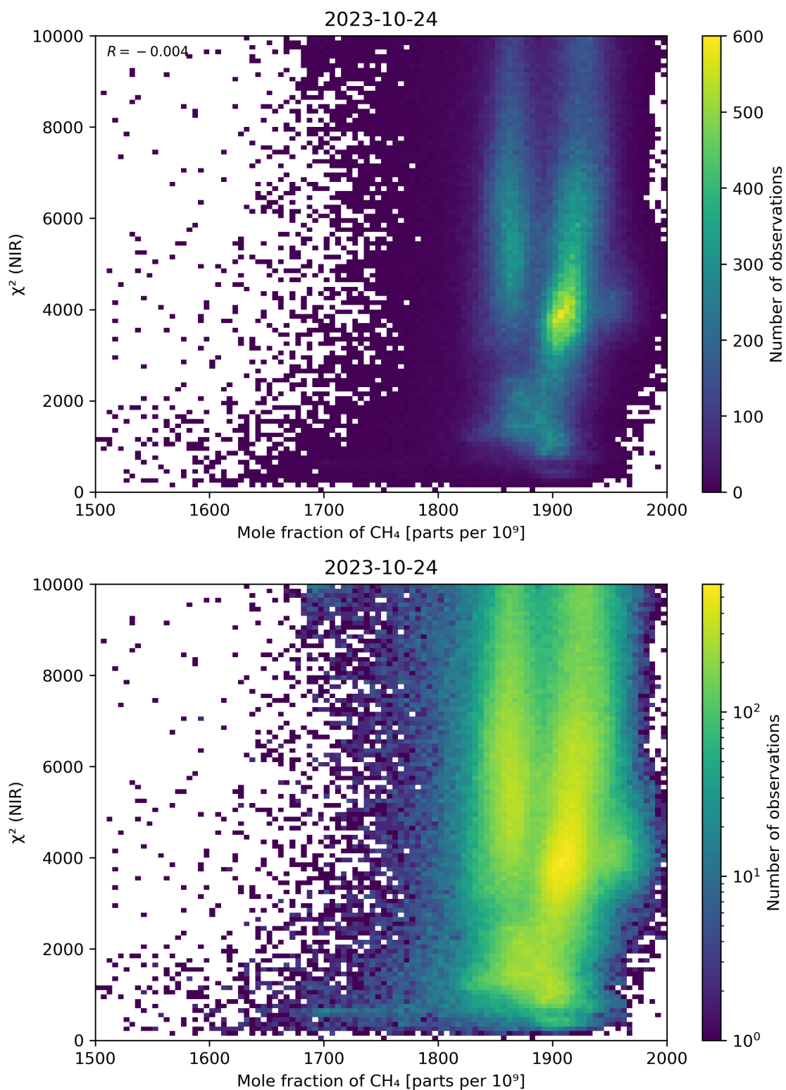
Figure 70: Scatter density plot of “Mole fraction of CH 4 ” against “ \chi^2 (NIR)” for 2023-10-23 to 2023-10-25.
