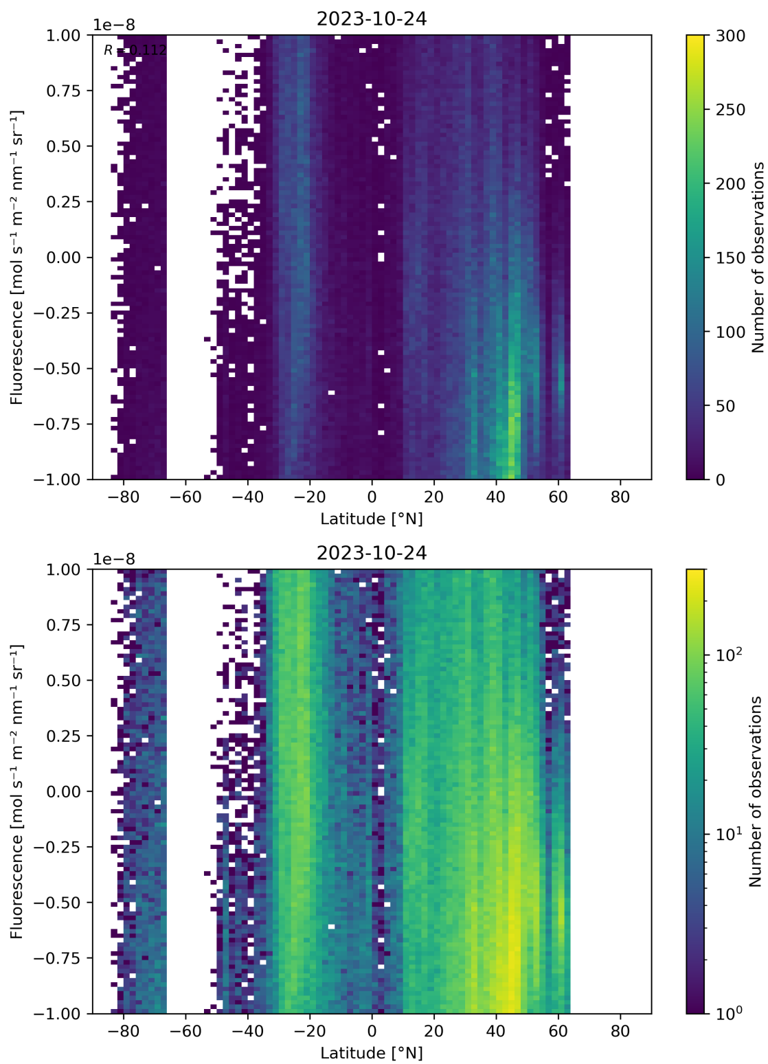
Figure 56: Scatter density plot of “Latitude” against “Fluorescence” for 2023-10-23 to 2023-10-25.
