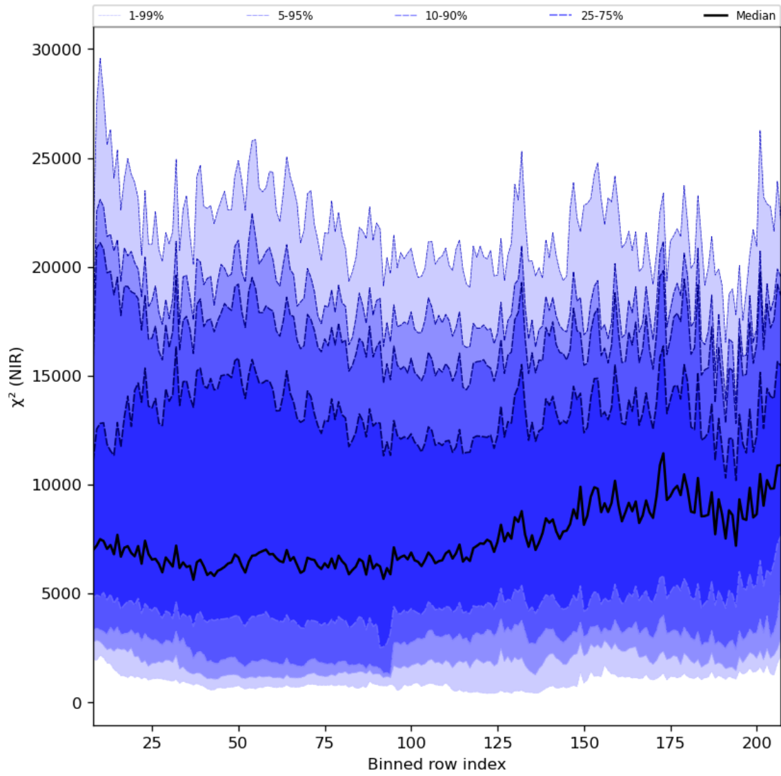
Figure 40: Along track statistics of " \chi^2 (NIR)" for 2023-10-23 to 2023-10-25
