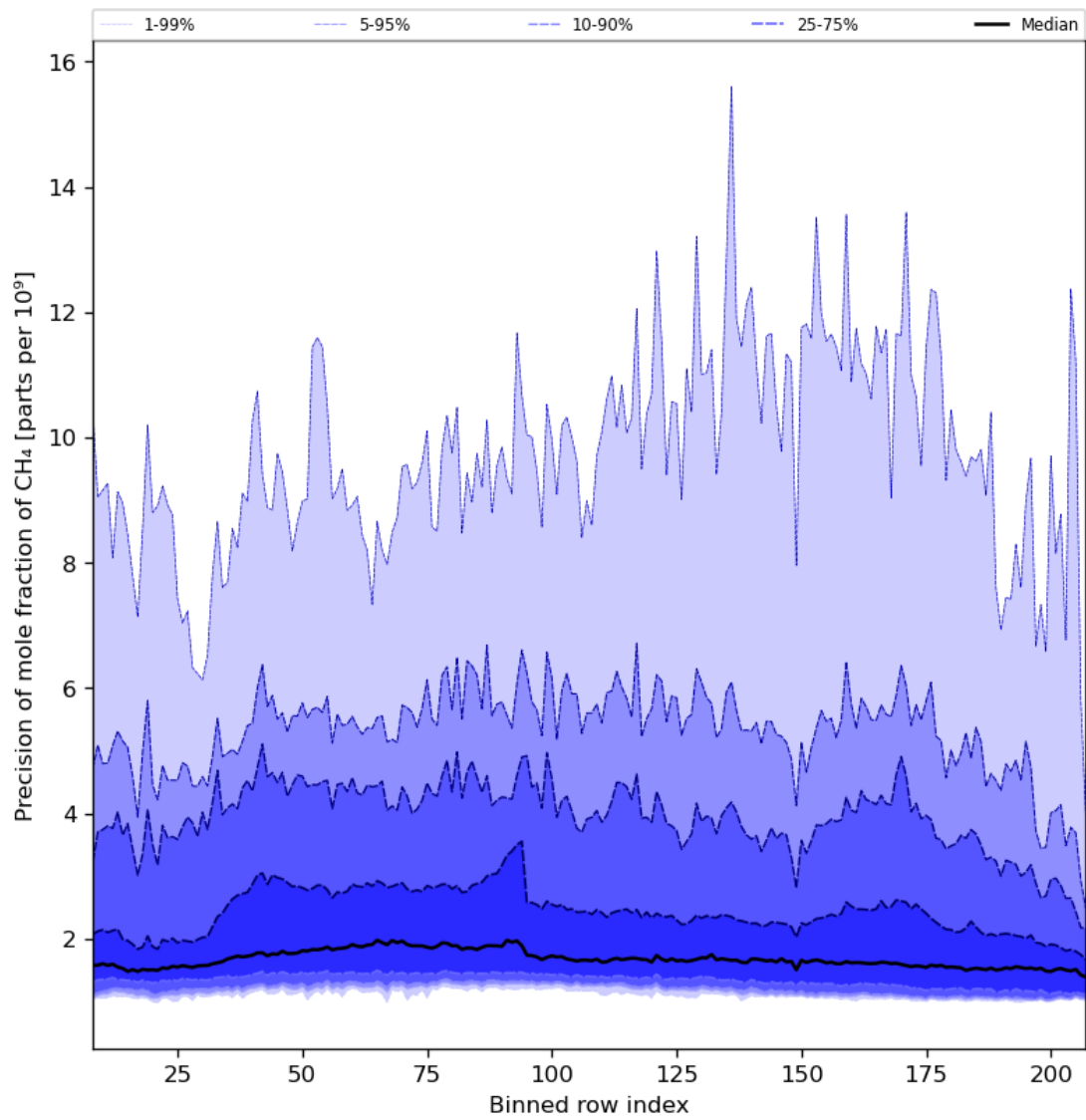
Figure 35: Along track statistics of “Precision of mole fraction of CH 4 ” for 2023-10-23 to 2023-10-25
