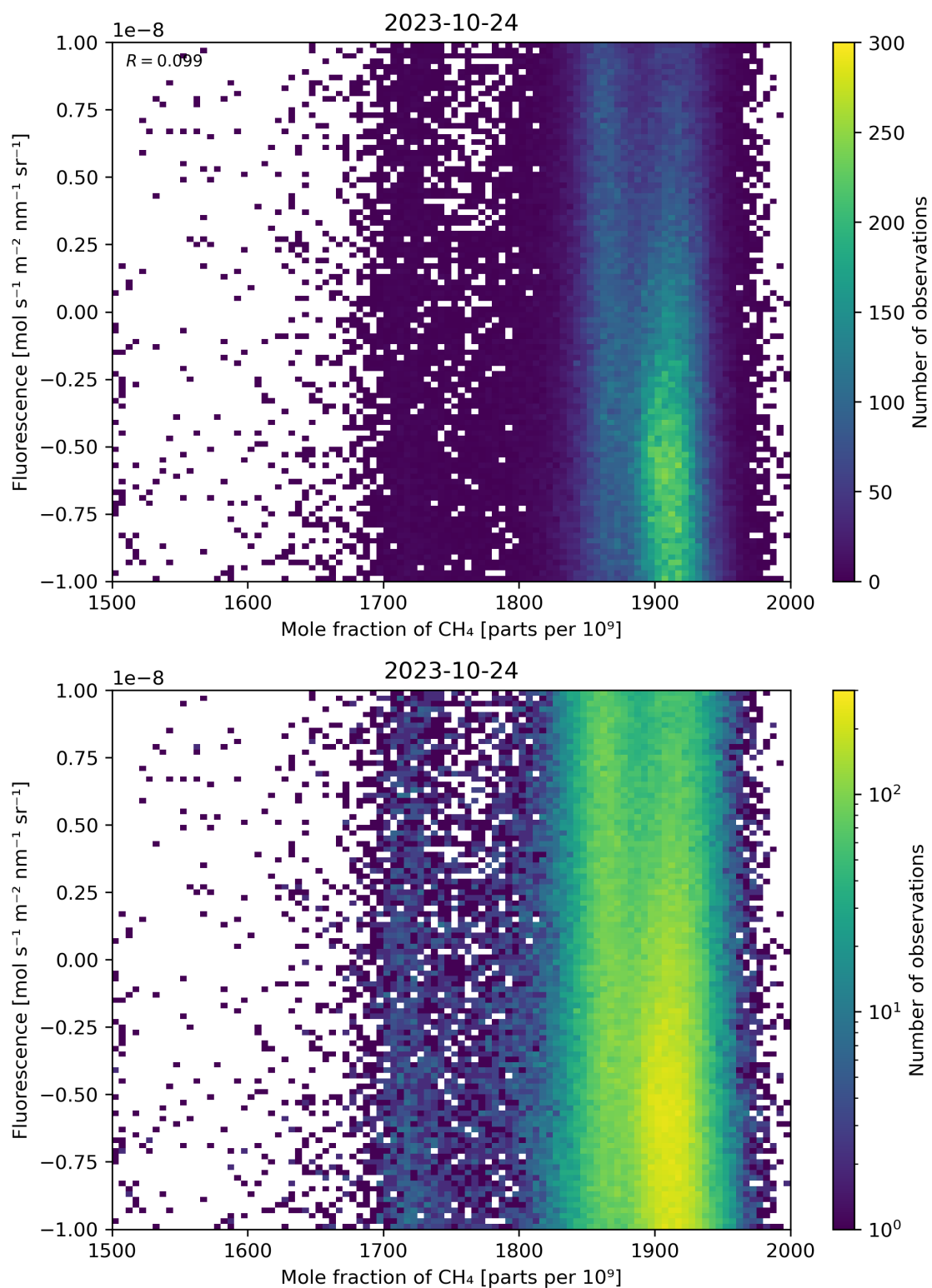
Figure 73: Scatter density plot of “Mole fraction of \text{CH}_4 ” against “Fluorescence” for 2023-10-23 to 2023-10-25.
