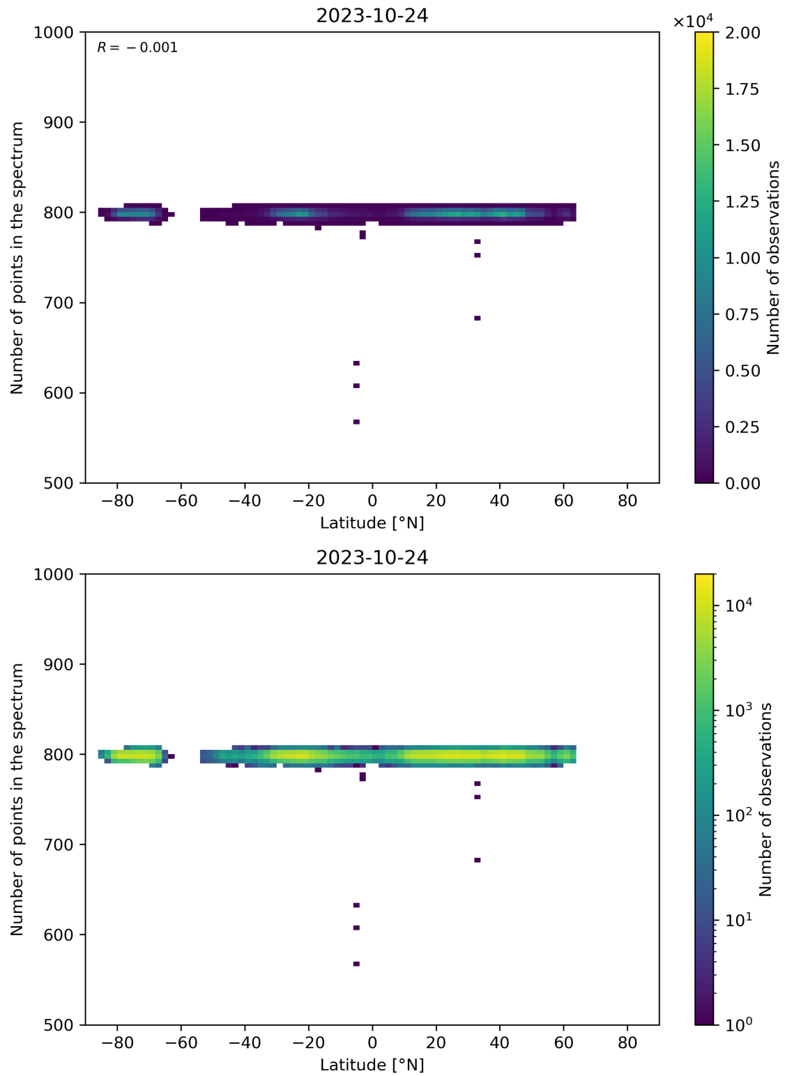
Figure 61: Scatter density plot of “Latitude” against “Number of points in the spectrum” for 2023-10-23 to 2023-10-25.
