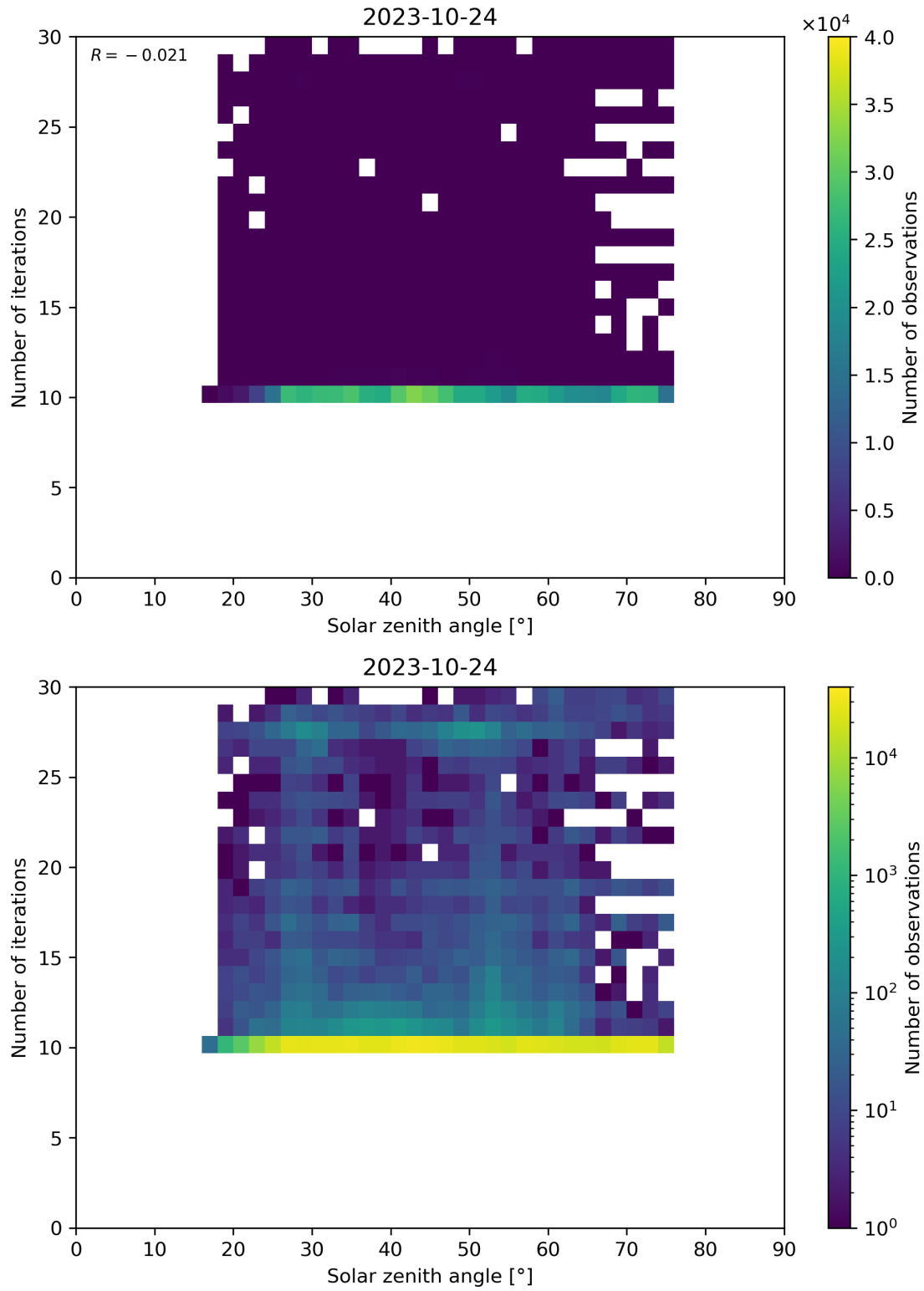
Figure 102: Scatter density plot of “Solar zenith angle” against “Number of iterations” for 2023-10-23 to 2023-10-25.
