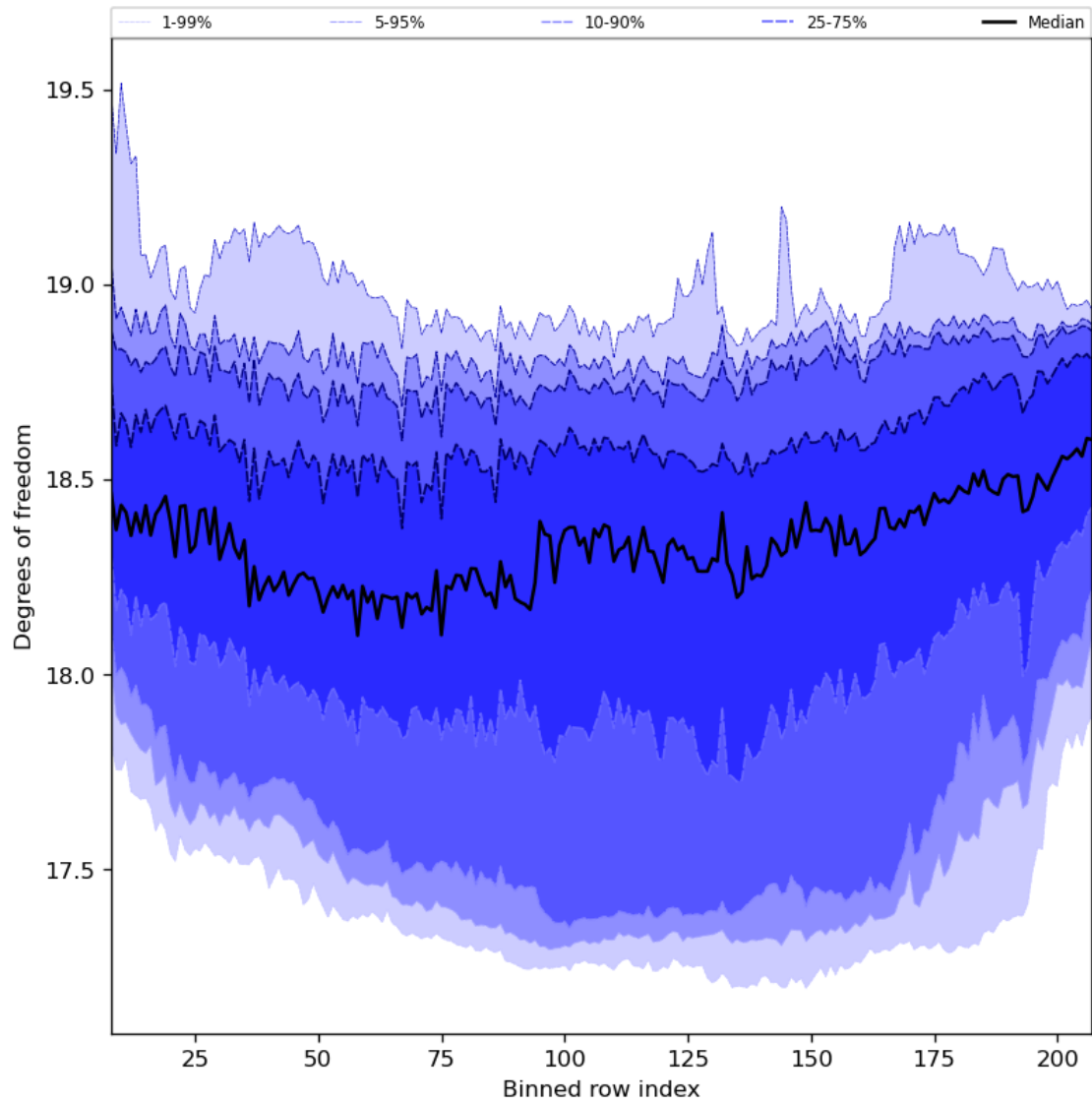
Figure 41: Along track statistics of “Degrees of freedom” for 2023-10-23 to 2023-10-25
