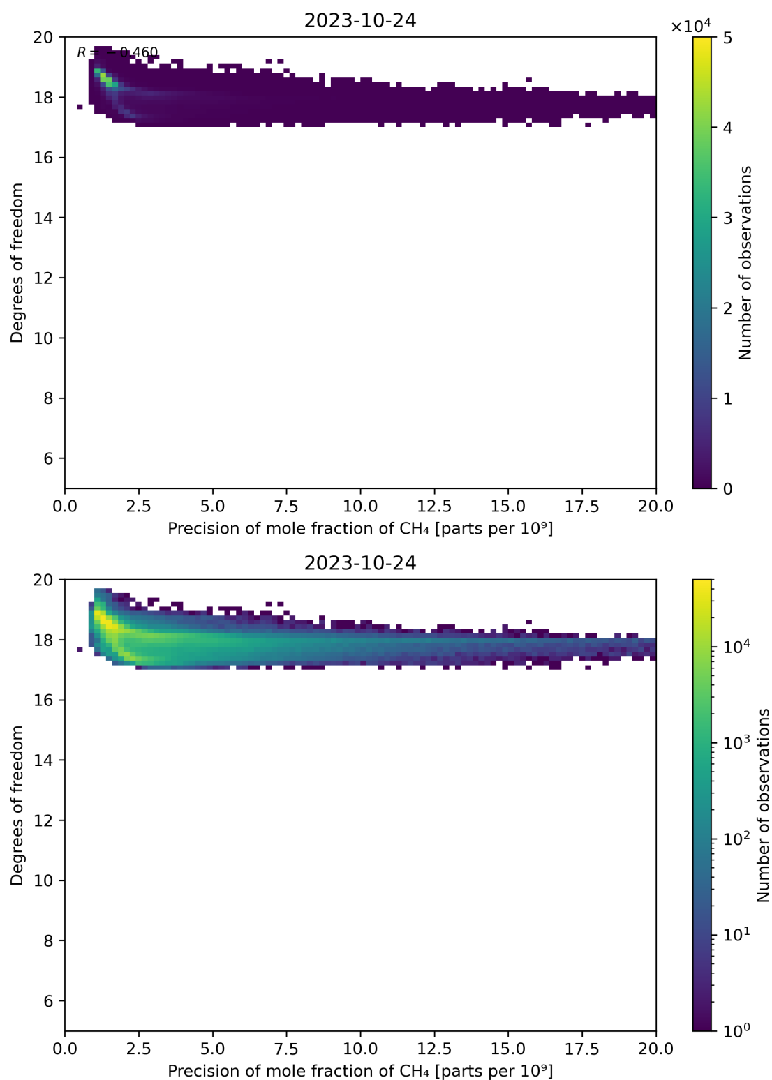
Figure 80: Scatter density plot of “Precision of mole fraction of CH 4 ” against “Degrees of freedom” for 2023-10-23 to 2023-10-25.
