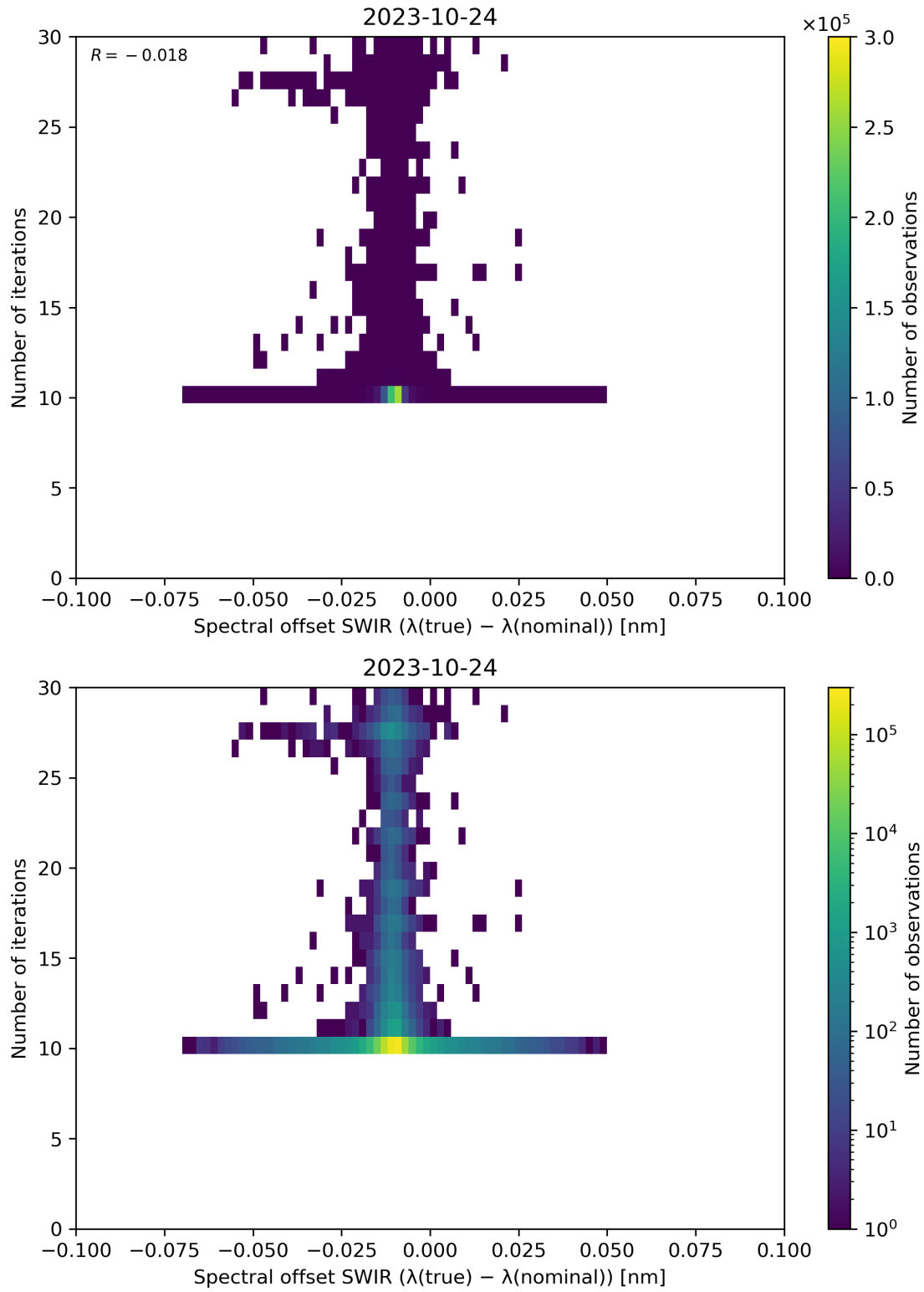
Figure 121: Scatter density plot of “Spectral offset SWIR ( \lambda(\text{true}) - \lambda(\text{nominal}) )” against “Number of iterations” for 2023-10-23 to 2023-10-25.
