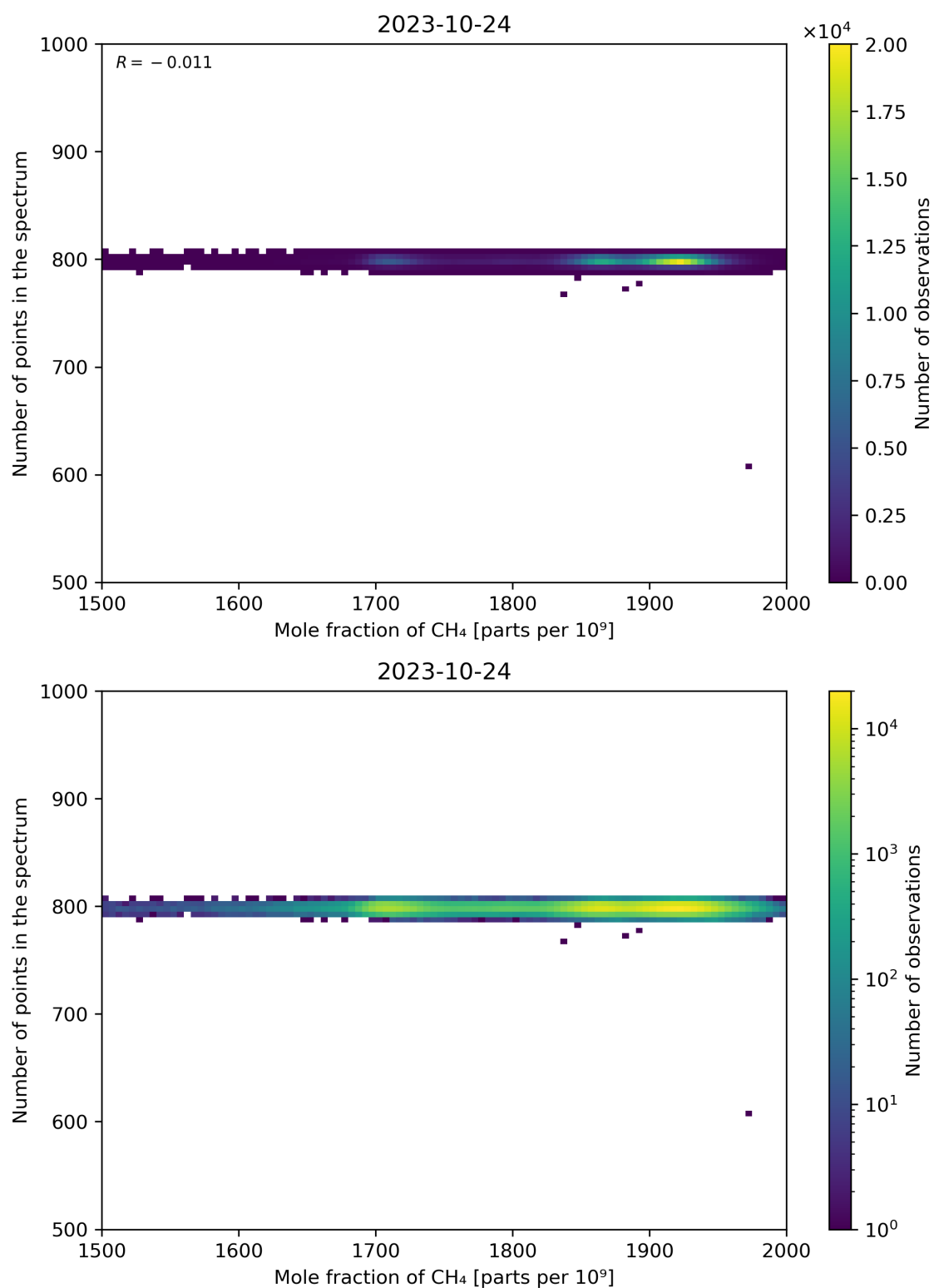
Figure 77: Scatter density plot of “Mole fraction of CH 4 ” against “Number of points in the spectrum” for 2023-10-23 to 2023-10-25.
