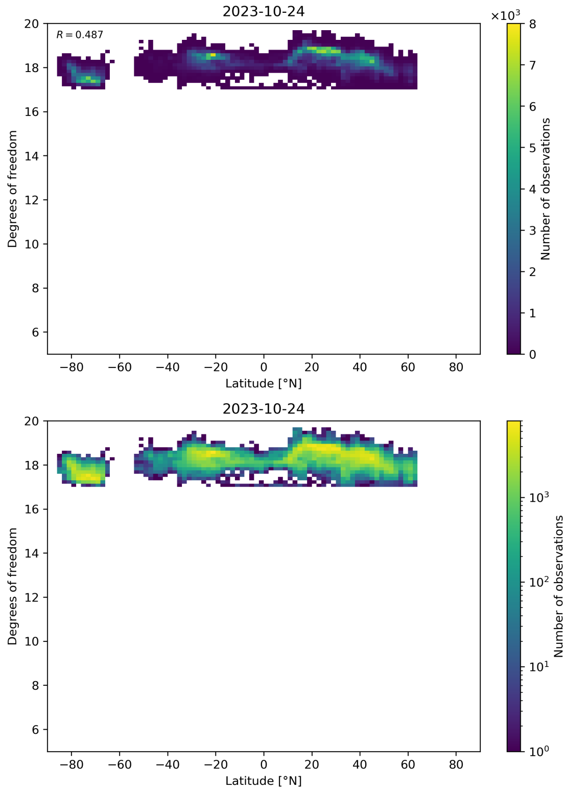
Figure 55: Scatter density plot of “Latitude” against “Degrees of freedom” for 2023-10-23 to 2023-10-25.
