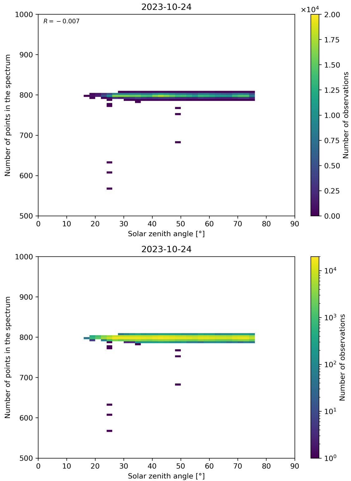
Figure 103: Scatter density plot of “Solar zenith angle” against “Number of points in the spectrum” for 2023-10-23 to 2023-10-25.
