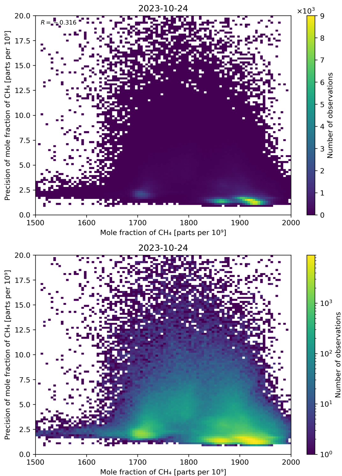
Figure 75: Scatter density plot of “Mole fraction of CH 4 ” against “Precision of mole fraction of CH 4 ” for 2023-10-23 to 2023-10-25.
