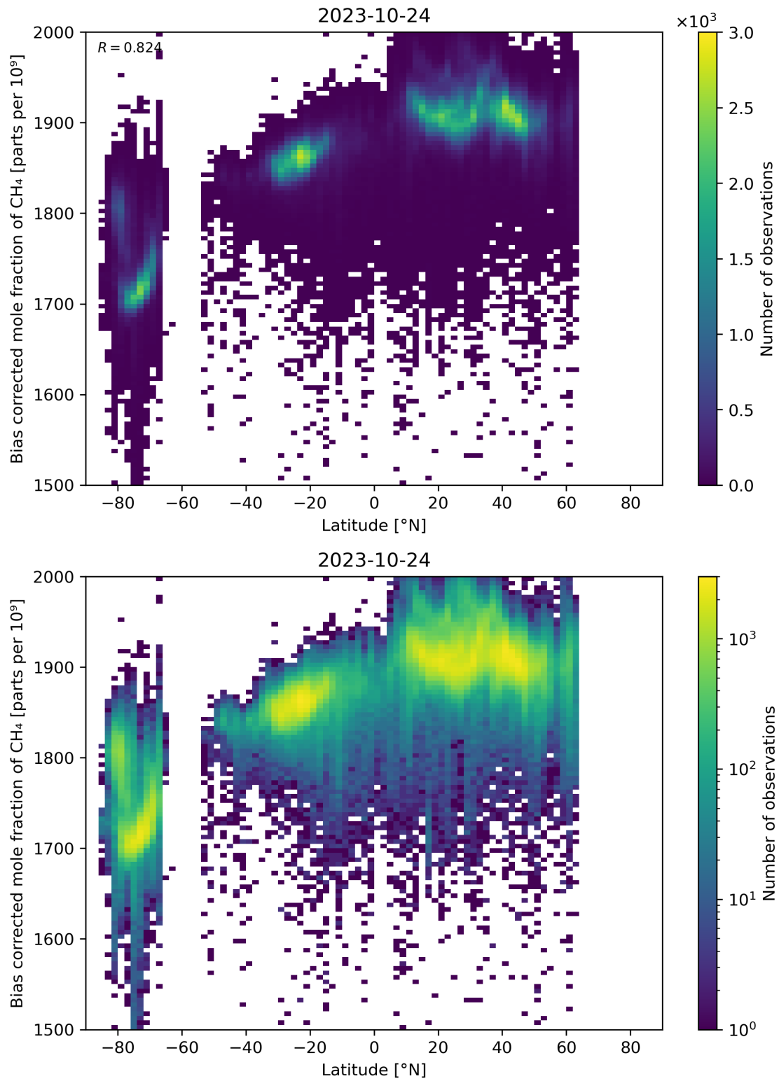
Figure 58: Scatter density plot of “Latitude” against “Bias corrected mole fraction of \text{CH}_4 ” for 2023-10-23 to 2023-10-25.
