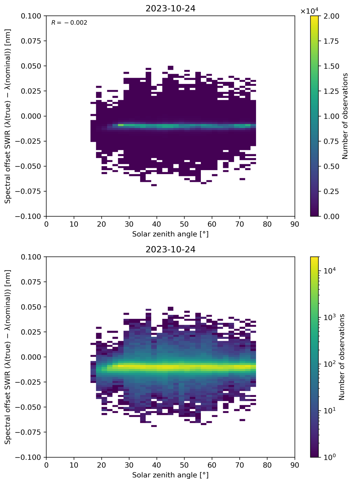
Figure 104: Scatter density plot of “Solar zenith angle” against “Spectral offset SWIR ( \lambda(\text{true}) - \lambda(\text{nominal}) )” for 2023-10-23 to 2023-10-25.
