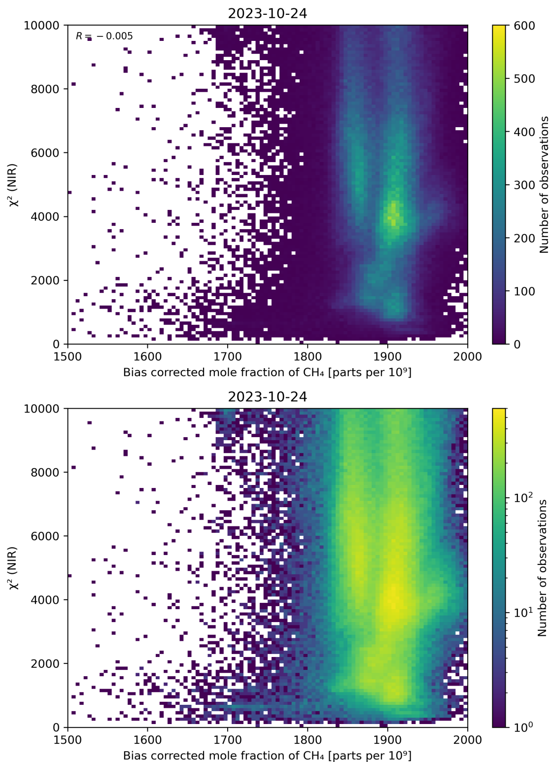
Figure 63: Scatter density plot of “Bias corrected mole fraction of CH 4 ” against “ \chi^2 (NIR)” for 2023-10-23 to 2023-10-25.
