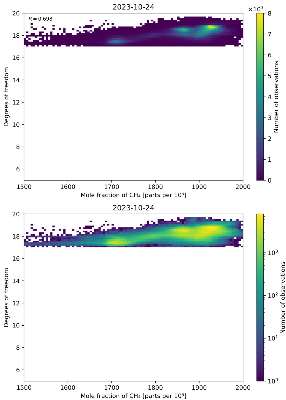
Figure 72: Scatter density plot of “Mole fraction of CH 4 ” against “Degrees of freedom” for 2023-10-23 to 2023-10-25.
