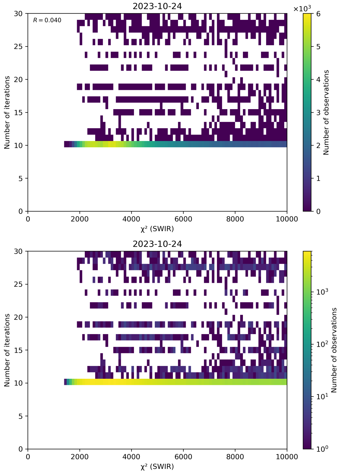
Figure 50: Scatter density plot of “ \chi^2 (SWIR)” against “Number of iterations” for 2023-10-23 to 2023-10-25.
