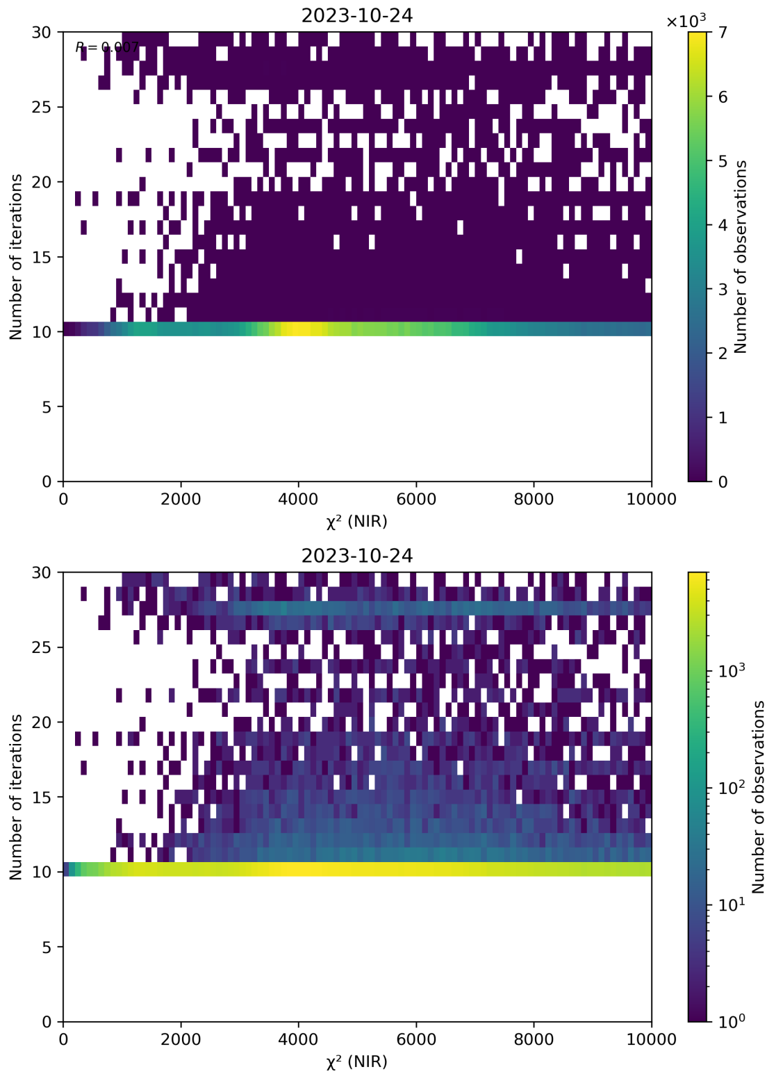
Figure 46: Scatter density plot of " \chi^2 (NIR)" against "Number of iterations" for 2023-10-23 to 2023-10-25.
