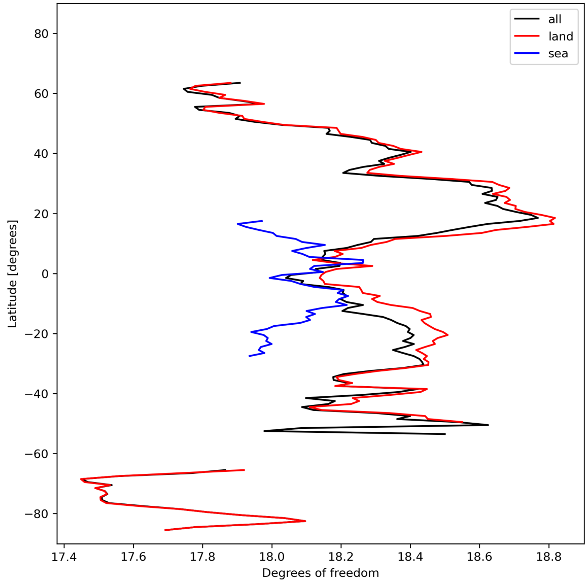
Figure 19: Zonal average of “Degrees of freedom” for 2023-10-23 to 2023-10-25.
