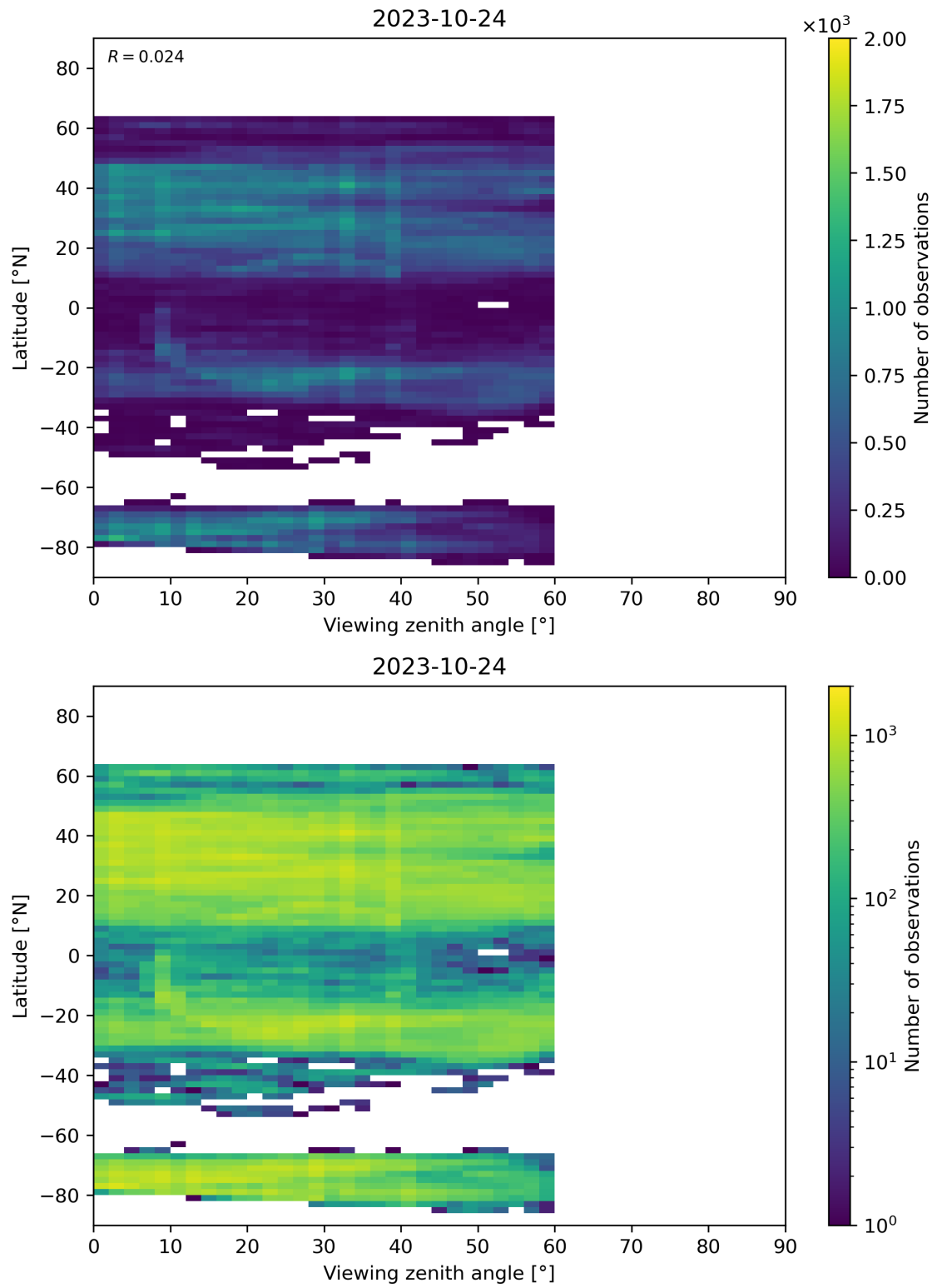
Figure 109: Scatter density plot of “Viewing zenith angle” against “Latitude” for 2023-10-23 to 2023-10-25.
