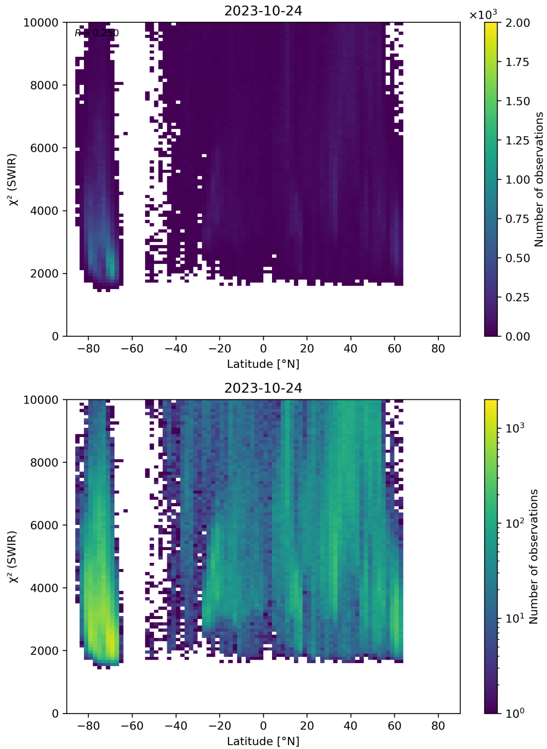
Figure 54: Scatter density plot of “Latitude” against “ \chi^2 (SWIR)” for 2023-10-23 to 2023-10-25.
