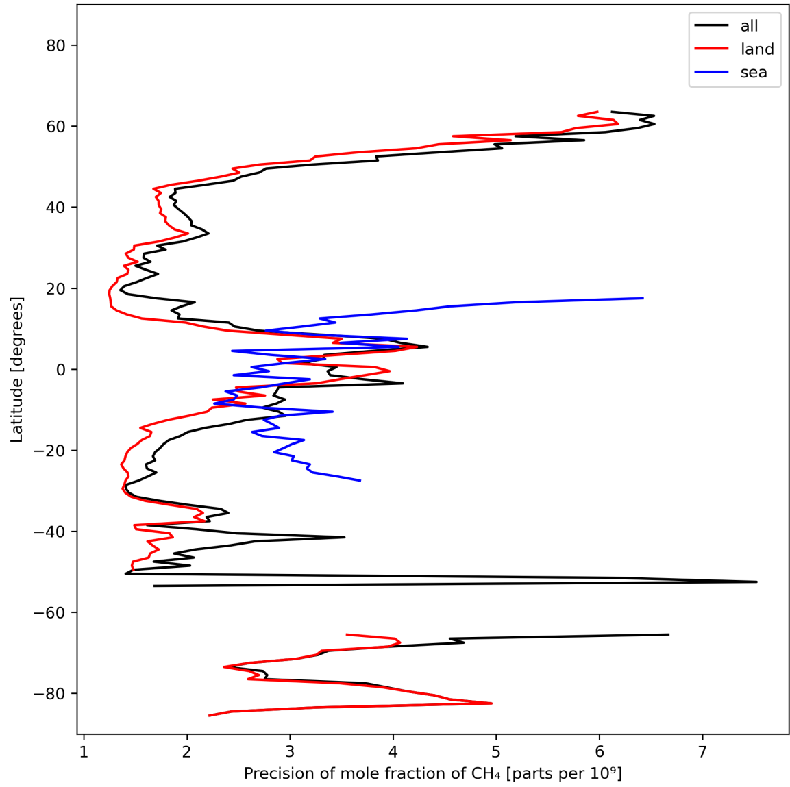
Figure 13: Zonal average of “Precision of mole fraction of CH 4 ” for 2023-10-23 to 2023-10-25.
