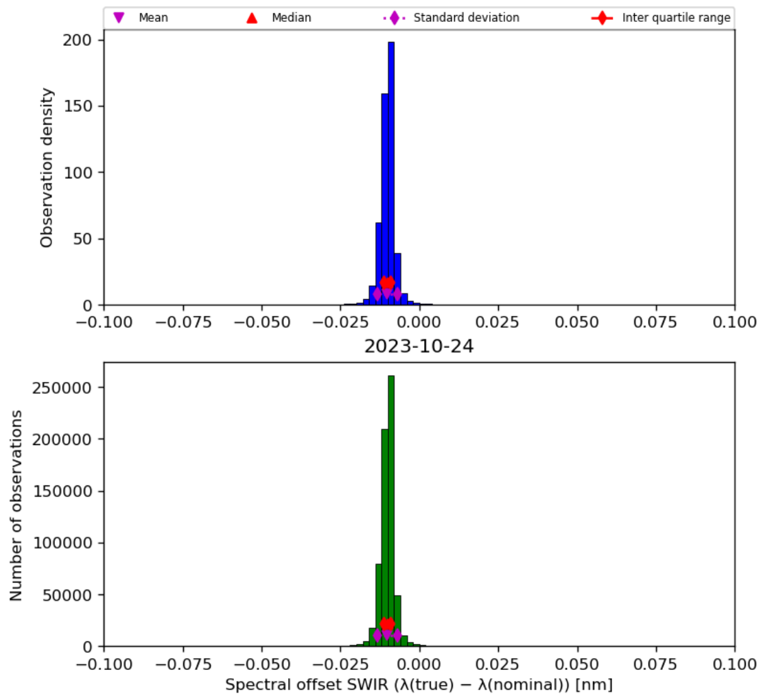
Figure 27: Histogram of “Spectral offset SWIR ( \lambda(\text{true}) - \lambda(\text{nominal}) )” for 2023-10-23 to 2023-10-25
