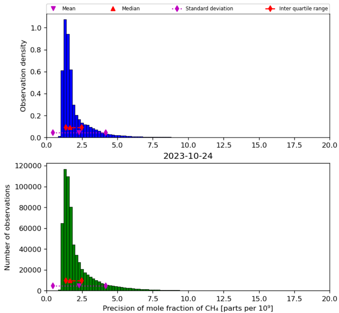
Figure 24: Histogram of “Precision of mole fraction of CH 4 ” for 2023-10-23 to 2023-10-25
