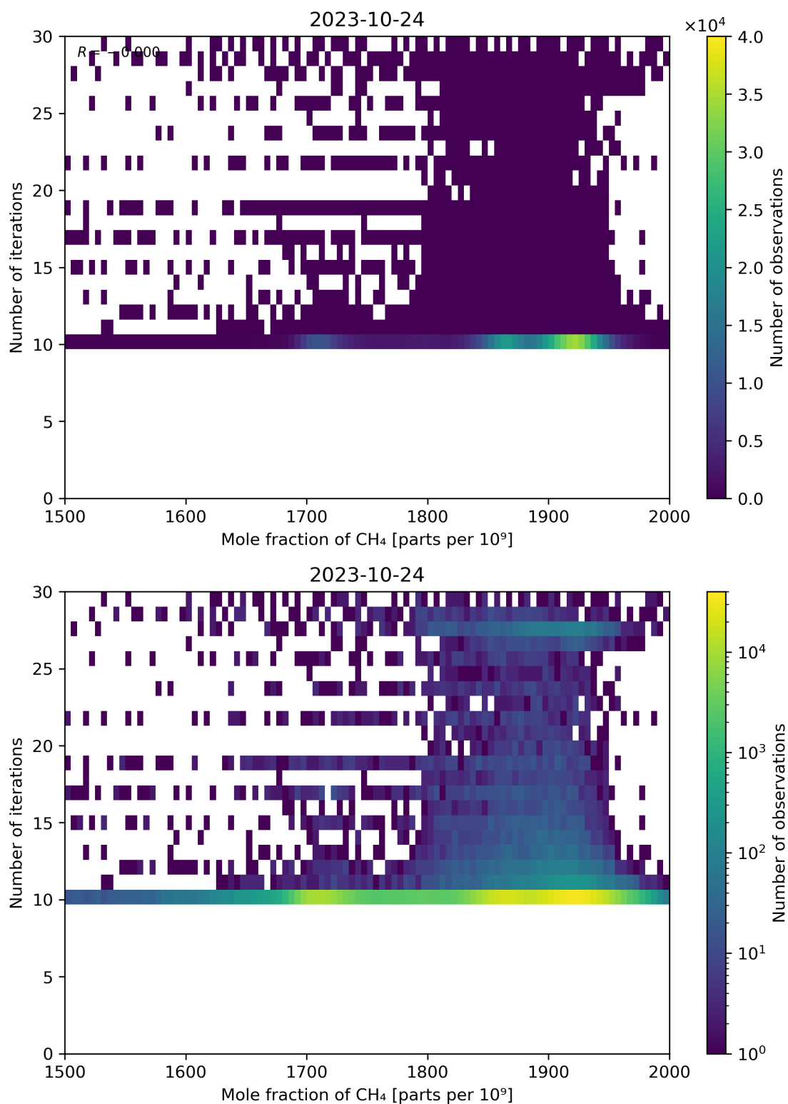
Figure 76: Scatter density plot of “Mole fraction of CH 4 ” against “Number of iterations” for 2023-10-23 to 2023-10-25.
