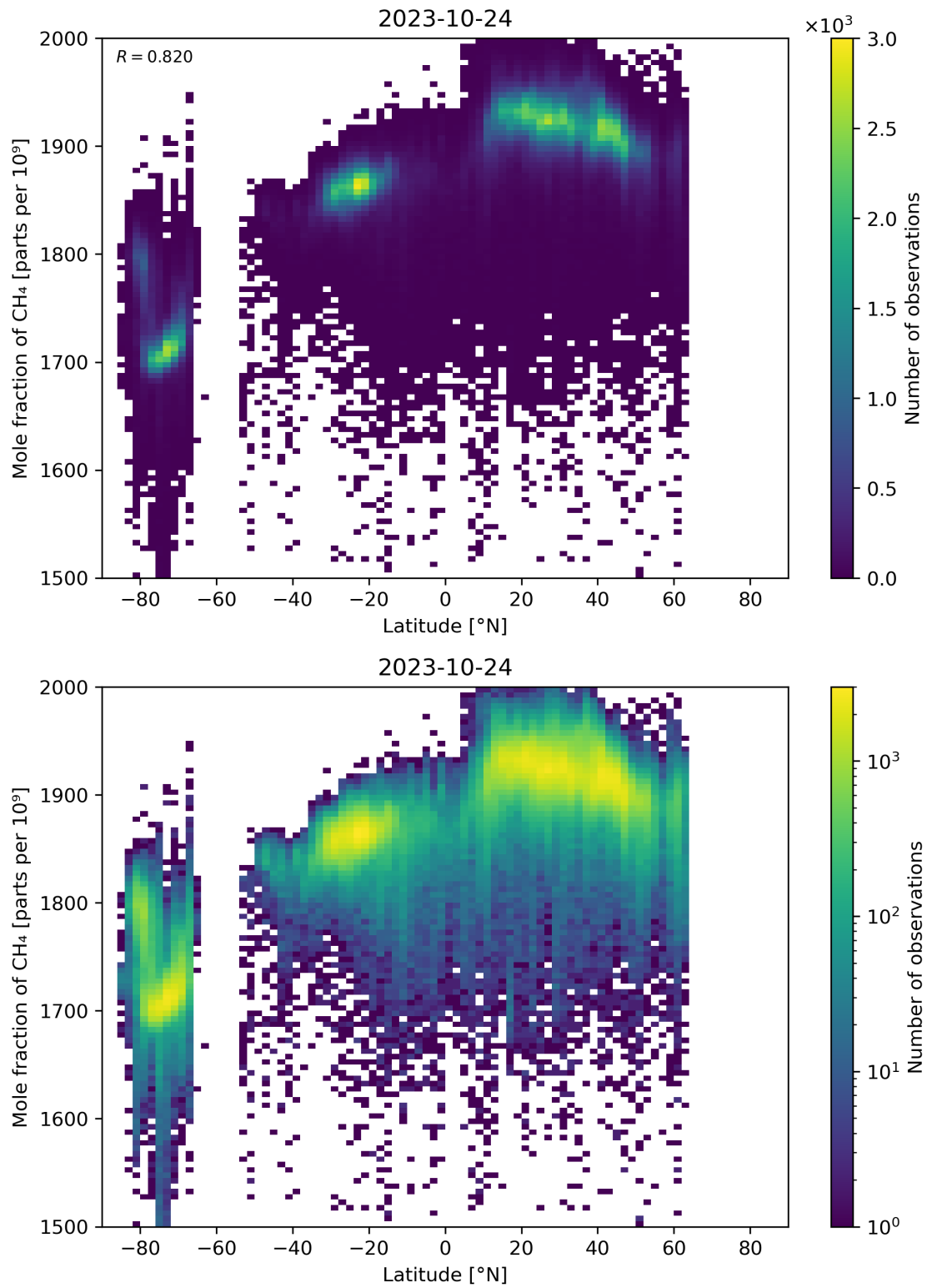
Figure 57: Scatter density plot of “Latitude” against “Mole fraction of \text{CH}_4 ” for 2023-10-23 to 2023-10-25.
