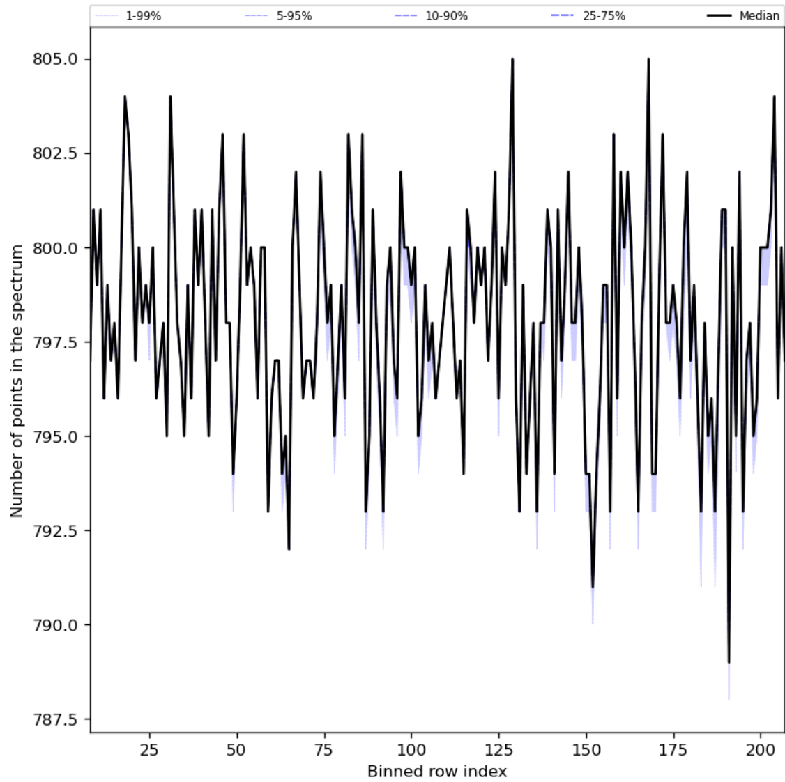
Figure 37: Along track statistics of “Number of points in the spectrum” for 2023-10-23 to 2023-10-25
