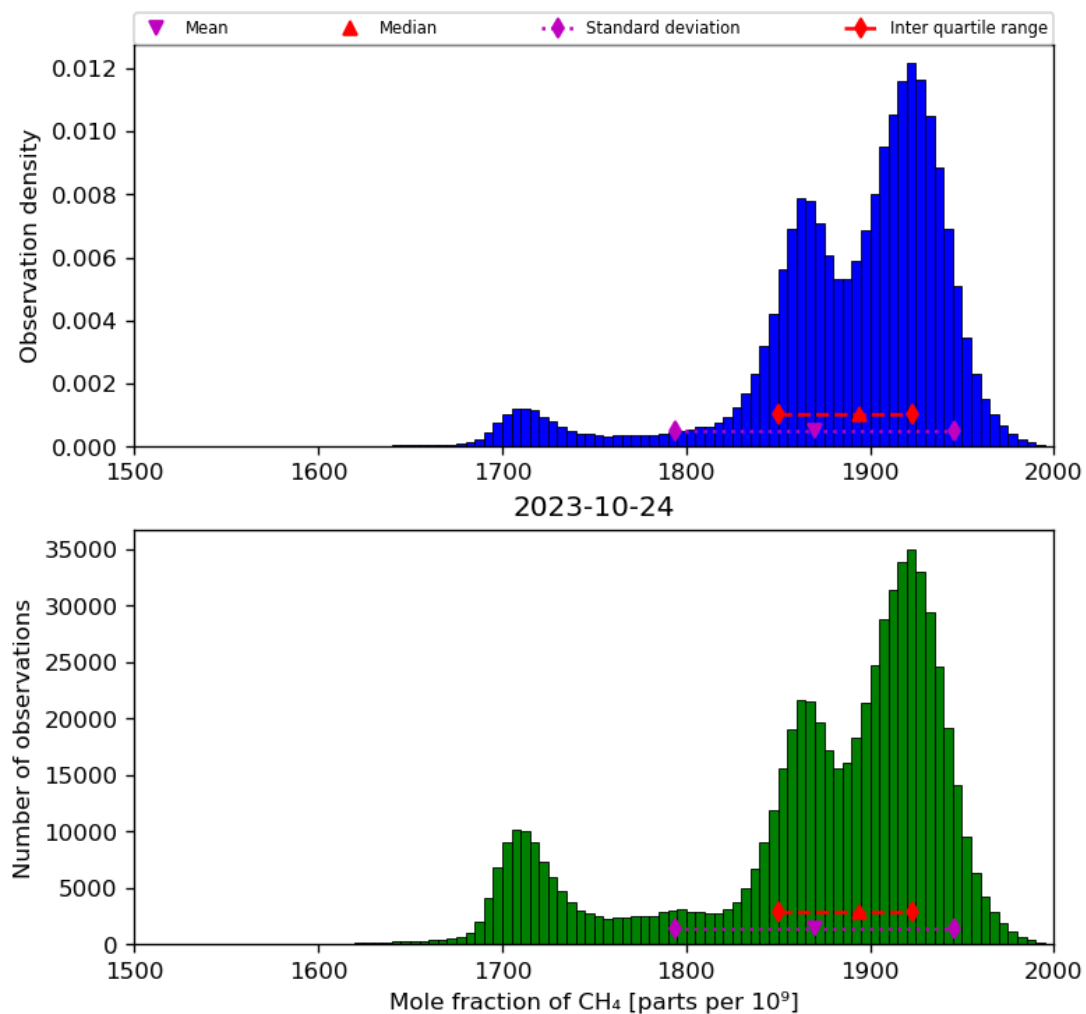
Figure 23: Histogram of “Mole fraction of CH 4 ” for 2023-10-23 to 2023-10-25
