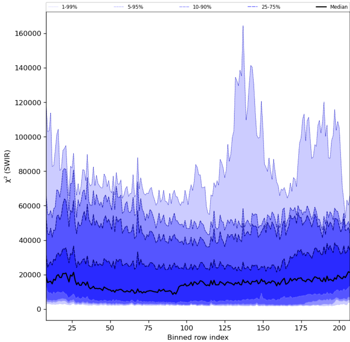
Figure 39: Along track statistics of “ \chi^2 (SWIR)” for 2023-10-23 to 2023-10-25
