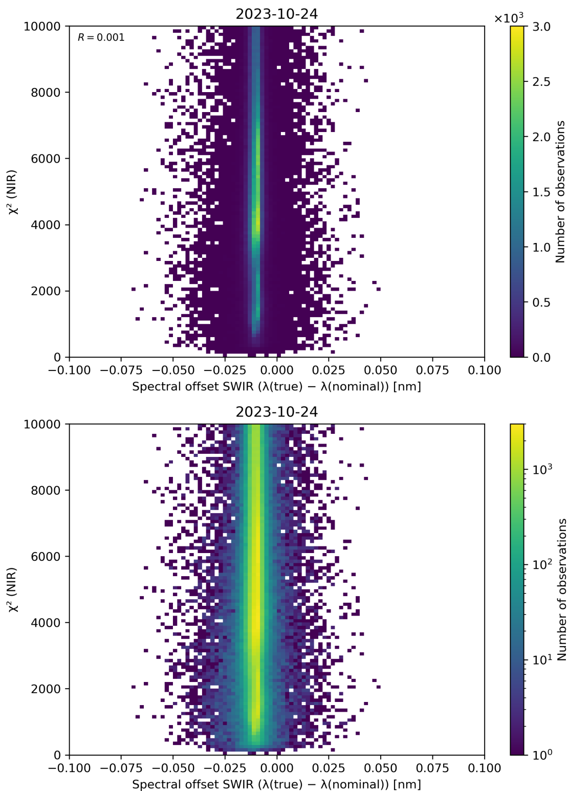
Figure 117: Scatter density plot of “Spectral offset SWIR ( \lambda(\text{true}) - \lambda(\text{nominal}) )” against “ \chi^2 (NIR)” for 2023-10-23 to 2023-10-25.
