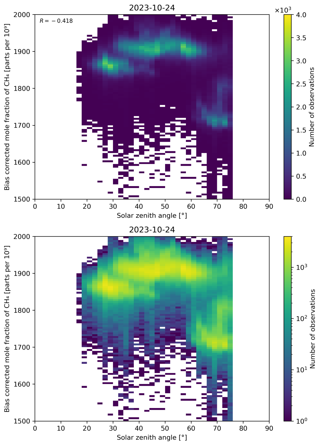
Figure 100: Scatter density plot of “Solar zenith angle” against “Bias corrected mole fraction of \text{CH}_4 ” for 2023-10-23 to 2023-10-25.
