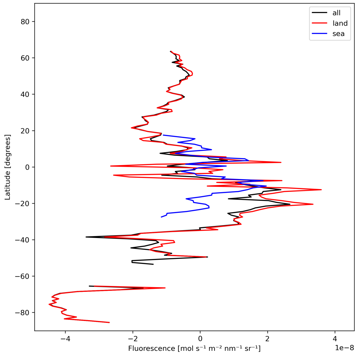
Figure 21: Zonal average of “Fluorescence” for 2023-10-23 to 2023-10-25.
