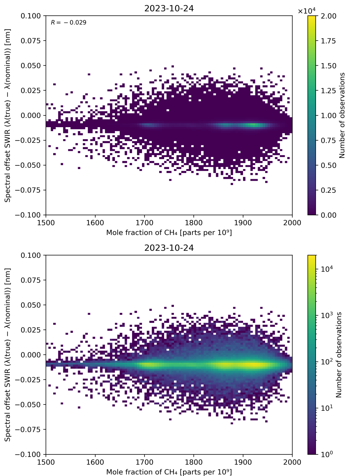
Figure 86: Scatter density plot of “Mole fraction of CH 4 ” against “Spectral offset SWIR ( \lambda(\text{true}) - \lambda(\text{nominal}) )” for 2023-10-23 to 2023-10-25.
