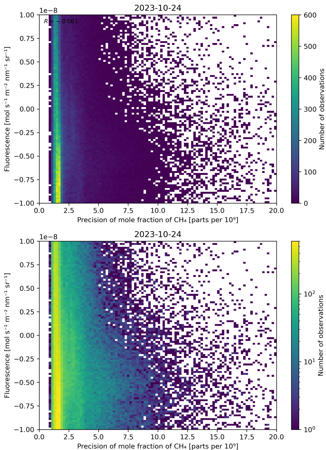
Figure 81: Scatter density plot of “Precision of mole fraction of \text{CH}_4 ” against “Fluorescence” for 2023-10-23 to 2023-10-25.
