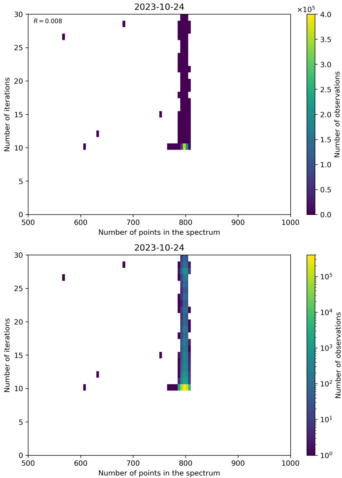
Figure 92: Scatter density plot of “Number of points in the spectrum” against “Number of iterations” for 2023-10-23 to 2023-10-25.
