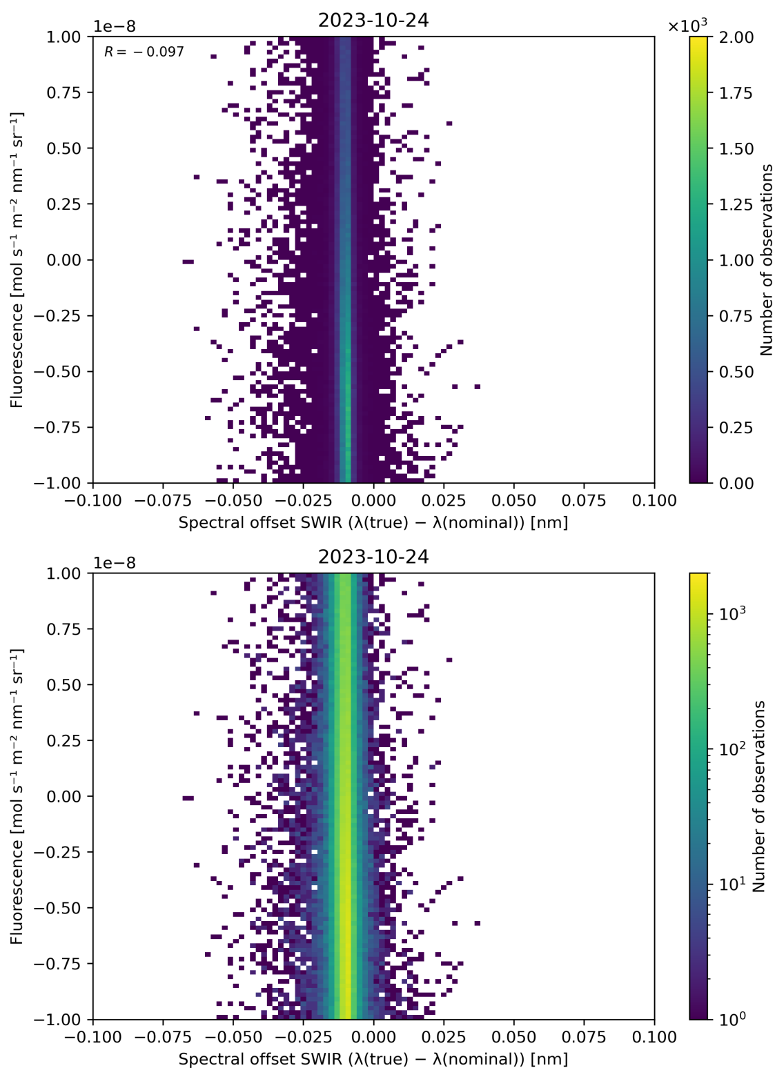
Figure 120: Scatter density plot of “Spectral offset SWIR ( \lambda(\text{true}) - \lambda(\text{nominal}) )” against “Fluorescence” for 2023-10-23 to 2023-10-25.
