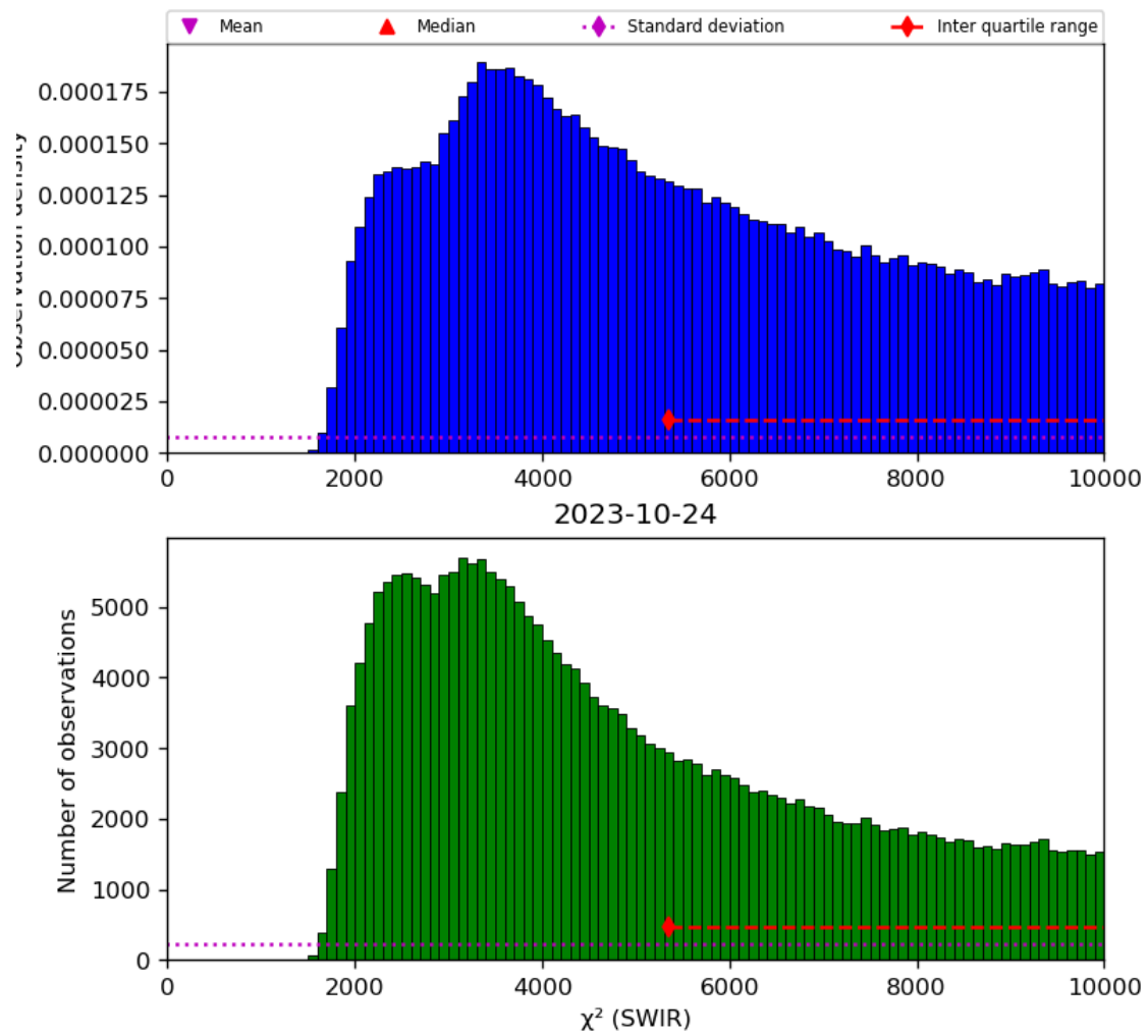
Figure 28: Histogram of “ \chi^2 (SWIR)” for 2023-10-23 to 2023-10-25
