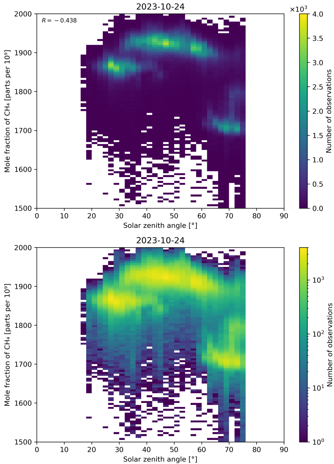
Figure 99: Scatter density plot of “Solar zenith angle” against “Mole fraction of CH 4 ” for 2023-10-23 to 2023-10-25.
