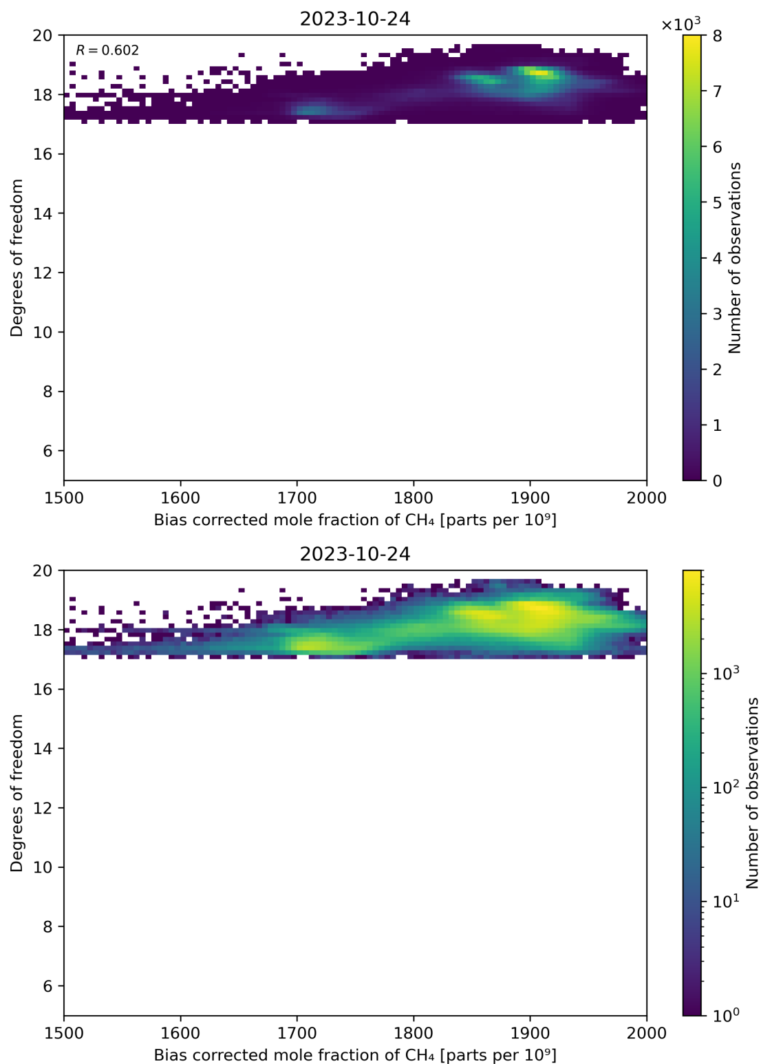
Figure 65: Scatter density plot of “Bias corrected mole fraction of CH 4 ” against “Degrees of freedom” for 2023-10-23 to 2023-10-25.
