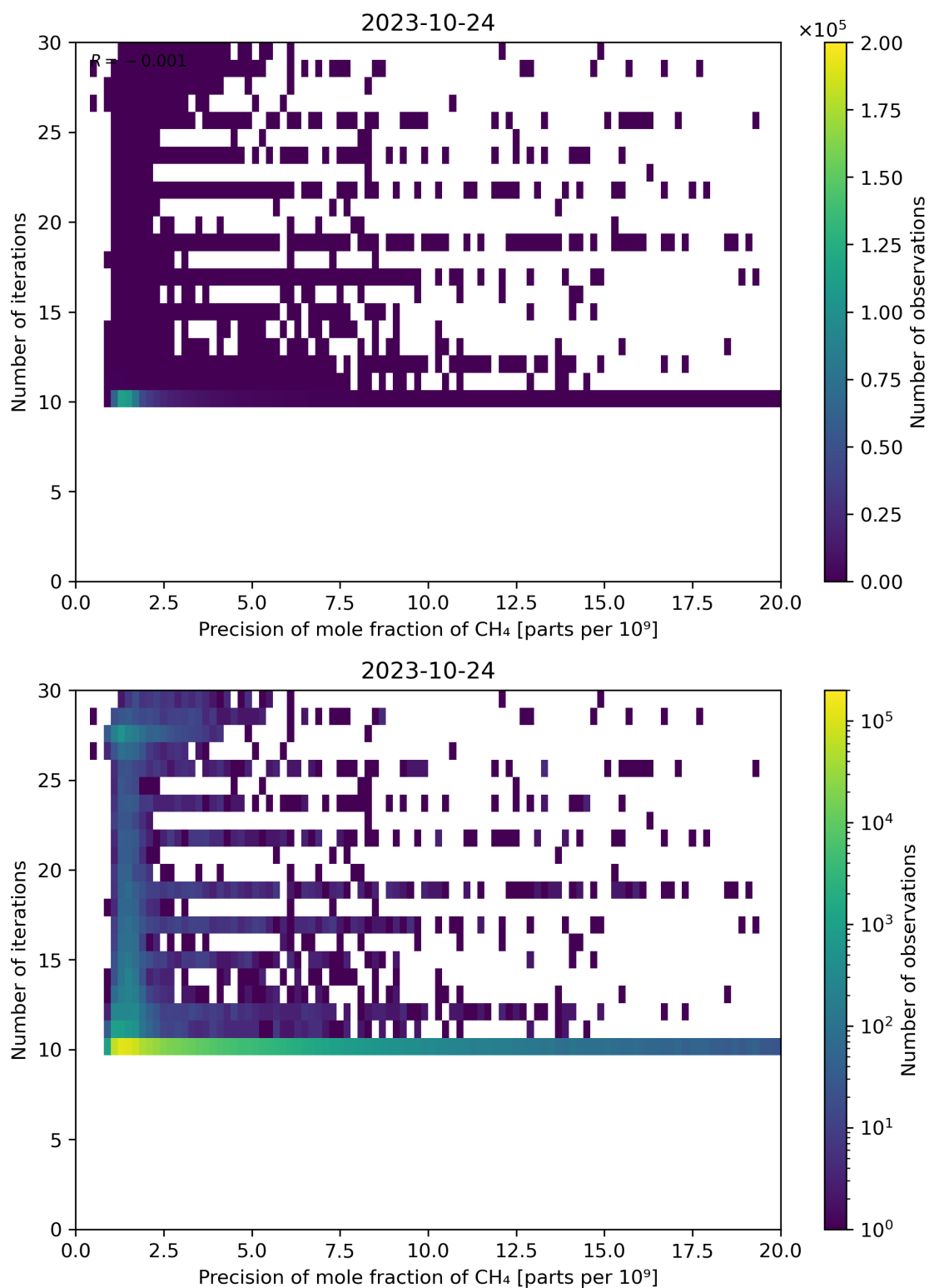
Figure 83: Scatter density plot of “Precision of mole fraction of CH 4 ” against “Number of iterations” for 2023-10-23 to 2023-10-25.
