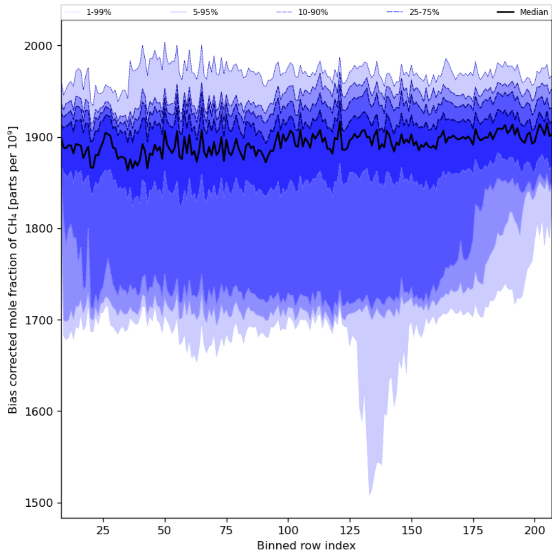
Figure 36: Along track statistics of “Bias corrected mole fraction of CH 4 ” for 2023-10-23 to 2023-10-25
