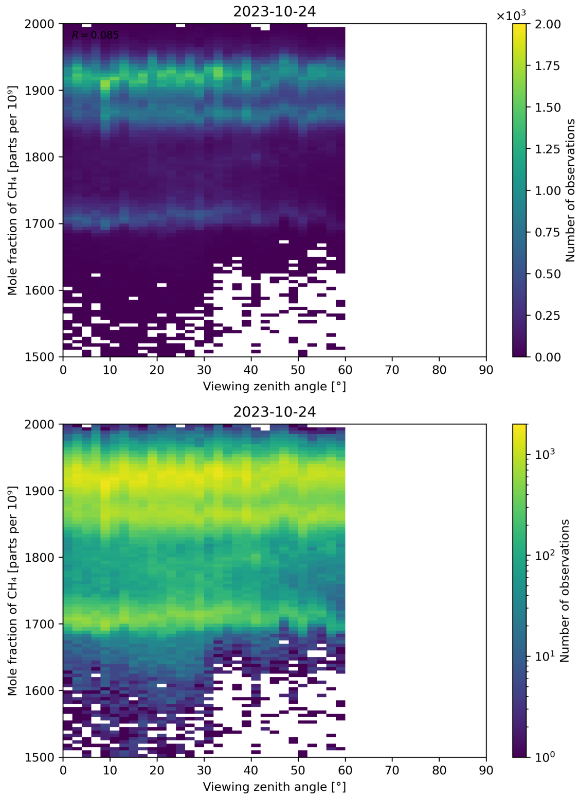
Figure 110: Scatter density plot of “Viewing zenith angle” against “Mole fraction of CH 4 ” for 2023-10-23 to 2023-10-25.
