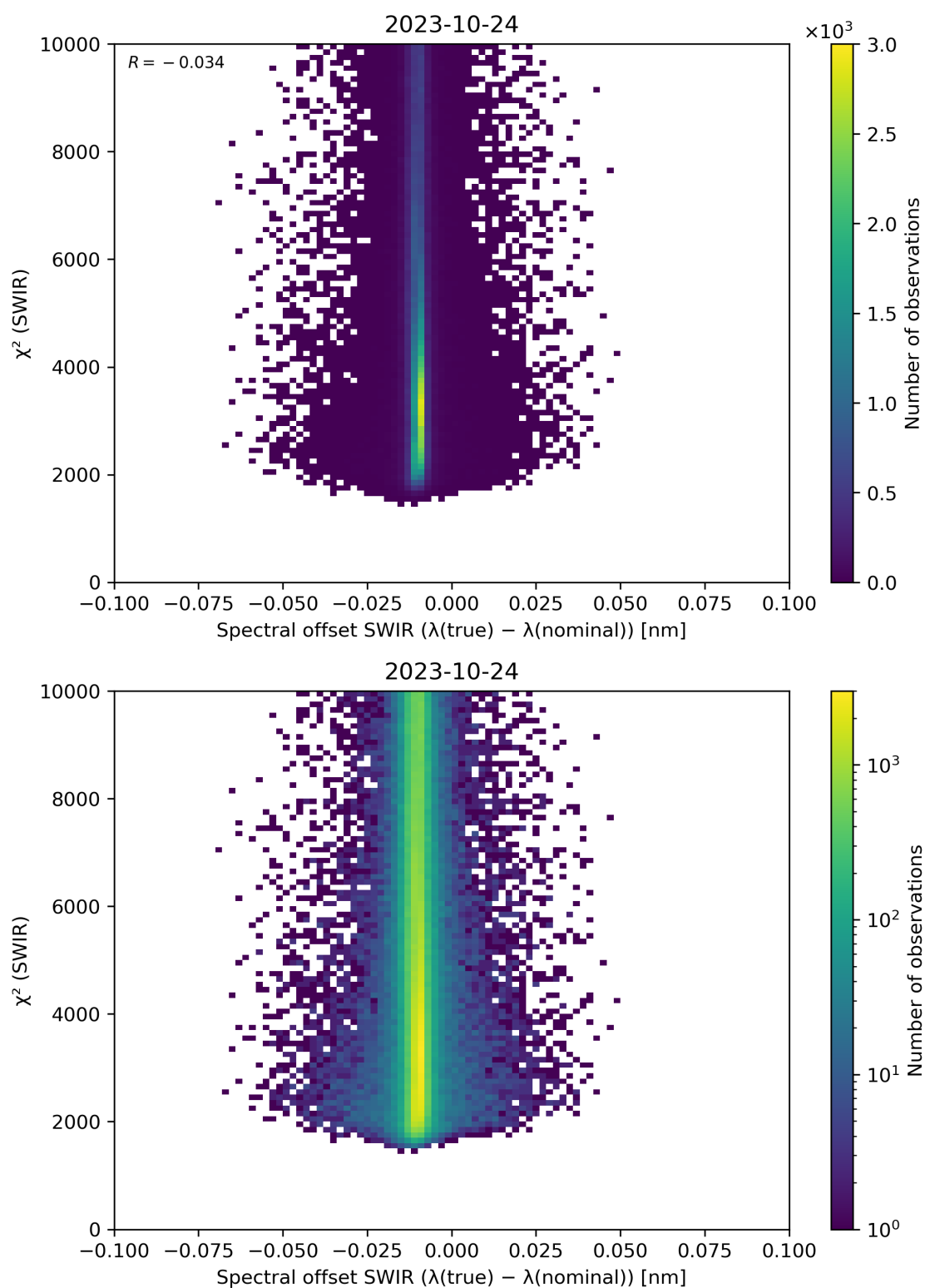
Figure 118: Scatter density plot of “Spectral offset SWIR ( \lambda(\text{true}) - \lambda(\text{nominal}) )” against “ \chi^2 (SWIR)” for 2023-10-23 to 2023-10-25.
