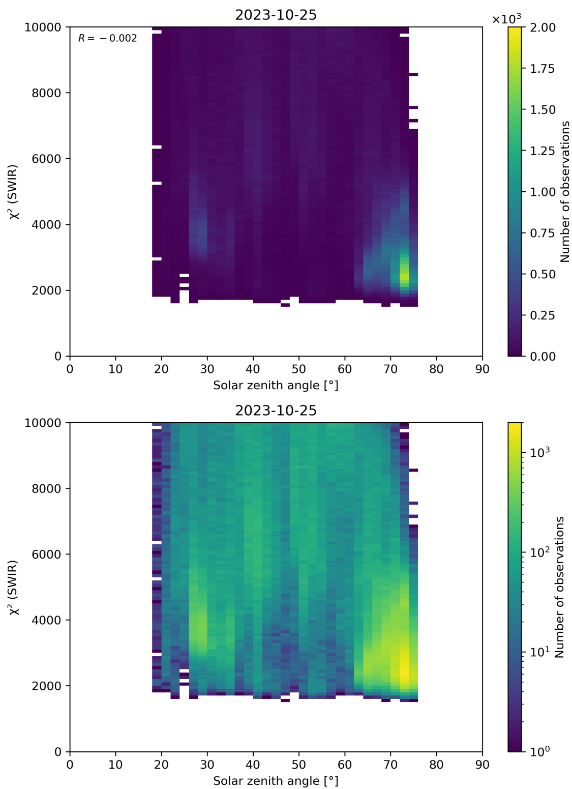
Figure 95: Scatter density plot of “Solar zenith angle” against “ \chi^2 (SWIR)” for 2023-10-24 to 2023-10-26.
