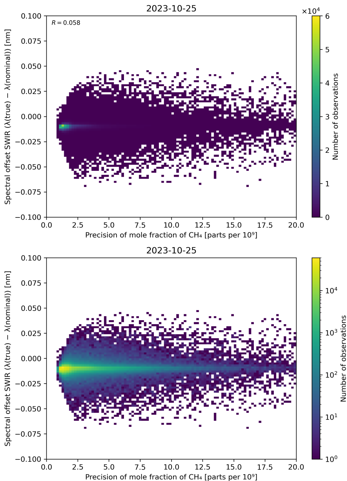
Figure 85: Scatter density plot of “Precision of mole fraction of \text{CH}_4 ” against “Spectral offset SWIR ( \lambda(\text{true}) - \lambda(\text{nominal}) )” for 2023-10-24 to 2023-10-26.
