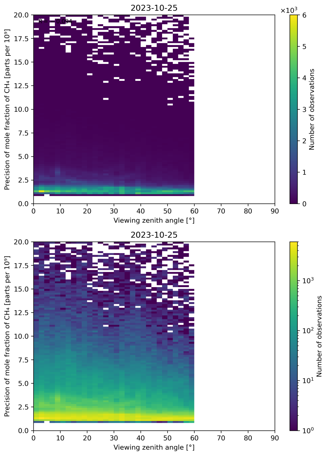
Figure 112: Scatter density plot of “Viewing zenith angle” against “Precision of mole fraction of CH 4 ” for 2023-10-24 to 2023-10-26.
