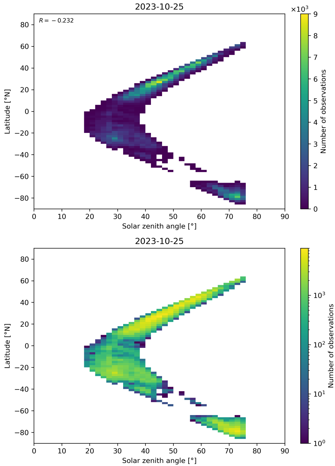
Figure 98: Scatter density plot of “Solar zenith angle” against “Latitude” for 2023-10-24 to 2023-10-26.
