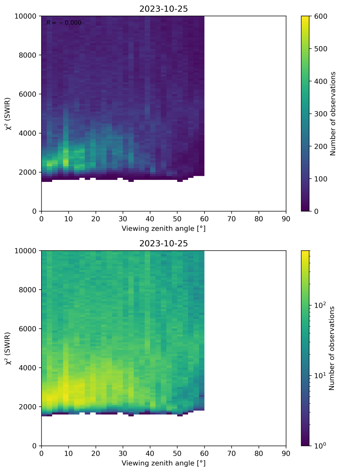
Figure 106: Scatter density plot of “Viewing zenith angle” against “ \chi^2 (SWIR)” for 2023-10-24 to 2023-10-26.
