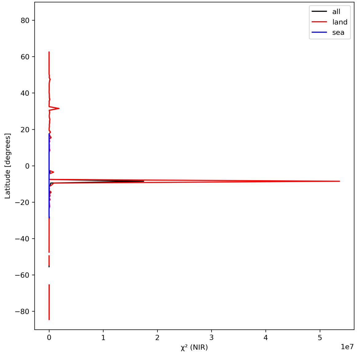
Figure 18: Zonal average of “ \chi^2 (NIR)” for 2023-10-24 to 2023-10-26.
