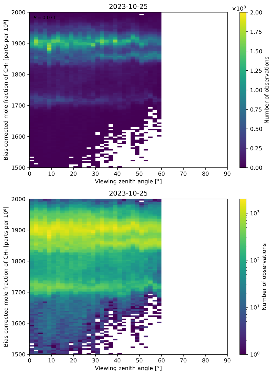
Figure 111: Scatter density plot of “Viewing zenith angle” against “Bias corrected mole fraction of CH 4 ” for 2023-10-24 to 2023-10-26.
