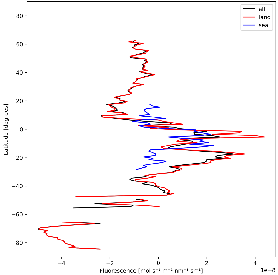
Figure 21: Zonal average of “Fluorescence” for 2023-10-24 to 2023-10-26.
