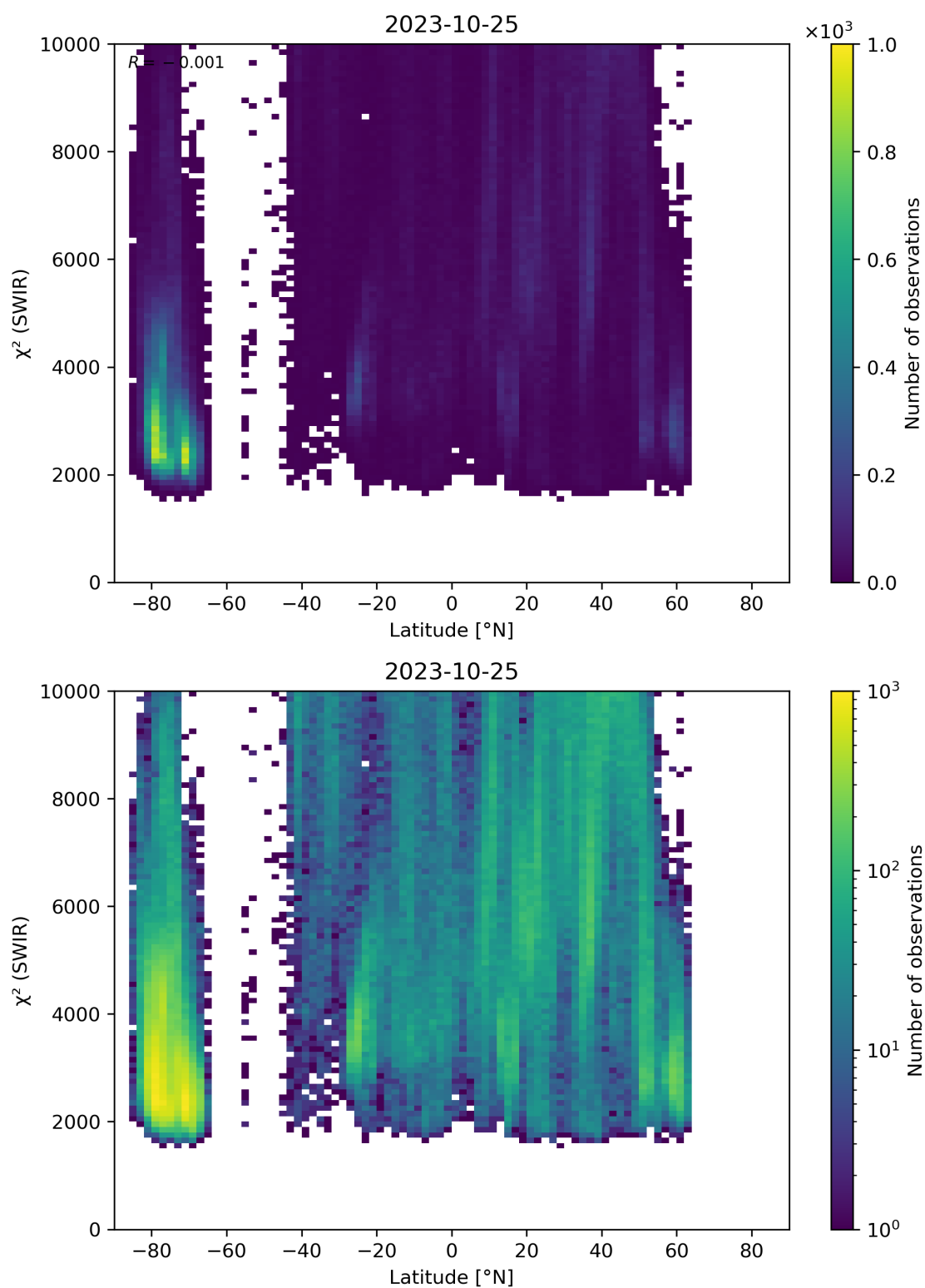
Figure 54: Scatter density plot of “Latitude” against “ \chi^2 (SWIR)” for 2023-10-24 to 2023-10-26.
