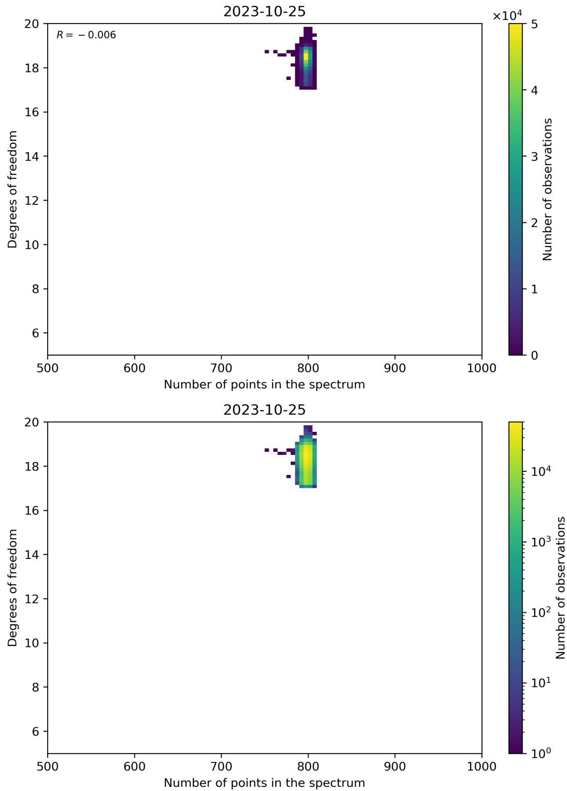
Figure 90: Scatter density plot of “Number of points in the spectrum” against “Degrees of freedom” for 2023-10-24 to 2023-10-26.
