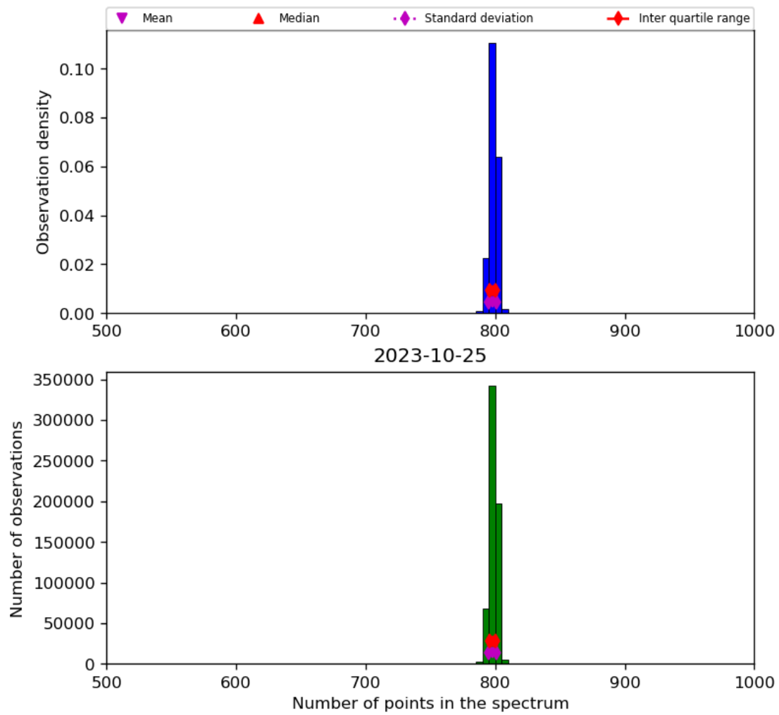
Figure 26: Histogram of “Number of points in the spectrum” for 2023-10-24 to 2023-10-26
