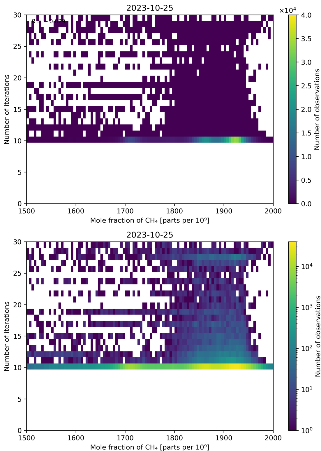
Figure 76: Scatter density plot of “Mole fraction of CH 4 ” against “Number of iterations” for 2023-10-24 to 2023-10-26.
