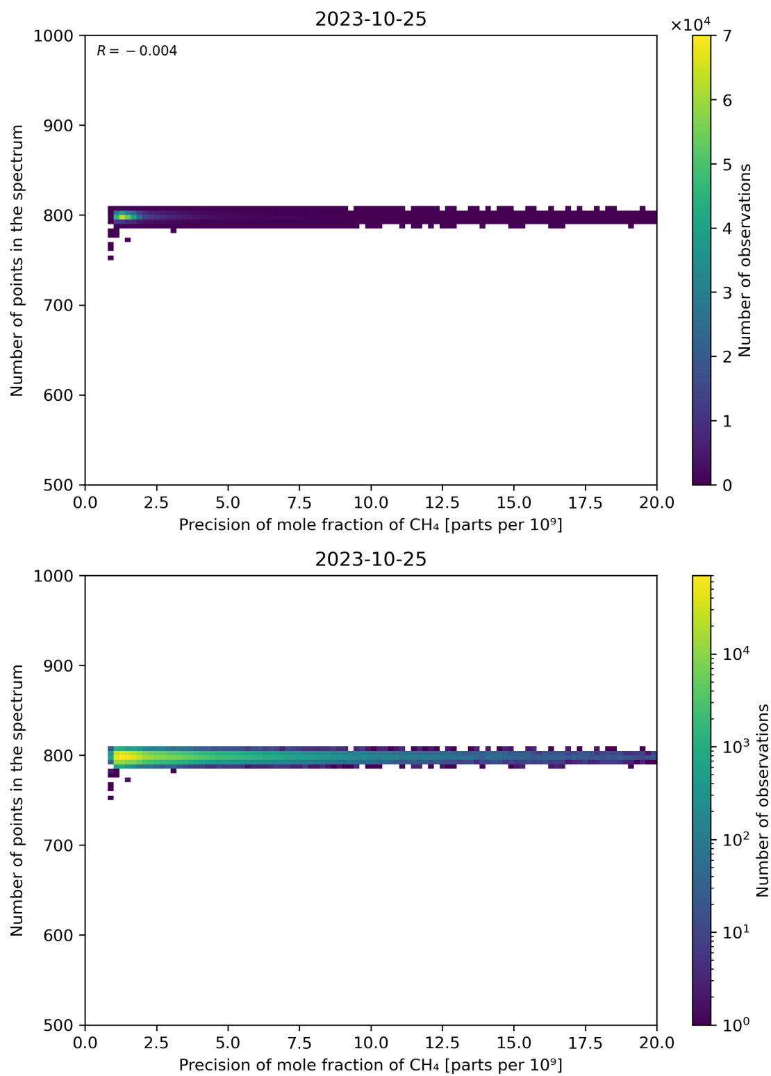
Figure 84: Scatter density plot of “Precision of mole fraction of CH 4 ” against “Number of points in the spectrum” for 2023-10-24 to 2023-10-26.
