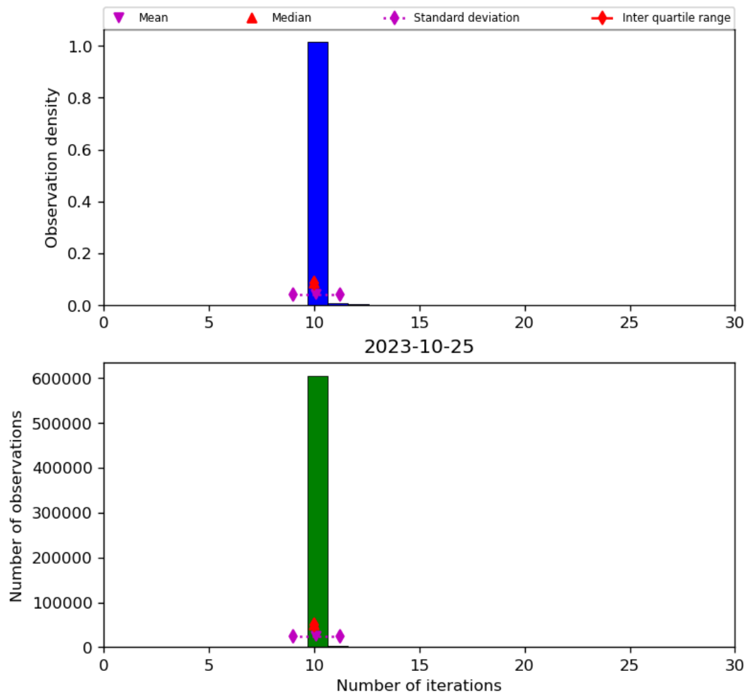
Figure 31: Histogram of “Number of iterations” for 2023-10-24 to 2023-10-26
