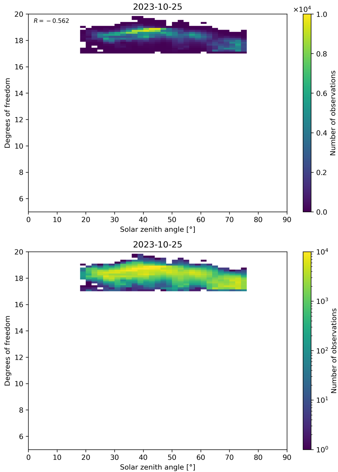
Figure 96: Scatter density plot of “Solar zenith angle” against “Degrees of freedom” for 2023-10-24 to 2023-10-26.
