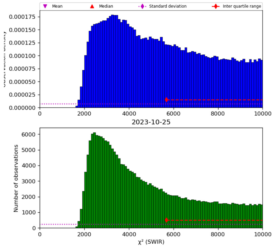
Figure 28: Histogram of “ \chi^2 (SWIR)” for 2023-10-24 to 2023-10-26
