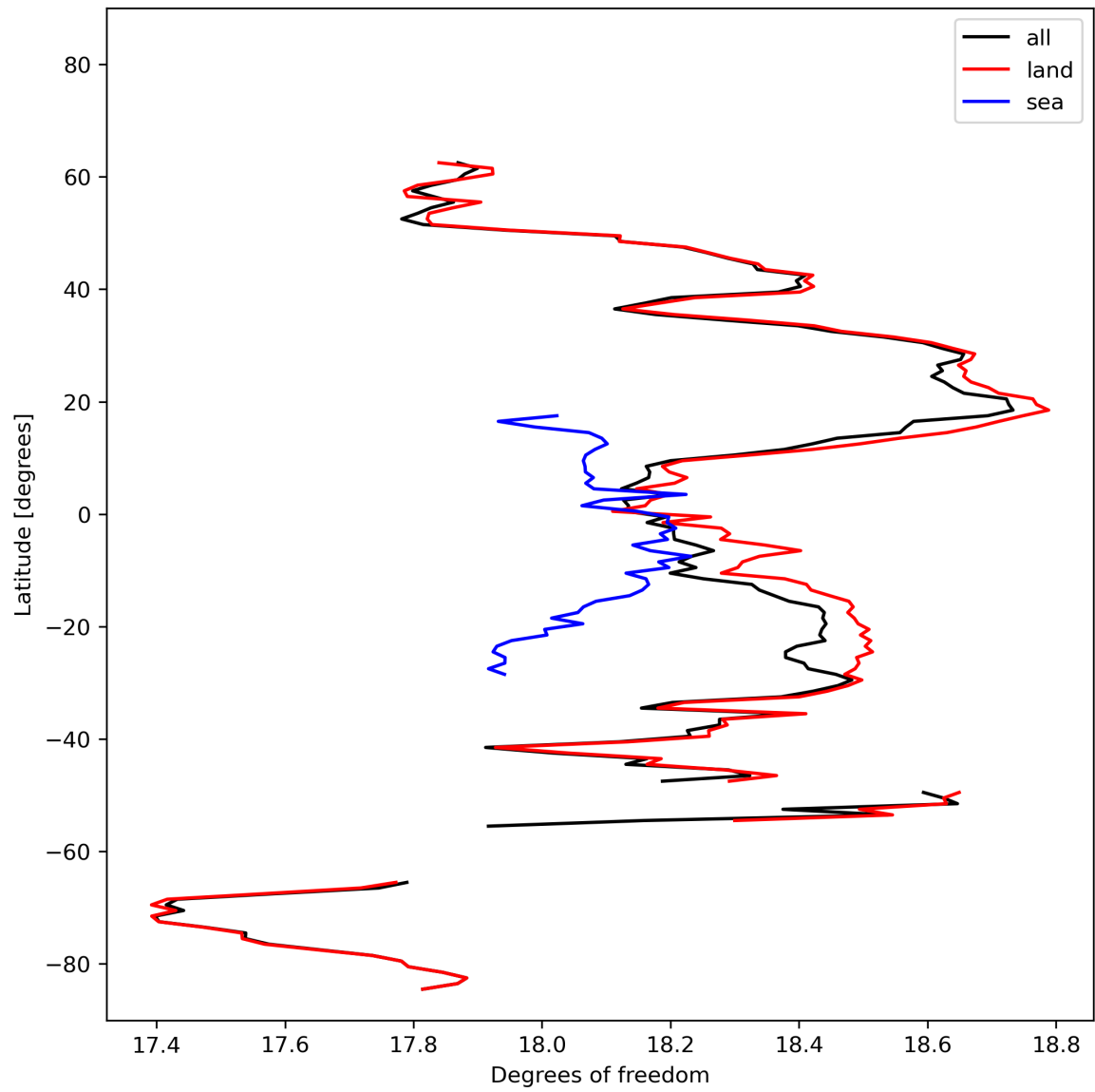
Figure 19: Zonal average of “Degrees of freedom” for 2023-10-24 to 2023-10-26.
