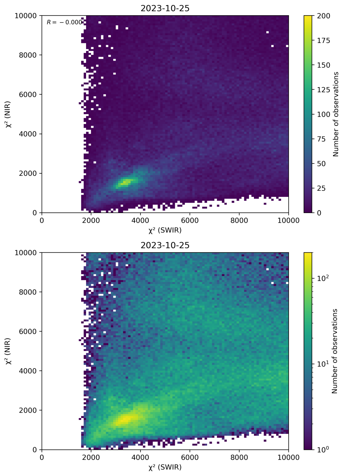
Figure 47: Scatter density plot of “ \chi^2 (SWIR)” against “ \chi^2 (NIR)” for 2023-10-24 to 2023-10-26.
