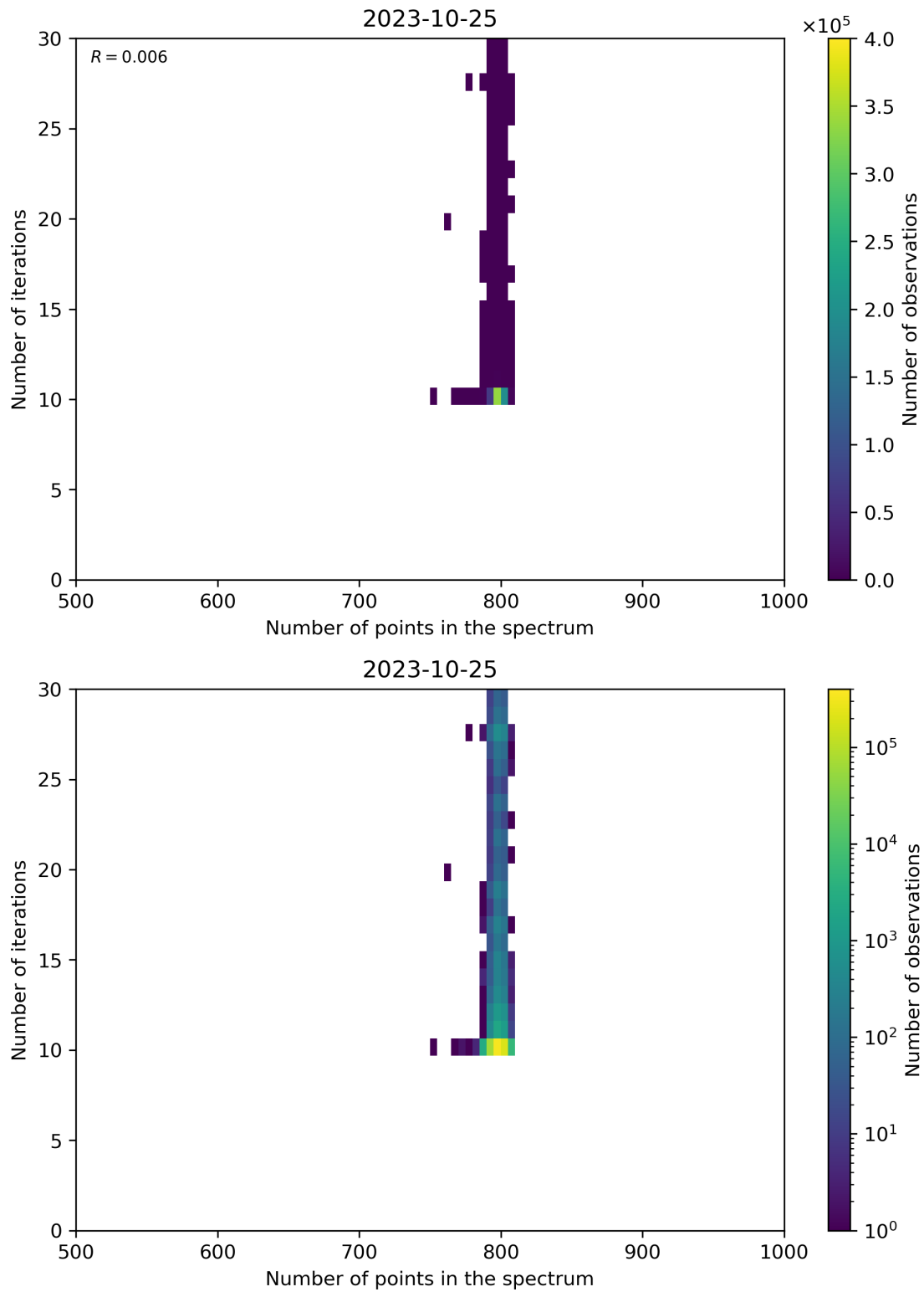
Figure 92: Scatter density plot of “Number of points in the spectrum” against “Number of iterations” for 2023-10-24 to 2023-10-26.
