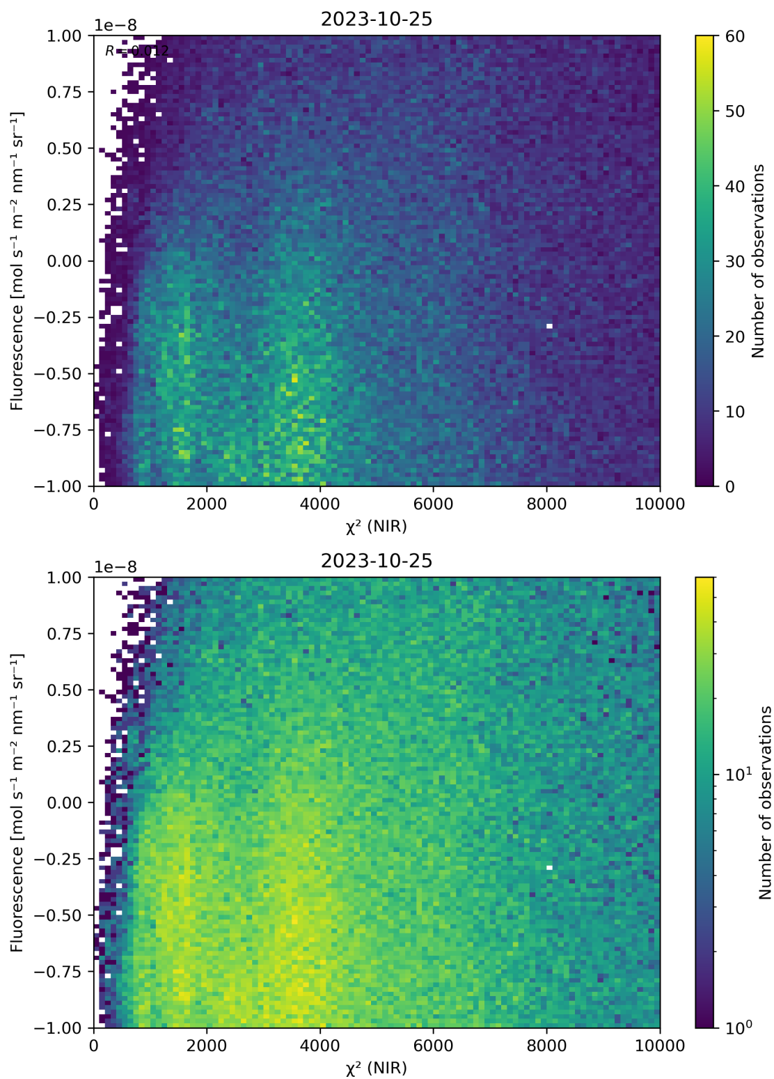
Figure 45: Scatter density plot of “ \chi^2 (NIR)” against “Fluorescence” for 2023-10-24 to 2023-10-26.
