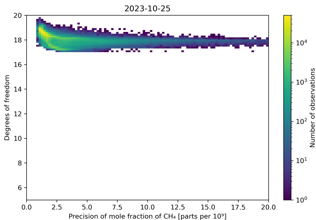
Figure 80: Scatter density plot of “Precision of mole fraction of CH 4 ” against “Degrees of freedom” for 2023-10-24 to 2023-10-26.
