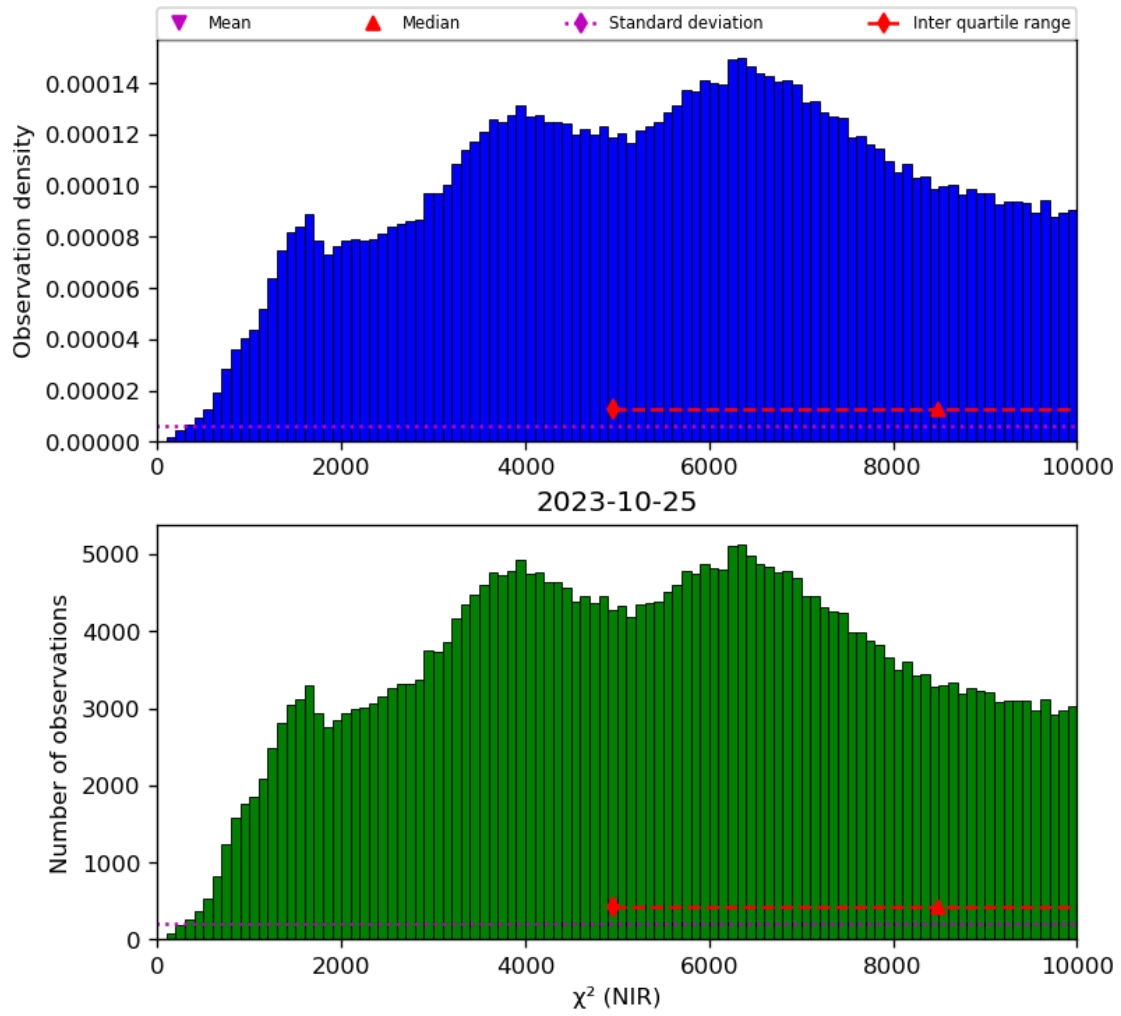
Figure 29: Histogram of “ \chi^2 (NIR)” for 2023-10-24 to 2023-10-26
