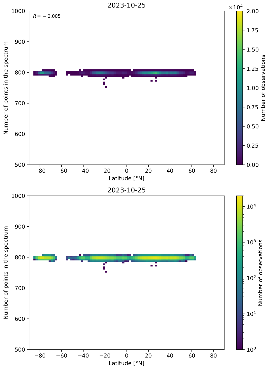
Figure 61: Scatter density plot of “Latitude” against “Number of points in the spectrum” for 2023-10-24 to 2023-10-26.
