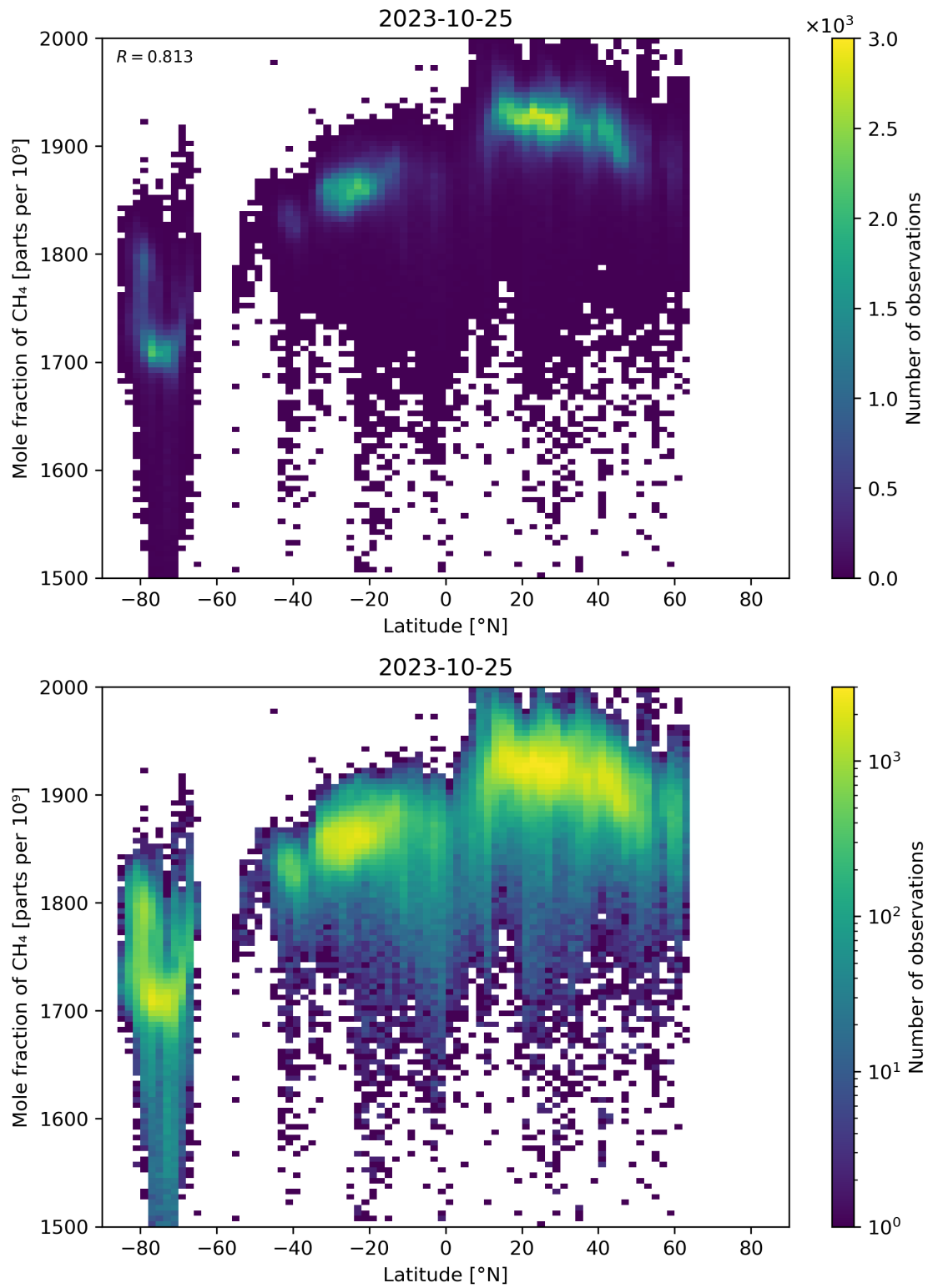
Figure 57: Scatter density plot of “Latitude” against “Mole fraction of \text{CH}_4 ” for 2023-10-24 to 2023-10-26.
