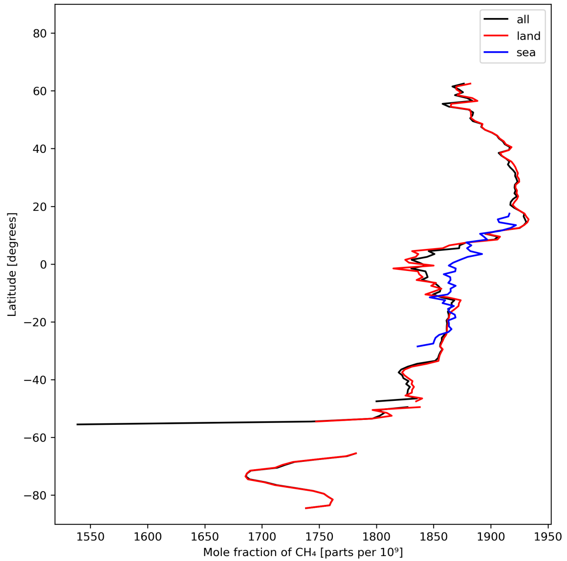
Figure 12: Zonal average of “Mole fraction of CH 4 ” for 2023-10-24 to 2023-10-26.
