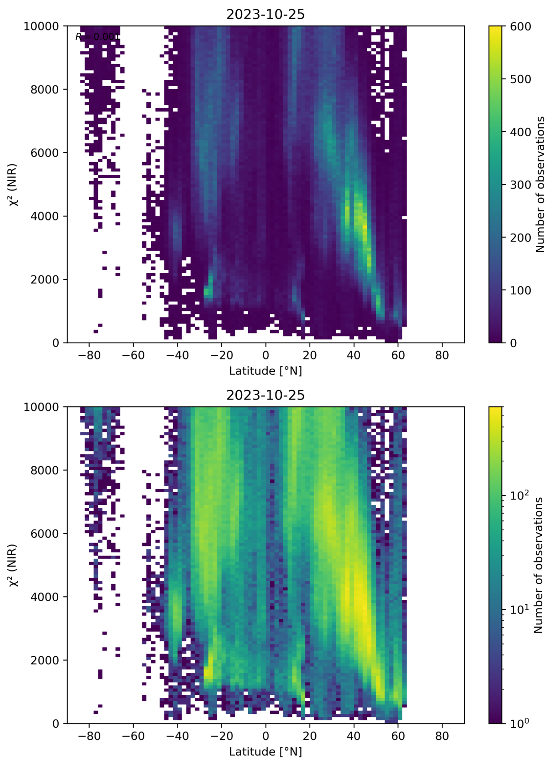
Figure 53: Scatter density plot of “Latitude” against “ \chi^2 (NIR)” for 2023-10-24 to 2023-10-26.
