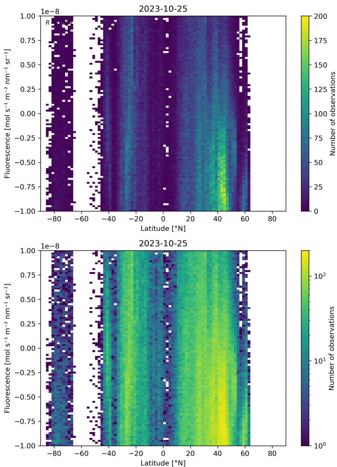
Figure 56: Scatter density plot of “Latitude” against “Fluorescence” for 2023-10-24 to 2023-10-26.
