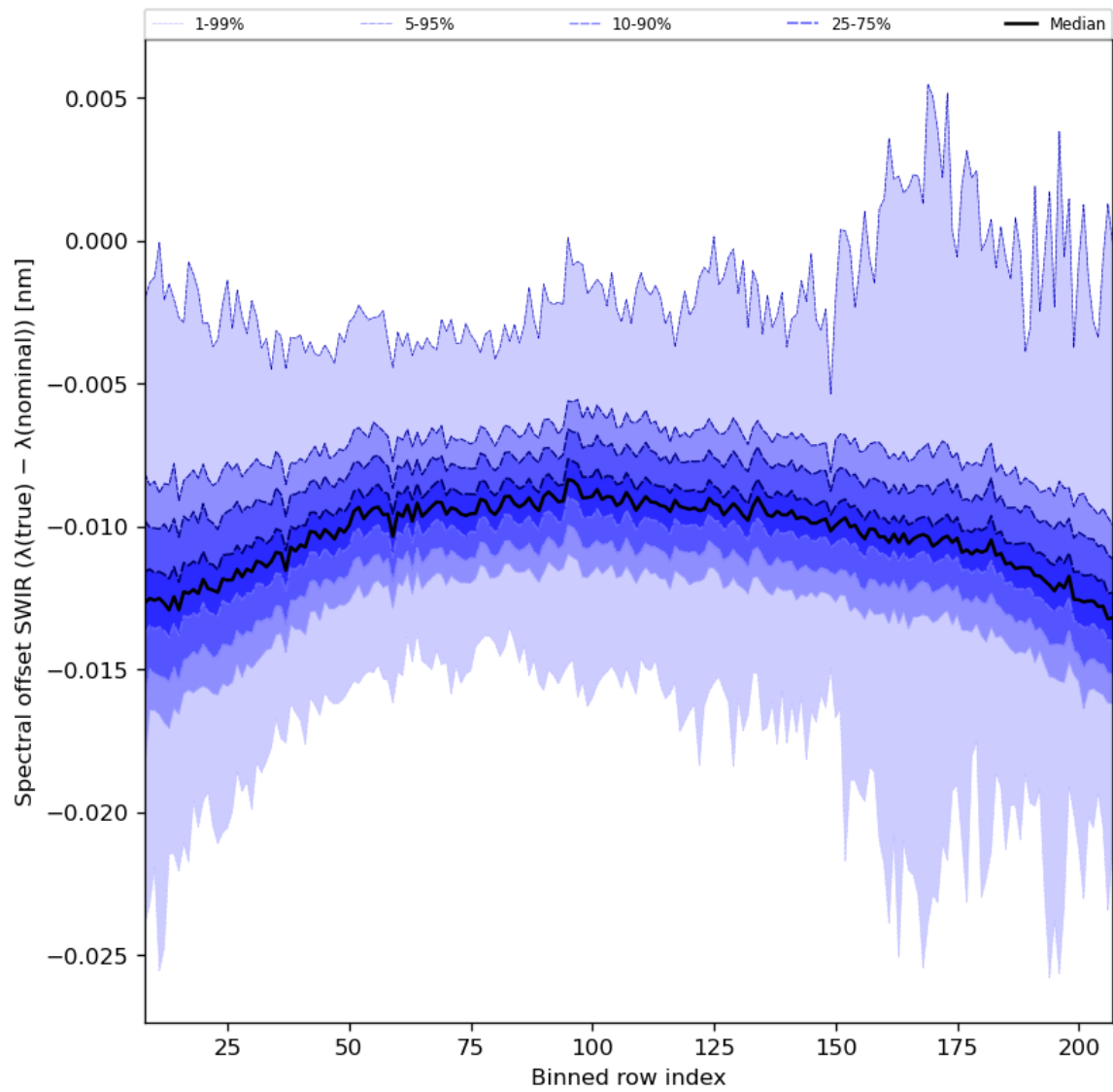
Figure 38: Along track statistics of “Spectral offset SWIR ( \lambda(\text{true}) - \lambda(\text{nominal}) )” for 2023-10-24 to 2023-10-26
