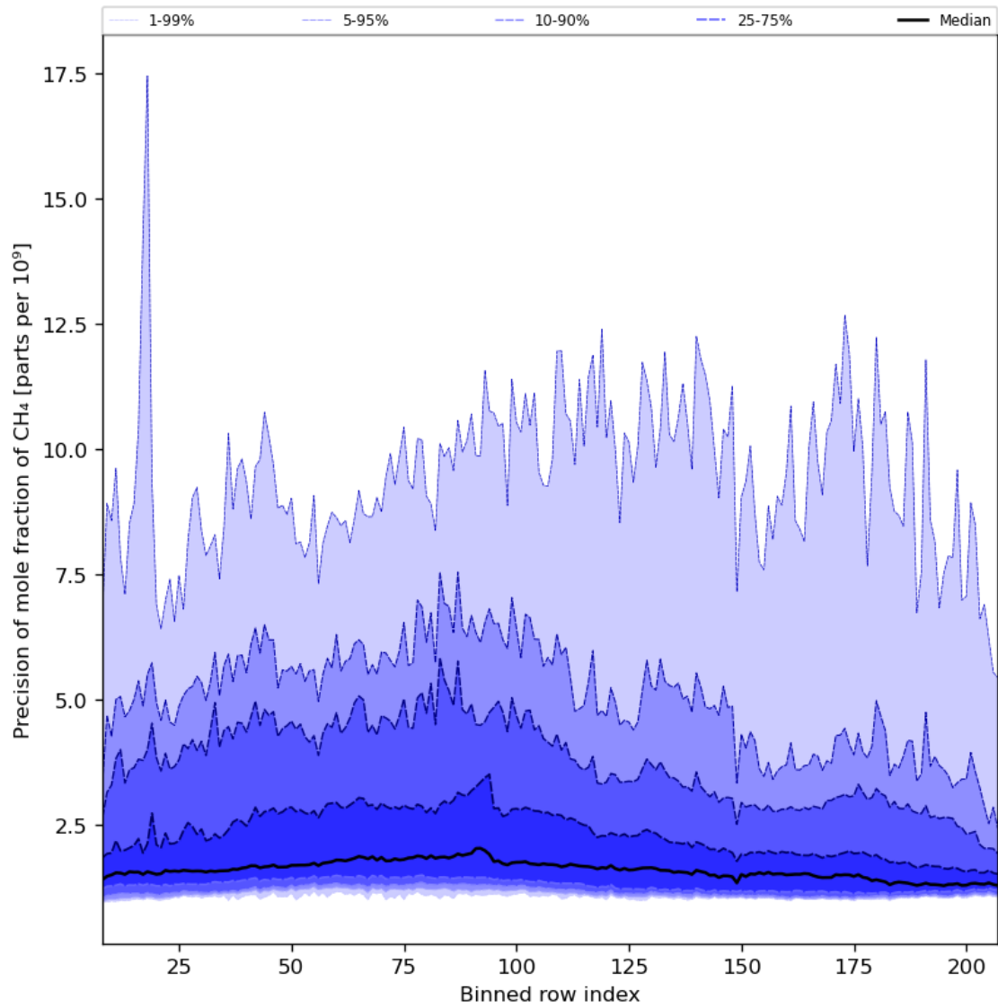
Figure 35: Along track statistics of “Precision of mole fraction of CH 4 ” for 2023-10-24 to 2023-10-26
