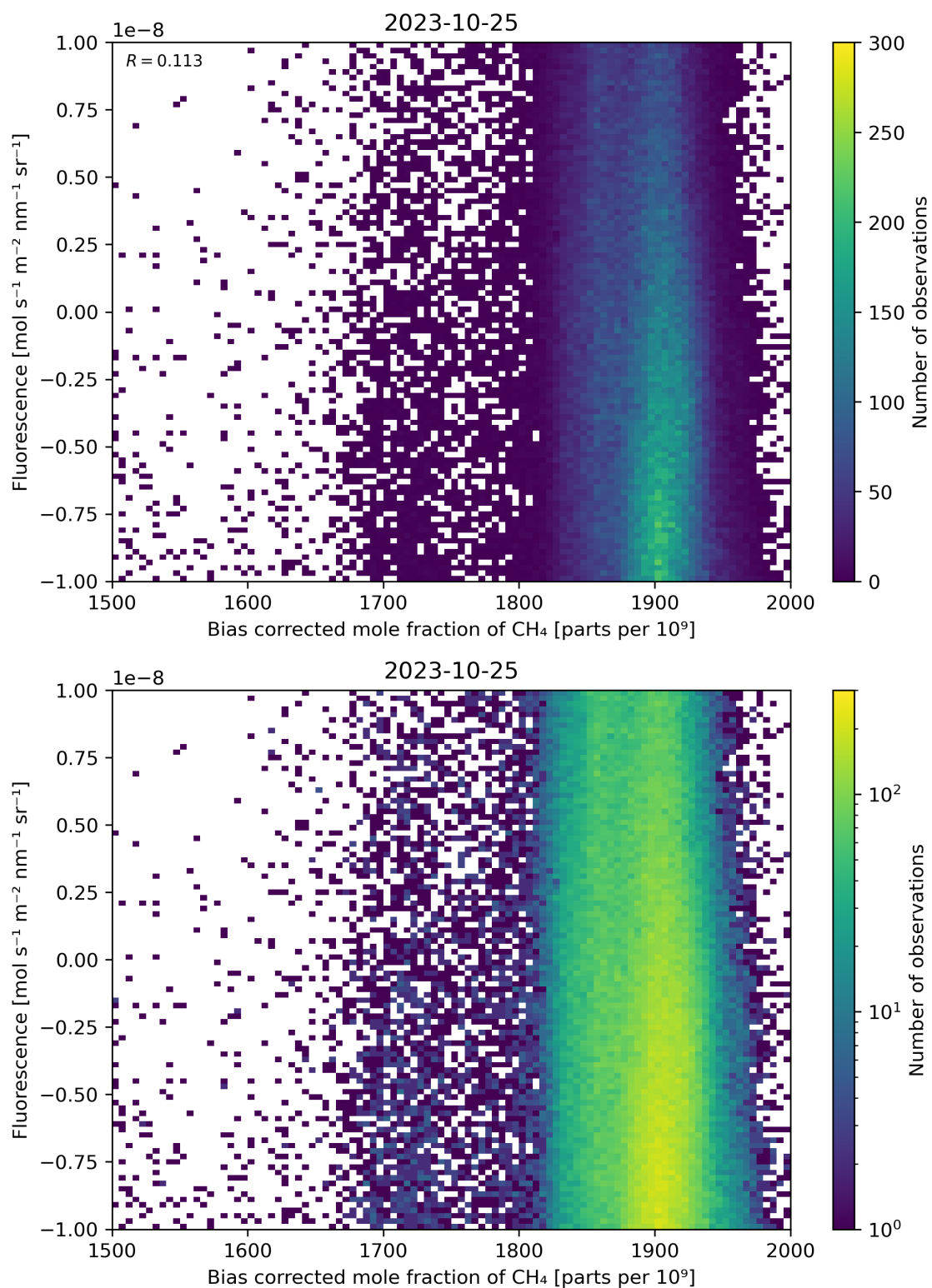
Figure 66: Scatter density plot of “Bias corrected mole fraction of \text{CH}_4 ” against “Fluorescence” for 2023-10-24 to 2023-10-26.
