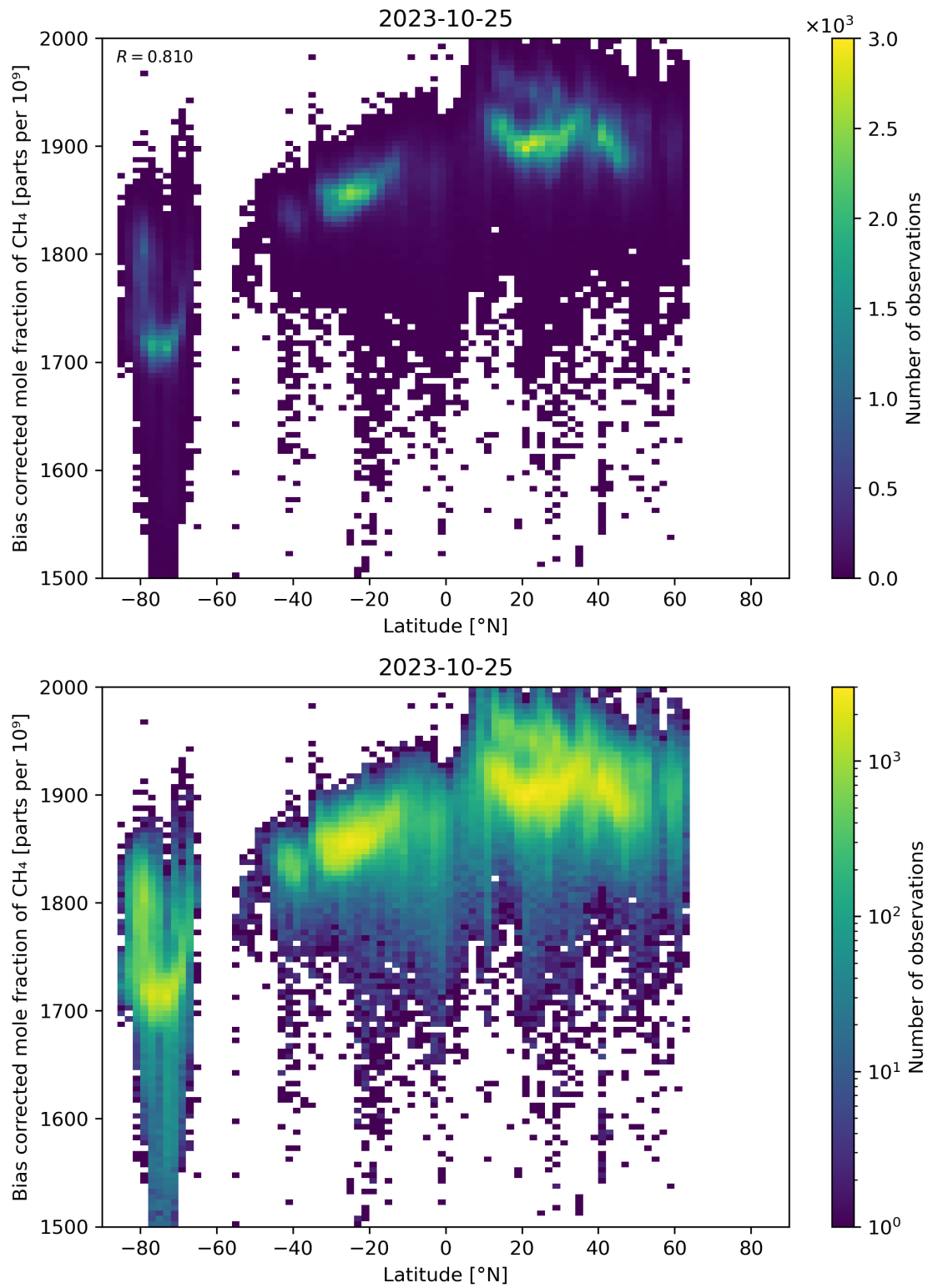
Figure 58: Scatter density plot of “Latitude” against “Bias corrected mole fraction of \text{CH}_4 ” for 2023-10-24 to 2023-10-26.
