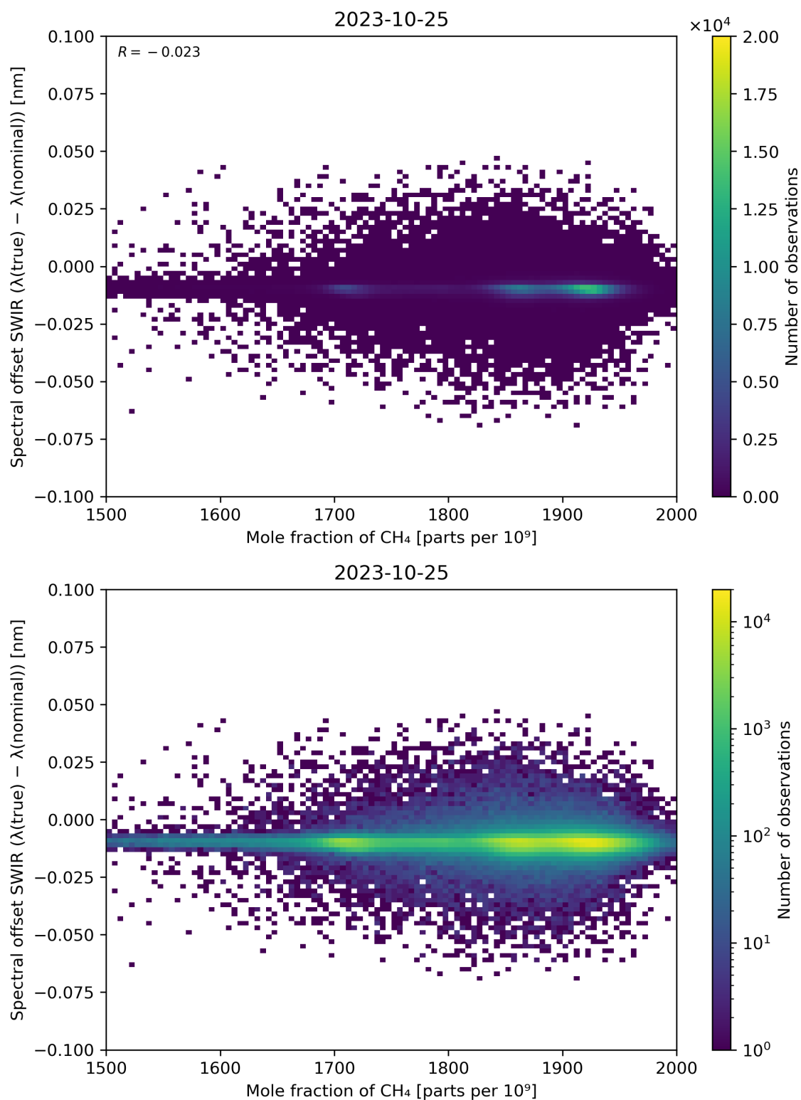
Figure 86: Scatter density plot of “Mole fraction of CH 4 ” against “Spectral offset SWIR ( \lambda(\text{true}) - \lambda(\text{nominal}) )” for 2023-10-24 to 2023-10-26.
