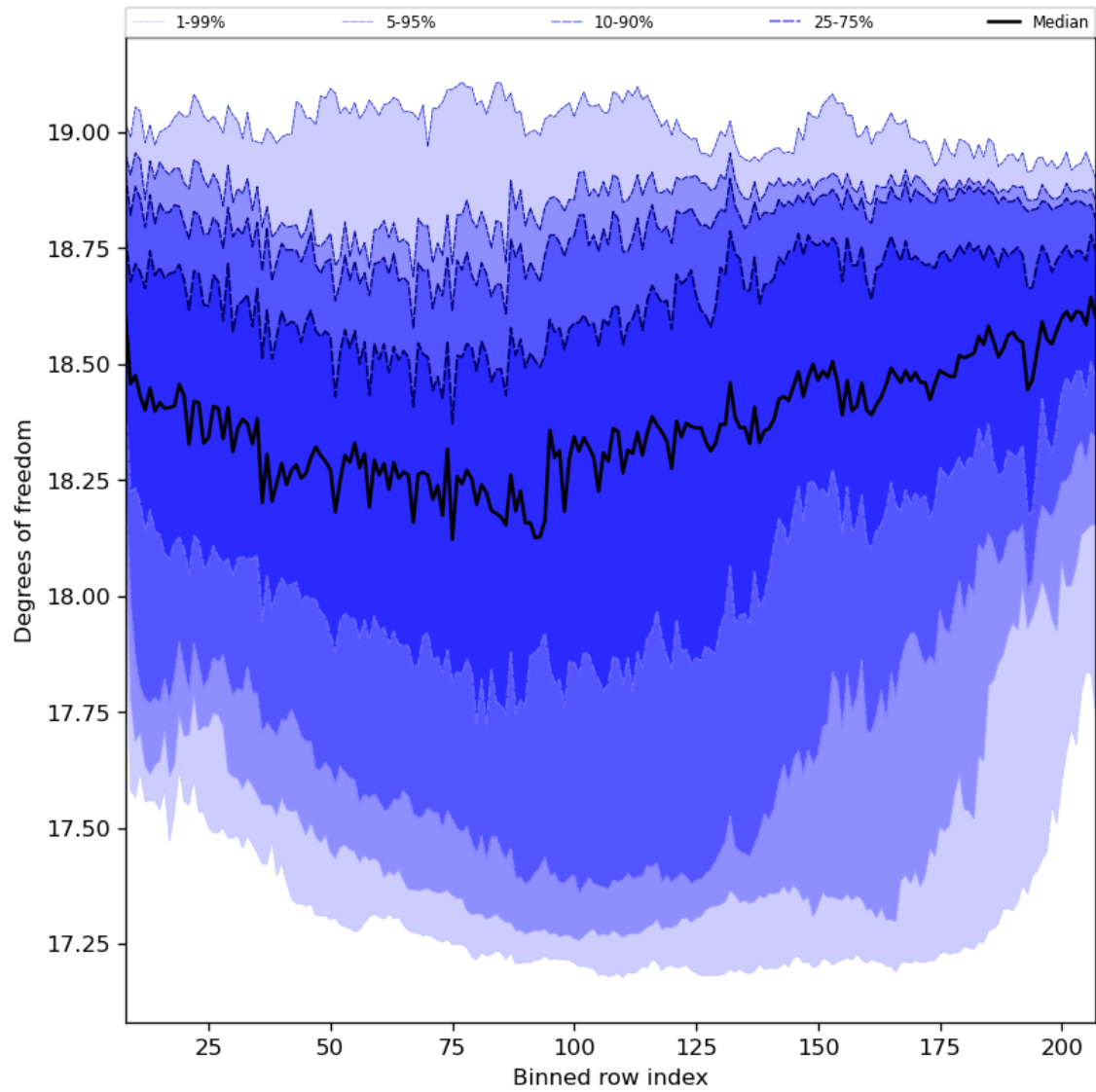
Figure 41: Along track statistics of “Degrees of freedom” for 2023-10-24 to 2023-10-26
