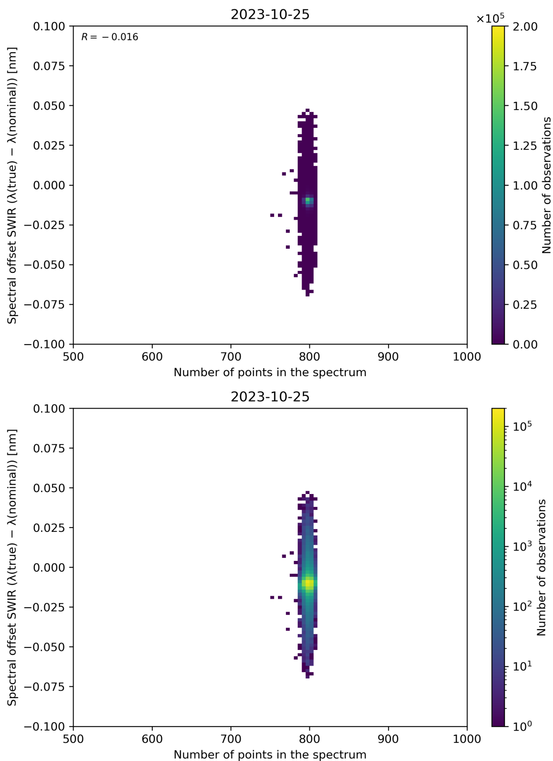
Figure 93: Scatter density plot of “Number of points in the spectrum” against “Spectral offset SWIR ( \lambda(\text{true}) - \lambda(\text{nominal}) )” for 2023-10-24 to 2023-10-26.
