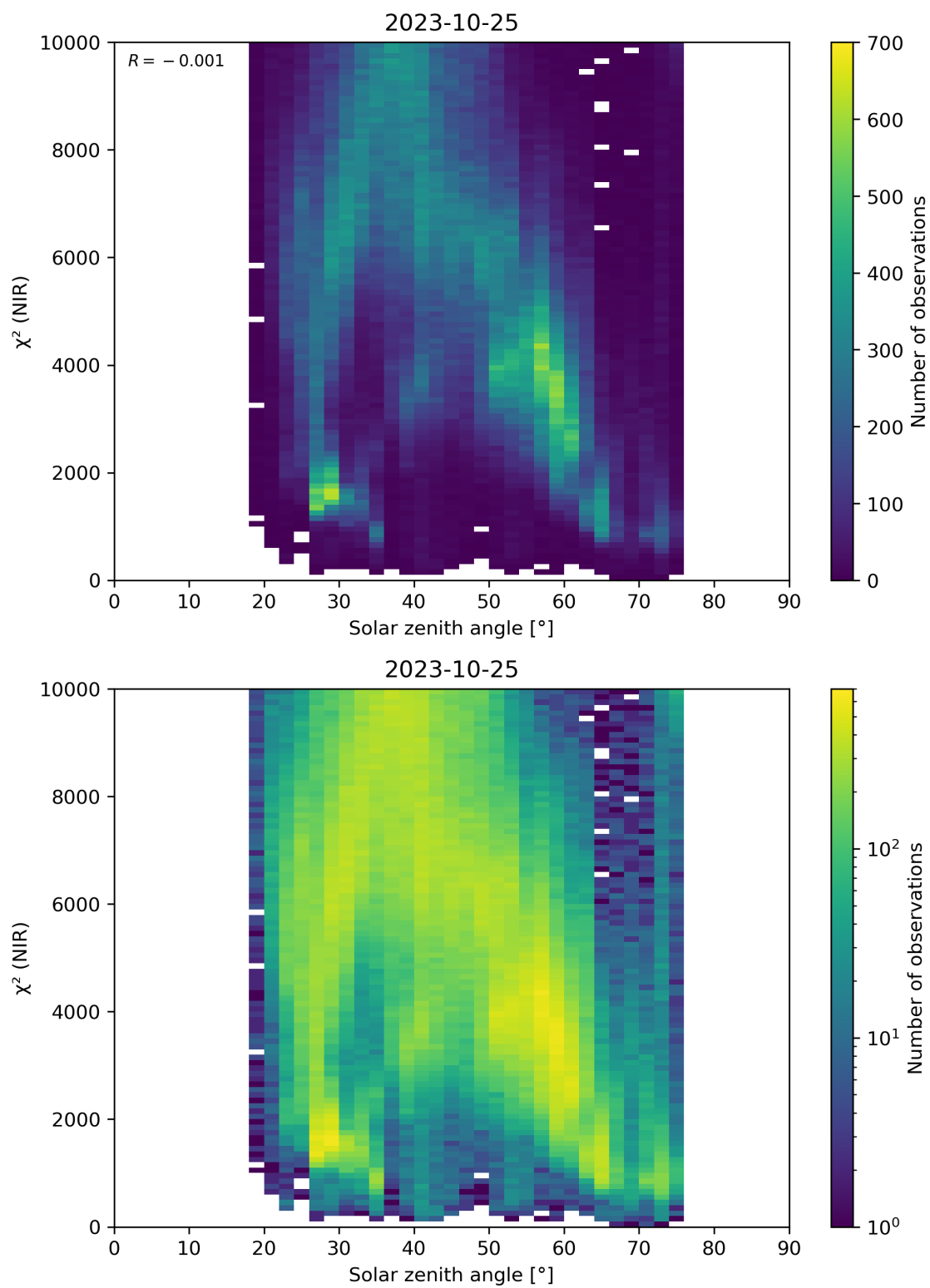
Figure 94: Scatter density plot of “Solar zenith angle” against “ \chi^2 (NIR)” for 2023-10-24 to 2023-10-26.
