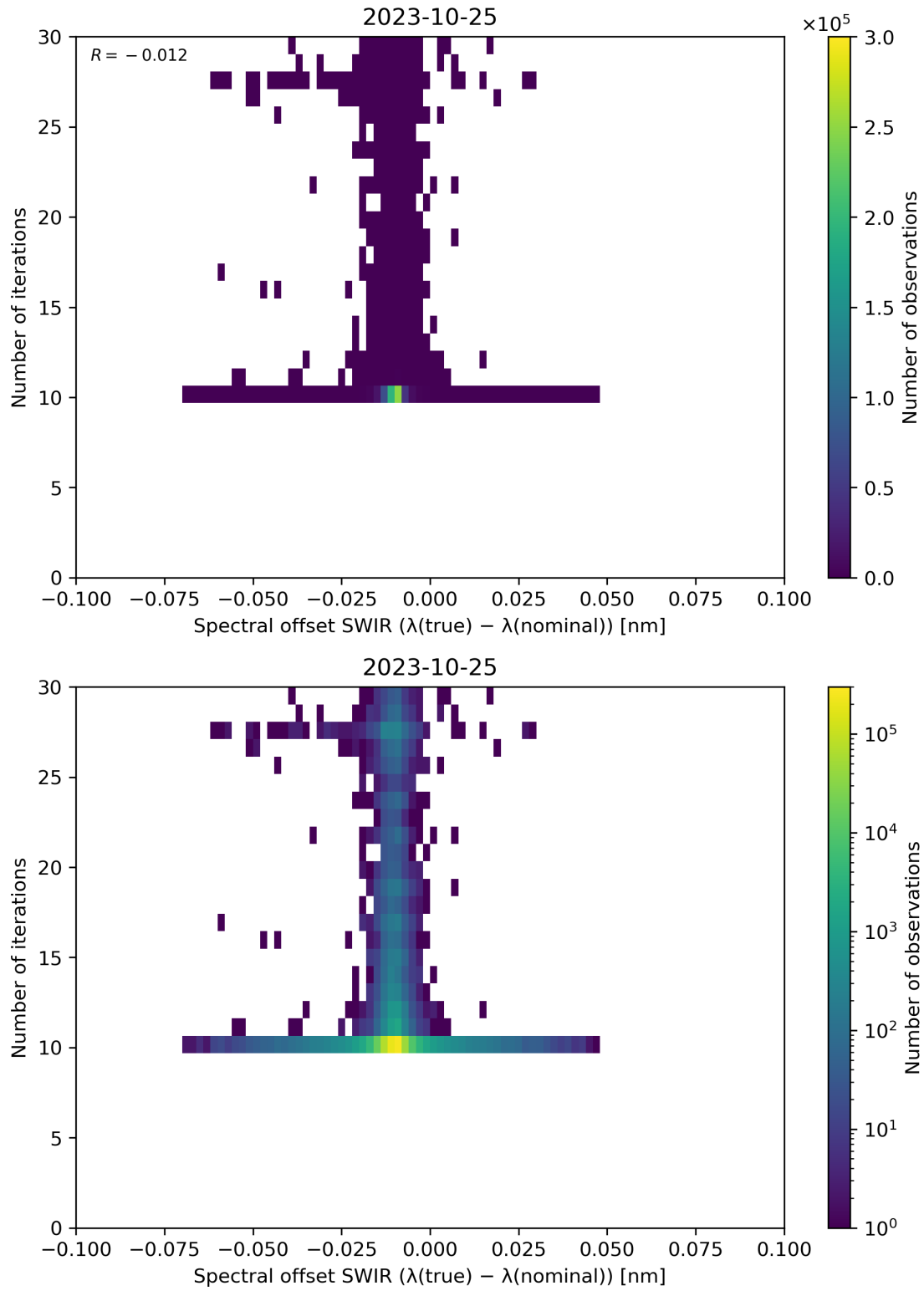
Figure 121: Scatter density plot of “Spectral offset SWIR ( \lambda(\text{true}) - \lambda(\text{nominal}) )” against “Number of iterations” for 2023-10-24 to 2023-10-26.
