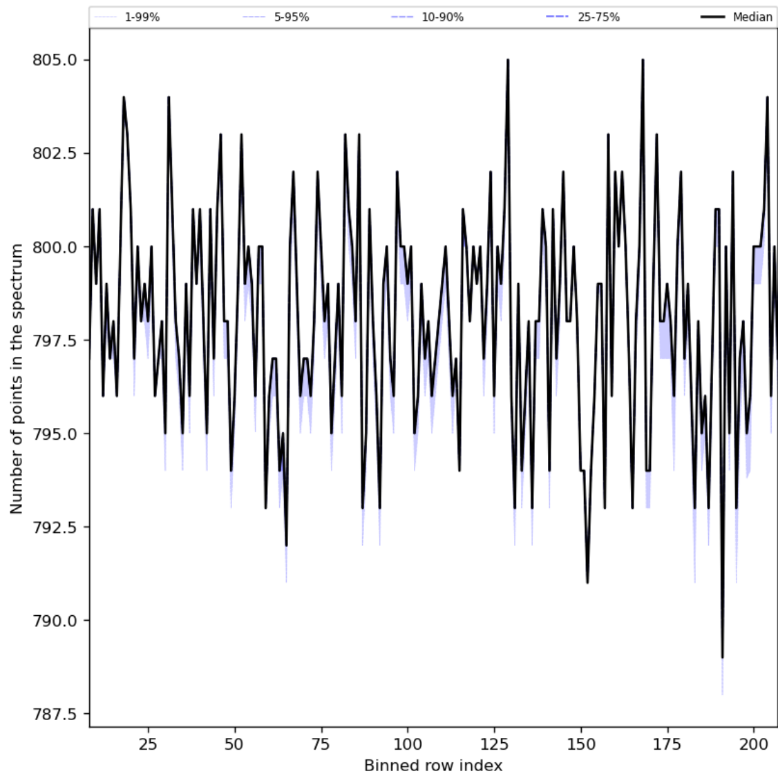
Figure 37: Along track statistics of “Number of points in the spectrum” for 2023-10-24 to 2023-10-26
