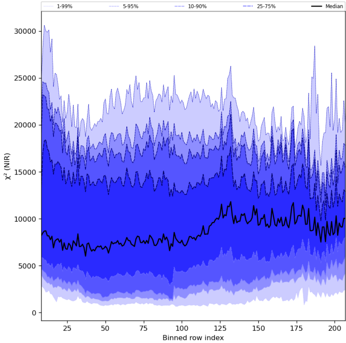
Figure 40: Along track statistics of “ \chi^2 (NIR)” for 2023-10-24 to 2023-10-26
