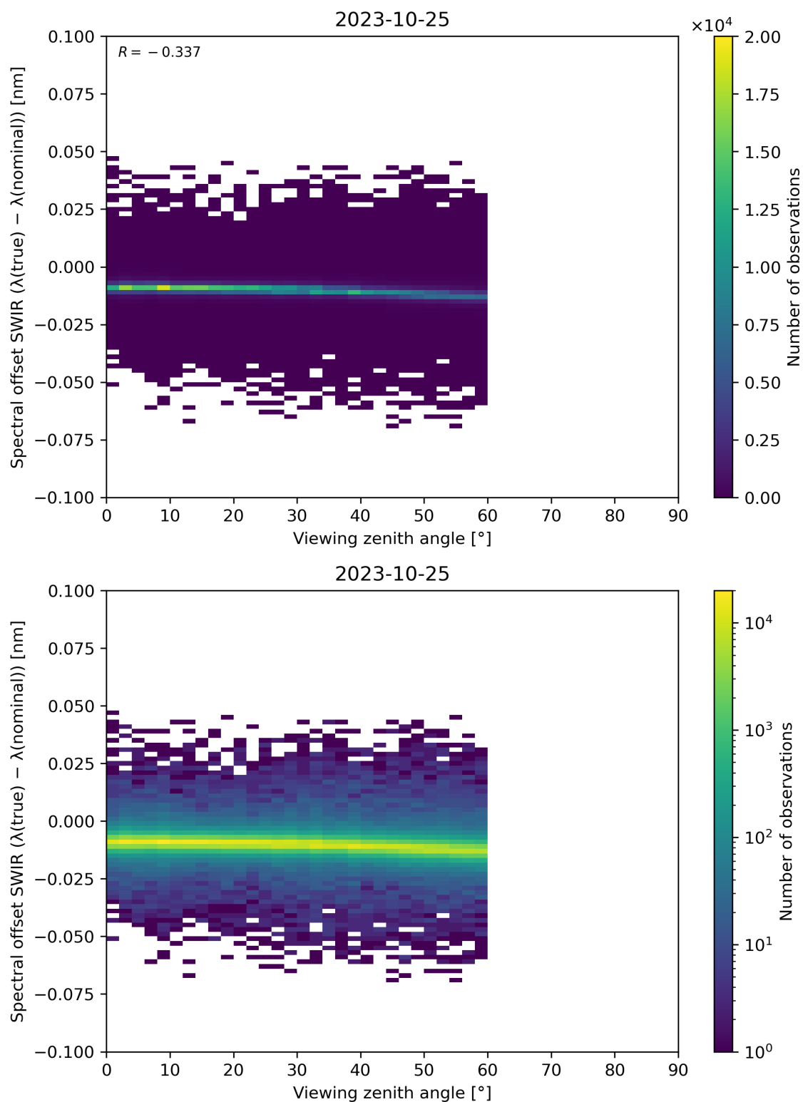
Figure 116: Scatter density plot of “Viewing zenith angle” against “Spectral offset SWIR ( \lambda(\text{true}) - \lambda(\text{nominal}) )” for 2023-10-24 to 2023-10-26.
