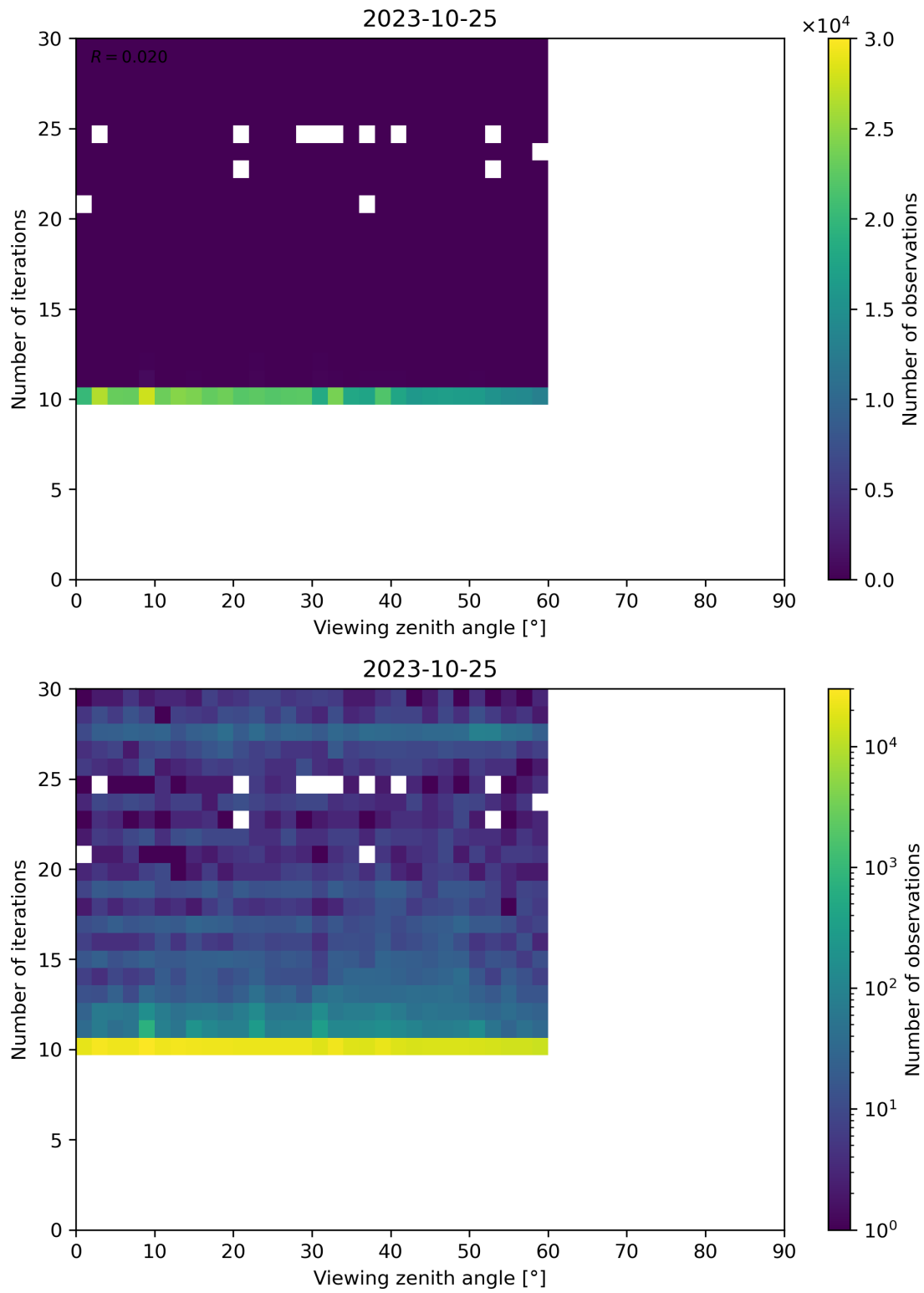
Figure 113: Scatter density plot of “Viewing zenith angle” against “Number of iterations” for 2023-10-24 to 2023-10-26.
