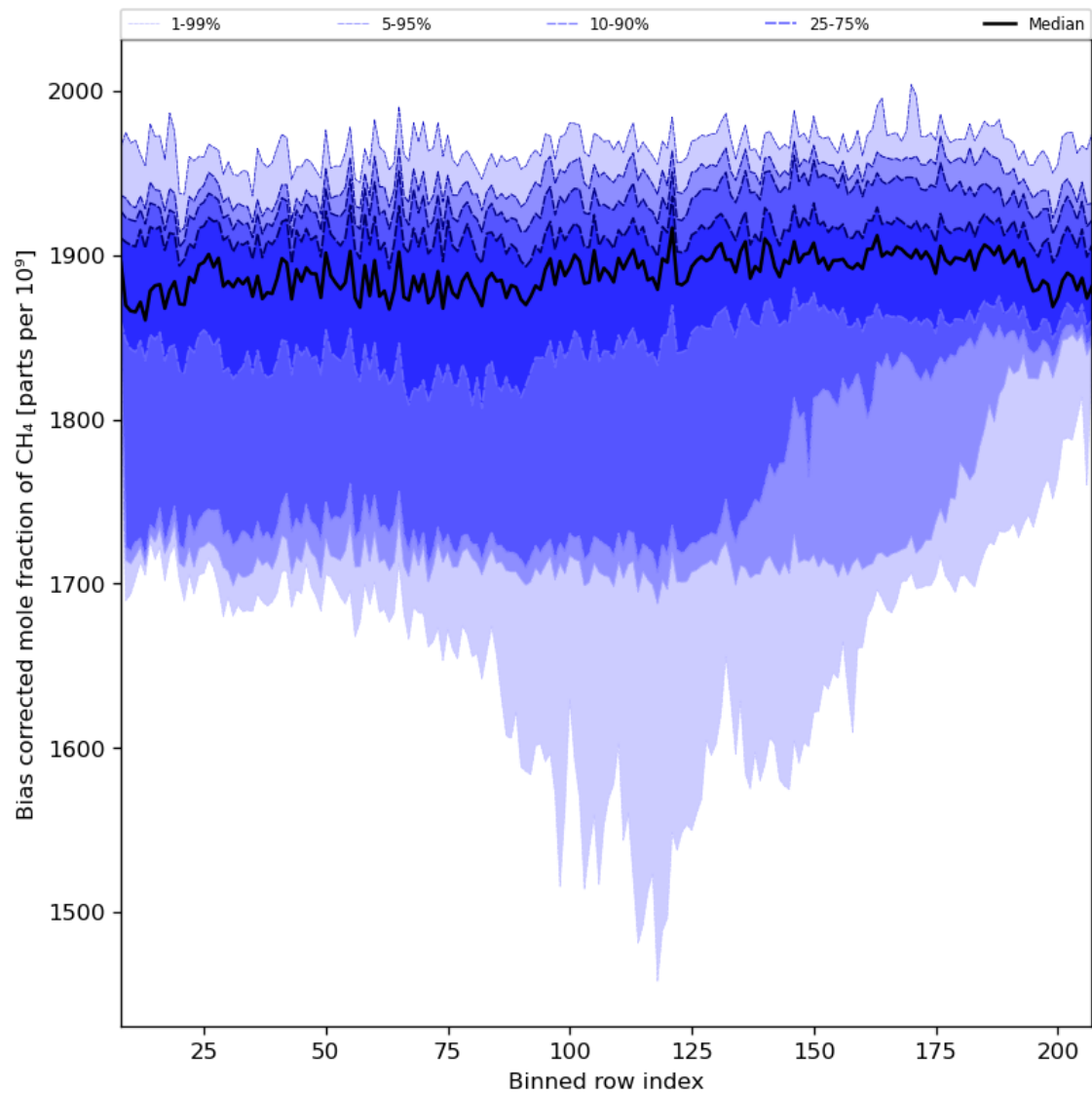
Figure 36: Along track statistics of “Bias corrected mole fraction of CH 4 ” for 2023-10-24 to 2023-10-26
