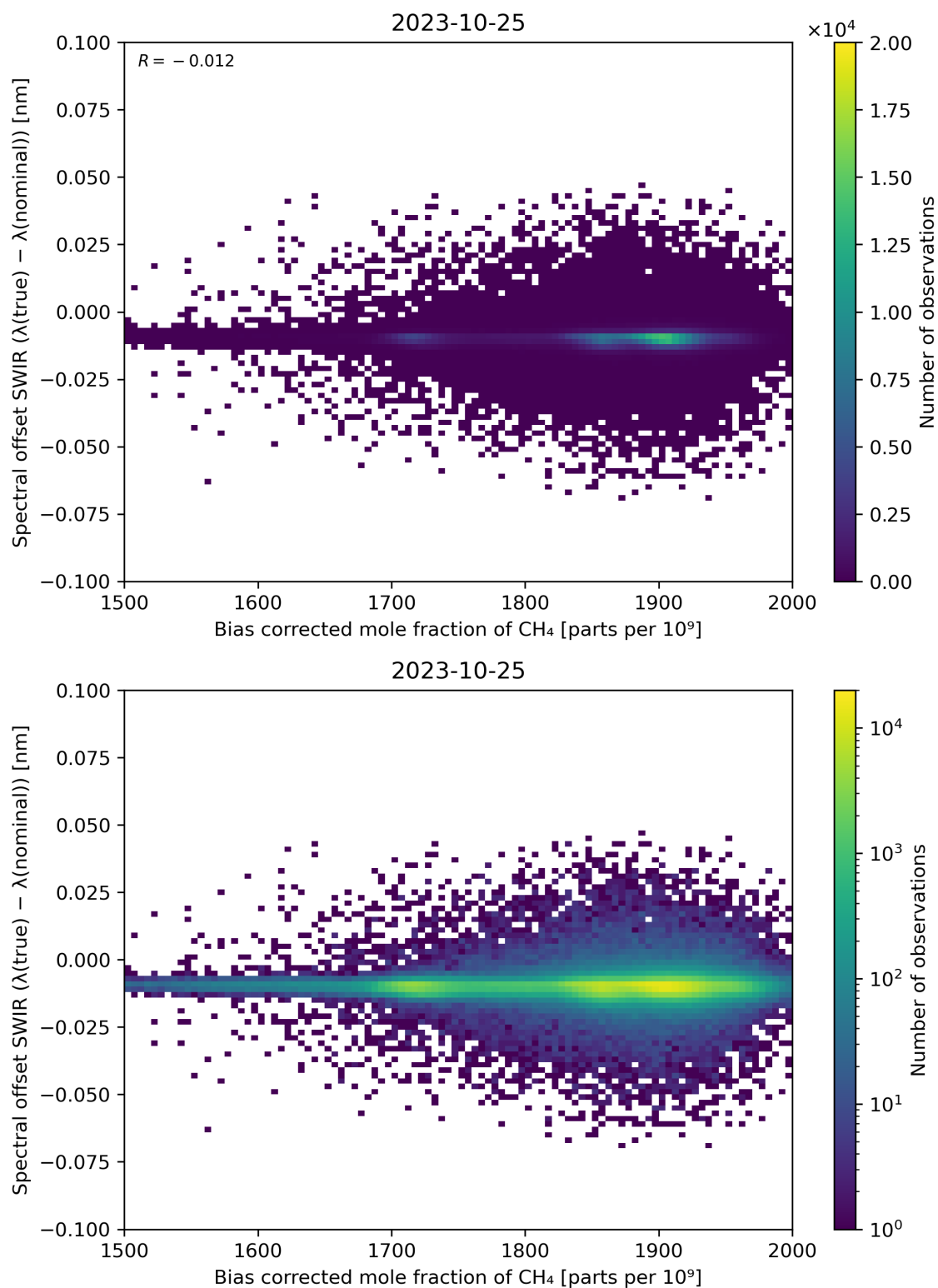
Figure 69: Scatter density plot of “Bias corrected mole fraction of \text{CH}_4 ” against “Spectral offset SWIR ( \lambda(\text{true}) - \lambda(\text{nominal}) )” for 2023-10-24 to 2023-10-26.
