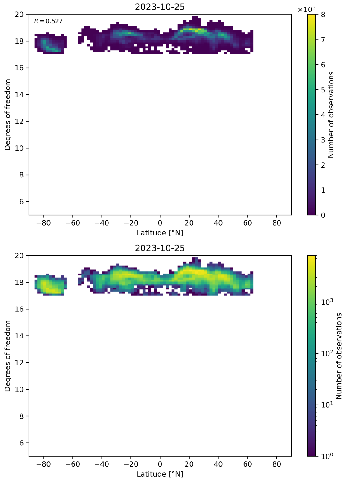
Figure 55: Scatter density plot of “Latitude” against “Degrees of freedom” for 2023-10-24 to 2023-10-26.
