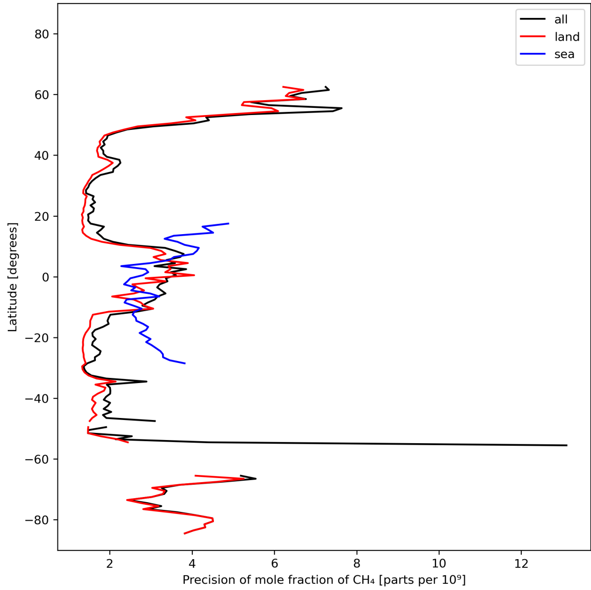
Figure 13: Zonal average of “Precision of mole fraction of CH 4 ” for 2023-10-24 to 2023-10-26.
