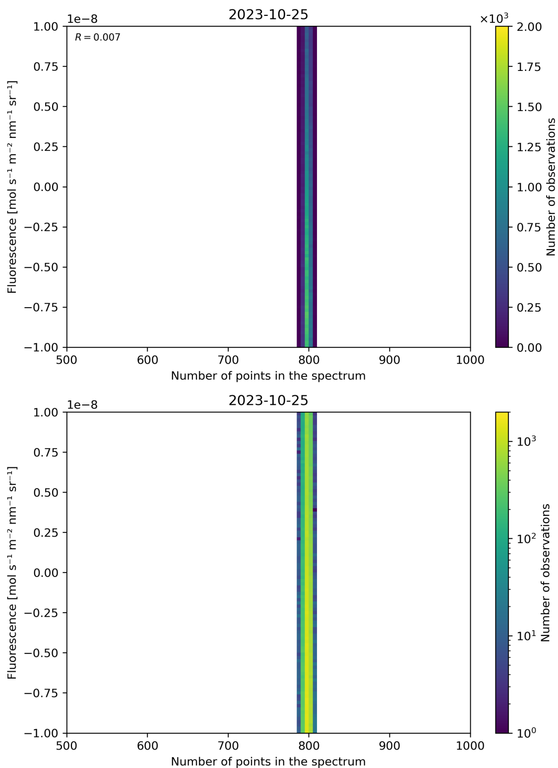
Figure 91: Scatter density plot of “Number of points in the spectrum” against “Fluorescence” for 2023-10-24 to 2023-10-26.
