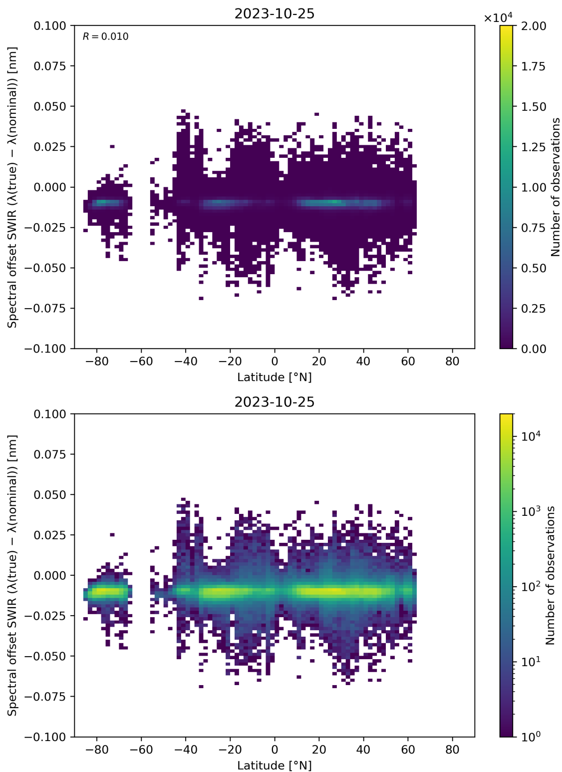
Figure 62: Scatter density plot of “Latitude” against “Spectral offset SWIR ( \lambda(\text{true}) - \lambda(\text{nominal}) )” for 2023-10-24 to 2023-10-26.
