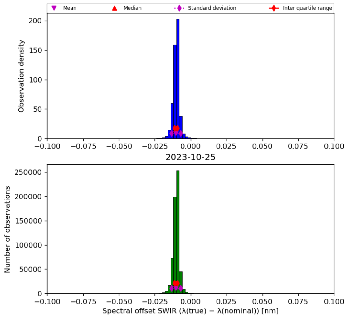
Figure 27: Histogram of “Spectral offset SWIR ( \lambda(\text{true}) - \lambda(\text{nominal}) )” for 2023-10-24 to 2023-10-26
