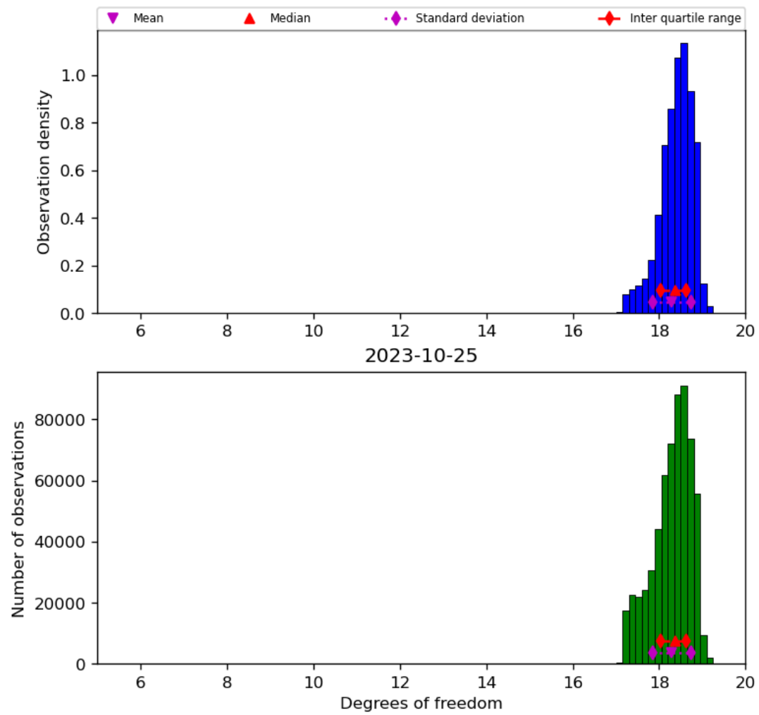
Figure 30: Histogram of “Degrees of freedom” for 2023-10-24 to 2023-10-26
