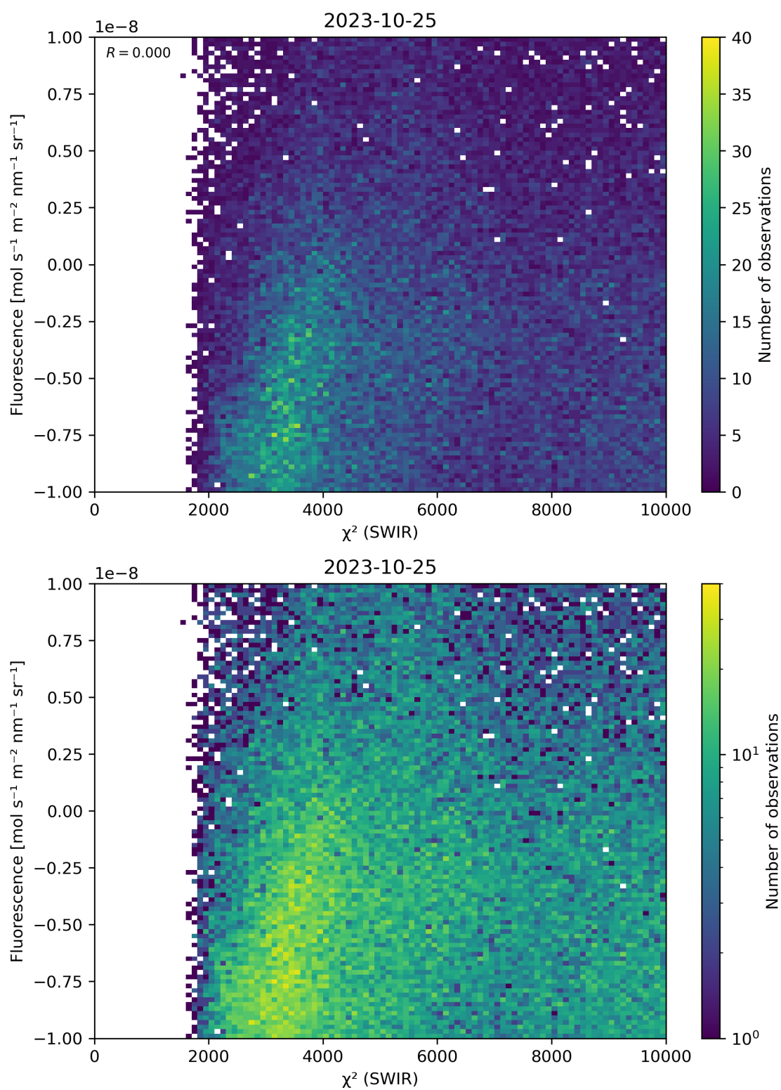
Figure 49: Scatter density plot of “ \chi^2 (SWIR)” against “Fluorescence” for 2023-10-24 to 2023-10-26.
