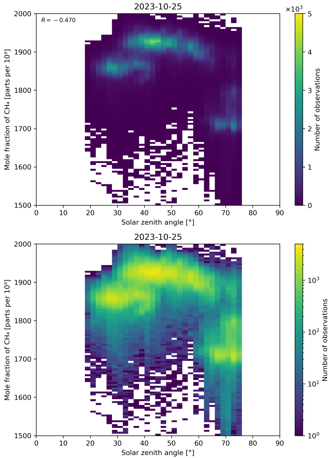
Figure 99: Scatter density plot of “Solar zenith angle” against “Mole fraction of \text{CH}_4 ” for 2023-10-24 to 2023-10-26.
