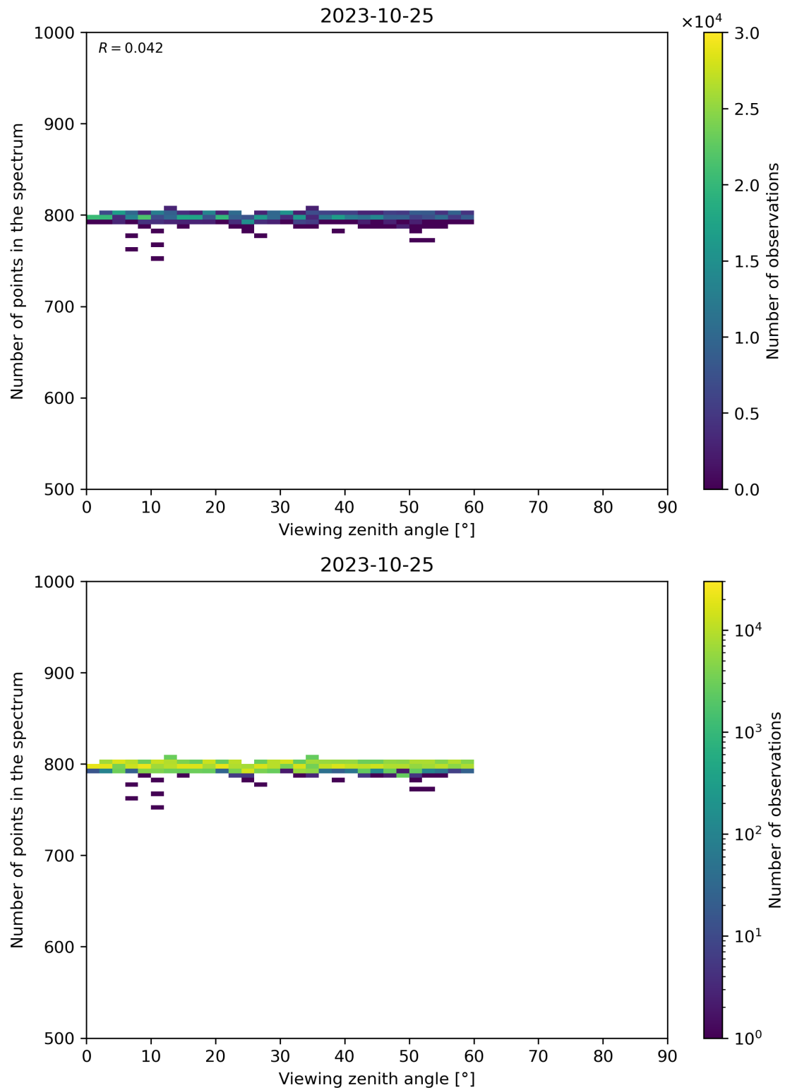
Figure 114: Scatter density plot of “Viewing zenith angle” against “Number of points in the spectrum” for 2023-10-24 to 2023-10-26.
