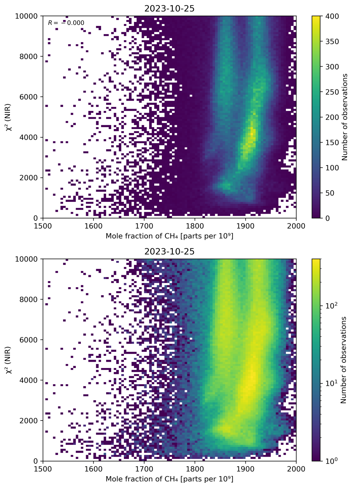
Figure 70: Scatter density plot of “Mole fraction of CH 4 ” against “ \chi^2 (NIR)” for 2023-10-24 to 2023-10-26.
