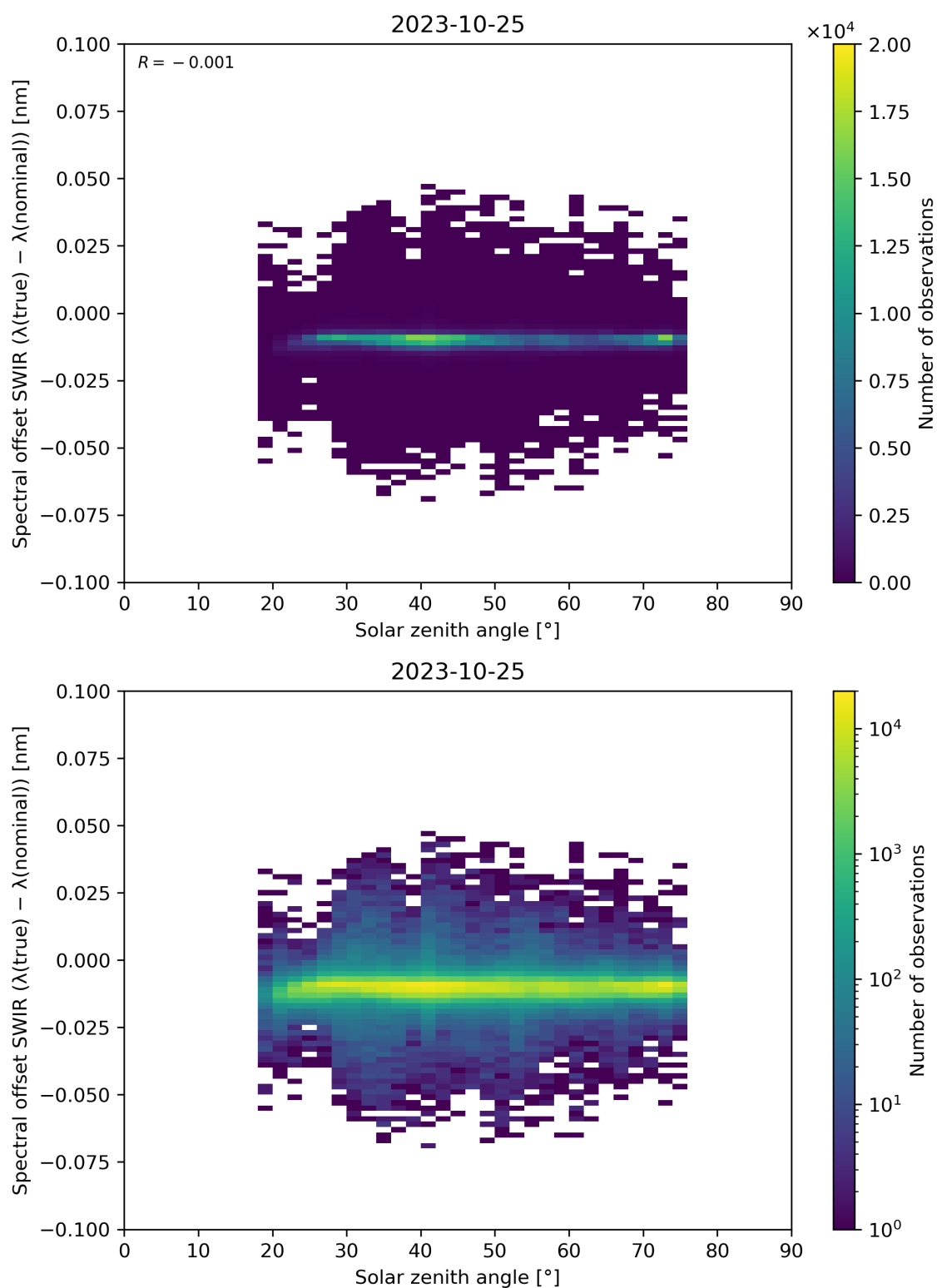
Figure 104: Scatter density plot of “Solar zenith angle” against “Spectral offset SWIR ( \lambda(\text{true}) - \lambda(\text{nominal}) )” for 2023-10-24 to 2023-10-26.
