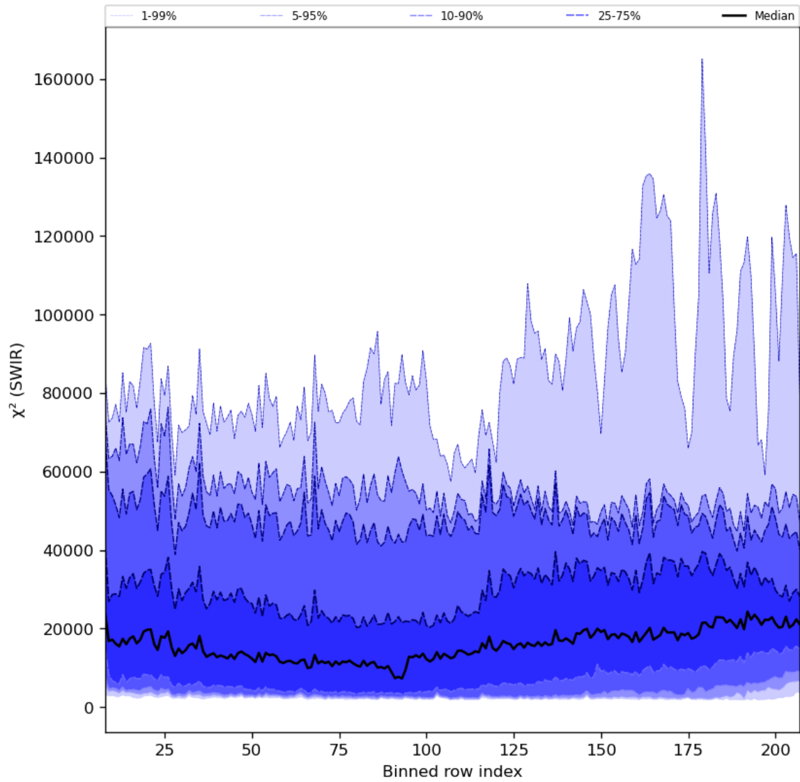
Figure 39: Along track statistics of “ \chi^2 (SWIR)” for 2023-10-24 to 2023-10-26
