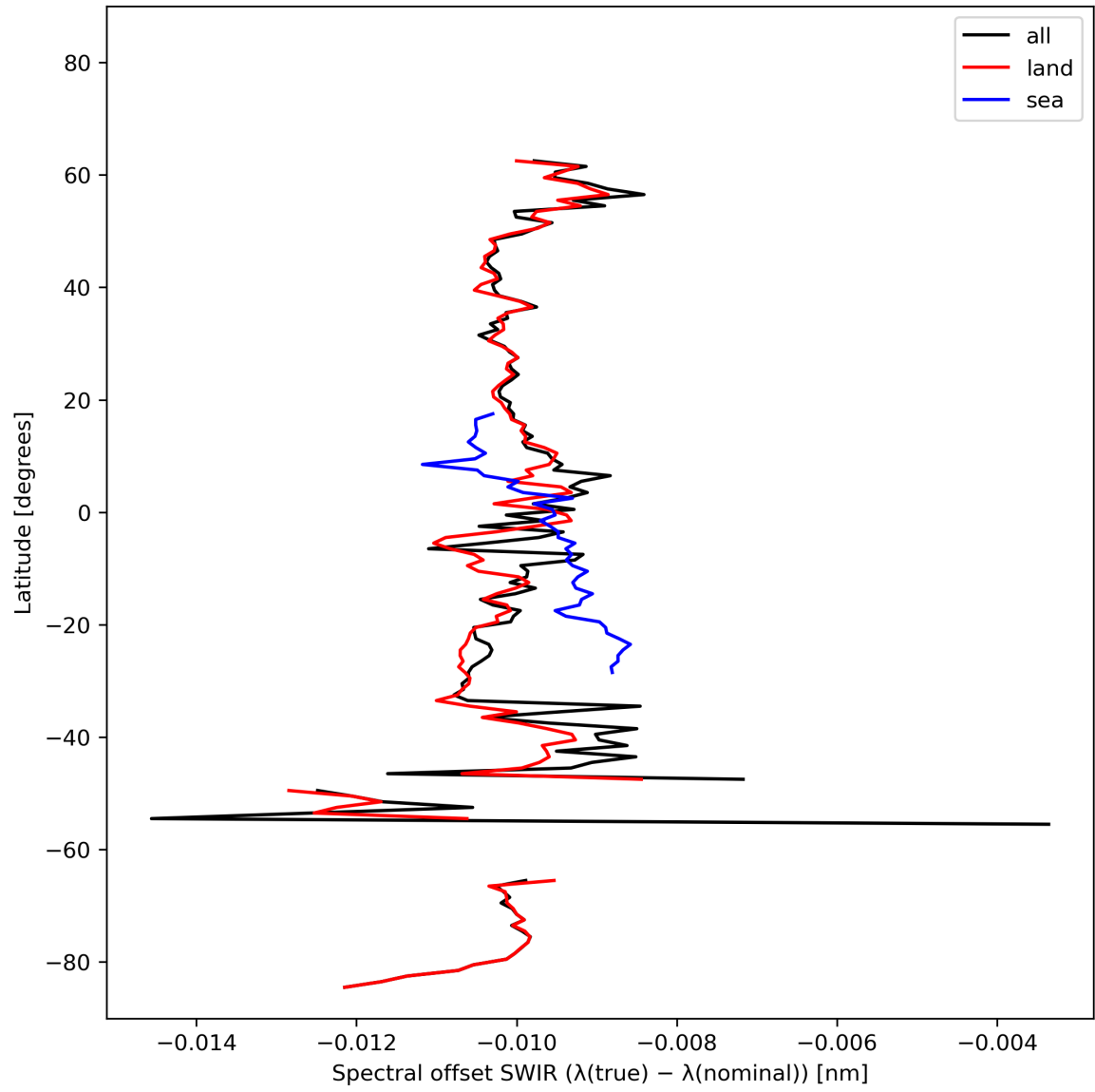
Figure 16: Zonal average of “Spectral offset SWIR ( \lambda(\text{true}) - \lambda(\text{nominal}) )” for 2023-10-24 to 2023-10-26.
