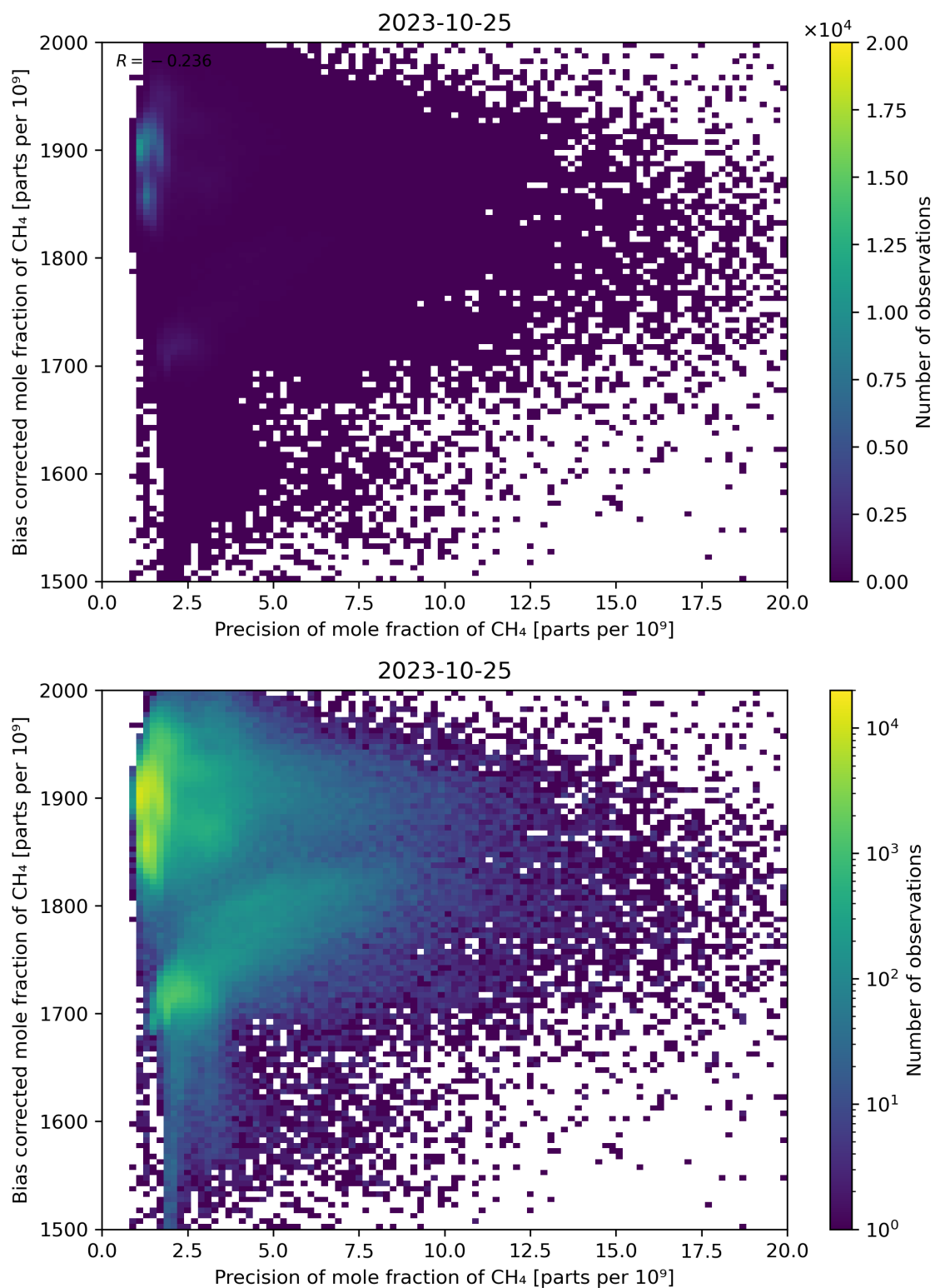
Figure 82: Scatter density plot of “Precision of mole fraction of CH 4 ” against “Bias corrected mole fraction of CH 4 ” for 2023-10-24 to 2023-10-26.
