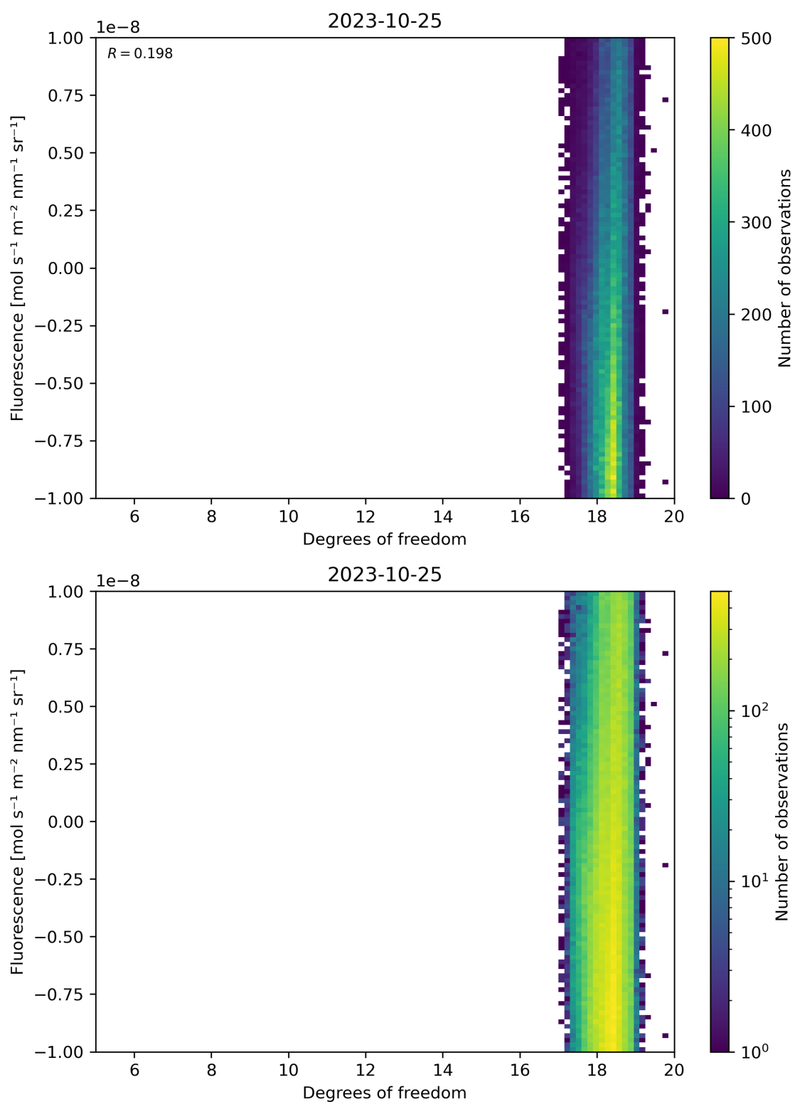
Figure 51: Scatter density plot of “Degrees of freedom” against “Fluorescence” for 2023-10-24 to 2023-10-26.
