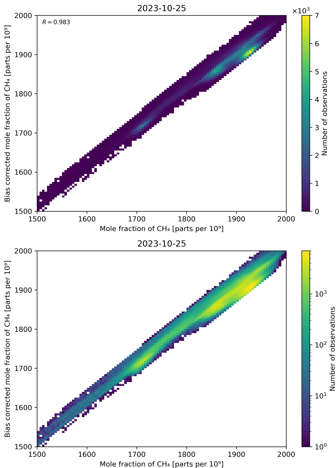
Figure 74: Scatter density plot of “Mole fraction of CH 4 ” against “Bias corrected mole fraction of CH 4 ” for 2023-10-24 to 2023-10-26.
