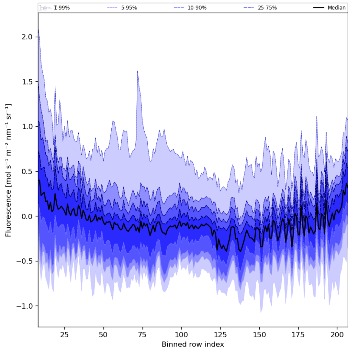
Figure 43: Along track statistics of “Fluorescence” for 2023-10-24 to 2023-10-26
