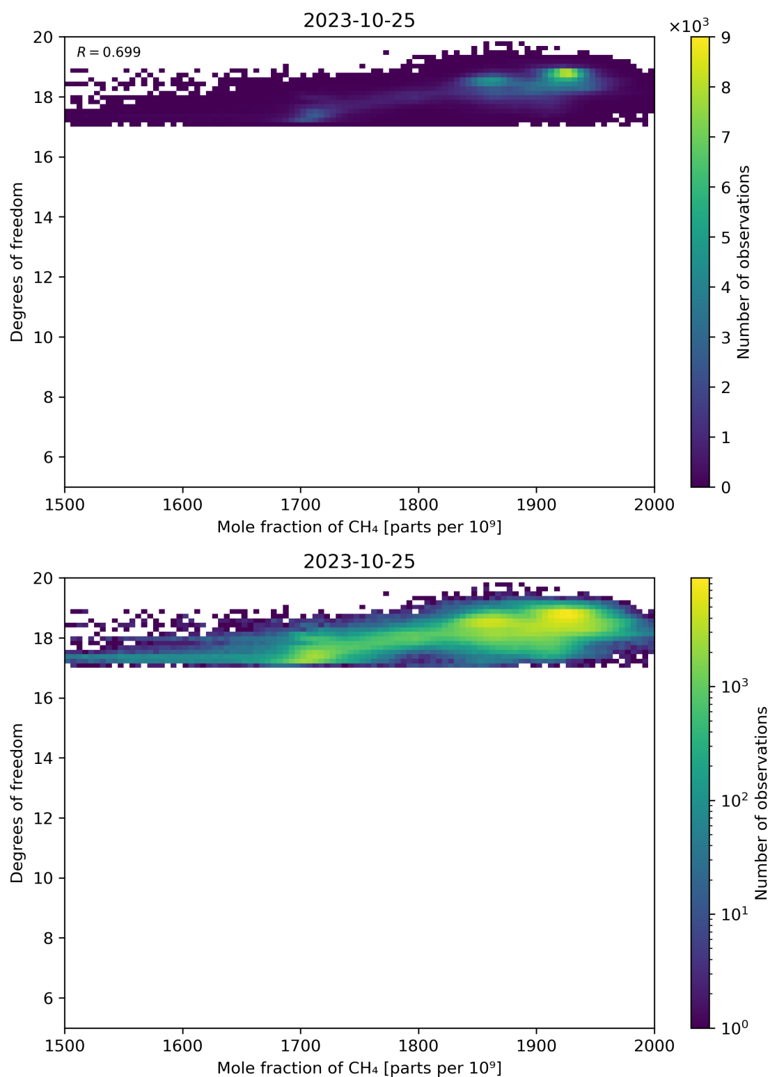
Figure 72: Scatter density plot of “Mole fraction of CH 4 ” against “Degrees of freedom” for 2023-10-24 to 2023-10-26.
