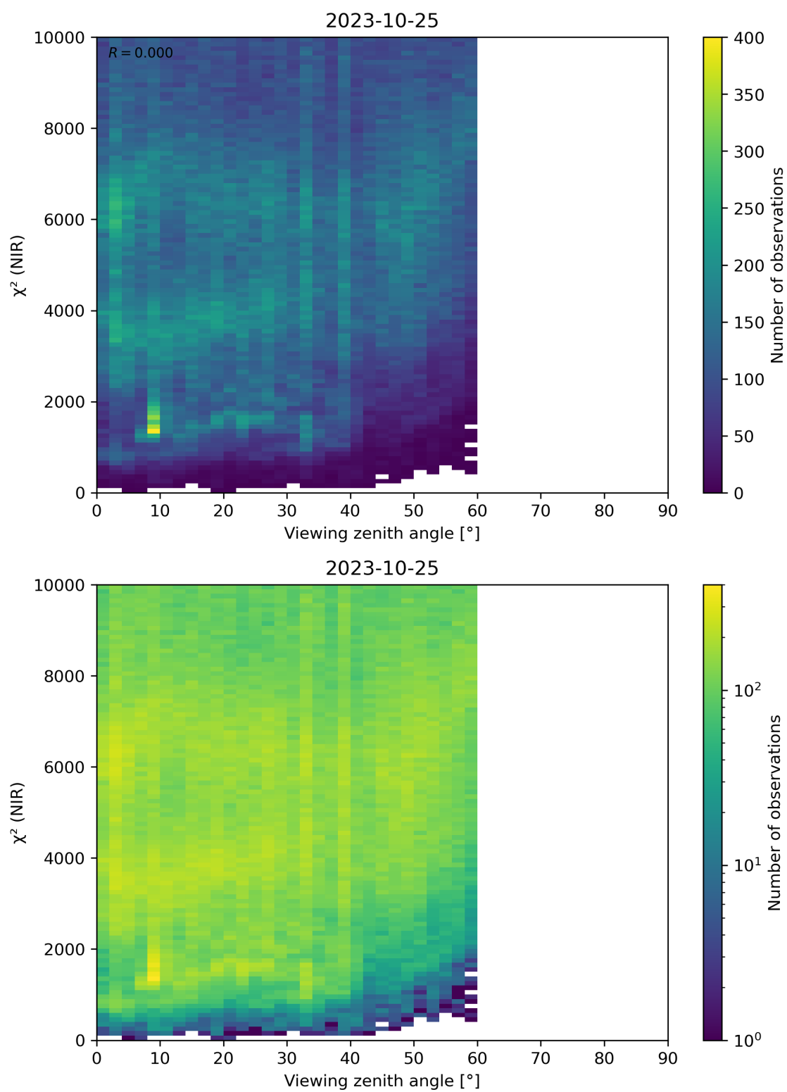
Figure 105: Scatter density plot of “Viewing zenith angle” against “ \chi^2 (NIR)” for 2023-10-24 to 2023-10-26.
