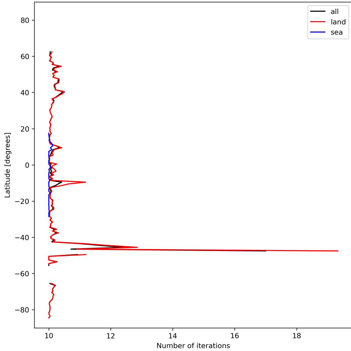
Figure 20: Zonal average of “Number of iterations” for 2023-10-24 to 2023-10-26.
