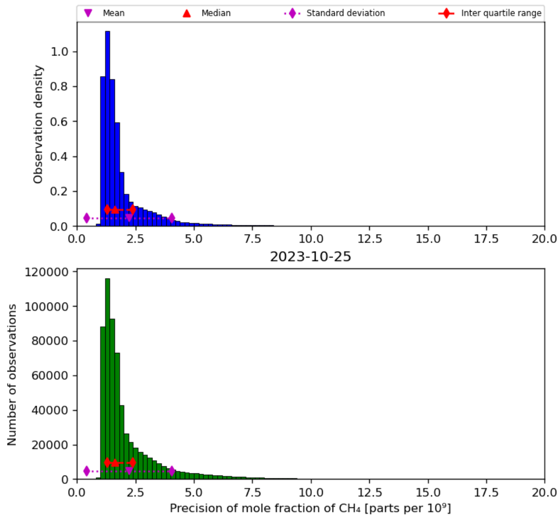
Figure 24: Histogram of “Precision of mole fraction of CH 4 ” for 2023-10-24 to 2023-10-26
