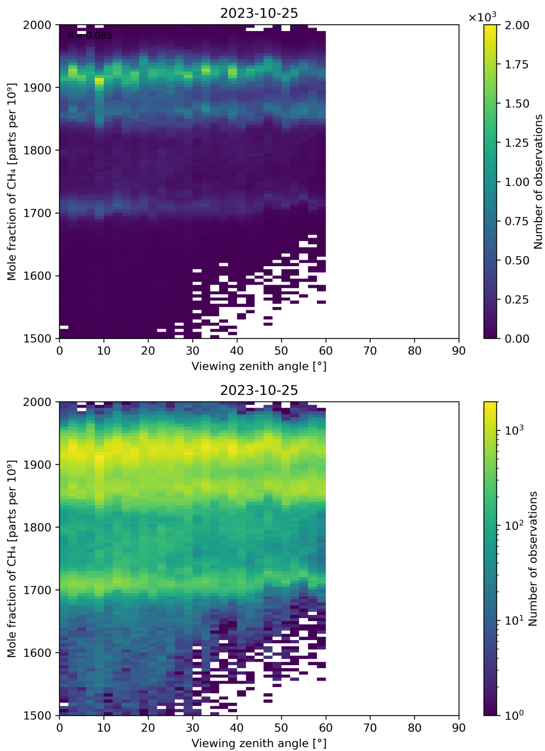
Figure 110: Scatter density plot of “Viewing zenith angle” against “Mole fraction of \text{CH}_4 ” for 2023-10-24 to 2023-10-26.
