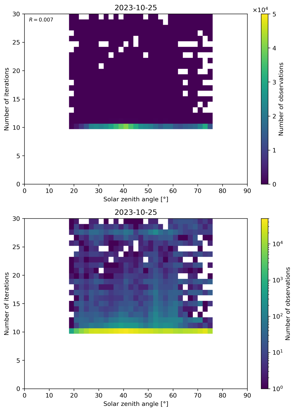
Figure 102: Scatter density plot of “Solar zenith angle” against “Number of iterations” for 2023-10-24 to 2023-10-26.
