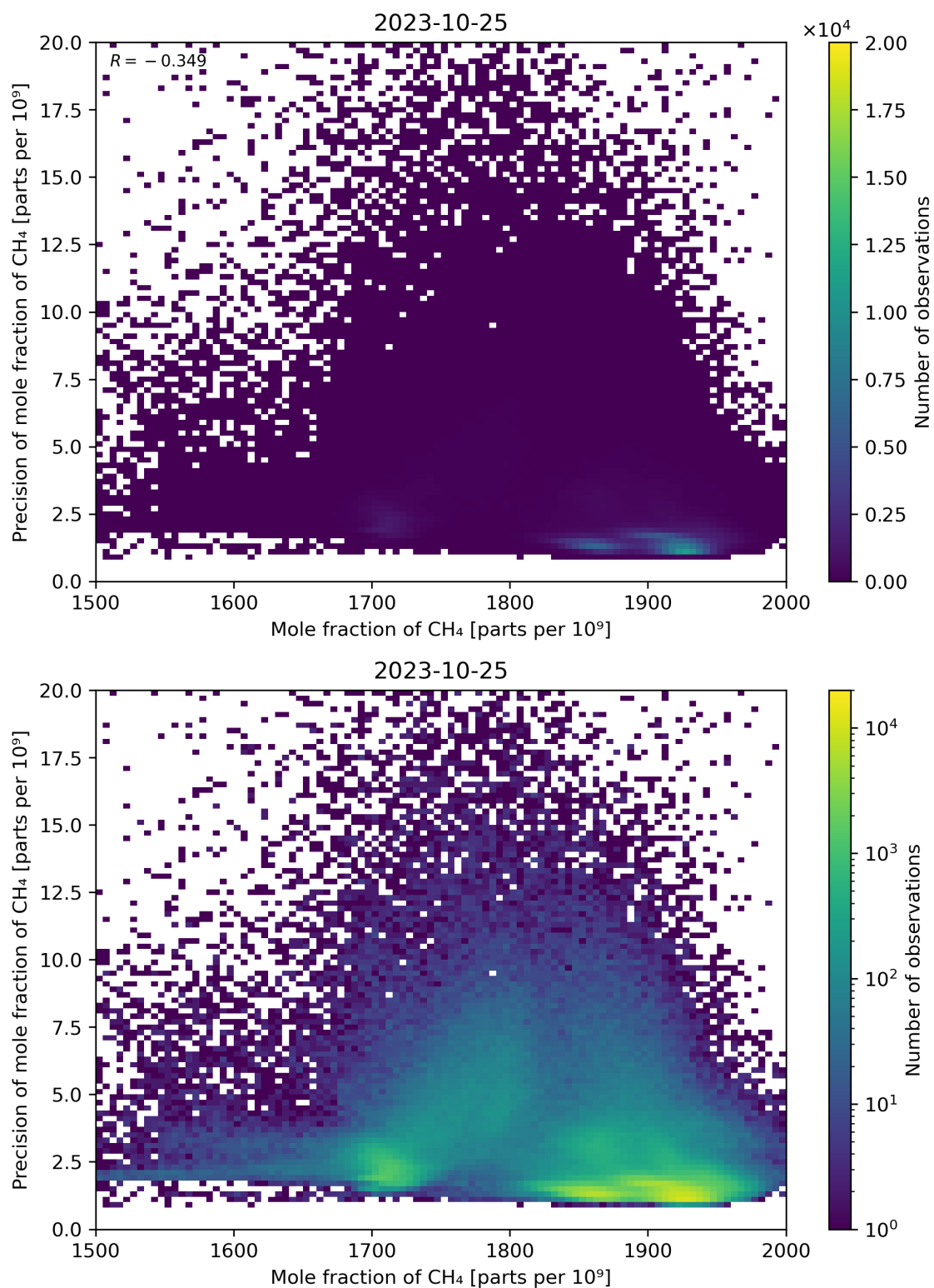
Figure 75: Scatter density plot of “Mole fraction of CH 4 ” against “Precision of mole fraction of CH 4 ” for 2023-10-24 to 2023-10-26.
