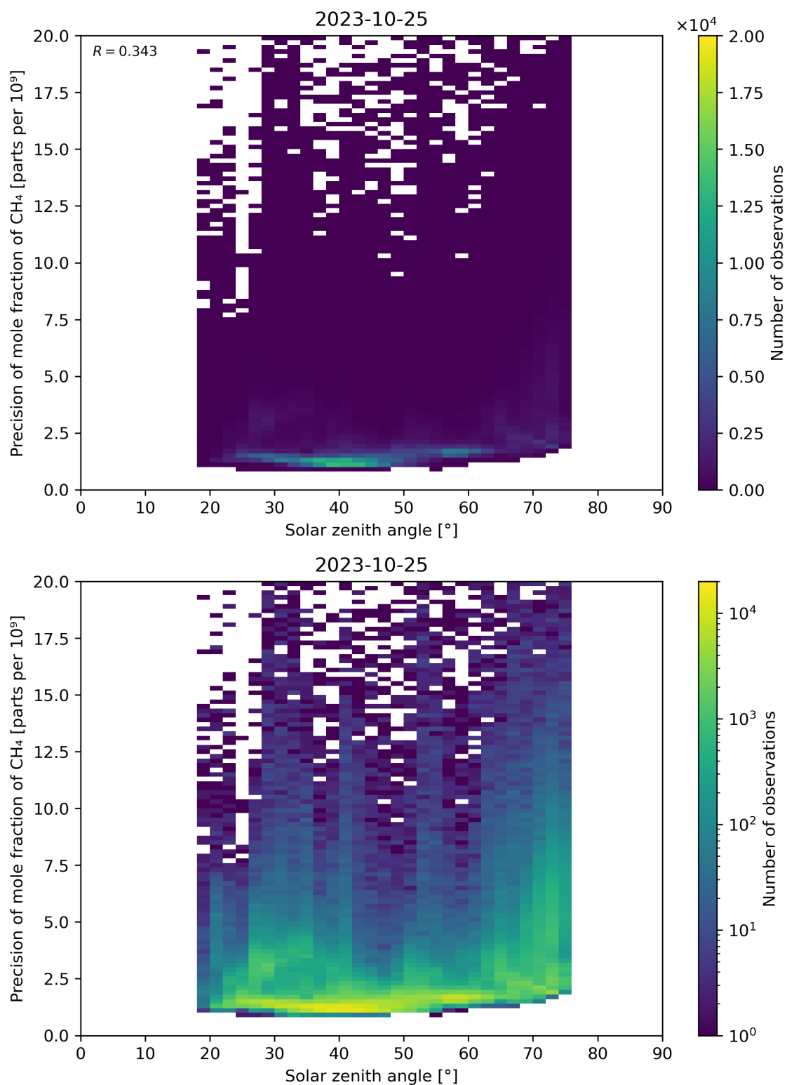
Figure 101: Scatter density plot of “Solar zenith angle” against “Precision of mole fraction of \text{CH}_4 ” for 2023-10-24 to 2023-10-26.
