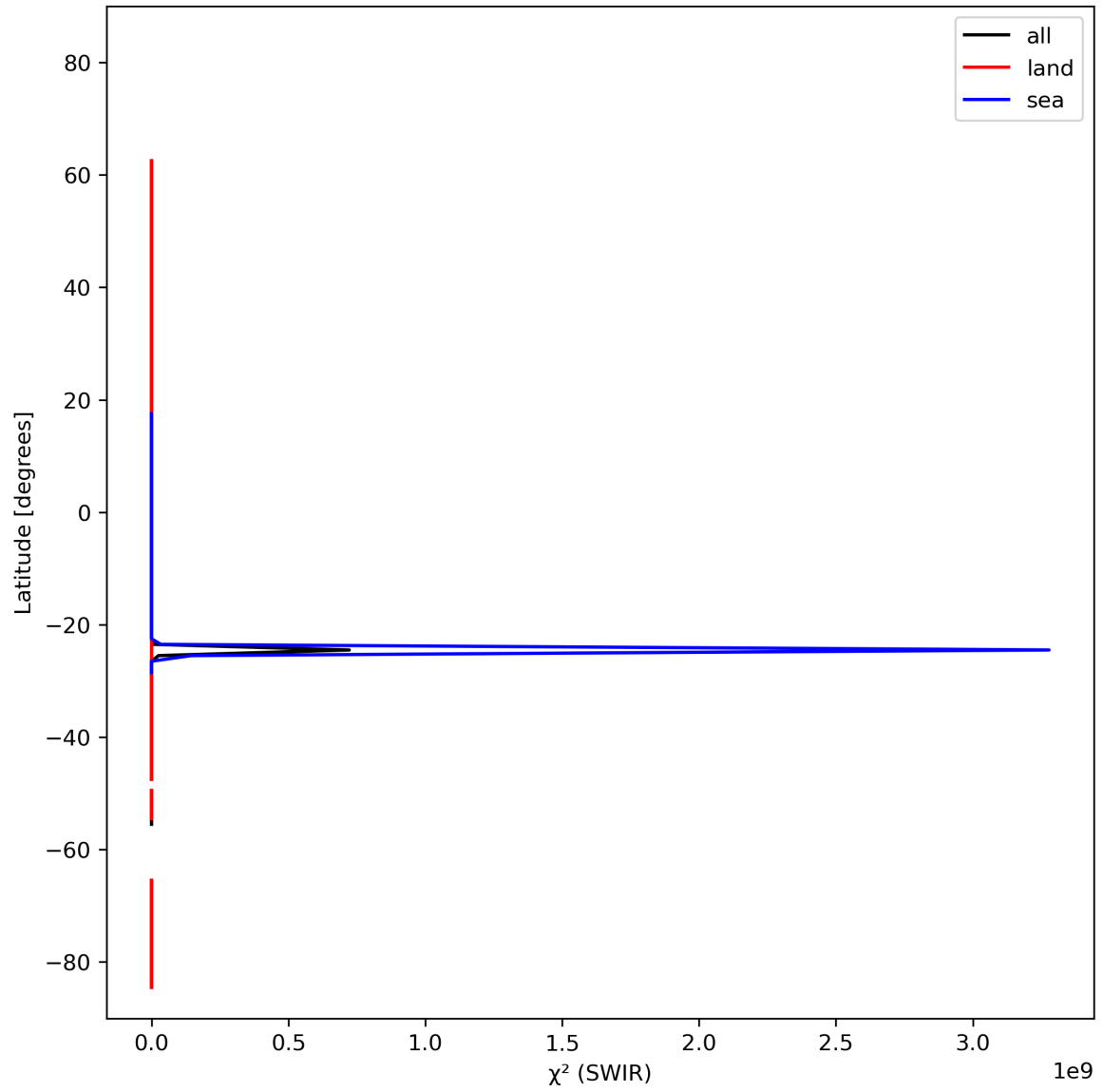
Figure 17: Zonal average of “ \chi^2 (SWIR)” for 2023-10-24 to 2023-10-26.
