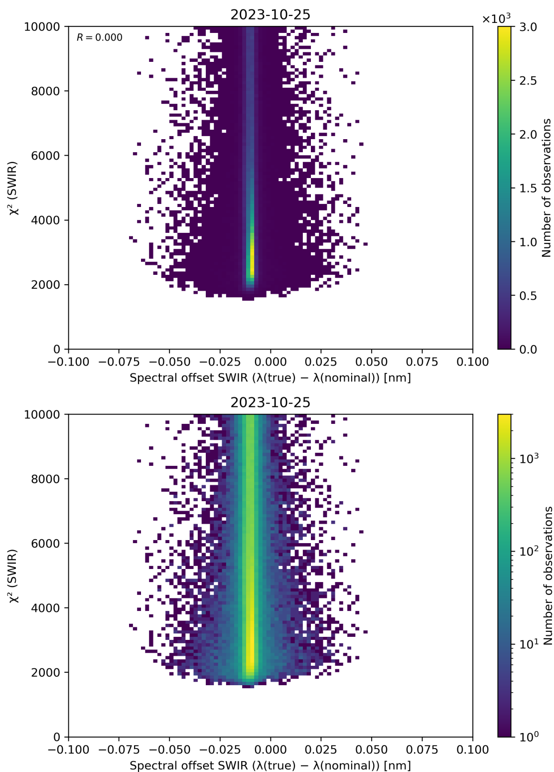
Figure 118: Scatter density plot of “Spectral offset SWIR ( \lambda(\text{true}) - \lambda(\text{nominal}) )” against “ \chi^2 (SWIR)” for 2023-10-24 to 2023-10-26.
