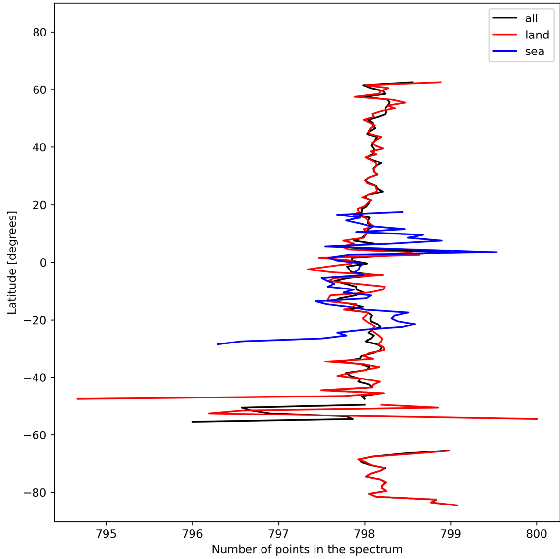
Figure 15: Zonal average of “Number of points in the spectrum” for 2023-10-24 to 2023-10-26.
