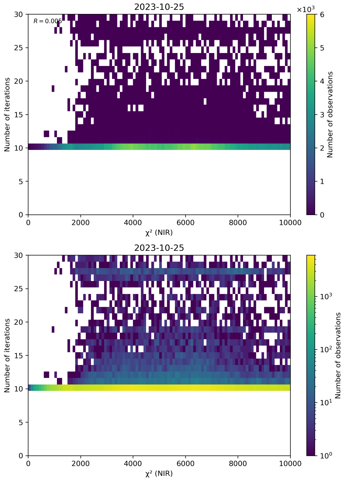
Figure 46: Scatter density plot of “ \chi^2 (NIR)” against “Number of iterations” for 2023-10-24 to 2023-10-26.
