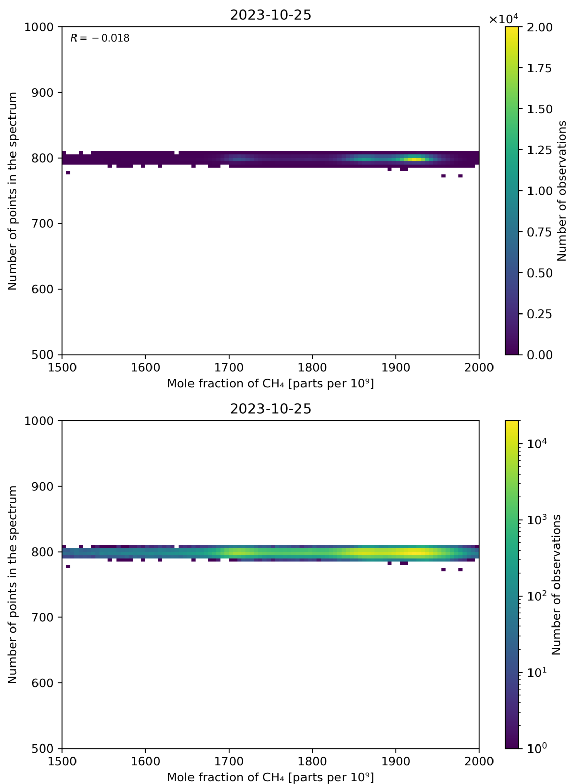
Figure 77: Scatter density plot of “Mole fraction of CH 4 ” against “Number of points in the spectrum” for 2023-10-24 to 2023-10-26.
