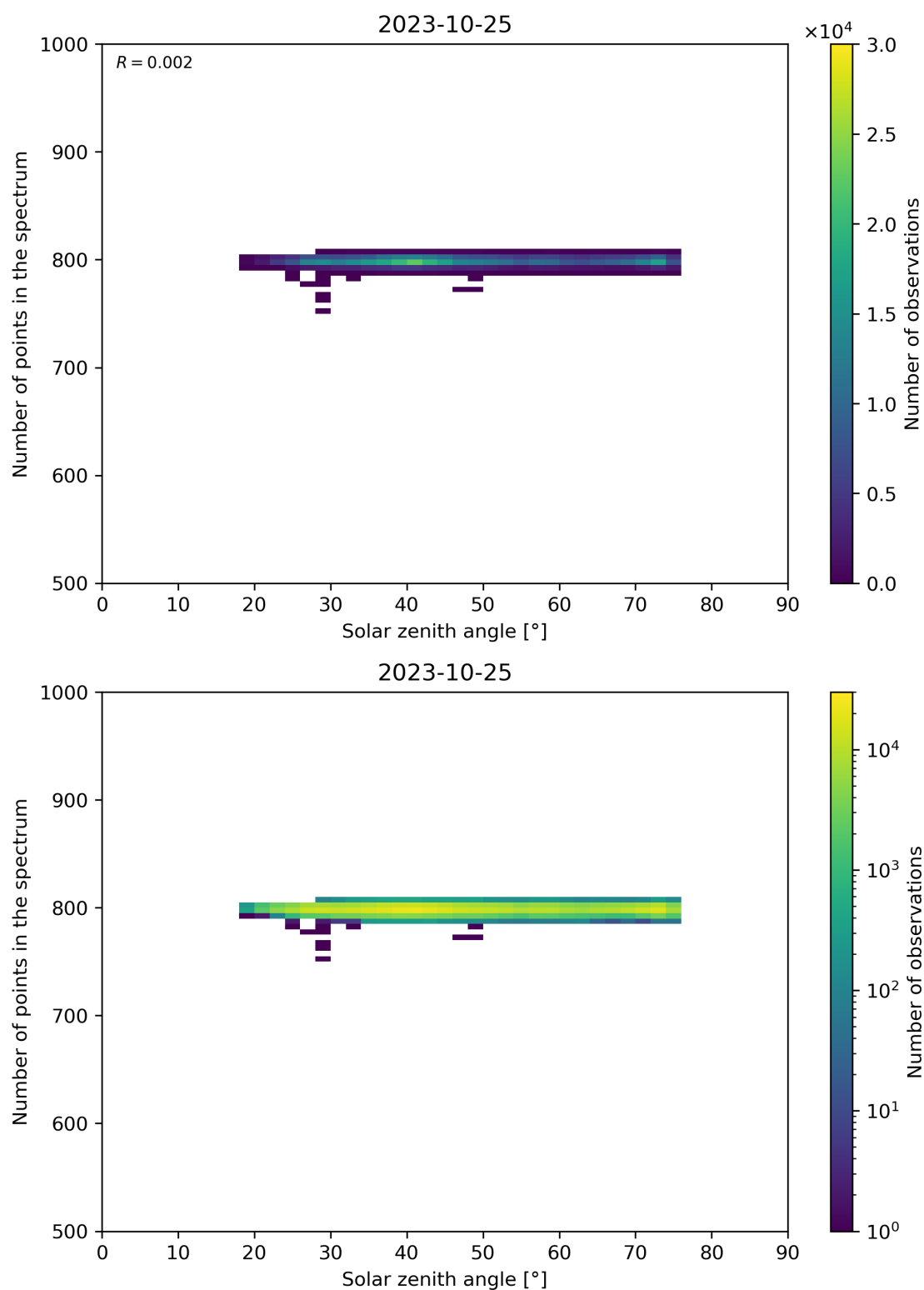
Figure 103: Scatter density plot of “Solar zenith angle” against “Number of points in the spectrum” for 2023-10-24 to 2023-10-26.
