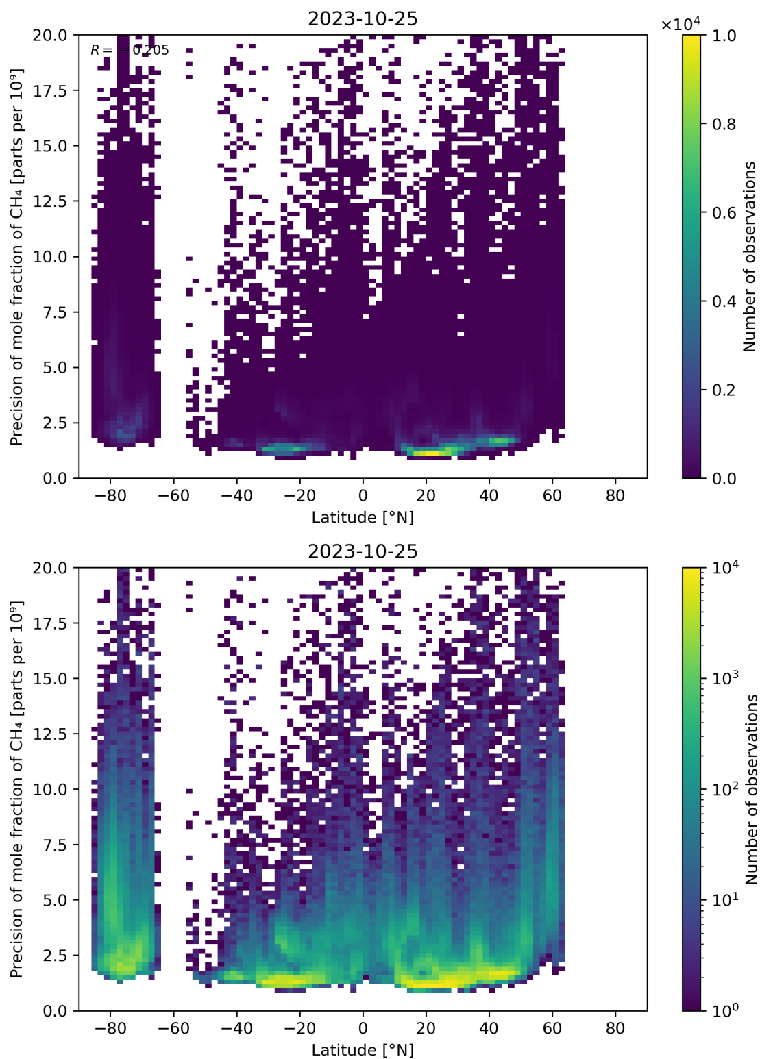
Figure 59: Scatter density plot of “Latitude” against “Precision of mole fraction of \text{CH}_4 ” for 2023-10-24 to 2023-10-26.
