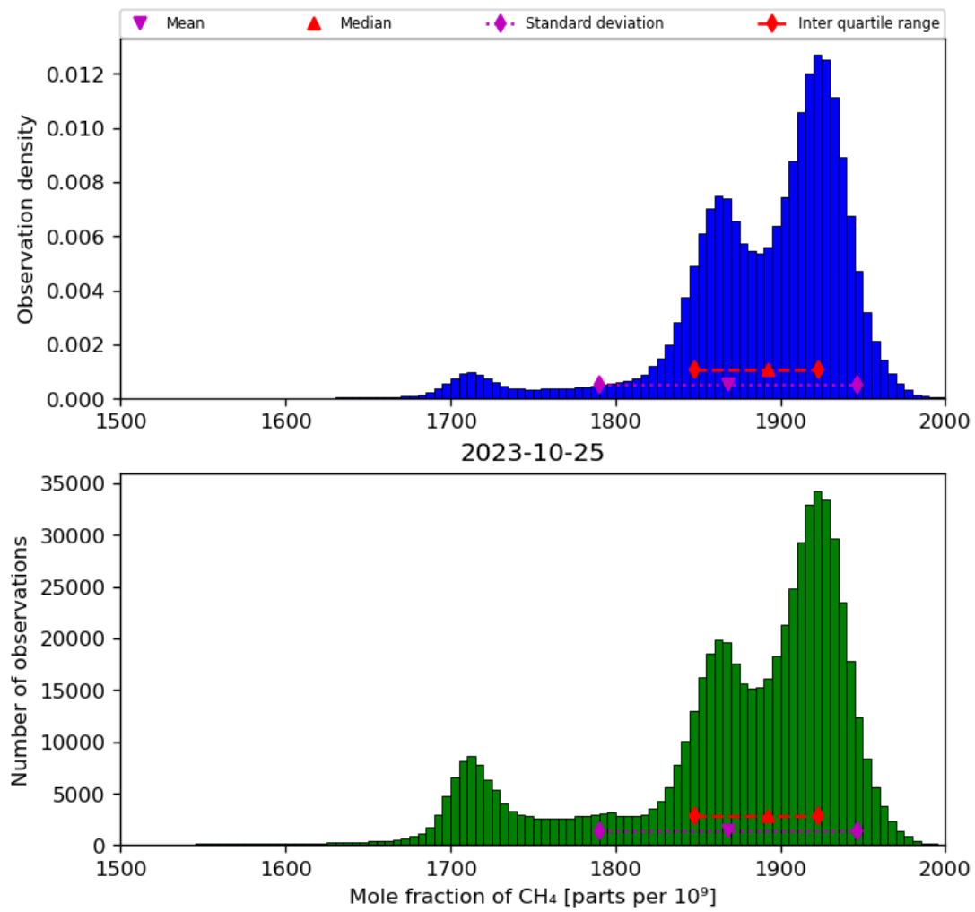
Figure 23: Histogram of “Mole fraction of CH 4 ” for 2023-10-24 to 2023-10-26
