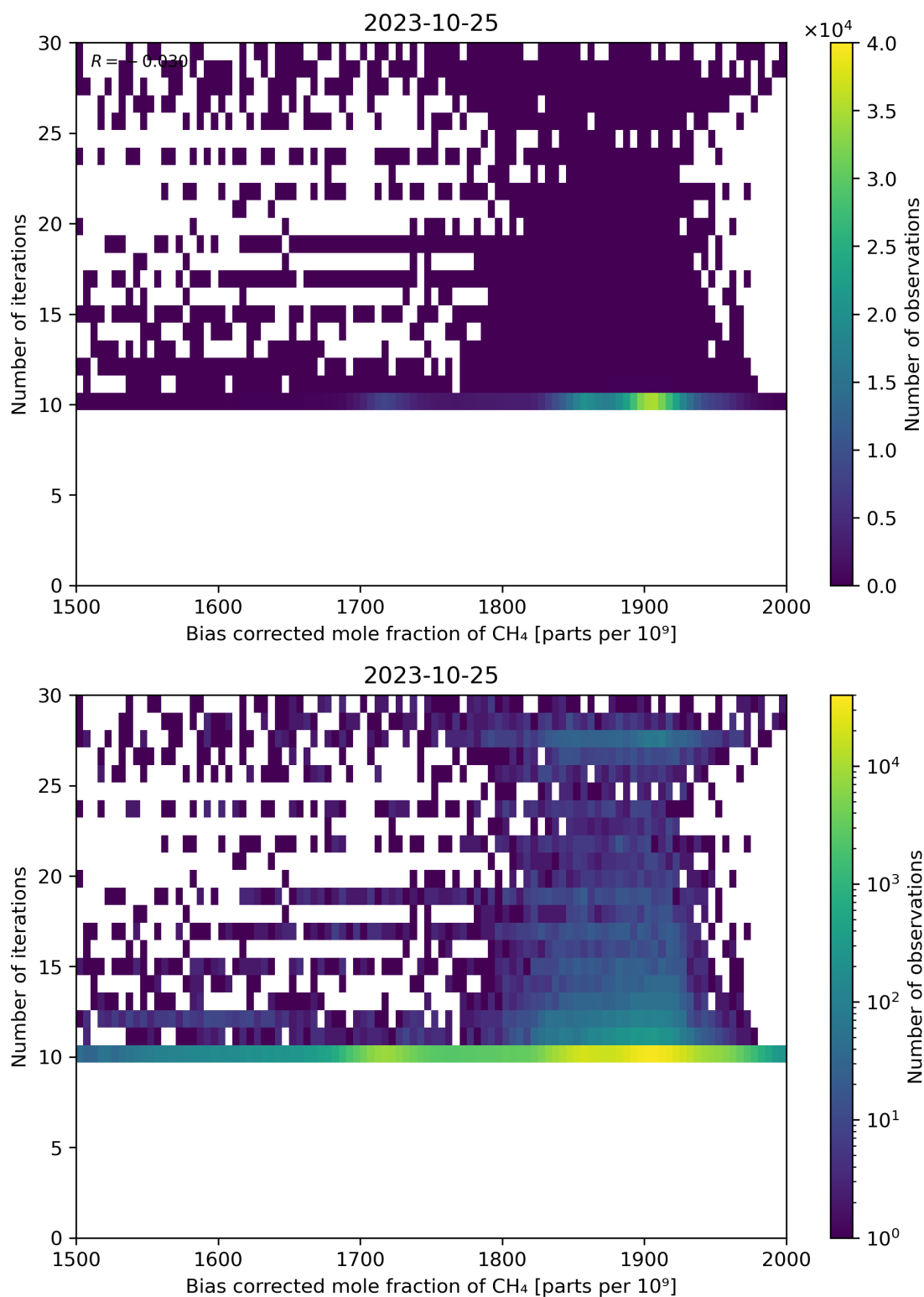
Figure 67: Scatter density plot of “Bias corrected mole fraction of \text{CH}_4 ” against “Number of iterations” for 2023-10-24 to 2023-10-26.
