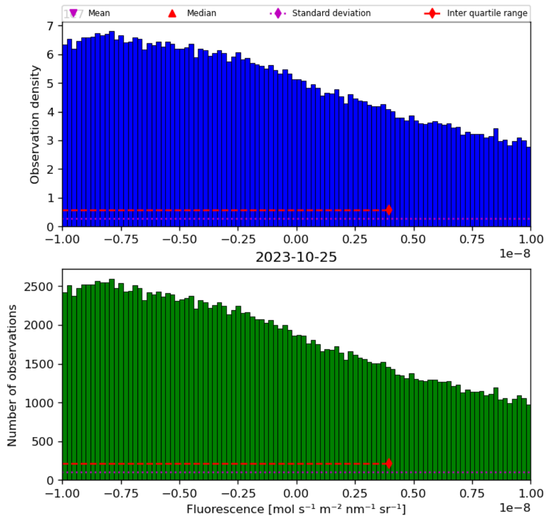
Figure 32: Histogram of “Fluorescence” for 2023-10-24 to 2023-10-26
