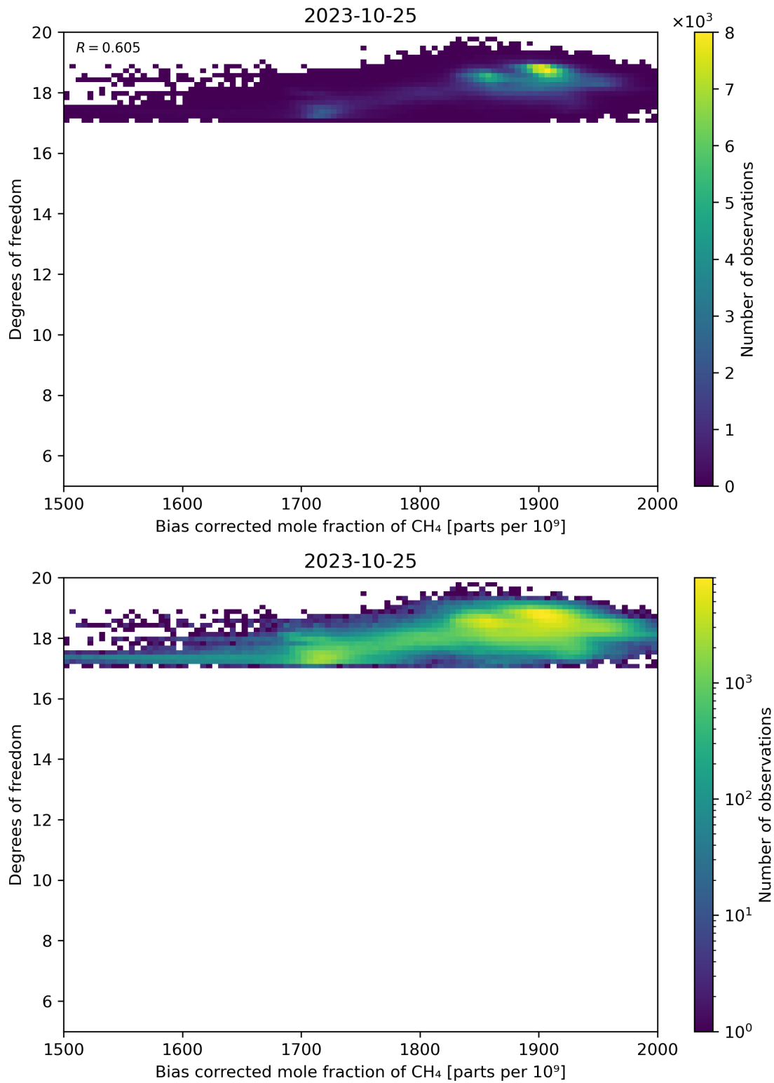
Figure 65: Scatter density plot of “Bias corrected mole fraction of CH 4 ” against “Degrees of freedom” for 2023-10-24 to 2023-10-26.
