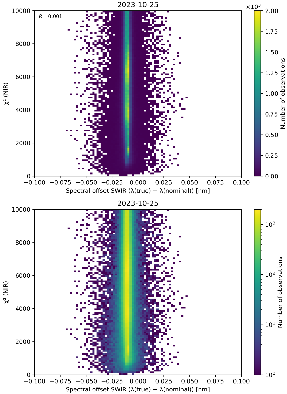
Figure 117: Scatter density plot of “Spectral offset SWIR ( \lambda(\text{true}) - \lambda(\text{nominal}) )” against “ \chi^2 (NIR)” for 2023-10-24 to 2023-10-26.
