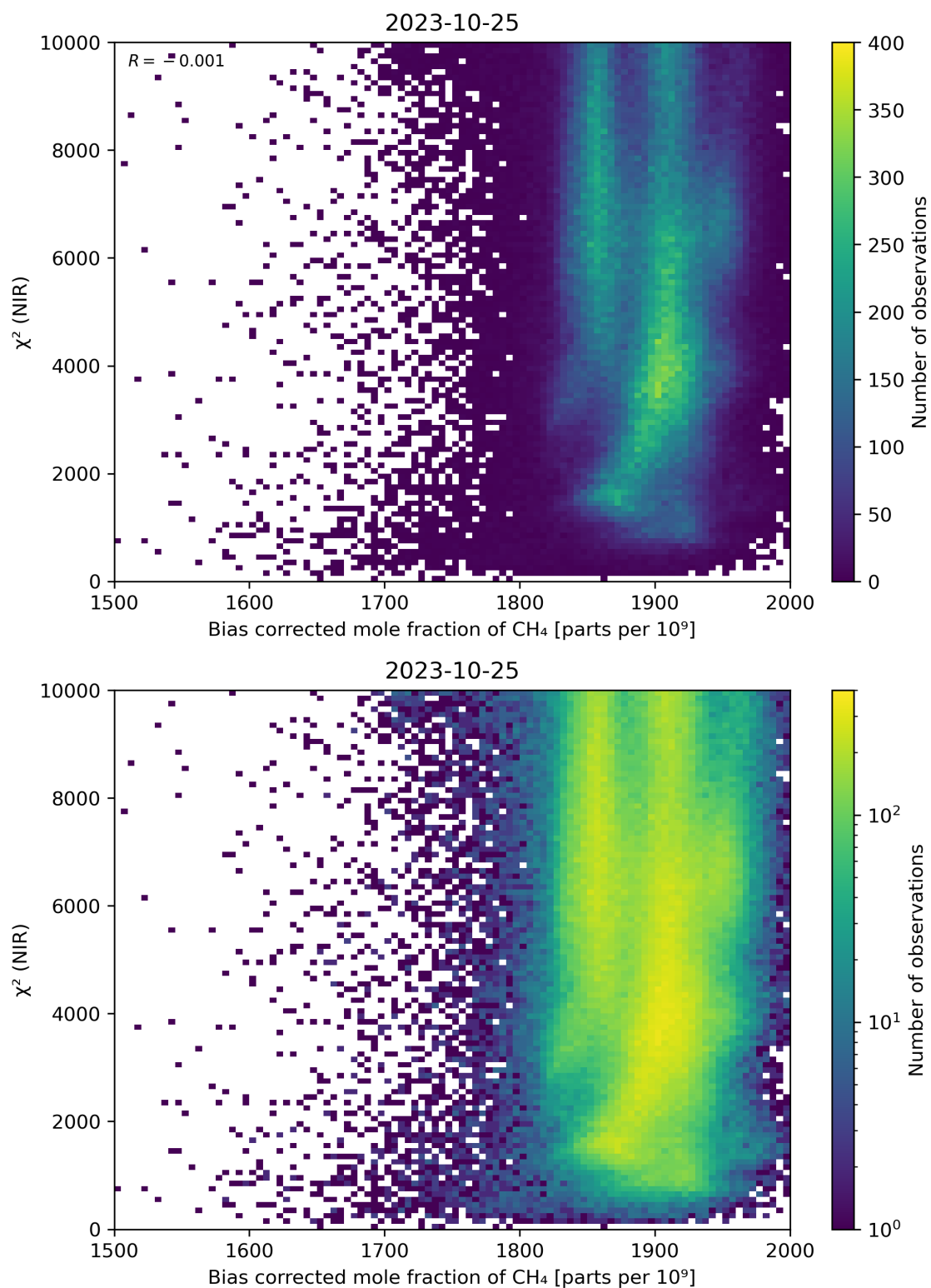
Figure 63: Scatter density plot of “Bias corrected mole fraction of CH 4 ” against “ \chi^2 (NIR)” for 2023-10-24 to 2023-10-26.
