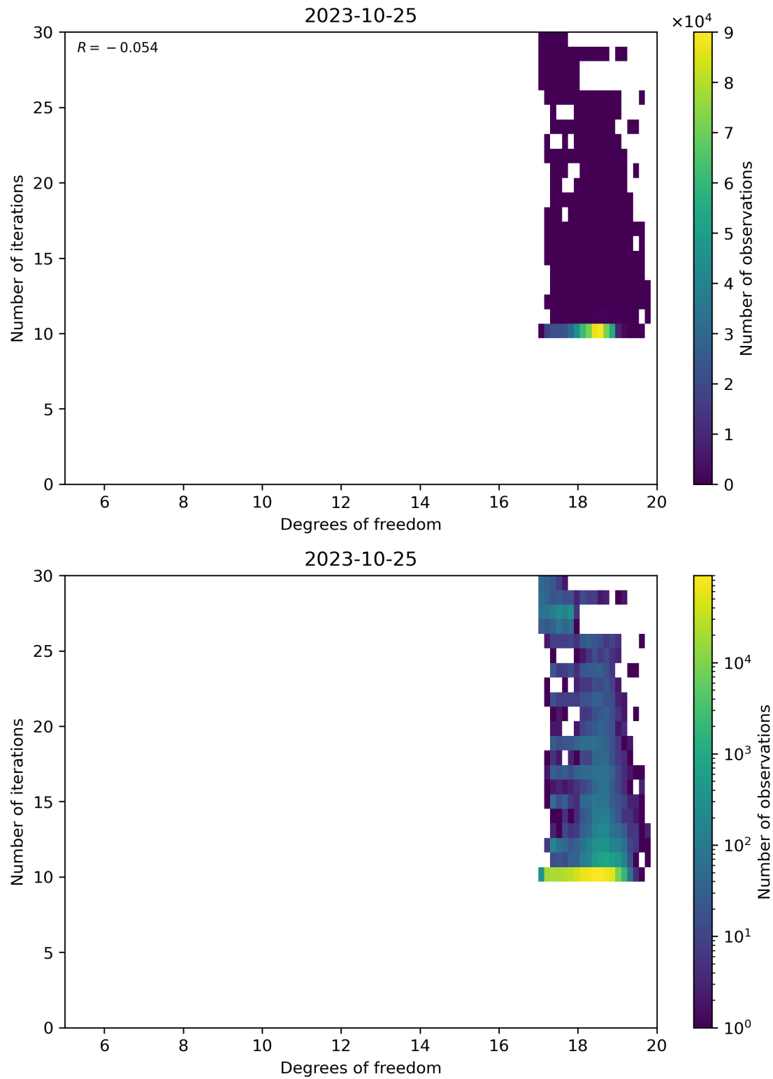
Figure 52: Scatter density plot of “Degrees of freedom” against “Number of iterations” for 2023-10-24 to 2023-10-26.
