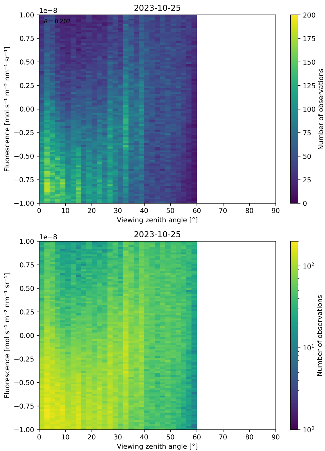
Figure 108: Scatter density plot of “Viewing zenith angle” against “Fluorescence” for 2023-10-24 to 2023-10-26.
