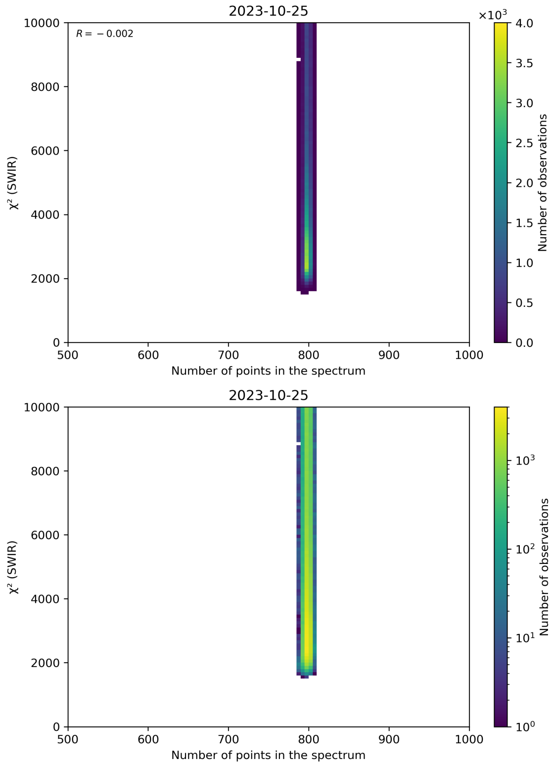
Figure 89: Scatter density plot of “Number of points in the spectrum” against “ \chi^2 (SWIR)” for 2023-10-24 to 2023-10-26.
