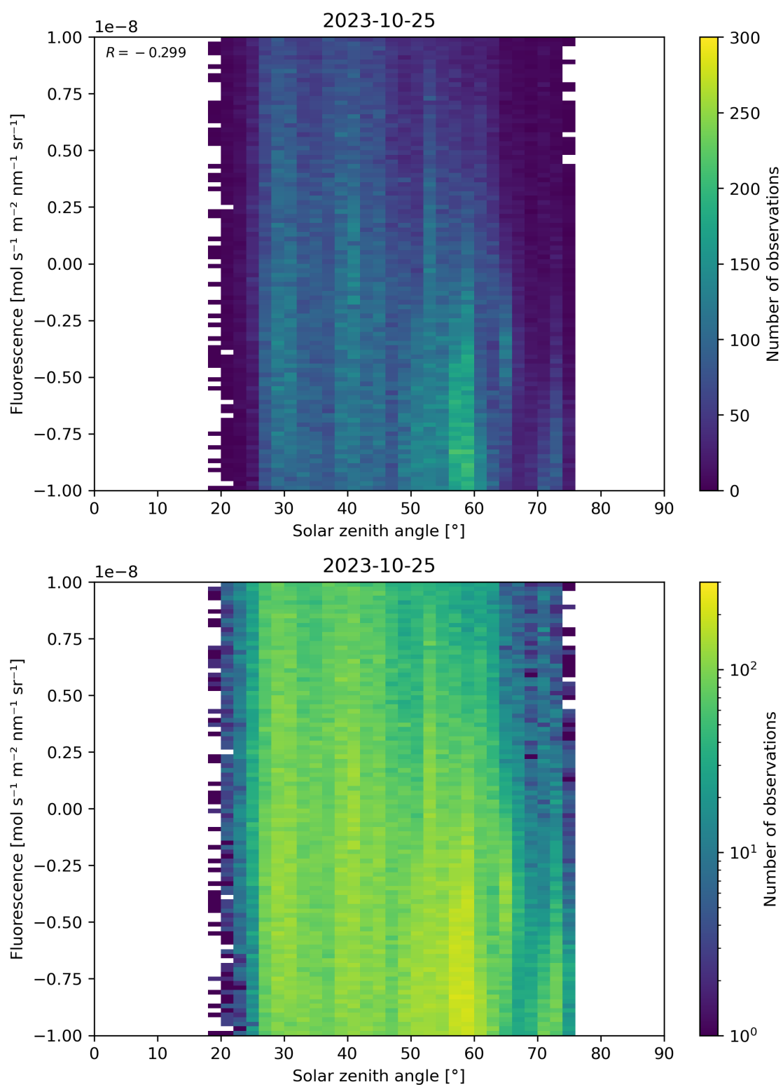
Figure 97: Scatter density plot of “Solar zenith angle” against “Fluorescence” for 2023-10-24 to 2023-10-26.
