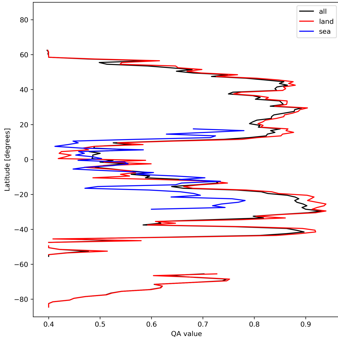
Figure 11: Zonal average of “QA value” for 2023-10-24 to 2023-10-26.
