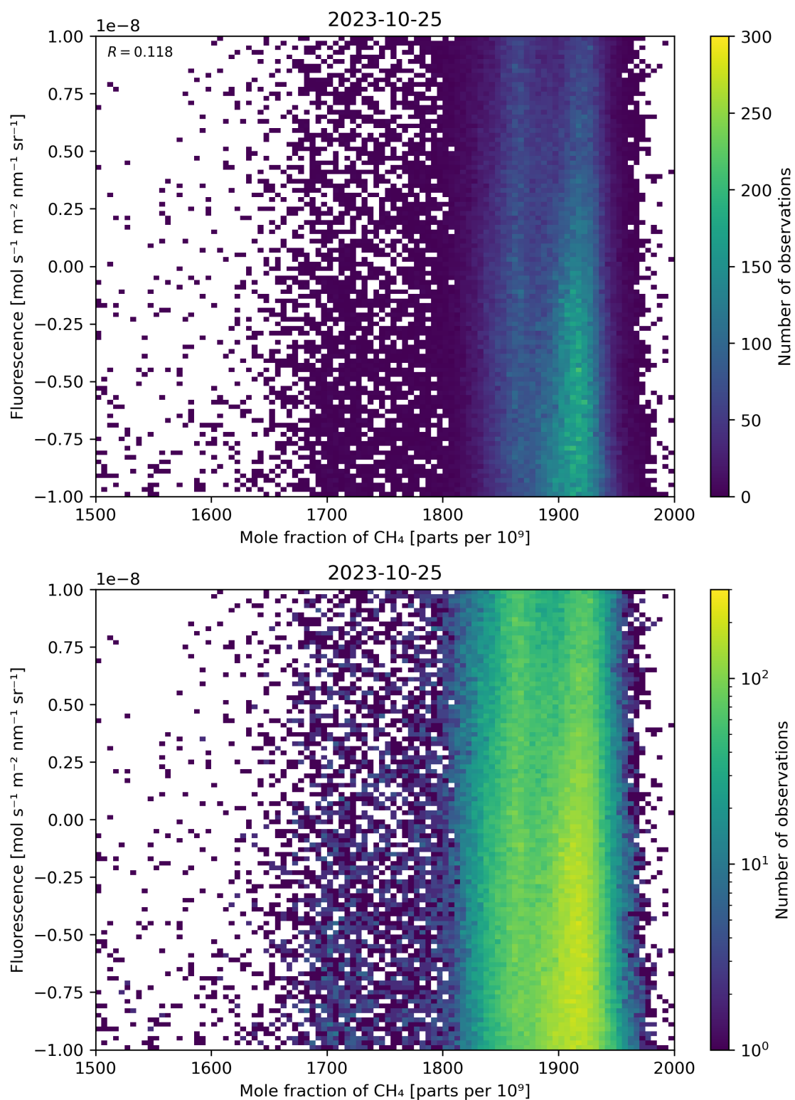
Figure 73: Scatter density plot of “Mole fraction of \text{CH}_4 ” against “Fluorescence” for 2023-10-24 to 2023-10-26.
