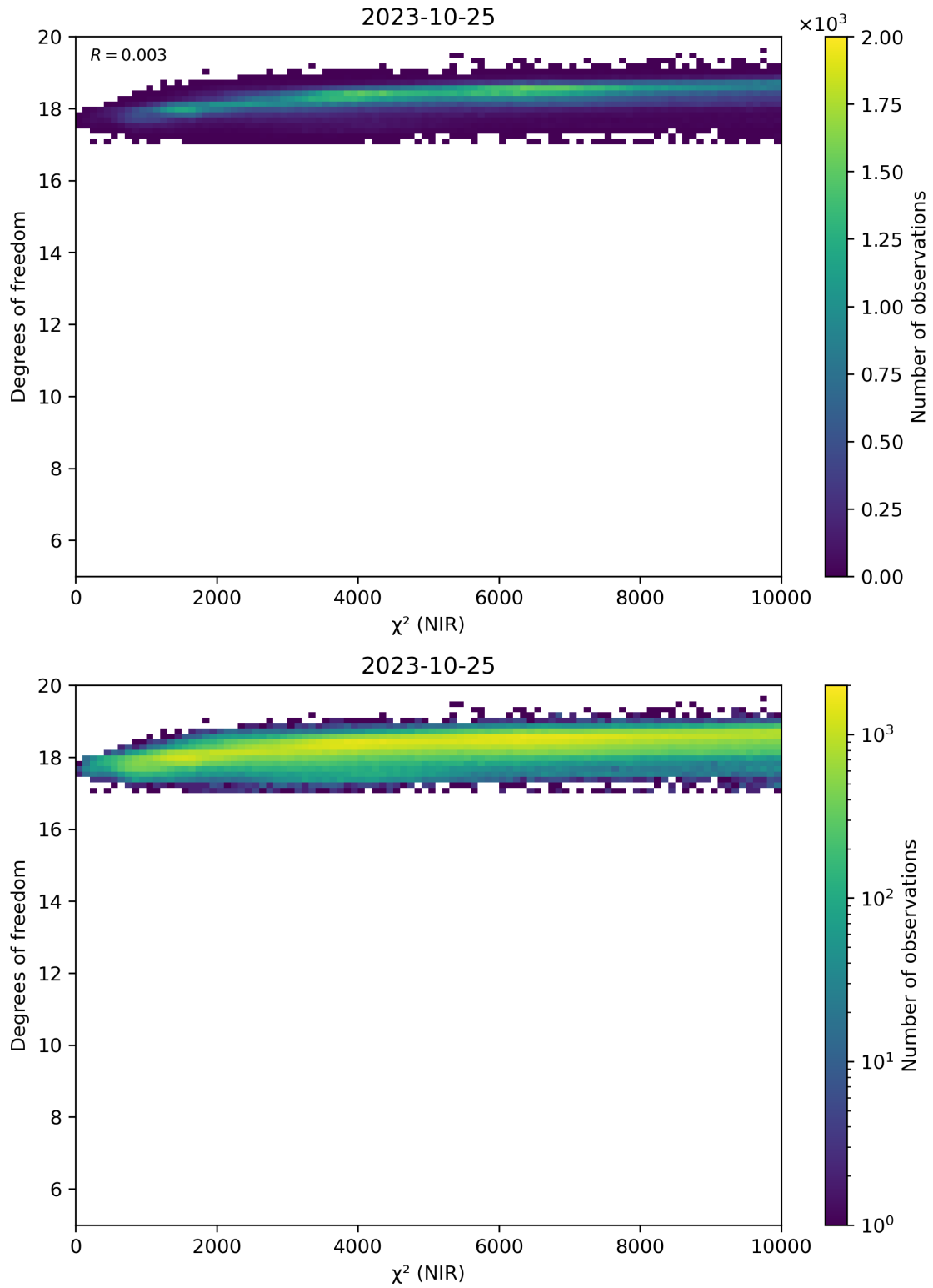
Figure 44: Scatter density plot of “ \chi^2 (NIR)” against “Degrees of freedom” for 2023-10-24 to 2023-10-26.
