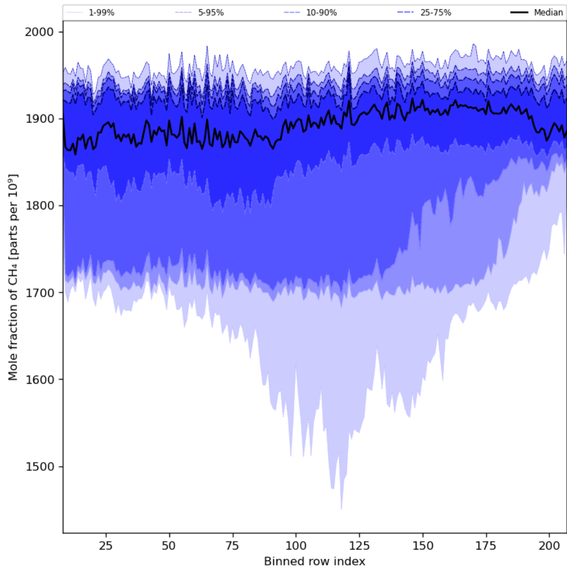
Figure 34: Along track statistics of “Mole fraction of CH 4 ” for 2023-10-24 to 2023-10-26
