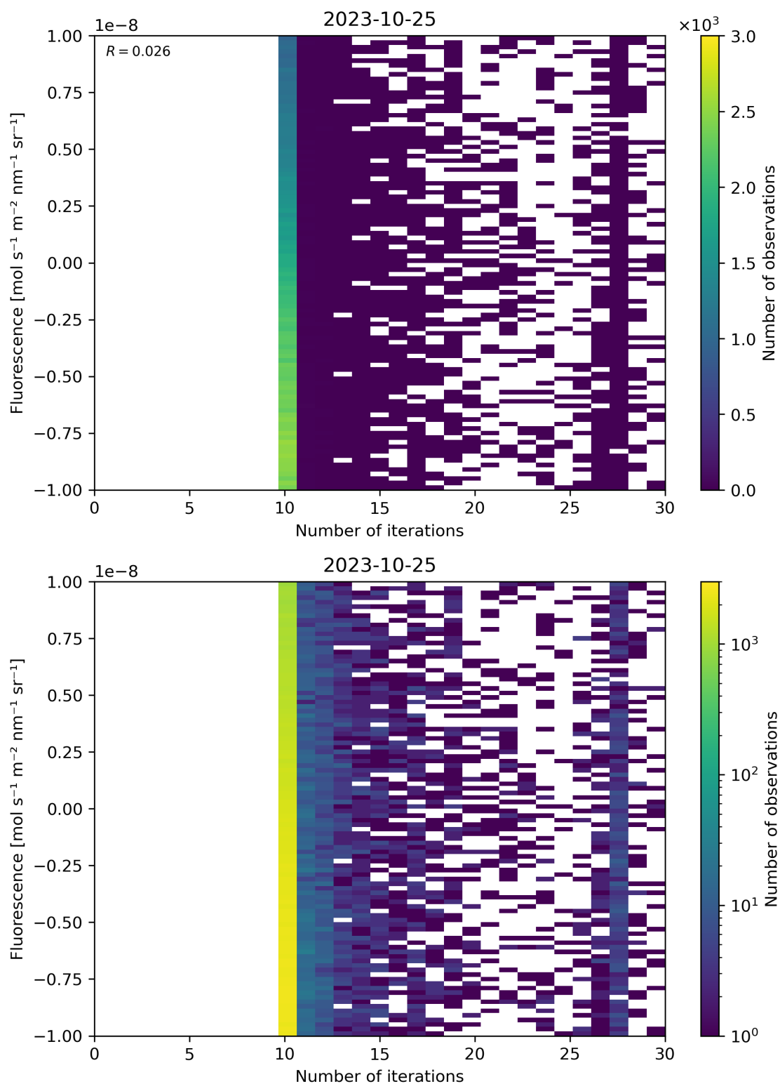
Figure 87: Scatter density plot of “Number of iterations” against “Fluorescence” for 2023-10-24 to 2023-10-26.
