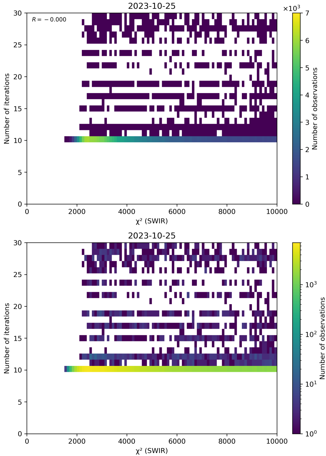
Figure 50: Scatter density plot of “ \chi^2 (SWIR)” against “Number of iterations” for 2023-10-24 to 2023-10-26.
