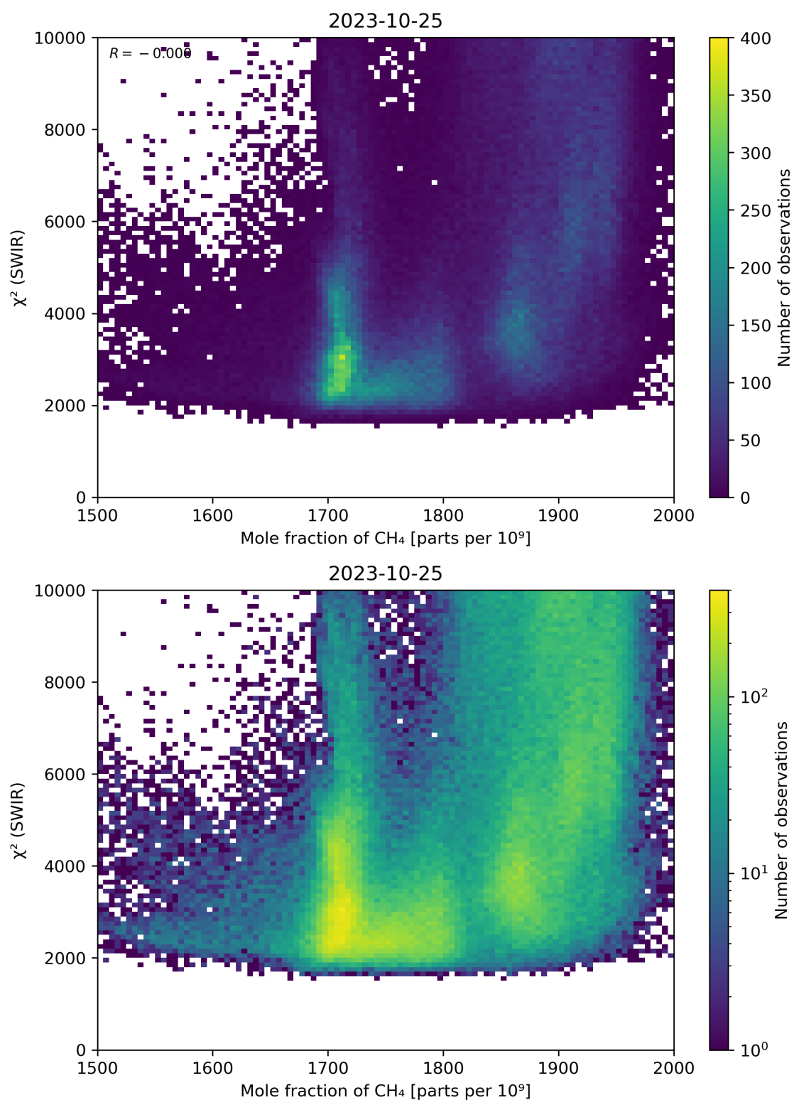
Figure 71: Scatter density plot of “Mole fraction of \text{CH}_4 ” against “ \chi^2 (SWIR)” for 2023-10-24 to 2023-10-26.
