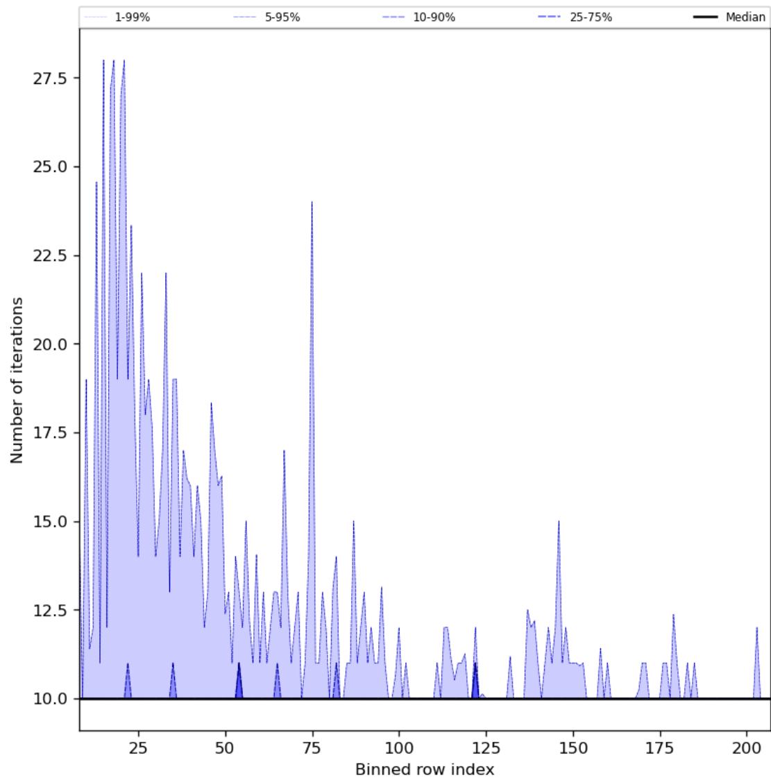
Figure 42: Along track statistics of “Number of iterations” for 2023-10-24 to 2023-10-26
