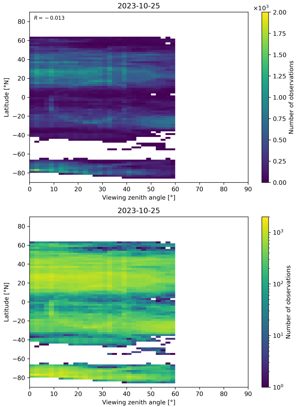
Figure 109: Scatter density plot of “Viewing zenith angle” against “Latitude” for 2023-10-24 to 2023-10-26.
