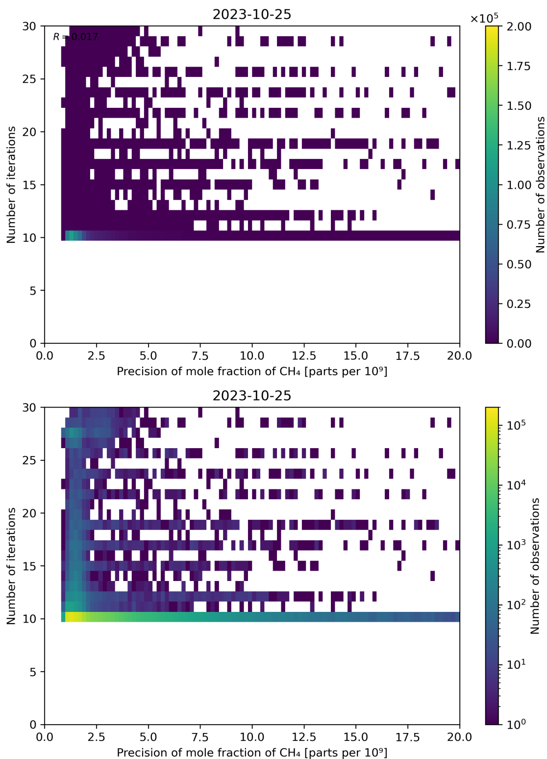
Figure 83: Scatter density plot of “Precision of mole fraction of CH 4 ” against “Number of iterations” for 2023-10-24 to 2023-10-26.
