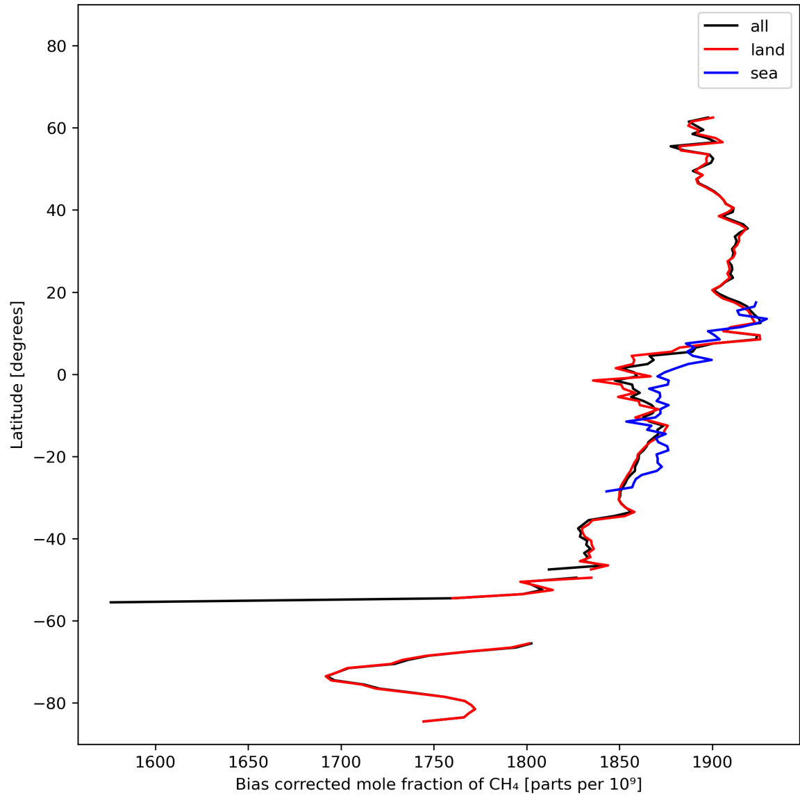
Figure 14: Zonal average of “Bias corrected mole fraction of CH 4 ” for 2023-10-24 to 2023-10-26.
