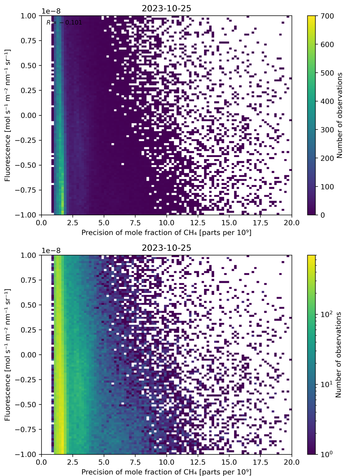
Figure 81: Scatter density plot of “Precision of mole fraction of \text{CH}_4 ” against “Fluorescence” for 2023-10-24 to 2023-10-26.
