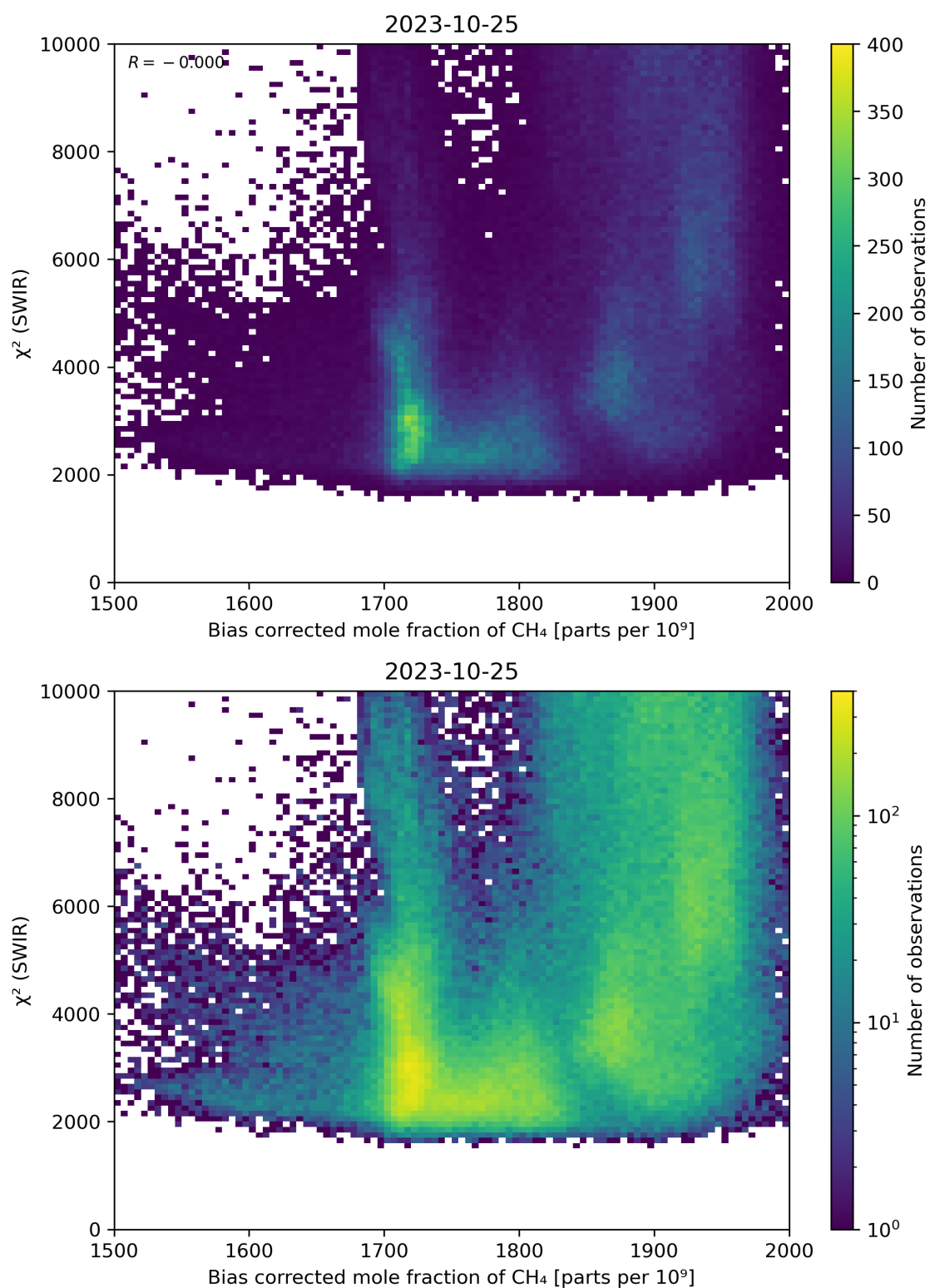
Figure 64: Scatter density plot of “Bias corrected mole fraction of CH 4 ” against “ \chi^2 (SWIR)” for 2023-10-24 to 2023-10-26.
