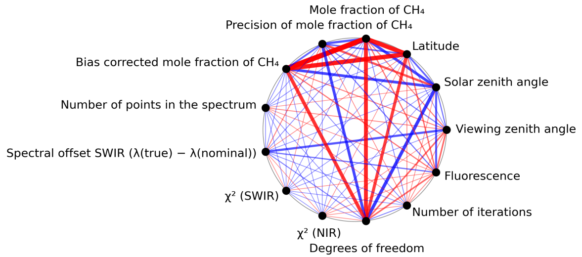
Figure 1: Map of correlation graph for 2023-10-24 to 2023-10-26.
