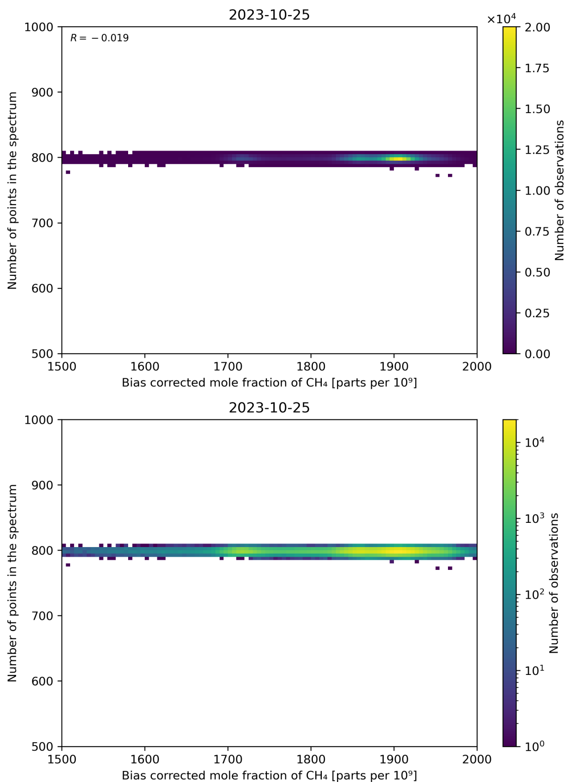
Figure 68: Scatter density plot of “Bias corrected mole fraction of CH 4 ” against “Number of points in the spectrum” for 2023-10-24 to 2023-10-26.
