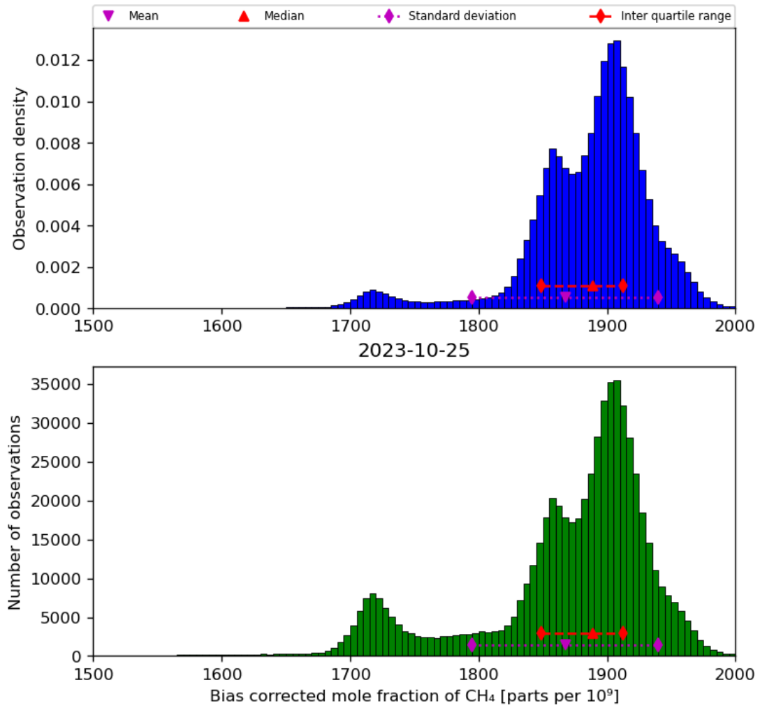
Figure 25: Histogram of “Bias corrected mole fraction of CH 4 ” for 2023-10-24 to 2023-10-26
