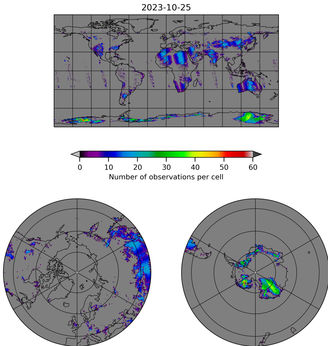
Figure 10: Map of the number of observations for 2023-10-24 to 2023-10-26
