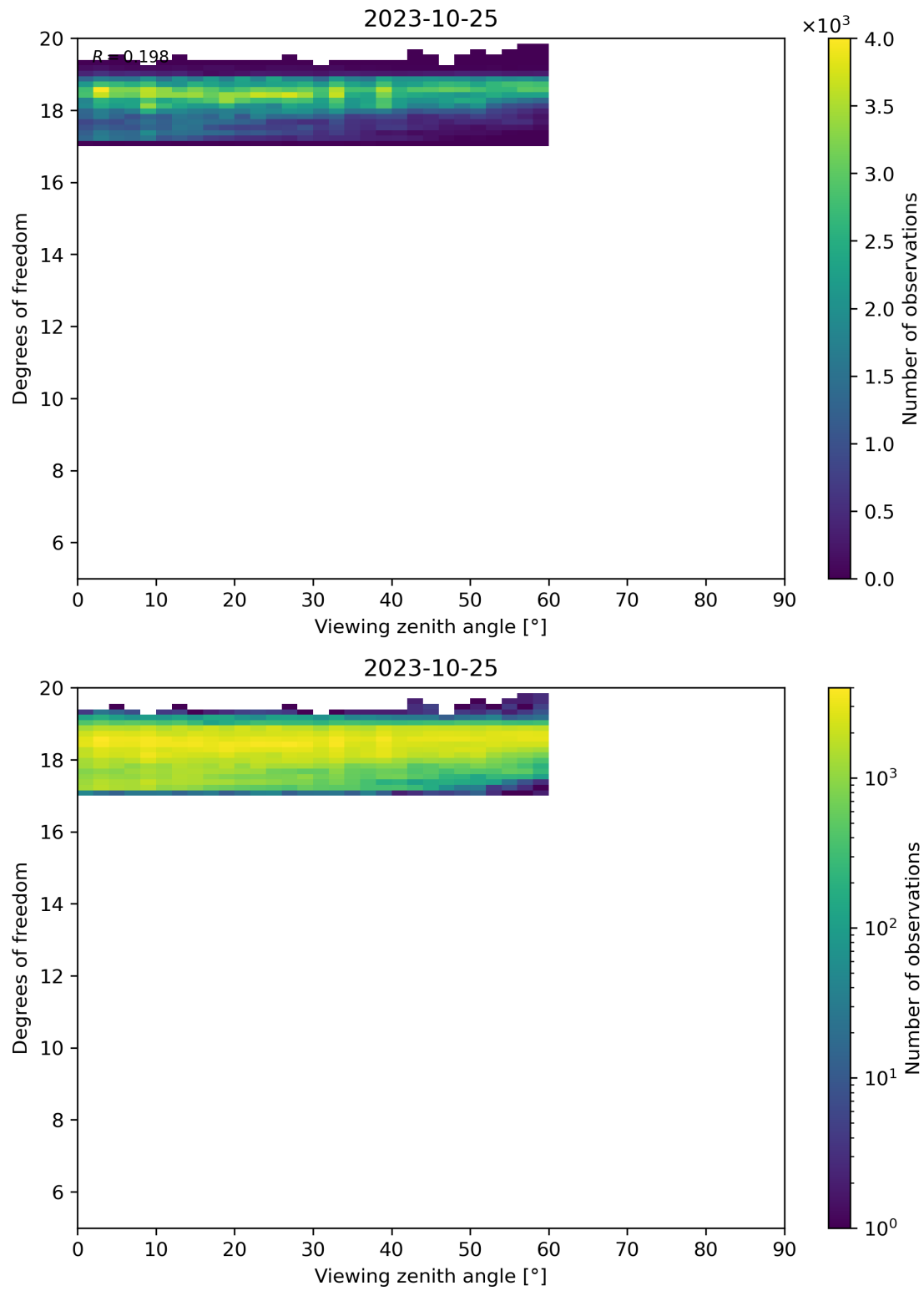
Figure 107: Scatter density plot of “Viewing zenith angle” against “Degrees of freedom” for 2023-10-24 to 2023-10-26.
