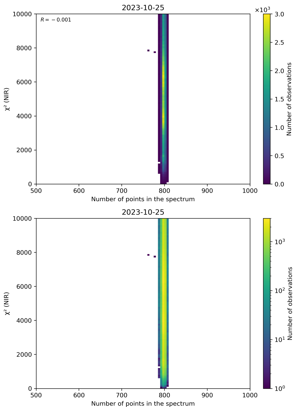
Figure 88: Scatter density plot of “Number of points in the spectrum” against “ \chi^2 (NIR)” for 2023-10-24 to 2023-10-26.
