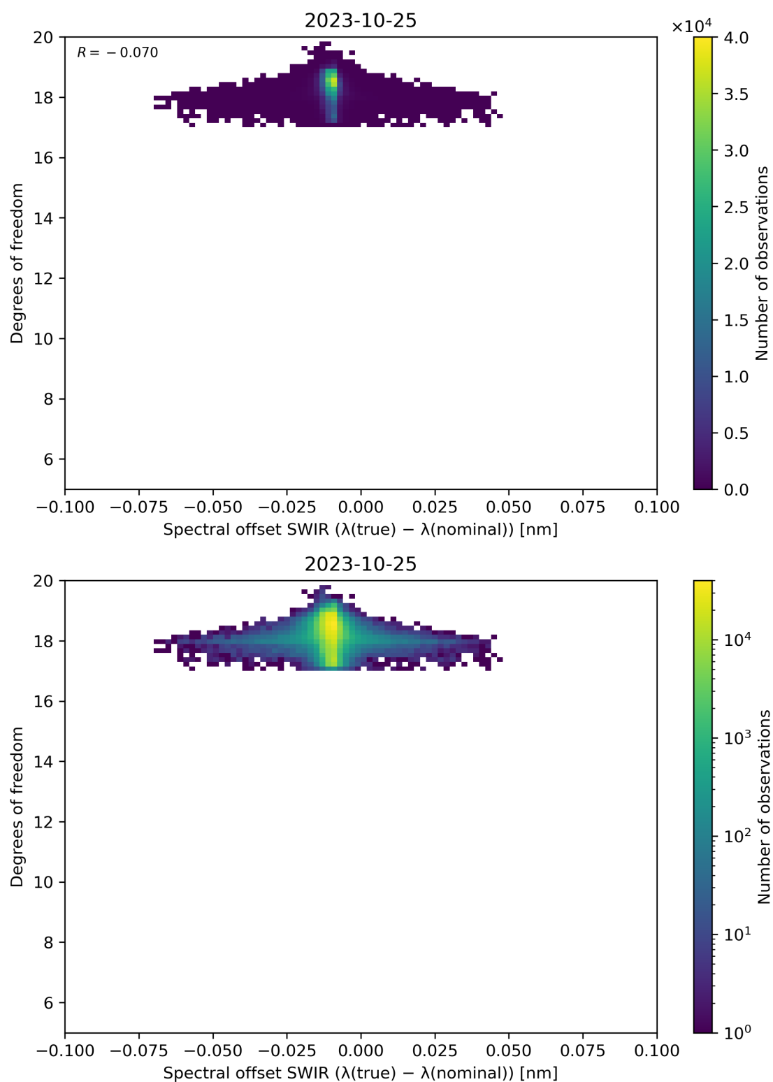
Figure 119: Scatter density plot of “Spectral offset SWIR ( \lambda(\text{true}) - \lambda(\text{nominal}) )” against “Degrees of freedom” for 2023-10-24 to 2023-10-26.
