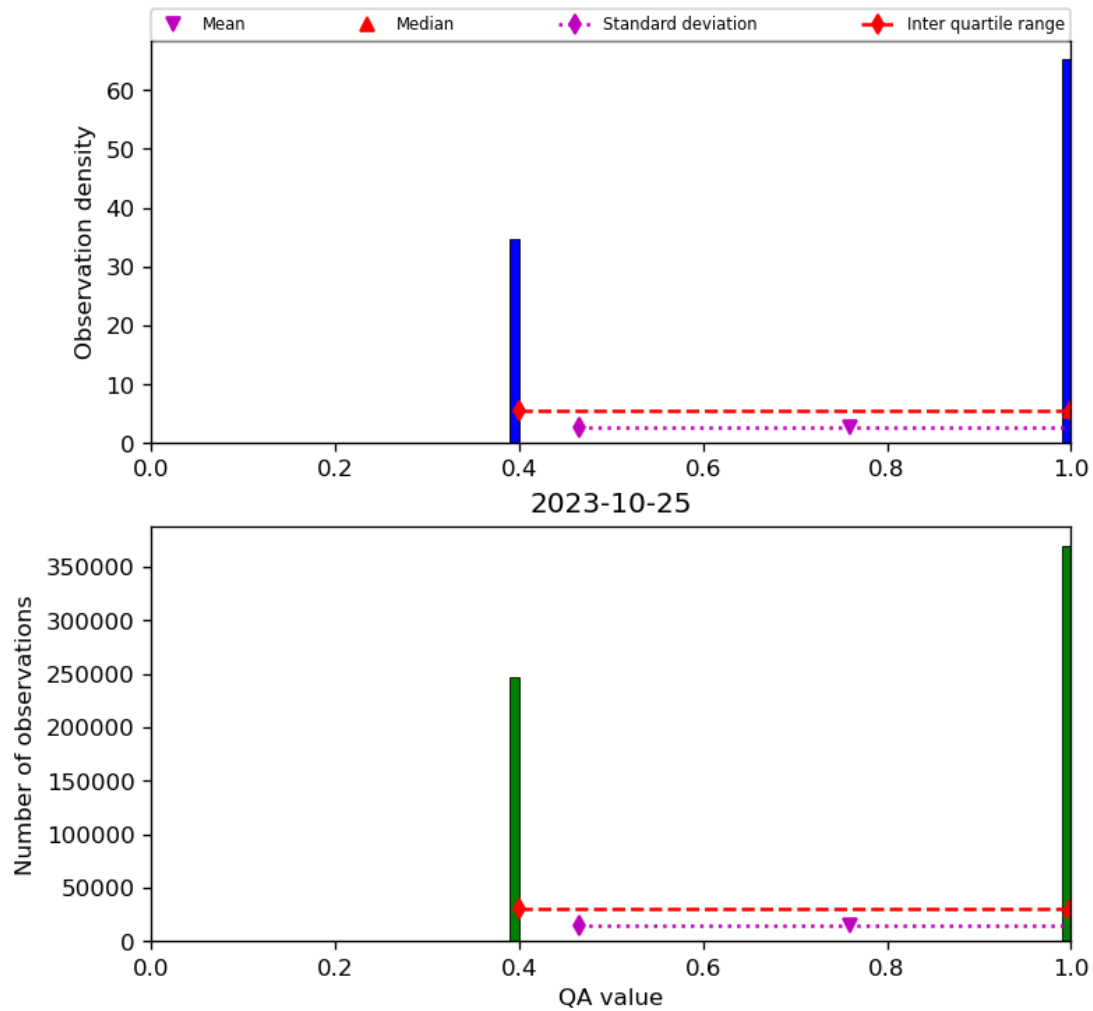
Figure 22: Histogram of “QA value” for 2023-10-24 to 2023-10-26
