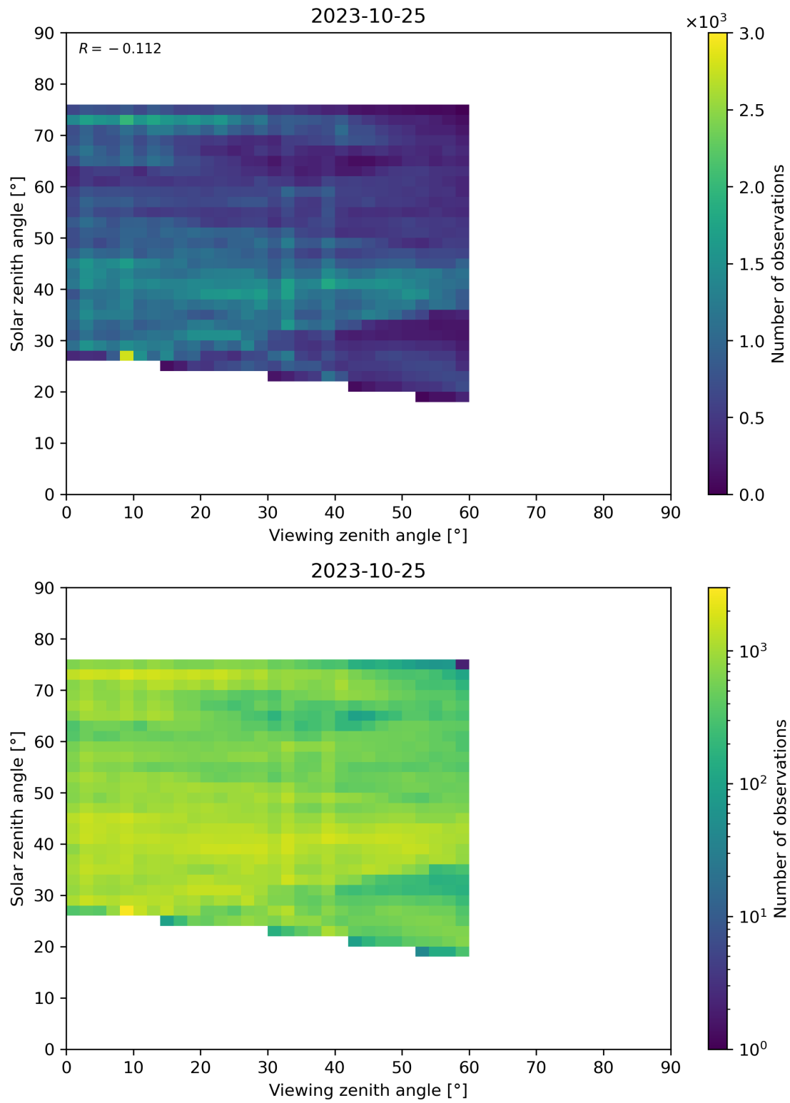
Figure 115: Scatter density plot of “Viewing zenith angle” against “Solar zenith angle” for 2023-10-24 to 2023-10-26.
