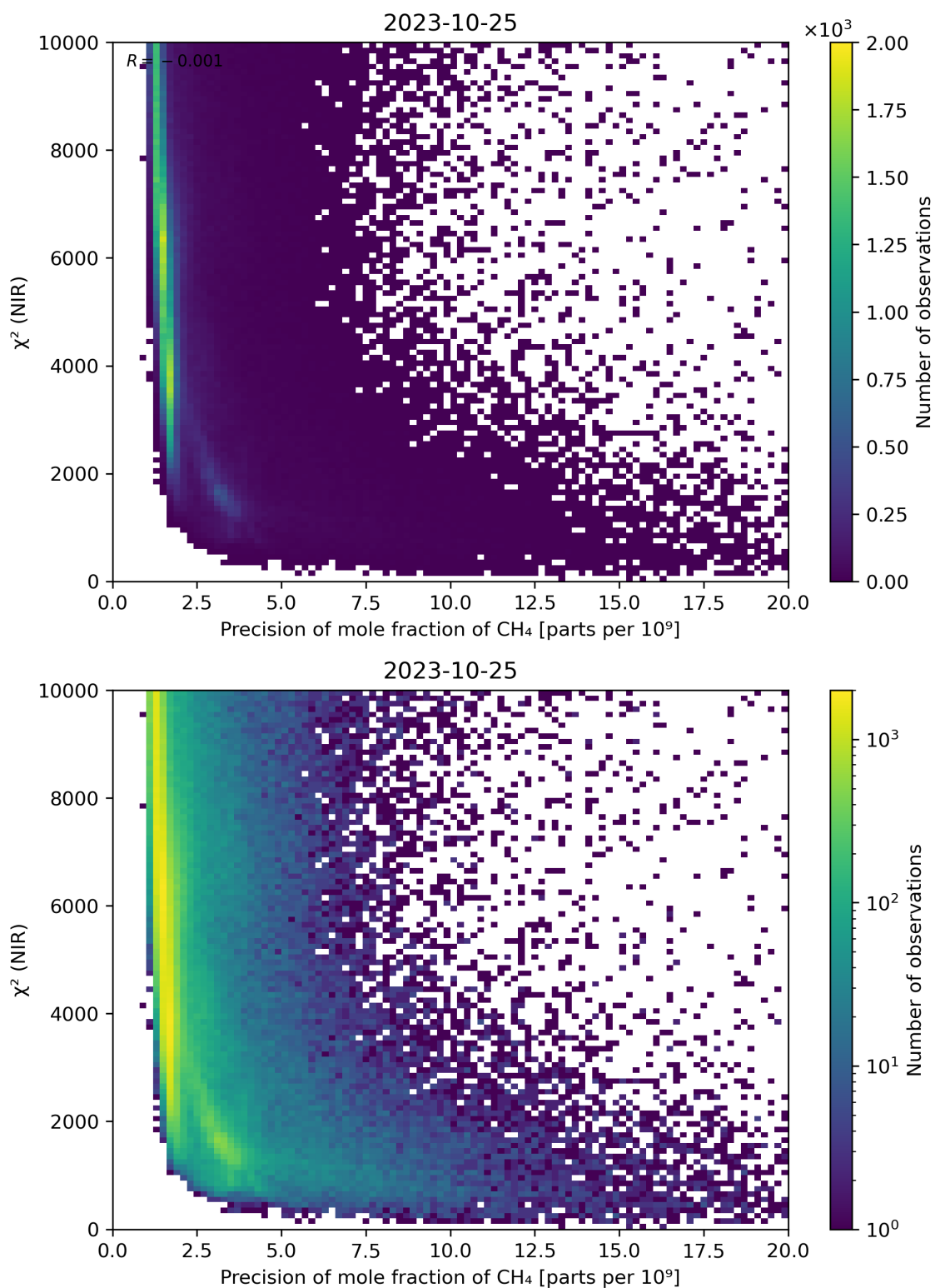
Figure 78: Scatter density plot of “Precision of mole fraction of CH 4 ” against “ \chi^2 (NIR)” for 2023-10-24 to 2023-10-26.
