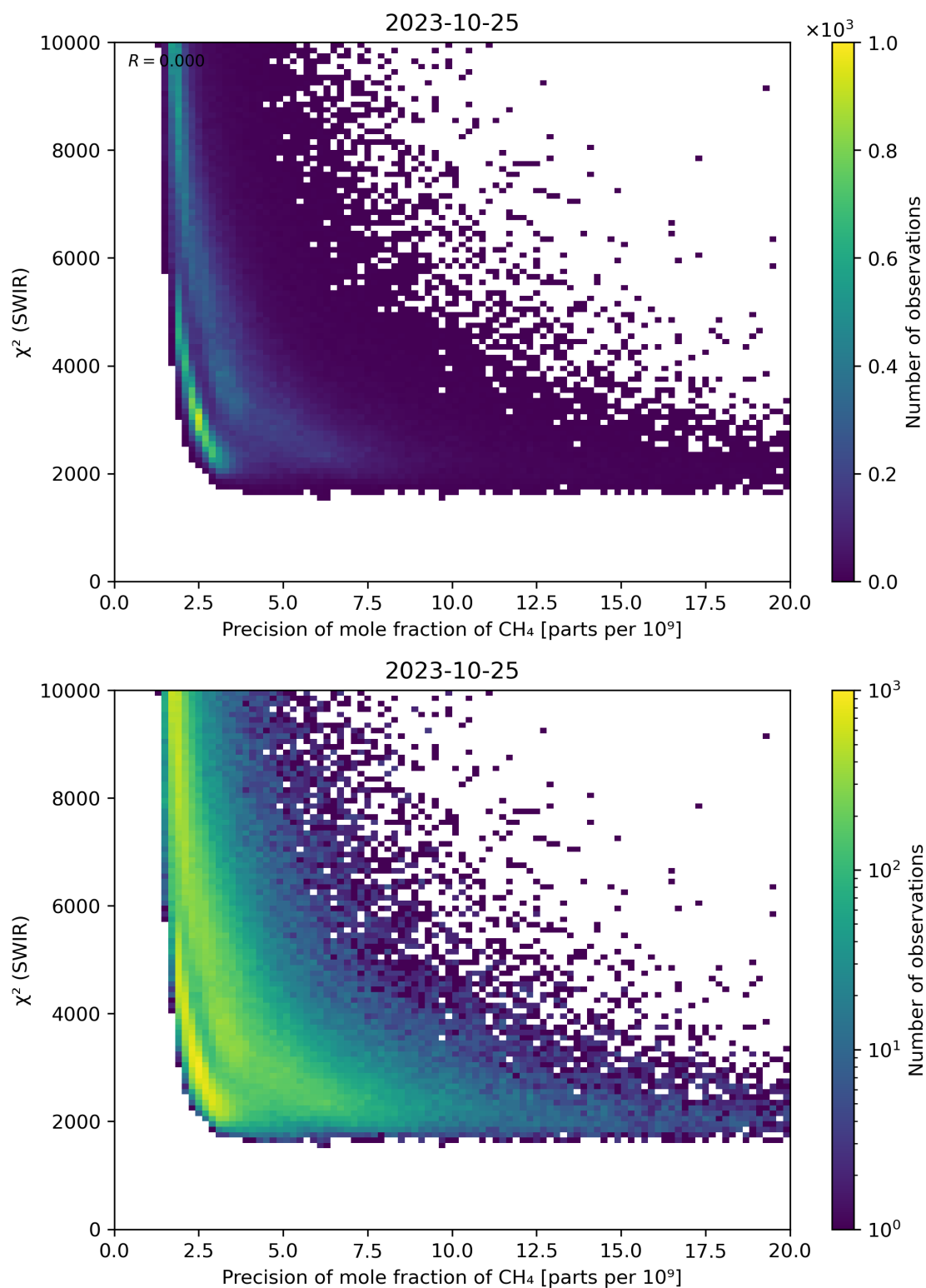
Figure 79: Scatter density plot of “Precision of mole fraction of \text{CH}_4 ” against “ \chi^2 (SWIR)” for 2023-10-24 to 2023-10-26.
