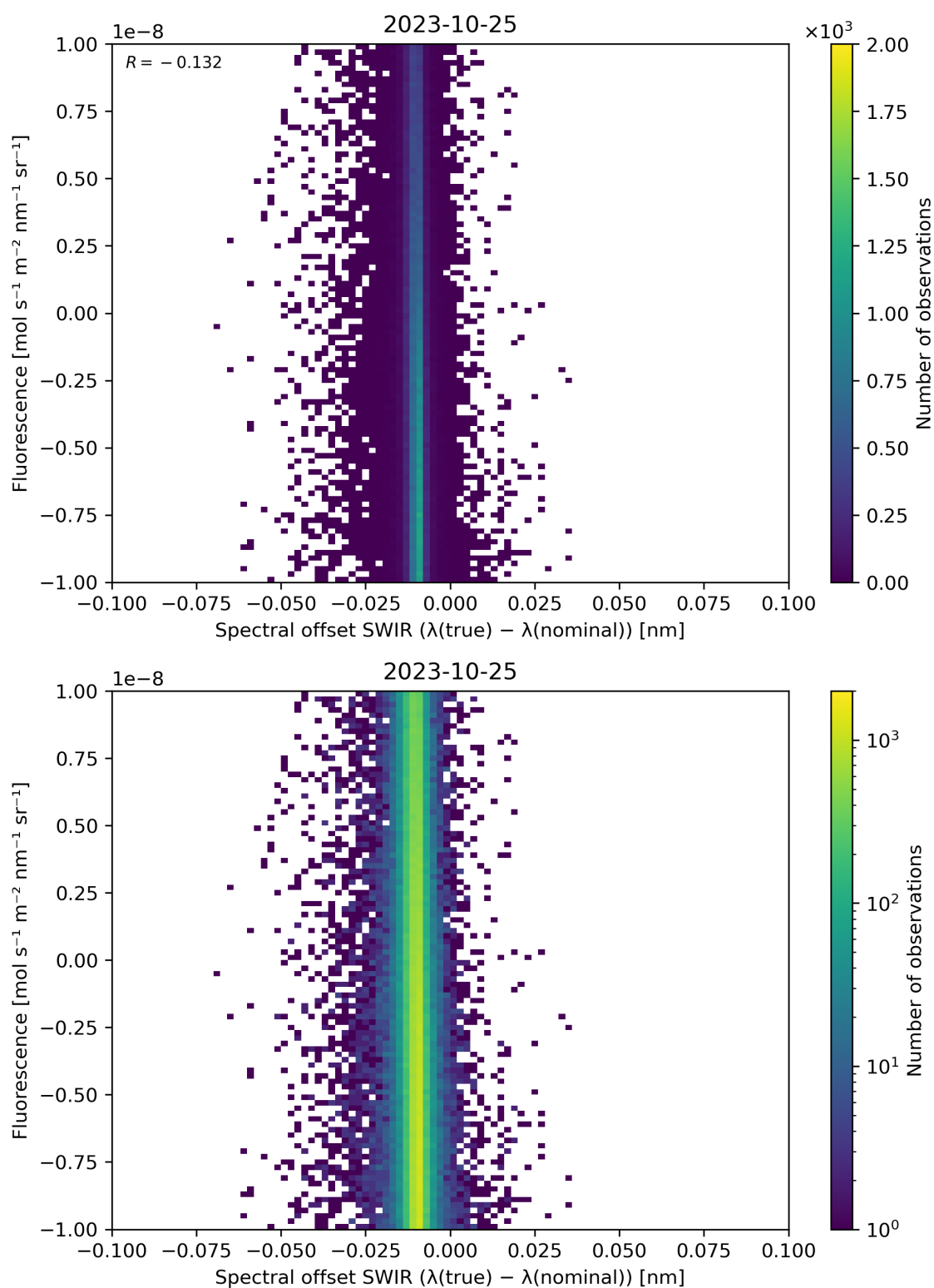
Figure 120: Scatter density plot of “Spectral offset SWIR ( \lambda(\text{true}) - \lambda(\text{nominal}) )” against “Fluorescence” for 2023-10-24 to 2023-10-26.
