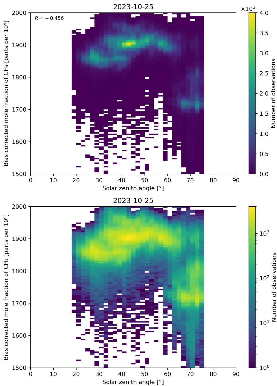
Figure 100: Scatter density plot of “Solar zenith angle” against “Bias corrected mole fraction of \text{CH}_4 ” for 2023-10-24 to 2023-10-26.
