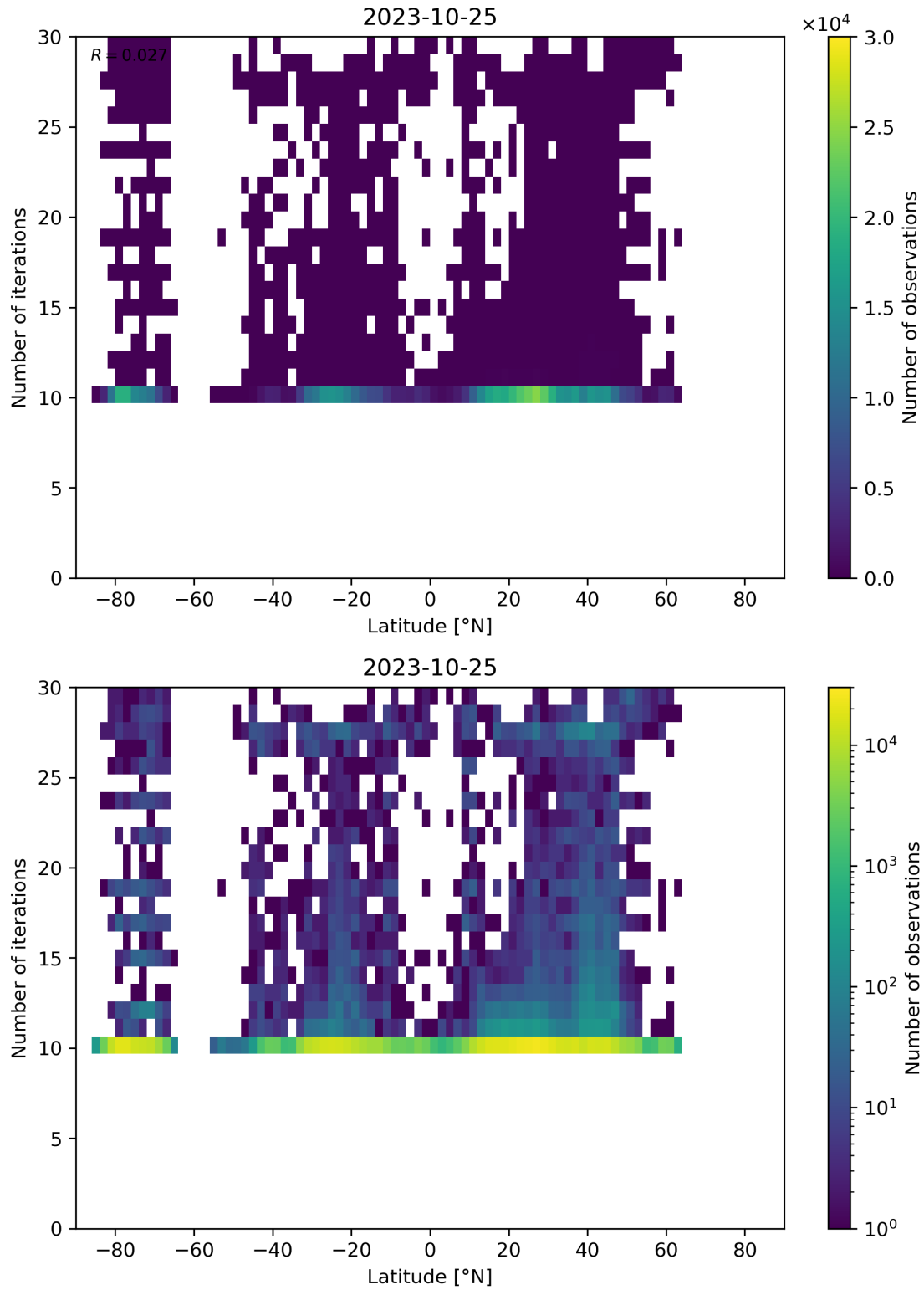
Figure 60: Scatter density plot of “Latitude” against “Number of iterations” for 2023-10-24 to 2023-10-26.
