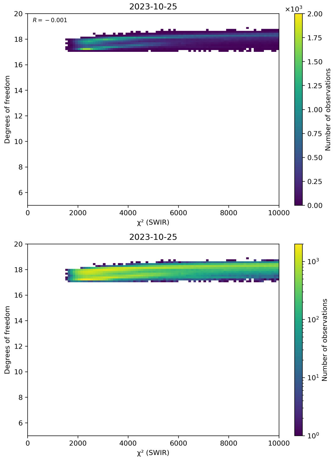
Figure 48: Scatter density plot of “ \chi^2 (SWIR)” against “Degrees of freedom” for 2023-10-24 to 2023-10-26.
