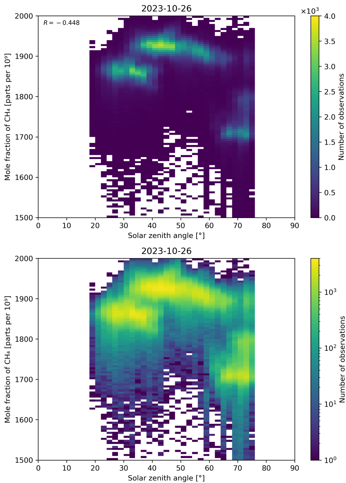
Figure 99: Scatter density plot of “Solar zenith angle” against “Mole fraction of CH 4 ” for 2023-10-25 to 2023-10-27.
