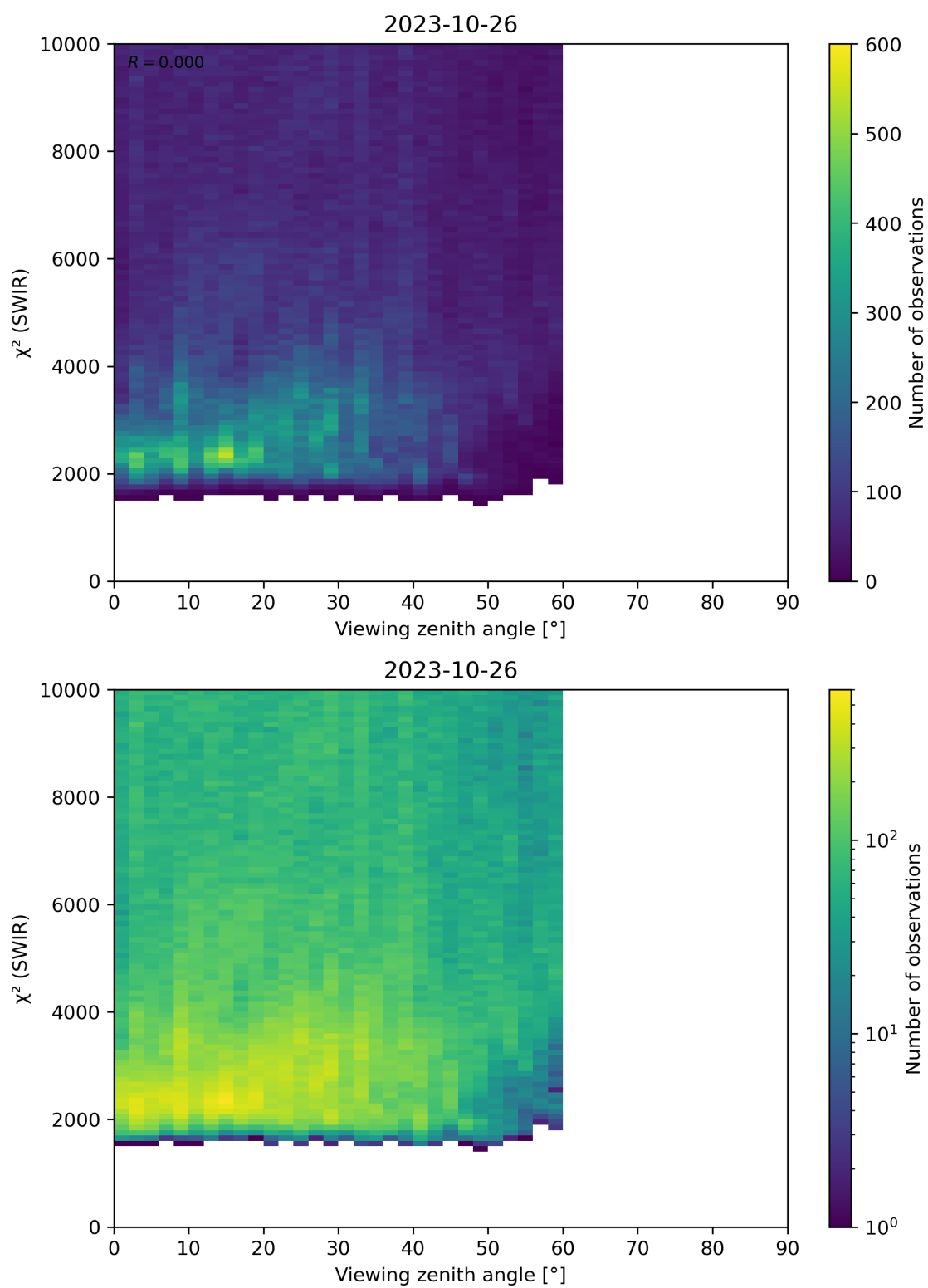
Figure 106: Scatter density plot of “Viewing zenith angle” against “ \chi^2 (SWIR)” for 2023-10-25 to 2023-10-27.
