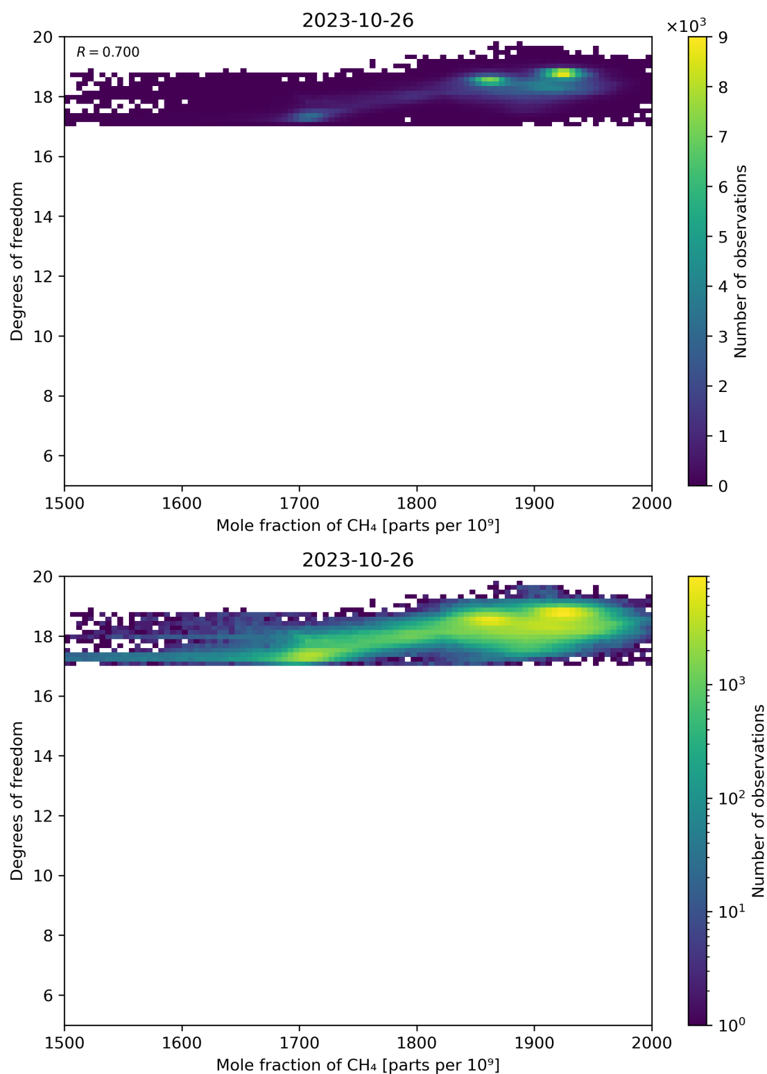
Figure 72: Scatter density plot of “Mole fraction of CH 4 ” against “Degrees of freedom” for 2023-10-25 to 2023-10-27.
