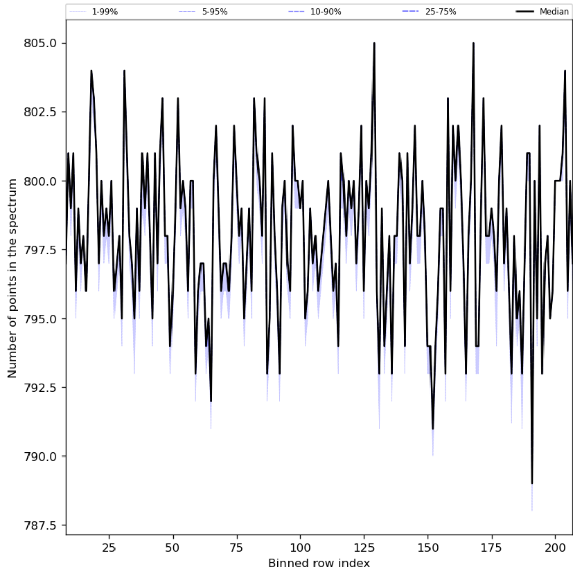
Figure 37: Along track statistics of “Number of points in the spectrum” for 2023-10-25 to 2023-10-27
