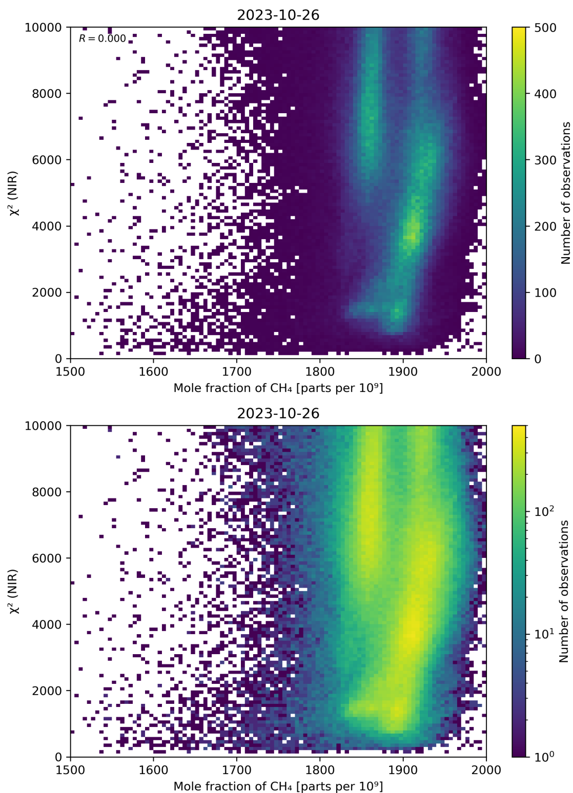
Figure 70: Scatter density plot of “Mole fraction of \text{CH}_4 ” against “ \chi^2 (NIR)” for 2023-10-25 to 2023-10-27.
