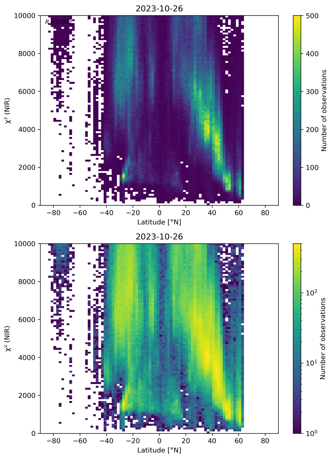
Figure 53: Scatter density plot of “Latitude” against “ \chi^2 (NIR)” for 2023-10-25 to 2023-10-27.
