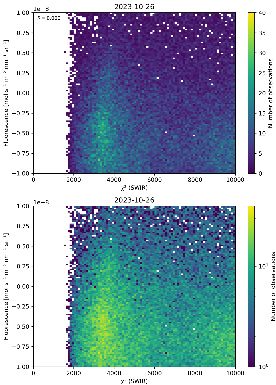
Figure 49: Scatter density plot of “ \chi^2 (SWIR)” against “Fluorescence” for 2023-10-25 to 2023-10-27.
