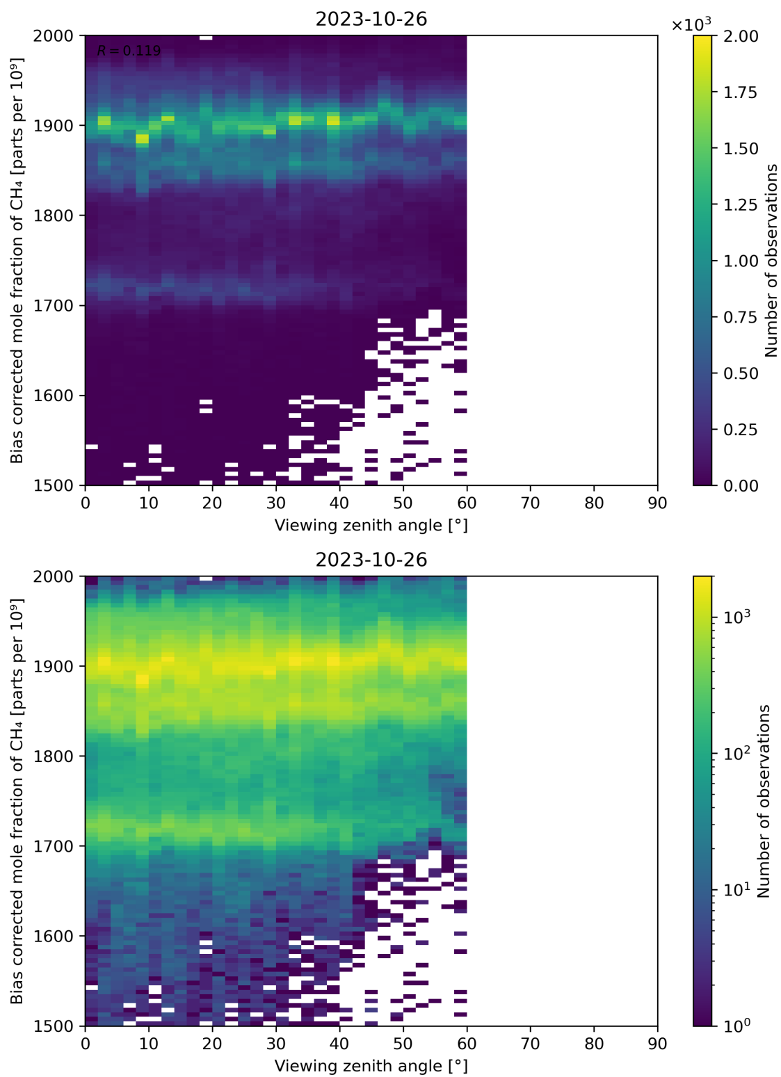
Figure 111: Scatter density plot of “Viewing zenith angle” against “Bias corrected mole fraction of CH 4 ” for 2023-10-25 to 2023-10-27.
