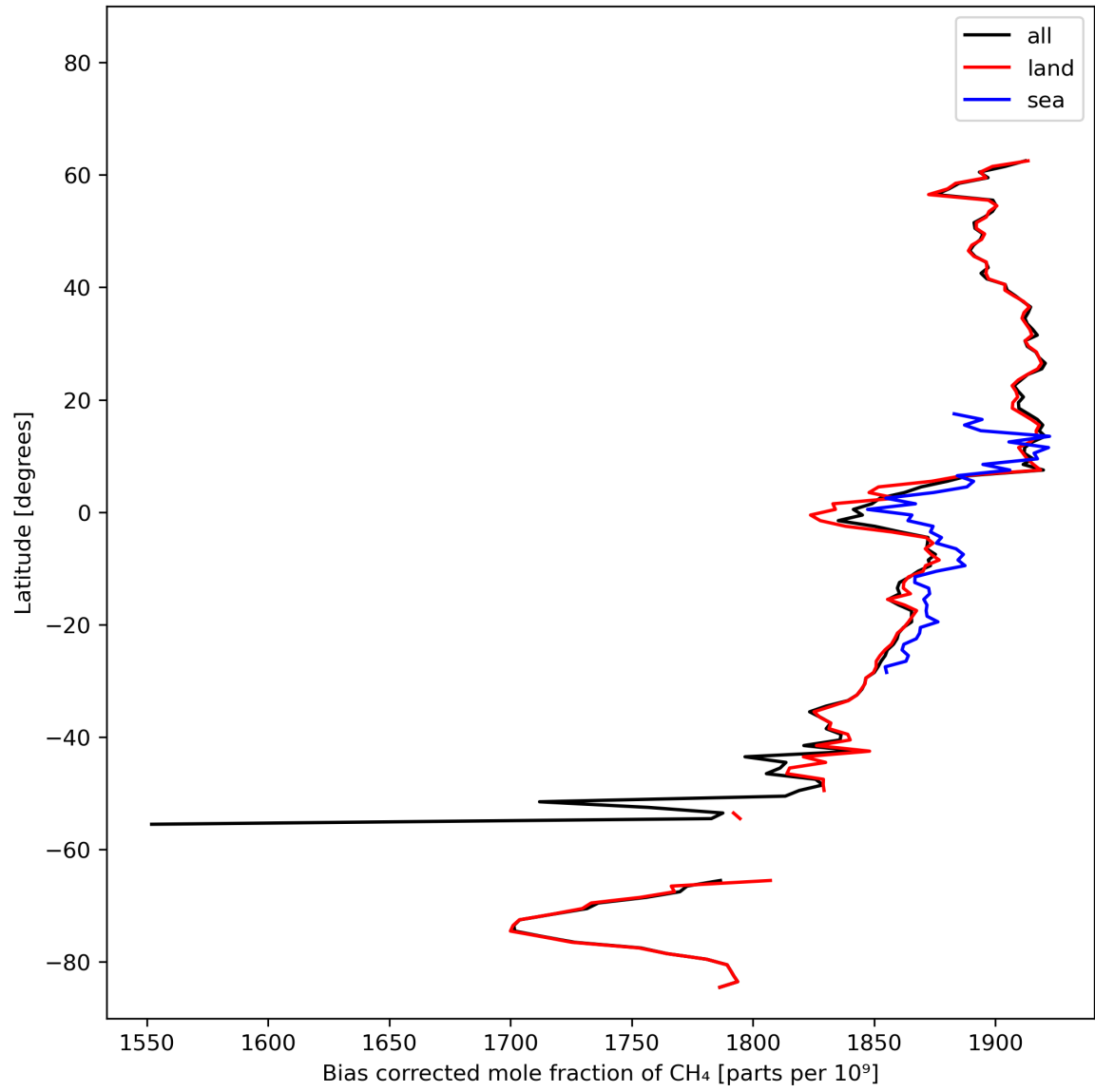
Figure 14: Zonal average of “Bias corrected mole fraction of CH 4 ” for 2023-10-25 to 2023-10-27.
