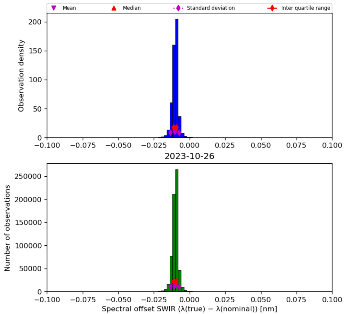
Figure 27: Histogram of “Spectral offset SWIR ( \lambda(\text{true}) - \lambda(\text{nominal}) )” for 2023-10-25 to 2023-10-27
