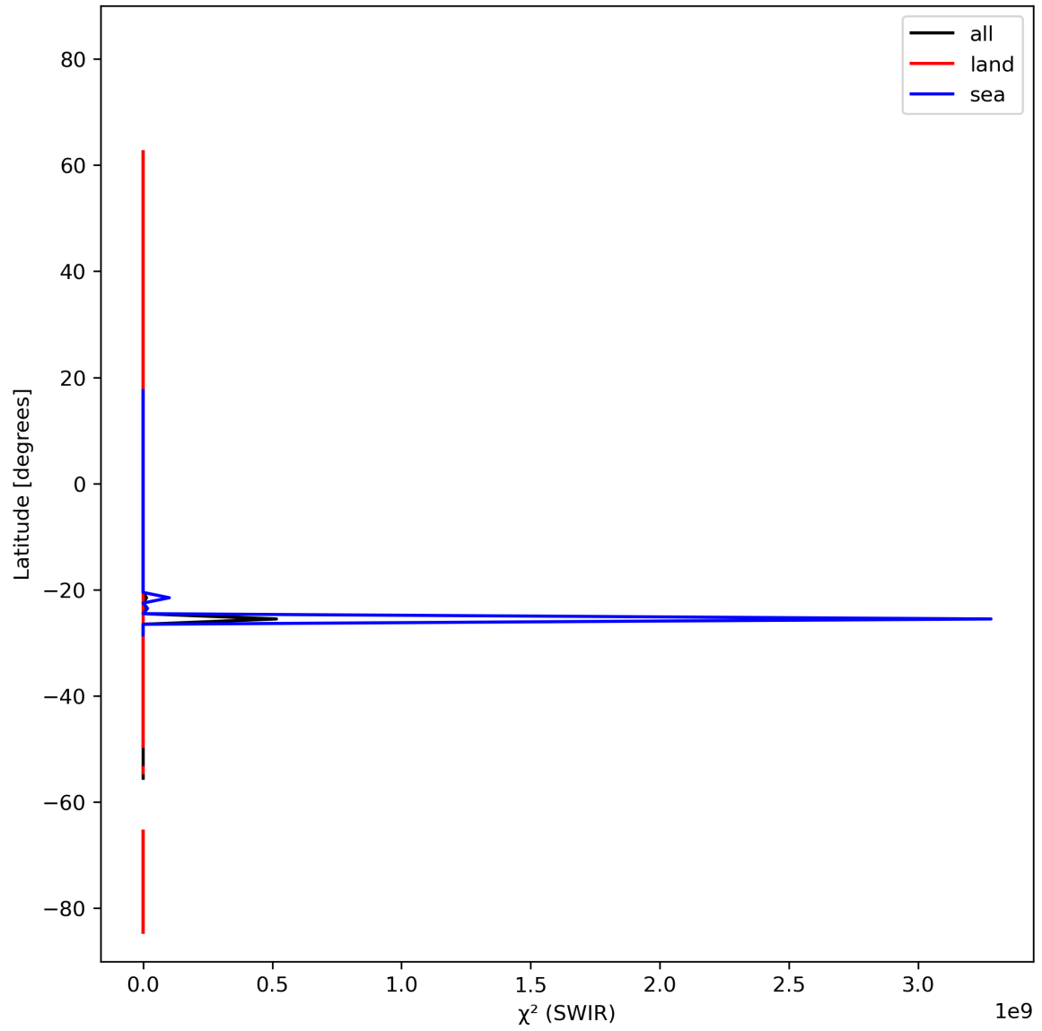
Figure 17: Zonal average of “ \chi^2 (SWIR)” for 2023-10-25 to 2023-10-27.
