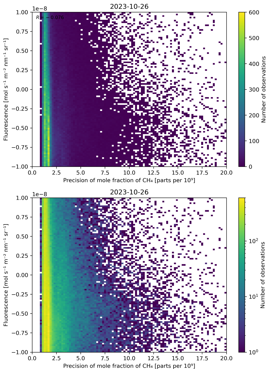
Figure 81: Scatter density plot of “Precision of mole fraction of CH 4 ” against “Fluorescence” for 2023-10-25 to 2023-10-27.
