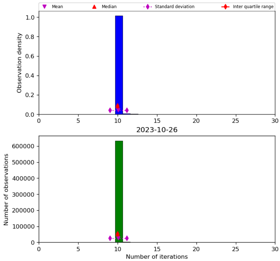
Figure 31: Histogram of “Number of iterations” for 2023-10-25 to 2023-10-27
