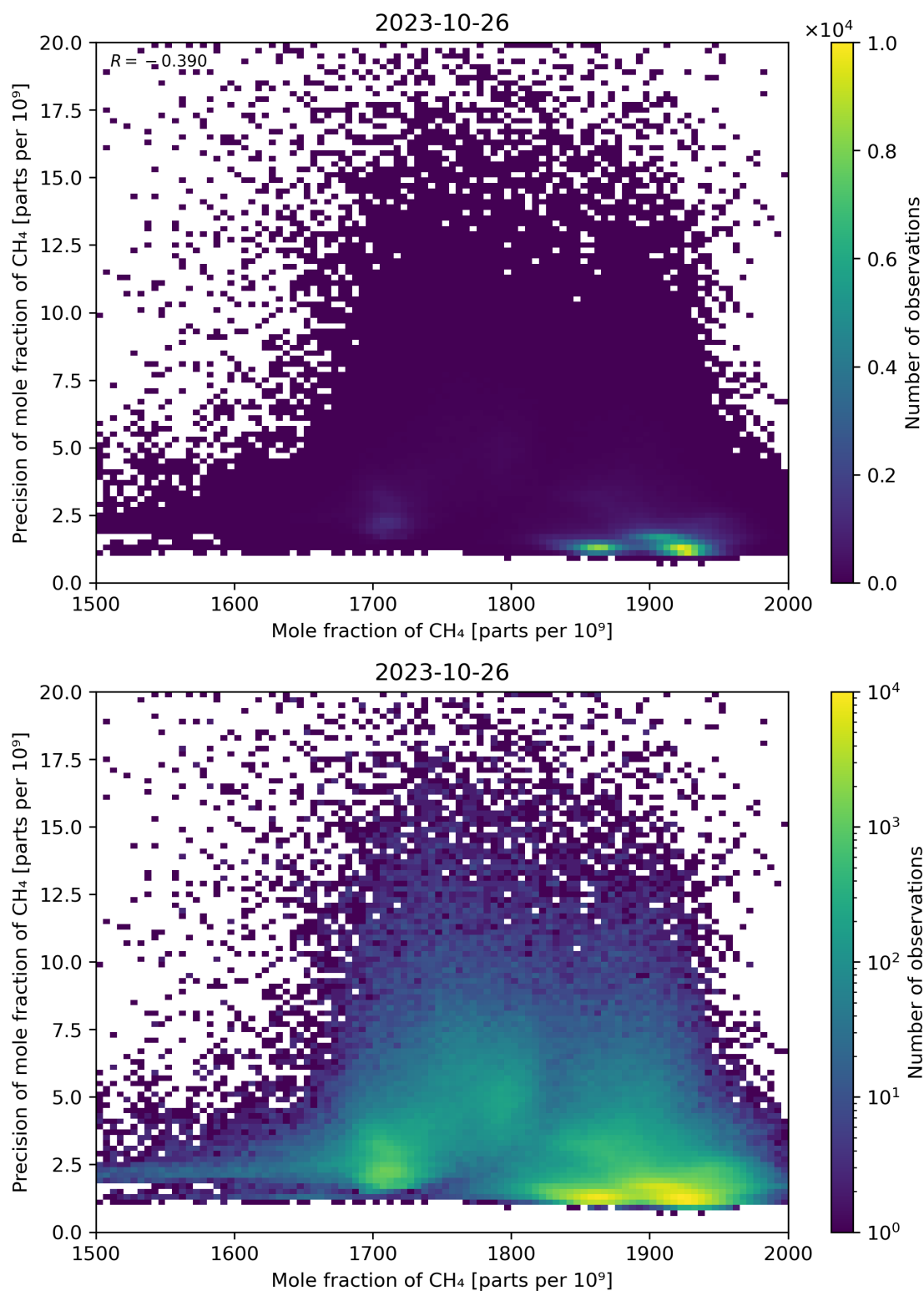
Figure 75: Scatter density plot of “Mole fraction of CH 4 ” against “Precision of mole fraction of CH 4 ” for 2023-10-25 to 2023-10-27.
