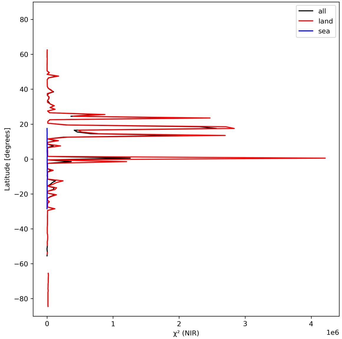
Figure 18: Zonal average of “ \chi^2 (NIR)” for 2023-10-25 to 2023-10-27.
