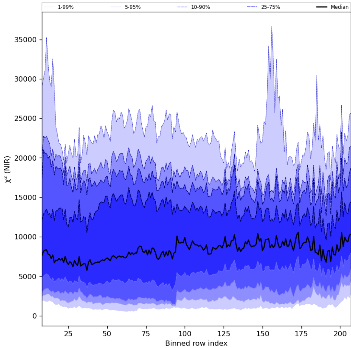
Figure 40: Along track statistics of “ \chi^2 (NIR)” for 2023-10-25 to 2023-10-27
