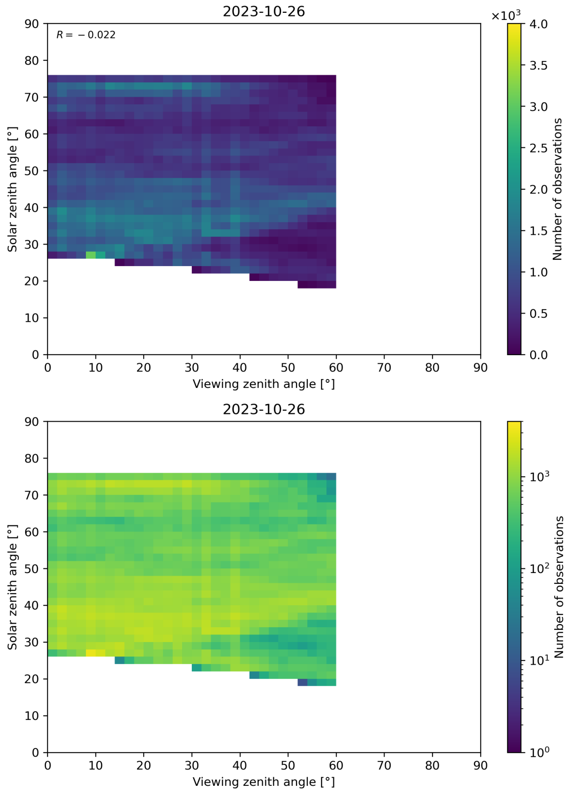
Figure 115: Scatter density plot of “Viewing zenith angle” against “Solar zenith angle” for 2023-10-25 to 2023-10-27.
