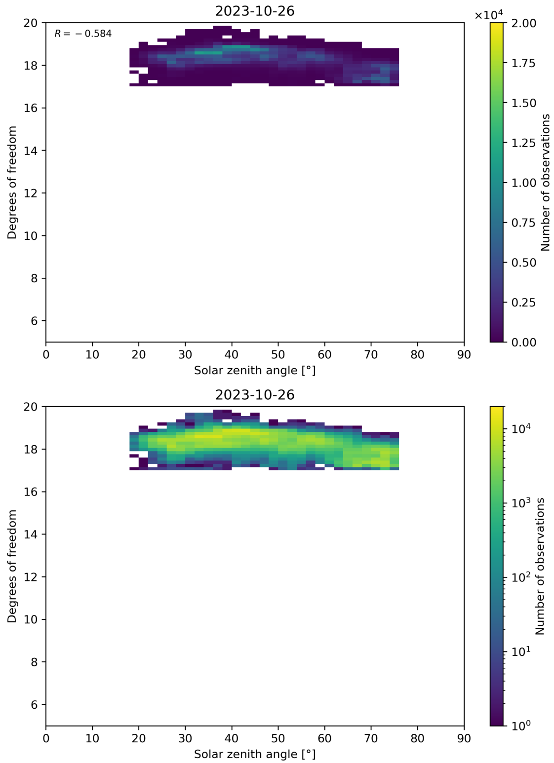
Figure 96: Scatter density plot of “Solar zenith angle” against “Degrees of freedom” for 2023-10-25 to 2023-10-27.
