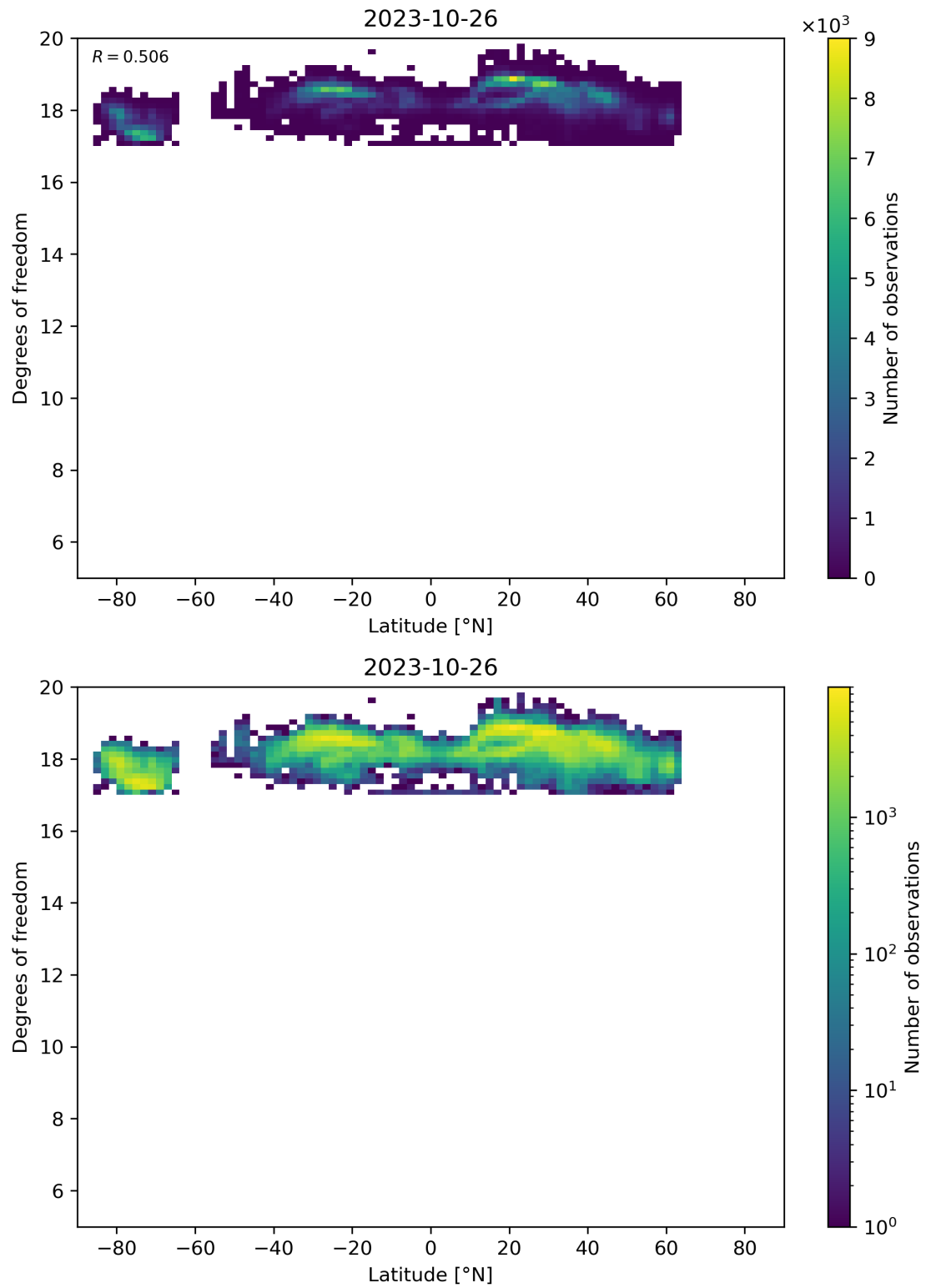
Figure 55: Scatter density plot of “Latitude” against “Degrees of freedom” for 2023-10-25 to 2023-10-27.
