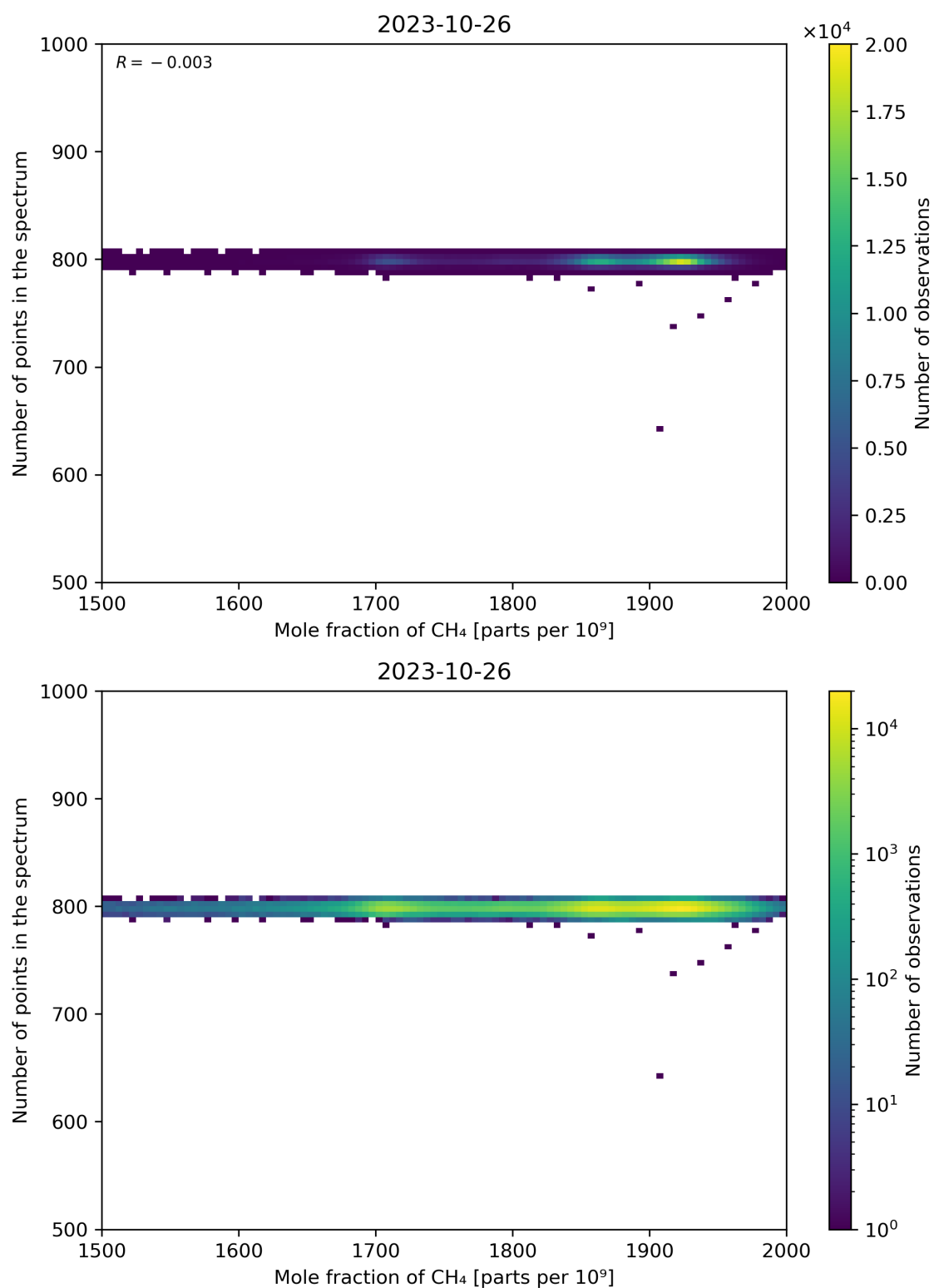
Figure 77: Scatter density plot of “Mole fraction of CH 4 ” against “Number of points in the spectrum” for 2023-10-25 to 2023-10-27.
