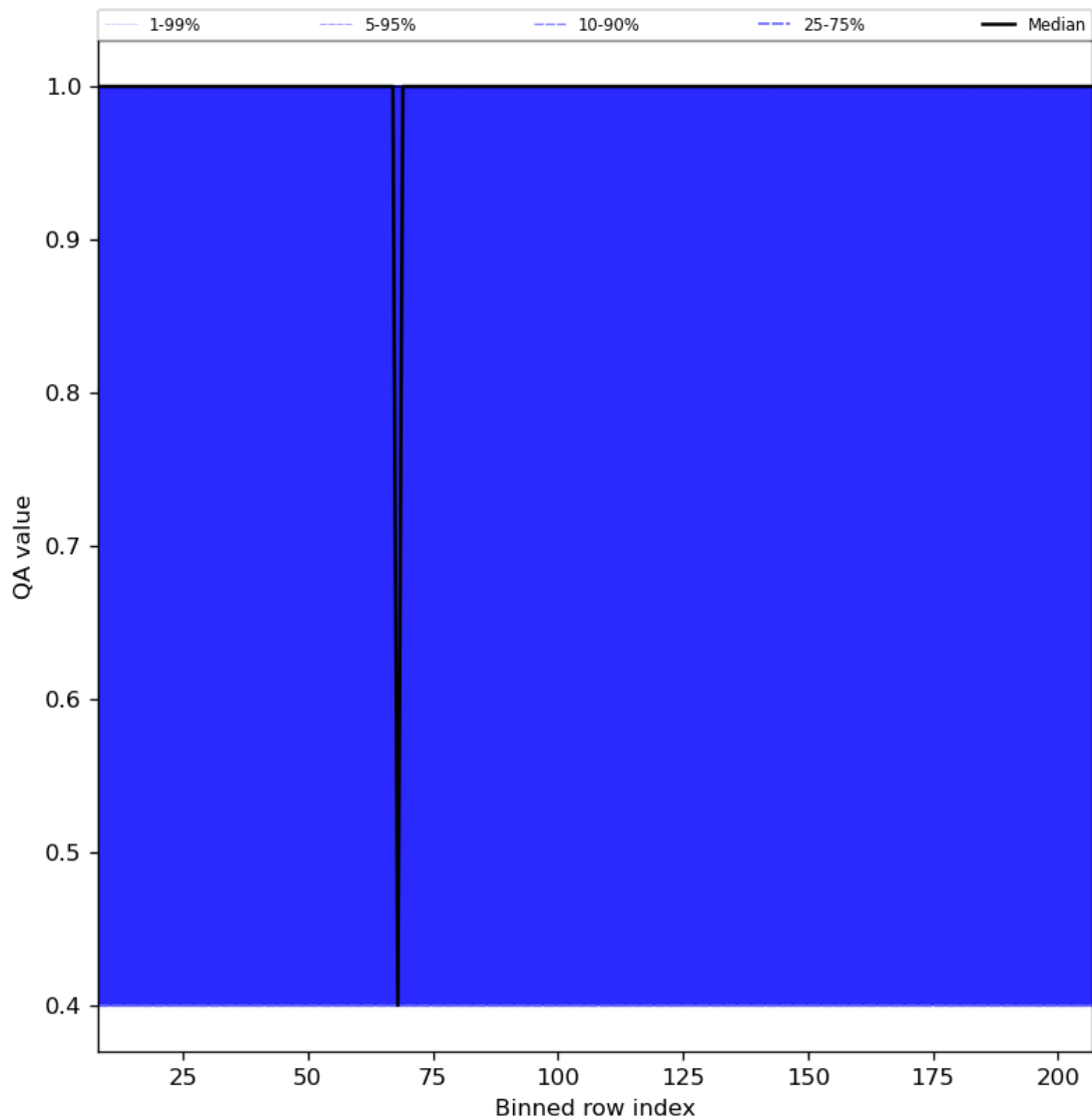
Figure 33: Along track statistics of “QA value” for 2023-10-25 to 2023-10-27
