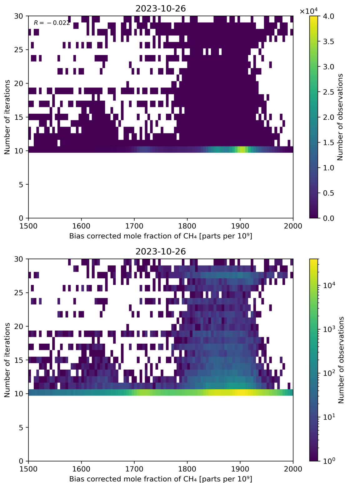
Figure 67: Scatter density plot of “Bias corrected mole fraction of CH 4 ” against “Number of iterations” for 2023-10-25 to 2023-10-27.
