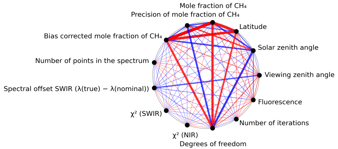
Figure 1: Map of correlation graph for 2023-10-25 to 2023-10-27.
