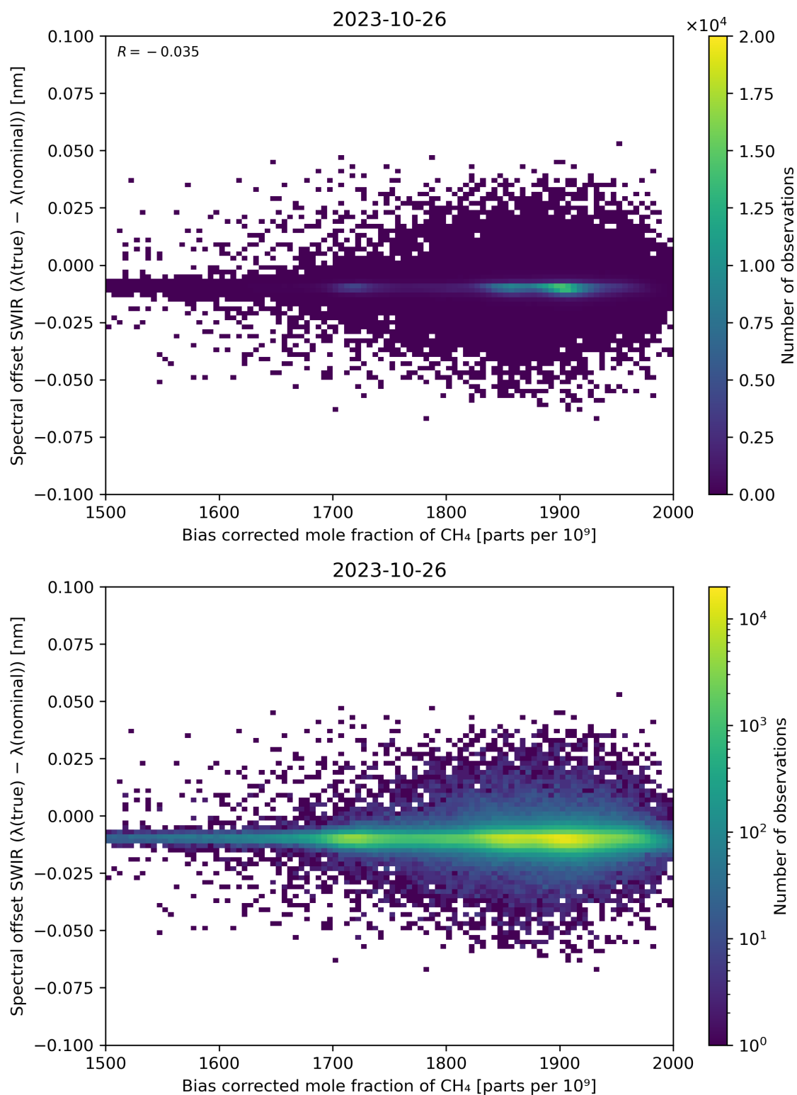
Figure 69: Scatter density plot of “Bias corrected mole fraction of \text{CH}_4 ” against “Spectral offset SWIR ( \lambda(\text{true}) - \lambda(\text{nominal}) )” for 2023-10-25 to 2023-10-27.
