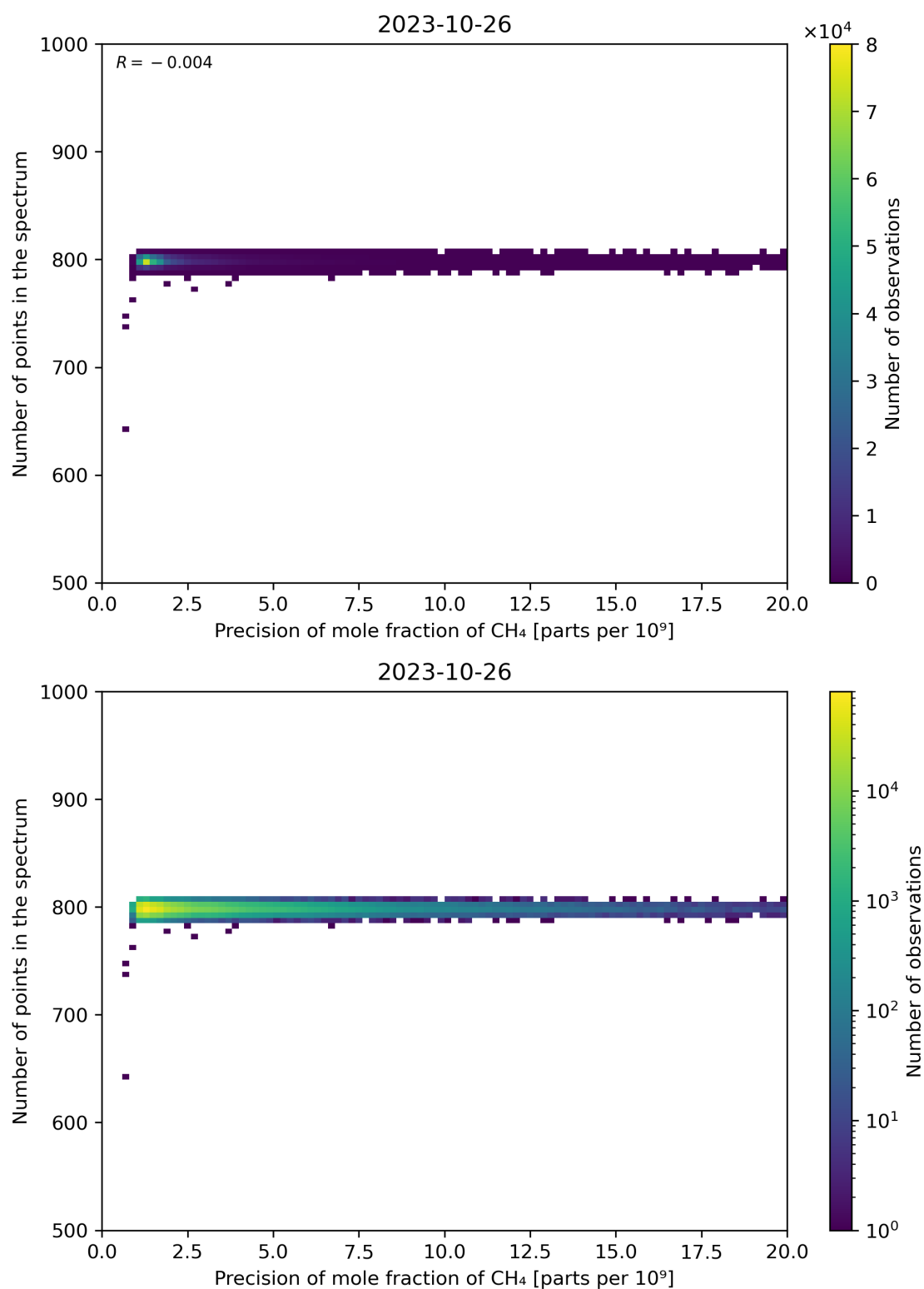
Figure 84: Scatter density plot of “Precision of mole fraction of CH 4 ” against “Number of points in the spectrum” for 2023-10-25 to 2023-10-27.
