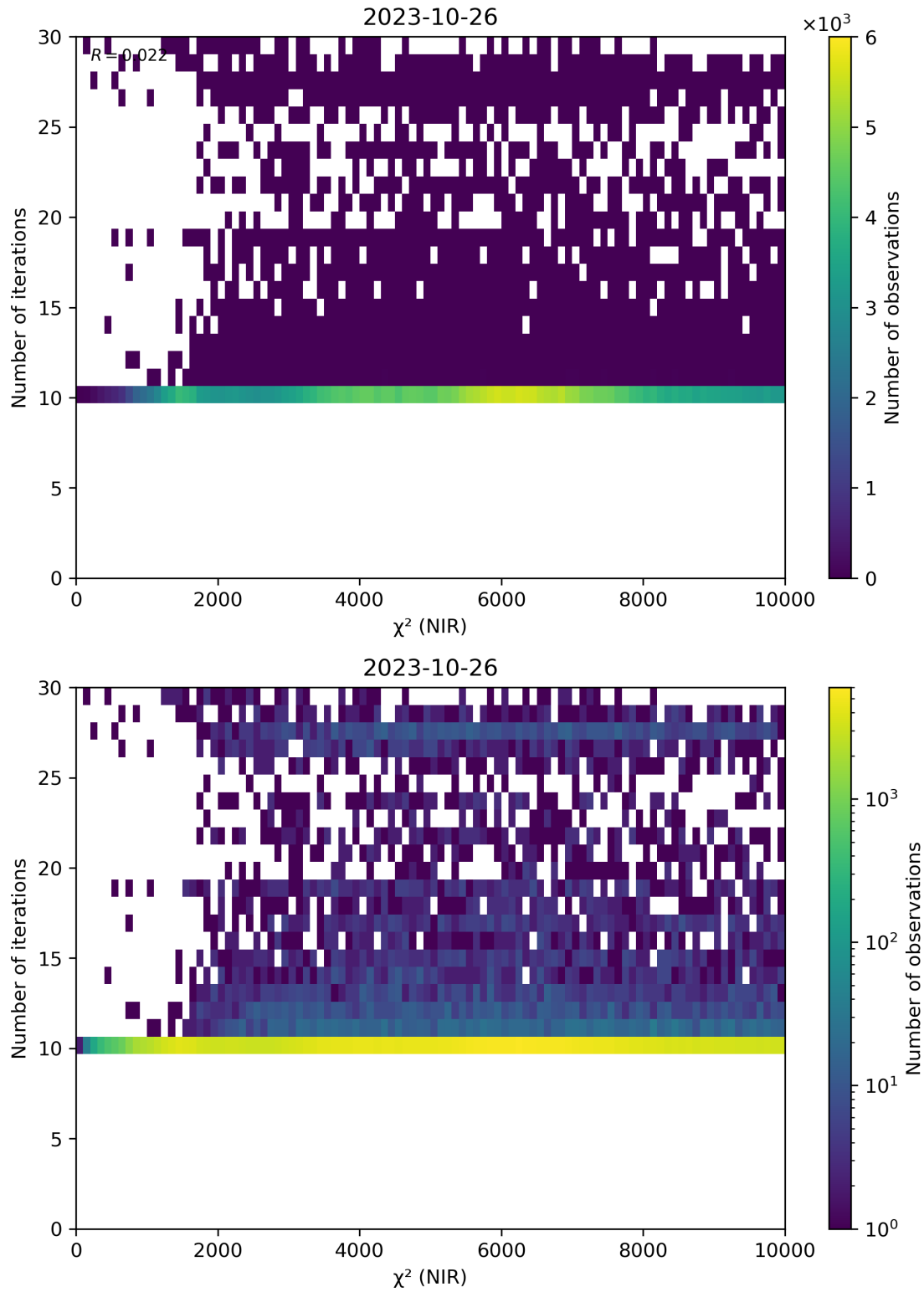
Figure 46: Scatter density plot of “ \chi^2 (NIR)” against “Number of iterations” for 2023-10-25 to 2023-10-27.
