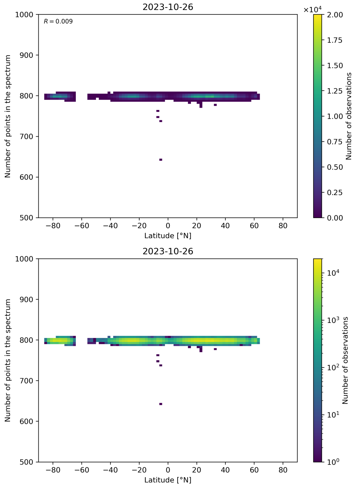
Figure 61: Scatter density plot of “Latitude” against “Number of points in the spectrum” for 2023-10-25 to 2023-10-27.
