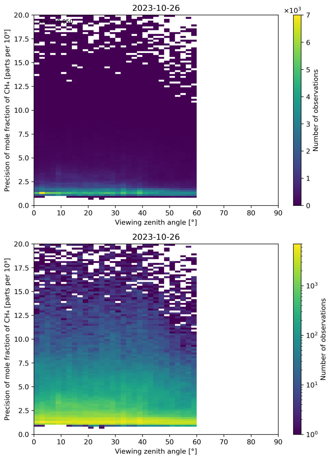
Figure 112: Scatter density plot of “Viewing zenith angle” against “Precision of mole fraction of CH 4 ” for 2023-10-25 to 2023-10-27.
