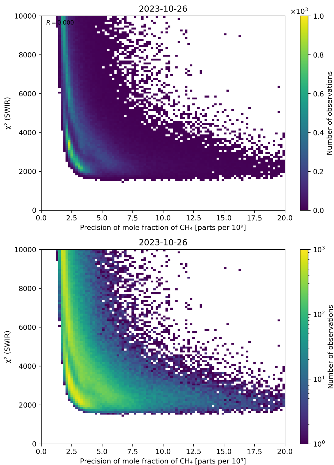
Figure 79: Scatter density plot of “Precision of mole fraction of CH 4 ” against “ \chi^2 (SWIR)” for 2023-10-25 to 2023-10-27.
