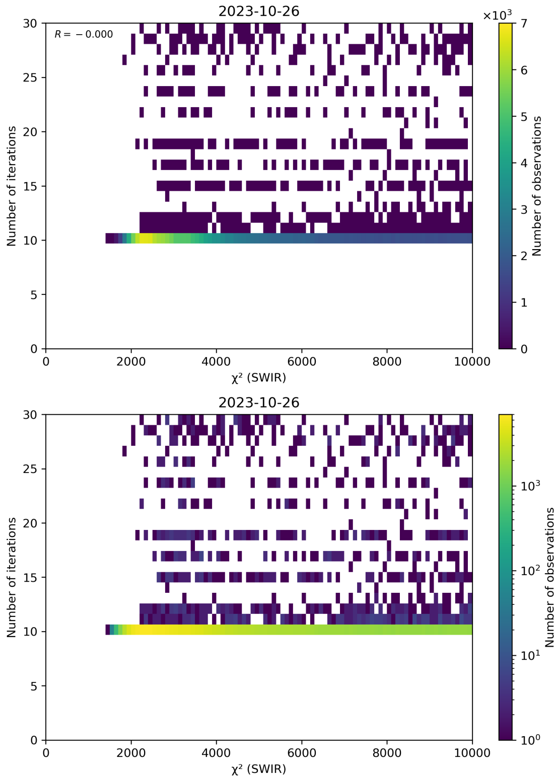
Figure 50: Scatter density plot of “ \chi^2 (SWIR)” against “Number of iterations” for 2023-10-25 to 2023-10-27.
