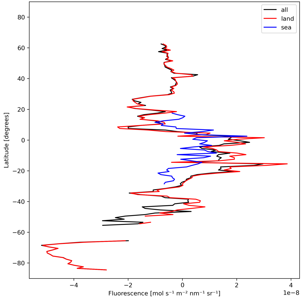
Figure 21: Zonal average of “Fluorescence” for 2023-10-25 to 2023-10-27.
