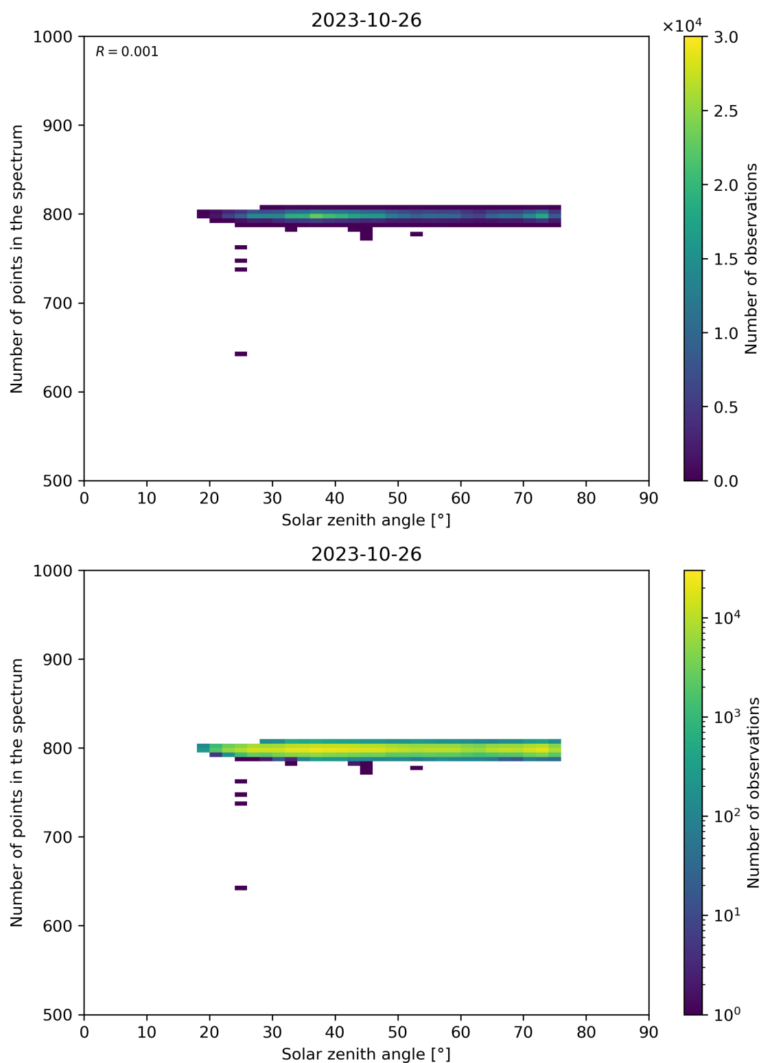
Figure 103: Scatter density plot of “Solar zenith angle” against “Number of points in the spectrum” for 2023-10-25 to 2023-10-27.
