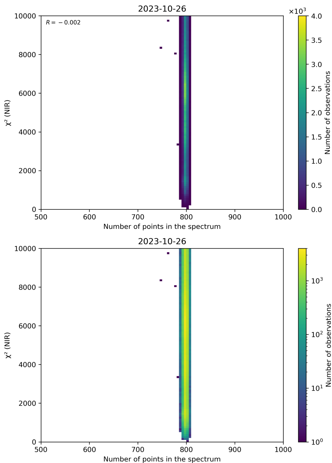
Figure 88: Scatter density plot of “Number of points in the spectrum” against “ \chi^2 (NIR)” for 2023-10-25 to 2023-10-27.
