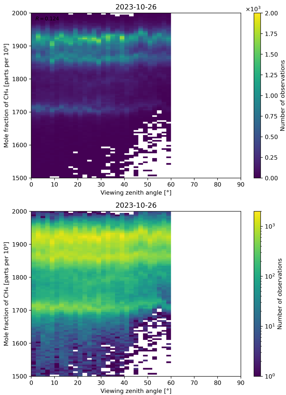
Figure 110: Scatter density plot of “Viewing zenith angle” against “Mole fraction of \text{CH}_4 ” for 2023-10-25 to 2023-10-27.
