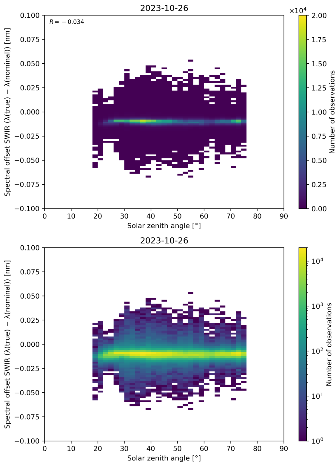
Figure 104: Scatter density plot of “Solar zenith angle” against “Spectral offset SWIR ( \lambda(\text{true}) - \lambda(\text{nominal}) )” for 2023-10-25 to 2023-10-27.
