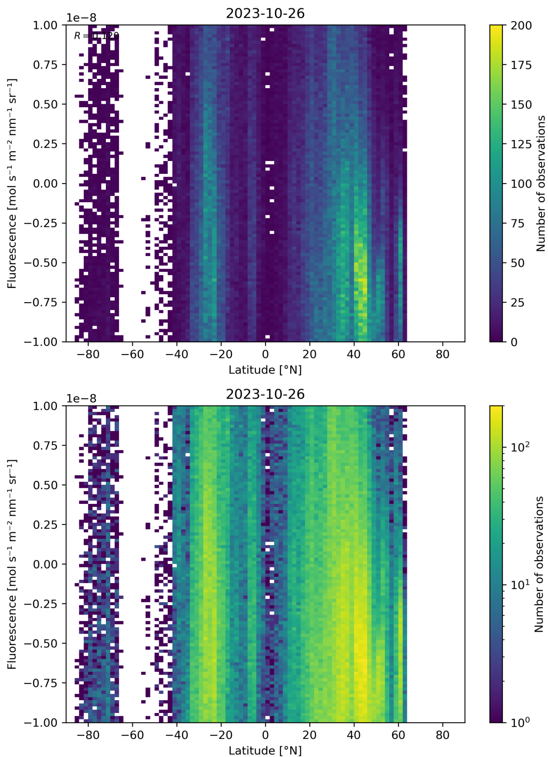
Figure 56: Scatter density plot of “Latitude” against “Fluorescence” for 2023-10-25 to 2023-10-27.
