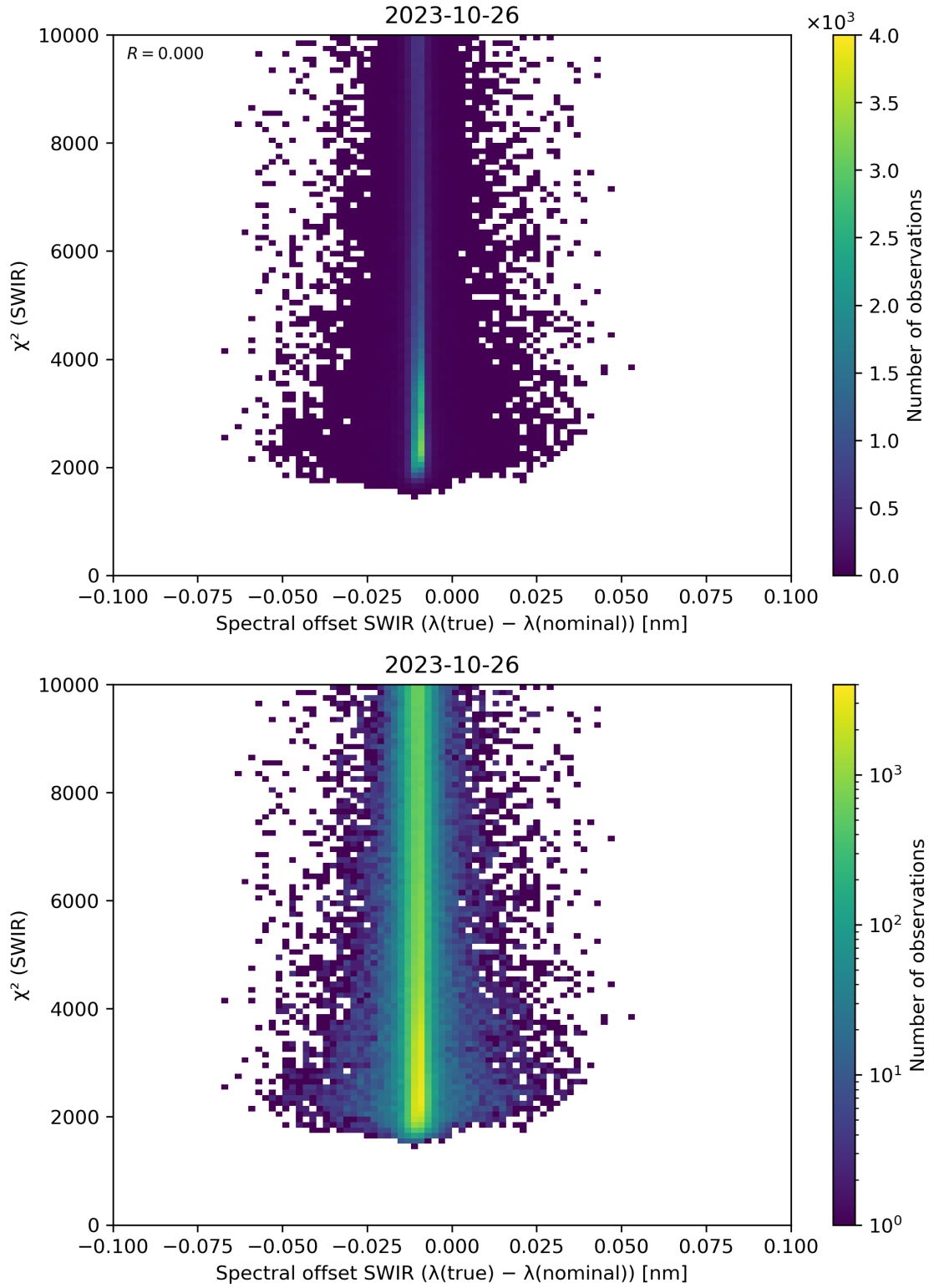
Figure 118: Scatter density plot of “Spectral offset SWIR ( \lambda(\text{true}) - \lambda(\text{nominal}) )” against “ \chi^2 (SWIR)” for 2023-10-25 to 2023-10-27.
