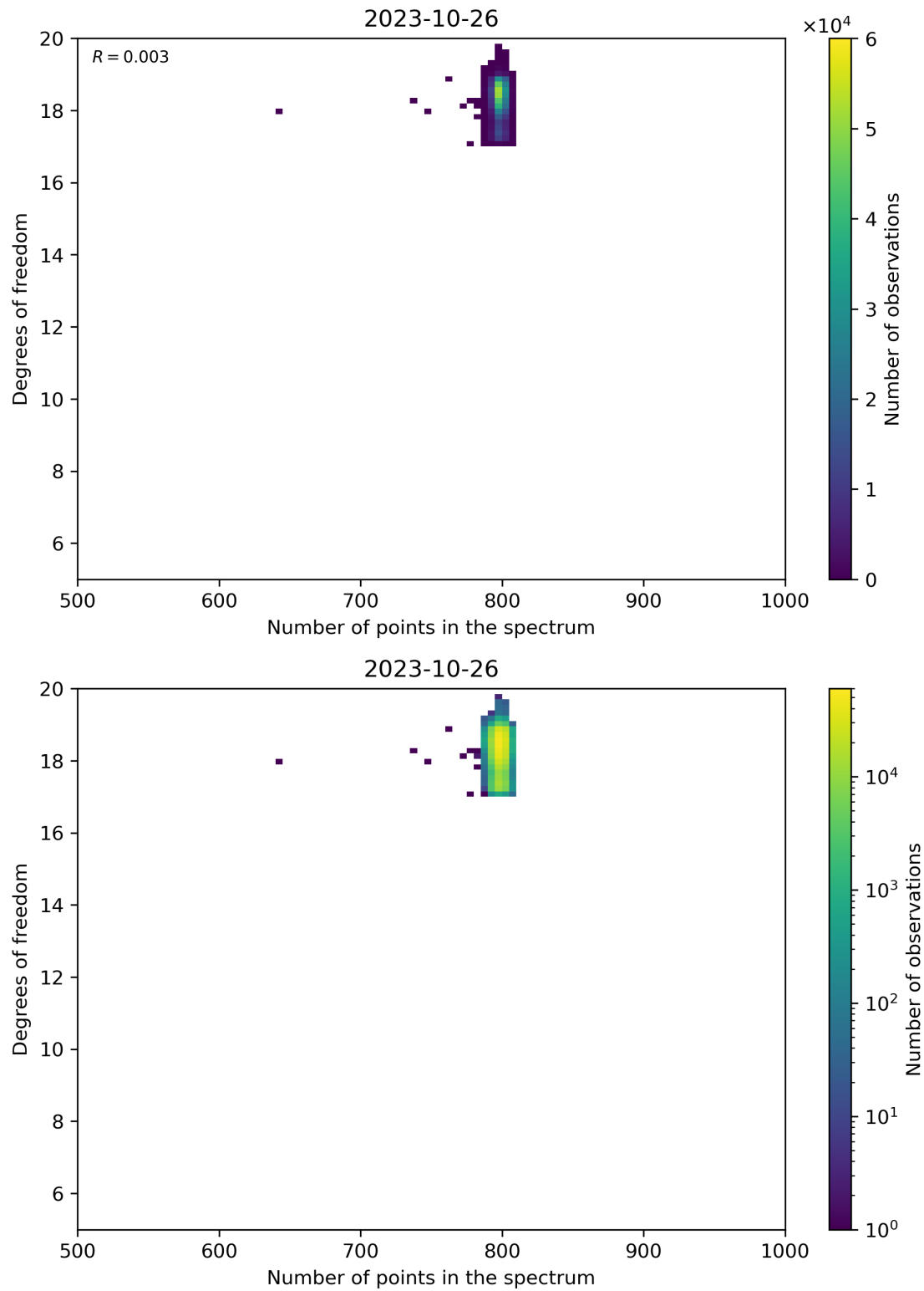
Figure 90: Scatter density plot of “Number of points in the spectrum” against “Degrees of freedom” for 2023-10-25 to 2023-10-27.
