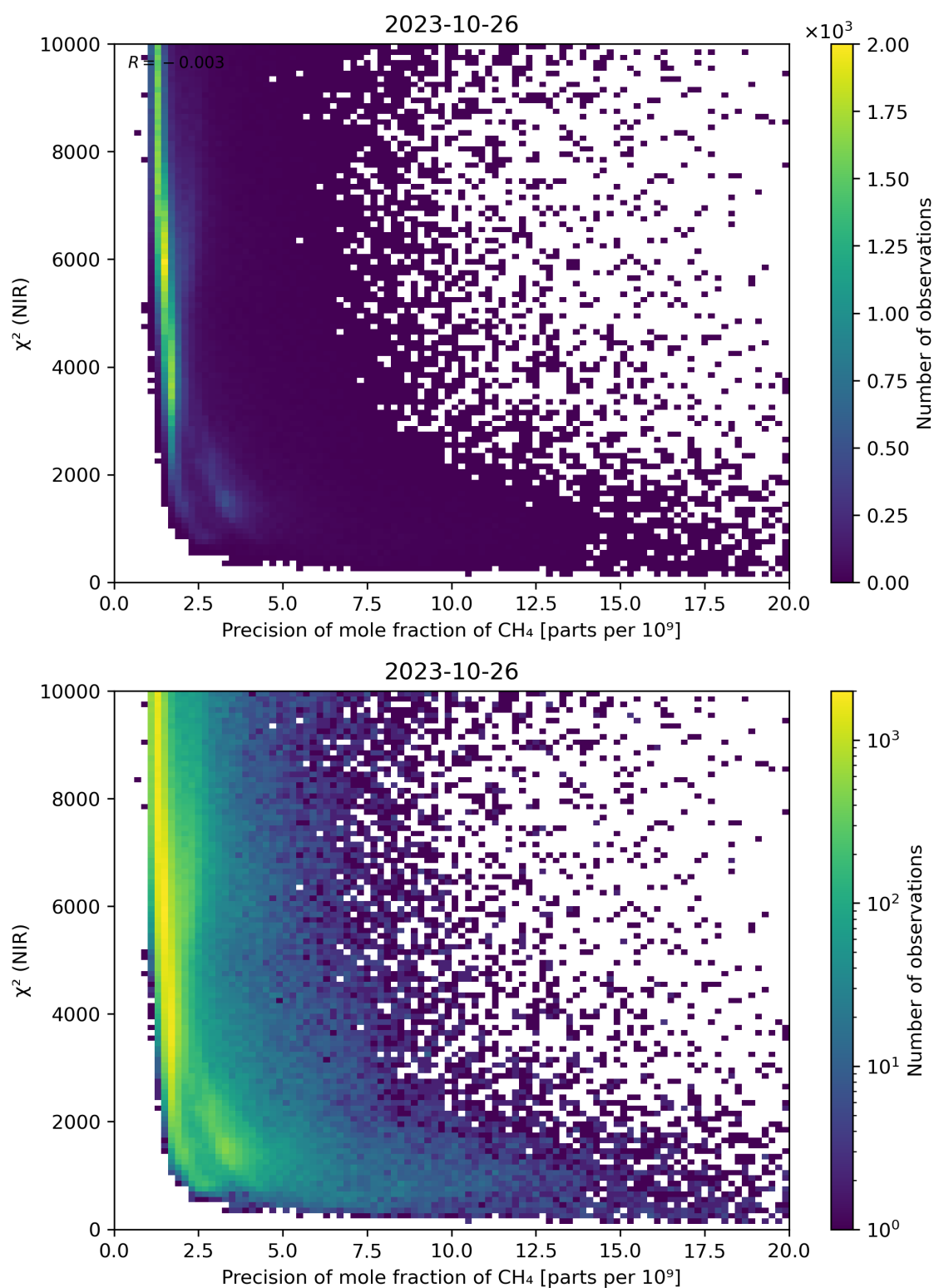
Figure 78: Scatter density plot of “Precision of mole fraction of \text{CH}_4 ” against “ \chi^2 (NIR)” for 2023-10-25 to 2023-10-27.
