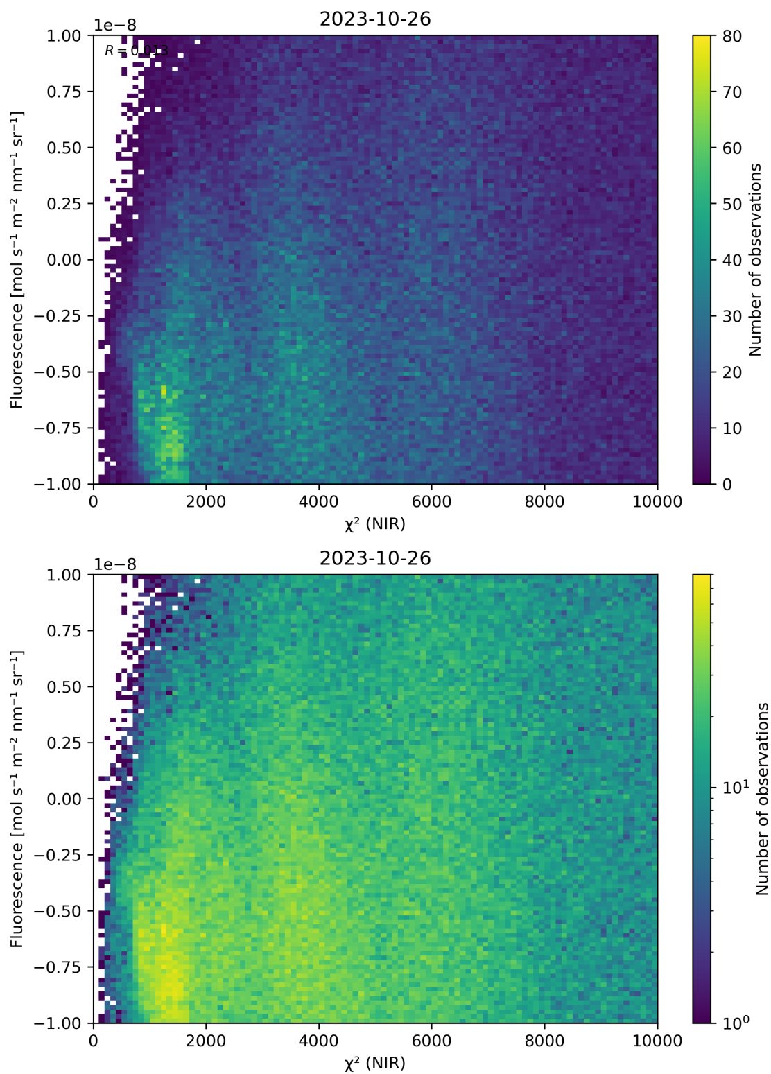
Figure 45: Scatter density plot of “ \chi^2 (NIR)” against “Fluorescence” for 2023-10-25 to 2023-10-27.
