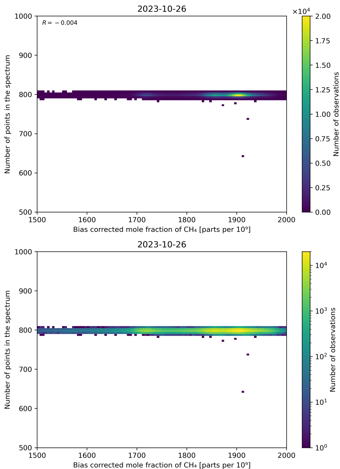
Figure 68: Scatter density plot of “Bias corrected mole fraction of CH 4 ” against “Number of points in the spectrum” for 2023-10-25 to 2023-10-27.
