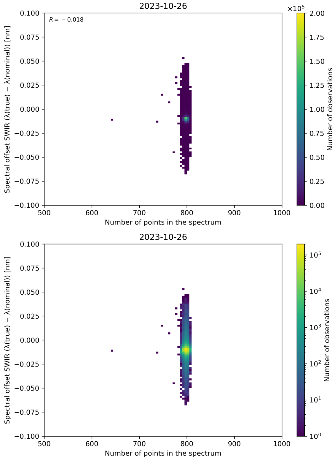
Figure 93: Scatter density plot of “Number of points in the spectrum” against “Spectral offset SWIR ( \lambda(\text{true}) - \lambda(\text{nominal}) )” for 2023-10-25 to 2023-10-27.
