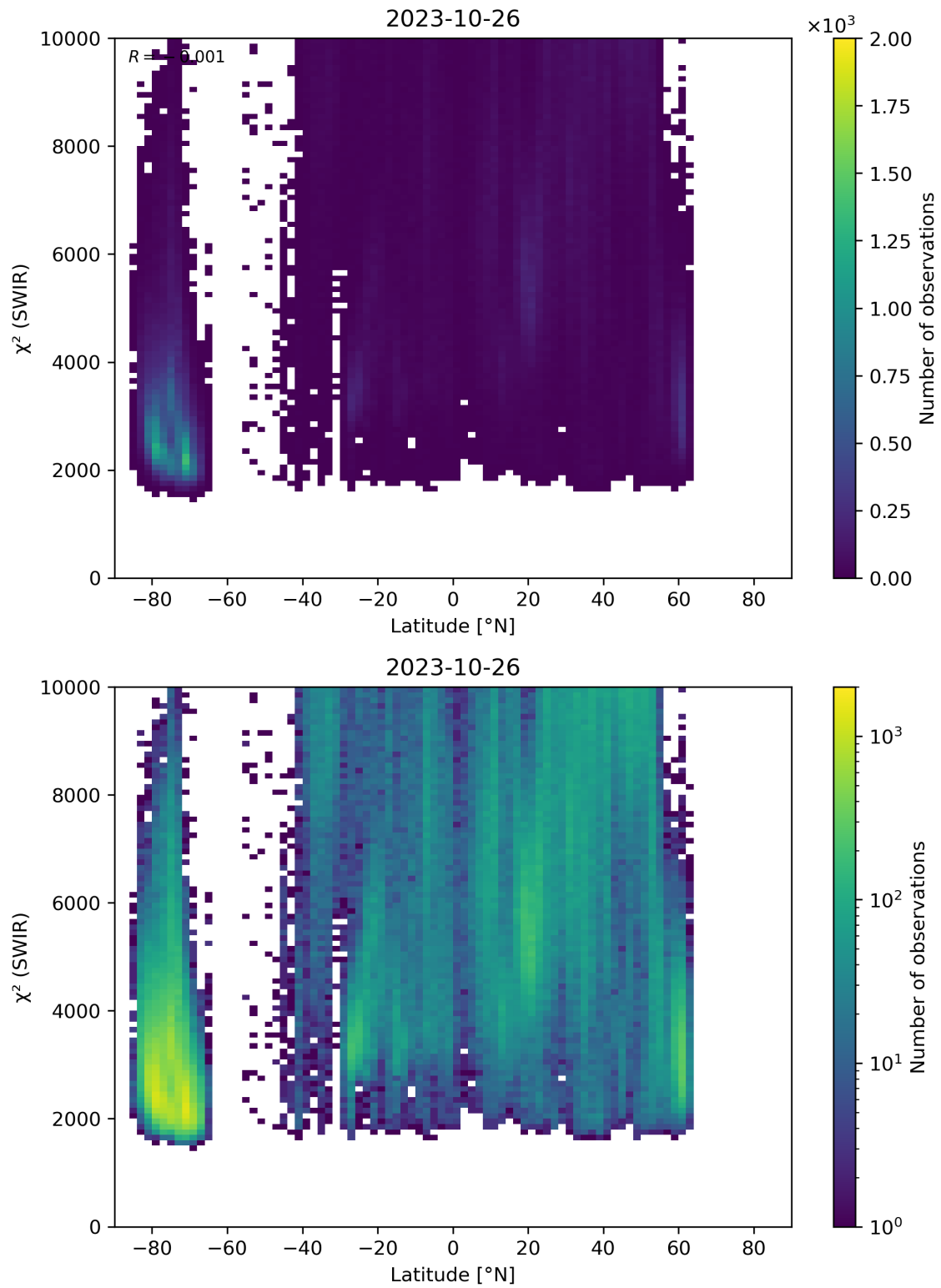
Figure 54: Scatter density plot of “Latitude” against “ \chi^2 (SWIR)” for 2023-10-25 to 2023-10-27.
