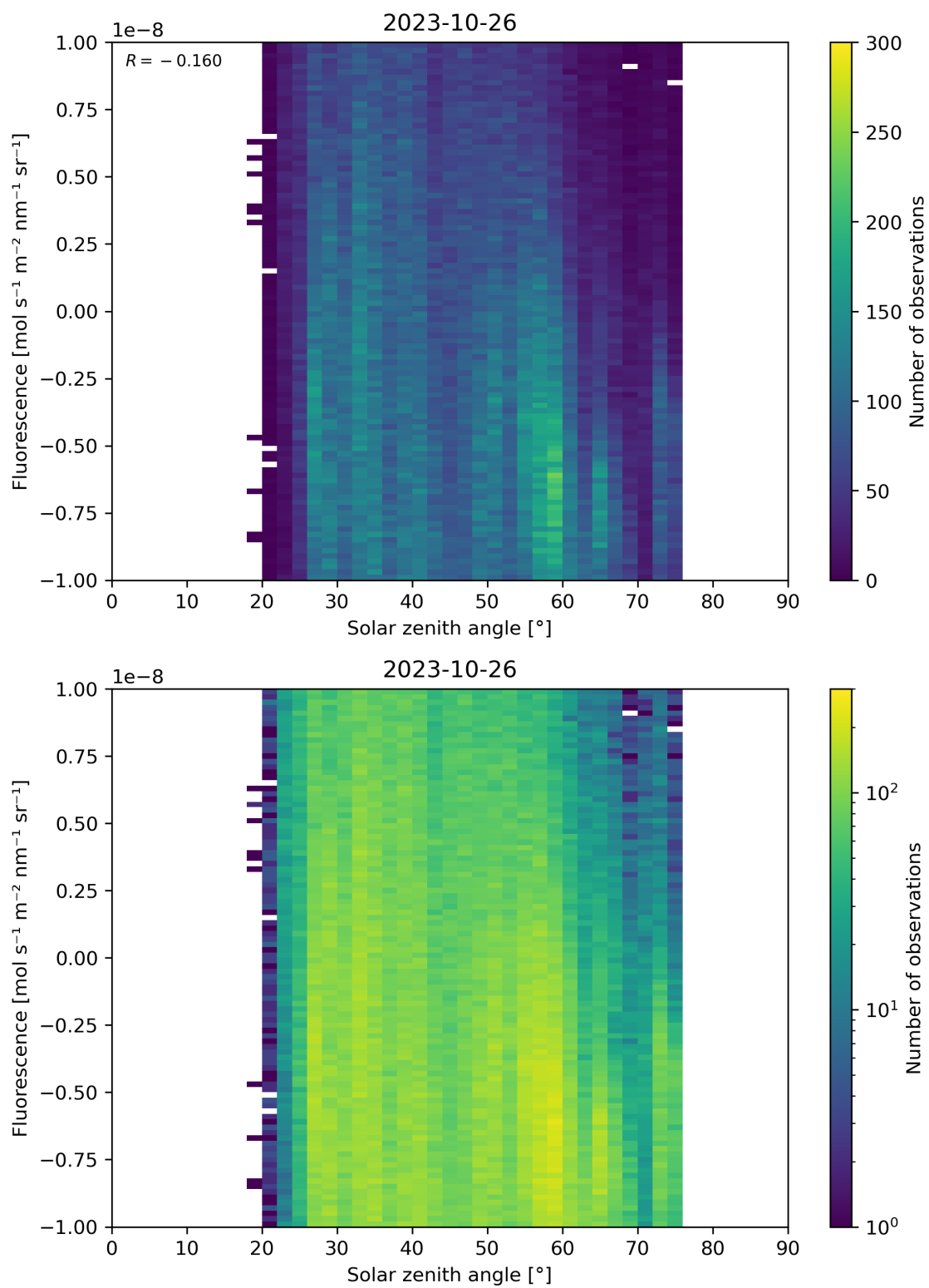
Figure 97: Scatter density plot of “Solar zenith angle” against “Fluorescence” for 2023-10-25 to 2023-10-27.
