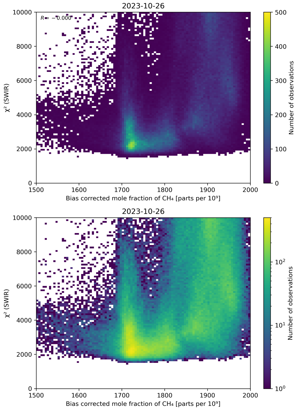
Figure 64: Scatter density plot of “Bias corrected mole fraction of CH 4 ” against “ \chi^2 (SWIR)” for 2023-10-25 to 2023-10-27.
