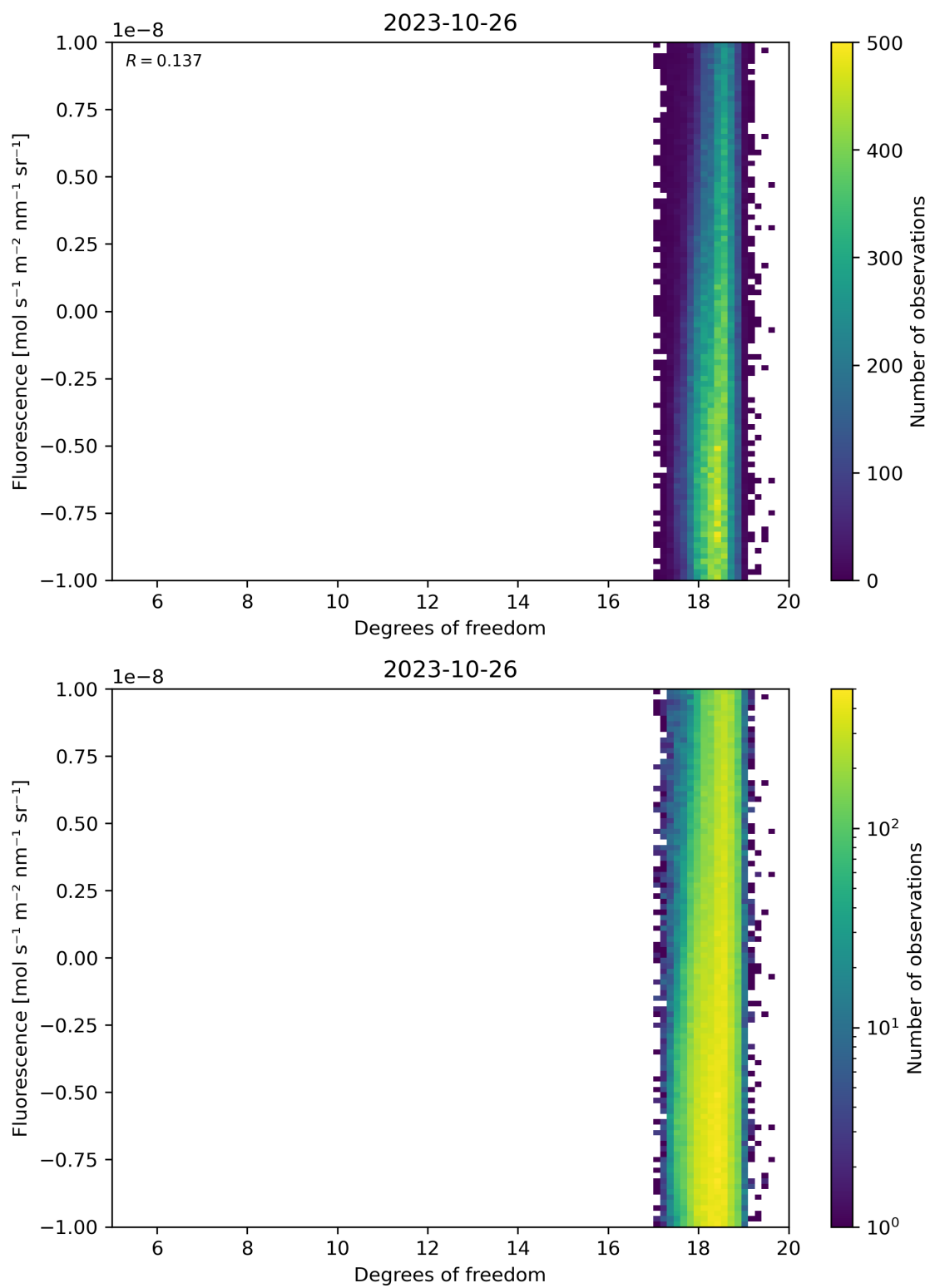
Figure 51: Scatter density plot of “Degrees of freedom” against “Fluorescence” for 2023-10-25 to 2023-10-27.
