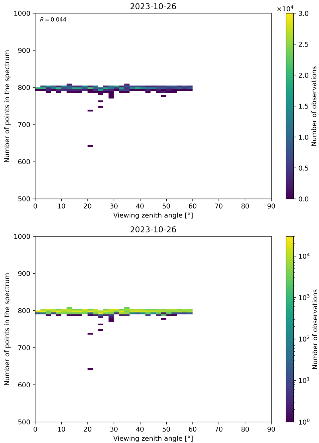
Figure 114: Scatter density plot of “Viewing zenith angle” against “Number of points in the spectrum” for 2023-10-25 to 2023-10-27.
