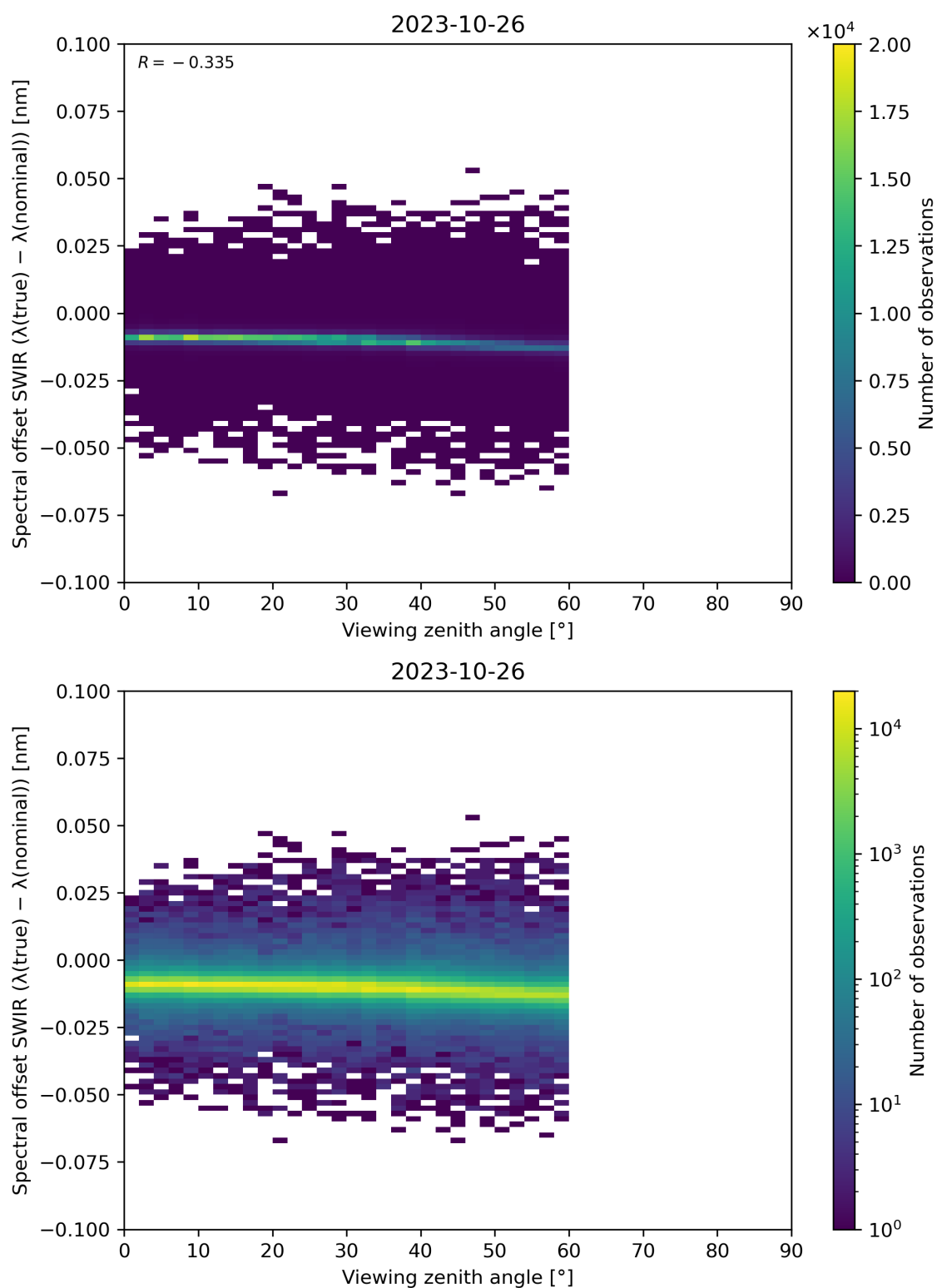
Figure 116: Scatter density plot of “Viewing zenith angle” against “Spectral offset SWIR ( \lambda(\text{true}) - \lambda(\text{nominal}) )” for 2023-10-25 to 2023-10-27.
