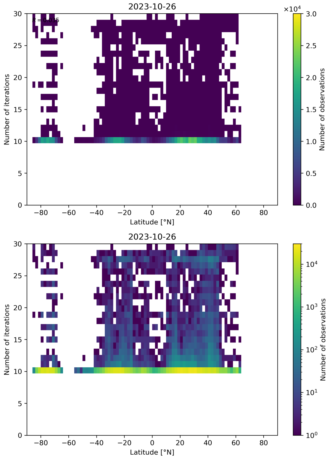
Figure 60: Scatter density plot of “Latitude” against “Number of iterations” for 2023-10-25 to 2023-10-27.
