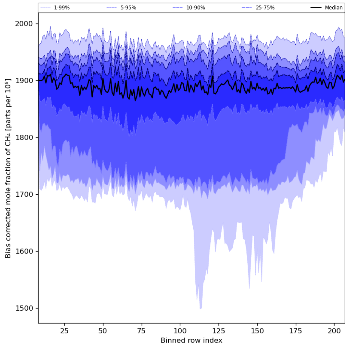
Figure 36: Along track statistics of “Bias corrected mole fraction of CH 4 ” for 2023-10-25 to 2023-10-27
