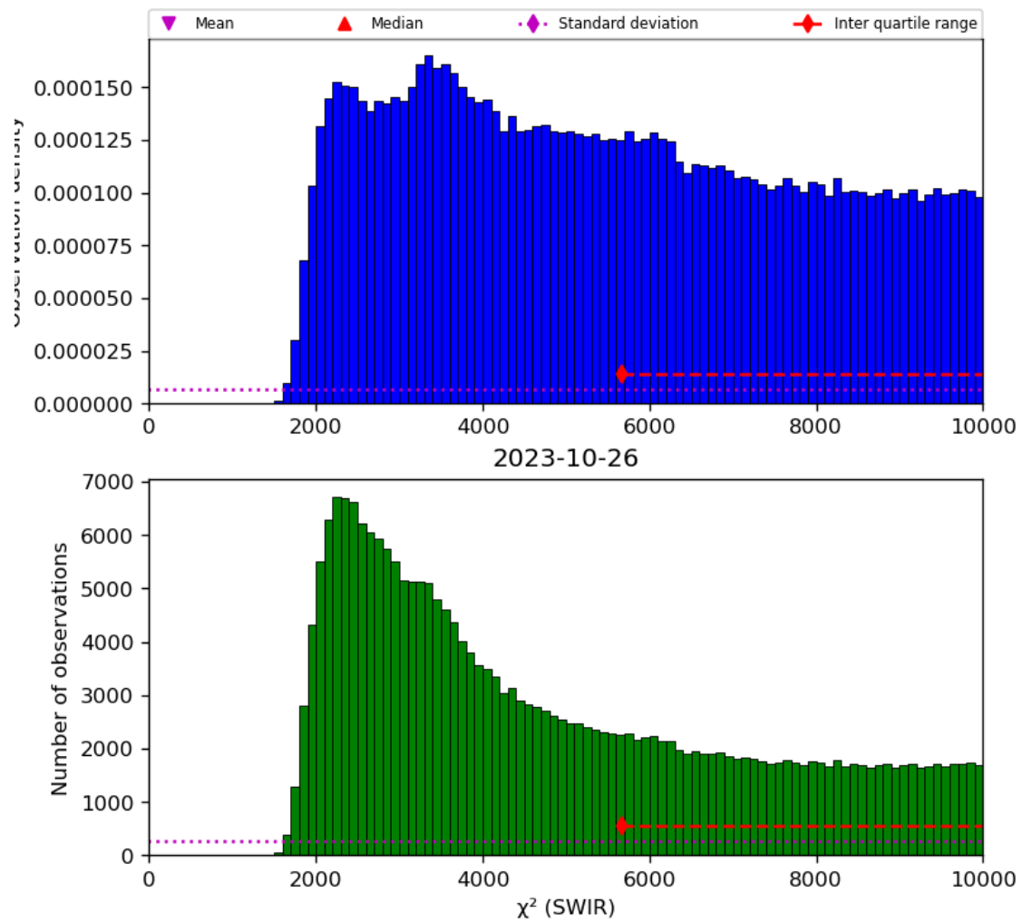
Figure 28: Histogram of “ \chi^2 (SWIR)” for 2023-10-25 to 2023-10-27
