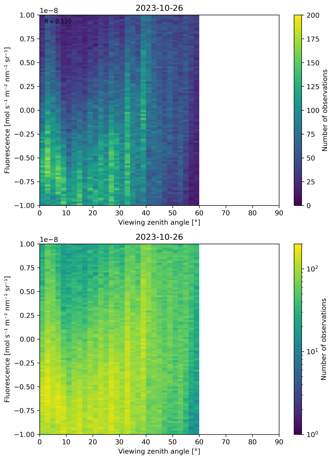
Figure 108: Scatter density plot of “Viewing zenith angle” against “Fluorescence” for 2023-10-25 to 2023-10-27.
