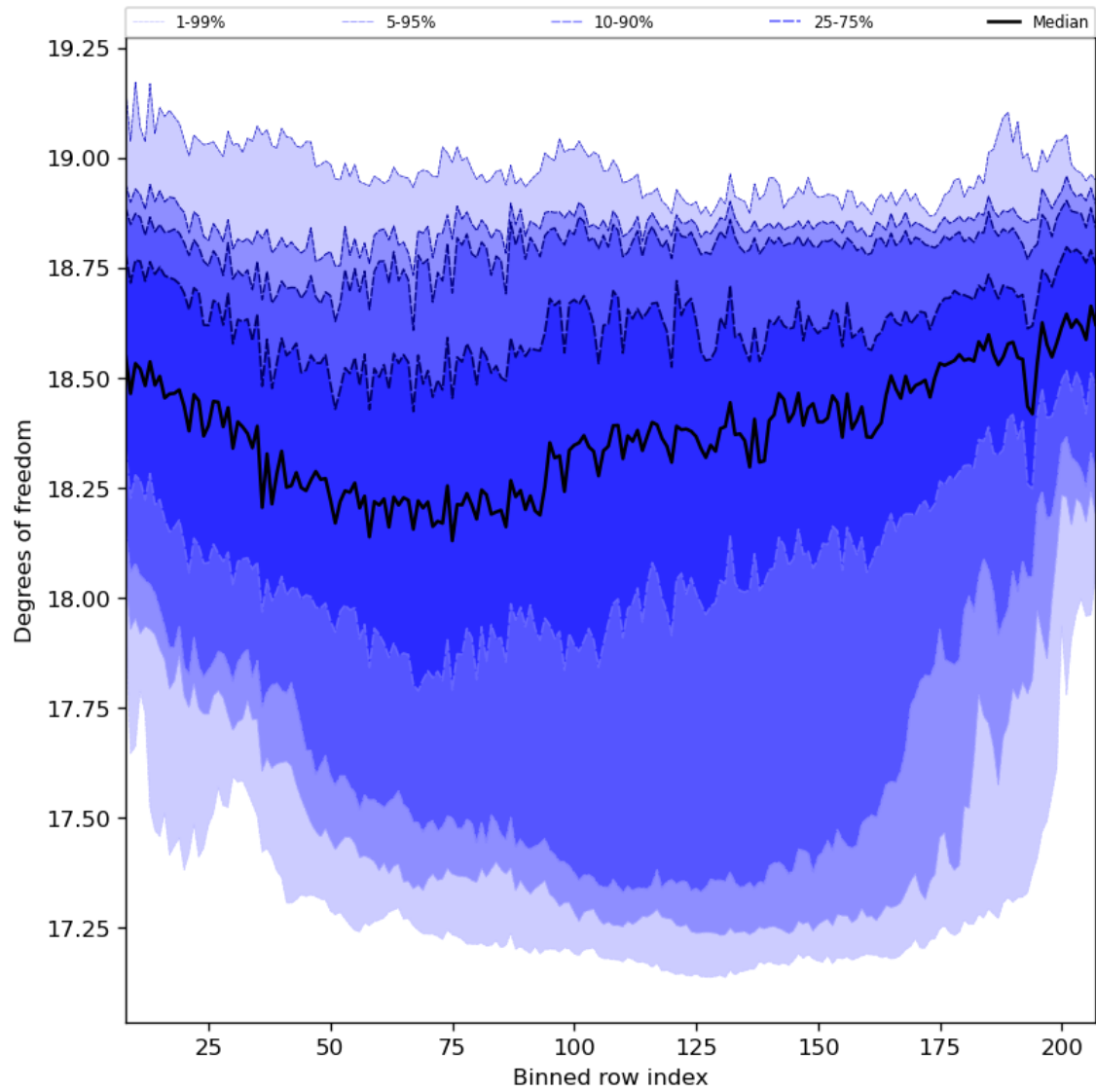
Figure 41: Along track statistics of “Degrees of freedom” for 2023-10-25 to 2023-10-27
