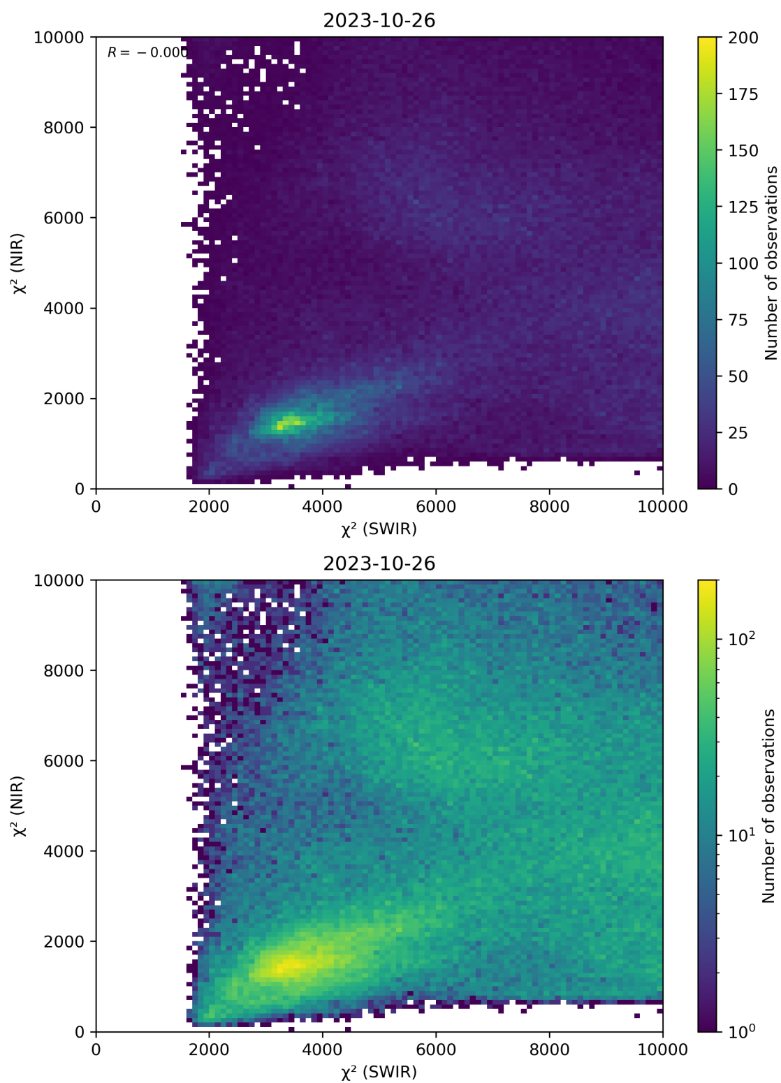
Figure 47: Scatter density plot of “ \chi^2 (SWIR)” against “ \chi^2 (NIR)” for 2023-10-25 to 2023-10-27.
