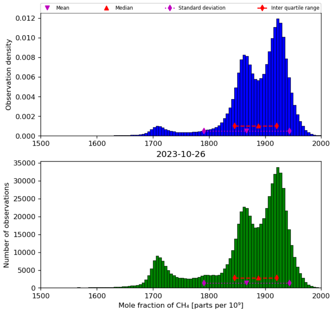
Figure 23: Histogram of “Mole fraction of CH 4 ” for 2023-10-25 to 2023-10-27
