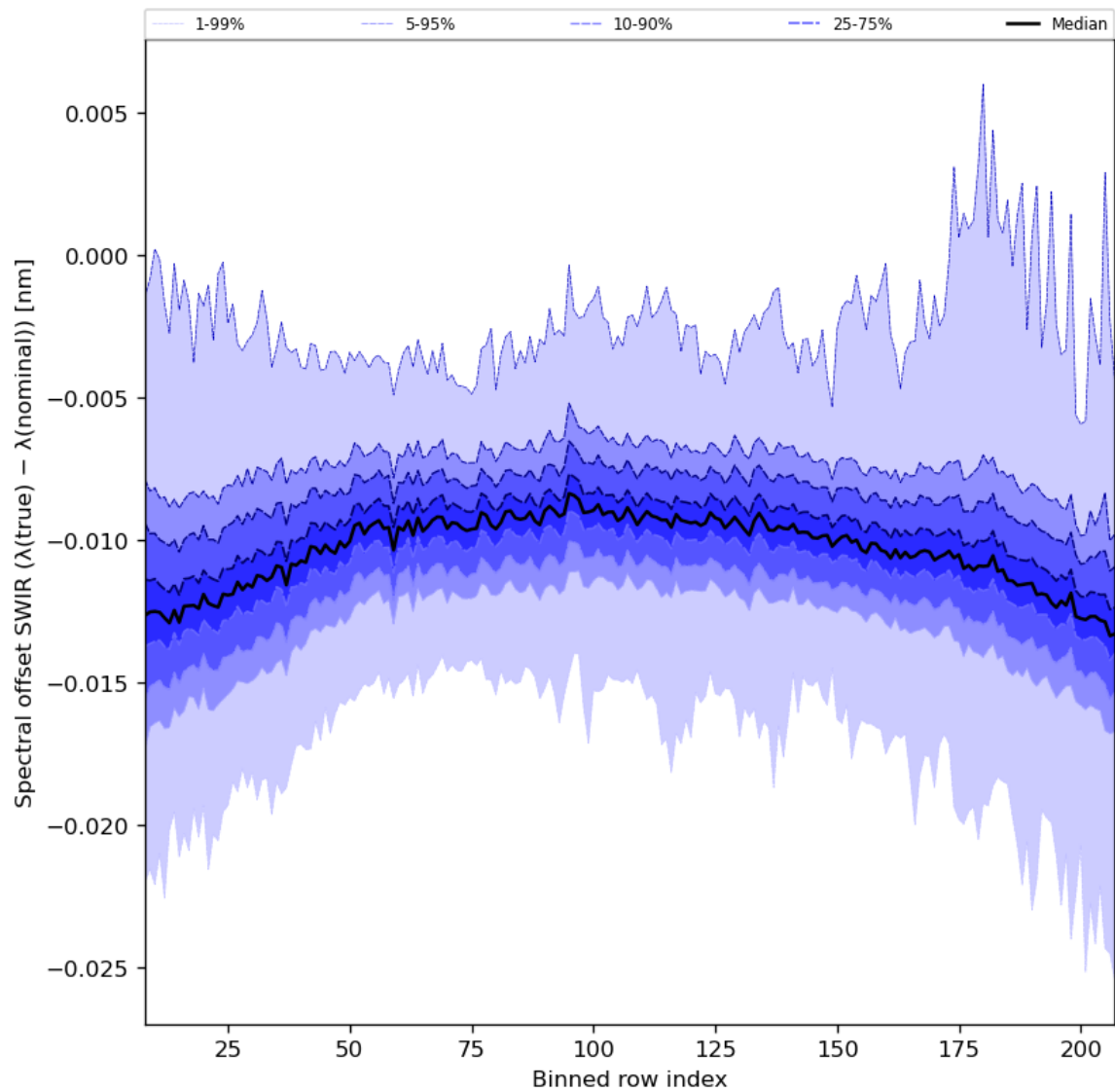
Figure 38: Along track statistics of “Spectral offset SWIR ( \lambda(\text{true}) - \lambda(\text{nominal}) )” for 2023-10-25 to 2023-10-27
