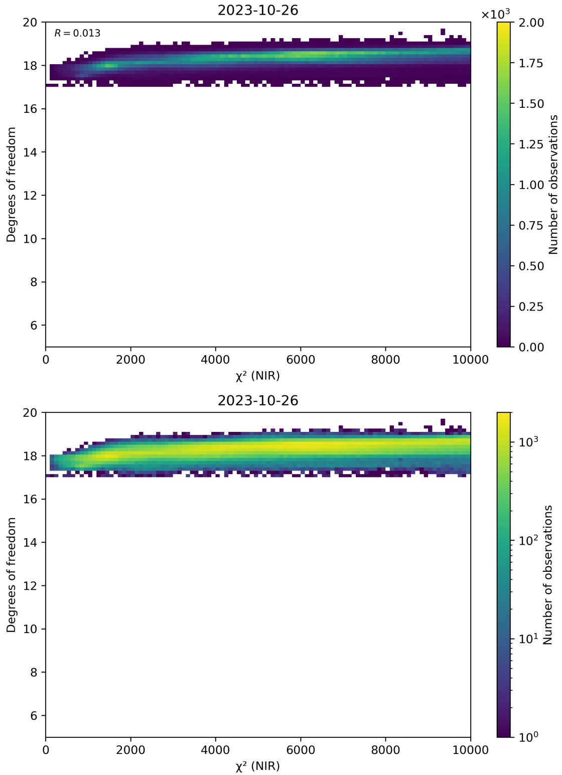
Figure 44: Scatter density plot of “ \chi^2 (NIR)” against “Degrees of freedom” for 2023-10-25 to 2023-10-27.
