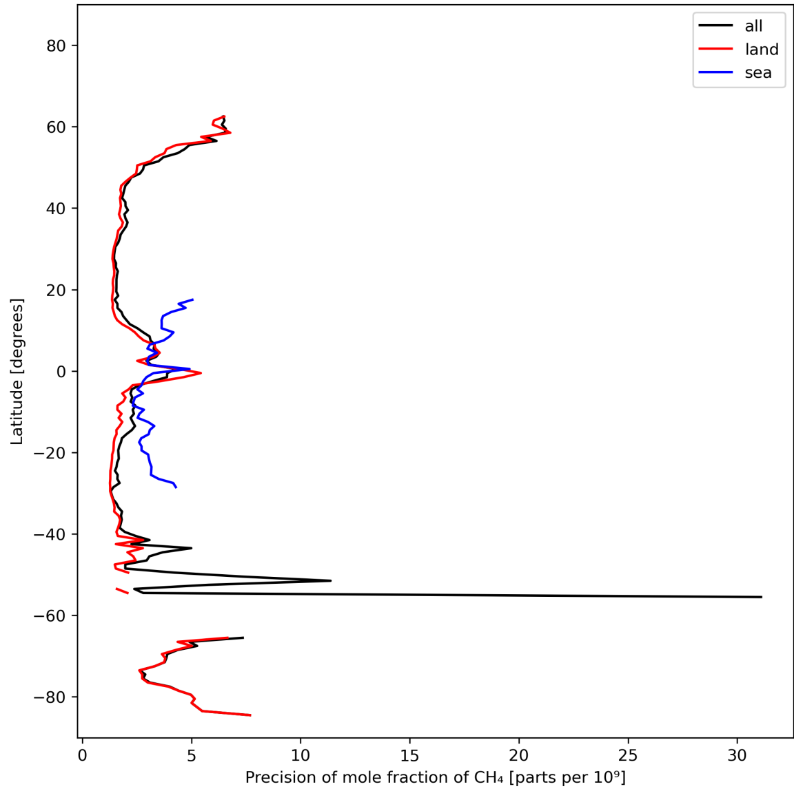
Figure 13: Zonal average of “Precision of mole fraction of CH 4 ” for 2023-10-25 to 2023-10-27.
