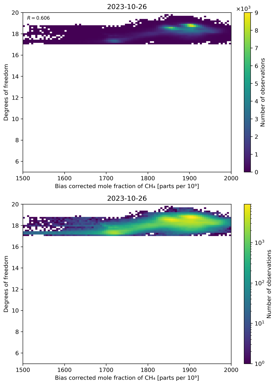
Figure 65: Scatter density plot of “Bias corrected mole fraction of CH 4 ” against “Degrees of freedom” for 2023-10-25 to 2023-10-27.
