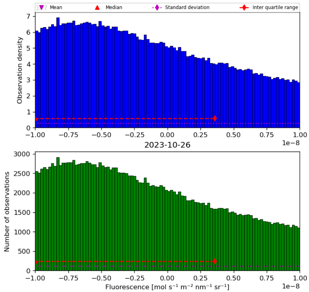
Figure 32: Histogram of “Fluorescence” for 2023-10-25 to 2023-10-27
