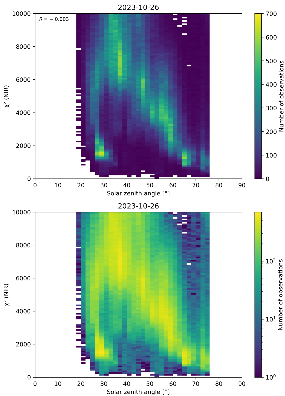
Figure 94: Scatter density plot of “Solar zenith angle” against “ \chi^2 (NIR)” for 2023-10-25 to 2023-10-27.
