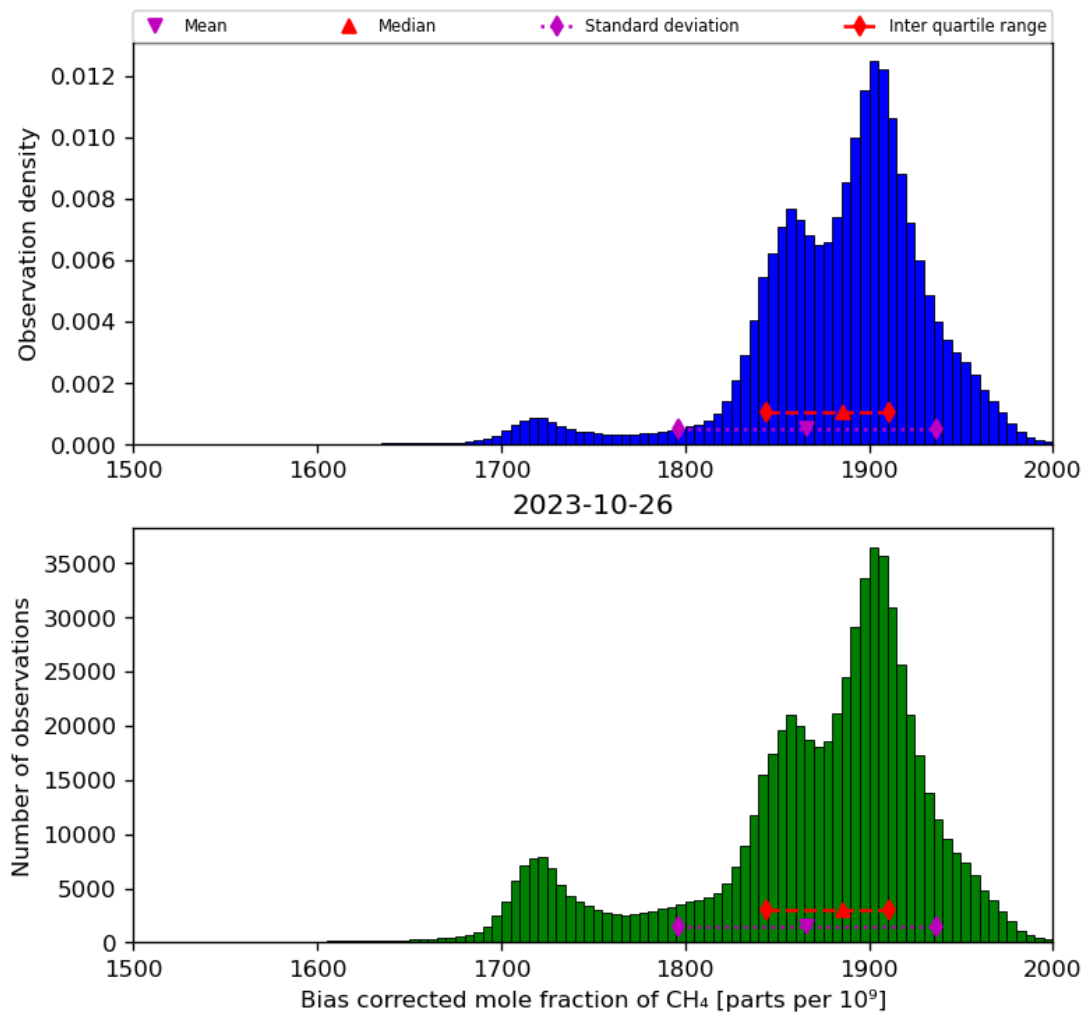
Figure 25: Histogram of “Bias corrected mole fraction of CH 4 ” for 2023-10-25 to 2023-10-27
