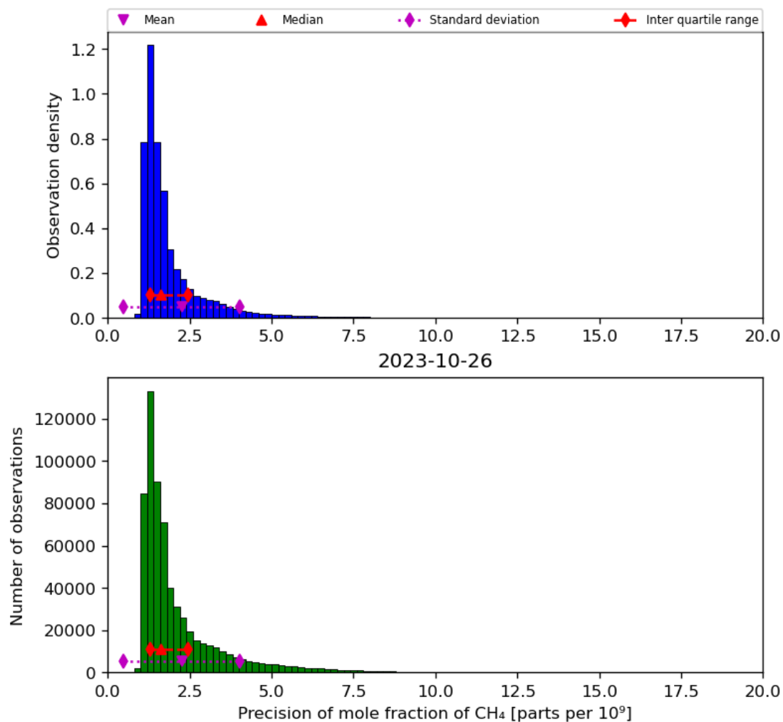
Figure 24: Histogram of “Precision of mole fraction of CH 4 ” for 2023-10-25 to 2023-10-27
