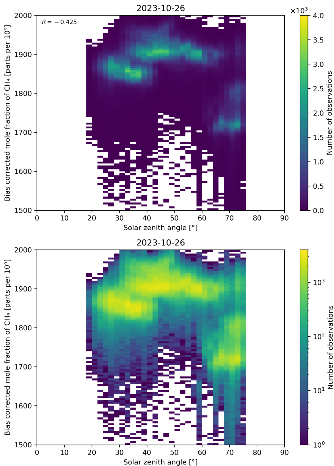
Figure 100: Scatter density plot of “Solar zenith angle” against “Bias corrected mole fraction of \text{CH}_4 ” for 2023-10-25 to 2023-10-27.
