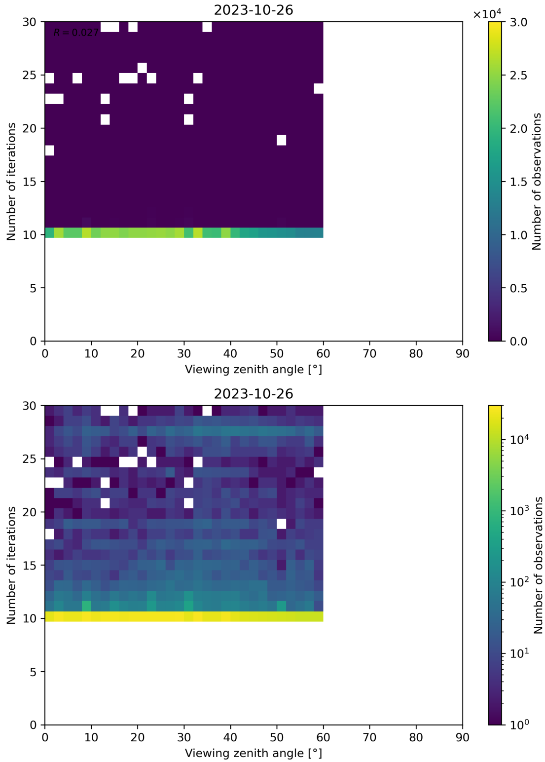
Figure 113: Scatter density plot of “Viewing zenith angle” against “Number of iterations” for 2023-10-25 to 2023-10-27.
