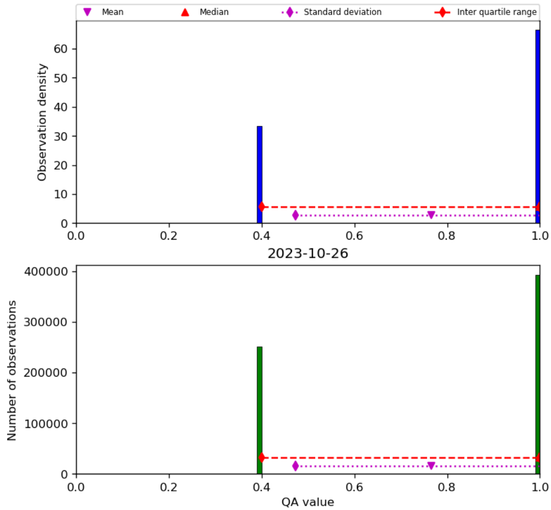
Figure 22: Histogram of “QA value” for 2023-10-25 to 2023-10-27
