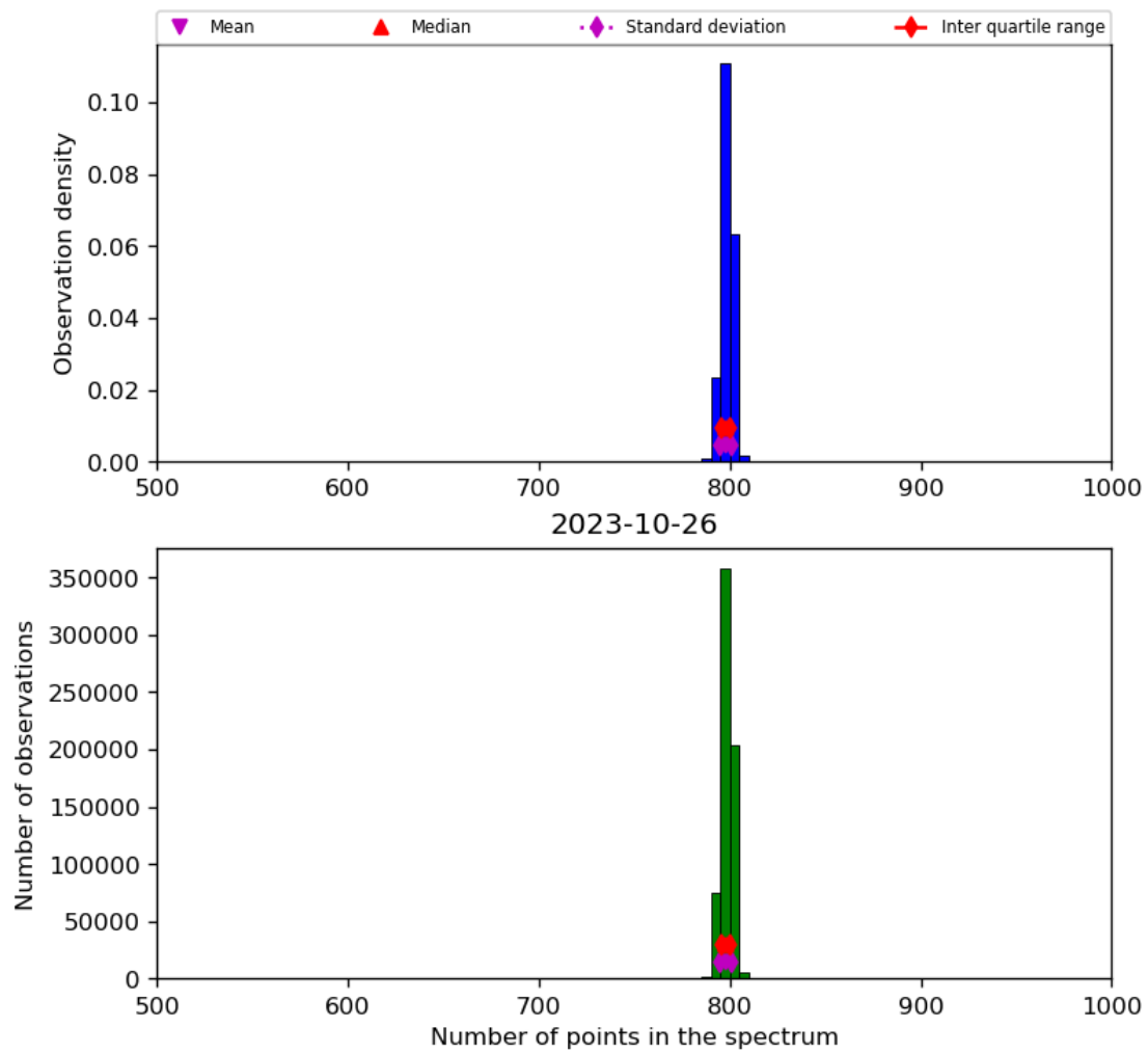
Figure 26: Histogram of “Number of points in the spectrum” for 2023-10-25 to 2023-10-27
