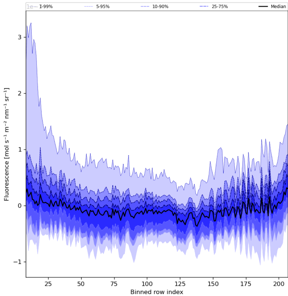
Figure 43: Along track statistics of “Fluorescence” for 2023-10-25 to 2023-10-27
