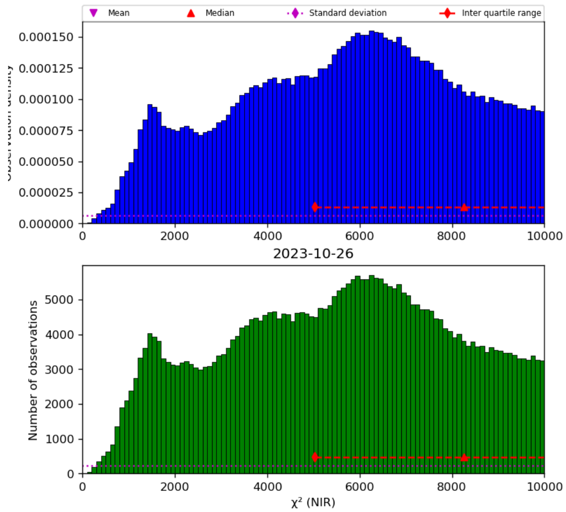
Figure 29: Histogram of “ \chi^2 (NIR)” for 2023-10-25 to 2023-10-27
