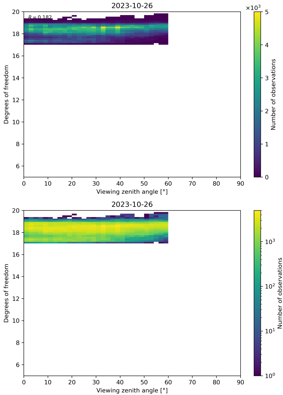
Figure 107: Scatter density plot of “Viewing zenith angle” against “Degrees of freedom” for 2023-10-25 to 2023-10-27.
