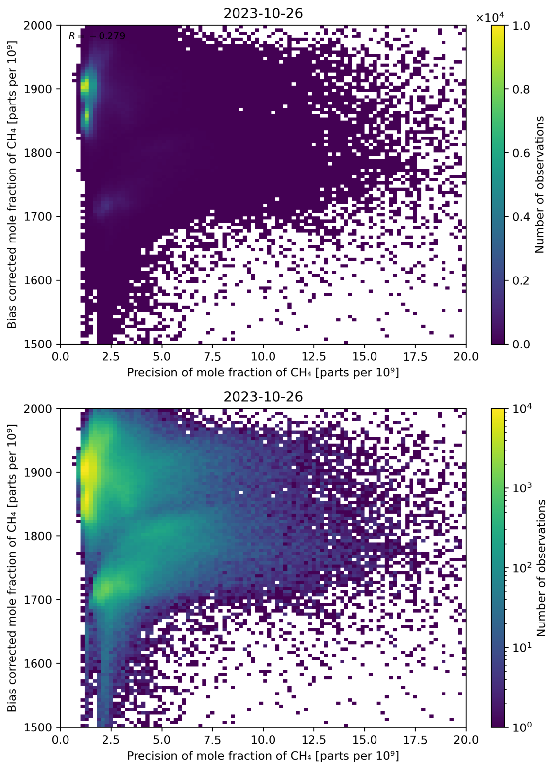
Figure 82: Scatter density plot of “Precision of mole fraction of \text{CH}_4 ” against “Bias corrected mole fraction of \text{CH}_4 ” for 2023-10-25 to 2023-10-27.
