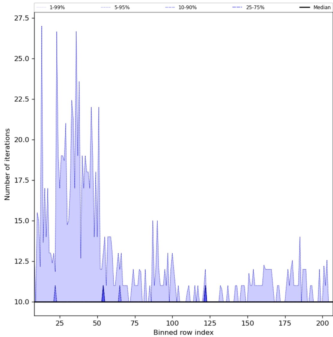
Figure 42: Along track statistics of “Number of iterations” for 2023-10-25 to 2023-10-27
