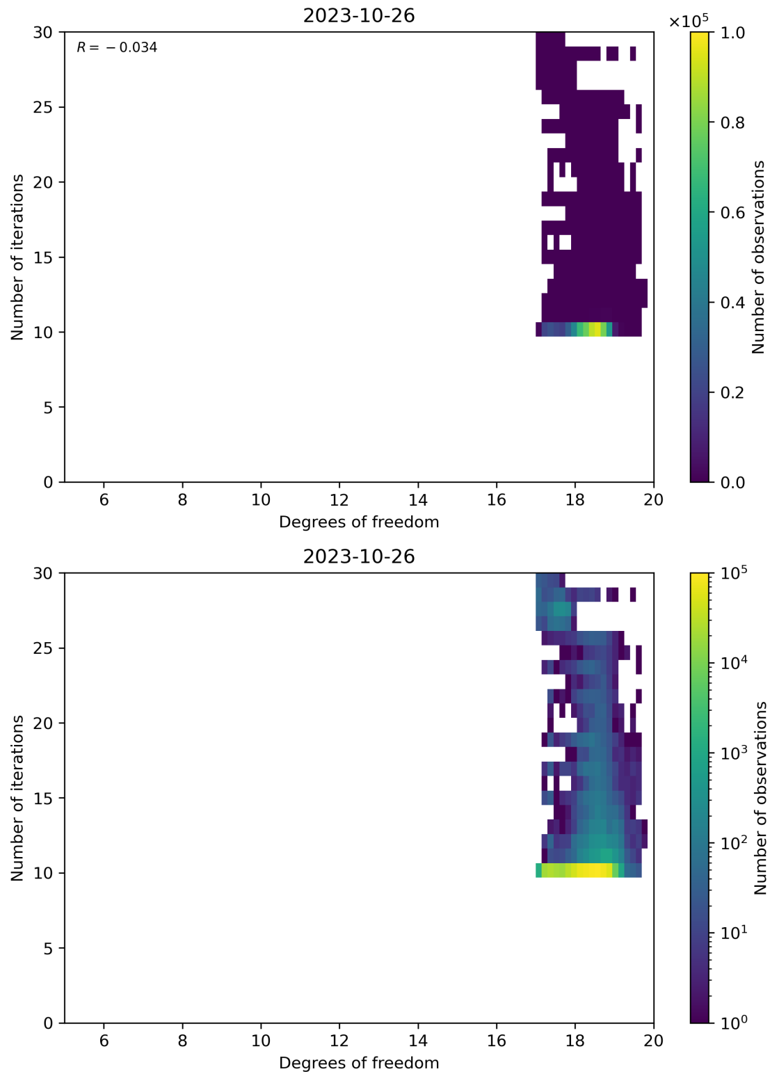
Figure 52: Scatter density plot of “Degrees of freedom” against “Number of iterations” for 2023-10-25 to 2023-10-27.
