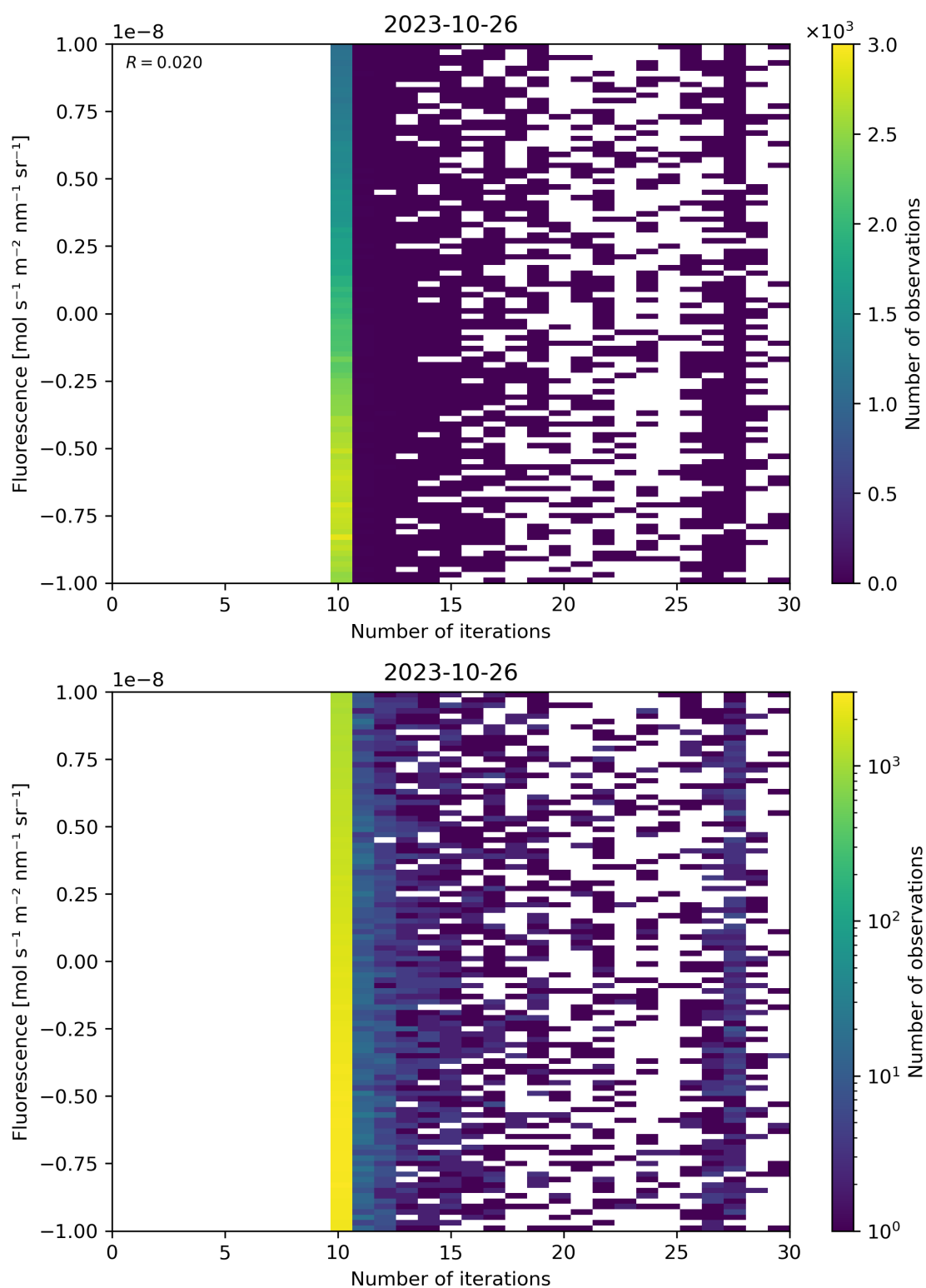
Figure 87: Scatter density plot of “Number of iterations” against “Fluorescence” for 2023-10-25 to 2023-10-27.
