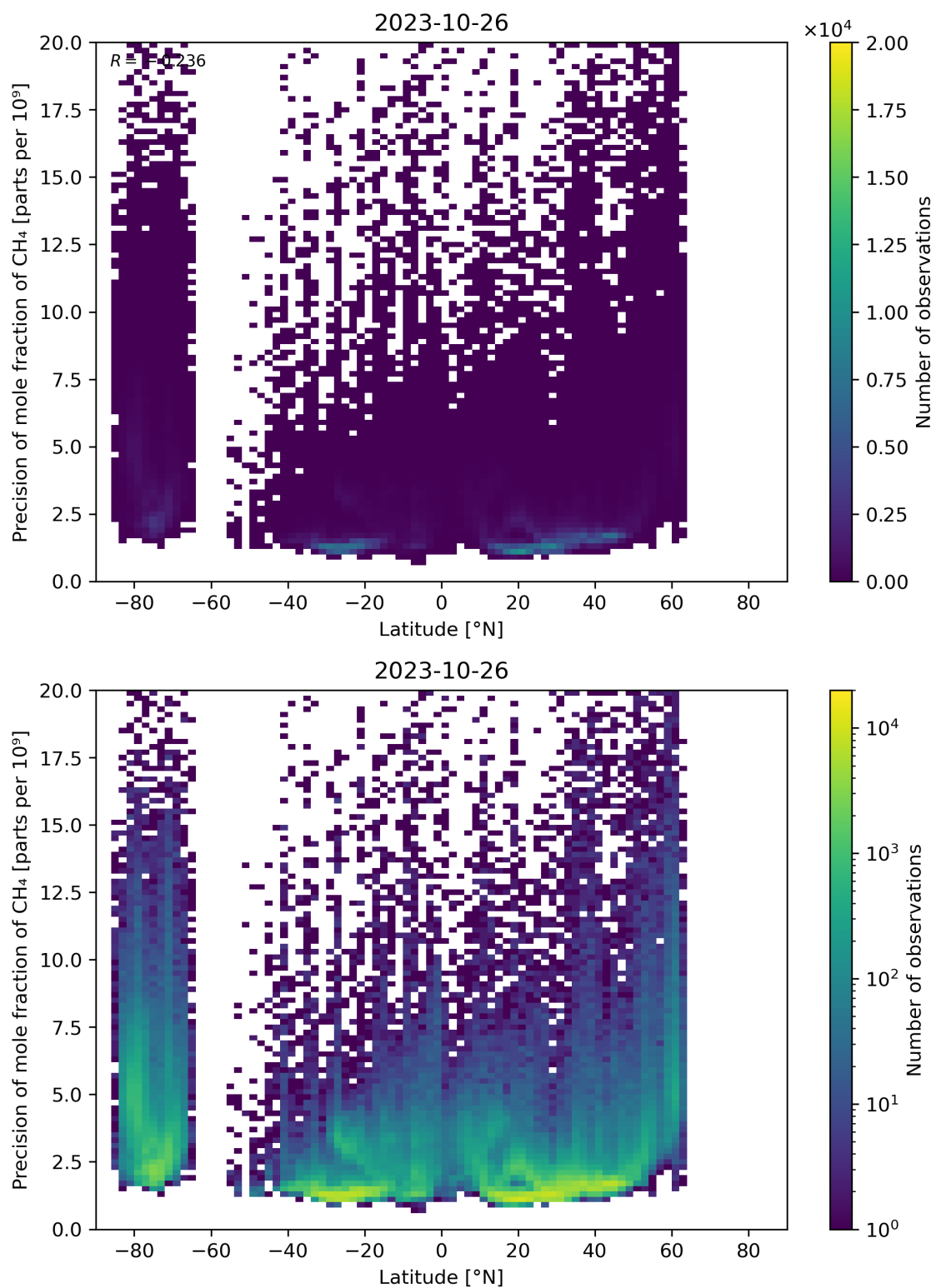
Figure 59: Scatter density plot of “Latitude” against “Precision of mole fraction of CH 4 ” for 2023-10-25 to 2023-10-27.
