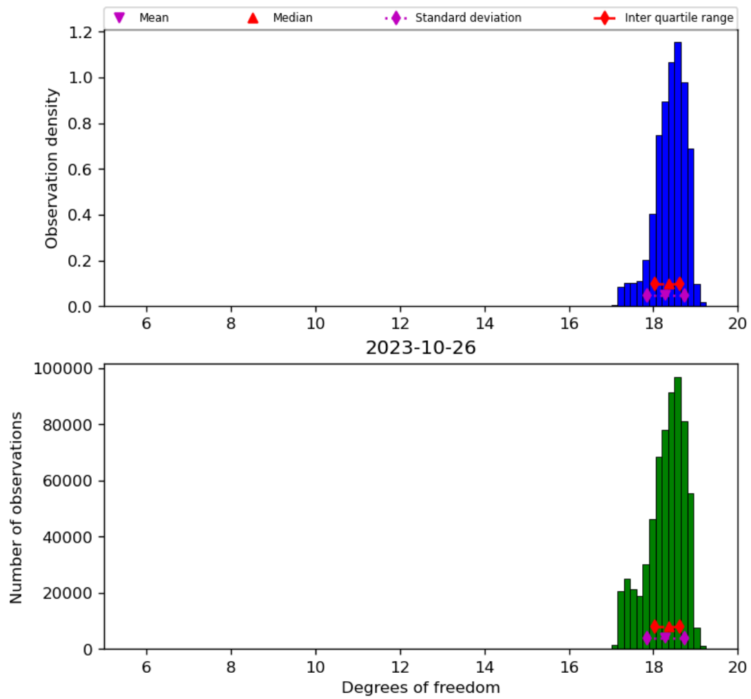
Figure 30: Histogram of “Degrees of freedom” for 2023-10-25 to 2023-10-27
