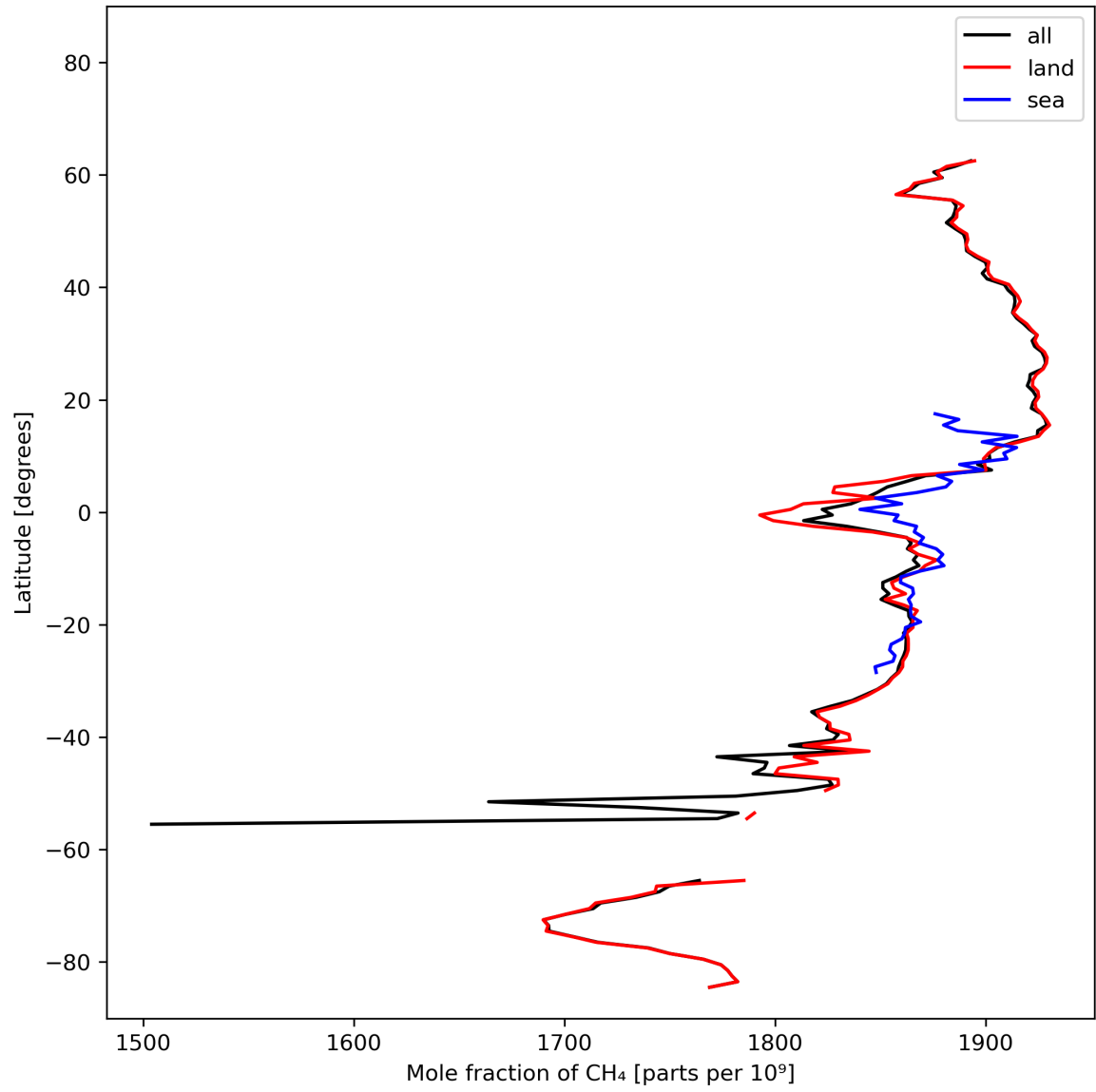
Figure 12: Zonal average of “Mole fraction of \text{CH}_4 ” for 2023-10-25 to 2023-10-27.
