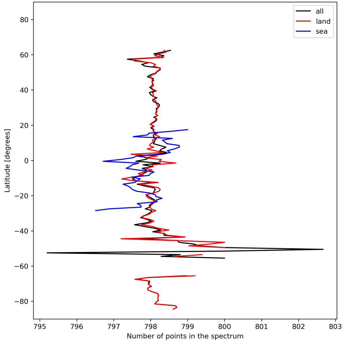
Figure 15: Zonal average of “Number of points in the spectrum” for 2023-10-25 to 2023-10-27.
