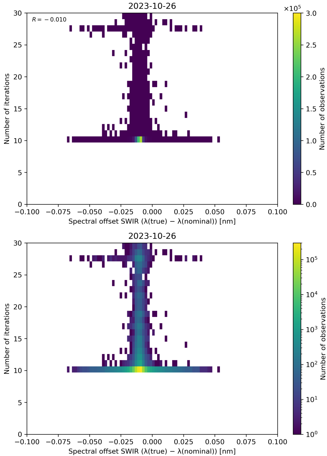
Figure 121: Scatter density plot of “Spectral offset SWIR ( \lambda(\text{true}) - \lambda(\text{nominal}) )” against “Number of iterations” for 2023-10-25 to 2023-10-27.
