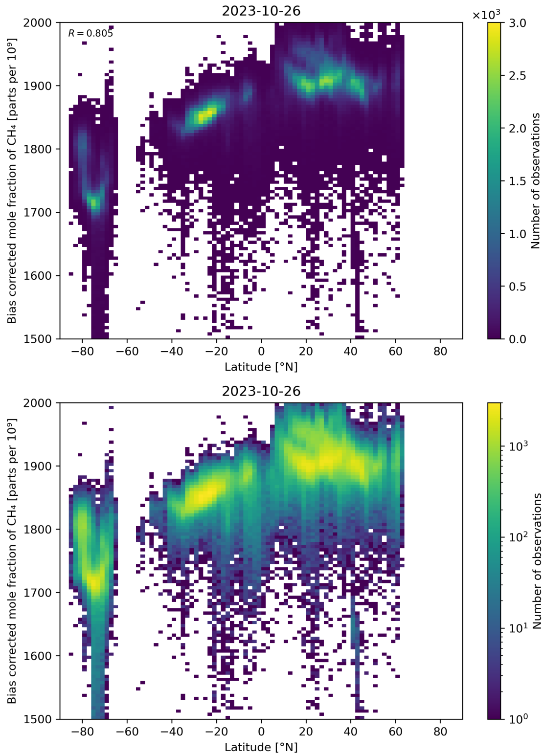
Figure 58: Scatter density plot of “Latitude” against “Bias corrected mole fraction of \text{CH}_4 ” for 2023-10-25 to 2023-10-27.
