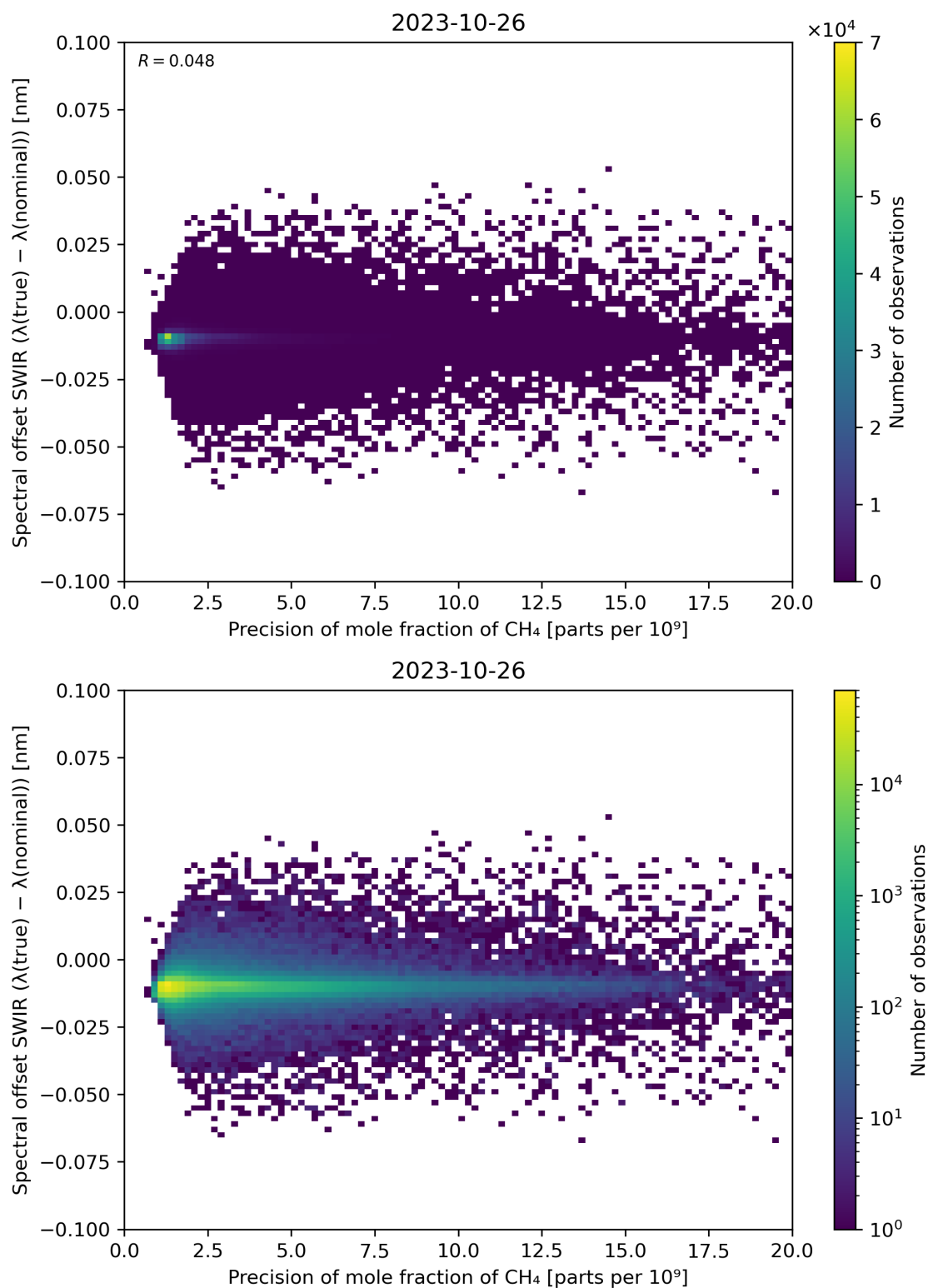
Figure 85: Scatter density plot of “Precision of mole fraction of CH 4 ” against “Spectral offset SWIR ( \lambda(\text{true}) - \lambda(\text{nominal}) )” for 2023-10-25 to 2023-10-27.
