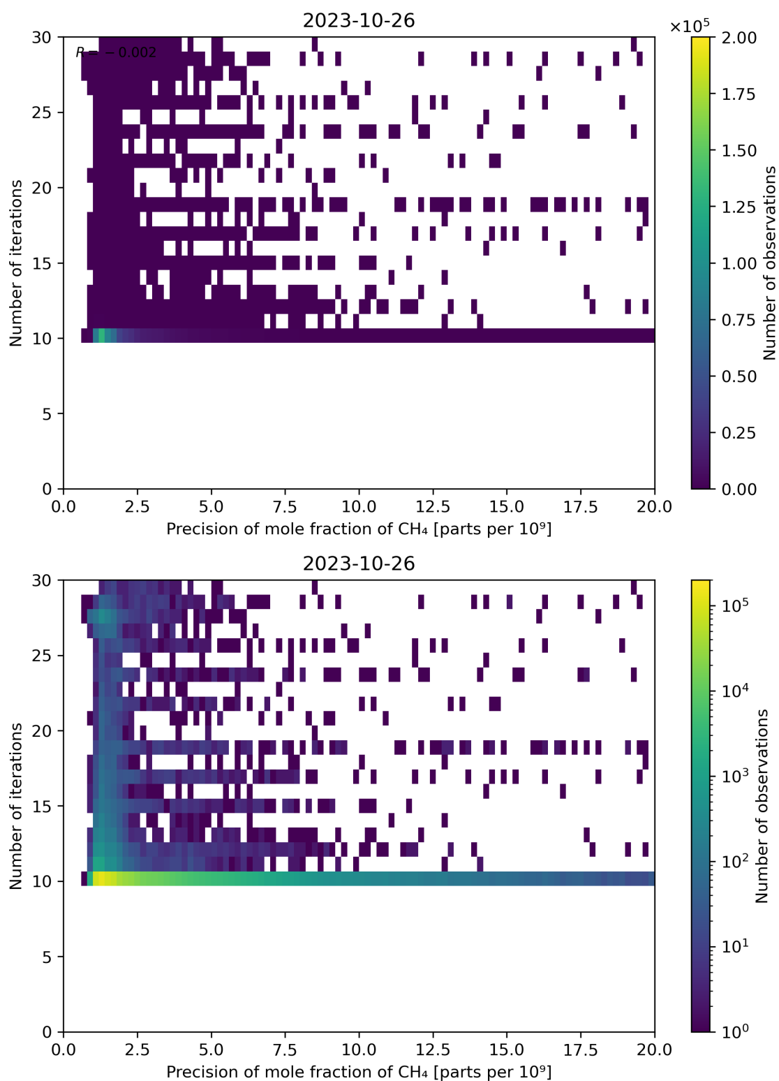
Figure 83: Scatter density plot of “Precision of mole fraction of CH 4 ” against “Number of iterations” for 2023-10-25 to 2023-10-27.
