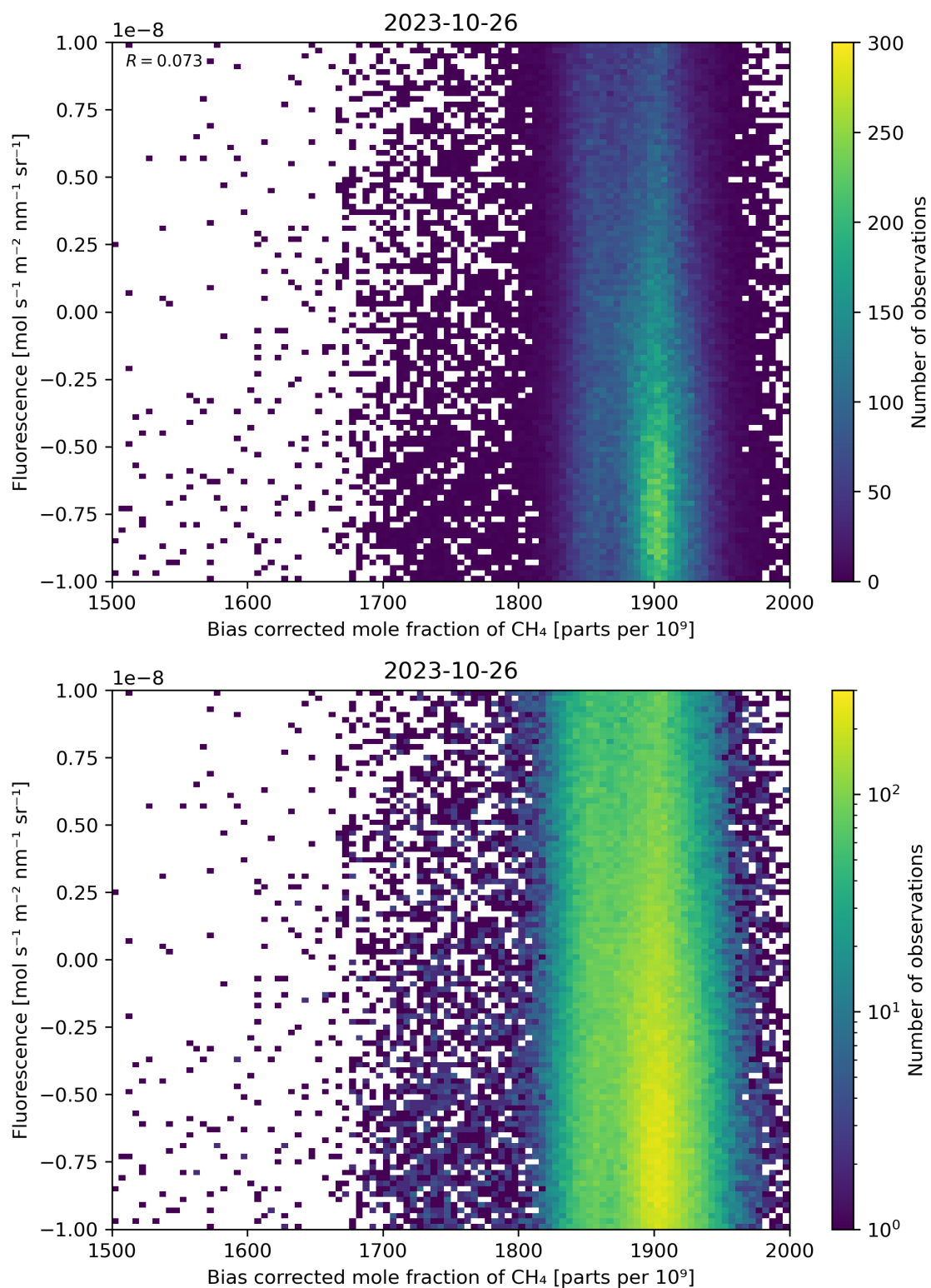
Figure 66: Scatter density plot of “Bias corrected mole fraction of \text{CH}_4 ” against “Fluorescence” for 2023-10-25 to 2023-10-27.
