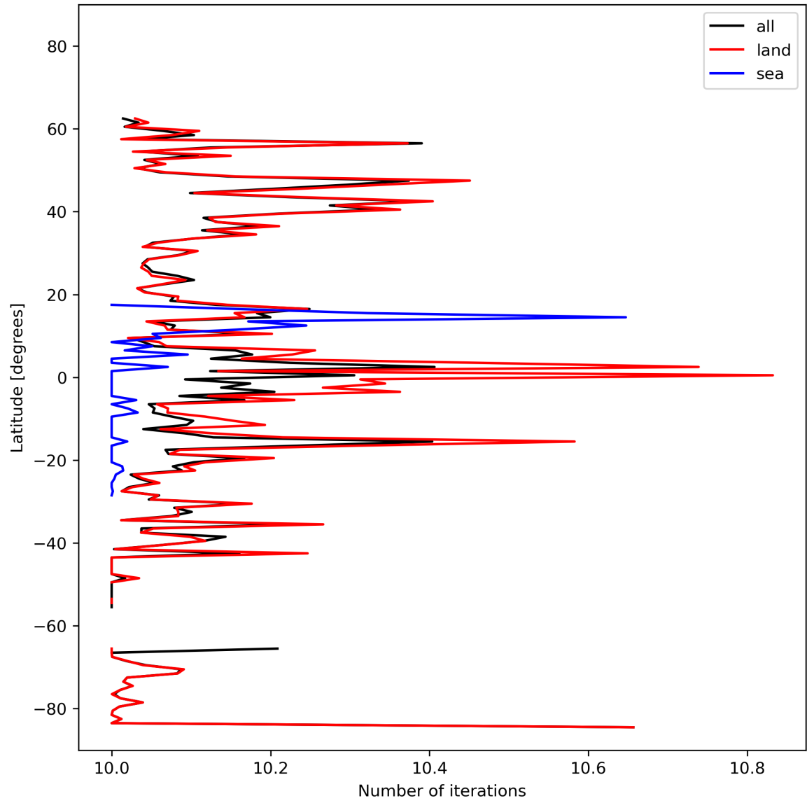
Figure 20: Zonal average of “Number of iterations” for 2023-10-25 to 2023-10-27.
