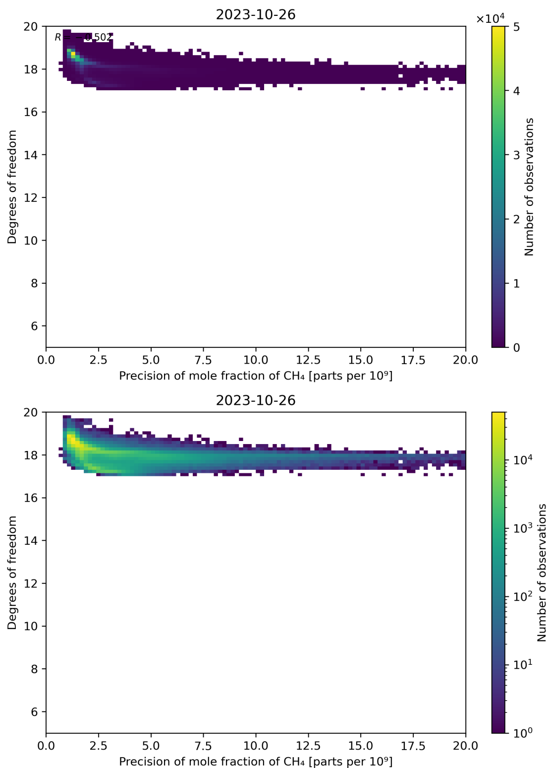
Figure 80: Scatter density plot of “Precision of mole fraction of CH 4 ” against “Degrees of freedom” for 2023-10-25 to 2023-10-27.
