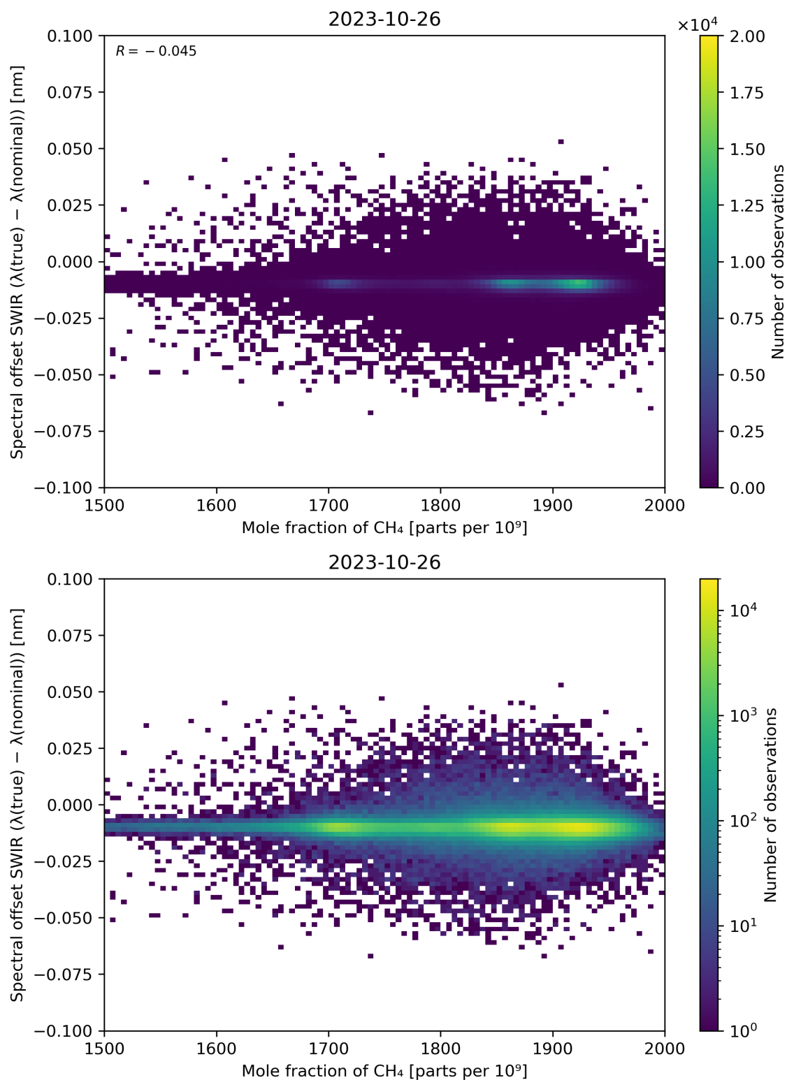
Figure 86: Scatter density plot of “Mole fraction of CH 4 ” against “Spectral offset SWIR ( \lambda(\text{true}) - \lambda(\text{nominal}) )” for 2023-10-25 to 2023-10-27.
