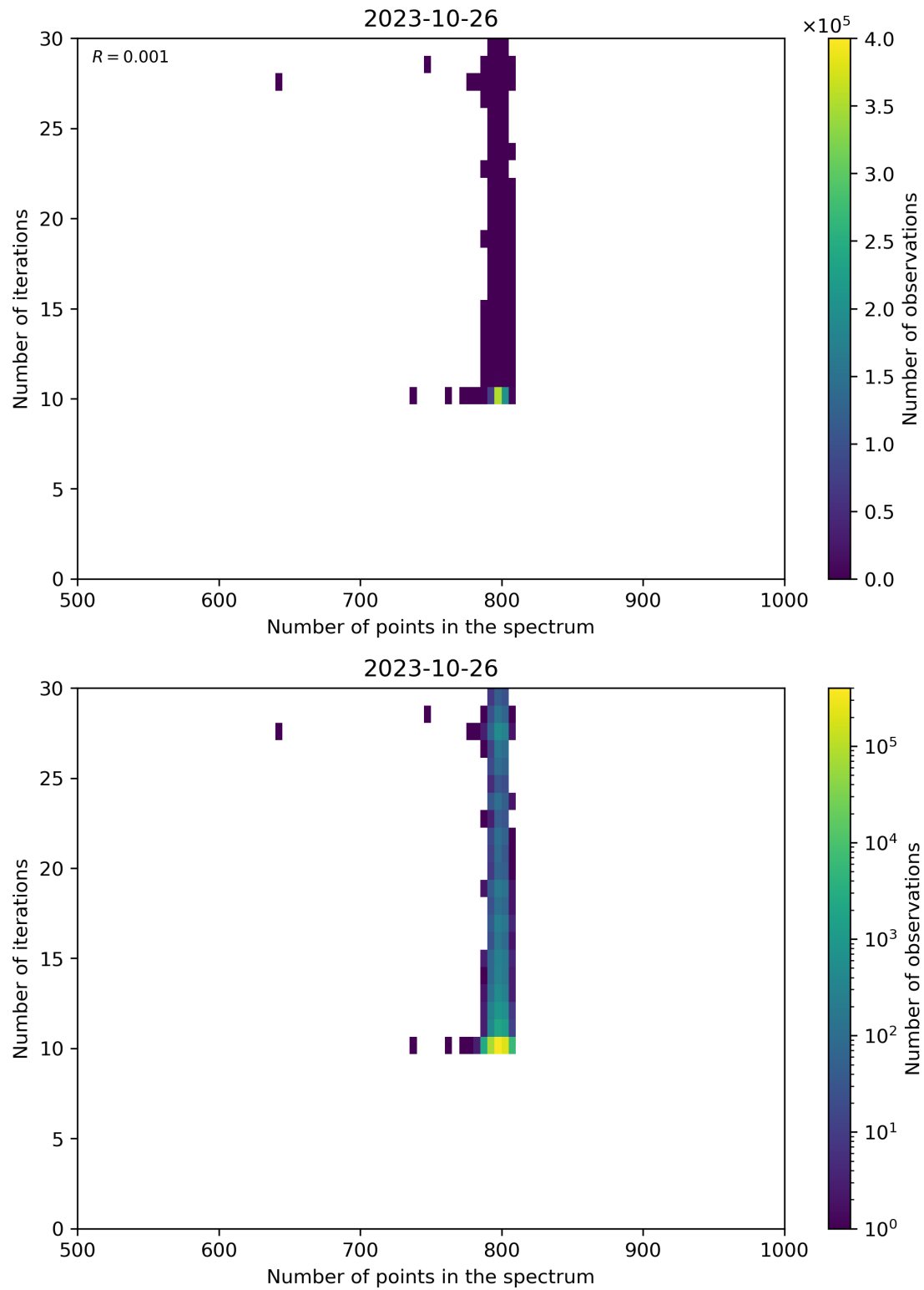
Figure 92: Scatter density plot of “Number of points in the spectrum” against “Number of iterations” for 2023-10-25 to 2023-10-27.
