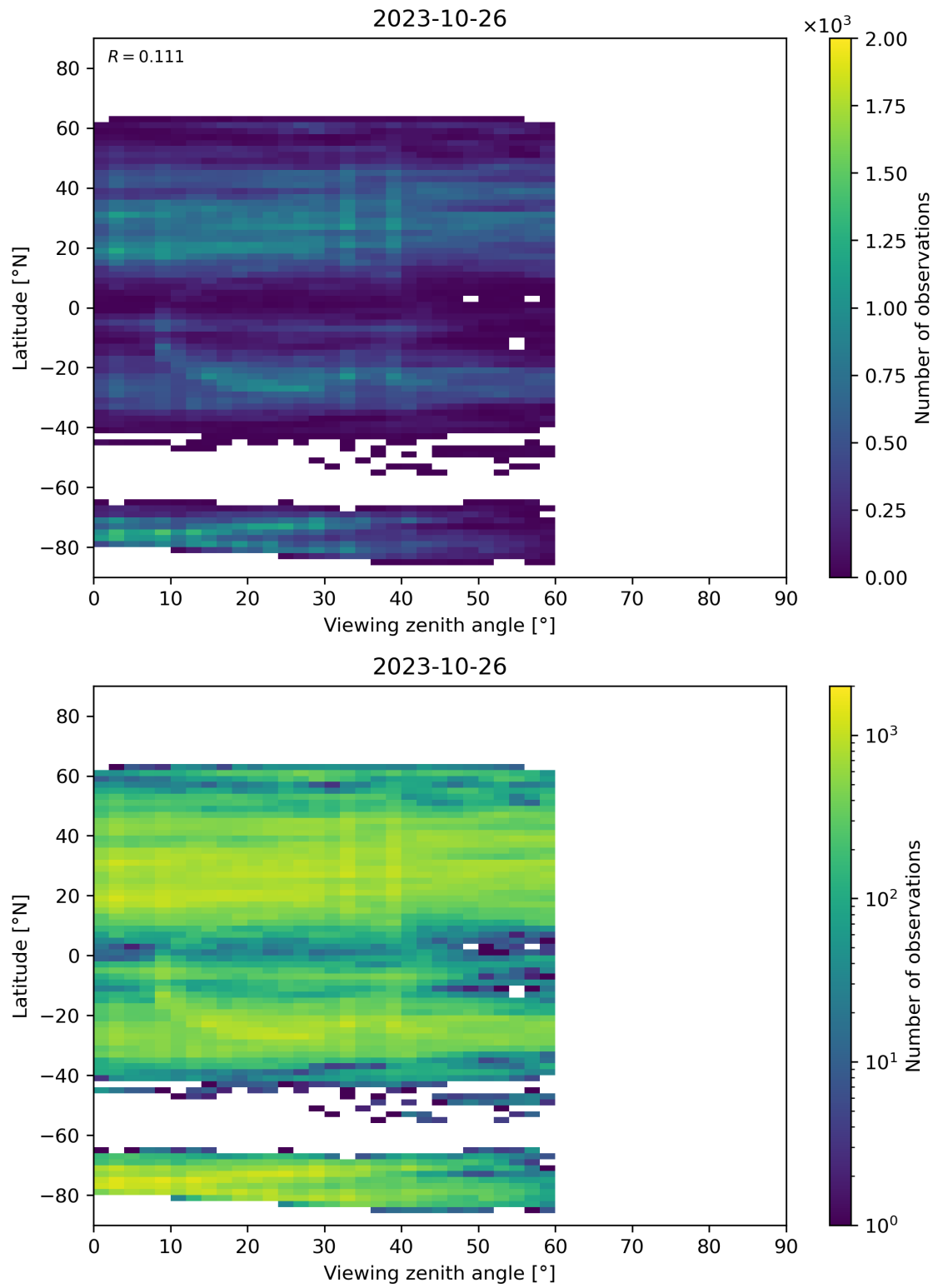
Figure 109: Scatter density plot of “Viewing zenith angle” against “Latitude” for 2023-10-25 to 2023-10-27.
