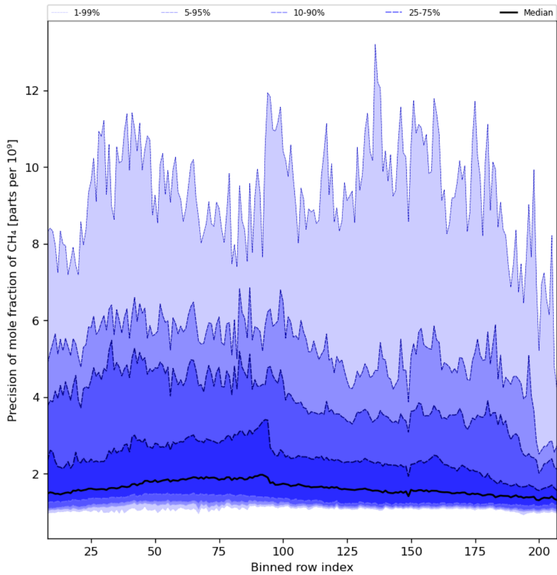
Figure 35: Along track statistics of “Precision of mole fraction of CH 4 ” for 2023-10-25 to 2023-10-27
