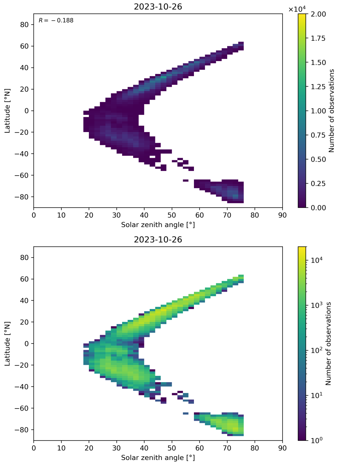
Figure 98: Scatter density plot of “Solar zenith angle” against “Latitude” for 2023-10-25 to 2023-10-27.
