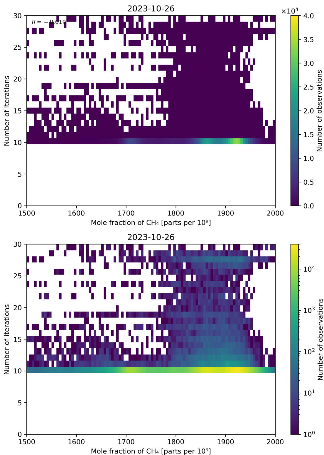
Figure 76: Scatter density plot of “Mole fraction of CH 4 ” against “Number of iterations” for 2023-10-25 to 2023-10-27.
