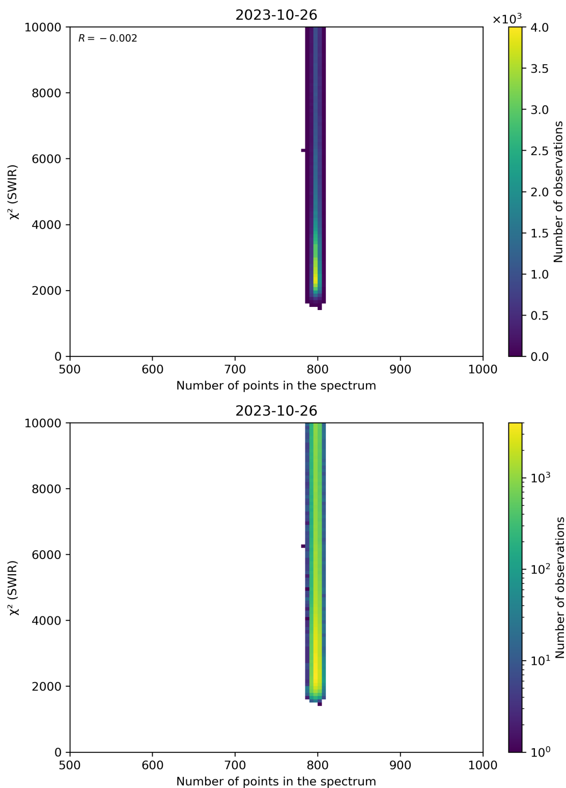
Figure 89: Scatter density plot of “Number of points in the spectrum” against “ \chi^2 (SWIR)” for 2023-10-25 to 2023-10-27.
