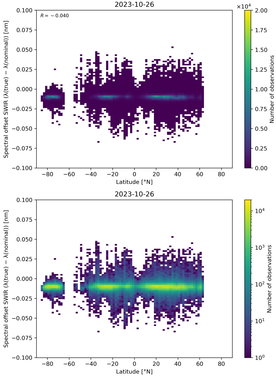
Figure 62: Scatter density plot of “Latitude” against “Spectral offset SWIR ( \lambda(\text{true}) - \lambda(\text{nominal}) )” for 2023-10-25 to 2023-10-27.
