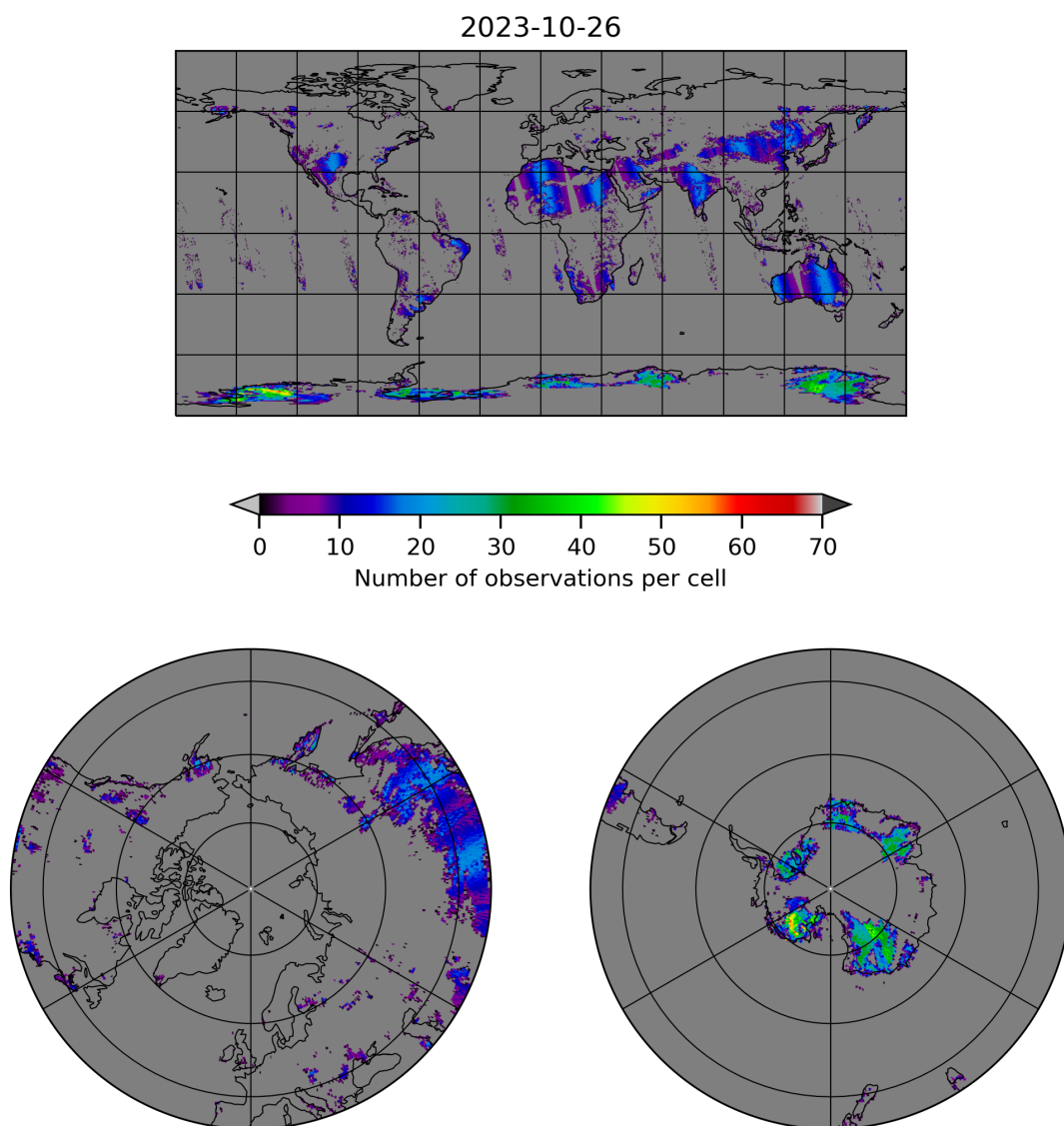
Figure 10: Map of the number of observations for 2023-10-25 to 2023-10-27
