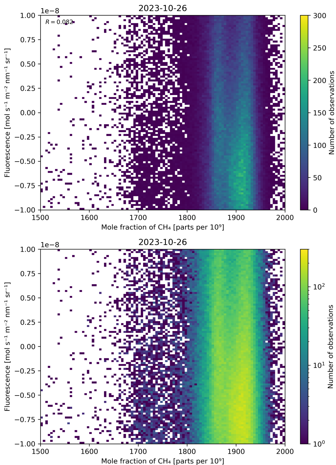
Figure 73: Scatter density plot of “Mole fraction of \text{CH}_4 ” against “Fluorescence” for 2023-10-25 to 2023-10-27.
