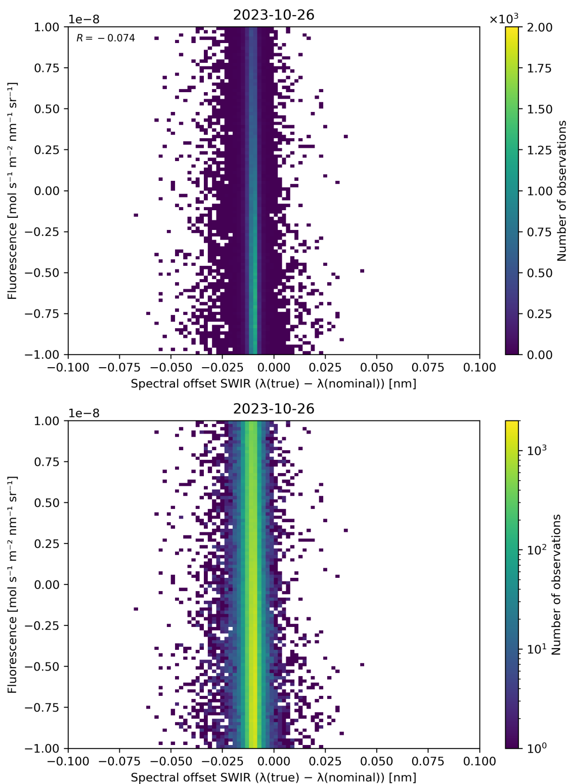
Figure 120: Scatter density plot of “Spectral offset SWIR ( \lambda(\text{true}) - \lambda(\text{nominal}) )” against “Fluorescence” for 2023-10-25 to 2023-10-27.
