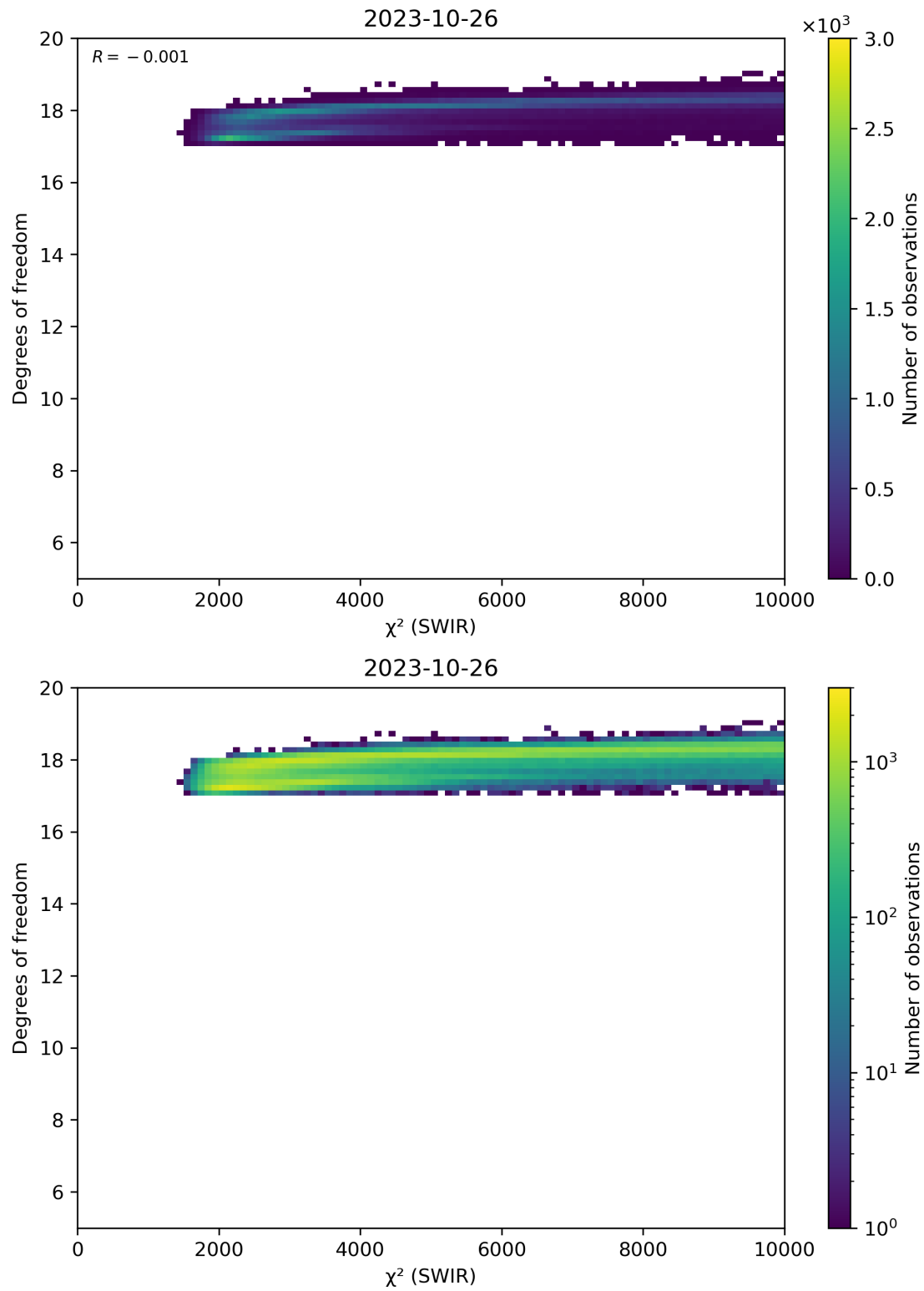
Figure 48: Scatter density plot of “ \chi^2 (SWIR)” against “Degrees of freedom” for 2023-10-25 to 2023-10-27.
