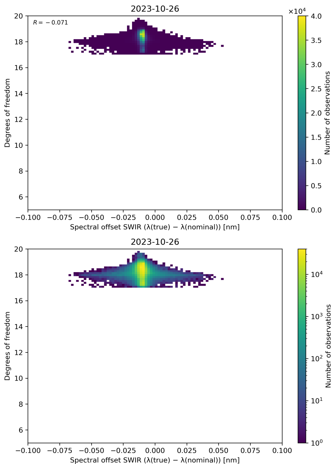
Figure 119: Scatter density plot of “Spectral offset SWIR ( \lambda(\text{true}) - \lambda(\text{nominal}) )” against “Degrees of freedom” for 2023-10-25 to 2023-10-27.
