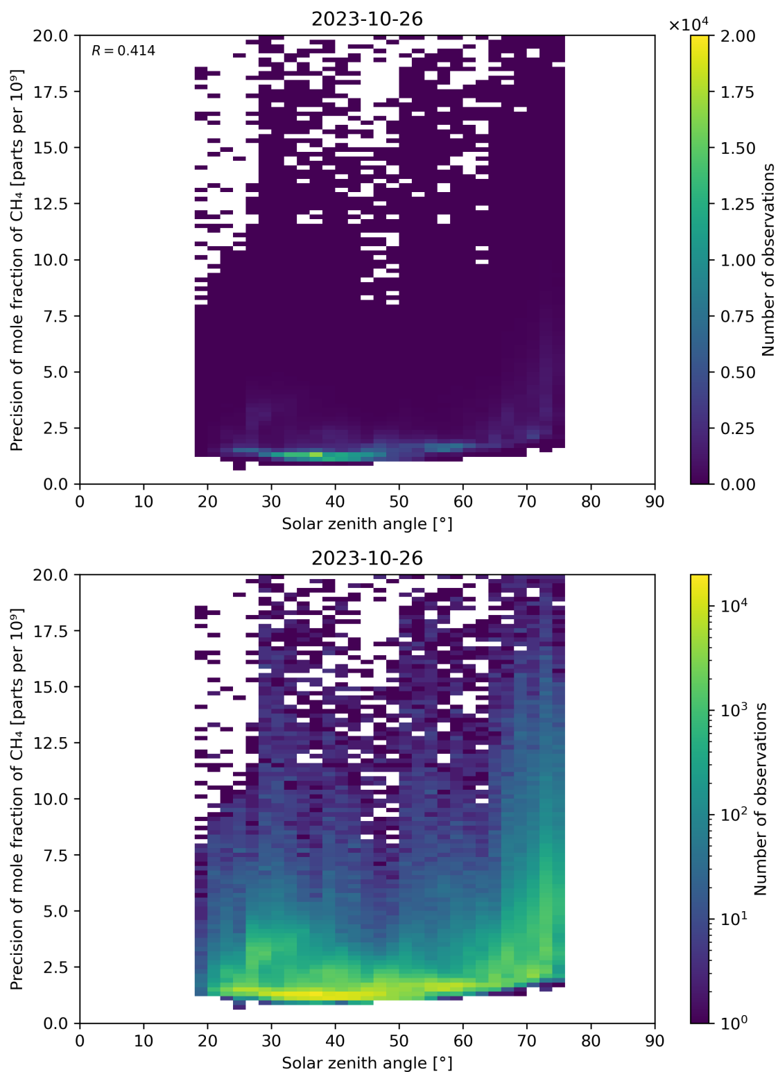
Figure 101: Scatter density plot of “Solar zenith angle” against “Precision of mole fraction of CH 4 ” for 2023-10-25 to 2023-10-27.
