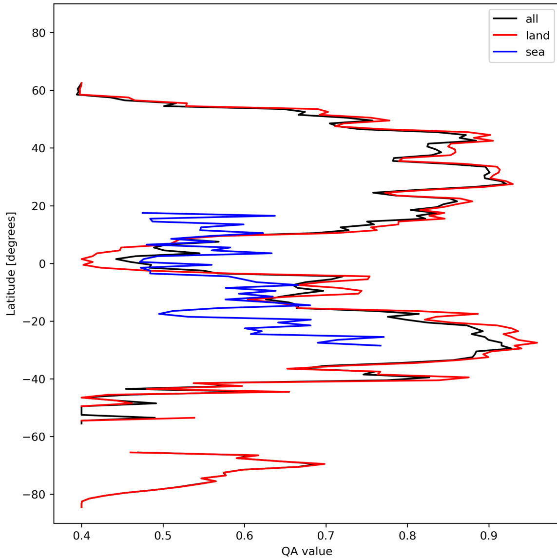
Figure 11: Zonal average of “QA value” for 2023-10-25 to 2023-10-27.
