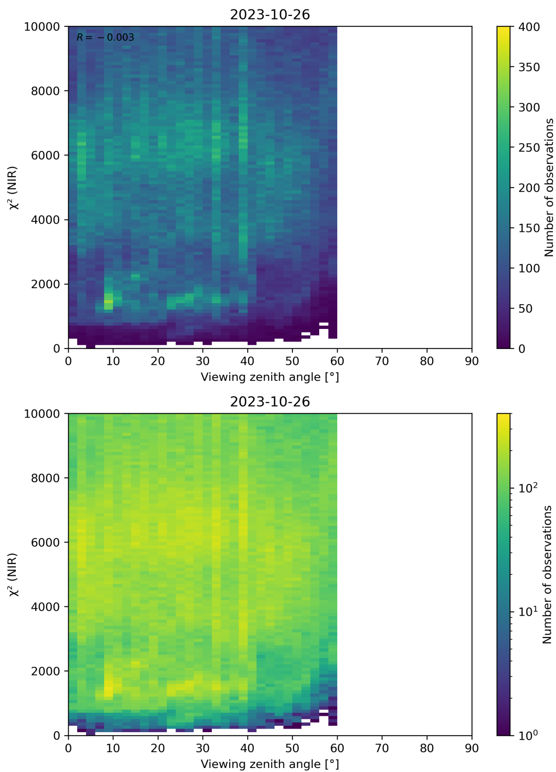
Figure 105: Scatter density plot of “Viewing zenith angle” against “ \chi^2 (NIR)” for 2023-10-25 to 2023-10-27.
