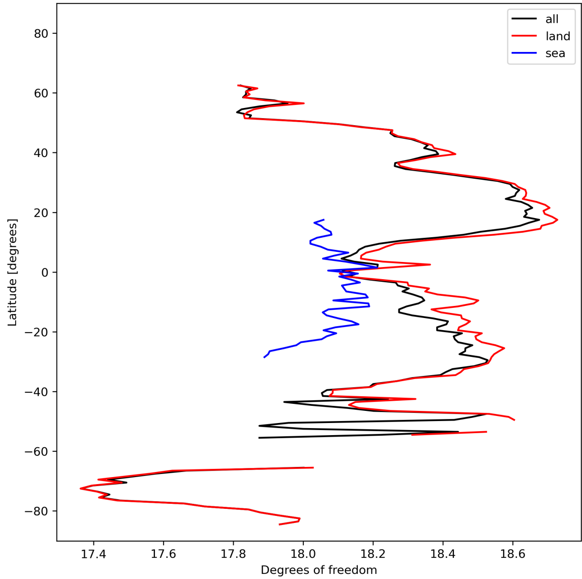
Figure 19: Zonal average of “Degrees of freedom” for 2023-10-25 to 2023-10-27.
