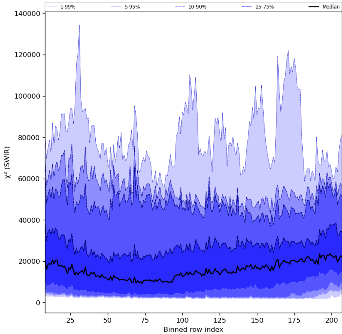
Figure 39: Along track statistics of " \chi^2 (SWIR)" for 2023-10-25 to 2023-10-27
