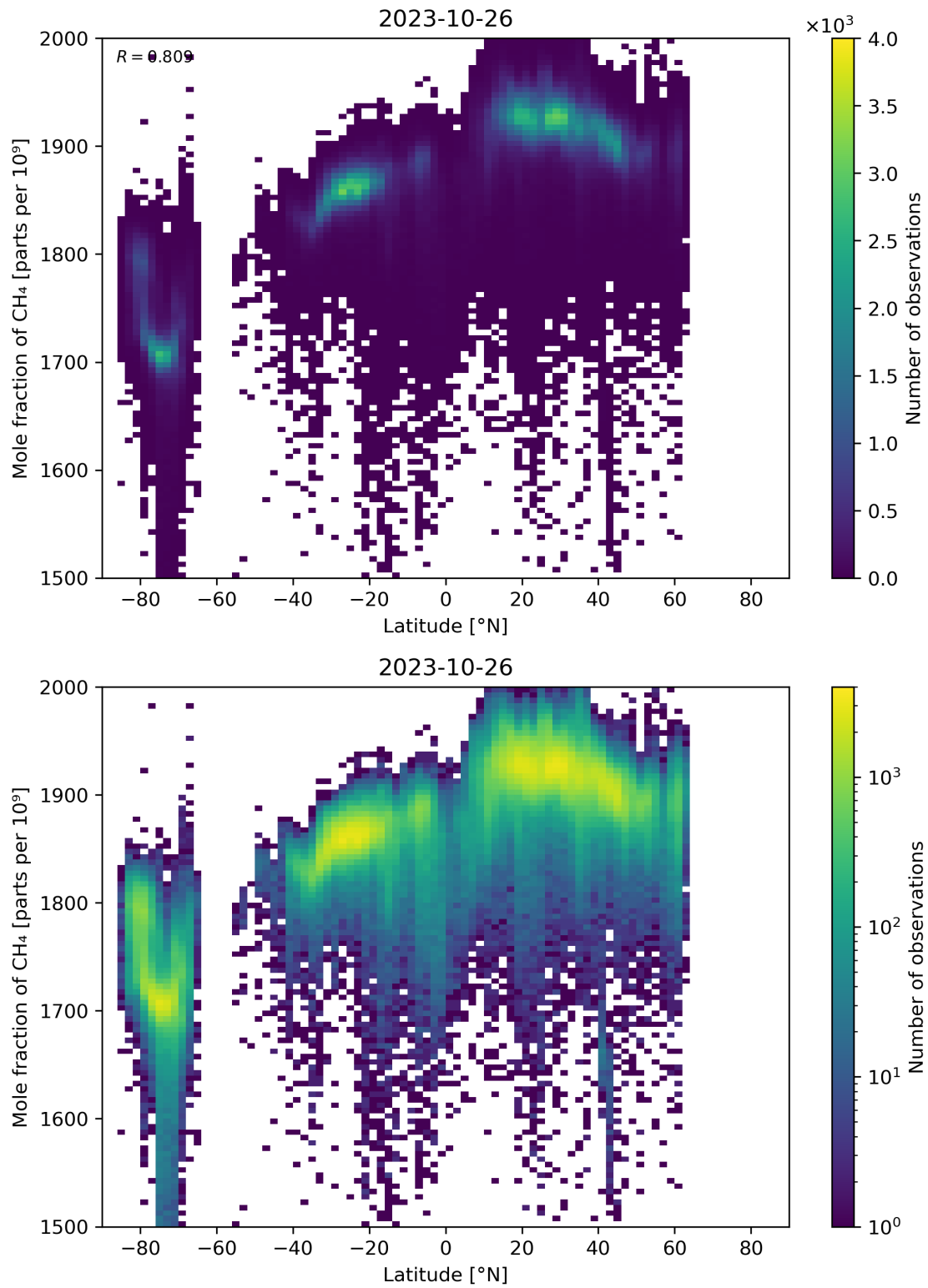
Figure 57: Scatter density plot of “Latitude” against “Mole fraction of CH 4 ” for 2023-10-25 to 2023-10-27.
