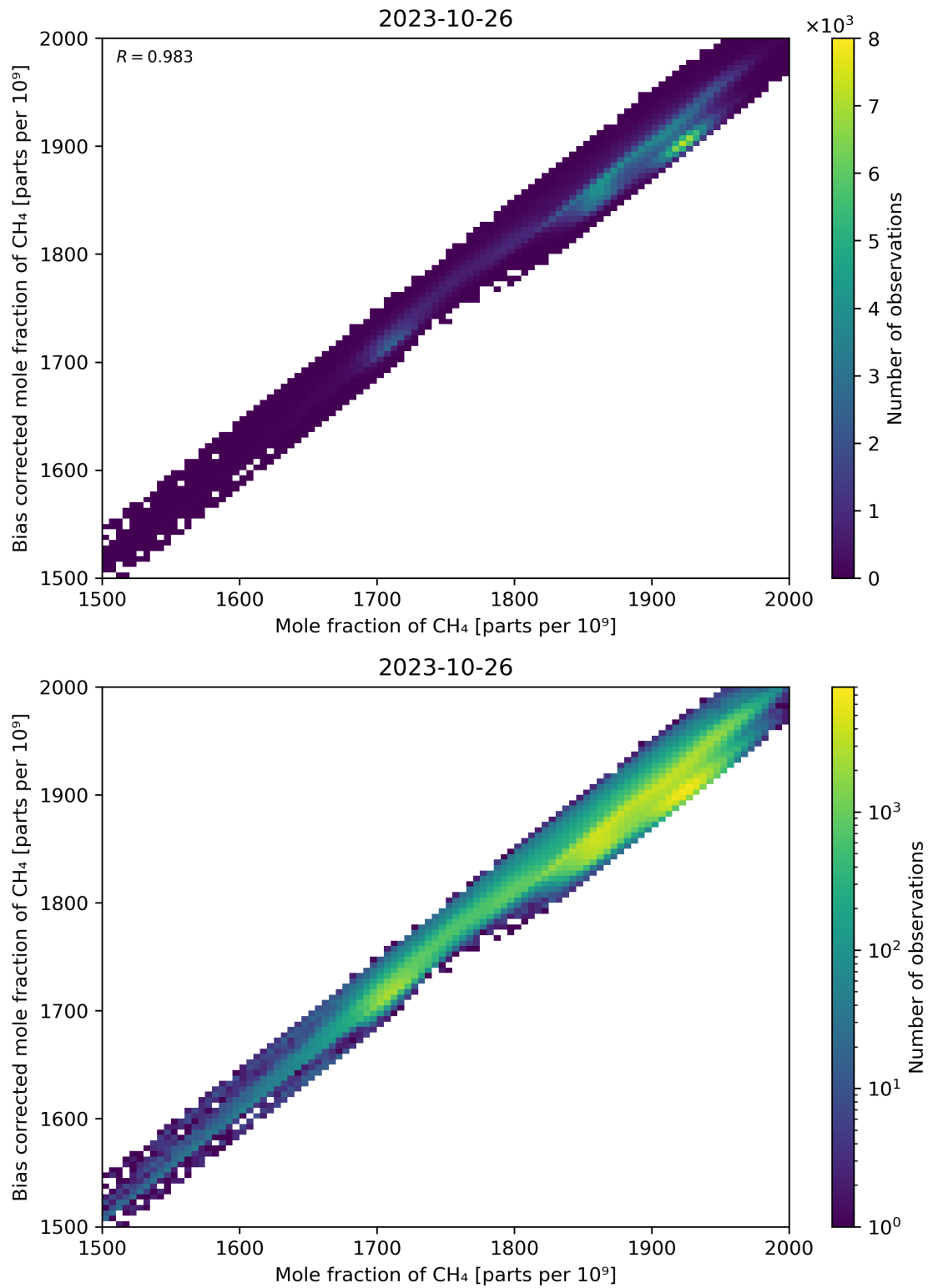
Figure 74: Scatter density plot of “Mole fraction of CH 4 ” against “Bias corrected mole fraction of CH 4 ” for 2023-10-25 to 2023-10-27.
