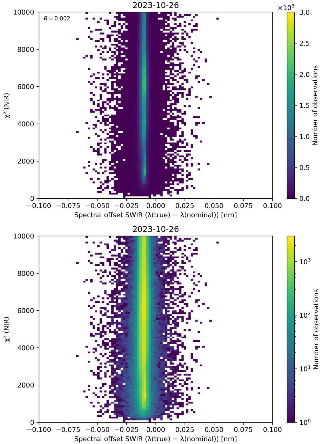
Figure 117: Scatter density plot of “Spectral offset SWIR ( \lambda(\text{true}) - \lambda(\text{nominal}) )” against “ \chi^2 (NIR)” for 2023-10-25 to 2023-10-27.
