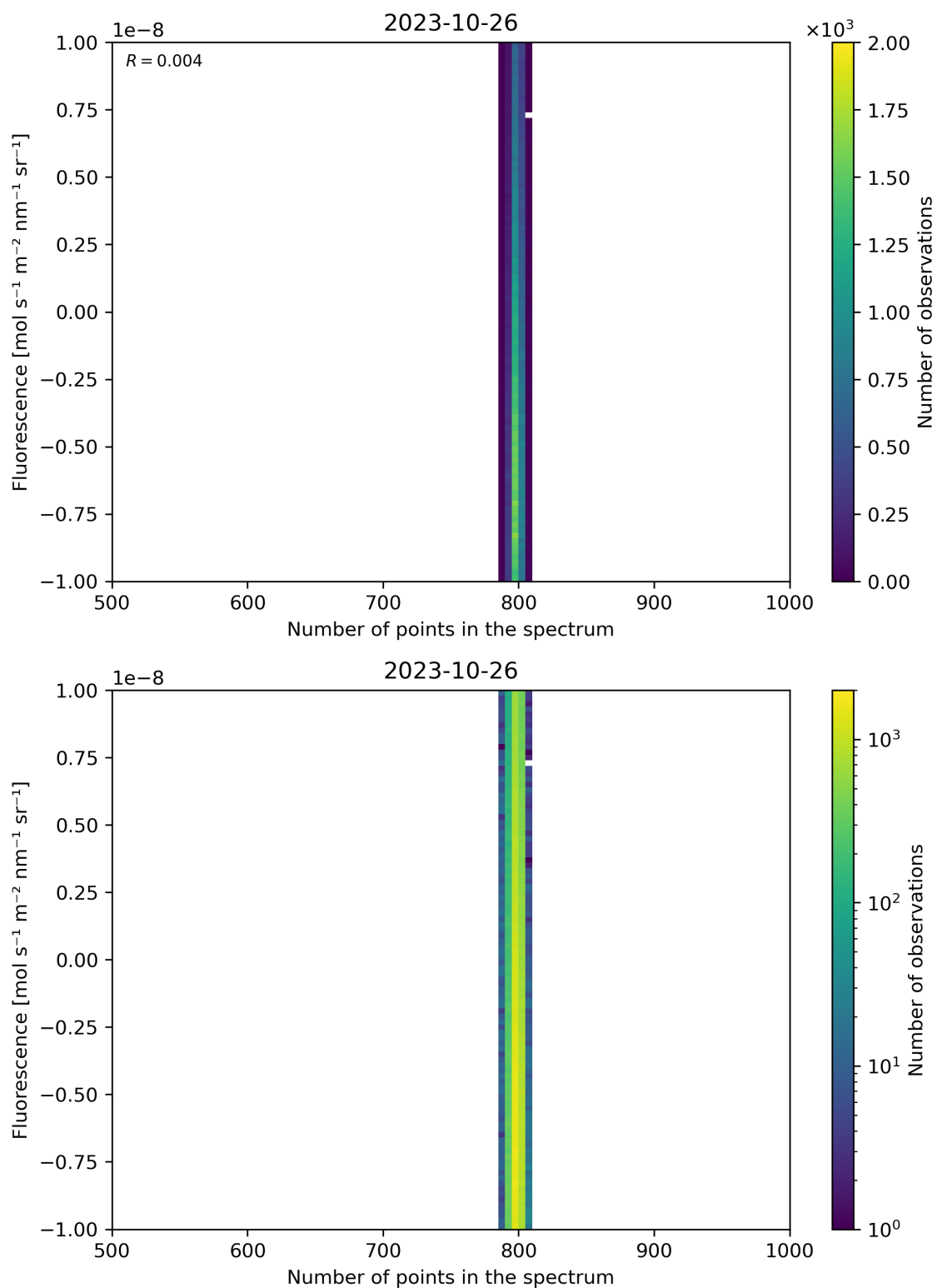
Figure 91: Scatter density plot of “Number of points in the spectrum” against “Fluorescence” for 2023-10-25 to 2023-10-27.
