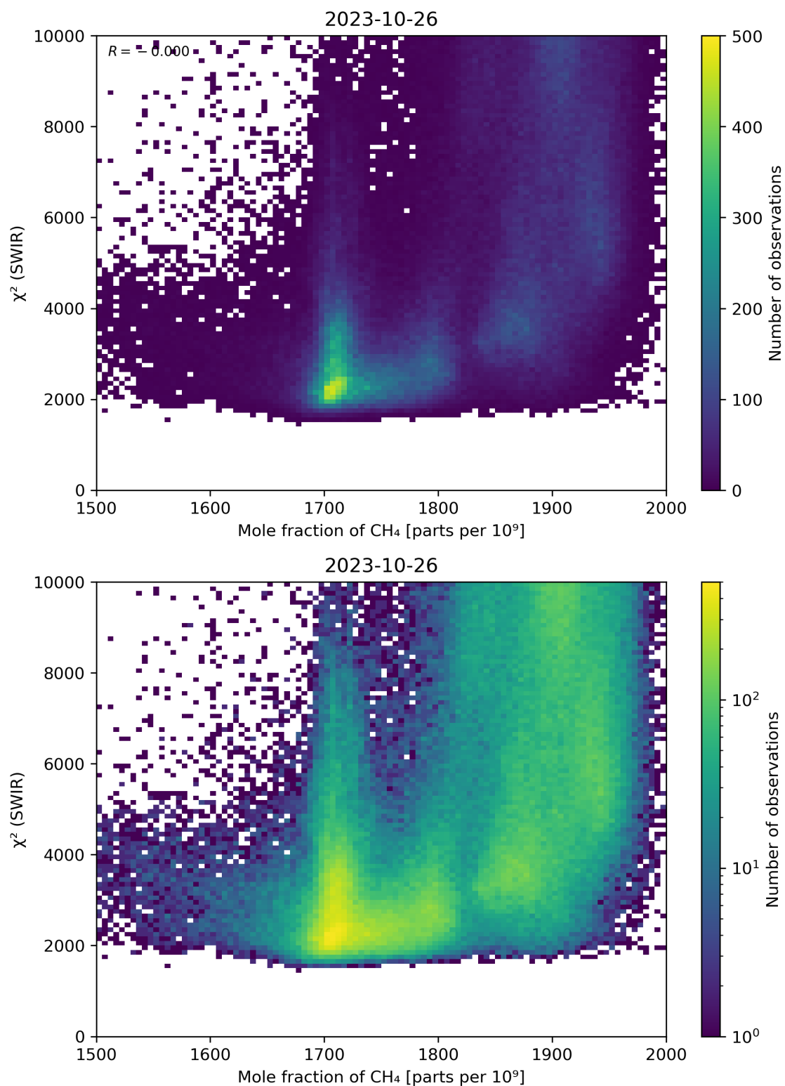
Figure 71: Scatter density plot of “Mole fraction of CH 4 ” against “ \chi^2 (SWIR)” for 2023-10-25 to 2023-10-27.
