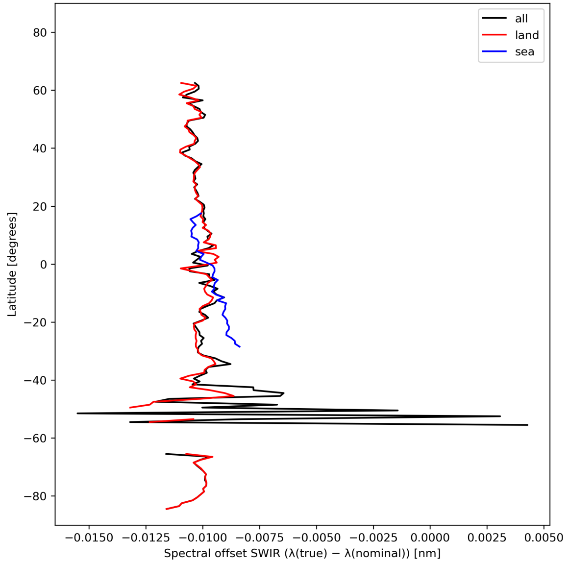
Figure 16: Zonal average of “Spectral offset SWIR ( \lambda(\text{true}) - \lambda(\text{nominal}) )” for 2023-10-25 to 2023-10-27.
