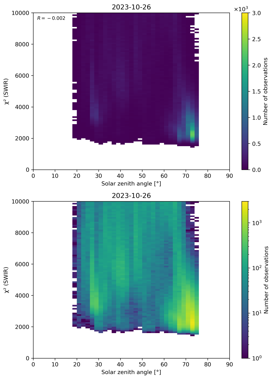
Figure 95: Scatter density plot of “Solar zenith angle” against “ \chi^2 (SWIR)” for 2023-10-25 to 2023-10-27.
