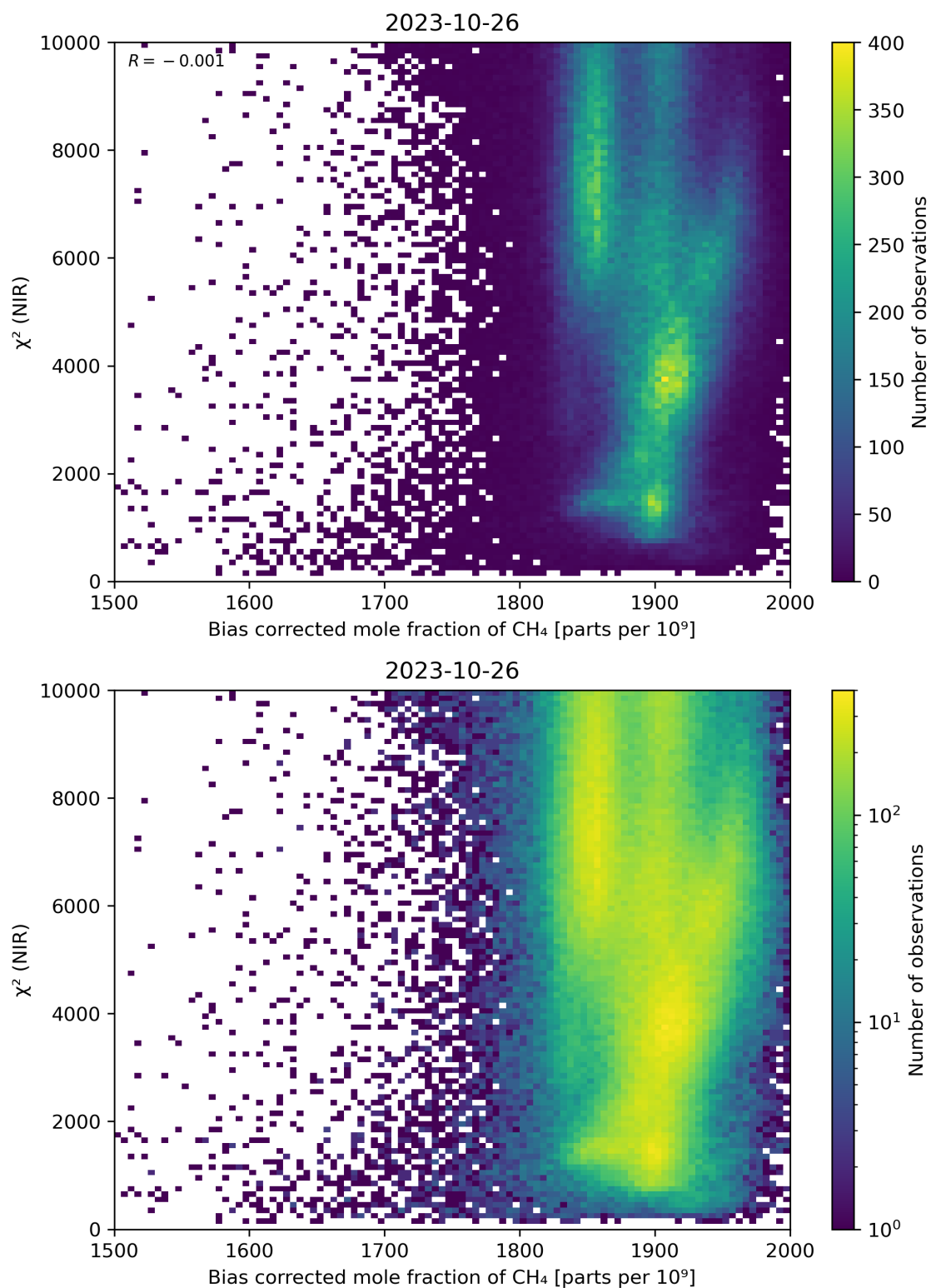
Figure 63: Scatter density plot of “Bias corrected mole fraction of CH 4 ” against “ \chi^2 (NIR)” for 2023-10-25 to 2023-10-27.
