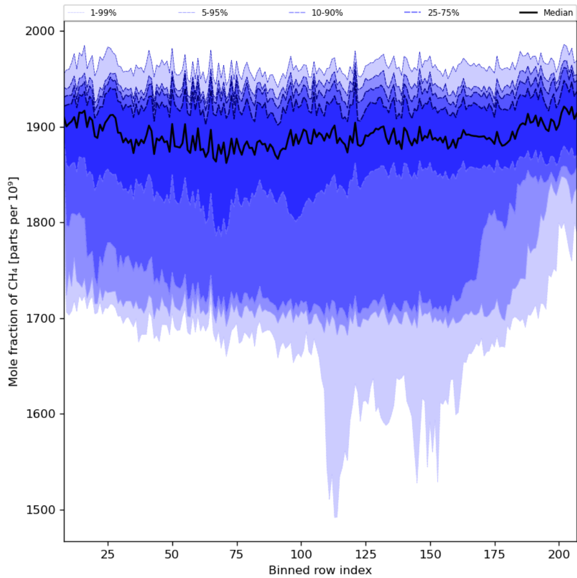
Figure 34: Along track statistics of “Mole fraction of CH 4 ” for 2023-10-25 to 2023-10-27
