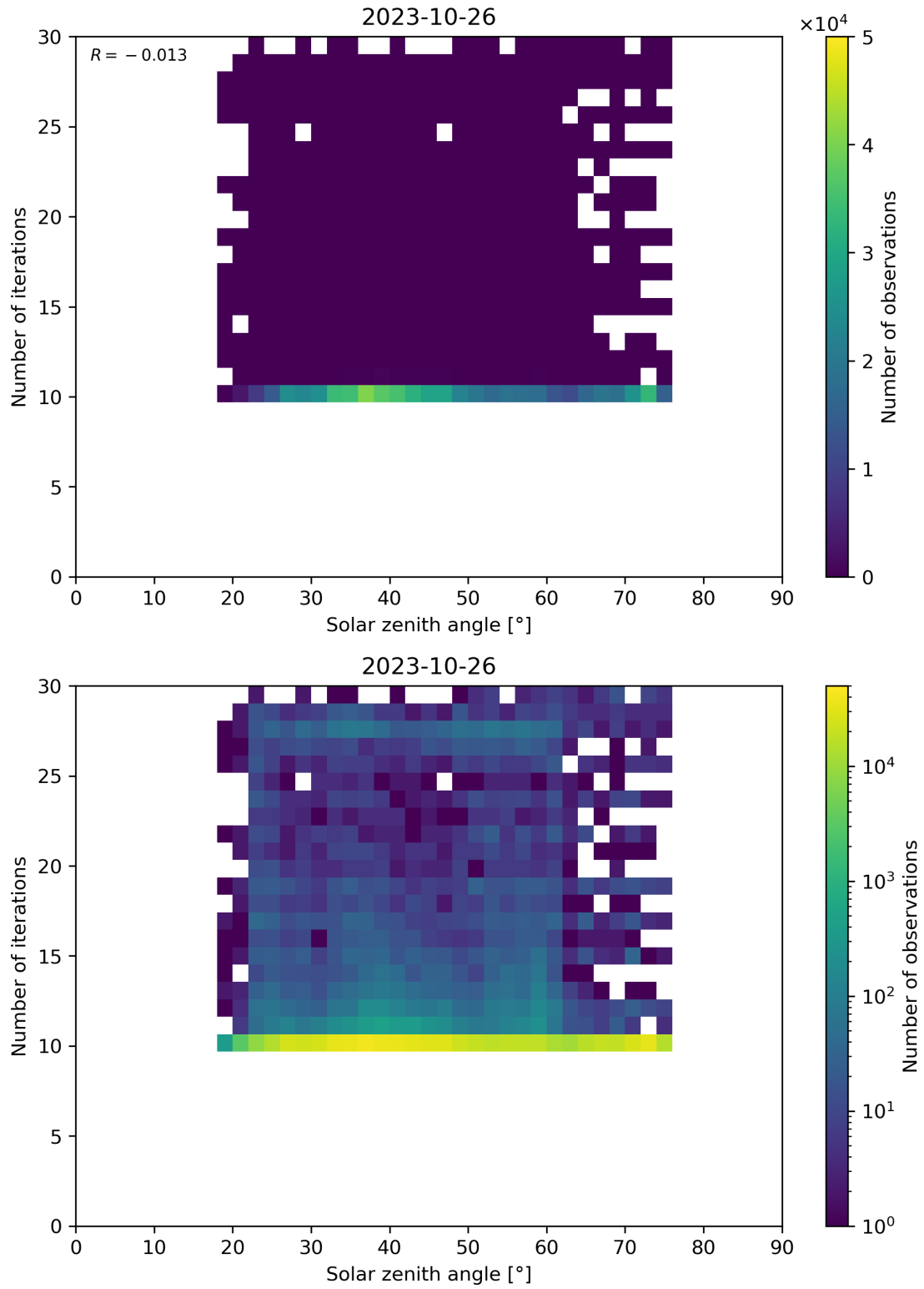
Figure 102: Scatter density plot of “Solar zenith angle” against “Number of iterations” for 2023-10-25 to 2023-10-27.
