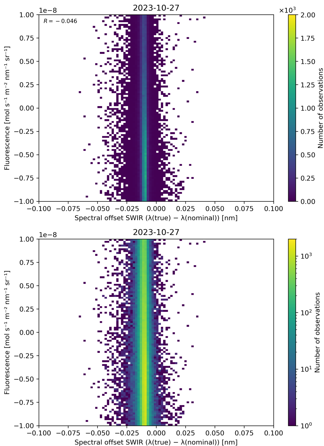
Figure 120: Scatter density plot of “Spectral offset SWIR ( \lambda(\text{true}) - \lambda(\text{nominal}) )” against “Fluorescence” for 2023-10-27 to 2023-10-28.
