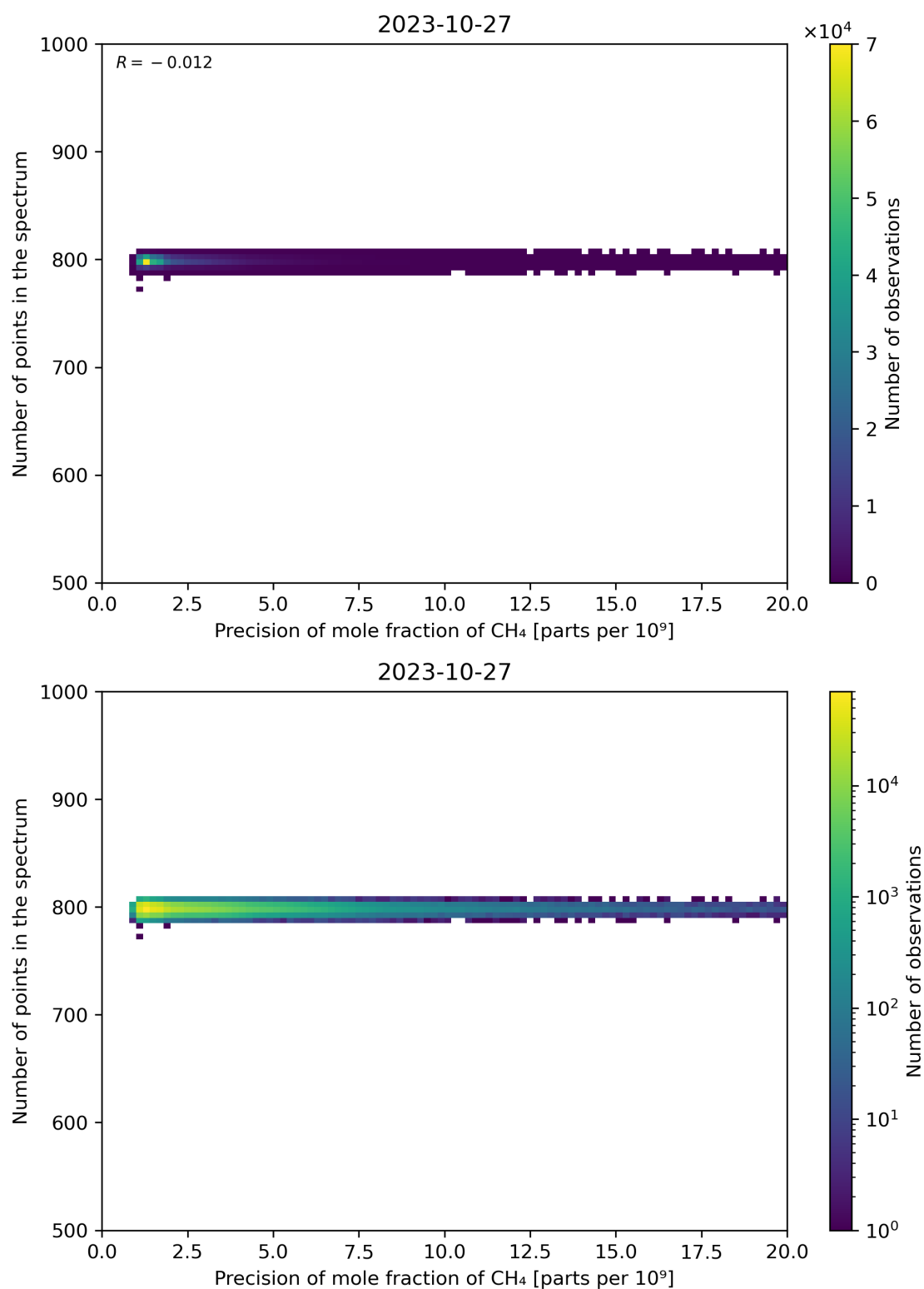
Figure 84: Scatter density plot of “Precision of mole fraction of CH 4 ” against “Number of points in the spectrum” for 2023-10-27 to 2023-10-28.
