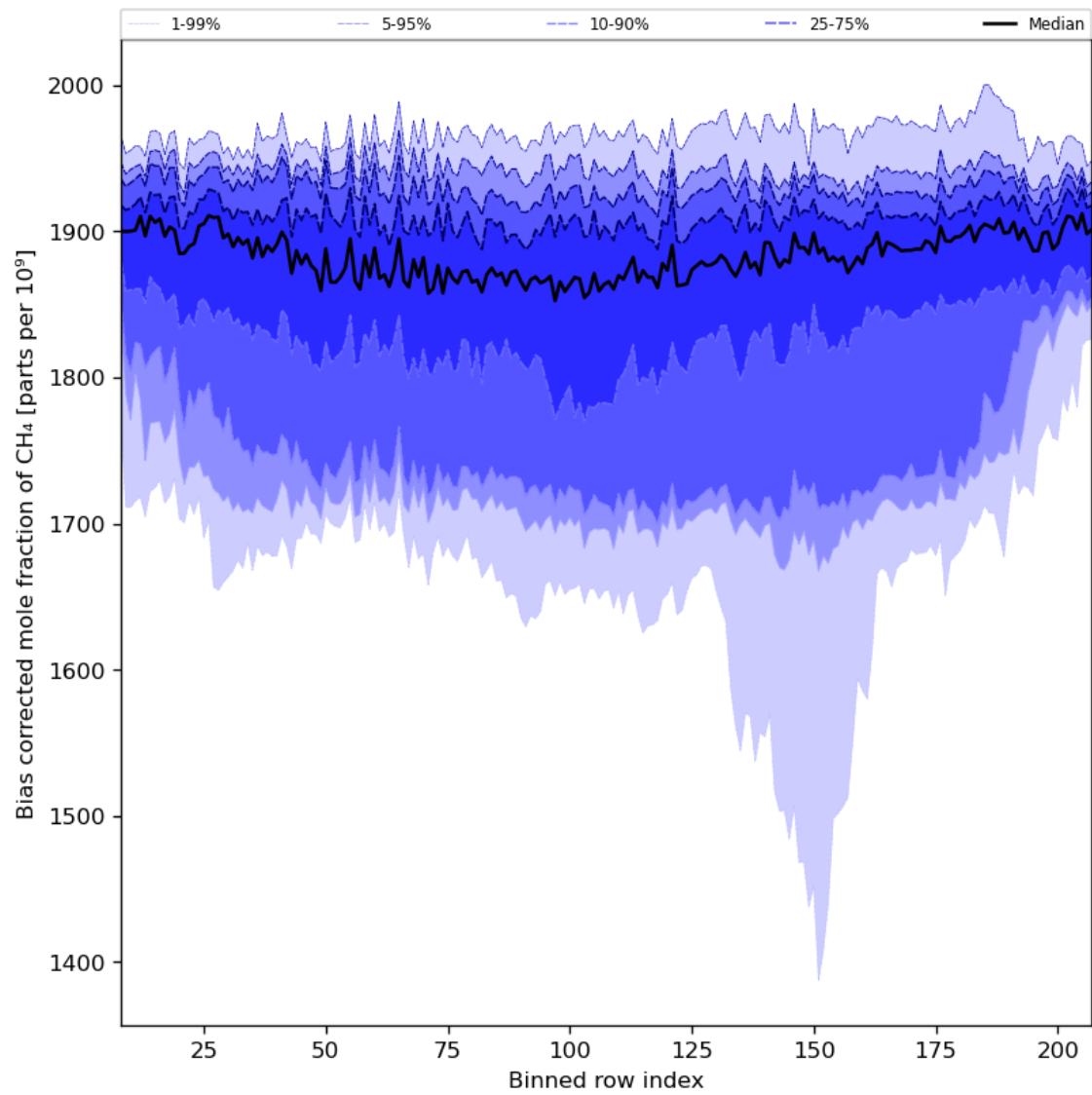
Figure 36: Along track statistics of “Bias corrected mole fraction of CH 4 ” for 2023-10-27 to 2023-10-28
