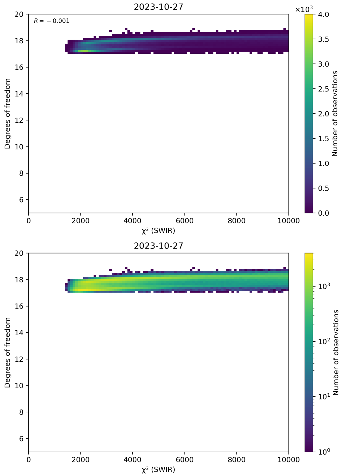
Figure 48: Scatter density plot of “ \chi^2 (SWIR)” against “Degrees of freedom” for 2023-10-27 to 2023-10-28.
