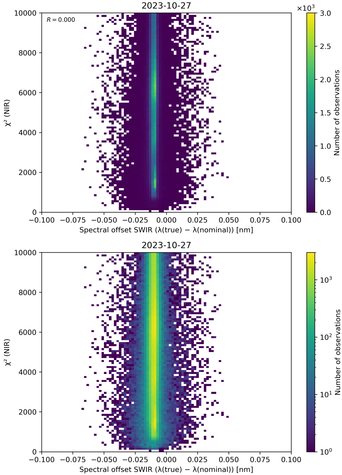
Figure 117: Scatter density plot of “Spectral offset SWIR ( \lambda(\text{true}) - \lambda(\text{nominal}) )” against “ \chi^2 (NIR)” for 2023-10-27 to 2023-10-28.
