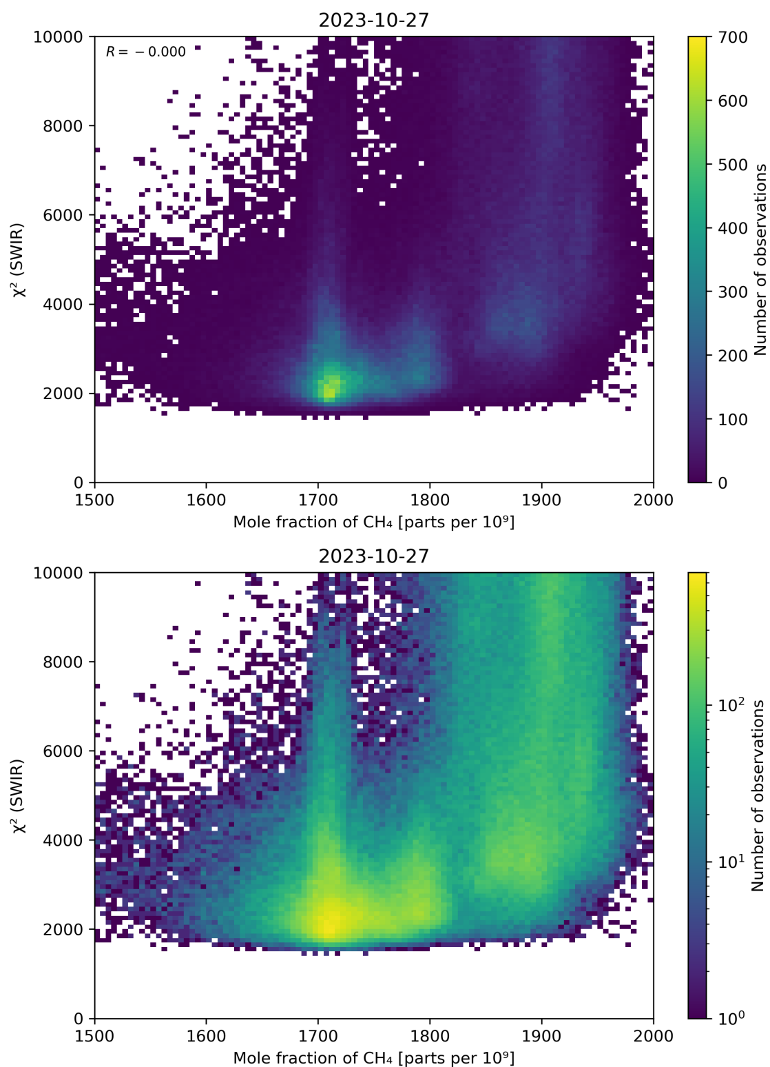
Figure 71: Scatter density plot of “Mole fraction of \text{CH}_4 ” against “ \chi^2 (SWIR)” for 2023-10-27 to 2023-10-28.
