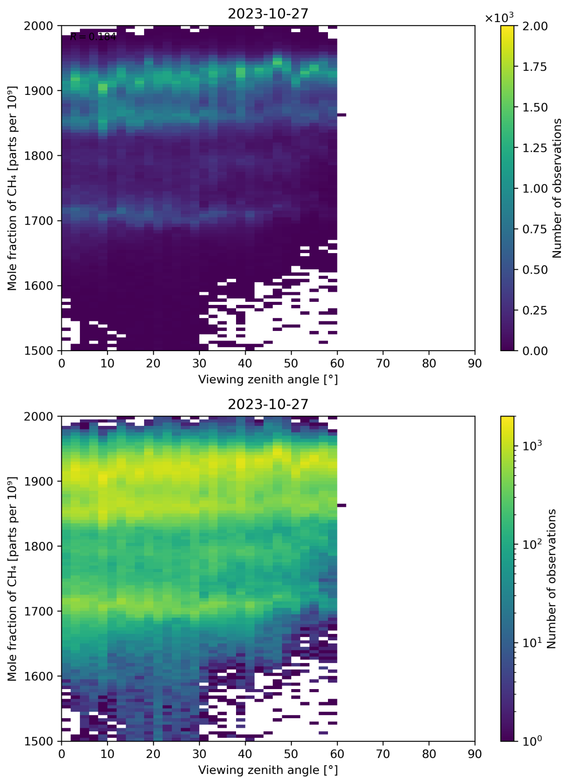
Figure 110: Scatter density plot of “Viewing zenith angle” against “Mole fraction of CH 4 ” for 2023-10-27 to 2023-10-28.
