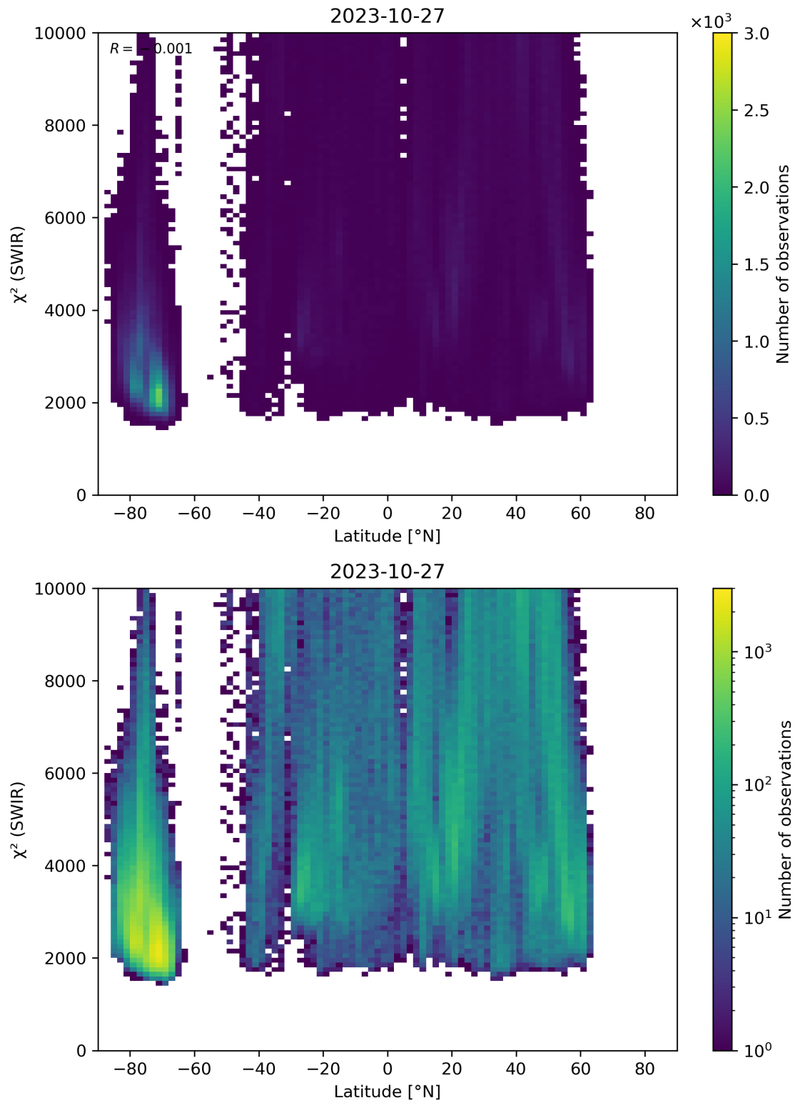
Figure 54: Scatter density plot of “Latitude” against “ \chi^2 (SWIR)” for 2023-10-27 to 2023-10-28.
