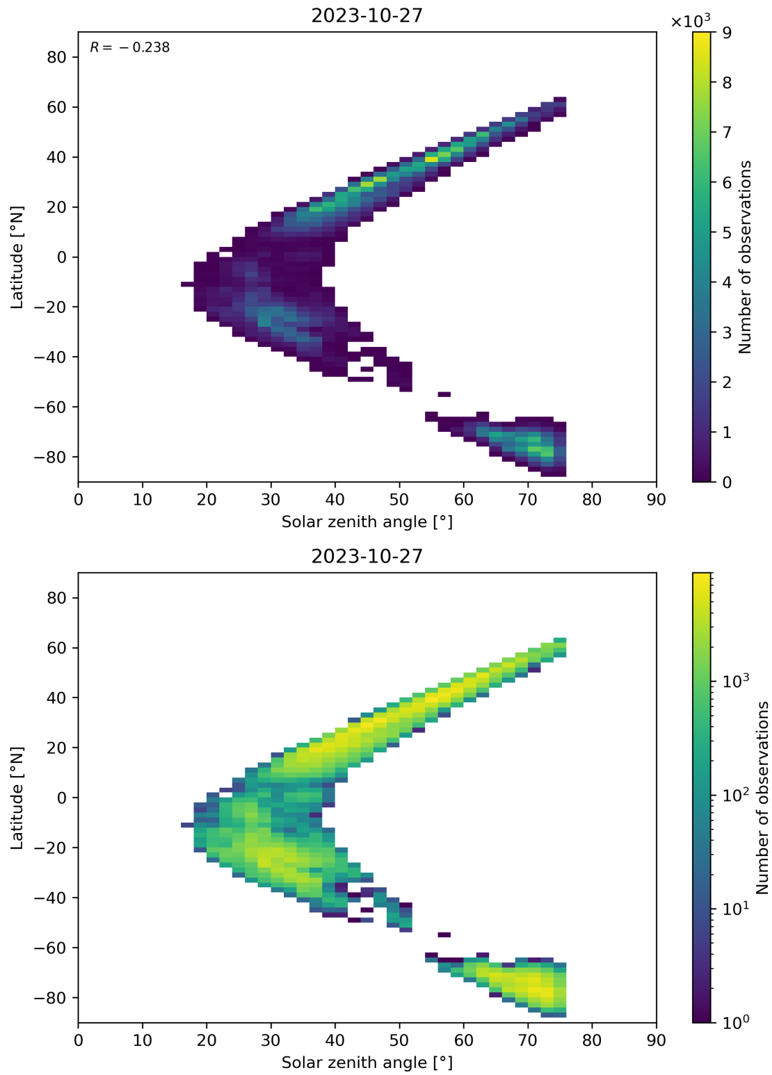
Figure 98: Scatter density plot of “Solar zenith angle” against “Latitude” for 2023-10-27 to 2023-10-28.
