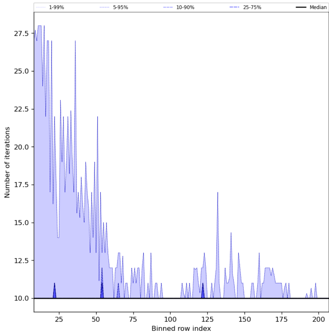
Figure 42: Along track statistics of “Number of iterations” for 2023-10-27 to 2023-10-28
