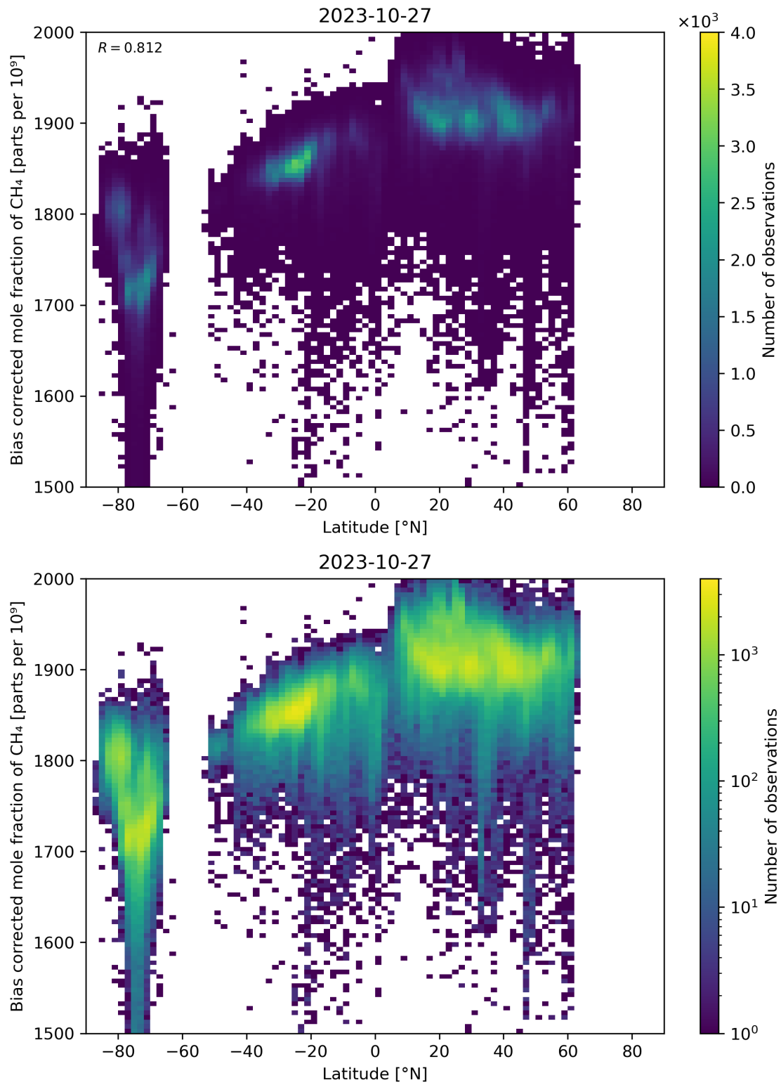
Figure 58: Scatter density plot of “Latitude” against “Bias corrected mole fraction of CH 4 ” for 2023-10-27 to 2023-10-28.
