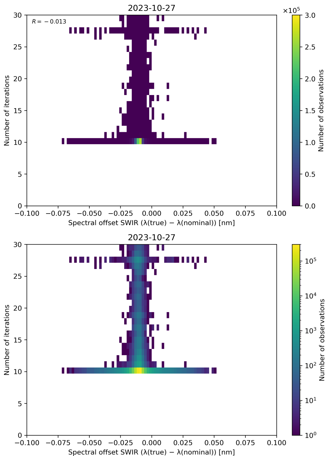
Figure 121: Scatter density plot of “Spectral offset SWIR ( \lambda(\text{true}) - \lambda(\text{nominal}) )” against “Number of iterations” for 2023-10-27 to 2023-10-28.
