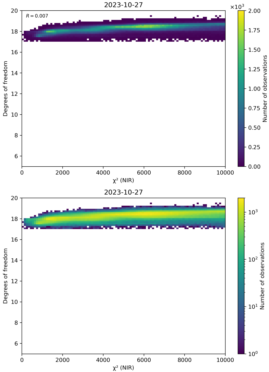
Figure 44: Scatter density plot of “ \chi^2 (NIR)” against “Degrees of freedom” for 2023-10-27 to 2023-10-28.
