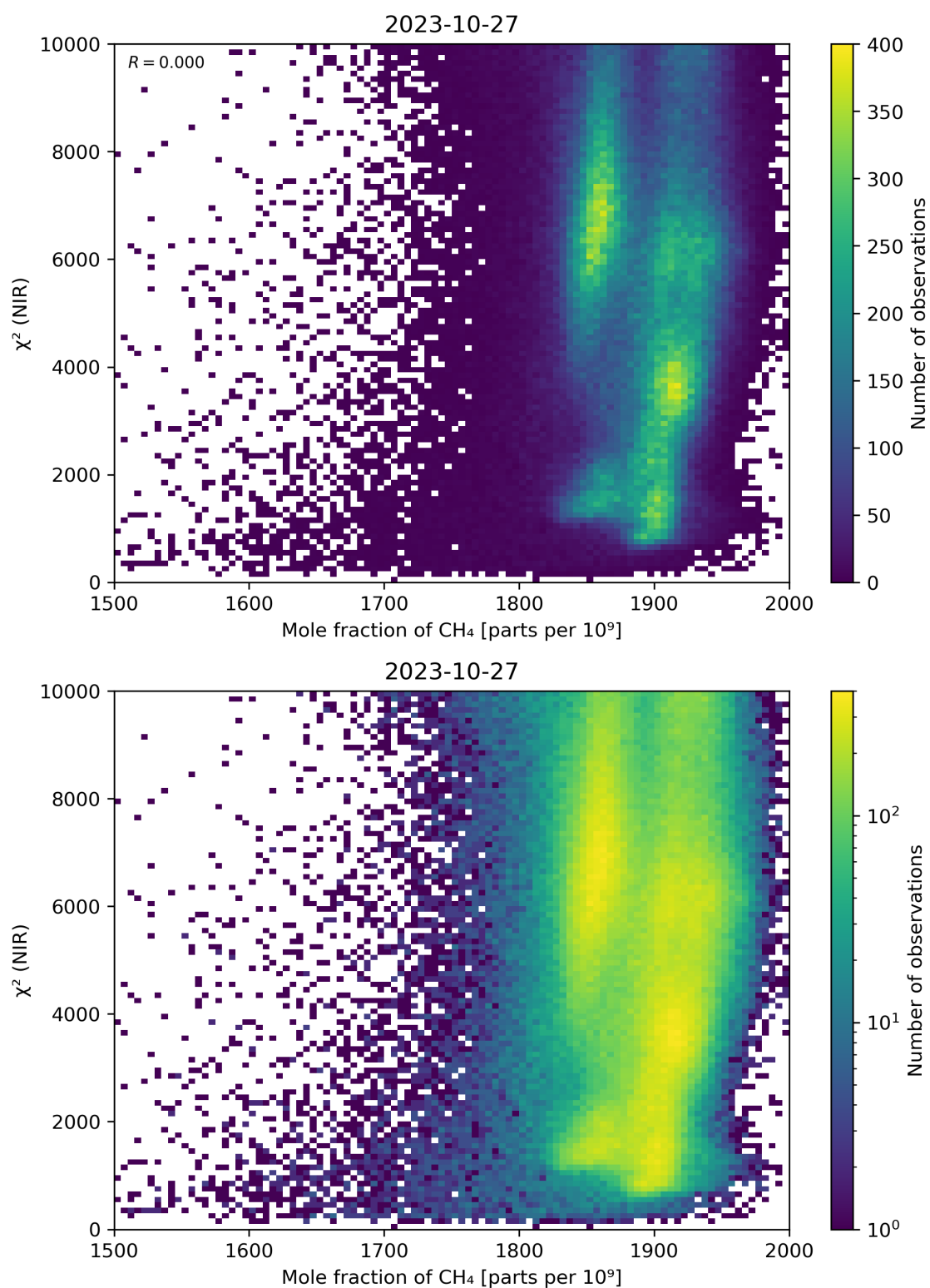
Figure 70: Scatter density plot of “Mole fraction of CH 4 ” against “ \chi^2 (NIR)” for 2023-10-27 to 2023-10-28.
