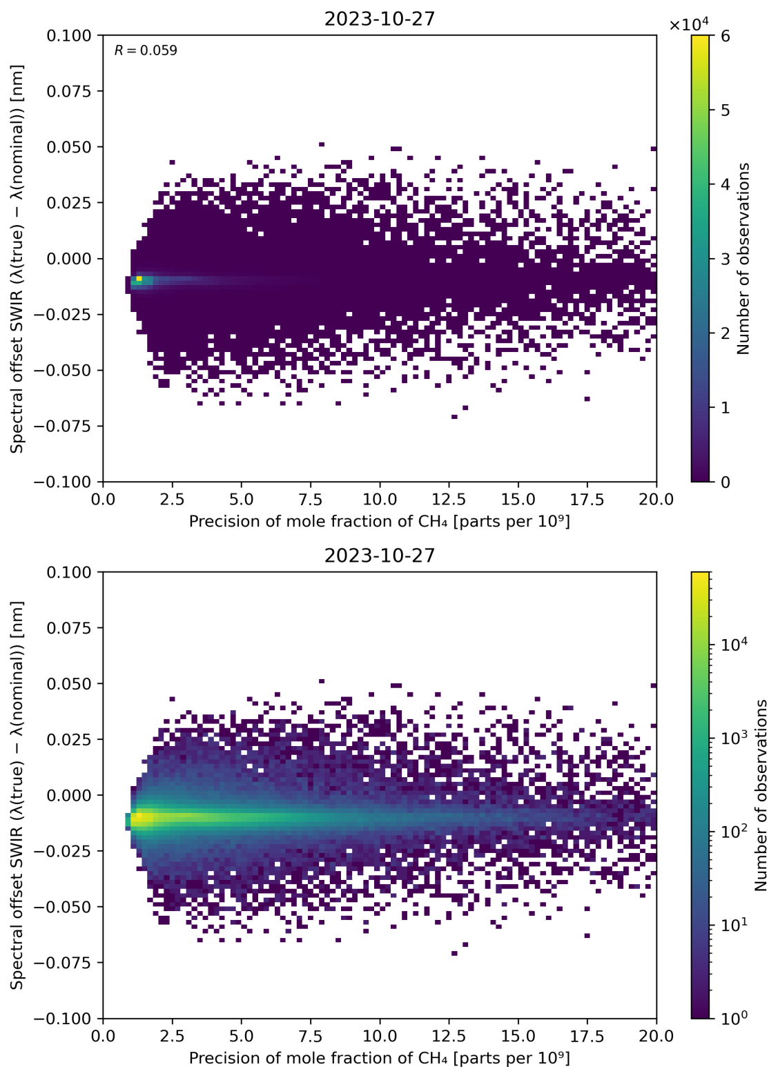
Figure 85: Scatter density plot of “Precision of mole fraction of \text{CH}_4 ” against “Spectral offset SWIR ( \lambda(\text{true}) - \lambda(\text{nominal}) )” for 2023-10-27 to 2023-10-28.
