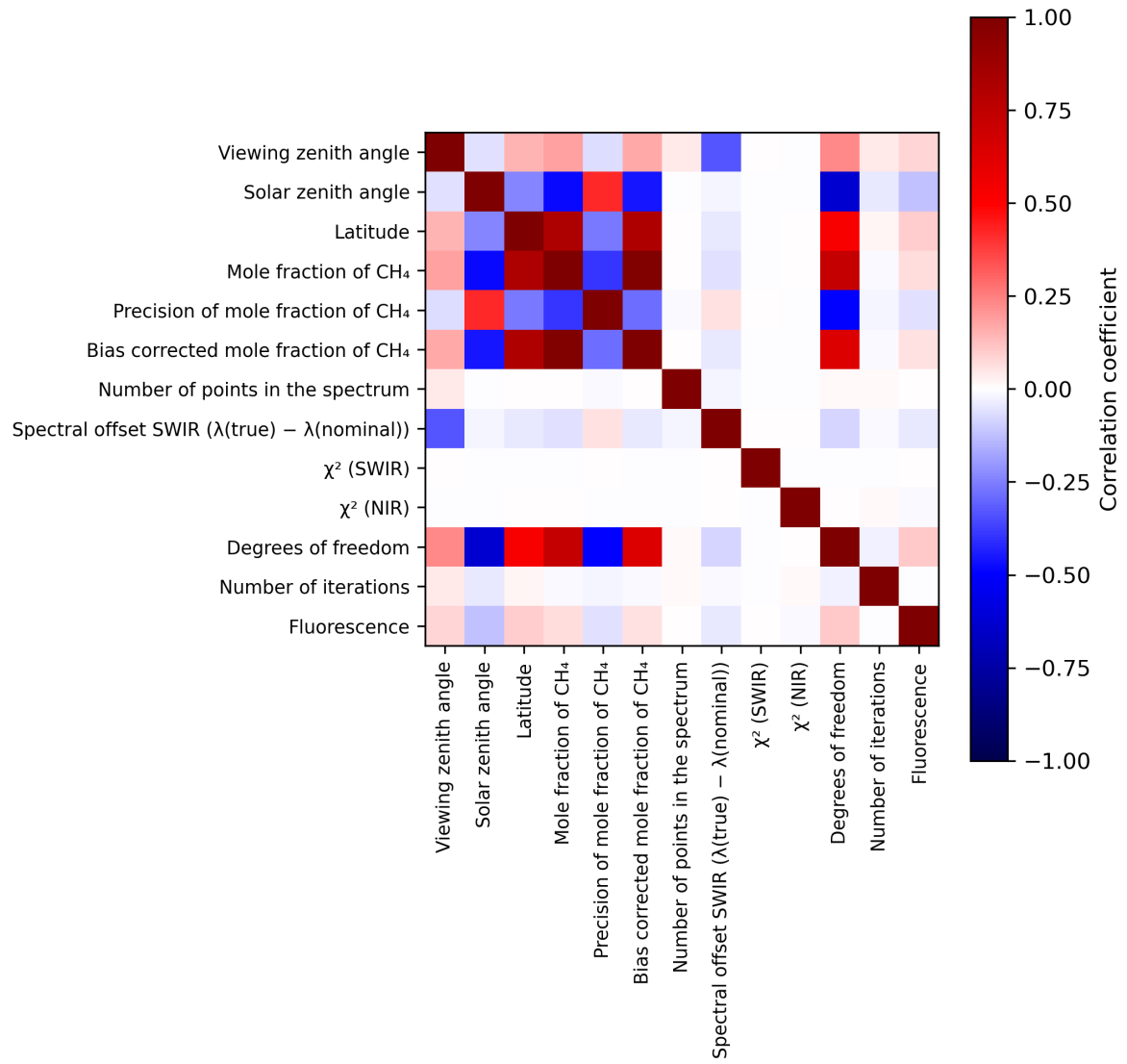
Figure 2: Map of correlation matrix for 2023-10-27 to 2023-10-28.
