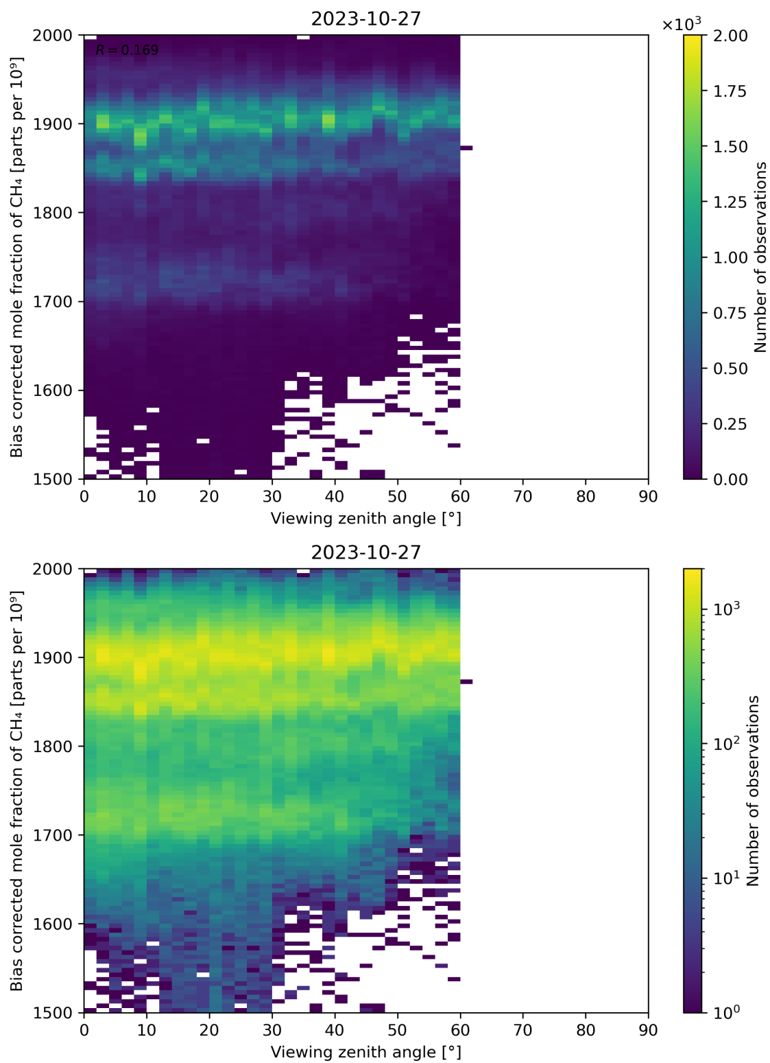
Figure 111: Scatter density plot of “Viewing zenith angle” against “Bias corrected mole fraction of CH 4 ” for 2023-10-27 to 2023-10-28.
