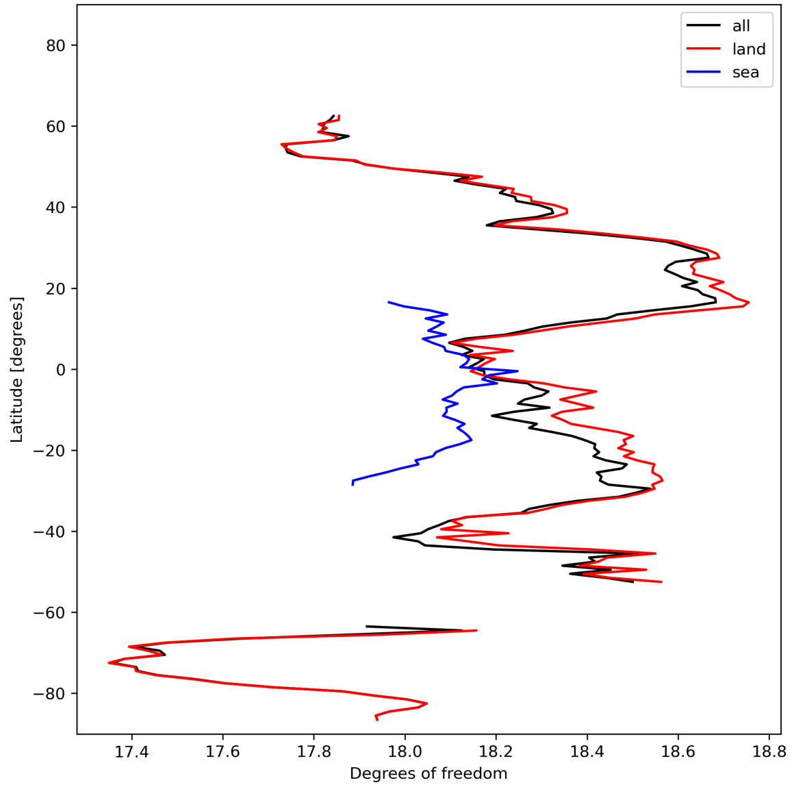
Figure 19: Zonal average of “Degrees of freedom” for 2023-10-27 to 2023-10-28.
