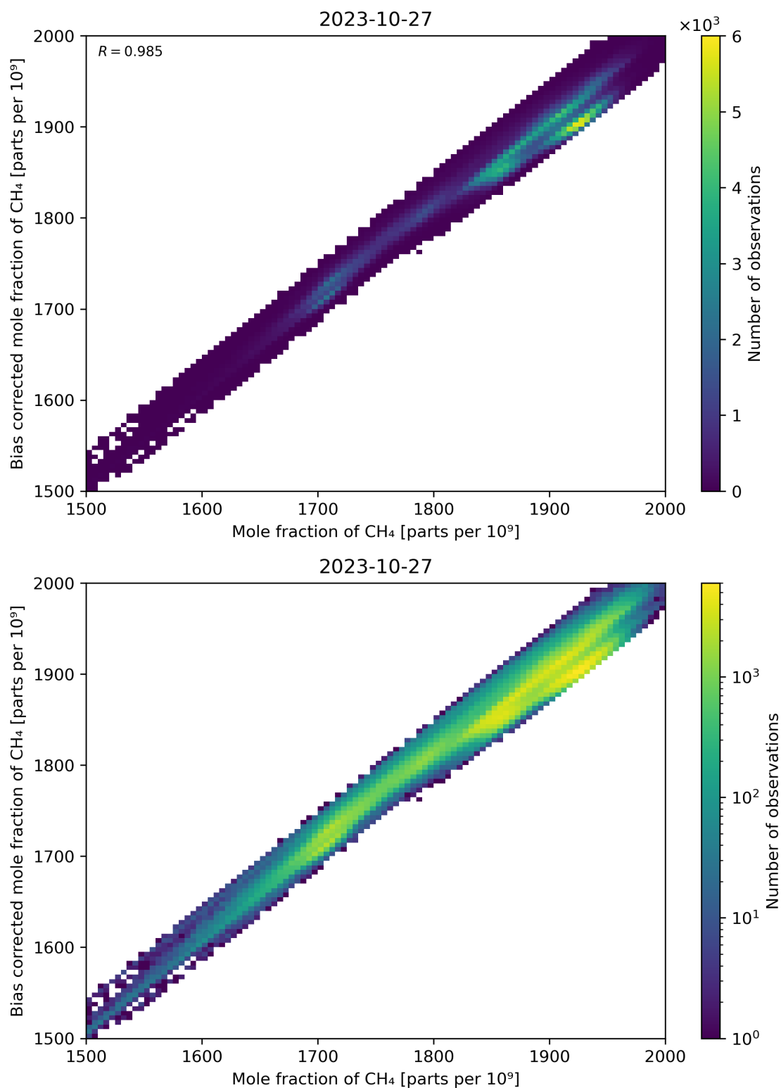
Figure 74: Scatter density plot of “Mole fraction of CH 4 ” against “Bias corrected mole fraction of CH 4 ” for 2023-10-27 to 2023-10-28.
