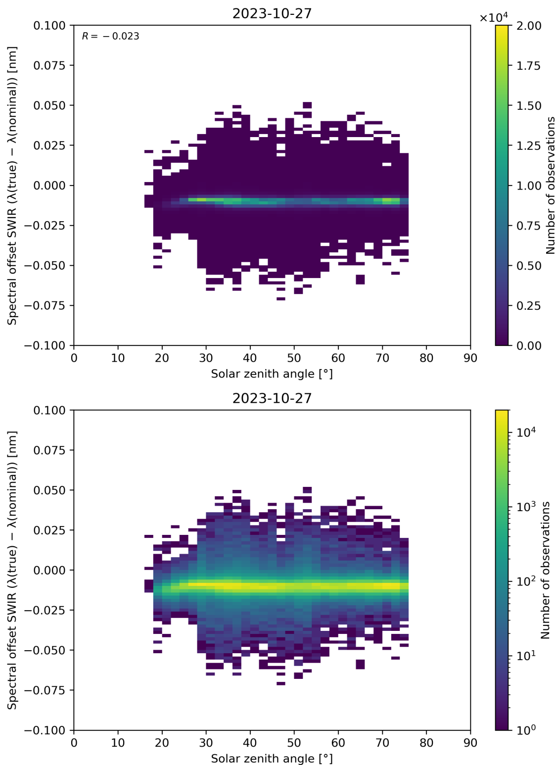
Figure 104: Scatter density plot of “Solar zenith angle” against “Spectral offset SWIR ( \lambda(\text{true}) - \lambda(\text{nominal}) )” for 2023-10-27 to 2023-10-28.
