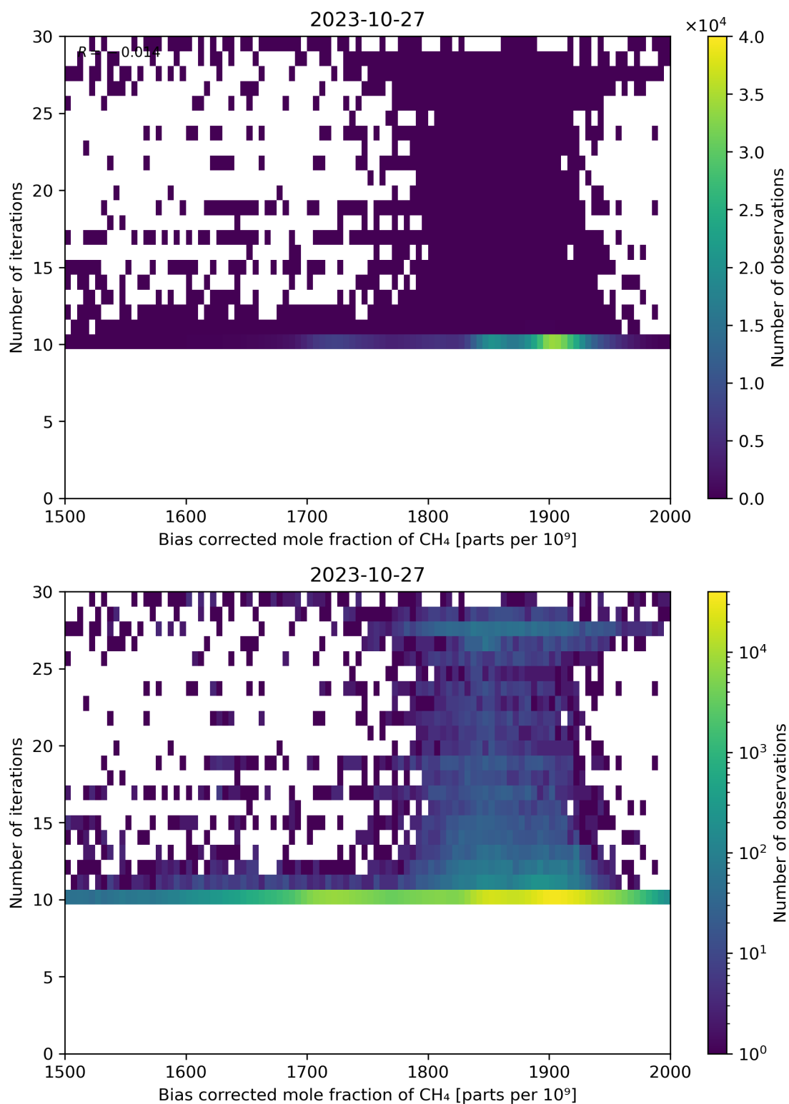
Figure 67: Scatter density plot of “Bias corrected mole fraction of CH 4 ” against “Number of iterations” for 2023-10-27 to 2023-10-28.
