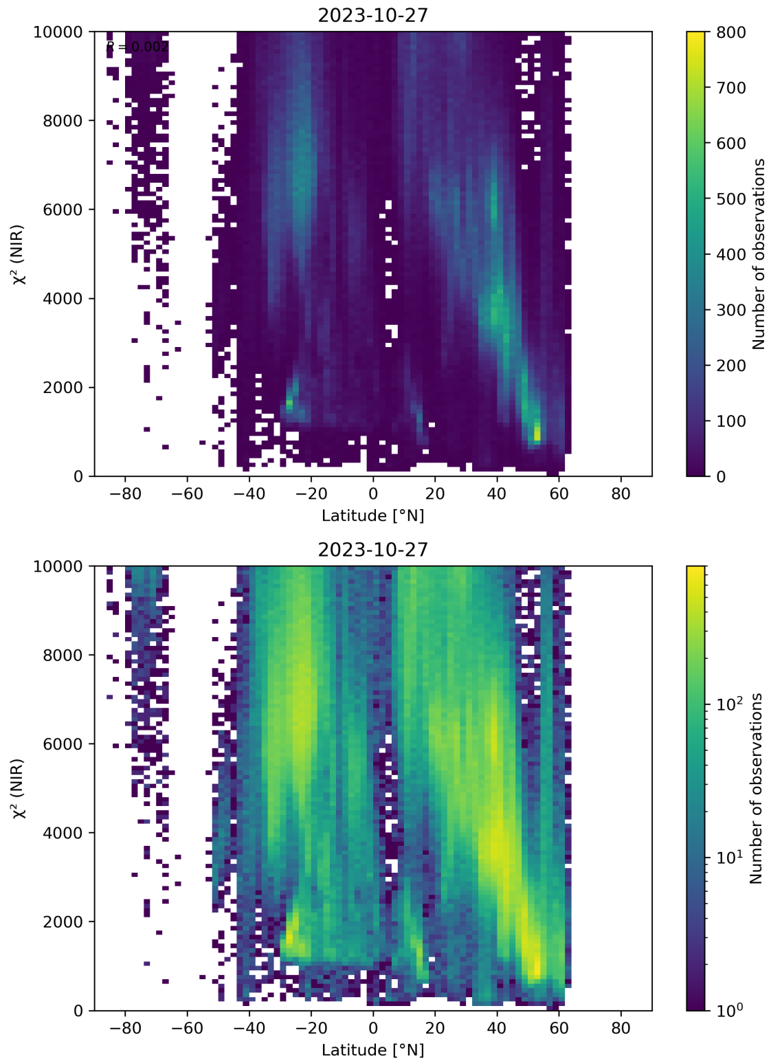
Figure 53: Scatter density plot of “Latitude” against “ \chi^2 (NIR)” for 2023-10-27 to 2023-10-28.
