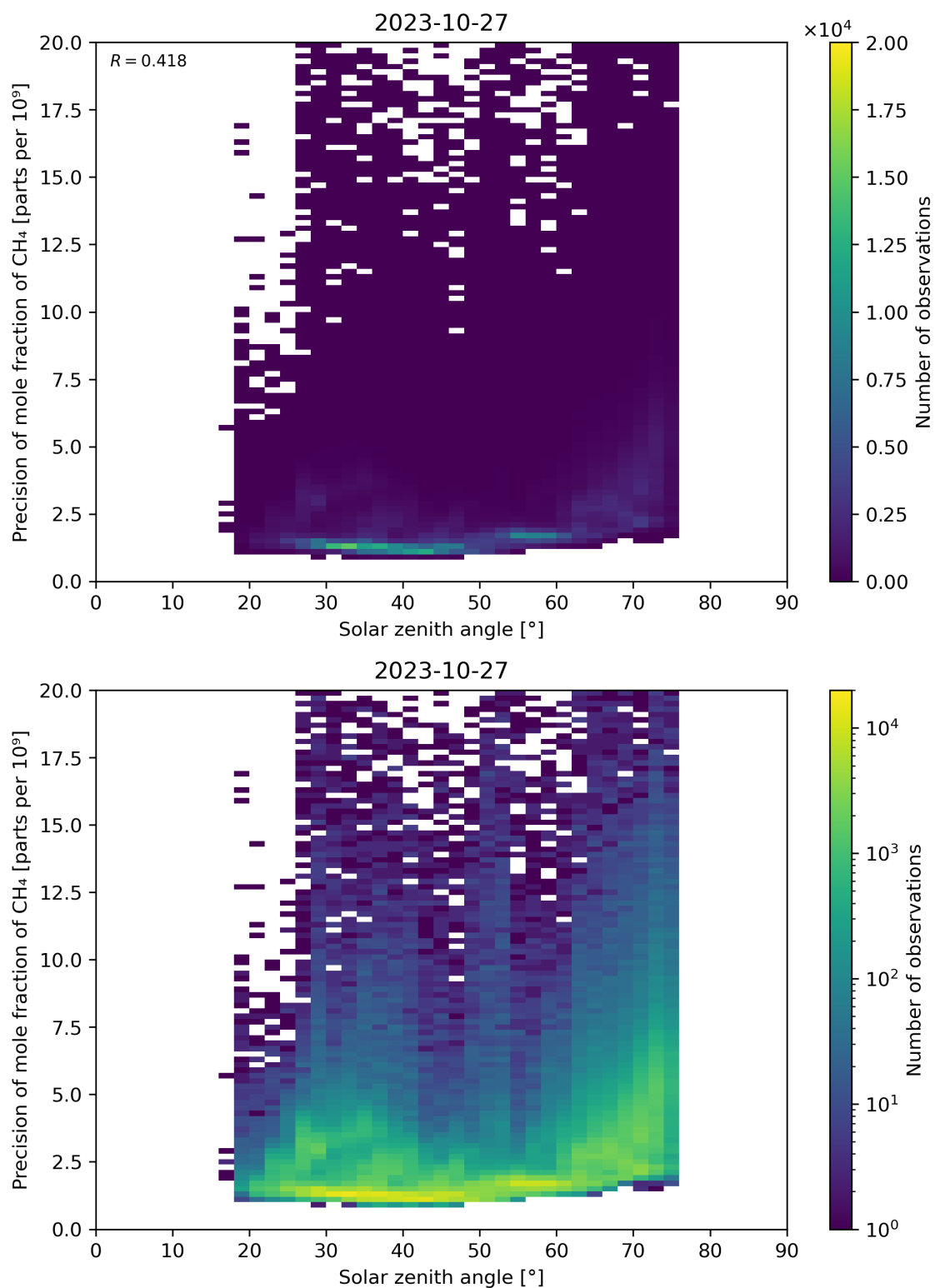
Figure 101: Scatter density plot of “Solar zenith angle” against “Precision of mole fraction of \text{CH}_4 ” for 2023-10-27 to 2023-10-28.
