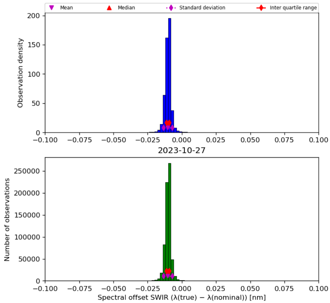
Figure 27: Histogram of “Spectral offset SWIR ( \lambda(\text{true}) - \lambda(\text{nominal}) )” for 2023-10-27 to 2023-10-28
