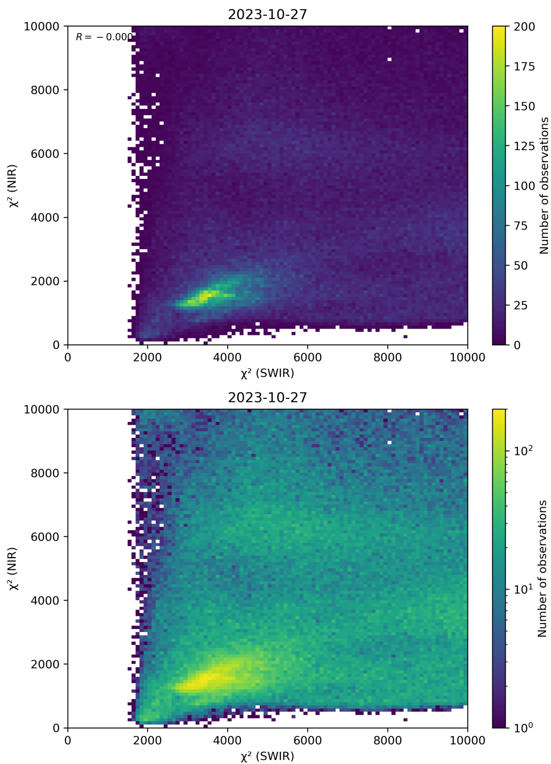
Figure 47: Scatter density plot of “ \chi^2 (SWIR)” against “ \chi^2 (NIR)” for 2023-10-27 to 2023-10-28.
