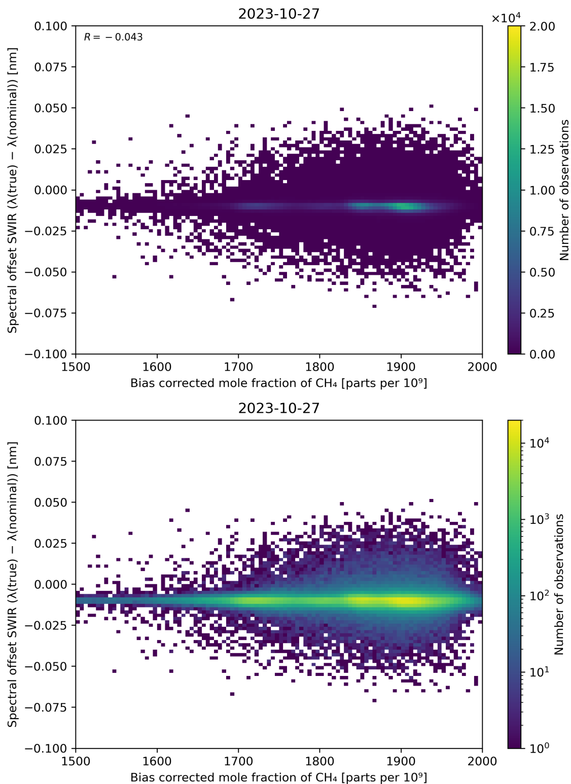
Figure 69: Scatter density plot of “Bias corrected mole fraction of \text{CH}_4 ” against “Spectral offset SWIR ( \lambda(\text{true}) - \lambda(\text{nominal}) )” for 2023-10-27 to 2023-10-28.
