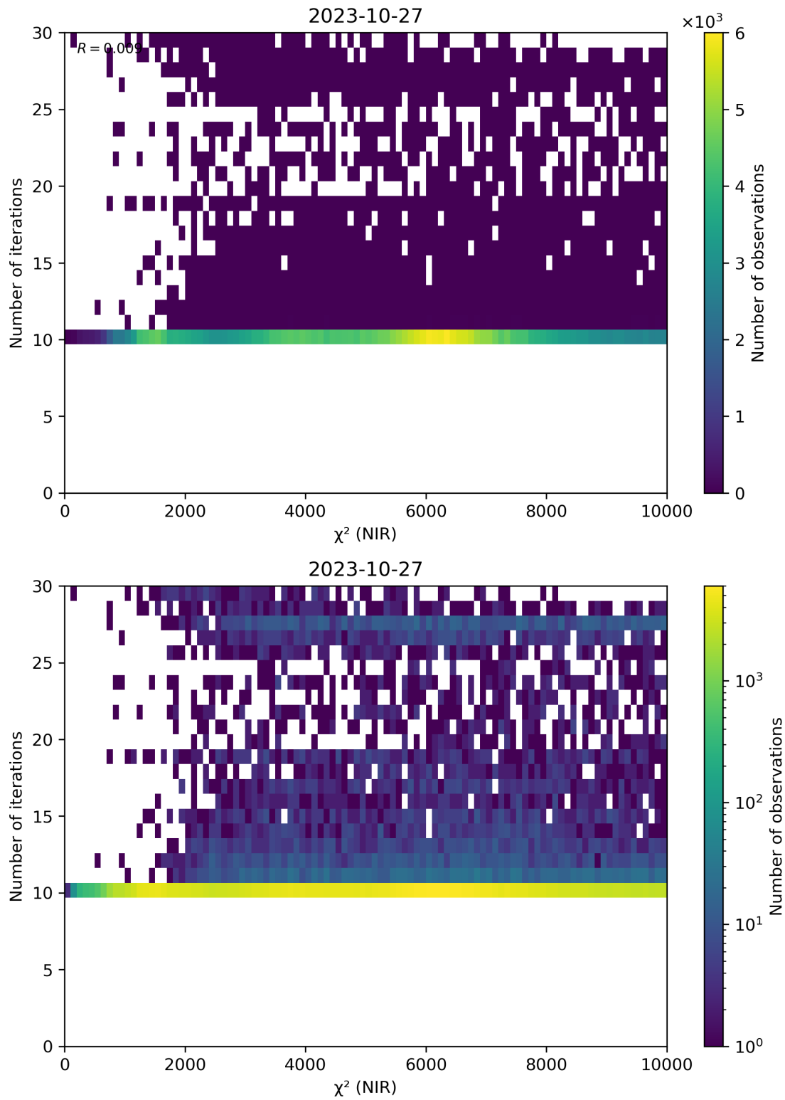
Figure 46: Scatter density plot of “ \chi^2 (NIR)” against “Number of iterations” for 2023-10-27 to 2023-10-28.
