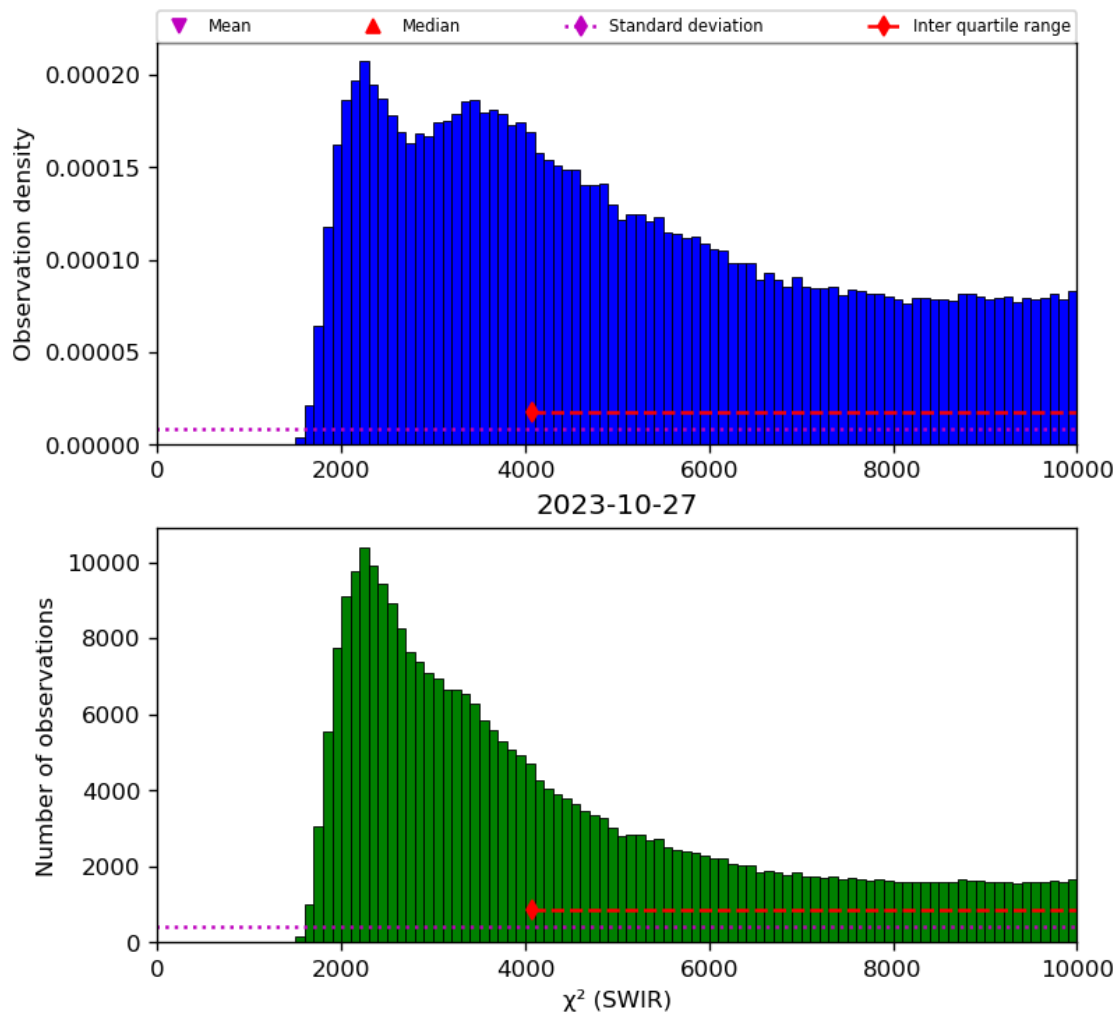
Figure 28: Histogram of “ \chi^2 (SWIR)” for 2023-10-27 to 2023-10-28
