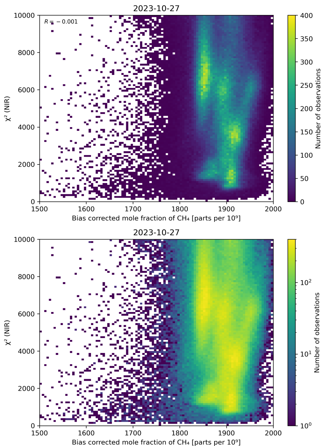
Figure 63: Scatter density plot of “Bias corrected mole fraction of CH 4 ” against “ \chi^2 (NIR)” for 2023-10-27 to 2023-10-28.
