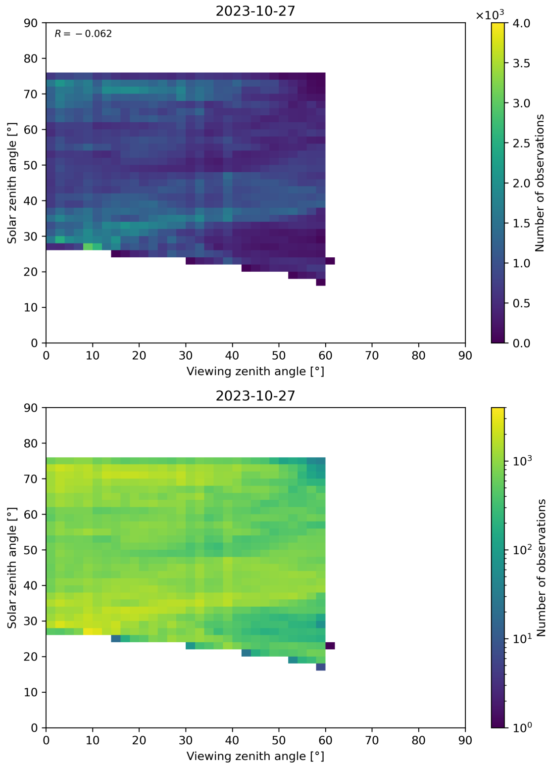
Figure 115: Scatter density plot of “Viewing zenith angle” against “Solar zenith angle” for 2023-10-27 to 2023-10-28.
