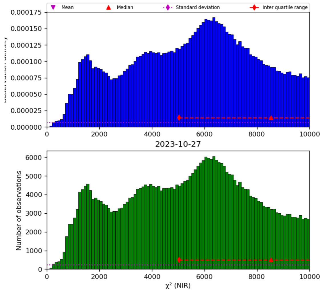
Figure 29: Histogram of “ \chi^2 (NIR)” for 2023-10-27 to 2023-10-28
