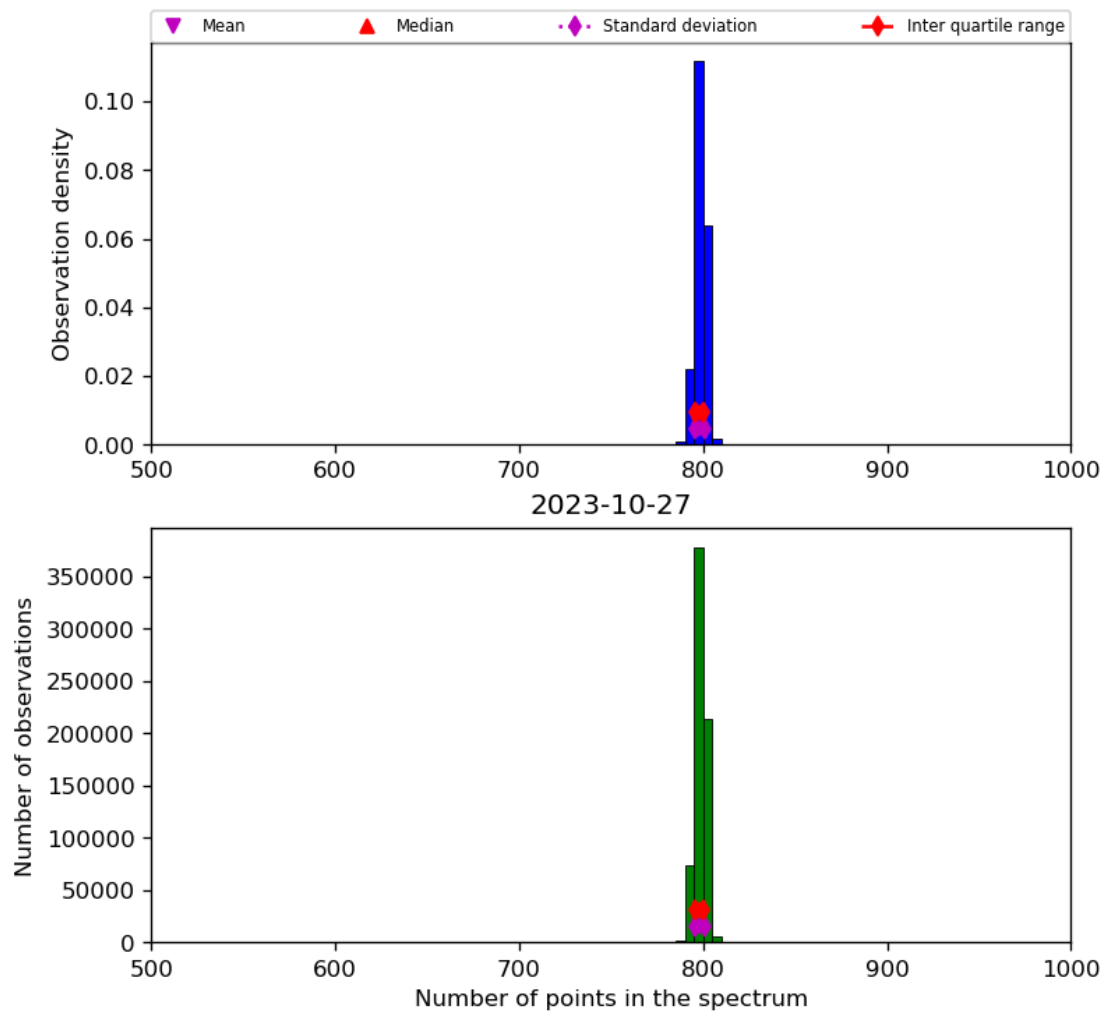
Figure 26: Histogram of “Number of points in the spectrum” for 2023-10-27 to 2023-10-28
