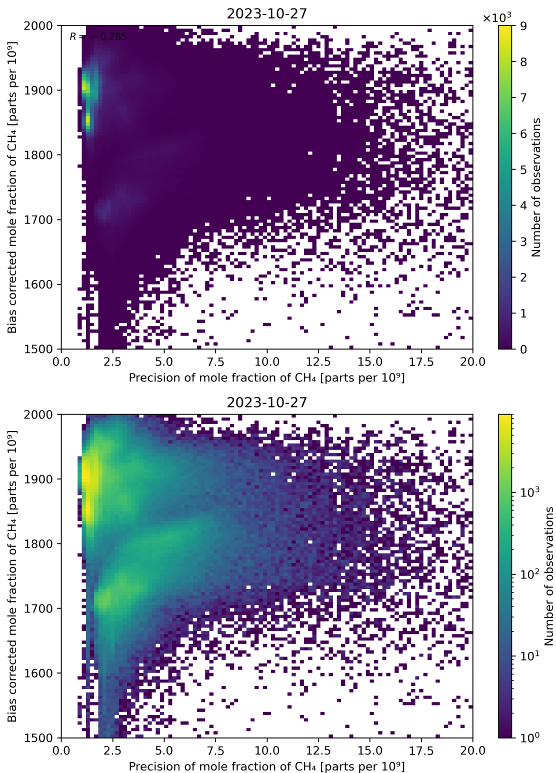
Figure 82: Scatter density plot of “Precision of mole fraction of CH 4 ” against “Bias corrected mole fraction of CH 4 ” for 2023-10-27 to 2023-10-28.
