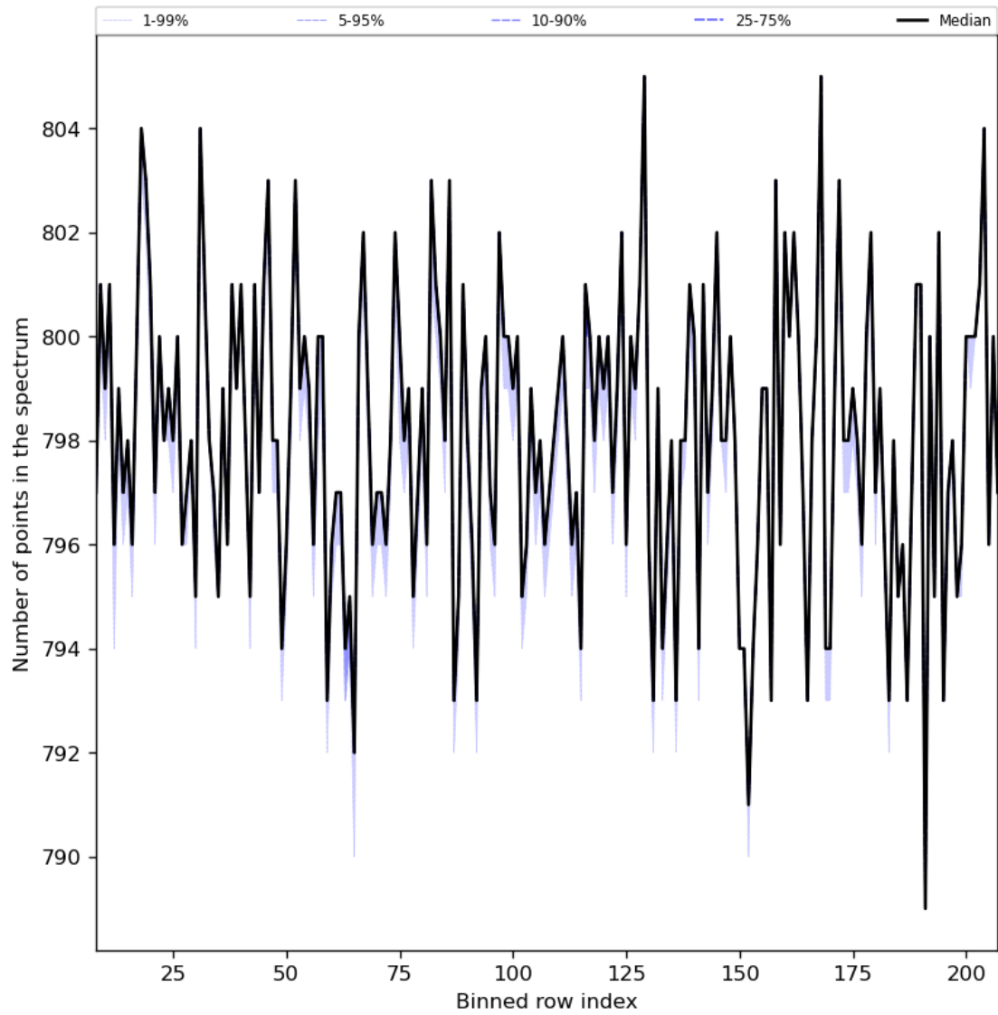
Figure 37: Along track statistics of “Number of points in the spectrum” for 2023-10-27 to 2023-10-28
