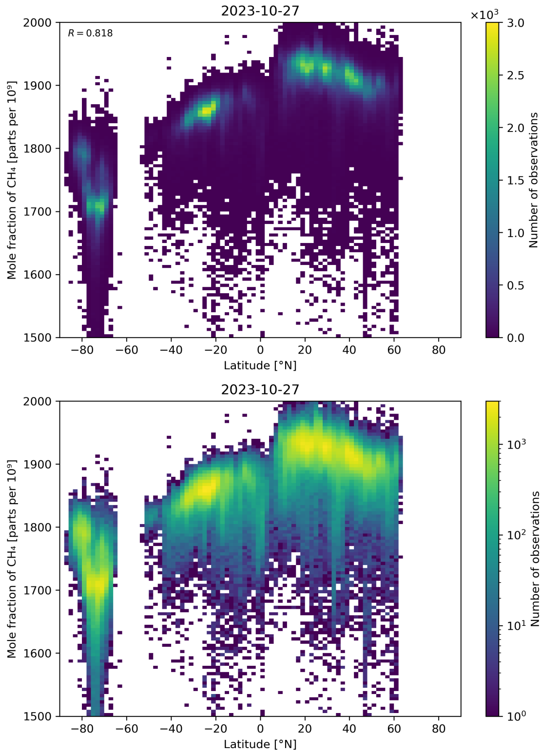
Figure 57: Scatter density plot of “Latitude” against “Mole fraction of \text{CH}_4 ” for 2023-10-27 to 2023-10-28.
