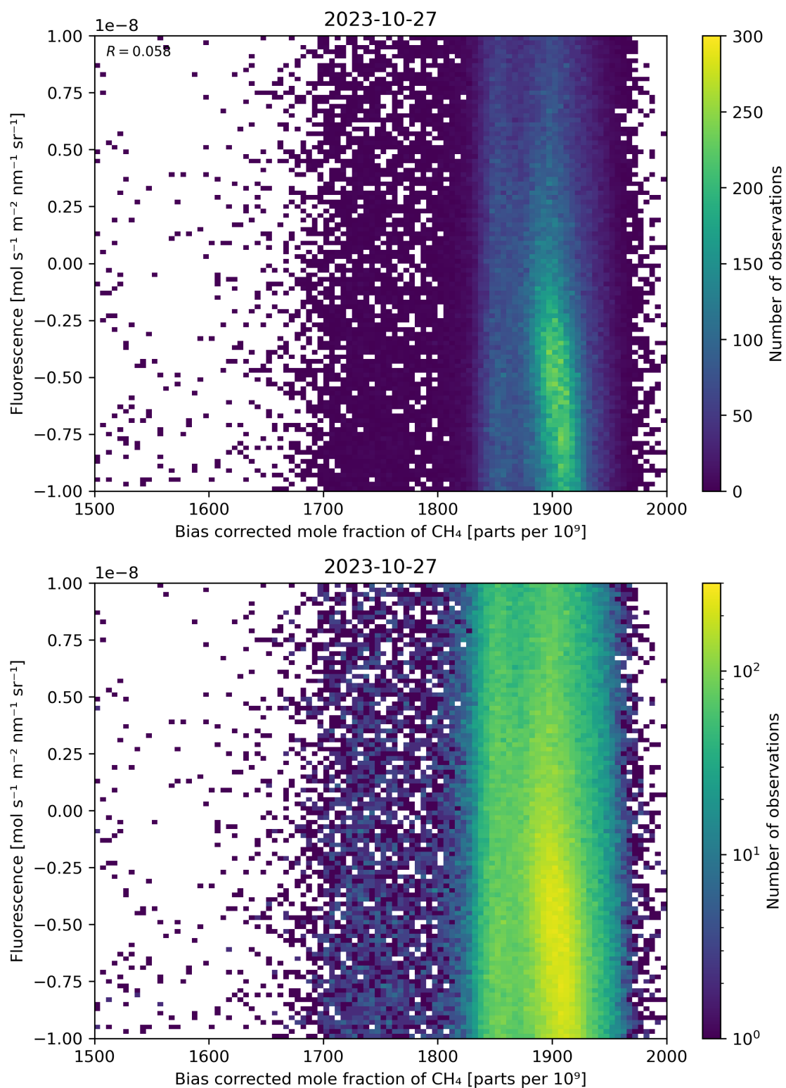
Figure 66: Scatter density plot of “Bias corrected mole fraction of \text{CH}_4 ” against “Fluorescence” for 2023-10-27 to 2023-10-28.
