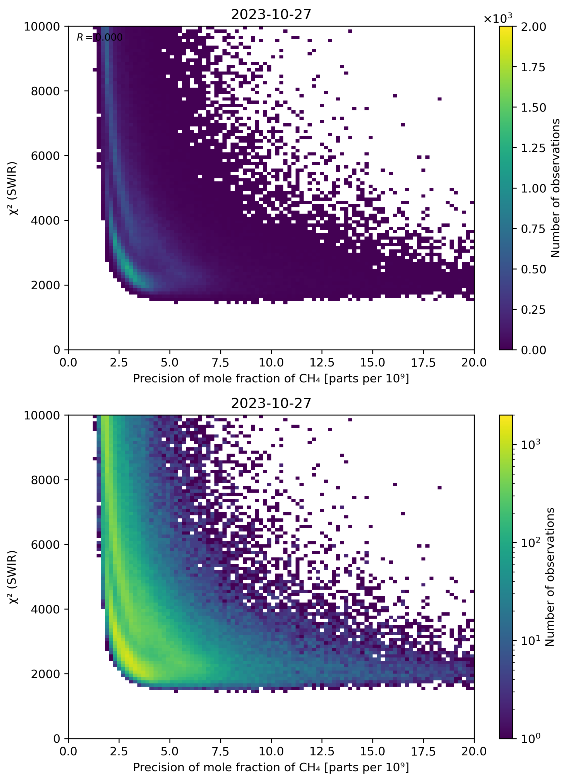
Figure 79: Scatter density plot of “Precision of mole fraction of CH 4 ” against “ \chi^2 (SWIR)” for 2023-10-27 to 2023-10-28.
