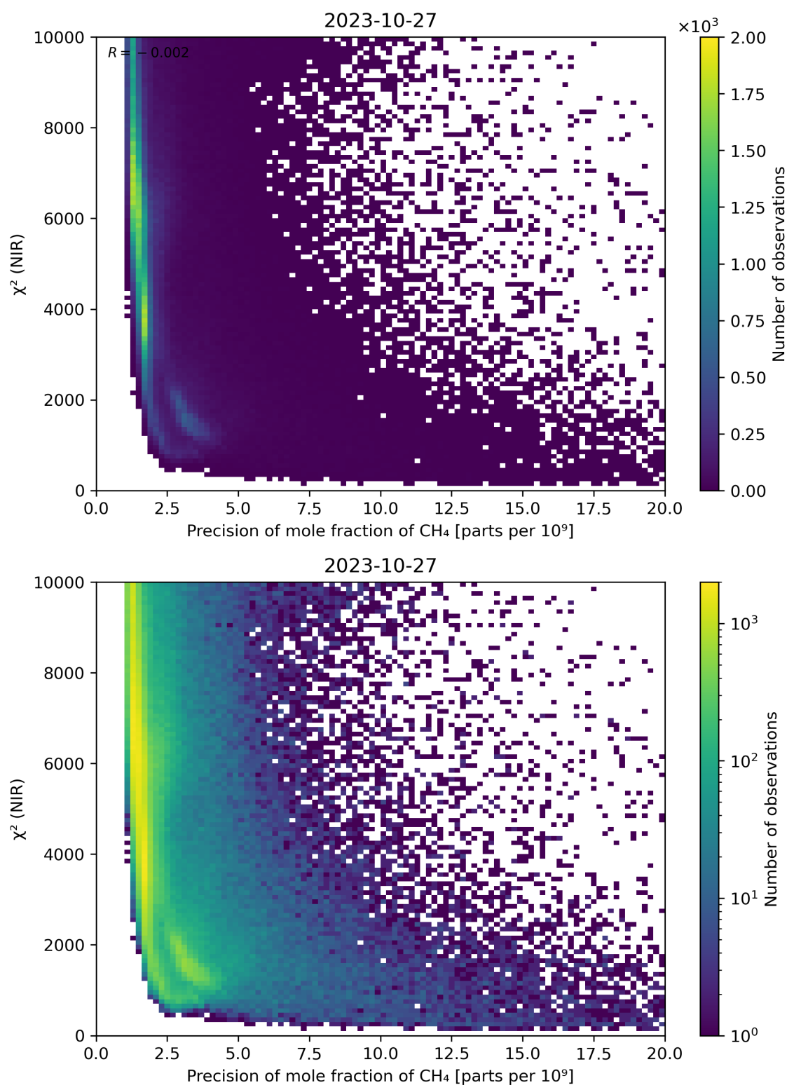
Figure 78: Scatter density plot of “Precision of mole fraction of \text{CH}_4 ” against “ \chi^2 (NIR)” for 2023-10-27 to 2023-10-28.
