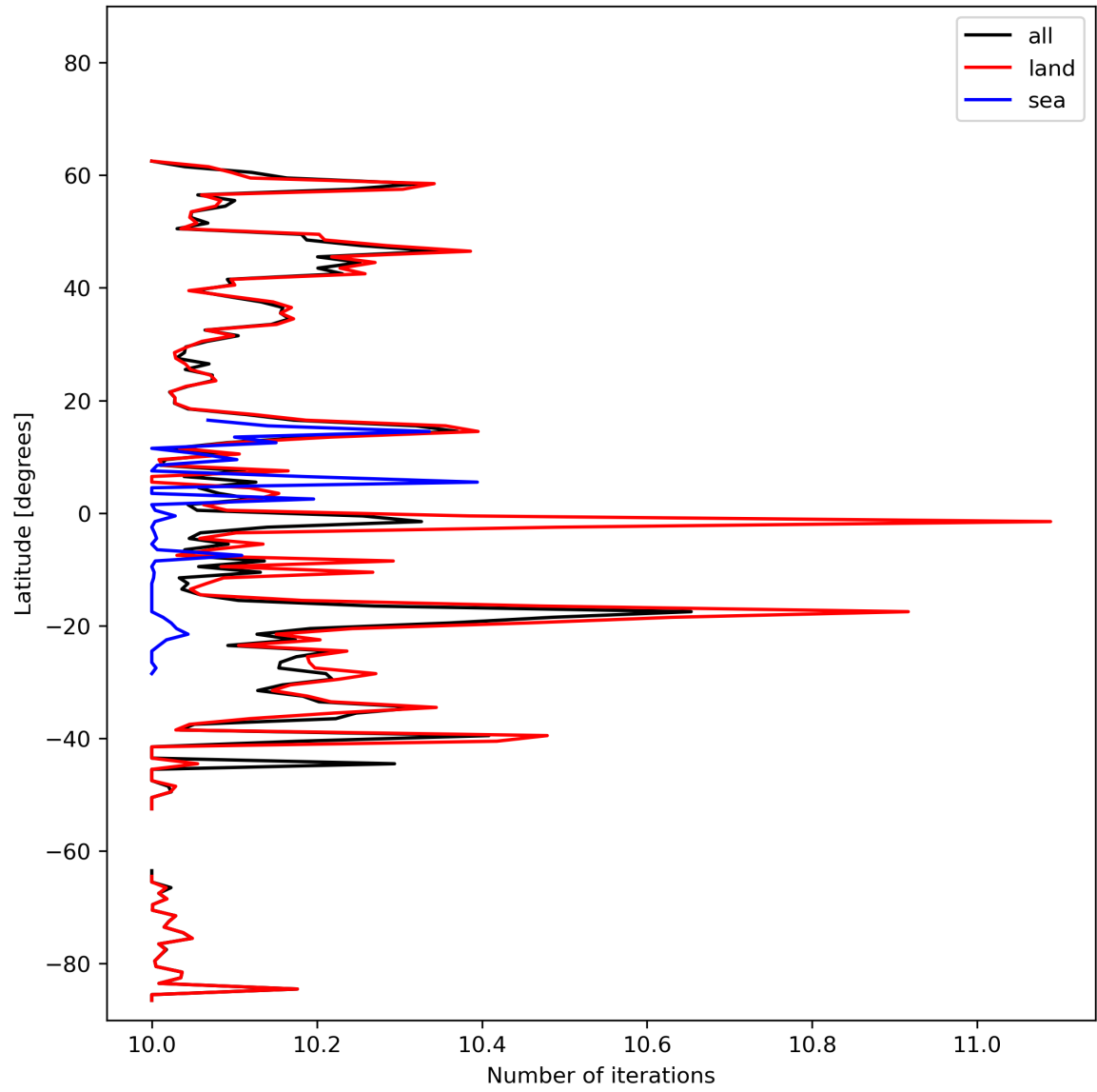
Figure 20: Zonal average of “Number of iterations” for 2023-10-27 to 2023-10-28.
