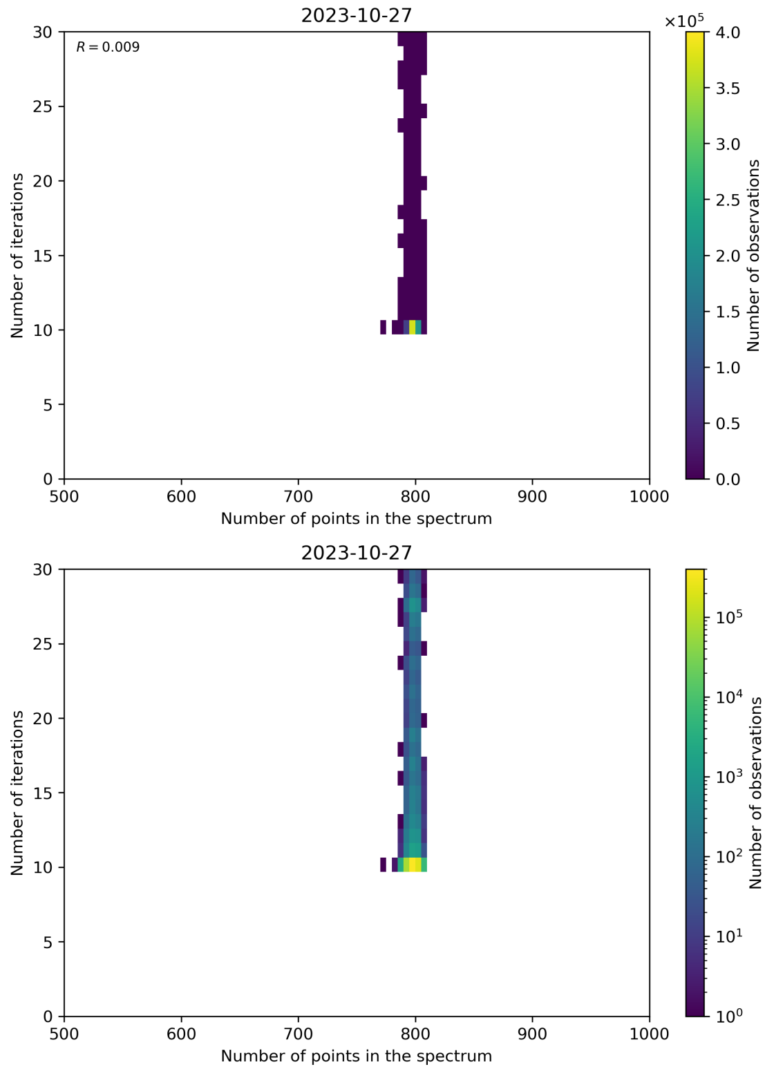
Figure 92: Scatter density plot of “Number of points in the spectrum” against “Number of iterations” for 2023-10-27 to 2023-10-28.
