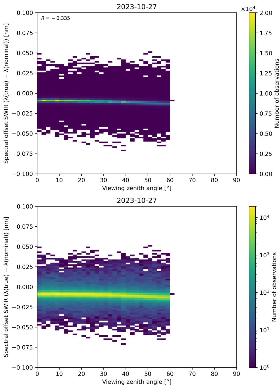
Figure 116: Scatter density plot of “Viewing zenith angle” against “Spectral offset SWIR ( \lambda(\text{true}) - \lambda(\text{nominal}) )” for 2023-10-27 to 2023-10-28.
