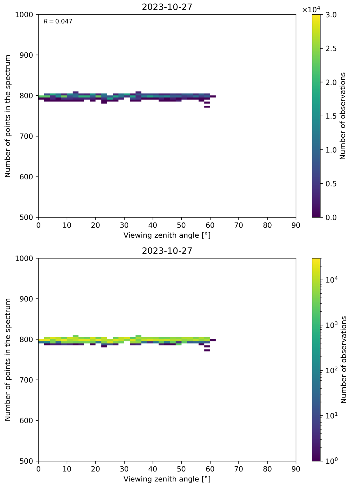
Figure 114: Scatter density plot of “Viewing zenith angle” against “Number of points in the spectrum” for 2023-10-27 to 2023-10-28.
