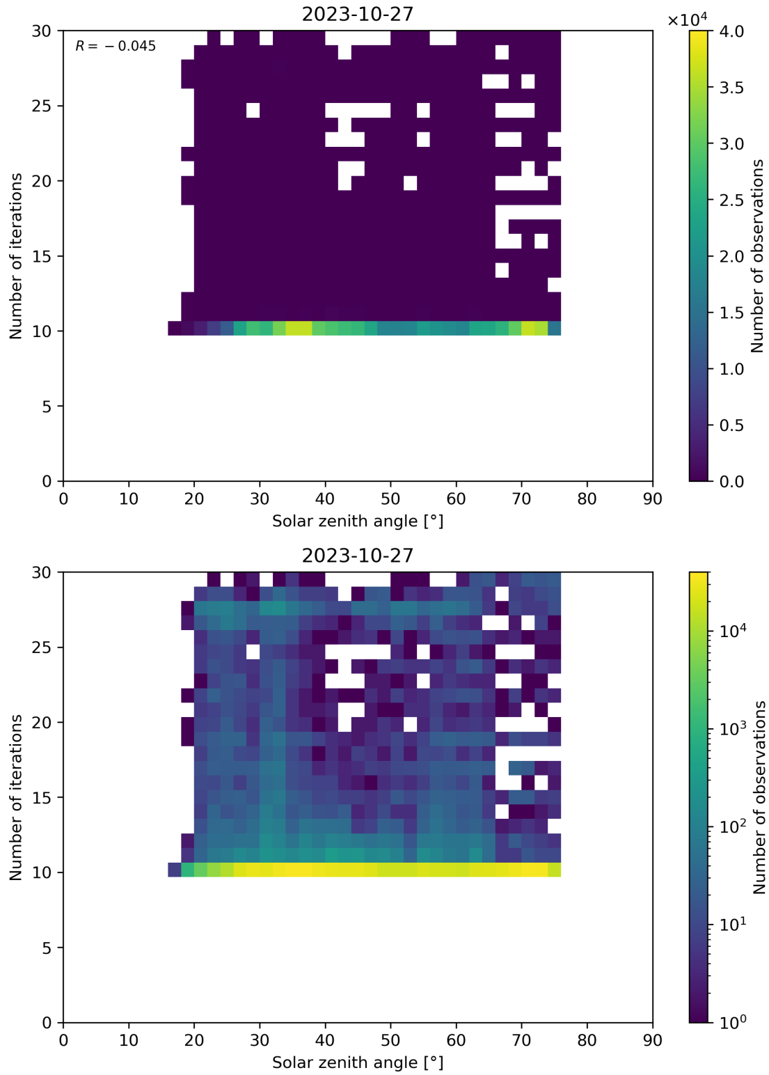
Figure 102: Scatter density plot of “Solar zenith angle” against “Number of iterations” for 2023-10-27 to 2023-10-28.
