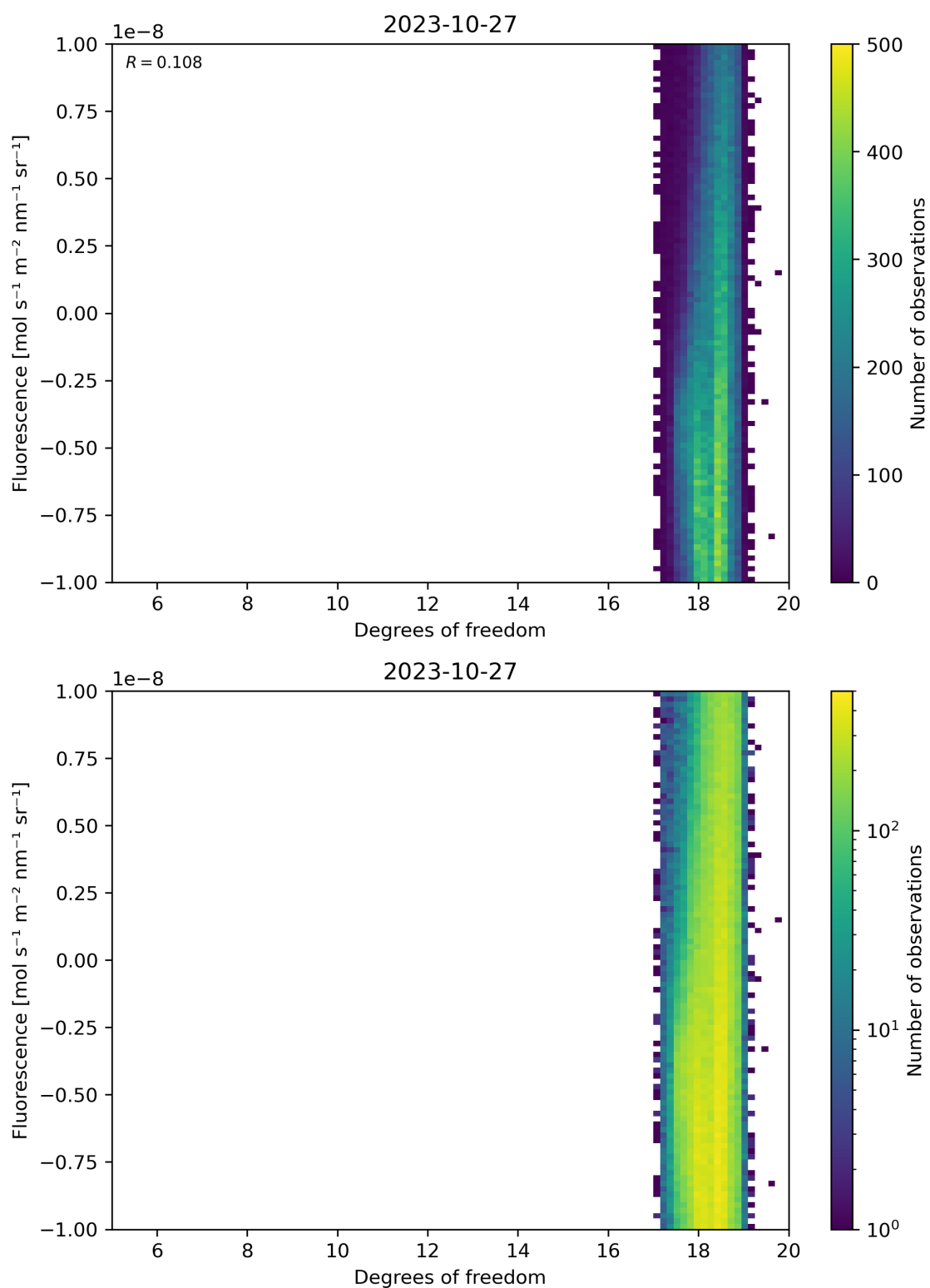
Figure 51: Scatter density plot of “Degrees of freedom” against “Fluorescence” for 2023-10-27 to 2023-10-28.
