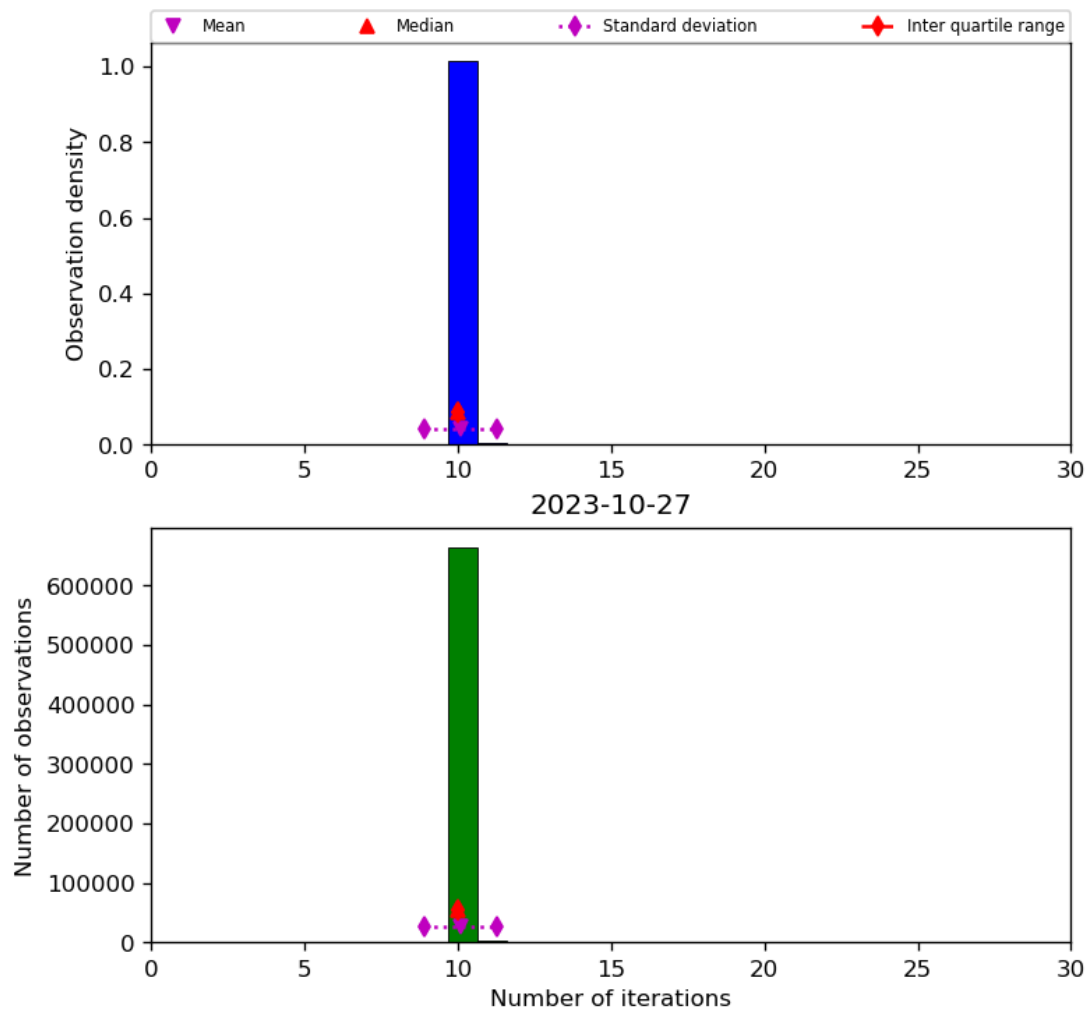
Figure 31: Histogram of “Number of iterations” for 2023-10-27 to 2023-10-28
