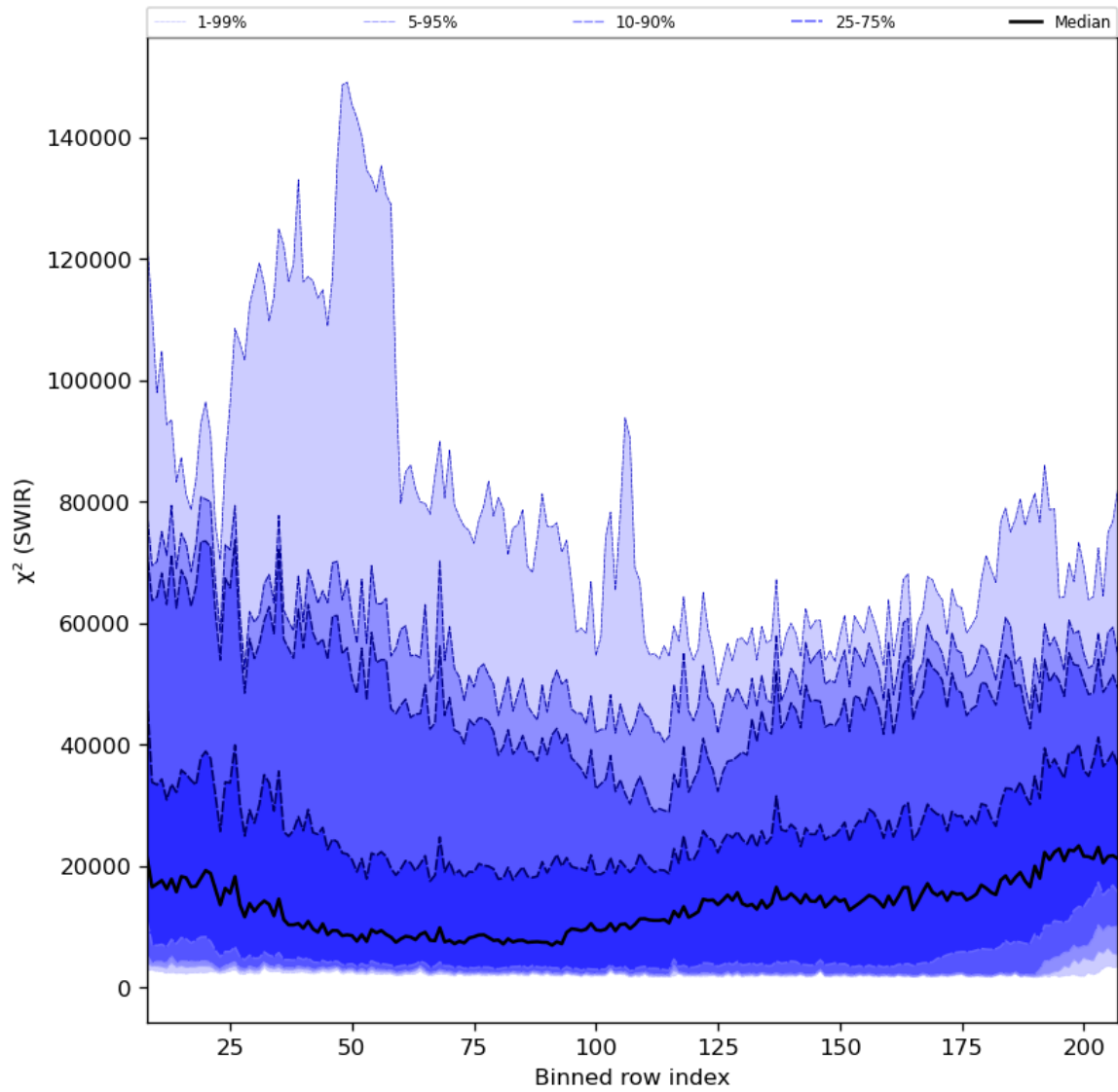
Figure 39: Along track statistics of “ \chi^2 (SWIR)” for 2023-10-27 to 2023-10-28
