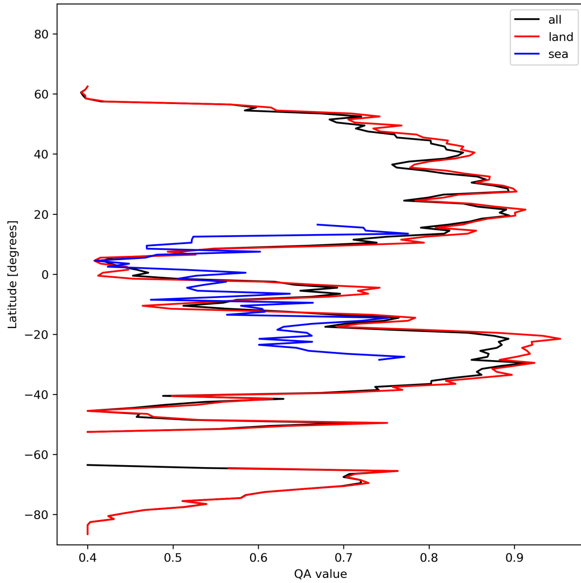
Figure 11: Zonal average of “QA value” for 2023-10-27 to 2023-10-28.
