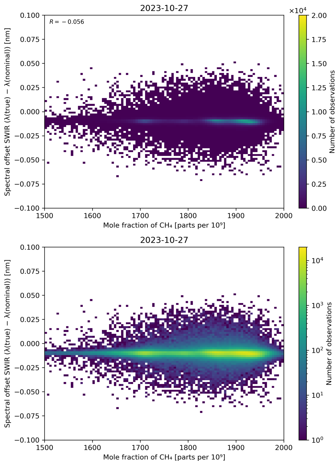
Figure 86: Scatter density plot of “Mole fraction of CH 4 ” against “Spectral offset SWIR ( \lambda(\text{true}) - \lambda(\text{nominal}) )” for 2023-10-27 to 2023-10-28.
