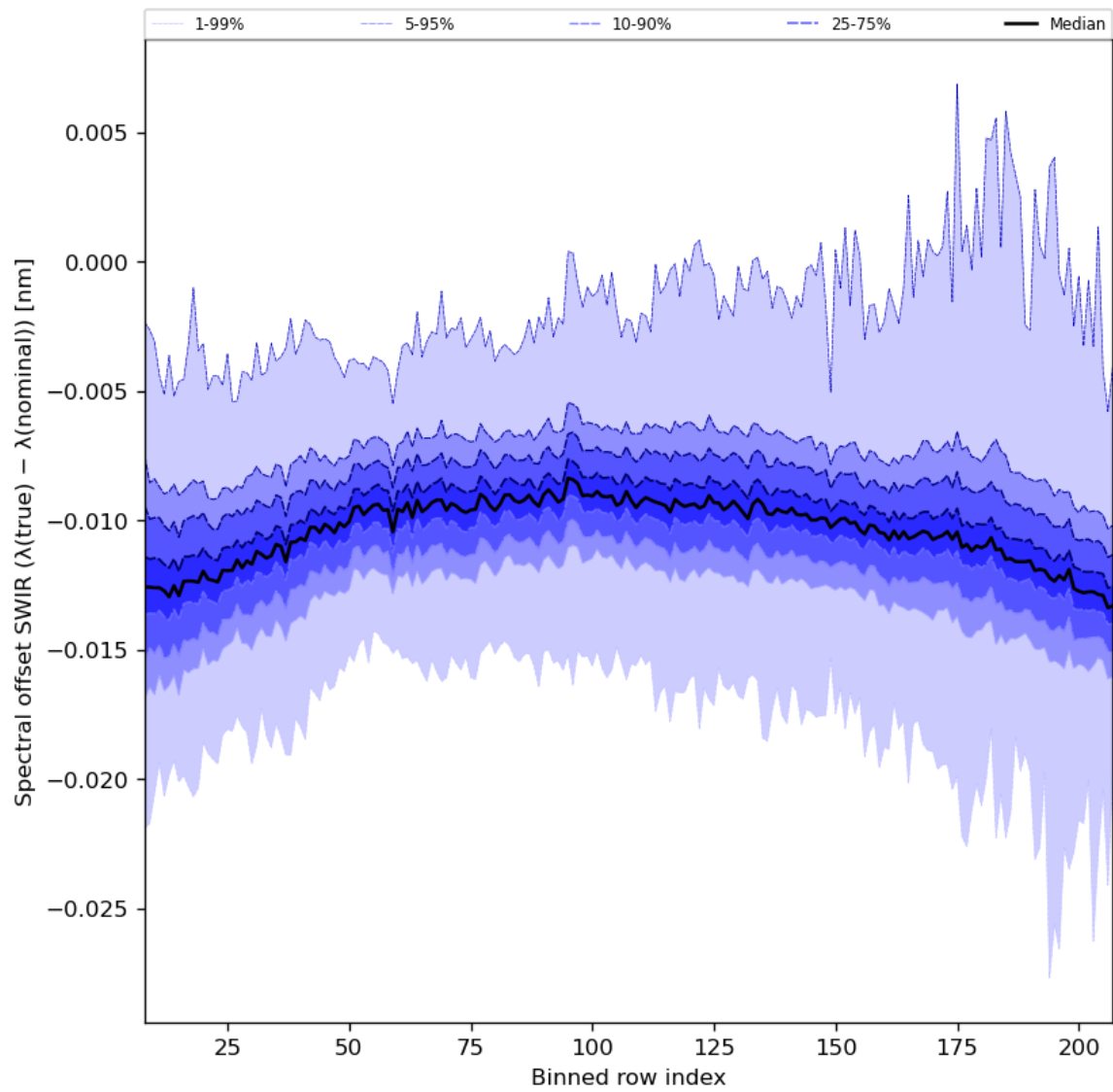
Figure 38: Along track statistics of “Spectral offset SWIR ( \lambda(\text{true}) - \lambda(\text{nominal}) )” for 2023-10-27 to 2023-10-28
