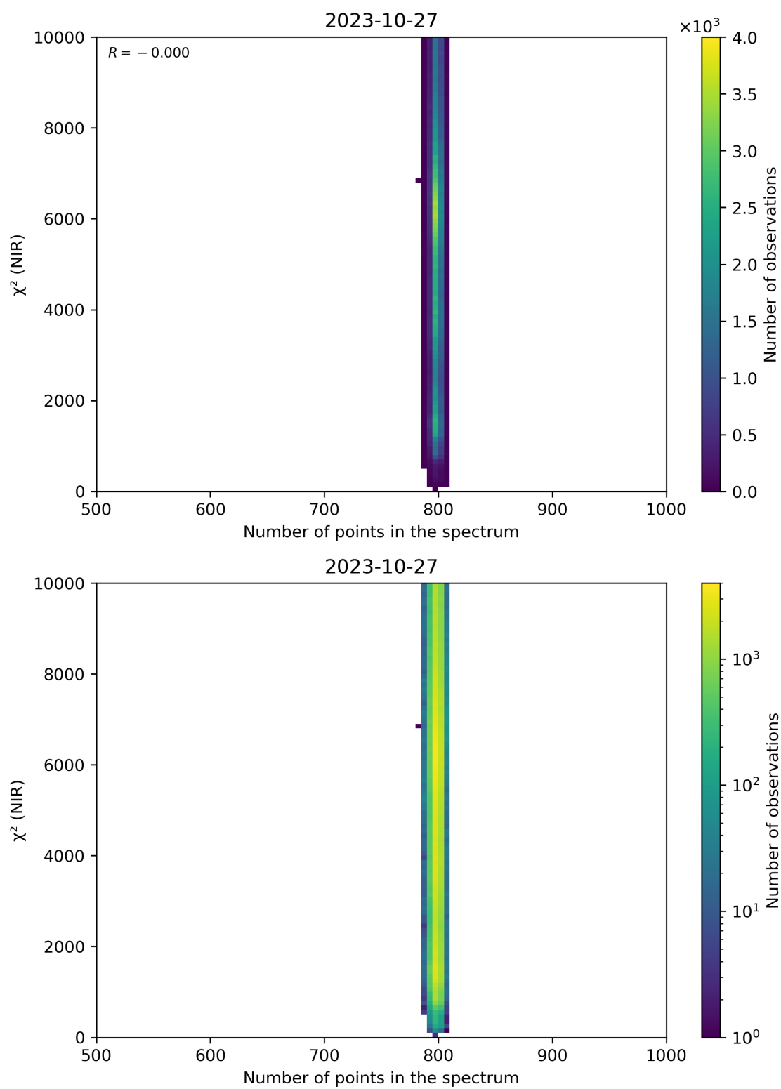
Figure 88: Scatter density plot of “Number of points in the spectrum” against “ \chi^2 (NIR)” for 2023-10-27 to 2023-10-28.
