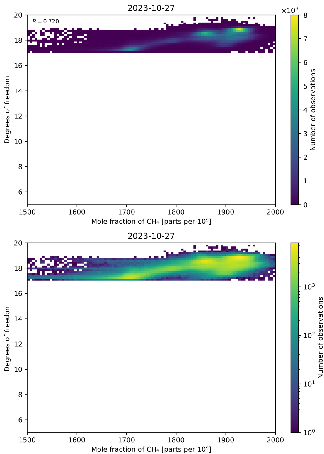
Figure 72: Scatter density plot of “Mole fraction of CH 4 ” against “Degrees of freedom” for 2023-10-27 to 2023-10-28.
