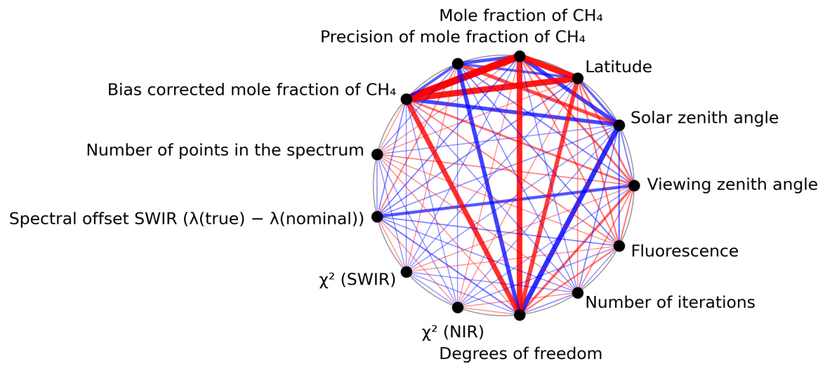
Figure 1: Map of correlation graph for 2023-10-27 to 2023-10-28.
