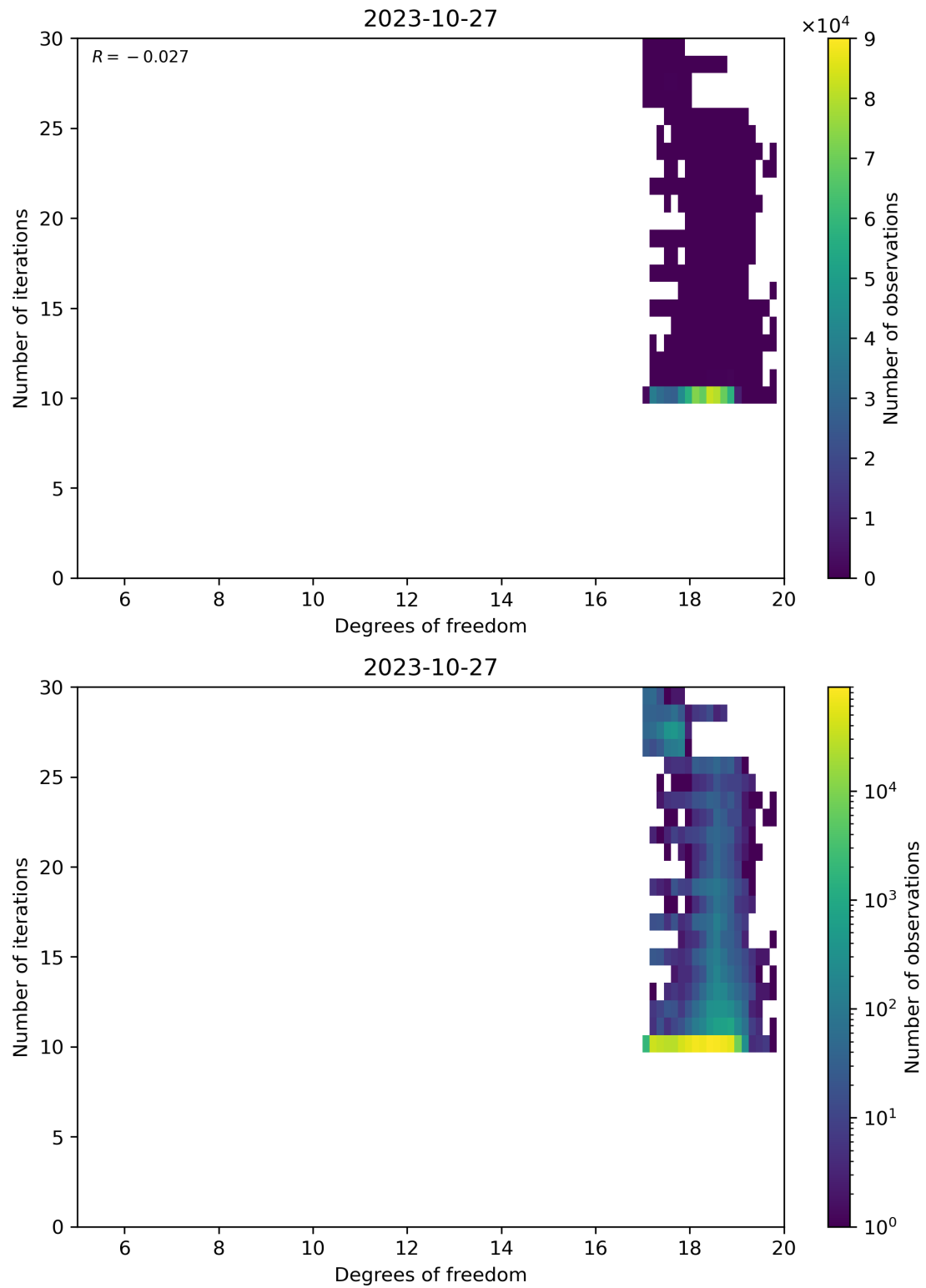
Figure 52: Scatter density plot of “Degrees of freedom” against “Number of iterations” for 2023-10-27 to 2023-10-28.
