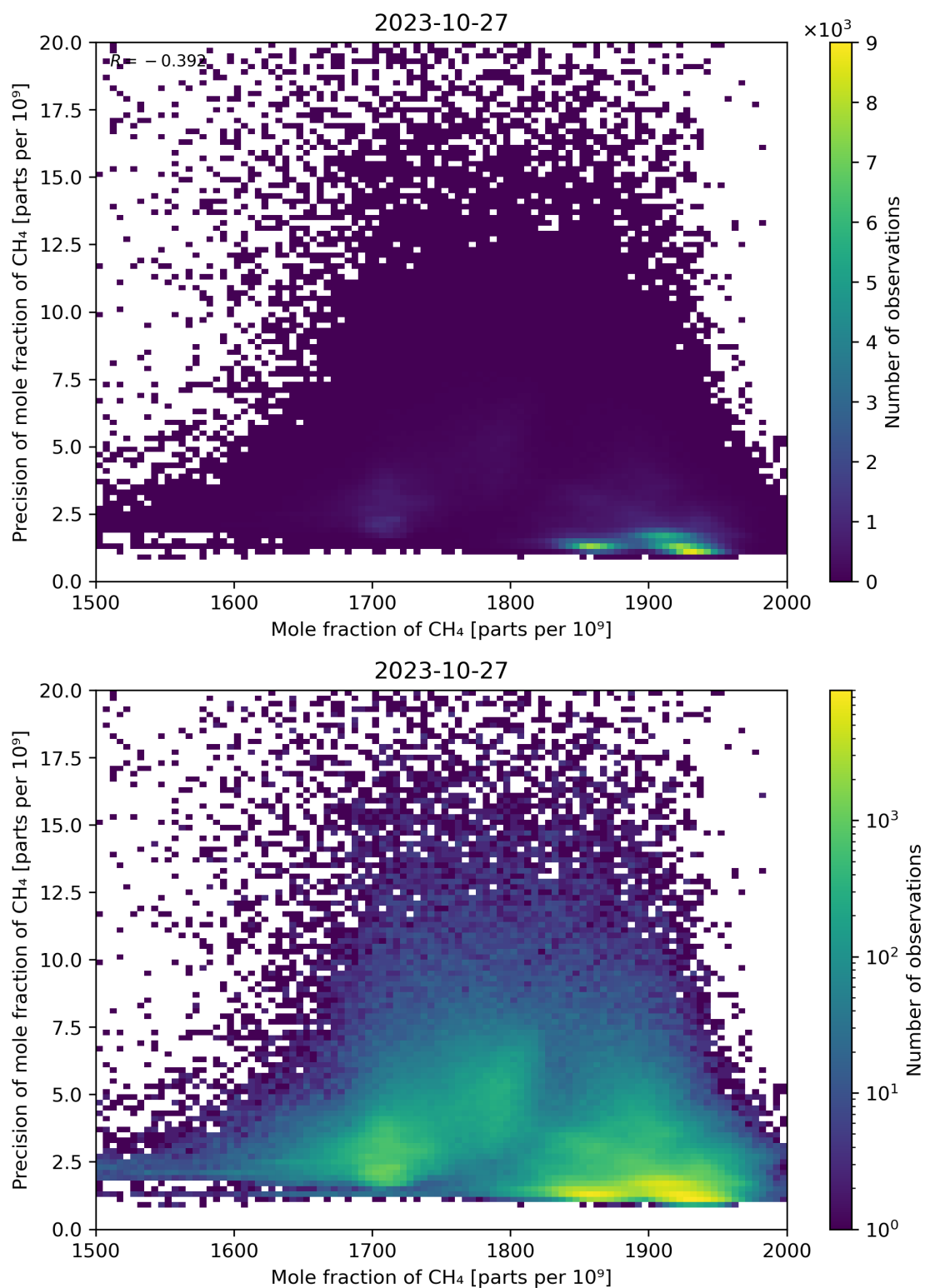
Figure 75: Scatter density plot of “Mole fraction of CH 4 ” against “Precision of mole fraction of CH 4 ” for 2023-10-27 to 2023-10-28.
