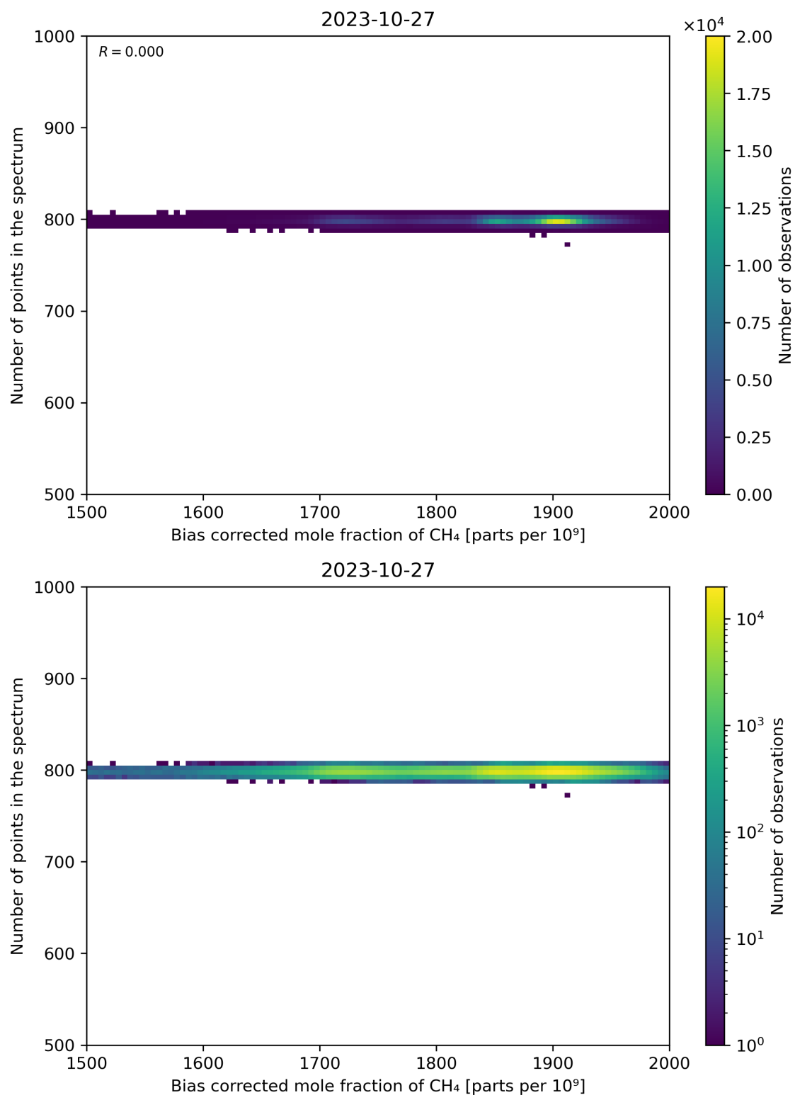
Figure 68: Scatter density plot of “Bias corrected mole fraction of CH 4 ” against “Number of points in the spectrum” for 2023-10-27 to 2023-10-28.
