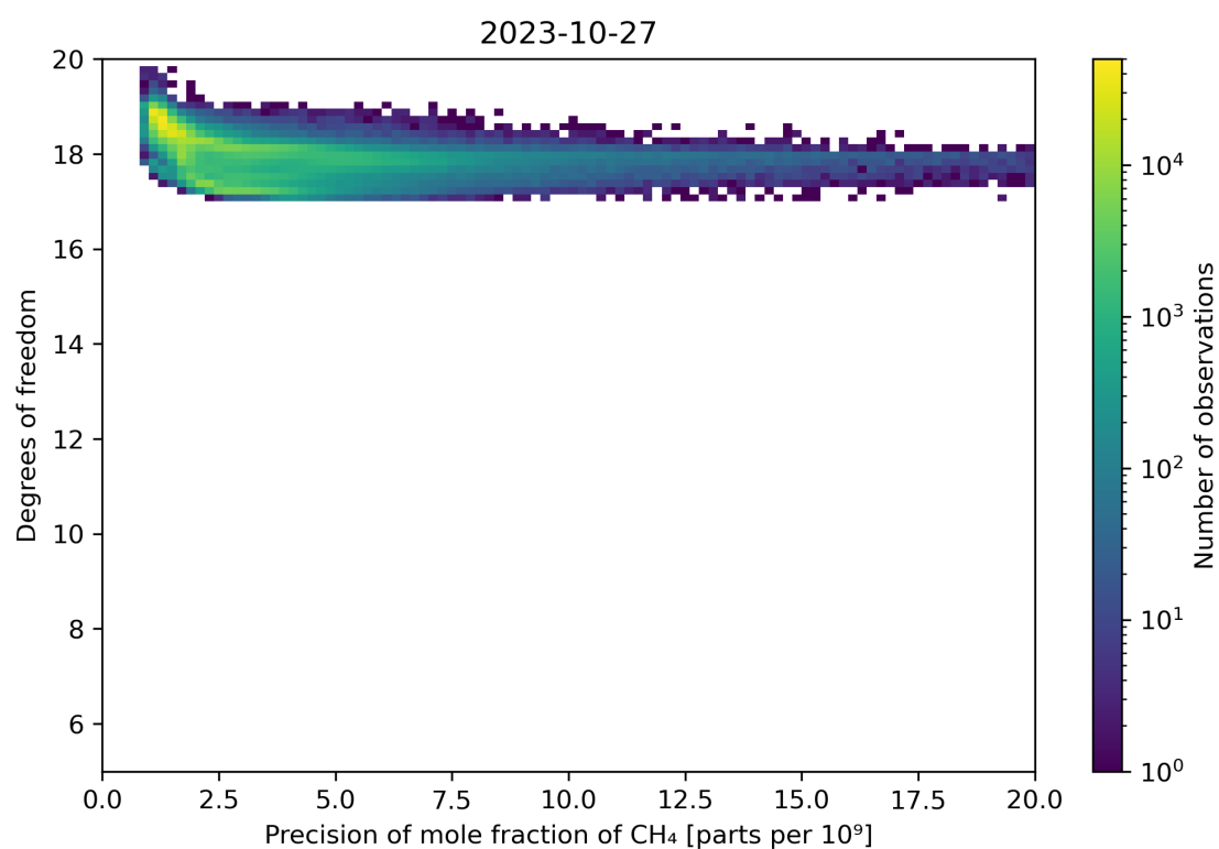
Figure 80: Scatter density plot of “Precision of mole fraction of CH 4 ” against “Degrees of freedom” for 2023-10-27 to 2023-10-28.
