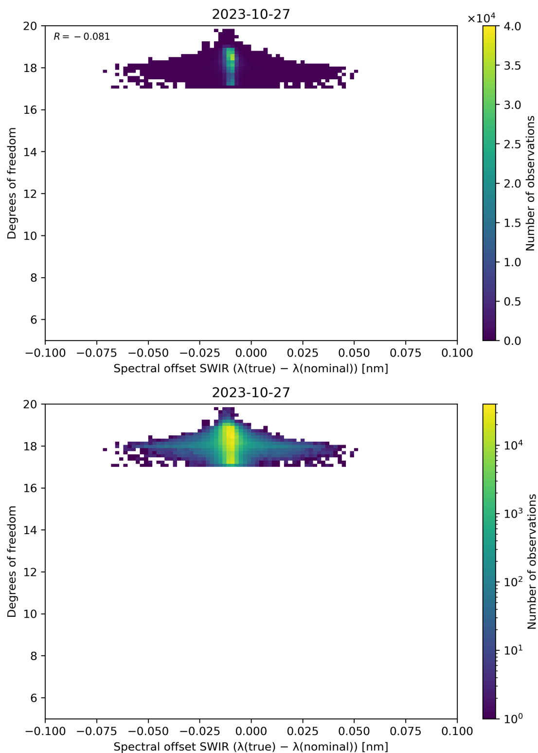
Figure 119: Scatter density plot of “Spectral offset SWIR ( \lambda(\text{true}) - \lambda(\text{nominal}) )” against “Degrees of freedom” for 2023-10-27 to 2023-10-28.
