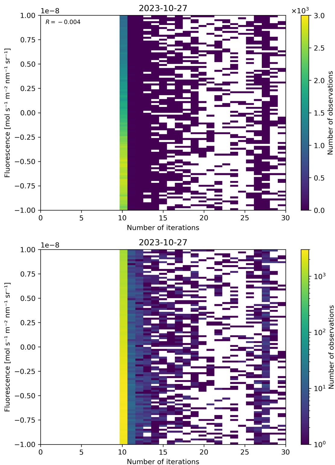
Figure 87: Scatter density plot of “Number of iterations” against “Fluorescence” for 2023-10-27 to 2023-10-28.
