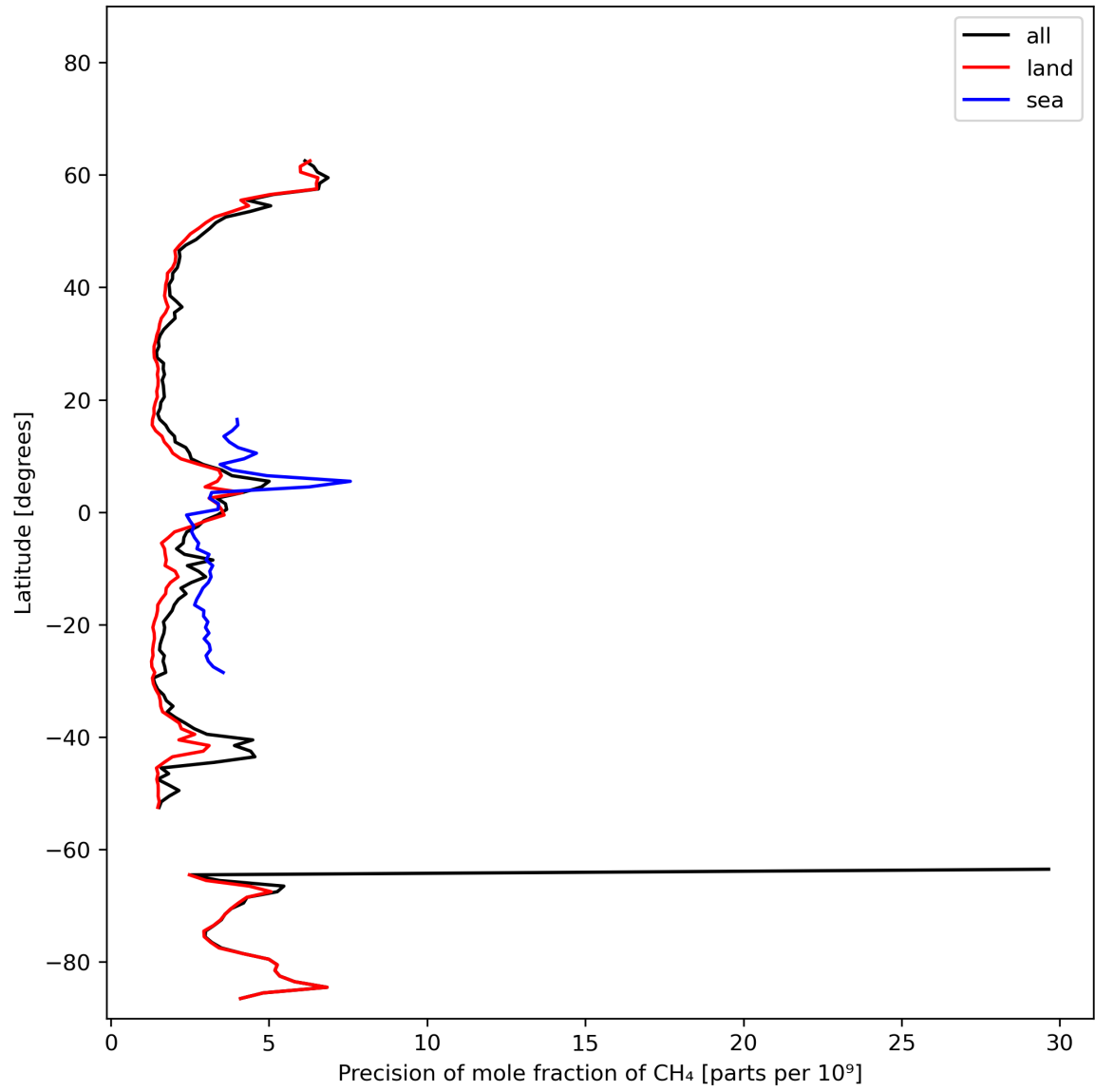
Figure 13: Zonal average of “Precision of mole fraction of CH 4 ” for 2023-10-27 to 2023-10-28.
