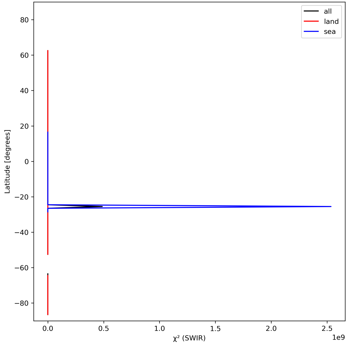
Figure 17: Zonal average of “ \chi^2 (SWIR)” for 2023-10-27 to 2023-10-28.
