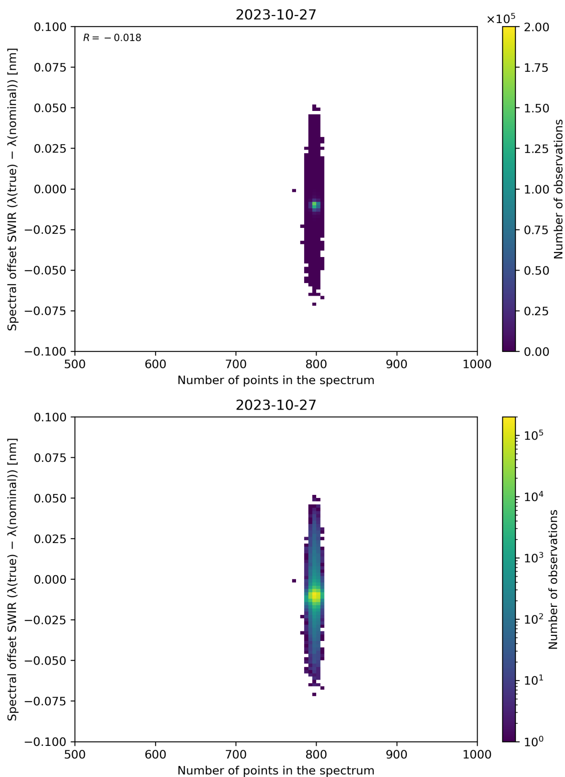
Figure 93: Scatter density plot of “Number of points in the spectrum” against “Spectral offset SWIR ( \lambda(\text{true}) - \lambda(\text{nominal}) )” for 2023-10-27 to 2023-10-28.
