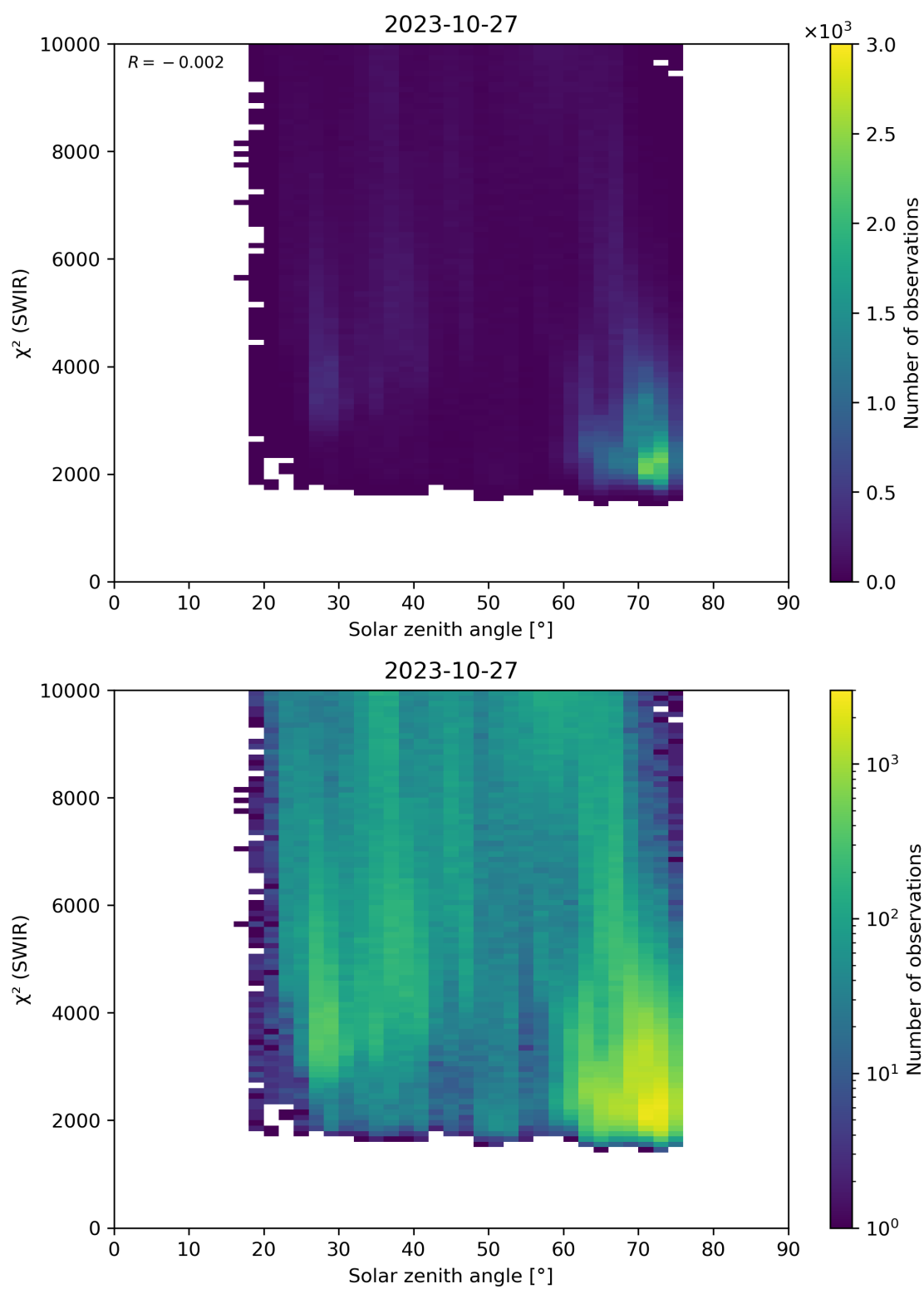
Figure 95: Scatter density plot of “Solar zenith angle” against “ \chi^2 (SWIR)” for 2023-10-27 to 2023-10-28.
