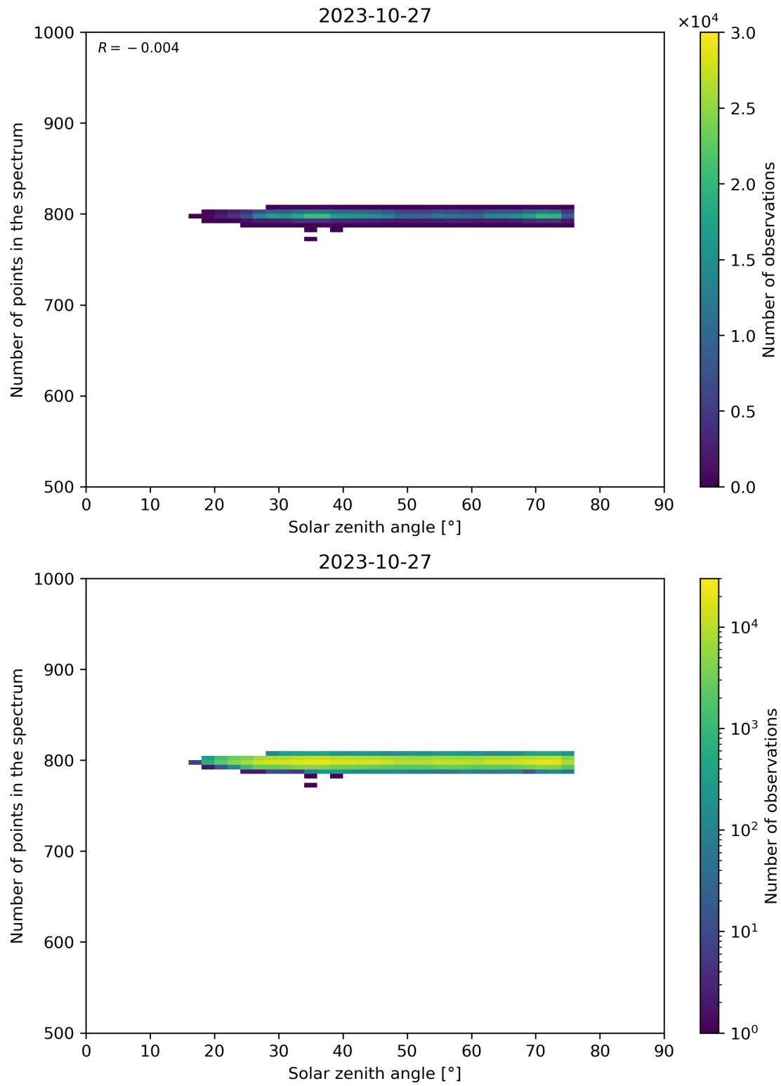
Figure 103: Scatter density plot of “Solar zenith angle” against “Number of points in the spectrum” for 2023-10-27 to 2023-10-28.
