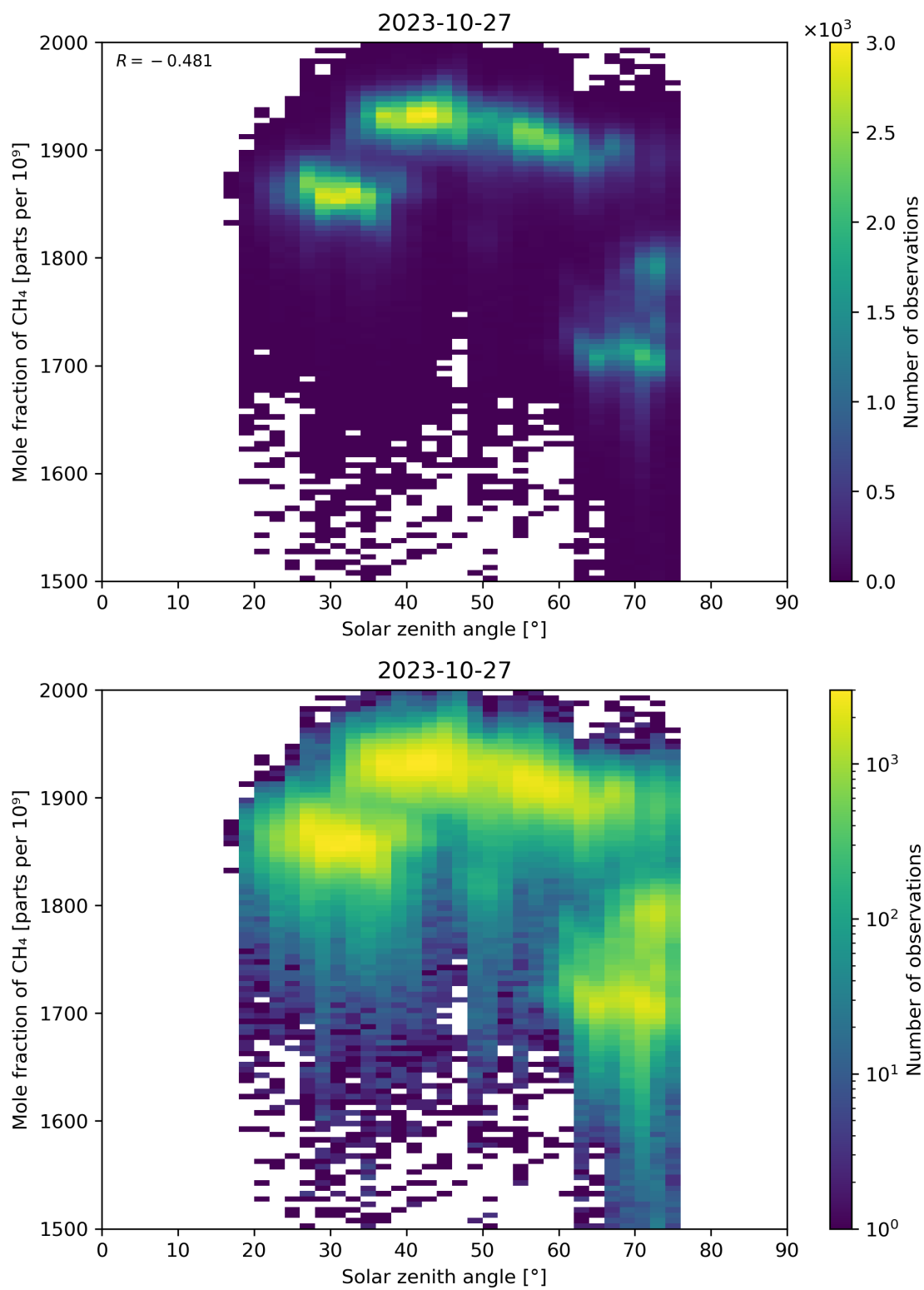
Figure 99: Scatter density plot of “Solar zenith angle” against “Mole fraction of CH 4 ” for 2023-10-27 to 2023-10-28.
