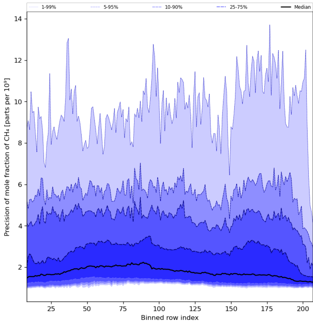
Figure 35: Along track statistics of “Precision of mole fraction of CH 4 ” for 2023-10-27 to 2023-10-28
