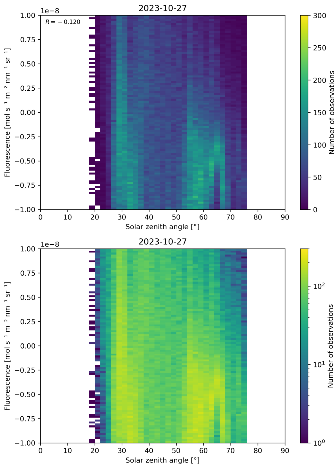
Figure 97: Scatter density plot of “Solar zenith angle” against “Fluorescence” for 2023-10-27 to 2023-10-28.
