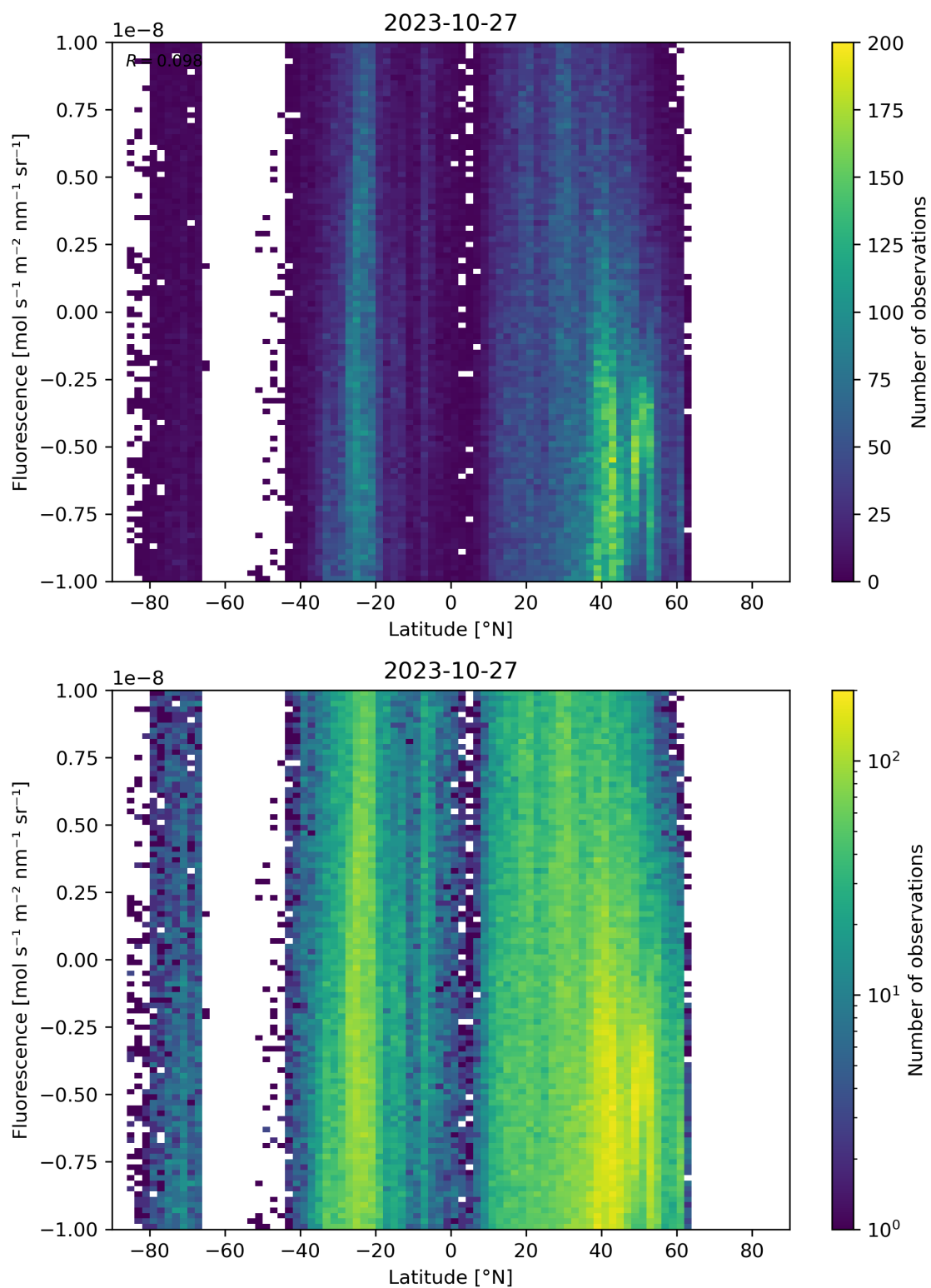
Figure 56: Scatter density plot of “Latitude” against “Fluorescence” for 2023-10-27 to 2023-10-28.
