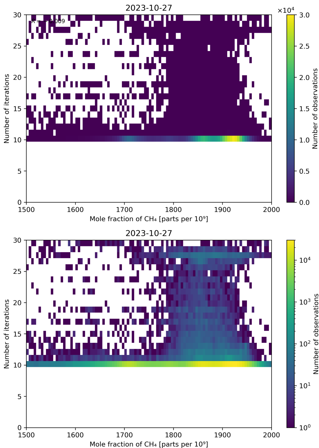
Figure 76: Scatter density plot of “Mole fraction of CH 4 ” against “Number of iterations” for 2023-10-27 to 2023-10-28.
