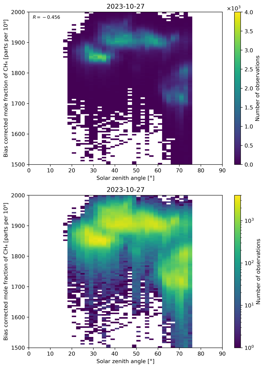
Figure 100: Scatter density plot of “Solar zenith angle” against “Bias corrected mole fraction of CH 4 ” for 2023-10-27 to 2023-10-28.
