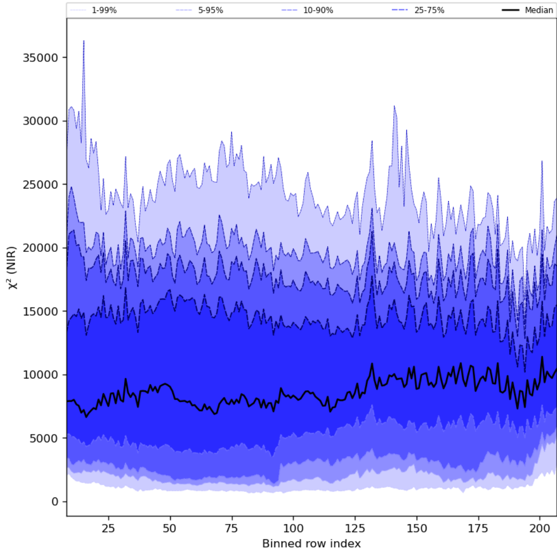
Figure 40: Along track statistics of " \chi^2 (NIR)" for 2023-10-27 to 2023-10-28
