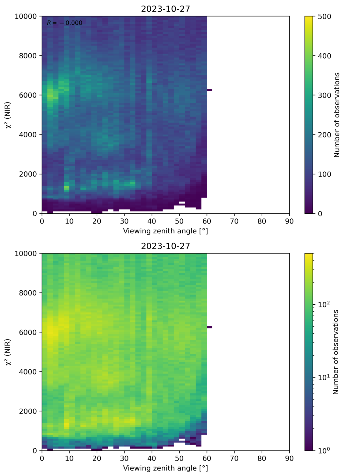
Figure 105: Scatter density plot of “Viewing zenith angle” against “ \chi^2 (NIR)” for 2023-10-27 to 2023-10-28.
