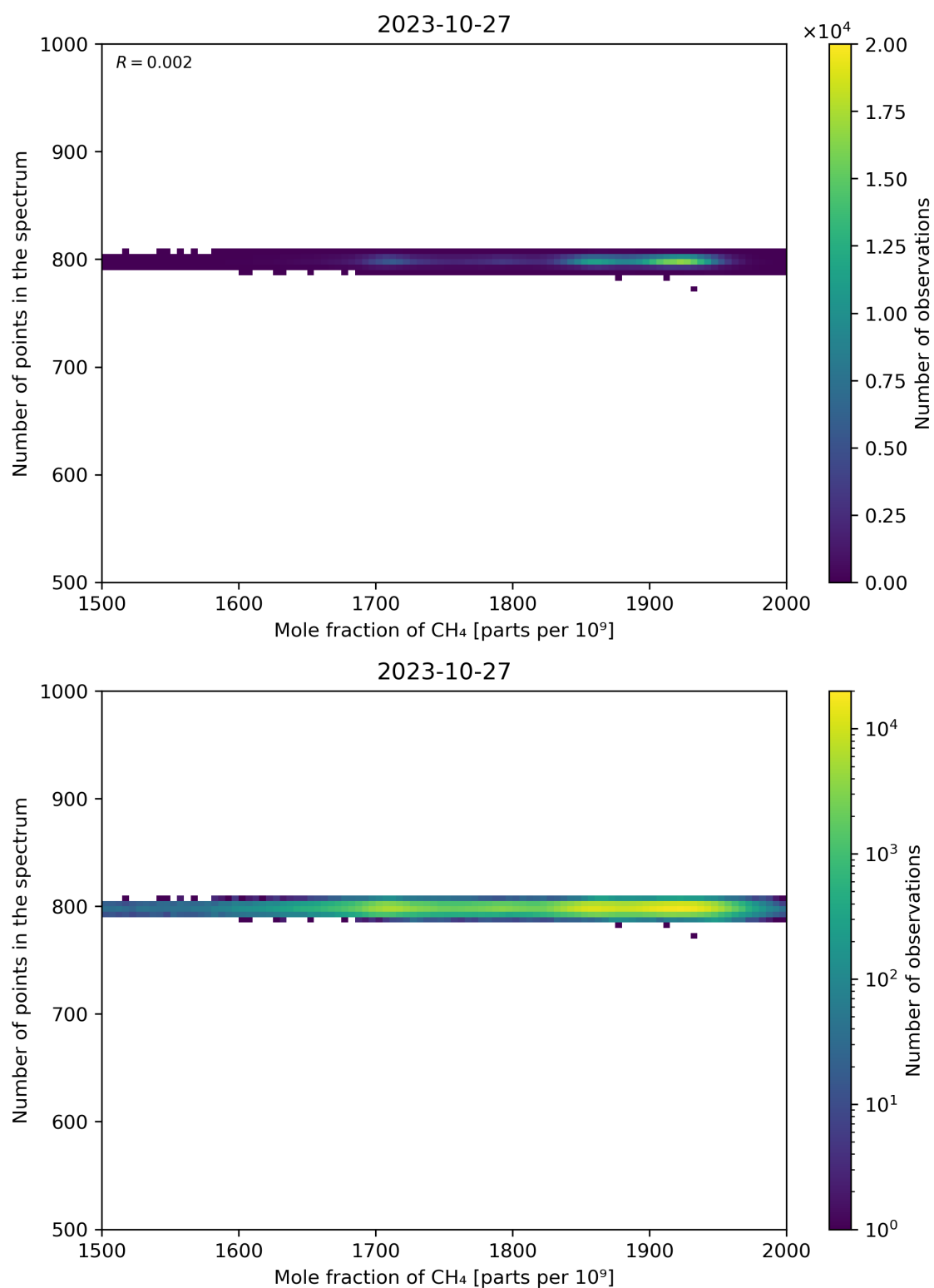
Figure 77: Scatter density plot of “Mole fraction of CH 4 ” against “Number of points in the spectrum” for 2023-10-27 to 2023-10-28.
