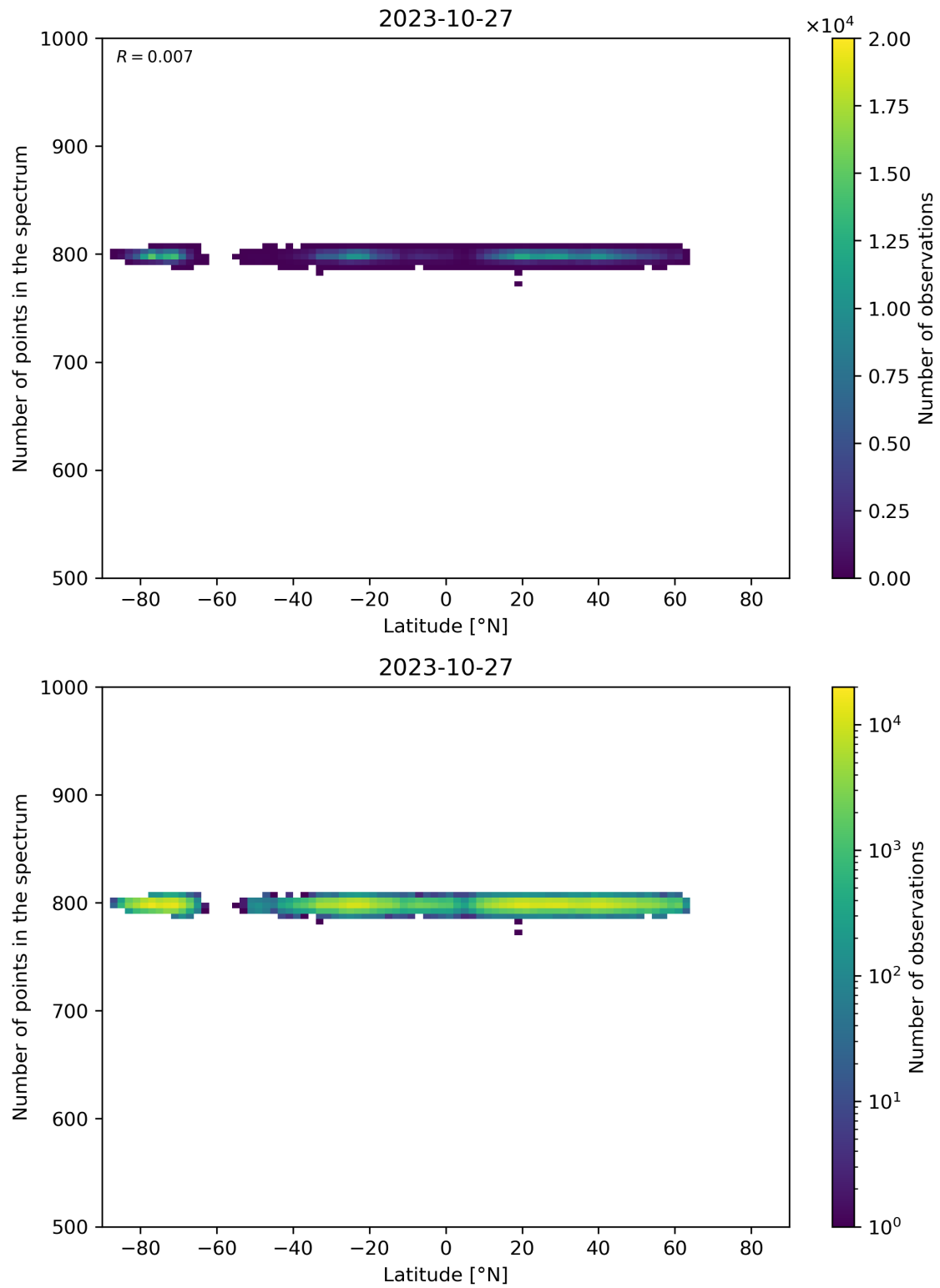
Figure 61: Scatter density plot of “Latitude” against “Number of points in the spectrum” for 2023-10-27 to 2023-10-28.
