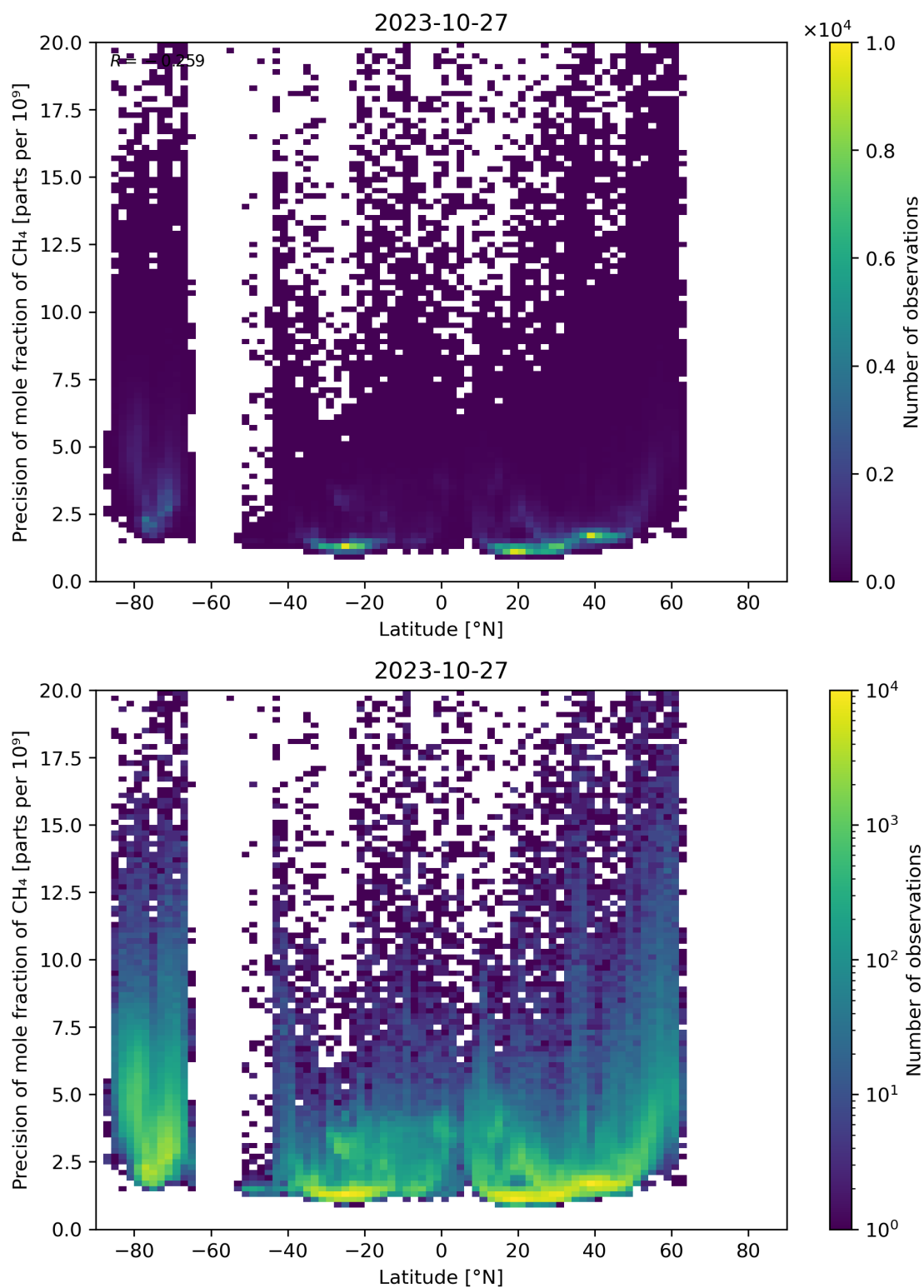
Figure 59: Scatter density plot of “Latitude” against “Precision of mole fraction of \text{CH}_4 ” for 2023-10-27 to 2023-10-28.
