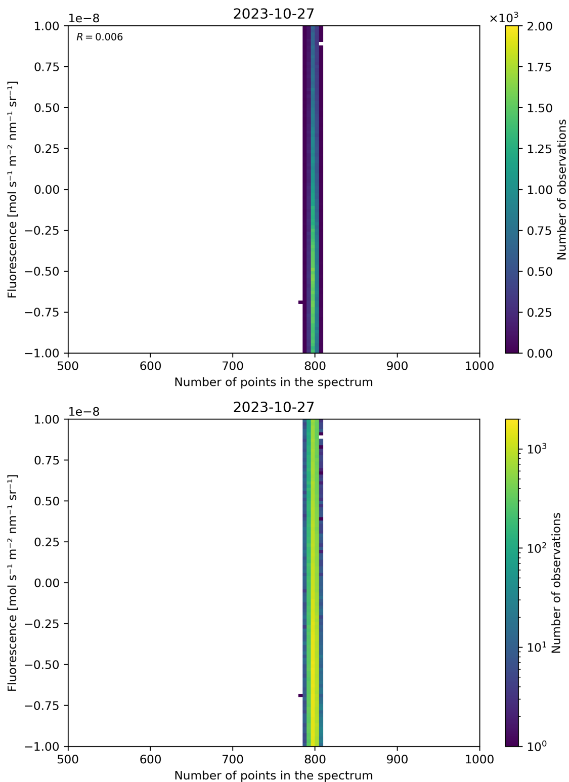
Figure 91: Scatter density plot of “Number of points in the spectrum” against “Fluorescence” for 2023-10-27 to 2023-10-28.
