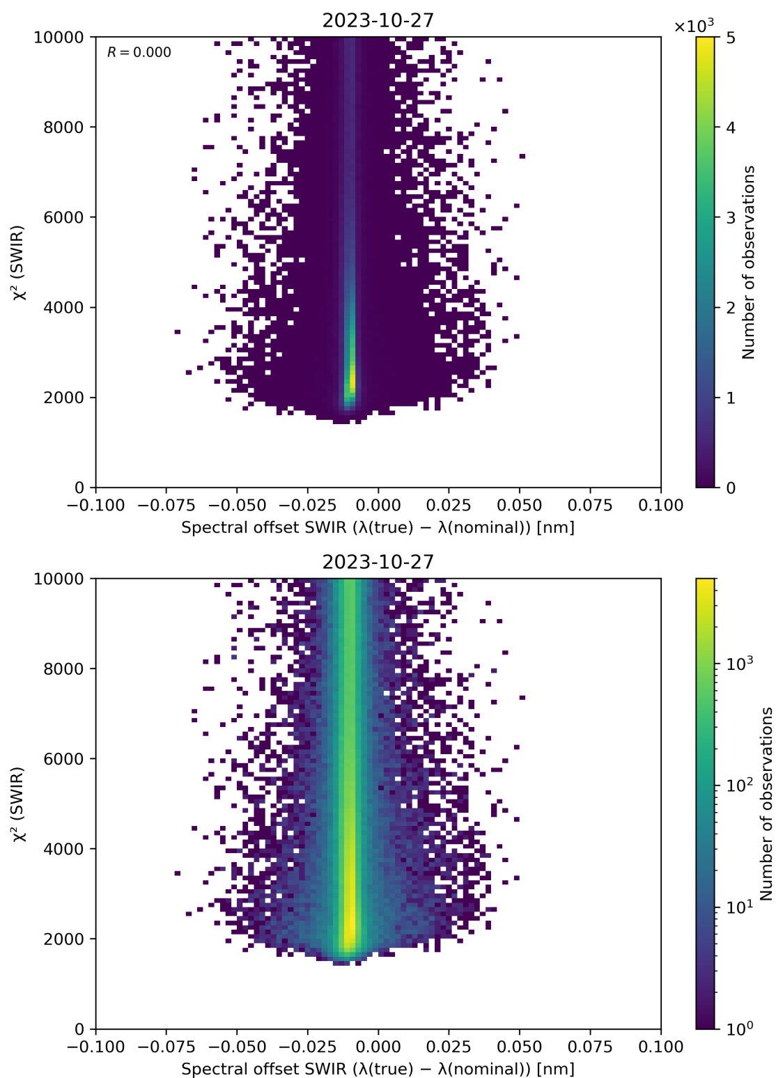
Figure 118: Scatter density plot of “Spectral offset SWIR ( \lambda(\text{true}) - \lambda(\text{nominal}) )” against “ \chi^2 (SWIR)” for 2023-10-27 to 2023-10-28.
