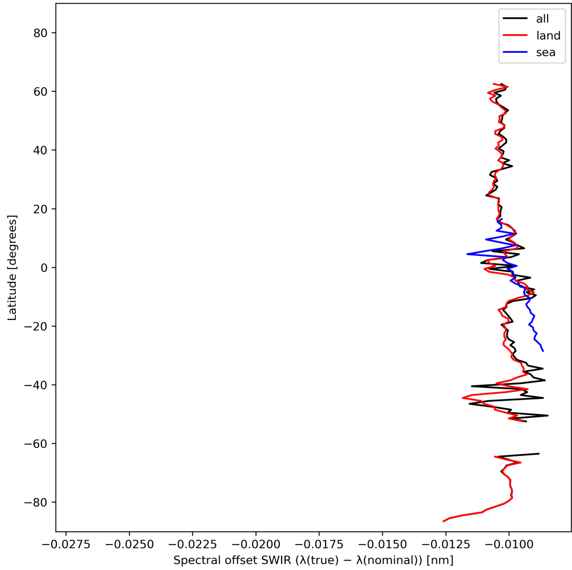
Figure 16: Zonal average of “Spectral offset SWIR ( \lambda(\text{true}) - \lambda(\text{nominal}) )” for 2023-10-27 to 2023-10-28.
