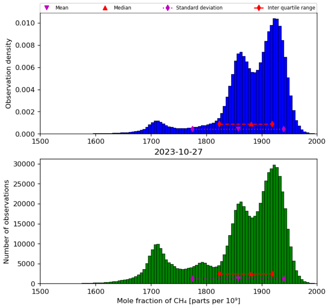
Figure 23: Histogram of “Mole fraction of CH 4 ” for 2023-10-27 to 2023-10-28
