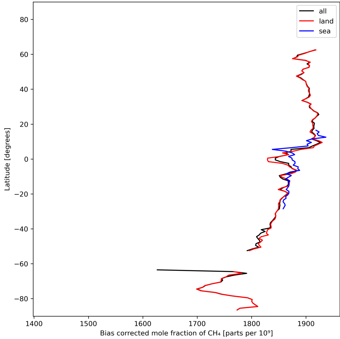
Figure 14: Zonal average of “Bias corrected mole fraction of CH 4 ” for 2023-10-27 to 2023-10-28.
