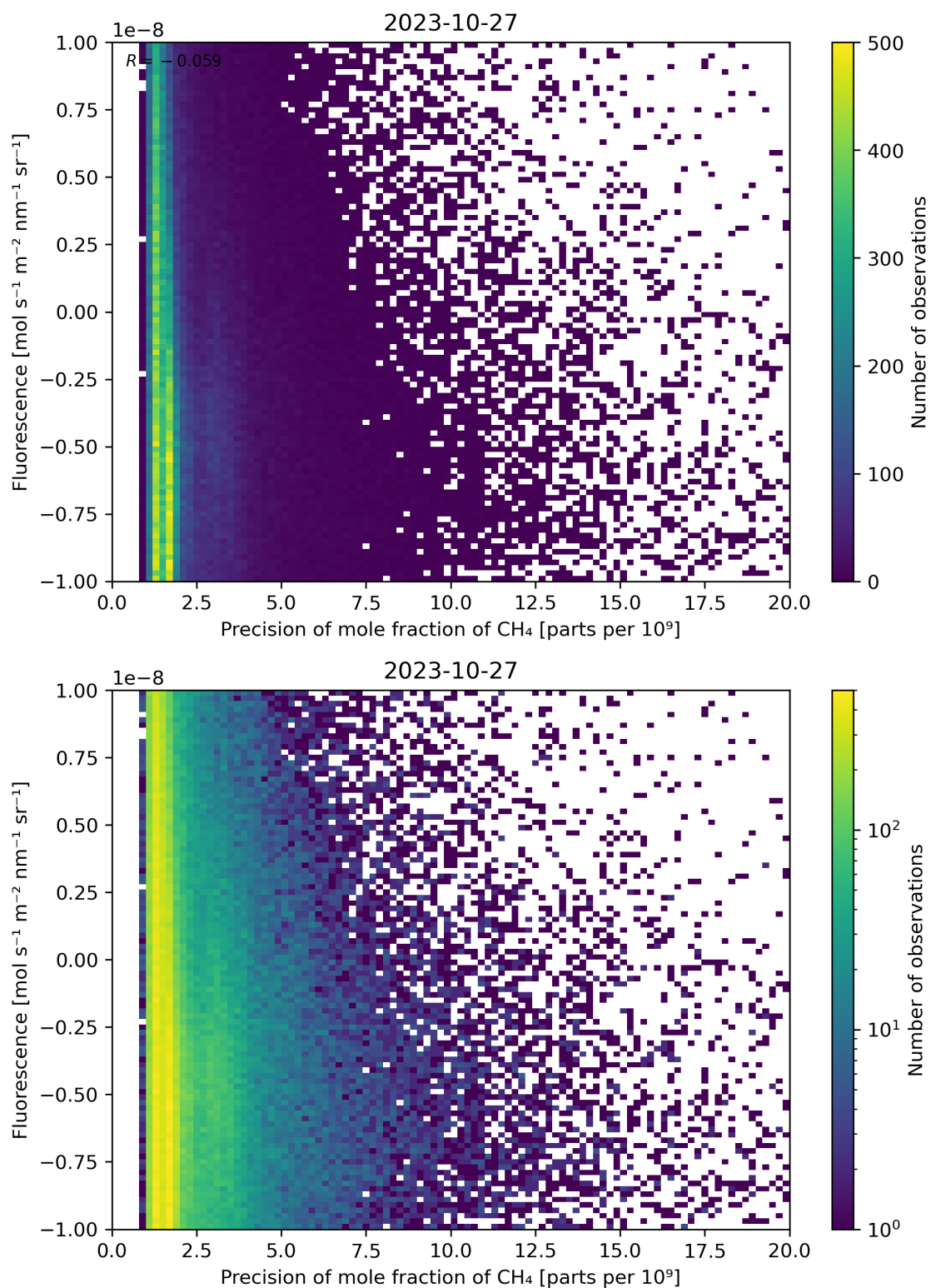
Figure 81: Scatter density plot of “Precision of mole fraction of \text{CH}_4 ” against “Fluorescence” for 2023-10-27 to 2023-10-28.
