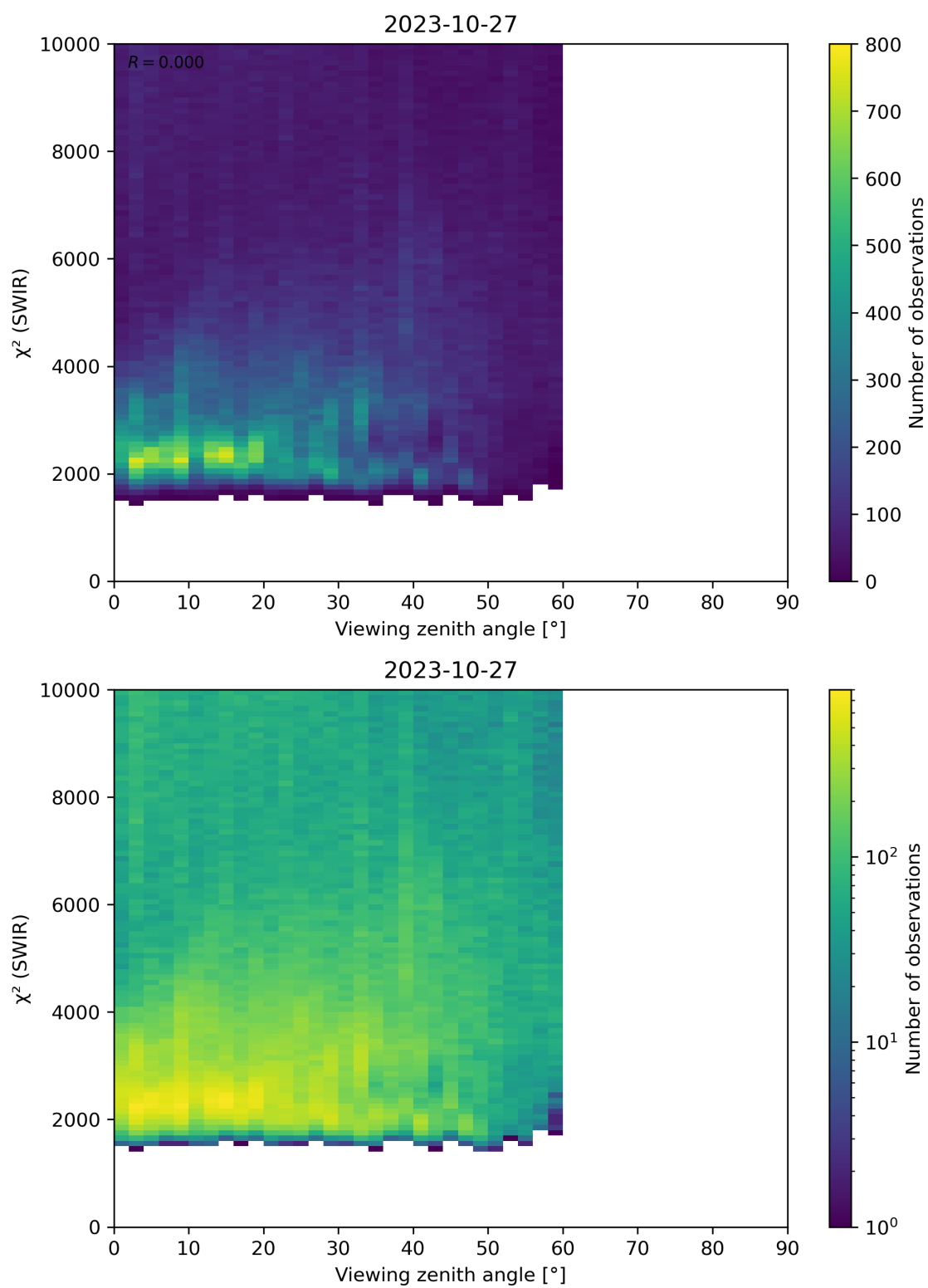
Figure 106: Scatter density plot of “Viewing zenith angle” against “ \chi^2 (SWIR)” for 2023-10-27 to 2023-10-28.
