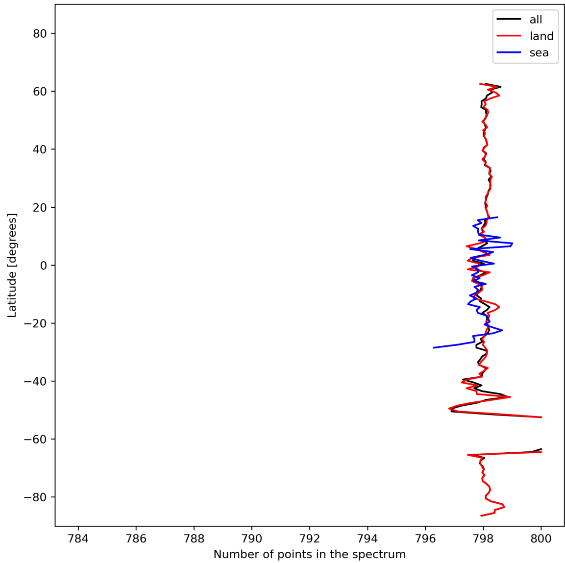
Figure 15: Zonal average of “Number of points in the spectrum” for 2023-10-27 to 2023-10-28.
