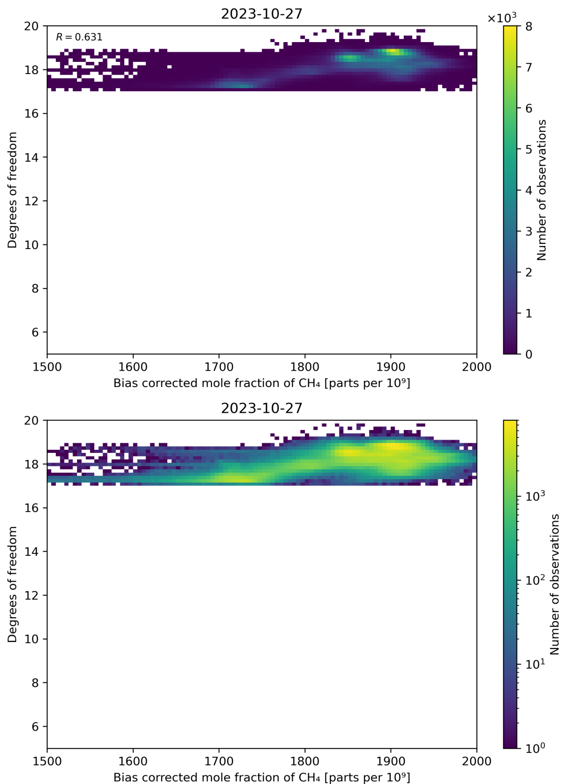
Figure 65: Scatter density plot of “Bias corrected mole fraction of CH 4 ” against “Degrees of freedom” for 2023-10-27 to 2023-10-28.
