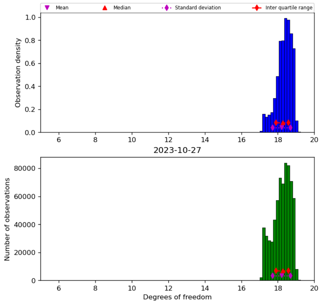
Figure 30: Histogram of “Degrees of freedom” for 2023-10-27 to 2023-10-28
