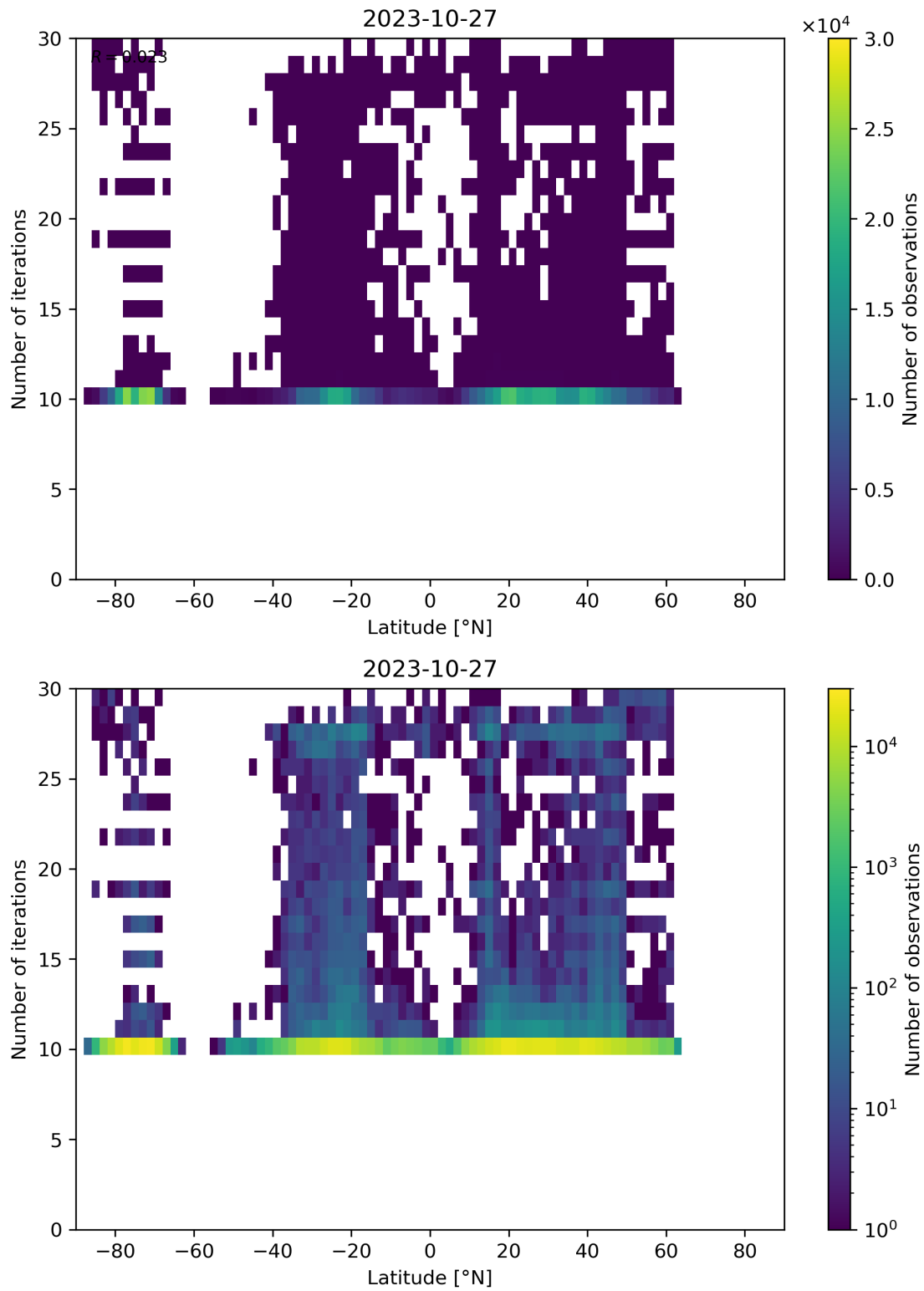
Figure 60: Scatter density plot of “Latitude” against “Number of iterations” for 2023-10-27 to 2023-10-28.
