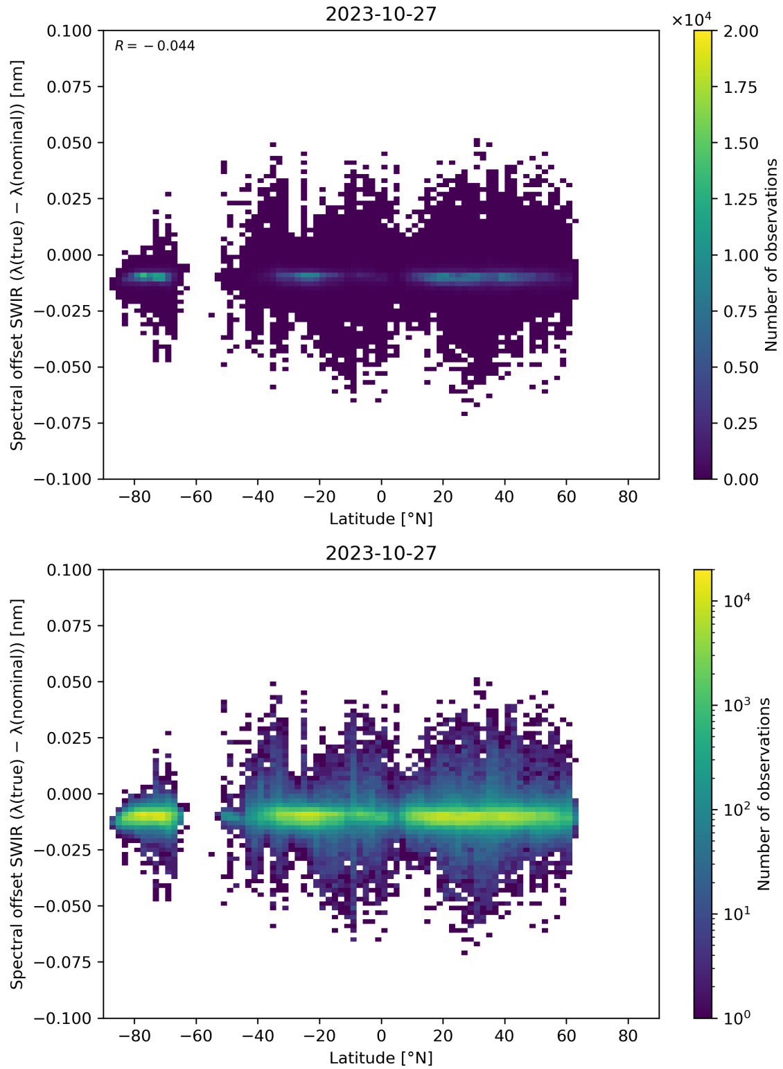
Figure 62: Scatter density plot of “Latitude” against “Spectral offset SWIR ( \lambda(\text{true}) - \lambda(\text{nominal}) )” for 2023-10-27 to 2023-10-28.
