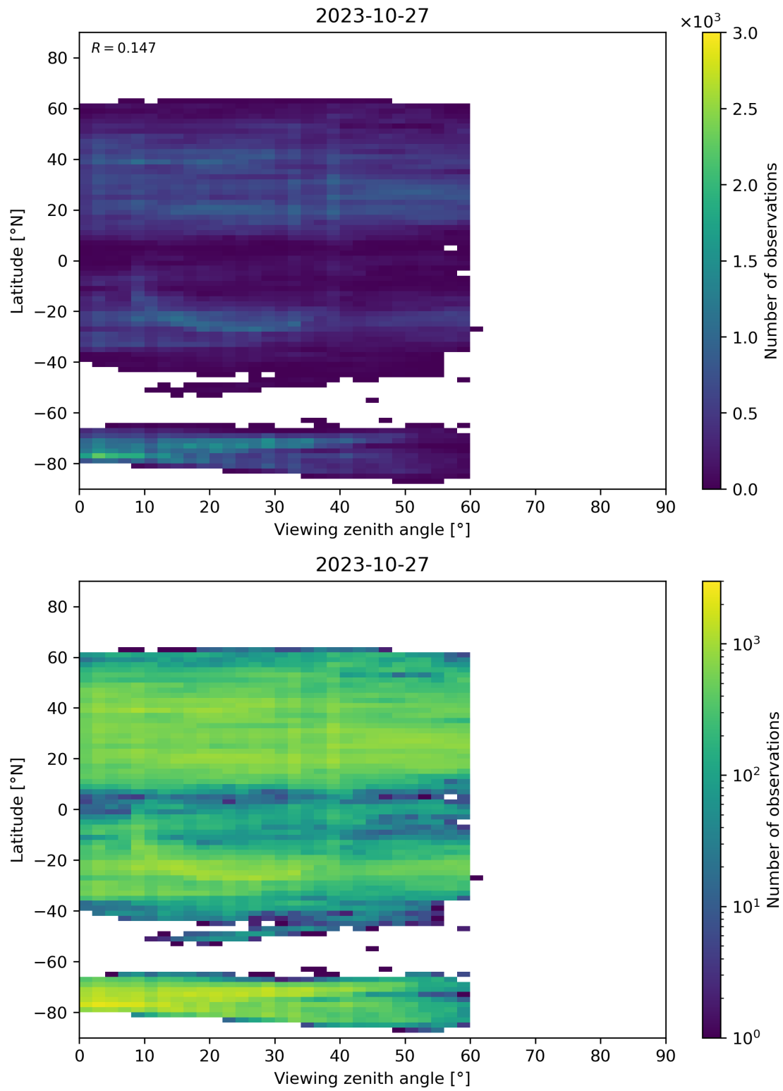
Figure 109: Scatter density plot of “Viewing zenith angle” against “Latitude” for 2023-10-27 to 2023-10-28.
