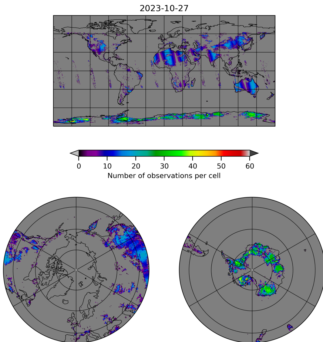
Figure 10: Map of the number of observations for 2023-10-27 to 2023-10-28
