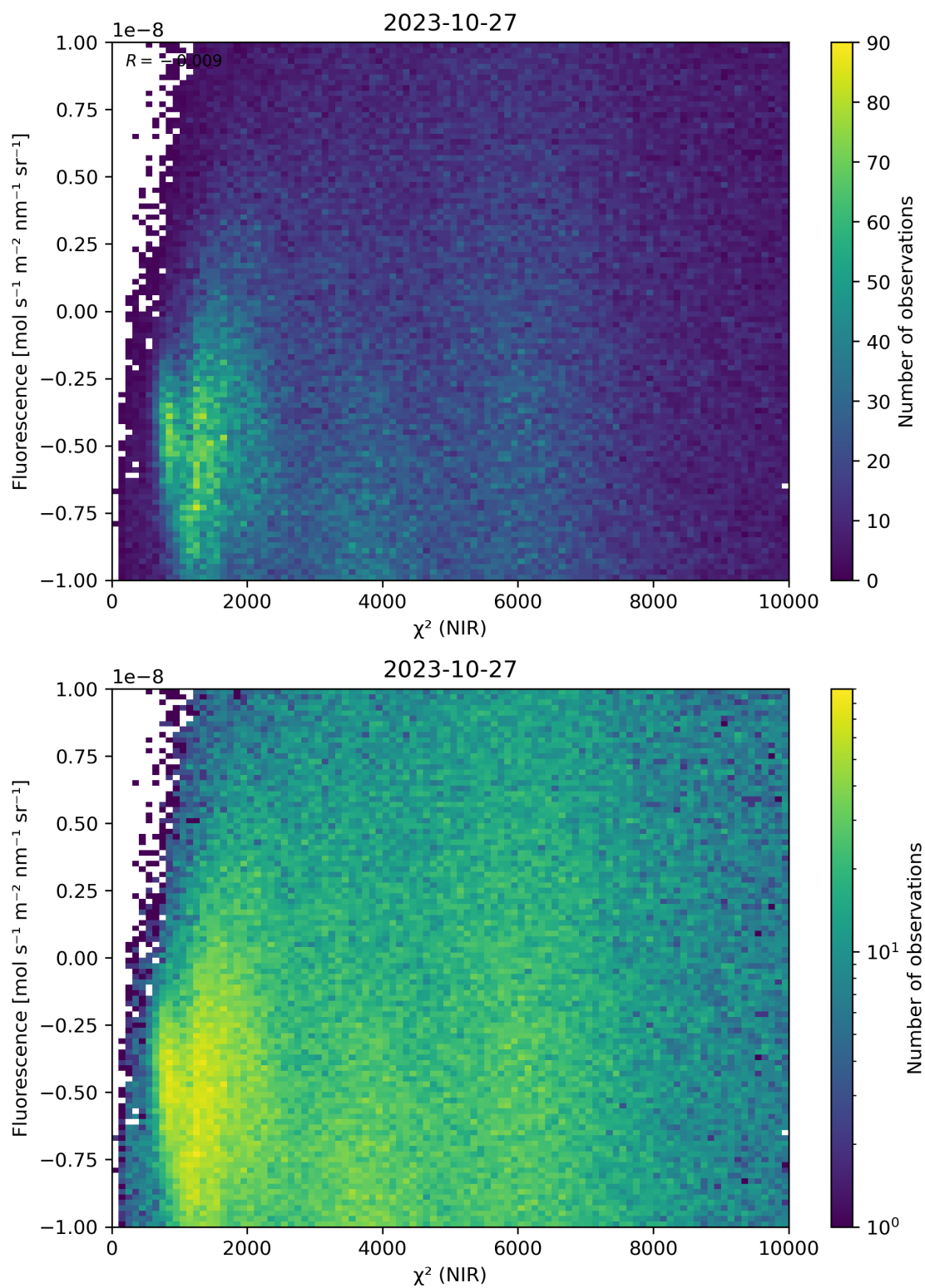
Figure 45: Scatter density plot of “ \chi^2 (NIR)” against “Fluorescence” for 2023-10-27 to 2023-10-28.
