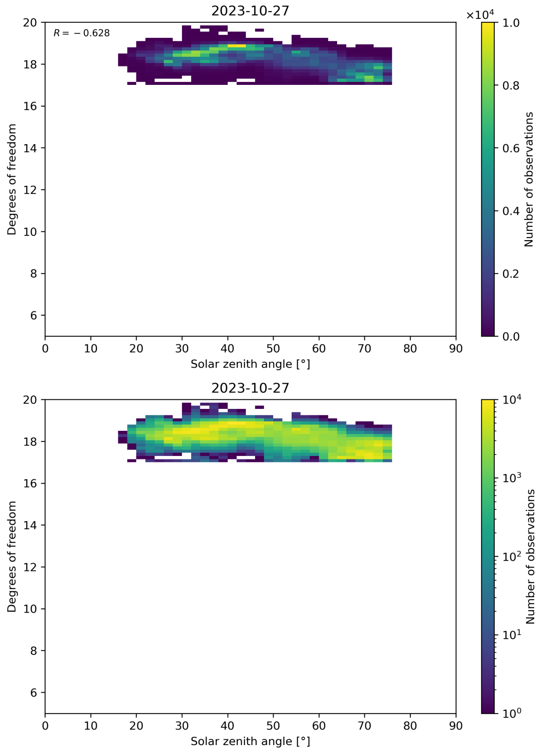
Figure 96: Scatter density plot of “Solar zenith angle” against “Degrees of freedom” for 2023-10-27 to 2023-10-28.
