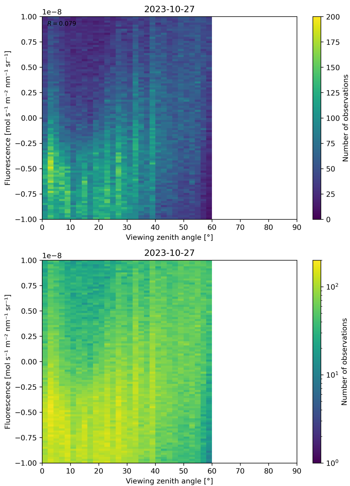
Figure 108: Scatter density plot of “Viewing zenith angle” against “Fluorescence” for 2023-10-27 to 2023-10-28.
