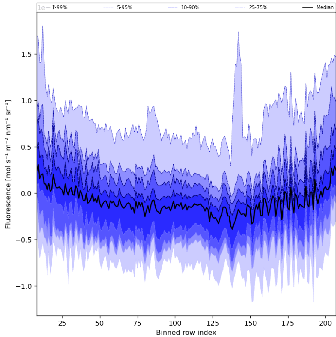
Figure 43: Along track statistics of “Fluorescence” for 2023-10-27 to 2023-10-28
