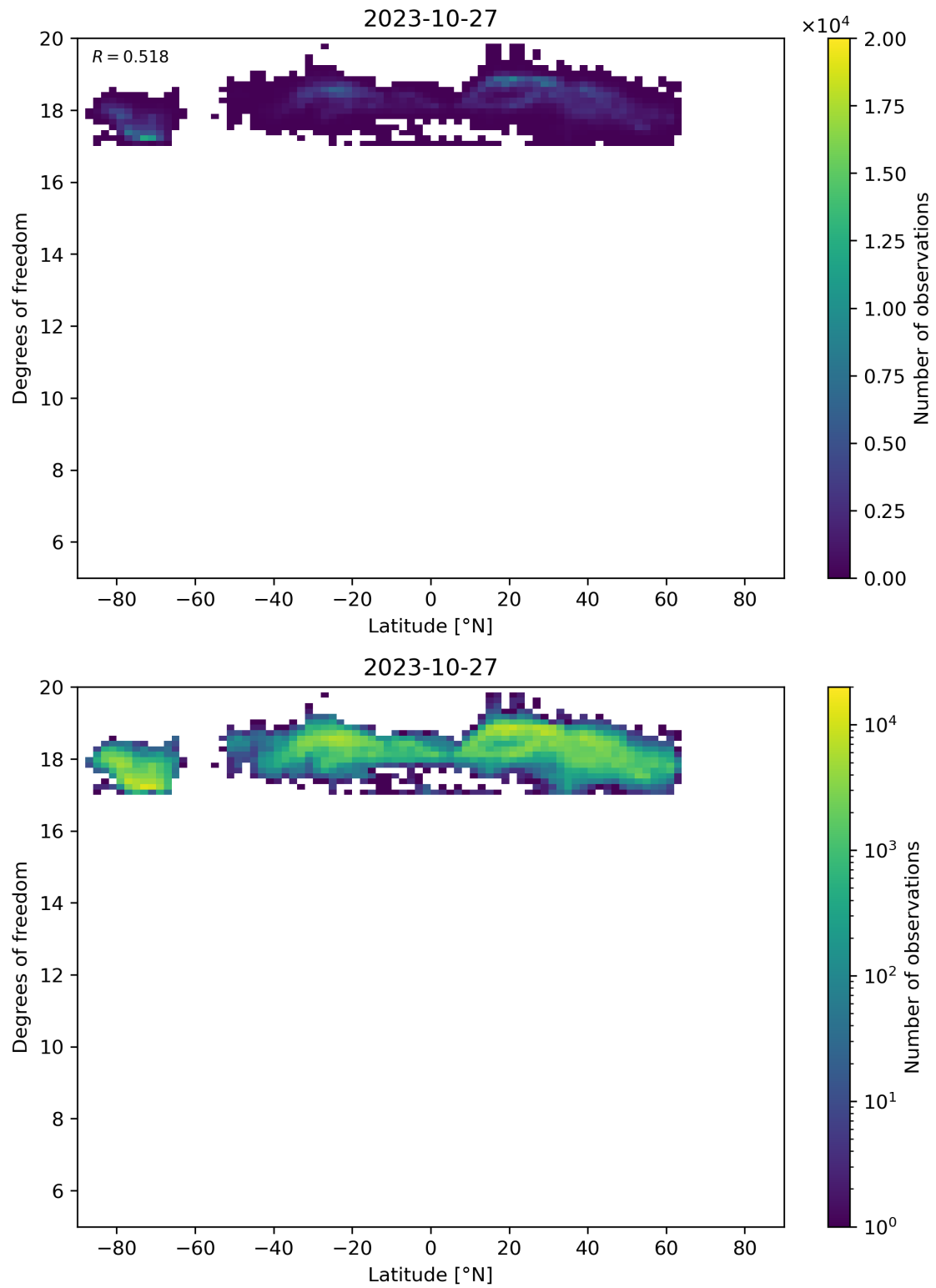
Figure 55: Scatter density plot of “Latitude” against “Degrees of freedom” for 2023-10-27 to 2023-10-28.
