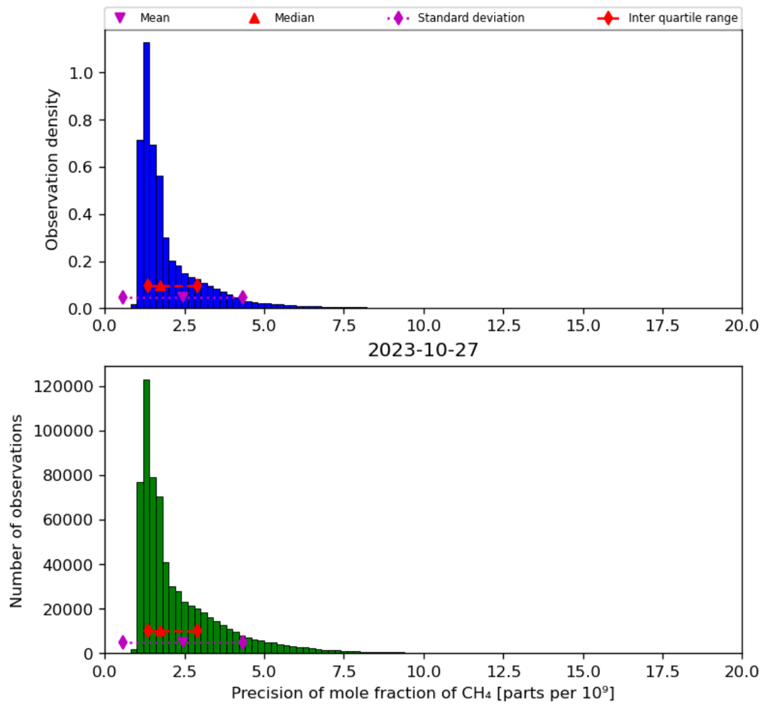
Figure 24: Histogram of “Precision of mole fraction of CH 4 ” for 2023-10-27 to 2023-10-28
