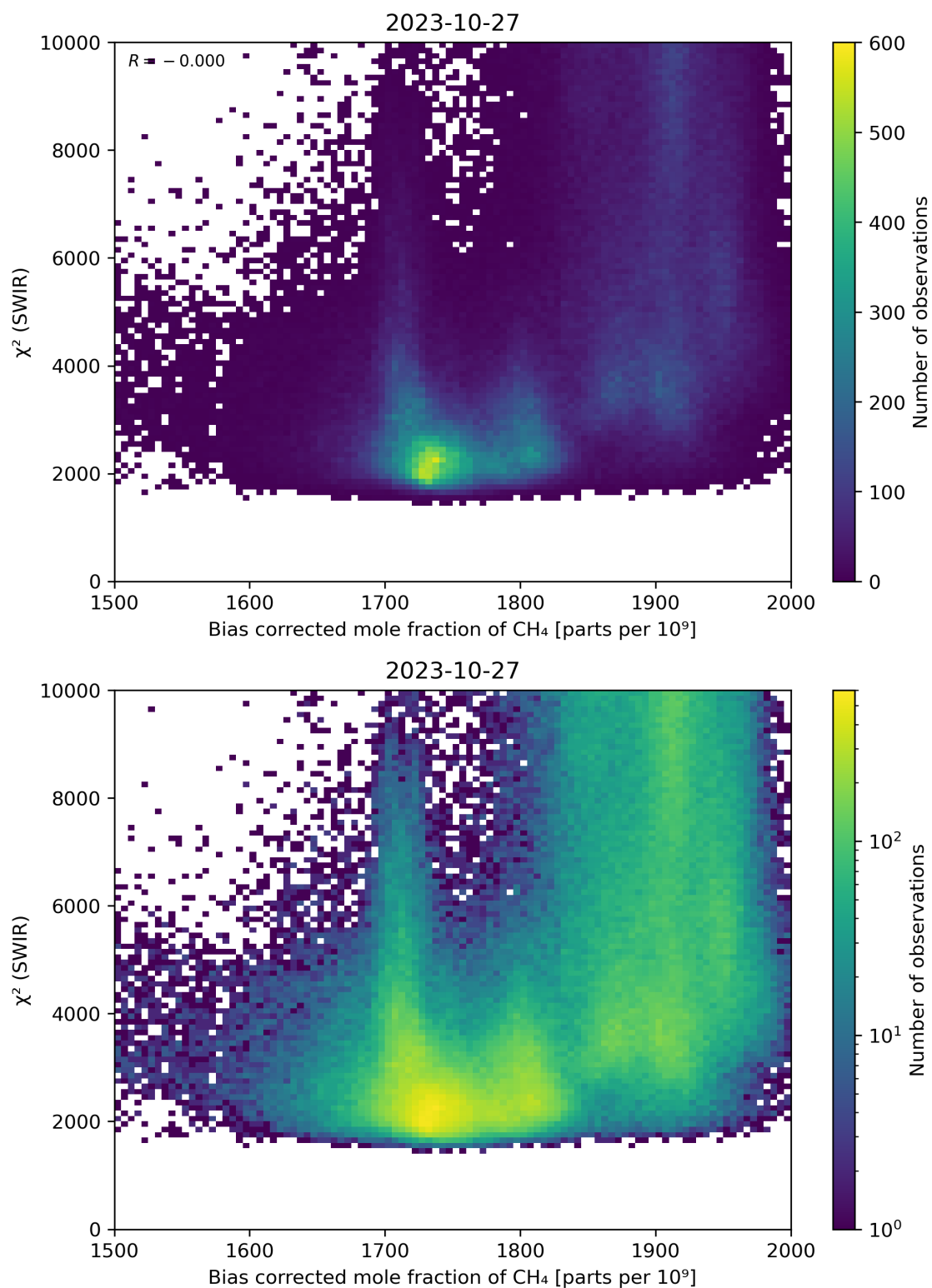
Figure 64: Scatter density plot of “Bias corrected mole fraction of CH 4 ” against “ \chi^2 (SWIR)” for 2023-10-27 to 2023-10-28.
