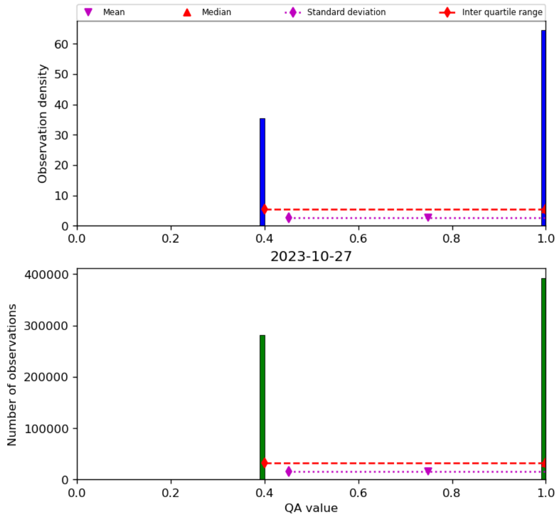
Figure 22: Histogram of “QA value” for 2023-10-27 to 2023-10-28
