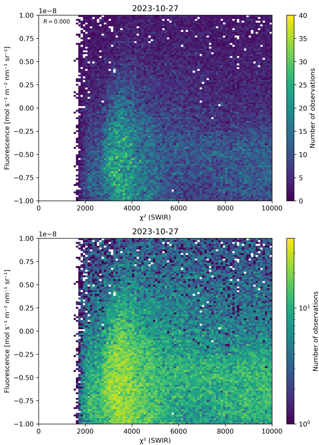
Figure 49: Scatter density plot of “ \chi^2 (SWIR)” against “Fluorescence” for 2023-10-27 to 2023-10-28.
