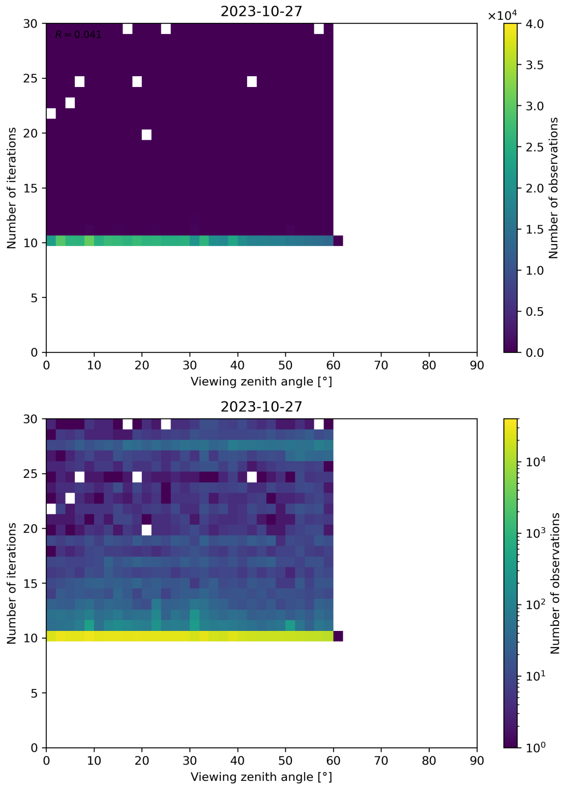
Figure 113: Scatter density plot of “Viewing zenith angle” against “Number of iterations” for 2023-10-27 to 2023-10-28.
