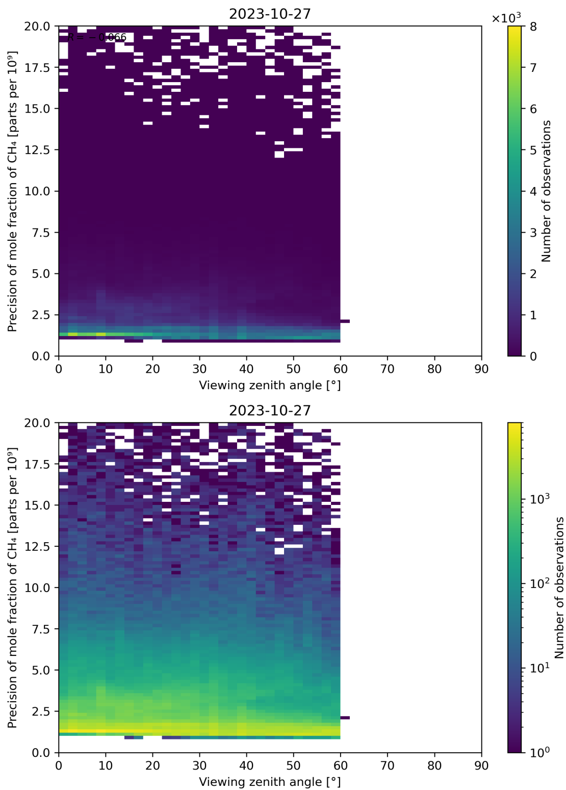
Figure 112: Scatter density plot of “Viewing zenith angle” against “Precision of mole fraction of CH 4 ” for 2023-10-27 to 2023-10-28.
