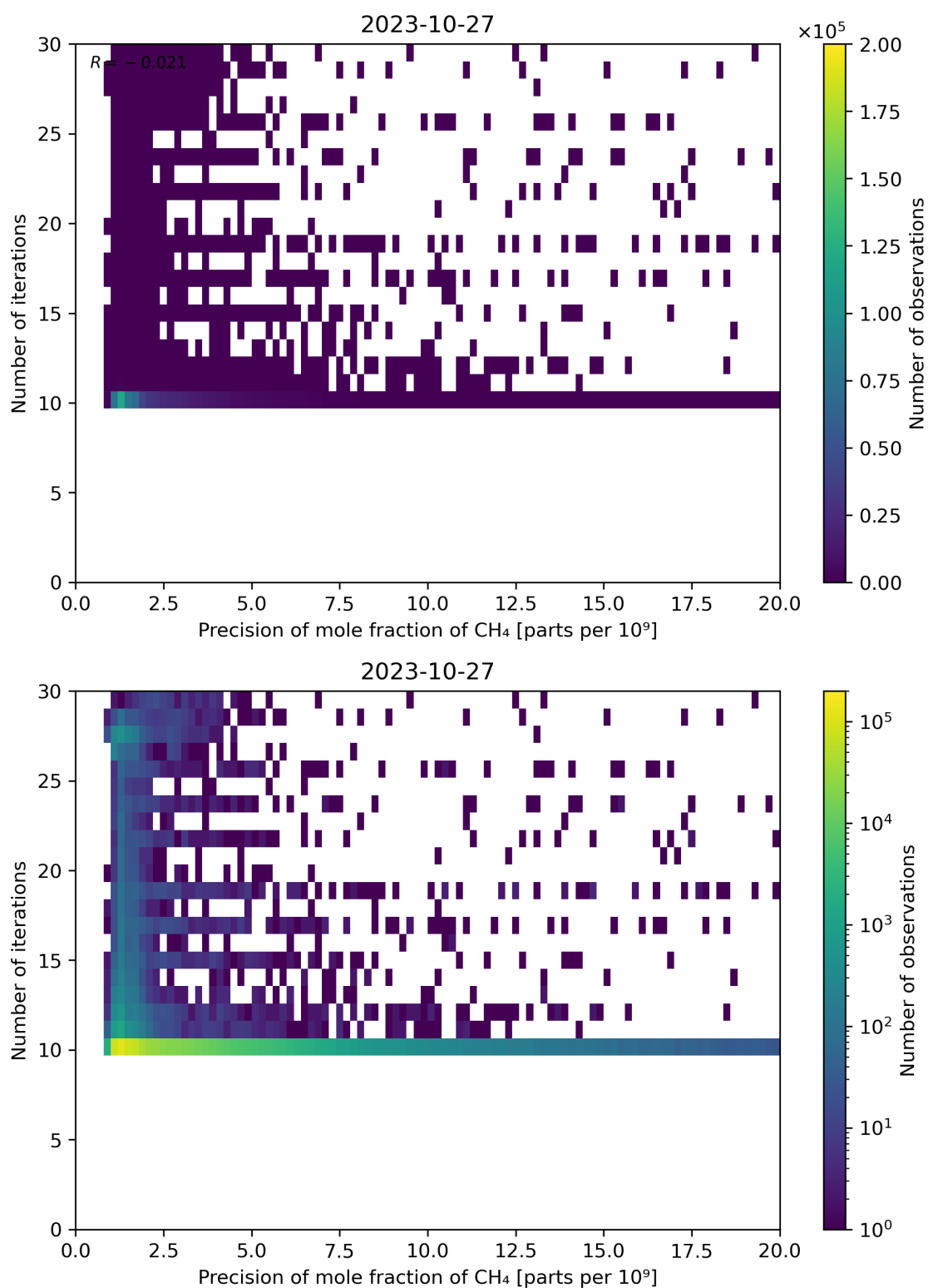
Figure 83: Scatter density plot of “Precision of mole fraction of CH 4 ” against “Number of iterations” for 2023-10-27 to 2023-10-28.
