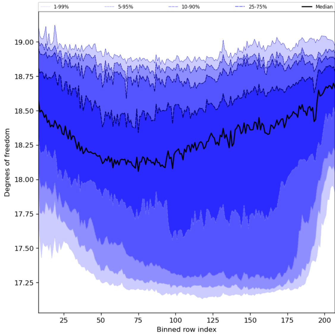
Figure 41: Along track statistics of “Degrees of freedom” for 2023-10-27 to 2023-10-28
