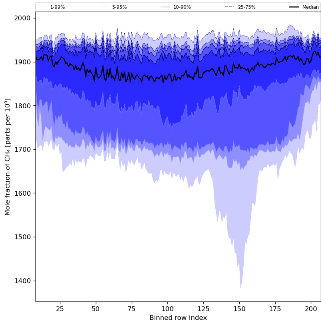
Figure 34: Along track statistics of “Mole fraction of CH 4 ” for 2023-10-27 to 2023-10-28
