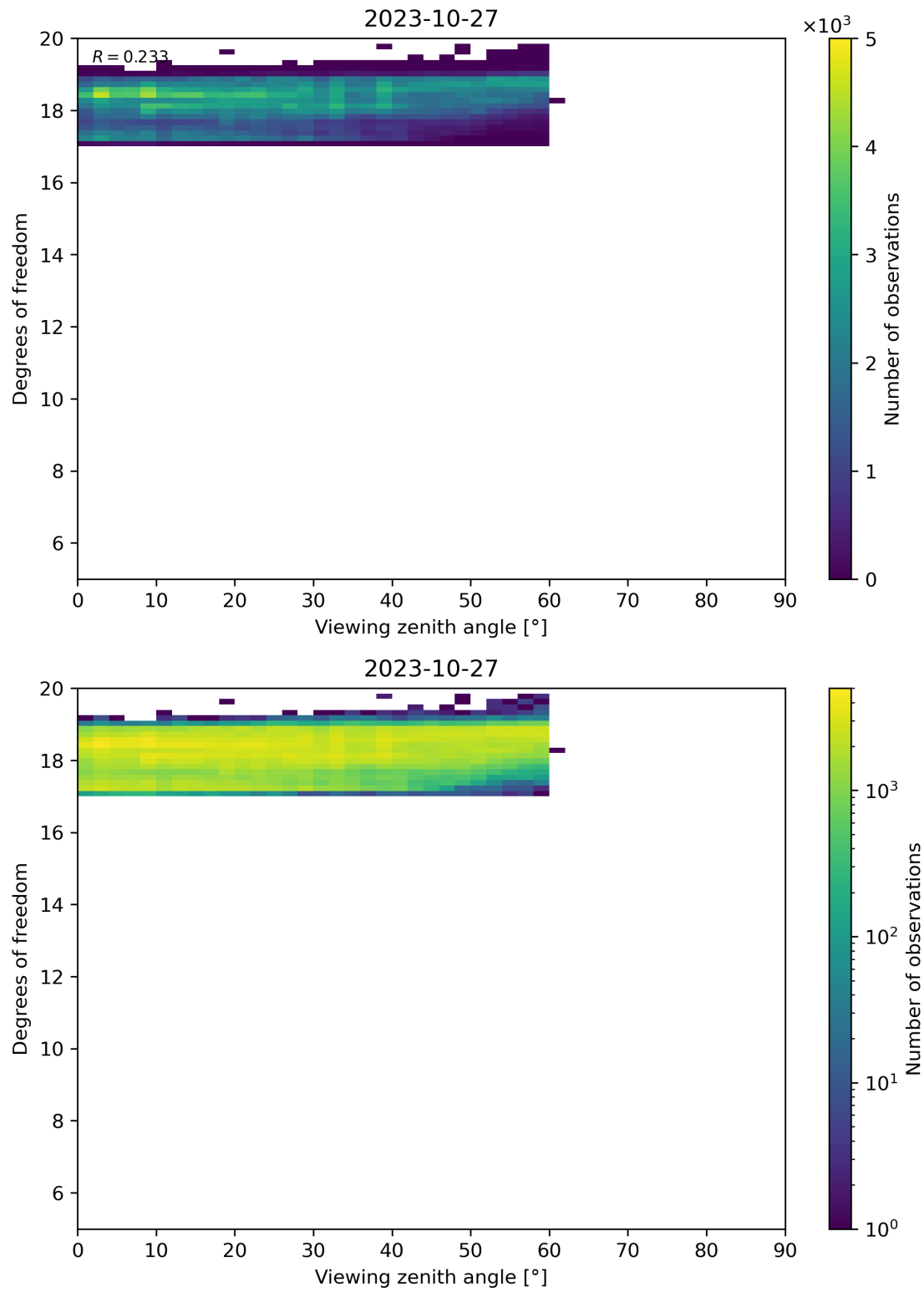
Figure 107: Scatter density plot of “Viewing zenith angle” against “Degrees of freedom” for 2023-10-27 to 2023-10-28.
