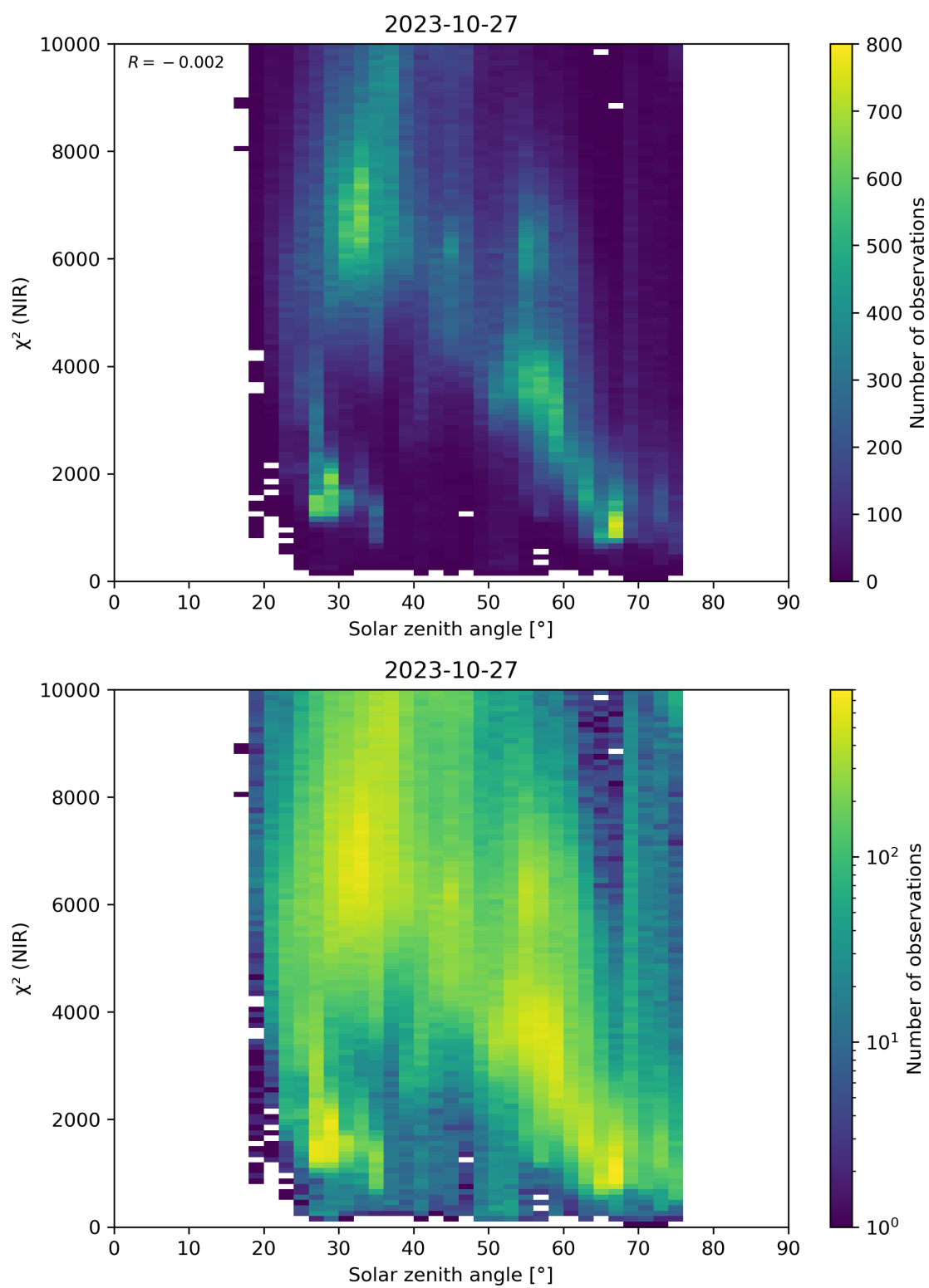
Figure 94: Scatter density plot of “Solar zenith angle” against “ \chi^2 (NIR)” for 2023-10-27 to 2023-10-28.
