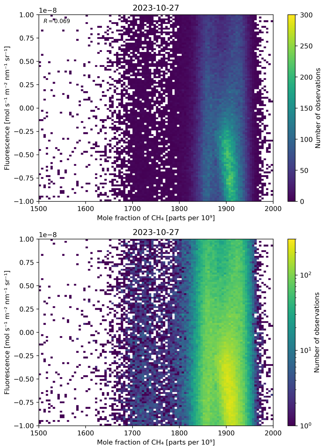
Figure 73: Scatter density plot of “Mole fraction of \text{CH}_4 ” against “Fluorescence” for 2023-10-27 to 2023-10-28.
