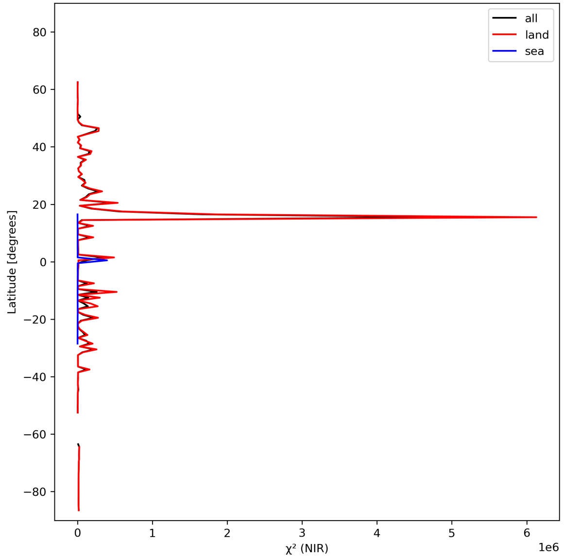
Figure 18: Zonal average of “ \chi^2 (NIR)” for 2023-10-27 to 2023-10-28.
