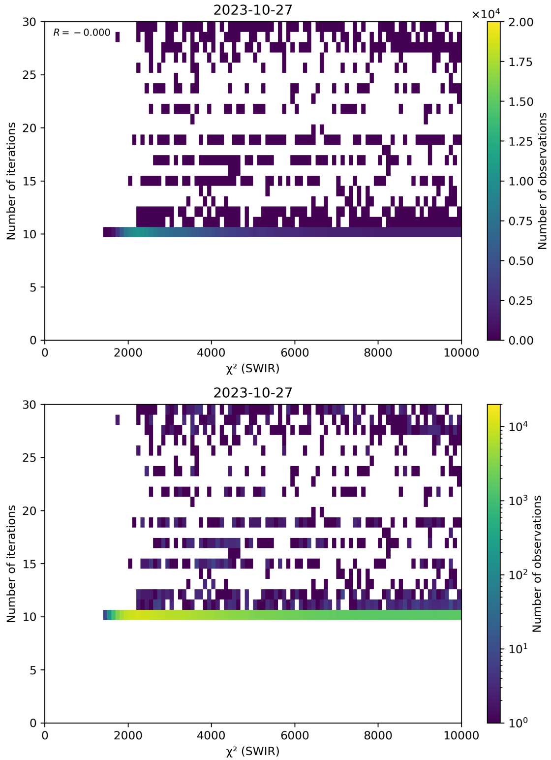
Figure 50: Scatter density plot of “ \chi^2 (SWIR)” against “Number of iterations” for 2023-10-27 to 2023-10-28.
