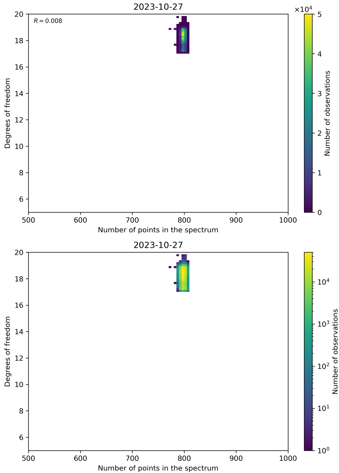
Figure 90: Scatter density plot of “Number of points in the spectrum” against “Degrees of freedom” for 2023-10-27 to 2023-10-28.
