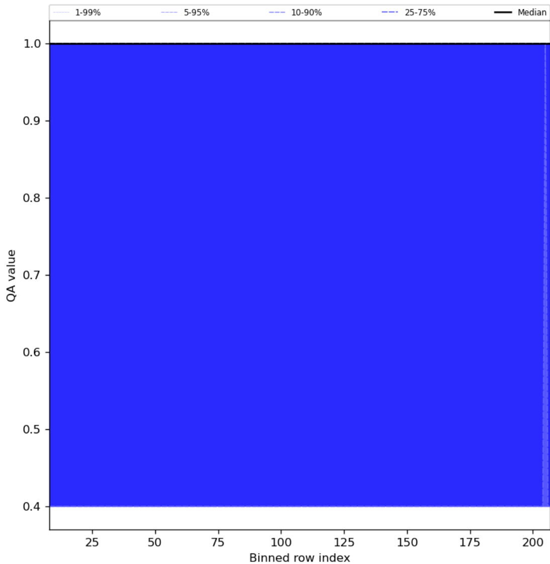
Figure 33: Along track statistics of “QA value” for 2023-10-27 to 2023-10-28
