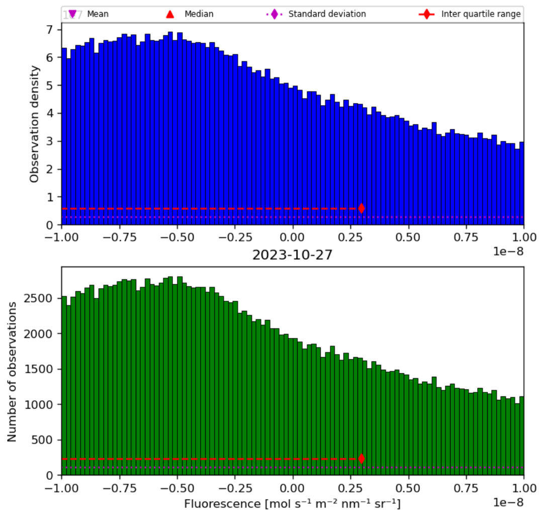
Figure 32: Histogram of “Fluorescence” for 2023-10-27 to 2023-10-28
