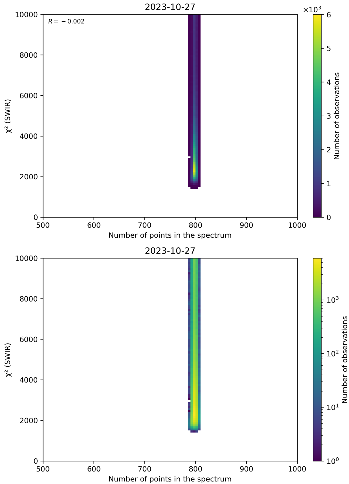
Figure 89: Scatter density plot of “Number of points in the spectrum” against “ \chi^2 (SWIR)” for 2023-10-27 to 2023-10-28.
