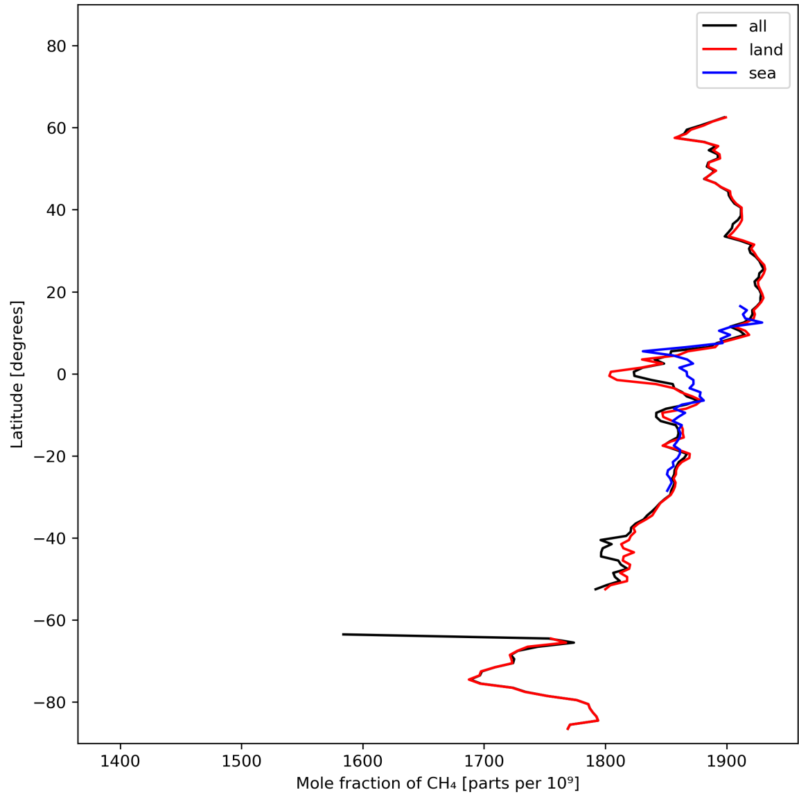
Figure 12: Zonal average of “Mole fraction of CH 4 ” for 2023-10-27 to 2023-10-28.
