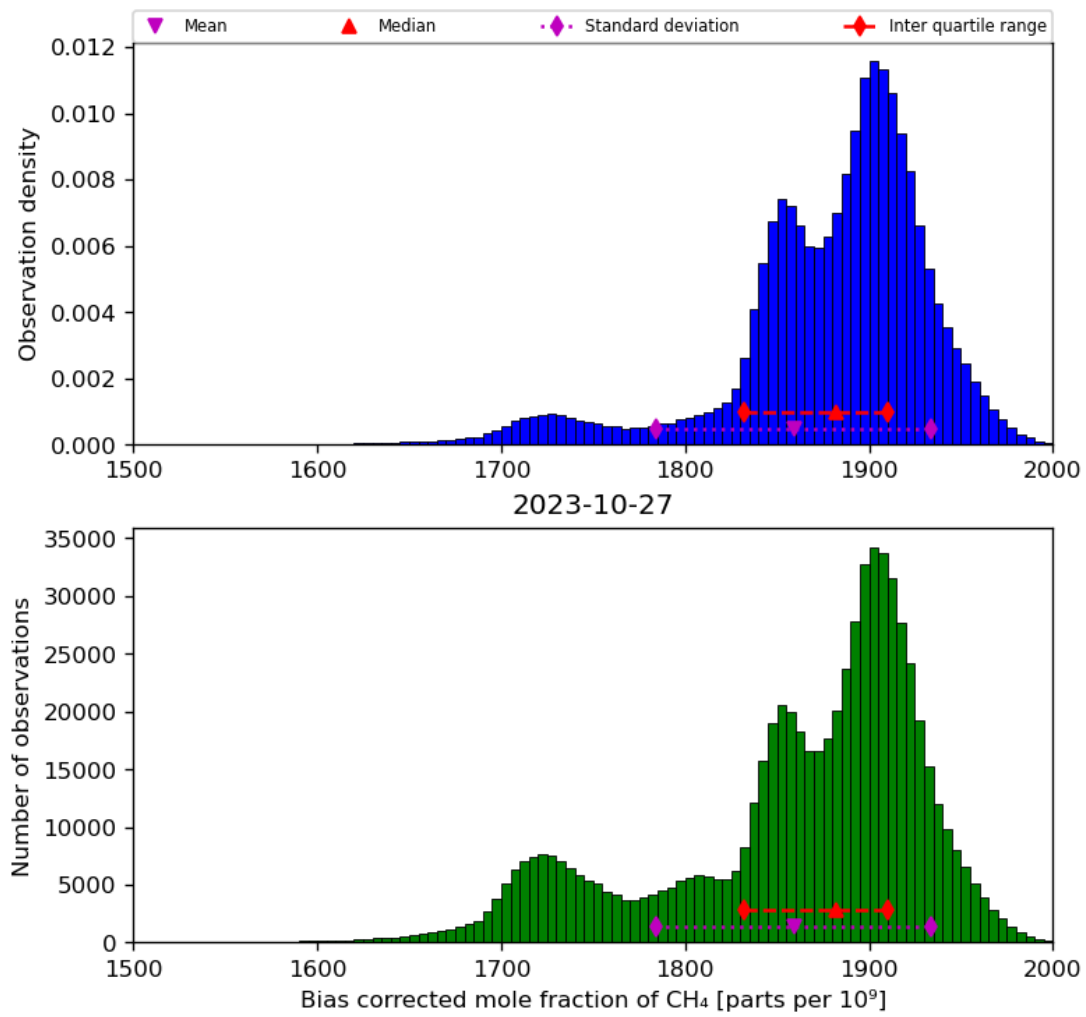
Figure 25: Histogram of “Bias corrected mole fraction of CH 4 ” for 2023-10-27 to 2023-10-28
