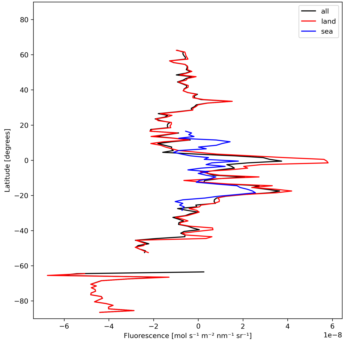
Figure 21: Zonal average of “Fluorescence” for 2023-10-27 to 2023-10-28.
