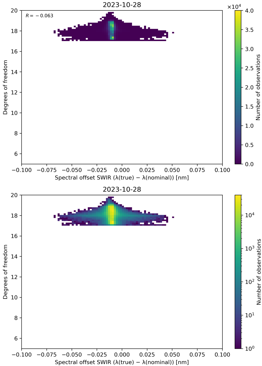
Figure 119: Scatter density plot of “Spectral offset SWIR ( \lambda(\text{true}) - \lambda(\text{nominal}) )” against “Degrees of freedom” for 2023-10-28 to 2023-10-29.
