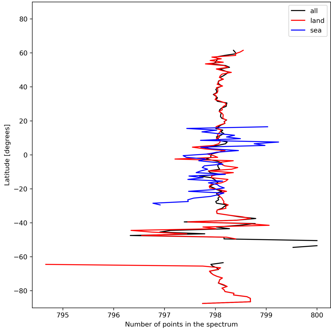
Figure 15: Zonal average of “Number of points in the spectrum” for 2023-10-28 to 2023-10-29.
