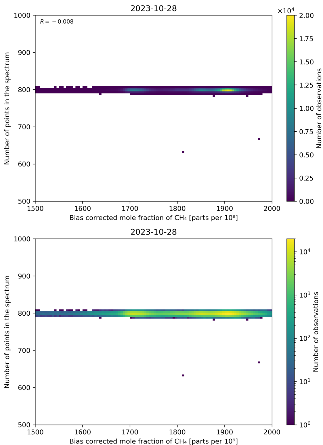
Figure 68: Scatter density plot of “Bias corrected mole fraction of CH 4 ” against “Number of points in the spectrum” for 2023-10-28 to 2023-10-29.
