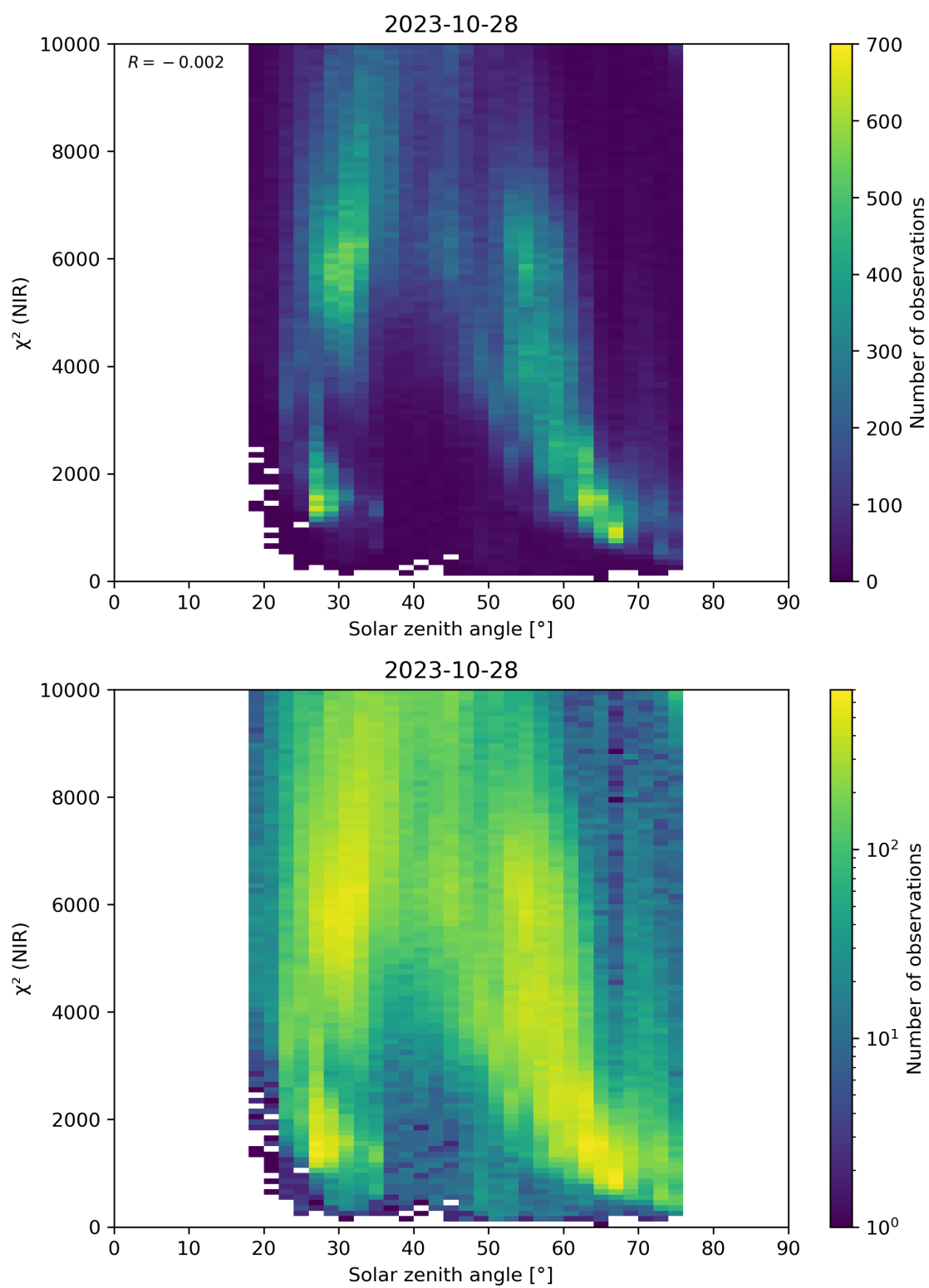
Figure 94: Scatter density plot of “Solar zenith angle” against “ \chi^2 (NIR)” for 2023-10-28 to 2023-10-29.
