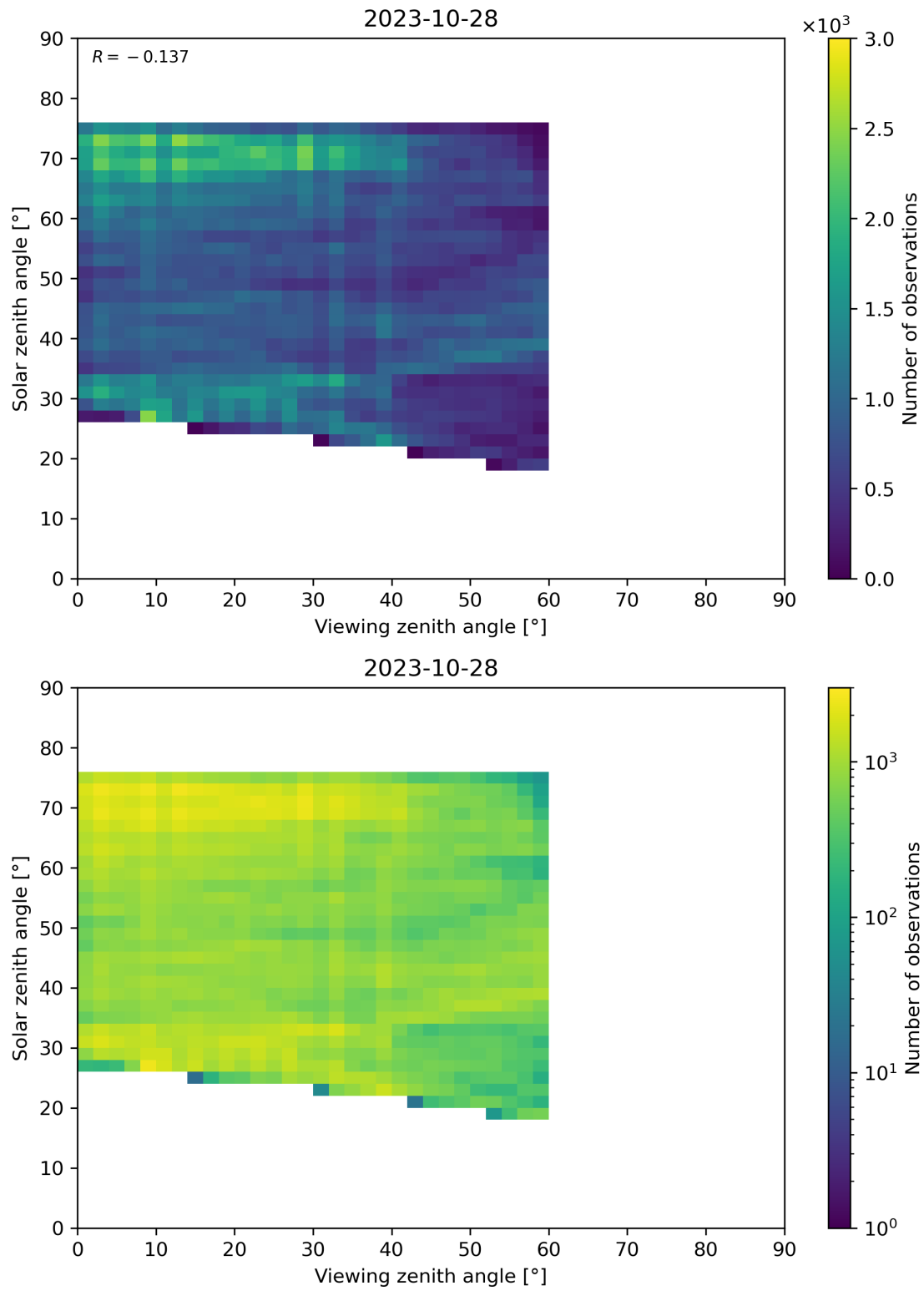
Figure 115: Scatter density plot of “Viewing zenith angle” against “Solar zenith angle” for 2023-10-28 to 2023-10-29.
