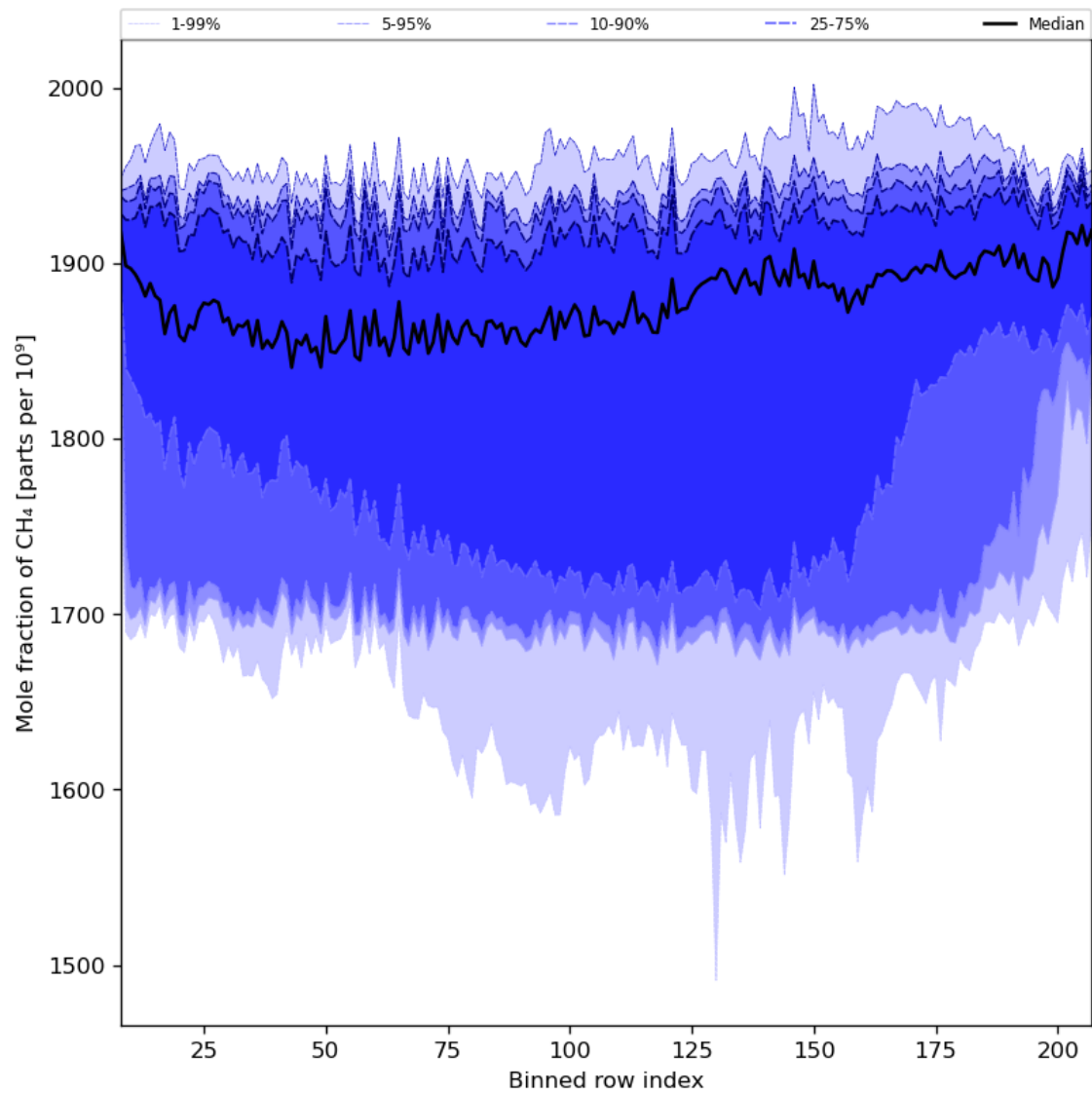
Figure 34: Along track statistics of “Mole fraction of CH 4 ” for 2023-10-28 to 2023-10-29
