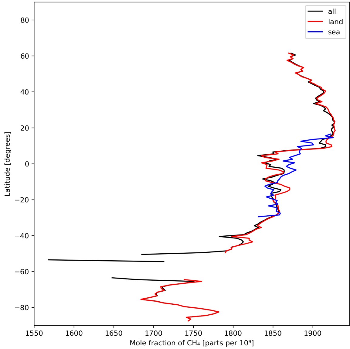
Figure 12: Zonal average of “Mole fraction of CH 4 ” for 2023-10-28 to 2023-10-29.
