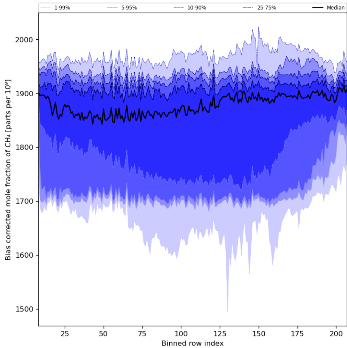
Figure 36: Along track statistics of “Bias corrected mole fraction of CH 4 ” for 2023-10-28 to 2023-10-29
