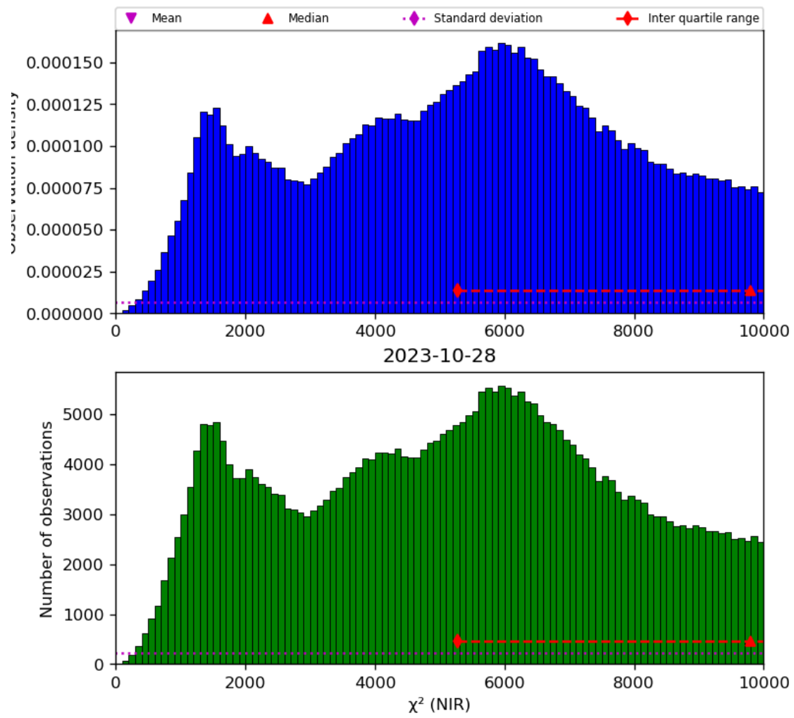
Figure 29: Histogram of “ \chi^2 (NIR)” for 2023-10-28 to 2023-10-29
