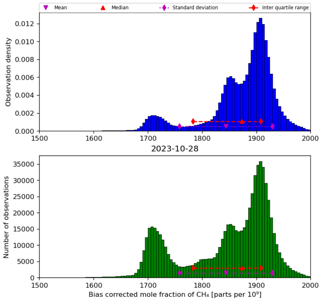
Figure 25: Histogram of “Bias corrected mole fraction of CH 4 ” for 2023-10-28 to 2023-10-29
