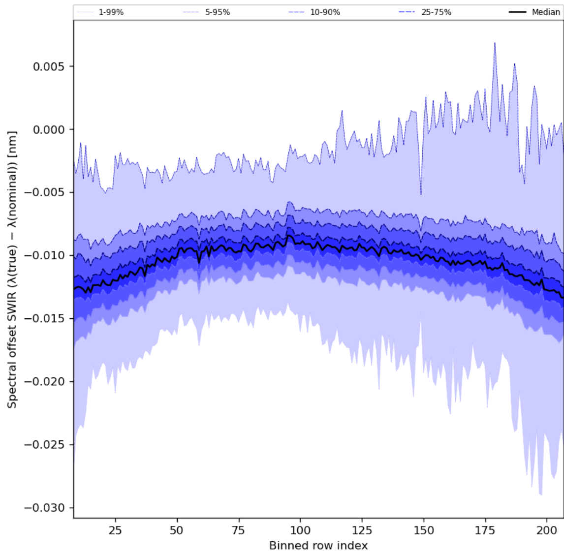
Figure 38: Along track statistics of “Spectral offset SWIR ( \lambda(\text{true}) - \lambda(\text{nominal}) )” for 2023-10-28 to 2023-10-29
