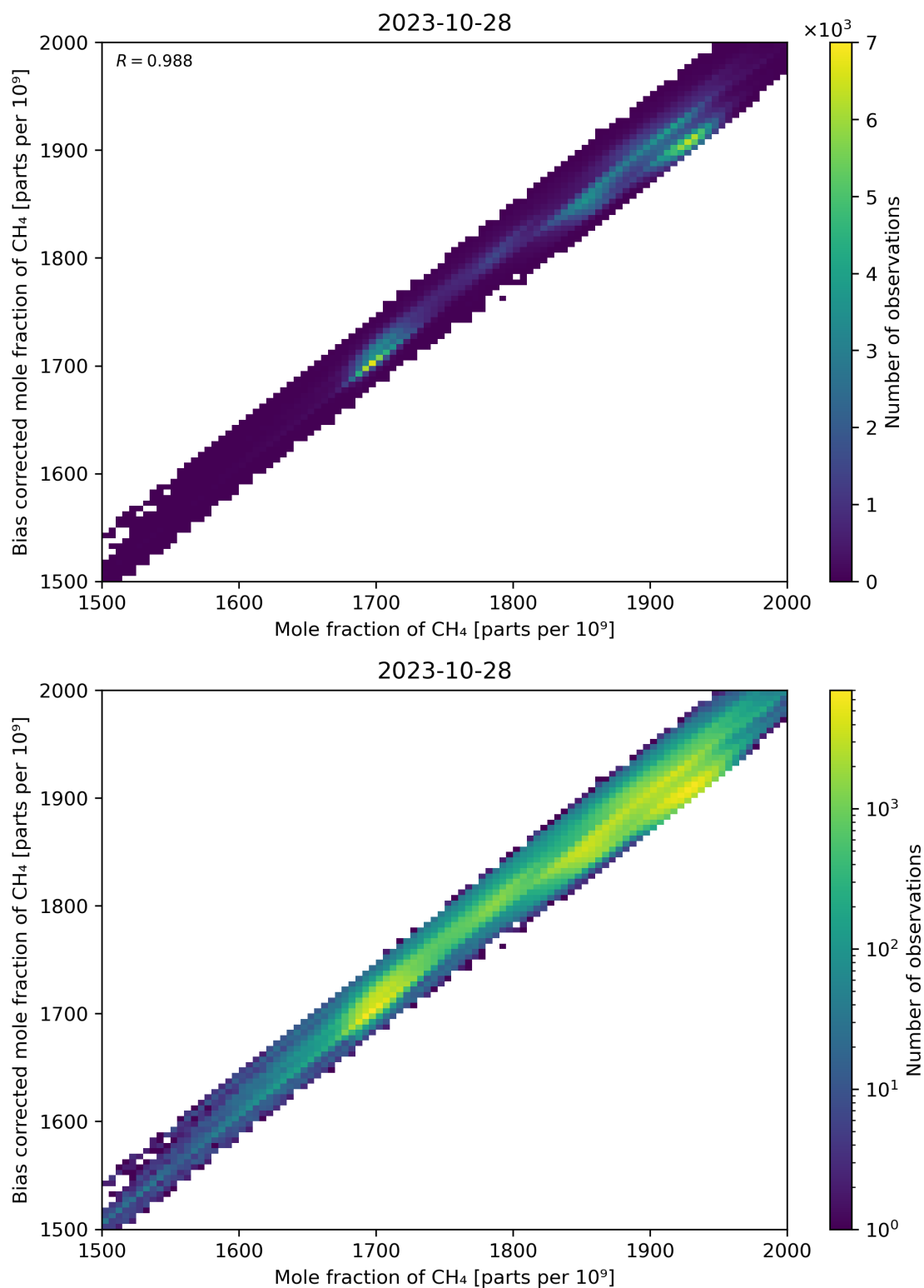
Figure 74: Scatter density plot of “Mole fraction of CH 4 ” against “Bias corrected mole fraction of CH 4 ” for 2023-10-28 to 2023-10-29.
