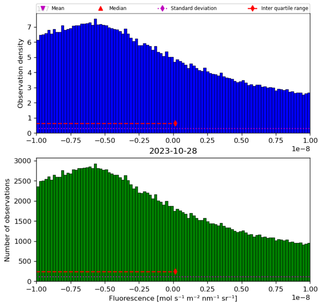
Figure 32: Histogram of “Fluorescence” for 2023-10-28 to 2023-10-29
