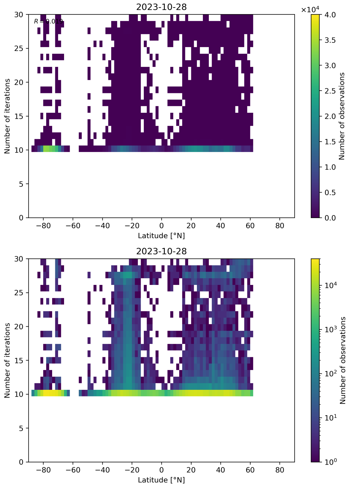
Figure 60: Scatter density plot of “Latitude” against “Number of iterations” for 2023-10-28 to 2023-10-29.
