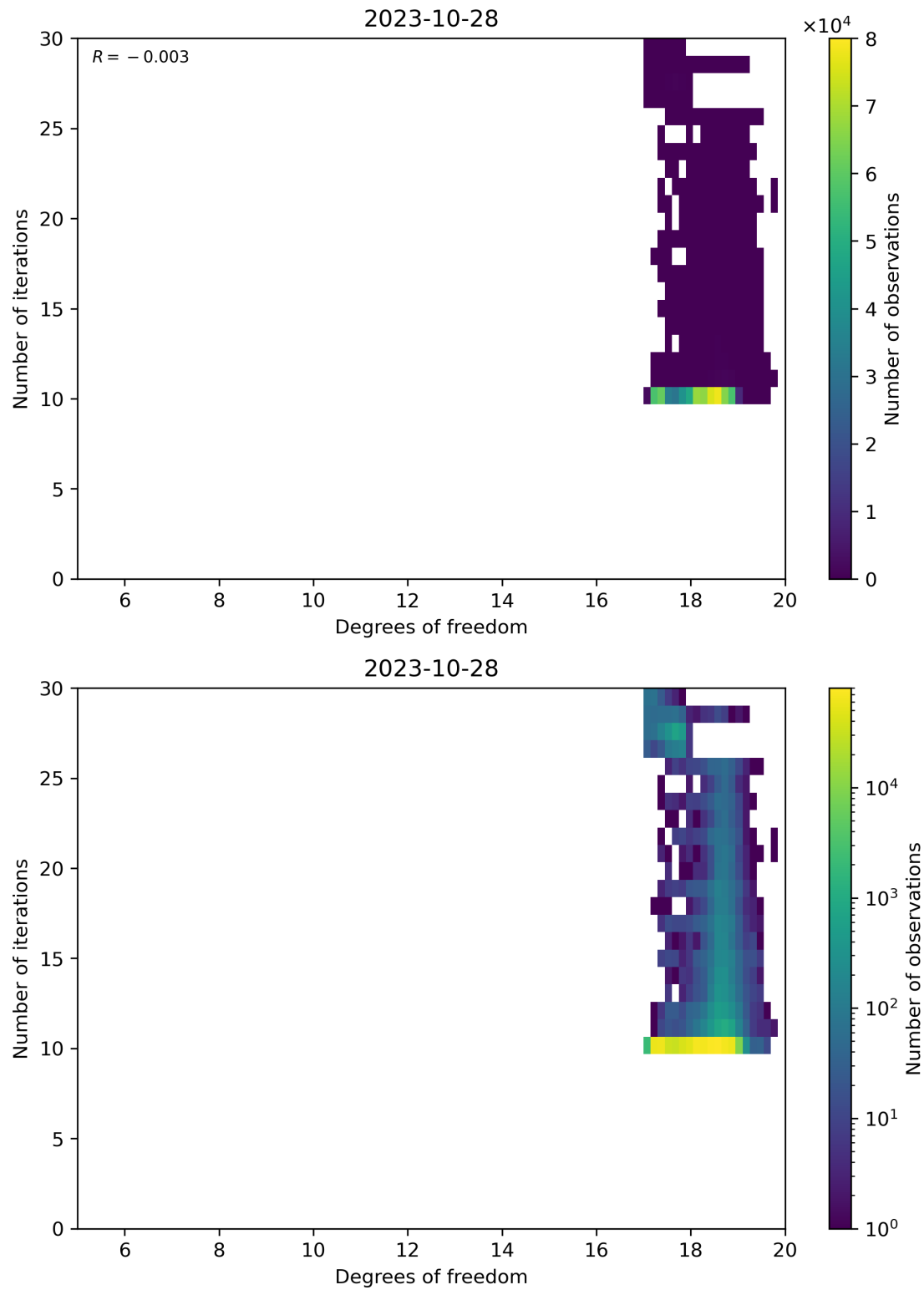
Figure 52: Scatter density plot of “Degrees of freedom” against “Number of iterations” for 2023-10-28 to 2023-10-29.
