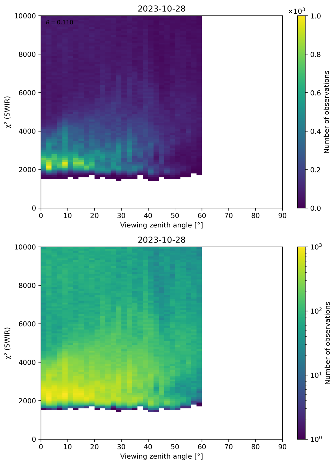
Figure 106: Scatter density plot of “Viewing zenith angle” against “ \chi^2 (SWIR)” for 2023-10-28 to 2023-10-29.
