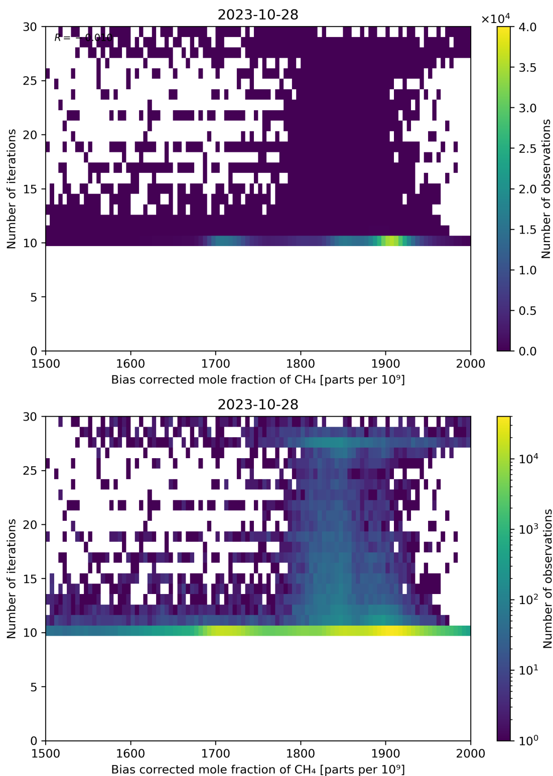
Figure 67: Scatter density plot of “Bias corrected mole fraction of \text{CH}_4 ” against “Number of iterations” for 2023-10-28 to 2023-10-29.
