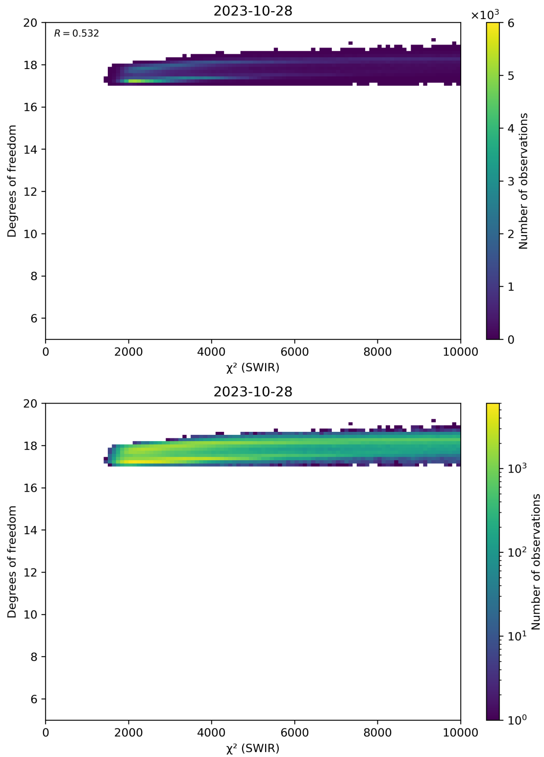
Figure 48: Scatter density plot of “ \chi^2 (SWIR)” against “Degrees of freedom” for 2023-10-28 to 2023-10-29.
