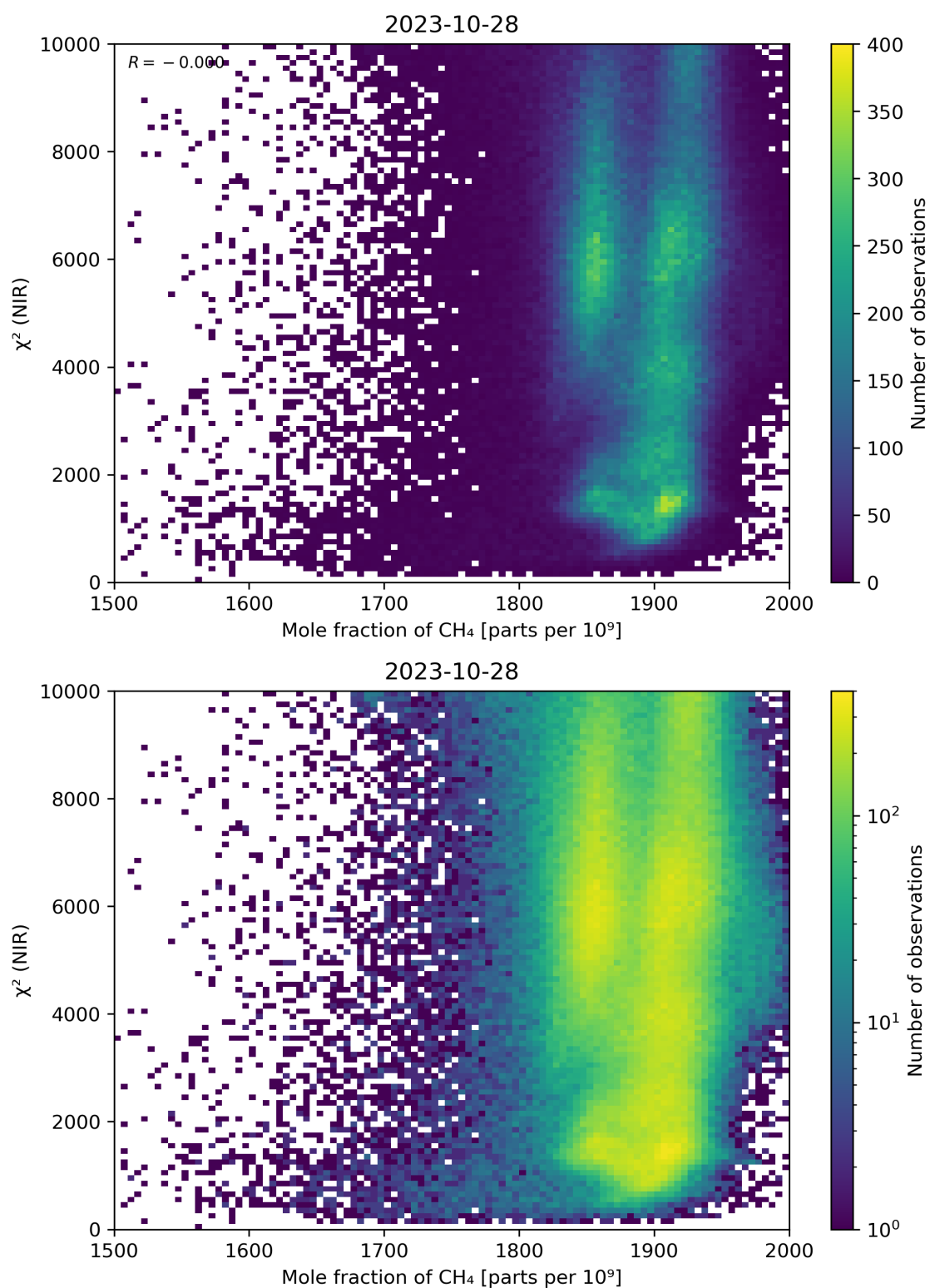
Figure 70: Scatter density plot of “Mole fraction of CH 4 ” against “ \chi^2 (NIR)” for 2023-10-28 to 2023-10-29.
