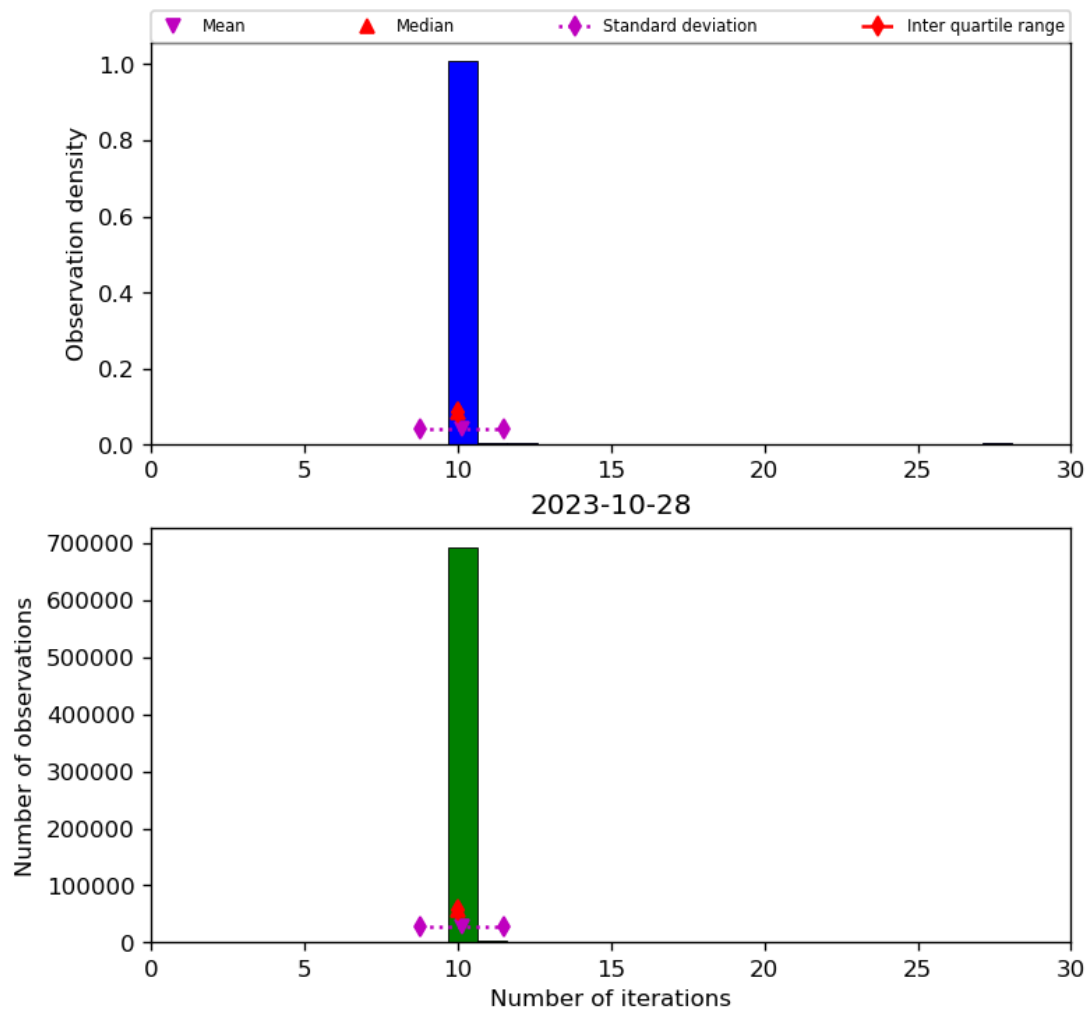
Figure 31: Histogram of “Number of iterations” for 2023-10-28 to 2023-10-29
