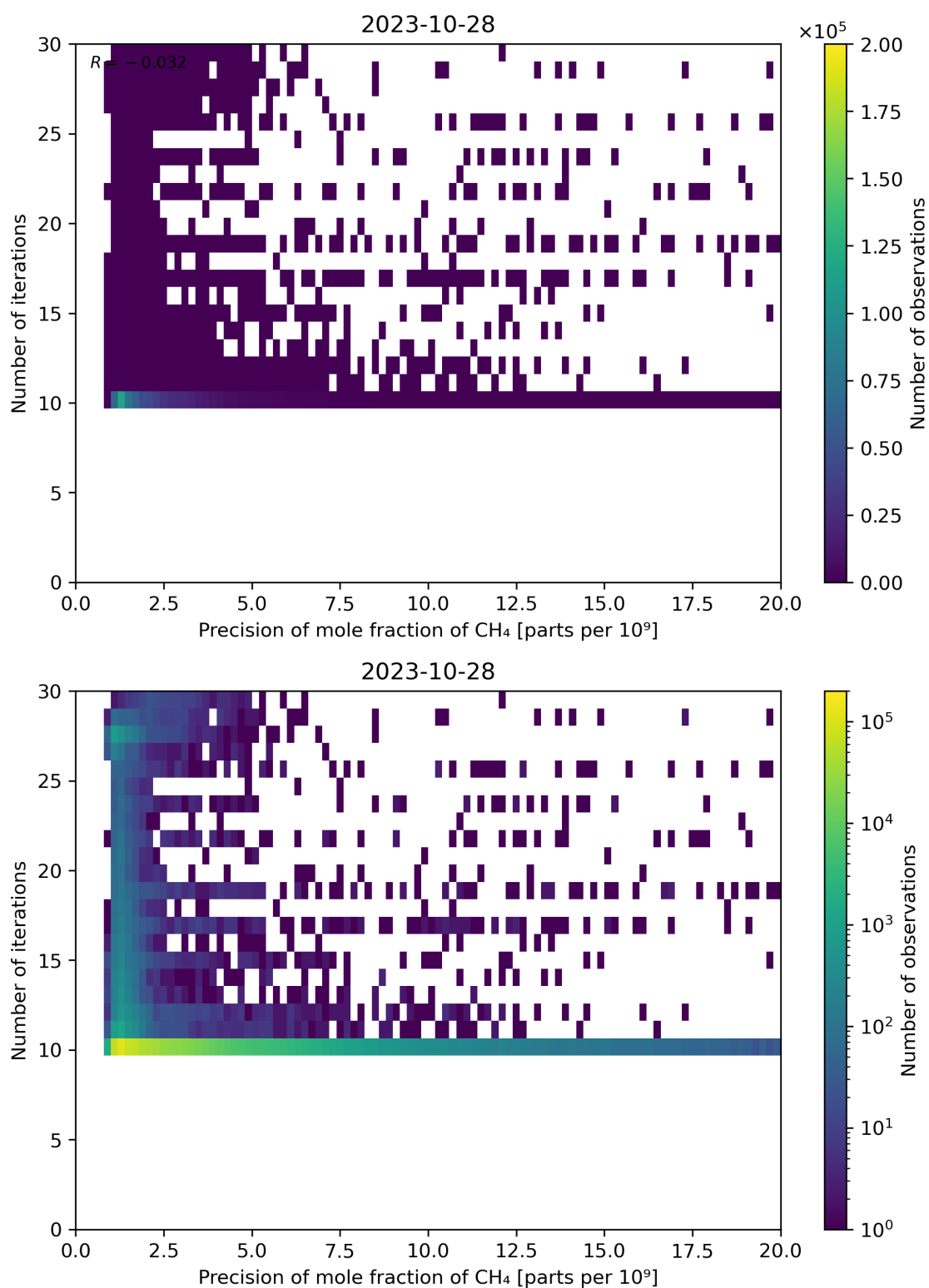
Figure 83: Scatter density plot of “Precision of mole fraction of CH 4 ” against “Number of iterations” for 2023-10-28 to 2023-10-29.
