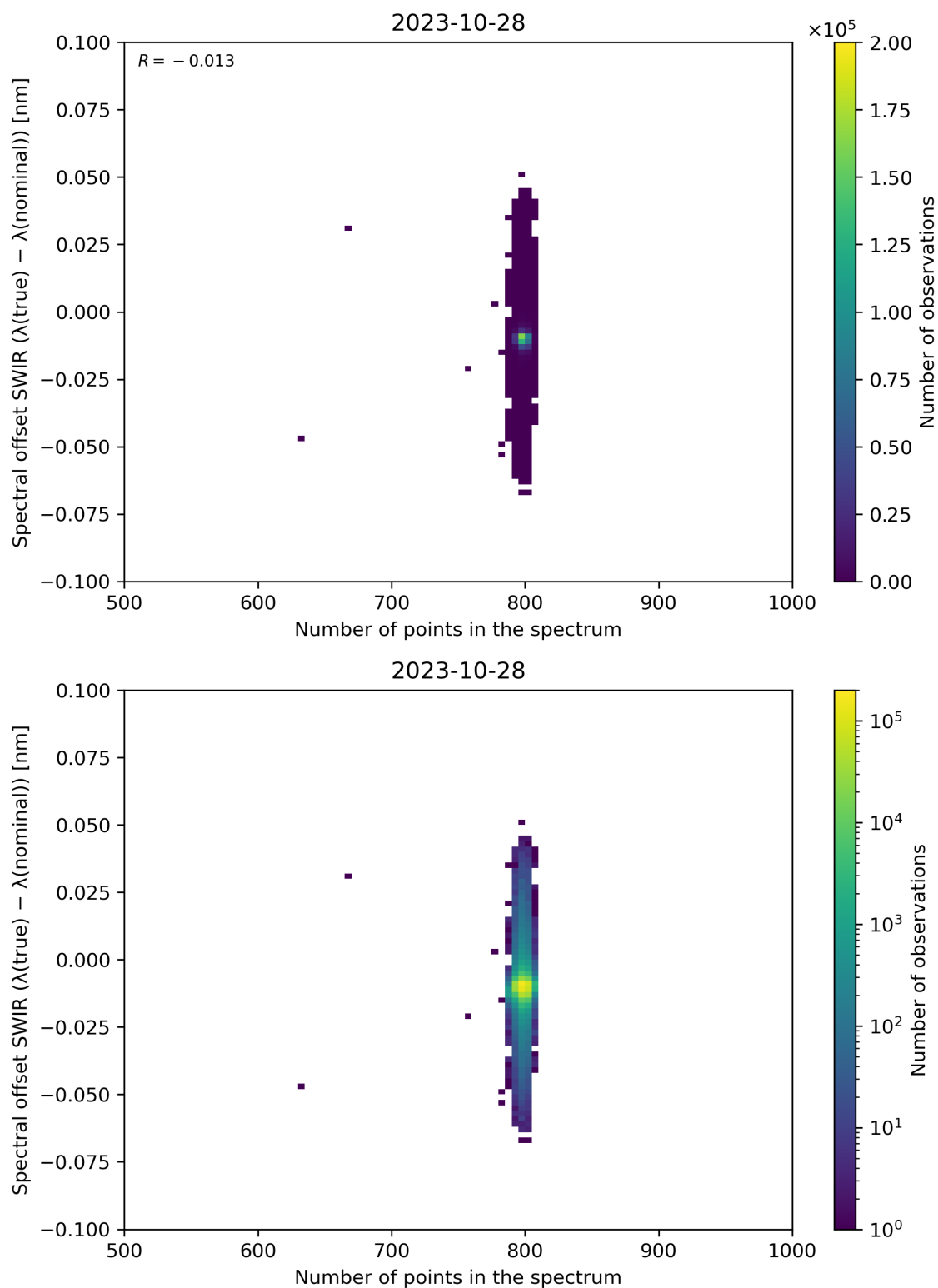
Figure 93: Scatter density plot of “Number of points in the spectrum” against “Spectral offset SWIR ( \lambda(\text{true}) - \lambda(\text{nominal}) )” for 2023-10-28 to 2023-10-29.
