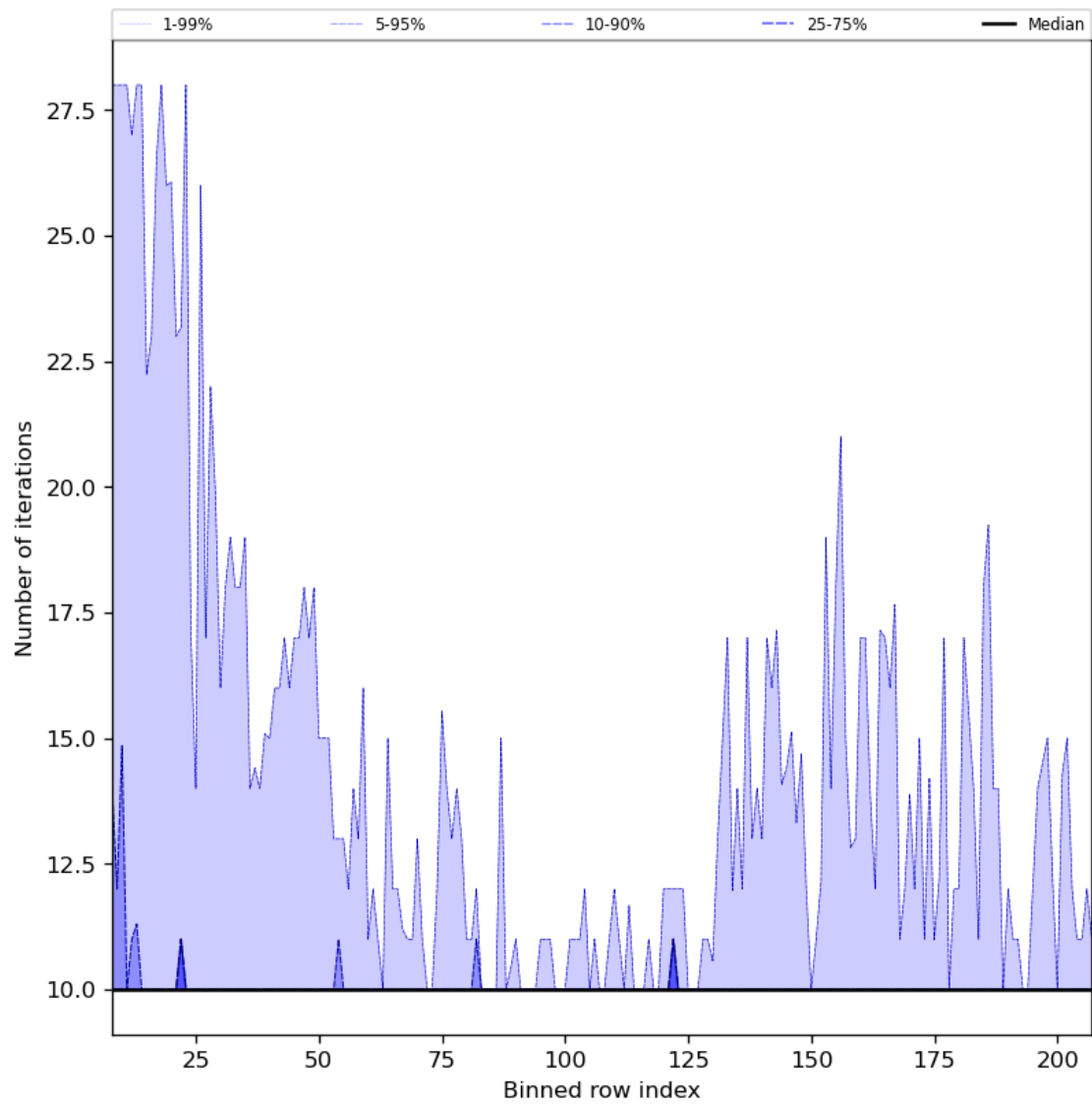
Figure 42: Along track statistics of “Number of iterations” for 2023-10-28 to 2023-10-29
