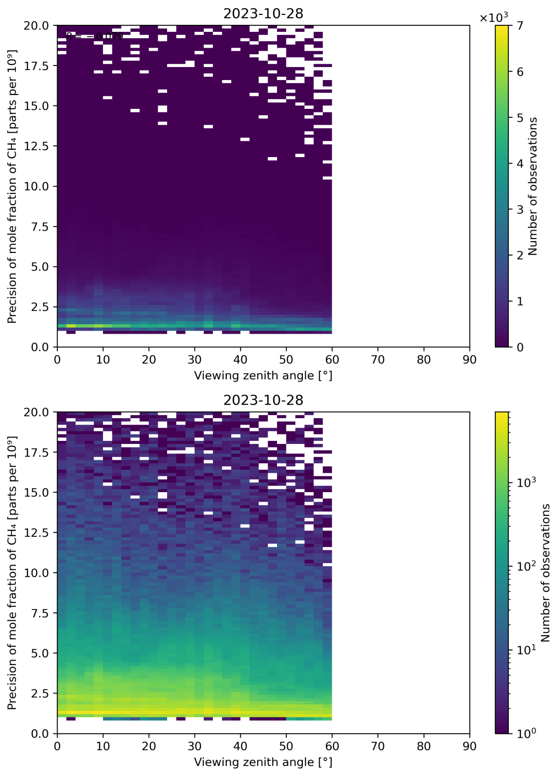
Figure 112: Scatter density plot of “Viewing zenith angle” against “Precision of mole fraction of CH 4 ” for 2023-10-28 to 2023-10-29.
