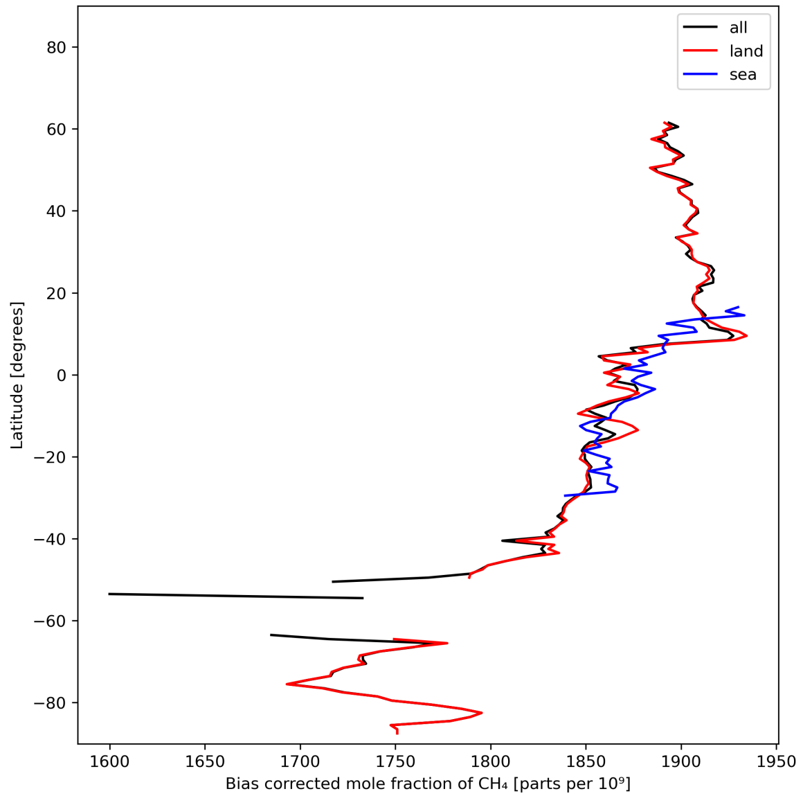
Figure 14: Zonal average of “Bias corrected mole fraction of CH 4 ” for 2023-10-28 to 2023-10-29.
