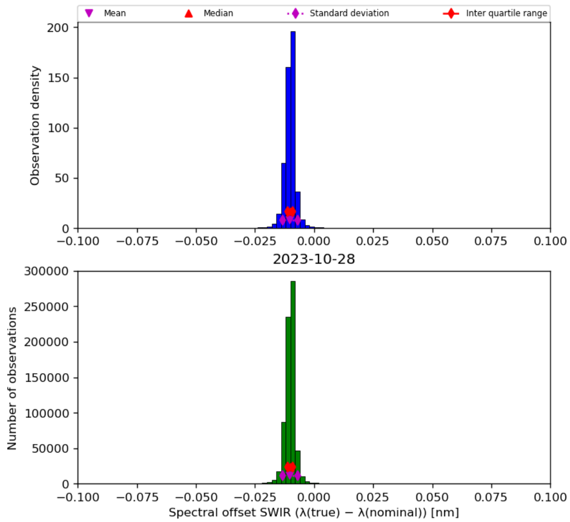
Figure 27: Histogram of “Spectral offset SWIR ( \lambda(\text{true}) - \lambda(\text{nominal}) )” for 2023-10-28 to 2023-10-29
