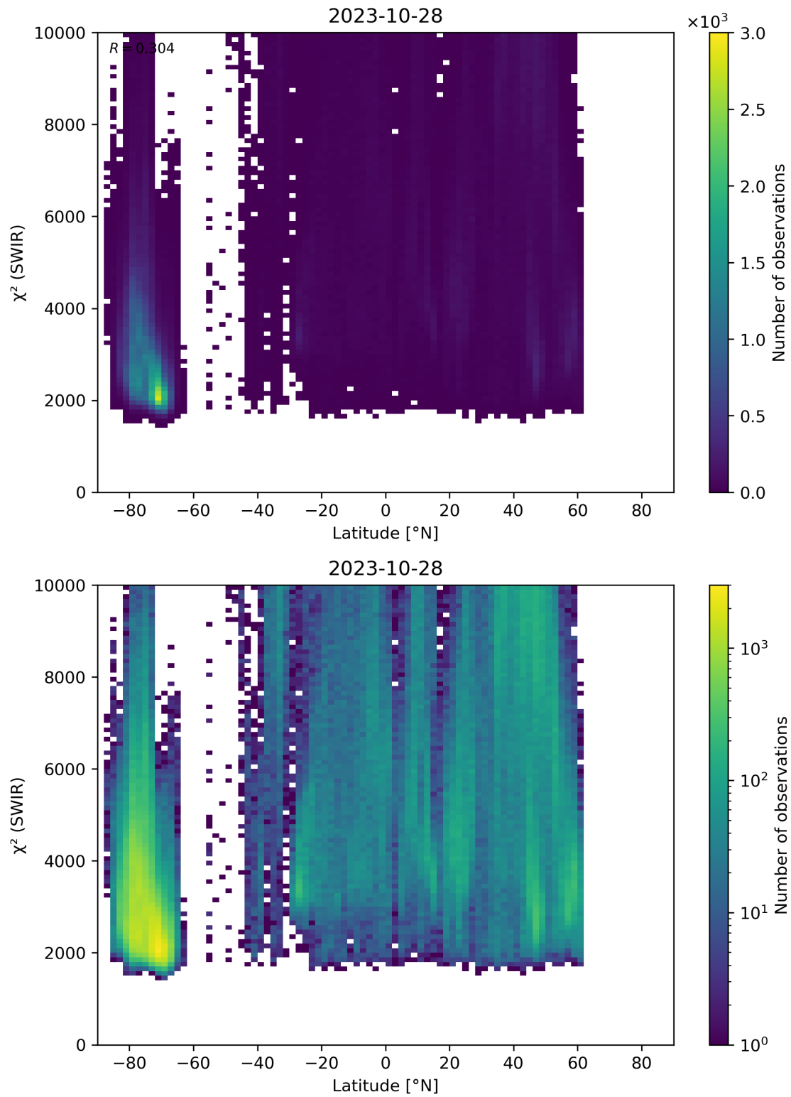
Figure 54: Scatter density plot of “Latitude” against “ \chi^2 (SWIR)” for 2023-10-28 to 2023-10-29.
