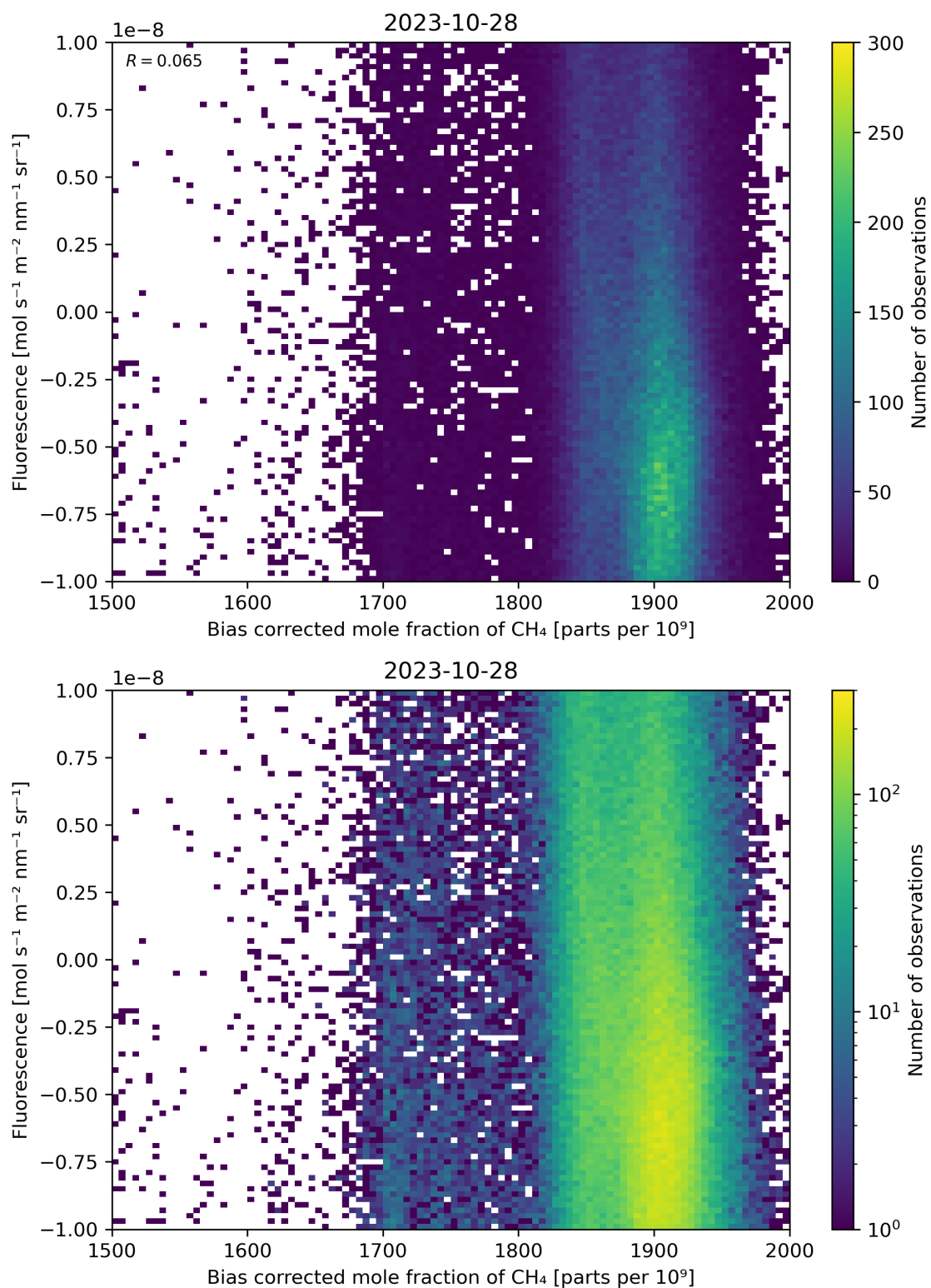
Figure 66: Scatter density plot of “Bias corrected mole fraction of \text{CH}_4 ” against “Fluorescence” for 2023-10-28 to 2023-10-29.
