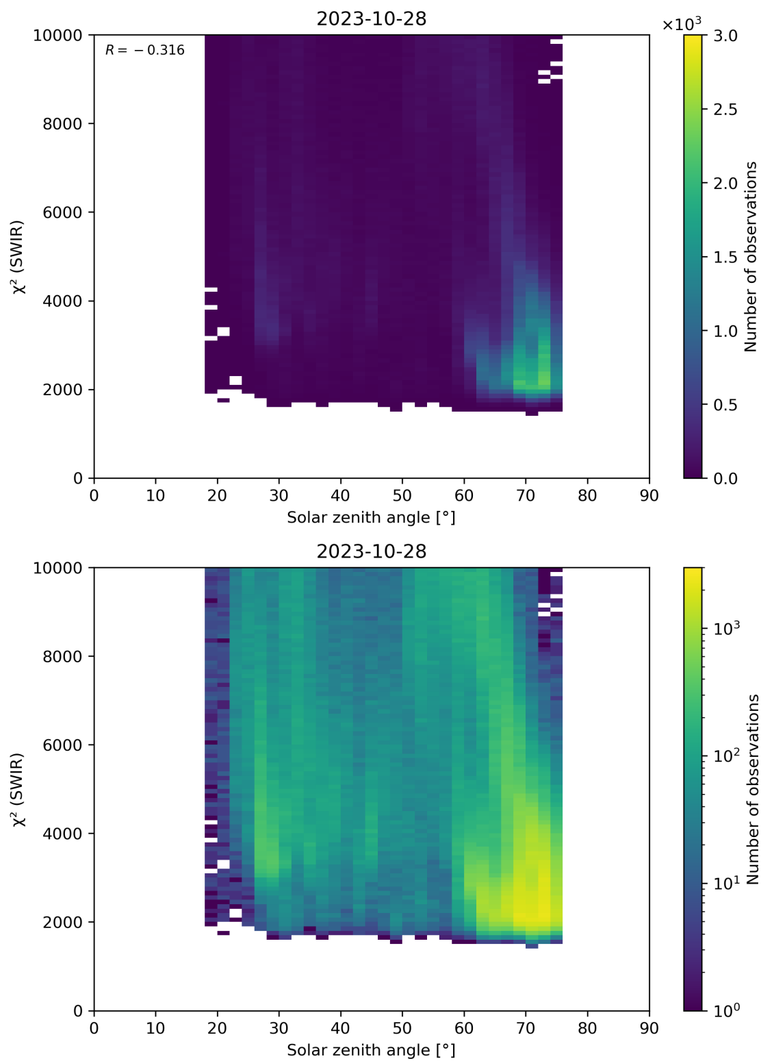
Figure 95: Scatter density plot of “Solar zenith angle” against “ \chi^2 (SWIR)” for 2023-10-28 to 2023-10-29.
