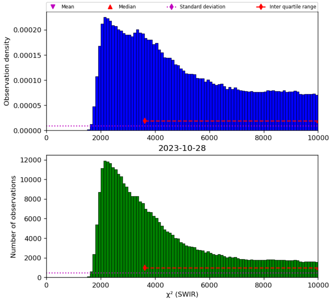
Figure 28: Histogram of “ \chi^2 (SWIR)” for 2023-10-28 to 2023-10-29
