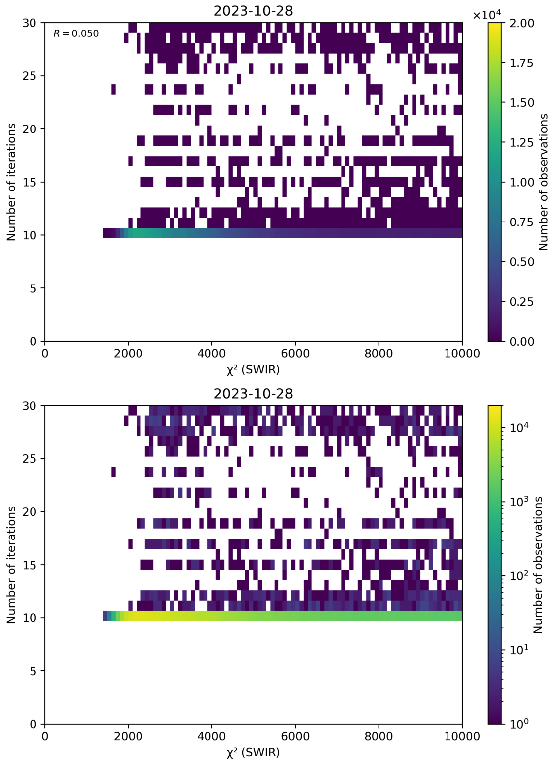
Figure 50: Scatter density plot of “ \chi^2 (SWIR)” against “Number of iterations” for 2023-10-28 to 2023-10-29.
