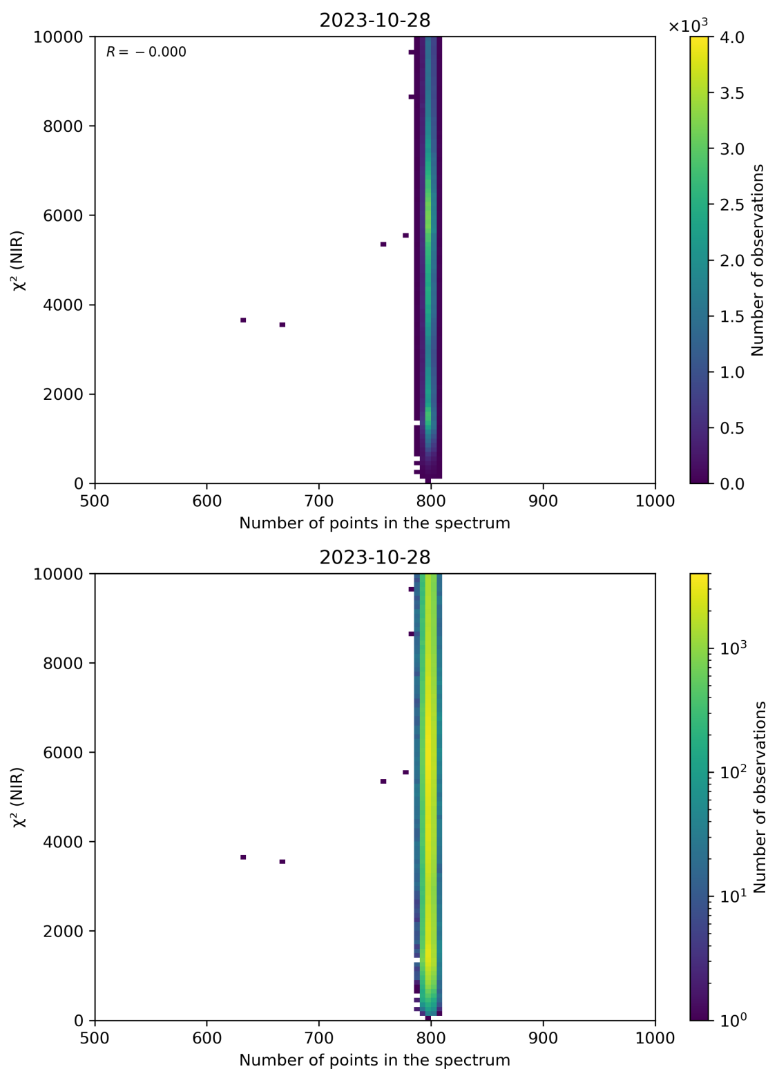
Figure 88: Scatter density plot of “Number of points in the spectrum” against “ \chi^2 (NIR)” for 2023-10-28 to 2023-10-29.
