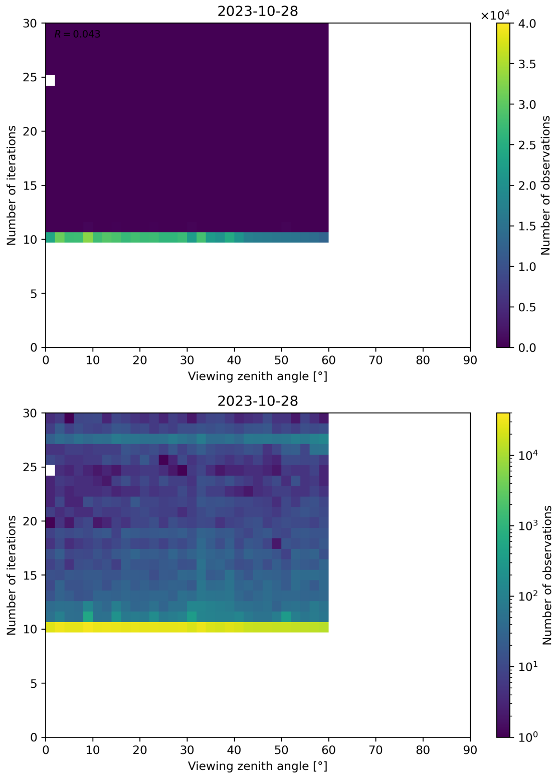
Figure 113: Scatter density plot of “Viewing zenith angle” against “Number of iterations” for 2023-10-28 to 2023-10-29.
