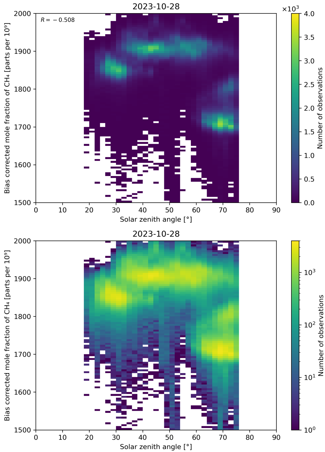
Figure 100: Scatter density plot of “Solar zenith angle” against “Bias corrected mole fraction of CH 4 ” for 2023-10-28 to 2023-10-29.
