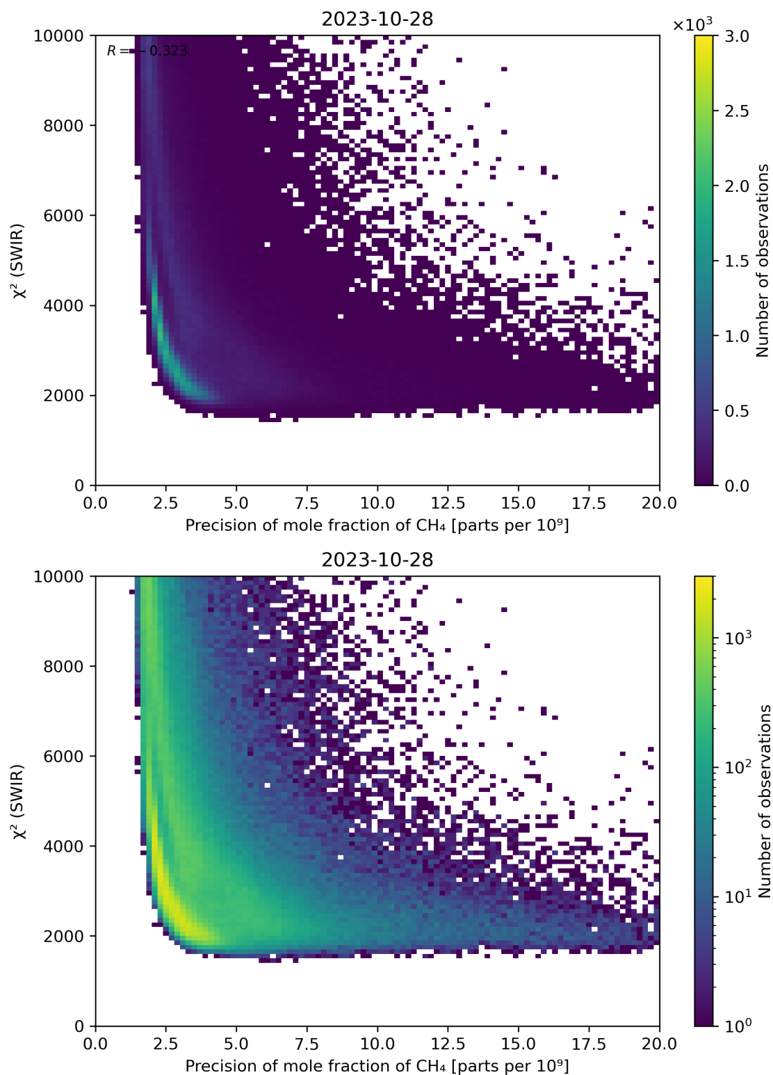
Figure 79: Scatter density plot of “Precision of mole fraction of \text{CH}_4 ” against “ \chi^2 (SWIR)” for 2023-10-28 to 2023-10-29.
