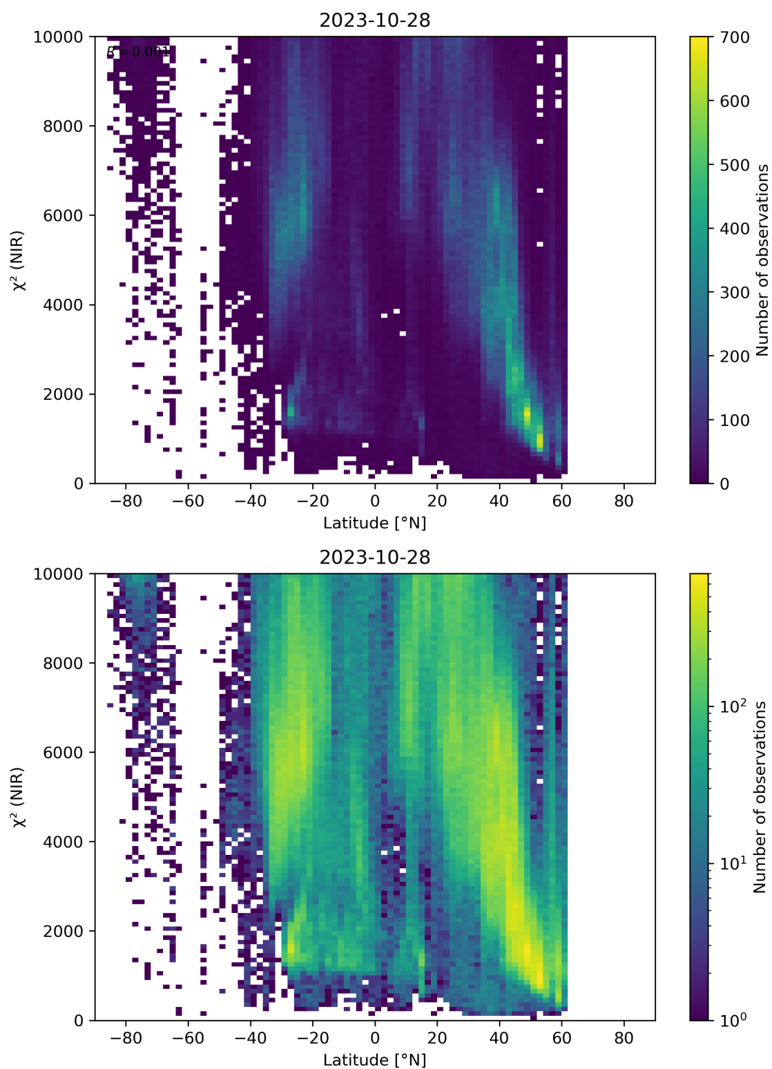
Figure 53: Scatter density plot of “Latitude” against “ \chi^2 (NIR)” for 2023-10-28 to 2023-10-29.
