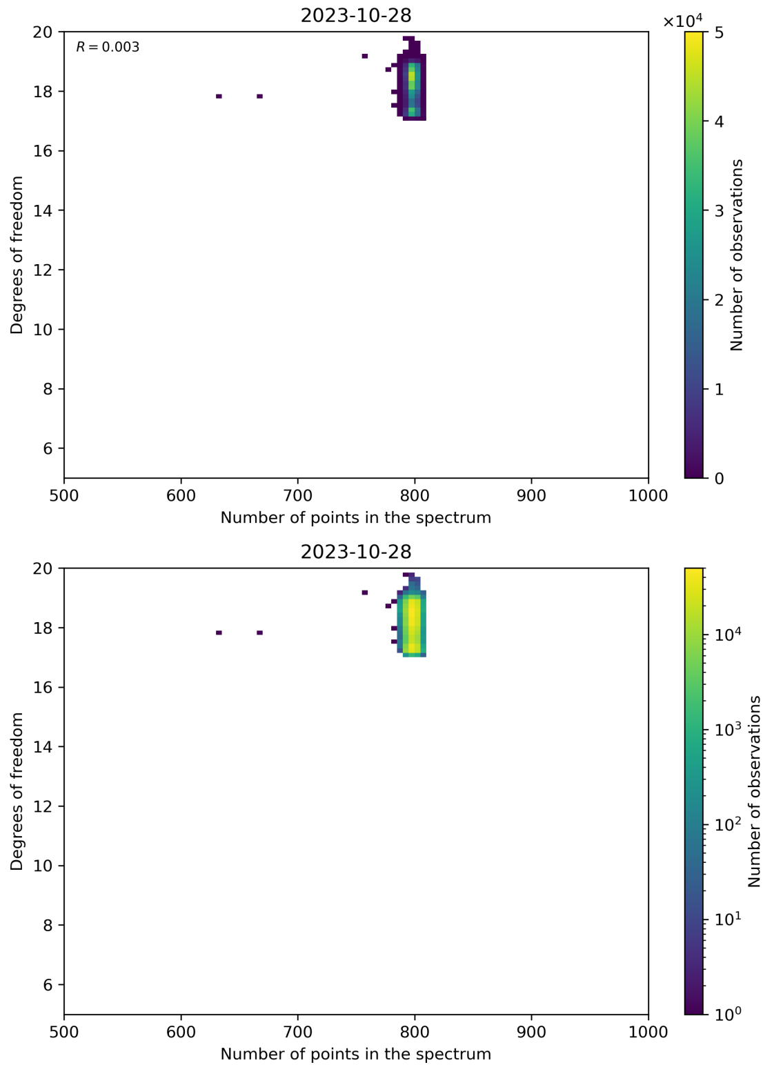
Figure 90: Scatter density plot of “Number of points in the spectrum” against “Degrees of freedom” for 2023-10-28 to 2023-10-29.
