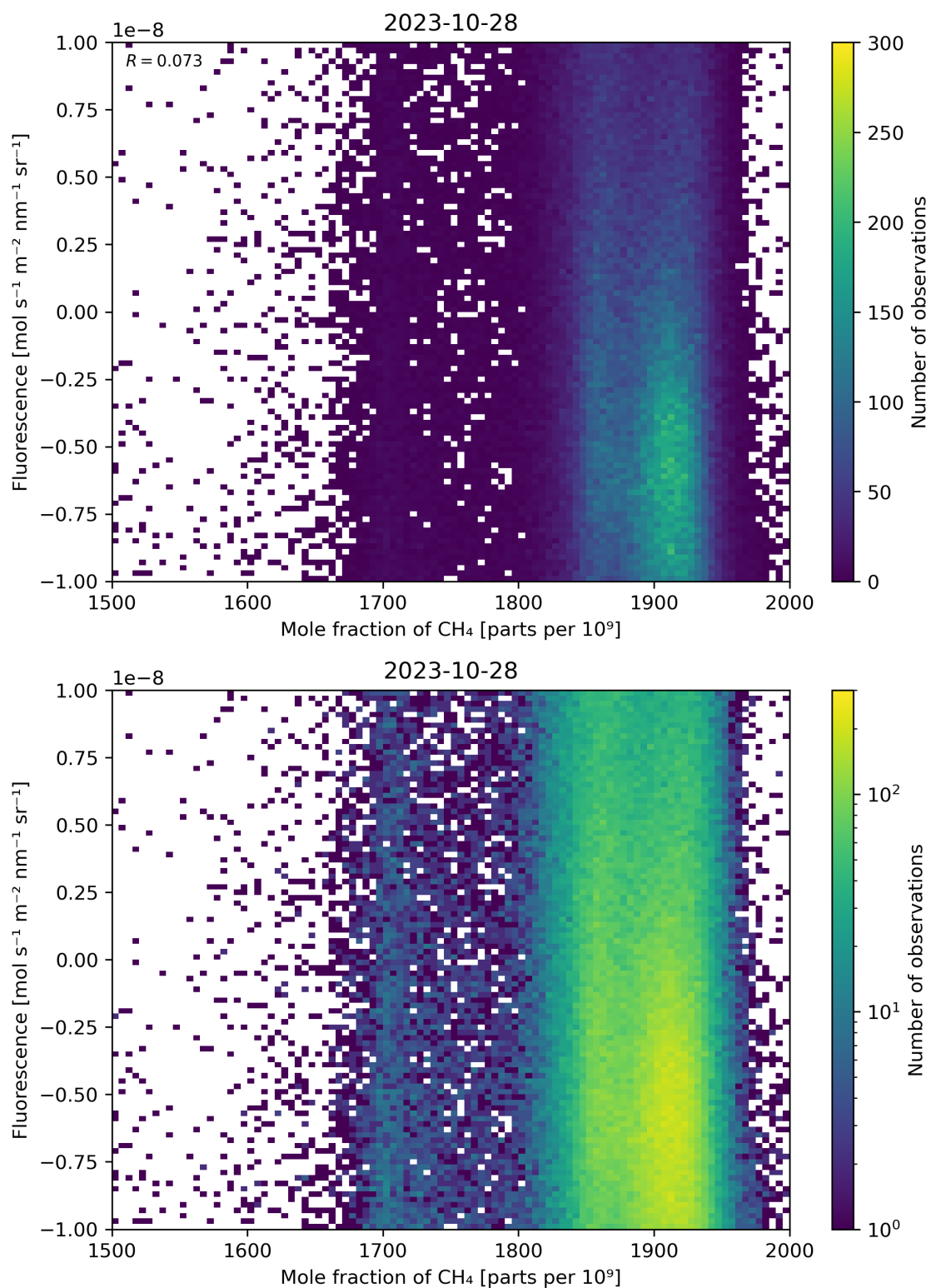
Figure 73: Scatter density plot of “Mole fraction of \text{CH}_4 ” against “Fluorescence” for 2023-10-28 to 2023-10-29.
