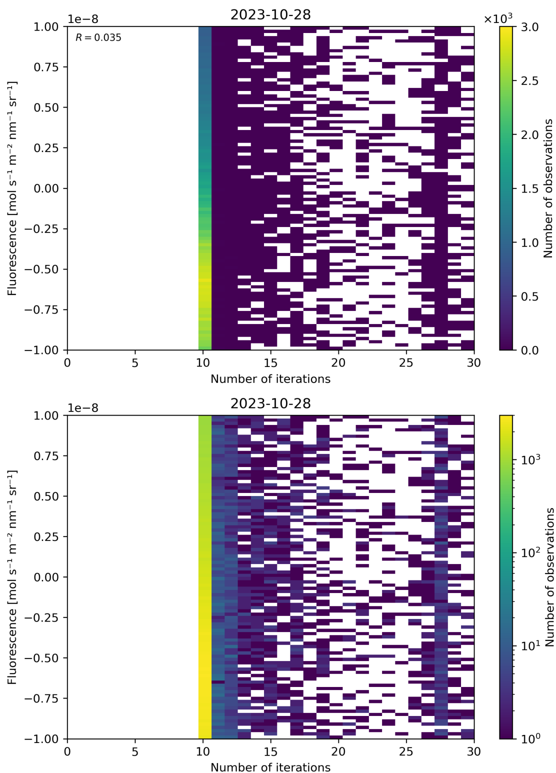
Figure 87: Scatter density plot of “Number of iterations” against “Fluorescence” for 2023-10-28 to 2023-10-29.
