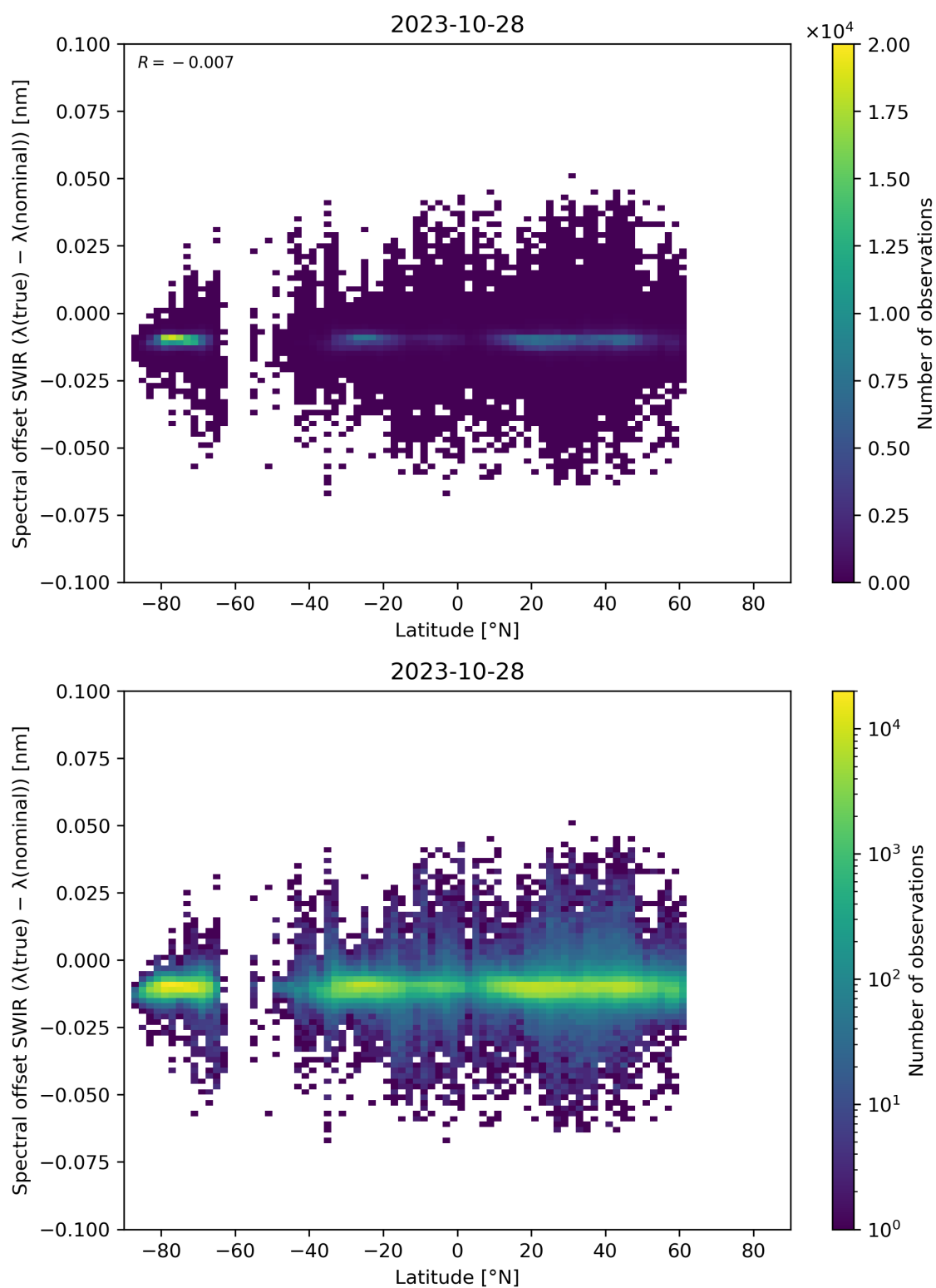
Figure 62: Scatter density plot of “Latitude” against “Spectral offset SWIR ( \lambda(\text{true}) - \lambda(\text{nominal}) )” for 2023-10-28 to 2023-10-29.
