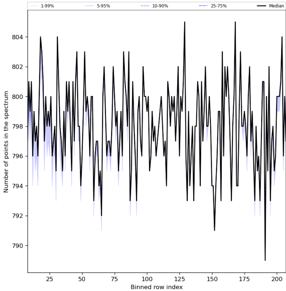
Figure 37: Along track statistics of “Number of points in the spectrum” for 2023-10-28 to 2023-10-29
