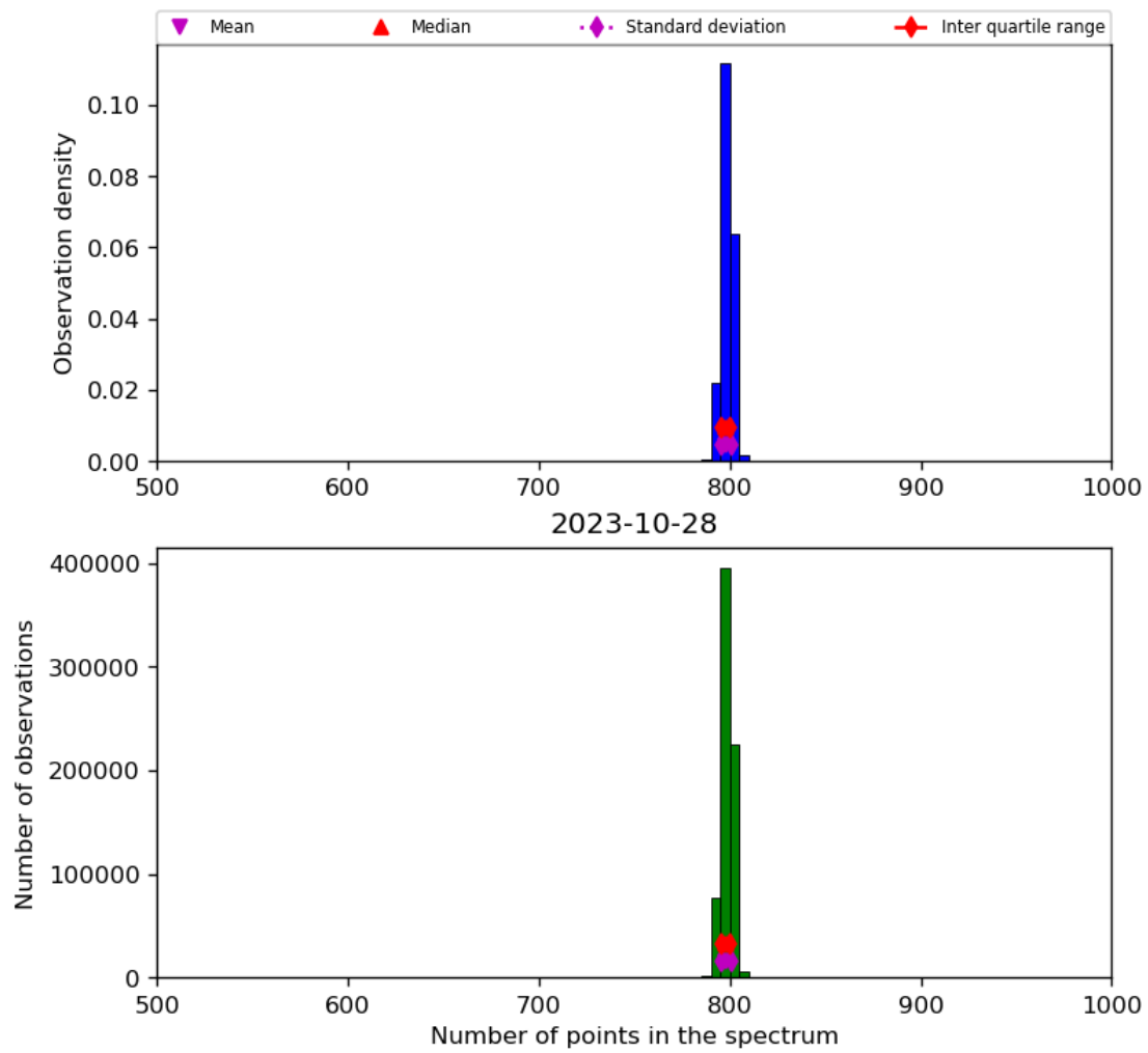
Figure 26: Histogram of “Number of points in the spectrum” for 2023-10-28 to 2023-10-29
