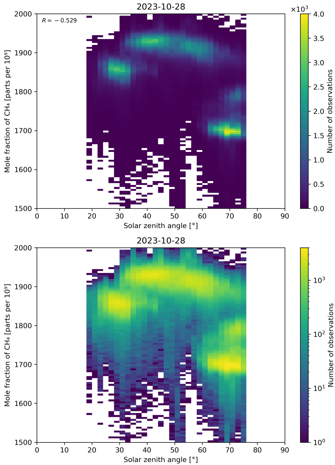
Figure 99: Scatter density plot of “Solar zenith angle” against “Mole fraction of CH 4 ” for 2023-10-28 to 2023-10-29.
