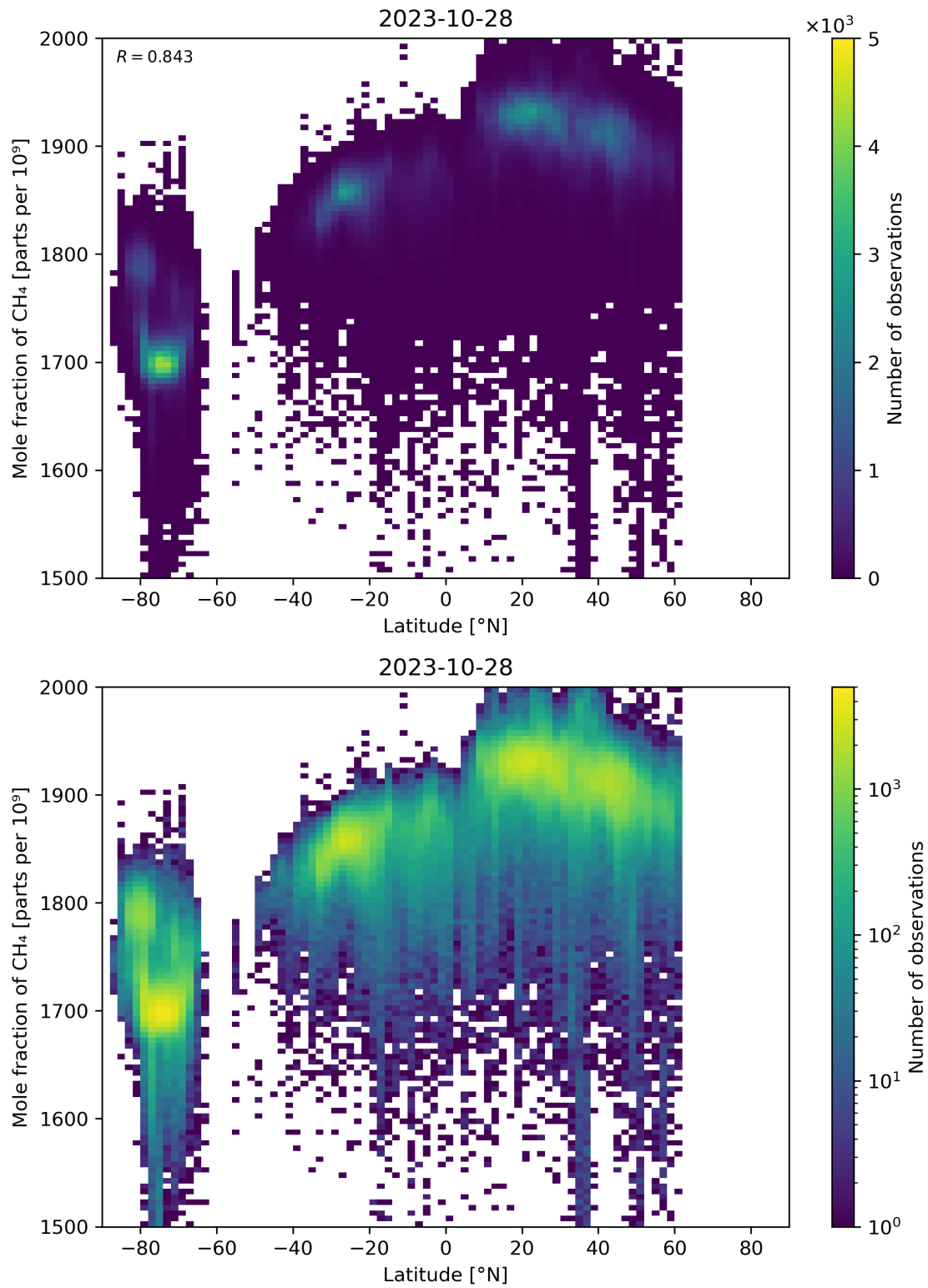
Figure 57: Scatter density plot of “Latitude” against “Mole fraction of CH 4 ” for 2023-10-28 to 2023-10-29.
