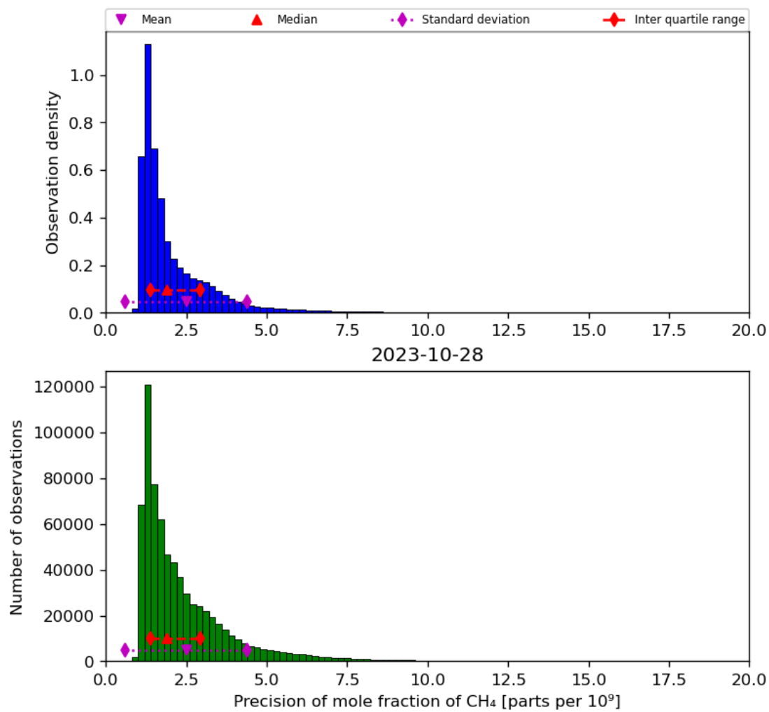
Figure 24: Histogram of “Precision of mole fraction of CH 4 ” for 2023-10-28 to 2023-10-29
