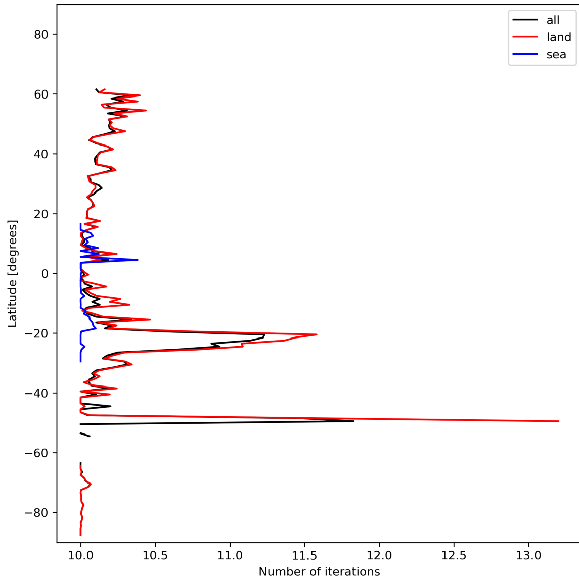
Figure 20: Zonal average of “Number of iterations” for 2023-10-28 to 2023-10-29.
