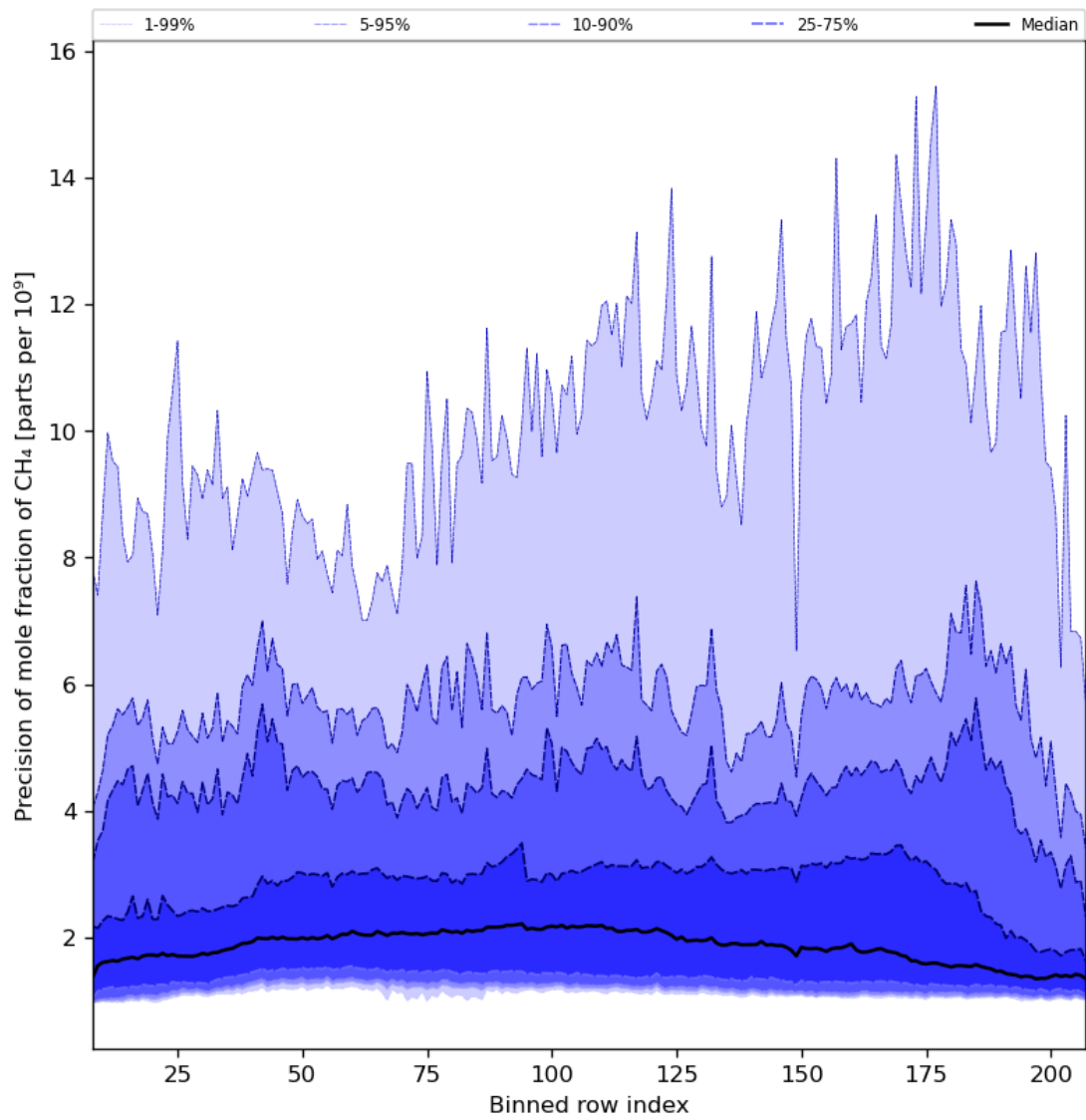
Figure 35: Along track statistics of “Precision of mole fraction of CH 4 ” for 2023-10-28 to 2023-10-29
