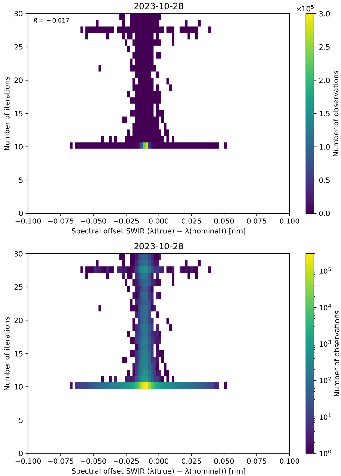
Figure 121: Scatter density plot of “Spectral offset SWIR ( \lambda(\text{true}) - \lambda(\text{nominal}) )” against “Number of iterations” for 2023-10-28 to 2023-10-29.
