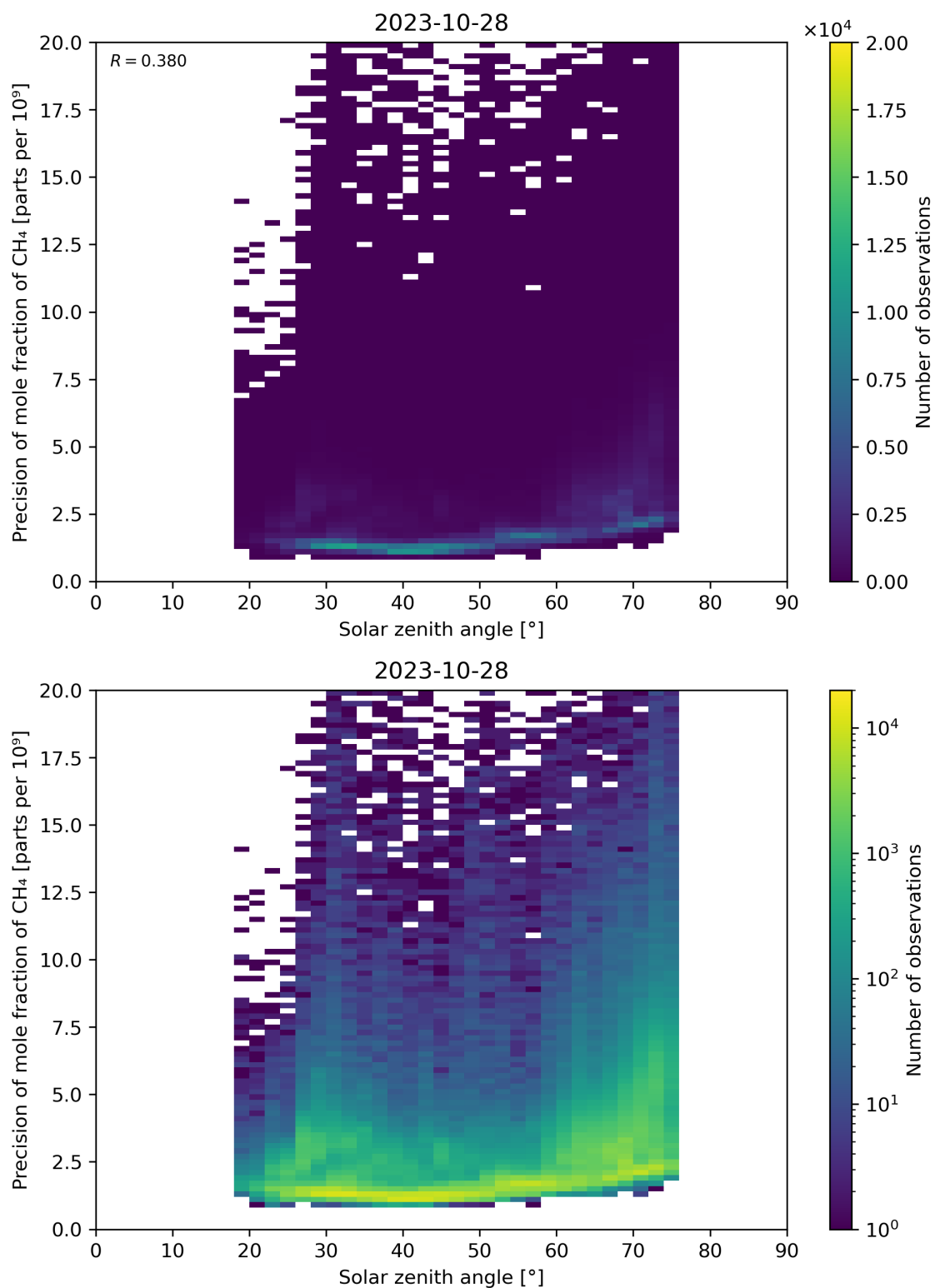
Figure 101: Scatter density plot of “Solar zenith angle” against “Precision of mole fraction of CH 4 ” for 2023-10-28 to 2023-10-29.
