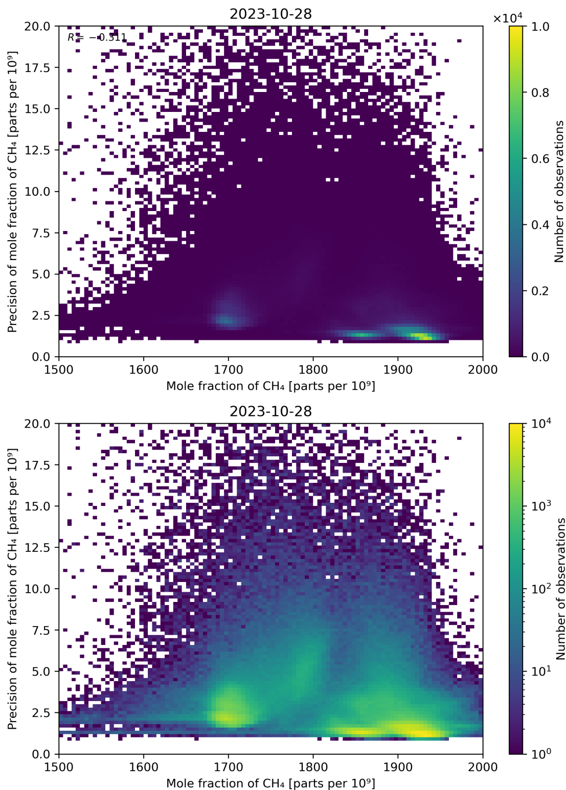
Figure 75: Scatter density plot of “Mole fraction of CH 4 ” against “Precision of mole fraction of CH 4 ” for 2023-10-28 to 2023-10-29.
