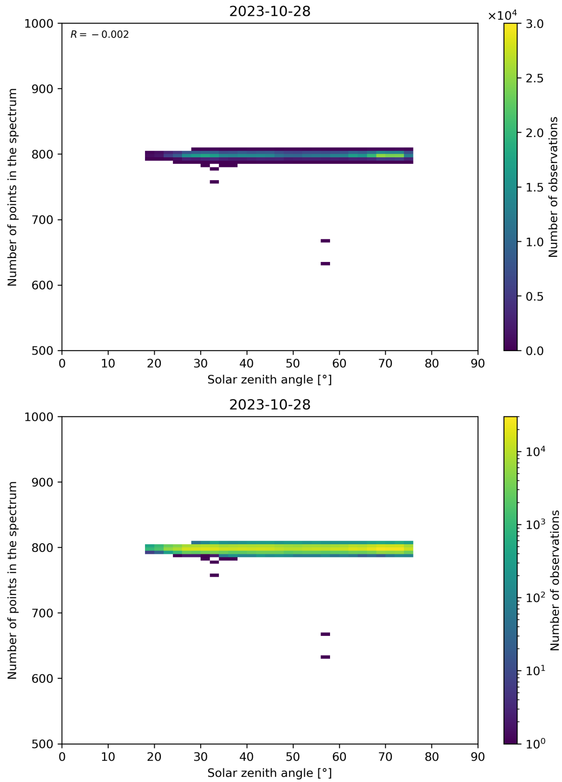
Figure 103: Scatter density plot of “Solar zenith angle” against “Number of points in the spectrum” for 2023-10-28 to 2023-10-29.
