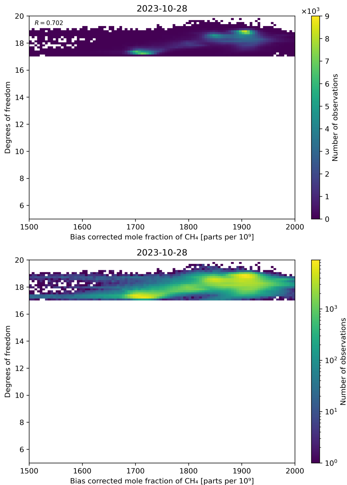
Figure 65: Scatter density plot of “Bias corrected mole fraction of CH 4 ” against “Degrees of freedom” for 2023-10-28 to 2023-10-29.
