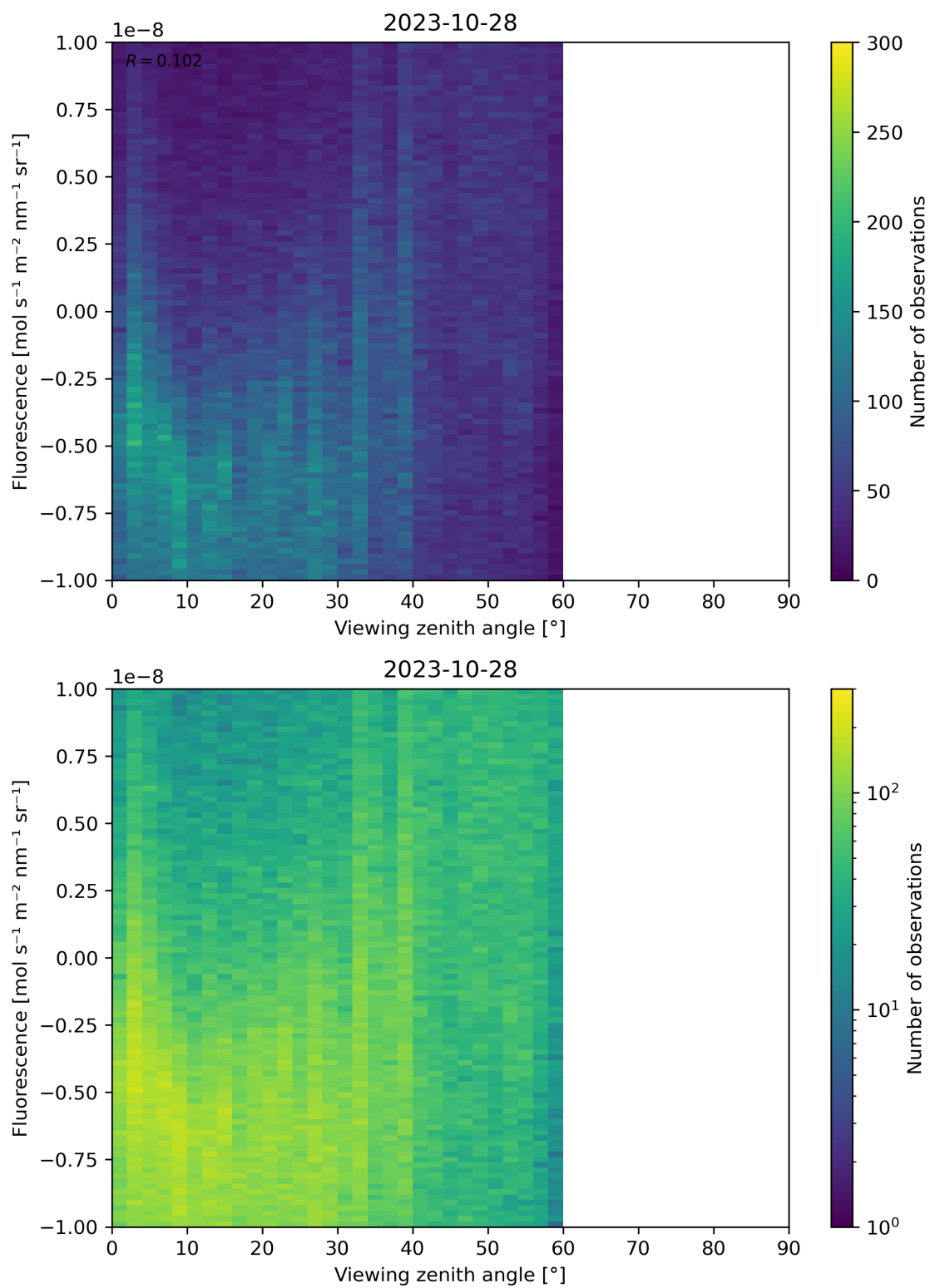
Figure 108: Scatter density plot of “Viewing zenith angle” against “Fluorescence” for 2023-10-28 to 2023-10-29.
