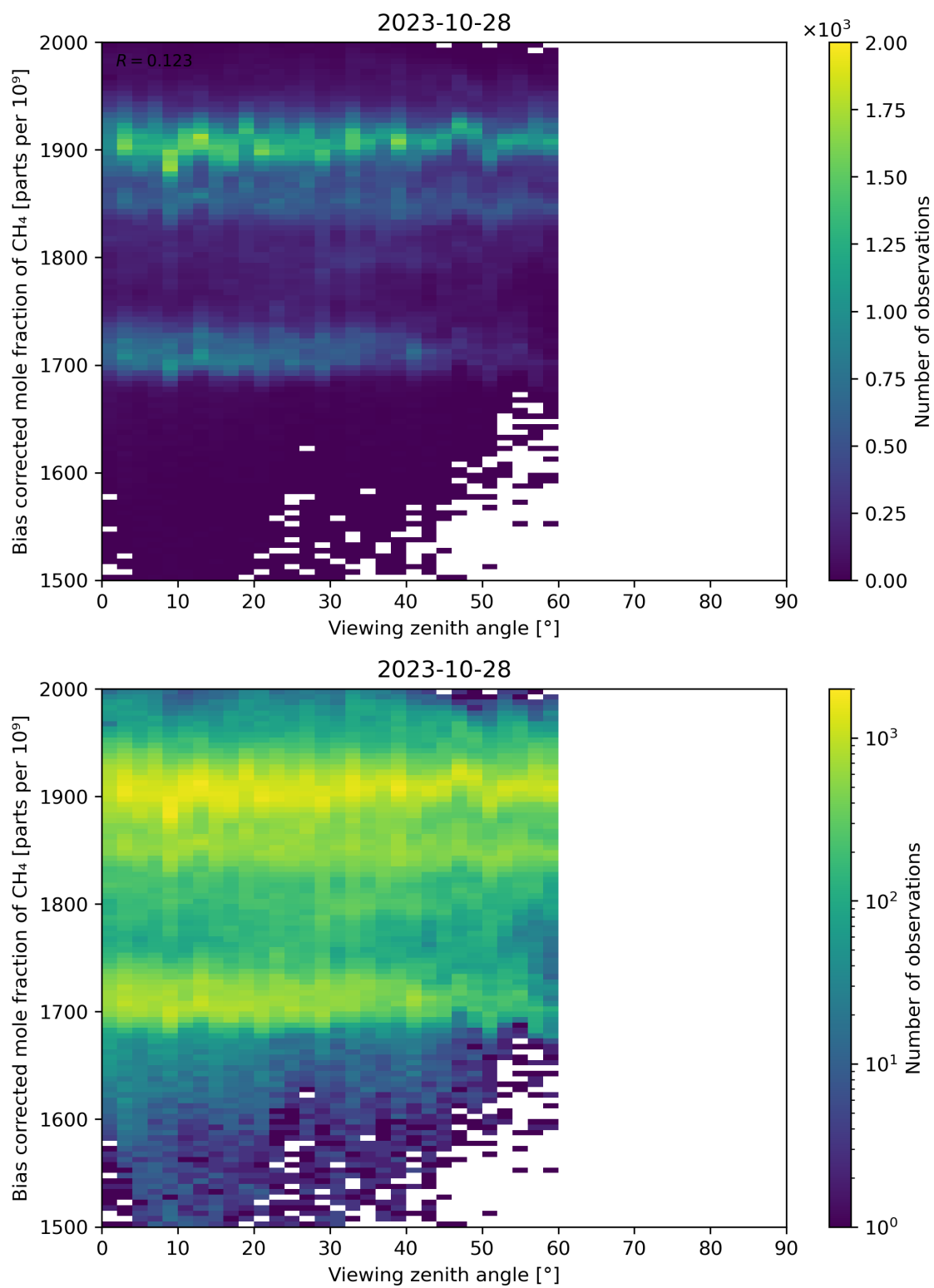
Figure 111: Scatter density plot of “Viewing zenith angle” against “Bias corrected mole fraction of CH 4 ” for 2023-10-28 to 2023-10-29.
