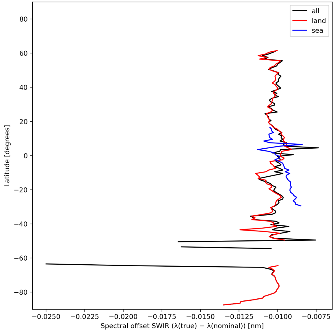
Figure 16: Zonal average of “Spectral offset SWIR ( \lambda(\text{true}) - \lambda(\text{nominal}) )” for 2023-10-28 to 2023-10-29.
