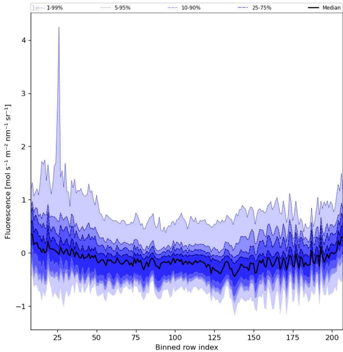
Figure 43: Along track statistics of “Fluorescence” for 2023-10-28 to 2023-10-29
