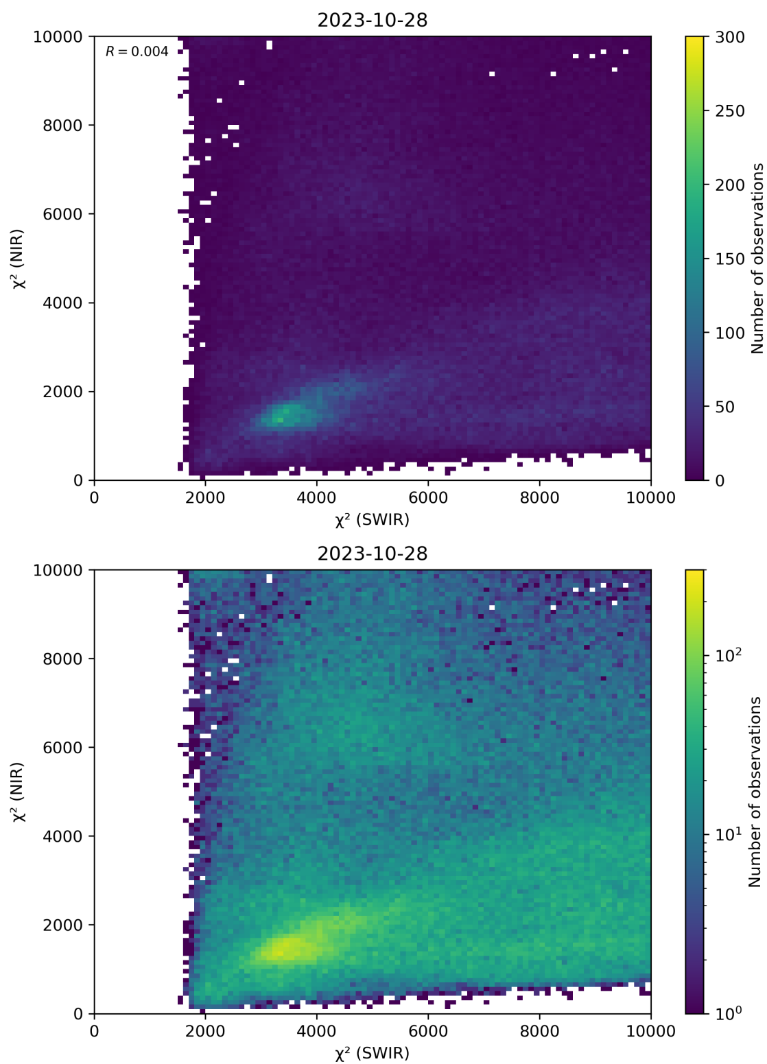
Figure 47: Scatter density plot of “ \chi^2 (SWIR)” against “ \chi^2 (NIR)” for 2023-10-28 to 2023-10-29.
