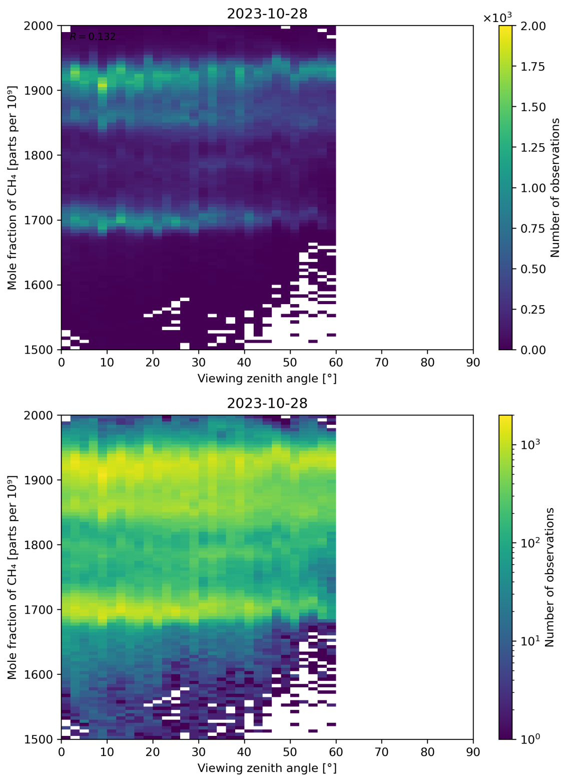
Figure 110: Scatter density plot of “Viewing zenith angle” against “Mole fraction of CH 4 ” for 2023-10-28 to 2023-10-29.
