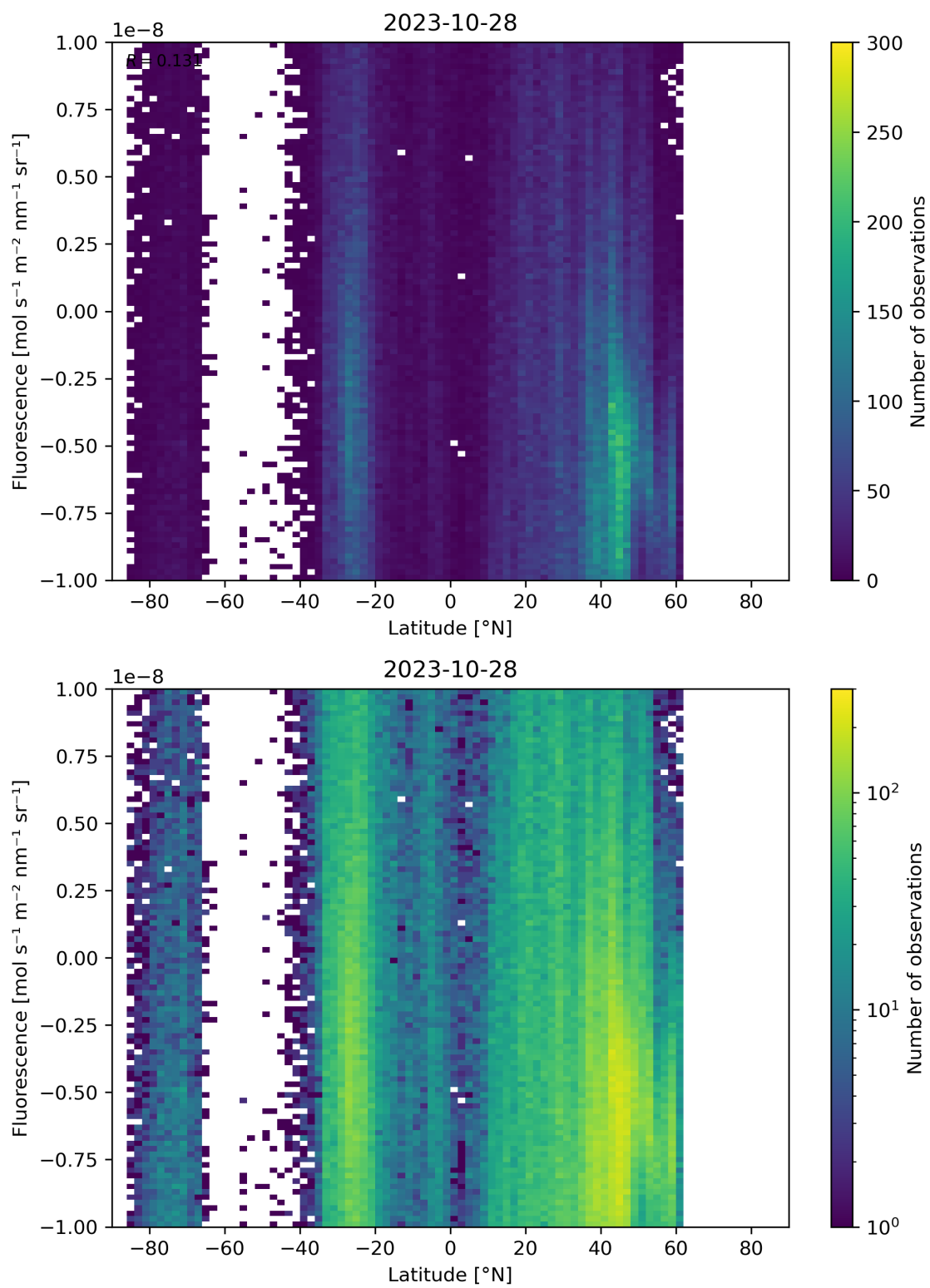
Figure 56: Scatter density plot of “Latitude” against “Fluorescence” for 2023-10-28 to 2023-10-29.
