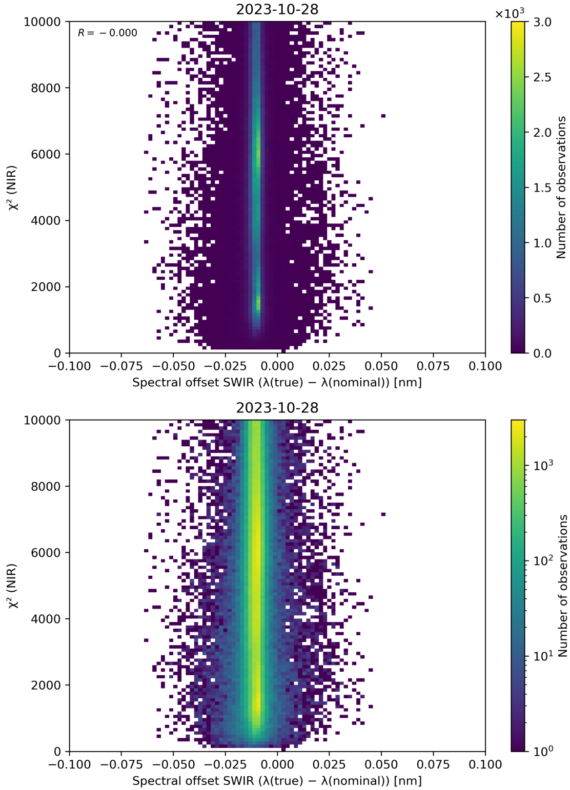
Figure 117: Scatter density plot of “Spectral offset SWIR ( \lambda(\text{true}) - \lambda(\text{nominal}) )” against “ \chi^2 (NIR)” for 2023-10-28 to 2023-10-29.
