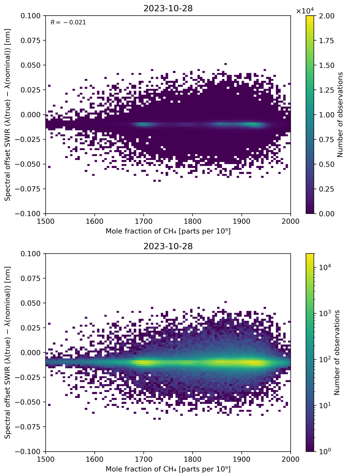
Figure 86: Scatter density plot of “Mole fraction of \text{CH}_4 ” against “Spectral offset SWIR ( \lambda(\text{true}) - \lambda(\text{nominal}) )” for 2023-10-28 to 2023-10-29.
