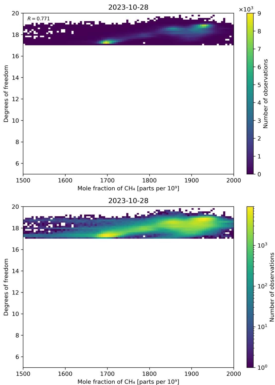
Figure 72: Scatter density plot of “Mole fraction of CH 4 ” against “Degrees of freedom” for 2023-10-28 to 2023-10-29.
