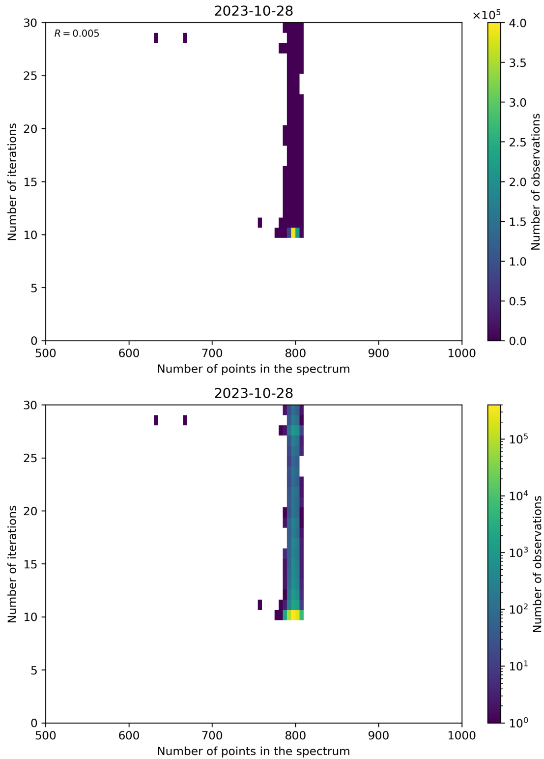
Figure 92: Scatter density plot of “Number of points in the spectrum” against “Number of iterations” for 2023-10-28 to 2023-10-29.
