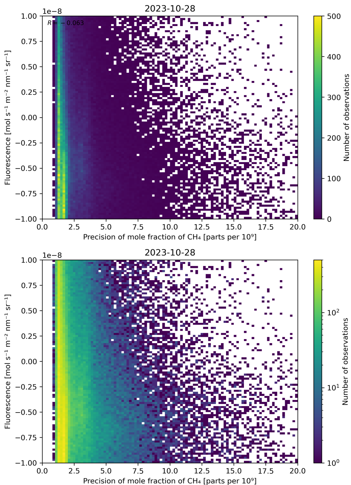
Figure 81: Scatter density plot of “Precision of mole fraction of CH 4 ” against “Fluorescence” for 2023-10-28 to 2023-10-29.
