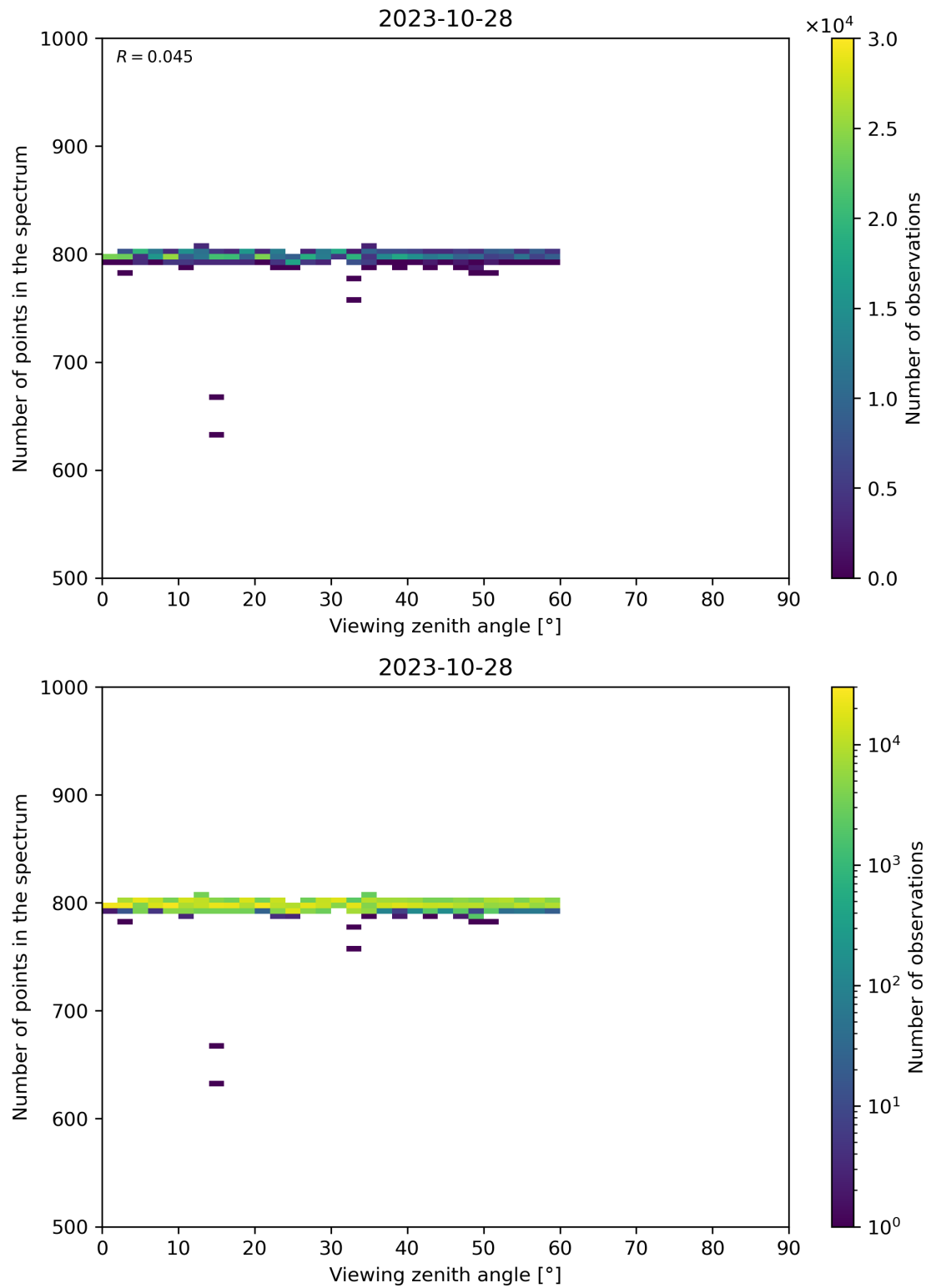
Figure 114: Scatter density plot of “Viewing zenith angle” against “Number of points in the spectrum” for 2023-10-28 to 2023-10-29.
