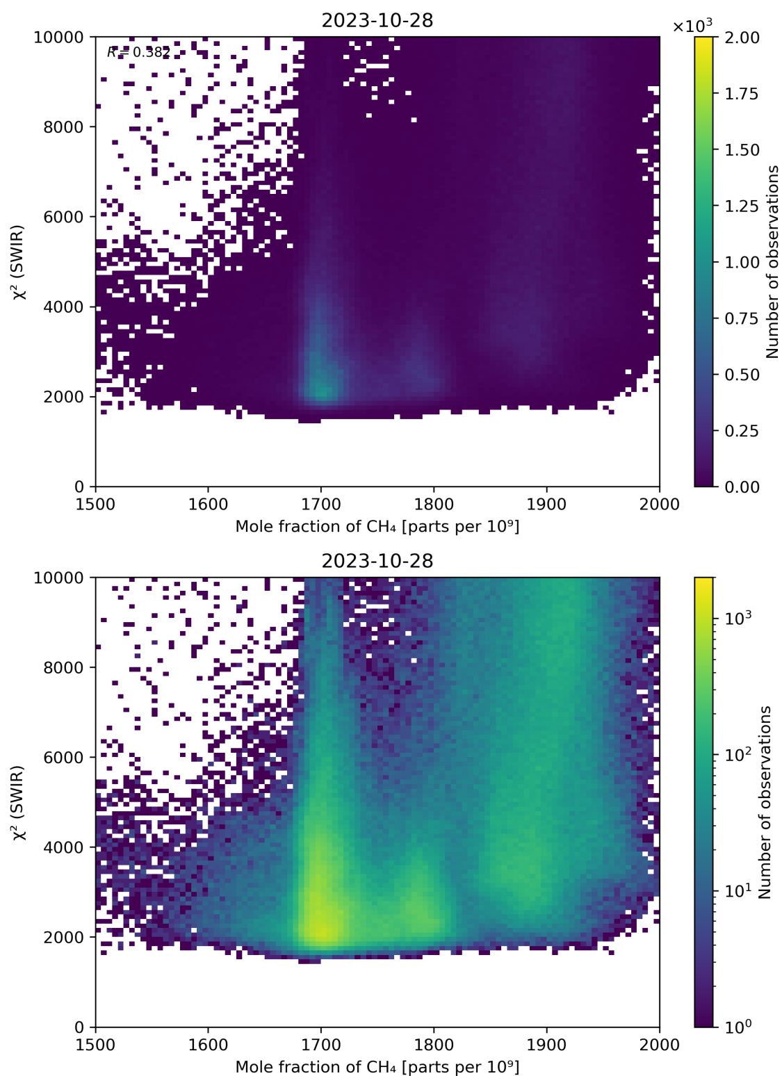
Figure 71: Scatter density plot of “Mole fraction of CH 4 ” against “ \chi^2 (SWIR)” for 2023-10-28 to 2023-10-29.
