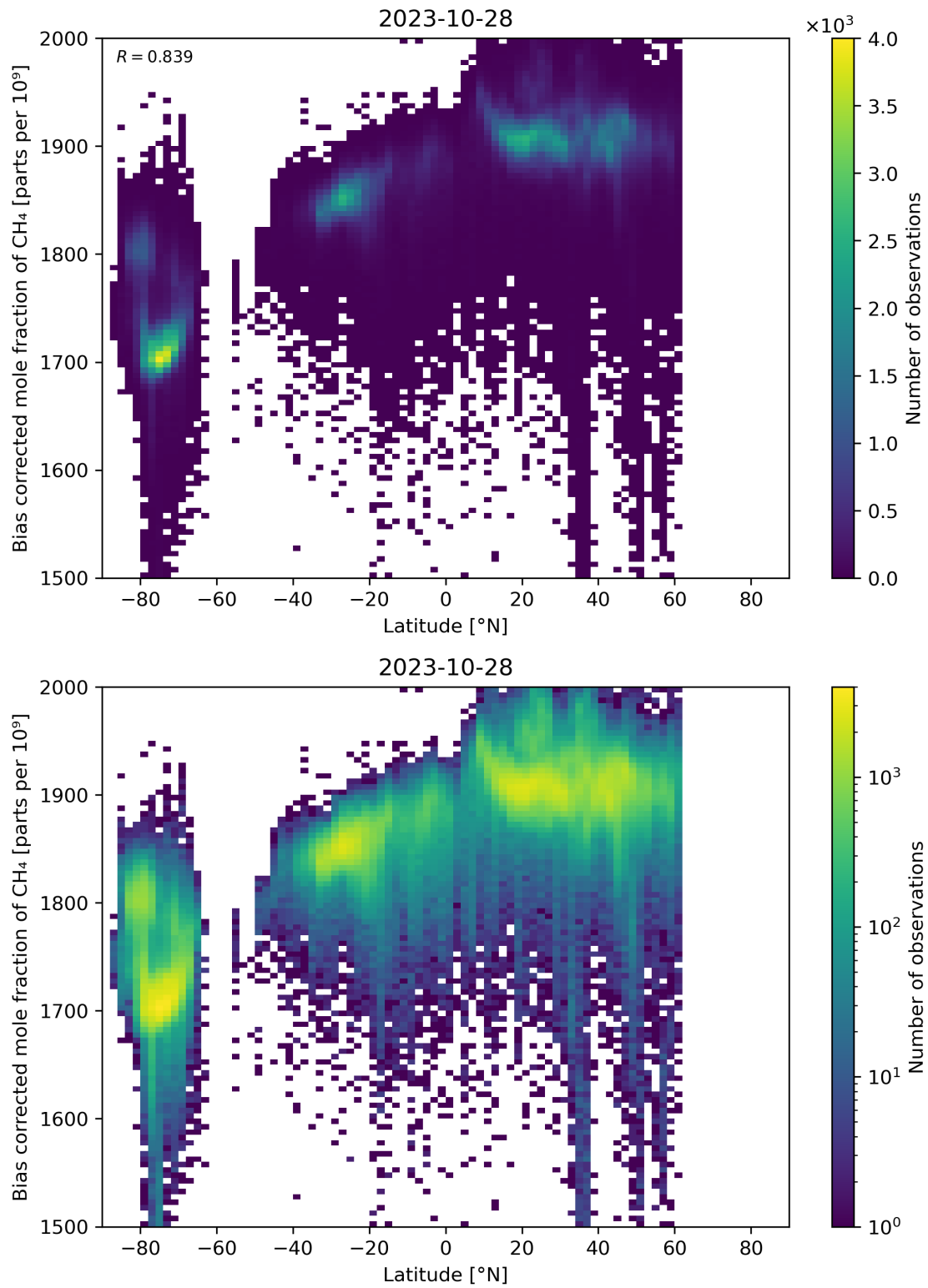
Figure 58: Scatter density plot of “Latitude” against “Bias corrected mole fraction of CH 4 ” for 2023-10-28 to 2023-10-29.
