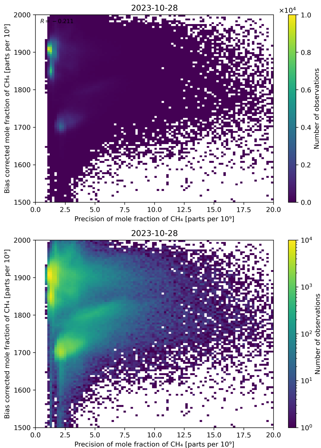
Figure 82: Scatter density plot of “Precision of mole fraction of CH 4 ” against “Bias corrected mole fraction of CH 4 ” for 2023-10-28 to 2023-10-29.
