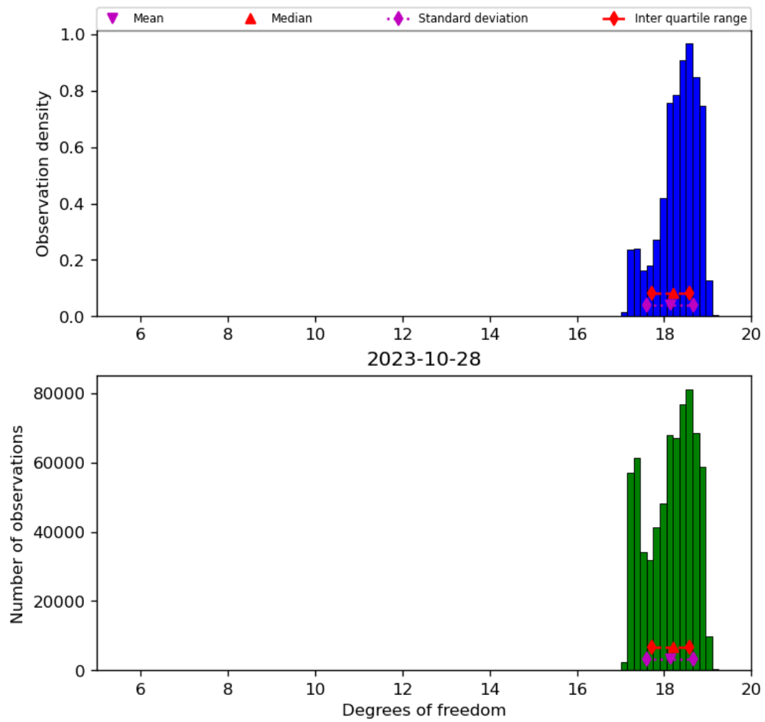
Figure 30: Histogram of “Degrees of freedom” for 2023-10-28 to 2023-10-29
