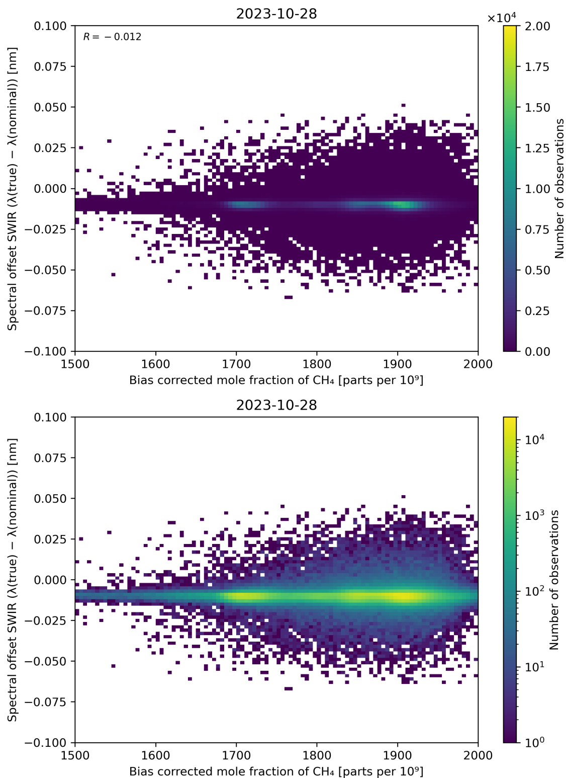
Figure 69: Scatter density plot of “Bias corrected mole fraction of \text{CH}_4 ” against “Spectral offset SWIR ( \lambda(\text{true}) - \lambda(\text{nominal}) )” for 2023-10-28 to 2023-10-29.
