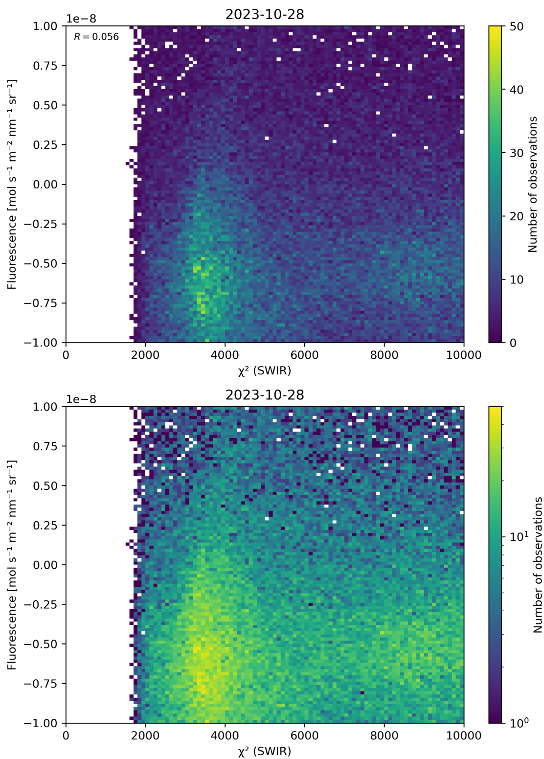
Figure 49: Scatter density plot of “ \chi^2 (SWIR)” against “Fluorescence” for 2023-10-28 to 2023-10-29.
