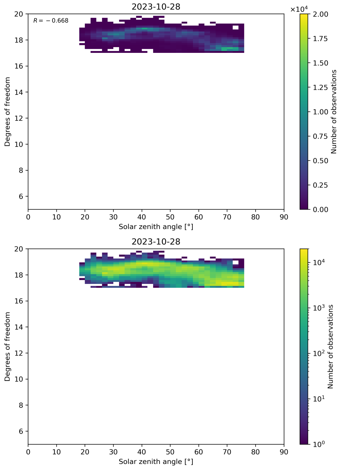
Figure 96: Scatter density plot of “Solar zenith angle” against “Degrees of freedom” for 2023-10-28 to 2023-10-29.
