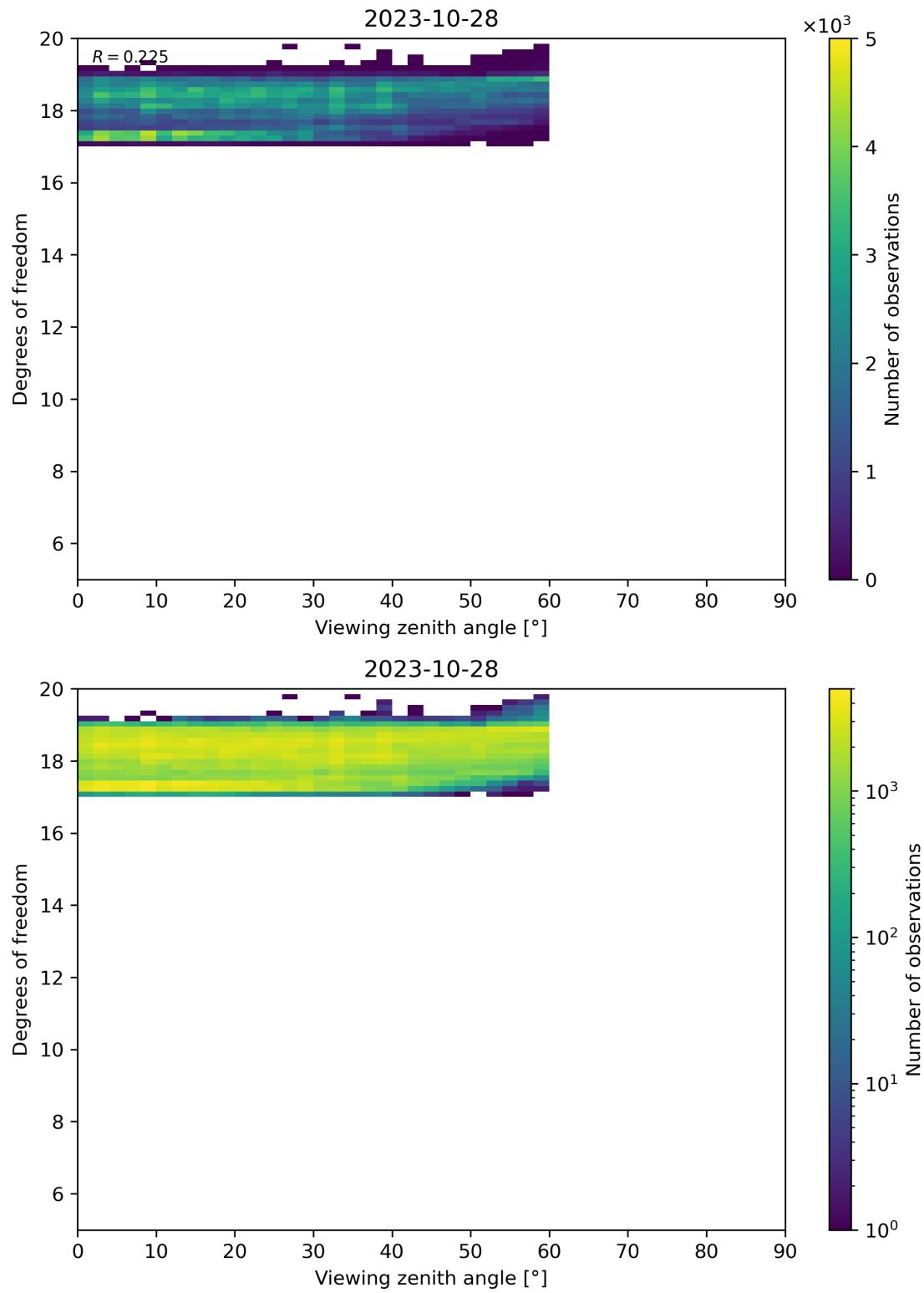
Figure 107: Scatter density plot of “Viewing zenith angle” against “Degrees of freedom” for 2023-10-28 to 2023-10-29.
