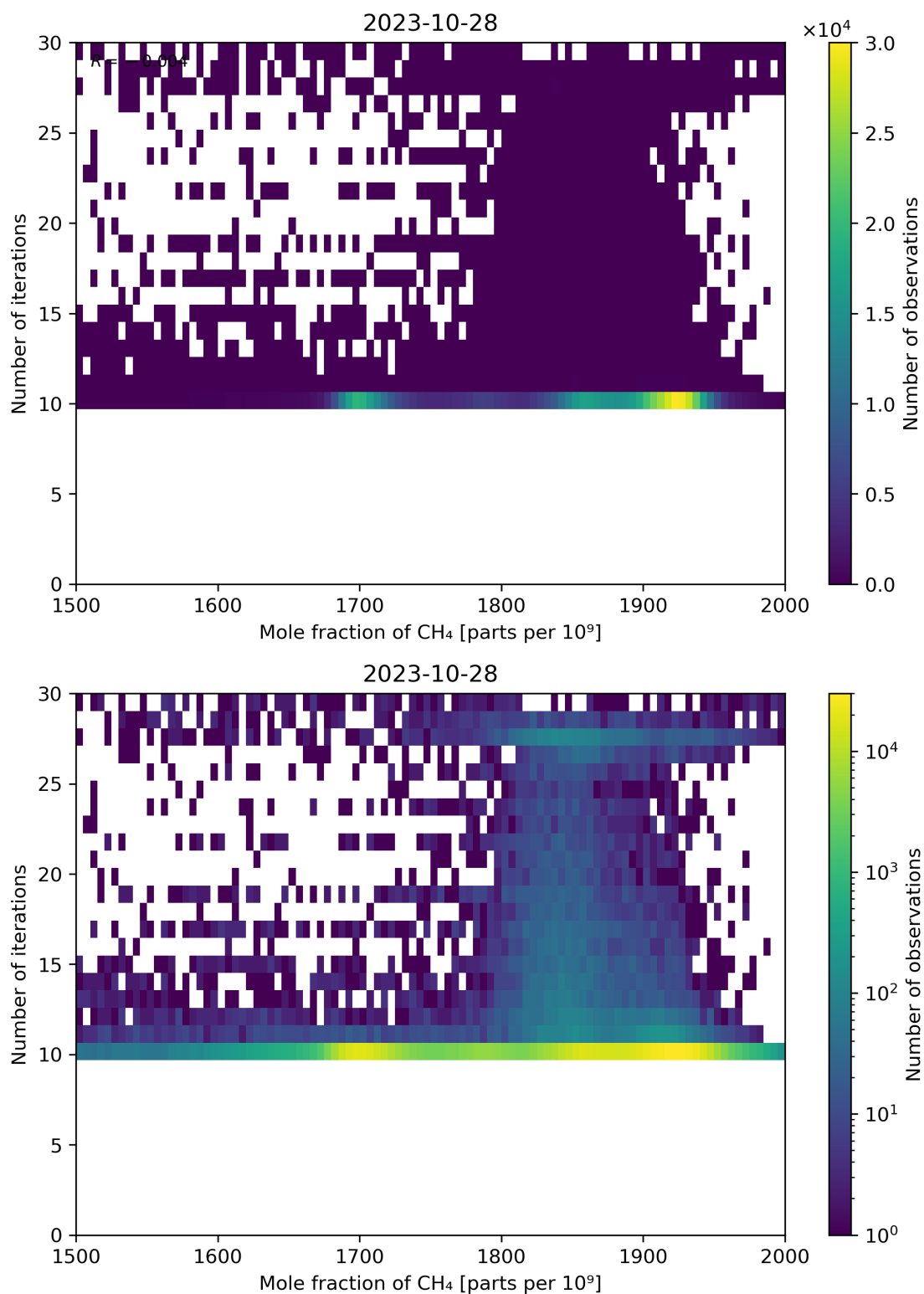
Figure 76: Scatter density plot of “Mole fraction of CH 4 ” against “Number of iterations” for 2023-10-28 to 2023-10-29.
