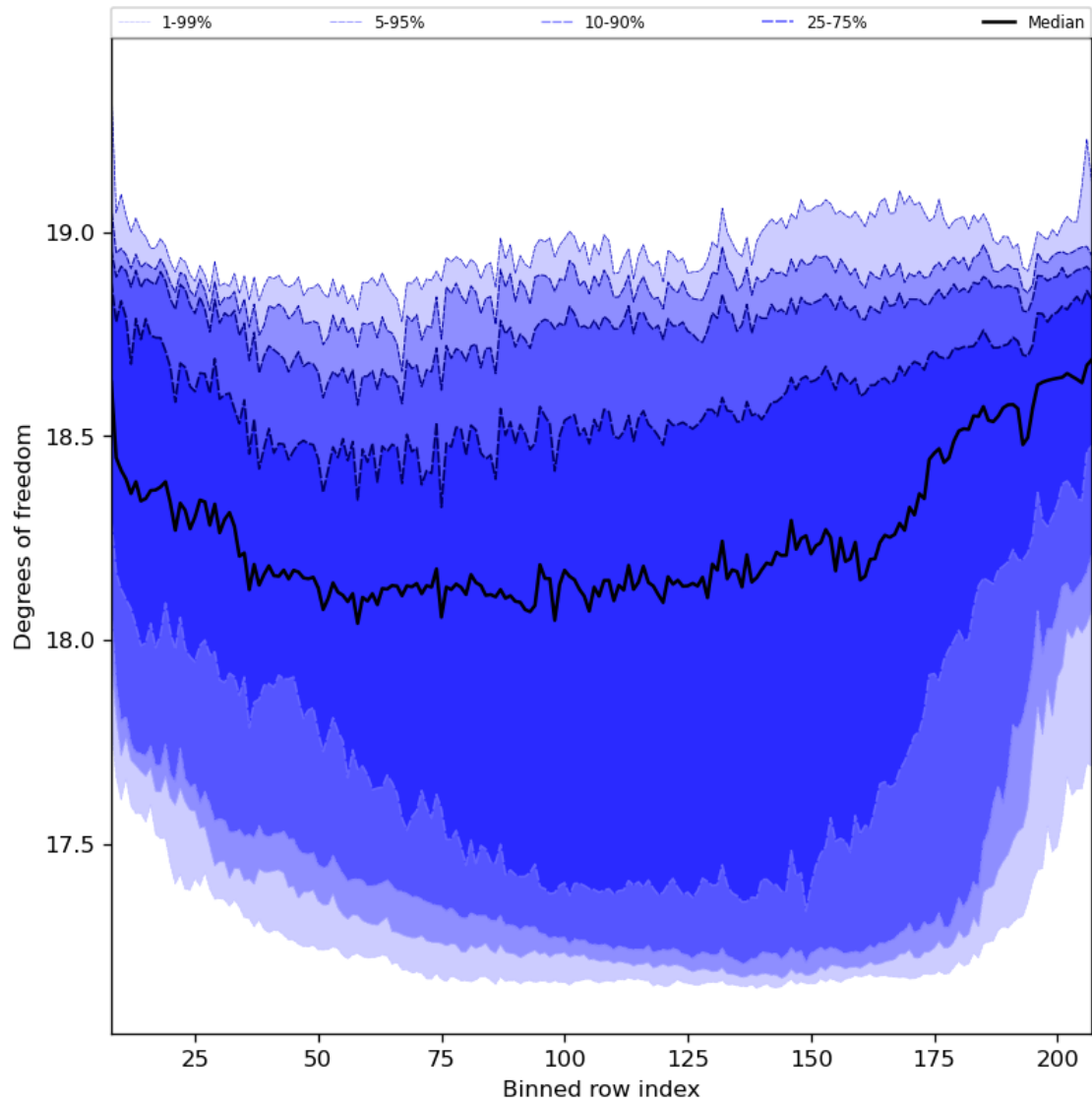
Figure 41: Along track statistics of “Degrees of freedom” for 2023-10-28 to 2023-10-29
