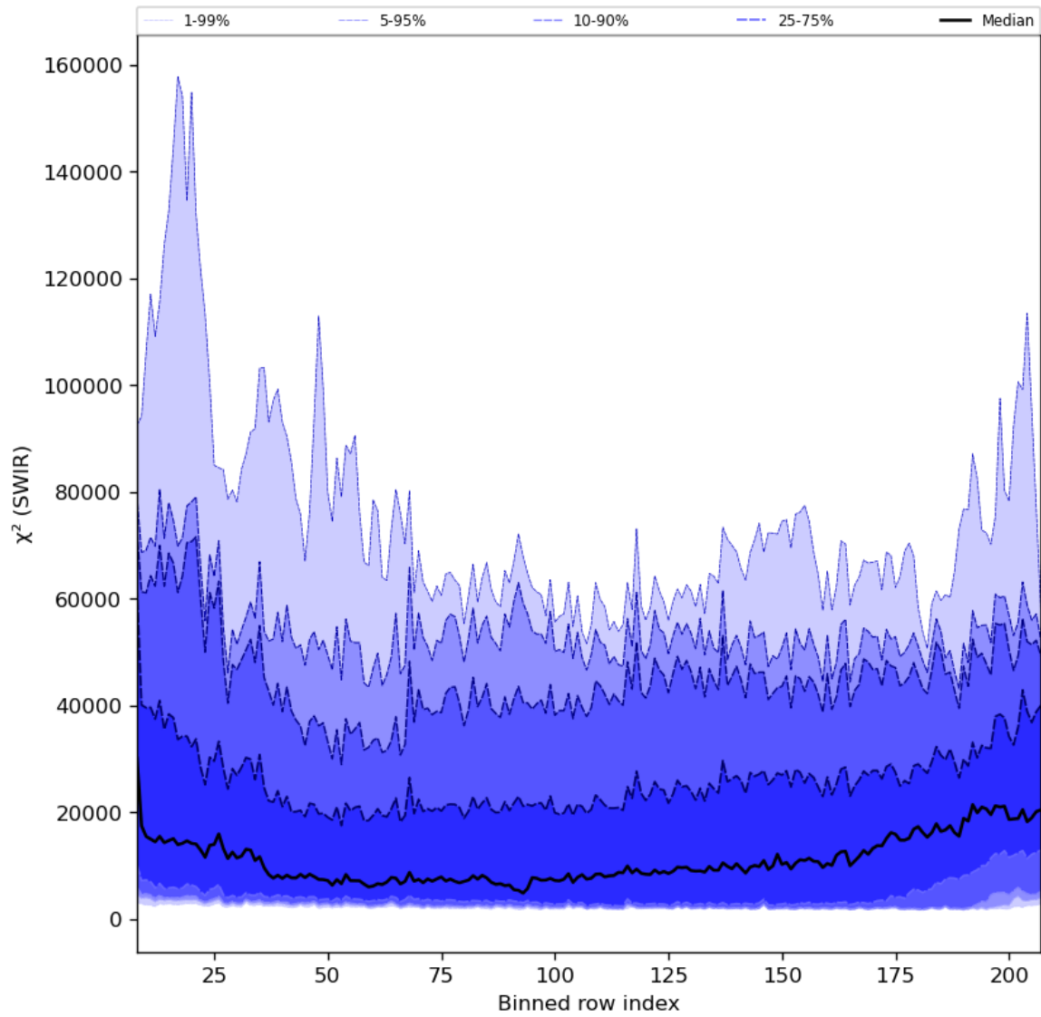
Figure 39: Along track statistics of “ \chi^2 (SWIR)” for 2023-10-28 to 2023-10-29
