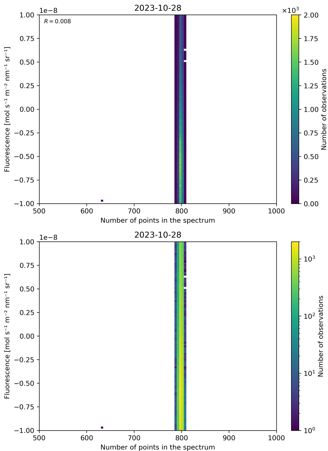
Figure 91: Scatter density plot of “Number of points in the spectrum” against “Fluorescence” for 2023-10-28 to 2023-10-29.
