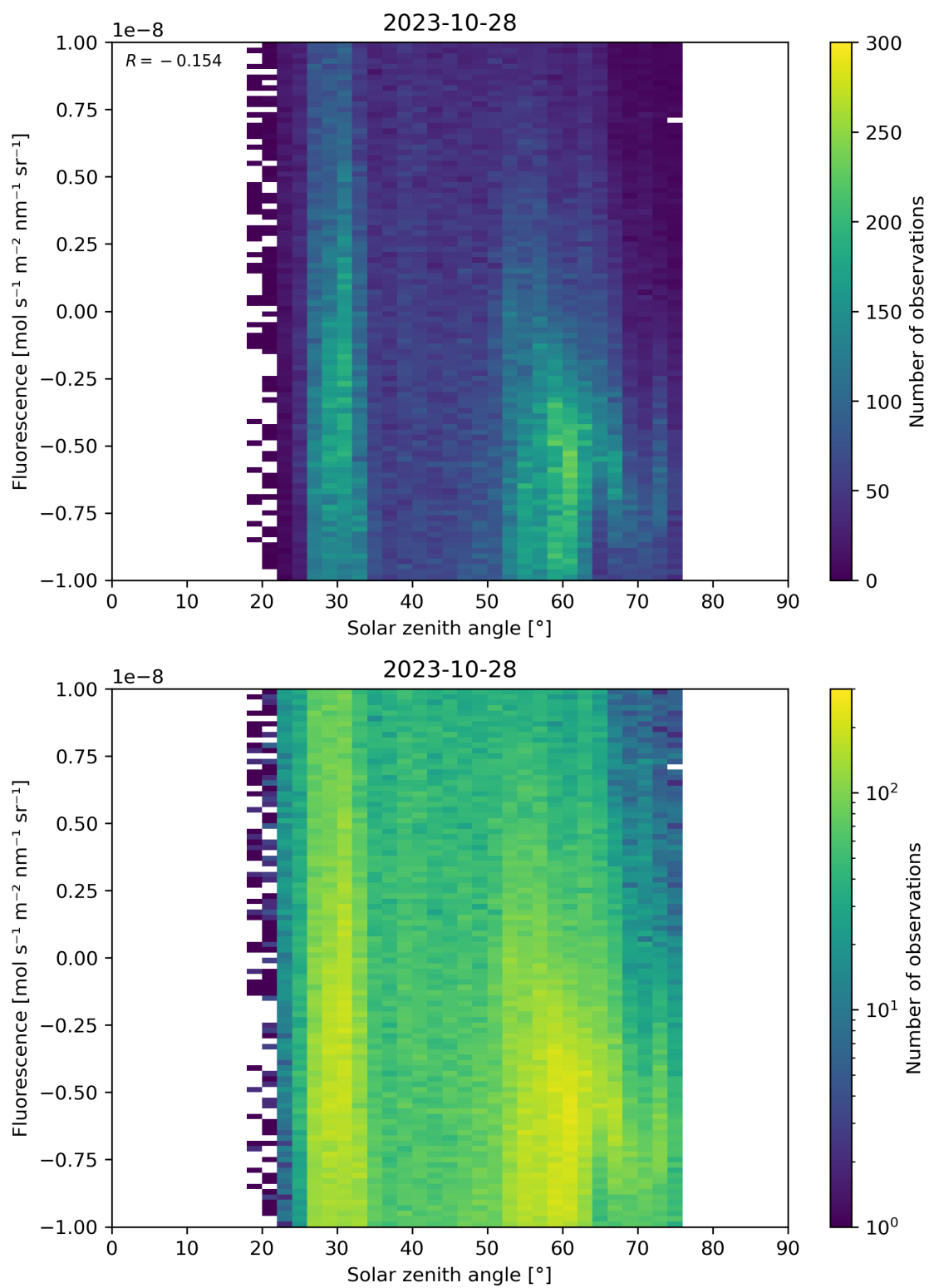
Figure 97: Scatter density plot of “Solar zenith angle” against “Fluorescence” for 2023-10-28 to 2023-10-29.
