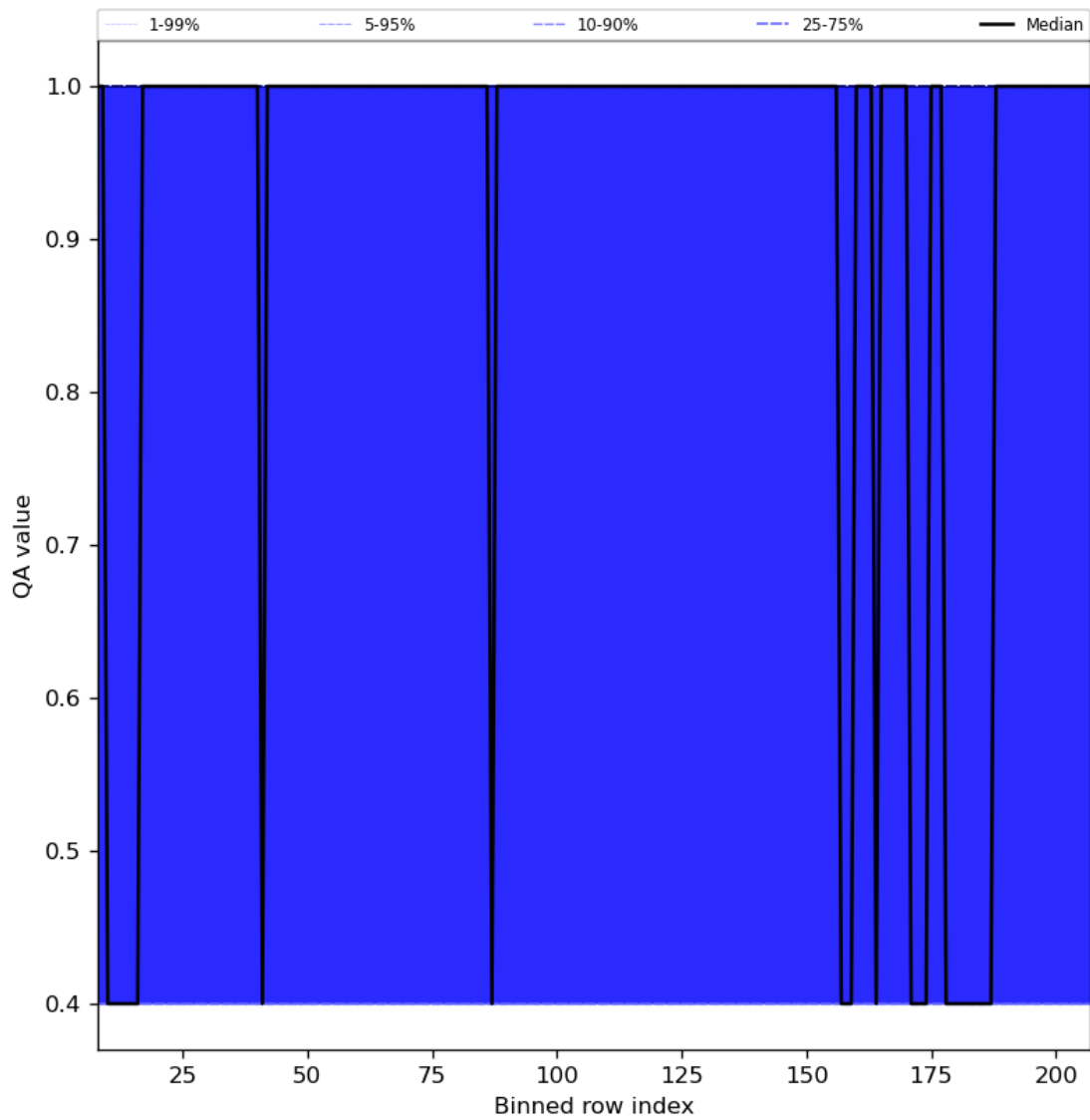
Figure 33: Along track statistics of “QA value” for 2023-10-28 to 2023-10-29
