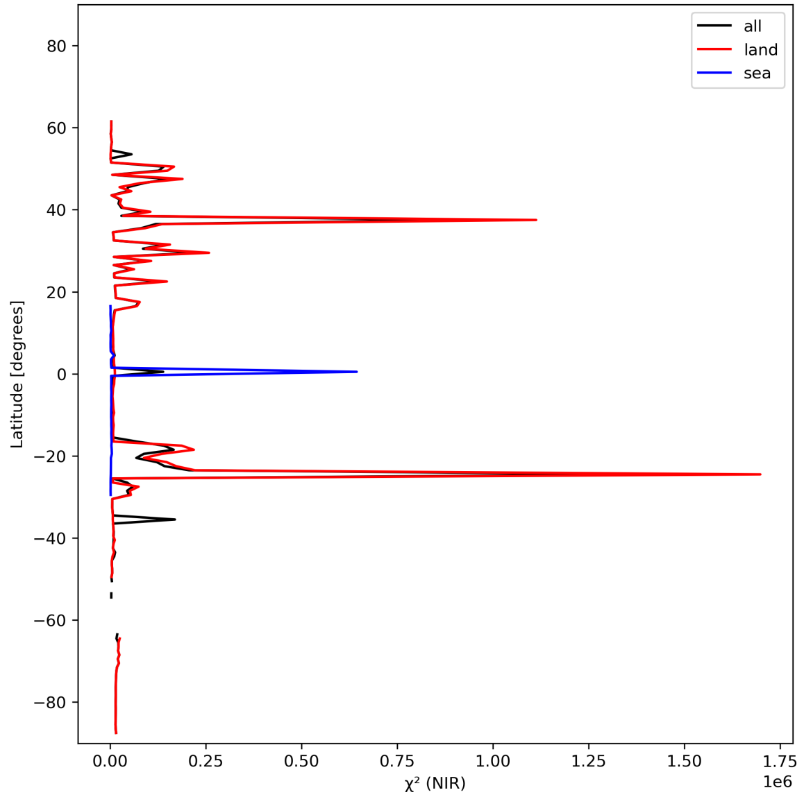
Figure 18: Zonal average of “ \chi^2 (NIR)” for 2023-10-28 to 2023-10-29.
