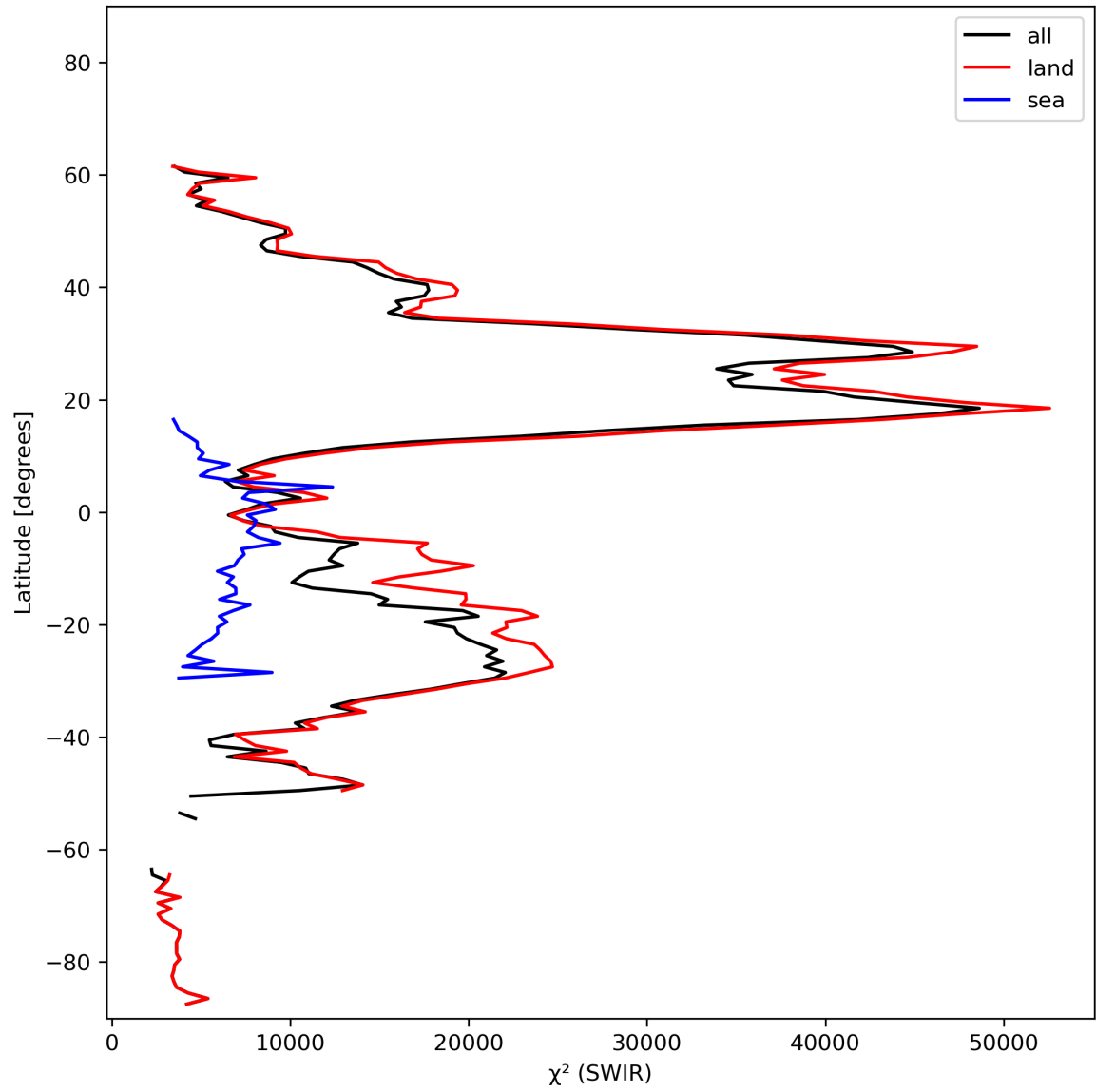
Figure 17: Zonal average of “ \chi^2 (SWIR)” for 2023-10-28 to 2023-10-29.
