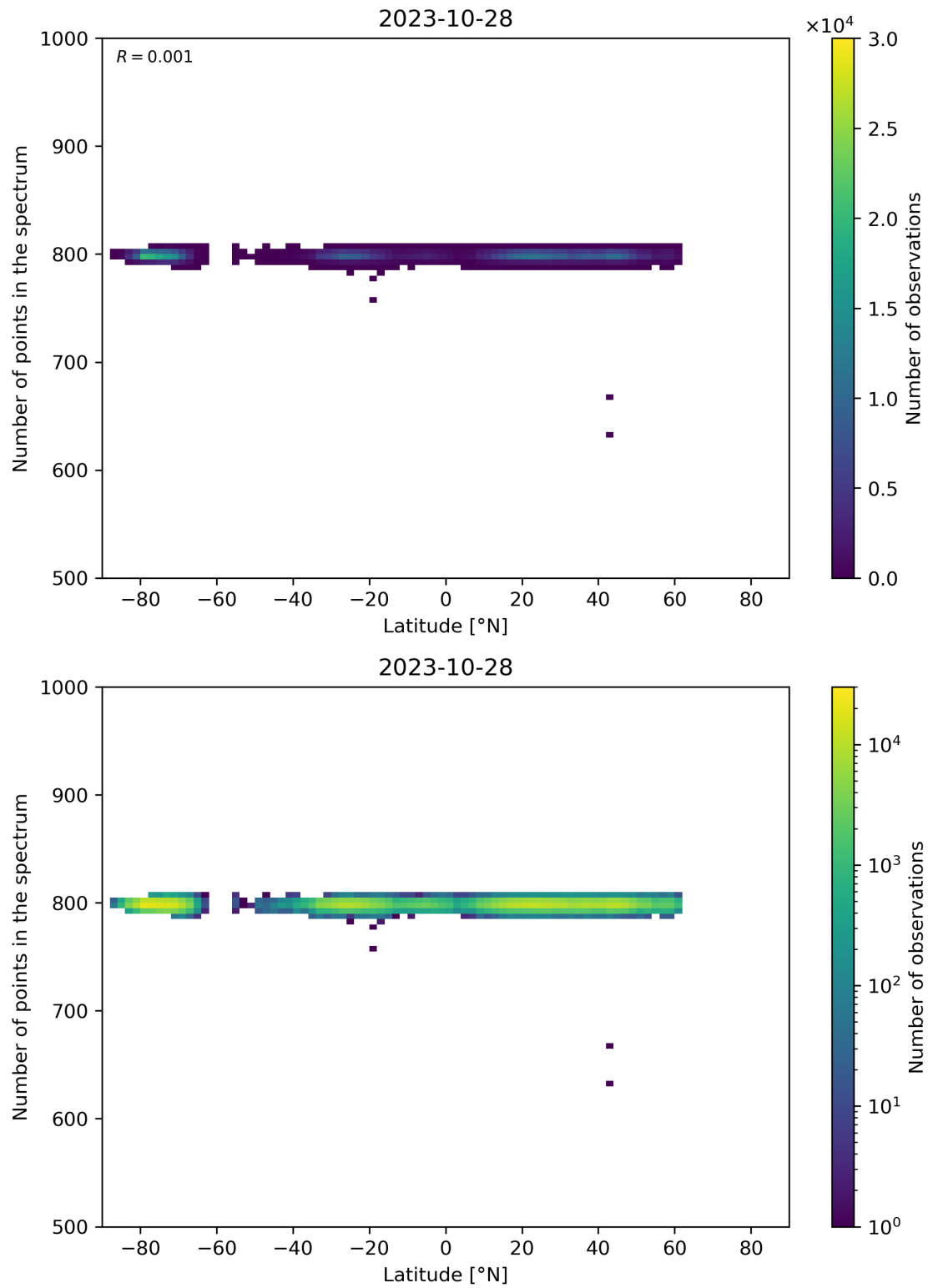
Figure 61: Scatter density plot of “Latitude” against “Number of points in the spectrum” for 2023-10-28 to 2023-10-29.
