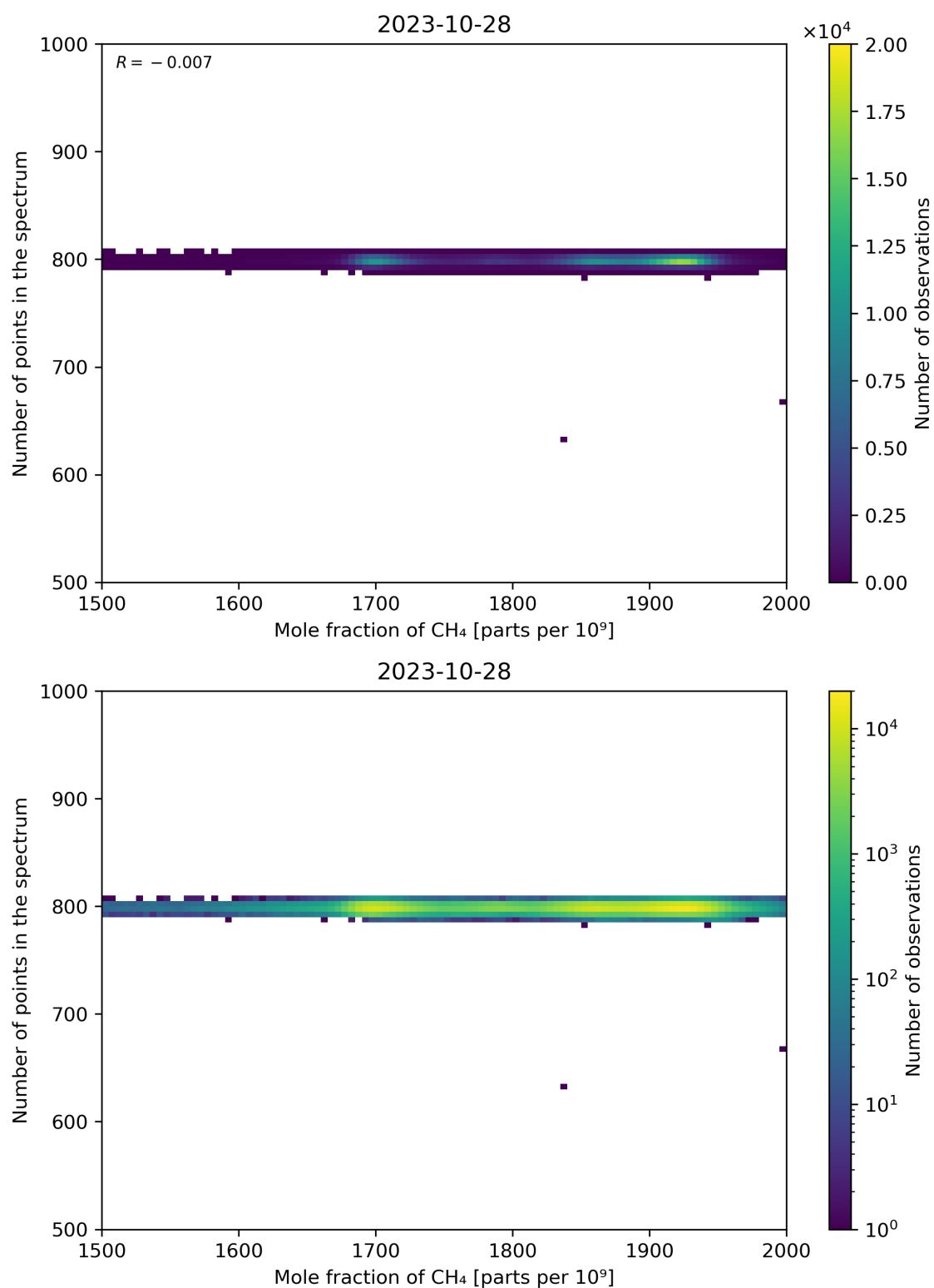
Figure 77: Scatter density plot of “Mole fraction of CH 4 ” against “Number of points in the spectrum” for 2023-10-28 to 2023-10-29.
