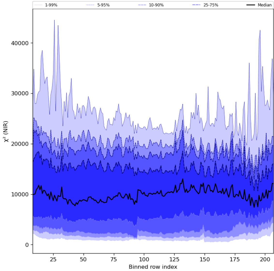
Figure 40: Along track statistics of " \chi^2 (NIR)" for 2023-10-28 to 2023-10-29
