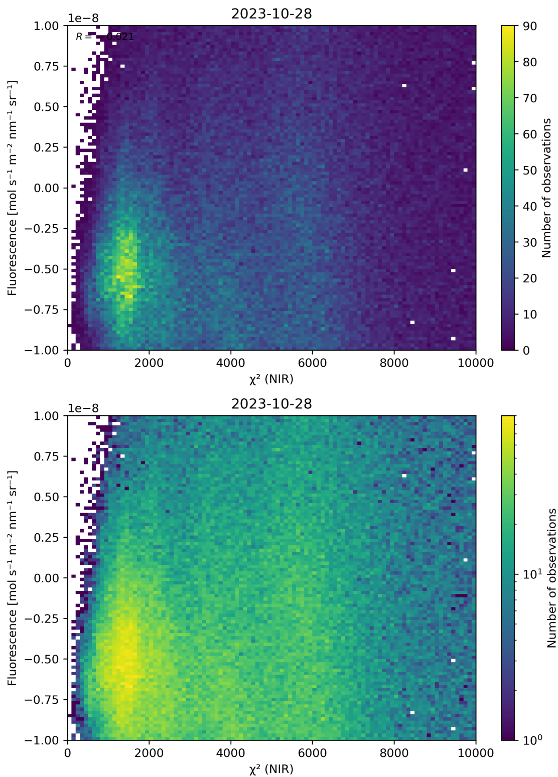
Figure 45: Scatter density plot of “ \chi^2 (NIR)” against “Fluorescence” for 2023-10-28 to 2023-10-29.
