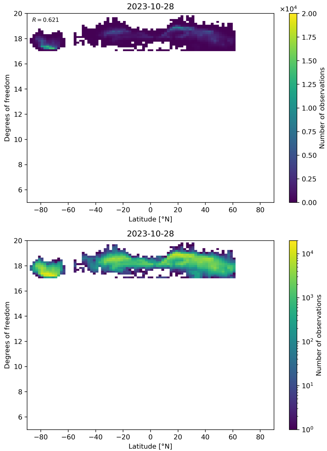
Figure 55: Scatter density plot of “Latitude” against “Degrees of freedom” for 2023-10-28 to 2023-10-29.
