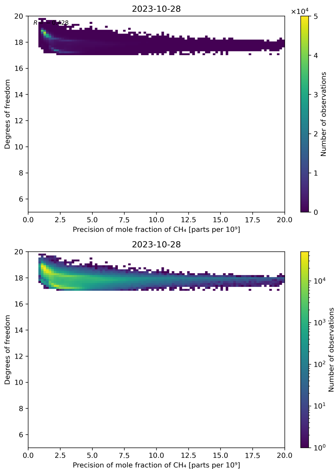
Figure 80: Scatter density plot of “Precision of mole fraction of CH 4 ” against “Degrees of freedom” for 2023-10-28 to 2023-10-29.
