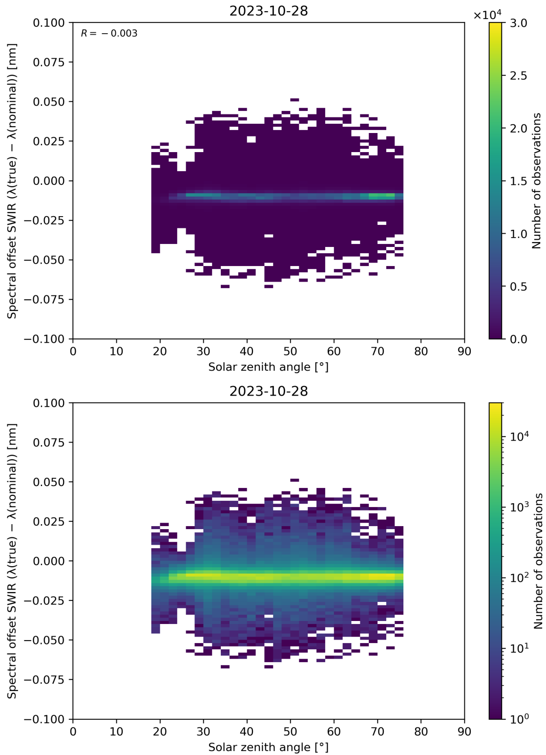
Figure 104: Scatter density plot of “Solar zenith angle” against “Spectral offset SWIR ( \lambda(\text{true}) - \lambda(\text{nominal}) )” for 2023-10-28 to 2023-10-29.
