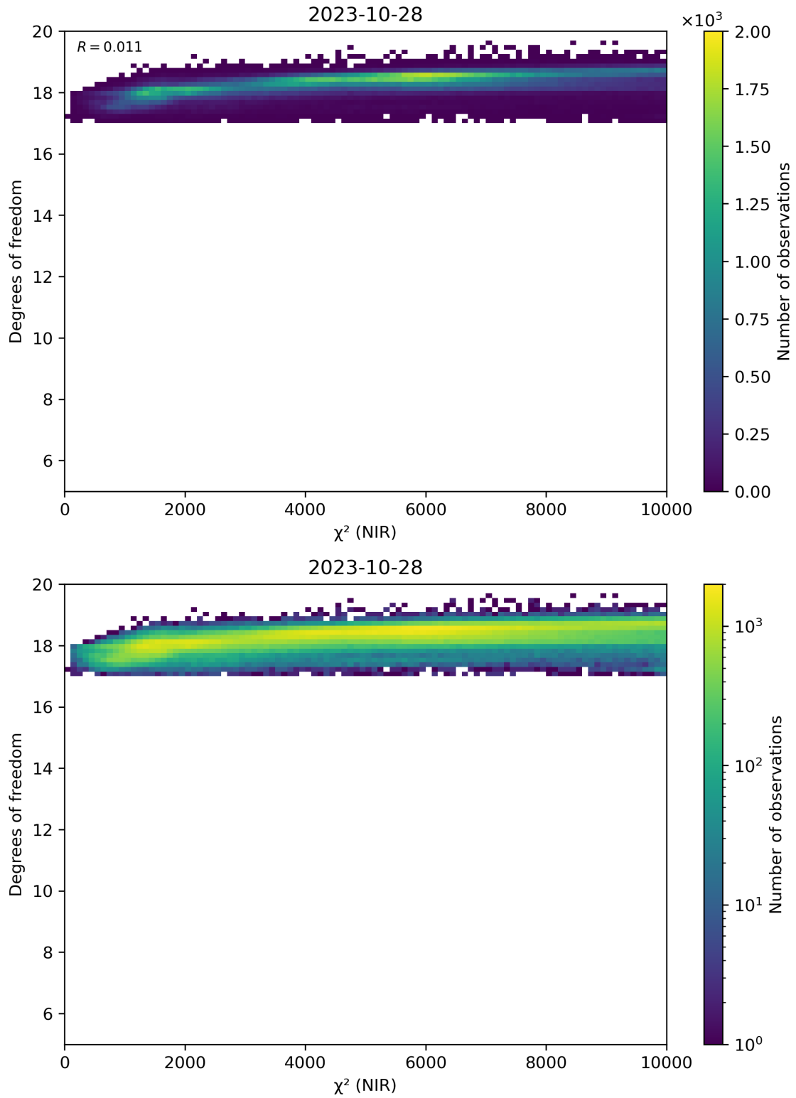
Figure 44: Scatter density plot of “ \chi^2 (NIR)” against “Degrees of freedom” for 2023-10-28 to 2023-10-29.
