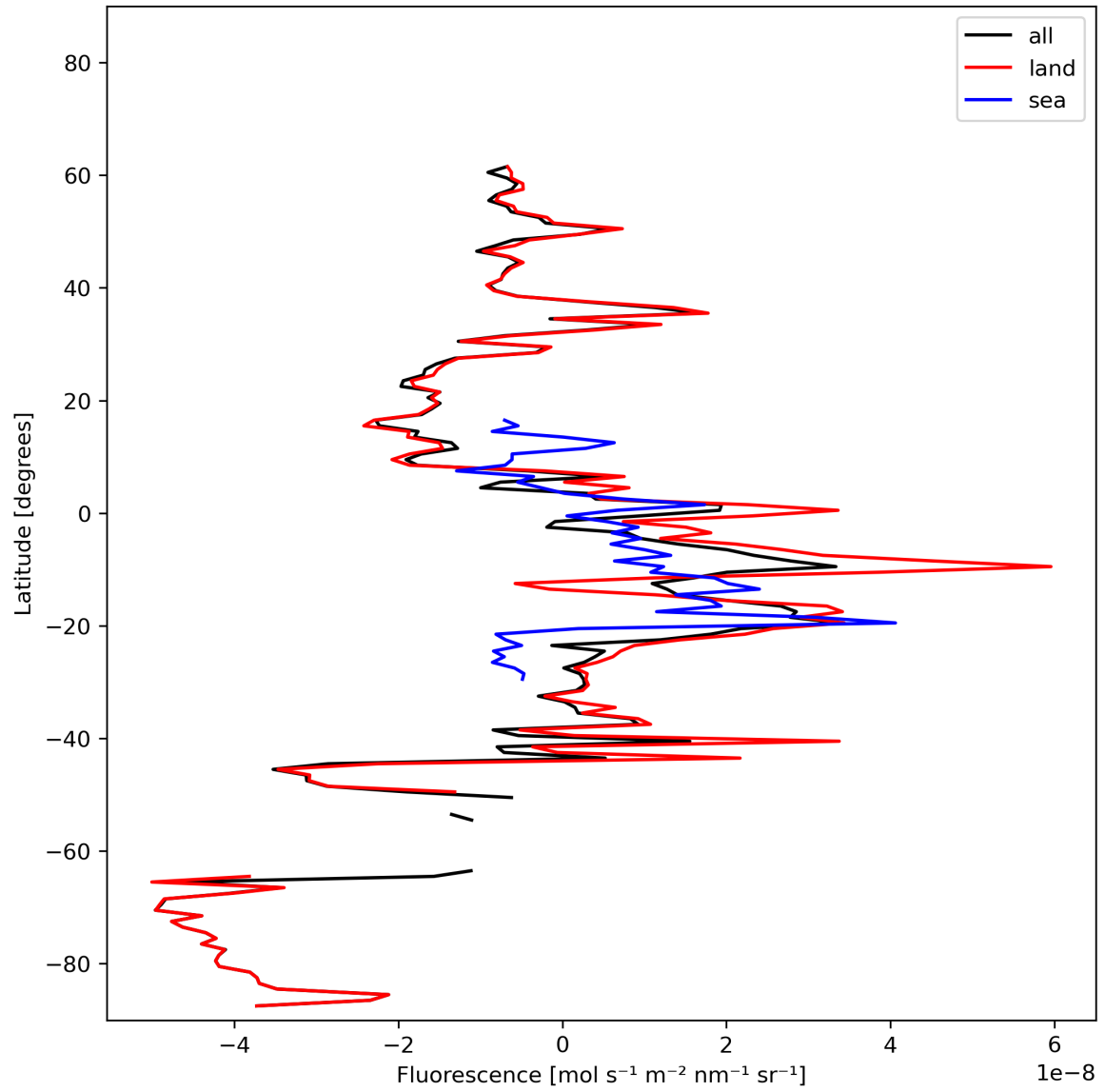
Figure 21: Zonal average of “Fluorescence” for 2023-10-28 to 2023-10-29.
