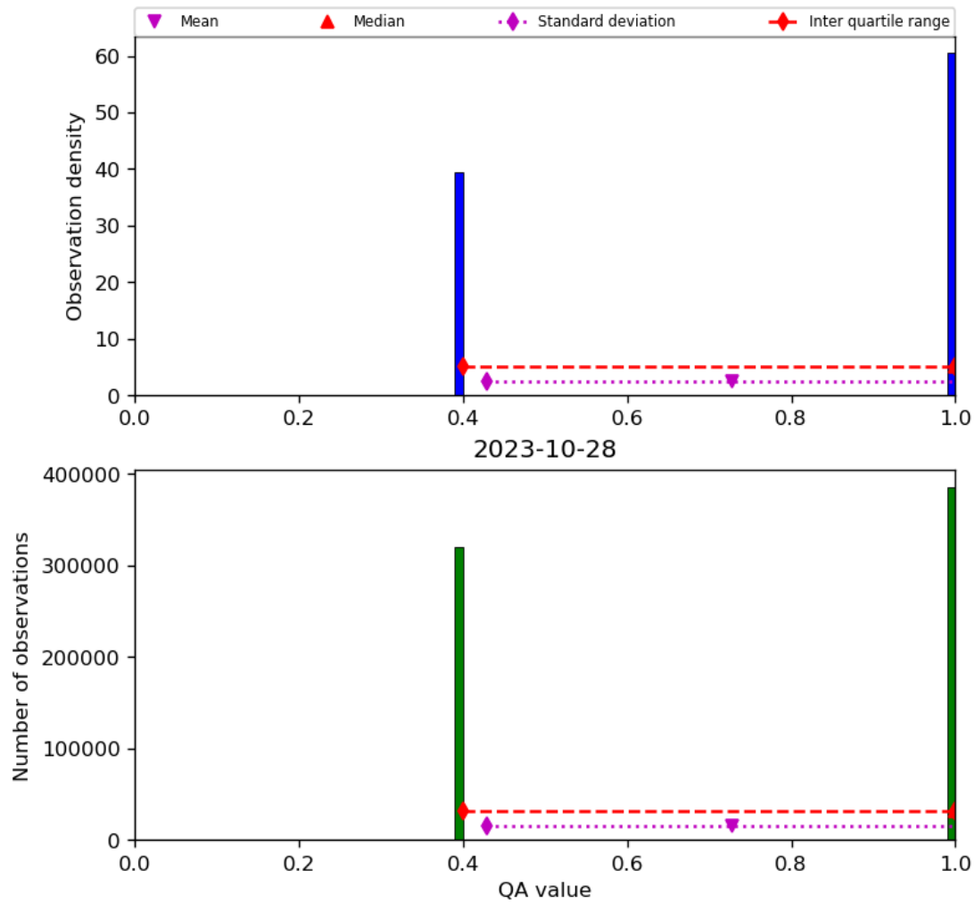
Figure 22: Histogram of “QA value” for 2023-10-28 to 2023-10-29
