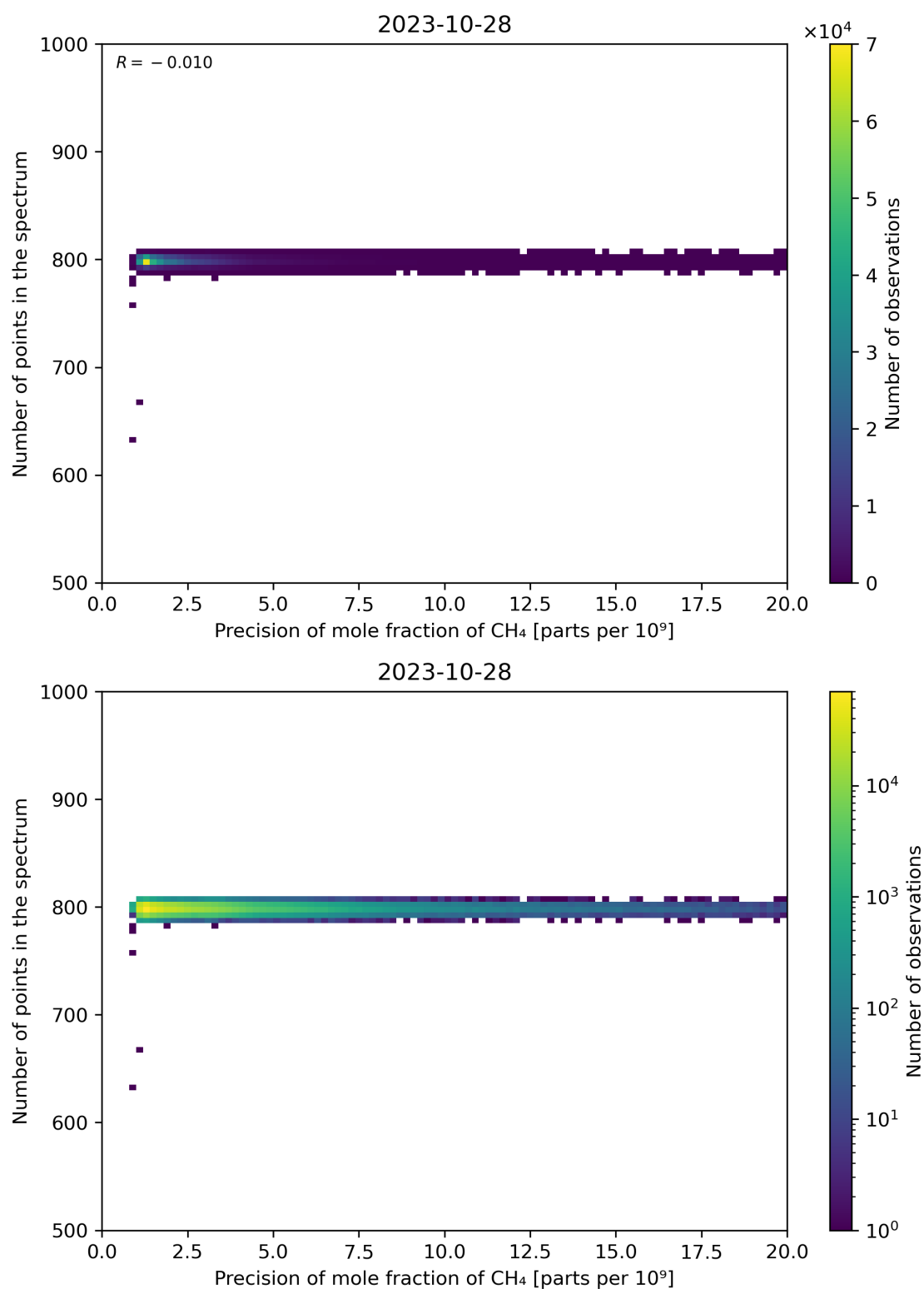
Figure 84: Scatter density plot of “Precision of mole fraction of CH 4 ” against “Number of points in the spectrum” for 2023-10-28 to 2023-10-29.
