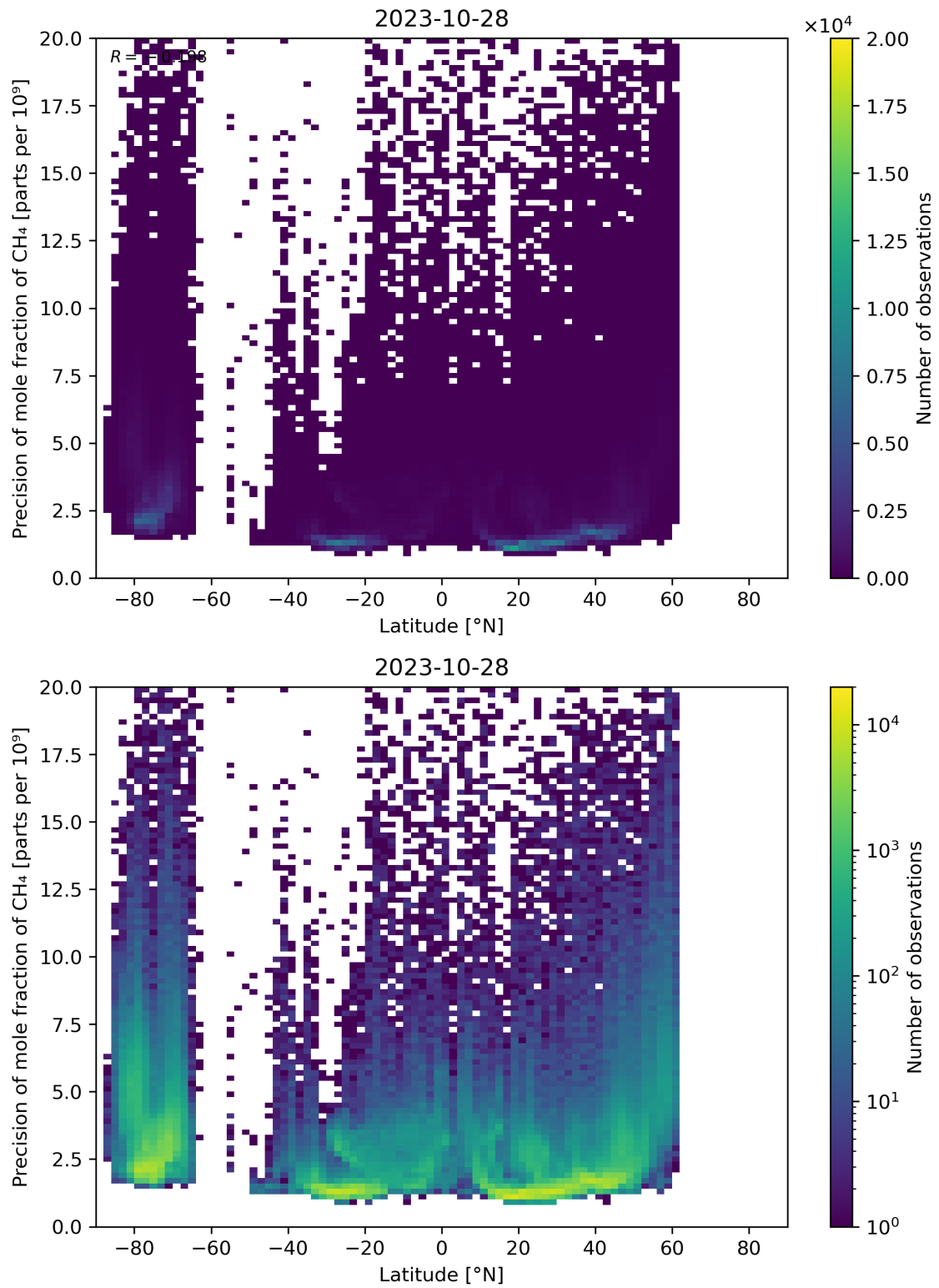
Figure 59: Scatter density plot of “Latitude” against “Precision of mole fraction of CH 4 ” for 2023-10-28 to 2023-10-29.
