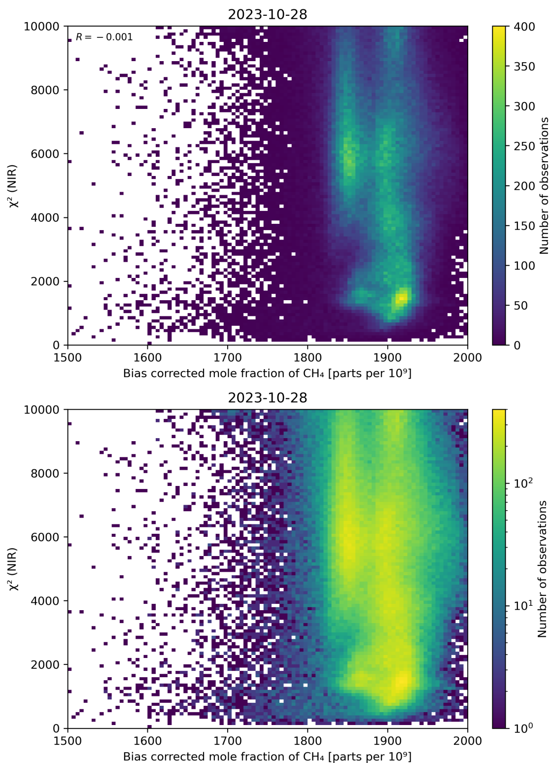
Figure 63: Scatter density plot of “Bias corrected mole fraction of CH 4 ” against “ \chi^2 (NIR)” for 2023-10-28 to 2023-10-29.
