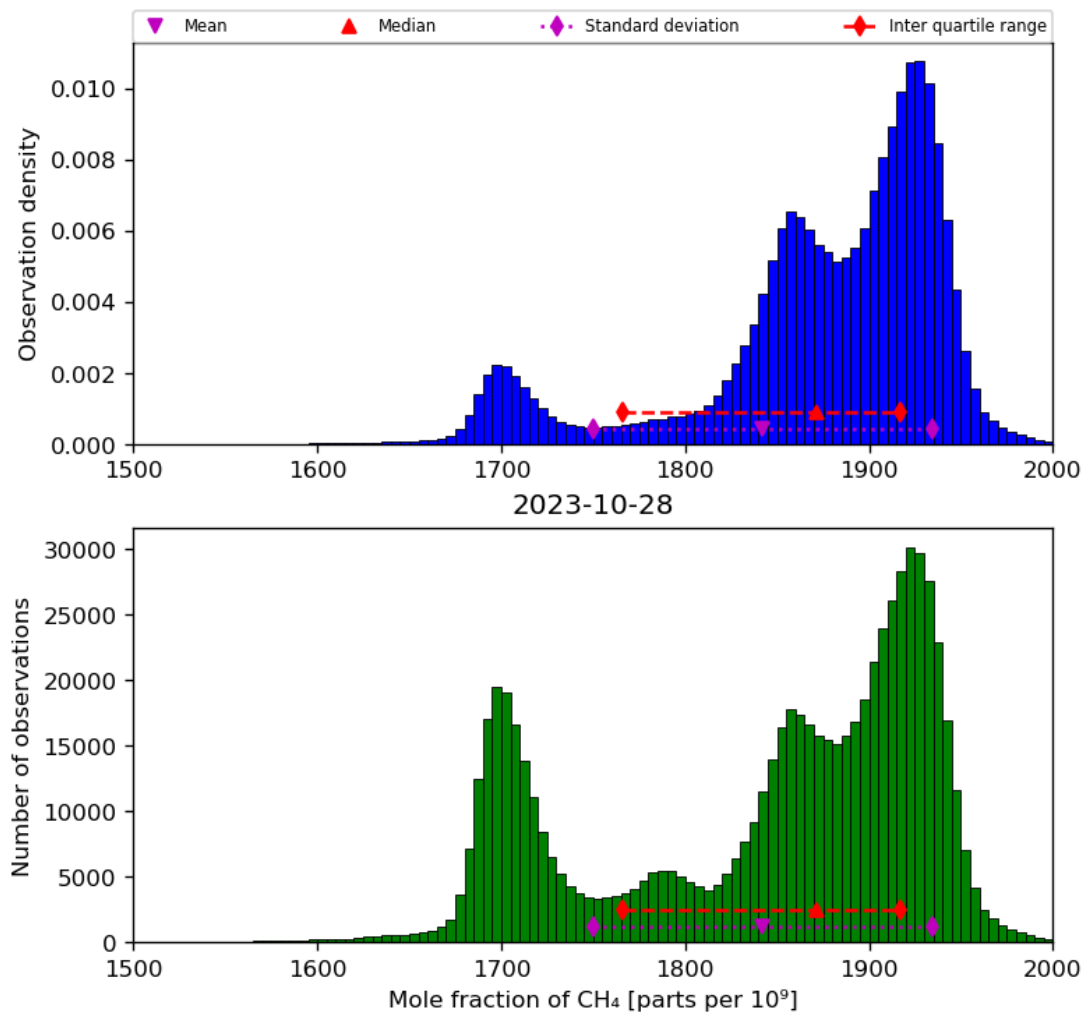
Figure 23: Histogram of “Mole fraction of CH 4 ” for 2023-10-28 to 2023-10-29
