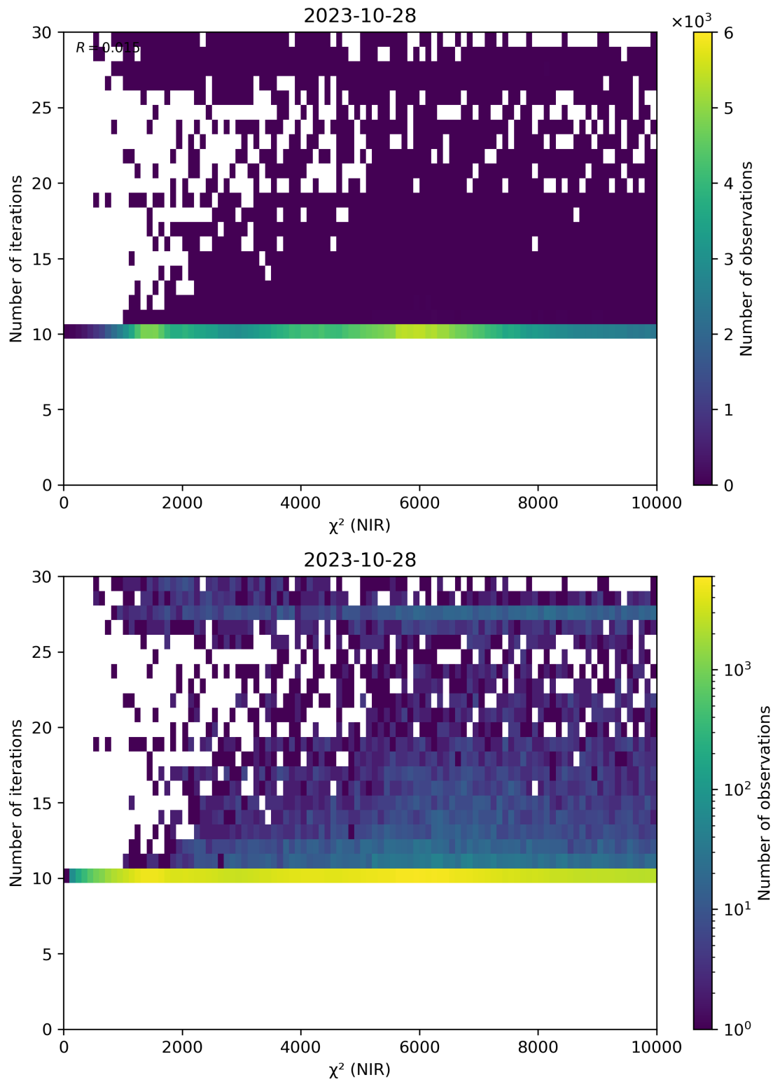
Figure 46: Scatter density plot of “ \chi^2 (NIR)” against “Number of iterations” for 2023-10-28 to 2023-10-29.
