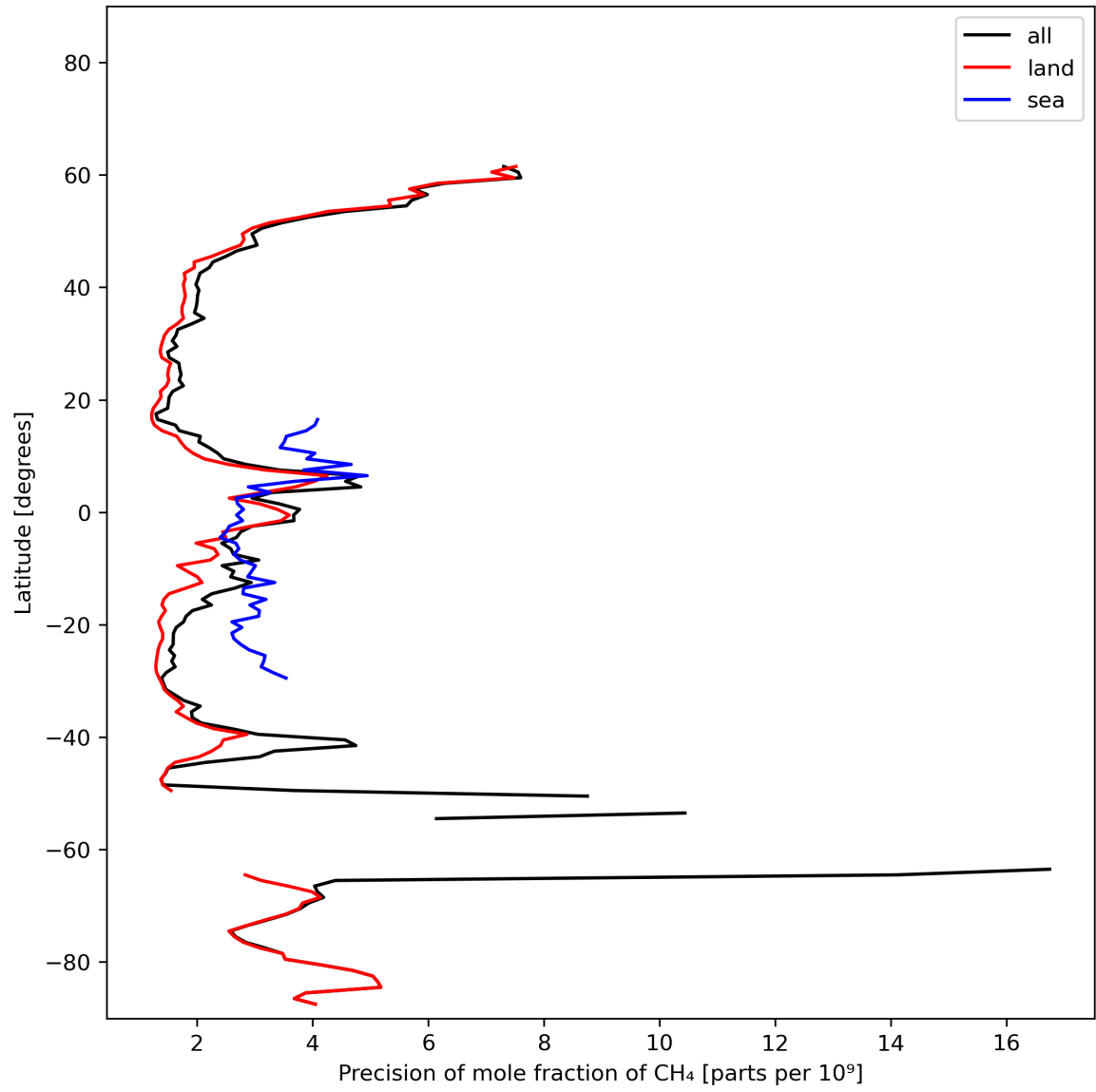
Figure 13: Zonal average of “Precision of mole fraction of \text{CH}_4 ” for 2023-10-28 to 2023-10-29.
