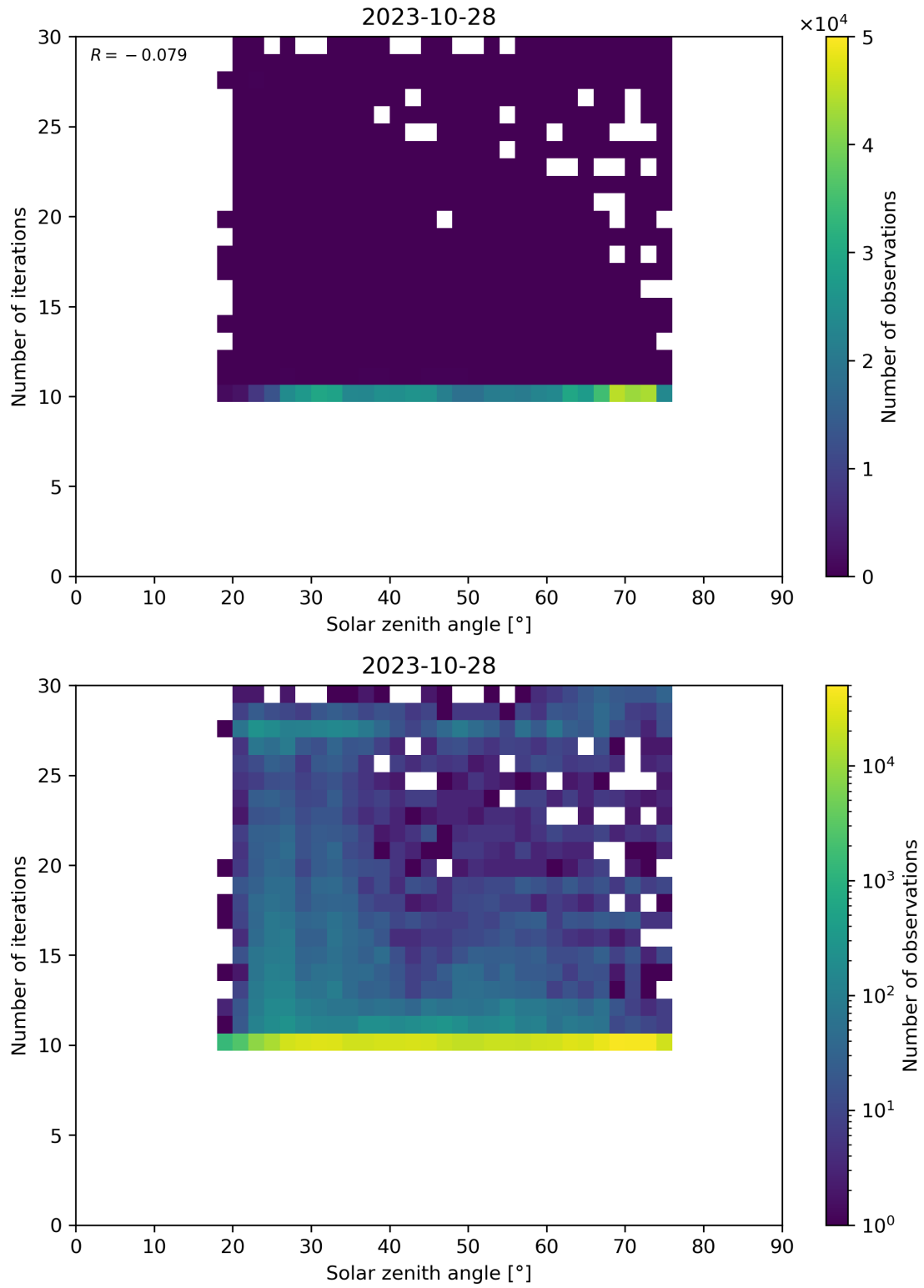
Figure 102: Scatter density plot of “Solar zenith angle” against “Number of iterations” for 2023-10-28 to 2023-10-29.
