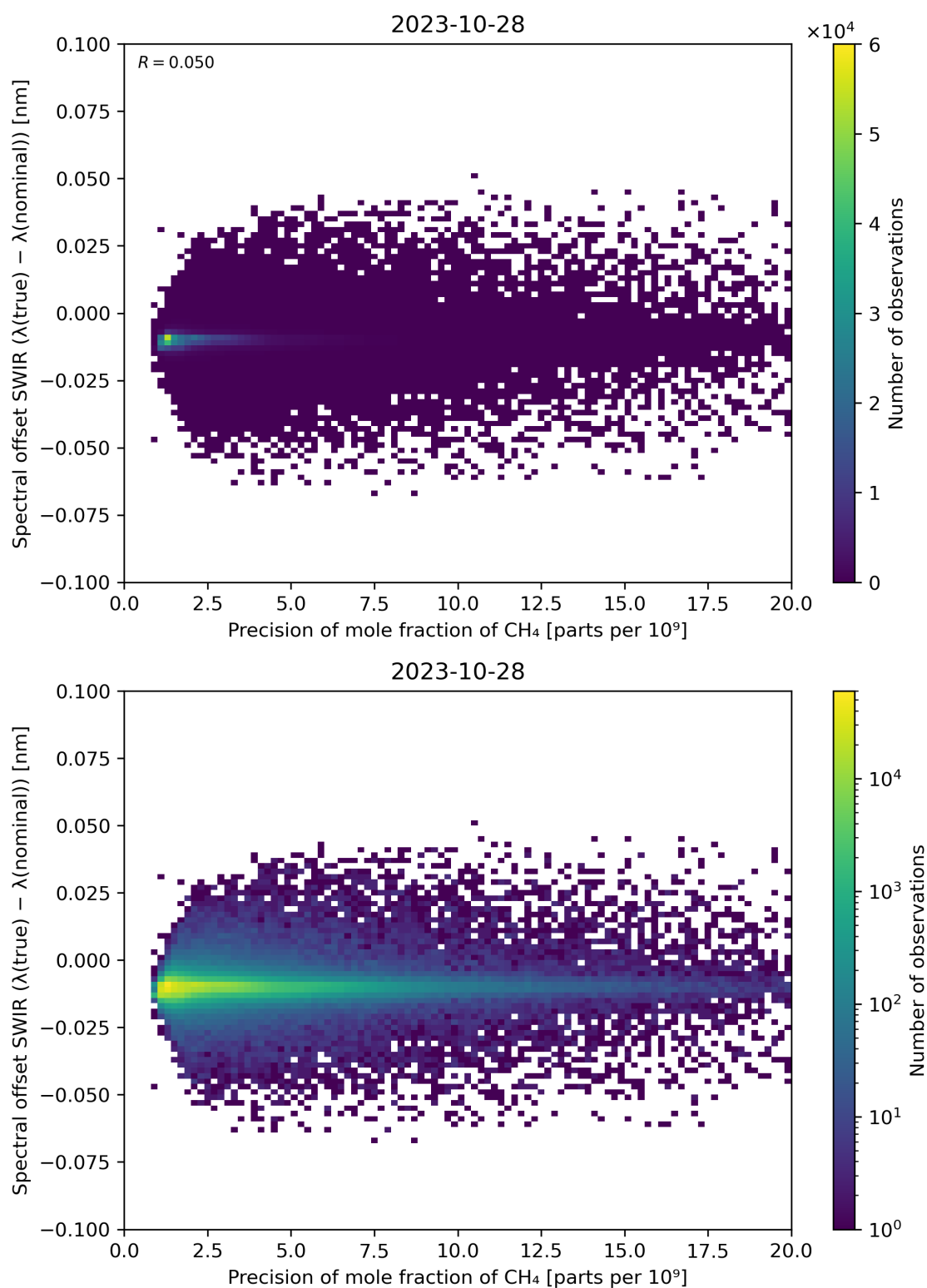
Figure 85: Scatter density plot of “Precision of mole fraction of \text{CH}_4 ” against “Spectral offset SWIR ( \lambda(\text{true}) - \lambda(\text{nominal}) )” for 2023-10-28 to 2023-10-29.
