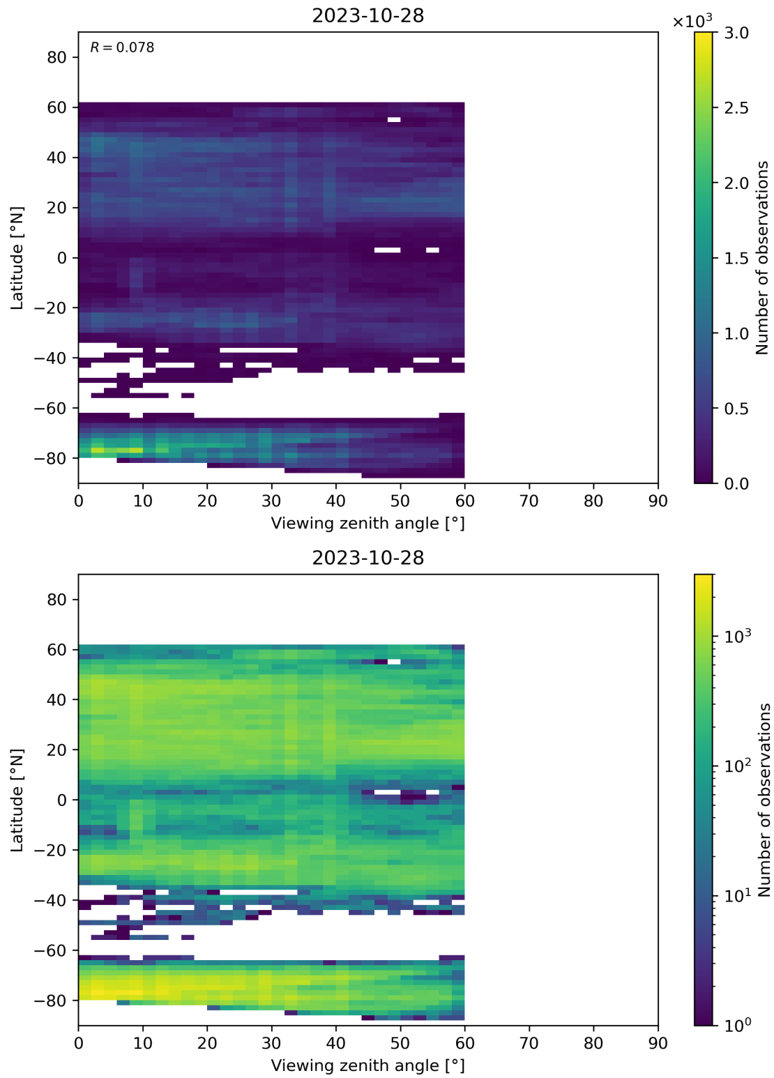
Figure 109: Scatter density plot of “Viewing zenith angle” against “Latitude” for 2023-10-28 to 2023-10-29.
