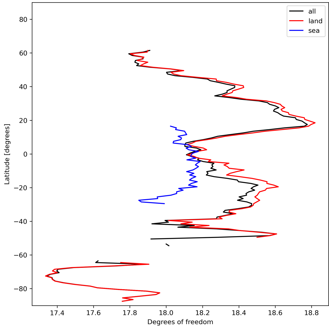
Figure 19: Zonal average of “Degrees of freedom” for 2023-10-28 to 2023-10-29.
