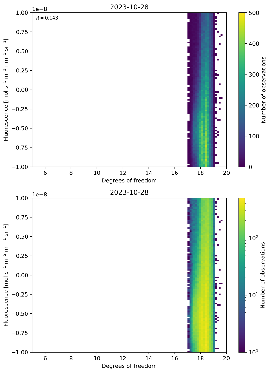
Figure 51: Scatter density plot of “Degrees of freedom” against “Fluorescence” for 2023-10-28 to 2023-10-29.
