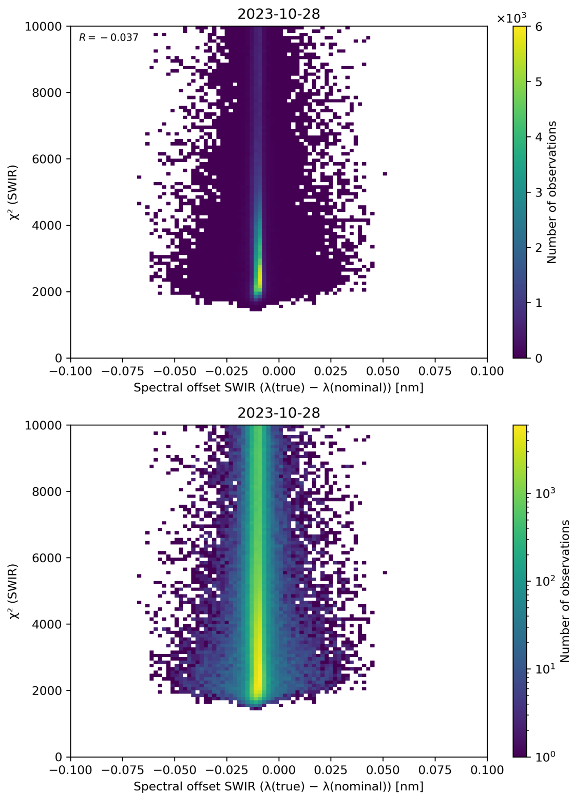
Figure 118: Scatter density plot of “Spectral offset SWIR ( \lambda(\text{true}) - \lambda(\text{nominal}) )” against “ \chi^2 (SWIR)” for 2023-10-28 to 2023-10-29.
