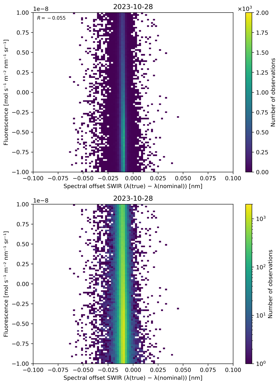
Figure 120: Scatter density plot of “Spectral offset SWIR ( \lambda(\text{true}) - \lambda(\text{nominal}) )” against “Fluorescence” for 2023-10-28 to 2023-10-29.
