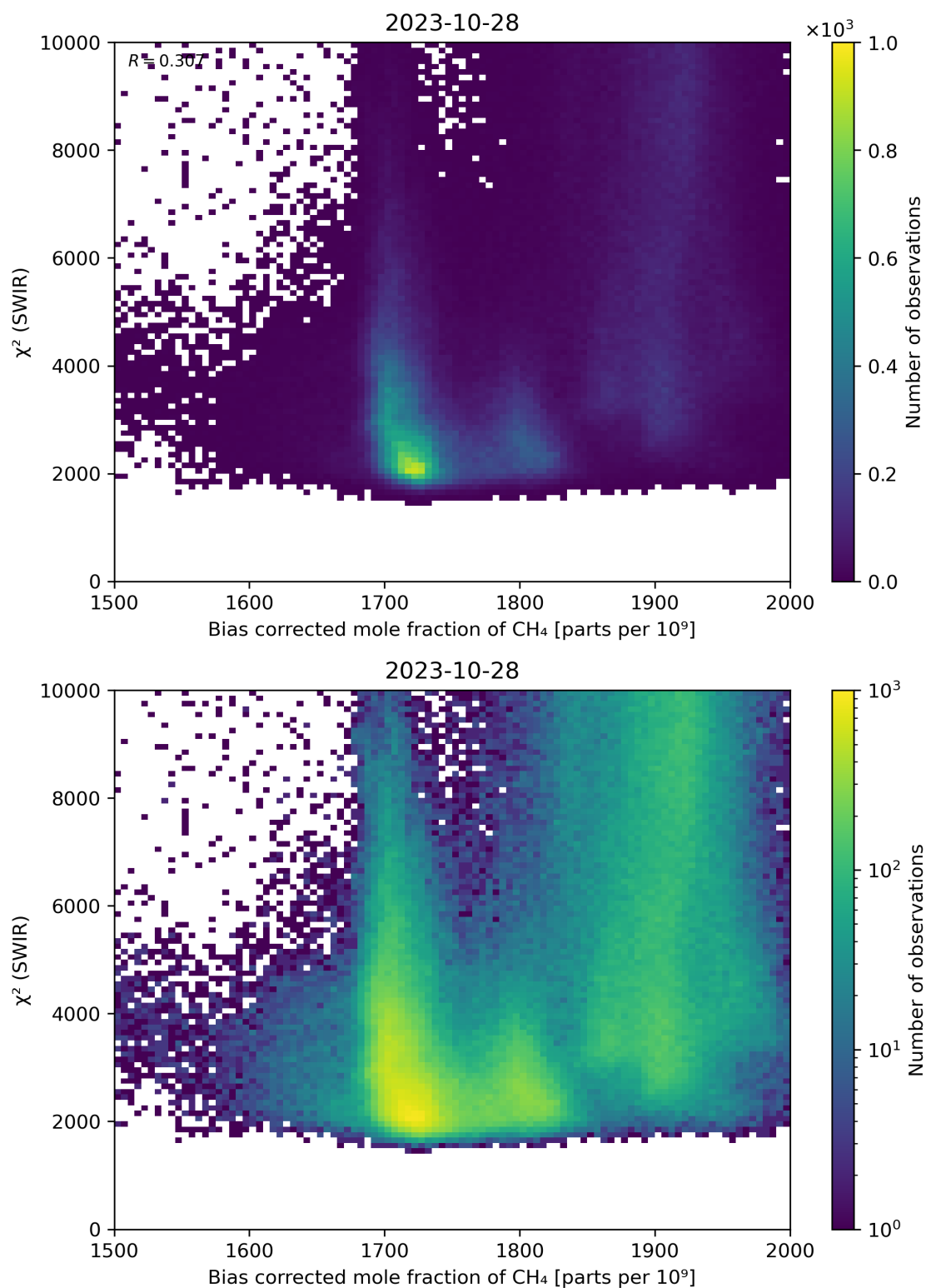
Figure 64: Scatter density plot of “Bias corrected mole fraction of CH 4 ” against “ \chi^2 (SWIR)” for 2023-10-28 to 2023-10-29.
