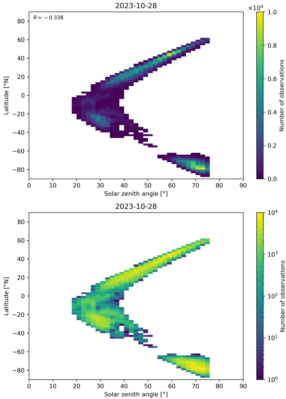
Figure 98: Scatter density plot of “Solar zenith angle” against “Latitude” for 2023-10-28 to 2023-10-29.
