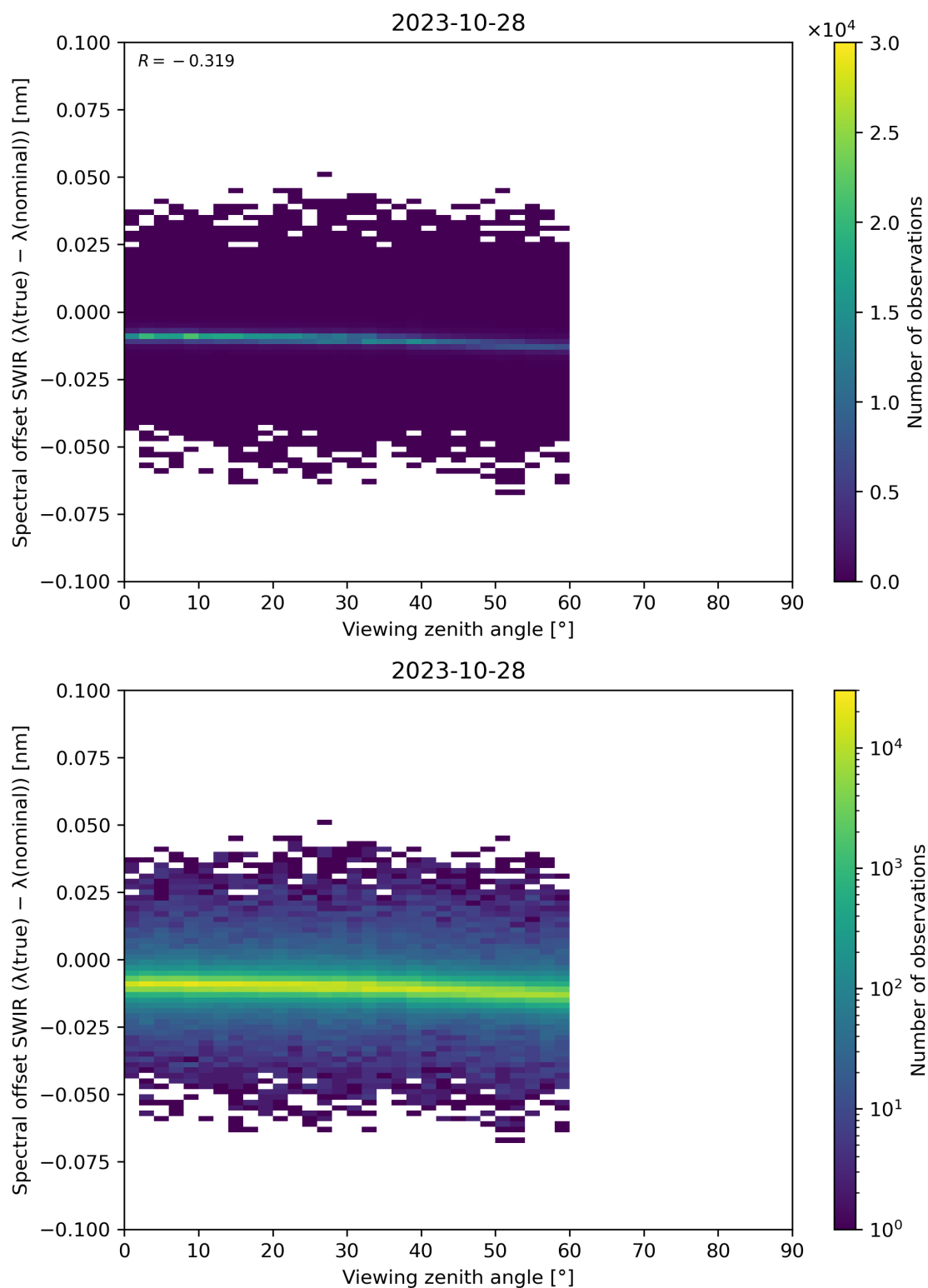
Figure 116: Scatter density plot of “Viewing zenith angle” against “Spectral offset SWIR ( \lambda(\text{true}) - \lambda(\text{nominal}) )” for 2023-10-28 to 2023-10-29.
