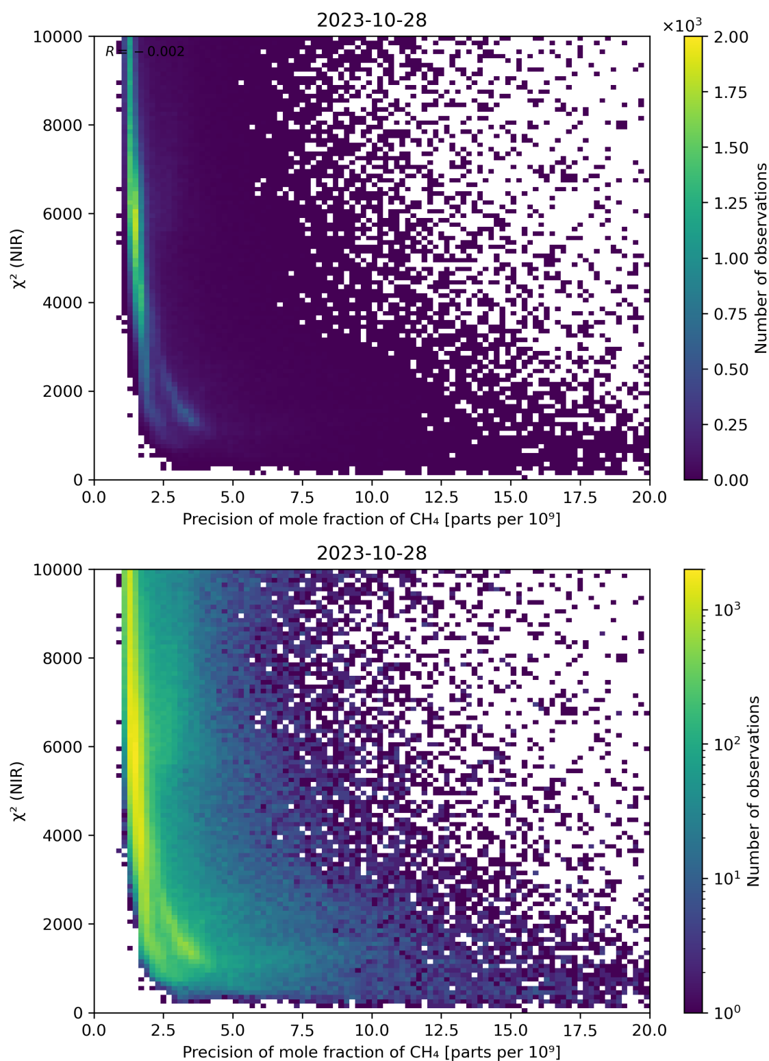
Figure 78: Scatter density plot of “Precision of mole fraction of CH 4 ” against “ \chi^2 (NIR)” for 2023-10-28 to 2023-10-29.
