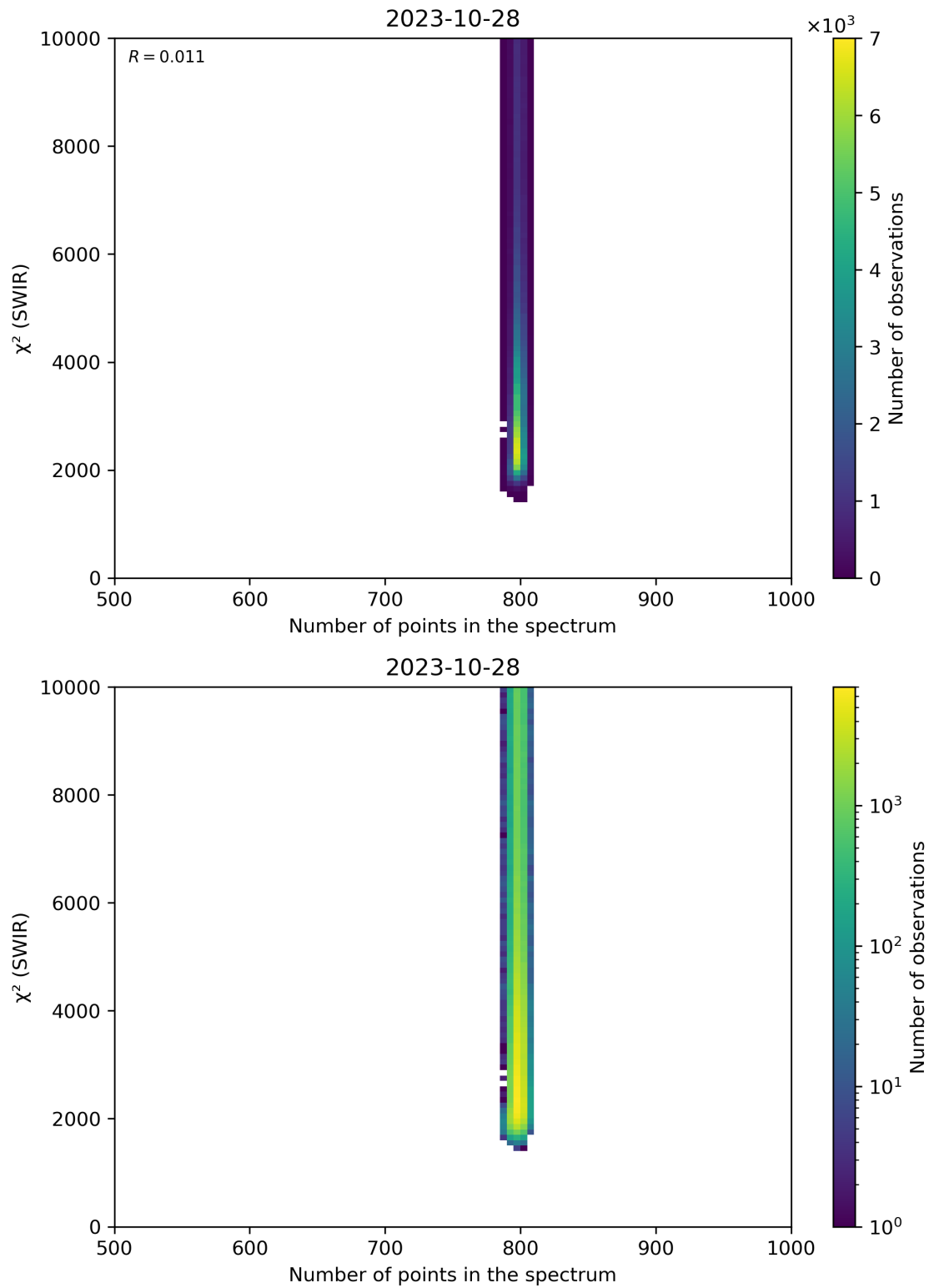
Figure 89: Scatter density plot of “Number of points in the spectrum” against “ \chi^2 (SWIR)” for 2023-10-28 to 2023-10-29.
