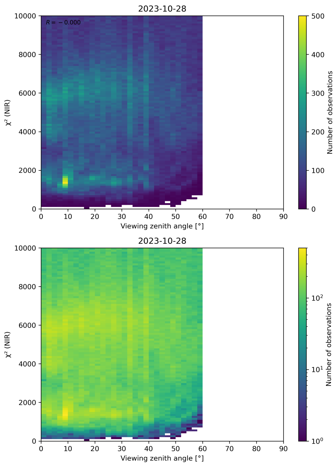
Figure 105: Scatter density plot of “Viewing zenith angle” against “ \chi^2 (NIR)” for 2023-10-28 to 2023-10-29.
