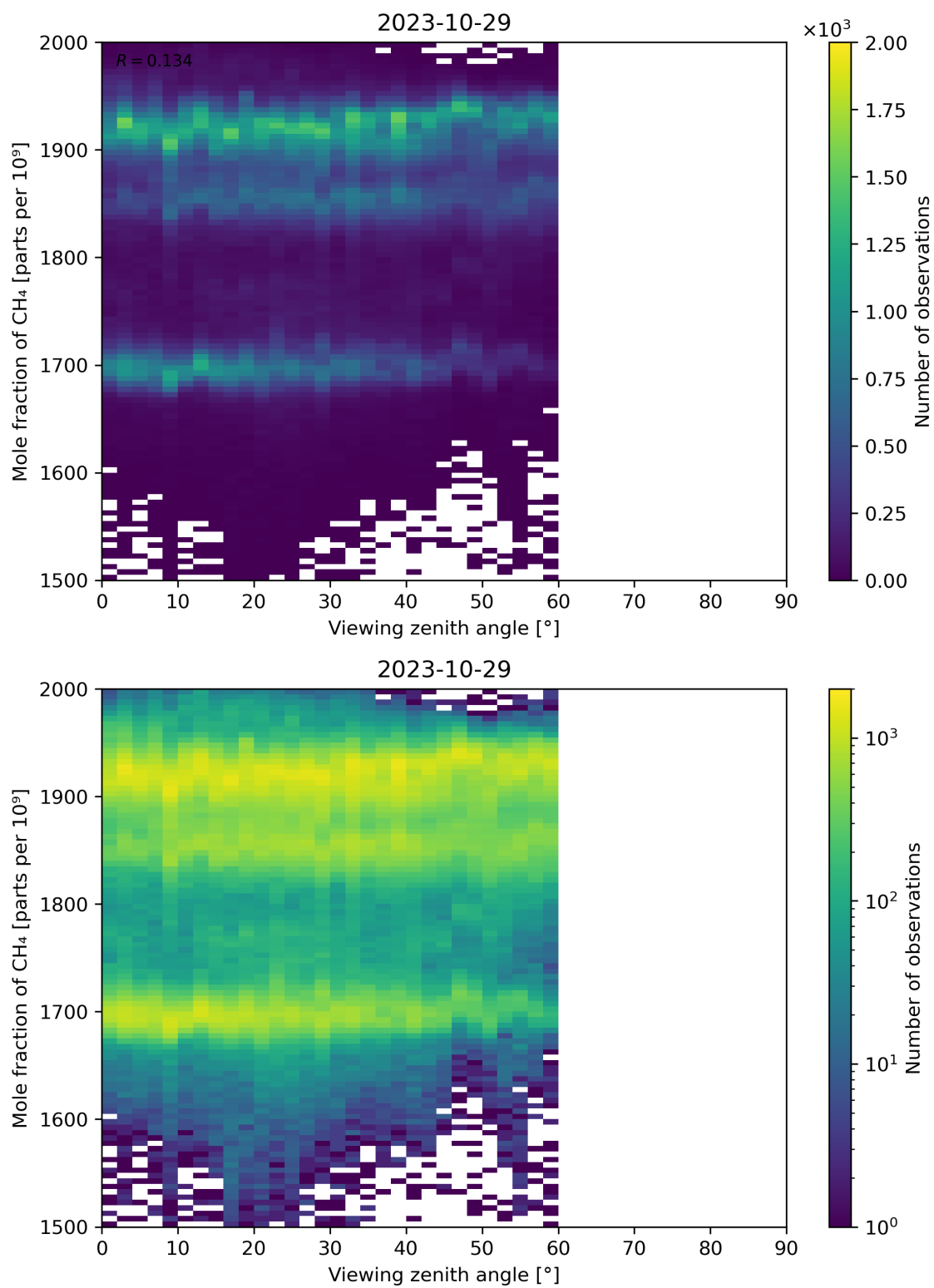
Figure 110: Scatter density plot of “Viewing zenith angle” against “Mole fraction of \text{CH}_4 ” for 2023-10-28 to 2023-10-30.
