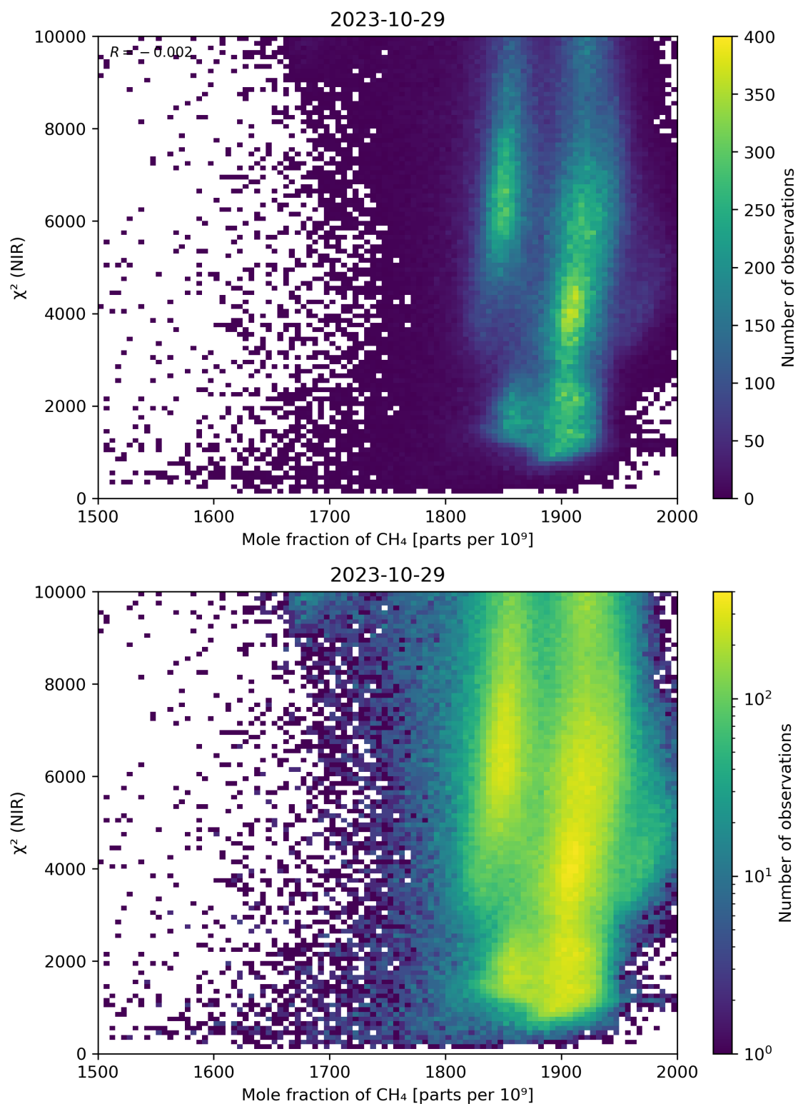
Figure 70: Scatter density plot of “Mole fraction of \text{CH}_4 ” against “ \chi^2 (NIR)” for 2023-10-28 to 2023-10-30.
