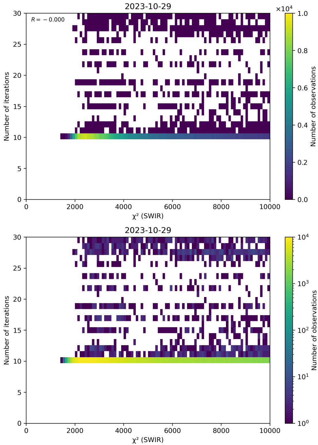
Figure 50: Scatter density plot of “ \chi^2 (SWIR)” against “Number of iterations” for 2023-10-28 to 2023-10-30.
