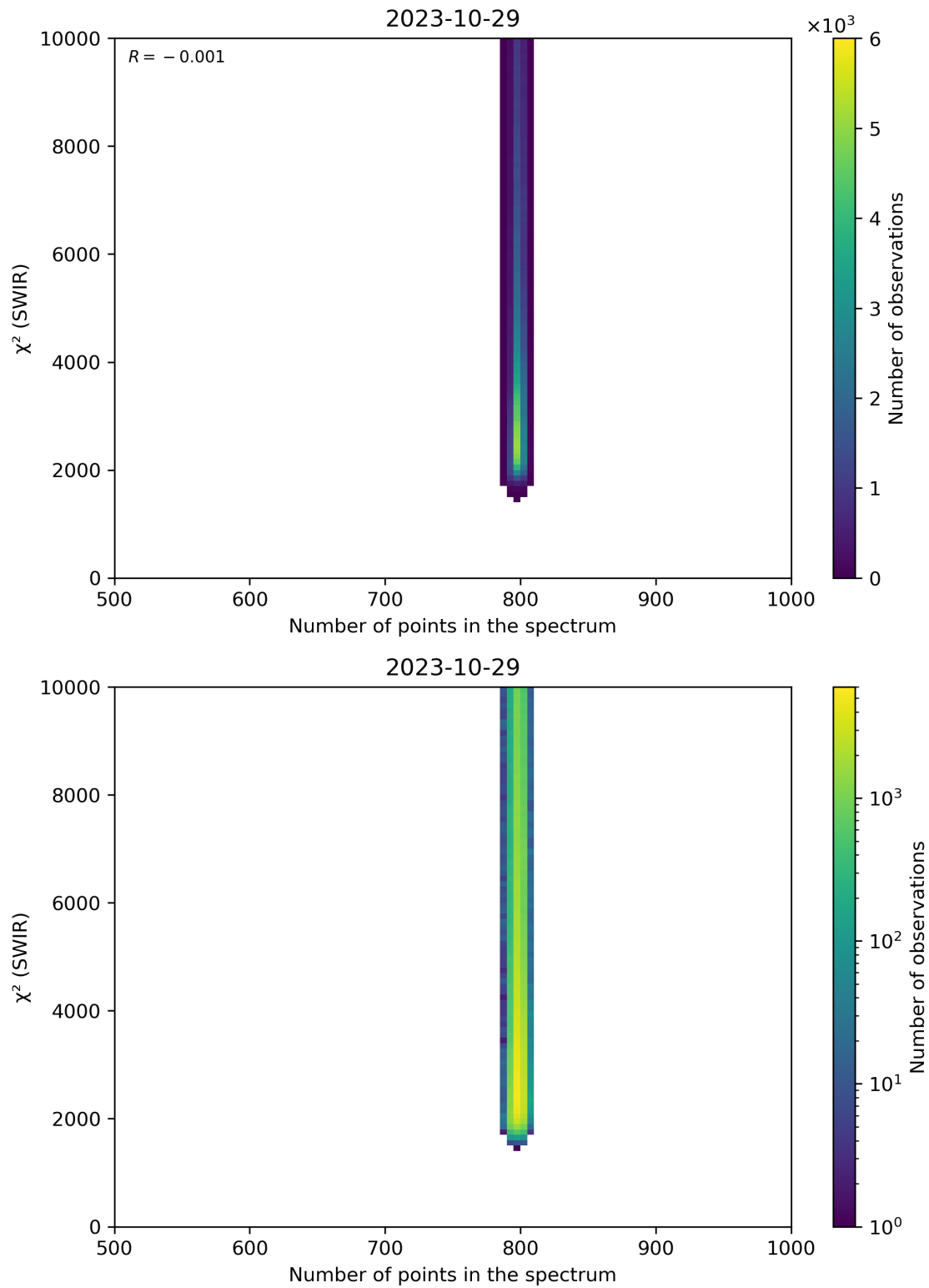
Figure 89: Scatter density plot of “Number of points in the spectrum” against “ \chi^2 (SWIR)” for 2023-10-28 to 2023-10-30.
