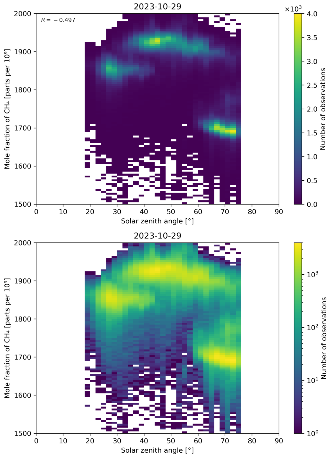
Figure 99: Scatter density plot of “Solar zenith angle” against “Mole fraction of CH 4 ” for 2023-10-28 to 2023-10-30.
