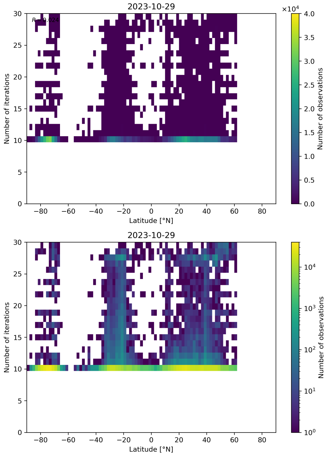
Figure 60: Scatter density plot of “Latitude” against “Number of iterations” for 2023-10-28 to 2023-10-30.
