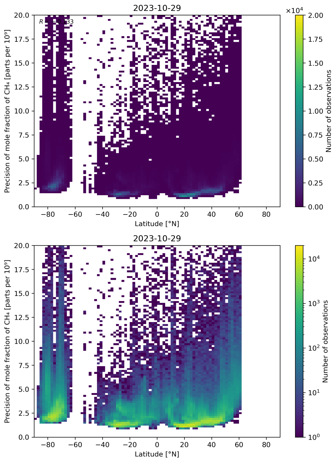
Figure 59: Scatter density plot of “Latitude” against “Precision of mole fraction of CH 4 ” for 2023-10-28 to 2023-10-30.
