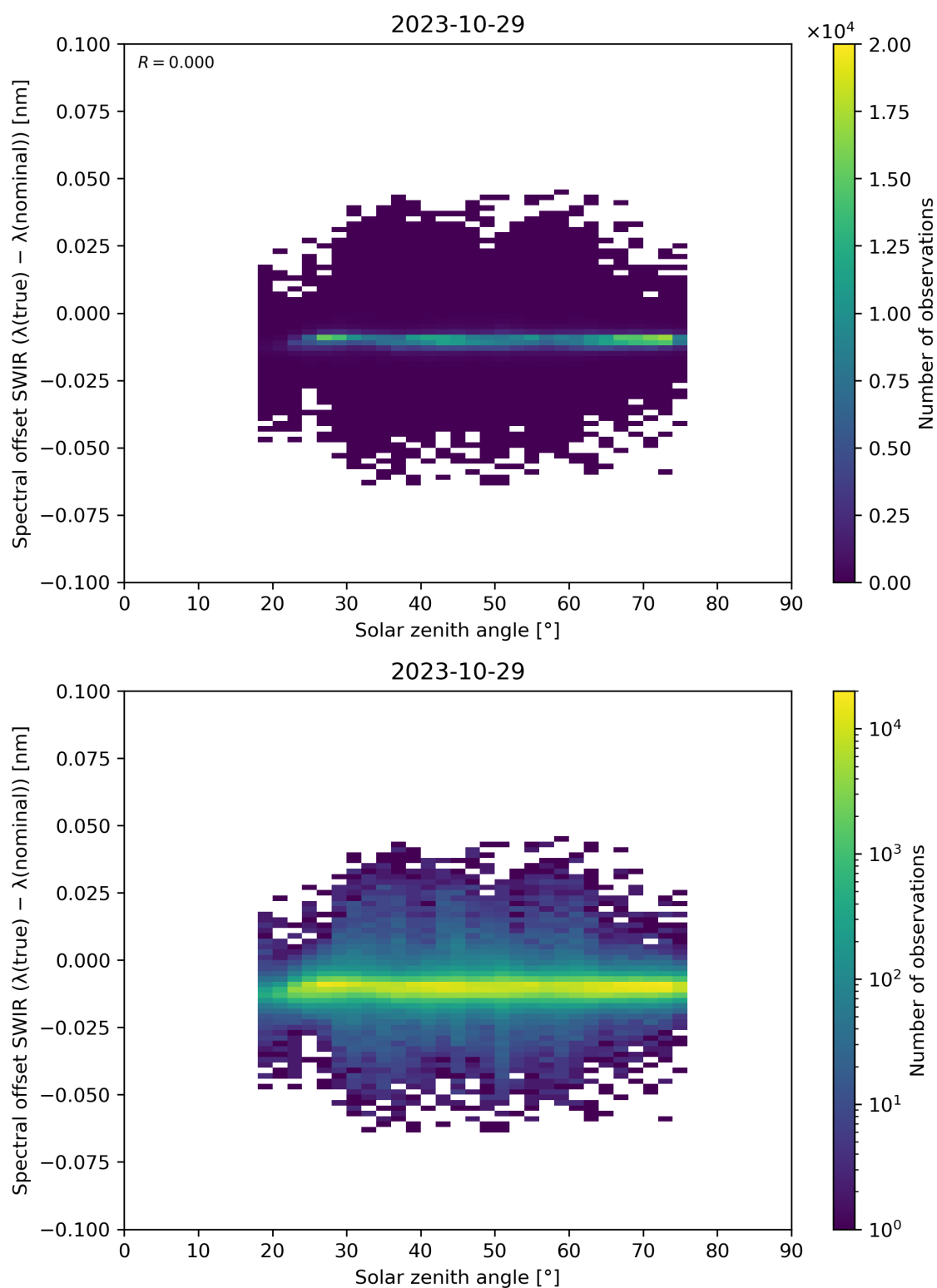
Figure 104: Scatter density plot of “Solar zenith angle” against “Spectral offset SWIR ( \lambda(\text{true}) - \lambda(\text{nominal}) )” for 2023-10-28 to 2023-10-30.
