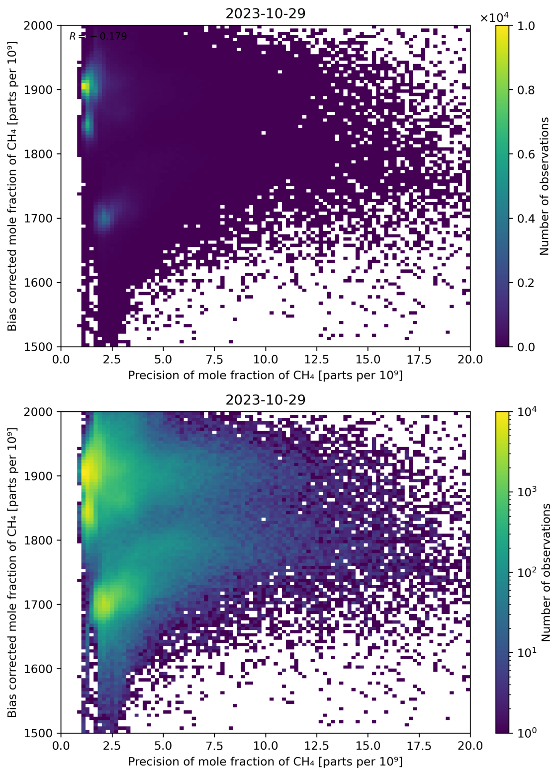
Figure 82: Scatter density plot of “Precision of mole fraction of \text{CH}_4 ” against “Bias corrected mole fraction of \text{CH}_4 ” for 2023-10-28 to 2023-10-30.
