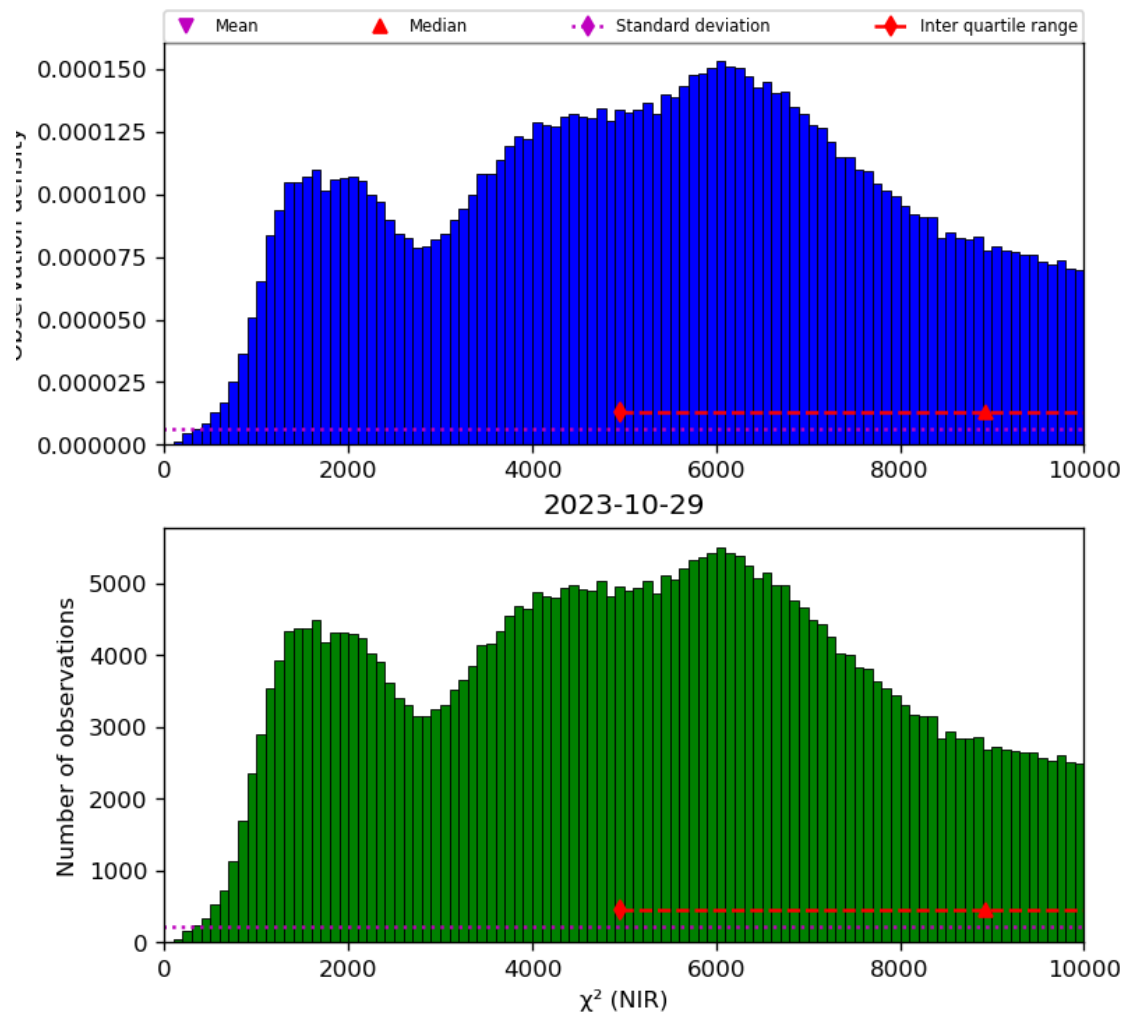
Figure 29: Histogram of “ \chi^2 (NIR)” for 2023-10-28 to 2023-10-30
