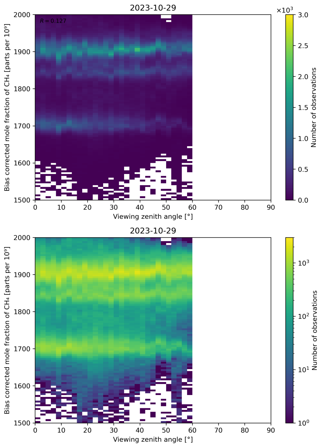
Figure 111: Scatter density plot of “Viewing zenith angle” against “Bias corrected mole fraction of CH 4 ” for 2023-10-28 to 2023-10-30.
