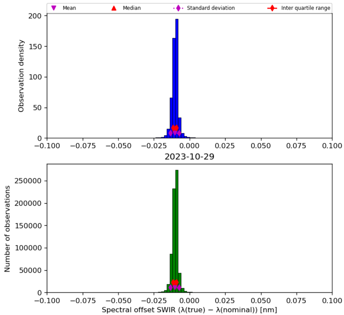
Figure 27: Histogram of “Spectral offset SWIR ( \lambda(\text{true}) - \lambda(\text{nominal}) )” for 2023-10-28 to 2023-10-30
