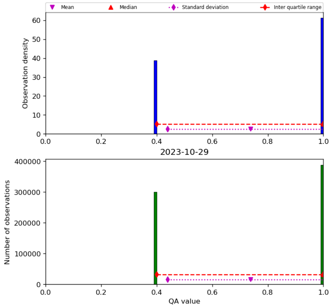
Figure 22: Histogram of “QA value” for 2023-10-28 to 2023-10-30
