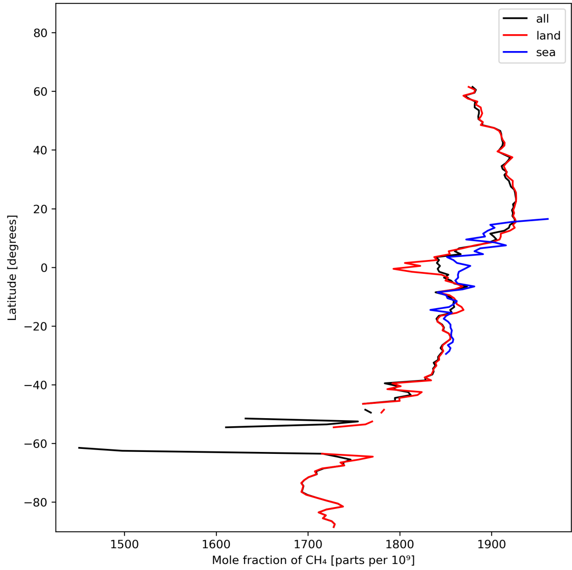
Figure 12: Zonal average of “Mole fraction of CH 4 ” for 2023-10-28 to 2023-10-30.
