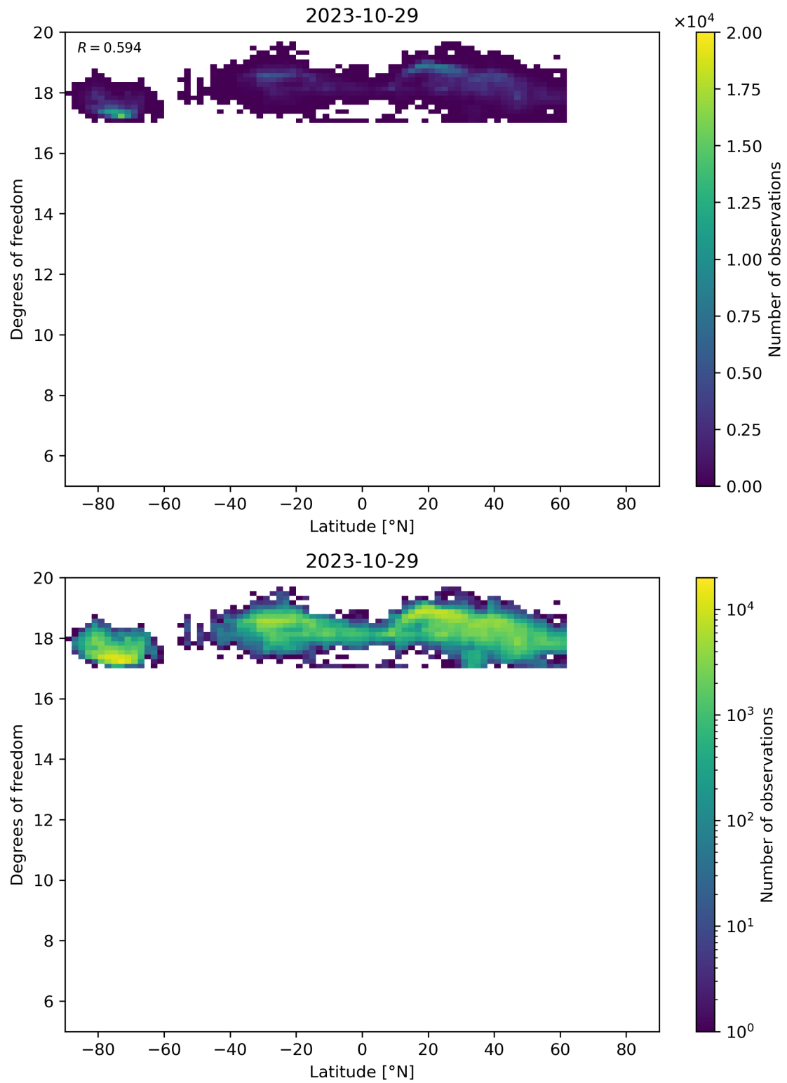
Figure 55: Scatter density plot of “Latitude” against “Degrees of freedom” for 2023-10-28 to 2023-10-30.
