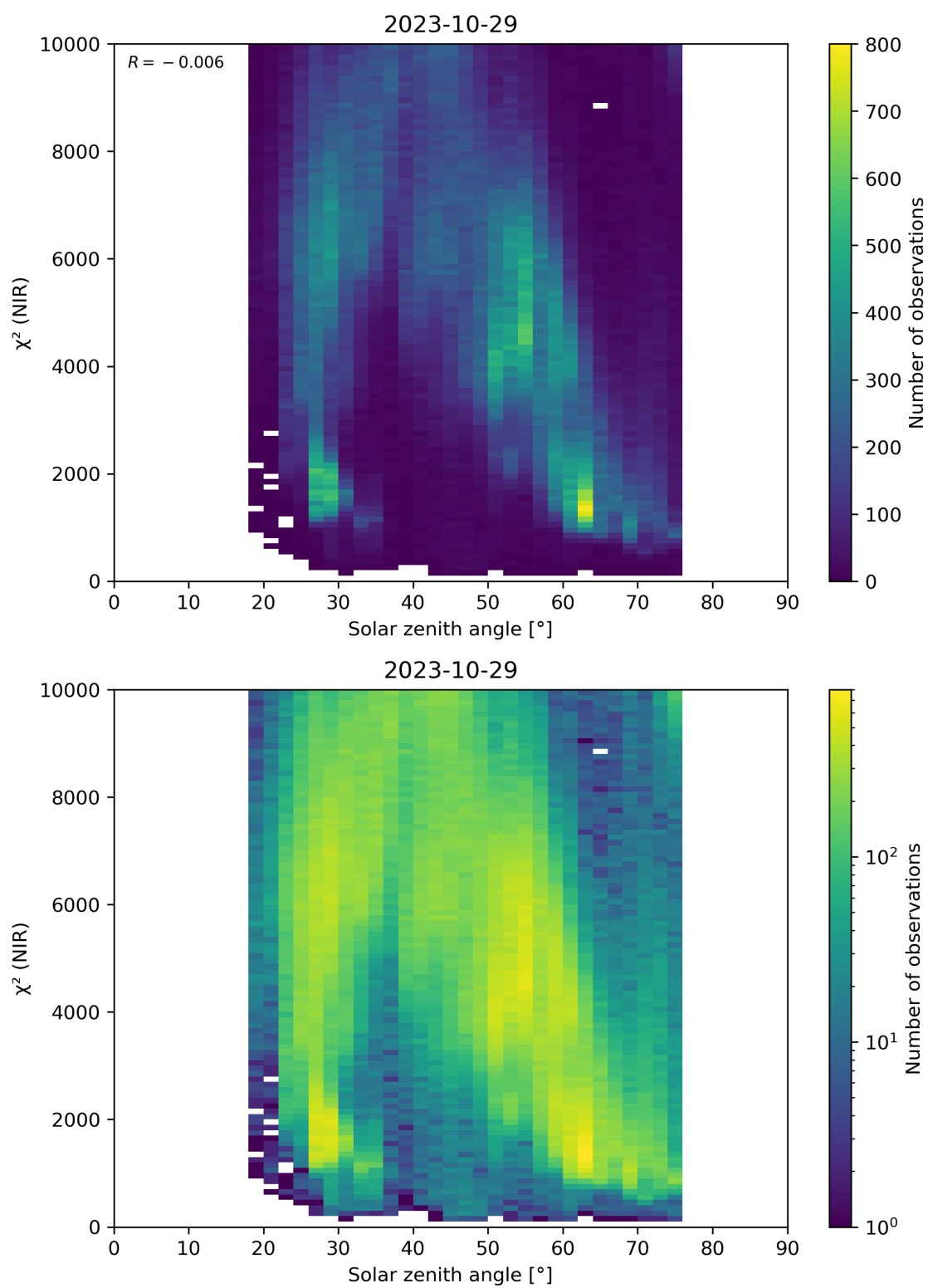
Figure 94: Scatter density plot of “Solar zenith angle” against “ \chi^2 (NIR)” for 2023-10-28 to 2023-10-30.
