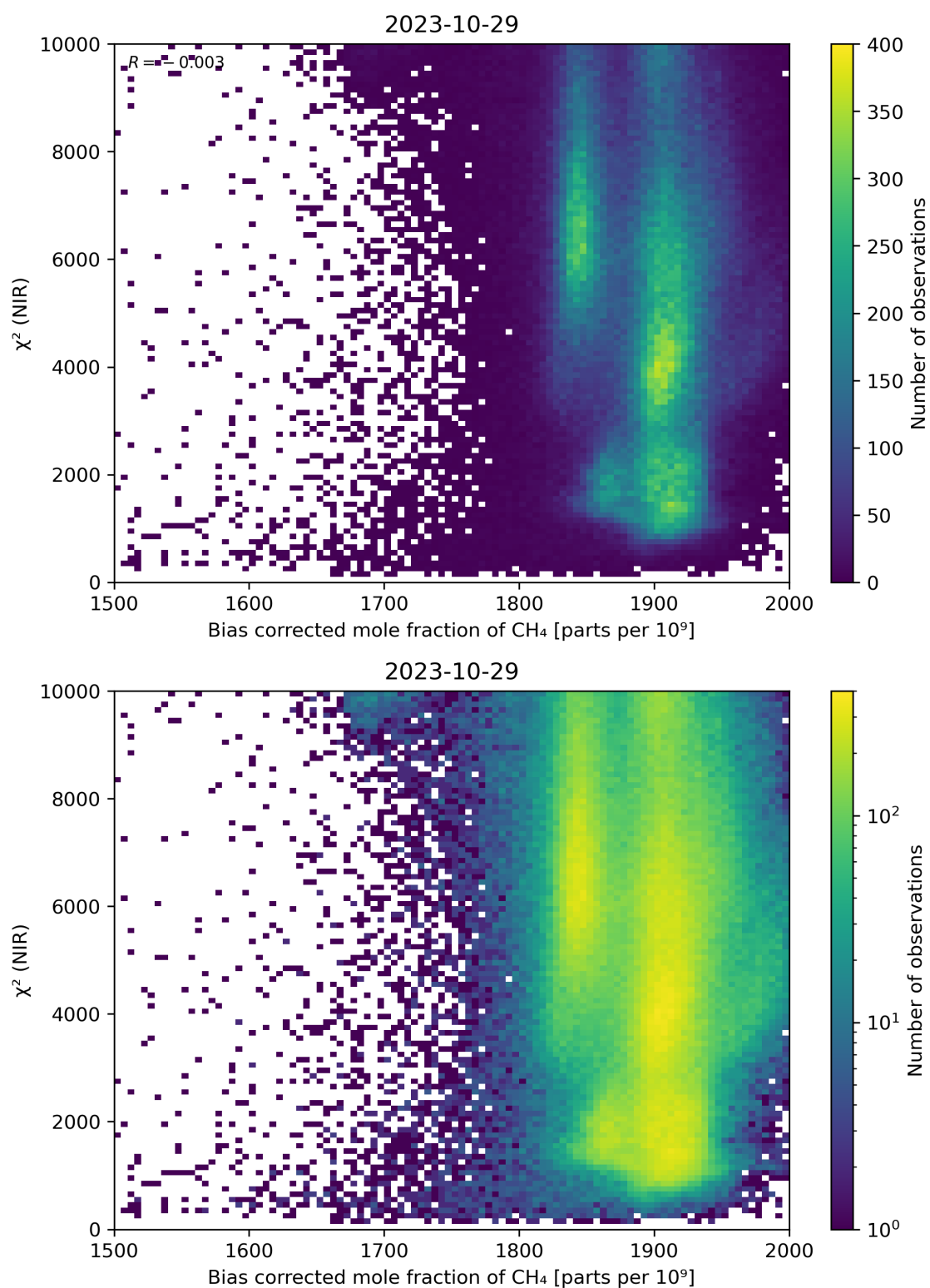
Figure 63: Scatter density plot of “Bias corrected mole fraction of \text{CH}_4 ” against “ \chi^2 (NIR)” for 2023-10-28 to 2023-10-30.
