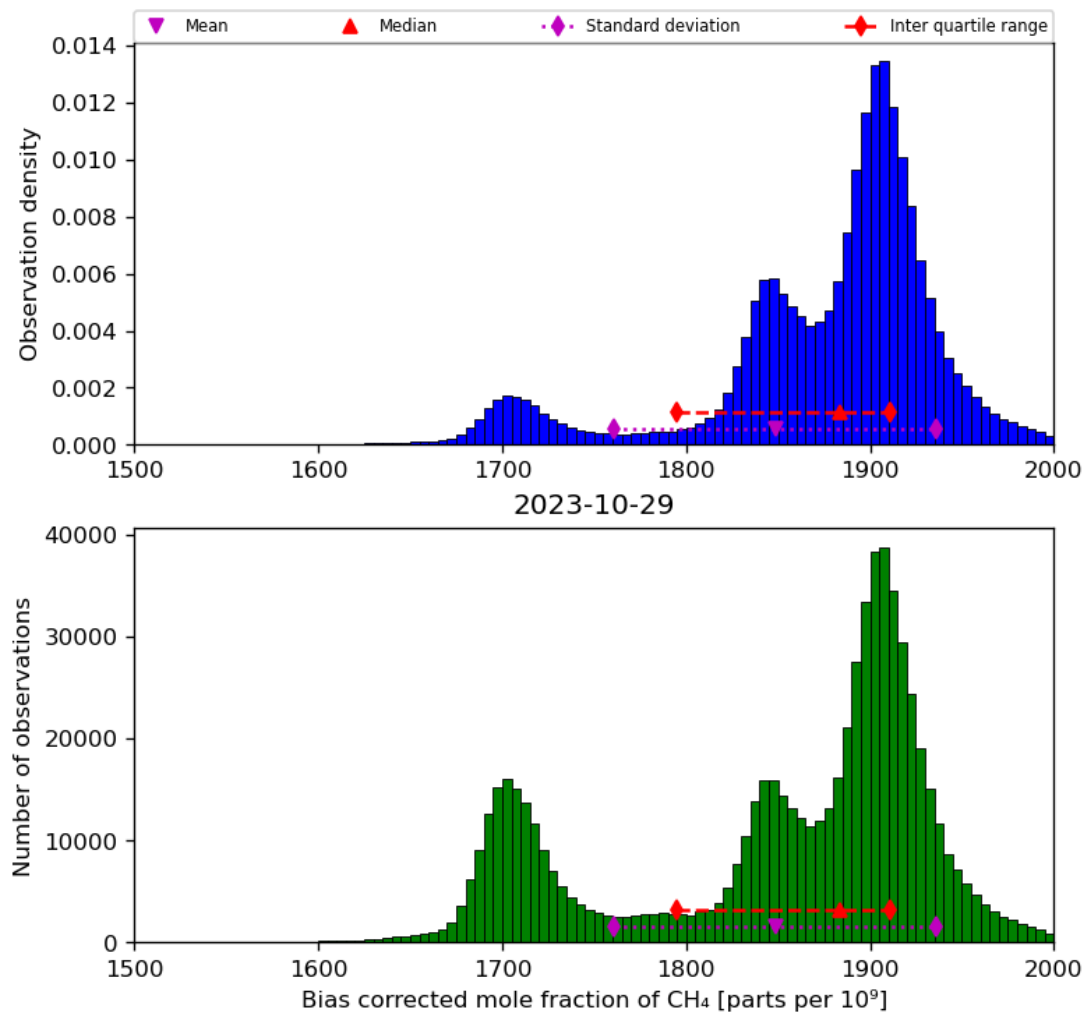
Figure 25: Histogram of “Bias corrected mole fraction of CH 4 ” for 2023-10-28 to 2023-10-30
