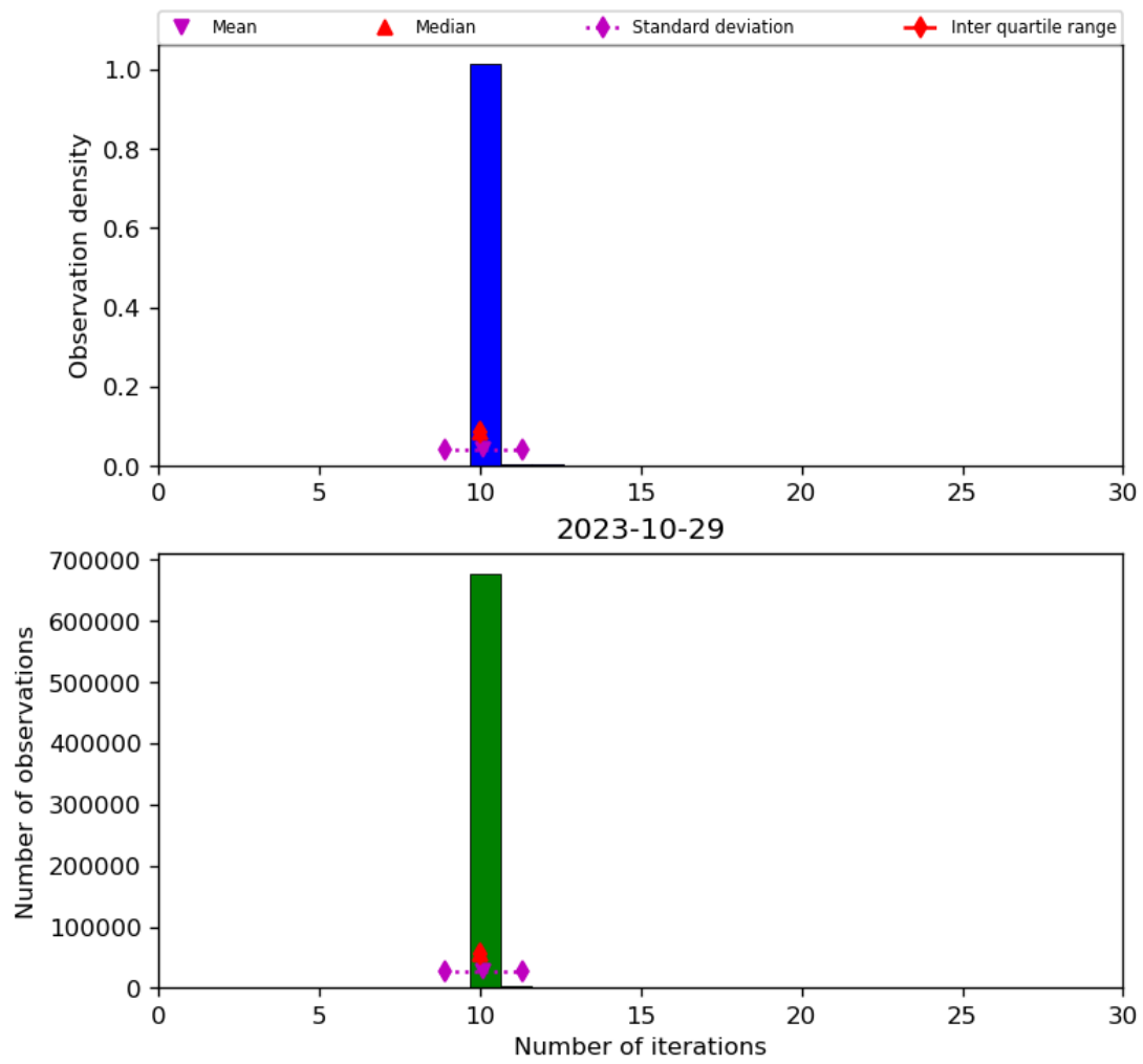
Figure 31: Histogram of “Number of iterations” for 2023-10-28 to 2023-10-30
