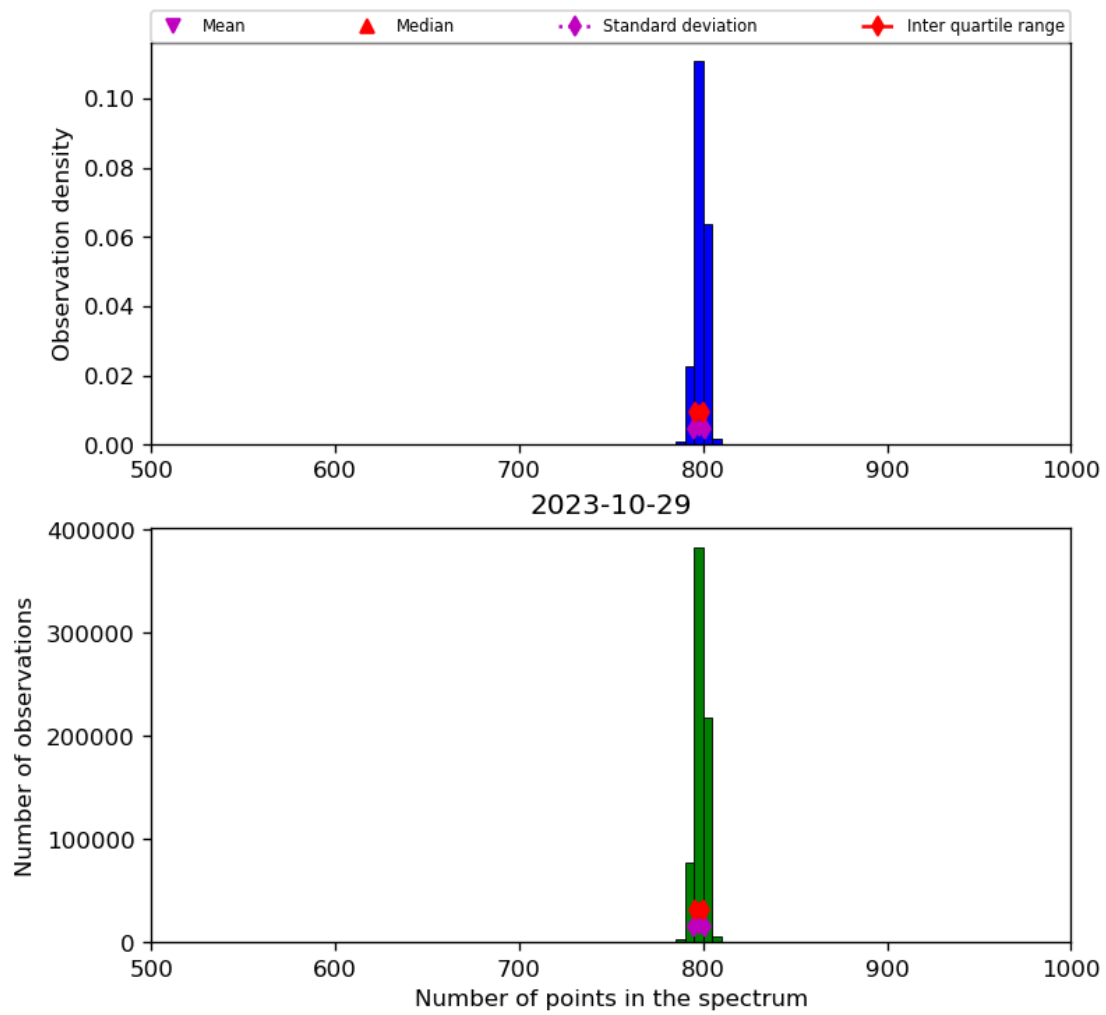
Figure 26: Histogram of “Number of points in the spectrum” for 2023-10-28 to 2023-10-30
