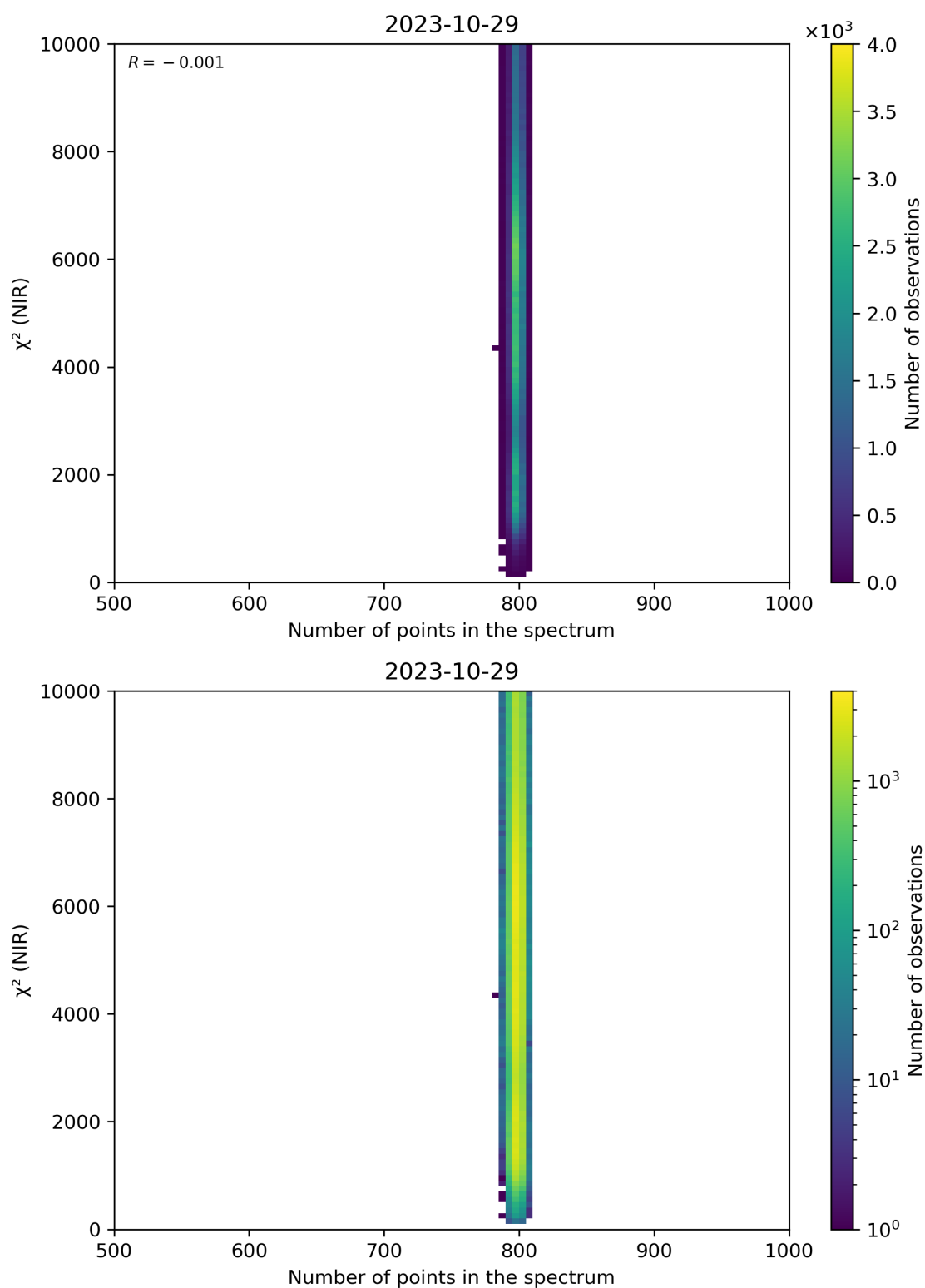
Figure 88: Scatter density plot of “Number of points in the spectrum” against “ \chi^2 (NIR)” for 2023-10-28 to 2023-10-30.
