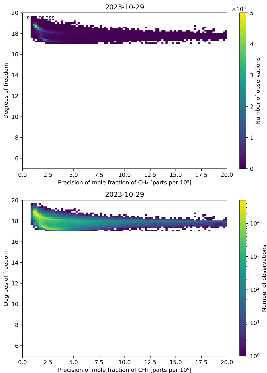
Figure 80: Scatter density plot of “Precision of mole fraction of CH 4 ” against “Degrees of freedom” for 2023-10-28 to 2023-10-30.
