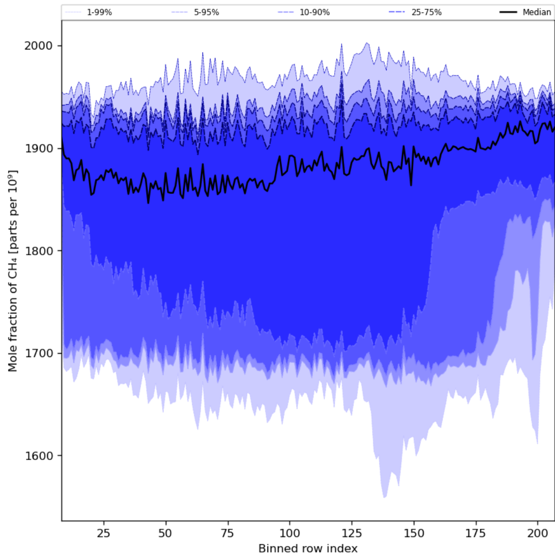
Figure 34: Along track statistics of “Mole fraction of CH 4 ” for 2023-10-28 to 2023-10-30
