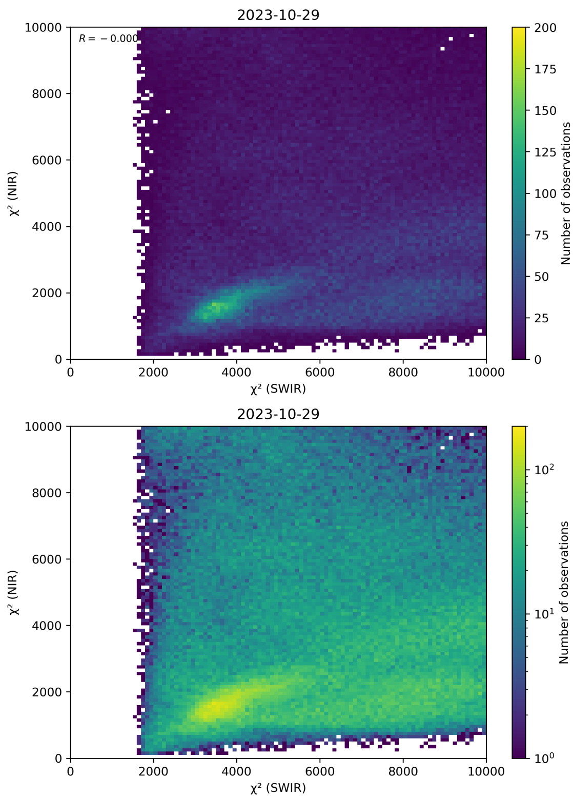
Figure 47: Scatter density plot of “ \chi^2 (SWIR)” against “ \chi^2 (NIR)” for 2023-10-28 to 2023-10-30.
