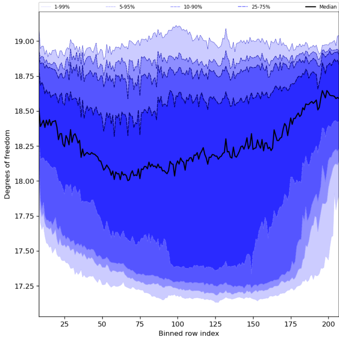
Figure 41: Along track statistics of “Degrees of freedom” for 2023-10-28 to 2023-10-30
