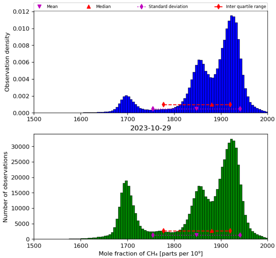
Figure 23: Histogram of “Mole fraction of CH 4 ” for 2023-10-28 to 2023-10-30
