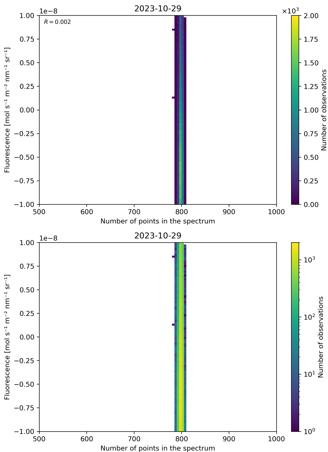
Figure 91: Scatter density plot of “Number of points in the spectrum” against “Fluorescence” for 2023-10-28 to 2023-10-30.
