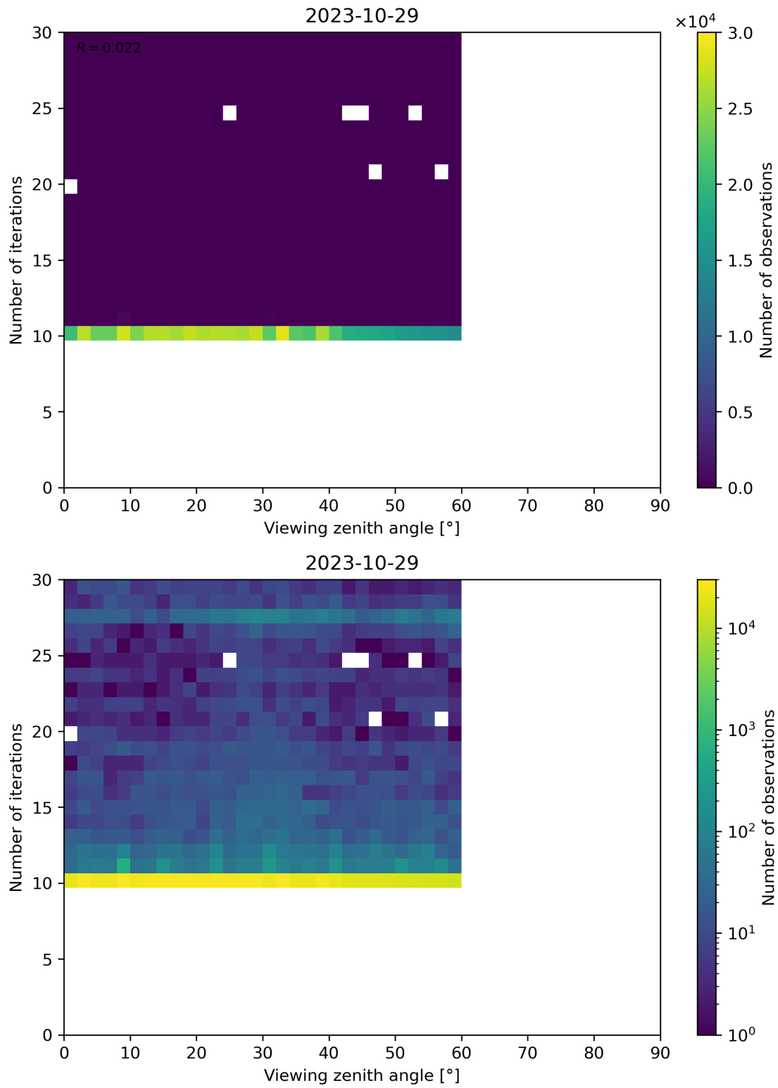
Figure 113: Scatter density plot of “Viewing zenith angle” against “Number of iterations” for 2023-10-28 to 2023-10-30.
