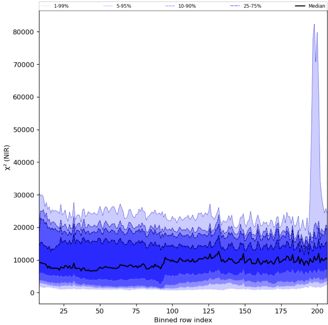
Figure 40: Along track statistics of “ \chi^2 (NIR)” for 2023-10-28 to 2023-10-30
