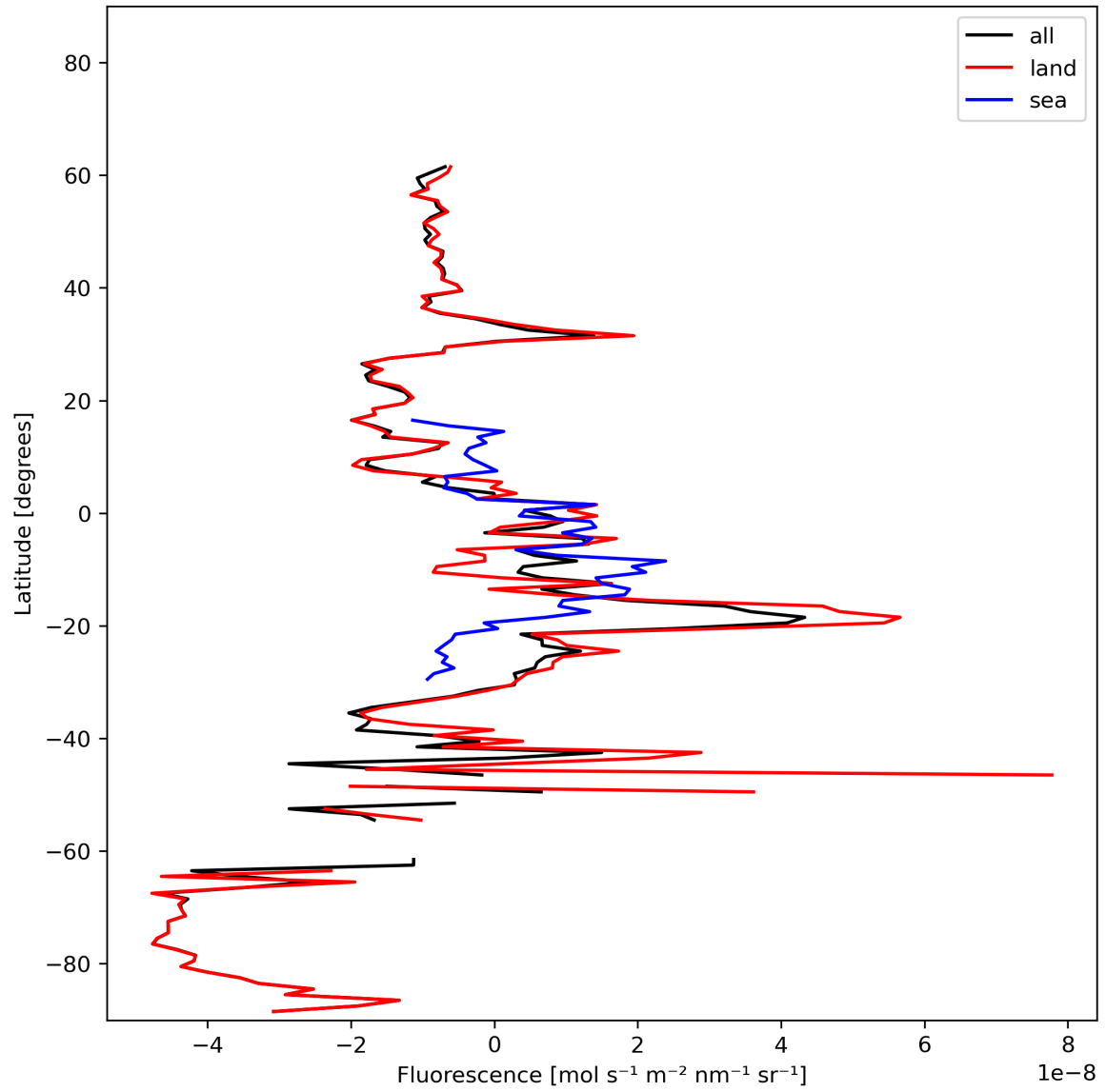
Figure 21: Zonal average of “Fluorescence” for 2023-10-28 to 2023-10-30.
