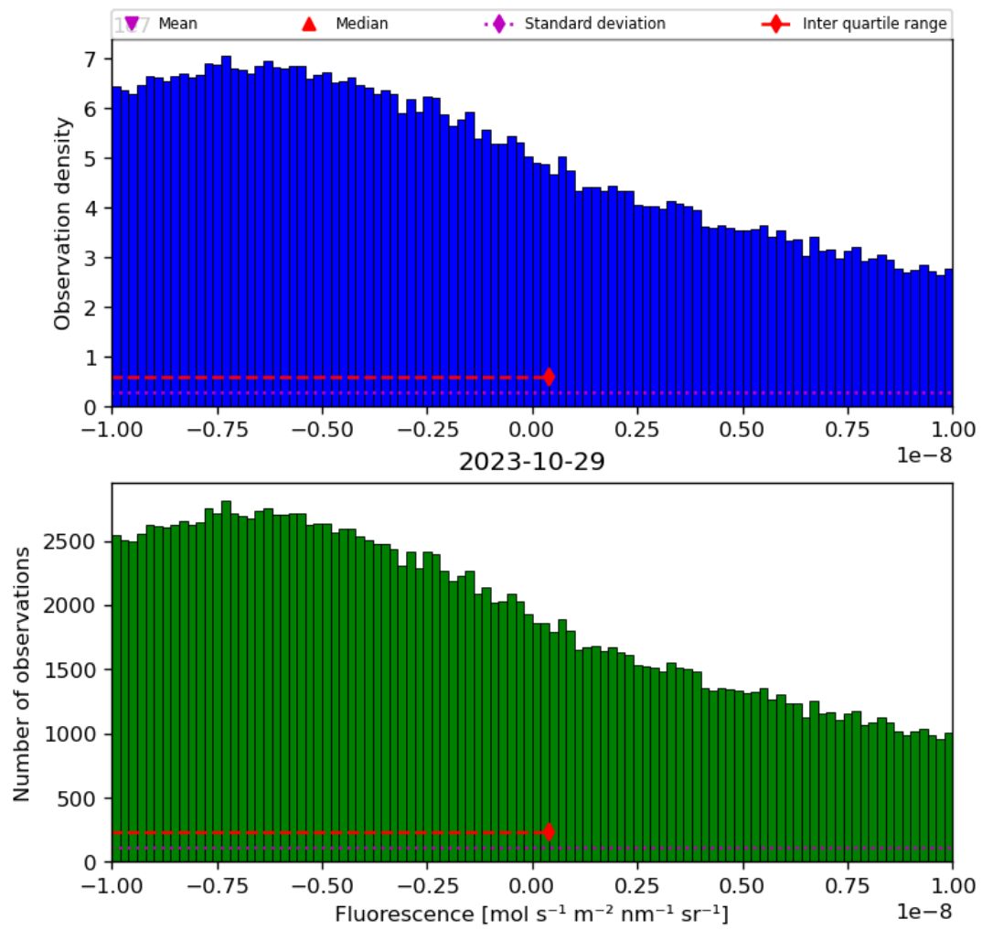
Figure 32: Histogram of “Fluorescence” for 2023-10-28 to 2023-10-30
