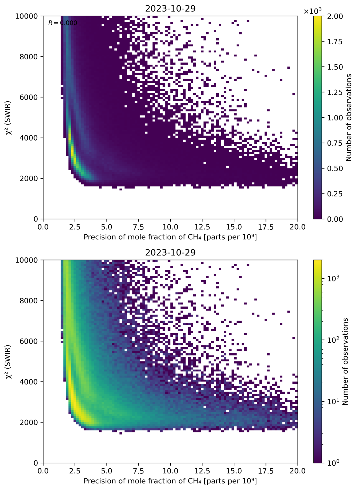
Figure 79: Scatter density plot of “Precision of mole fraction of CH 4 ” against “ \chi^2 (SWIR)” for 2023-10-28 to 2023-10-30.
