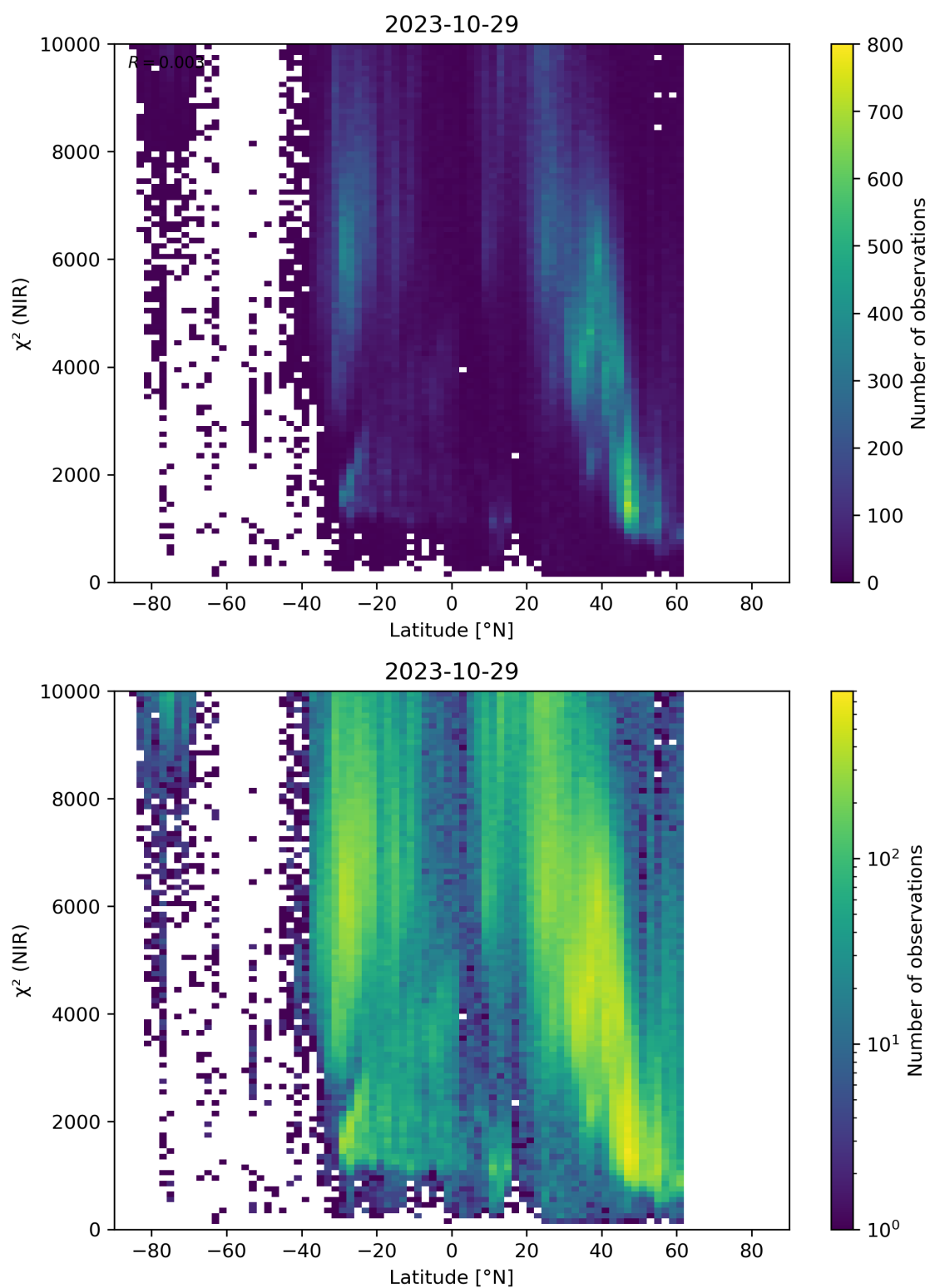
Figure 53: Scatter density plot of “Latitude” against “ \chi^2 (NIR)” for 2023-10-28 to 2023-10-30.
