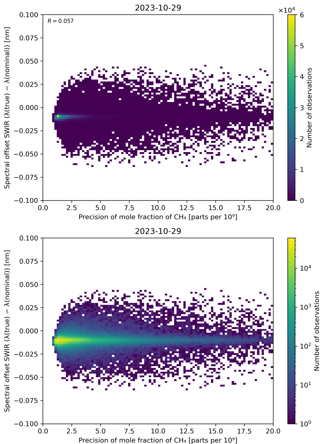
Figure 85: Scatter density plot of “Precision of mole fraction of CH 4 ” against “Spectral offset SWIR ( \lambda(\text{true}) - \lambda(\text{nominal}) )” for 2023-10-28 to 2023-10-30.
