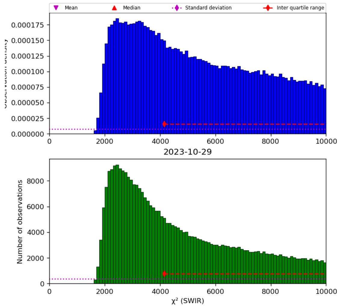
Figure 28: Histogram of " \chi^2 (SWIR)" for 2023-10-28 to 2023-10-30
