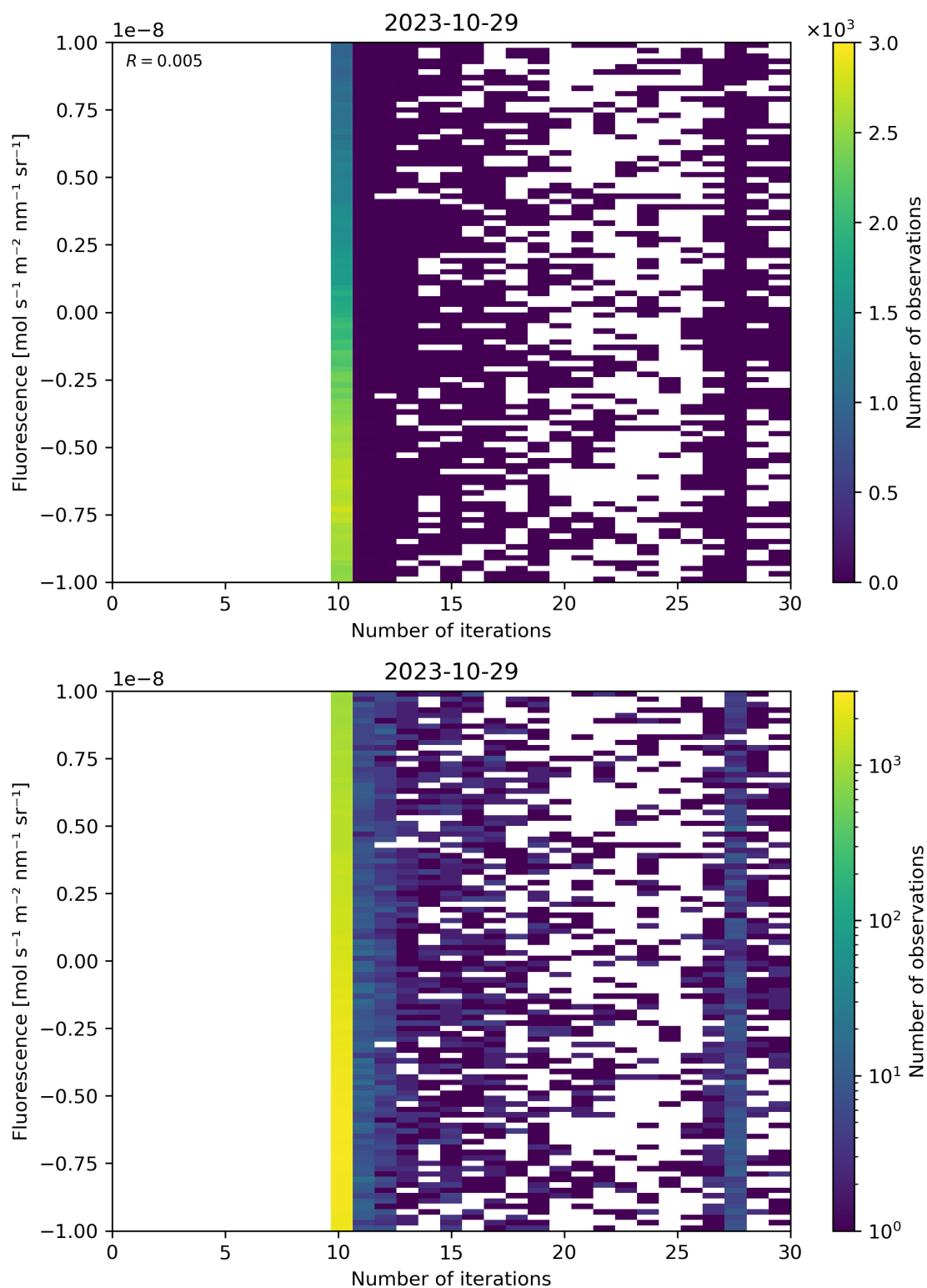
Figure 87: Scatter density plot of “Number of iterations” against “Fluorescence” for 2023-10-28 to 2023-10-30.
