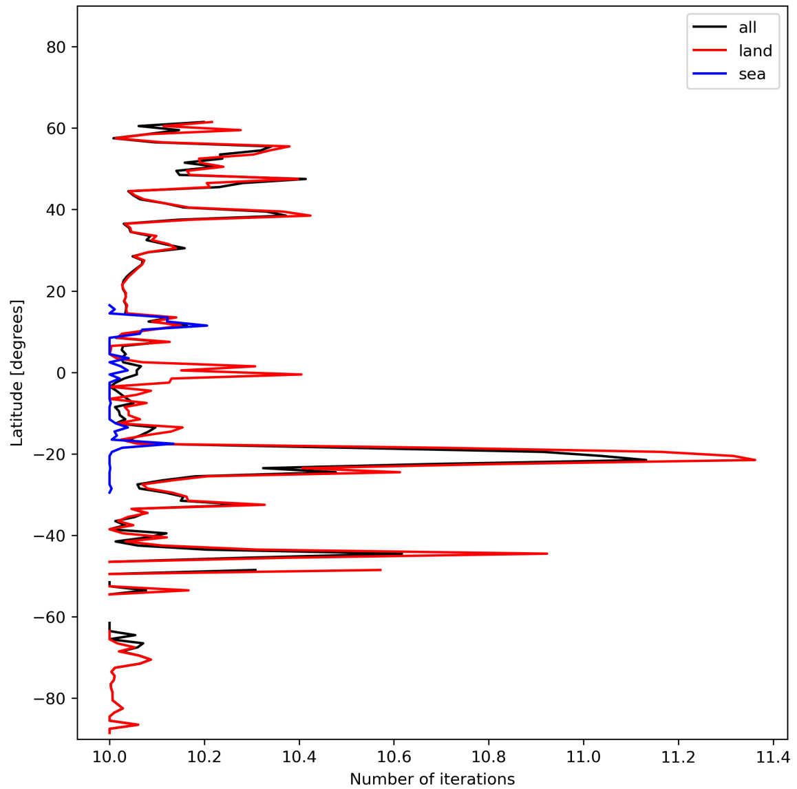
Figure 20: Zonal average of “Number of iterations” for 2023-10-28 to 2023-10-30.
