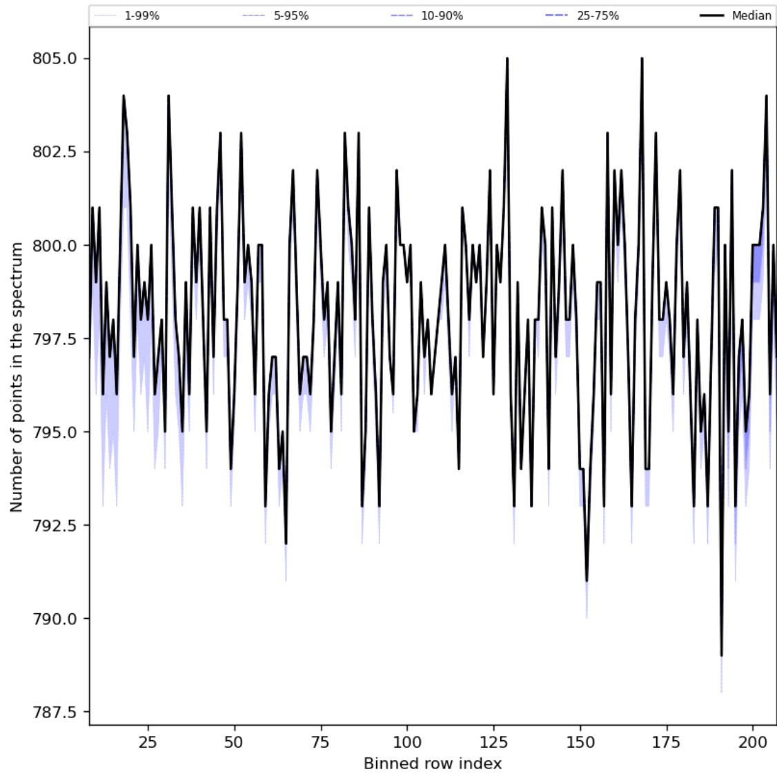
Figure 37: Along track statistics of “Number of points in the spectrum” for 2023-10-28 to 2023-10-30
