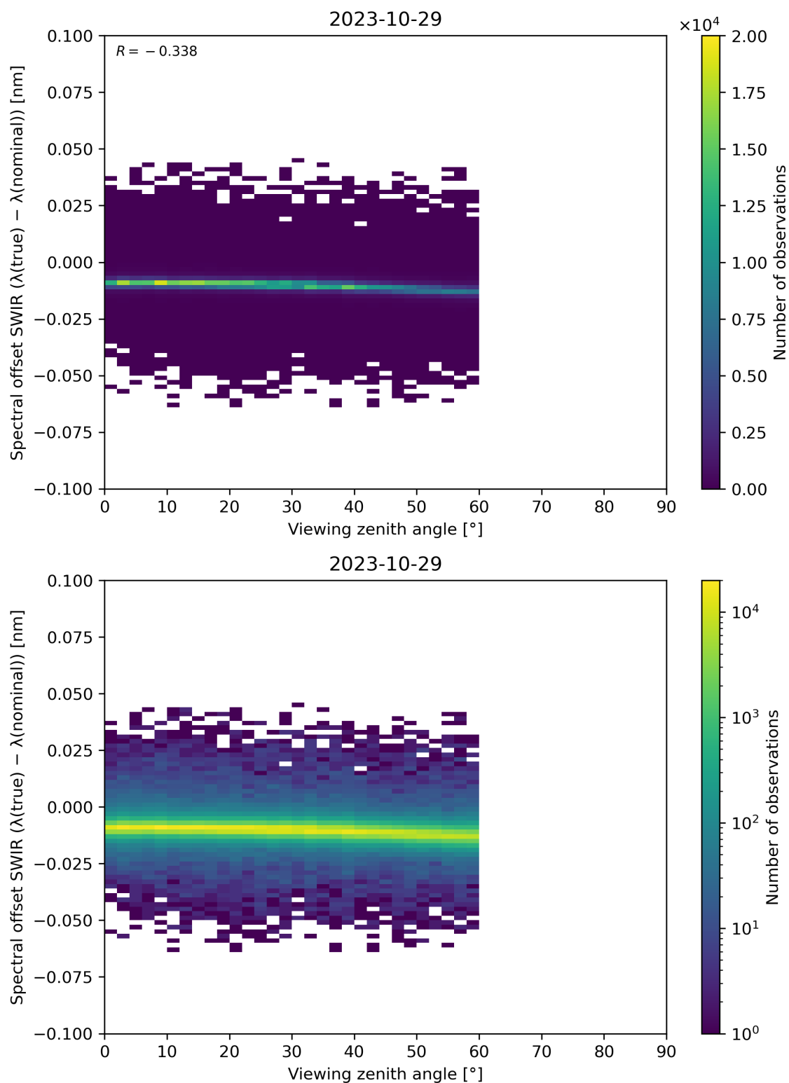
Figure 116: Scatter density plot of “Viewing zenith angle” against “Spectral offset SWIR ( \lambda(\text{true}) - \lambda(\text{nominal}) )” for 2023-10-28 to 2023-10-30.
