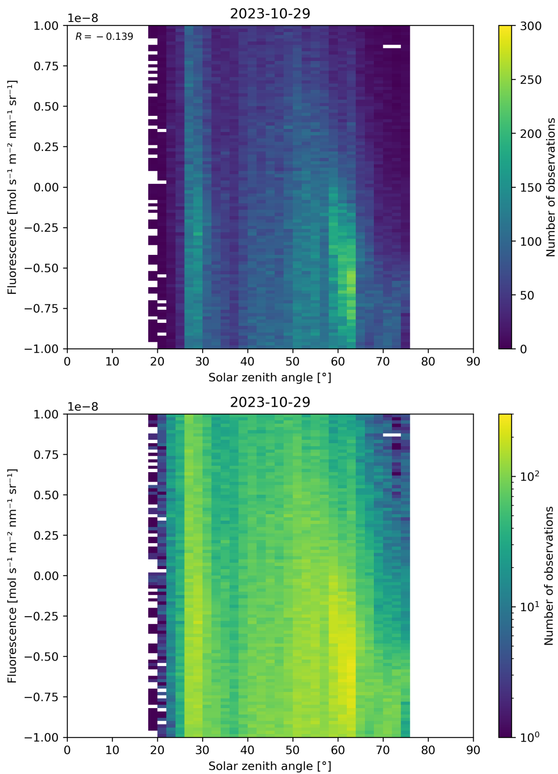
Figure 97: Scatter density plot of “Solar zenith angle” against “Fluorescence” for 2023-10-28 to 2023-10-30.
