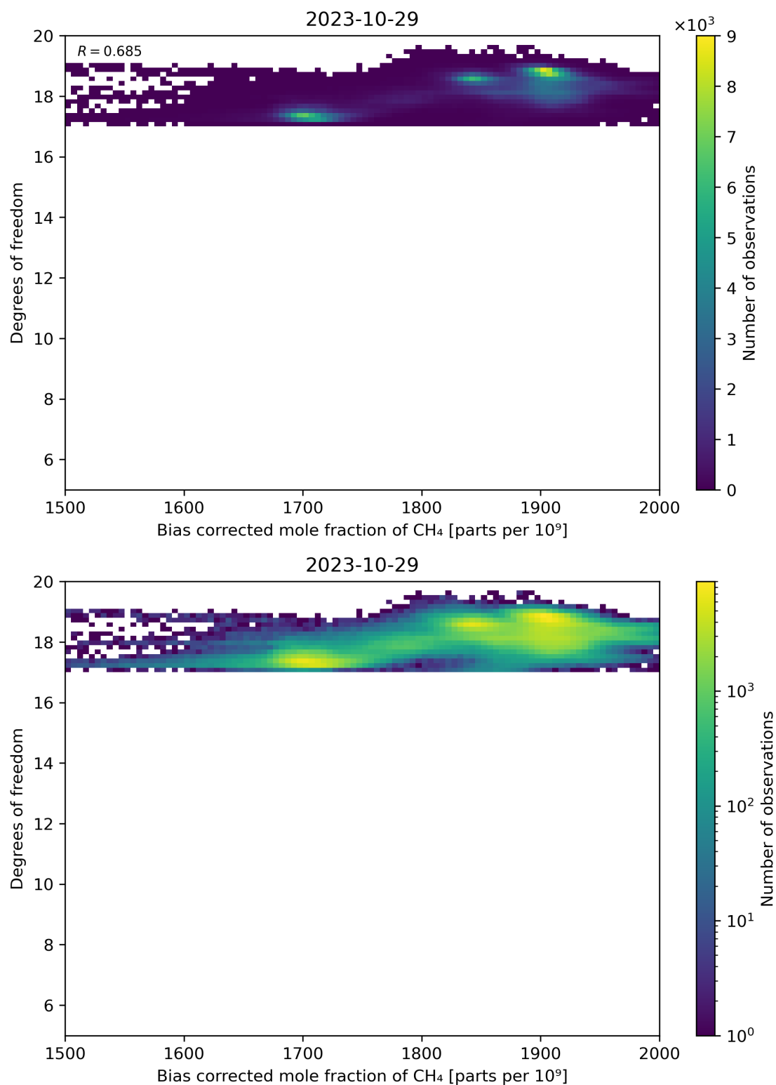
Figure 65: Scatter density plot of “Bias corrected mole fraction of \text{CH}_4 ” against “Degrees of freedom” for 2023-10-28 to 2023-10-30.
