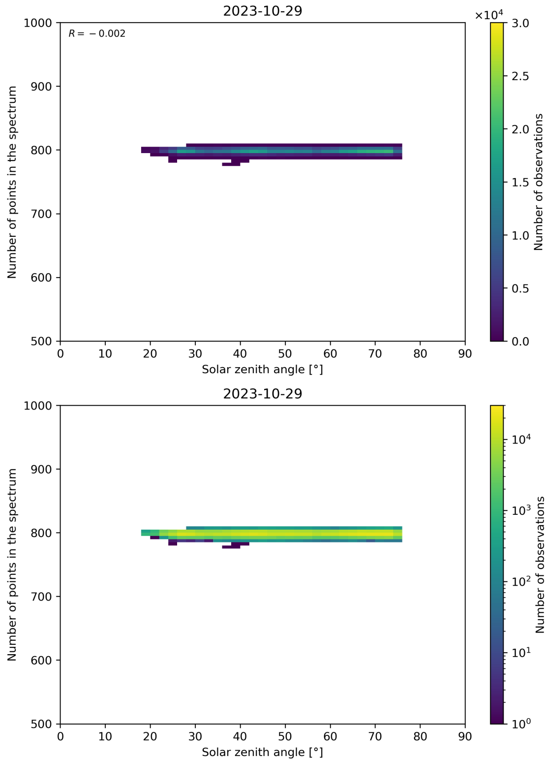
Figure 103: Scatter density plot of “Solar zenith angle” against “Number of points in the spectrum” for 2023-10-28 to 2023-10-30.
