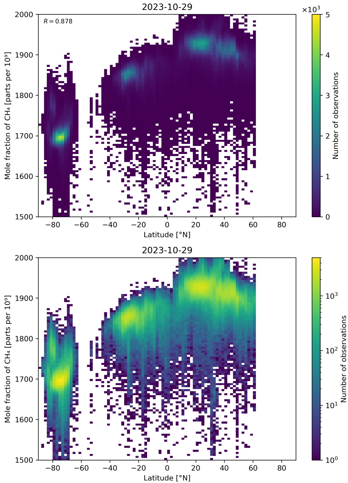
Figure 57: Scatter density plot of “Latitude” against “Mole fraction of CH 4 ” for 2023-10-28 to 2023-10-30.
