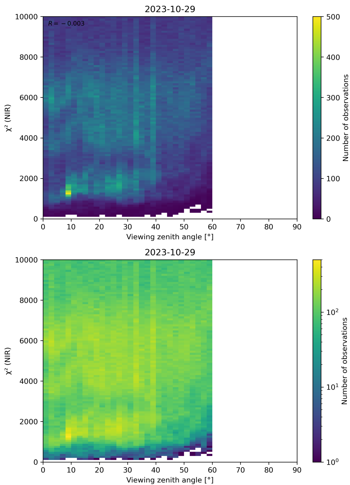
Figure 105: Scatter density plot of “Viewing zenith angle” against “ \chi^2 (NIR)” for 2023-10-28 to 2023-10-30.
