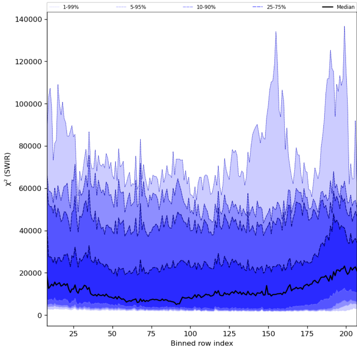
Figure 39: Along track statistics of " \chi^2 (SWIR)" for 2023-10-28 to 2023-10-30
