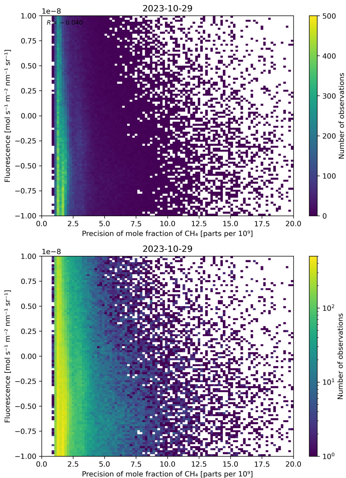
Figure 81: Scatter density plot of “Precision of mole fraction of CH 4 ” against “Fluorescence” for 2023-10-28 to 2023-10-30.
