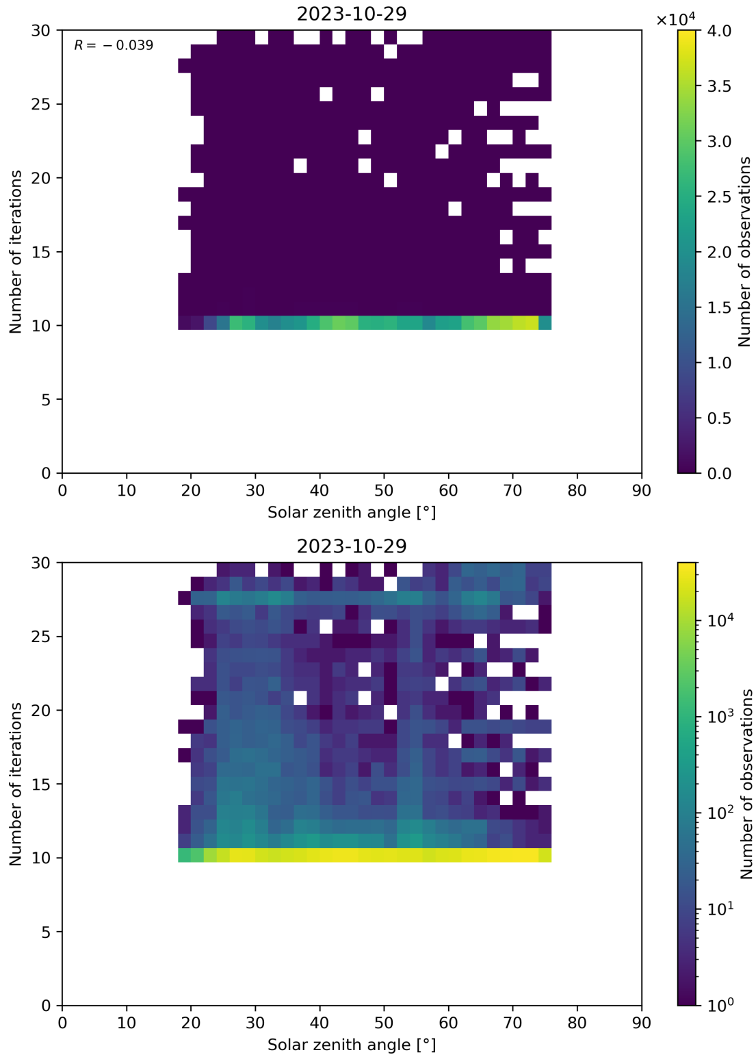
Figure 102: Scatter density plot of “Solar zenith angle” against “Number of iterations” for 2023-10-28 to 2023-10-30.
