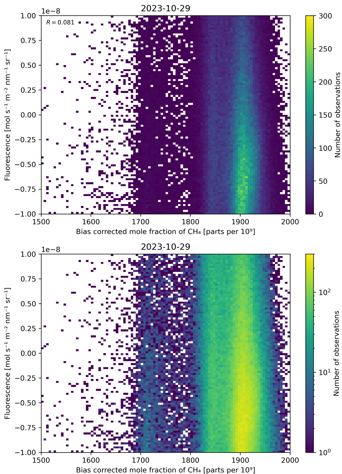
Figure 66: Scatter density plot of “Bias corrected mole fraction of \text{CH}_4 ” against “Fluorescence” for 2023-10-28 to 2023-10-30.
