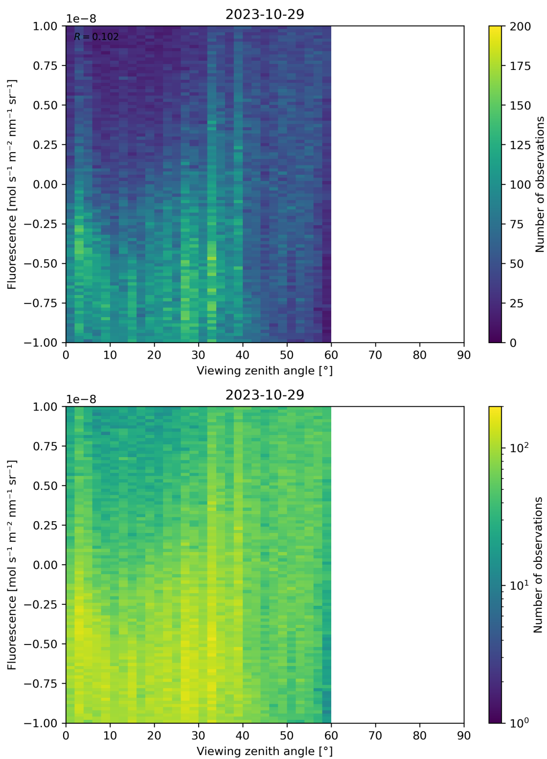
Figure 108: Scatter density plot of “Viewing zenith angle” against “Fluorescence” for 2023-10-28 to 2023-10-30.
