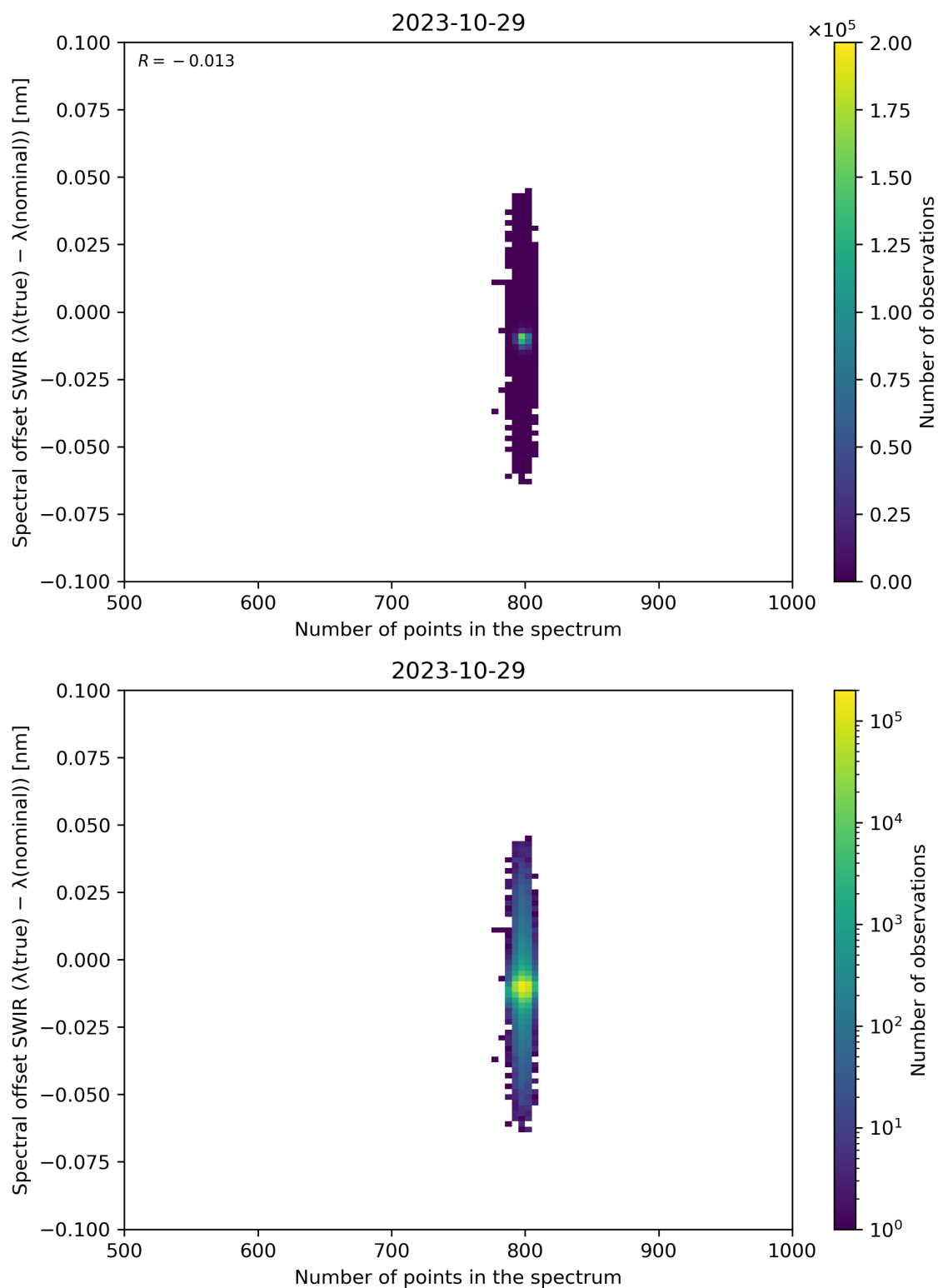
Figure 93: Scatter density plot of “Number of points in the spectrum” against “Spectral offset SWIR ( \lambda(\text{true}) - \lambda(\text{nominal}) )” for 2023-10-28 to 2023-10-30.
