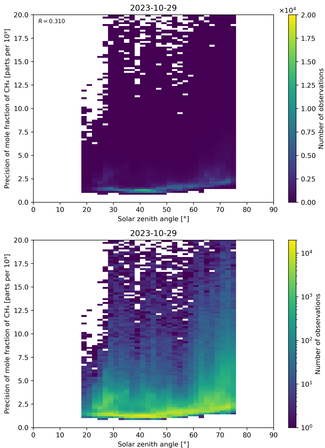
Figure 101: Scatter density plot of “Solar zenith angle” against “Precision of mole fraction of \text{CH}_4 ” for 2023-10-28 to 2023-10-30.
