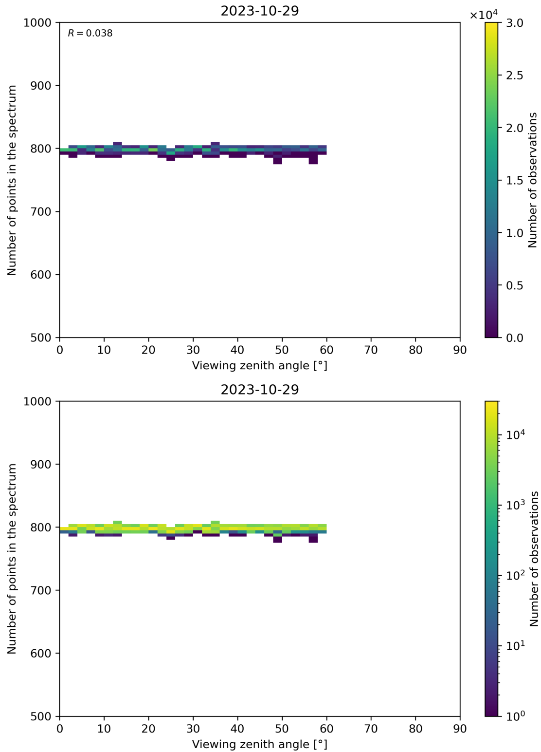
Figure 114: Scatter density plot of “Viewing zenith angle” against “Number of points in the spectrum” for 2023-10-28 to 2023-10-30.
