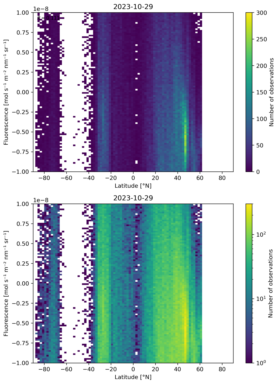
Figure 56: Scatter density plot of “Latitude” against “Fluorescence” for 2023-10-28 to 2023-10-30.
