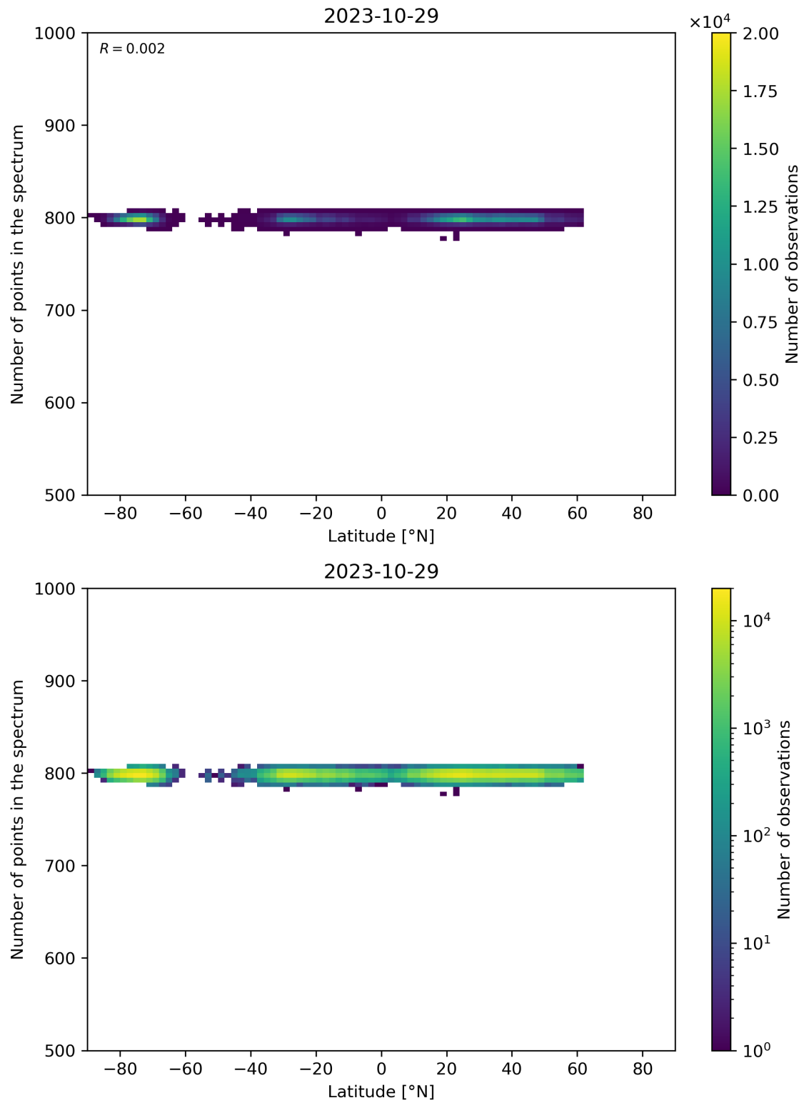
Figure 61: Scatter density plot of “Latitude” against “Number of points in the spectrum” for 2023-10-28 to 2023-10-30.
