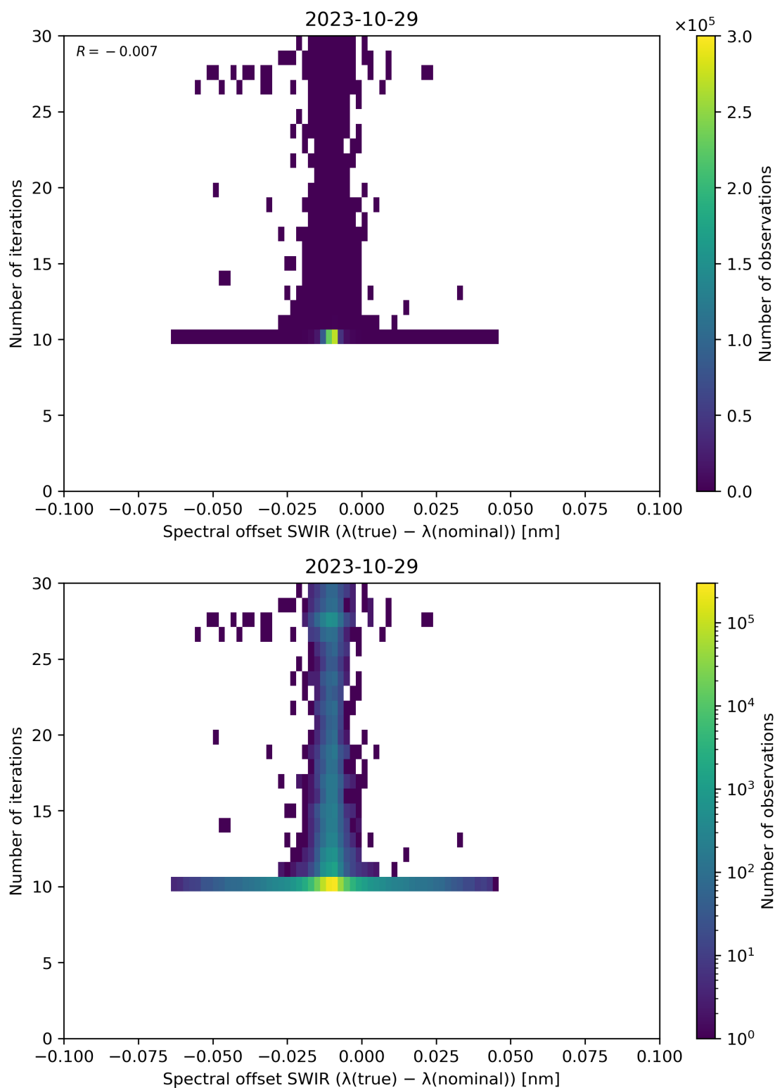
Figure 121: Scatter density plot of “Spectral offset SWIR ( \lambda(\text{true}) - \lambda(\text{nominal}) )” against “Number of iterations” for 2023-10-28 to 2023-10-30.
