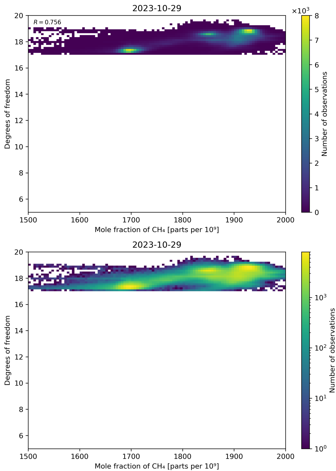
Figure 72: Scatter density plot of “Mole fraction of CH 4 ” against “Degrees of freedom” for 2023-10-28 to 2023-10-30.
