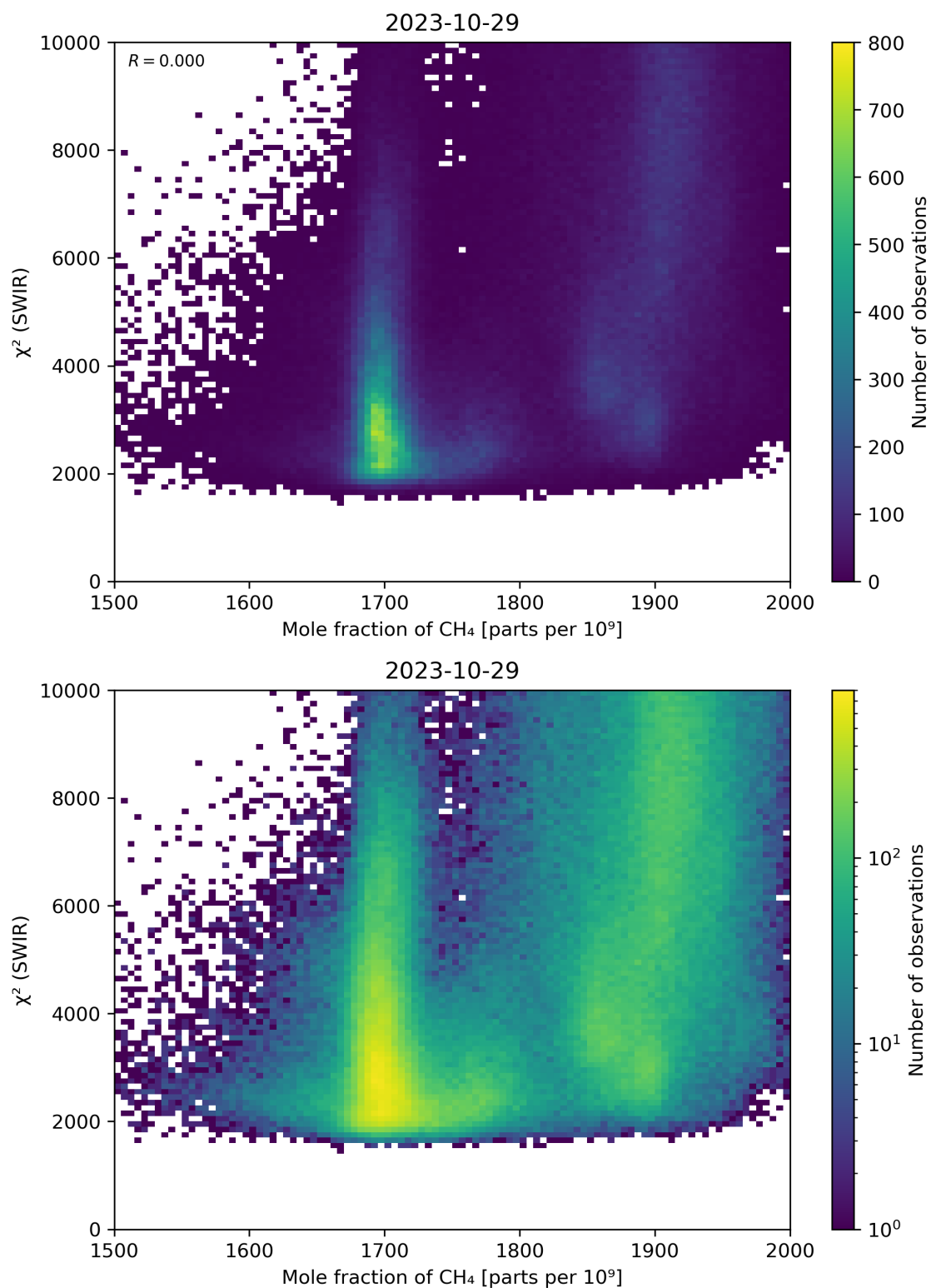
Figure 71: Scatter density plot of “Mole fraction of CH 4 ” against “ \chi^2 (SWIR)” for 2023-10-28 to 2023-10-30.
