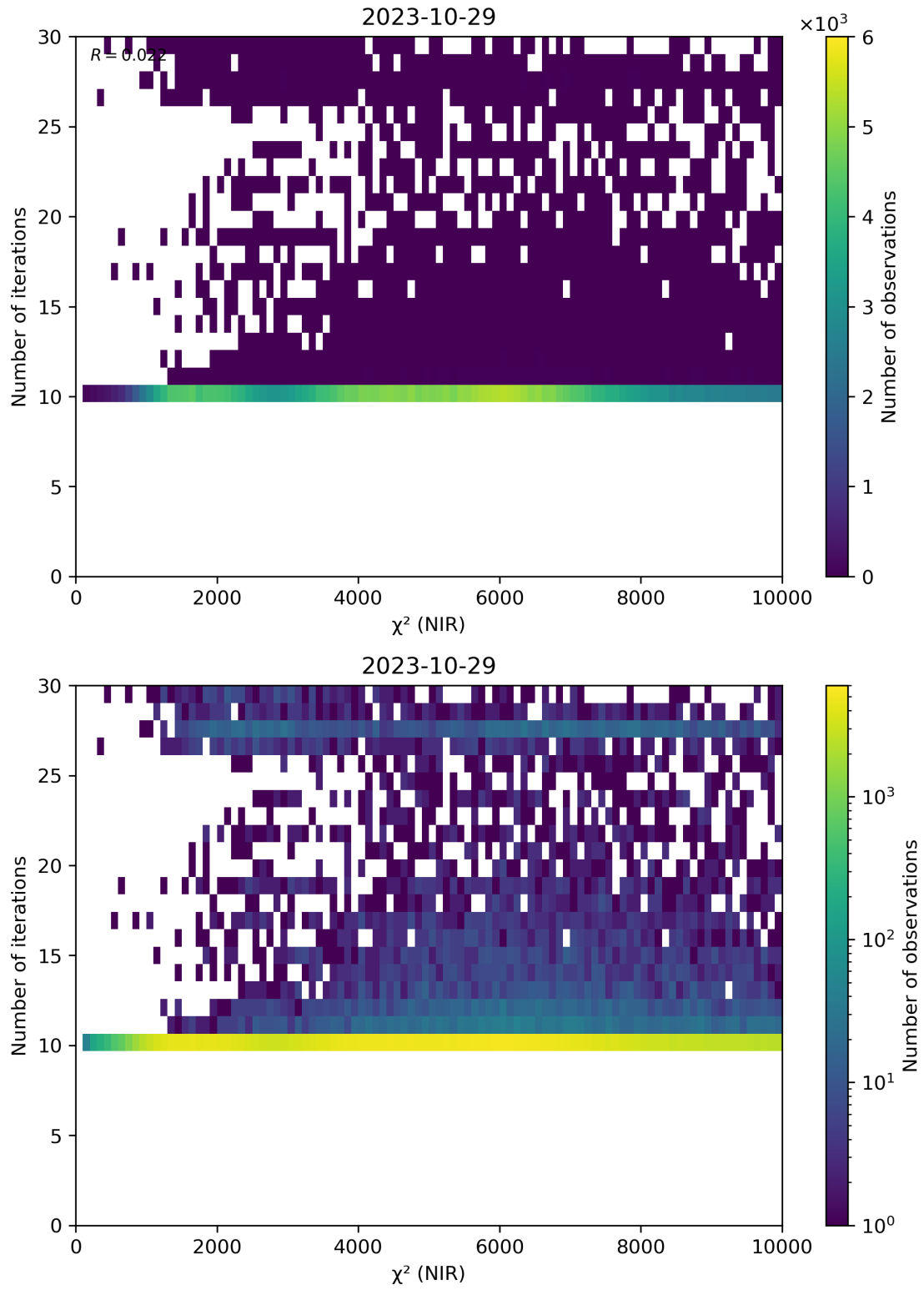
Figure 46: Scatter density plot of “ \chi^2 (NIR)” against “Number of iterations” for 2023-10-28 to 2023-10-30.
