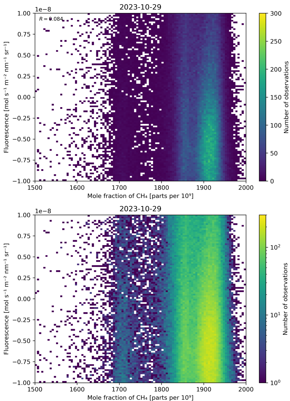
Figure 73: Scatter density plot of “Mole fraction of CH 4 ” against “Fluorescence” for 2023-10-28 to 2023-10-30.
