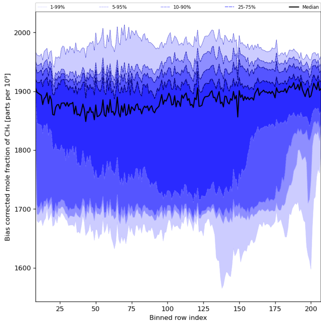
Figure 36: Along track statistics of “Bias corrected mole fraction of \text{CH}_4 ” for 2023-10-28 to 2023-10-30
