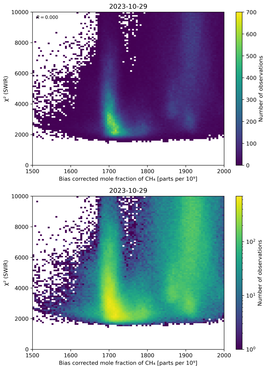
Figure 64: Scatter density plot of “Bias corrected mole fraction of CH 4 ” against “ \chi^2 (SWIR)” for 2023-10-28 to 2023-10-30.
