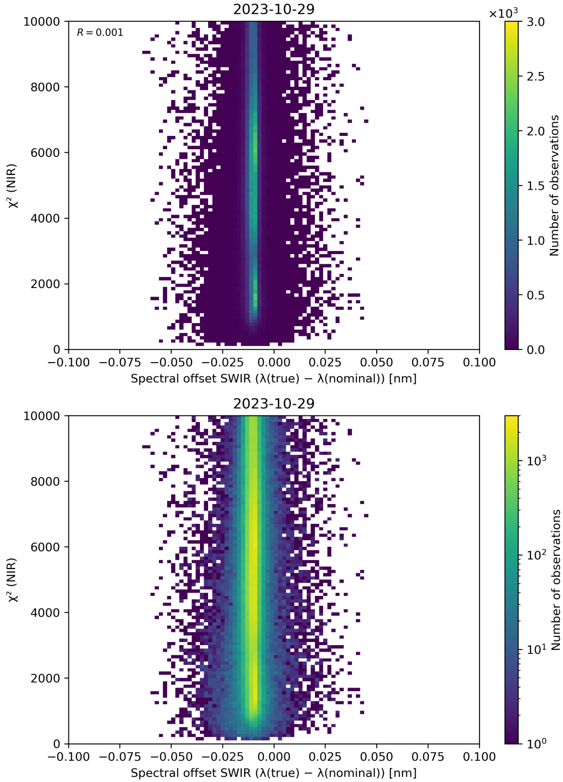
Figure 117: Scatter density plot of “Spectral offset SWIR ( \lambda(\text{true}) - \lambda(\text{nominal}) )” against “ \chi^2 (NIR)” for 2023-10-28 to 2023-10-30.
