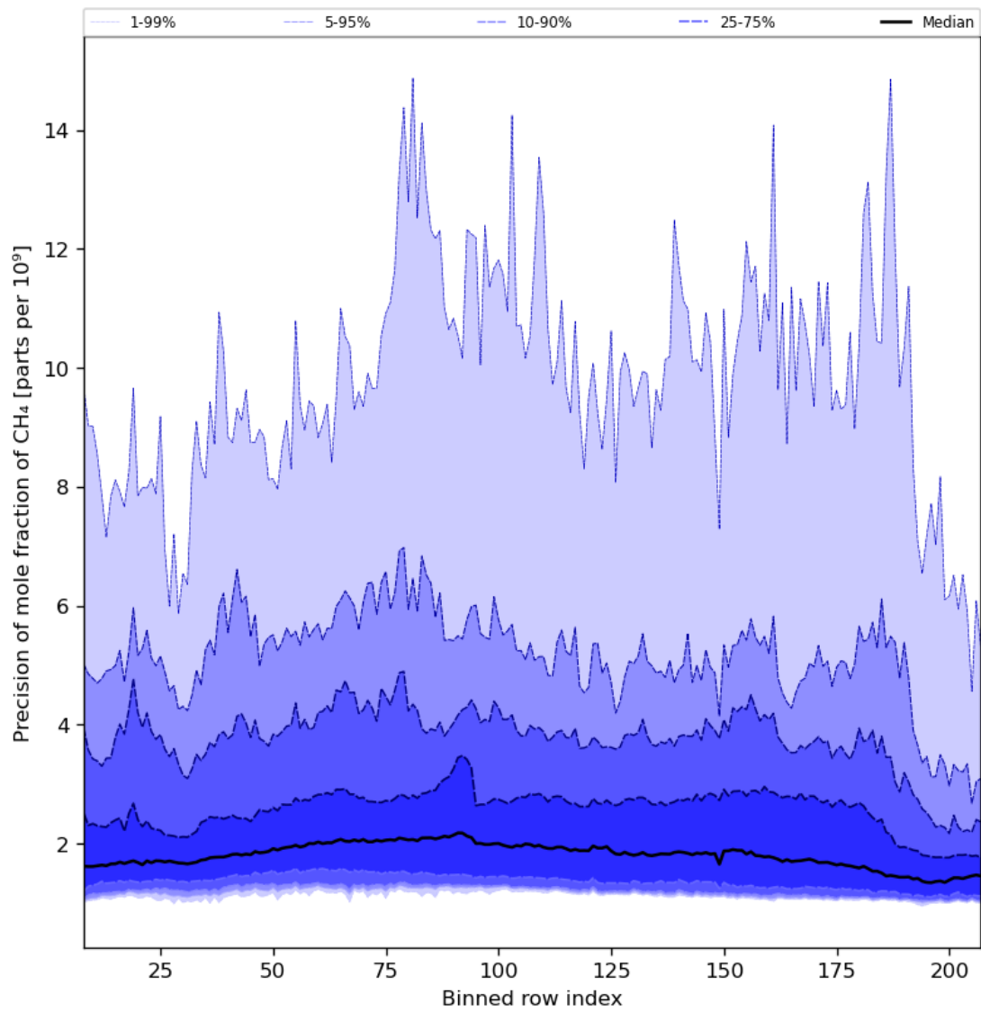
Figure 35: Along track statistics of “Precision of mole fraction of CH 4 ” for 2023-10-28 to 2023-10-30
