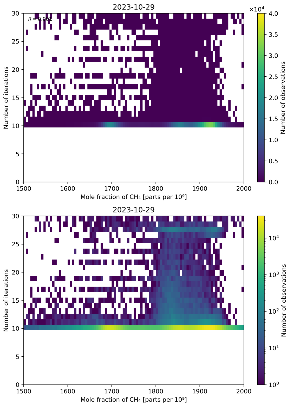
Figure 76: Scatter density plot of “Mole fraction of CH 4 ” against “Number of iterations” for 2023-10-28 to 2023-10-30.
