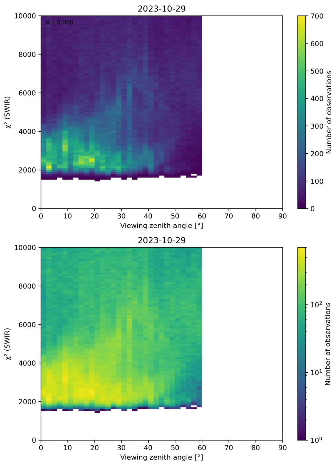
Figure 106: Scatter density plot of “Viewing zenith angle” against “ \chi^2 (SWIR)” for 2023-10-28 to 2023-10-30.
