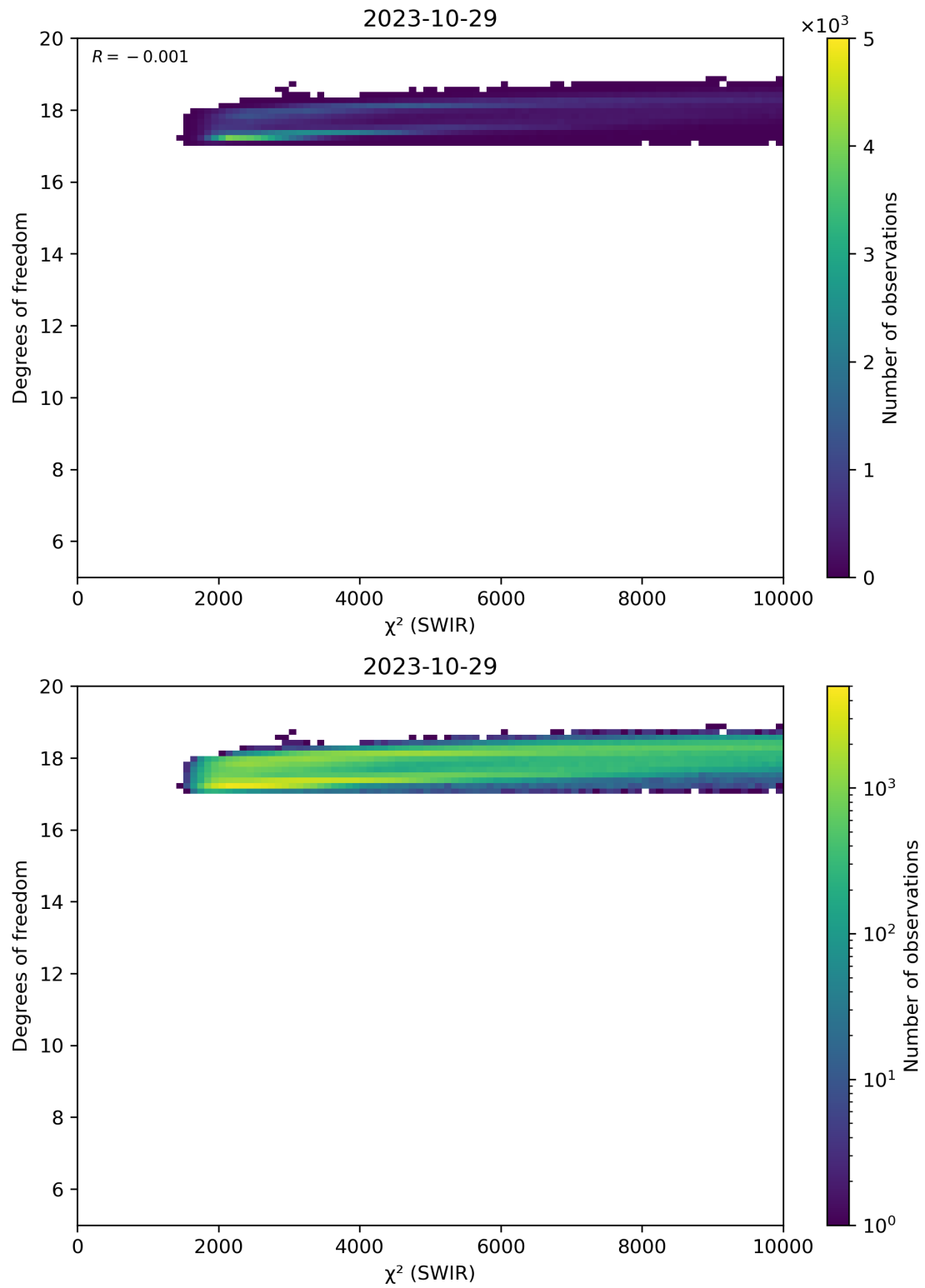
Figure 48: Scatter density plot of “ \chi^2 (SWIR)” against “Degrees of freedom” for 2023-10-28 to 2023-10-30.
