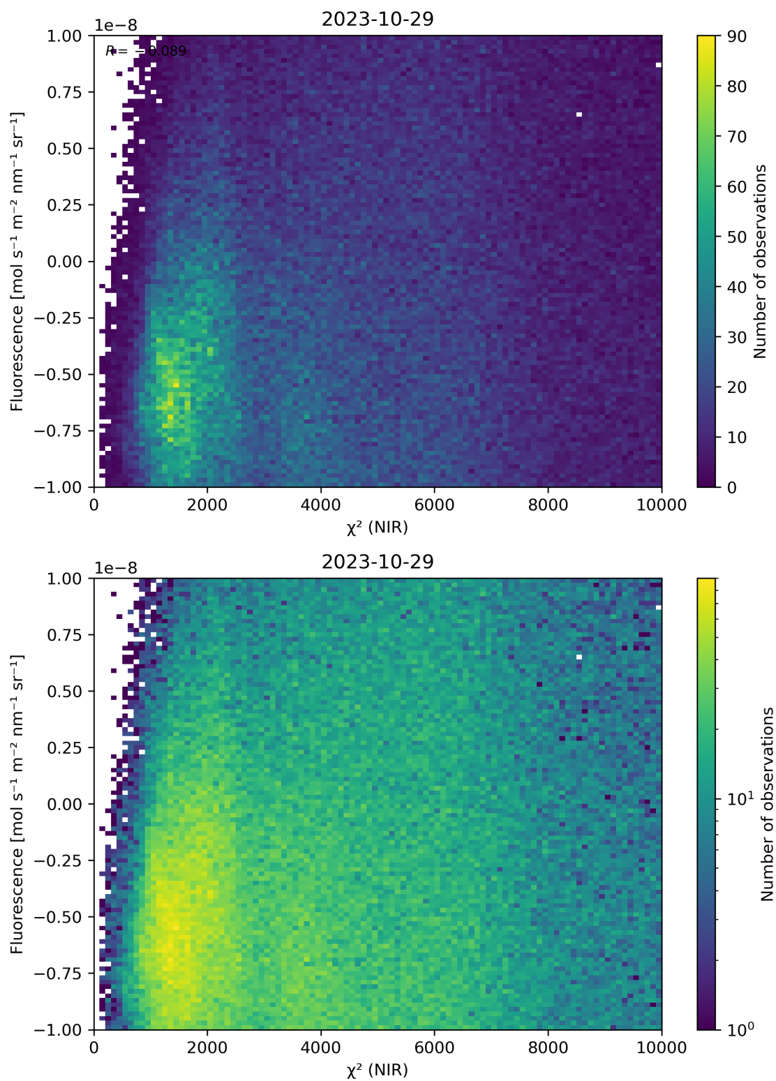
Figure 45: Scatter density plot of “ \chi^2 (NIR)” against “Fluorescence” for 2023-10-28 to 2023-10-30.
