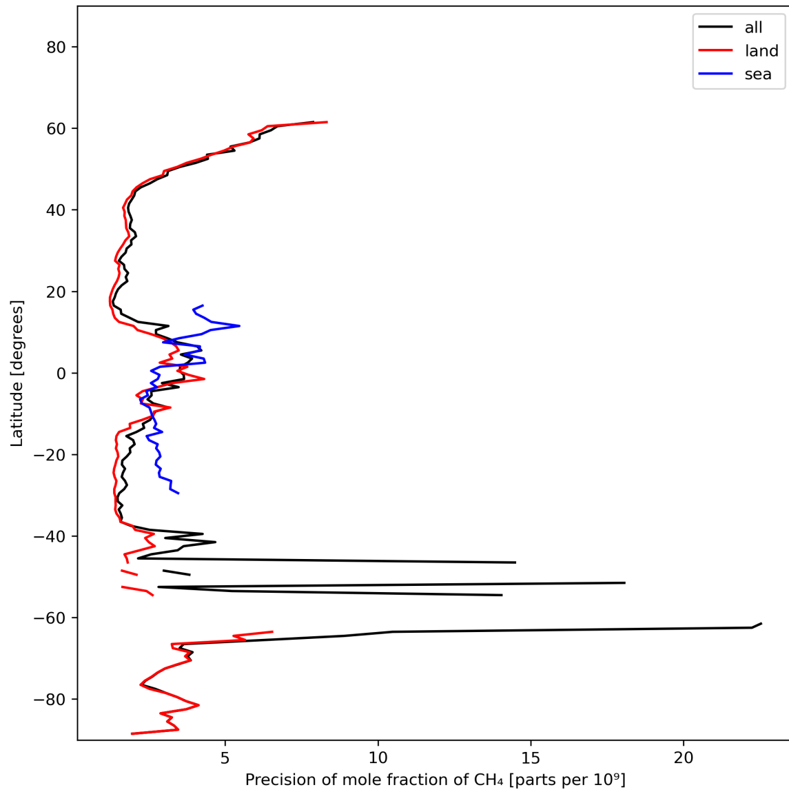
Figure 13: Zonal average of “Precision of mole fraction of CH 4 ” for 2023-10-28 to 2023-10-30.
