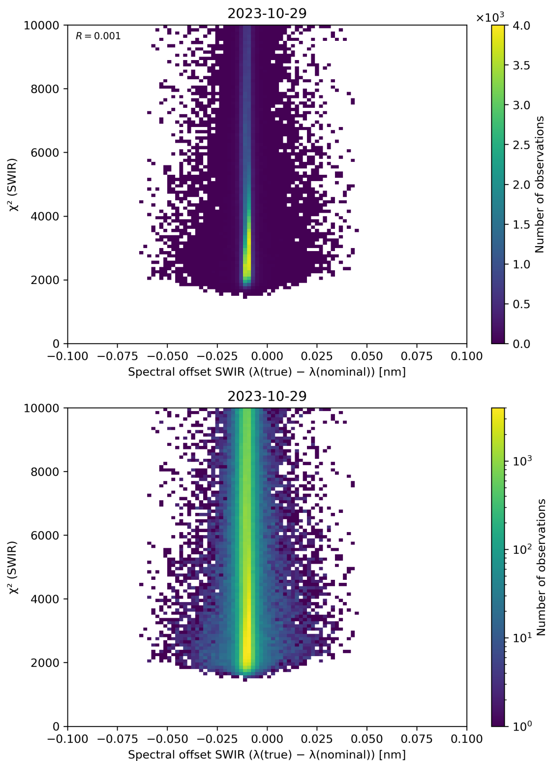
Figure 118: Scatter density plot of “Spectral offset SWIR ( \lambda(\text{true}) - \lambda(\text{nominal}) )” against “ \chi^2 (SWIR)” for 2023-10-28 to 2023-10-30.
