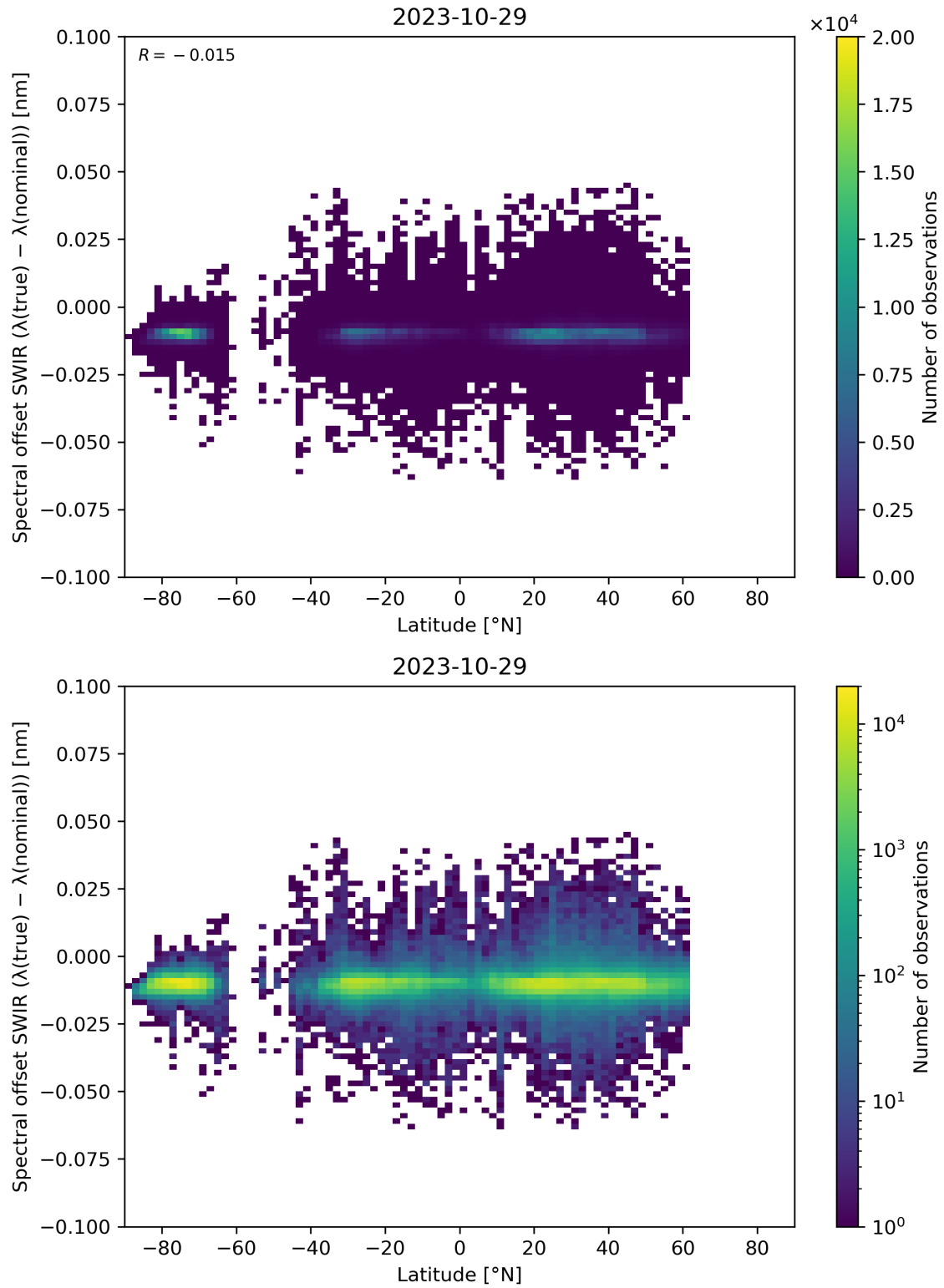
Figure 62: Scatter density plot of “Latitude” against “Spectral offset SWIR ( \lambda(\text{true}) - \lambda(\text{nominal}) )” for 2023-10-28 to 2023-10-30.
