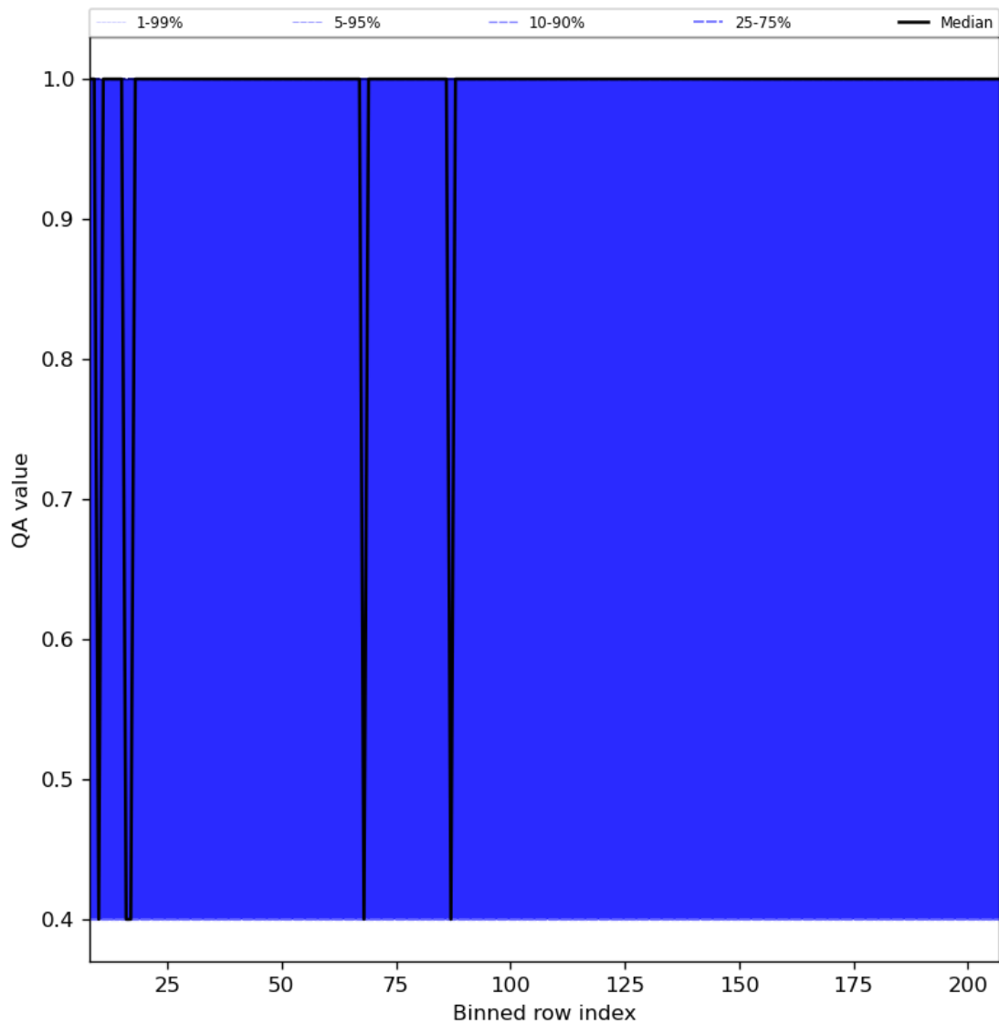
Figure 33: Along track statistics of “QA value” for 2023-10-28 to 2023-10-30
