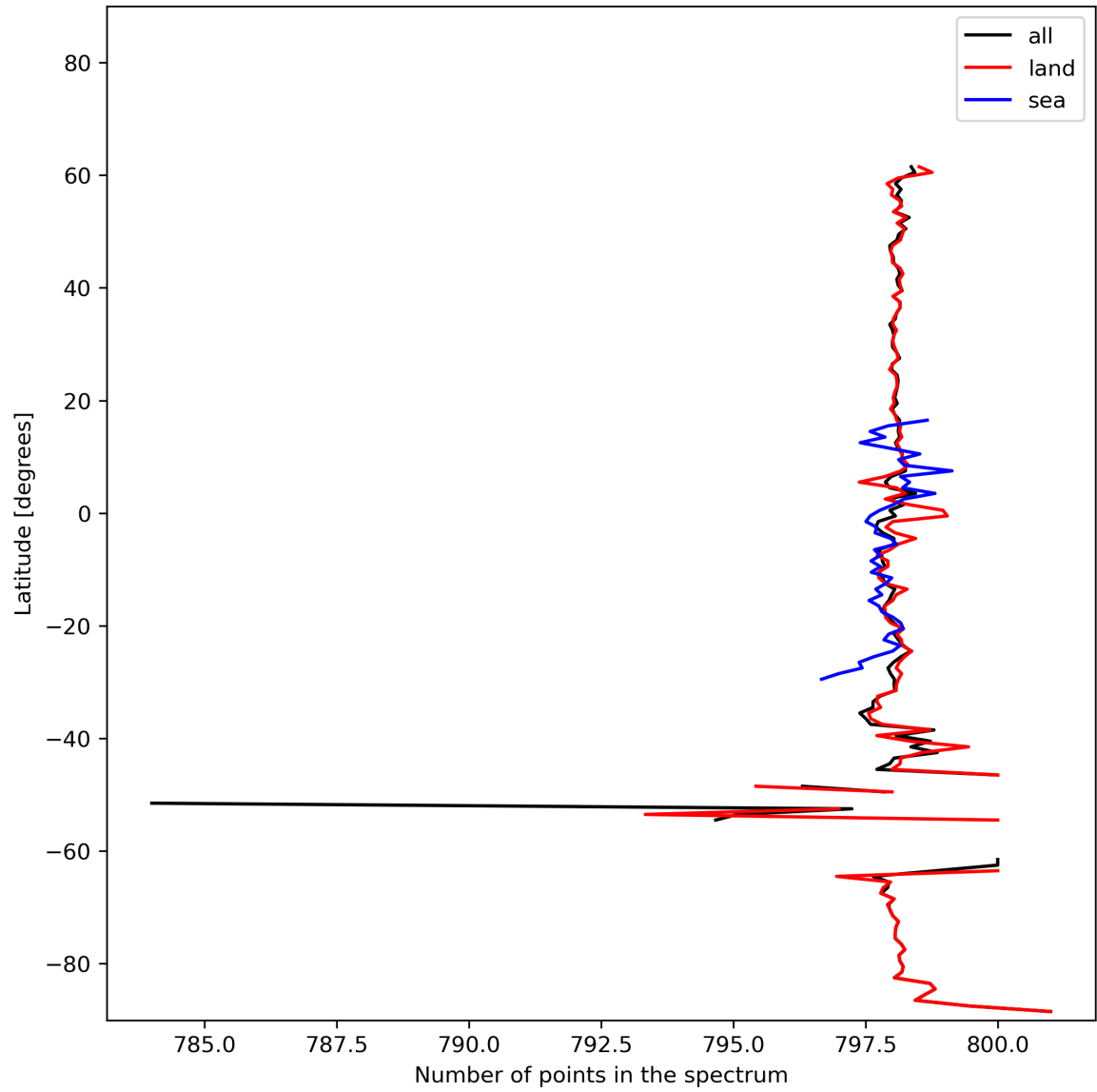
Figure 15: Zonal average of “Number of points in the spectrum” for 2023-10-28 to 2023-10-30.
