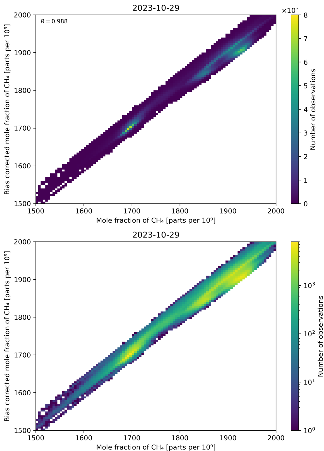
Figure 74: Scatter density plot of “Mole fraction of CH 4 ” against “Bias corrected mole fraction of CH 4 ” for 2023-10-28 to 2023-10-30.
