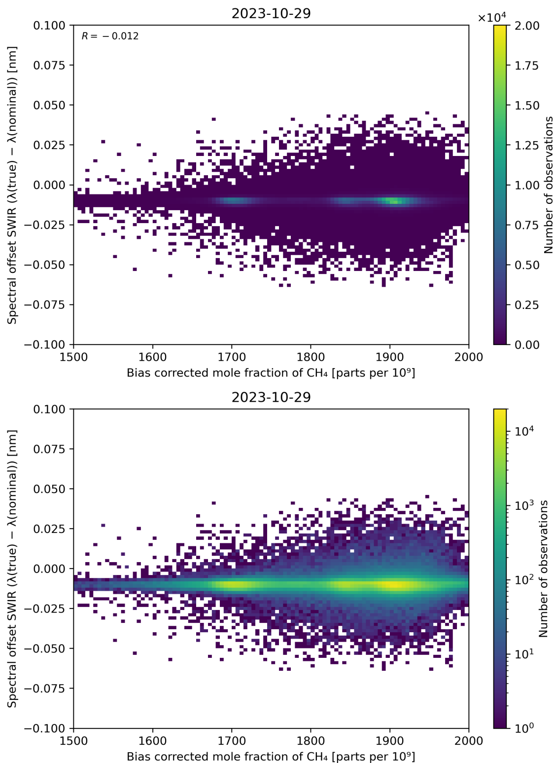
Figure 69: Scatter density plot of “Bias corrected mole fraction of \text{CH}_4 ” against “Spectral offset SWIR ( \lambda(\text{true}) - \lambda(\text{nominal}) )” for 2023-10-28 to 2023-10-30.
