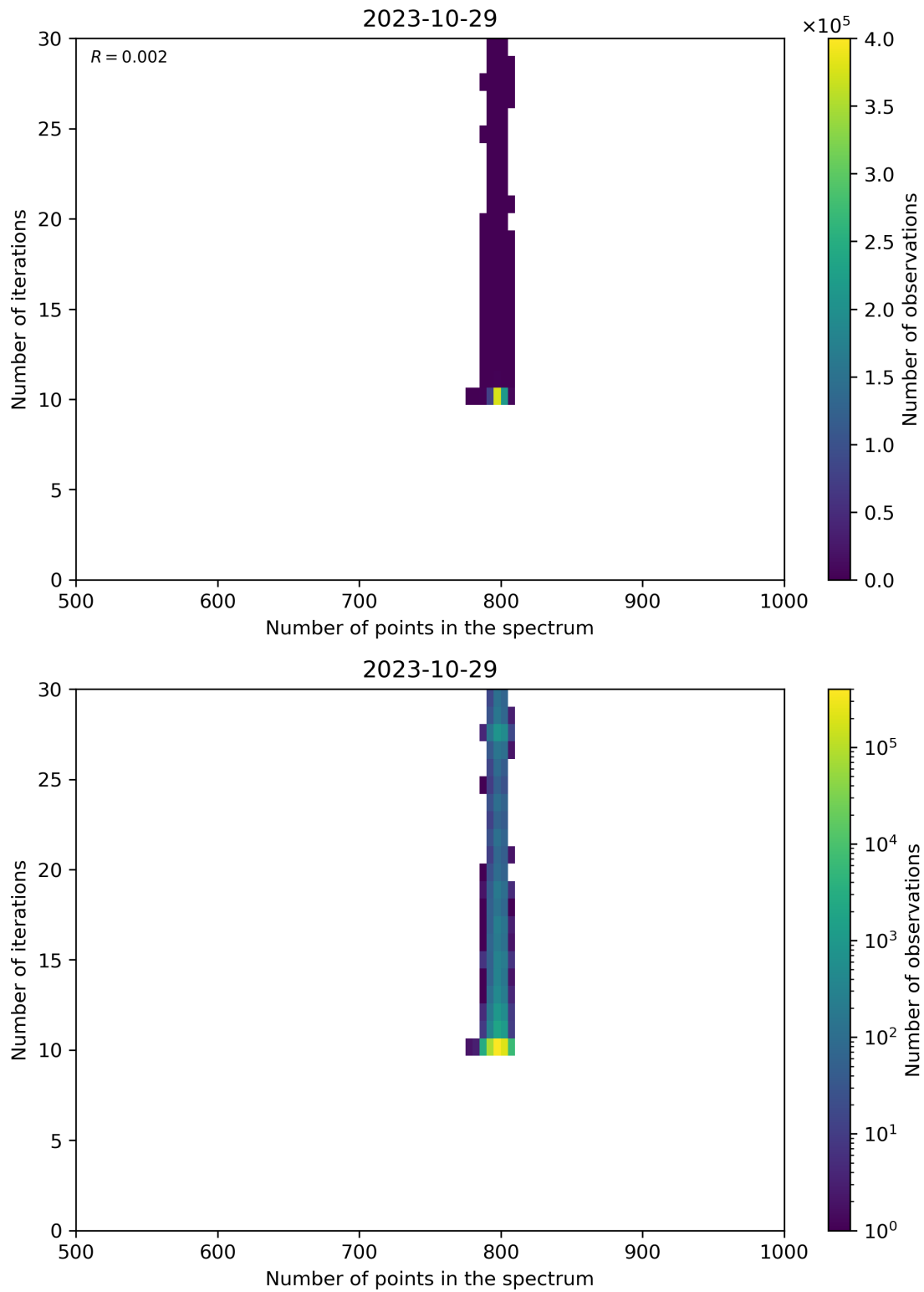
Figure 92: Scatter density plot of “Number of points in the spectrum” against “Number of iterations” for 2023-10-28 to 2023-10-30.
