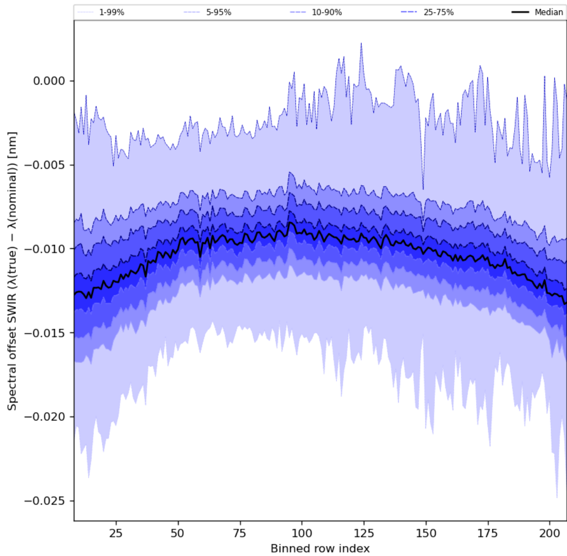
Figure 38: Along track statistics of “Spectral offset SWIR ( \lambda(\text{true}) - \lambda(\text{nominal}) )” for 2023-10-28 to 2023-10-30
