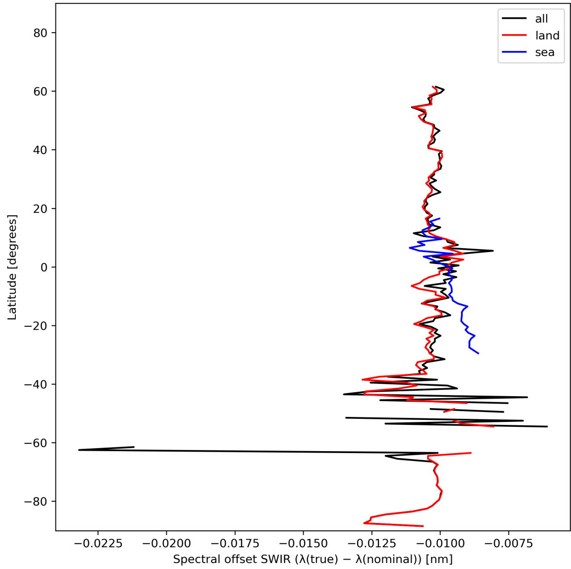
Figure 16: Zonal average of “Spectral offset SWIR ( \lambda(\text{true}) - \lambda(\text{nominal}) )” for 2023-10-28 to 2023-10-30.
