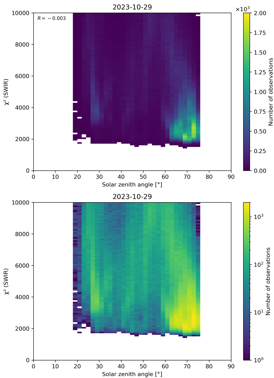
Figure 95: Scatter density plot of “Solar zenith angle” against “ \chi^2 (SWIR)” for 2023-10-28 to 2023-10-30.
