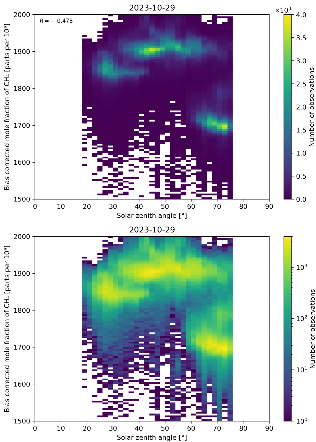
Figure 100: Scatter density plot of “Solar zenith angle” against “Bias corrected mole fraction of \text{CH}_4 ” for 2023-10-28 to 2023-10-30.
