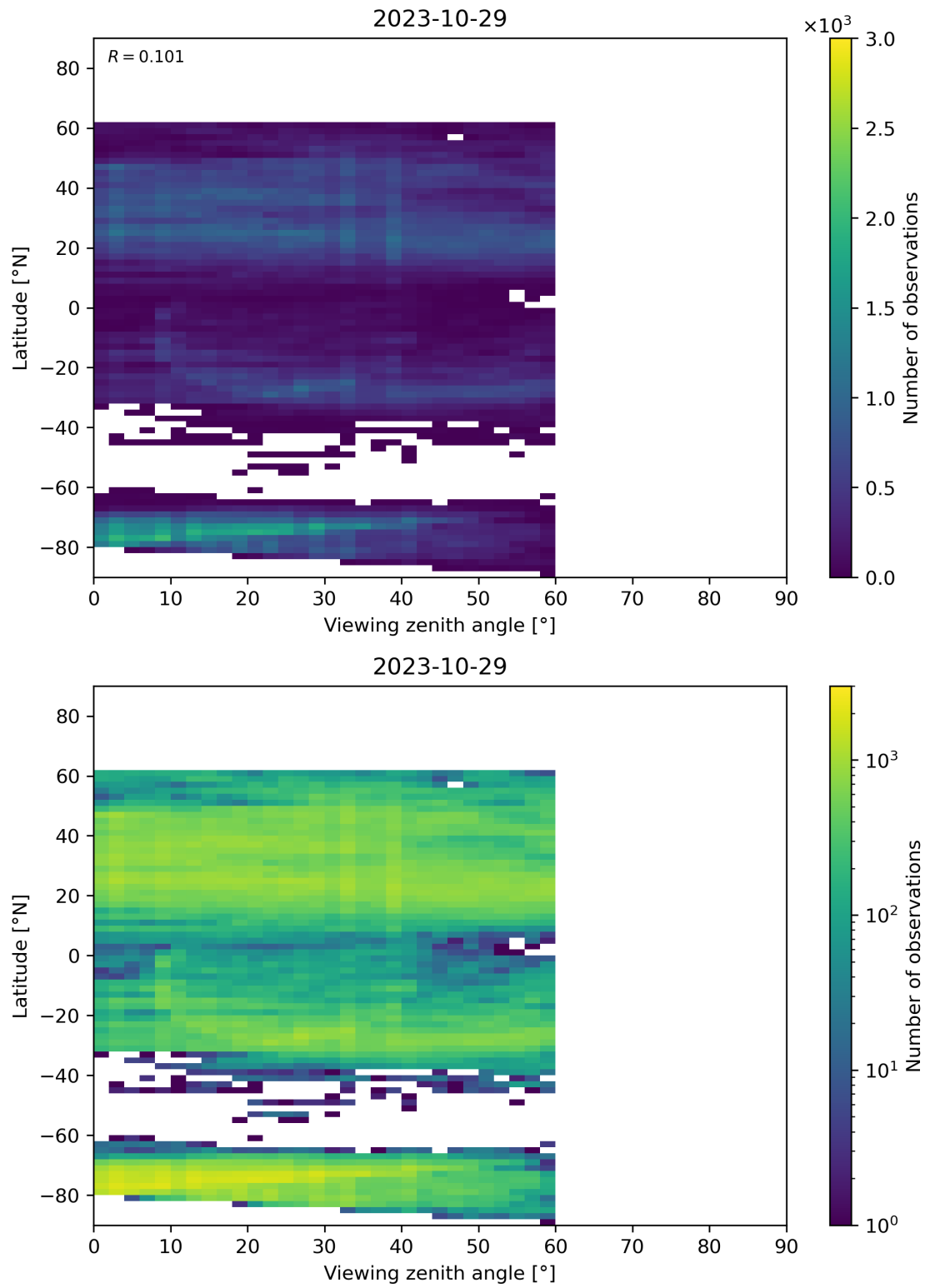
Figure 109: Scatter density plot of “Viewing zenith angle” against “Latitude” for 2023-10-28 to 2023-10-30.
