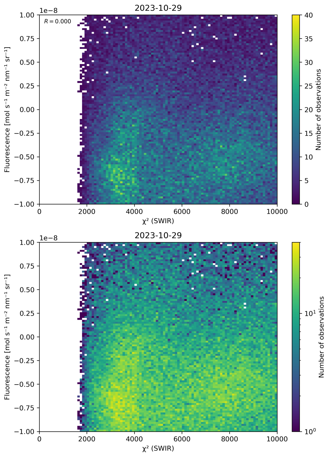
Figure 49: Scatter density plot of “ \chi^2 (SWIR)” against “Fluorescence” for 2023-10-28 to 2023-10-30.
