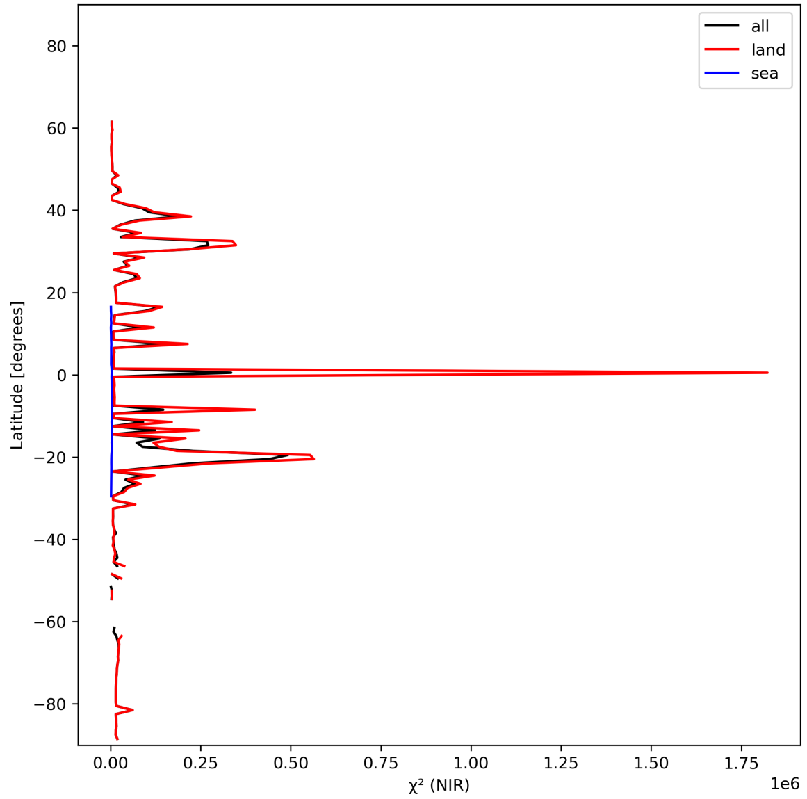
Figure 18: Zonal average of “ \chi^2 (NIR)” for 2023-10-28 to 2023-10-30.
