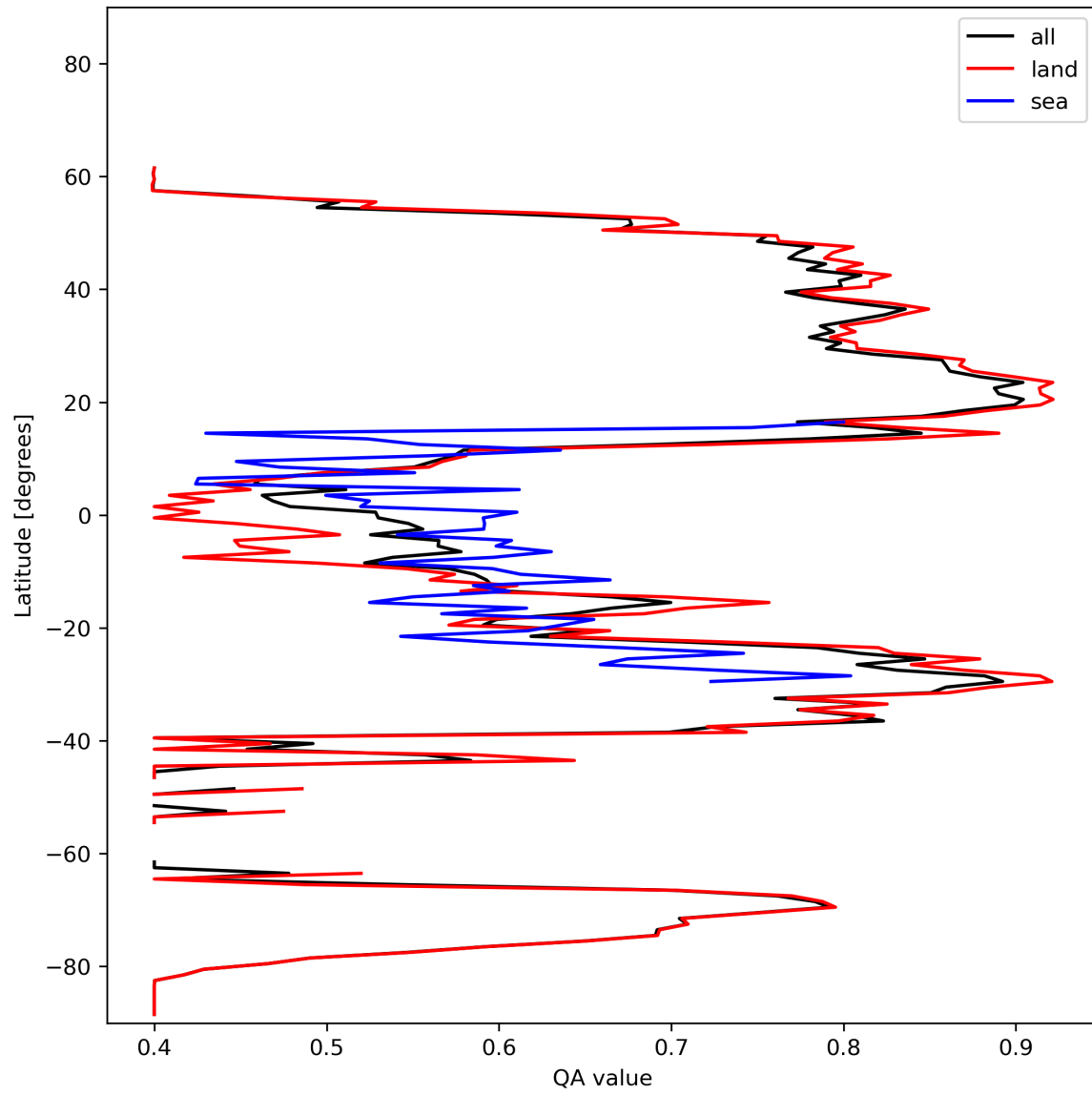
Figure 11: Zonal average of “QA value” for 2023-10-28 to 2023-10-30.
