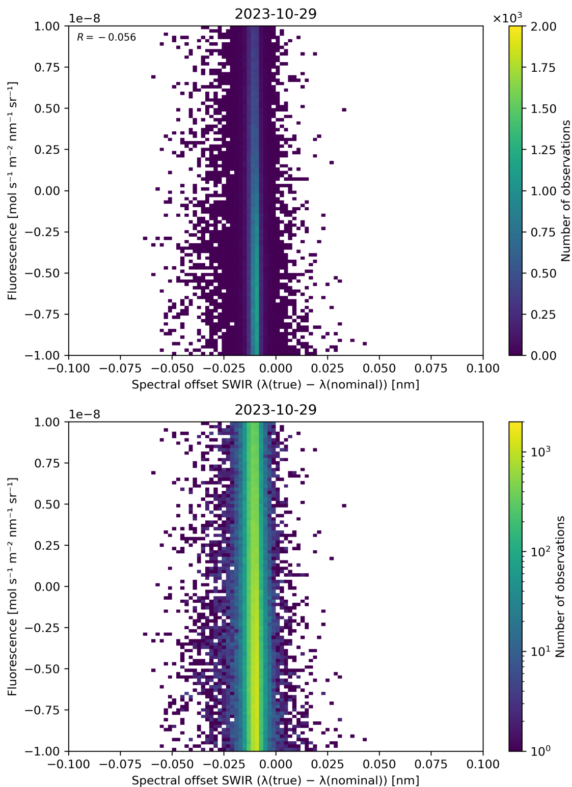
Figure 120: Scatter density plot of “Spectral offset SWIR ( \lambda(\text{true}) - \lambda(\text{nominal}) )” against “Fluorescence” for 2023-10-28 to 2023-10-30.
