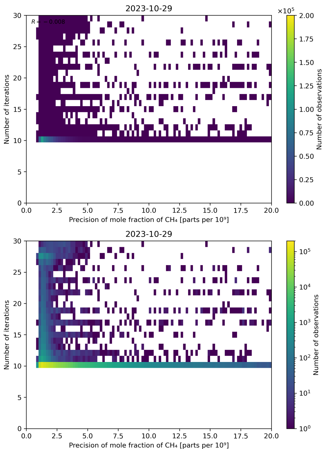
Figure 83: Scatter density plot of “Precision of mole fraction of CH 4 ” against “Number of iterations” for 2023-10-28 to 2023-10-30.
