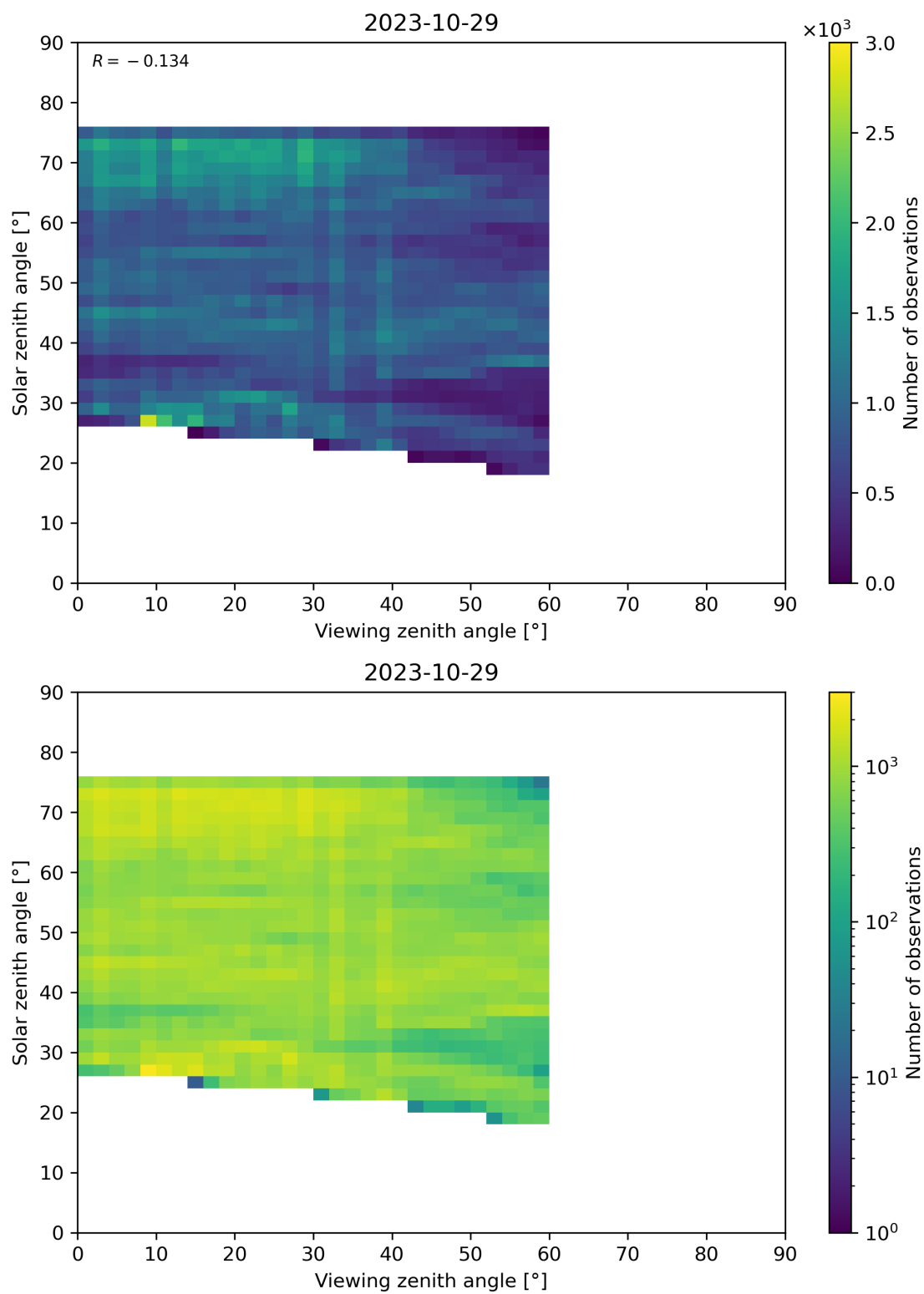
Figure 115: Scatter density plot of “Viewing zenith angle” against “Solar zenith angle” for 2023-10-28 to 2023-10-30.
