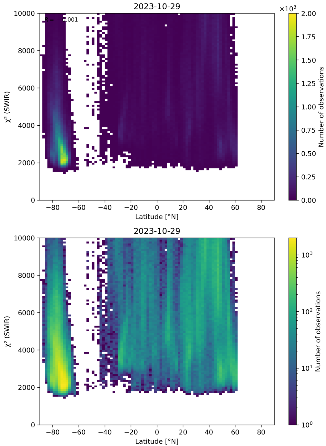
Figure 54: Scatter density plot of “Latitude” against “ \chi^2 (SWIR)” for 2023-10-28 to 2023-10-30.
