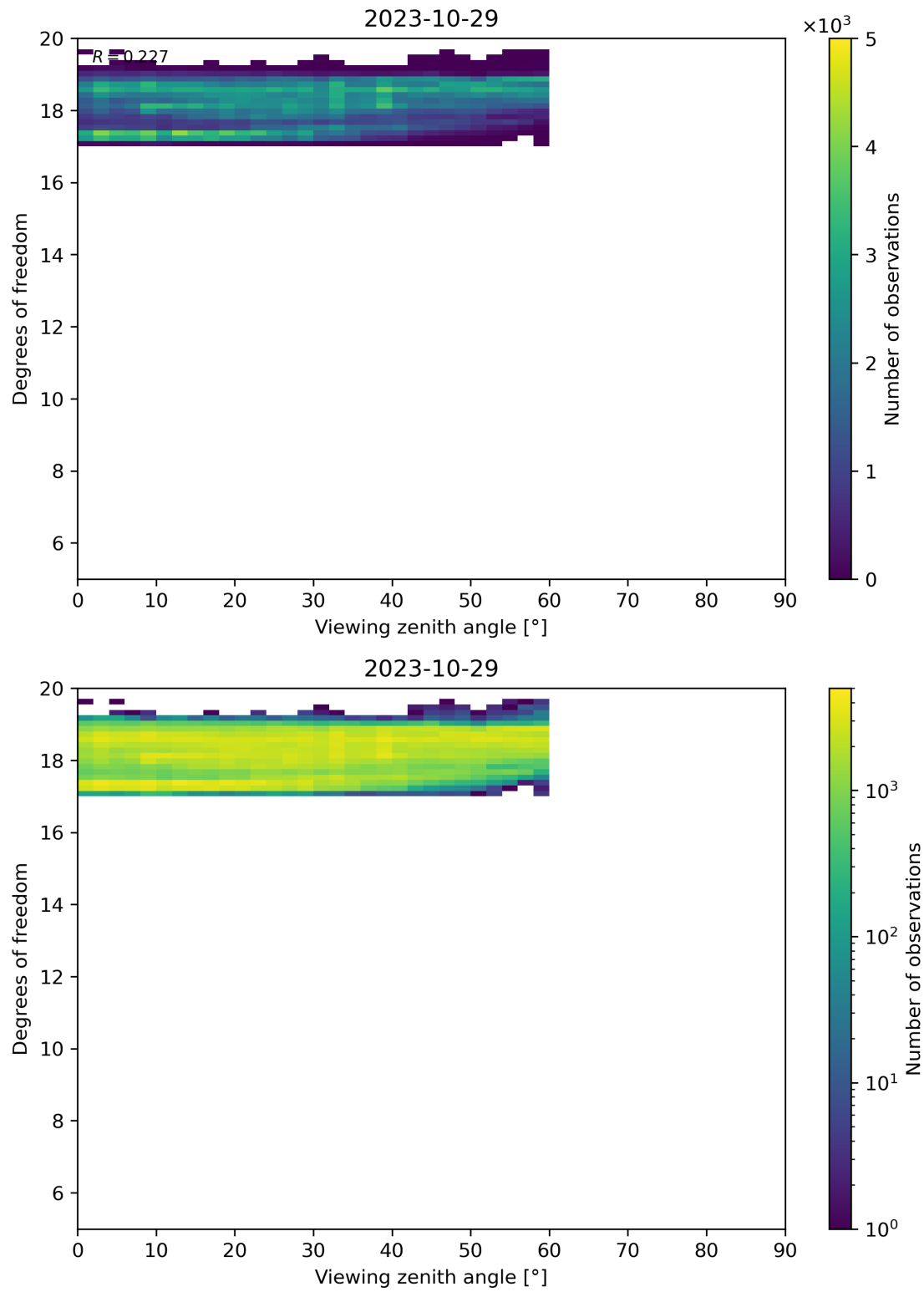
Figure 107: Scatter density plot of “Viewing zenith angle” against “Degrees of freedom” for 2023-10-28 to 2023-10-30.
