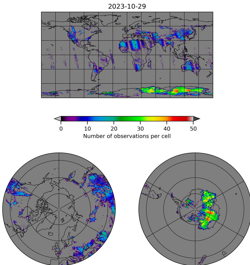
Figure 10: Map of the number of observations for 2023-10-28 to 2023-10-30
