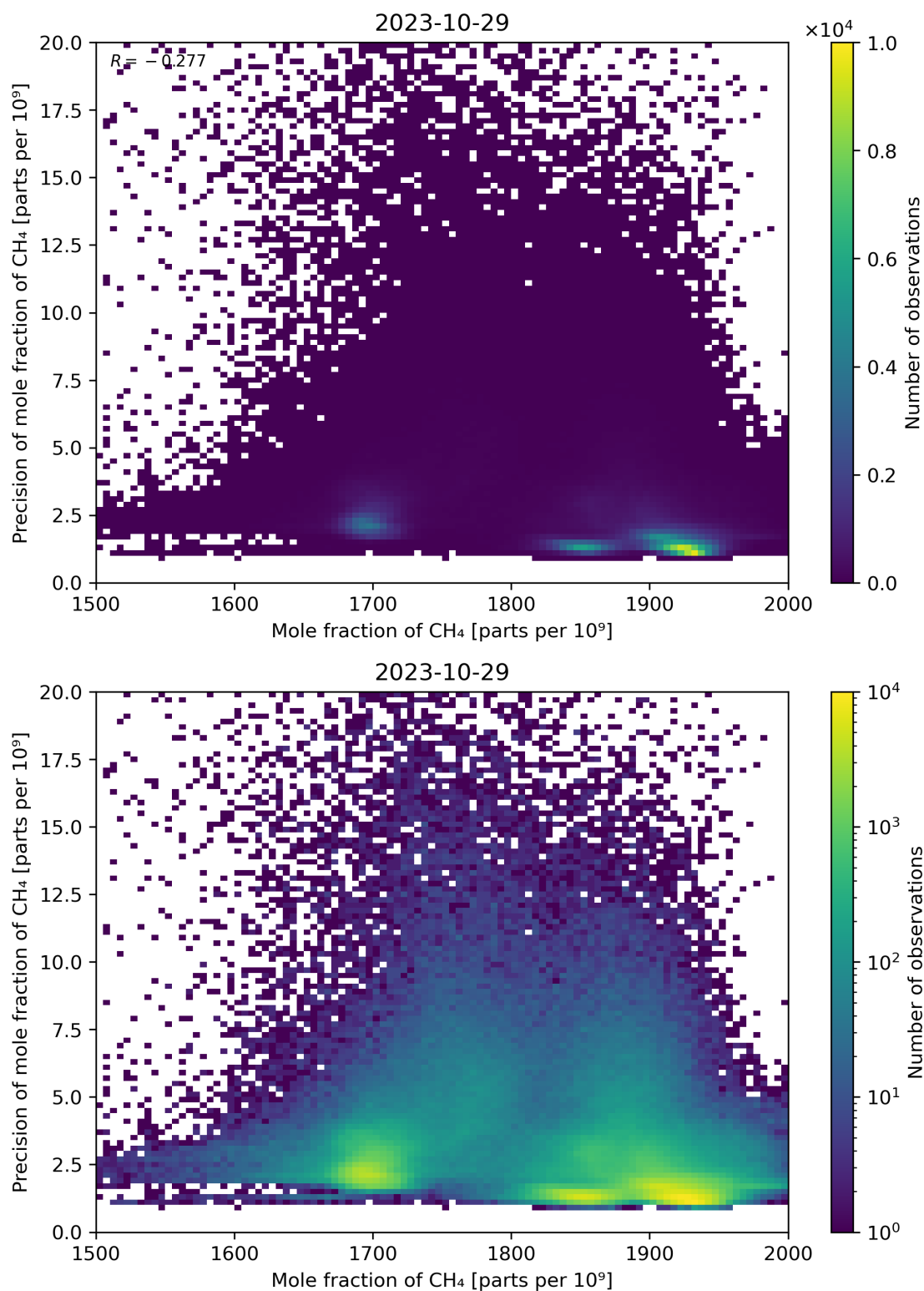
Figure 75: Scatter density plot of “Mole fraction of CH 4 ” against “Precision of mole fraction of CH 4 ” for 2023-10-28 to 2023-10-30.
