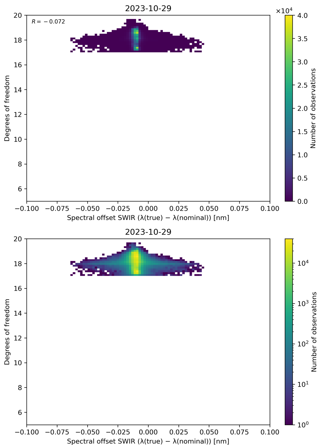
Figure 119: Scatter density plot of “Spectral offset SWIR ( \lambda(\text{true}) - \lambda(\text{nominal}) )” against “Degrees of freedom” for 2023-10-28 to 2023-10-30.
