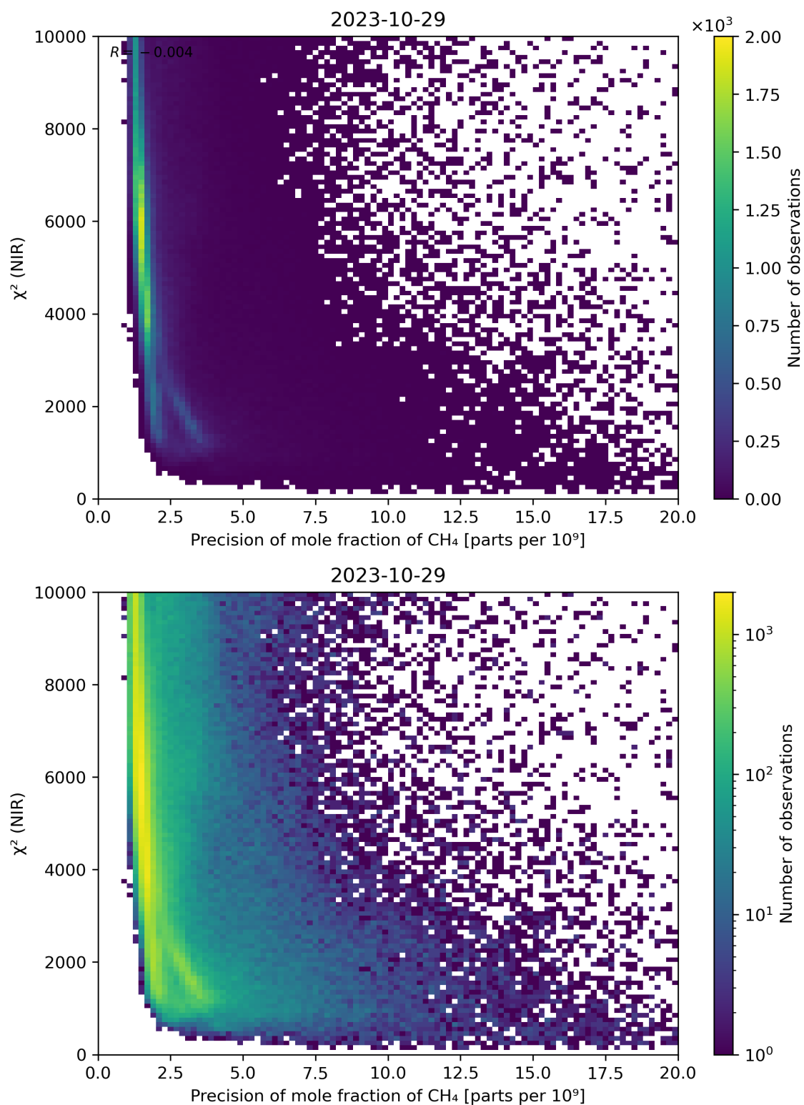
Figure 78: Scatter density plot of “Precision of mole fraction of \text{CH}_4 ” against “ \chi^2 (NIR)” for 2023-10-28 to 2023-10-30.
