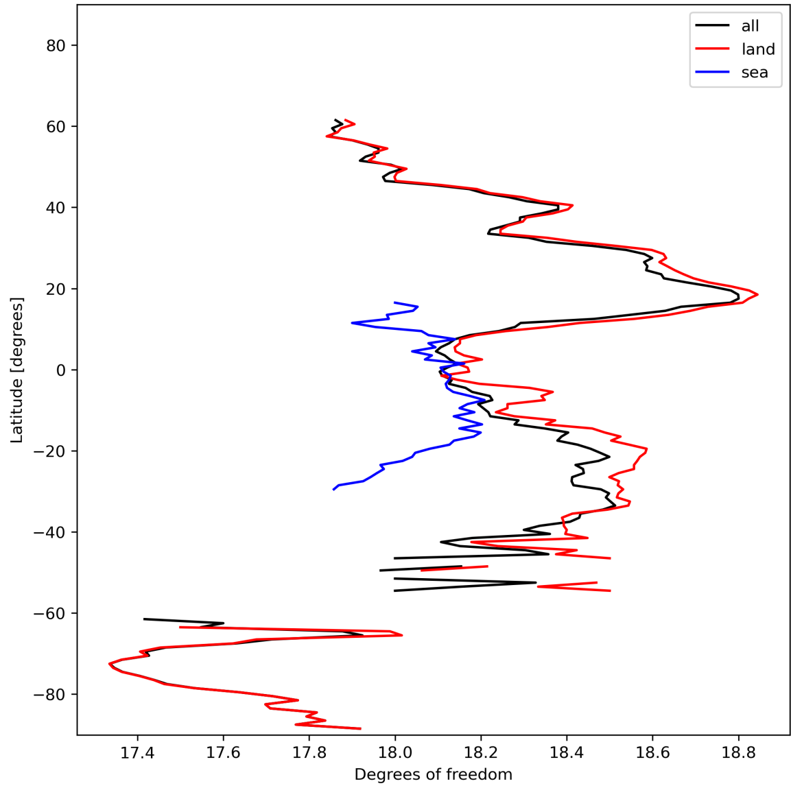
Figure 19: Zonal average of “Degrees of freedom” for 2023-10-28 to 2023-10-30.
