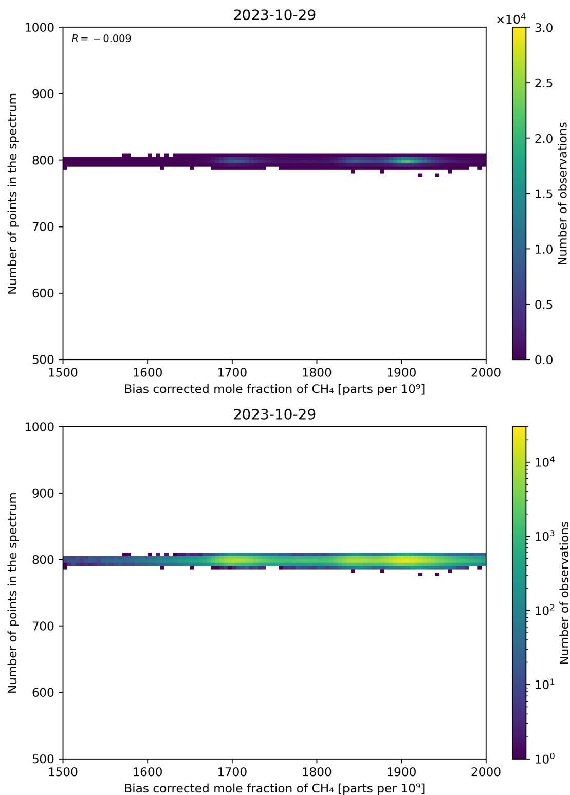
Figure 68: Scatter density plot of “Bias corrected mole fraction of CH 4 ” against “Number of points in the spectrum” for 2023-10-28 to 2023-10-30.
