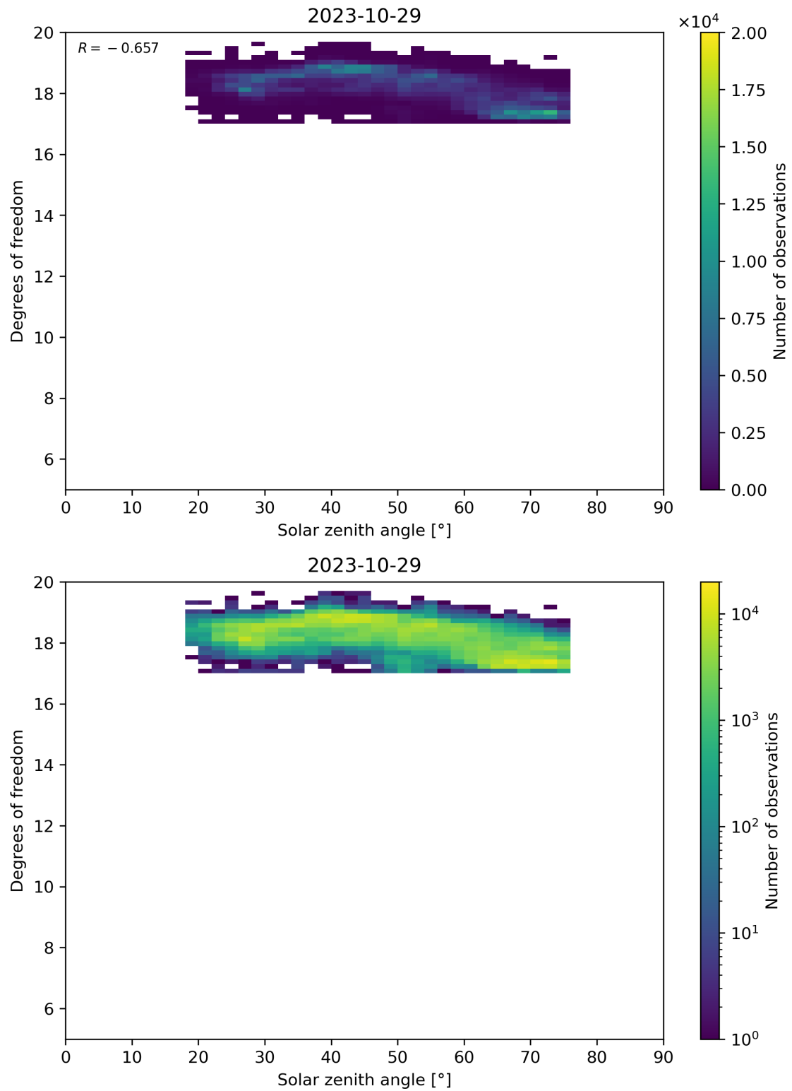
Figure 96: Scatter density plot of “Solar zenith angle” against “Degrees of freedom” for 2023-10-28 to 2023-10-30.
