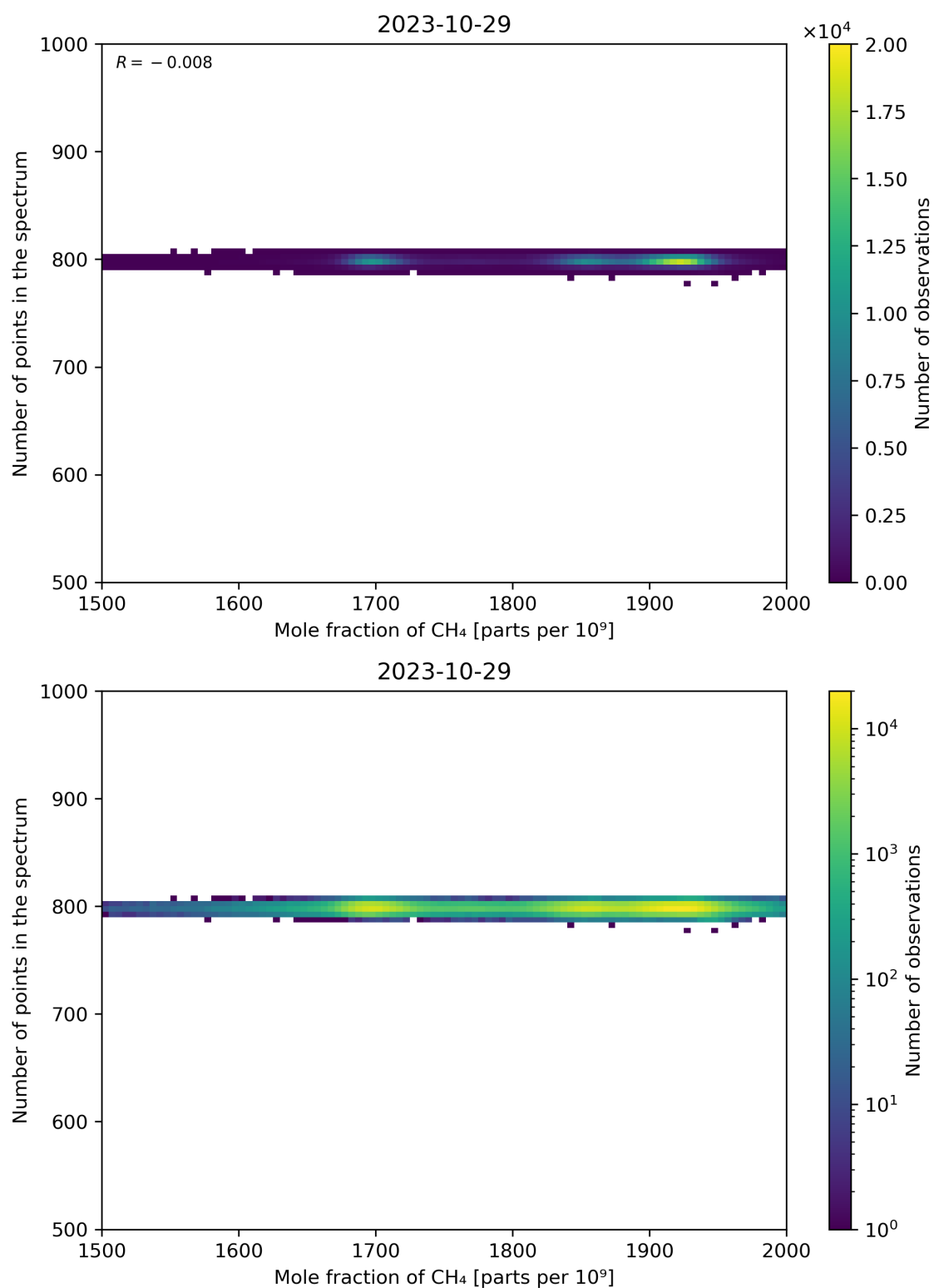
Figure 77: Scatter density plot of “Mole fraction of CH 4 ” against “Number of points in the spectrum” for 2023-10-28 to 2023-10-30.
