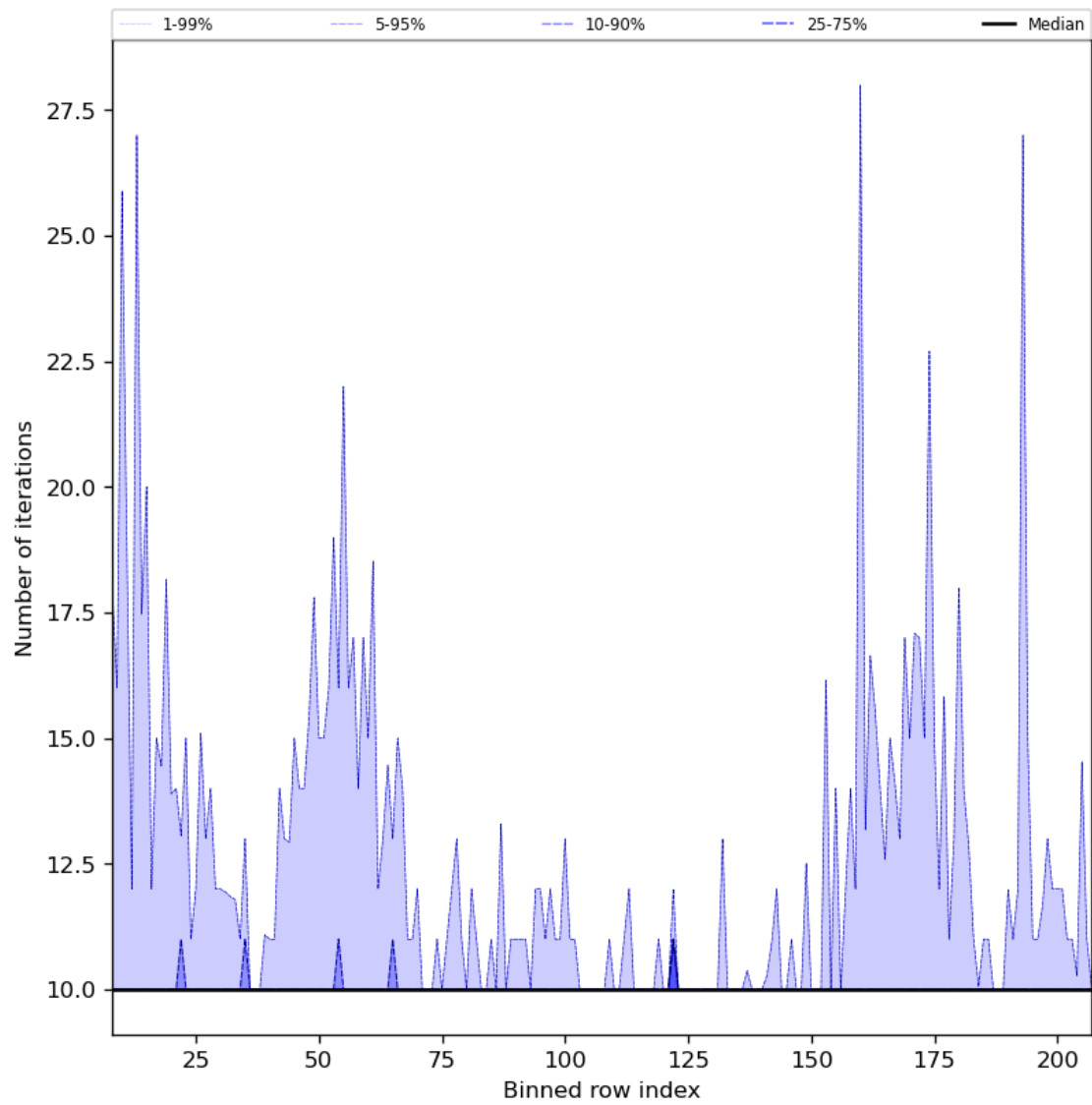
Figure 42: Along track statistics of “Number of iterations” for 2023-10-28 to 2023-10-30
