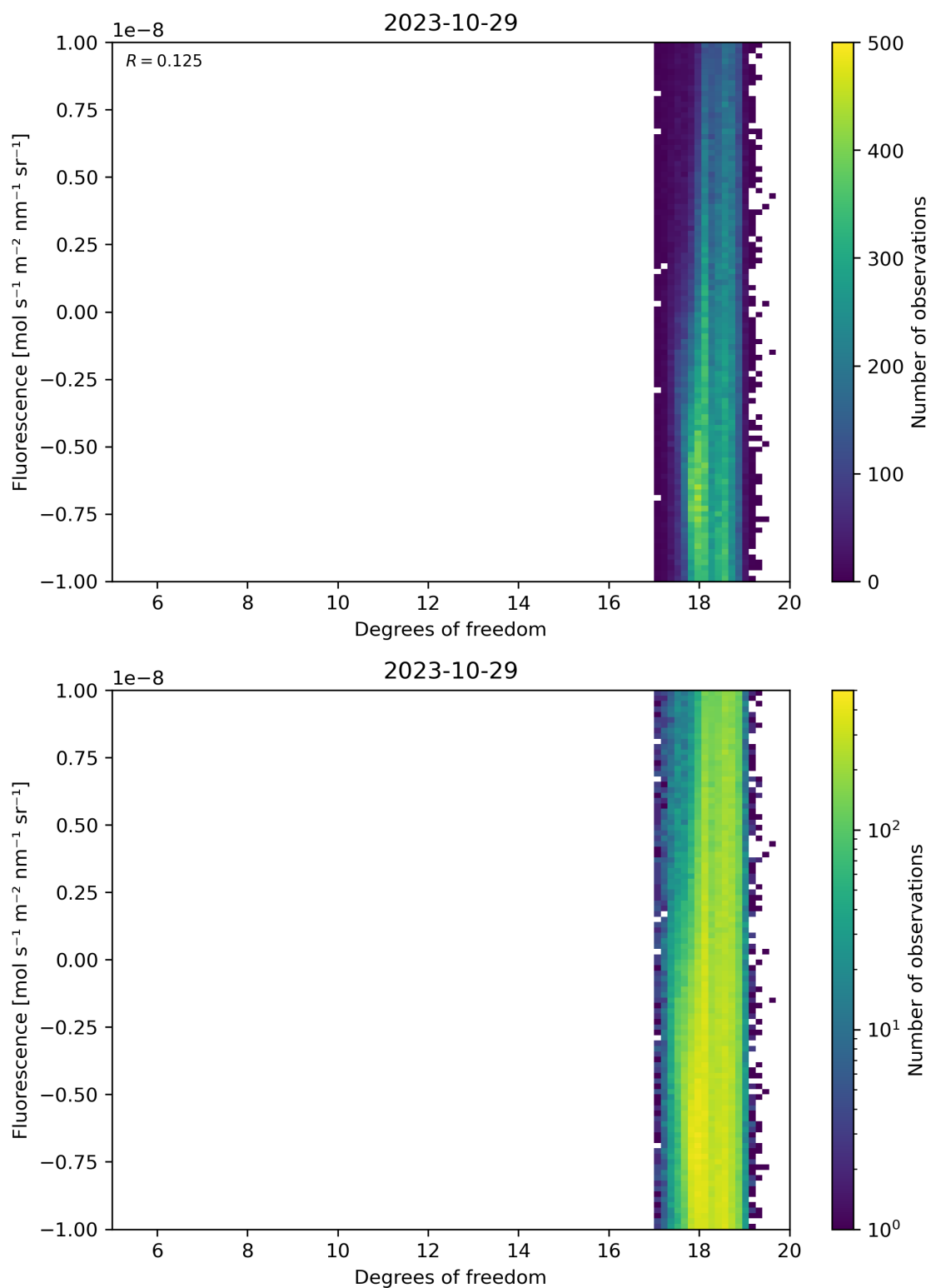
Figure 51: Scatter density plot of “Degrees of freedom” against “Fluorescence” for 2023-10-28 to 2023-10-30.
