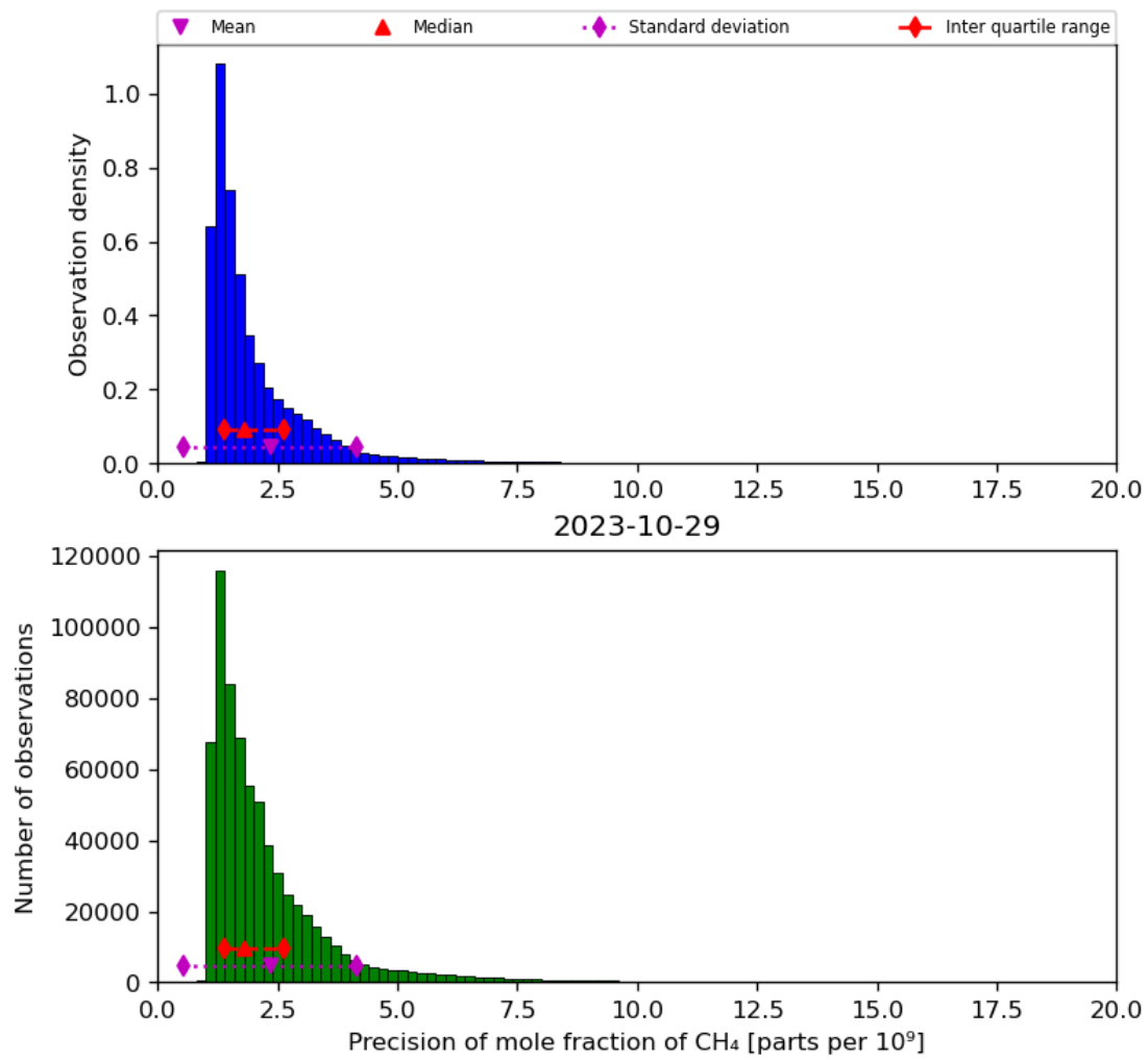
Figure 24: Histogram of “Precision of mole fraction of CH 4 ” for 2023-10-28 to 2023-10-30
