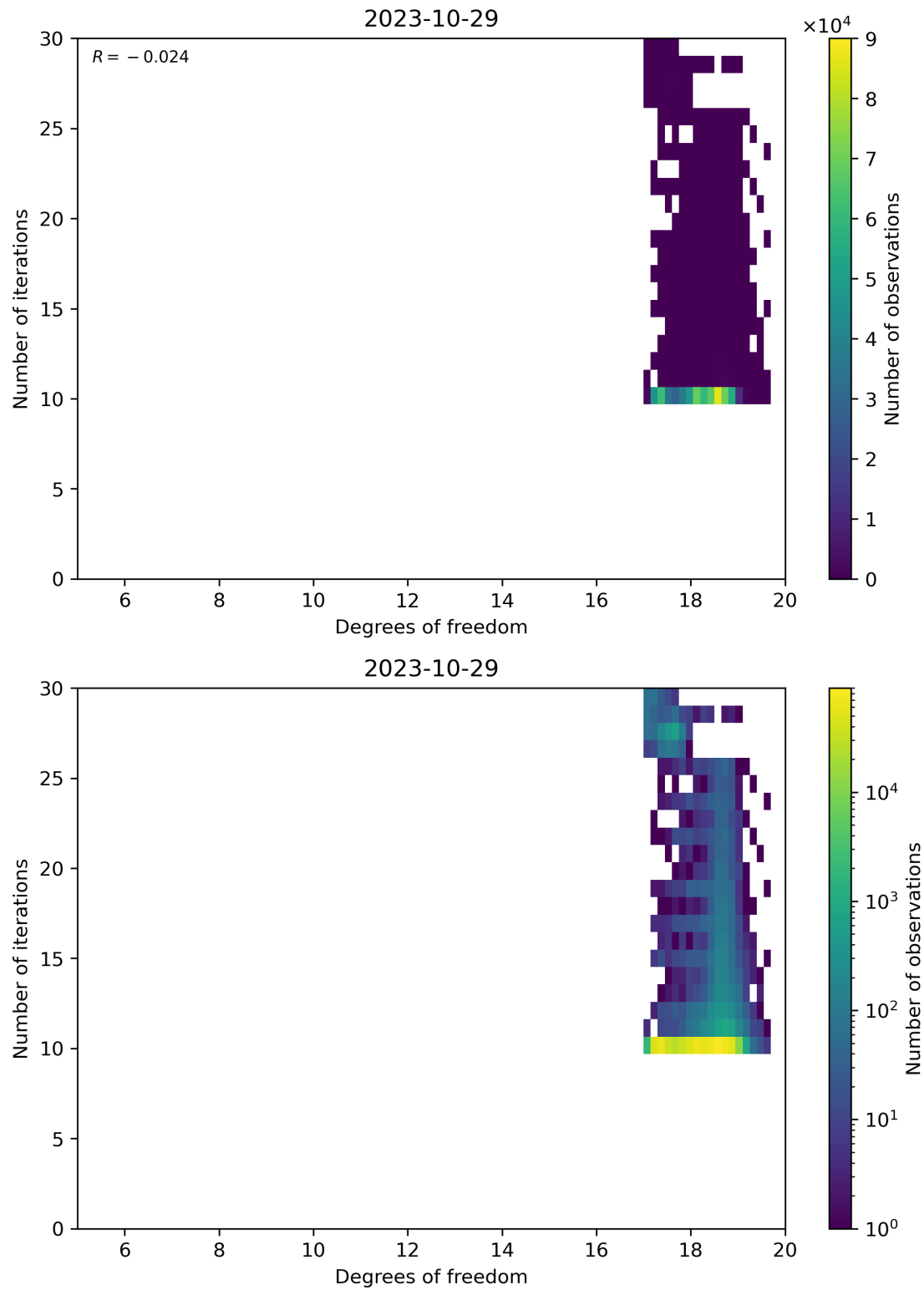
Figure 52: Scatter density plot of “Degrees of freedom” against “Number of iterations” for 2023-10-28 to 2023-10-30.
