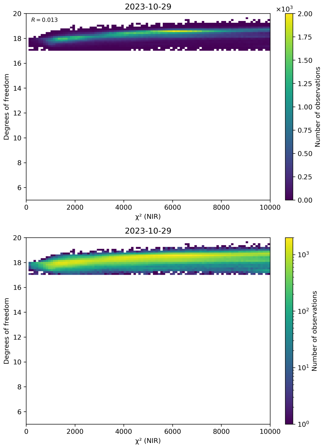
Figure 44: Scatter density plot of “ \chi^2 (NIR)” against “Degrees of freedom” for 2023-10-28 to 2023-10-30.
