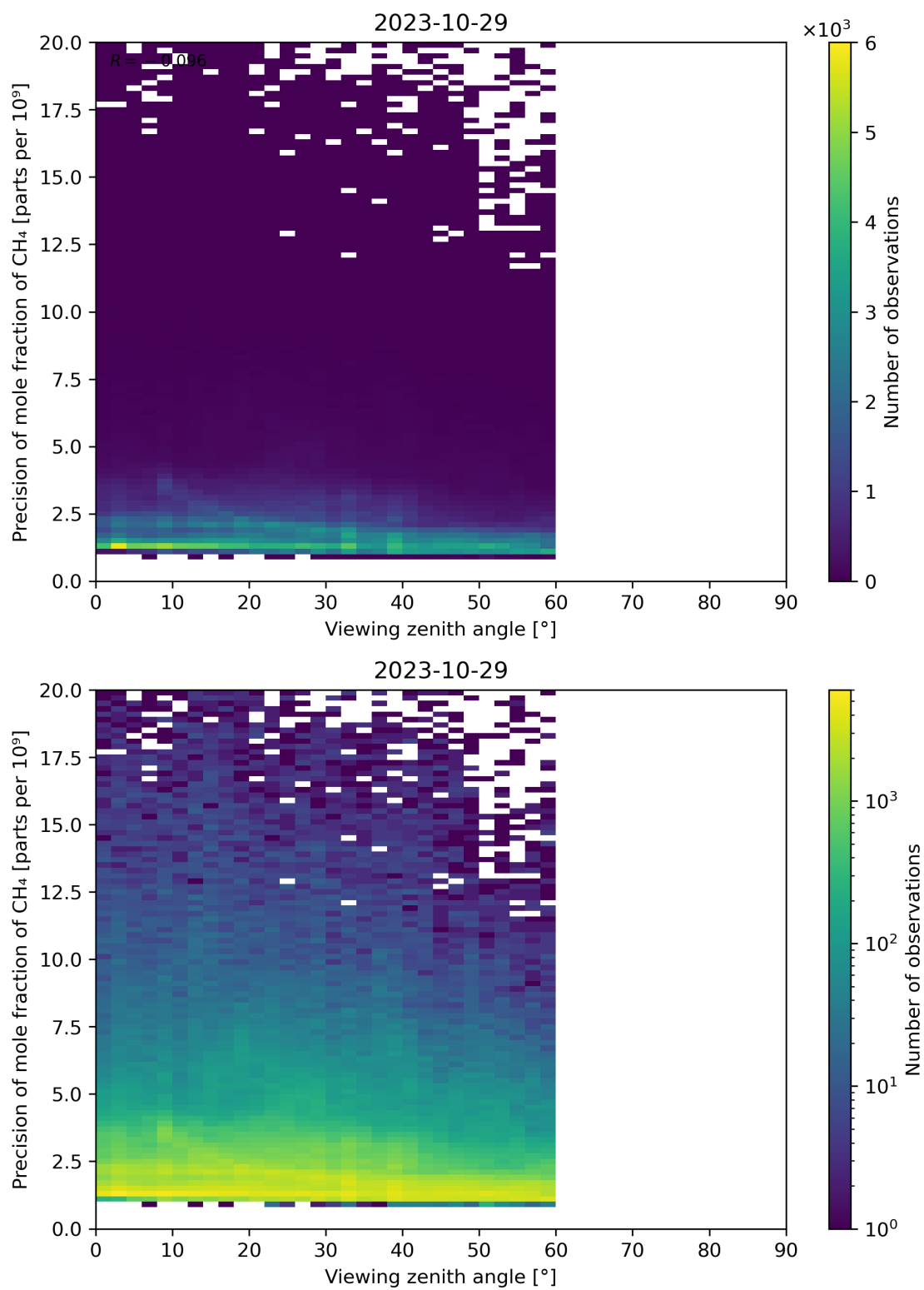
Figure 112: Scatter density plot of “Viewing zenith angle” against “Precision of mole fraction of CH 4 ” for 2023-10-28 to 2023-10-30.
