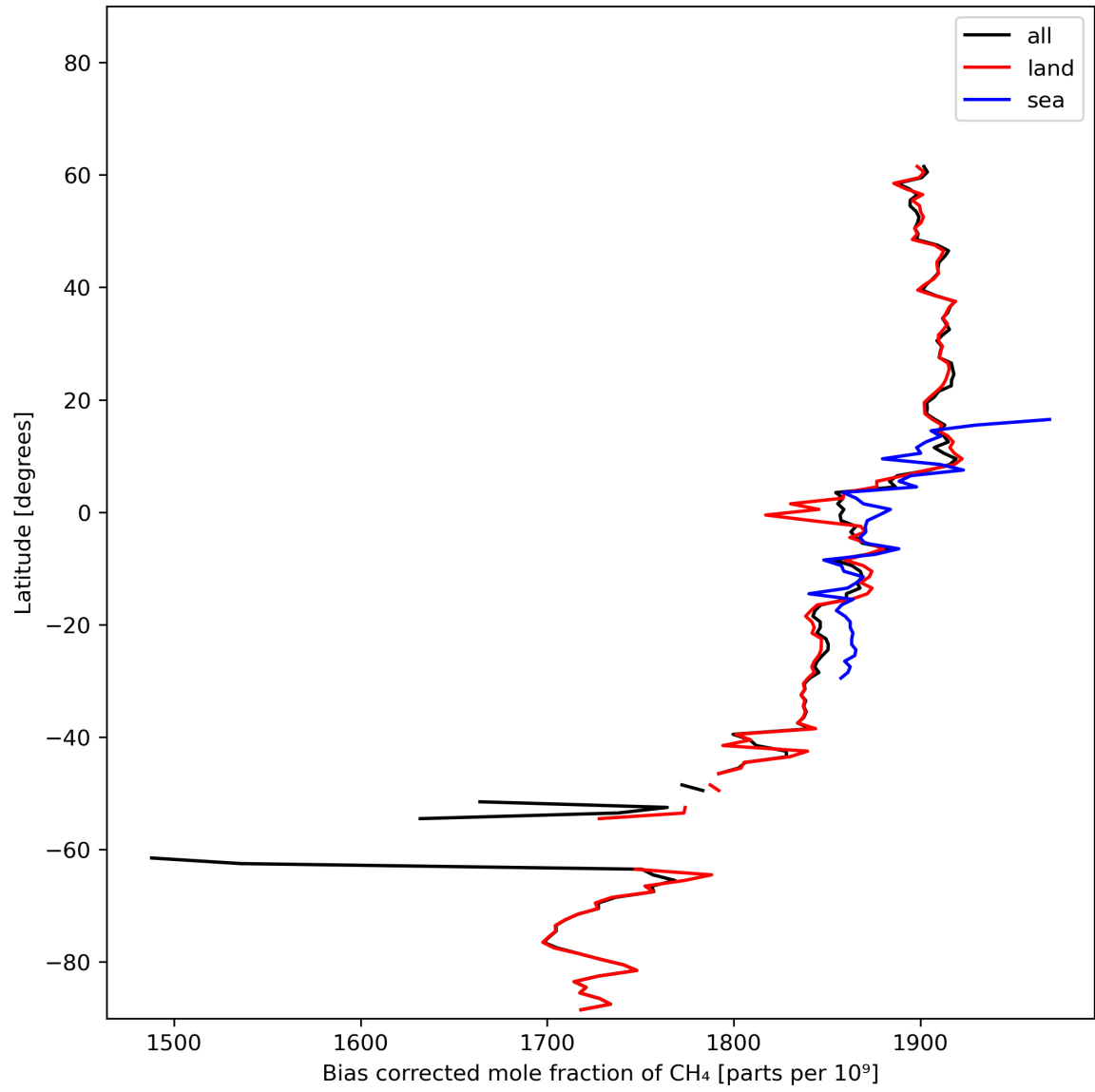
Figure 14: Zonal average of “Bias corrected mole fraction of CH 4 ” for 2023-10-28 to 2023-10-30.
