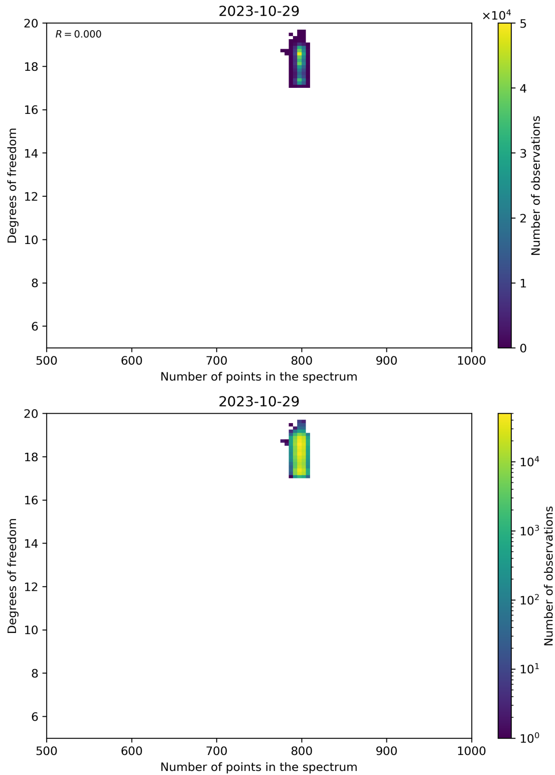
Figure 90: Scatter density plot of “Number of points in the spectrum” against “Degrees of freedom” for 2023-10-28 to 2023-10-30.
