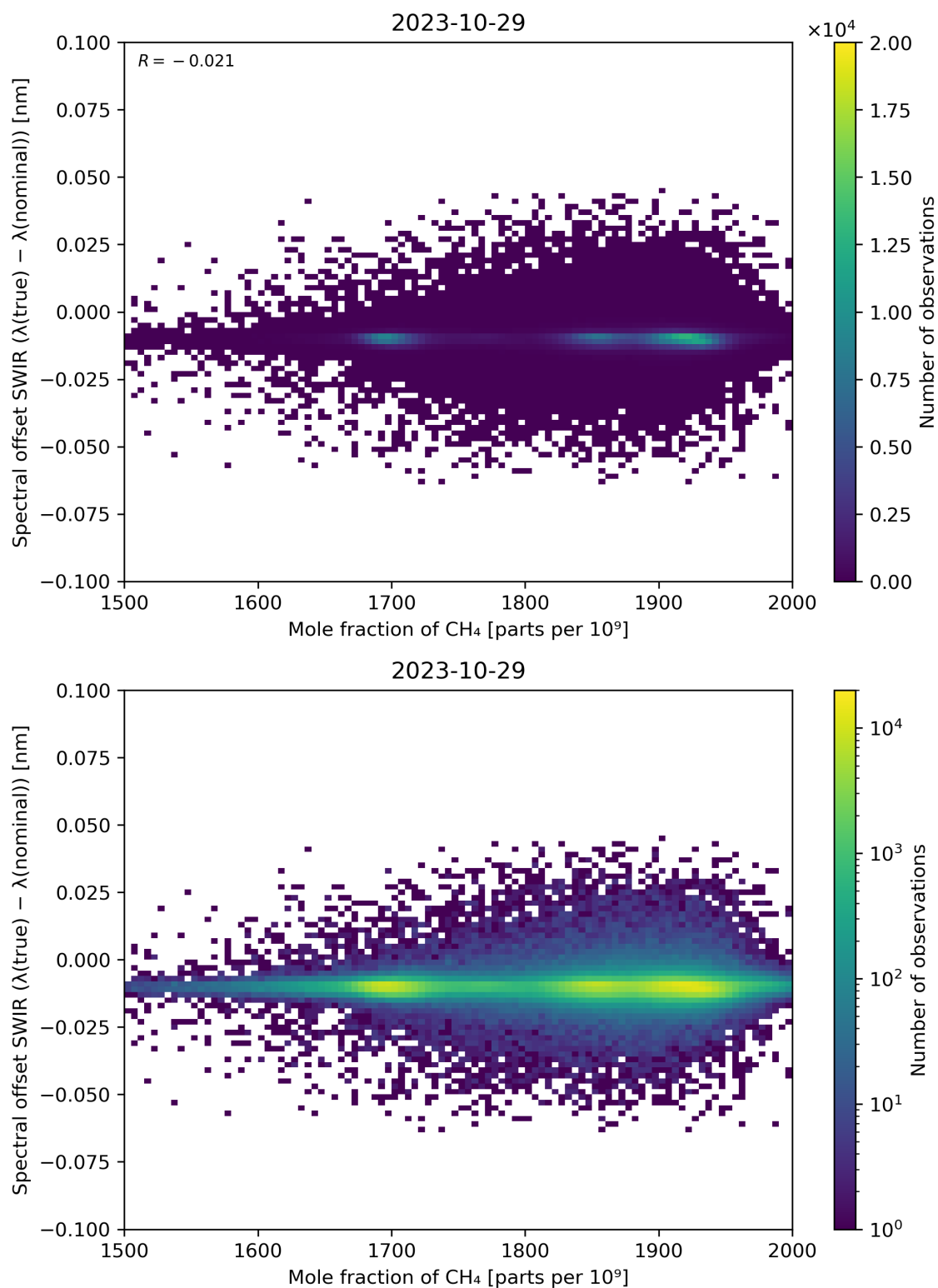
Figure 86: Scatter density plot of “Mole fraction of CH 4 ” against “Spectral offset SWIR ( \lambda(\text{true}) - \lambda(\text{nominal}) )” for 2023-10-28 to 2023-10-30.
