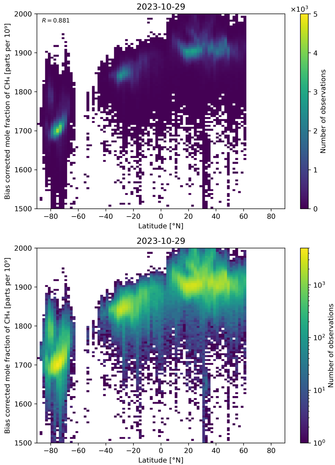
Figure 58: Scatter density plot of “Latitude” against “Bias corrected mole fraction of CH 4 ” for 2023-10-28 to 2023-10-30.
