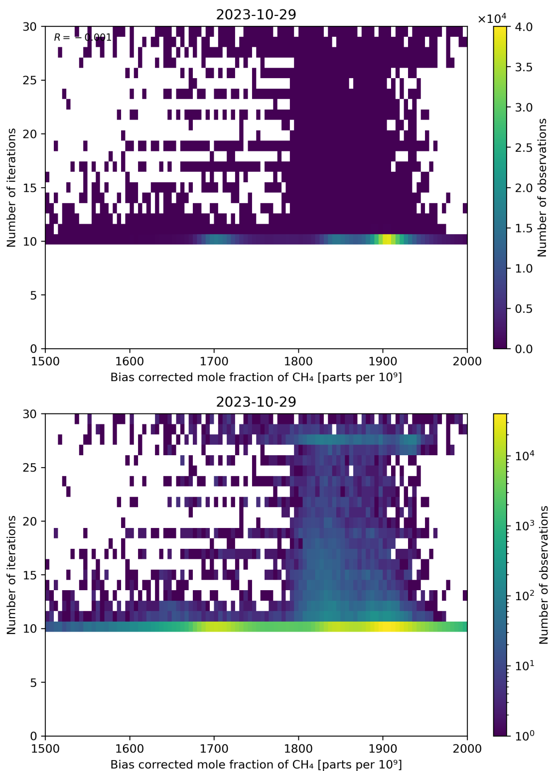
Figure 67: Scatter density plot of “Bias corrected mole fraction of \text{CH}_4 ” against “Number of iterations” for 2023-10-28 to 2023-10-30.
