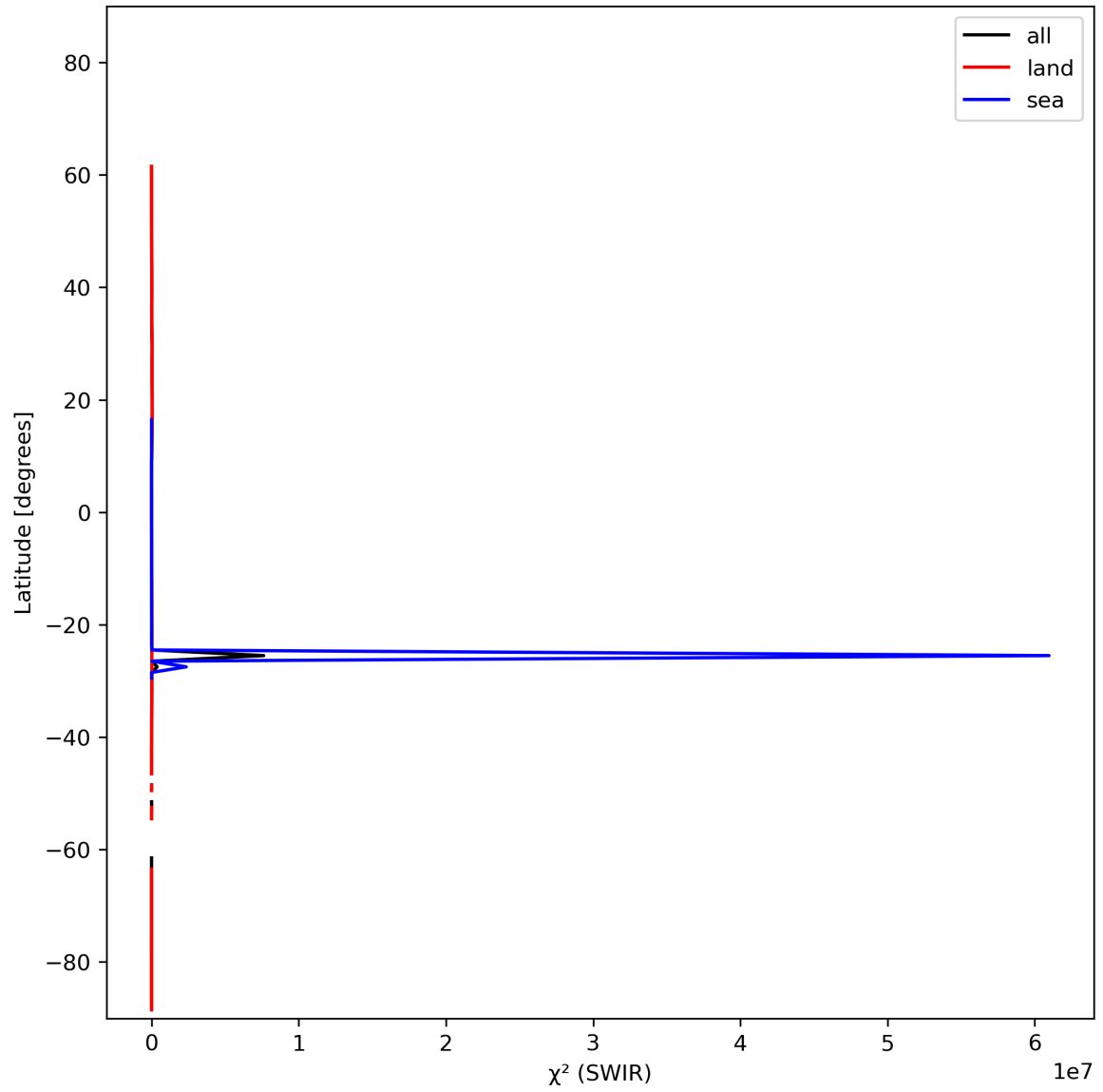
Figure 17: Zonal average of “ \chi^2 (SWIR)” for 2023-10-28 to 2023-10-30.
