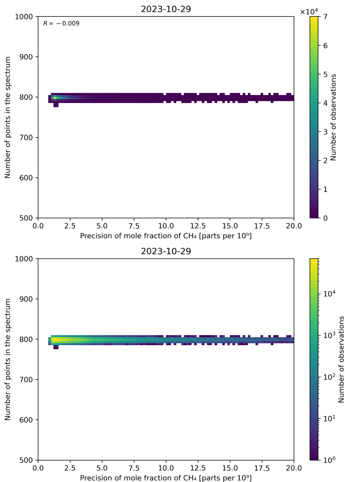
Figure 84: Scatter density plot of “Precision of mole fraction of CH 4 ” against “Number of points in the spectrum” for 2023-10-28 to 2023-10-30.
