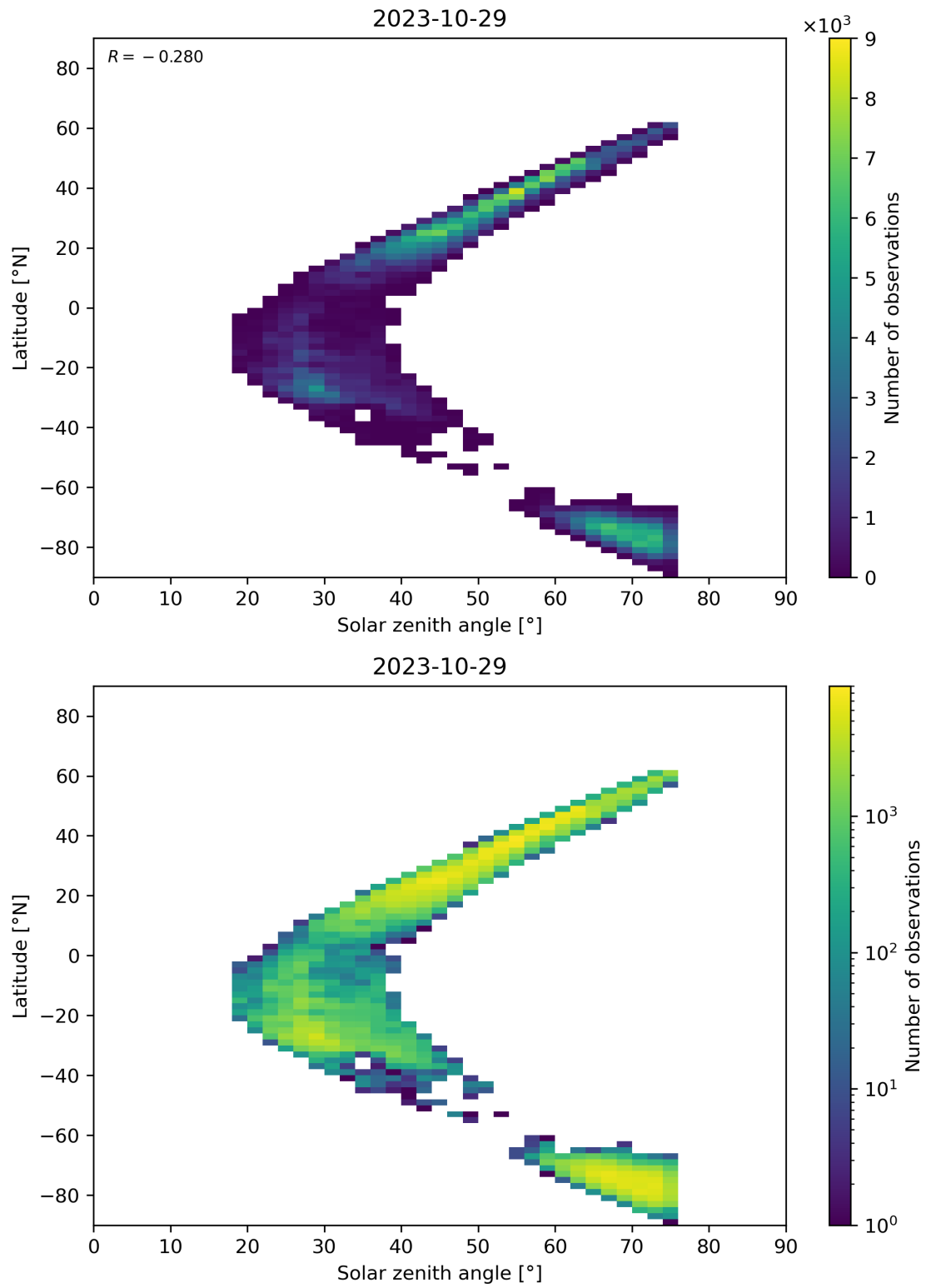
Figure 98: Scatter density plot of “Solar zenith angle” against “Latitude” for 2023-10-28 to 2023-10-30.
