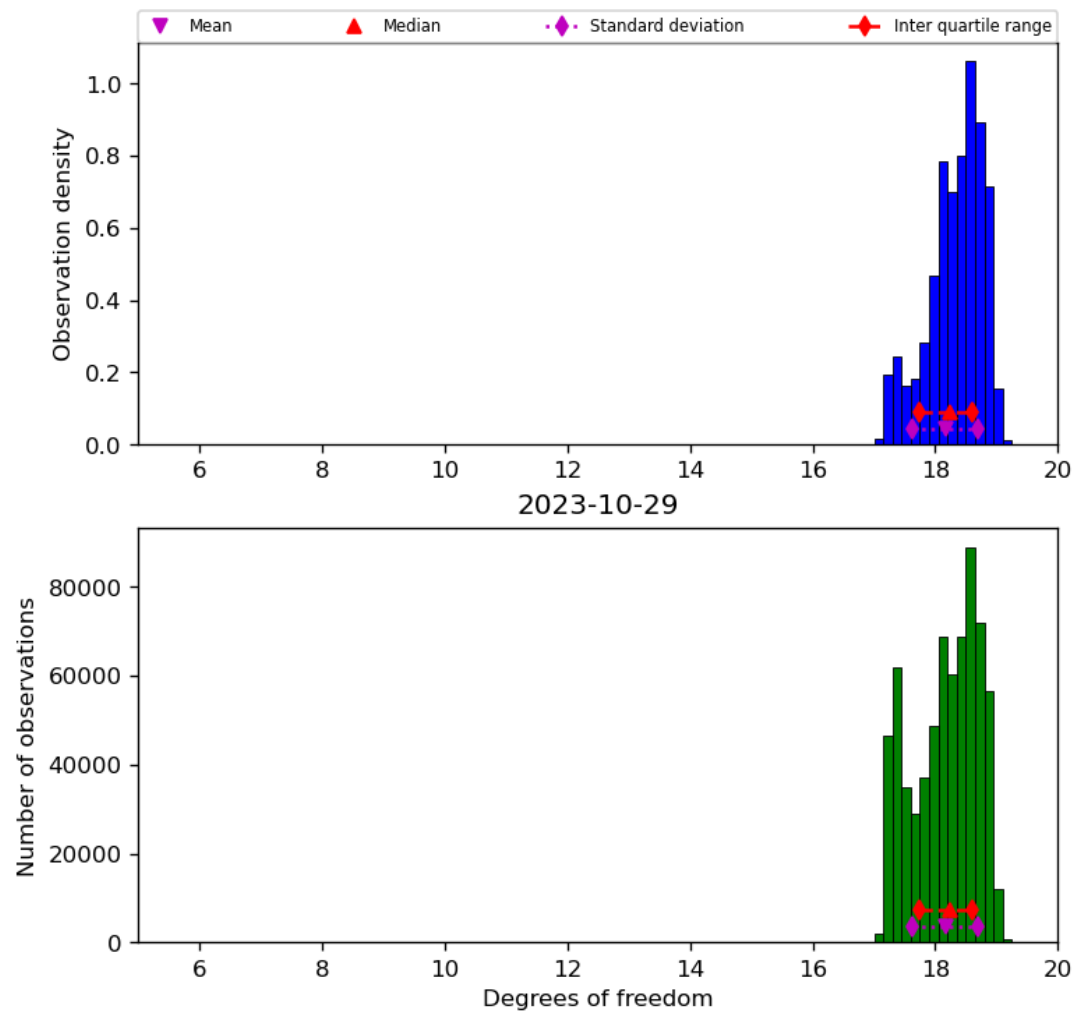
Figure 30: Histogram of “Degrees of freedom” for 2023-10-28 to 2023-10-30
