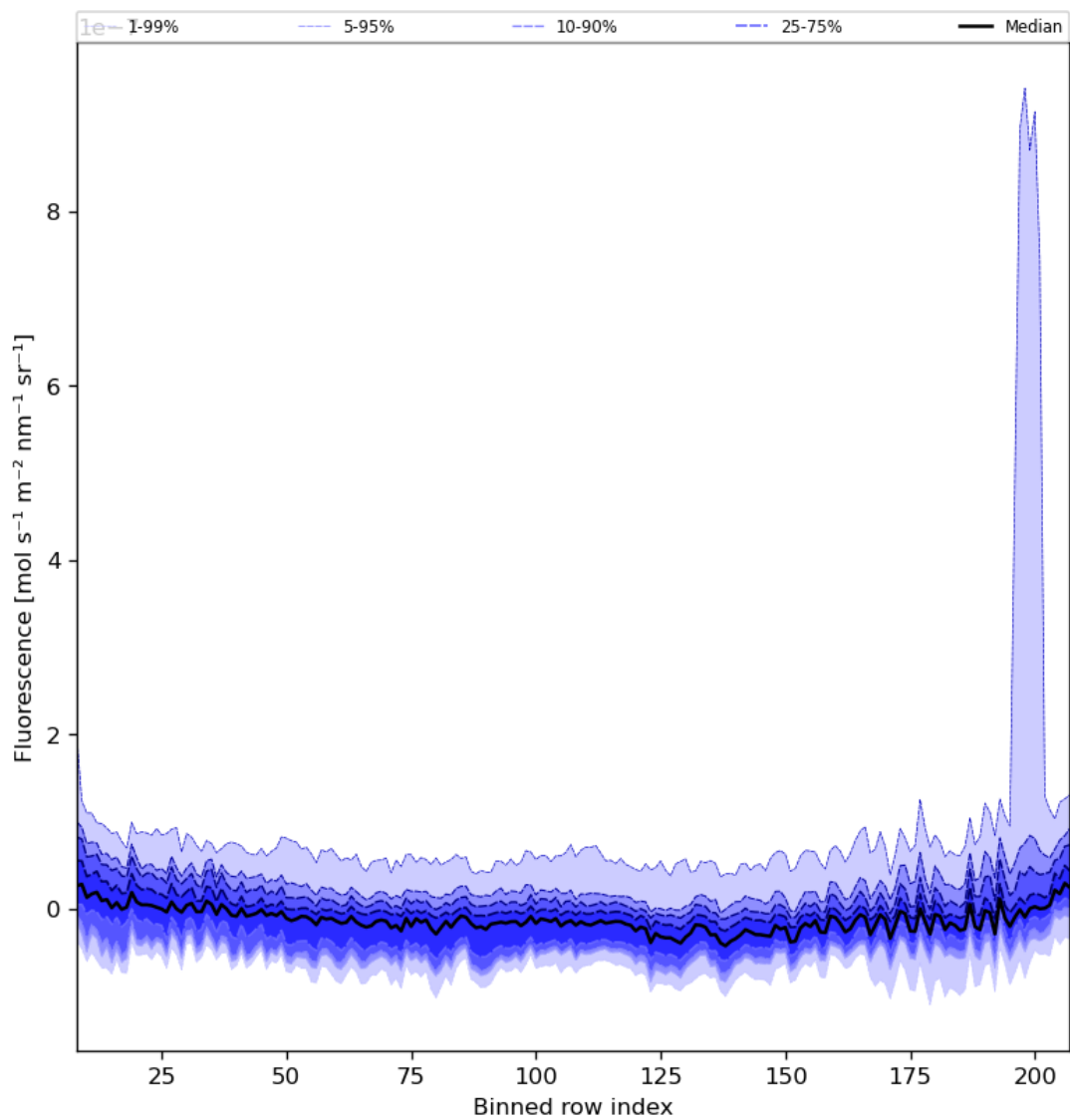
Figure 43: Along track statistics of “Fluorescence” for 2023-10-28 to 2023-10-30
