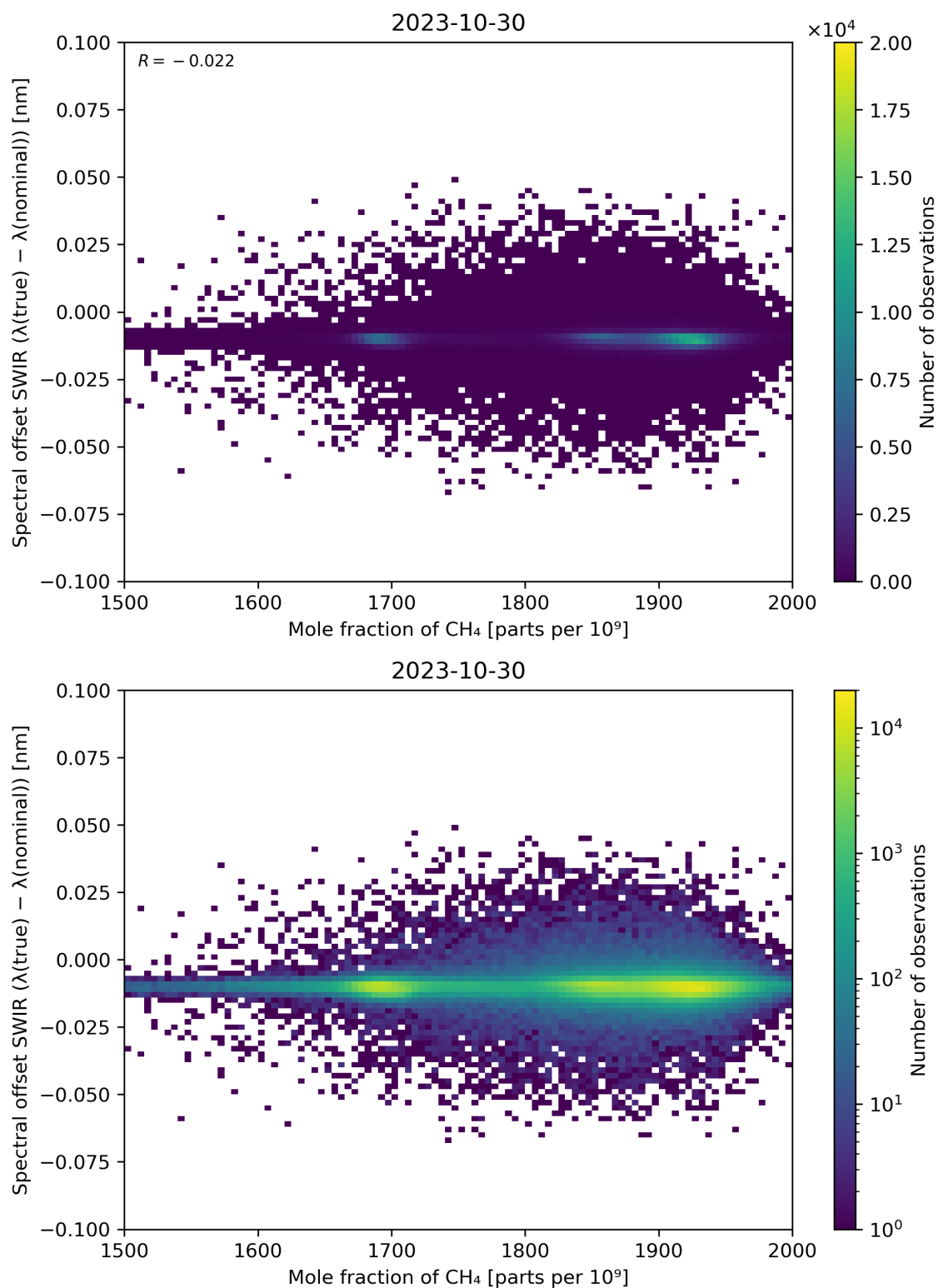
Figure 86: Scatter density plot of “Mole fraction of CH 4 ” against “Spectral offset SWIR ( \lambda(\text{true}) - \lambda(\text{nominal}) )” for 2023-10-29 to 2023-10-31.
