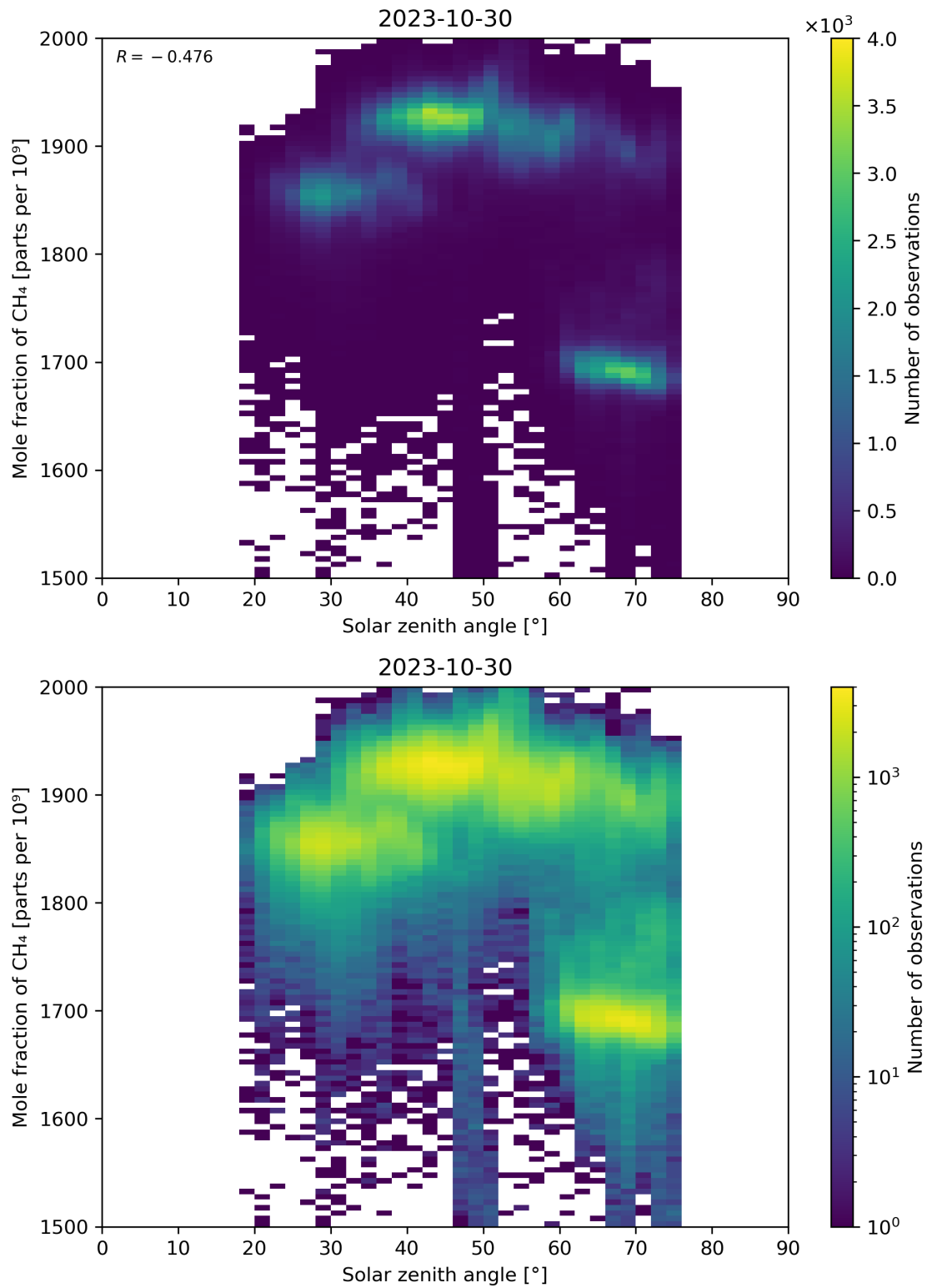
Figure 99: Scatter density plot of “Solar zenith angle” against “Mole fraction of CH 4 ” for 2023-10-29 to 2023-10-31.
