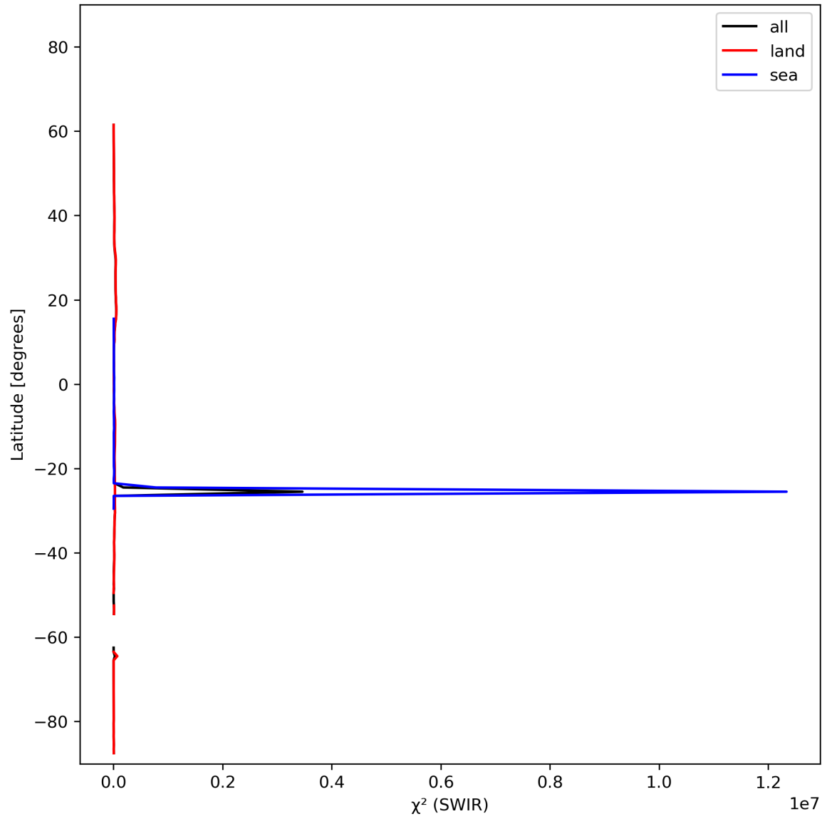
Figure 17: Zonal average of “ \chi^2 (SWIR)” for 2023-10-29 to 2023-10-31.
