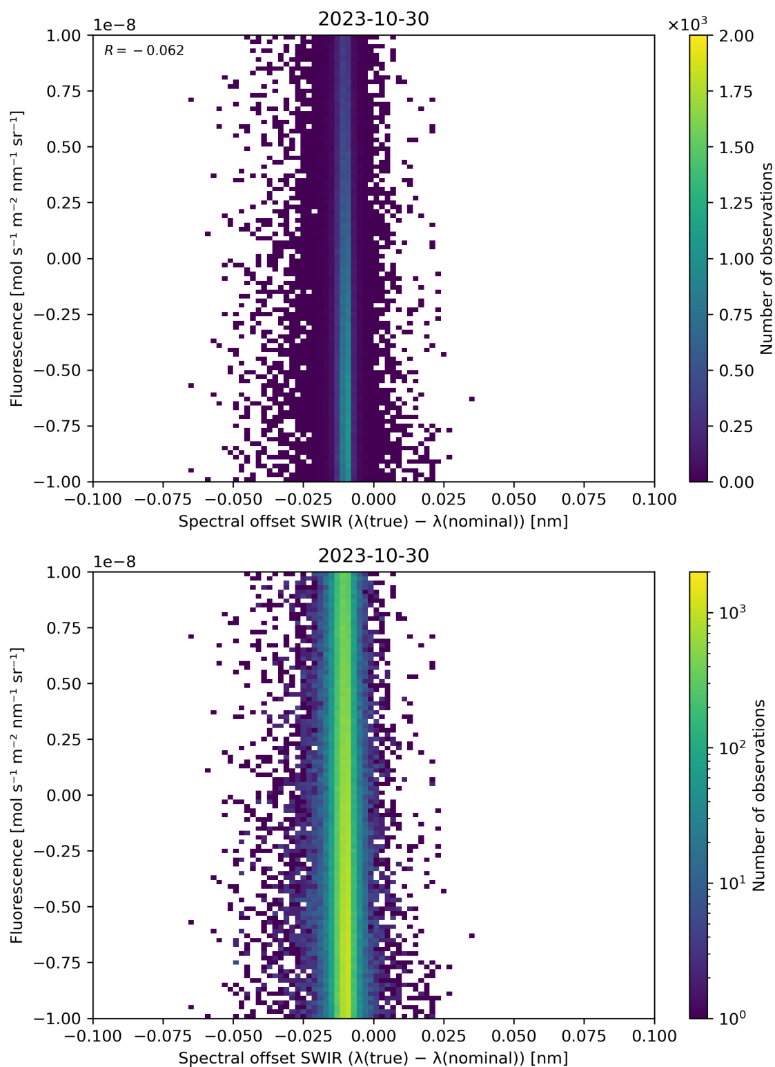
Figure 120: Scatter density plot of “Spectral offset SWIR ( \lambda(\text{true}) - \lambda(\text{nominal}) )” against “Fluorescence” for 2023-10-29 to 2023-10-31.
