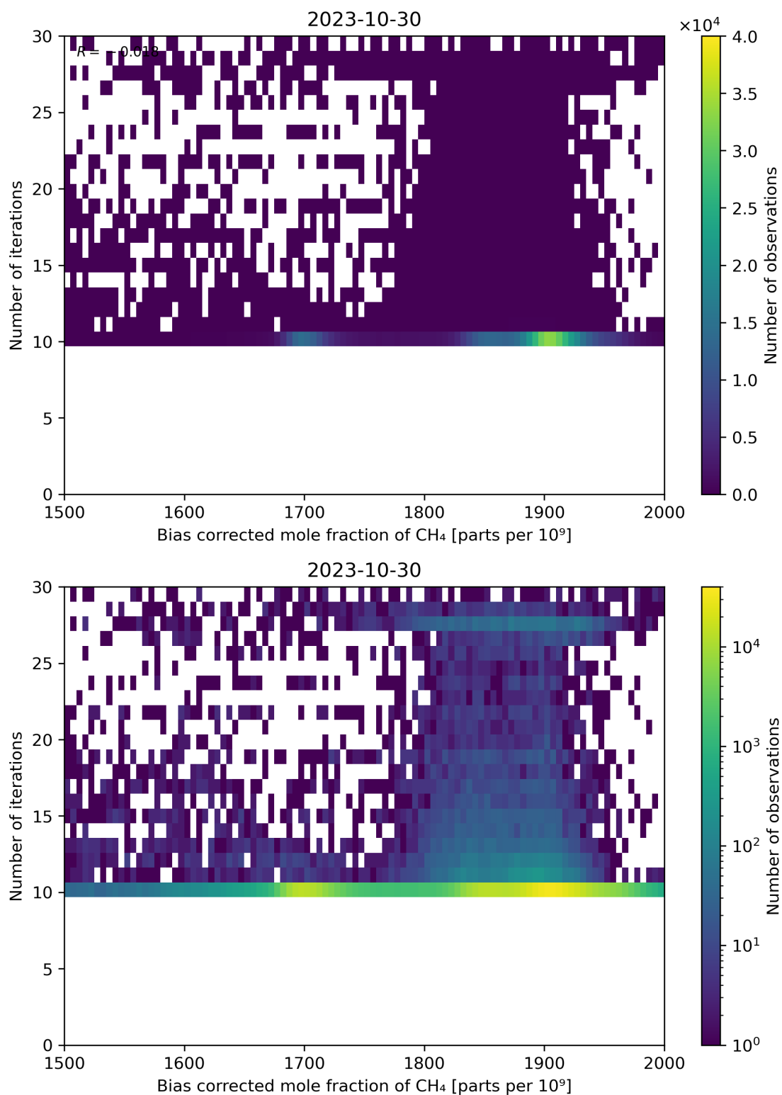
Figure 67: Scatter density plot of “Bias corrected mole fraction of \text{CH}_4 ” against “Number of iterations” for 2023-10-29 to 2023-10-31.
