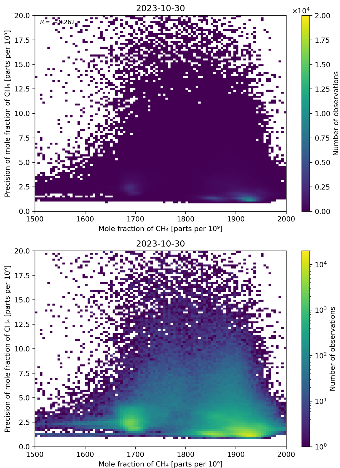
Figure 75: Scatter density plot of “Mole fraction of CH 4 ” against “Precision of mole fraction of CH 4 ” for 2023-10-29 to 2023-10-31.
