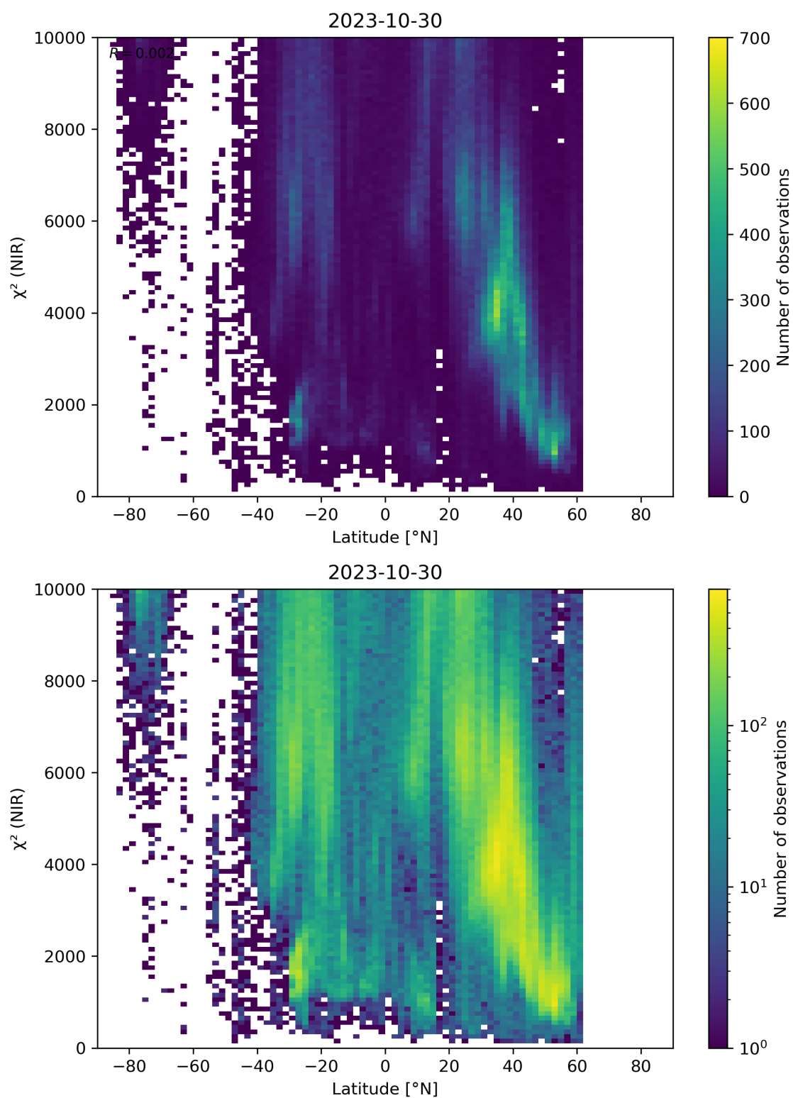
Figure 53: Scatter density plot of “Latitude” against “ \chi^2 (NIR)” for 2023-10-29 to 2023-10-31.
