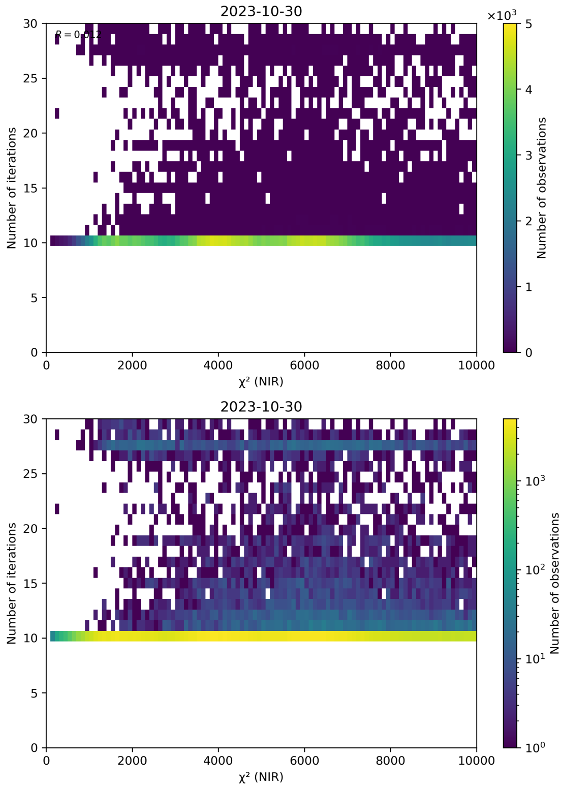
Figure 46: Scatter density plot of “ \chi^2 (NIR)” against “Number of iterations” for 2023-10-29 to 2023-10-31.
