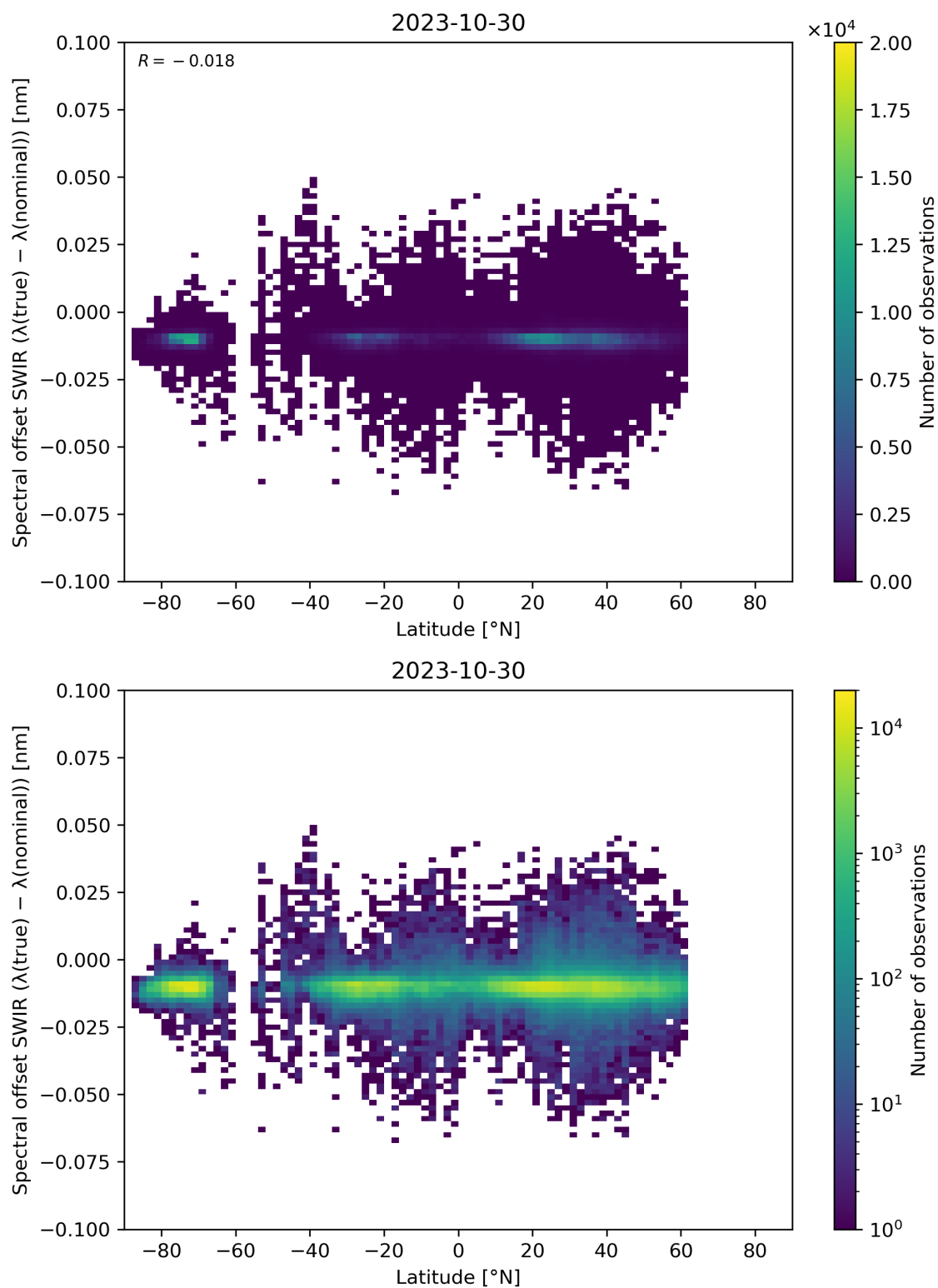
Figure 62: Scatter density plot of “Latitude” against “Spectral offset SWIR ( \lambda(\text{true}) - \lambda(\text{nominal}) )” for 2023-10-29 to 2023-10-31.
