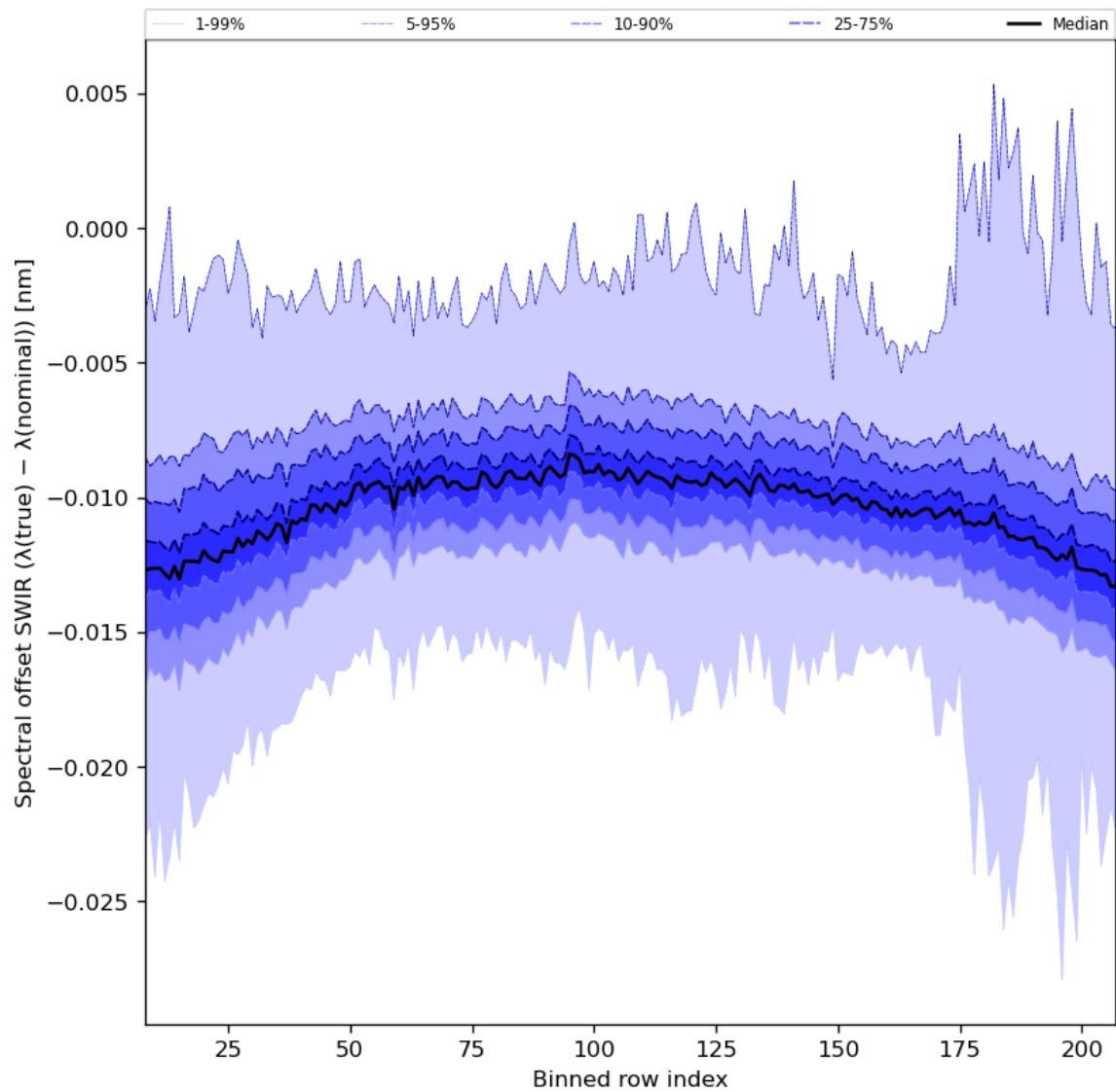
Figure 38: Along track statistics of “Spectral offset SWIR ( \lambda(\text{true}) - \lambda(\text{nominal}) )” for 2023-10-29 to 2023-10-31
