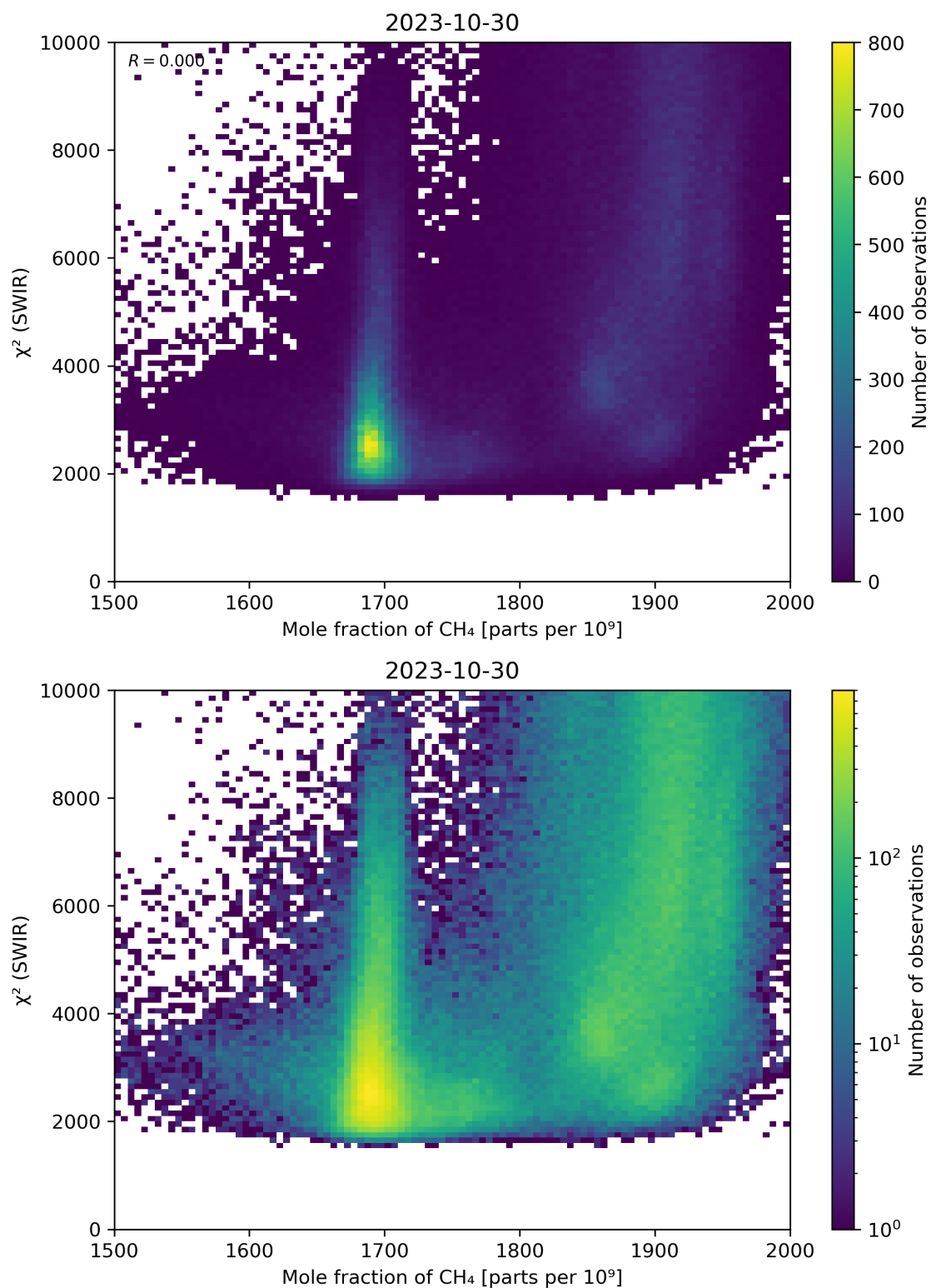
Figure 71: Scatter density plot of “Mole fraction of \text{CH}_4 ” against “ \chi^2 (SWIR)” for 2023-10-29 to 2023-10-31.
