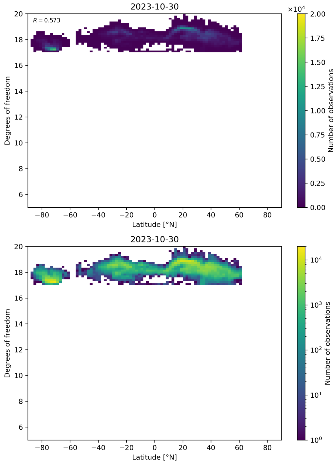
Figure 55: Scatter density plot of “Latitude” against “Degrees of freedom” for 2023-10-29 to 2023-10-31.
