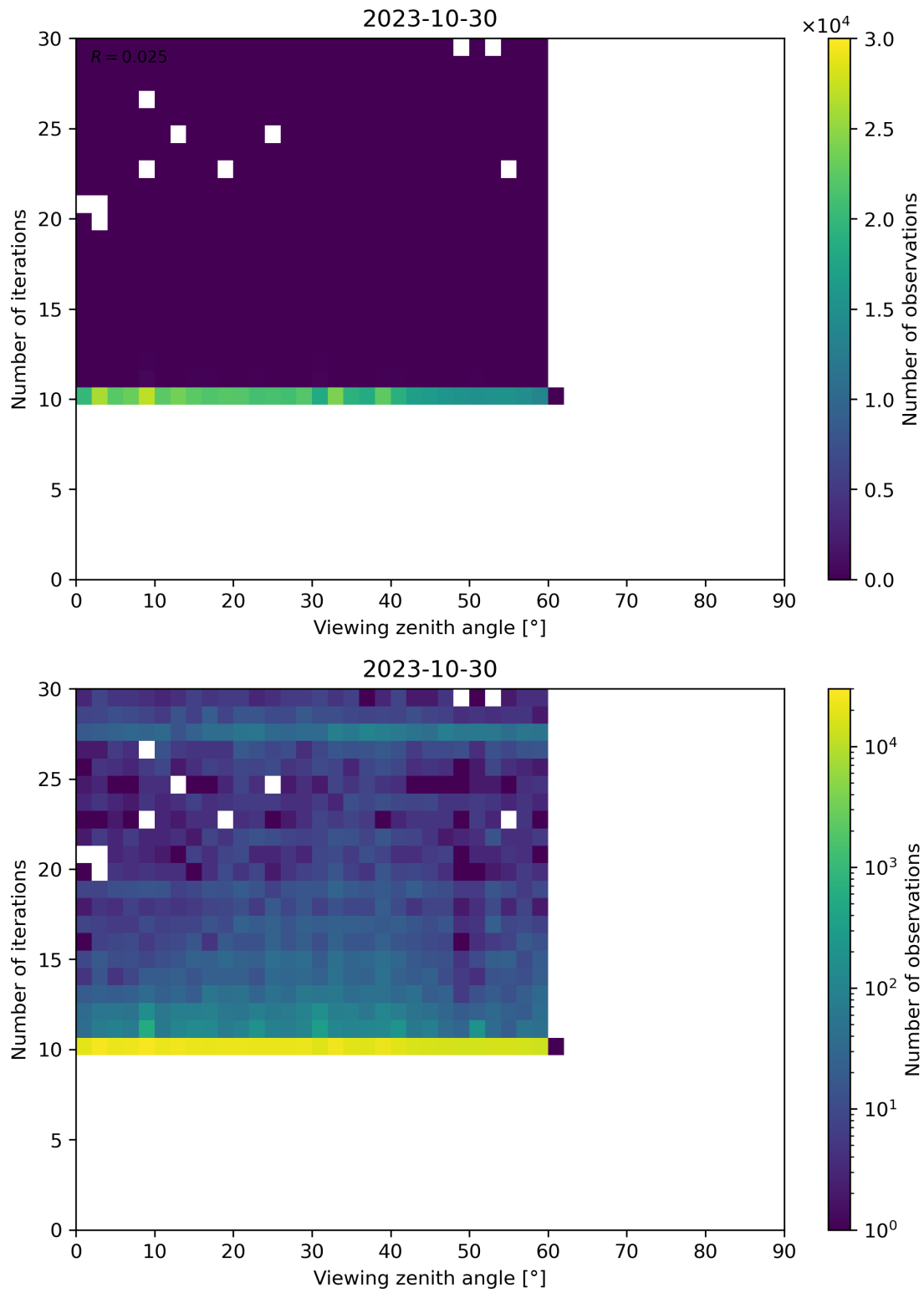
Figure 113: Scatter density plot of “Viewing zenith angle” against “Number of iterations” for 2023-10-29 to 2023-10-31.
