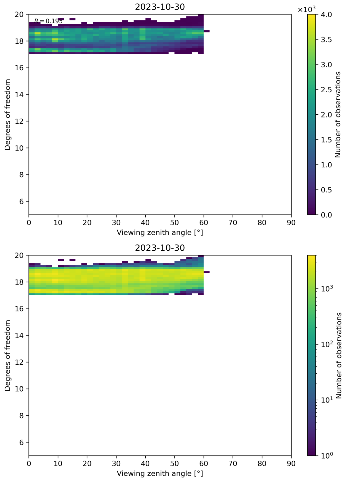
Figure 107: Scatter density plot of “Viewing zenith angle” against “Degrees of freedom” for 2023-10-29 to 2023-10-31.
