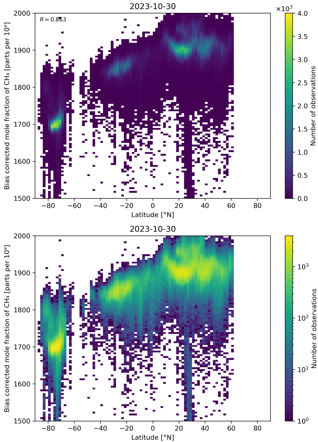
Figure 58: Scatter density plot of “Latitude” against “Bias corrected mole fraction of CH 4 ” for 2023-10-29 to 2023-10-31.
