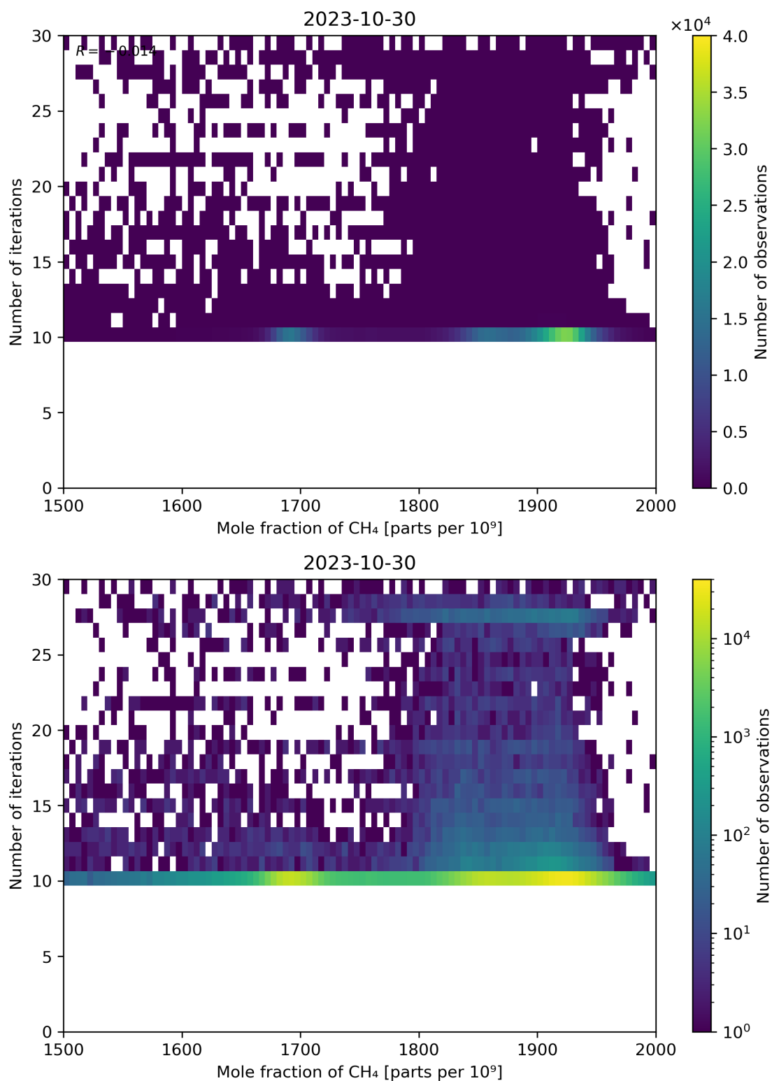
Figure 76: Scatter density plot of “Mole fraction of CH 4 ” against “Number of iterations” for 2023-10-29 to 2023-10-31.
