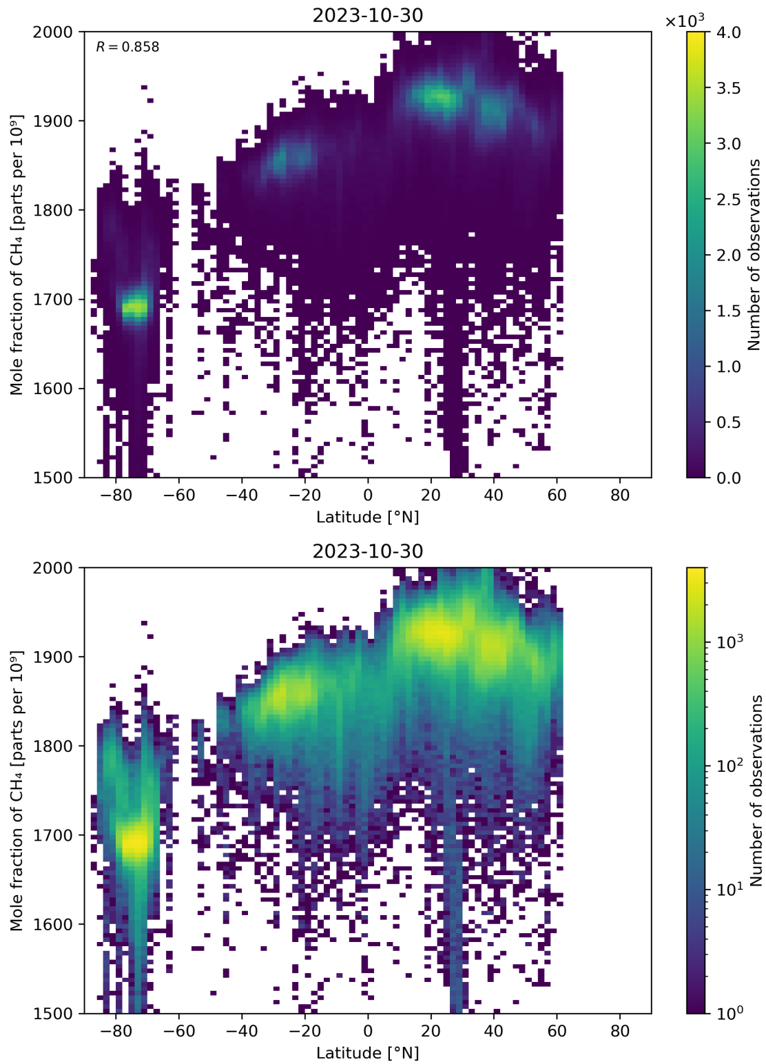
Figure 57: Scatter density plot of “Latitude” against “Mole fraction of CH 4 ” for 2023-10-29 to 2023-10-31.
