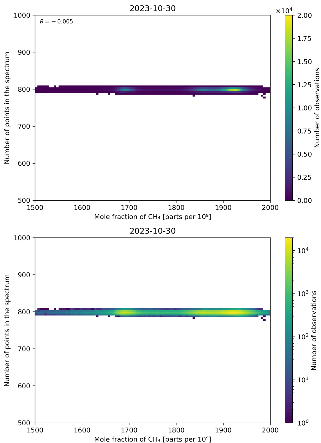
Figure 77: Scatter density plot of “Mole fraction of CH 4 ” against “Number of points in the spectrum” for 2023-10-29 to 2023-10-31.
