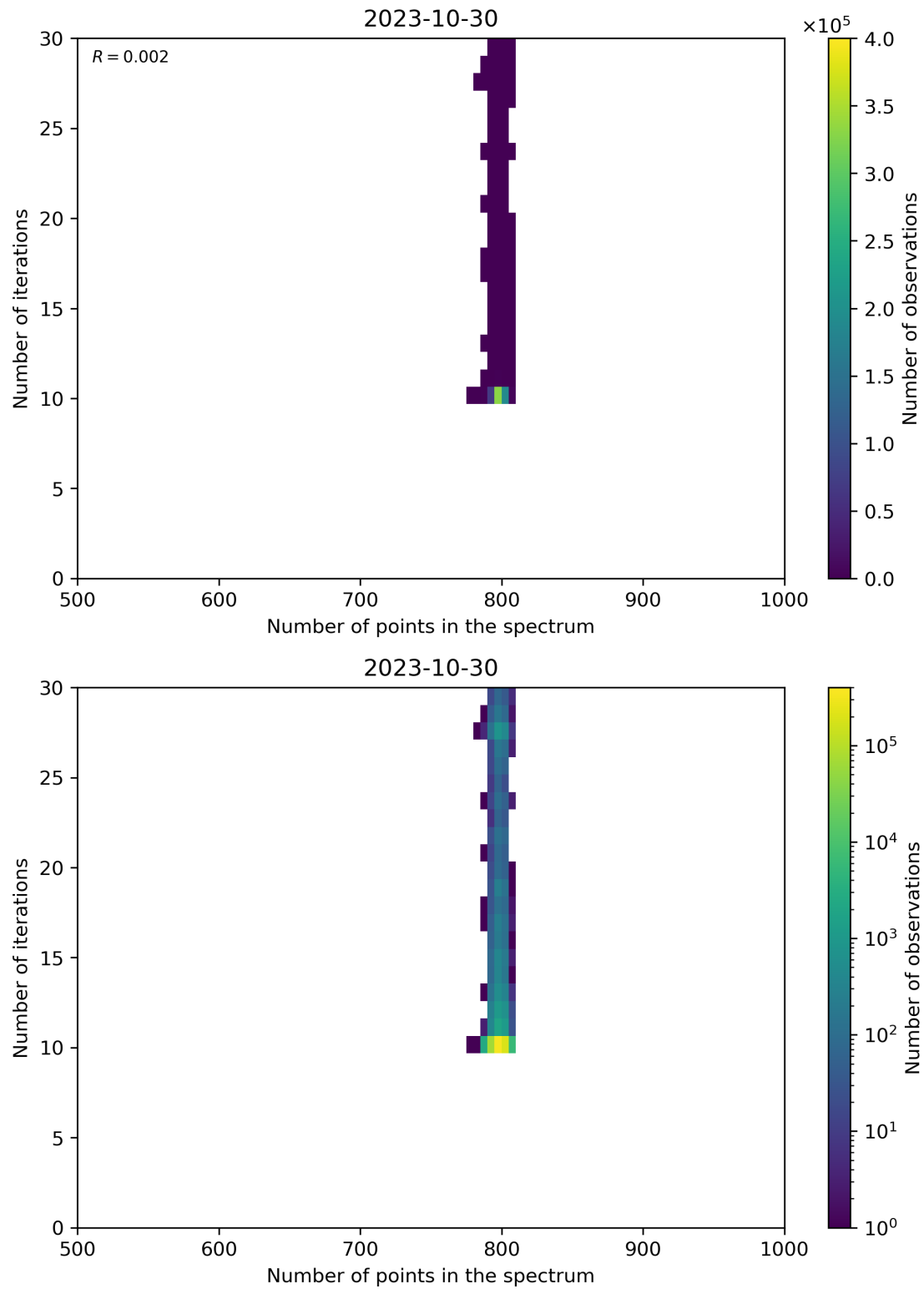
Figure 92: Scatter density plot of “Number of points in the spectrum” against “Number of iterations” for 2023-10-29 to 2023-10-31.
