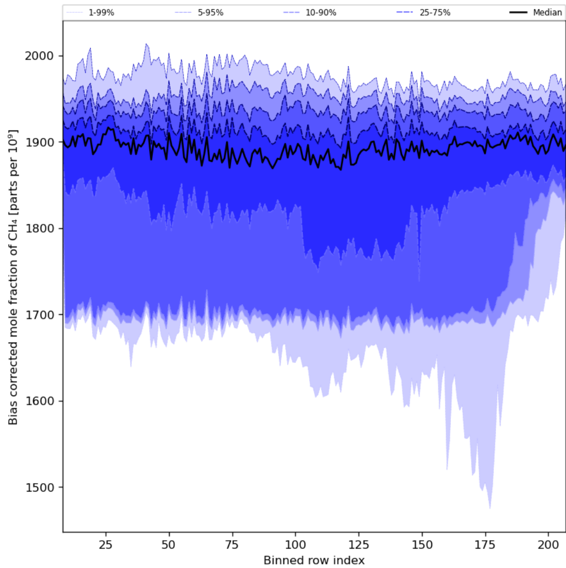
Figure 36: Along track statistics of “Bias corrected mole fraction of CH 4 ” for 2023-10-29 to 2023-10-31
