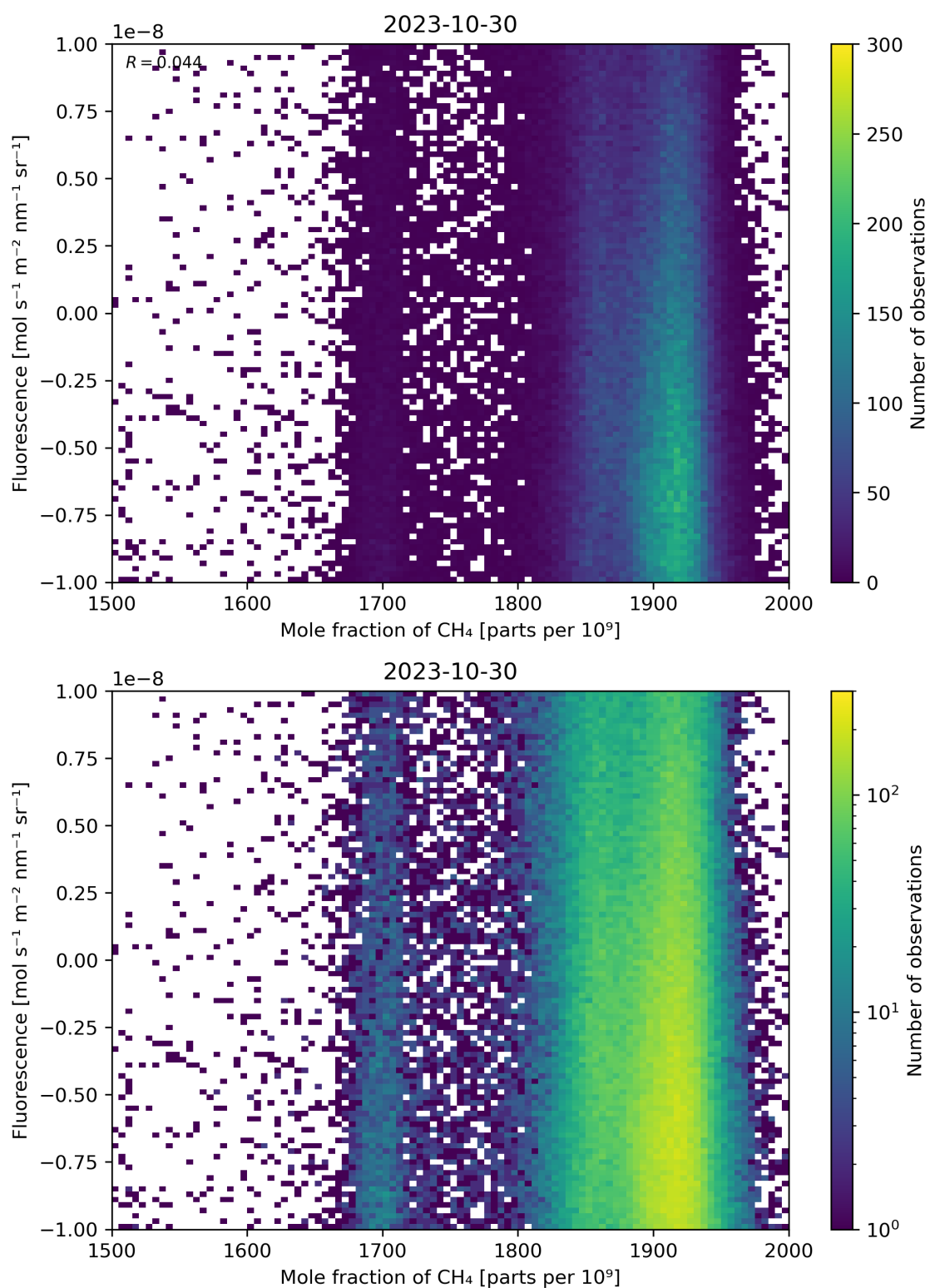
Figure 73: Scatter density plot of “Mole fraction of \text{CH}_4 ” against “Fluorescence” for 2023-10-29 to 2023-10-31.
