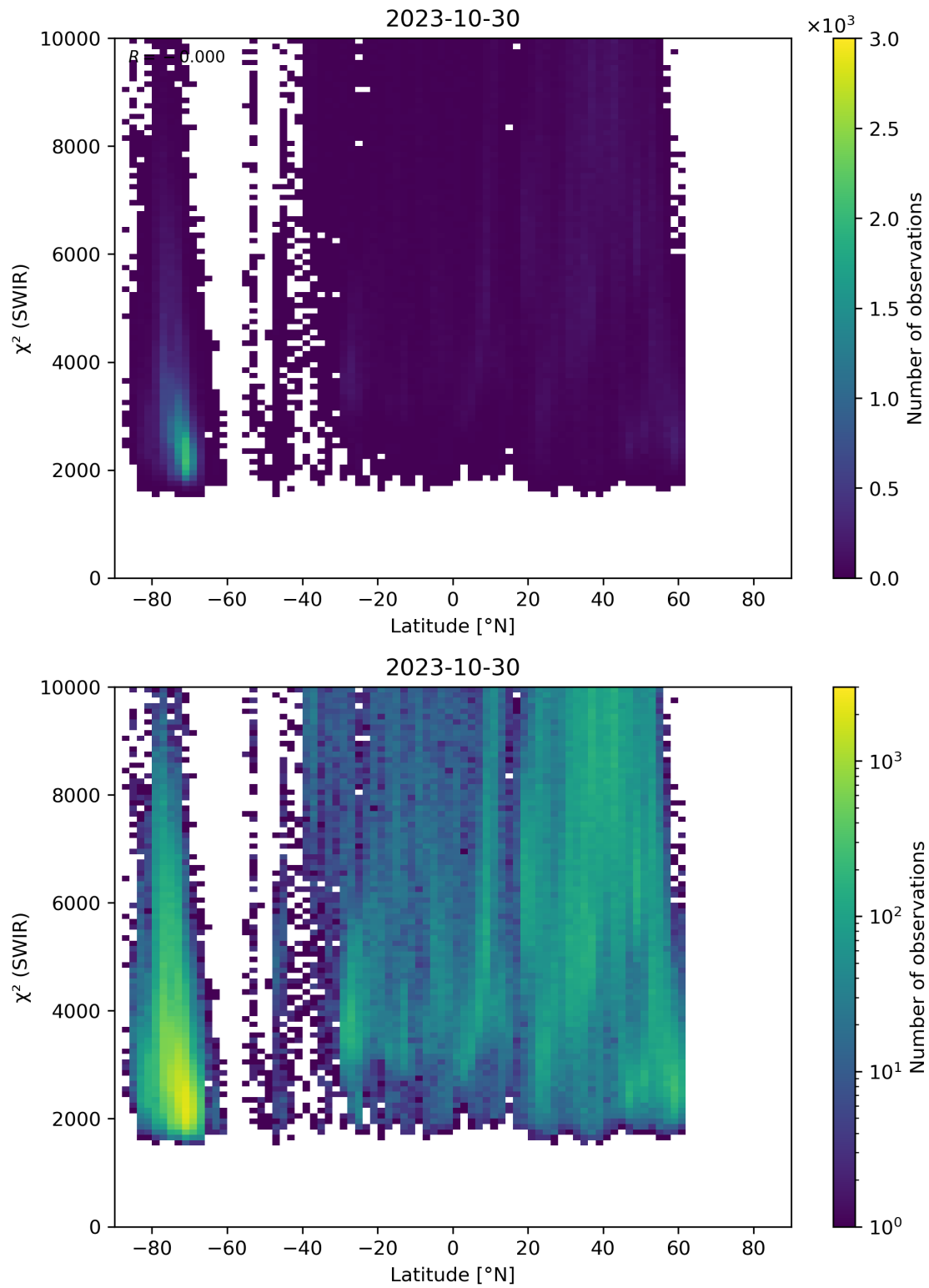
Figure 54: Scatter density plot of “Latitude” against “ \chi^2 (SWIR)” for 2023-10-29 to 2023-10-31.
