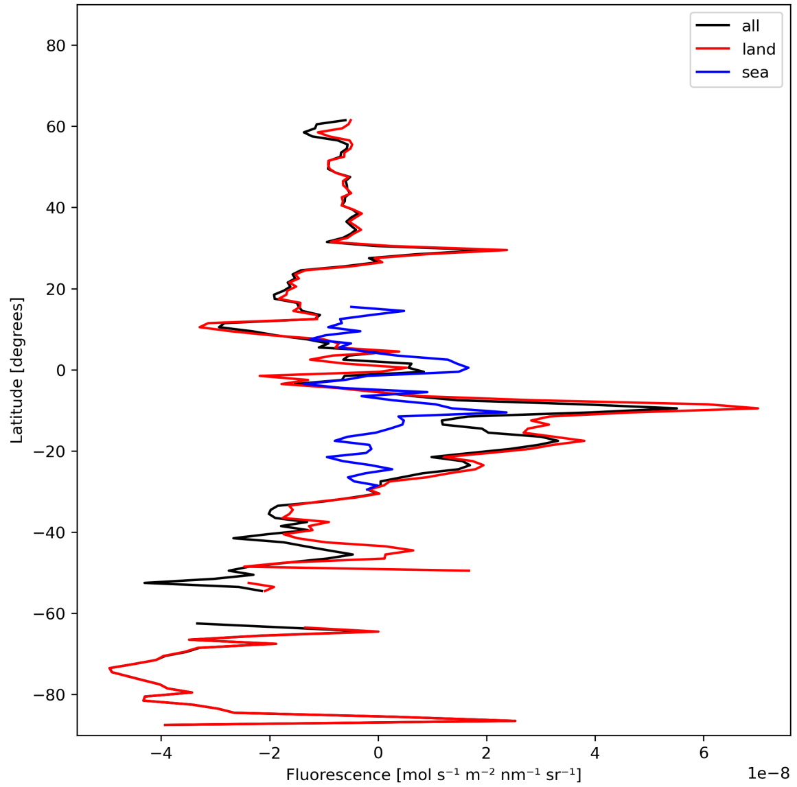
Figure 21: Zonal average of “Fluorescence” for 2023-10-29 to 2023-10-31.
