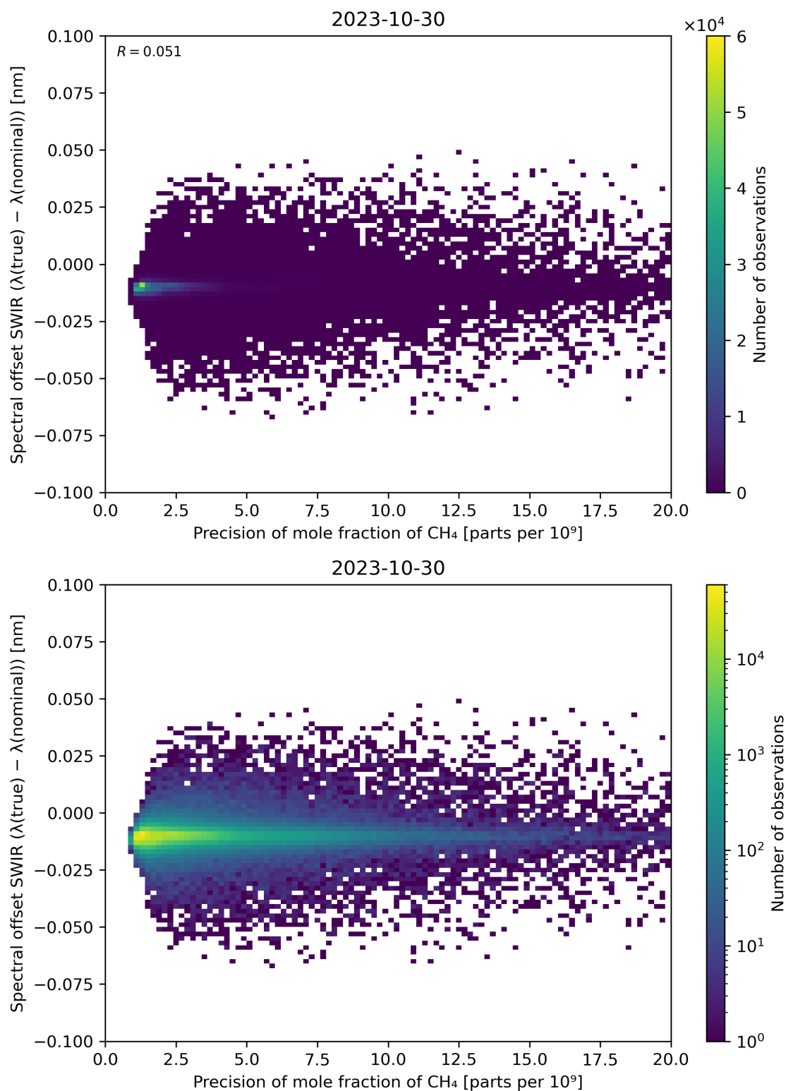
Figure 85: Scatter density plot of “Precision of mole fraction of CH 4 ” against “Spectral offset SWIR ( \lambda(\text{true}) - \lambda(\text{nominal}) )” for 2023-10-29 to 2023-10-31.
