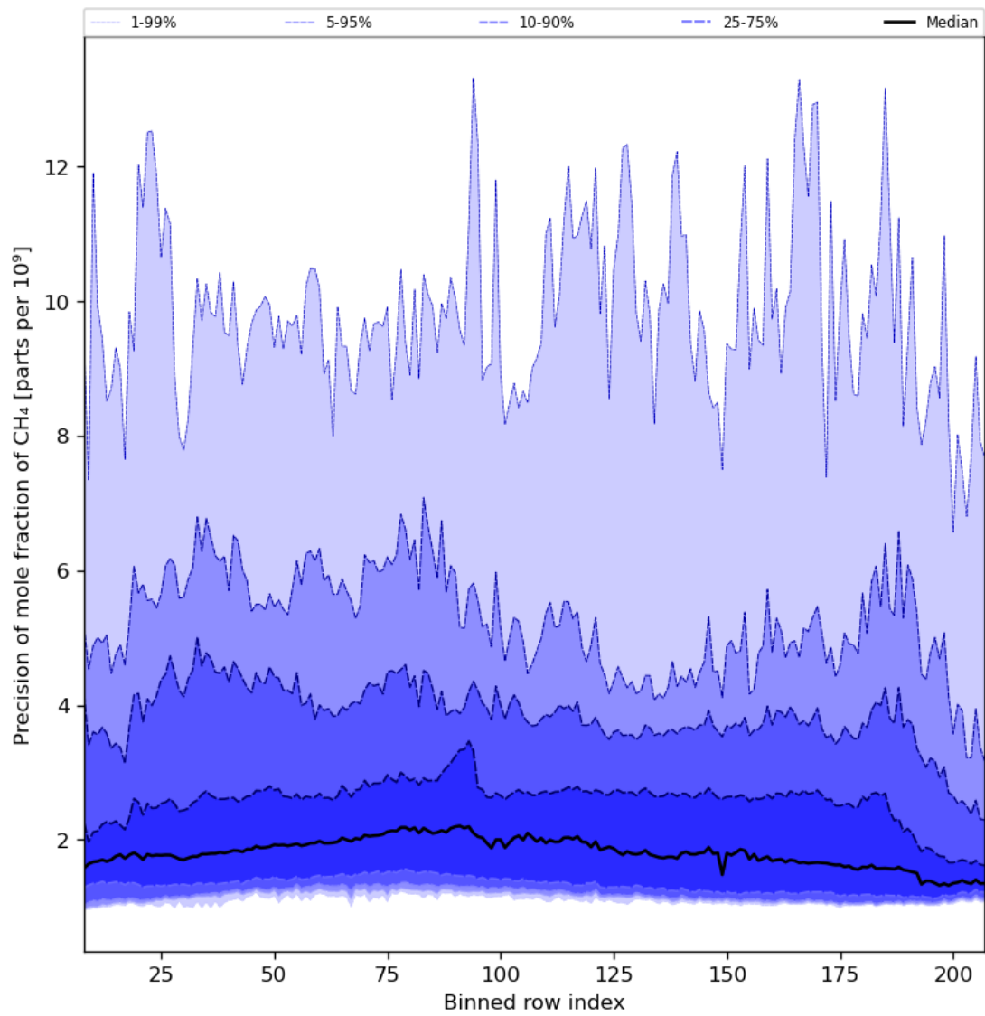
Figure 35: Along track statistics of “Precision of mole fraction of CH 4 ” for 2023-10-29 to 2023-10-31
