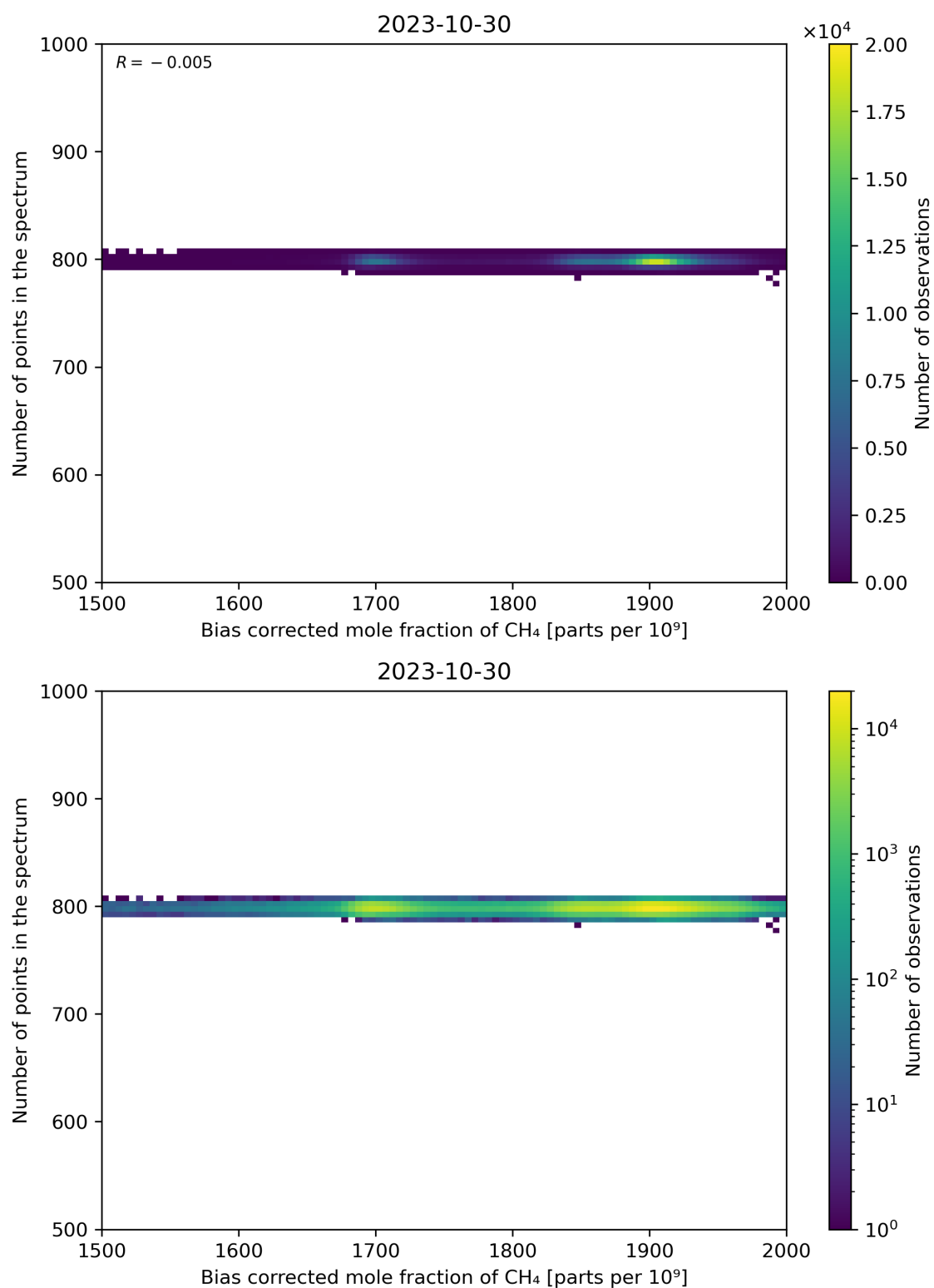
Figure 68: Scatter density plot of “Bias corrected mole fraction of CH 4 ” against “Number of points in the spectrum” for 2023-10-29 to 2023-10-31.
