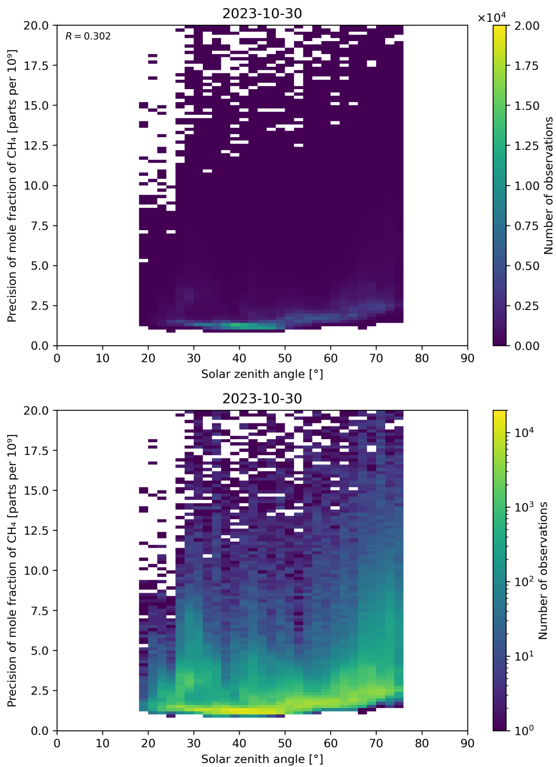
Figure 101: Scatter density plot of “Solar zenith angle” against “Precision of mole fraction of CH 4 ” for 2023-10-29 to 2023-10-31.
