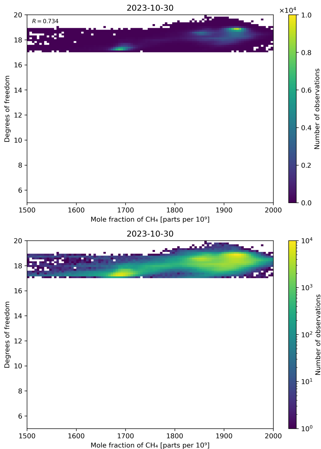
Figure 72: Scatter density plot of “Mole fraction of CH 4 ” against “Degrees of freedom” for 2023-10-29 to 2023-10-31.
