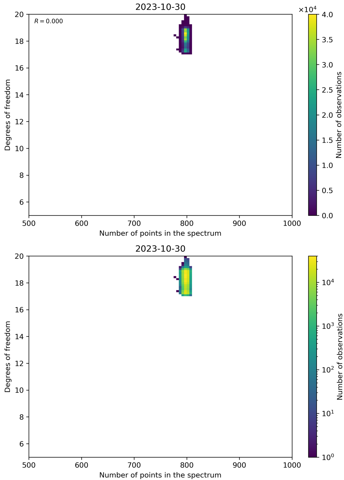
Figure 90: Scatter density plot of “Number of points in the spectrum” against “Degrees of freedom” for 2023-10-29 to 2023-10-31.
