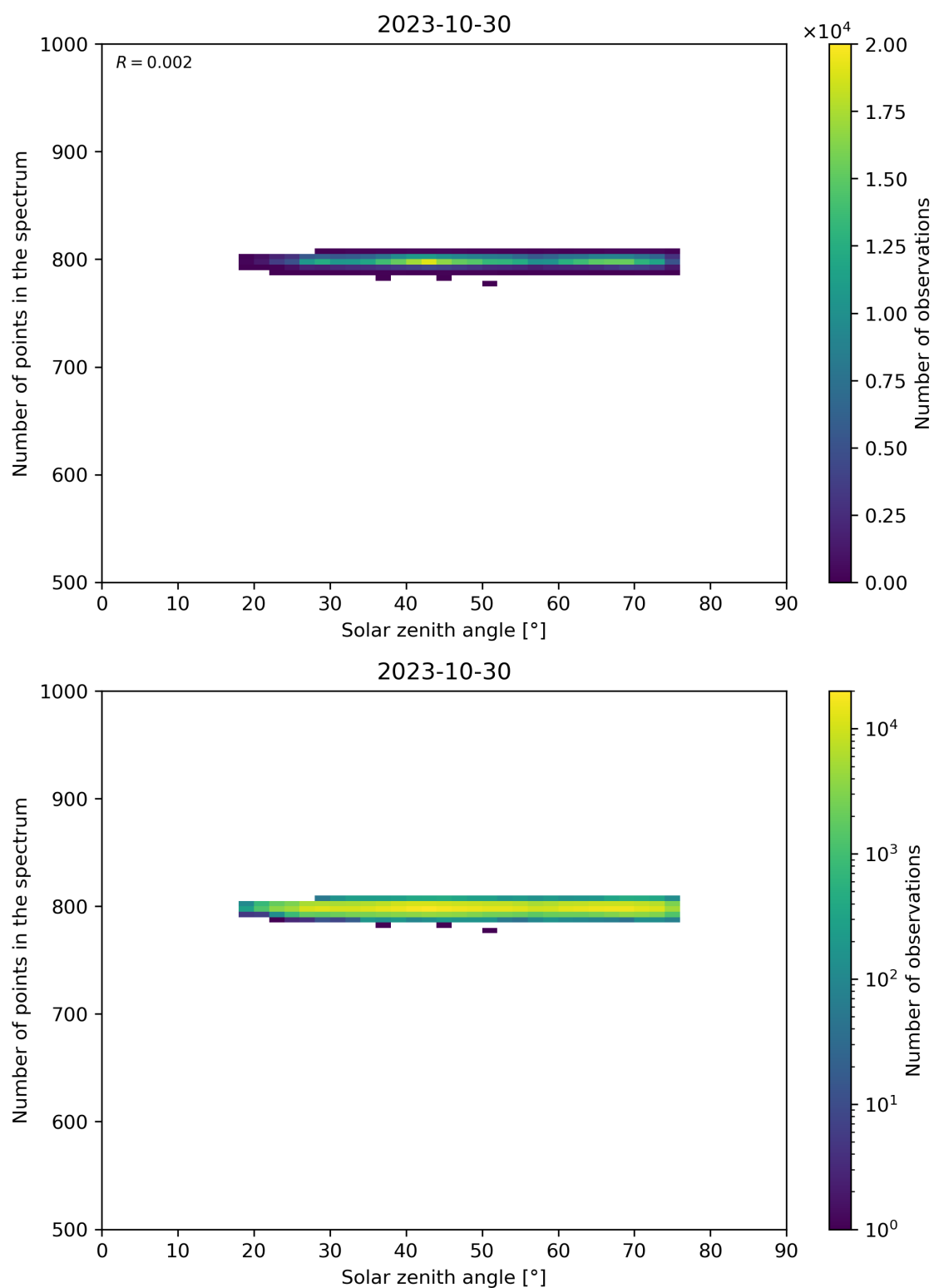
Figure 103: Scatter density plot of “Solar zenith angle” against “Number of points in the spectrum” for 2023-10-29 to 2023-10-31.
