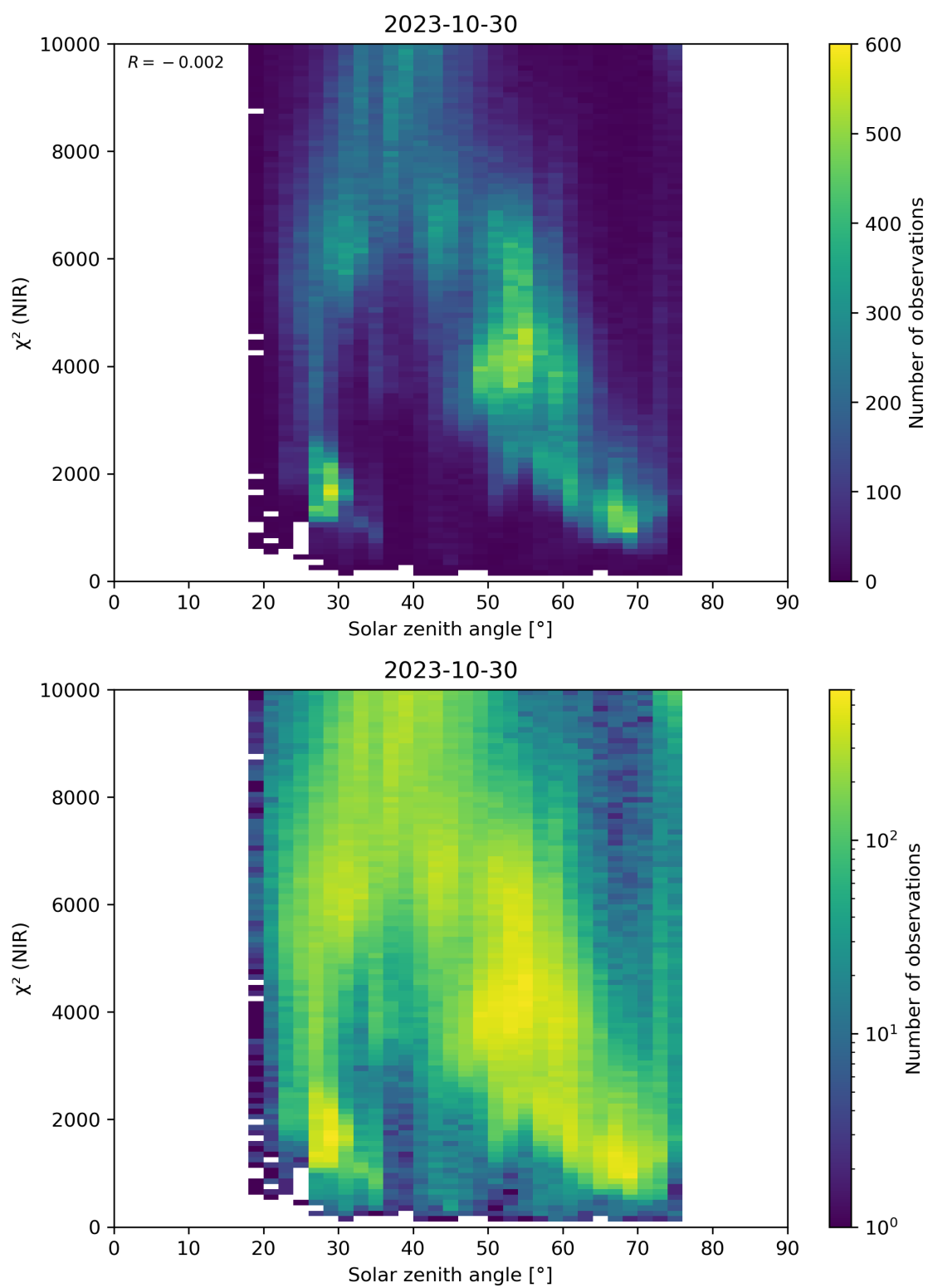
Figure 94: Scatter density plot of “Solar zenith angle” against “ \chi^2 (NIR)” for 2023-10-29 to 2023-10-31.
