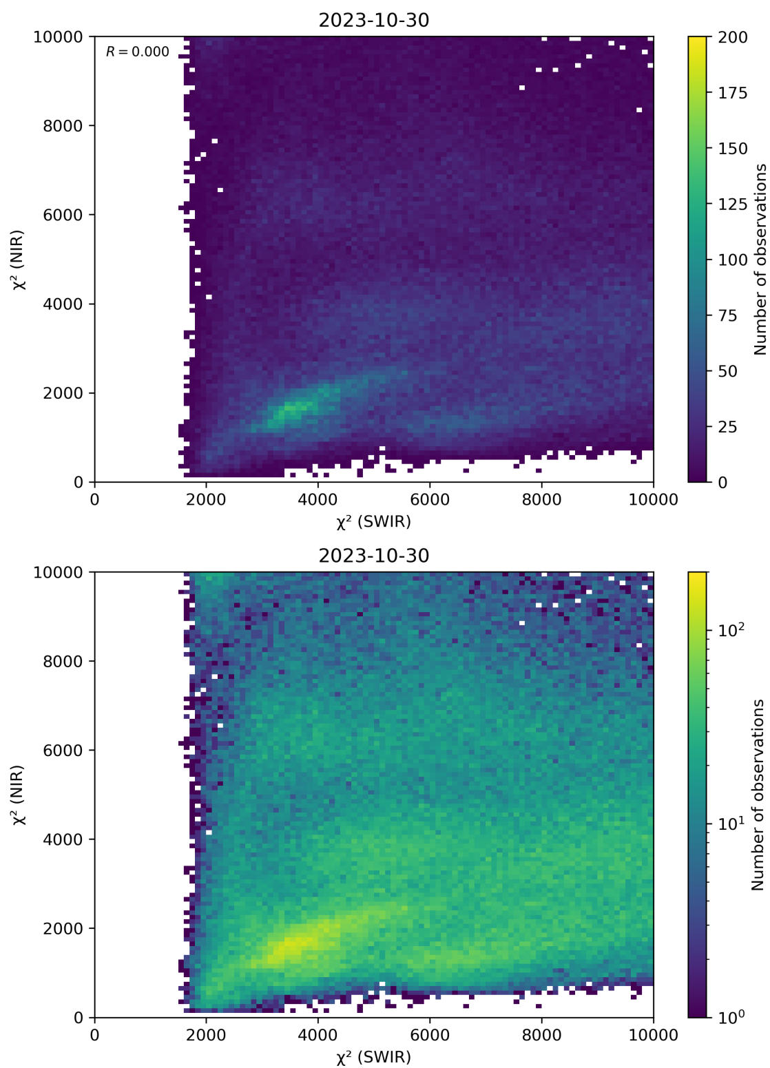
Figure 47: Scatter density plot of “ \chi^2 (SWIR)” against “ \chi^2 (NIR)” for 2023-10-29 to 2023-10-31.
