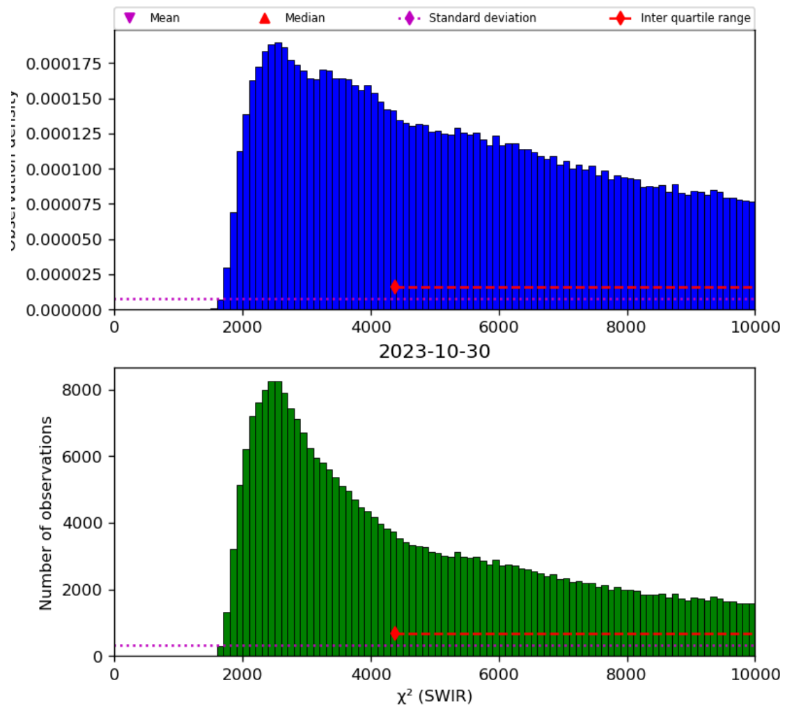
Figure 28: Histogram of “ \chi^2 (SWIR)” for 2023-10-29 to 2023-10-31
