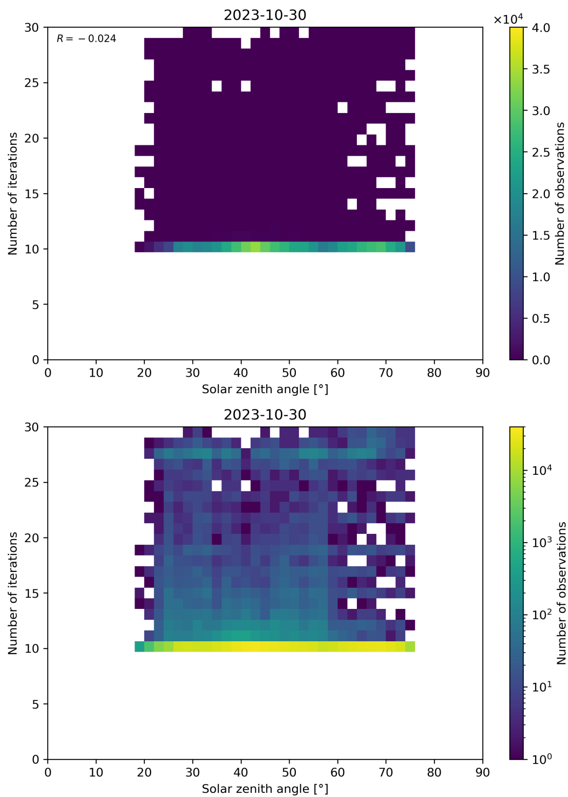
Figure 102: Scatter density plot of “Solar zenith angle” against “Number of iterations” for 2023-10-29 to 2023-10-31.
