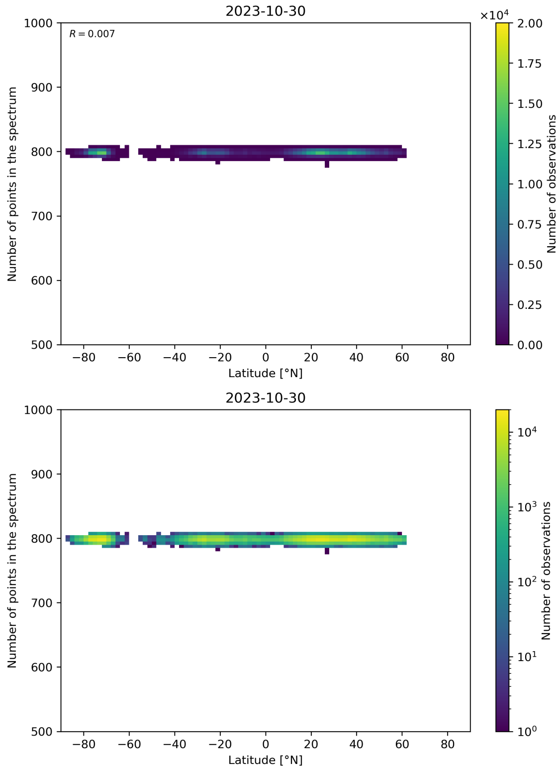
Figure 61: Scatter density plot of “Latitude” against “Number of points in the spectrum” for 2023-10-29 to 2023-10-31.
