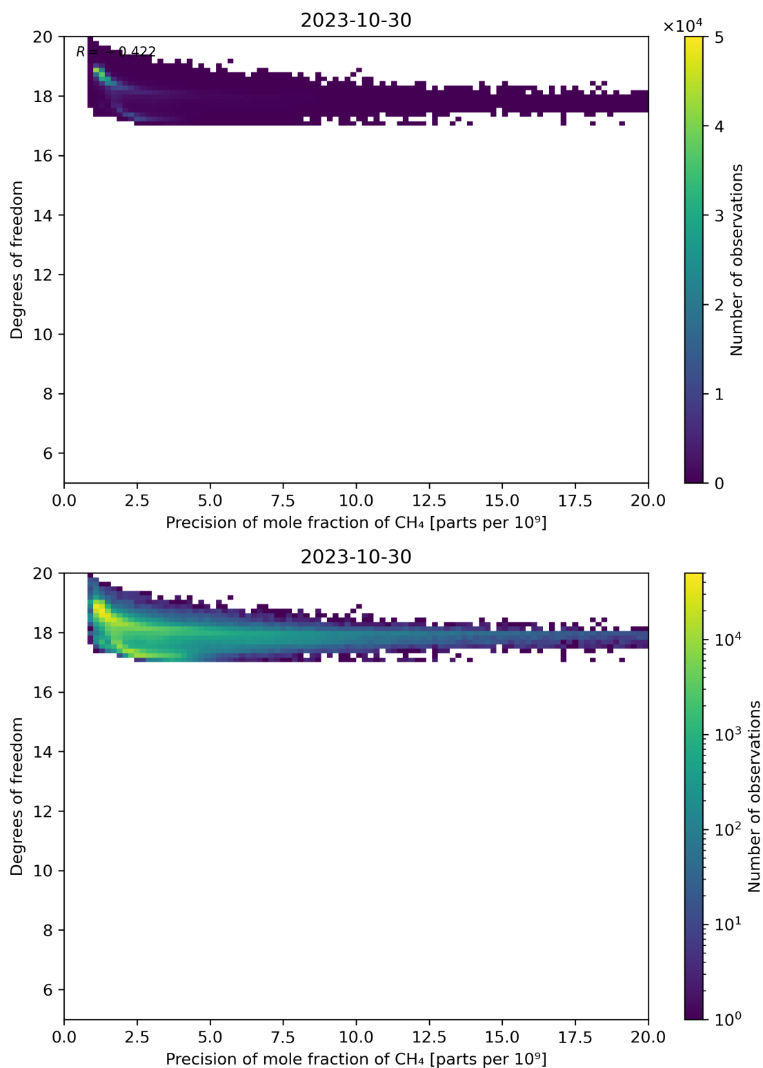
Figure 80: Scatter density plot of “Precision of mole fraction of CH 4 ” against “Degrees of freedom” for 2023-10-29 to 2023-10-31.
