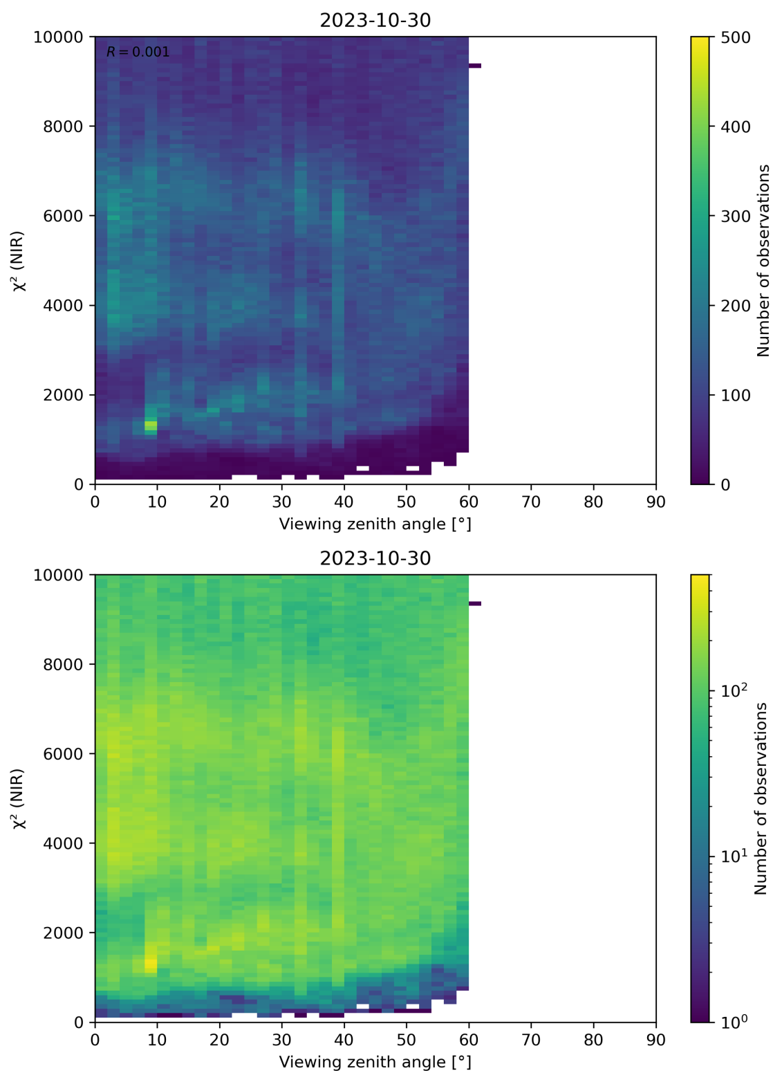
Figure 105: Scatter density plot of “Viewing zenith angle” against “ \chi^2 (NIR)” for 2023-10-29 to 2023-10-31.
