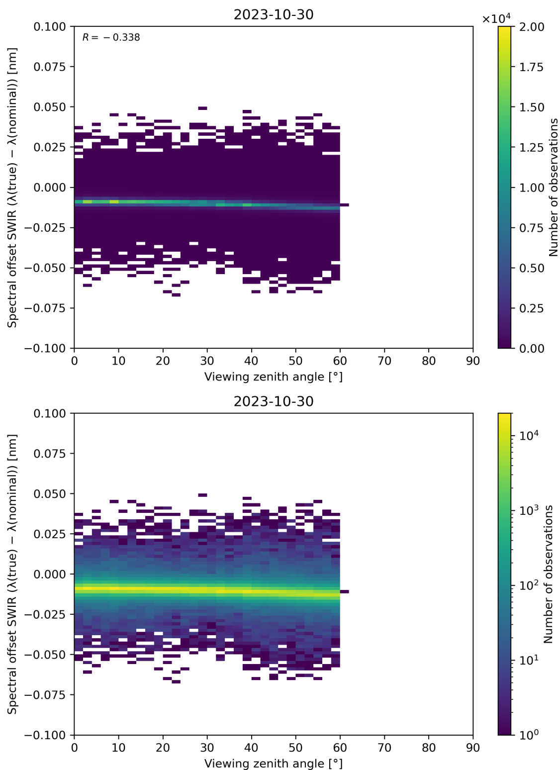
Figure 116: Scatter density plot of “Viewing zenith angle” against “Spectral offset SWIR ( \lambda(\text{true}) - \lambda(\text{nominal}) )” for 2023-10-29 to 2023-10-31.
