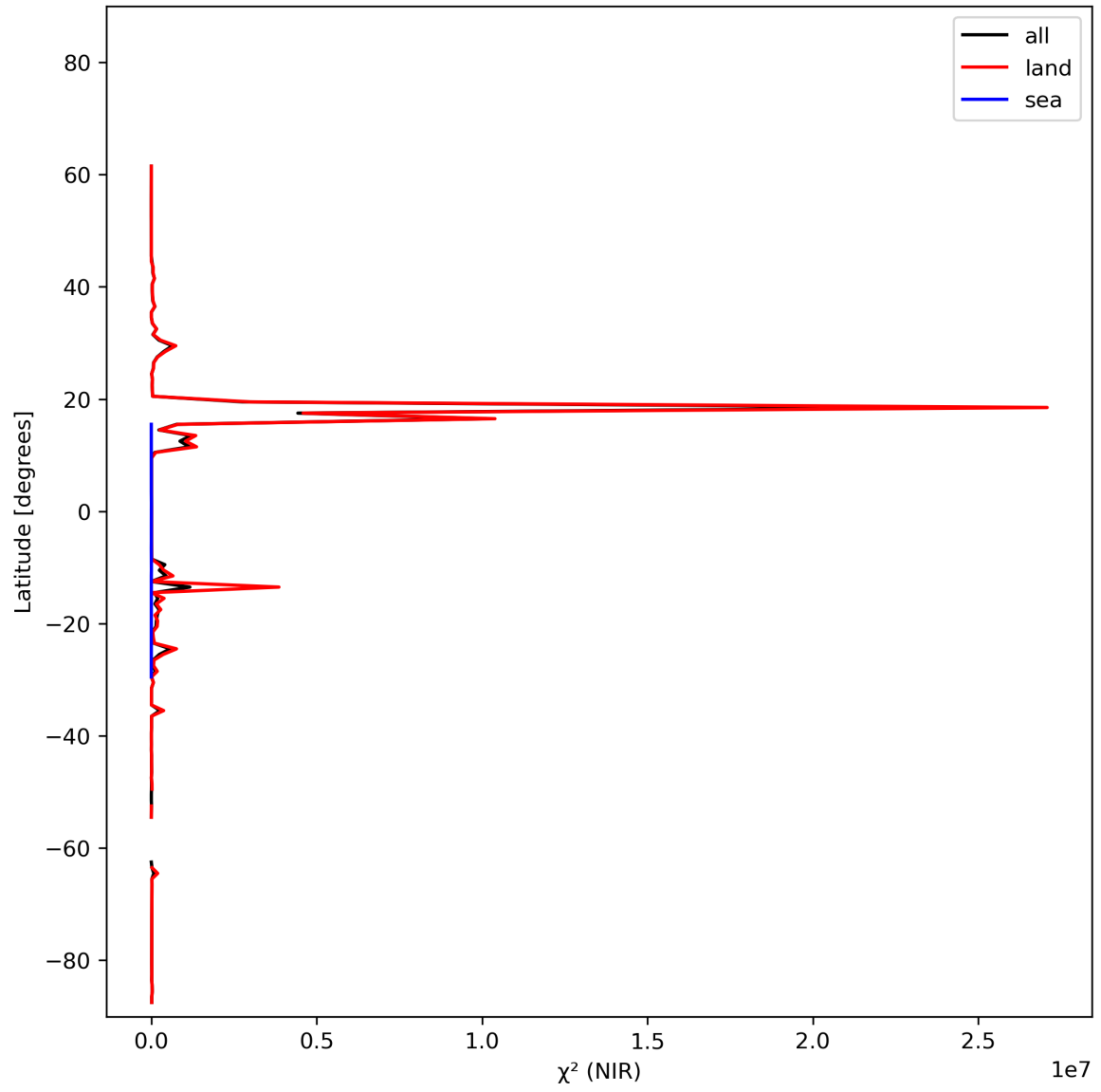
Figure 18: Zonal average of “ \chi^2 (NIR)” for 2023-10-29 to 2023-10-31.
