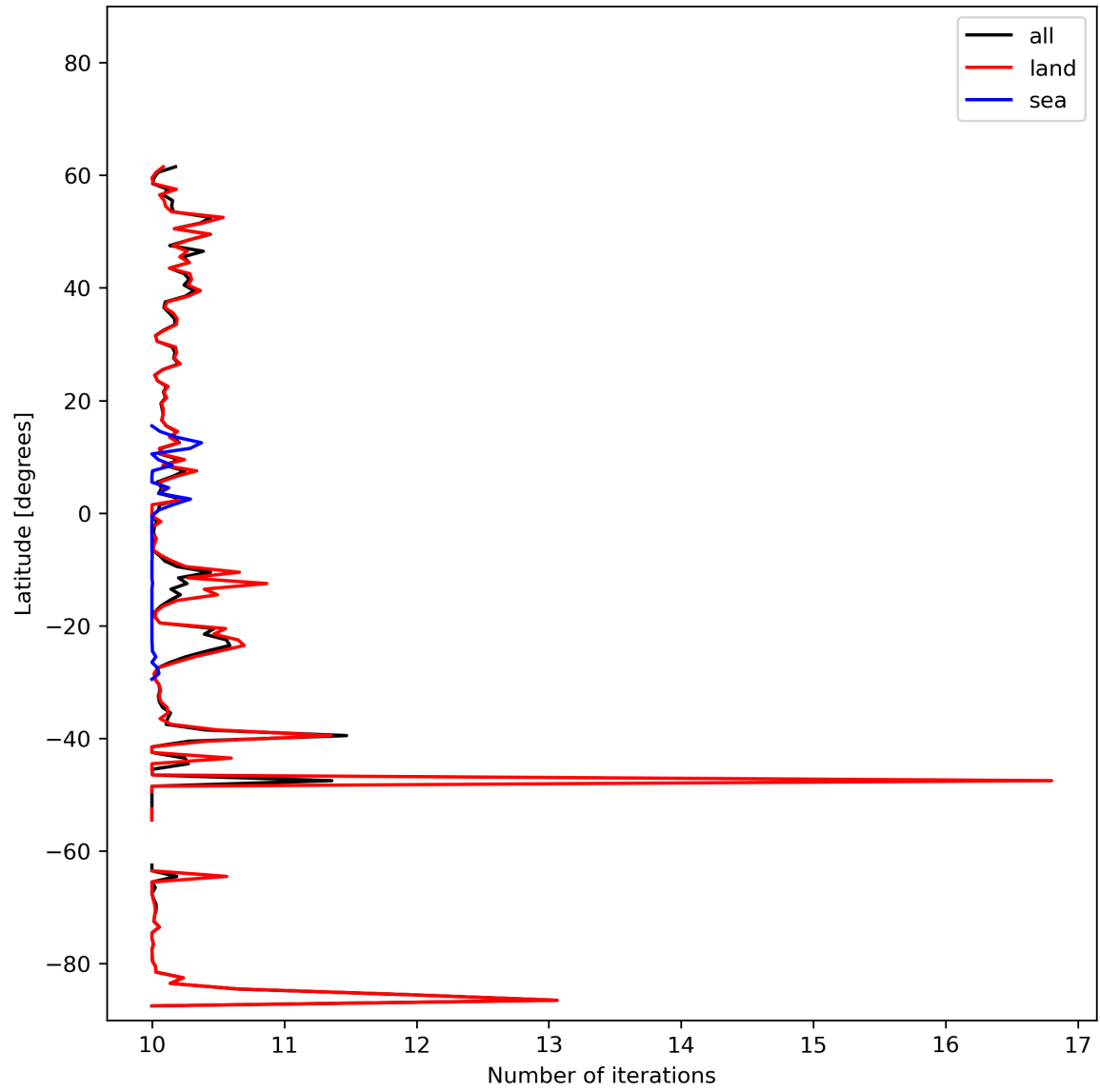
Figure 20: Zonal average of “Number of iterations” for 2023-10-29 to 2023-10-31.
