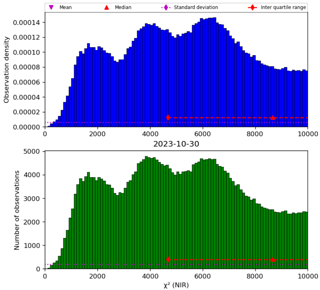
Figure 29: Histogram of “ \chi^2 (NIR)” for 2023-10-29 to 2023-10-31
