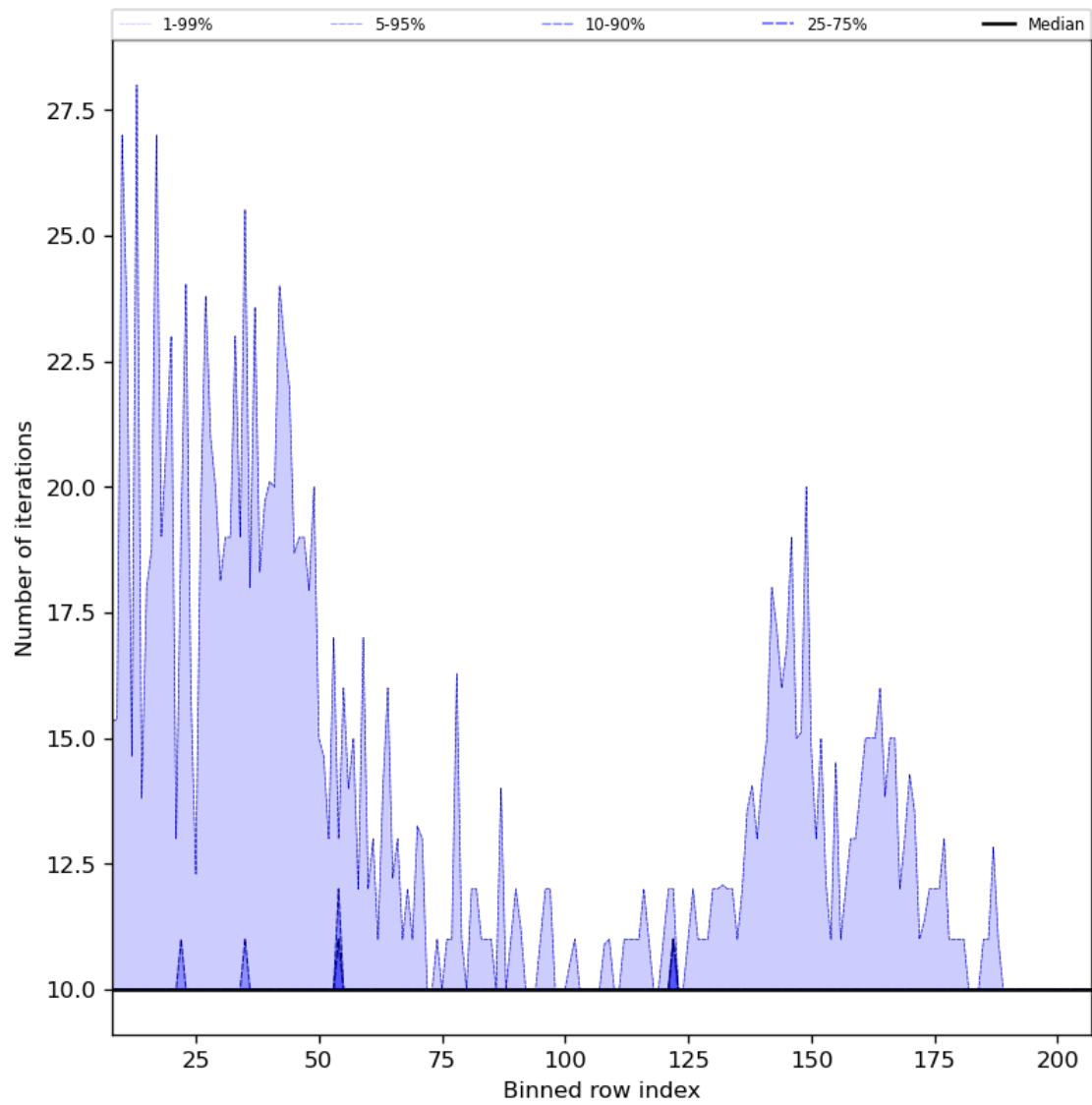
Figure 42: Along track statistics of “Number of iterations” for 2023-10-29 to 2023-10-31
