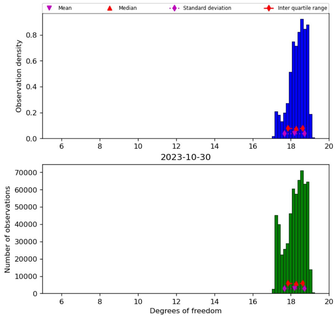
Figure 30: Histogram of “Degrees of freedom” for 2023-10-29 to 2023-10-31
