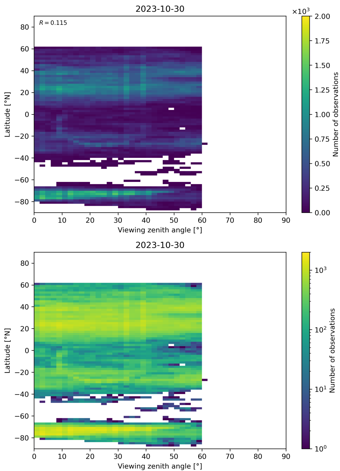
Figure 109: Scatter density plot of “Viewing zenith angle” against “Latitude” for 2023-10-29 to 2023-10-31.
