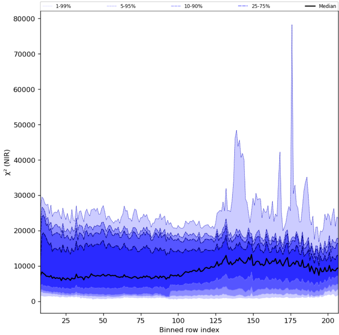
Figure 40: Along track statistics of “ \chi^2 (NIR)” for 2023-10-29 to 2023-10-31
