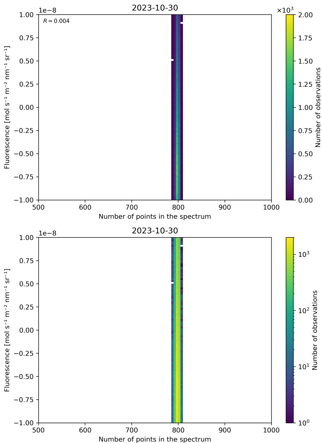
Figure 91: Scatter density plot of “Number of points in the spectrum” against “Fluorescence” for 2023-10-29 to 2023-10-31.
