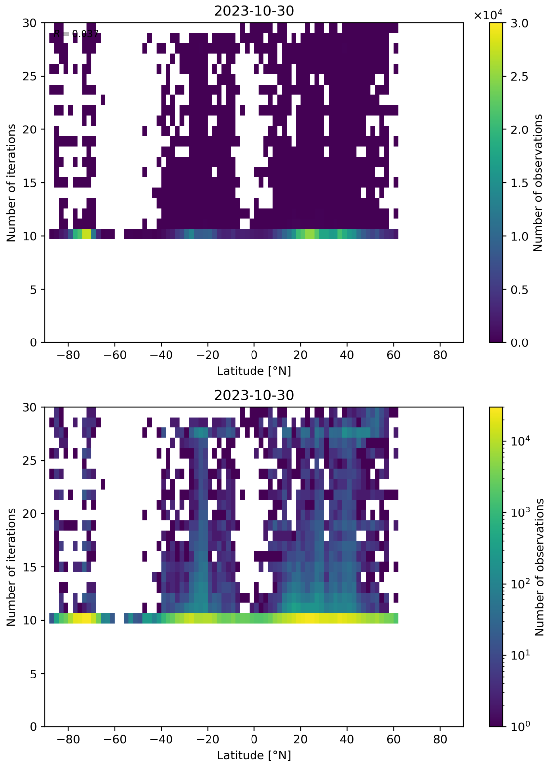
Figure 60: Scatter density plot of “Latitude” against “Number of iterations” for 2023-10-29 to 2023-10-31.
