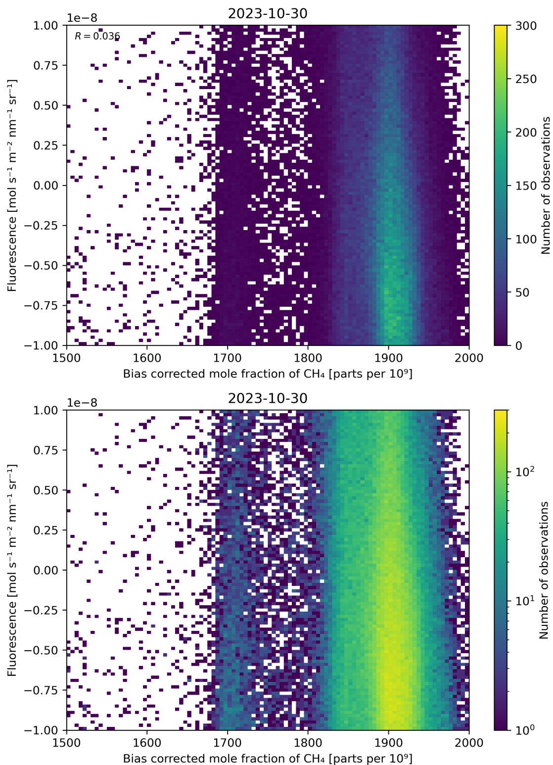
Figure 66: Scatter density plot of “Bias corrected mole fraction of \text{CH}_4 ” against “Fluorescence” for 2023-10-29 to 2023-10-31.
