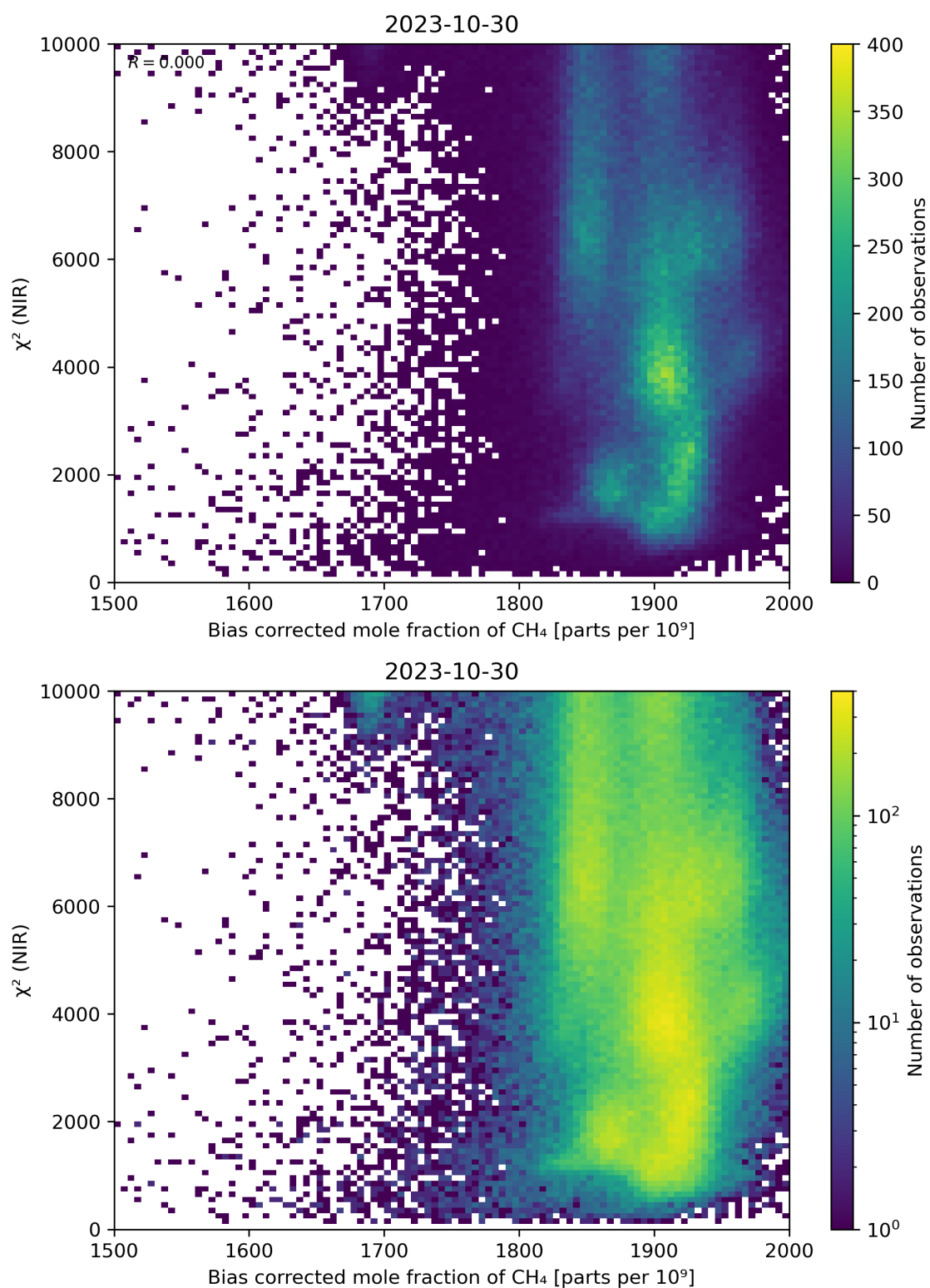
Figure 63: Scatter density plot of “Bias corrected mole fraction of CH 4 ” against “ \chi^2 (NIR)” for 2023-10-29 to 2023-10-31.
