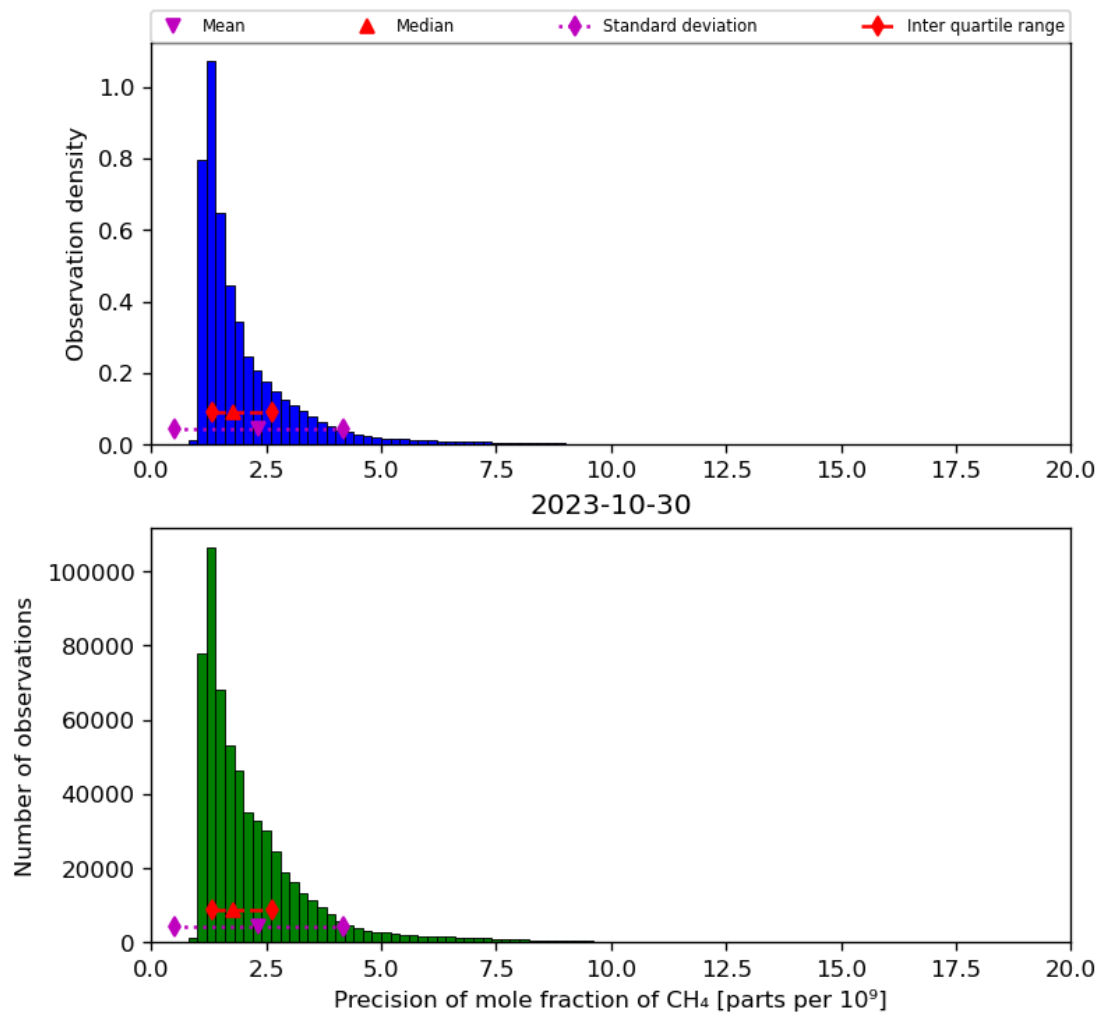
Figure 24: Histogram of “Precision of mole fraction of CH 4 ” for 2023-10-29 to 2023-10-31
