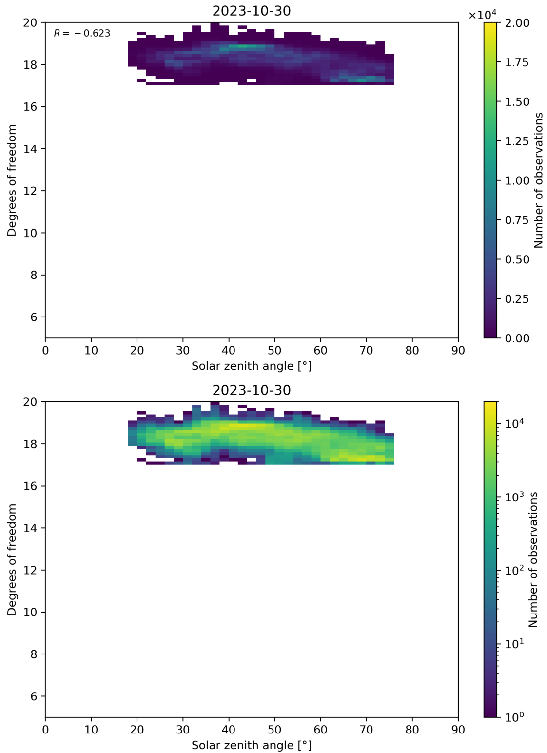
Figure 96: Scatter density plot of “Solar zenith angle” against “Degrees of freedom” for 2023-10-29 to 2023-10-31.
