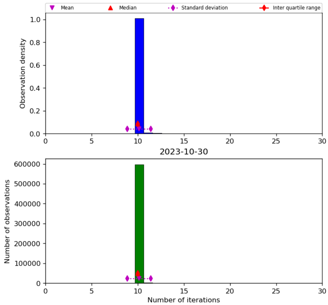
Figure 31: Histogram of “Number of iterations” for 2023-10-29 to 2023-10-31
