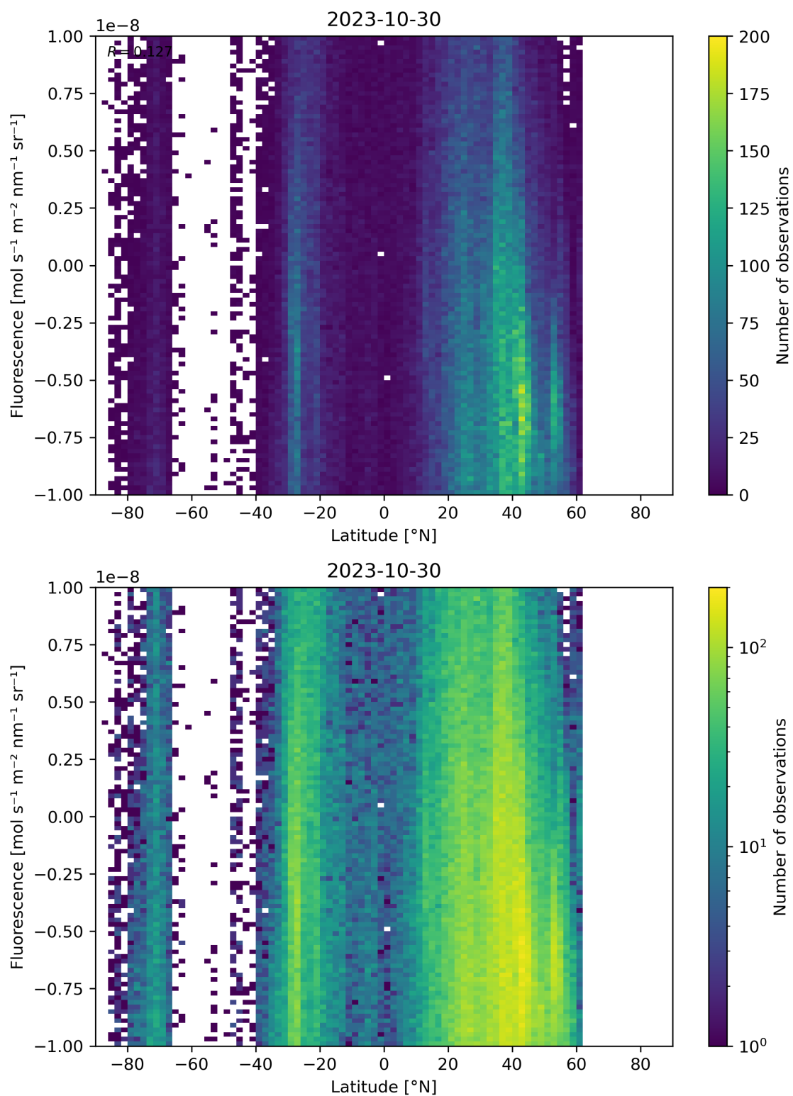
Figure 56: Scatter density plot of “Latitude” against “Fluorescence” for 2023-10-29 to 2023-10-31.
