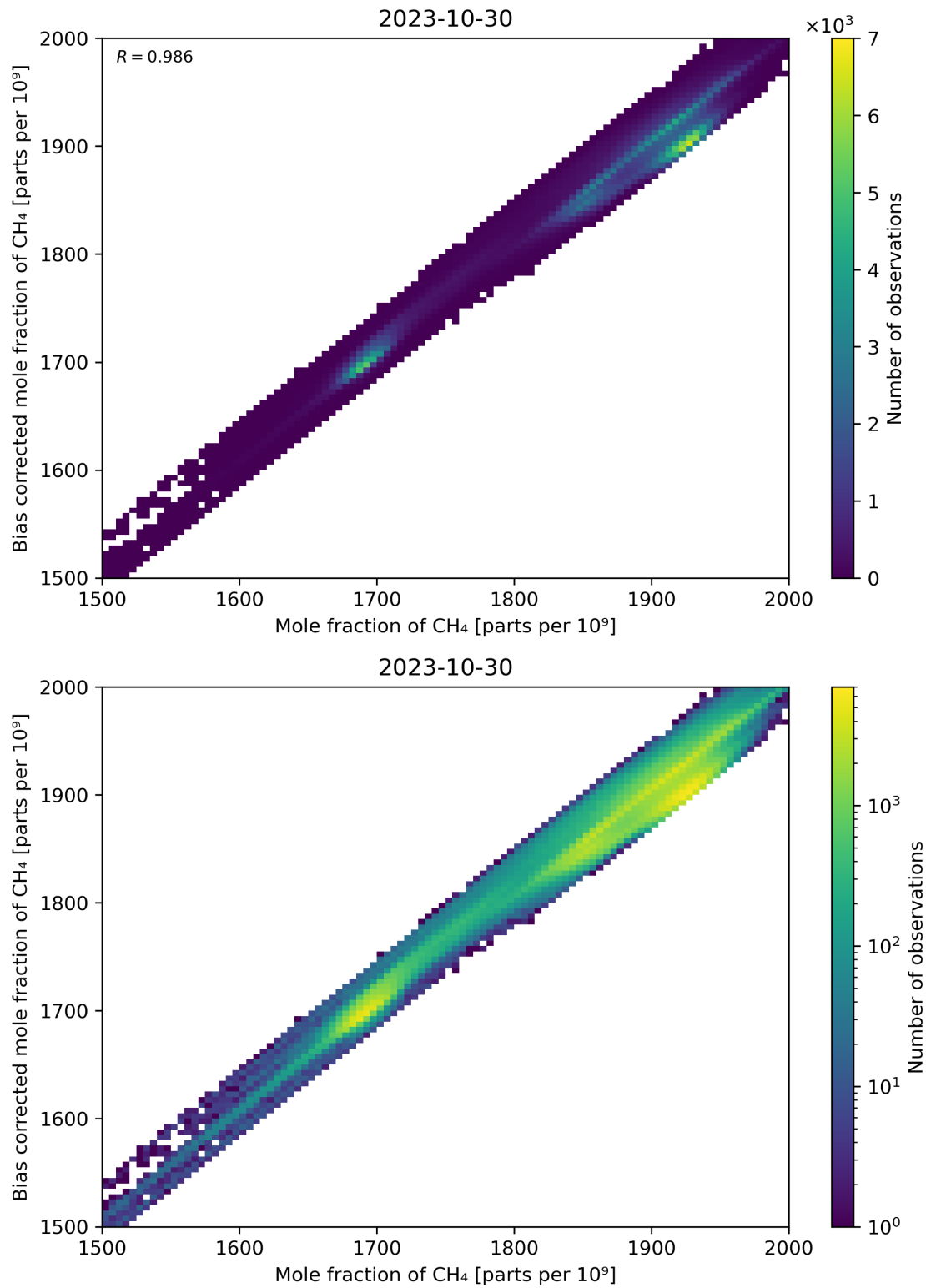
Figure 74: Scatter density plot of “Mole fraction of CH 4 ” against “Bias corrected mole fraction of CH 4 ” for 2023-10-29 to 2023-10-31.
