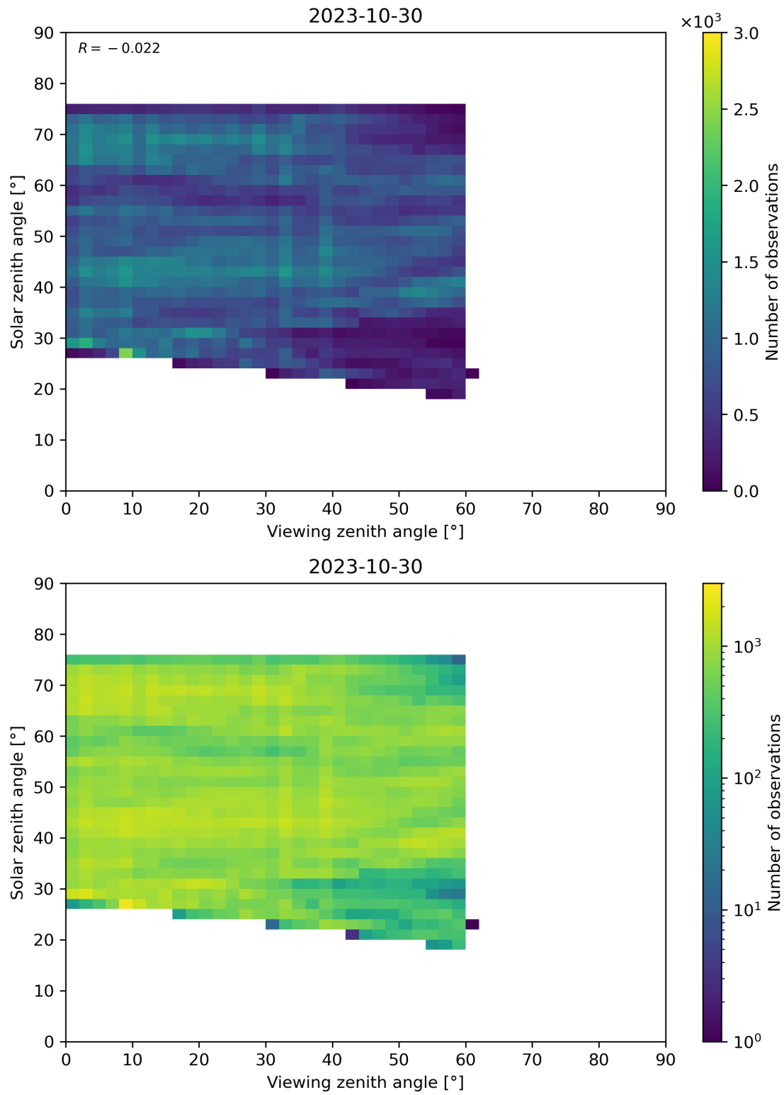
Figure 115: Scatter density plot of “Viewing zenith angle” against “Solar zenith angle” for 2023-10-29 to 2023-10-31.
