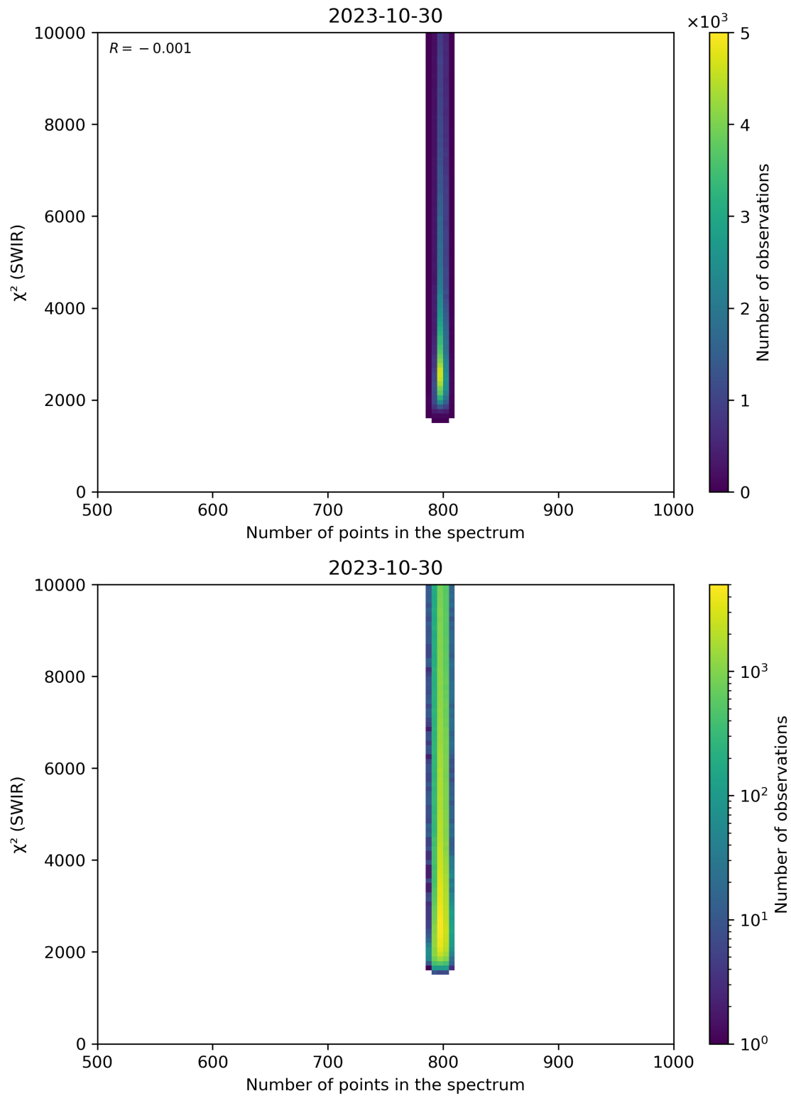
Figure 89: Scatter density plot of “Number of points in the spectrum” against “ \chi^2 (SWIR)” for 2023-10-29 to 2023-10-31.
