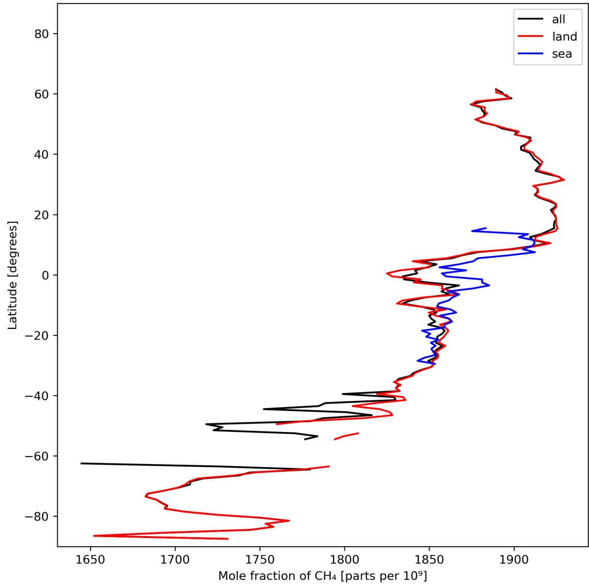
Figure 12: Zonal average of “Mole fraction of \text{CH}_4 ” for 2023-10-29 to 2023-10-31.
