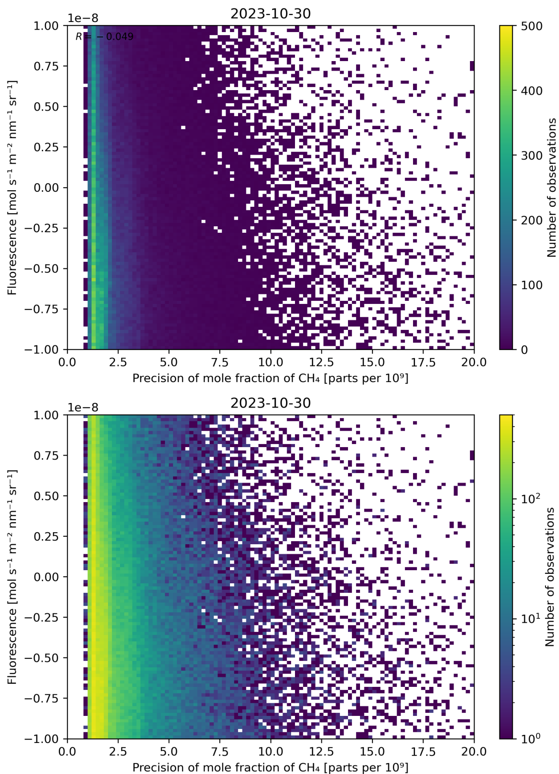
Figure 81: Scatter density plot of “Precision of mole fraction of \text{CH}_4 ” against “Fluorescence” for 2023-10-29 to 2023-10-31.
