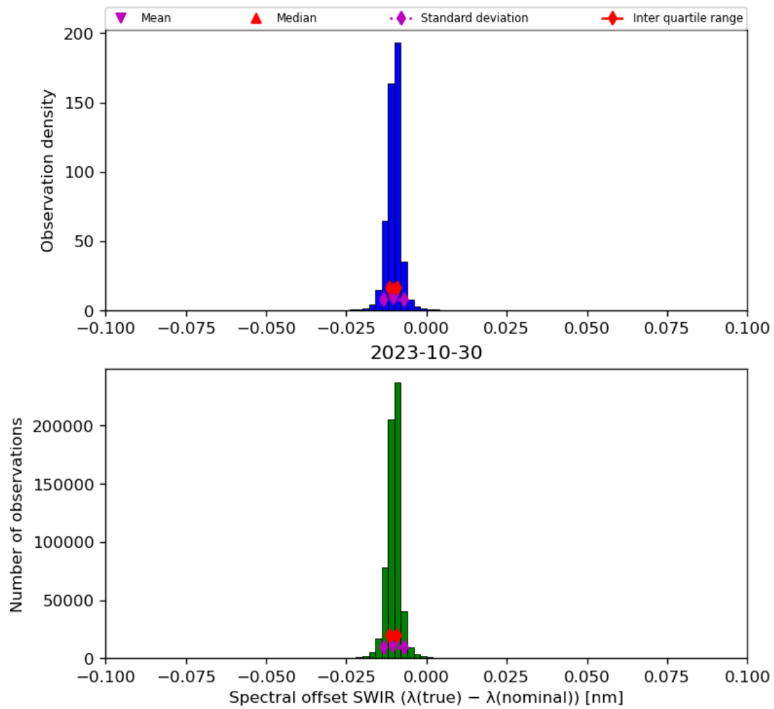
Figure 27: Histogram of “Spectral offset SWIR ( \lambda(\text{true}) - \lambda(\text{nominal}) )” for 2023-10-29 to 2023-10-31
