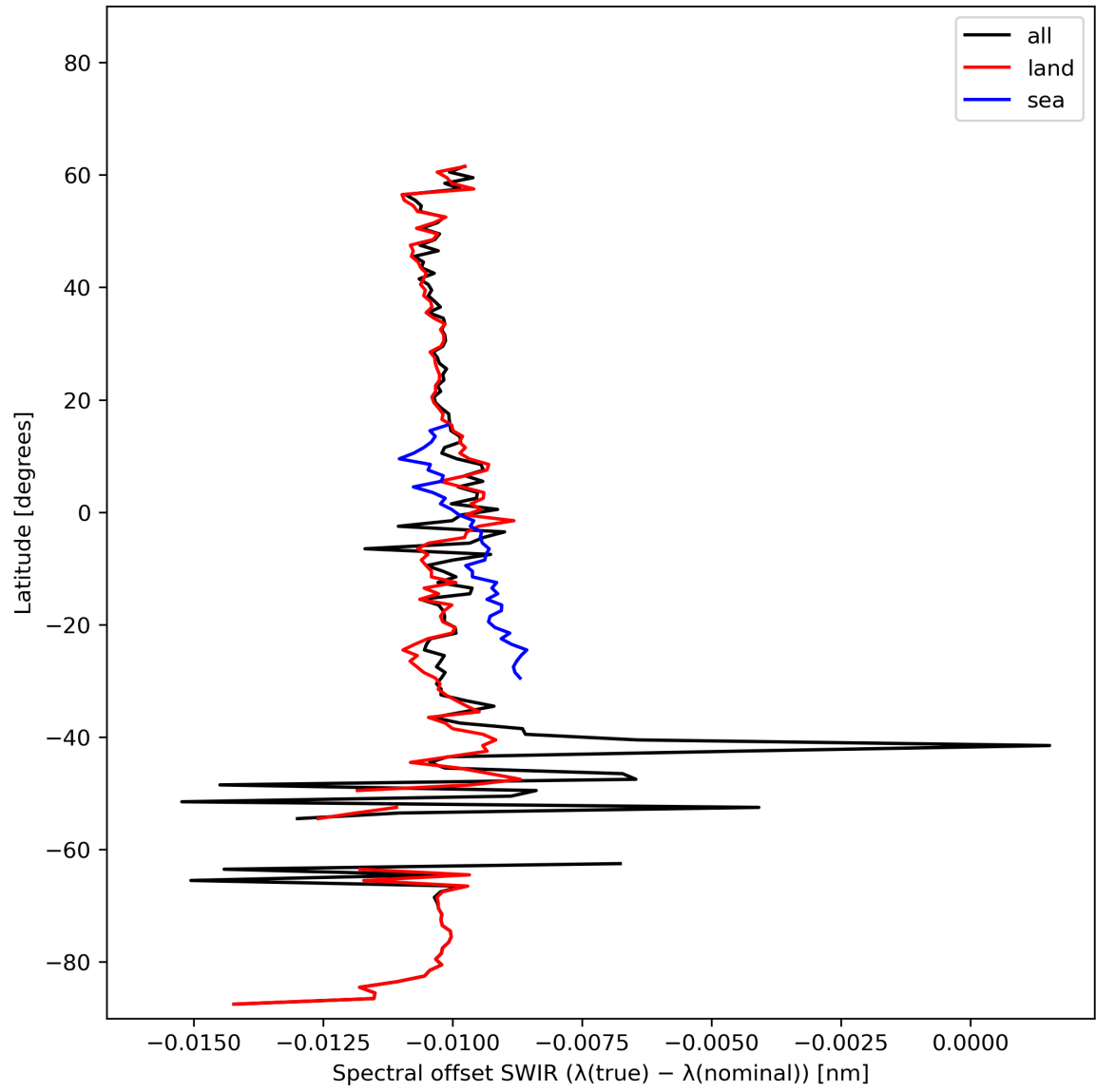
Figure 16: Zonal average of “Spectral offset SWIR ( \lambda(\text{true}) - \lambda(\text{nominal}) )” for 2023-10-29 to 2023-10-31.
