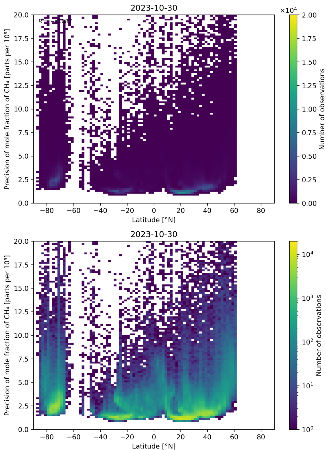
Figure 59: Scatter density plot of “Latitude” against “Precision of mole fraction of CH 4 ” for 2023-10-29 to 2023-10-31.
