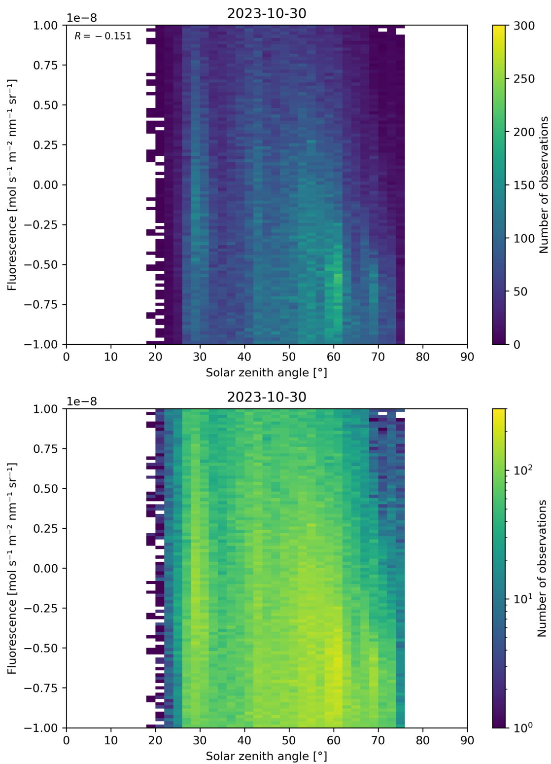
Figure 97: Scatter density plot of “Solar zenith angle” against “Fluorescence” for 2023-10-29 to 2023-10-31.
