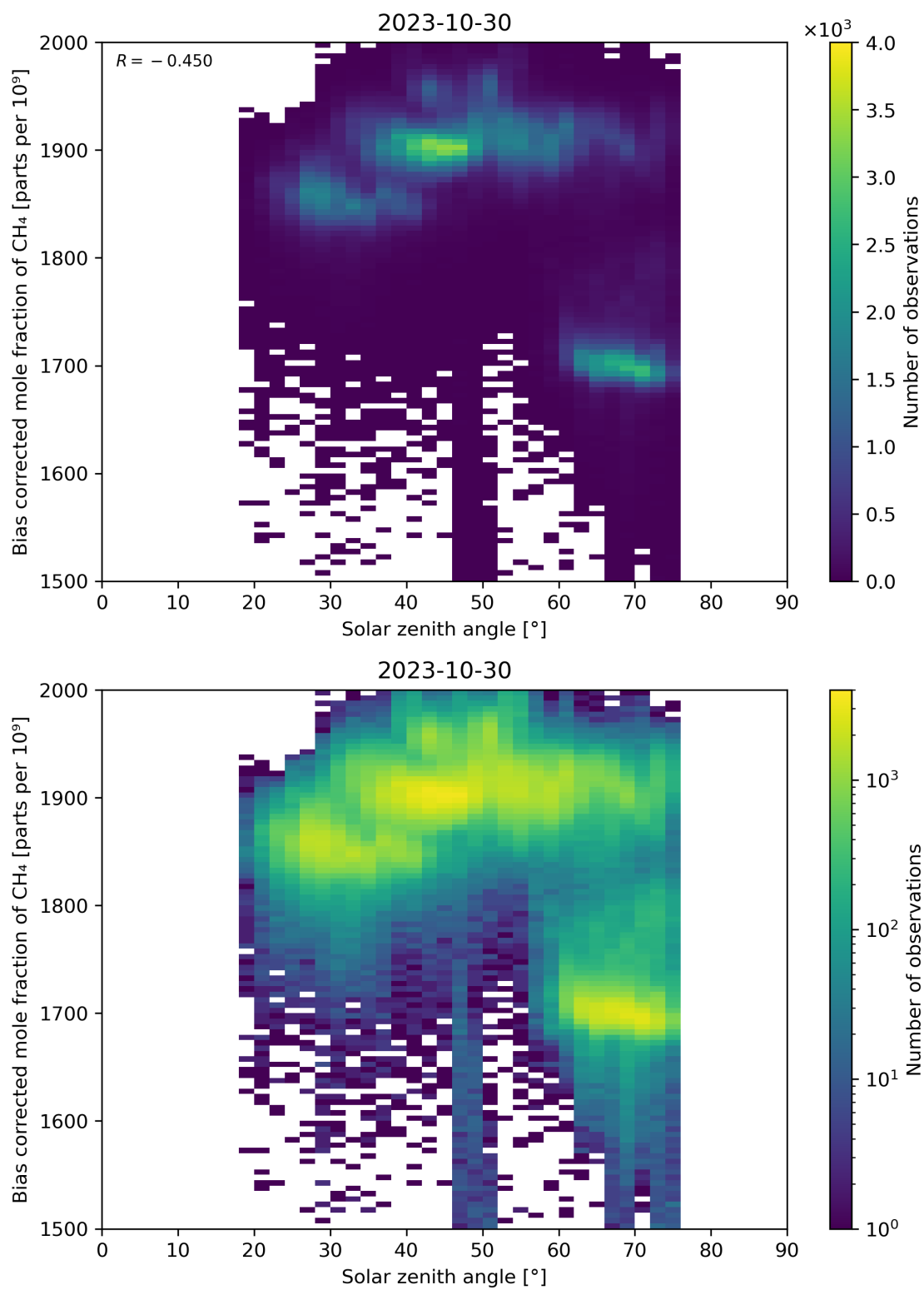
Figure 100: Scatter density plot of “Solar zenith angle” against “Bias corrected mole fraction of \text{CH}_4 ” for 2023-10-29 to 2023-10-31.
