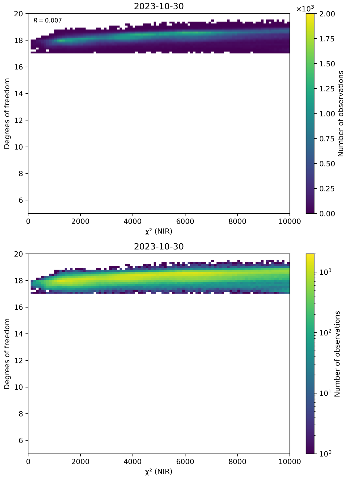
Figure 44: Scatter density plot of “ \chi^2 (NIR)” against “Degrees of freedom” for 2023-10-29 to 2023-10-31.
