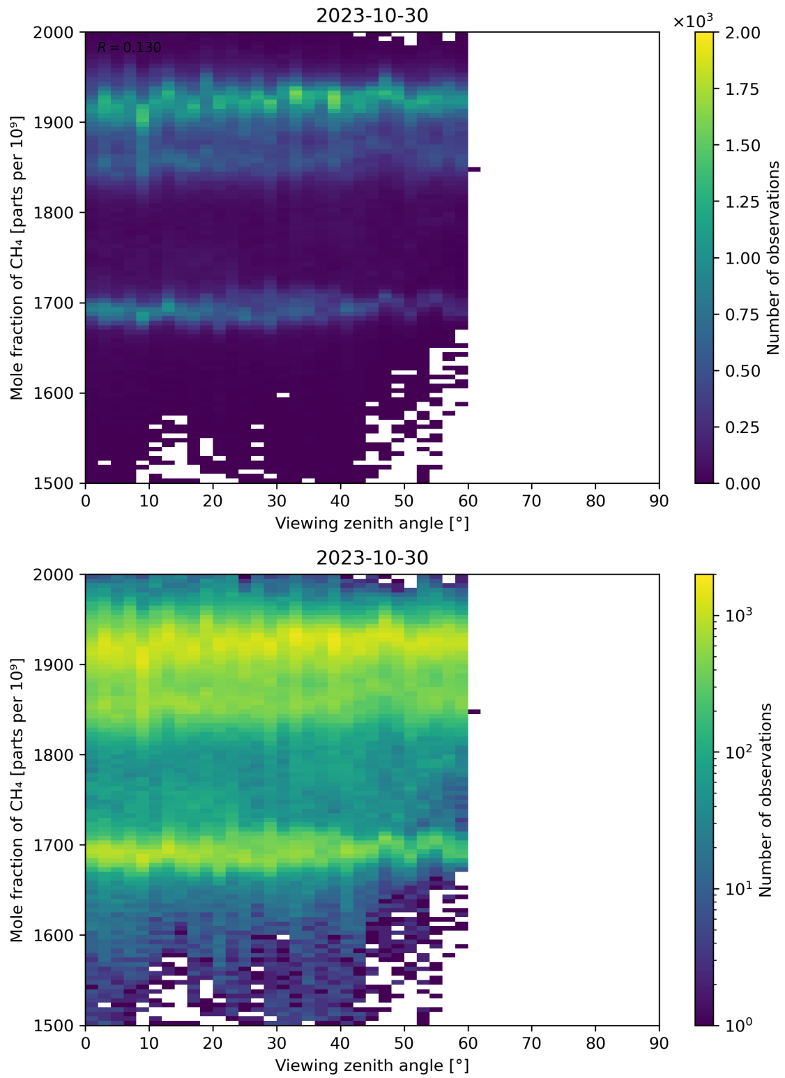
Figure 110: Scatter density plot of “Viewing zenith angle” against “Mole fraction of \text{CH}_4 ” for 2023-10-29 to 2023-10-31.
