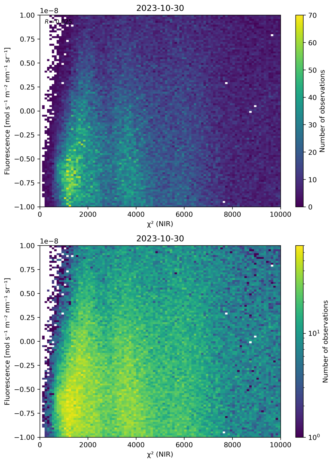
Figure 45: Scatter density plot of “ \chi^2 (NIR)” against “Fluorescence” for 2023-10-29 to 2023-10-31.
