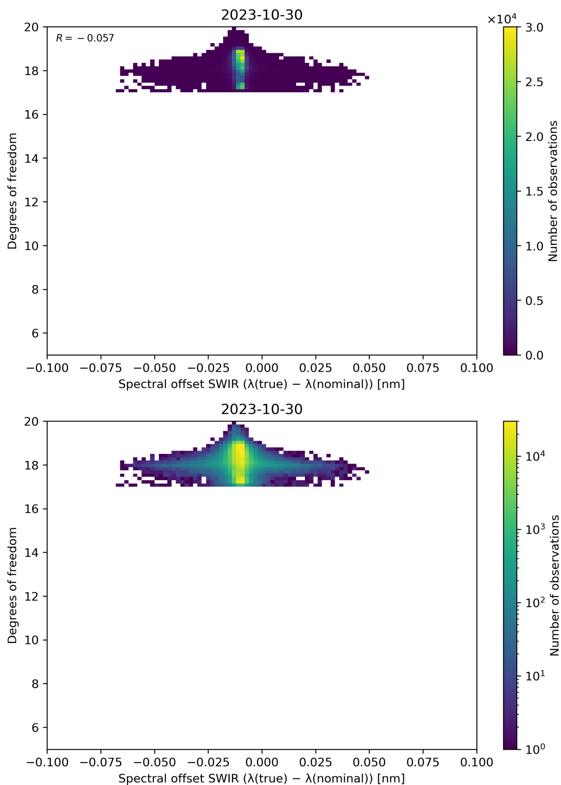
Figure 119: Scatter density plot of “Spectral offset SWIR ( \lambda(\text{true}) - \lambda(\text{nominal}) )” against “Degrees of freedom” for 2023-10-29 to 2023-10-31.
