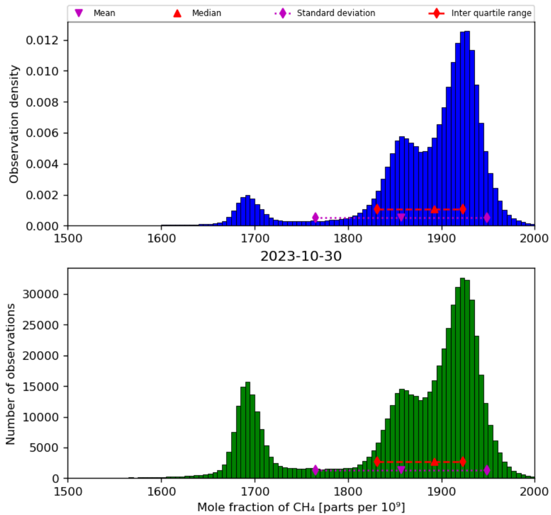
Figure 23: Histogram of “Mole fraction of CH 4 ” for 2023-10-29 to 2023-10-31
