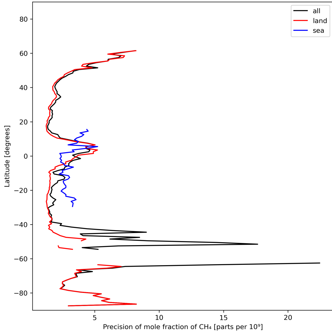
Figure 13: Zonal average of “Precision of mole fraction of CH 4 ” for 2023-10-29 to 2023-10-31.
