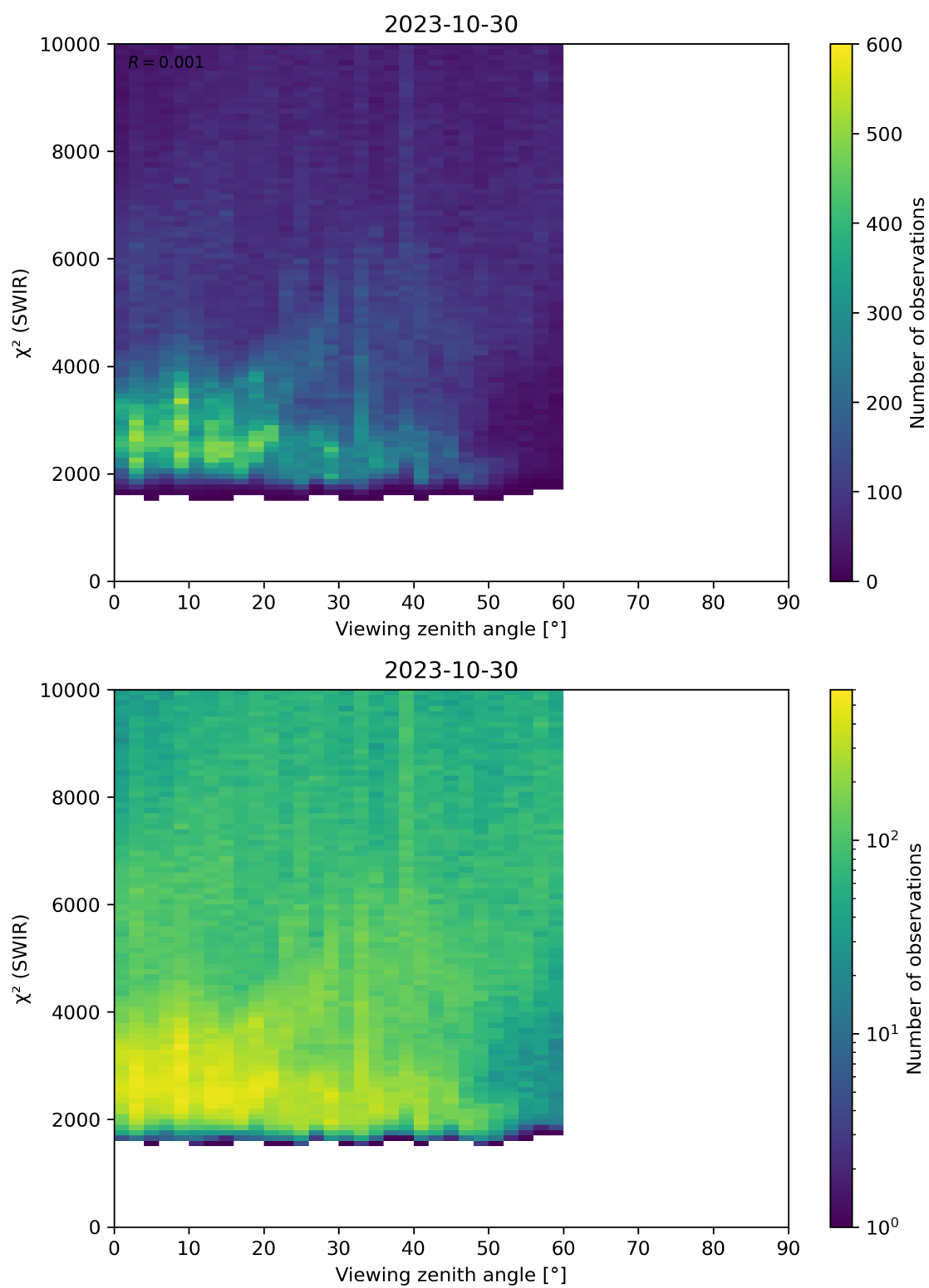
Figure 106: Scatter density plot of “Viewing zenith angle” against “ \chi^2 (SWIR)” for 2023-10-29 to 2023-10-31.
