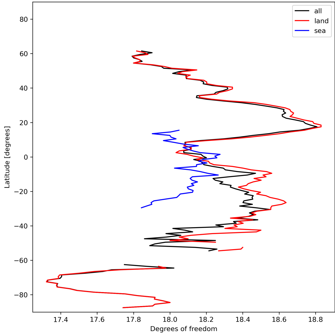
Figure 19: Zonal average of “Degrees of freedom” for 2023-10-29 to 2023-10-31.
