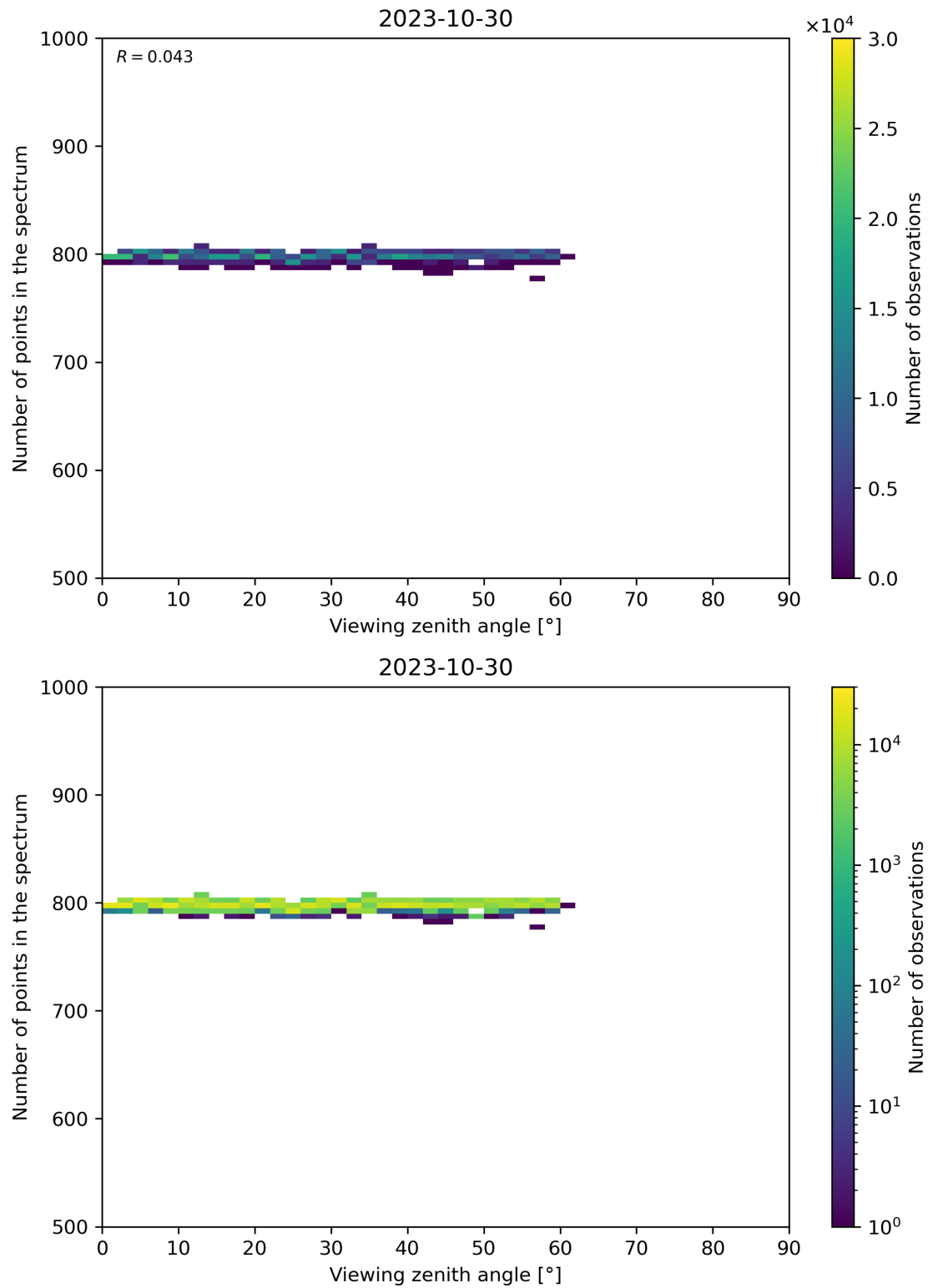
Figure 114: Scatter density plot of “Viewing zenith angle” against “Number of points in the spectrum” for 2023-10-29 to 2023-10-31.
