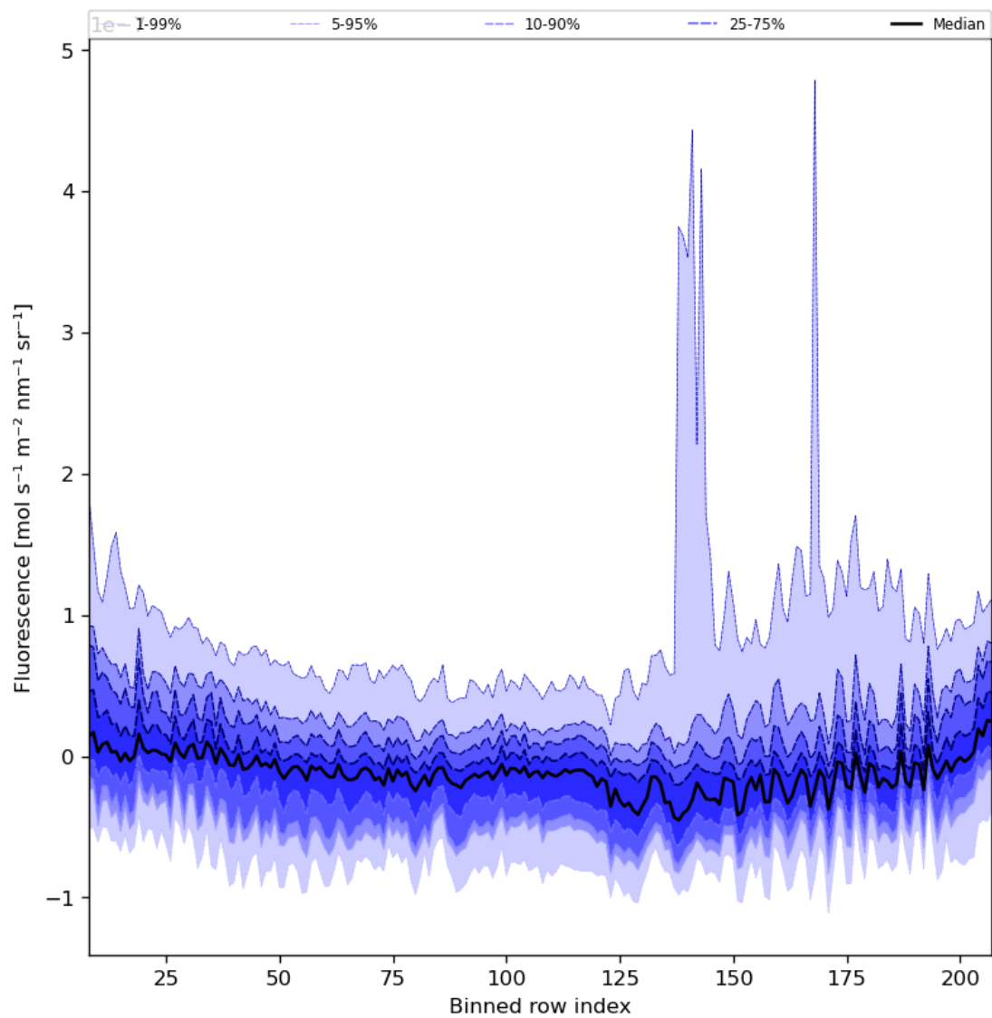
Figure 43: Along track statistics of “Fluorescence” for 2023-10-29 to 2023-10-31
