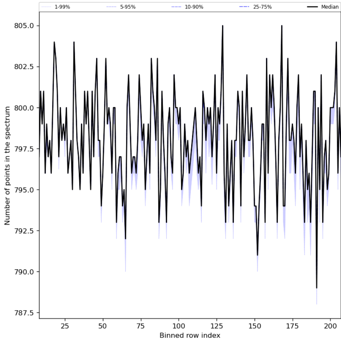
Figure 37: Along track statistics of “Number of points in the spectrum” for 2023-10-29 to 2023-10-31
