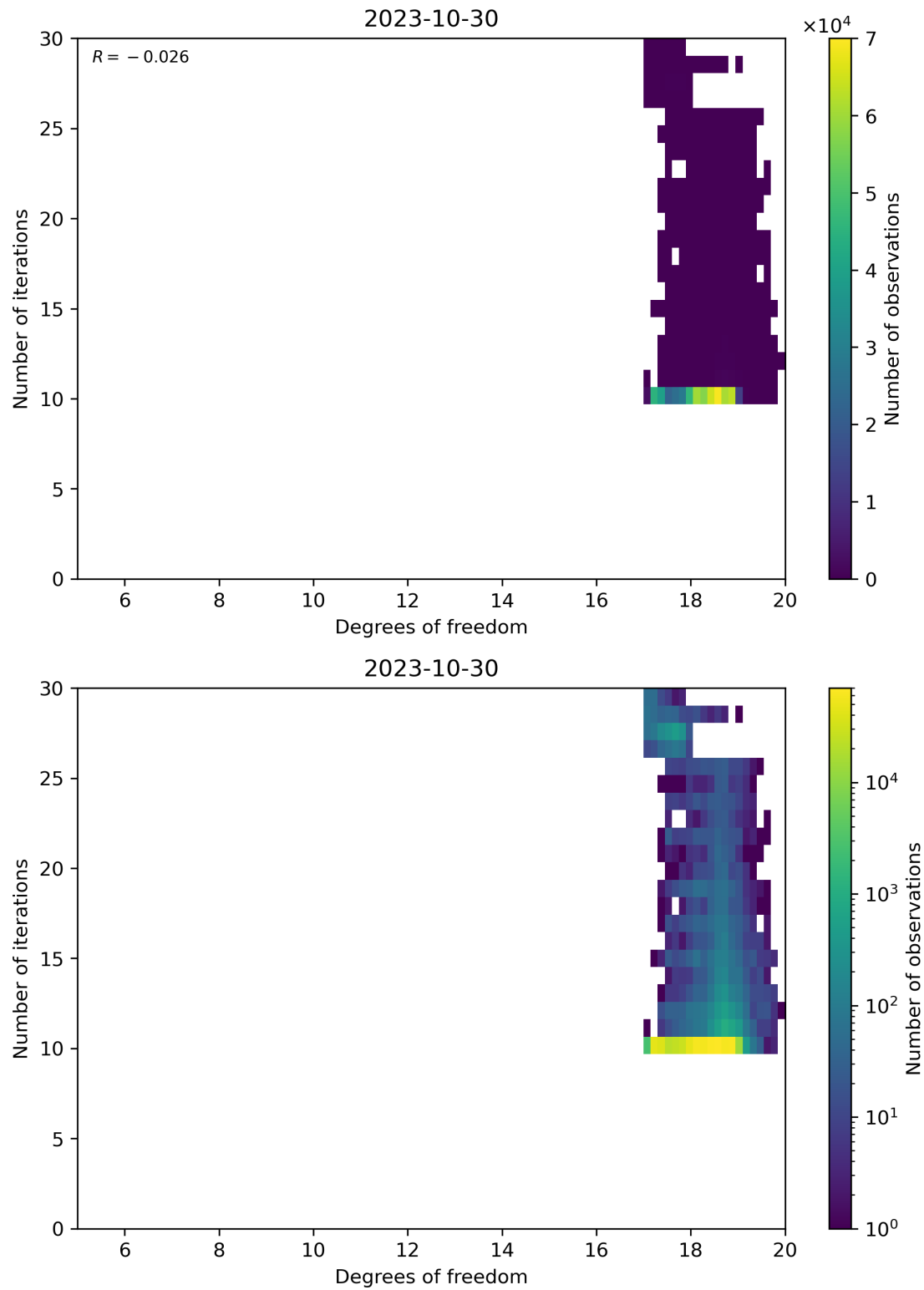
Figure 52: Scatter density plot of “Degrees of freedom” against “Number of iterations” for 2023-10-29 to 2023-10-31.
