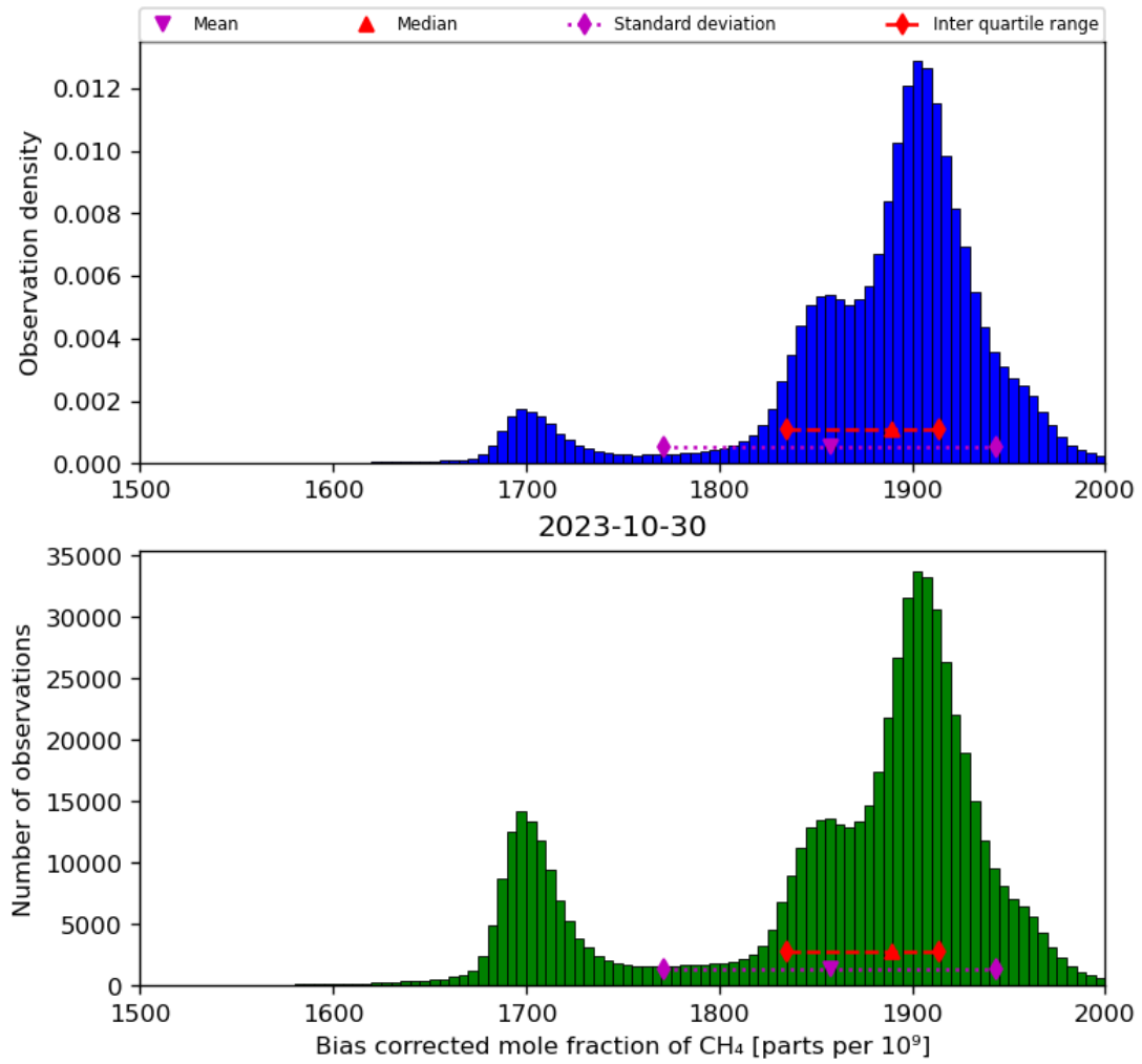
Figure 25: Histogram of “Bias corrected mole fraction of CH 4 ” for 2023-10-29 to 2023-10-31
