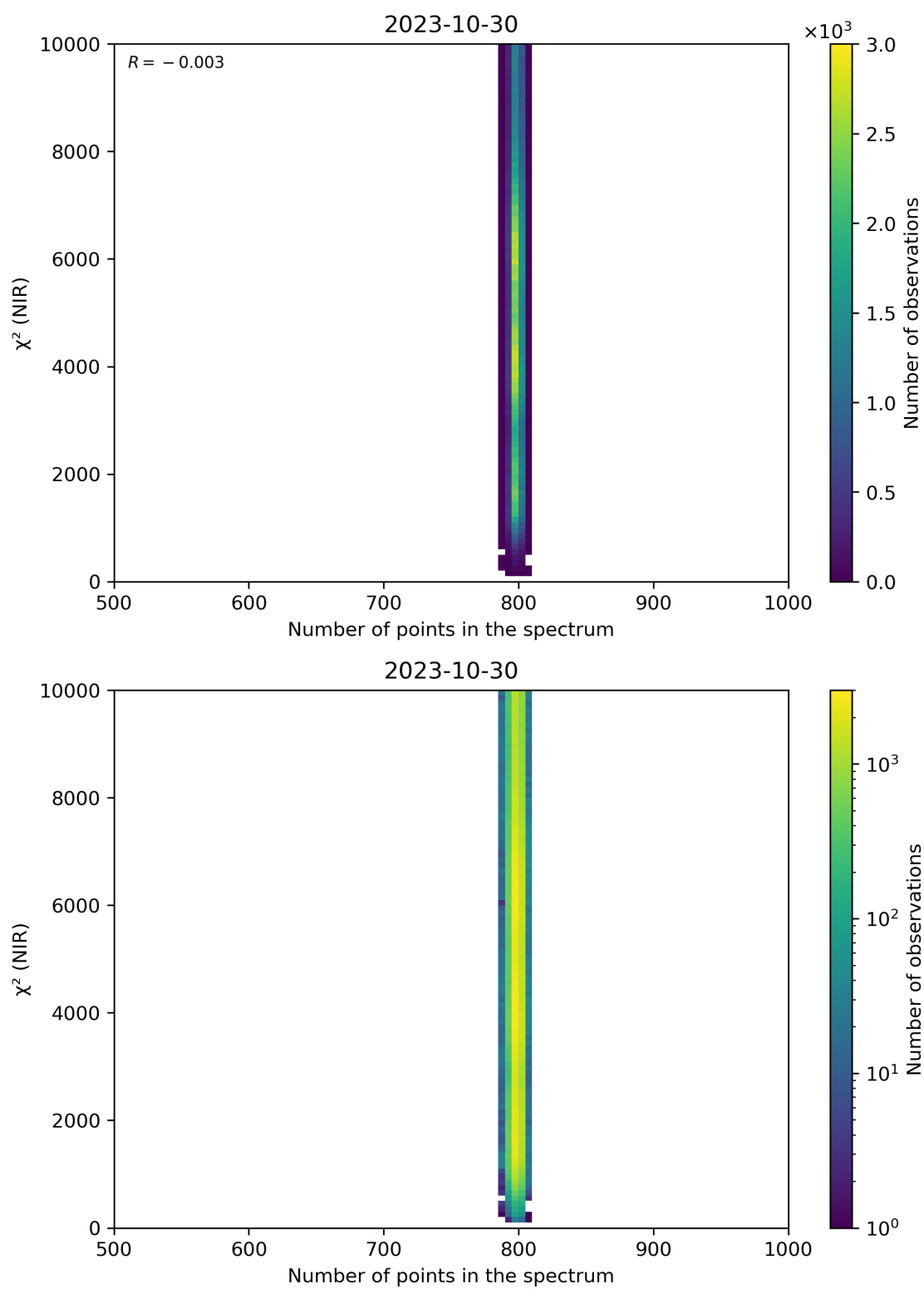
Figure 88: Scatter density plot of “Number of points in the spectrum” against “ \chi^2 (NIR)” for 2023-10-29 to 2023-10-31.
