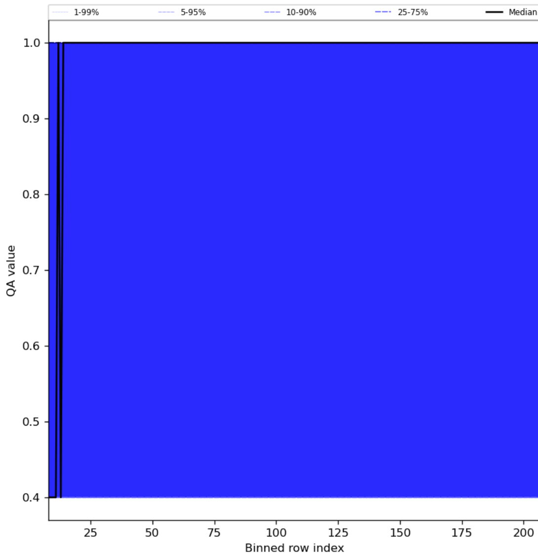
Figure 33: Along track statistics of “QA value” for 2023-10-29 to 2023-10-31
