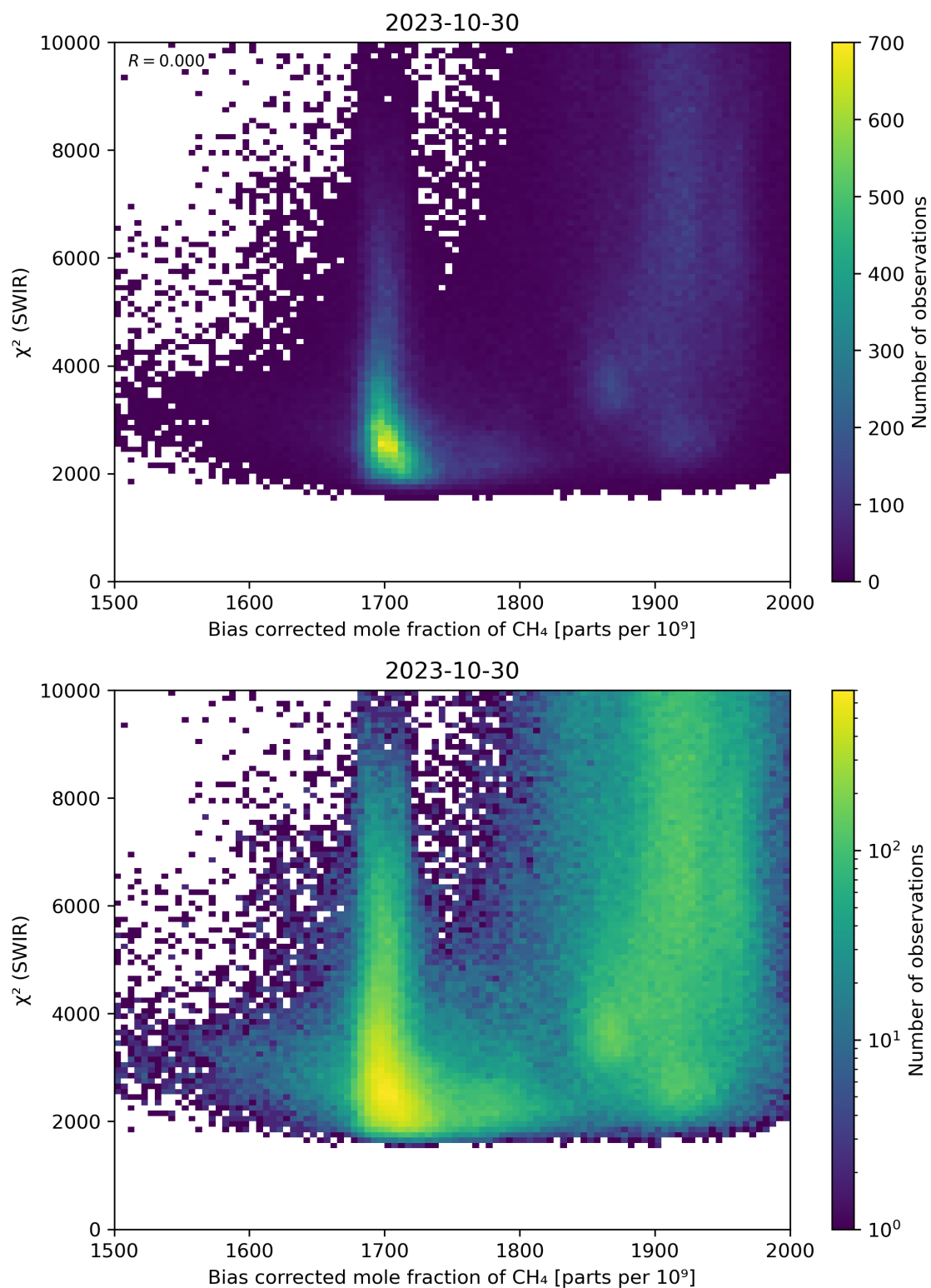
Figure 64: Scatter density plot of “Bias corrected mole fraction of CH 4 ” against “ \chi^2 (SWIR)” for 2023-10-29 to 2023-10-31.
