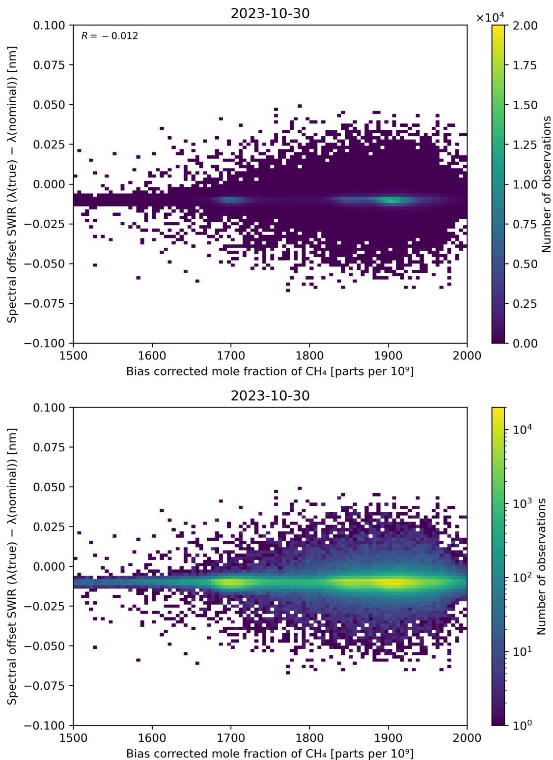
Figure 69: Scatter density plot of “Bias corrected mole fraction of \text{CH}_4 ” against “Spectral offset SWIR ( \lambda(\text{true}) - \lambda(\text{nominal}) )” for 2023-10-29 to 2023-10-31.
