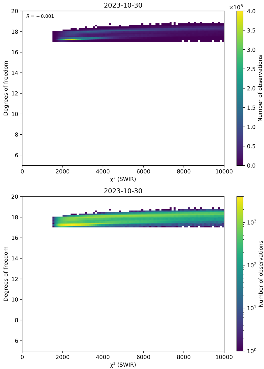
Figure 48: Scatter density plot of “ \chi^2 (SWIR)” against “Degrees of freedom” for 2023-10-29 to 2023-10-31.
