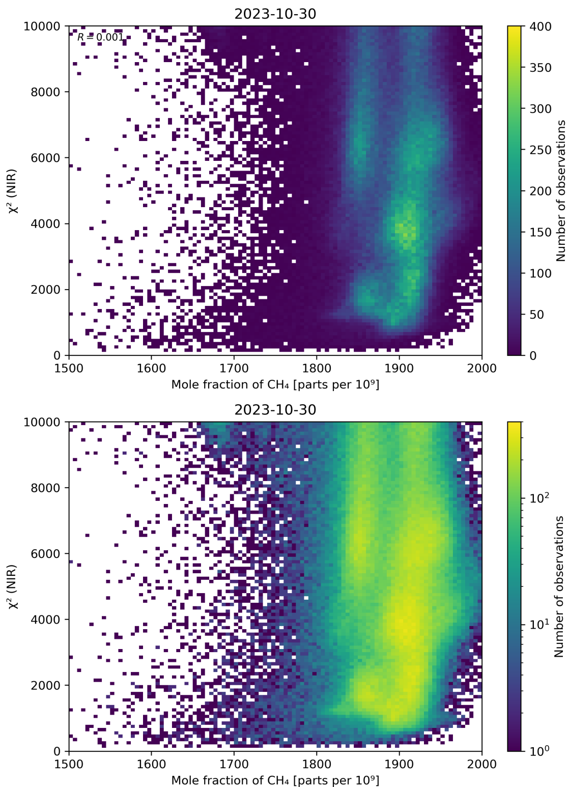
Figure 70: Scatter density plot of “Mole fraction of CH 4 ” against “ \chi^2 (NIR)” for 2023-10-29 to 2023-10-31.
