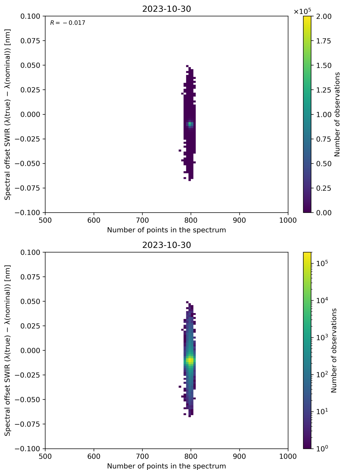
Figure 93: Scatter density plot of “Number of points in the spectrum” against “Spectral offset SWIR ( \lambda(\text{true}) - \lambda(\text{nominal}) )” for 2023-10-29 to 2023-10-31.
