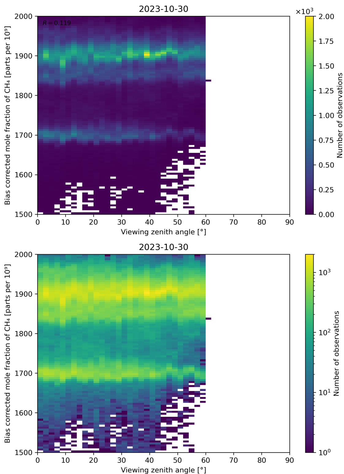
Figure 111: Scatter density plot of “Viewing zenith angle” against “Bias corrected mole fraction of CH 4 ” for 2023-10-29 to 2023-10-31.
