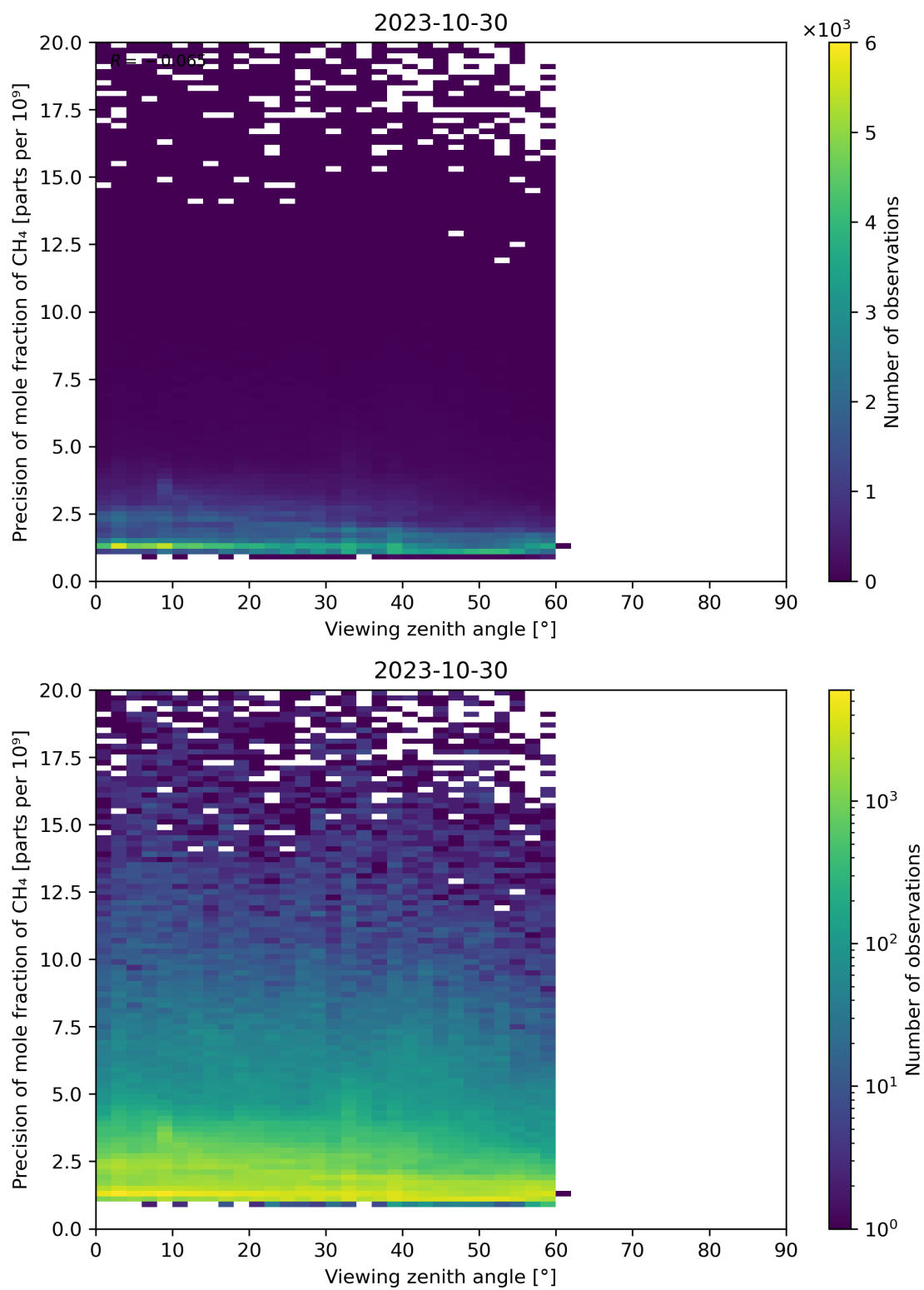
Figure 112: Scatter density plot of “Viewing zenith angle” against “Precision of mole fraction of CH 4 ” for 2023-10-29 to 2023-10-31.
