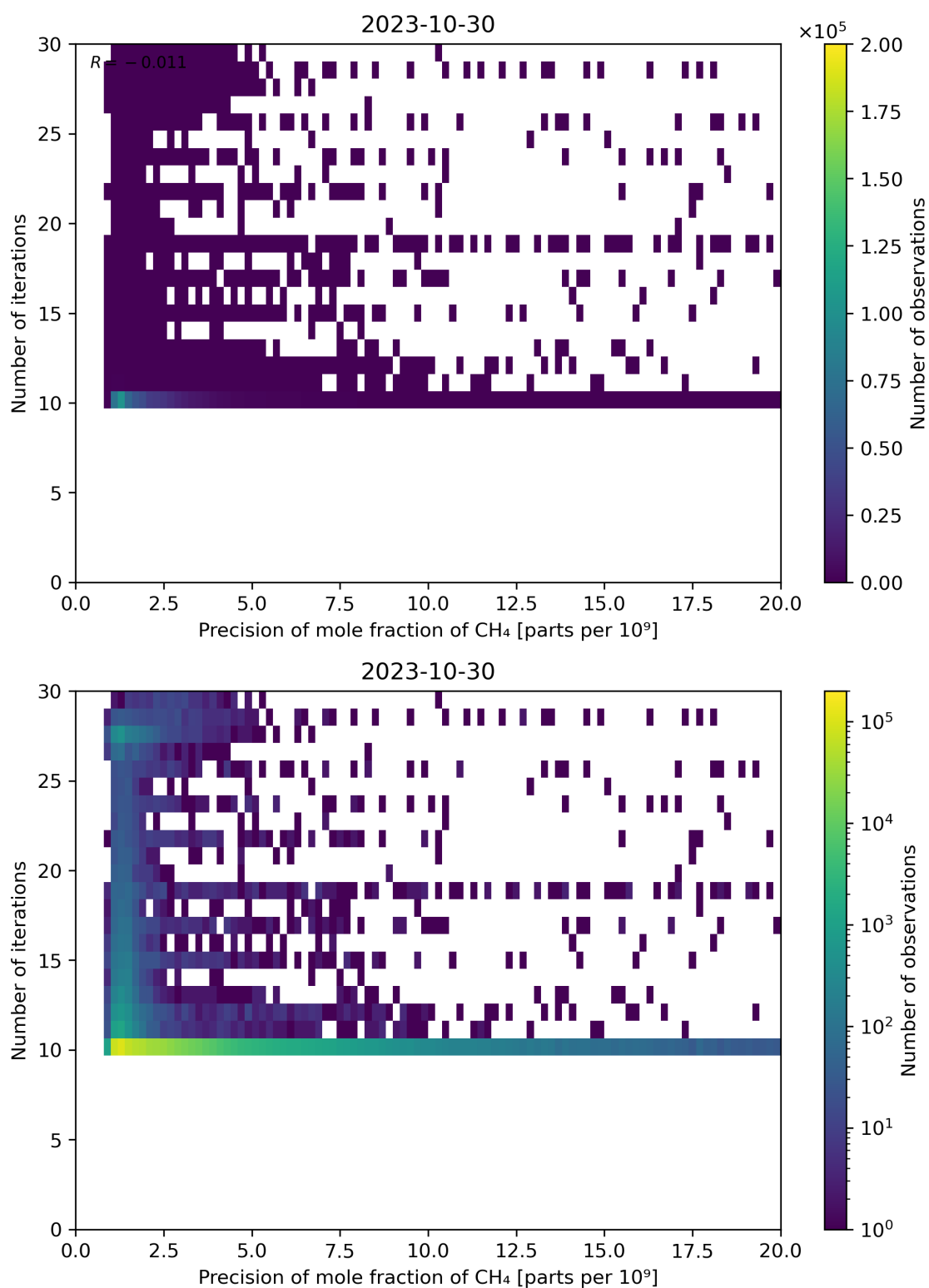
Figure 83: Scatter density plot of “Precision of mole fraction of CH 4 ” against “Number of iterations” for 2023-10-29 to 2023-10-31.
