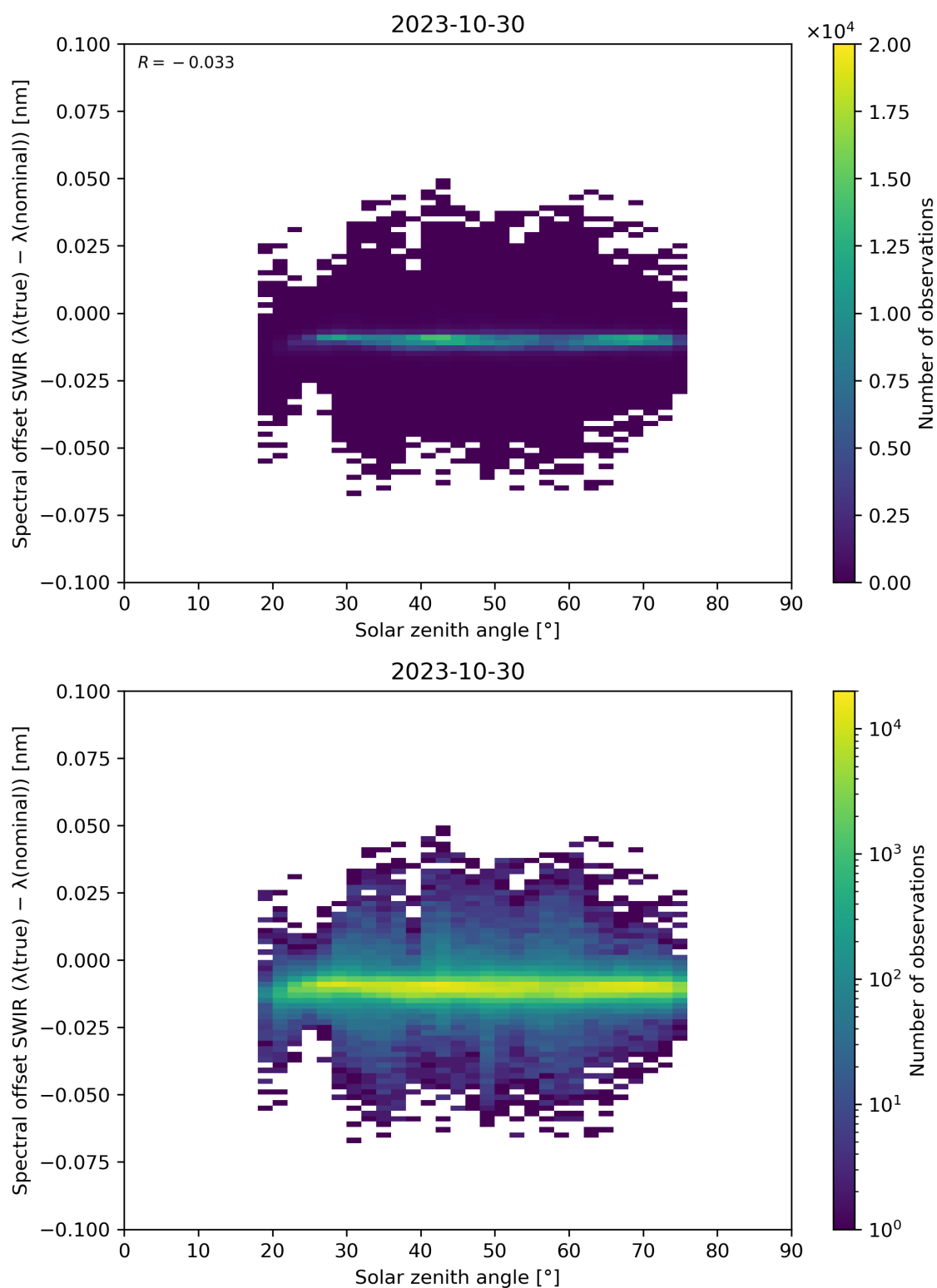
Figure 104: Scatter density plot of “Solar zenith angle” against “Spectral offset SWIR ( \lambda(\text{true}) - \lambda(\text{nominal}) )” for 2023-10-29 to 2023-10-31.
