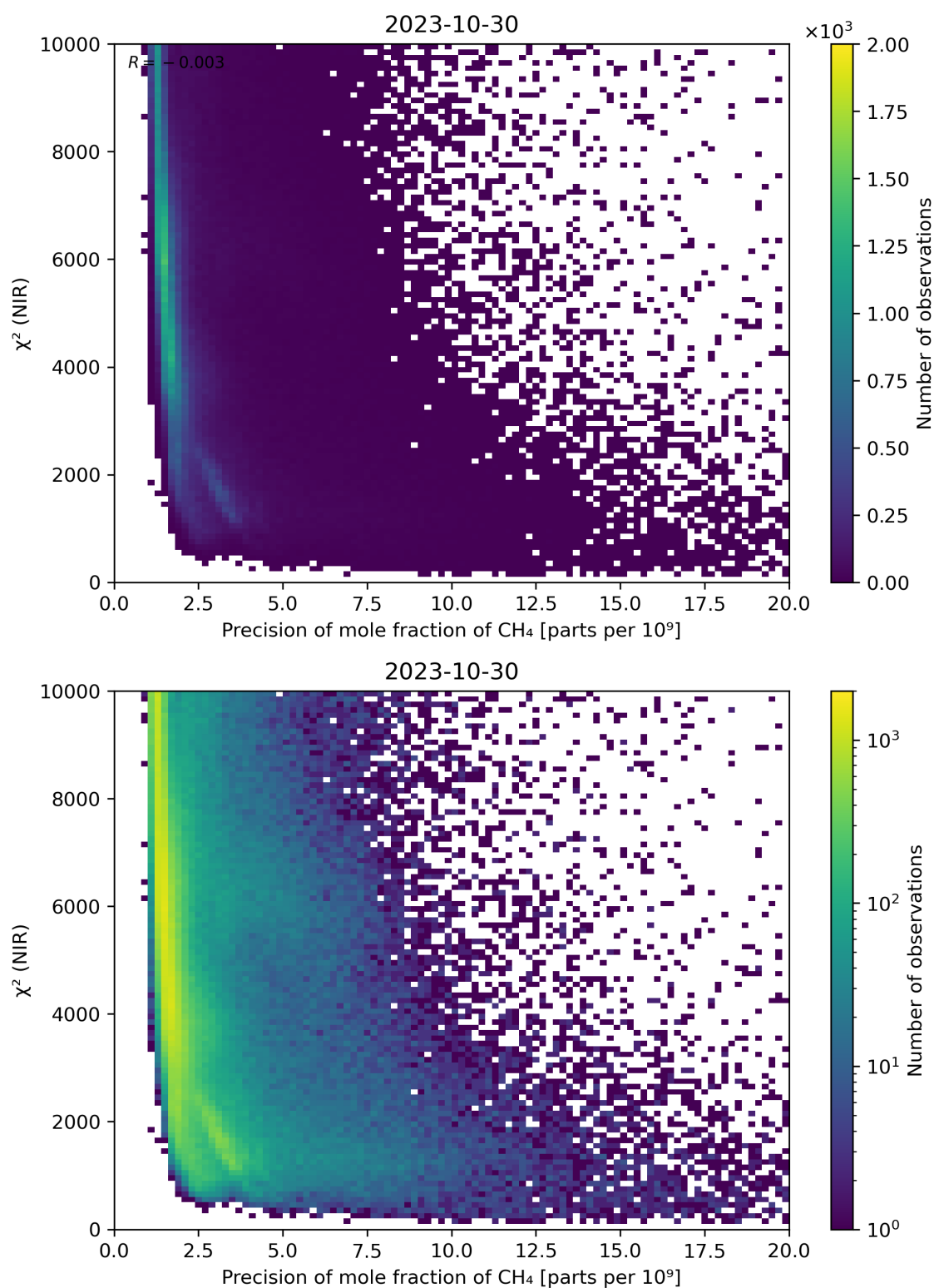
Figure 78: Scatter density plot of “Precision of mole fraction of \text{CH}_4 ” against “ \chi^2 (NIR)” for 2023-10-29 to 2023-10-31.
