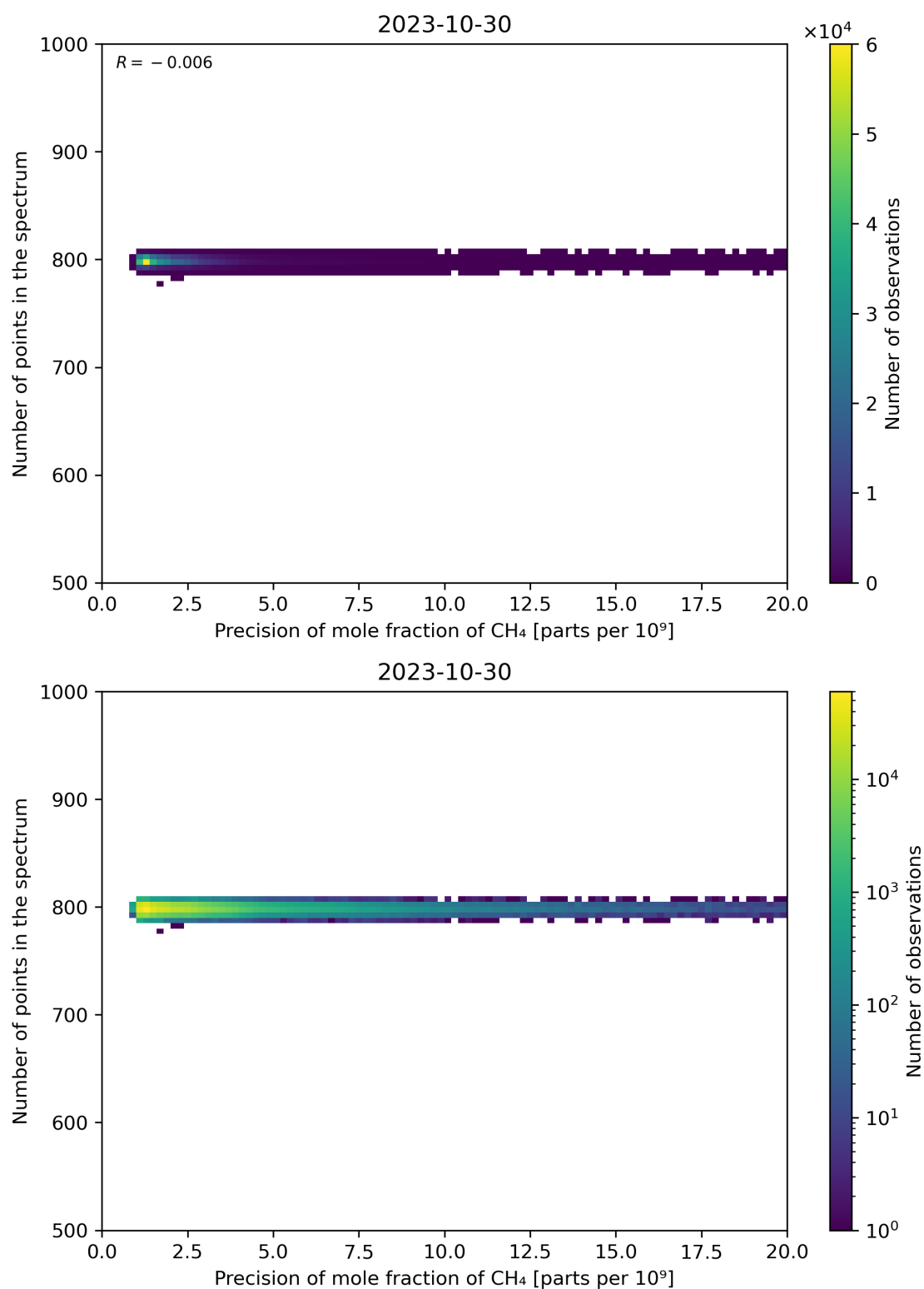
Figure 84: Scatter density plot of “Precision of mole fraction of CH 4 ” against “Number of points in the spectrum” for 2023-10-29 to 2023-10-31.
