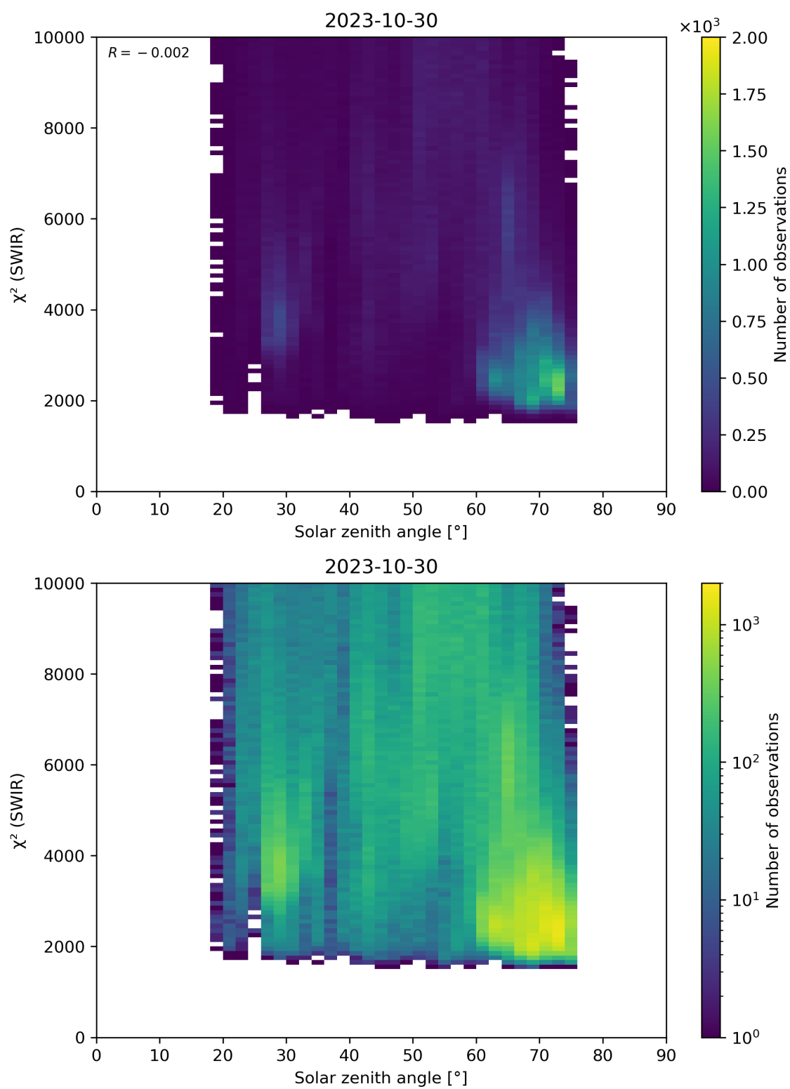
Figure 95: Scatter density plot of “Solar zenith angle” against “ \chi^2 (SWIR)” for 2023-10-29 to 2023-10-31.
