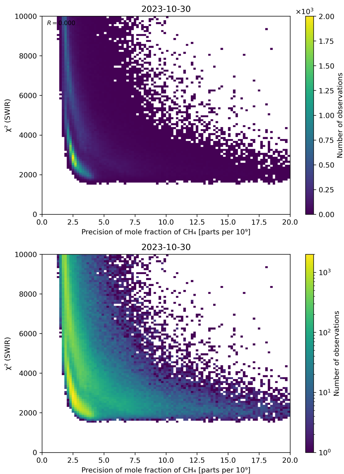
Figure 79: Scatter density plot of “Precision of mole fraction of \text{CH}_4 ” against “ \chi^2 (SWIR)” for 2023-10-29 to 2023-10-31.
