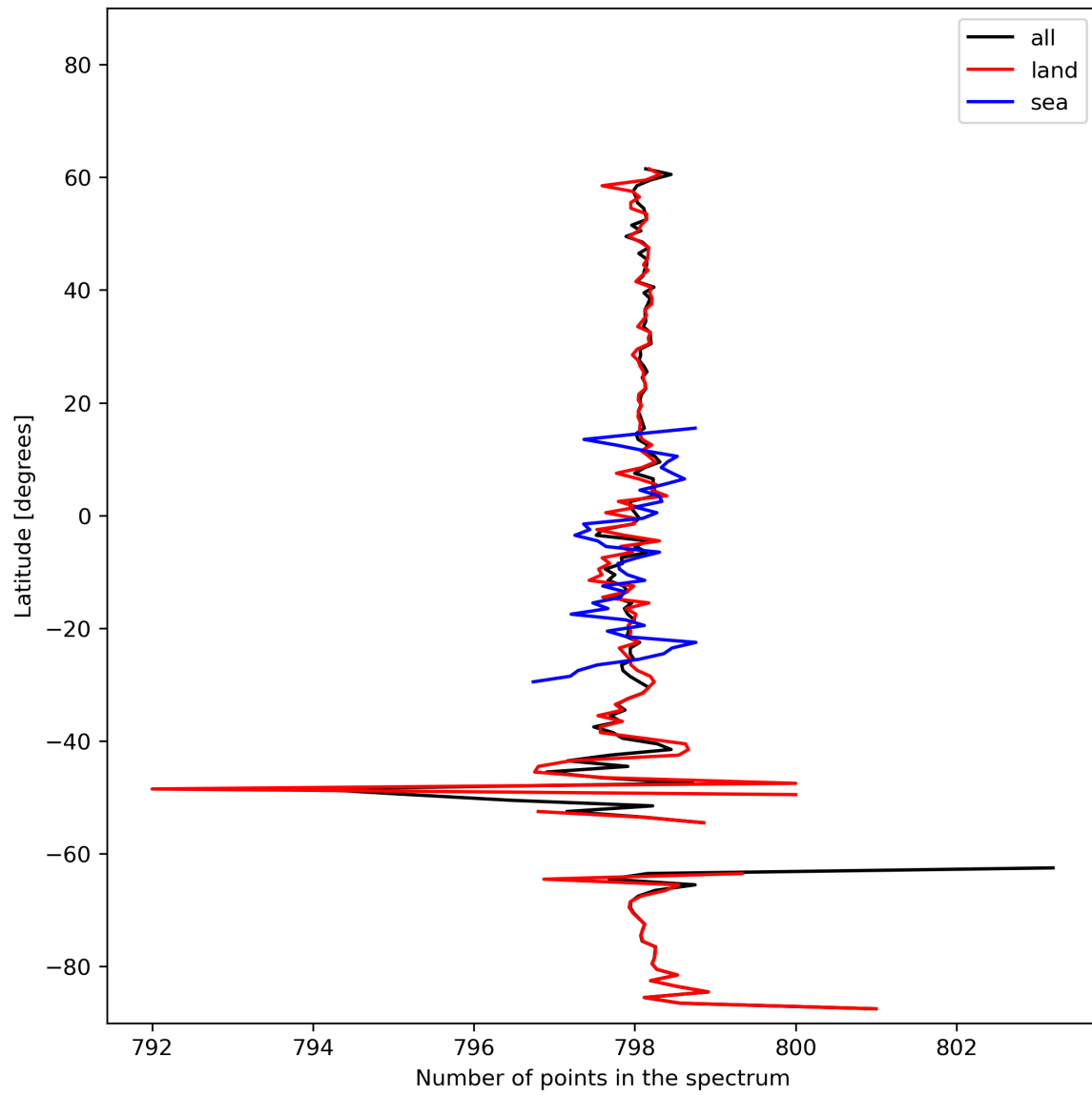
Figure 15: Zonal average of “Number of points in the spectrum” for 2023-10-29 to 2023-10-31.
