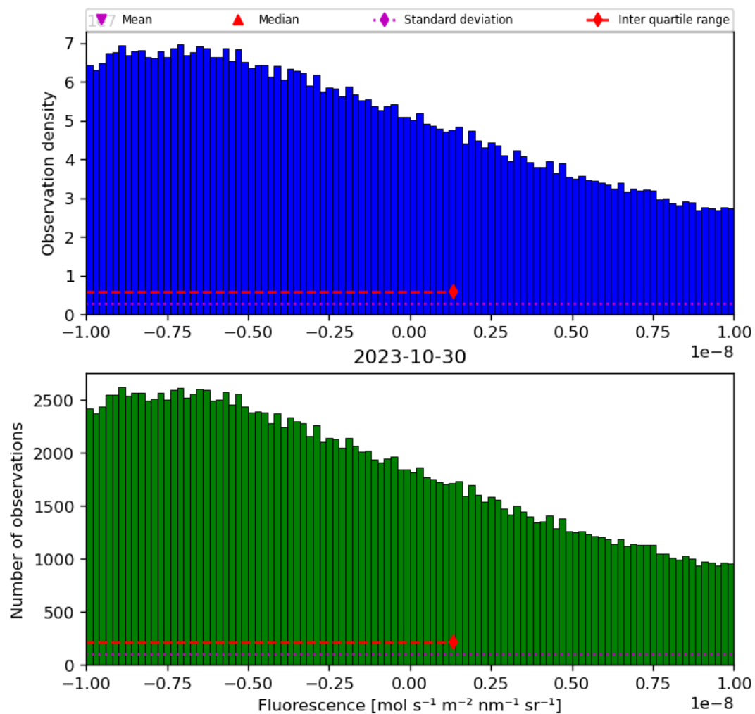
Figure 32: Histogram of “Fluorescence” for 2023-10-29 to 2023-10-31
