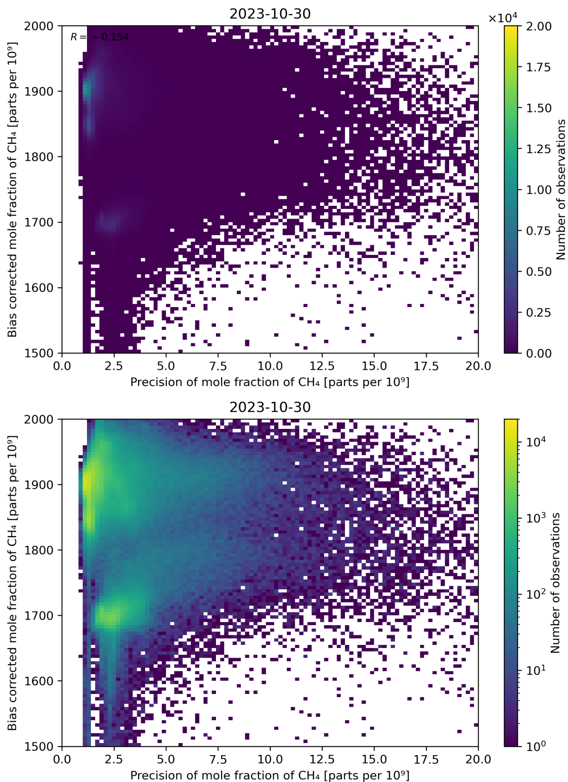
Figure 82: Scatter density plot of “Precision of mole fraction of CH 4 ” against “Bias corrected mole fraction of CH 4 ” for 2023-10-29 to 2023-10-31.
