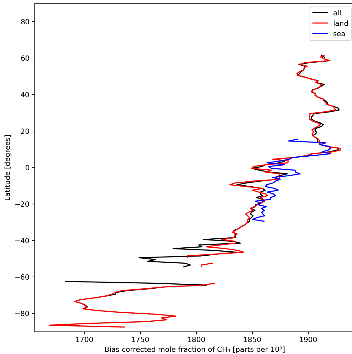
Figure 14: Zonal average of “Bias corrected mole fraction of CH 4 ” for 2023-10-29 to 2023-10-31.
