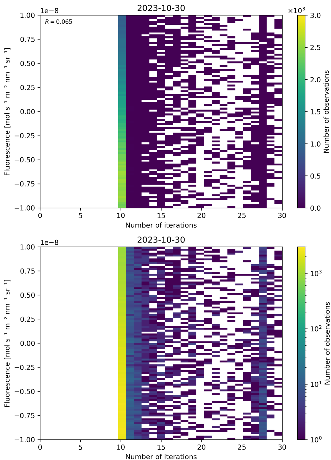
Figure 87: Scatter density plot of “Number of iterations” against “Fluorescence” for 2023-10-29 to 2023-10-31.
