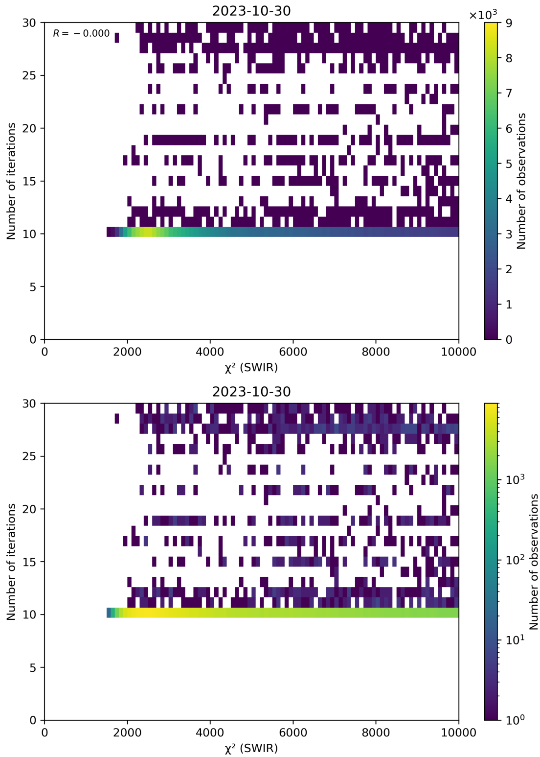
Figure 50: Scatter density plot of “ \chi^2 (SWIR)” against “Number of iterations” for 2023-10-29 to 2023-10-31.
