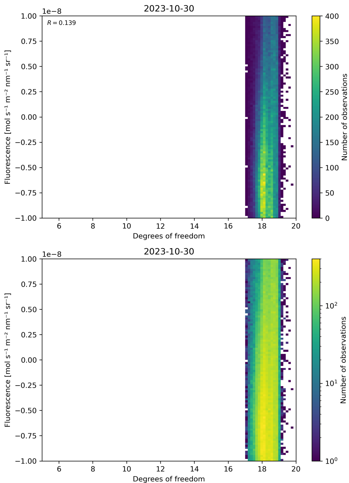
Figure 51: Scatter density plot of “Degrees of freedom” against “Fluorescence” for 2023-10-29 to 2023-10-31.
