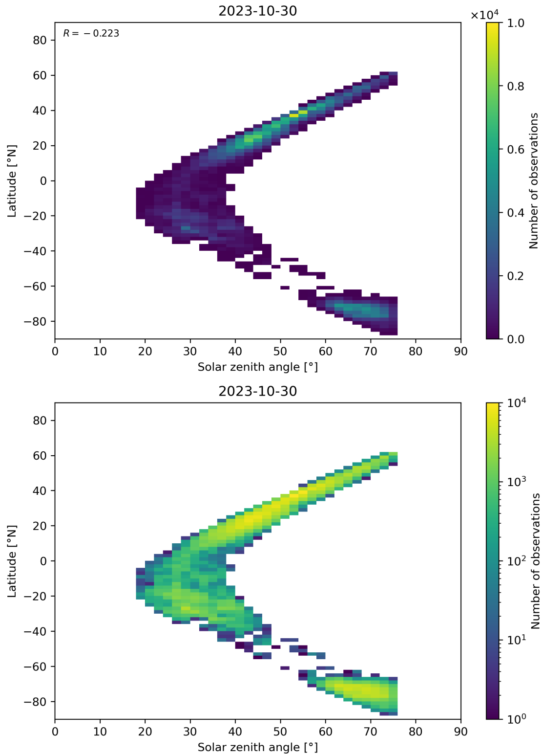
Figure 98: Scatter density plot of “Solar zenith angle” against “Latitude” for 2023-10-29 to 2023-10-31.
