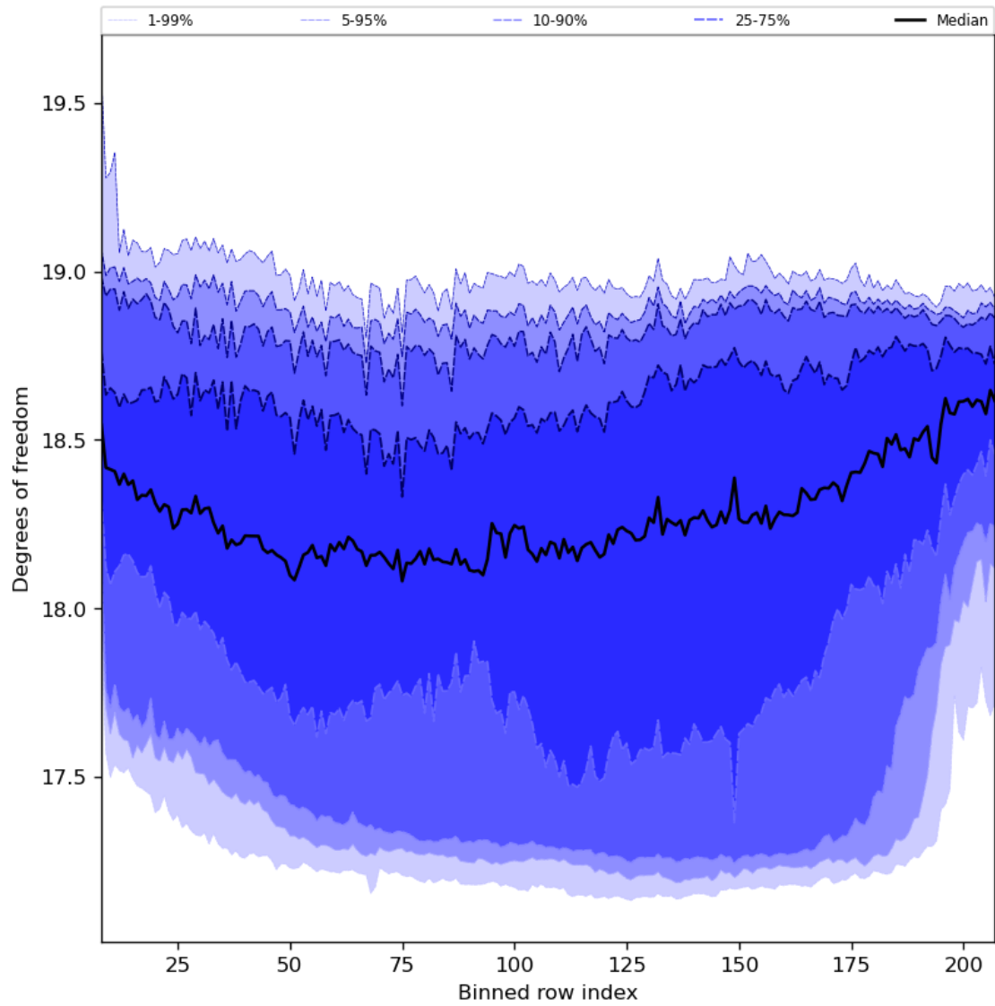
Figure 41: Along track statistics of “Degrees of freedom” for 2023-10-29 to 2023-10-31
