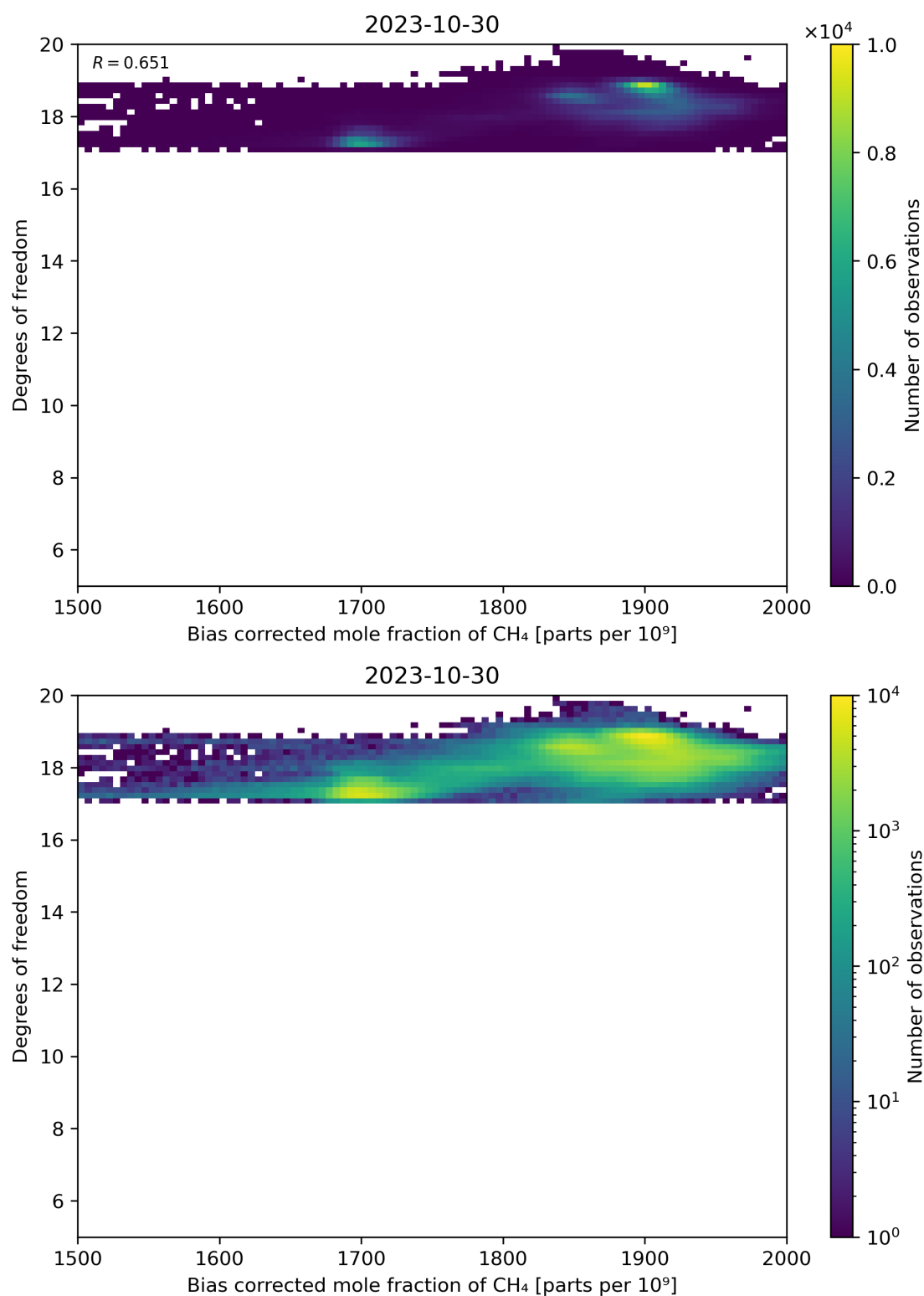
Figure 65: Scatter density plot of “Bias corrected mole fraction of CH 4 ” against “Degrees of freedom” for 2023-10-29 to 2023-10-31.
