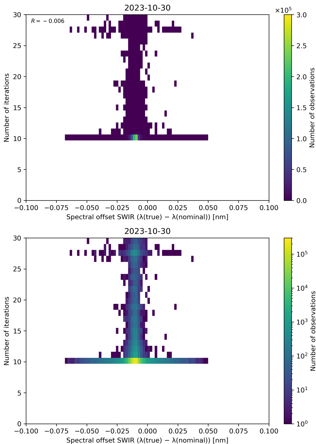
Figure 121: Scatter density plot of “Spectral offset SWIR ( \lambda(\text{true}) - \lambda(\text{nominal}) )” against “Number of iterations” for 2023-10-29 to 2023-10-31.
