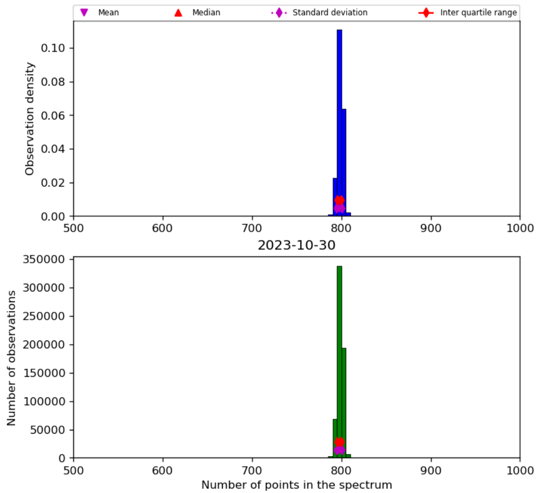
Figure 26: Histogram of “Number of points in the spectrum” for 2023-10-29 to 2023-10-31
