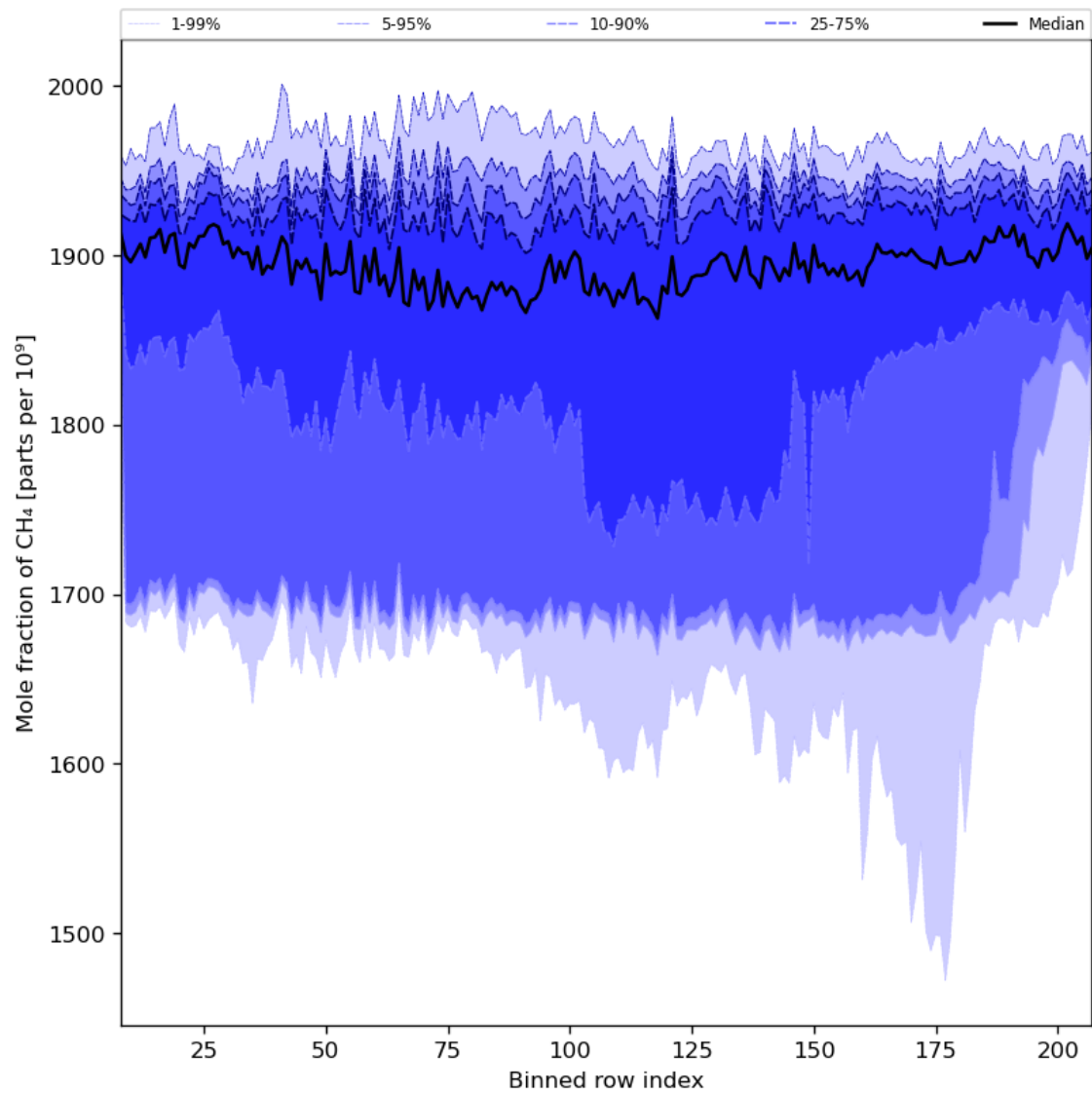
Figure 34: Along track statistics of “Mole fraction of CH 4 ” for 2023-10-29 to 2023-10-31
