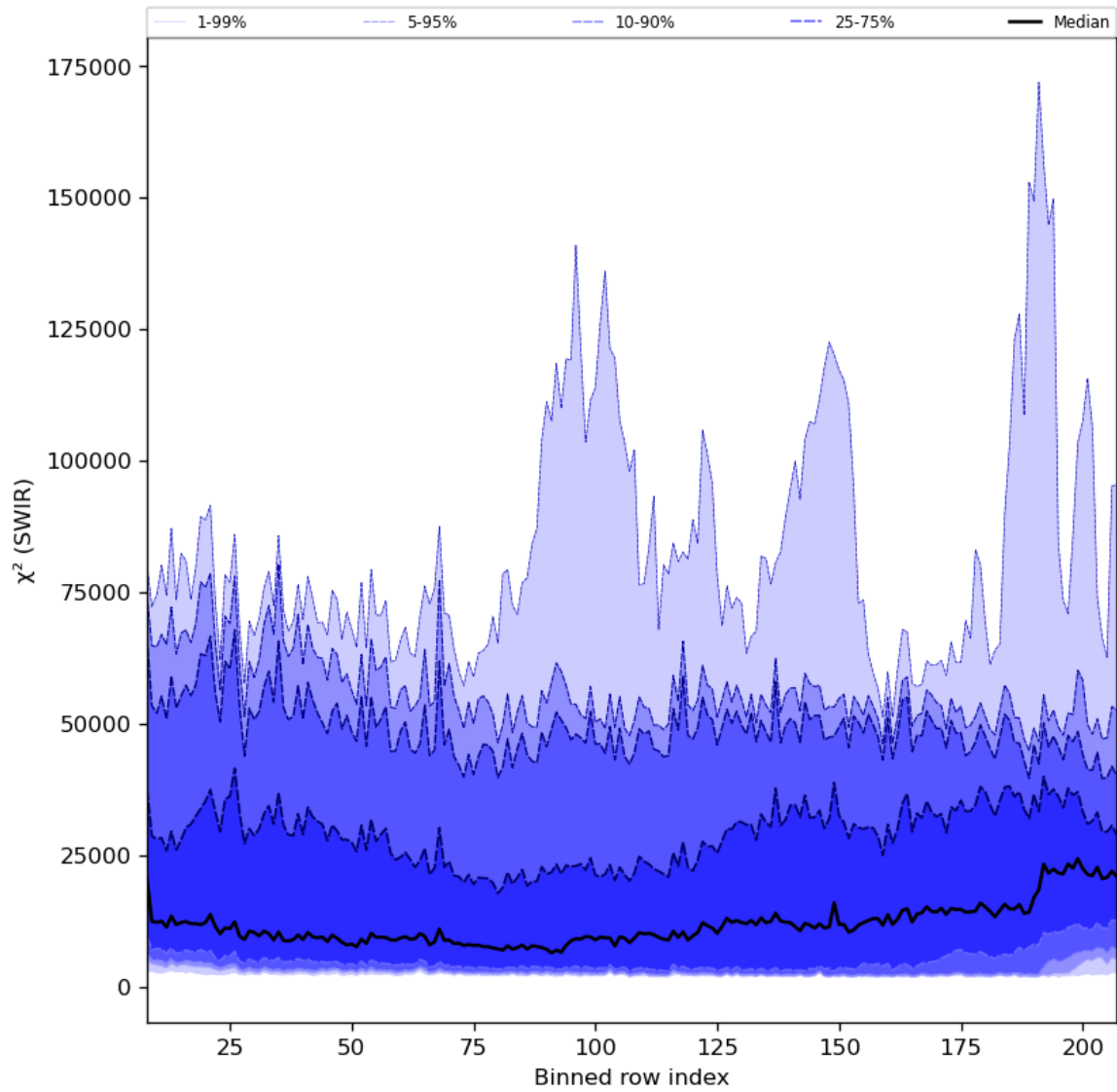
Figure 39: Along track statistics of " \chi^2 (SWIR)" for 2023-10-29 to 2023-10-31
