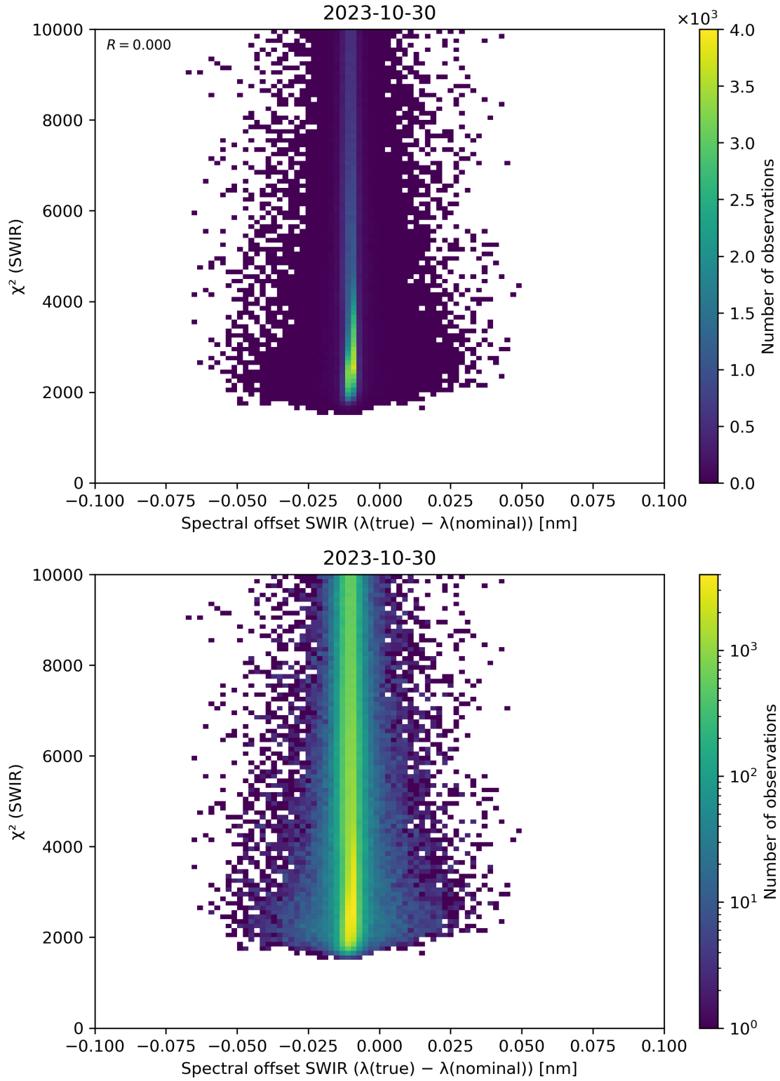
Figure 118: Scatter density plot of “Spectral offset SWIR ( \lambda(\text{true}) - \lambda(\text{nominal}) )” against “ \chi^2 (SWIR)” for 2023-10-29 to 2023-10-31.
