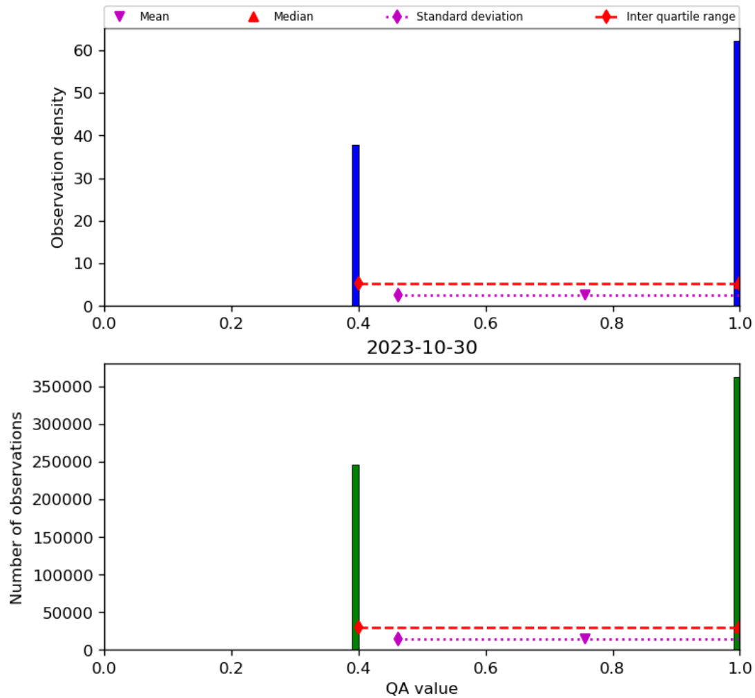
Figure 22: Histogram of “QA value” for 2023-10-29 to 2023-10-31
