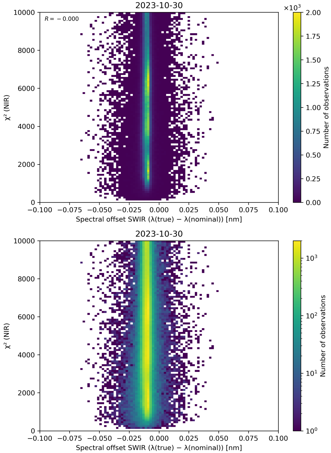
Figure 117: Scatter density plot of “Spectral offset SWIR ( \lambda(\text{true}) - \lambda(\text{nominal}) )” against “ \chi^2 (NIR)” for 2023-10-29 to 2023-10-31.
