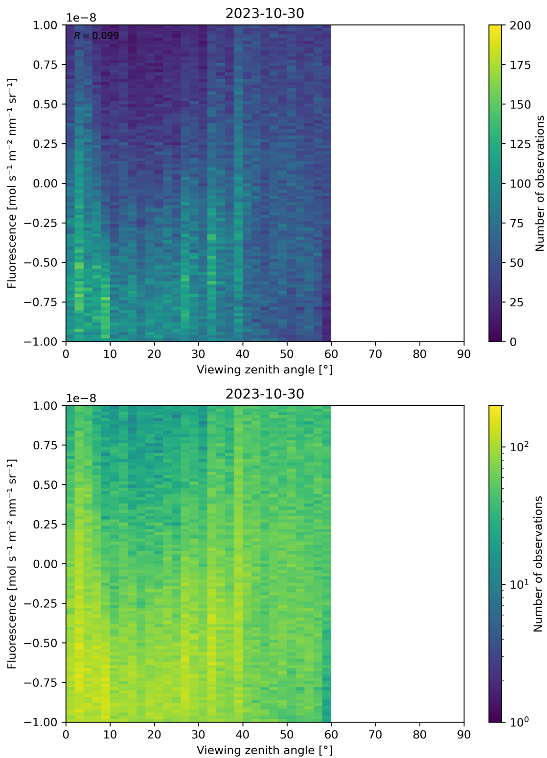
Figure 108: Scatter density plot of “Viewing zenith angle” against “Fluorescence” for 2023-10-29 to 2023-10-31.
