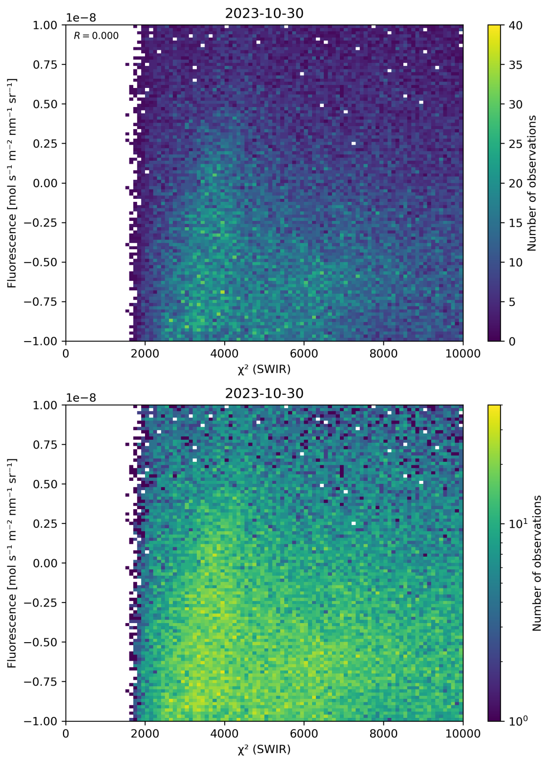
Figure 49: Scatter density plot of “ \chi^2 (SWIR)” against “Fluorescence” for 2023-10-29 to 2023-10-31.
