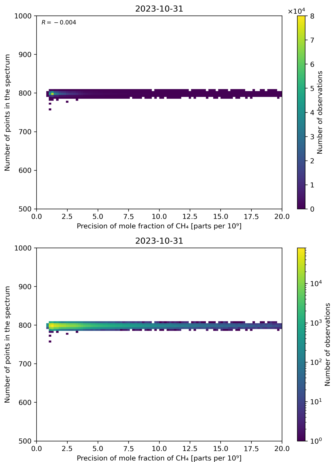
Figure 84: Scatter density plot of “Precision of mole fraction of CH 4 ” against “Number of points in the spectrum” for 2023-10-30 to 2023-11-01.
