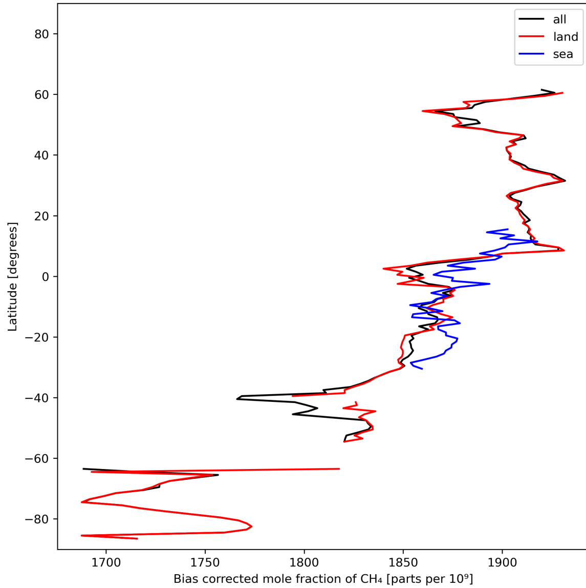
Figure 14: Zonal average of “Bias corrected mole fraction of CH 4 ” for 2023-10-30 to 2023-11-01.
