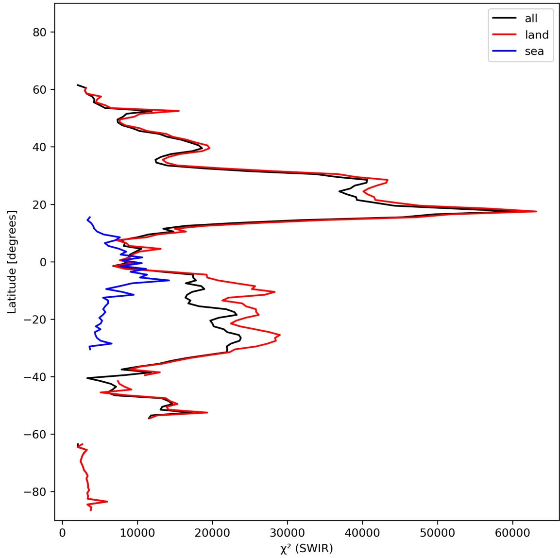
Figure 17: Zonal average of “ \chi^2 (SWIR)” for 2023-10-30 to 2023-11-01.
