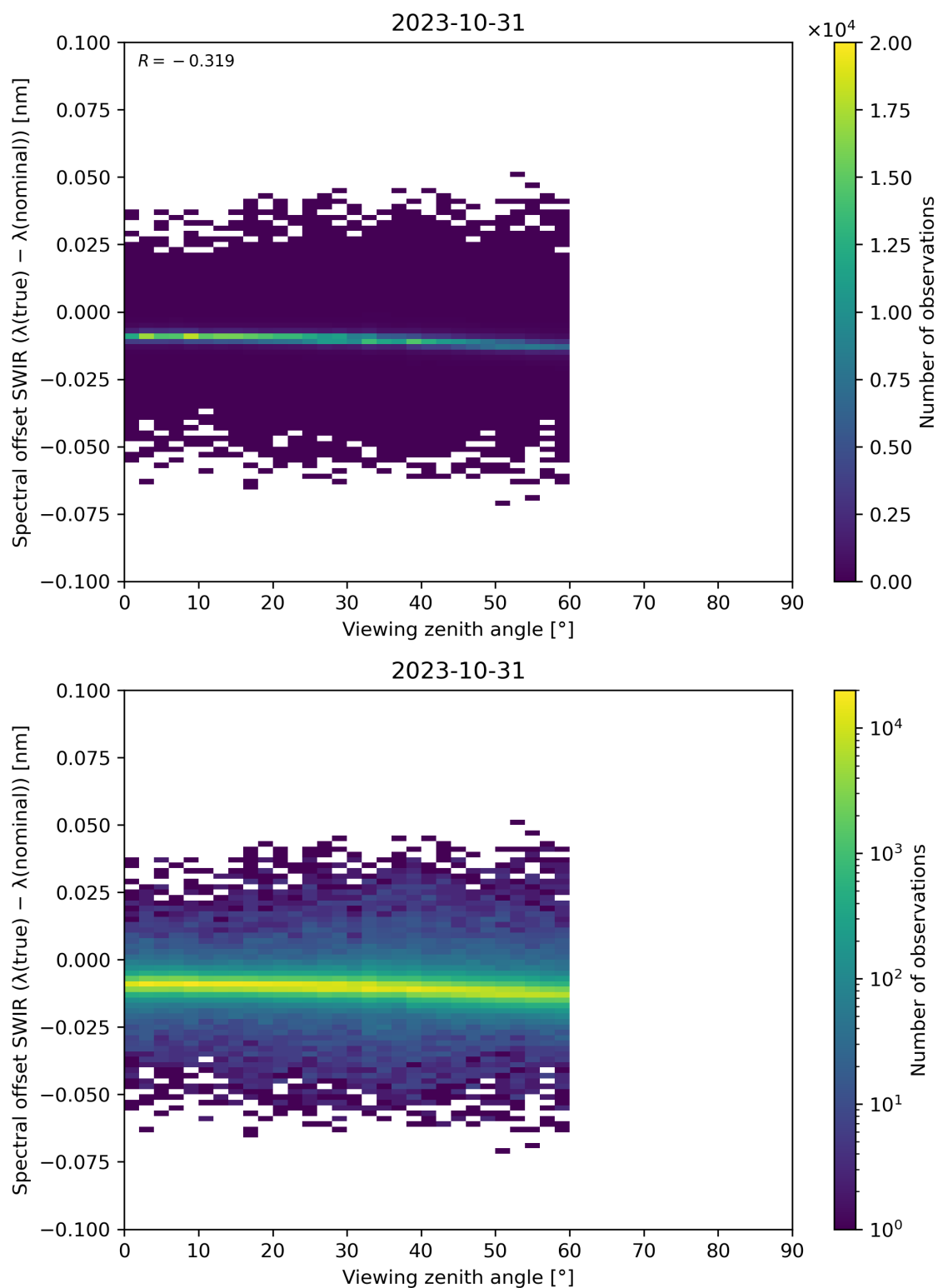
Figure 116: Scatter density plot of “Viewing zenith angle” against “Spectral offset SWIR ( \lambda(\text{true}) - \lambda(\text{nominal}) )” for 2023-10-30 to 2023-11-01.
