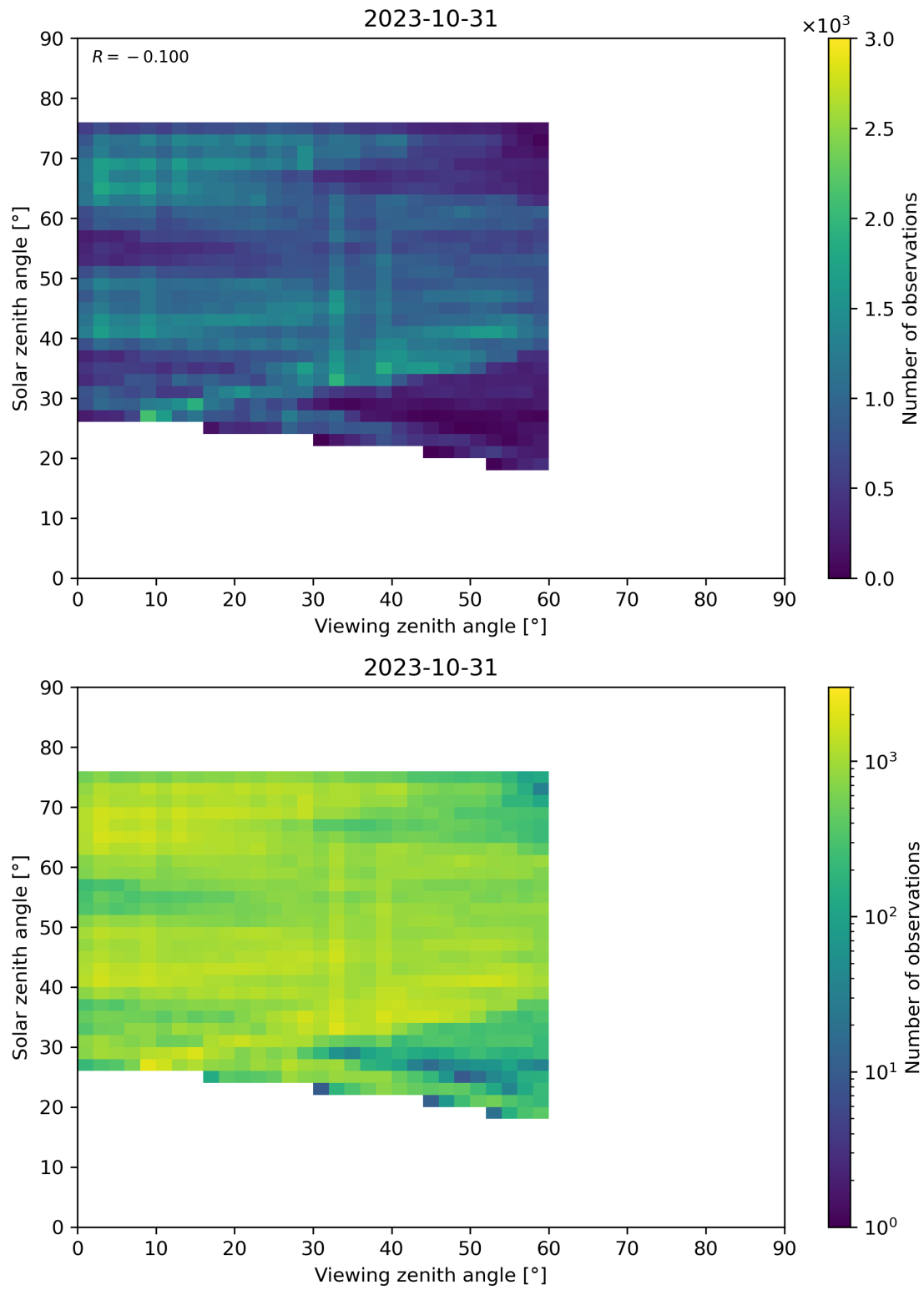
Figure 115: Scatter density plot of “Viewing zenith angle” against “Solar zenith angle” for 2023-10-30 to 2023-11-01.
