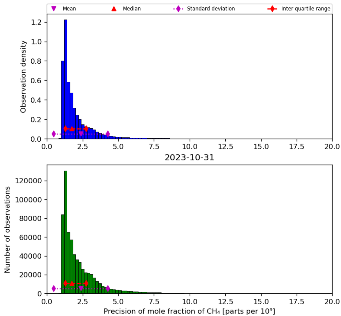
Figure 24: Histogram of “Precision of mole fraction of CH 4 ” for 2023-10-30 to 2023-11-01
