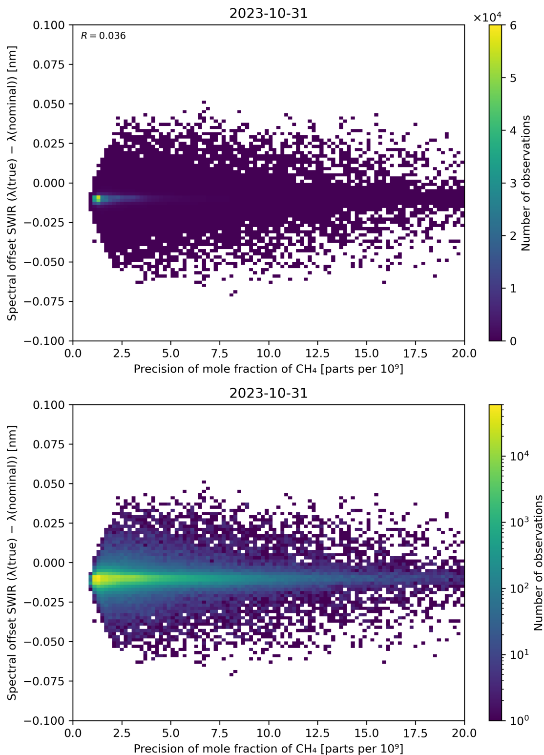
Figure 85: Scatter density plot of “Precision of mole fraction of \text{CH}_4 ” against “Spectral offset SWIR ( \lambda(\text{true}) - \lambda(\text{nominal}) )” for 2023-10-30 to 2023-11-01.
