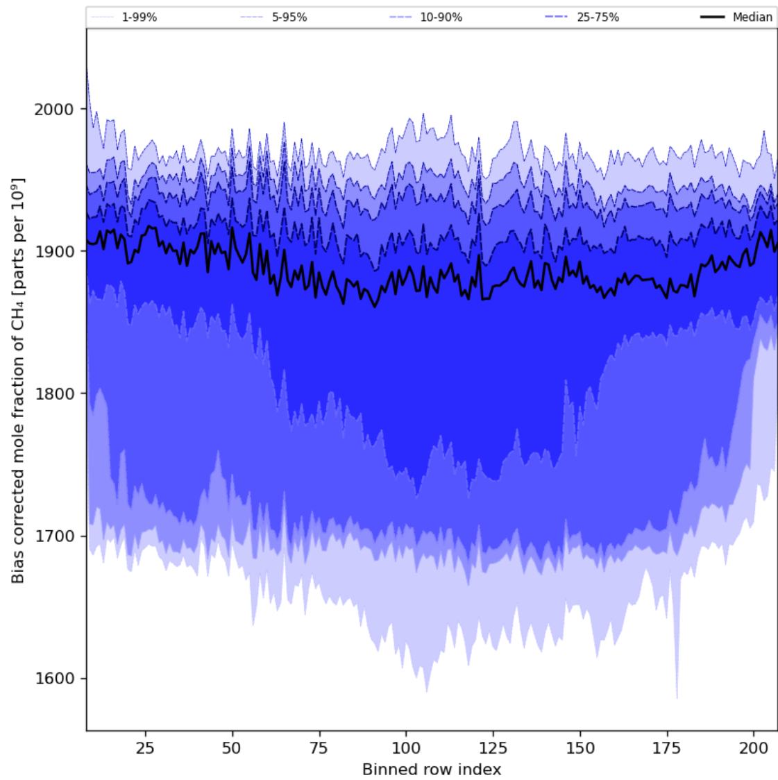
Figure 36: Along track statistics of “Bias corrected mole fraction of CH 4 ” for 2023-10-30 to 2023-11-01
