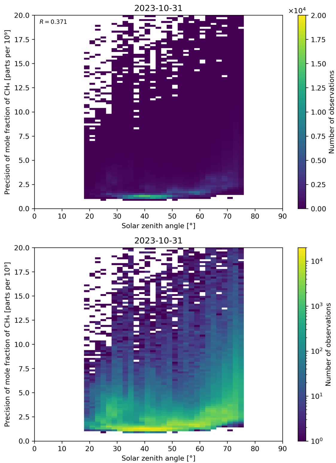
Figure 101: Scatter density plot of “Solar zenith angle” against “Precision of mole fraction of CH 4 ” for 2023-10-30 to 2023-11-01.
