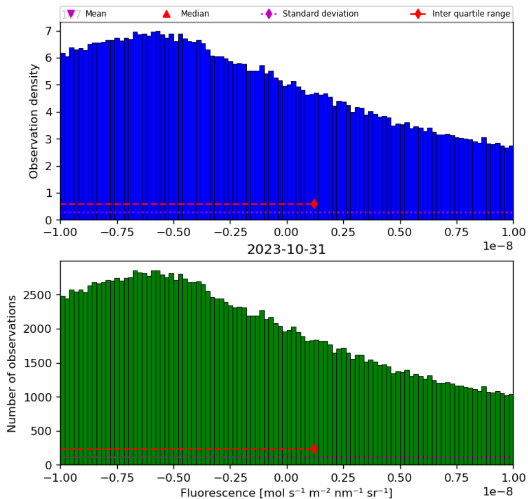
Figure 32: Histogram of “Fluorescence” for 2023-10-30 to 2023-11-01
