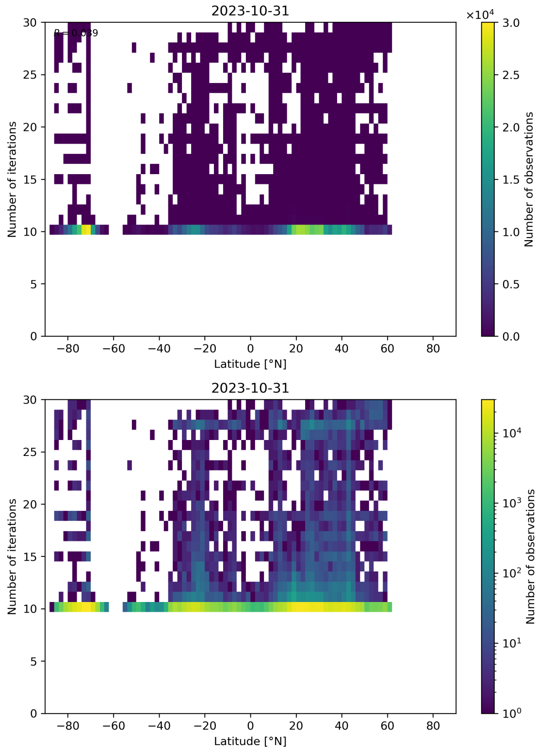
Figure 60: Scatter density plot of “Latitude” against “Number of iterations” for 2023-10-30 to 2023-11-01.
