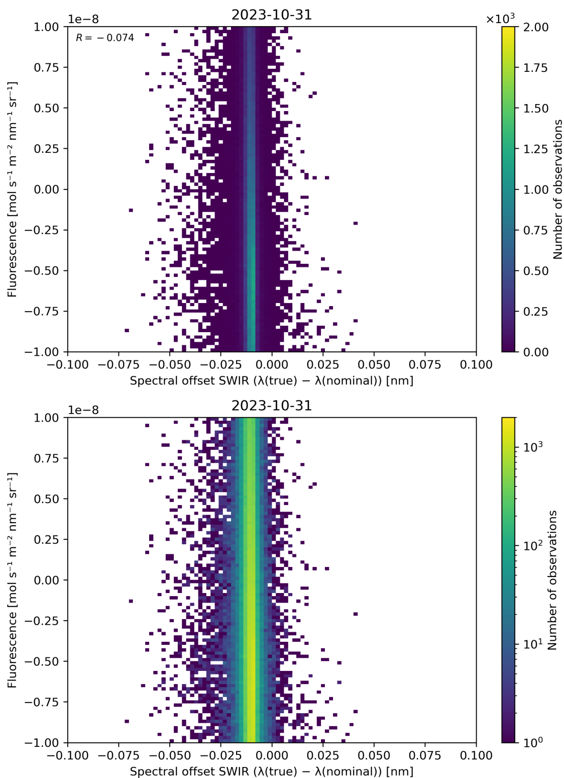
Figure 120: Scatter density plot of “Spectral offset SWIR ( \lambda(\text{true}) - \lambda(\text{nominal}) )” against “Fluorescence” for 2023-10-30 to 2023-11-01.
