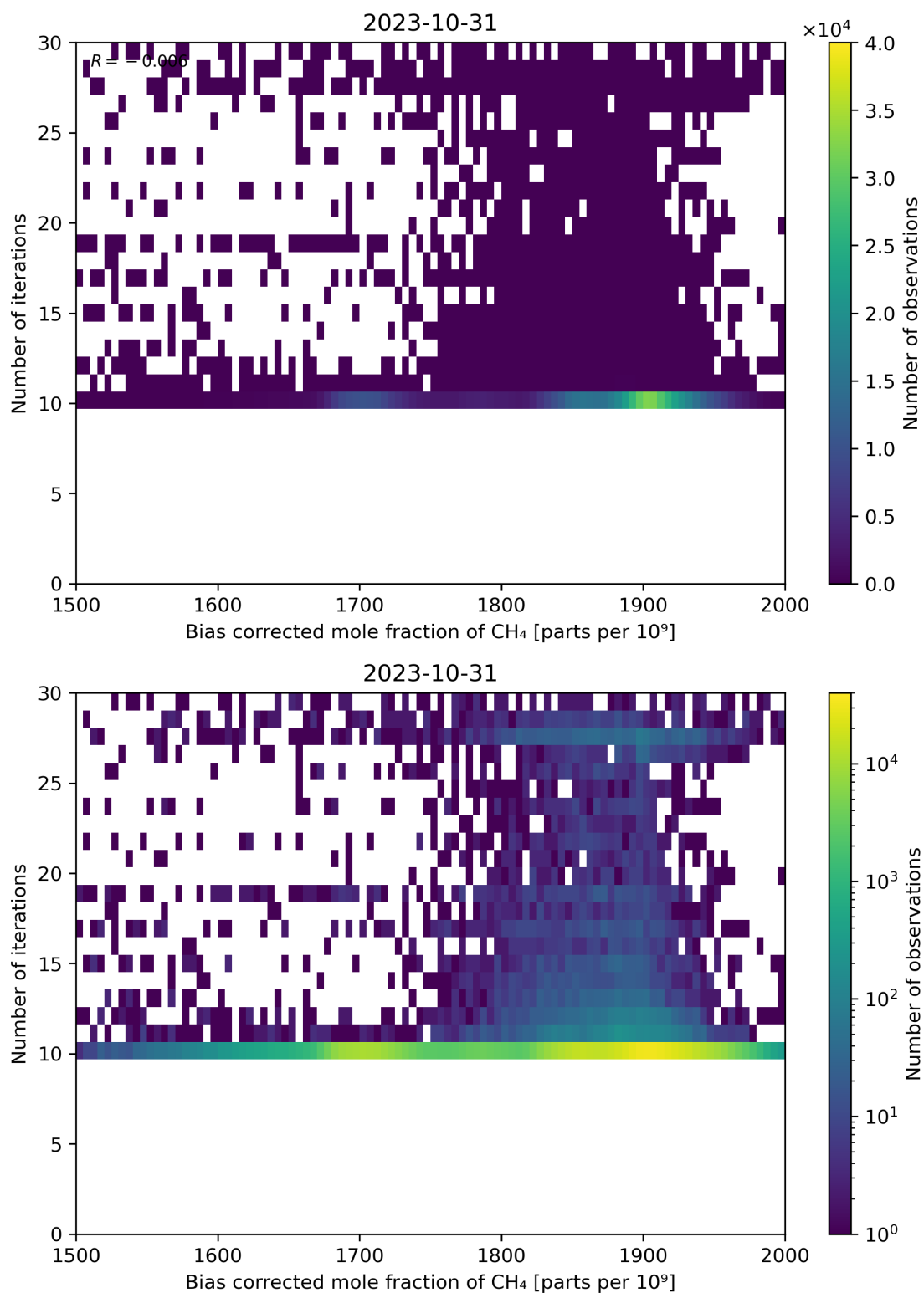
Figure 67: Scatter density plot of “Bias corrected mole fraction of \text{CH}_4 ” against “Number of iterations” for 2023-10-30 to 2023-11-01.
