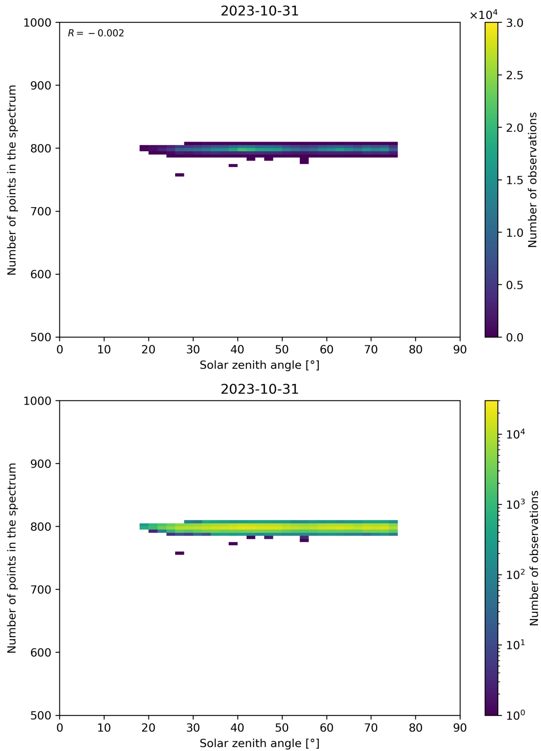
Figure 103: Scatter density plot of “Solar zenith angle” against “Number of points in the spectrum” for 2023-10-30 to 2023-11-01.
