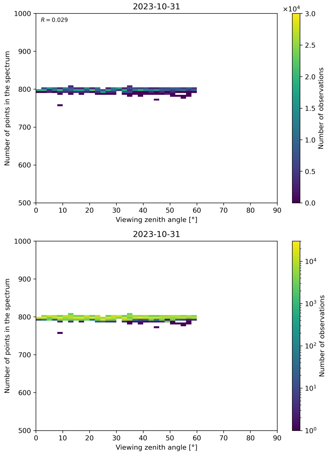
Figure 114: Scatter density plot of “Viewing zenith angle” against “Number of points in the spectrum” for 2023-10-30 to 2023-11-01.
