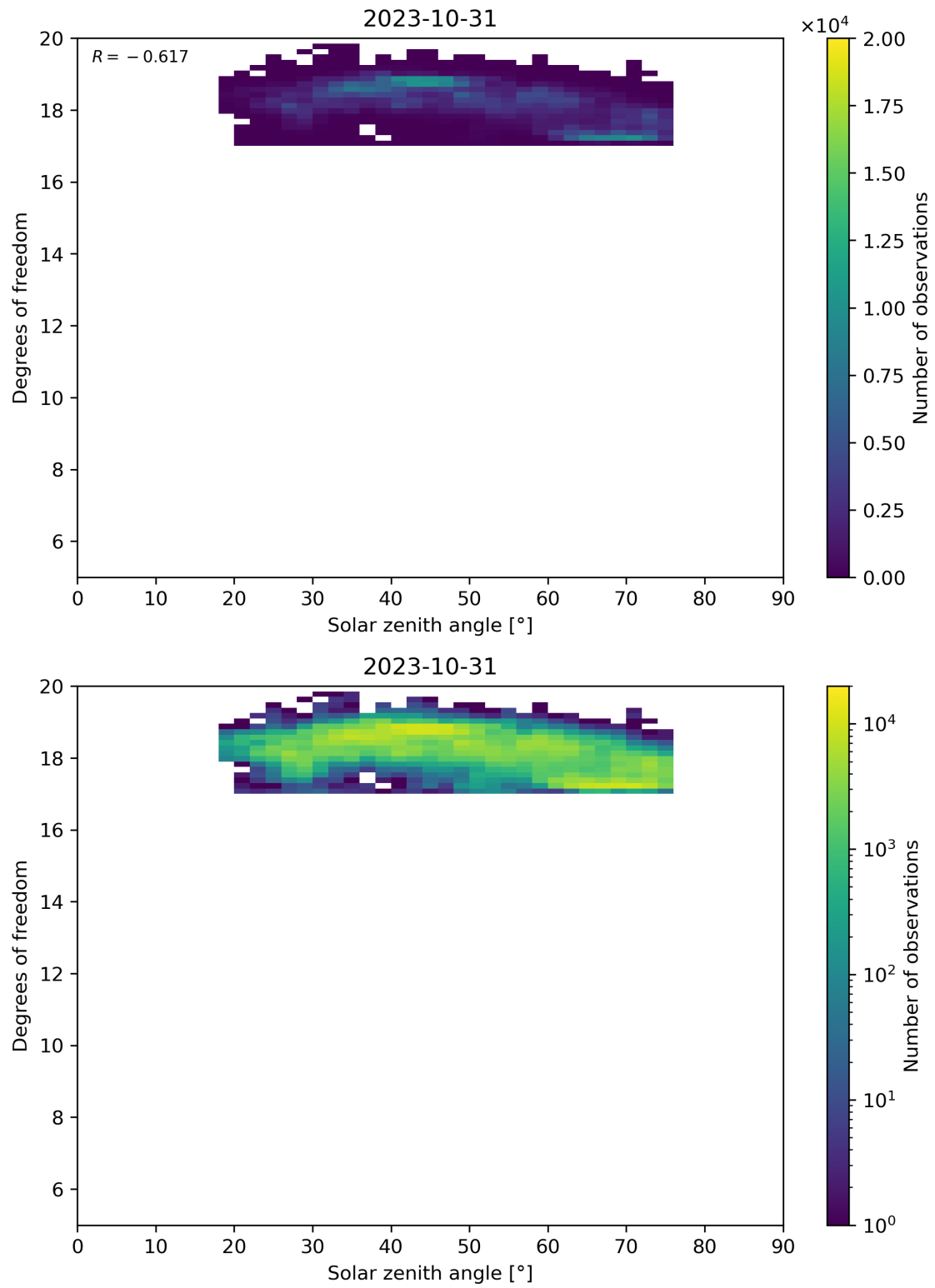
Figure 96: Scatter density plot of “Solar zenith angle” against “Degrees of freedom” for 2023-10-30 to 2023-11-01.
