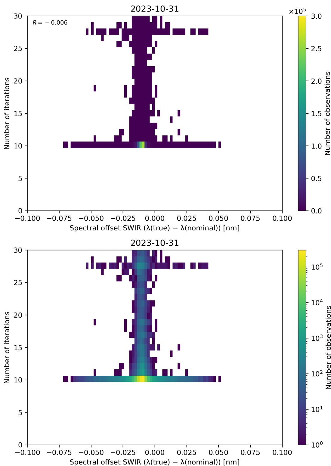
Figure 121: Scatter density plot of “Spectral offset SWIR ( \lambda(\text{true}) - \lambda(\text{nominal}) )” against “Number of iterations” for 2023-10-30 to 2023-11-01.
