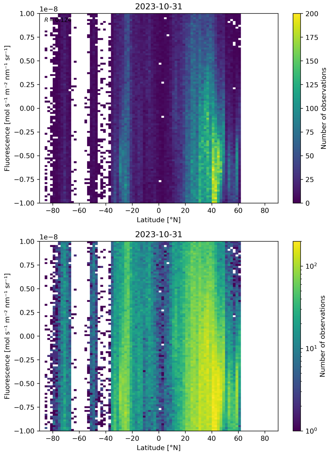
Figure 56: Scatter density plot of “Latitude” against “Fluorescence” for 2023-10-30 to 2023-11-01.
