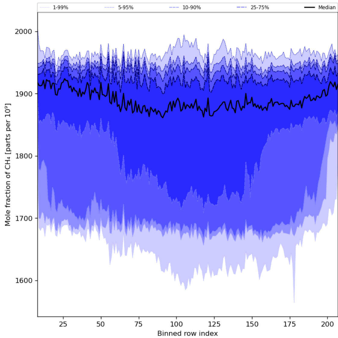
Figure 34: Along track statistics of “Mole fraction of CH 4 ” for 2023-10-30 to 2023-11-01
