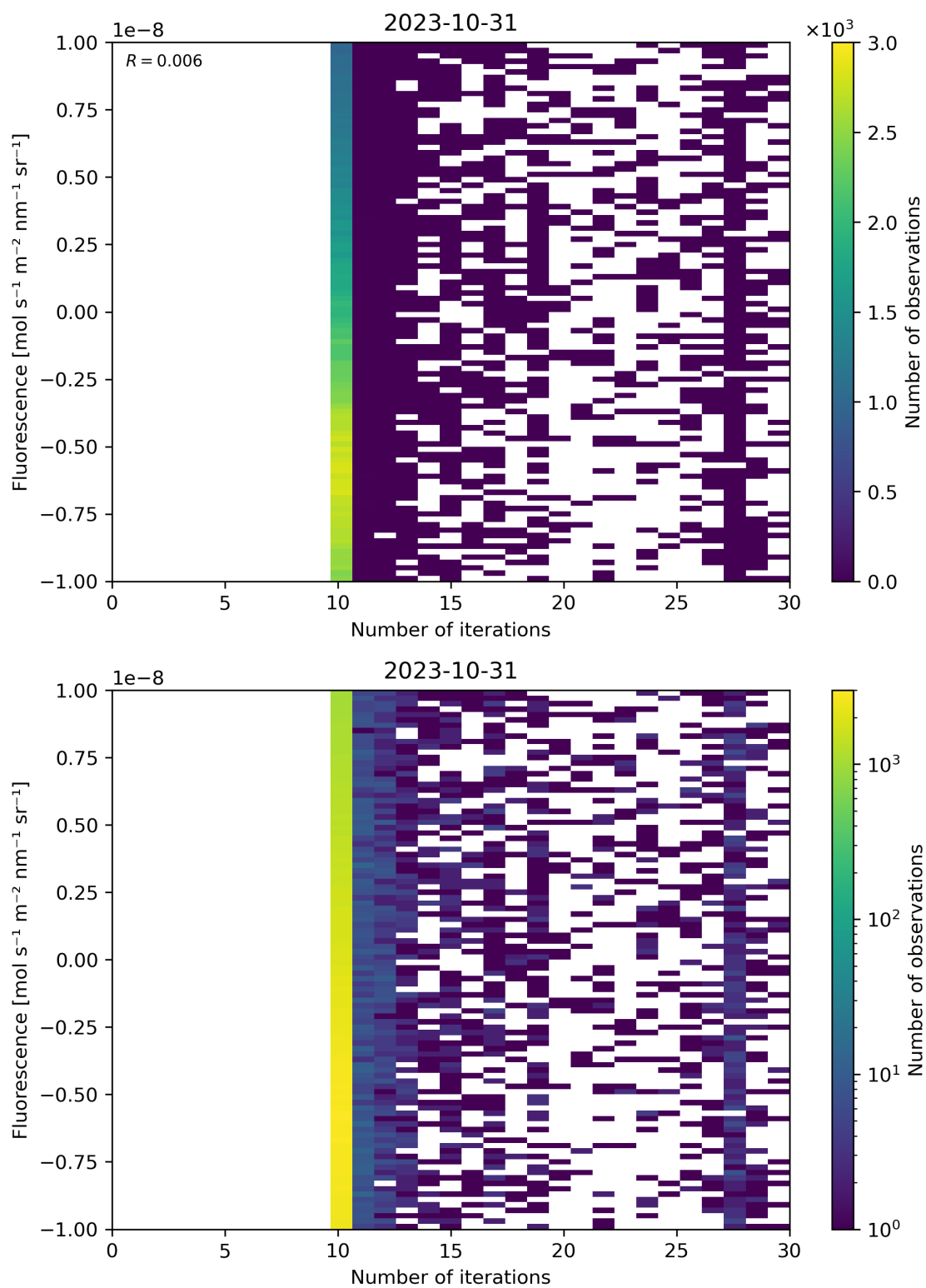
Figure 87: Scatter density plot of “Number of iterations” against “Fluorescence” for 2023-10-30 to 2023-11-01.
