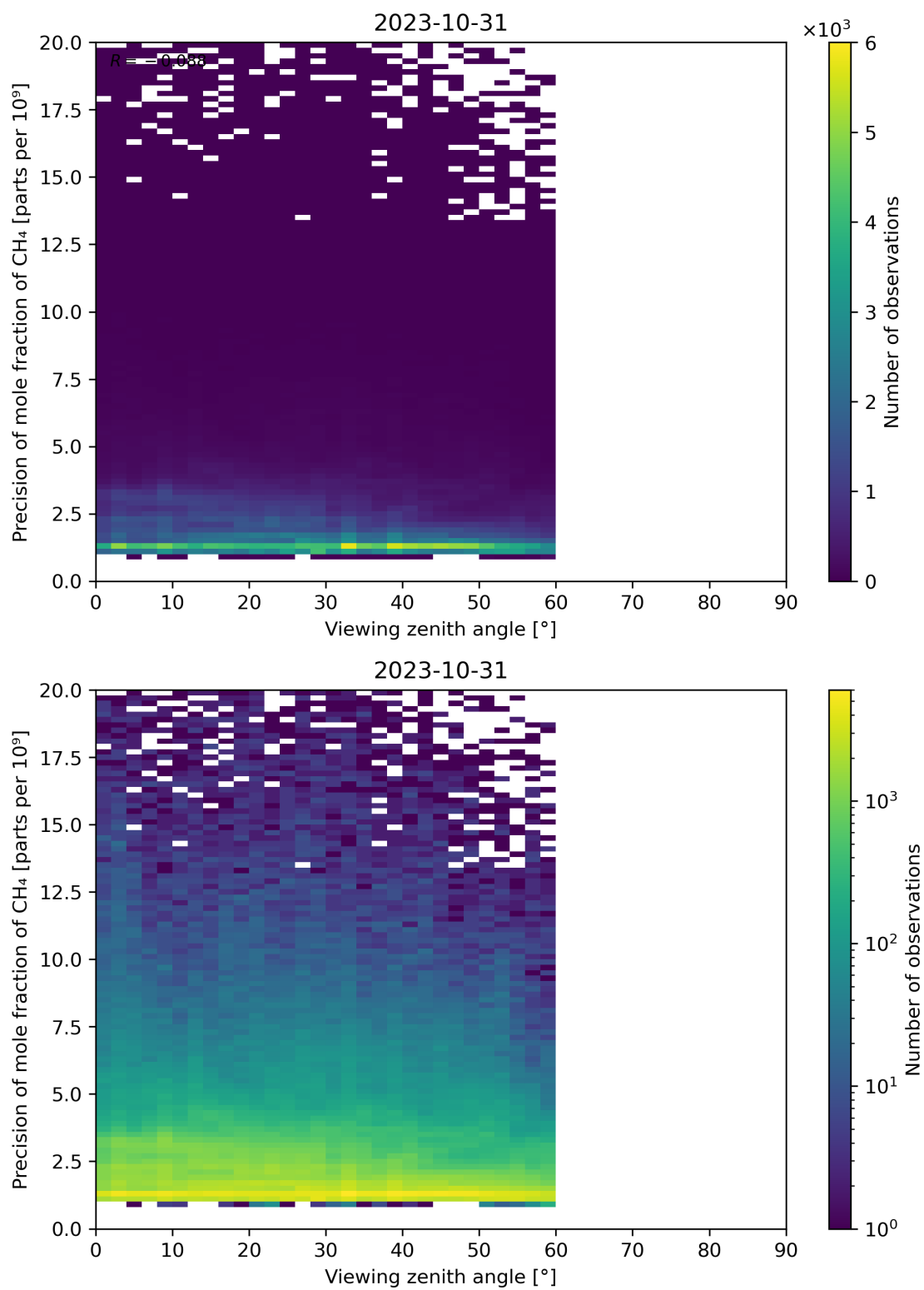
Figure 112: Scatter density plot of “Viewing zenith angle” against “Precision of mole fraction of CH 4 ” for 2023-10-30 to 2023-11-01.
