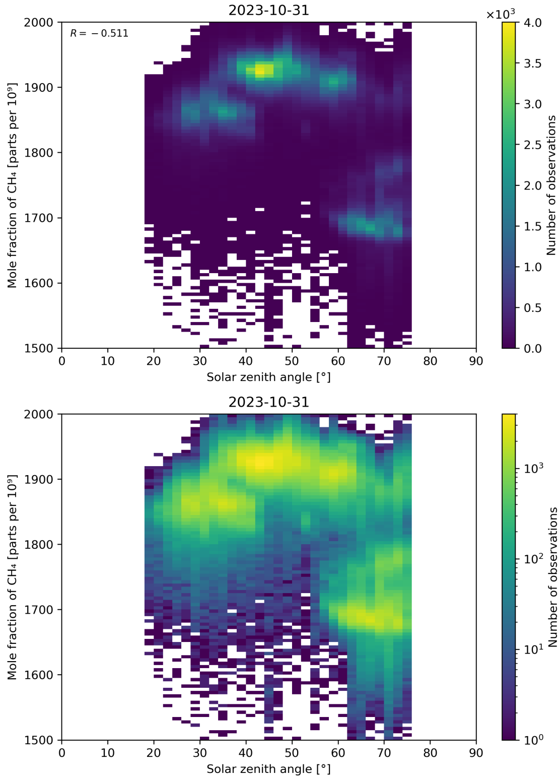
Figure 99: Scatter density plot of “Solar zenith angle” against “Mole fraction of \text{CH}_4 ” for 2023-10-30 to 2023-11-01.
