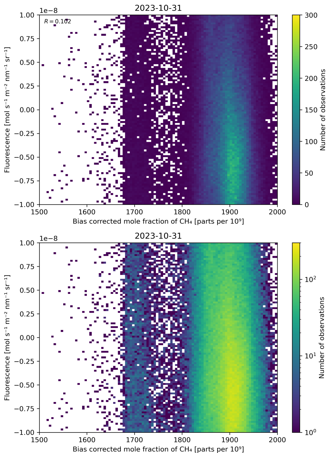
Figure 66: Scatter density plot of “Bias corrected mole fraction of \text{CH}_4 ” against “Fluorescence” for 2023-10-30 to 2023-11-01.
