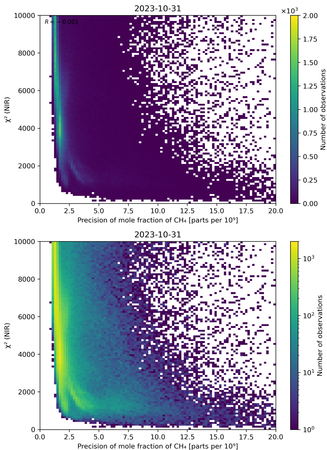
Figure 78: Scatter density plot of “Precision of mole fraction of \text{CH}_4 ” against “ \chi^2 (NIR)” for 2023-10-30 to 2023-11-01.
