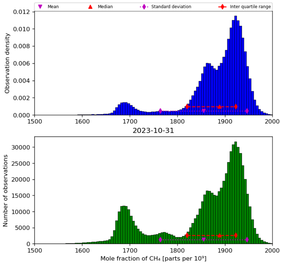
Figure 23: Histogram of “Mole fraction of CH 4 ” for 2023-10-30 to 2023-11-01
