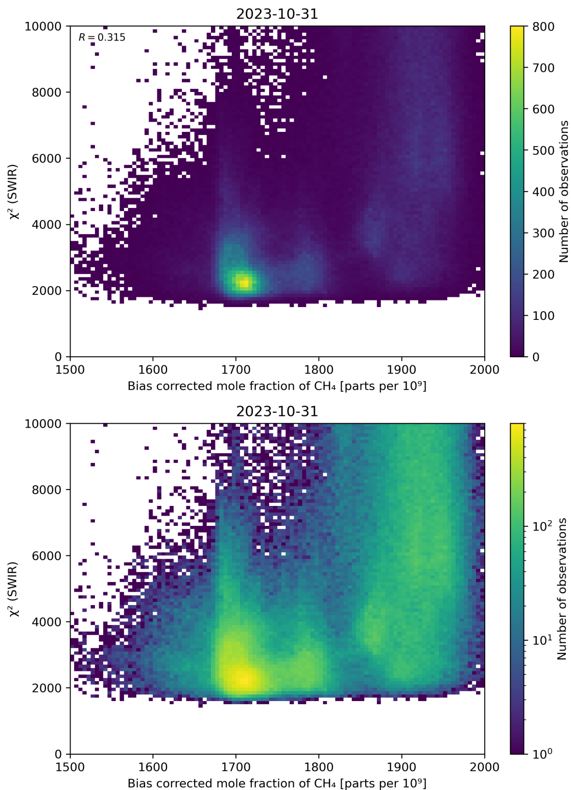
Figure 64: Scatter density plot of “Bias corrected mole fraction of CH 4 ” against “ \chi^2 (SWIR)” for 2023-10-30 to 2023-11-01.
