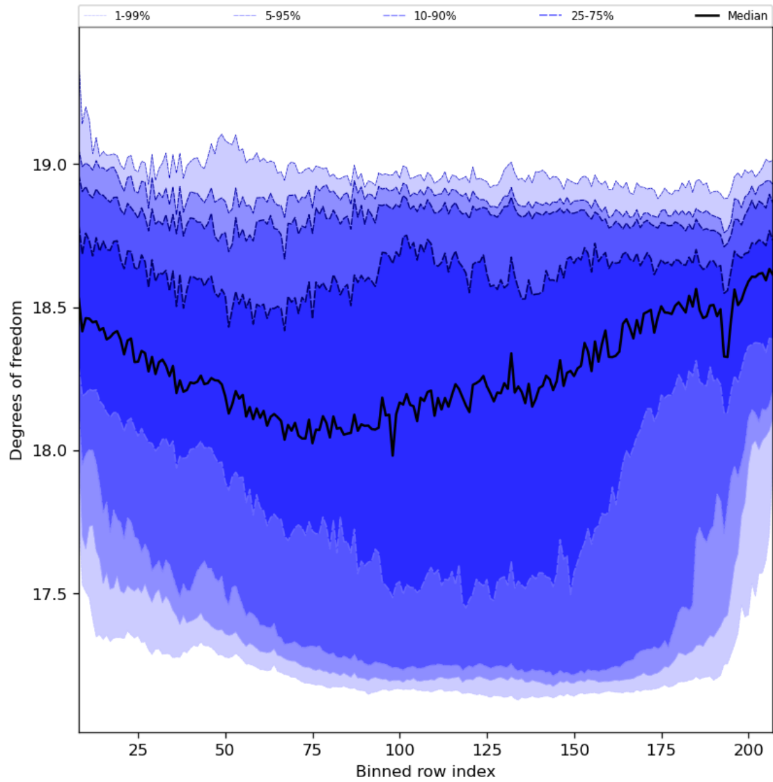
Figure 41: Along track statistics of “Degrees of freedom” for 2023-10-30 to 2023-11-01
