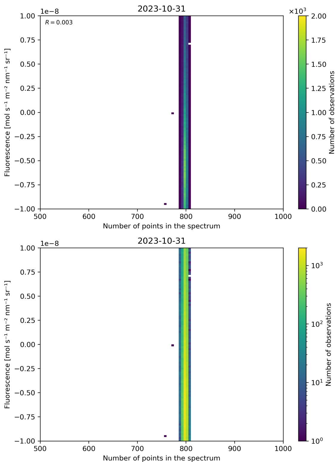
Figure 91: Scatter density plot of “Number of points in the spectrum” against “Fluorescence” for 2023-10-30 to 2023-11-01.
