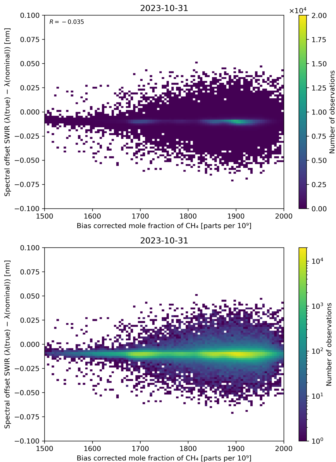
Figure 69: Scatter density plot of “Bias corrected mole fraction of \text{CH}_4 ” against “Spectral offset SWIR ( \lambda(\text{true}) - \lambda(\text{nominal}) )” for 2023-10-30 to 2023-11-01.
