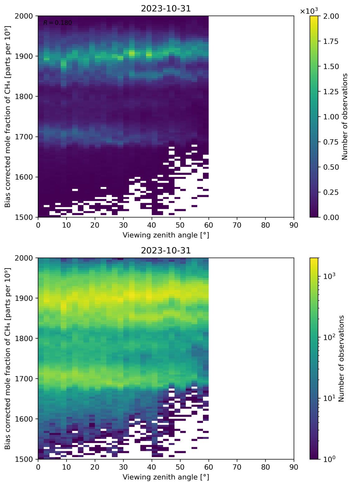
Figure 111: Scatter density plot of “Viewing zenith angle” against “Bias corrected mole fraction of CH 4 ” for 2023-10-30 to 2023-11-01.
