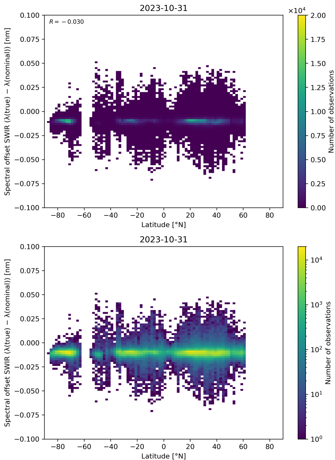
Figure 62: Scatter density plot of “Latitude” against “Spectral offset SWIR ( \lambda(\text{true}) - \lambda(\text{nominal}) )” for 2023-10-30 to 2023-11-01.
