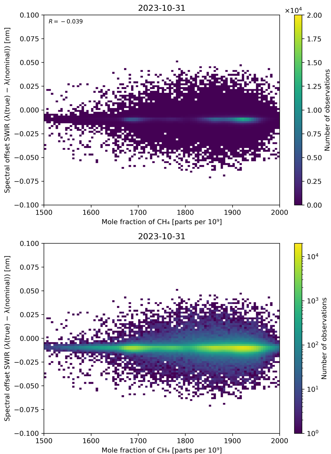
Figure 86: Scatter density plot of “Mole fraction of CH 4 ” against “Spectral offset SWIR ( \lambda(\text{true}) - \lambda(\text{nominal}) )” for 2023-10-30 to 2023-11-01.
