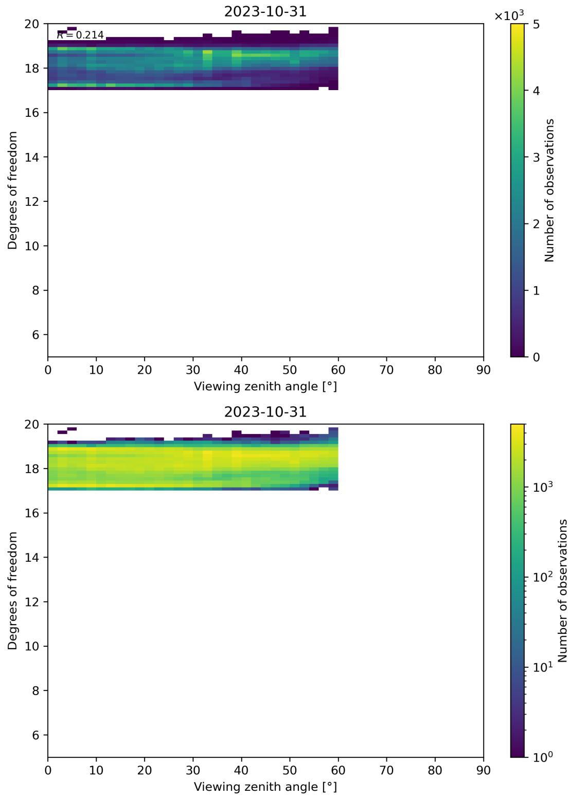
Figure 107: Scatter density plot of “Viewing zenith angle” against “Degrees of freedom” for 2023-10-30 to 2023-11-01.
