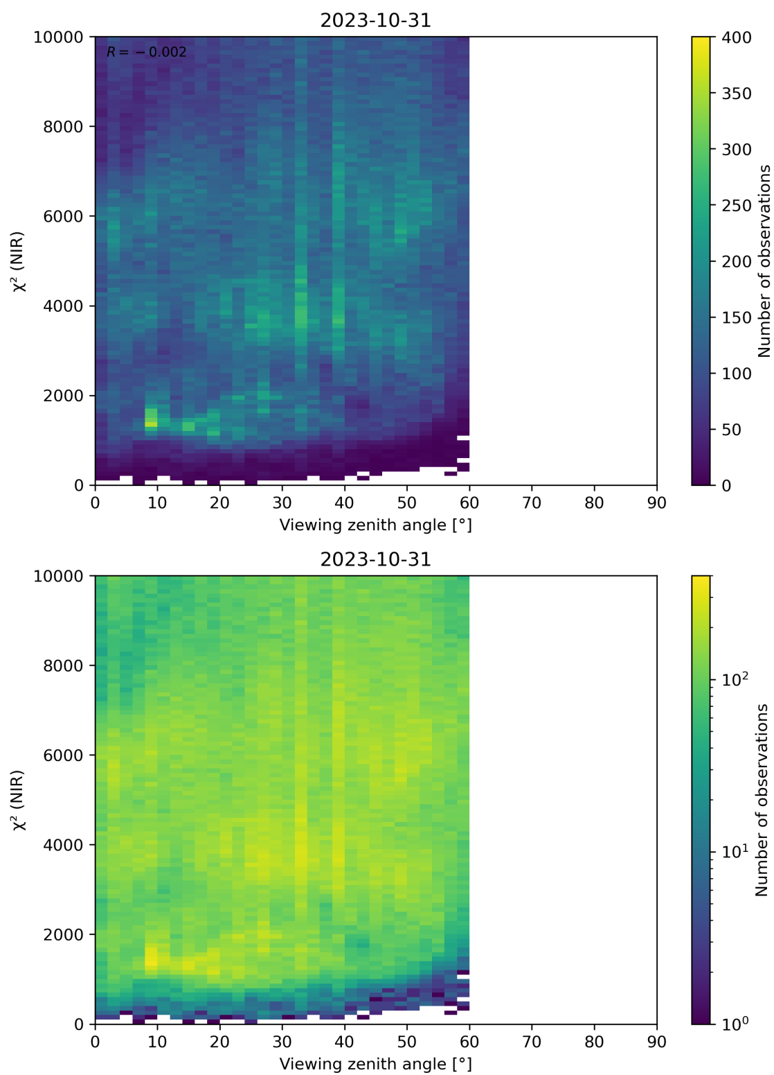
Figure 105: Scatter density plot of “Viewing zenith angle” against “ \chi^2 (NIR)” for 2023-10-30 to 2023-11-01.
