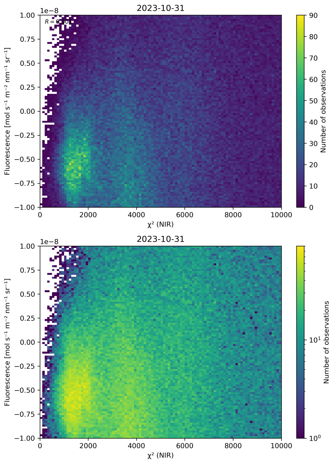
Figure 45: Scatter density plot of “ \chi^2 (NIR)” against “Fluorescence” for 2023-10-30 to 2023-11-01.
