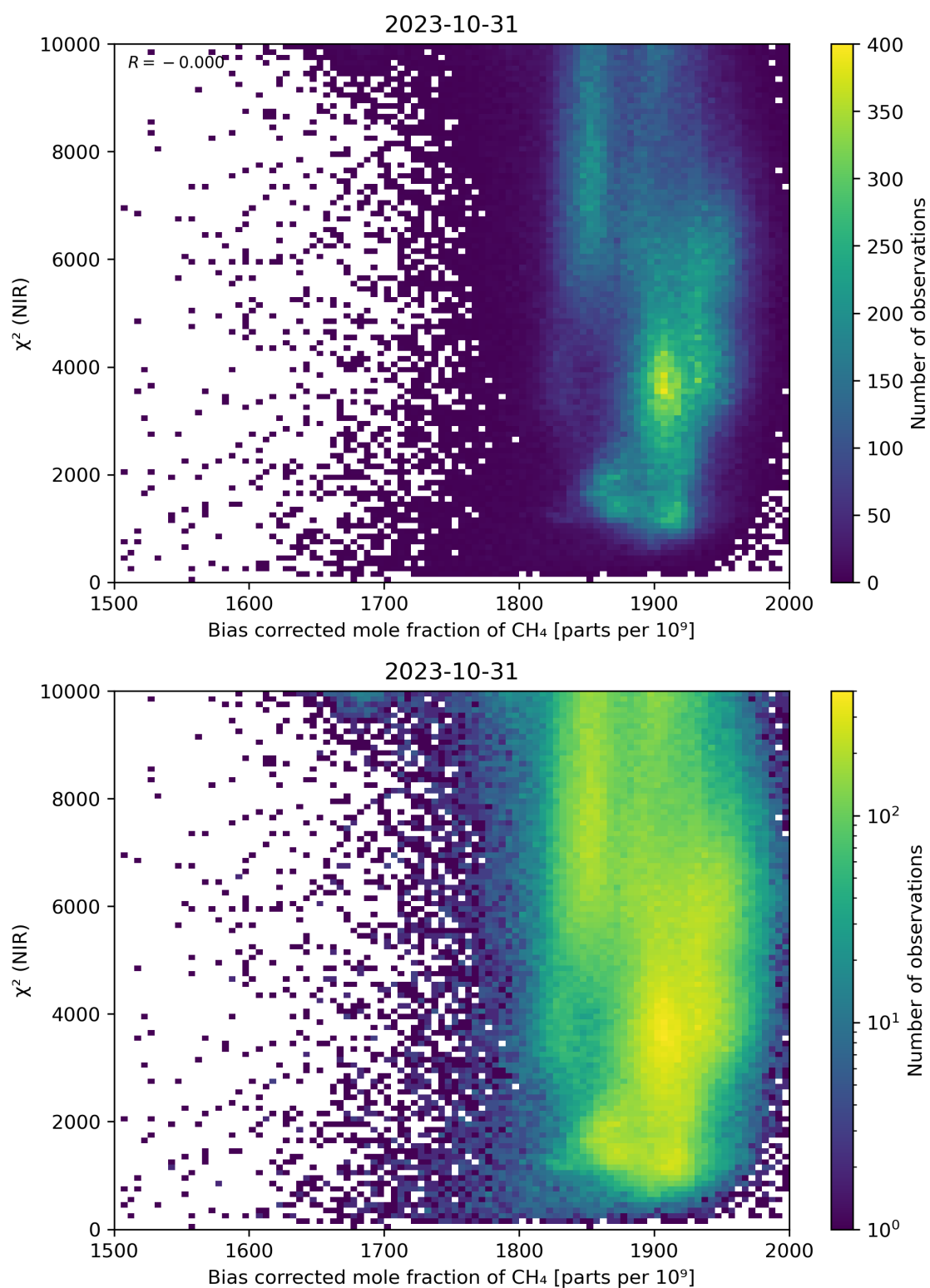
Figure 63: Scatter density plot of “Bias corrected mole fraction of CH 4 ” against “ \chi^2 (NIR)” for 2023-10-30 to 2023-11-01.
