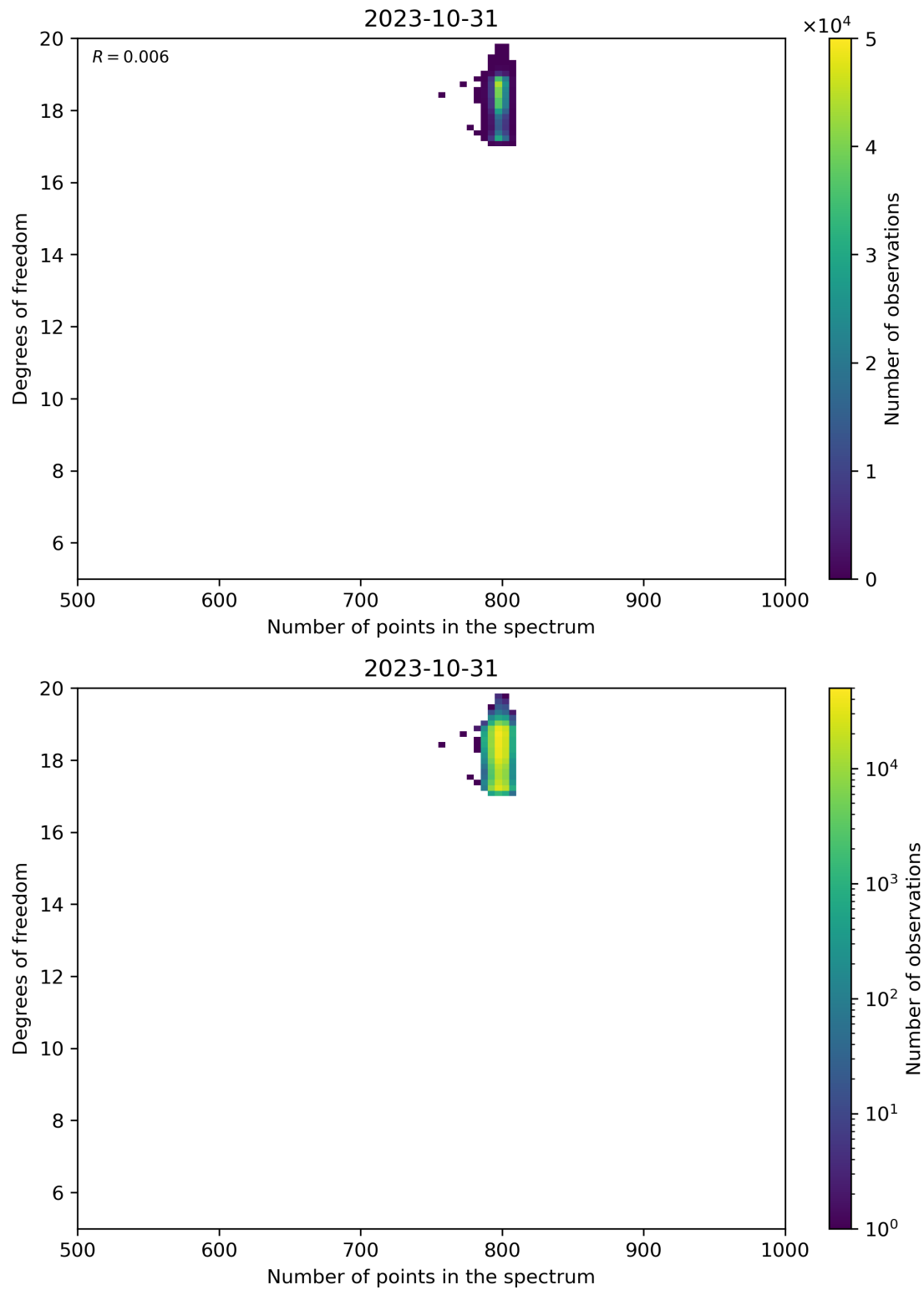
Figure 90: Scatter density plot of “Number of points in the spectrum” against “Degrees of freedom” for 2023-10-30 to 2023-11-01.
