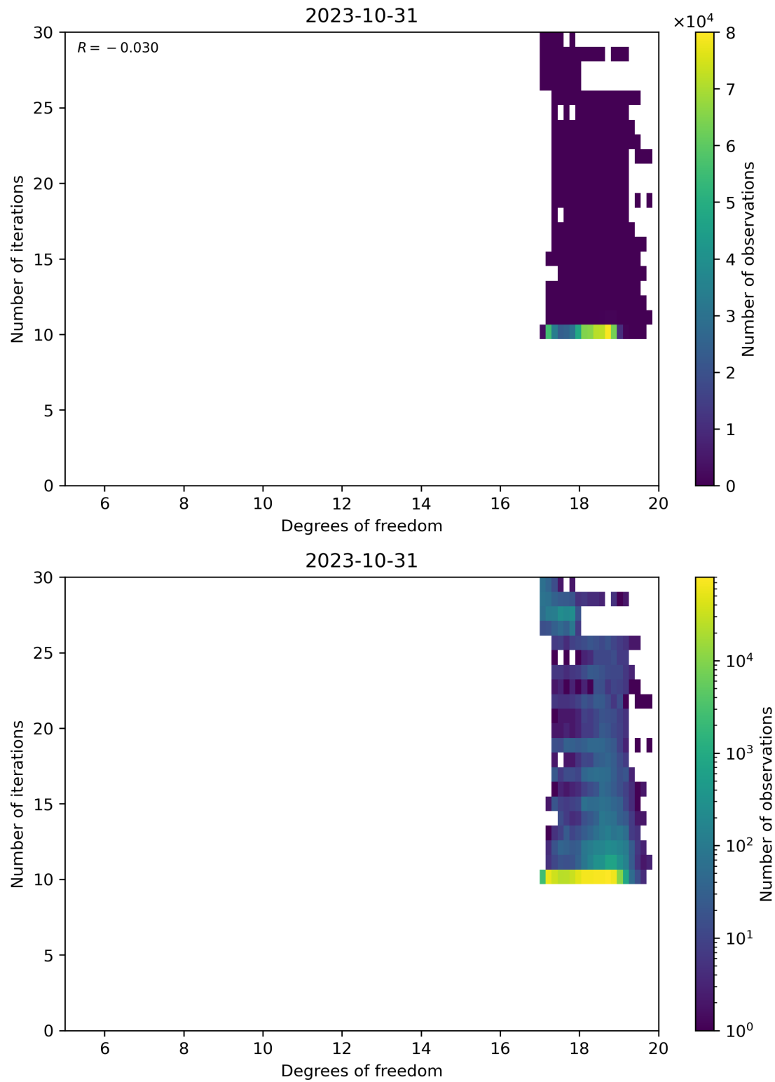
Figure 52: Scatter density plot of “Degrees of freedom” against “Number of iterations” for 2023-10-30 to 2023-11-01.
