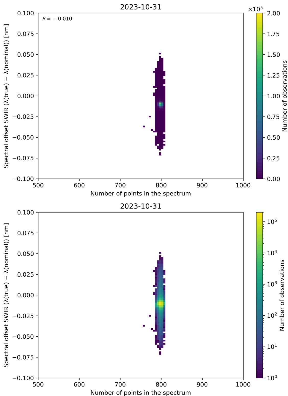
Figure 93: Scatter density plot of “Number of points in the spectrum” against “Spectral offset SWIR ( \lambda(\text{true}) - \lambda(\text{nominal}) )” for 2023-10-30 to 2023-11-01.
