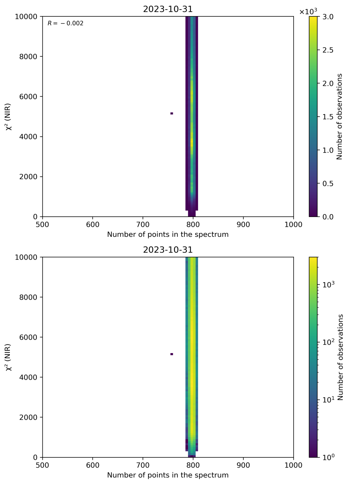
Figure 88: Scatter density plot of “Number of points in the spectrum” against “ \chi^2 (NIR)” for 2023-10-30 to 2023-11-01.
