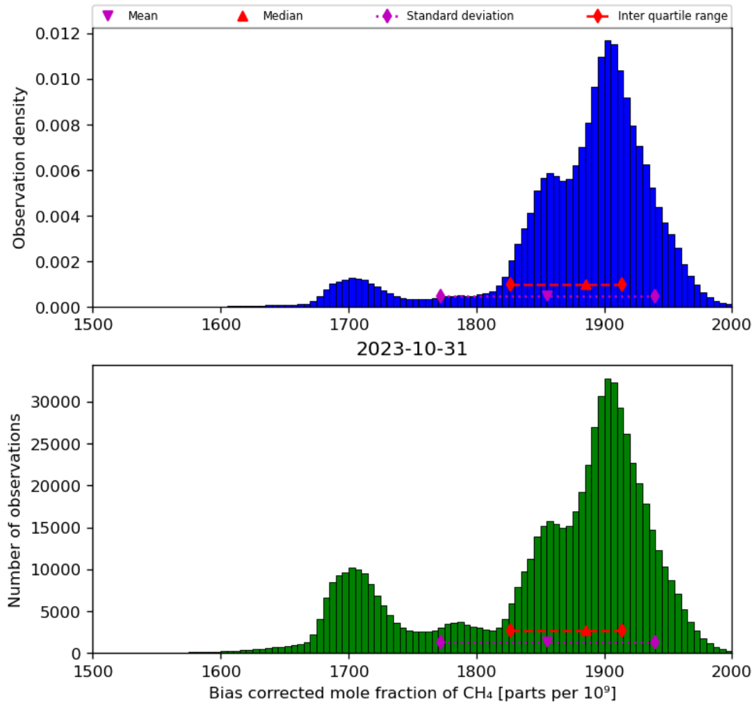
Figure 25: Histogram of “Bias corrected mole fraction of CH 4 ” for 2023-10-30 to 2023-11-01
