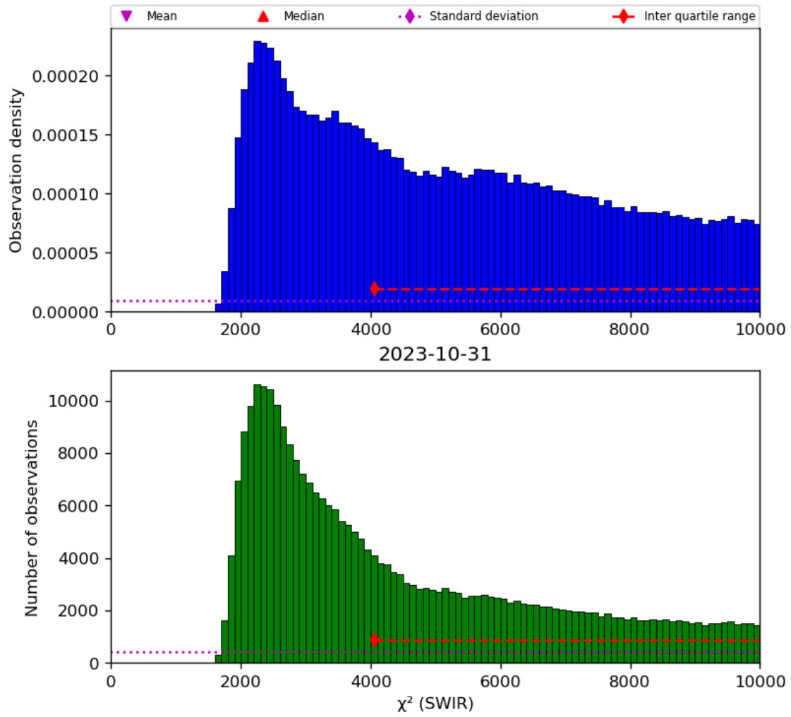
Figure 28: Histogram of " \chi^2 (SWIR)" for 2023-10-30 to 2023-11-01
