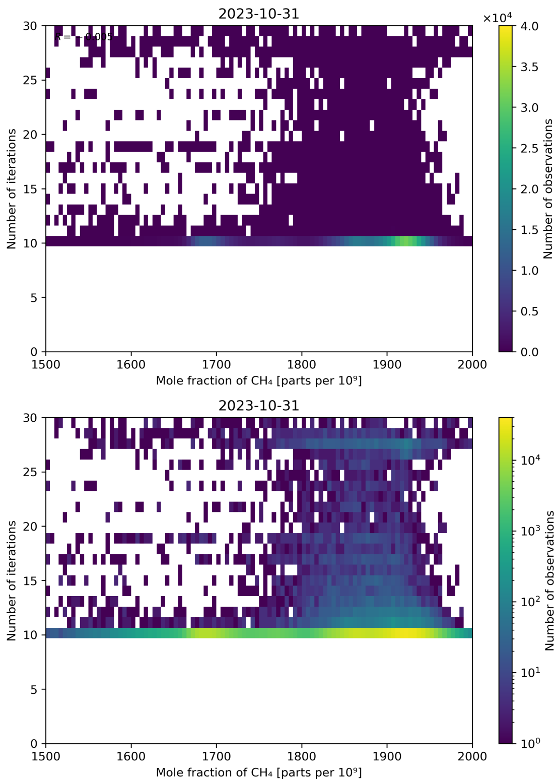
Figure 76: Scatter density plot of “Mole fraction of CH 4 ” against “Number of iterations” for 2023-10-30 to 2023-11-01.
