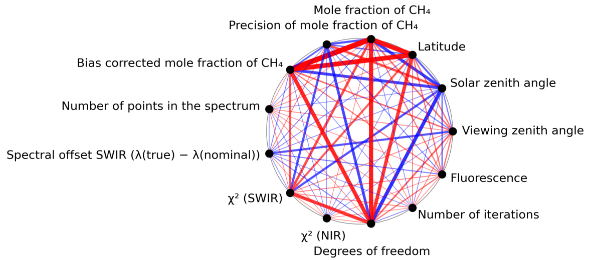
Figure 1: Map of correlation graph for 2023-10-30 to 2023-11-01.
