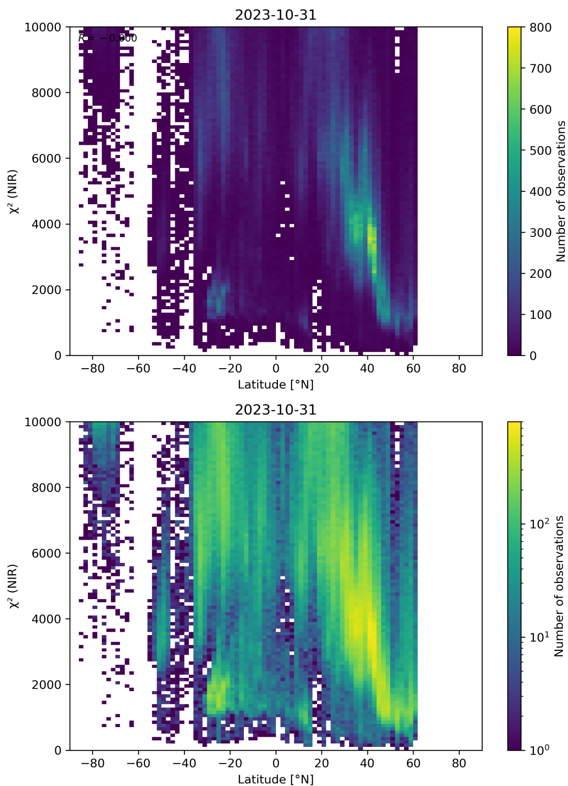
Figure 53: Scatter density plot of “Latitude” against “ \chi^2 (NIR)” for 2023-10-30 to 2023-11-01.
