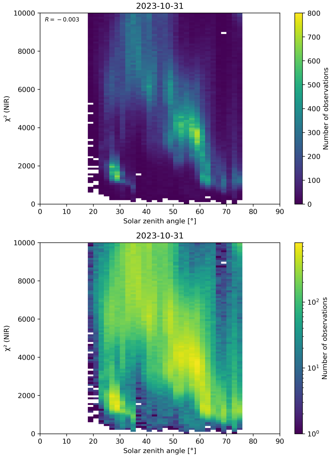
Figure 94: Scatter density plot of “Solar zenith angle” against “ \chi^2 (NIR)” for 2023-10-30 to 2023-11-01.
