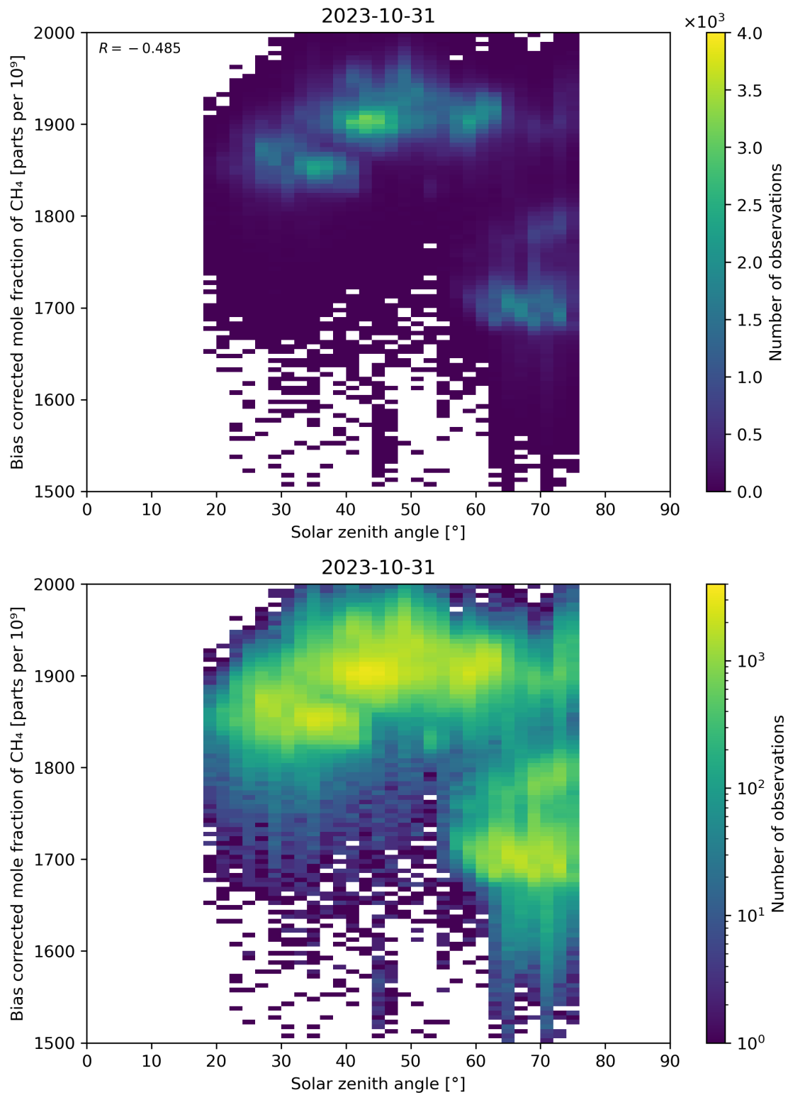
Figure 100: Scatter density plot of “Solar zenith angle” against “Bias corrected mole fraction of \text{CH}_4 ” for 2023-10-30 to 2023-11-01.
