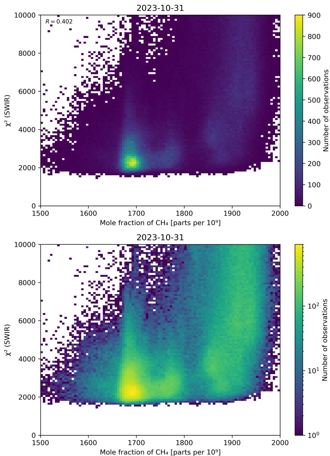
Figure 71: Scatter density plot of “Mole fraction of \text{CH}_4 ” against “ \chi^2 (SWIR)” for 2023-10-30 to 2023-11-01.
