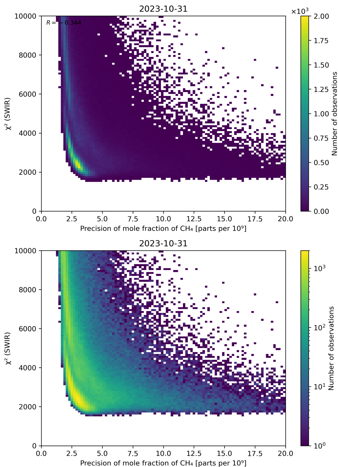
Figure 79: Scatter density plot of “Precision of mole fraction of CH 4 ” against “ \chi^2 (SWIR)” for 2023-10-30 to 2023-11-01.
