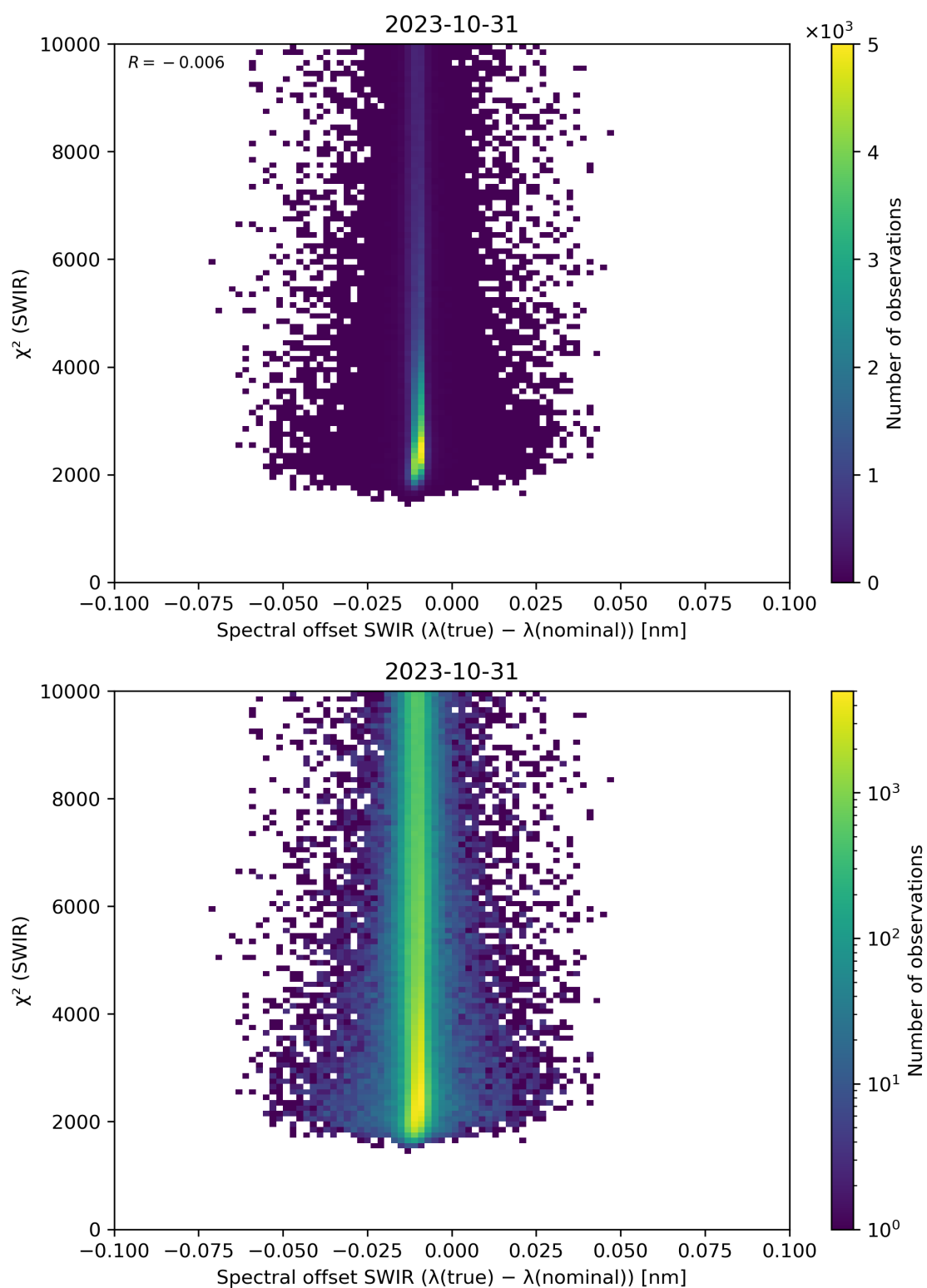
Figure 118: Scatter density plot of “Spectral offset SWIR ( \lambda(\text{true}) - \lambda(\text{nominal}) )” against “ \chi^2 (SWIR)” for 2023-10-30 to 2023-11-01.
