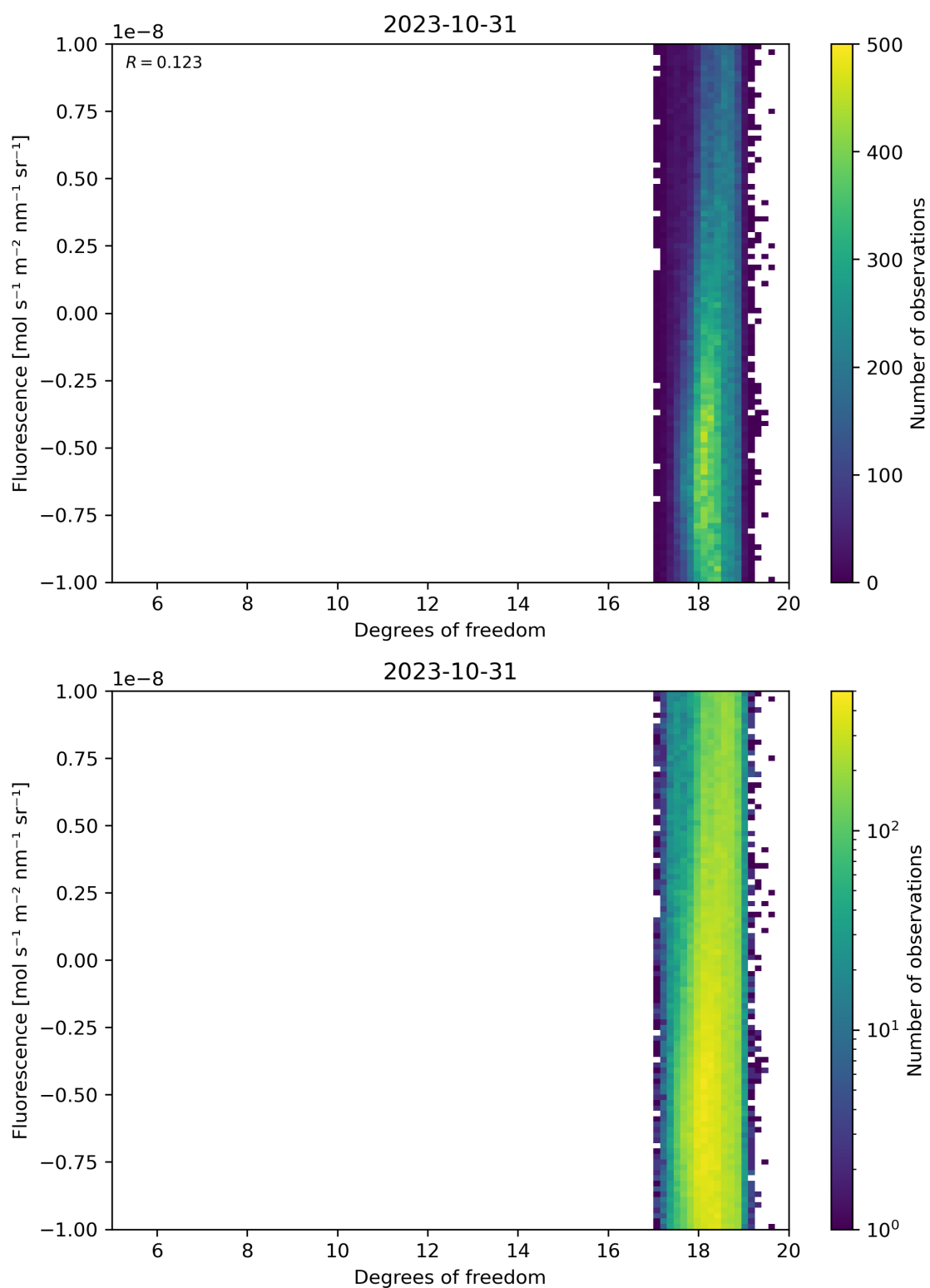
Figure 51: Scatter density plot of “Degrees of freedom” against “Fluorescence” for 2023-10-30 to 2023-11-01.
