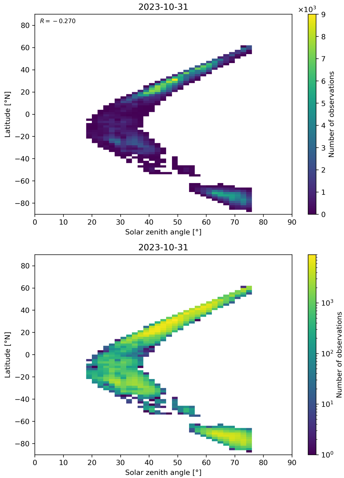
Figure 98: Scatter density plot of “Solar zenith angle” against “Latitude” for 2023-10-30 to 2023-11-01.
