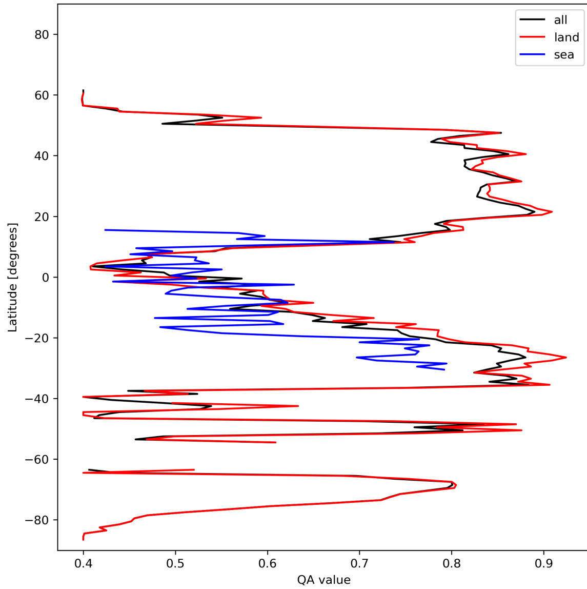
Figure 11: Zonal average of “QA value” for 2023-10-30 to 2023-11-01.
