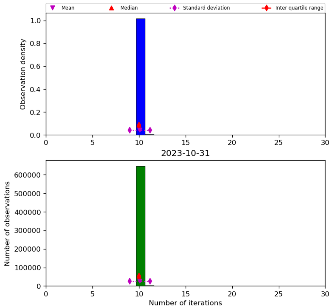
Figure 31: Histogram of “Number of iterations” for 2023-10-30 to 2023-11-01
