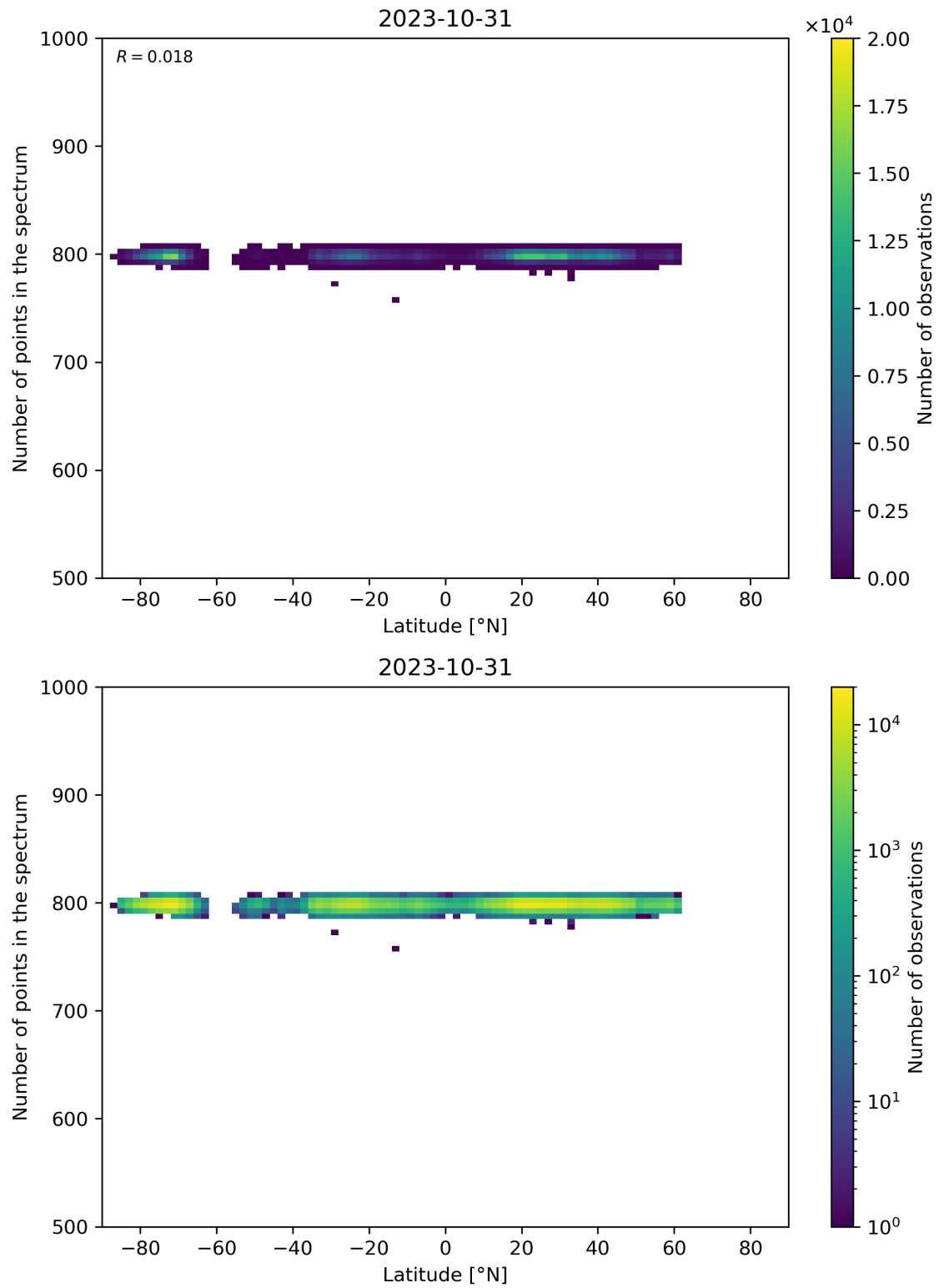
Figure 61: Scatter density plot of “Latitude” against “Number of points in the spectrum” for 2023-10-30 to 2023-11-01.
