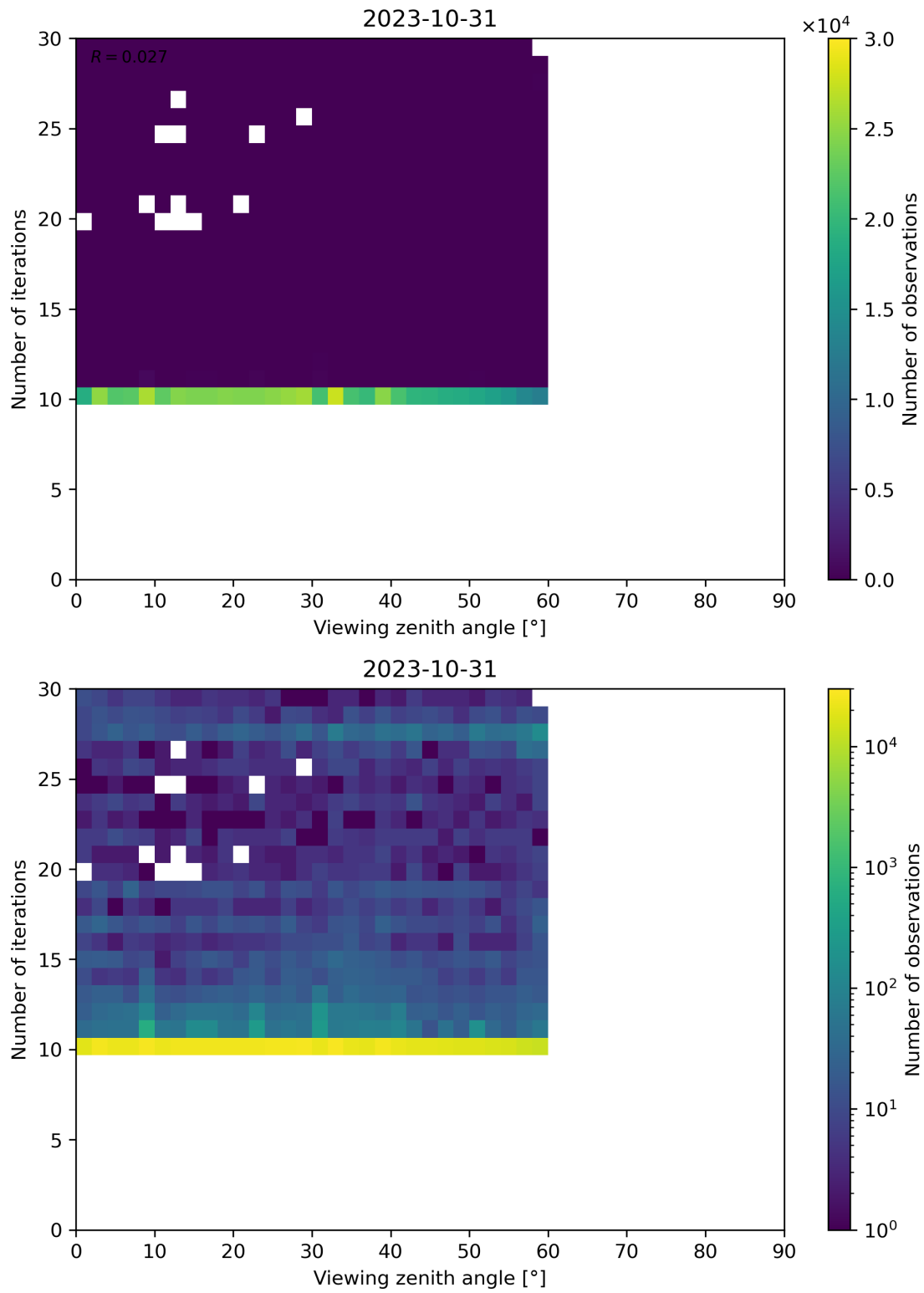
Figure 113: Scatter density plot of “Viewing zenith angle” against “Number of iterations” for 2023-10-30 to 2023-11-01.
