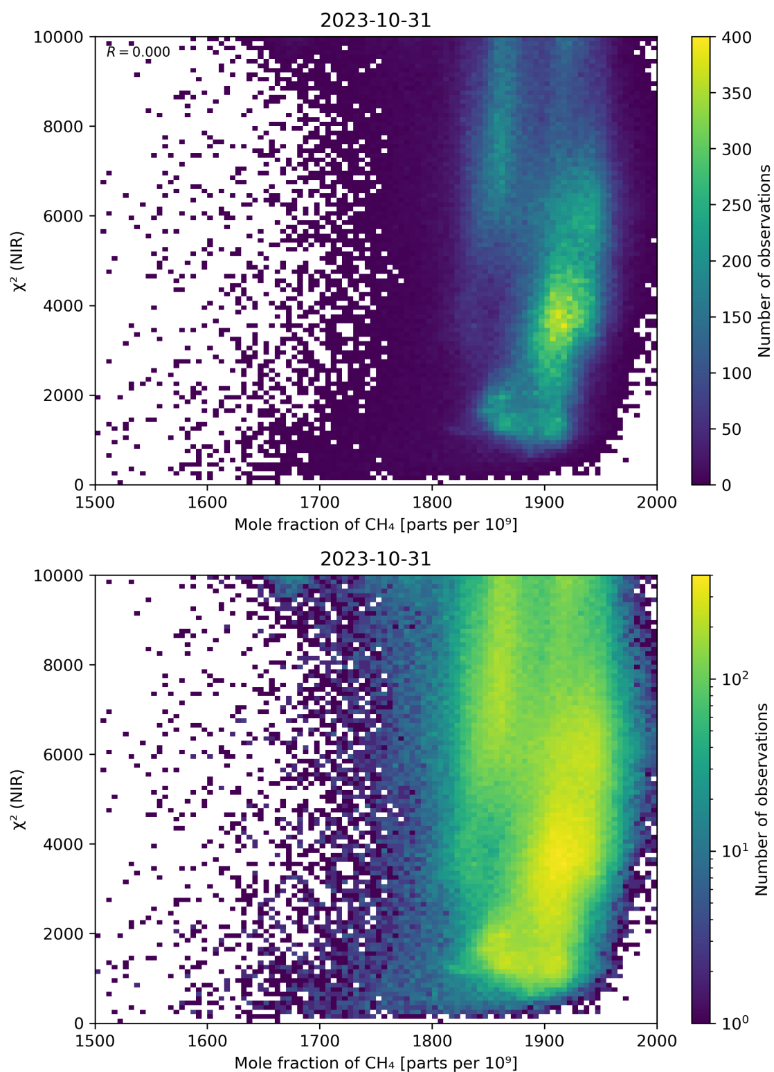
Figure 70: Scatter density plot of “Mole fraction of CH 4 ” against “ \chi^2 (NIR)” for 2023-10-30 to 2023-11-01.
