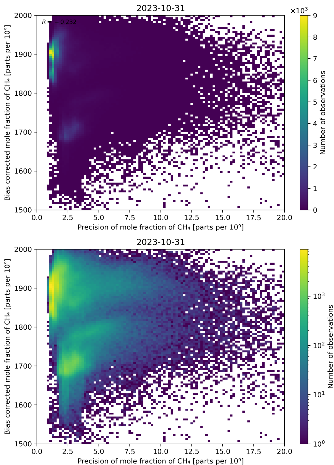
Figure 82: Scatter density plot of “Precision of mole fraction of CH 4 ” against “Bias corrected mole fraction of CH 4 ” for 2023-10-30 to 2023-11-01.
