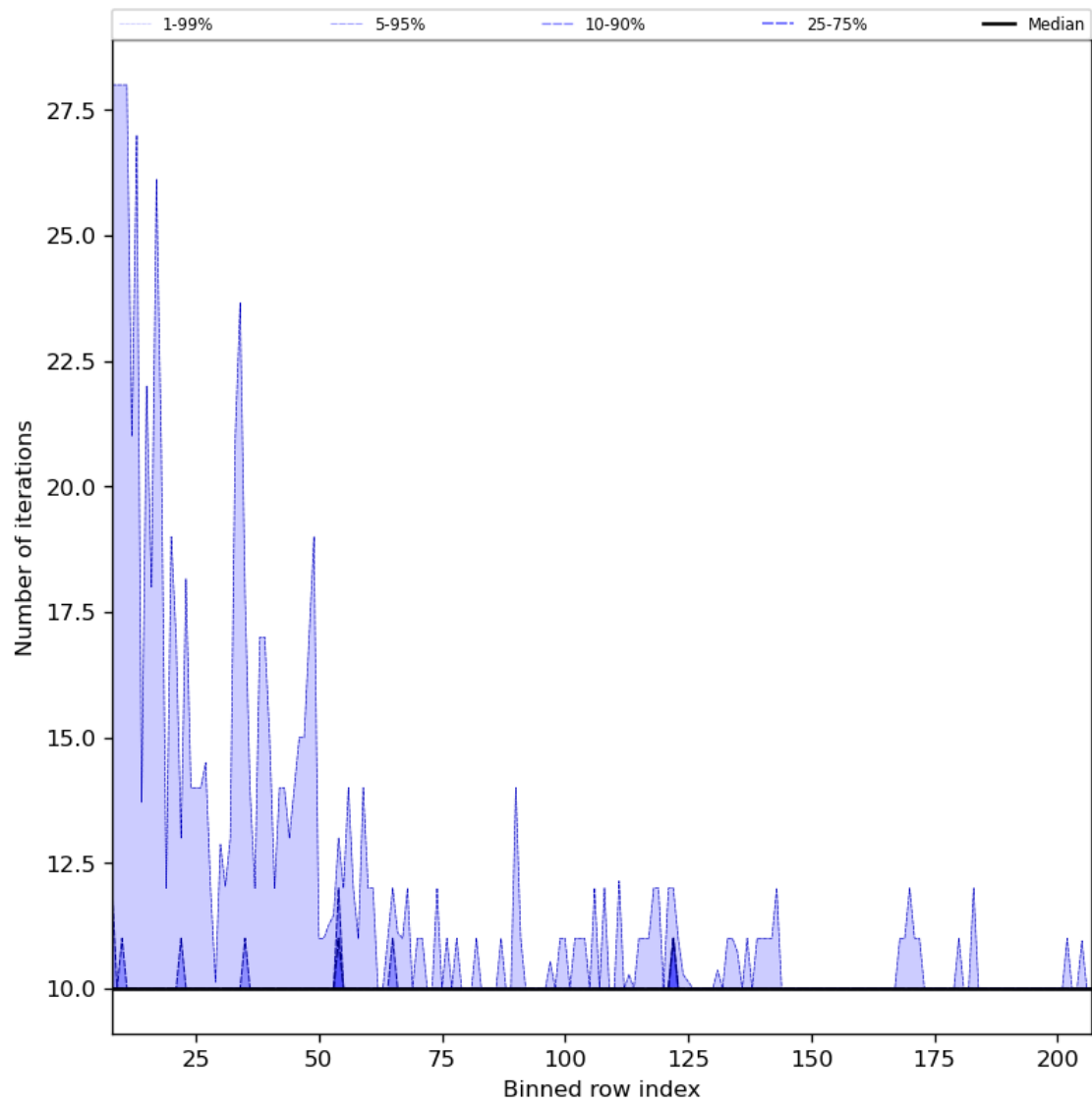
Figure 42: Along track statistics of “Number of iterations” for 2023-10-30 to 2023-11-01
