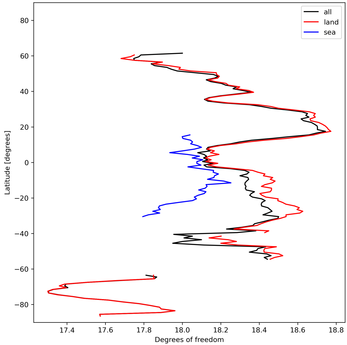
Figure 19: Zonal average of “Degrees of freedom” for 2023-10-30 to 2023-11-01.
