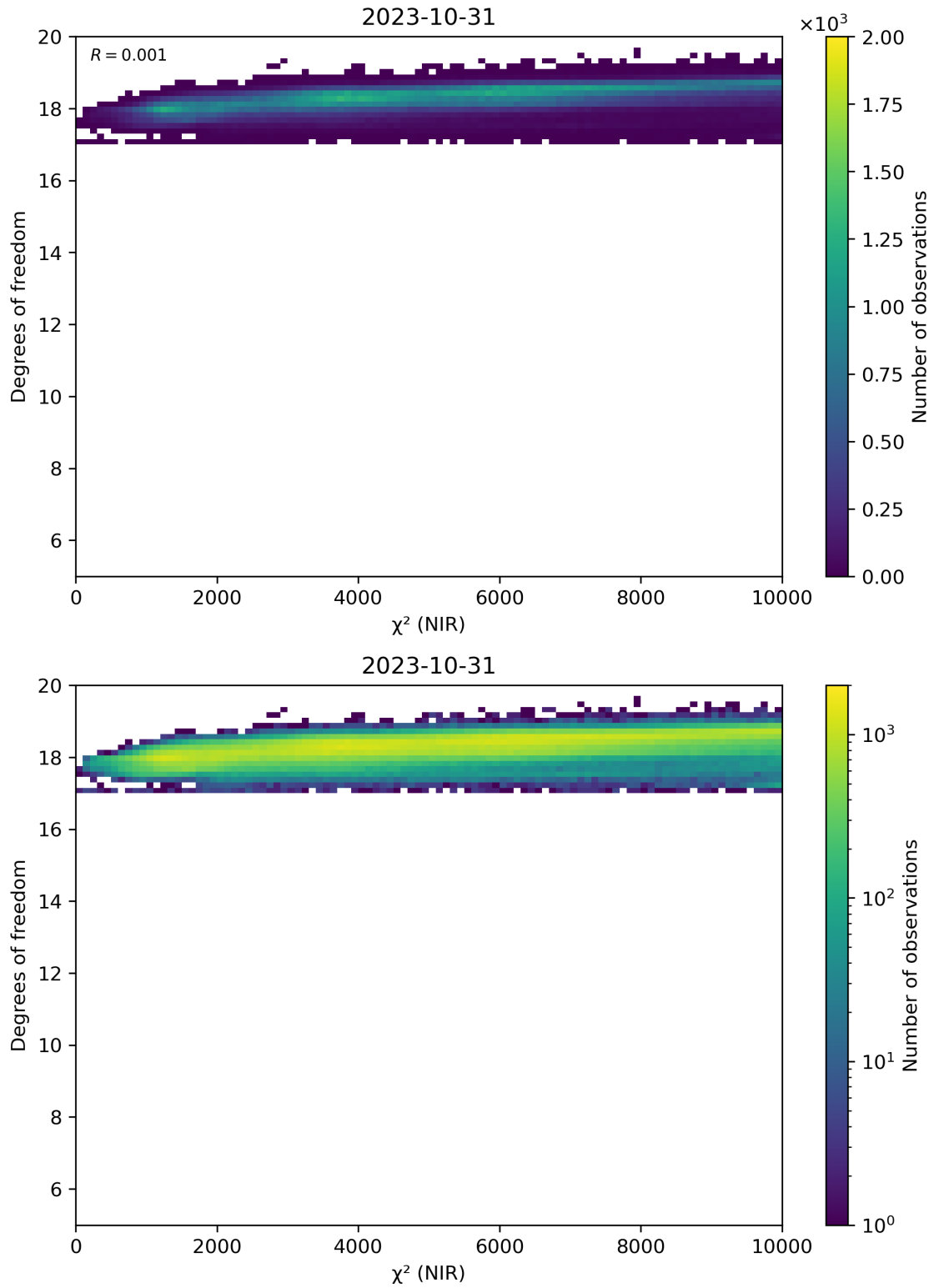
Figure 44: Scatter density plot of “ \chi^2 (NIR)” against “Degrees of freedom” for 2023-10-30 to 2023-11-01.
