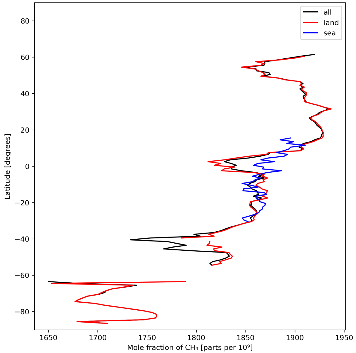
Figure 12: Zonal average of “Mole fraction of \text{CH}_4 ” for 2023-10-30 to 2023-11-01.
