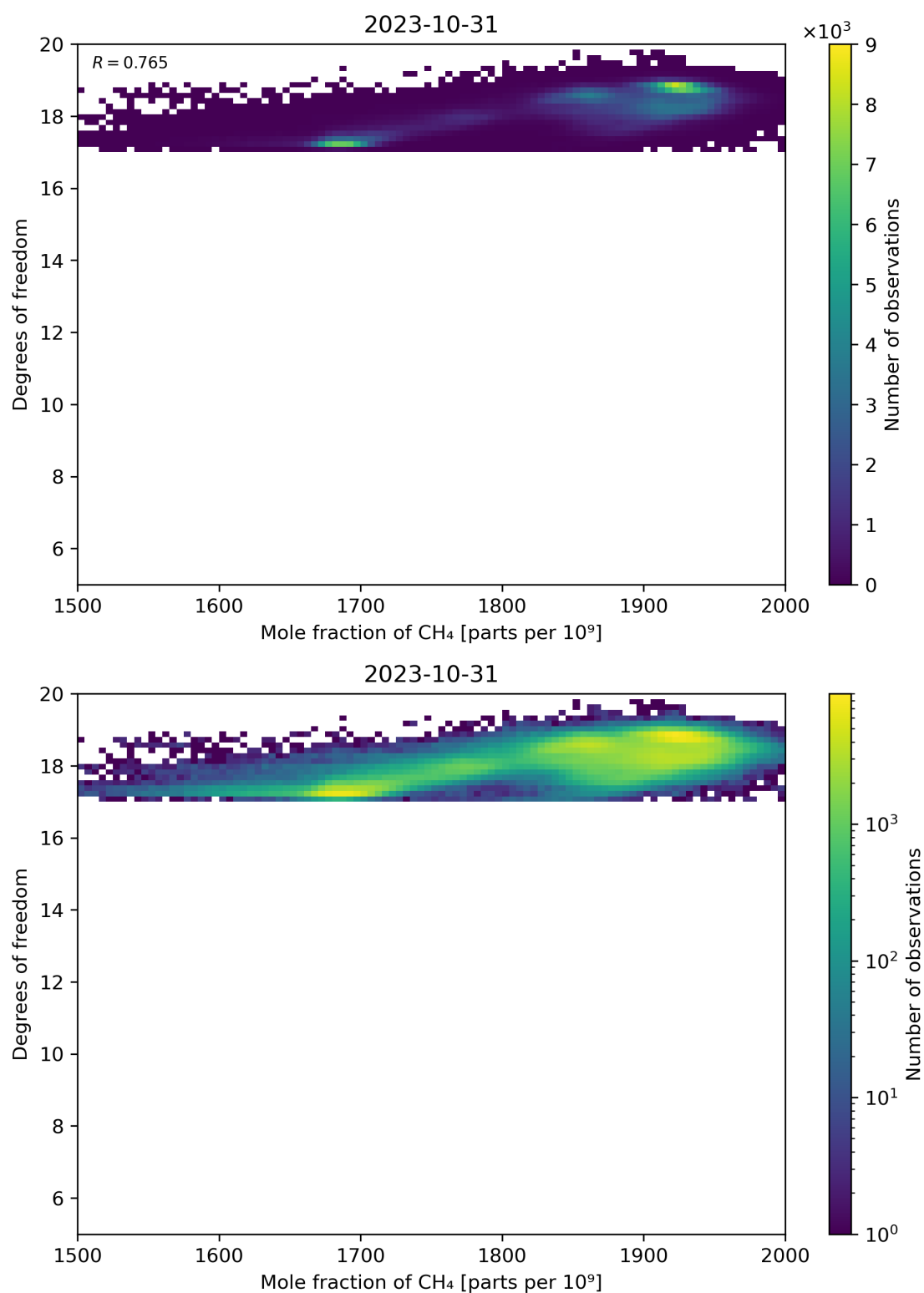
Figure 72: Scatter density plot of “Mole fraction of CH 4 ” against “Degrees of freedom” for 2023-10-30 to 2023-11-01.
