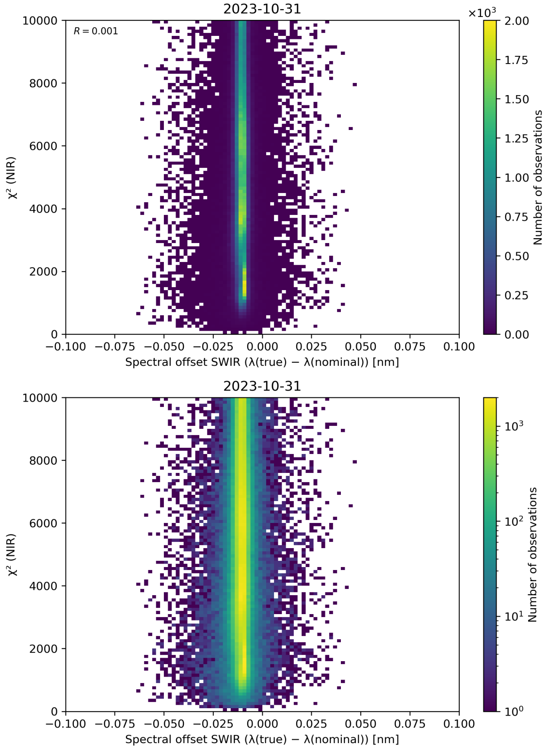
Figure 117: Scatter density plot of “Spectral offset SWIR ( \lambda(\text{true}) - \lambda(\text{nominal}) )” against “ \chi^2 (NIR)” for 2023-10-30 to 2023-11-01.
