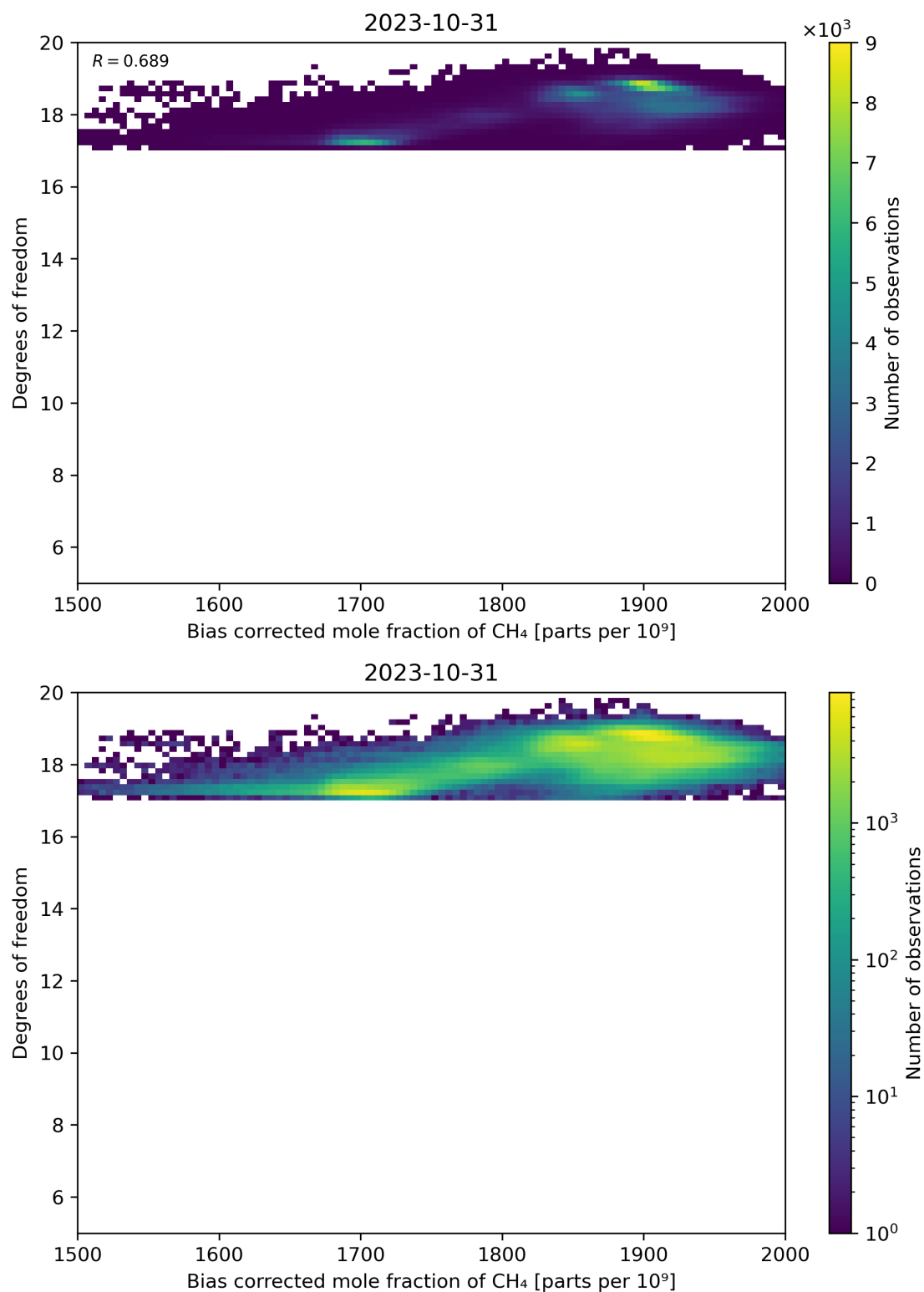
Figure 65: Scatter density plot of “Bias corrected mole fraction of CH 4 ” against “Degrees of freedom” for 2023-10-30 to 2023-11-01.
