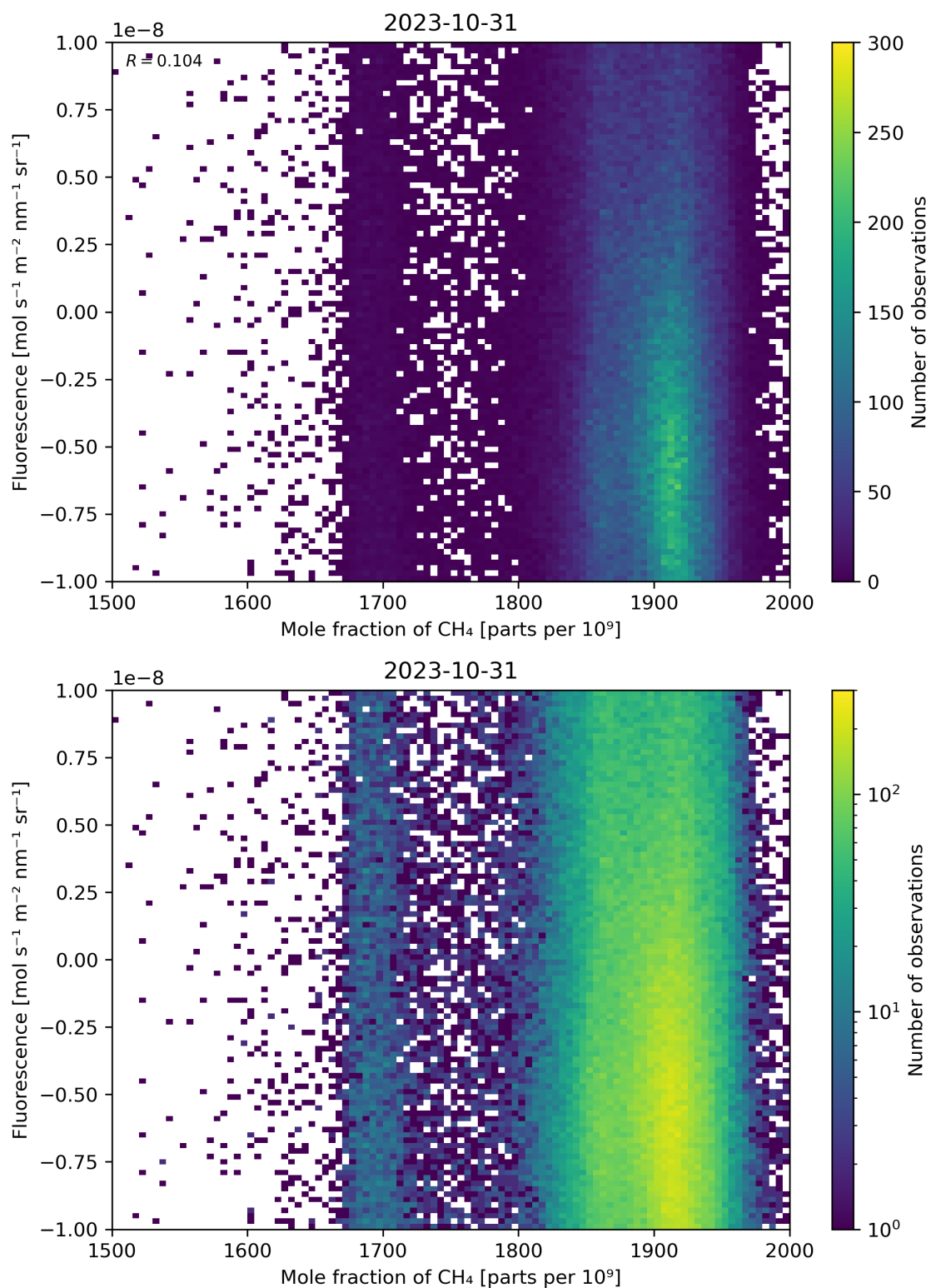
Figure 73: Scatter density plot of “Mole fraction of \text{CH}_4 ” against “Fluorescence” for 2023-10-30 to 2023-11-01.
