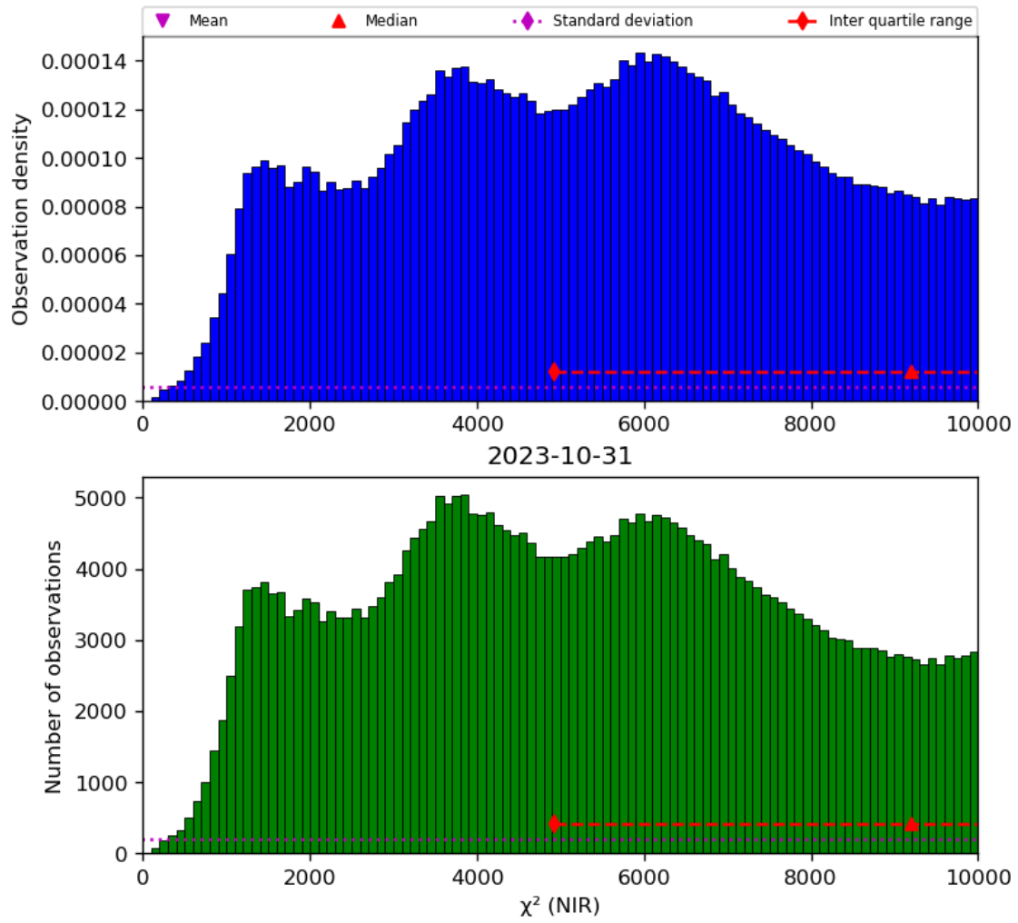
Figure 29: Histogram of “ \chi^2 (NIR)” for 2023-10-30 to 2023-11-01
