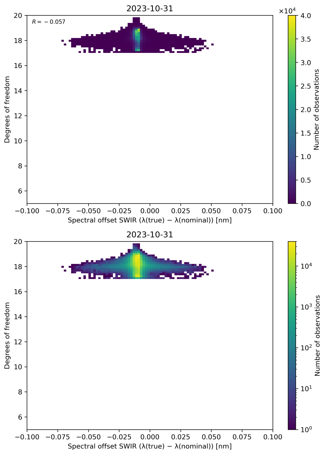
Figure 119: Scatter density plot of “Spectral offset SWIR ( \lambda(\text{true}) - \lambda(\text{nominal}) )” against “Degrees of freedom” for 2023-10-30 to 2023-11-01.
