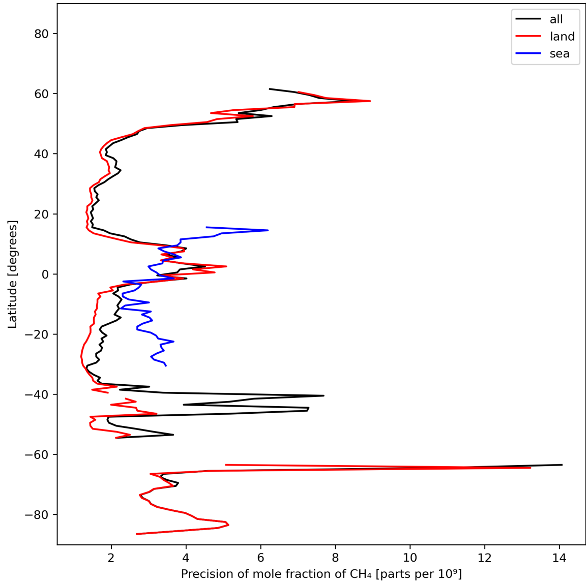
Figure 13: Zonal average of “Precision of mole fraction of CH 4 ” for 2023-10-30 to 2023-11-01.
