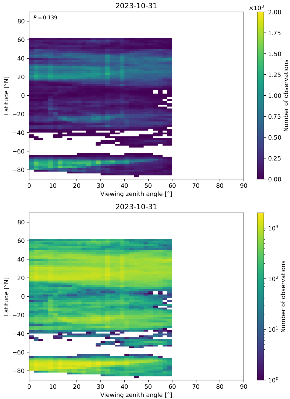
Figure 109: Scatter density plot of “Viewing zenith angle” against “Latitude” for 2023-10-30 to 2023-11-01.
