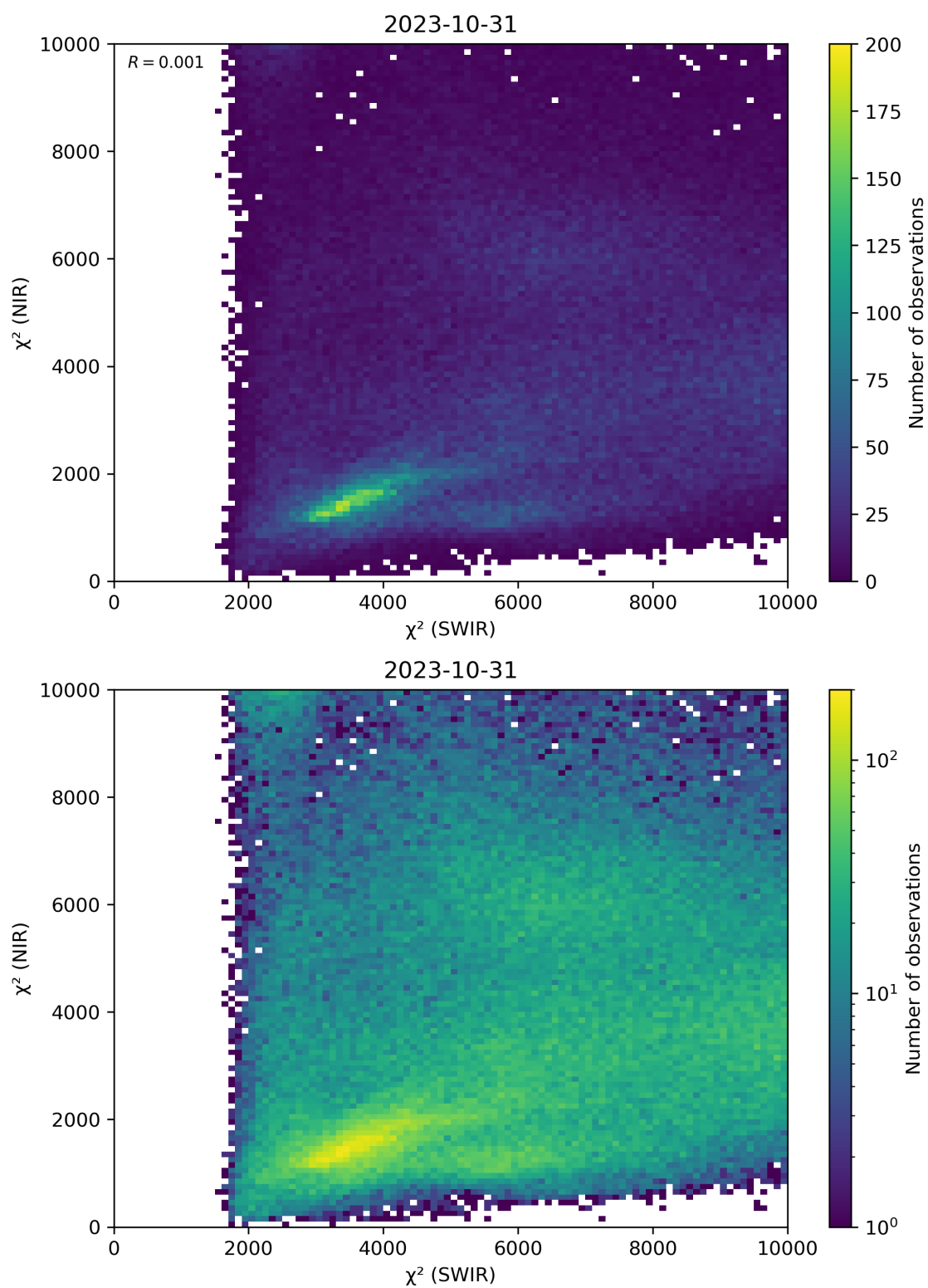
Figure 47: Scatter density plot of “ \chi^2 (SWIR)” against “ \chi^2 (NIR)” for 2023-10-30 to 2023-11-01.
