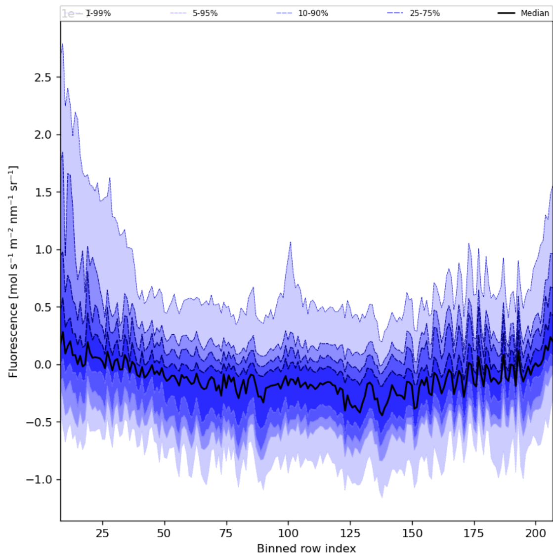
Figure 43: Along track statistics of “Fluorescence” for 2023-10-30 to 2023-11-01
