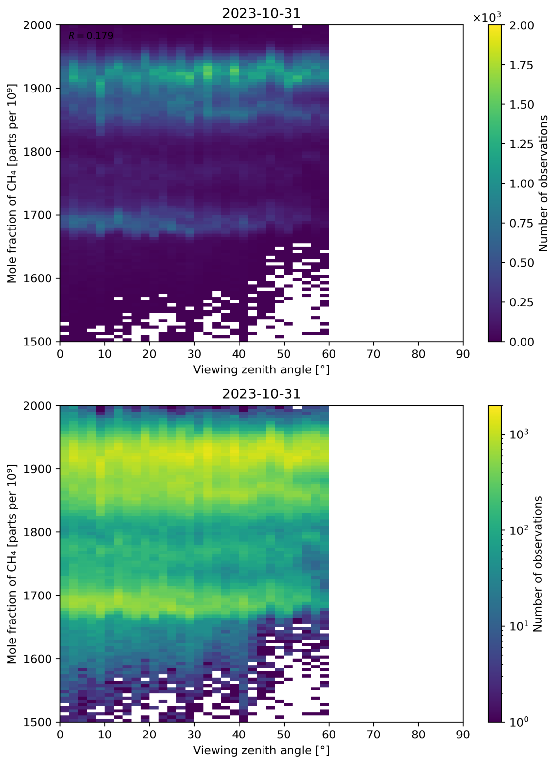
Figure 110: Scatter density plot of “Viewing zenith angle” against “Mole fraction of CH 4 ” for 2023-10-30 to 2023-11-01.
