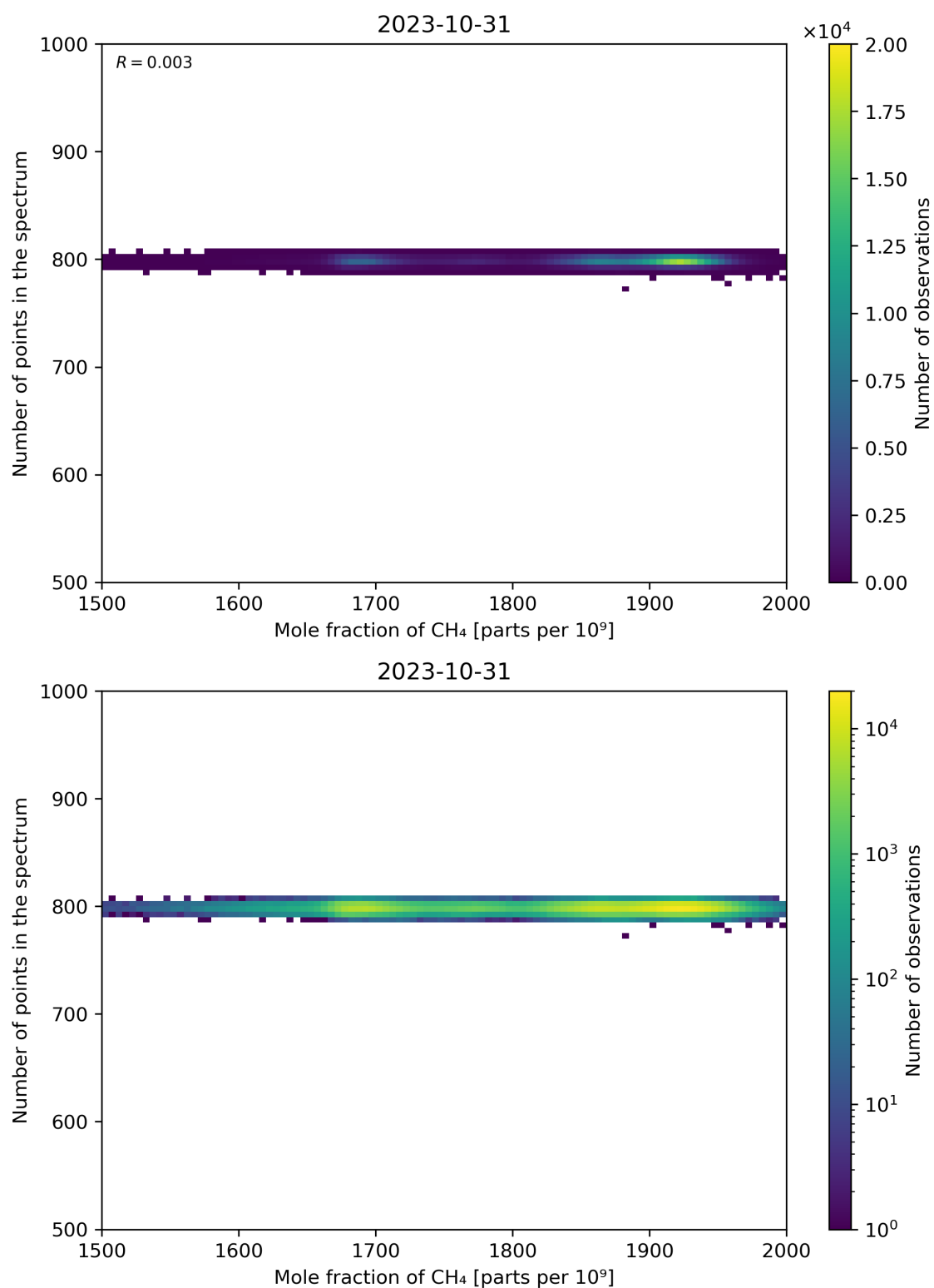
Figure 77: Scatter density plot of “Mole fraction of CH 4 ” against “Number of points in the spectrum” for 2023-10-30 to 2023-11-01.
