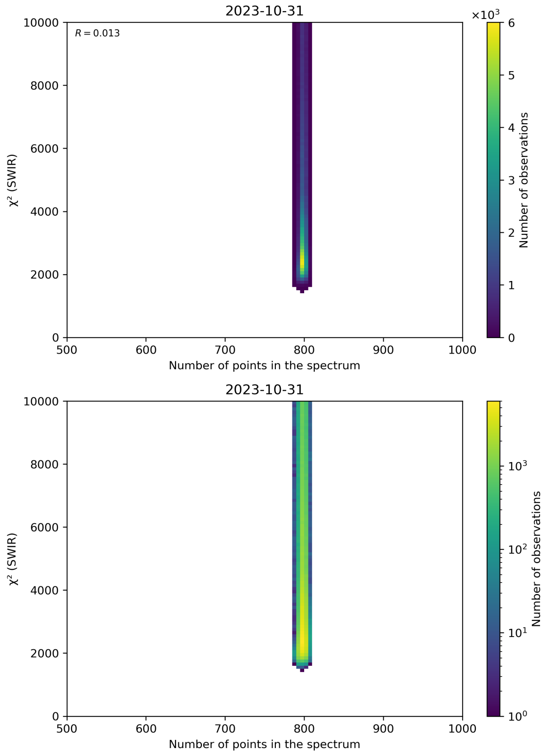
Figure 89: Scatter density plot of “Number of points in the spectrum” against “ \chi^2 (SWIR)” for 2023-10-30 to 2023-11-01.
