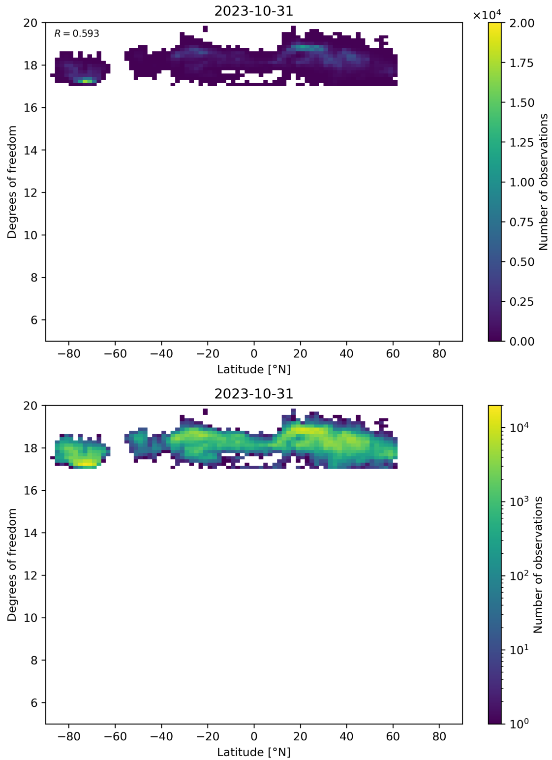
Figure 55: Scatter density plot of “Latitude” against “Degrees of freedom” for 2023-10-30 to 2023-11-01.
