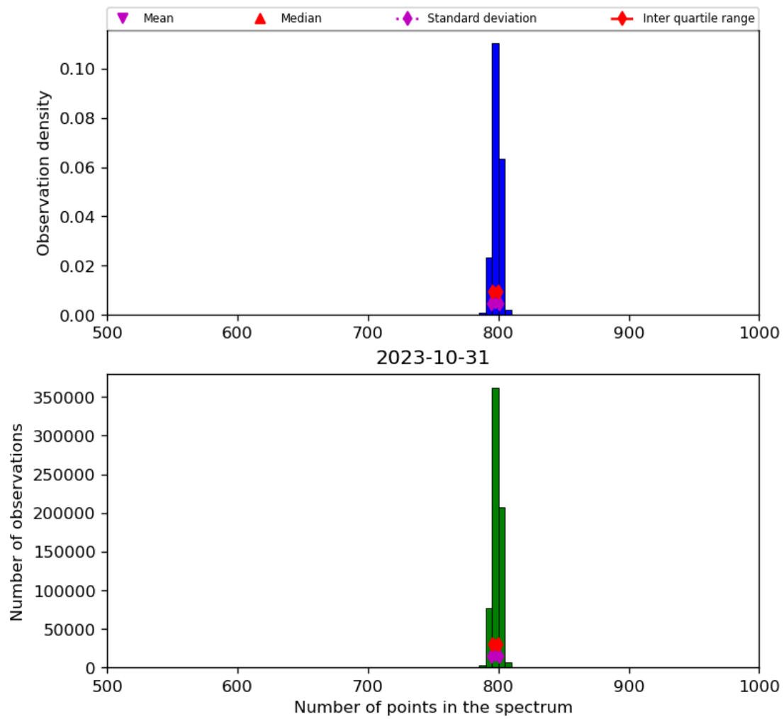
Figure 26: Histogram of “Number of points in the spectrum” for 2023-10-30 to 2023-11-01
