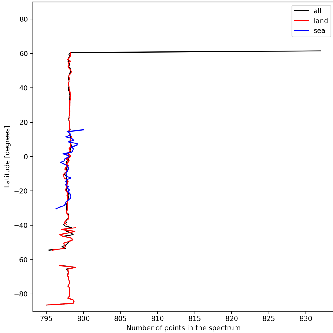
Figure 15: Zonal average of “Number of points in the spectrum” for 2023-10-30 to 2023-11-01.
