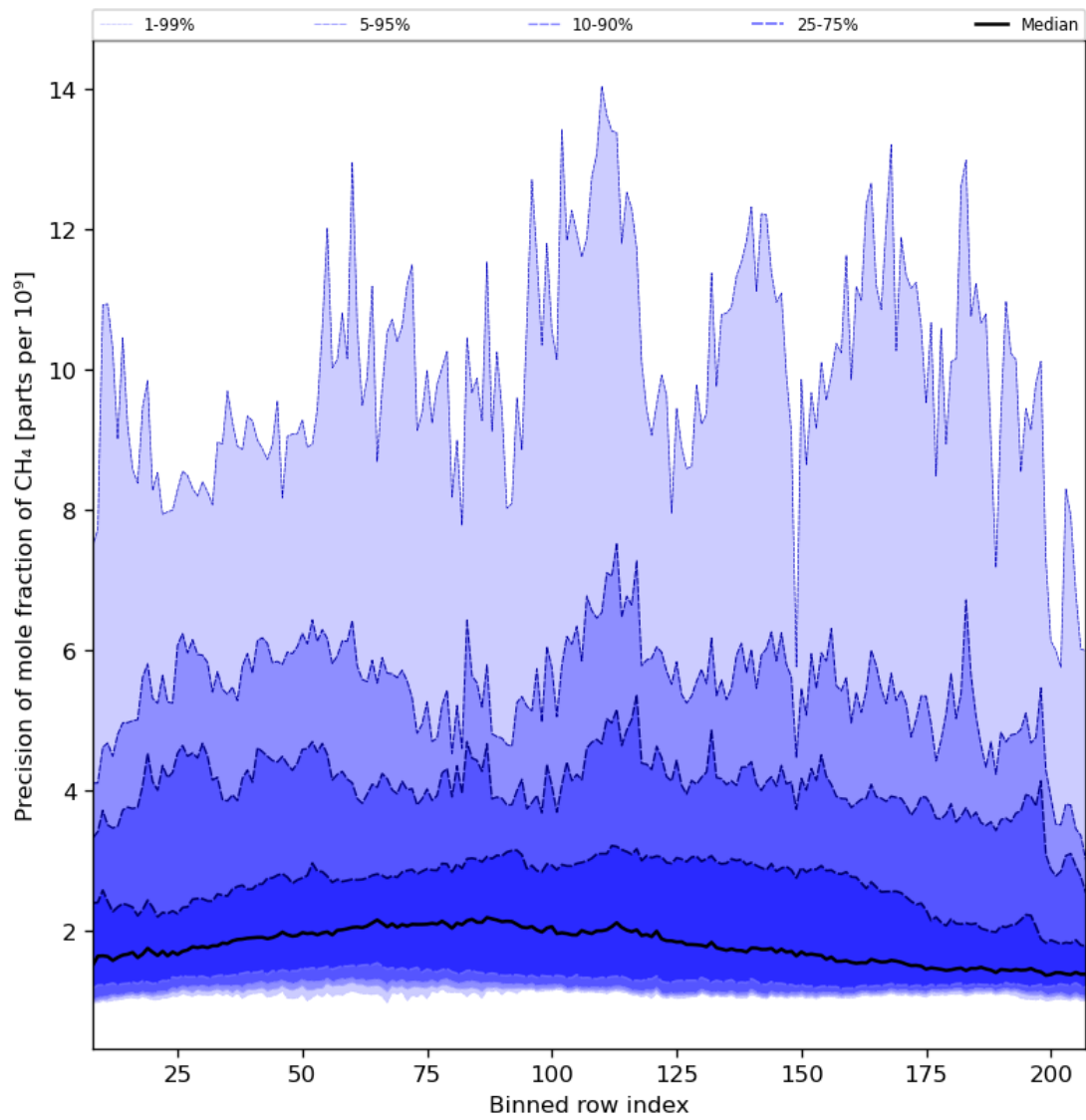
Figure 35: Along track statistics of “Precision of mole fraction of CH 4 ” for 2023-10-30 to 2023-11-01
