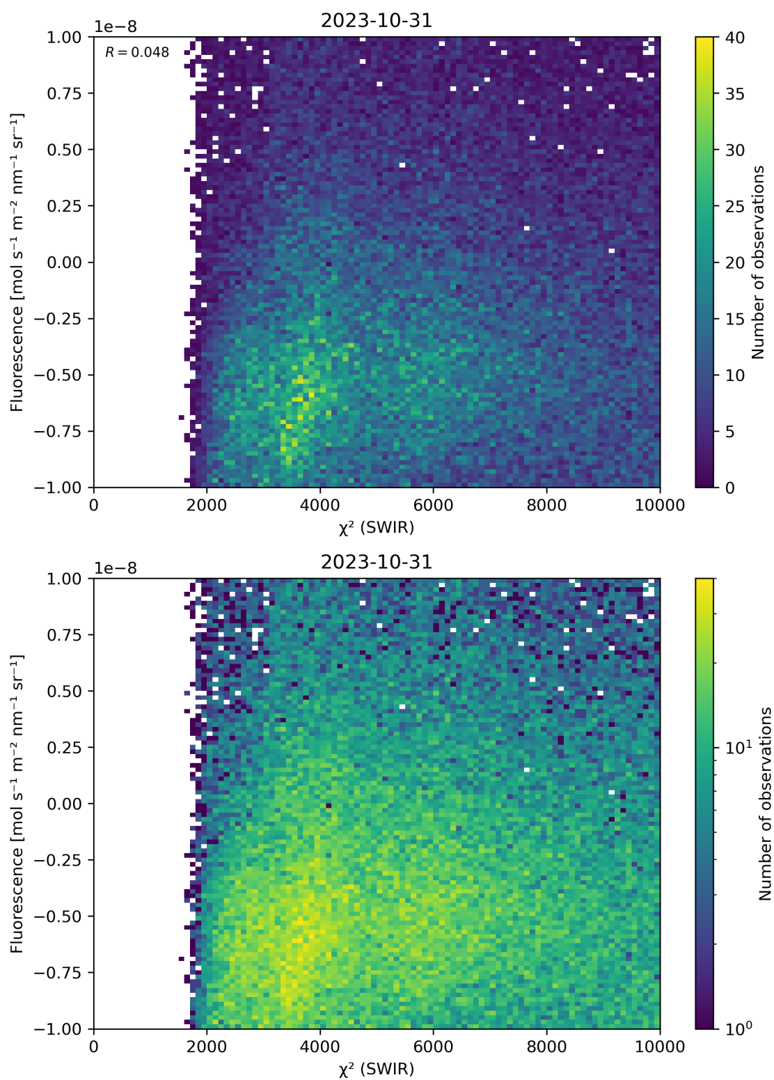
Figure 49: Scatter density plot of “ \chi^2 (SWIR)” against “Fluorescence” for 2023-10-30 to 2023-11-01.
