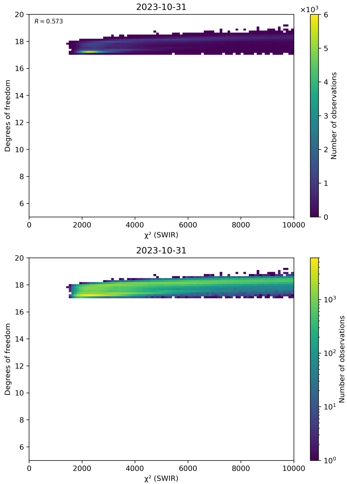
Figure 48: Scatter density plot of “ \chi^2 (SWIR)” against “Degrees of freedom” for 2023-10-30 to 2023-11-01.
