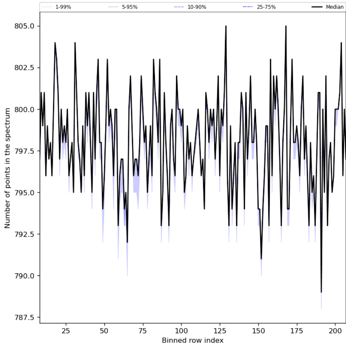
Figure 37: Along track statistics of “Number of points in the spectrum” for 2023-10-30 to 2023-11-01
