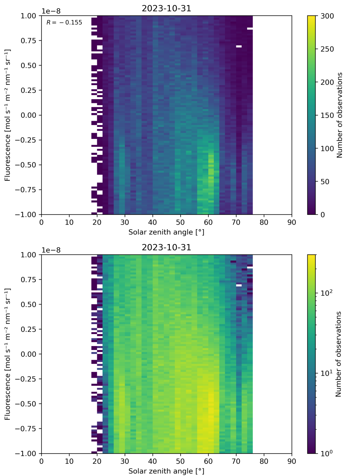
Figure 97: Scatter density plot of “Solar zenith angle” against “Fluorescence” for 2023-10-30 to 2023-11-01.
