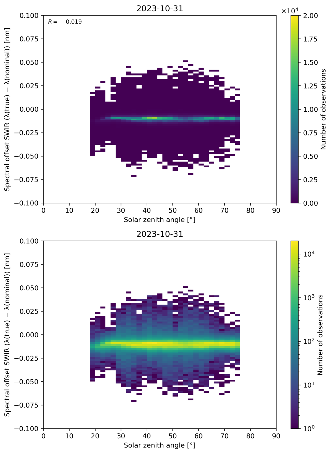
Figure 104: Scatter density plot of “Solar zenith angle” against “Spectral offset SWIR ( \lambda(\text{true}) - \lambda(\text{nominal}) )” for 2023-10-30 to 2023-11-01.
