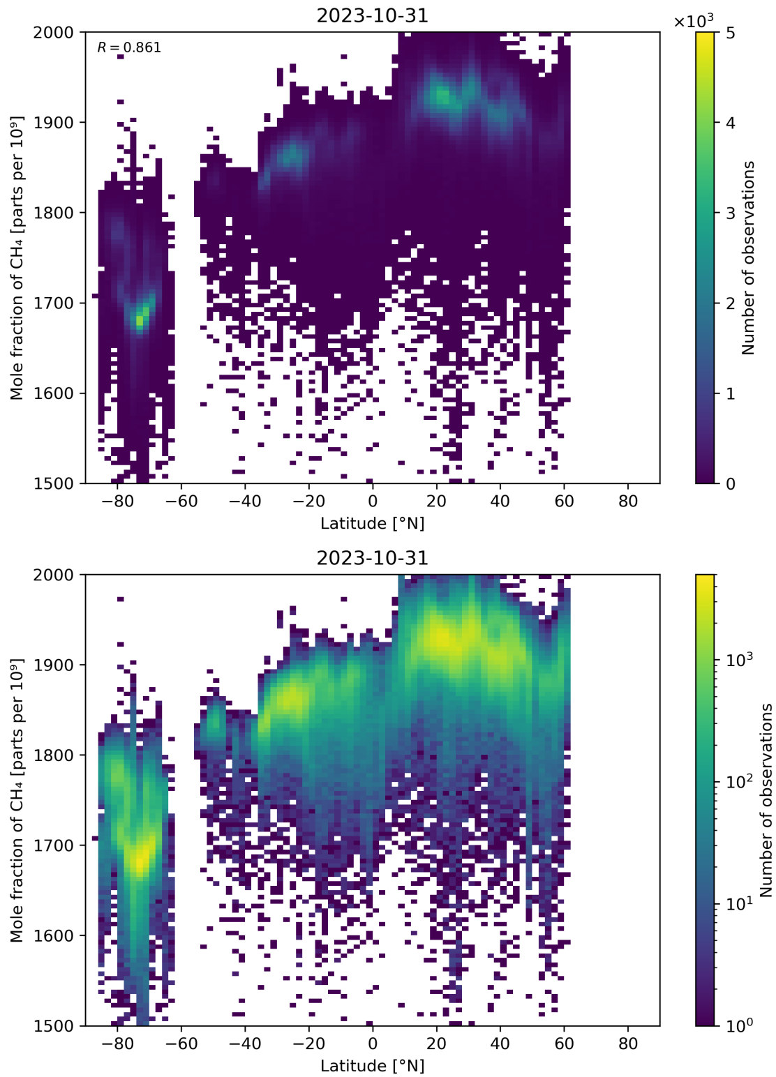
Figure 57: Scatter density plot of “Latitude” against “Mole fraction of CH 4 ” for 2023-10-30 to 2023-11-01.
