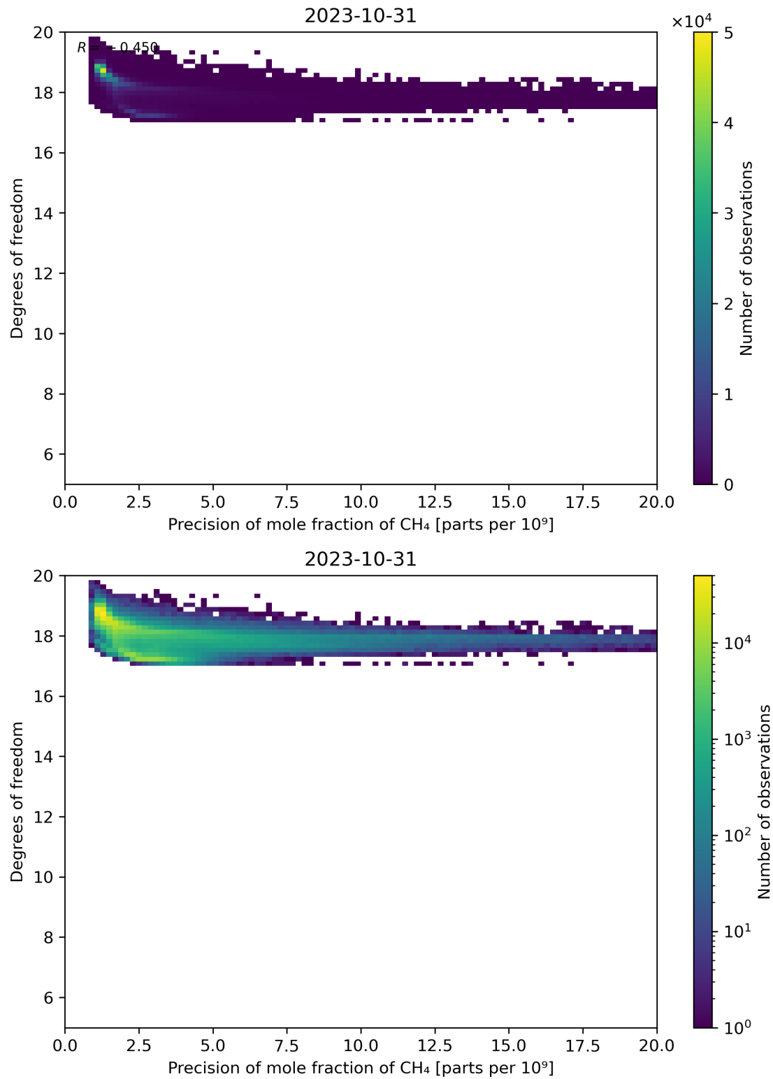
Figure 80: Scatter density plot of “Precision of mole fraction of CH 4 ” against “Degrees of freedom” for 2023-10-30 to 2023-11-01.
