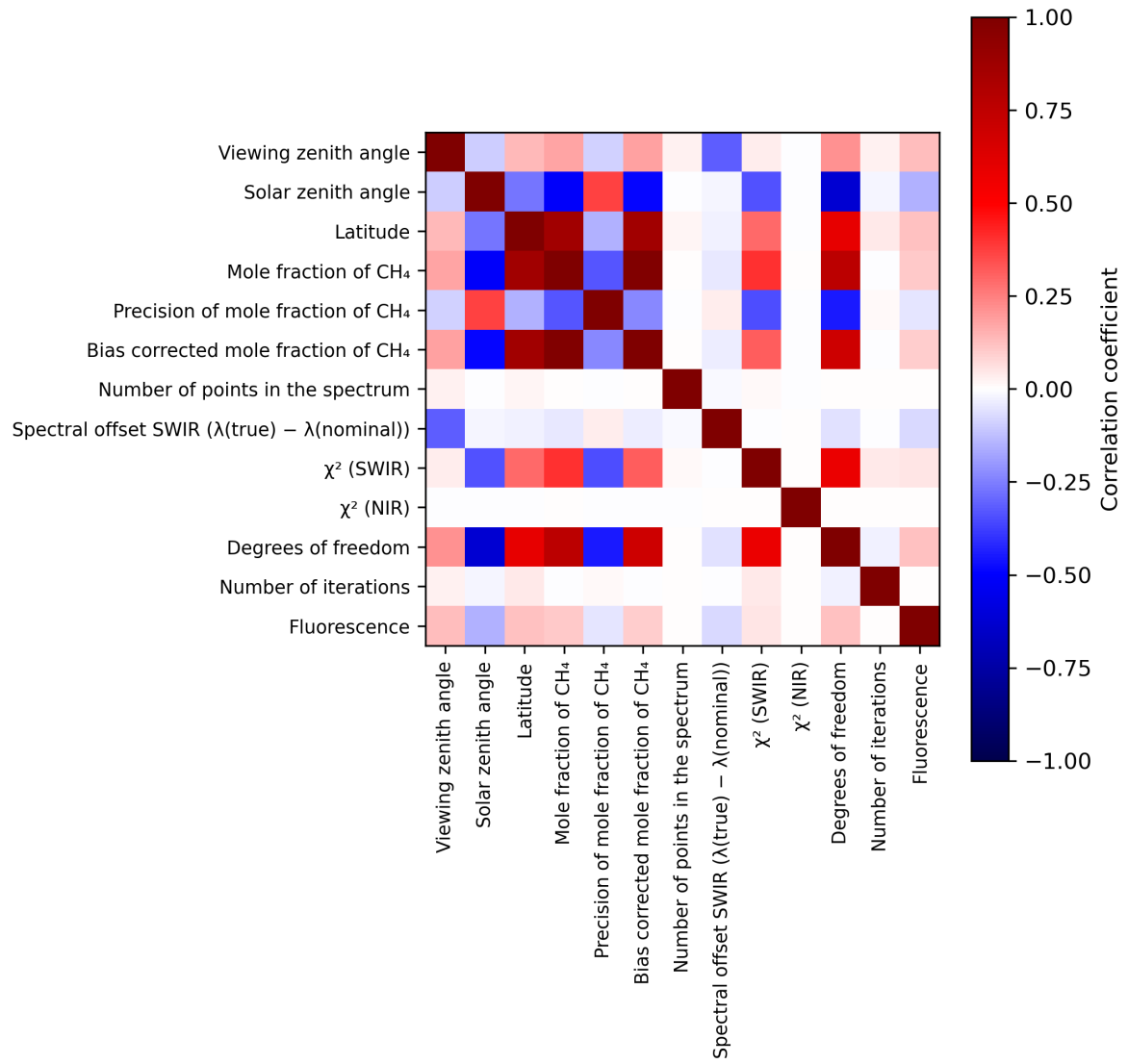
Figure 2: Map of correlation matrix for 2023-10-30 to 2023-11-01.
