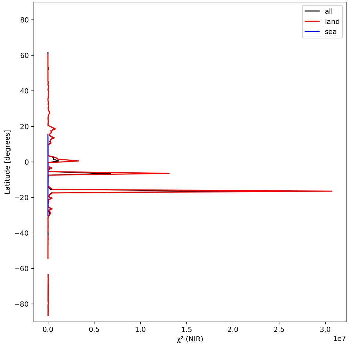
Figure 18: Zonal average of “ \chi^2 (NIR)” for 2023-10-30 to 2023-11-01.
