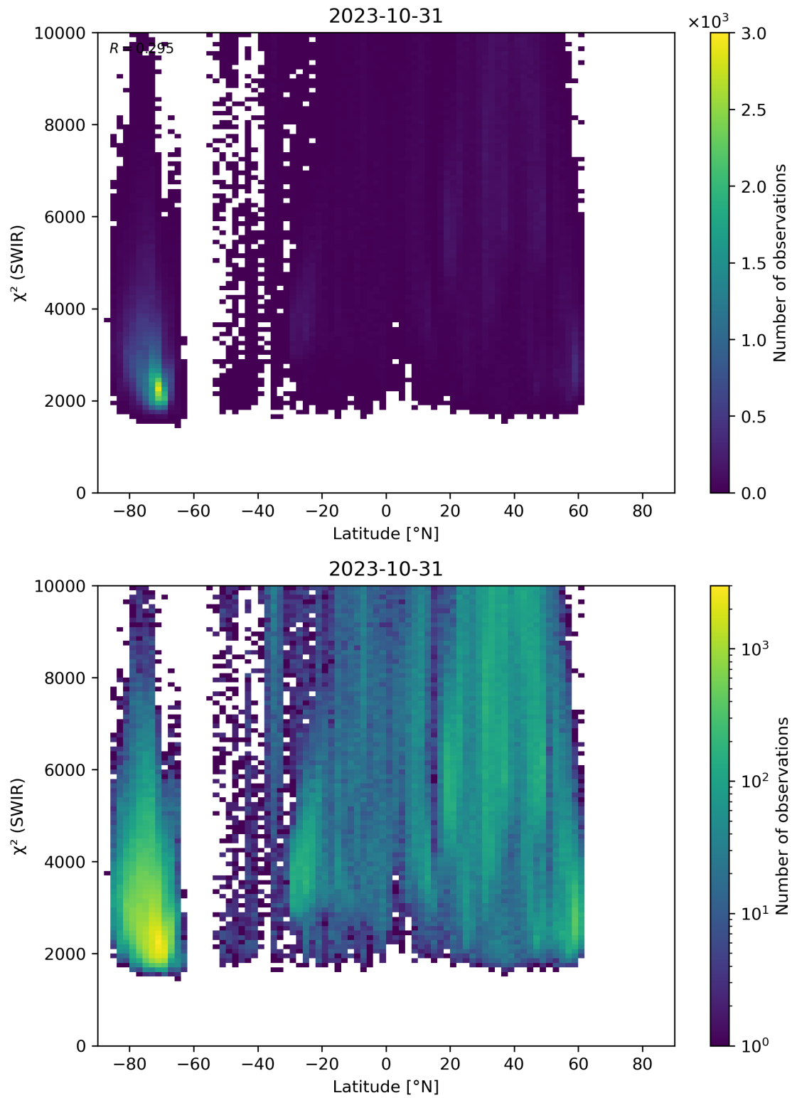
Figure 54: Scatter density plot of “Latitude” against “ \chi^2 (SWIR)” for 2023-10-30 to 2023-11-01.
