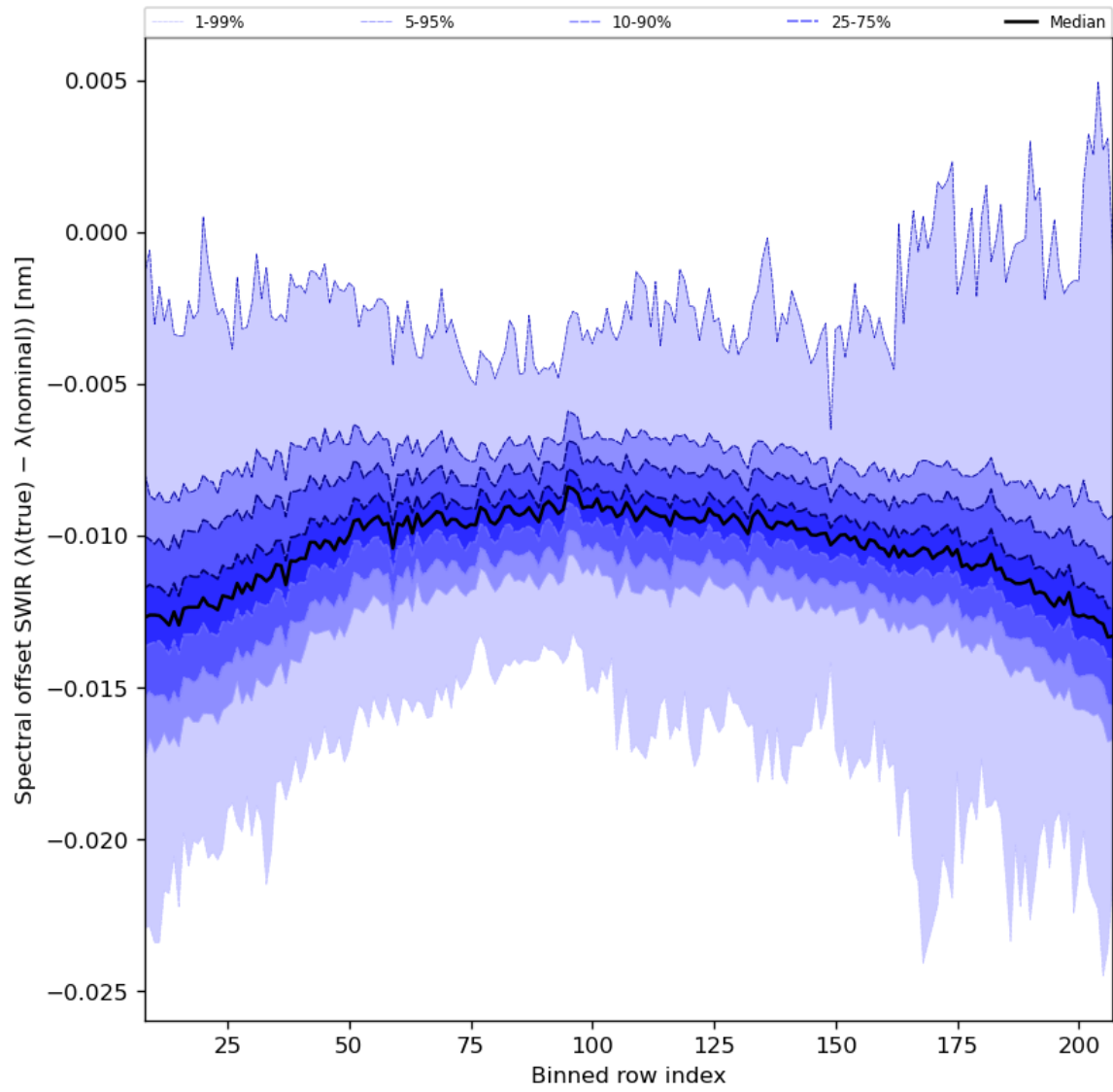
Figure 38: Along track statistics of “Spectral offset SWIR ( \lambda(\text{true}) - \lambda(\text{nominal}) )” for 2023-10-30 to 2023-11-01
