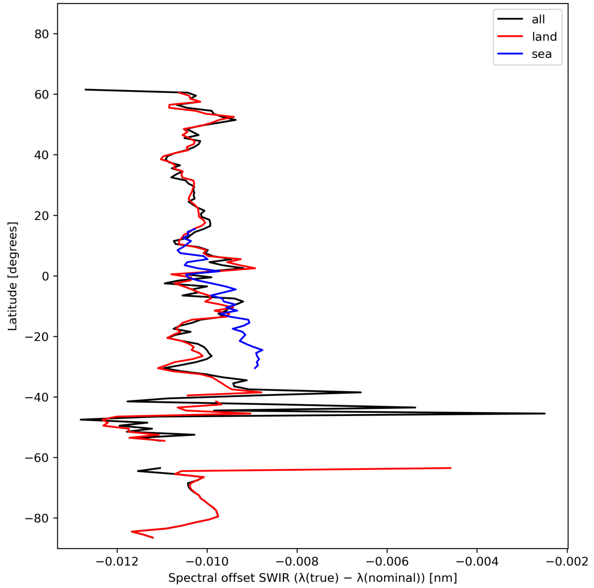
Figure 16: Zonal average of “Spectral offset SWIR ( \lambda(\text{true}) - \lambda(\text{nominal}) )” for 2023-10-30 to 2023-11-01.
