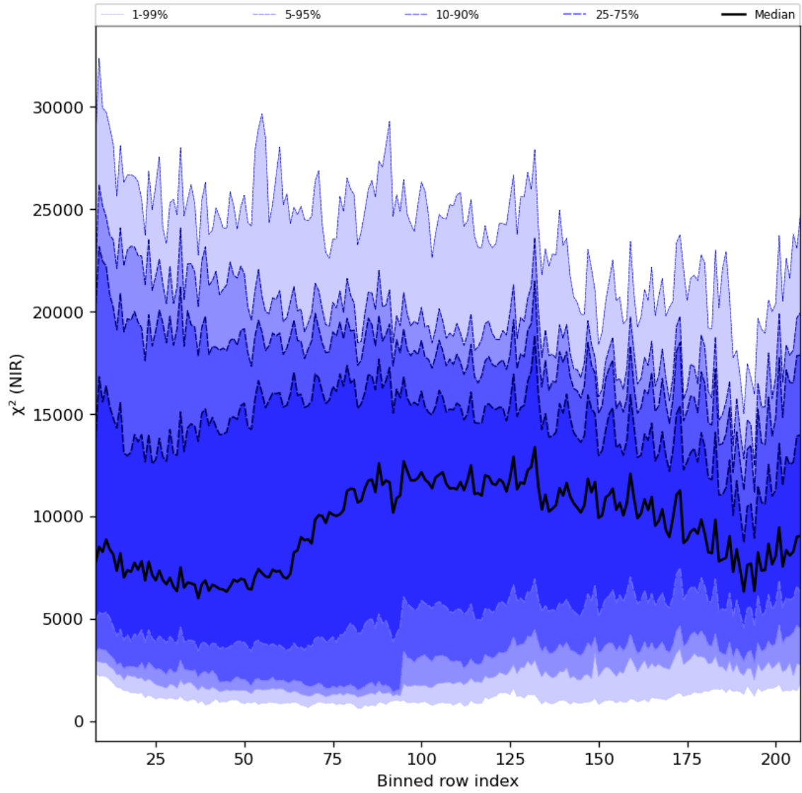
Figure 40: Along track statistics of “ \chi^2 (NIR)” for 2023-10-30 to 2023-11-01
