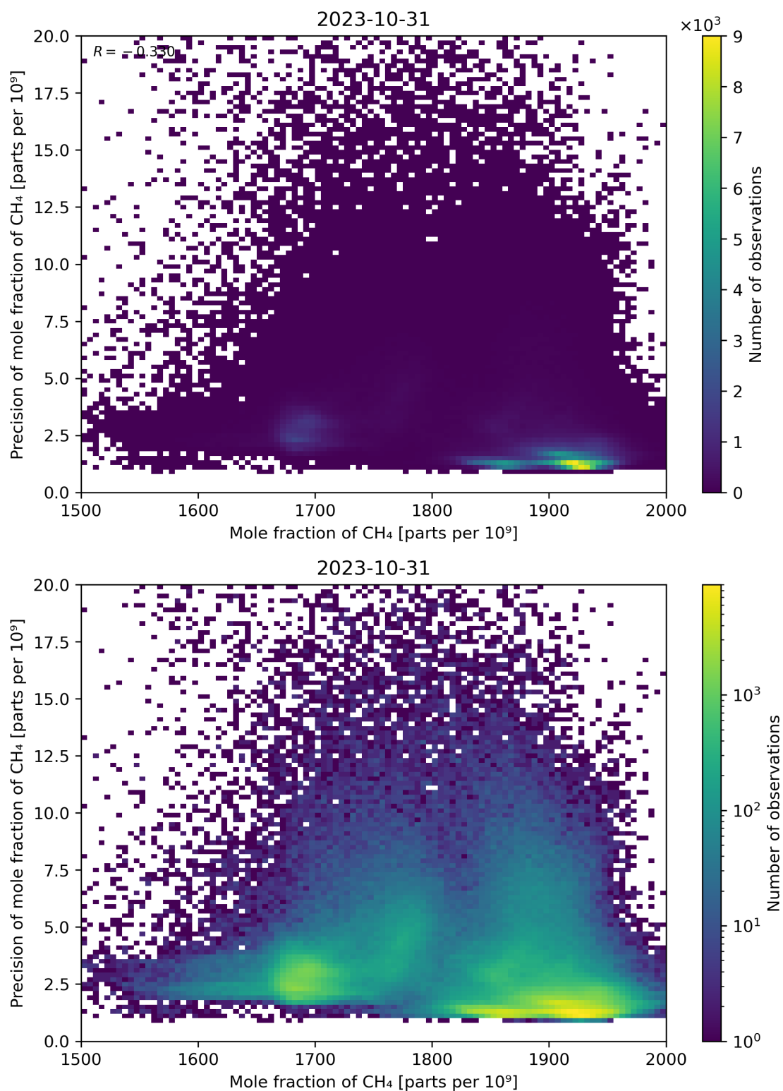
Figure 75: Scatter density plot of “Mole fraction of CH 4 ” against “Precision of mole fraction of CH 4 ” for 2023-10-30 to 2023-11-01.
