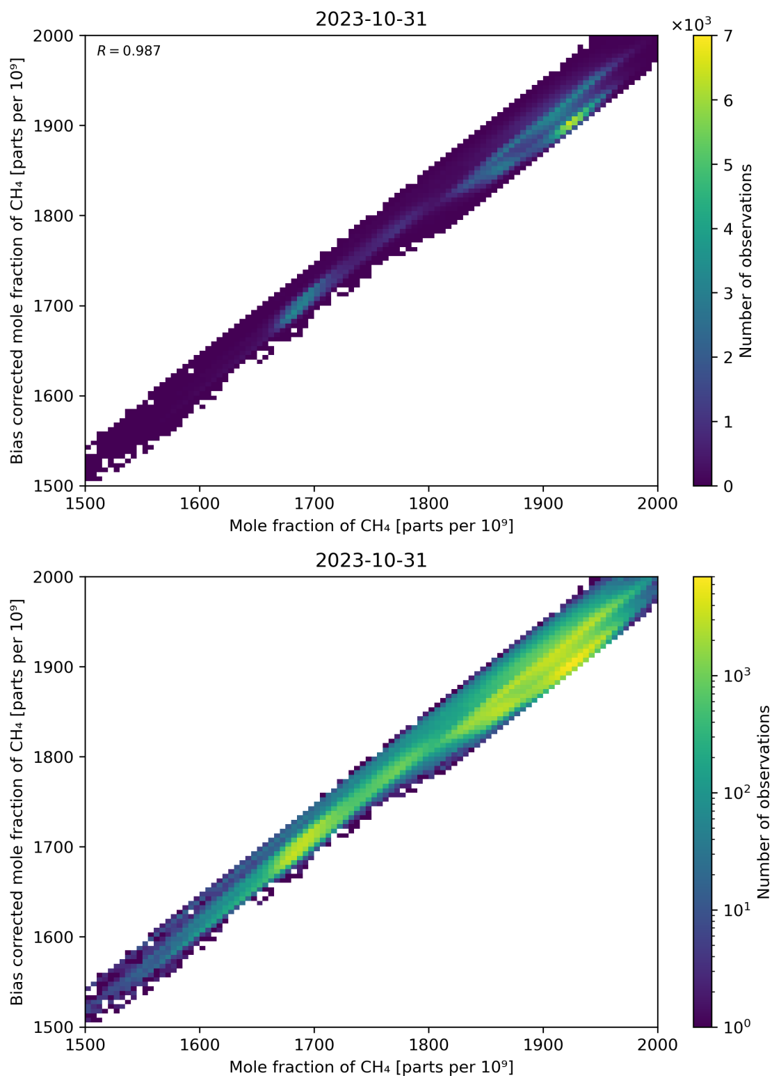
Figure 74: Scatter density plot of “Mole fraction of CH 4 ” against “Bias corrected mole fraction of CH 4 ” for 2023-10-30 to 2023-11-01.
