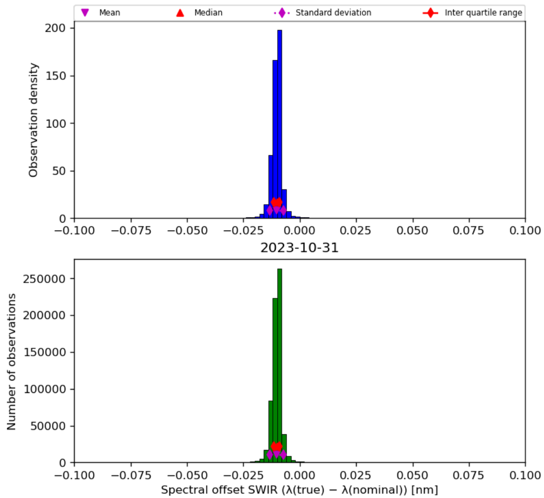
Figure 27: Histogram of “Spectral offset SWIR ( \lambda(\text{true}) - \lambda(\text{nominal}) )” for 2023-10-30 to 2023-11-01
