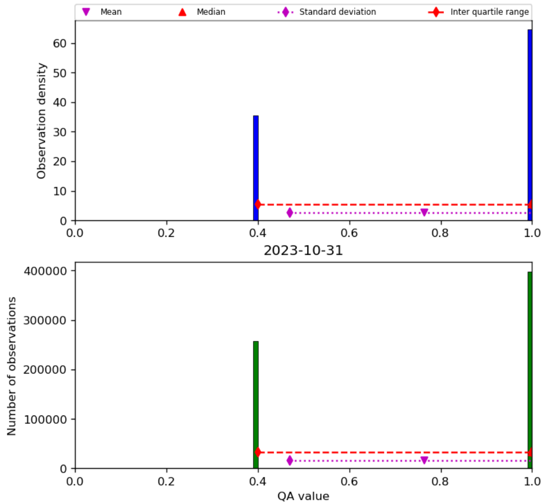
Figure 22: Histogram of “QA value” for 2023-10-30 to 2023-11-01
