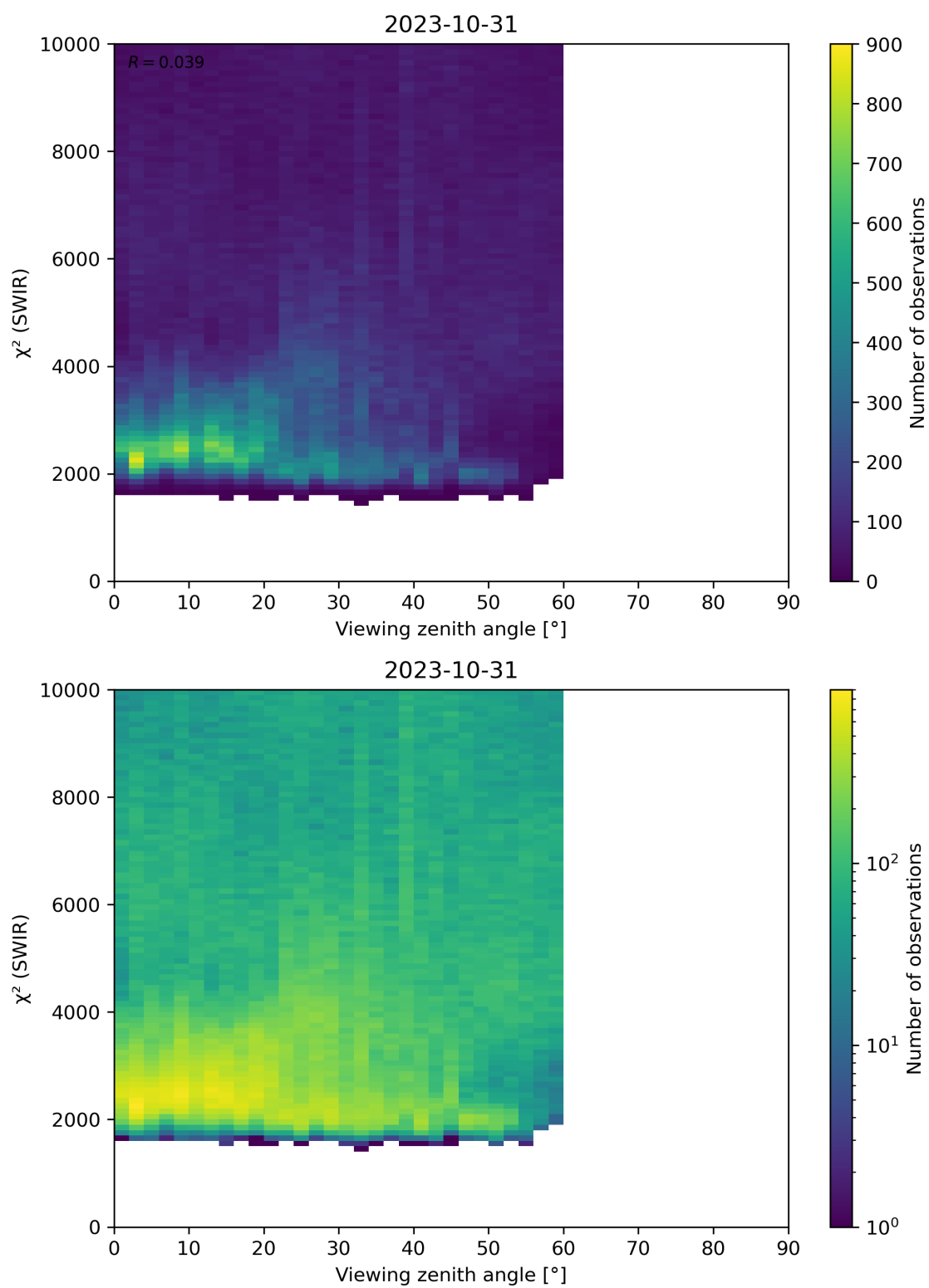
Figure 106: Scatter density plot of “Viewing zenith angle” against “ \chi^2 (SWIR)” for 2023-10-30 to 2023-11-01.
