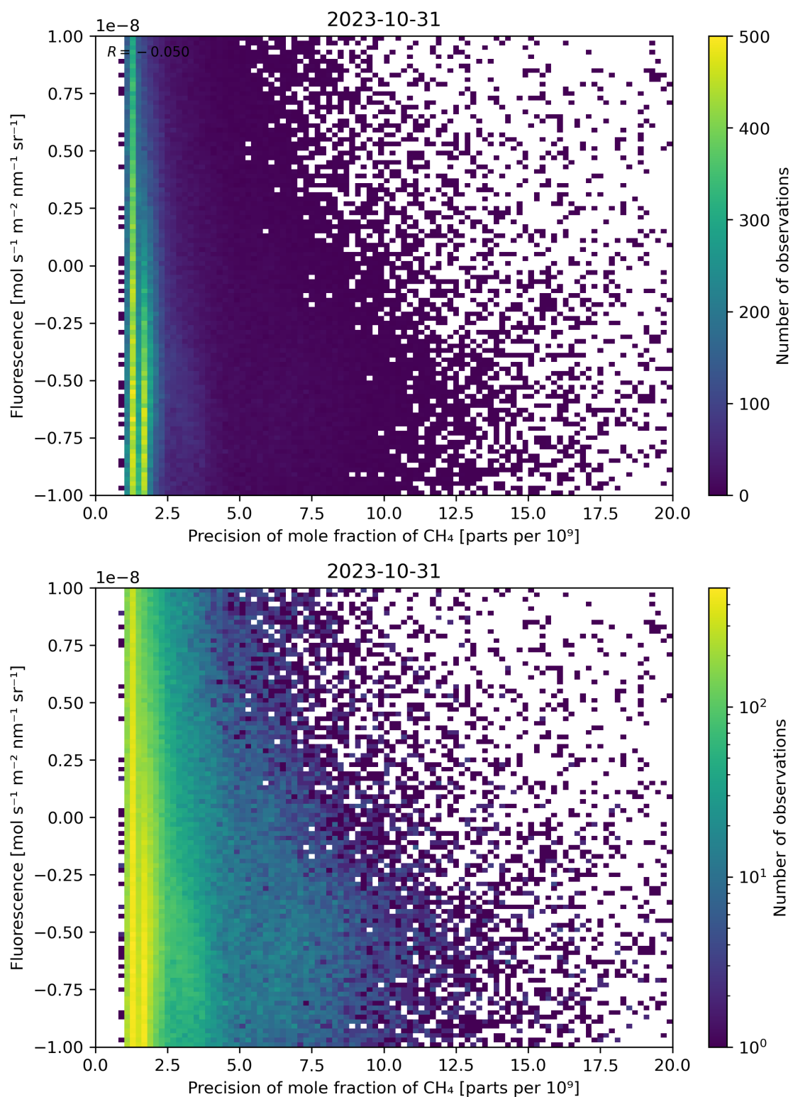
Figure 81: Scatter density plot of “Precision of mole fraction of \text{CH}_4 ” against “Fluorescence” for 2023-10-30 to 2023-11-01.
