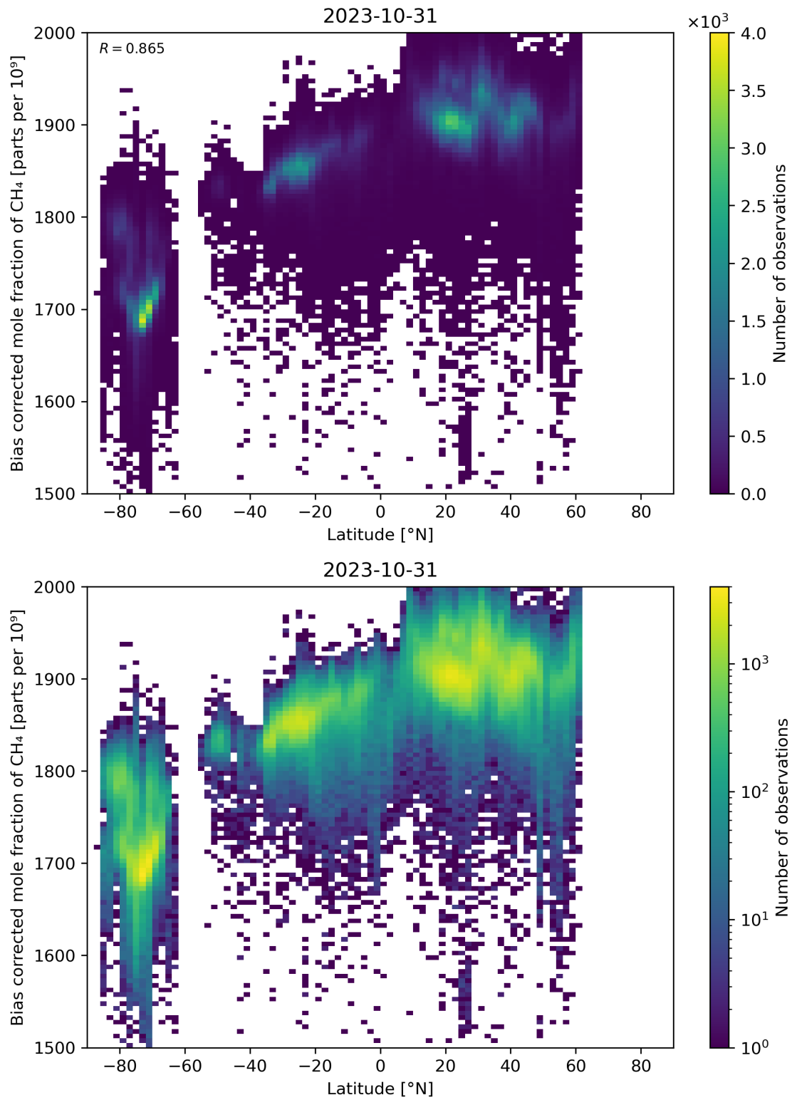
Figure 58: Scatter density plot of “Latitude” against “Bias corrected mole fraction of CH 4 ” for 2023-10-30 to 2023-11-01.
