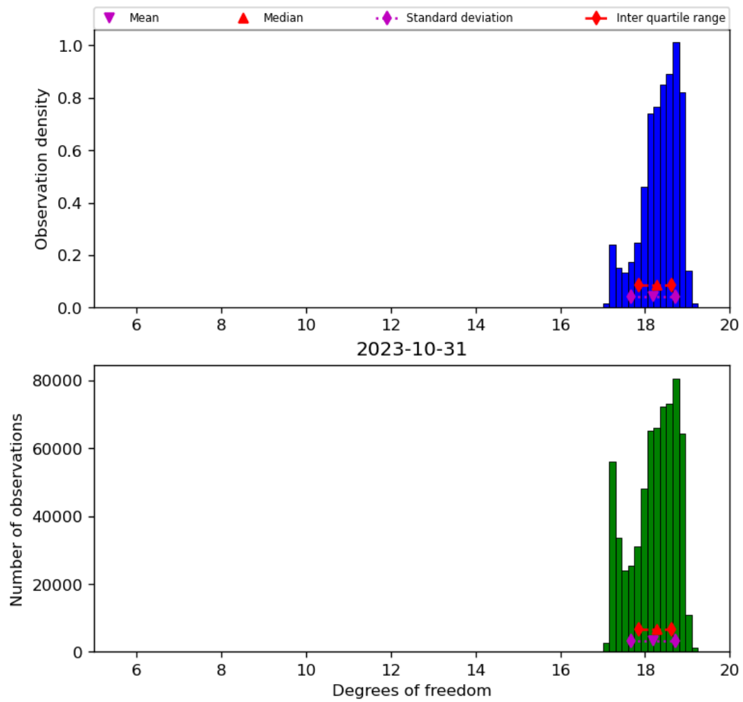
Figure 30: Histogram of “Degrees of freedom” for 2023-10-30 to 2023-11-01
