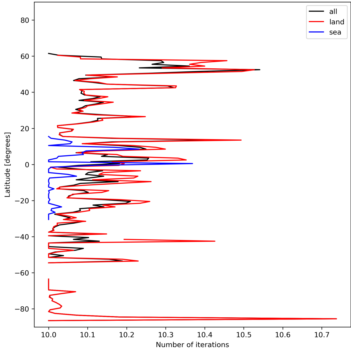
Figure 20: Zonal average of “Number of iterations” for 2023-10-30 to 2023-11-01.
