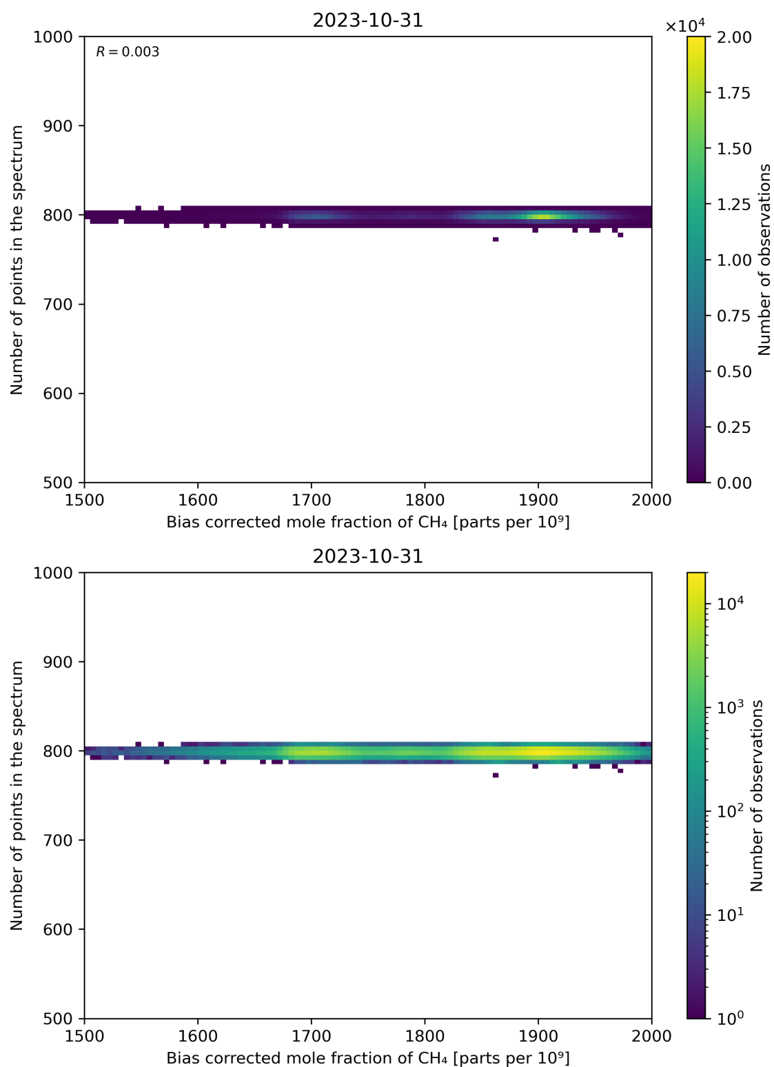
Figure 68: Scatter density plot of “Bias corrected mole fraction of CH 4 ” against “Number of points in the spectrum” for 2023-10-30 to 2023-11-01.
