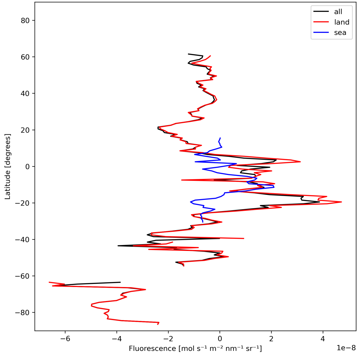
Figure 21: Zonal average of “Fluorescence” for 2023-10-30 to 2023-11-01.
