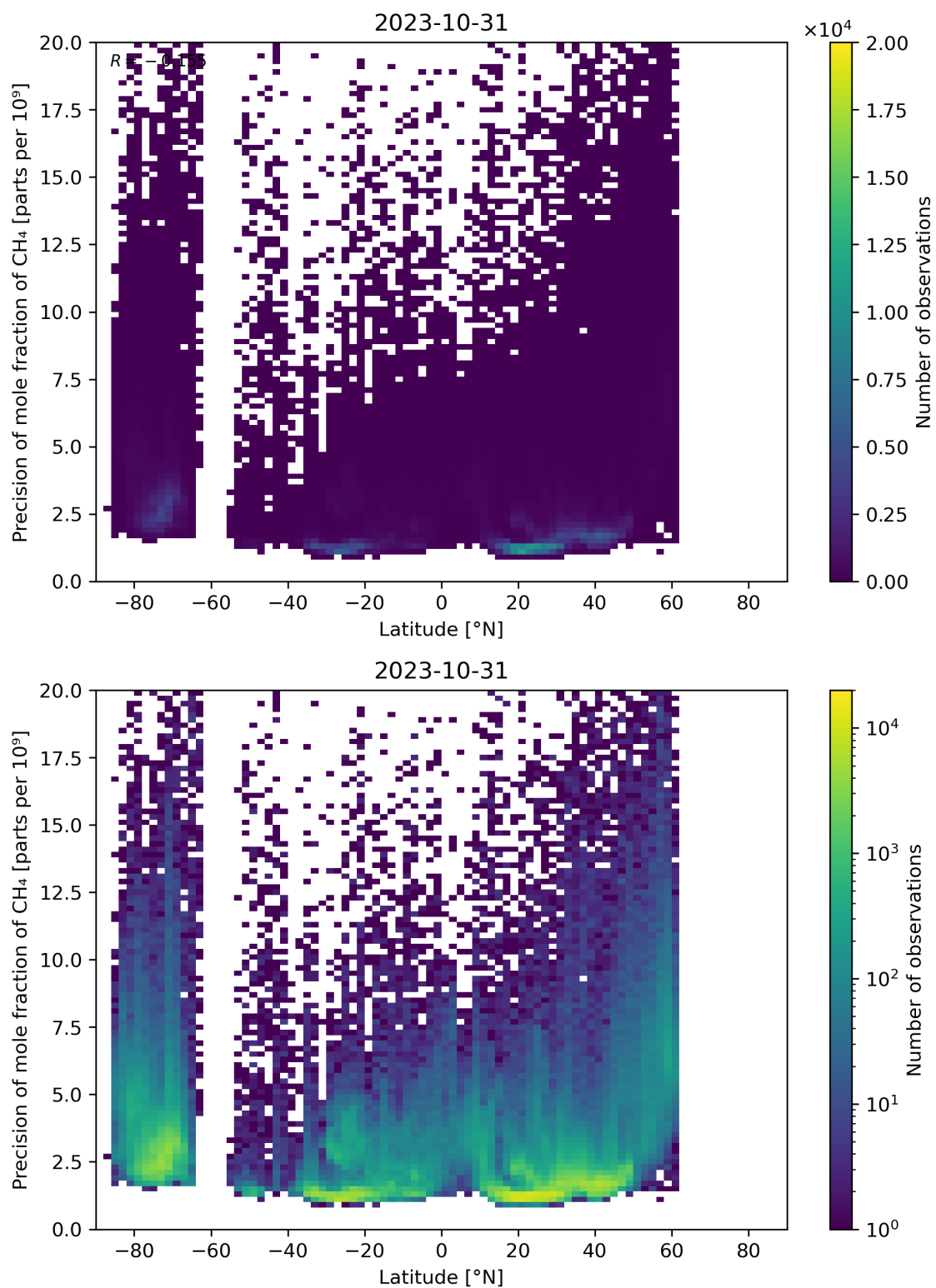
Figure 59: Scatter density plot of “Latitude” against “Precision of mole fraction of CH 4 ” for 2023-10-30 to 2023-11-01.
