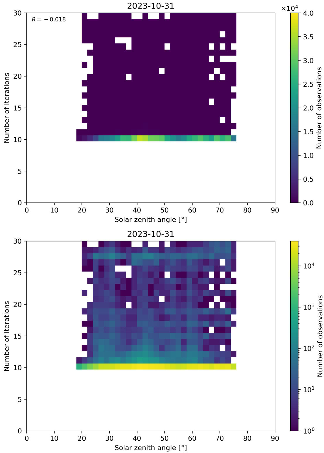
Figure 102: Scatter density plot of “Solar zenith angle” against “Number of iterations” for 2023-10-30 to 2023-11-01.
