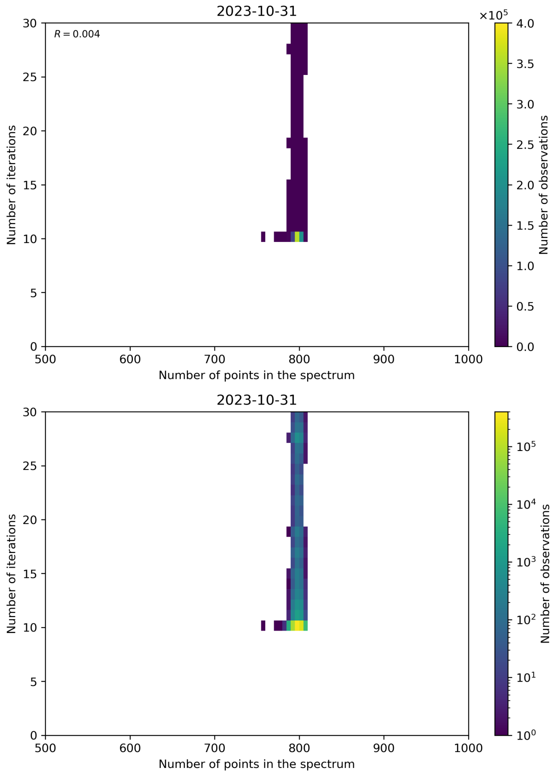
Figure 92: Scatter density plot of “Number of points in the spectrum” against “Number of iterations” for 2023-10-30 to 2023-11-01.
