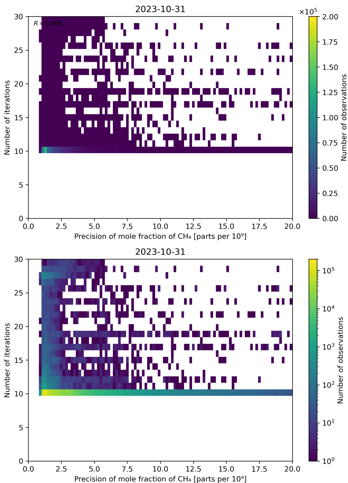
Figure 83: Scatter density plot of “Precision of mole fraction of CH 4 ” against “Number of iterations” for 2023-10-30 to 2023-11-01.
