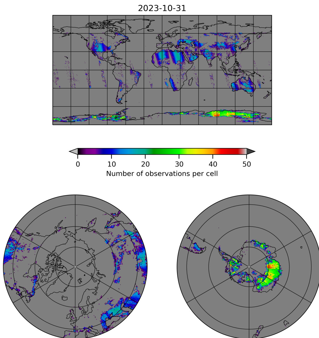
Figure 10: Map of the number of observations for 2023-10-30 to 2023-11-01
