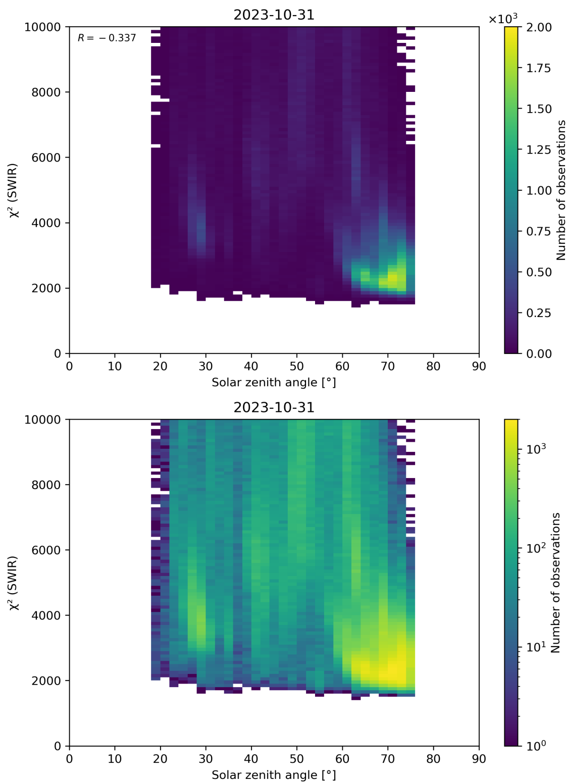
Figure 95: Scatter density plot of “Solar zenith angle” against “ \chi^2 (SWIR)” for 2023-10-30 to 2023-11-01.
