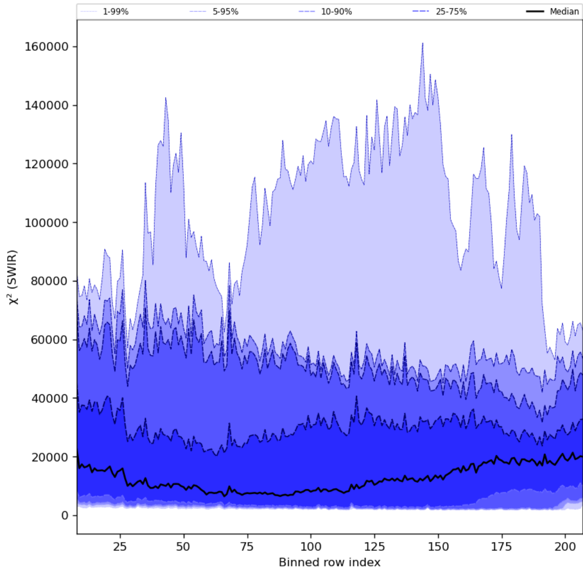
Figure 39: Along track statistics of “ \chi^2 (SWIR)” for 2023-10-30 to 2023-11-01
