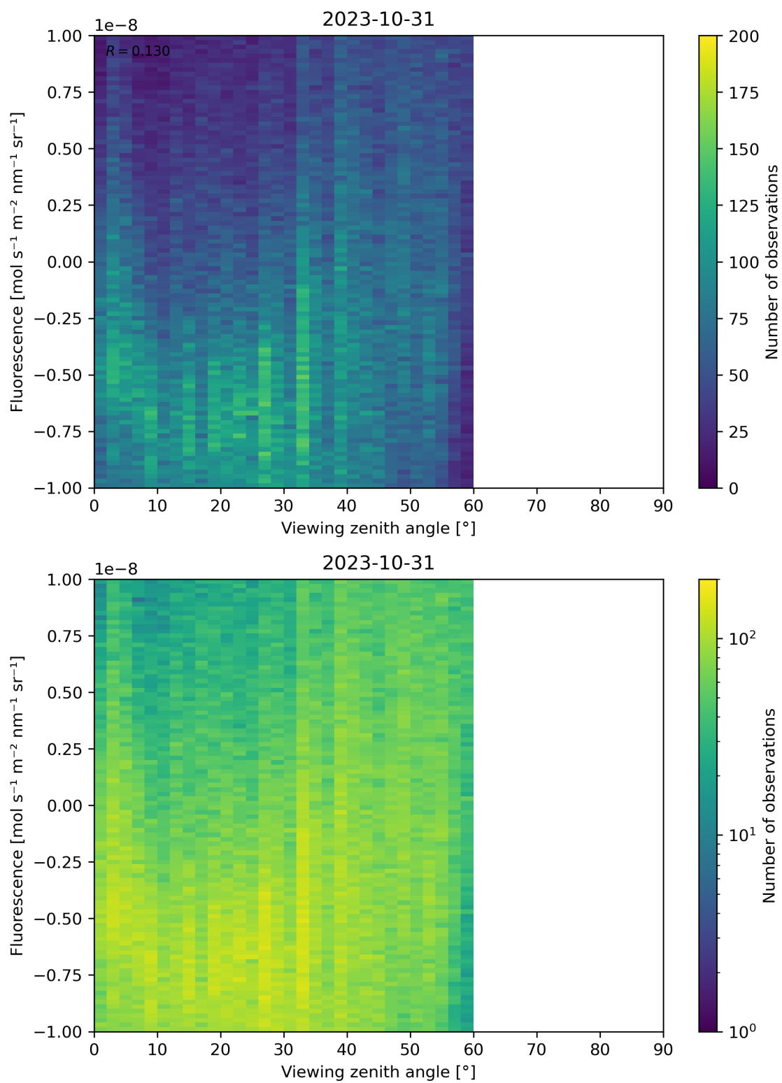
Figure 108: Scatter density plot of “Viewing zenith angle” against “Fluorescence” for 2023-10-30 to 2023-11-01.
