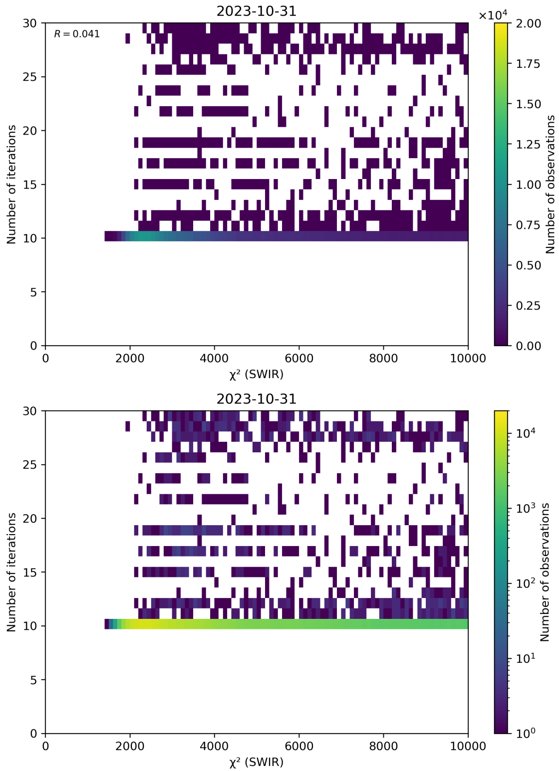
Figure 50: Scatter density plot of “ \chi^2 (SWIR)” against “Number of iterations” for 2023-10-30 to 2023-11-01.
