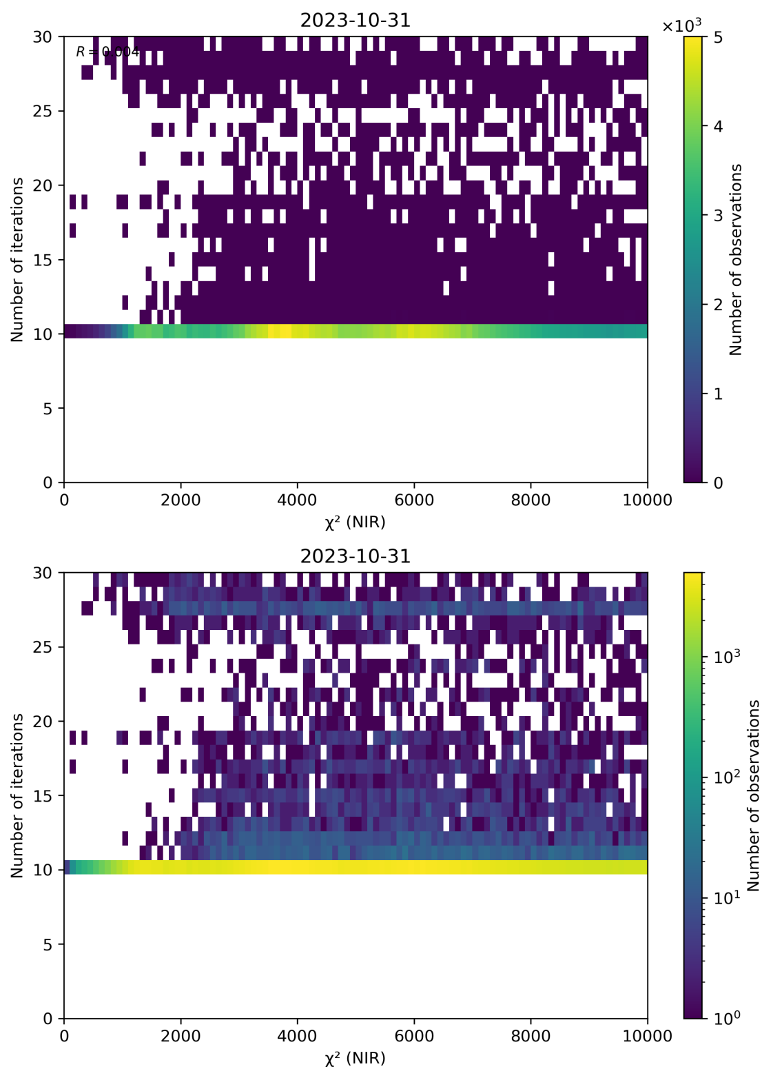
Figure 46: Scatter density plot of “ \chi^2 (NIR)” against “Number of iterations” for 2023-10-30 to 2023-11-01.
