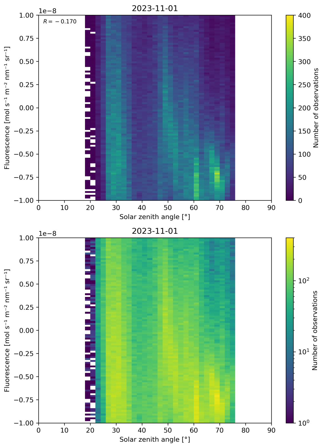
Figure 97: Scatter density plot of “Solar zenith angle” against “Fluorescence” for 2023-10-31 to 2023-11-02.
