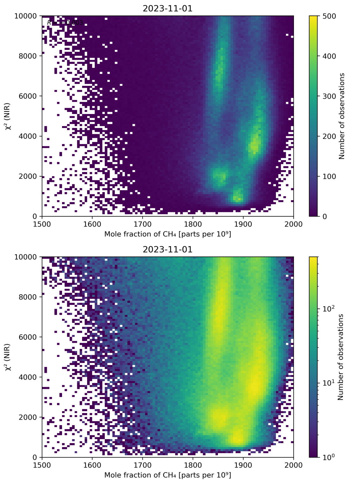
Figure 70: Scatter density plot of “Mole fraction of \text{CH}_4 ” against “ \chi^2 (NIR)” for 2023-10-31 to 2023-11-02.
