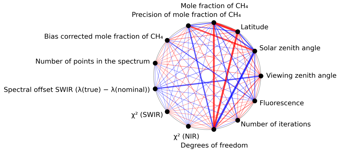
Figure 1: Map of correlation graph for 2023-10-31 to 2023-11-02.
