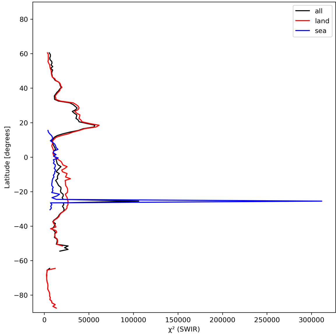
Figure 17: Zonal average of “ \chi^2 (SWIR)” for 2023-10-31 to 2023-11-02.
