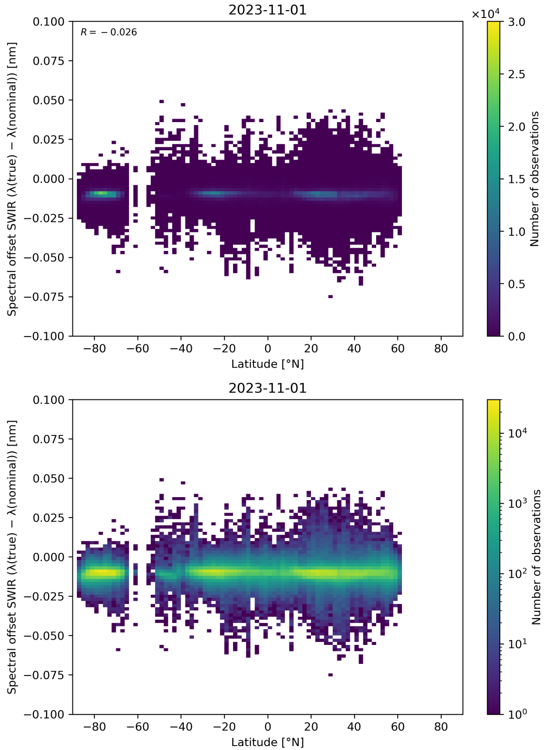
Figure 62: Scatter density plot of “Latitude” against “Spectral offset SWIR ( \lambda(\text{true}) - \lambda(\text{nominal}) )” for 2023-10-31 to 2023-11-02.
