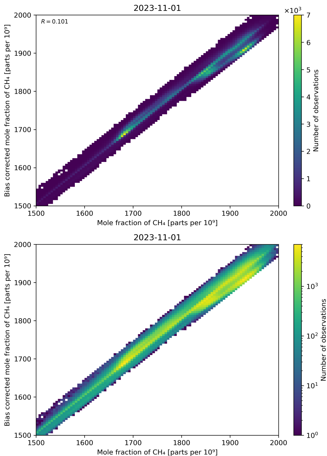
Figure 74: Scatter density plot of “Mole fraction of CH 4 ” against “Bias corrected mole fraction of CH 4 ” for 2023-10-31 to 2023-11-02.
