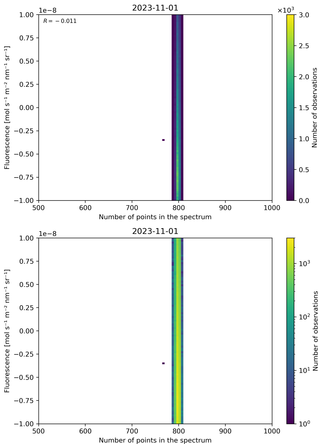
Figure 91: Scatter density plot of “Number of points in the spectrum” against “Fluorescence” for 2023-10-31 to 2023-11-02.
