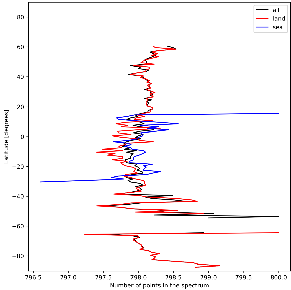
Figure 15: Zonal average of “Number of points in the spectrum” for 2023-10-31 to 2023-11-02.
