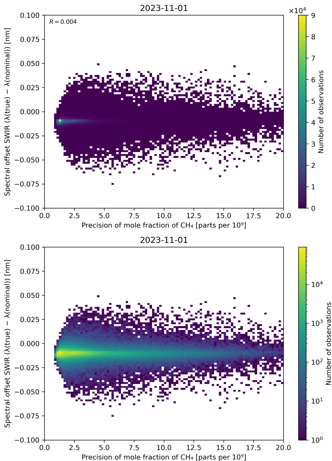
Figure 85: Scatter density plot of “Precision of mole fraction of \text{CH}_4 ” against “Spectral offset SWIR ( \lambda(\text{true}) - \lambda(\text{nominal}) )” for 2023-10-31 to 2023-11-02.
