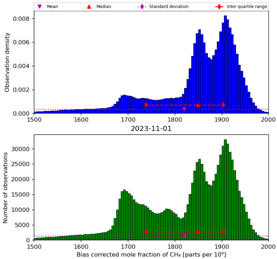
Figure 25: Histogram of “Bias corrected mole fraction of CH 4 ” for 2023-10-31 to 2023-11-02
