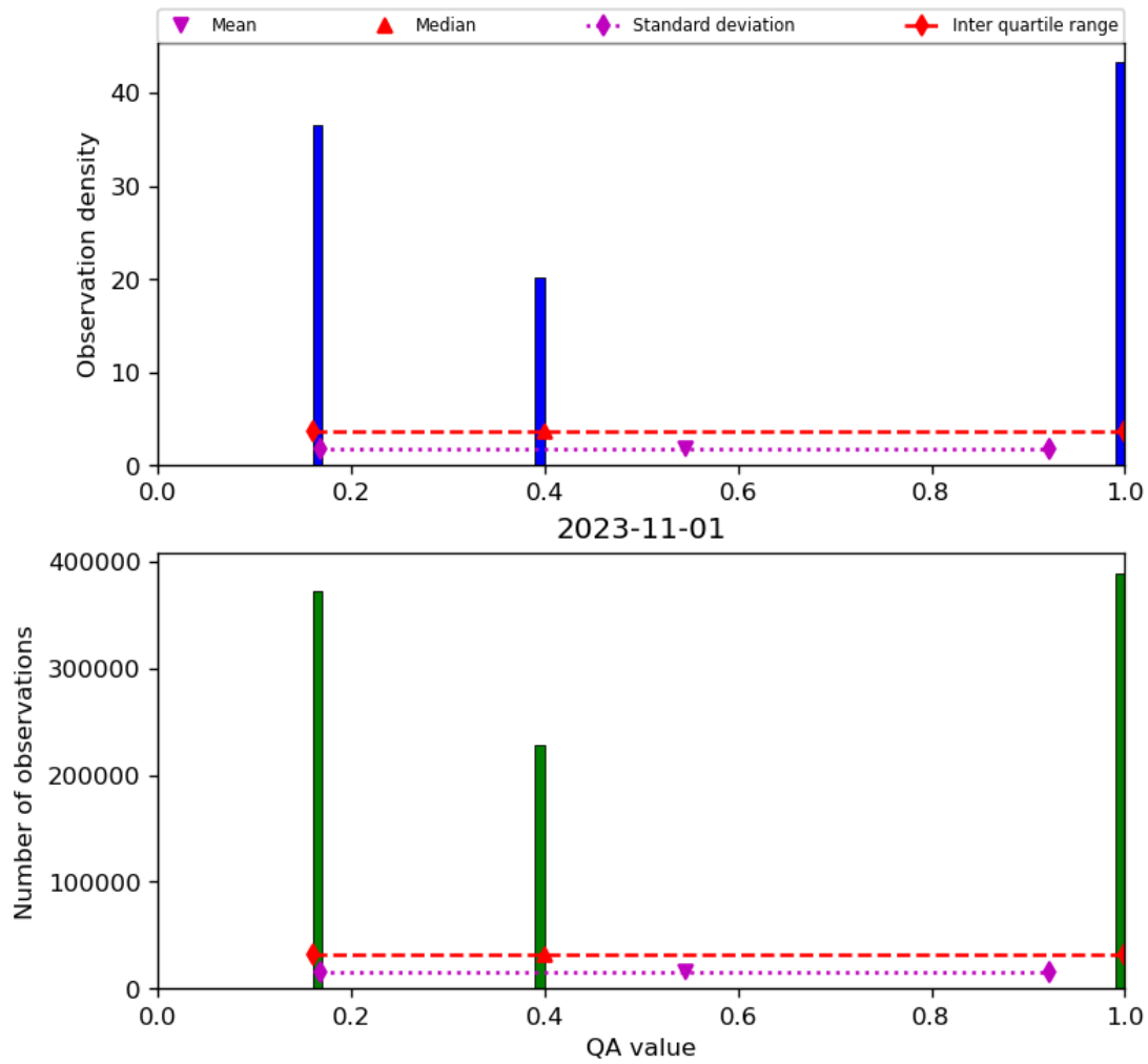
Figure 22: Histogram of “QA value” for 2023-10-31 to 2023-11-02
