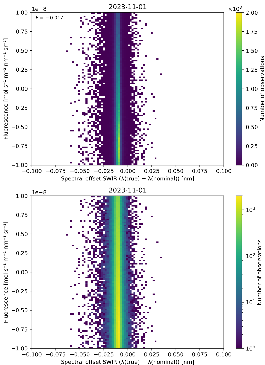
Figure 120: Scatter density plot of “Spectral offset SWIR ( \lambda(\text{true}) - \lambda(\text{nominal}) )” against “Fluorescence” for 2023-10-31 to 2023-11-02.
