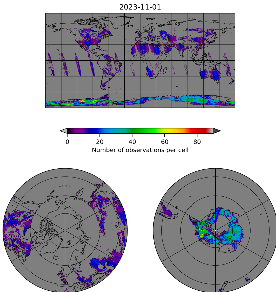
Figure 10: Map of the number of observations for 2023-10-31 to 2023-11-02
