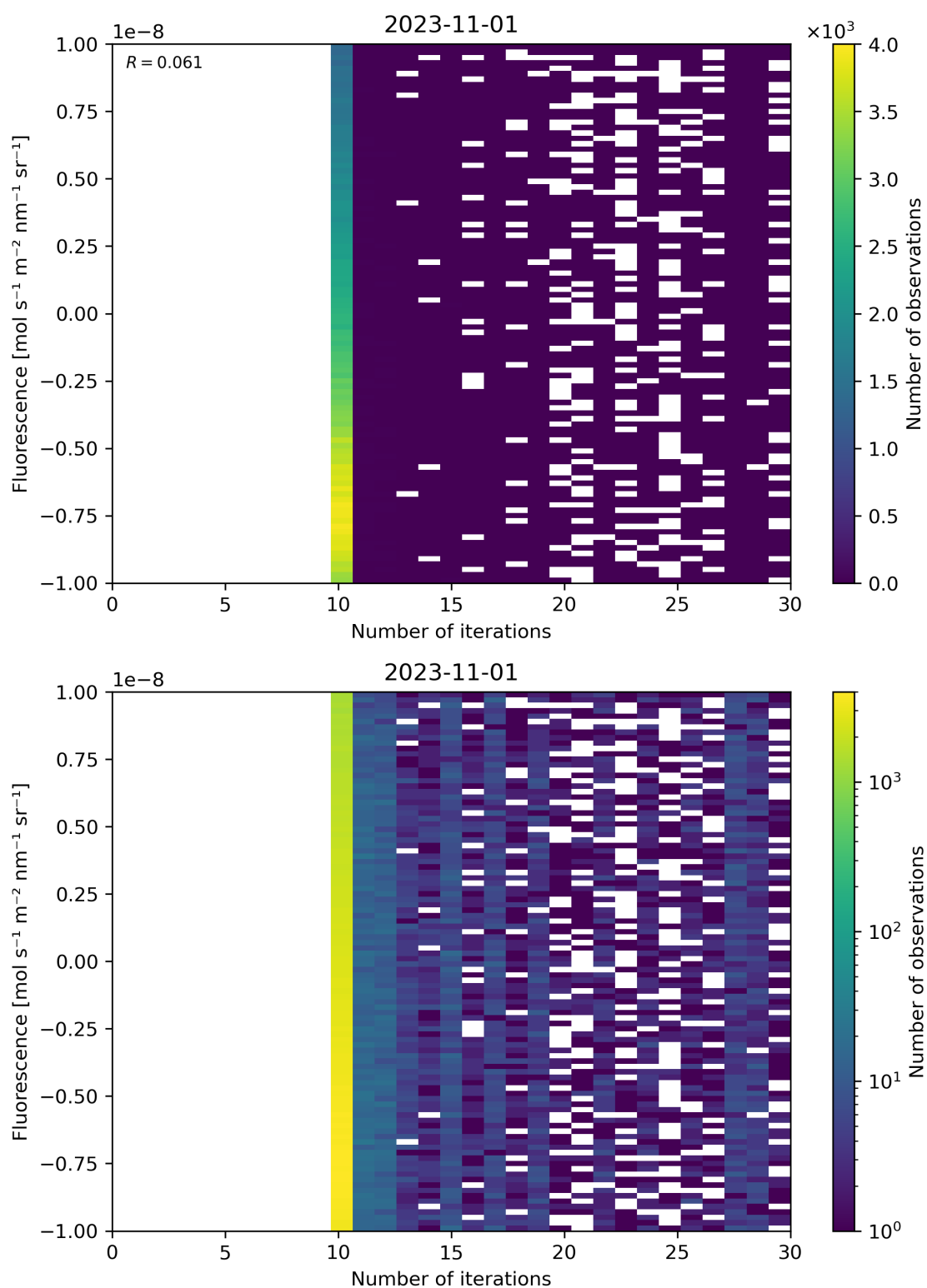
Figure 87: Scatter density plot of “Number of iterations” against “Fluorescence” for 2023-10-31 to 2023-11-02.
