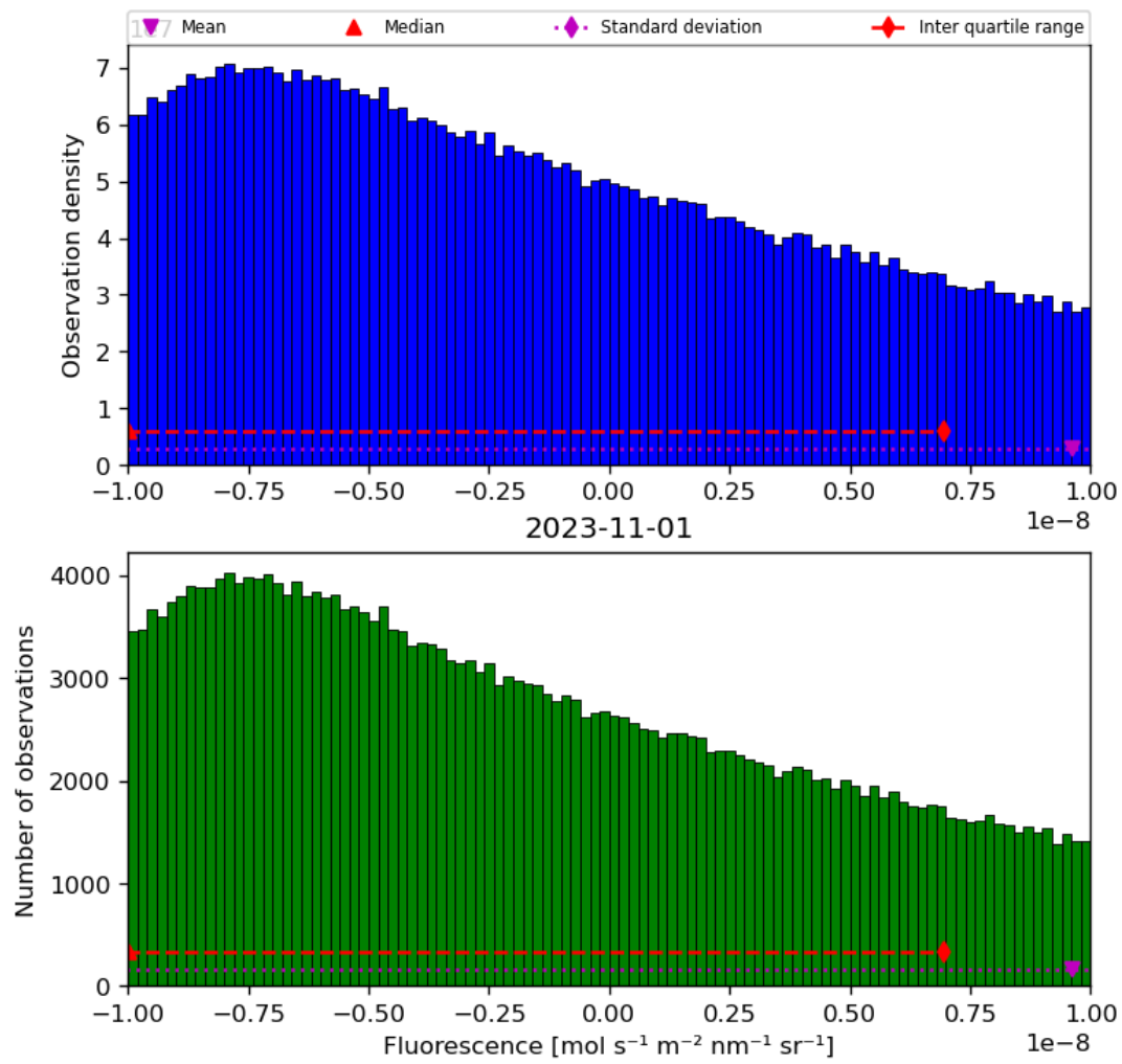
Figure 32: Histogram of “Fluorescence” for 2023-10-31 to 2023-11-02
