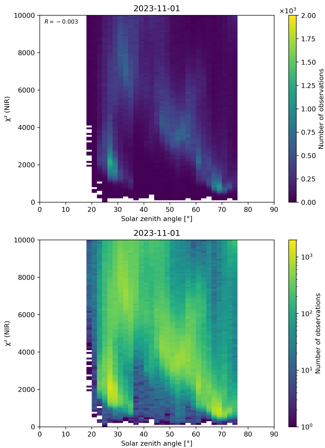
Figure 94: Scatter density plot of “Solar zenith angle” against “ \chi^2 (NIR)” for 2023-10-31 to 2023-11-02.
