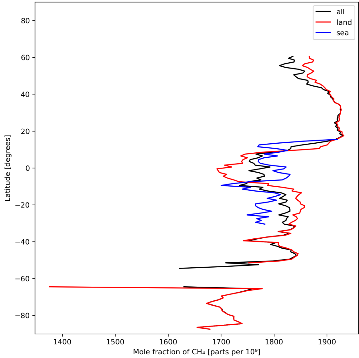
Figure 12: Zonal average of “Mole fraction of \text{CH}_4 ” for 2023-10-31 to 2023-11-02.
