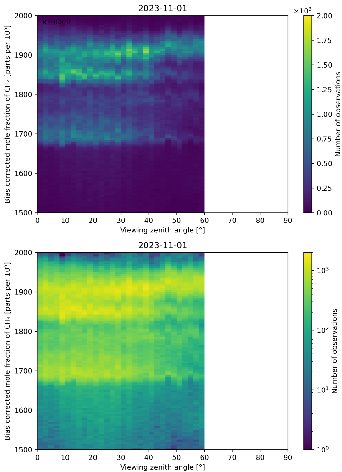
Figure 111: Scatter density plot of “Viewing zenith angle” against “Bias corrected mole fraction of CH 4 ” for 2023-10-31 to 2023-11-02.
