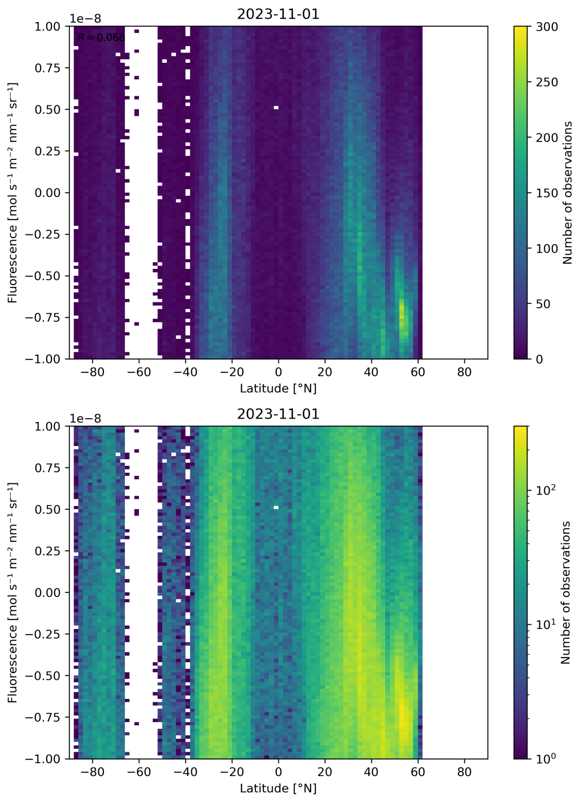
Figure 56: Scatter density plot of “Latitude” against “Fluorescence” for 2023-10-31 to 2023-11-02.
