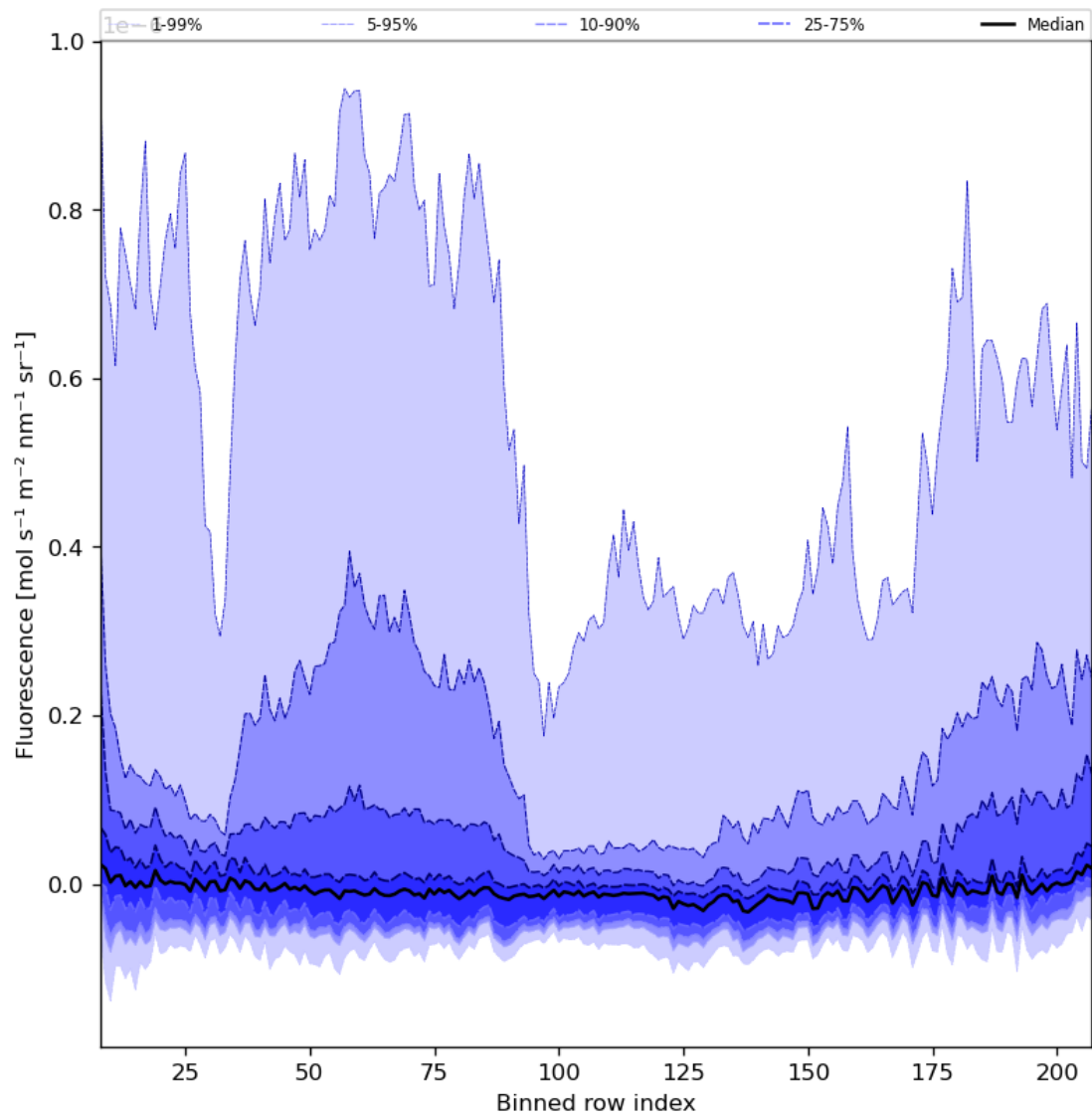
Figure 43: Along track statistics of “Fluorescence” for 2023-10-31 to 2023-11-02
