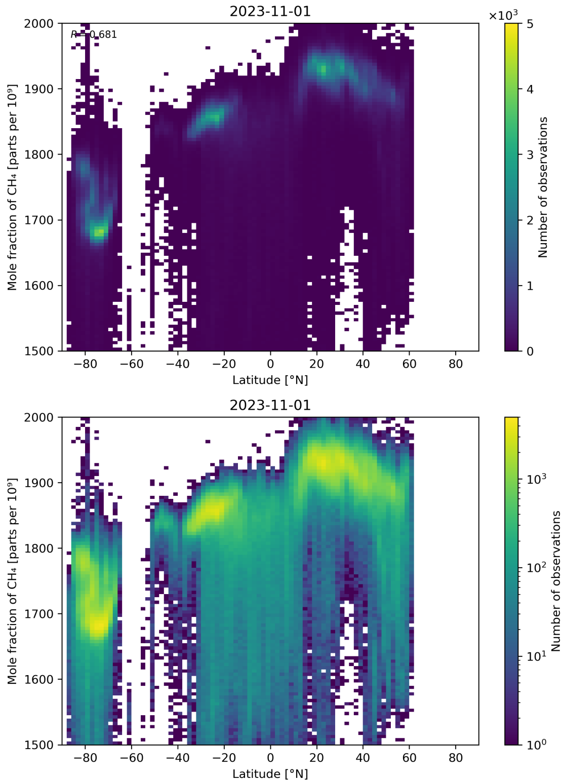
Figure 57: Scatter density plot of “Latitude” against “Mole fraction of CH 4 ” for 2023-10-31 to 2023-11-02.
