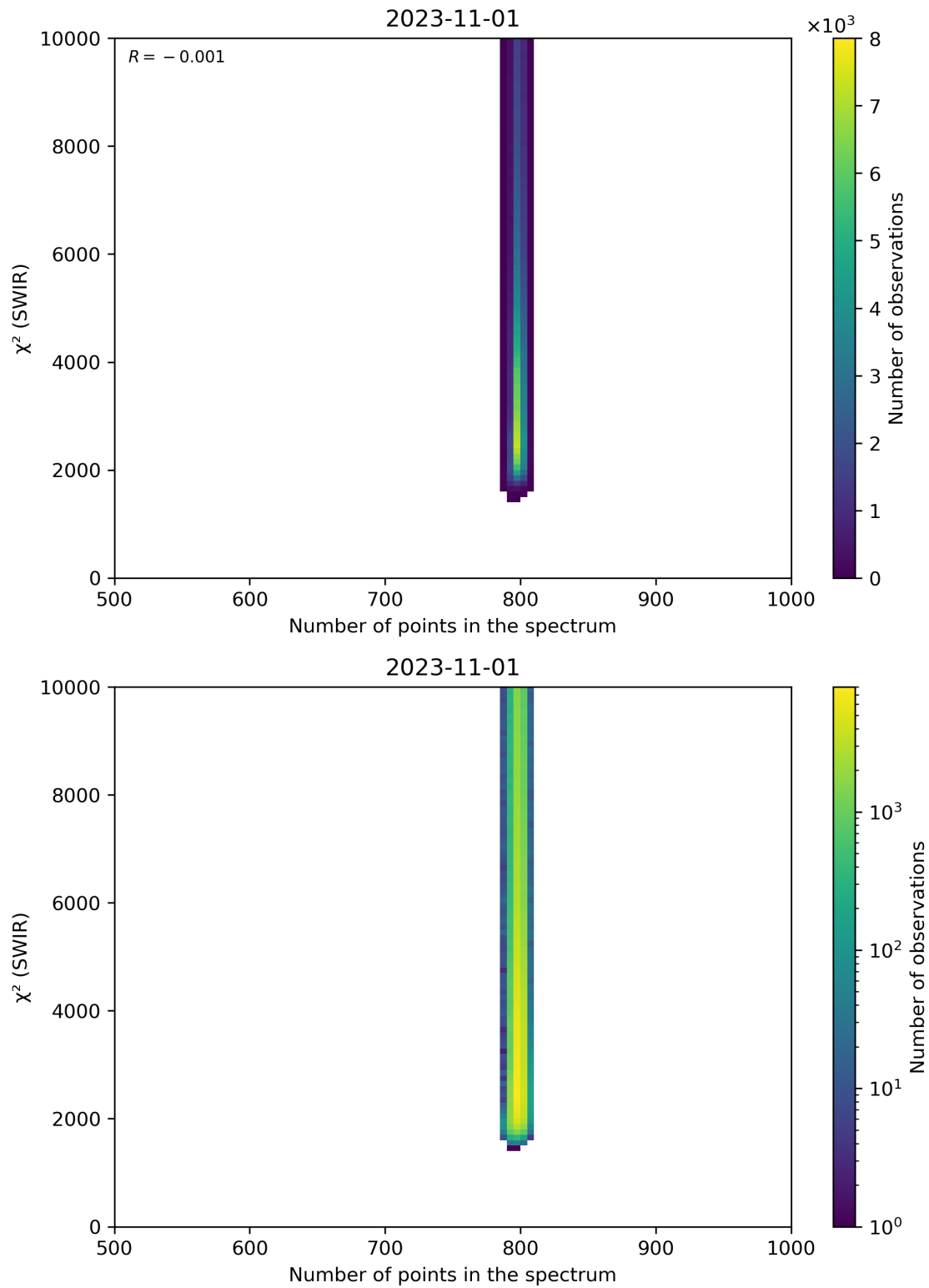
Figure 89: Scatter density plot of “Number of points in the spectrum” against “ \chi^2 (SWIR)” for 2023-10-31 to 2023-11-02.
