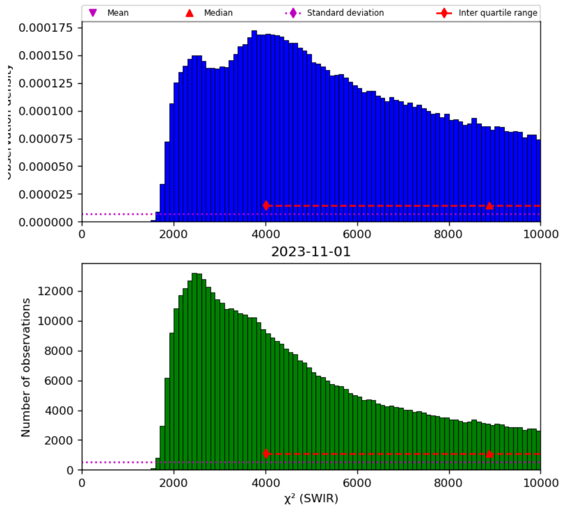
Figure 28: Histogram of “ \chi^2 (SWIR)” for 2023-10-31 to 2023-11-02
