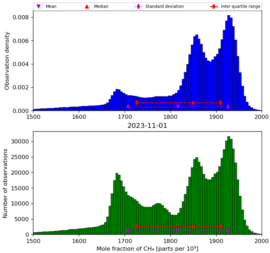
Figure 23: Histogram of “Mole fraction of CH 4 ” for 2023-10-31 to 2023-11-02
