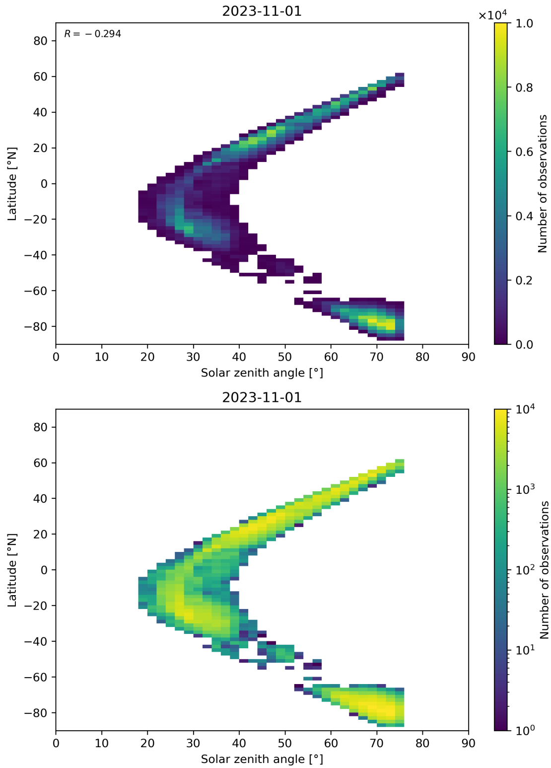
Figure 98: Scatter density plot of “Solar zenith angle” against “Latitude” for 2023-10-31 to 2023-11-02.
