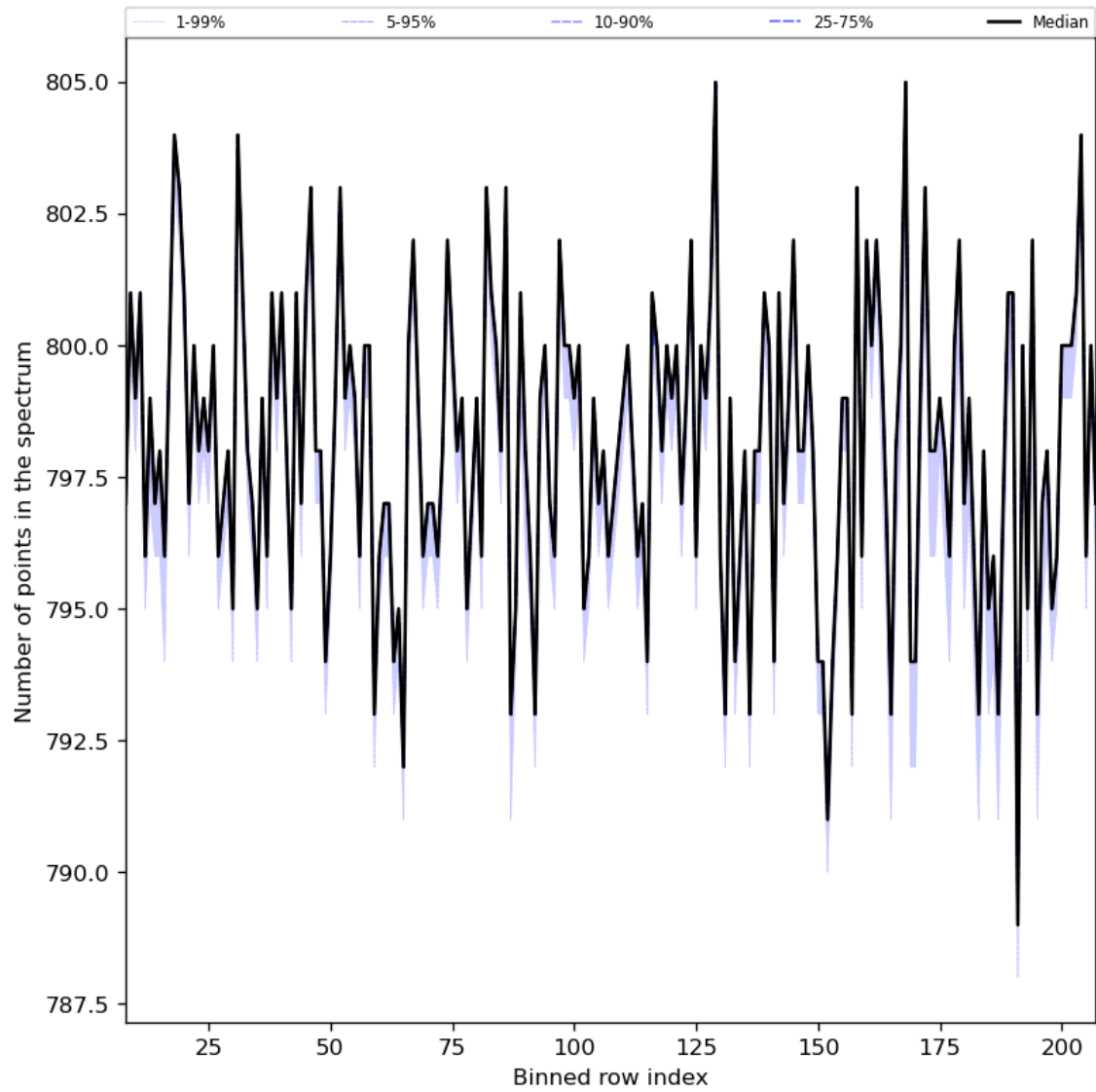
Figure 37: Along track statistics of “Number of points in the spectrum” for 2023-10-31 to 2023-11-02
