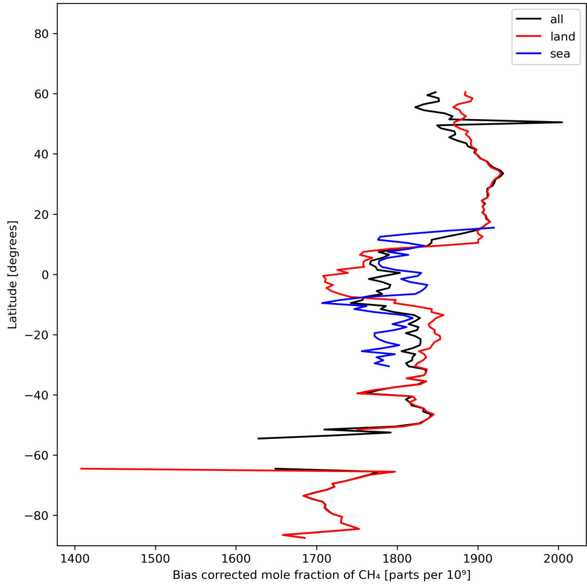
Figure 14: Zonal average of “Bias corrected mole fraction of CH 4 ” for 2023-10-31 to 2023-11-02.
