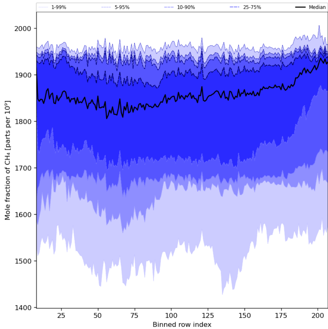
Figure 34: Along track statistics of “Mole fraction of CH 4 ” for 2023-10-31 to 2023-11-02
