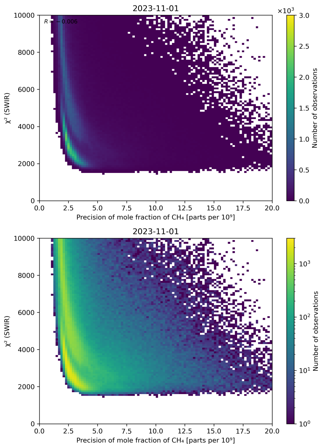
Figure 79: Scatter density plot of “Precision of mole fraction of \text{CH}_4 ” against “ \chi^2 (SWIR)” for 2023-10-31 to 2023-11-02.
