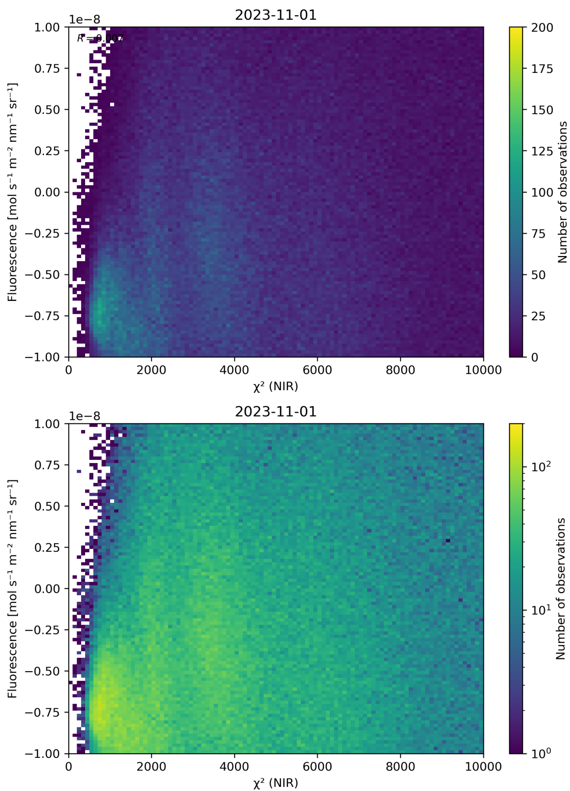
Figure 45: Scatter density plot of “ \chi^2 (NIR)” against “Fluorescence” for 2023-10-31 to 2023-11-02.
