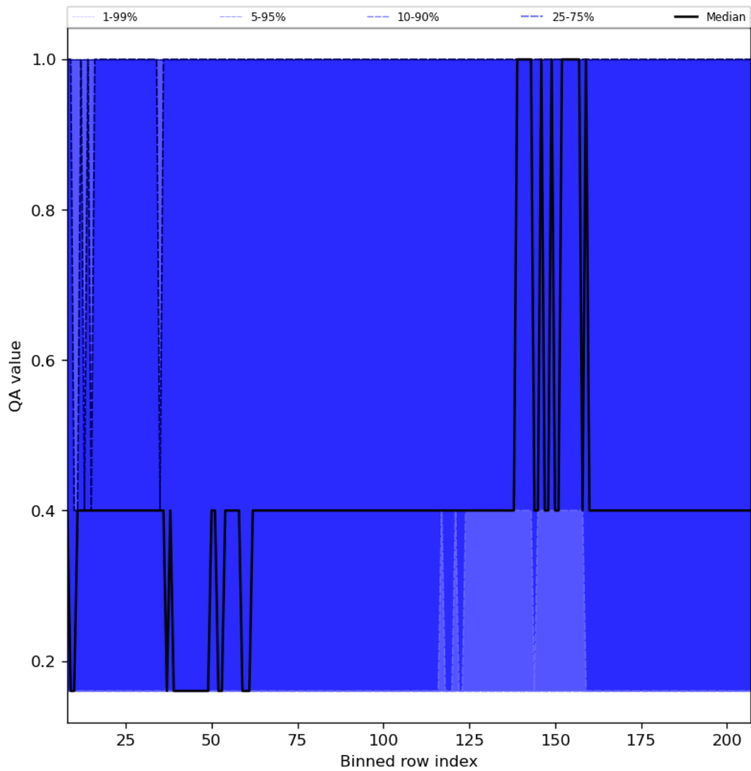
Figure 33: Along track statistics of “QA value” for 2023-10-31 to 2023-11-02
