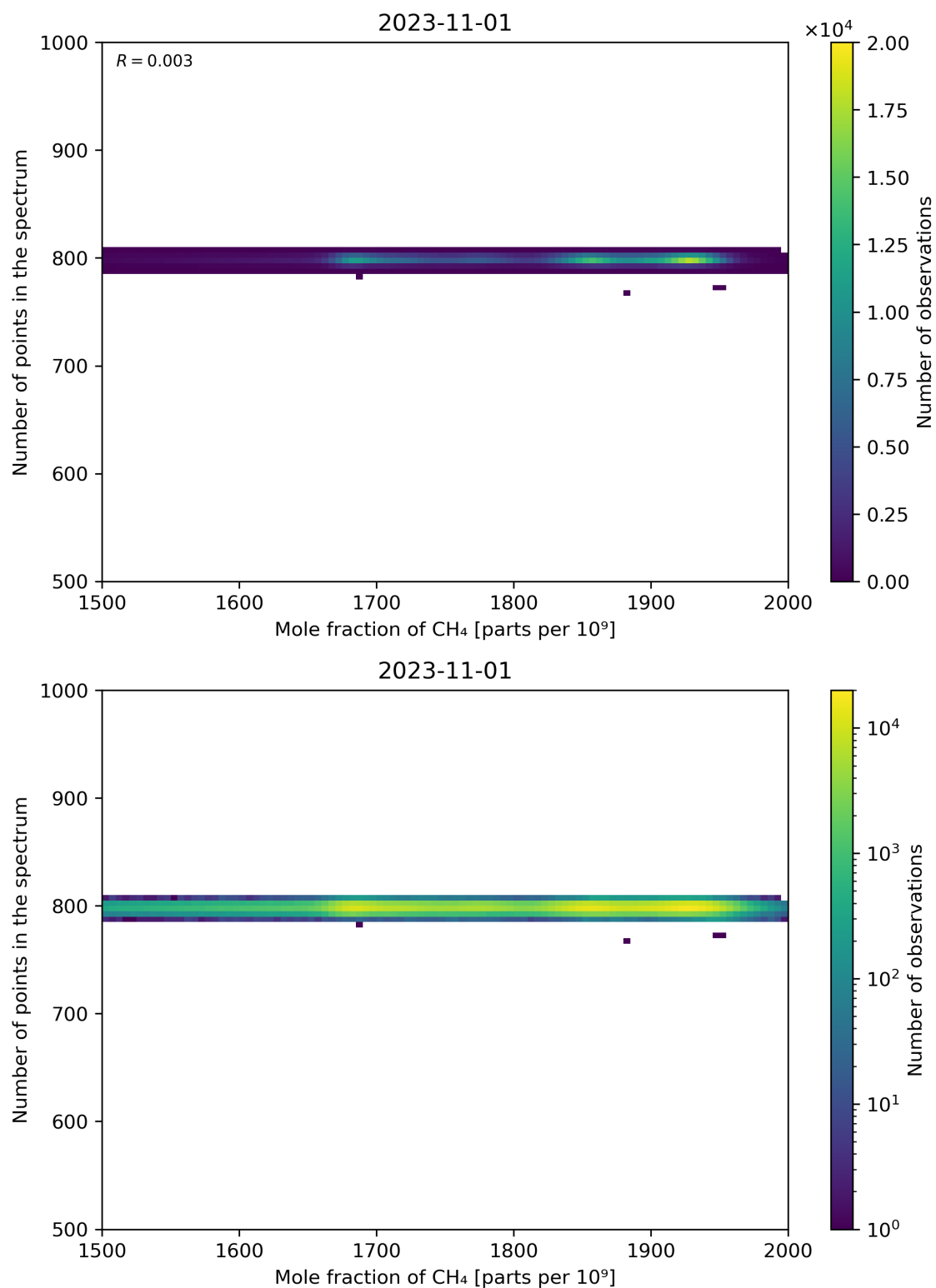
Figure 77: Scatter density plot of “Mole fraction of CH 4 ” against “Number of points in the spectrum” for 2023-10-31 to 2023-11-02.
