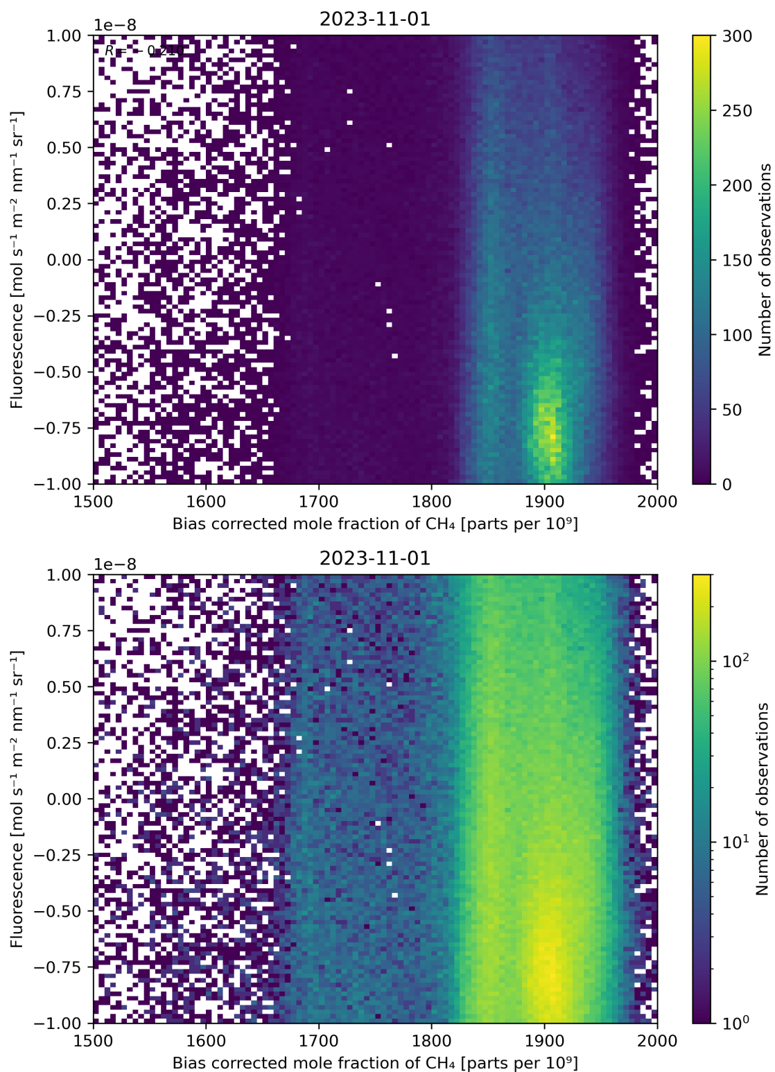
Figure 66: Scatter density plot of “Bias corrected mole fraction of \text{CH}_4 ” against “Fluorescence” for 2023-10-31 to 2023-11-02.
