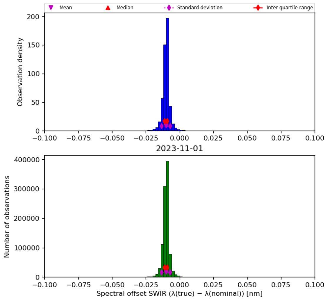
Figure 27: Histogram of “Spectral offset SWIR ( \lambda(\text{true}) - \lambda(\text{nominal}) )” for 2023-10-31 to 2023-11-02
