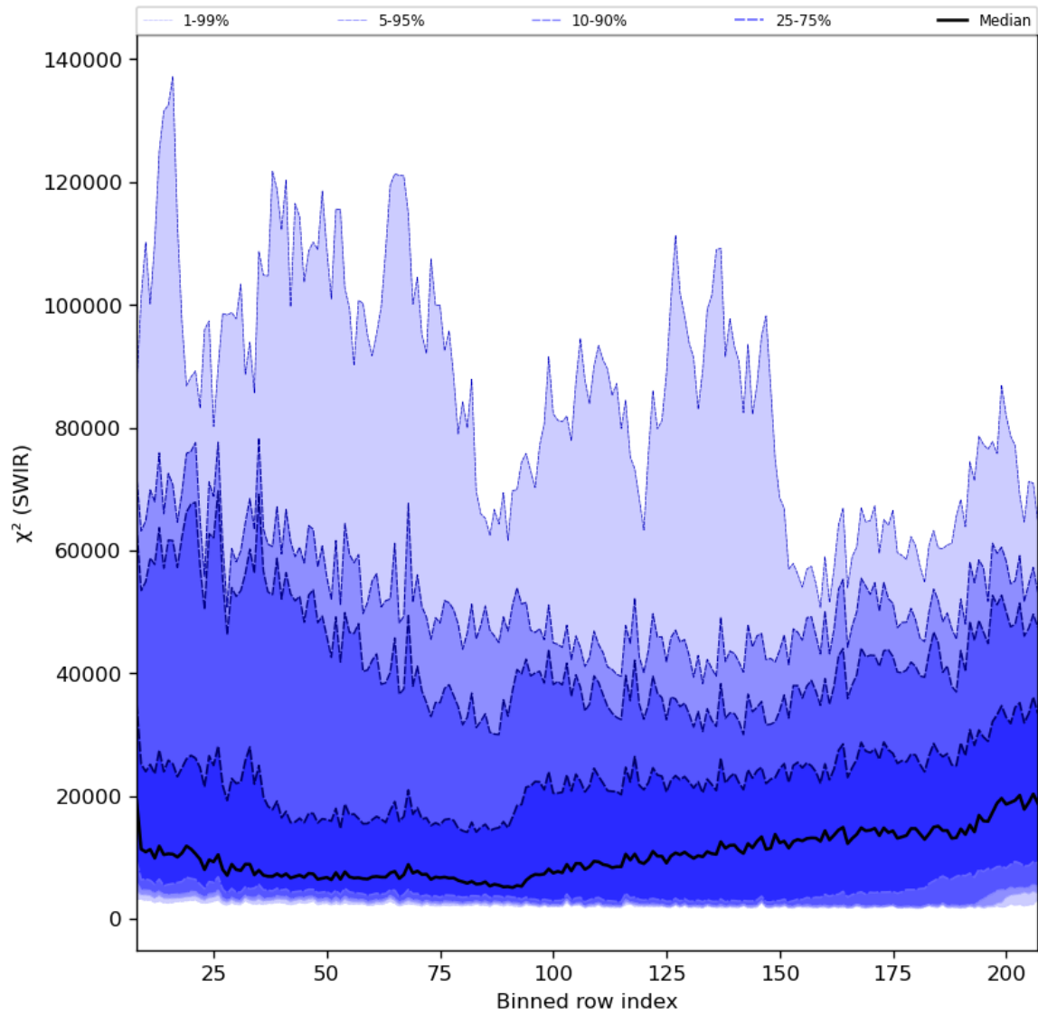
Figure 39: Along track statistics of “ \chi^2 (SWIR)” for 2023-10-31 to 2023-11-02
