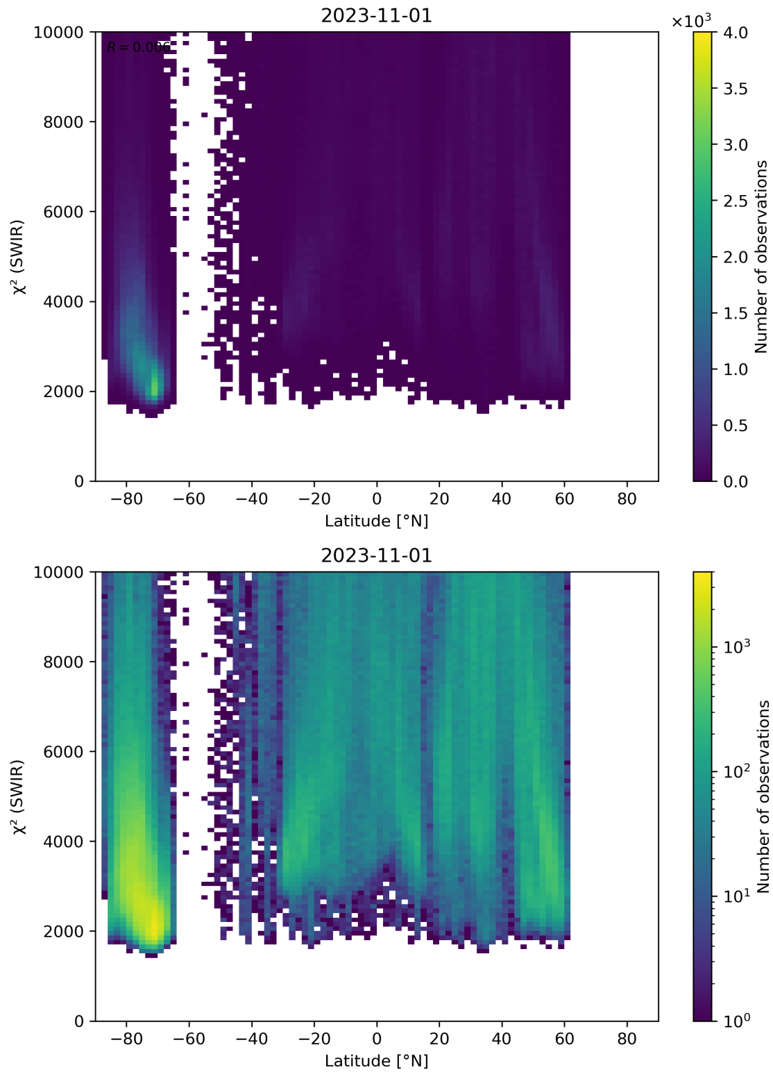
Figure 54: Scatter density plot of “Latitude” against “ \chi^2 (SWIR)” for 2023-10-31 to 2023-11-02.
