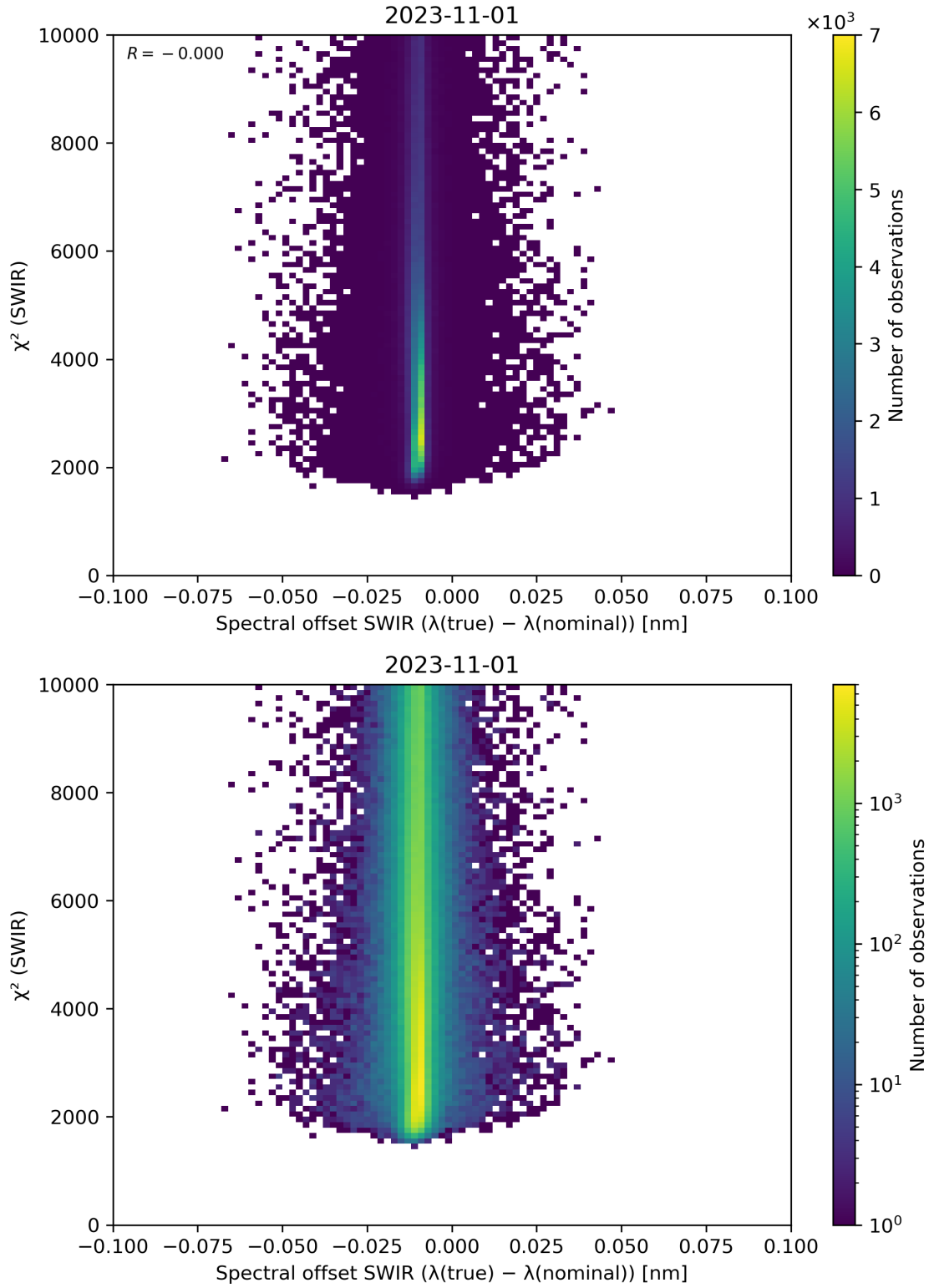
Figure 118: Scatter density plot of “Spectral offset SWIR ( \lambda(\text{true}) - \lambda(\text{nominal}) )” against “ \chi^2 (SWIR)” for 2023-10-31 to 2023-11-02.
