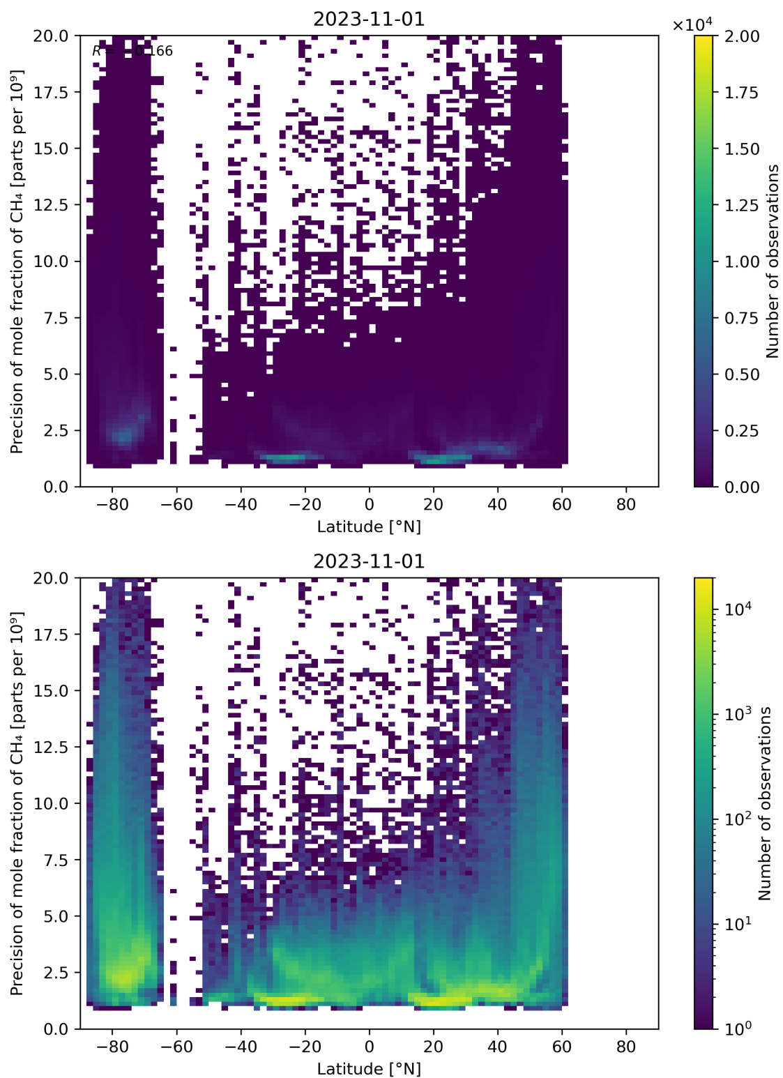
Figure 59: Scatter density plot of “Latitude” against “Precision of mole fraction of CH 4 ” for 2023-10-31 to 2023-11-02.
