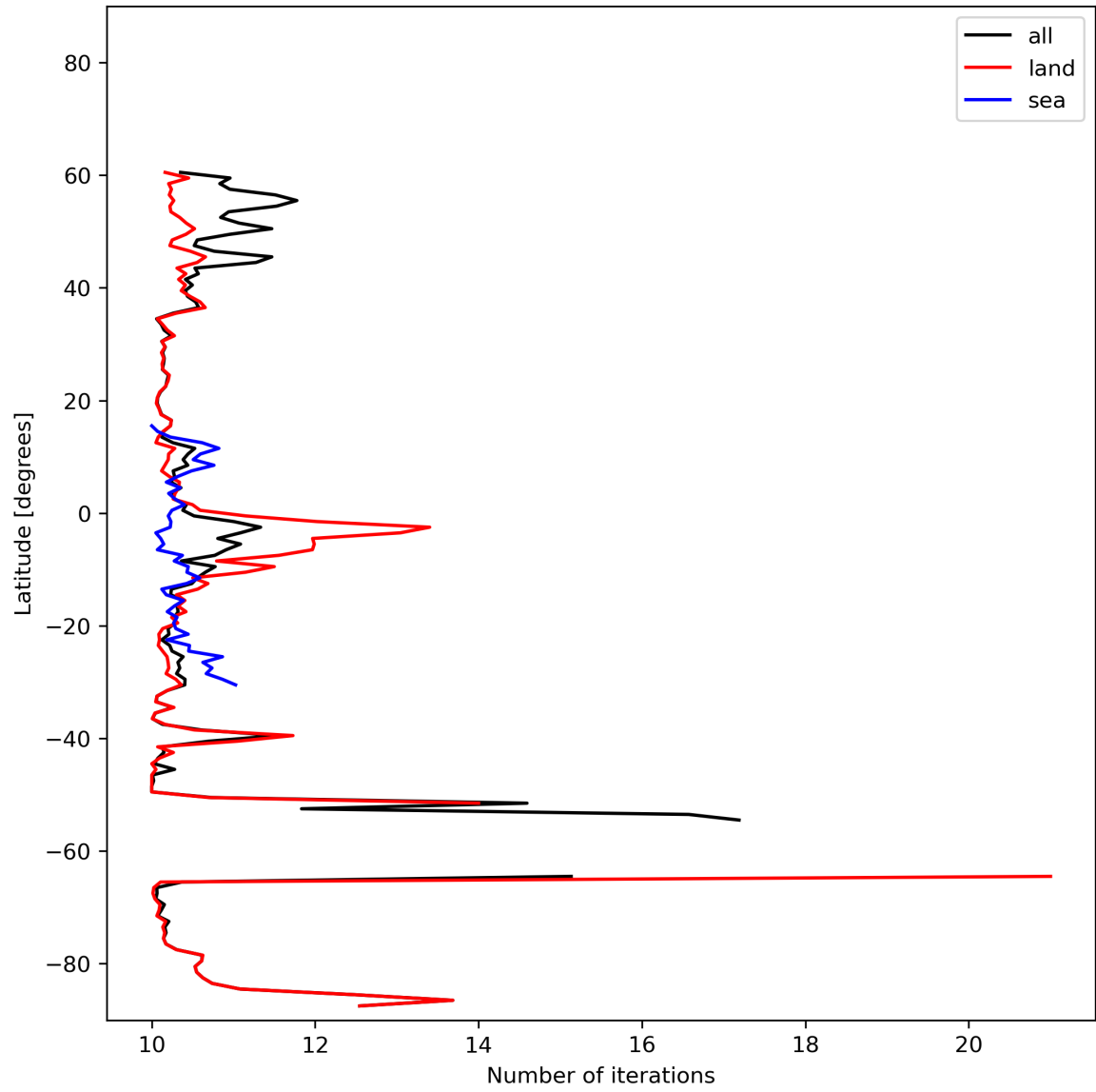
Figure 20: Zonal average of “Number of iterations” for 2023-10-31 to 2023-11-02.
