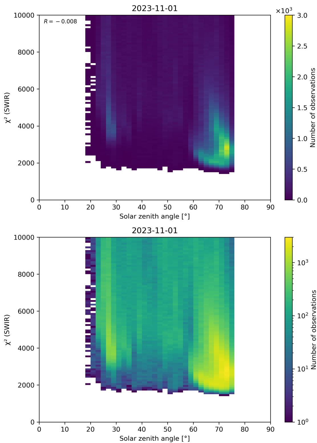
Figure 95: Scatter density plot of “Solar zenith angle” against “ \chi^2 (SWIR)” for 2023-10-31 to 2023-11-02.
