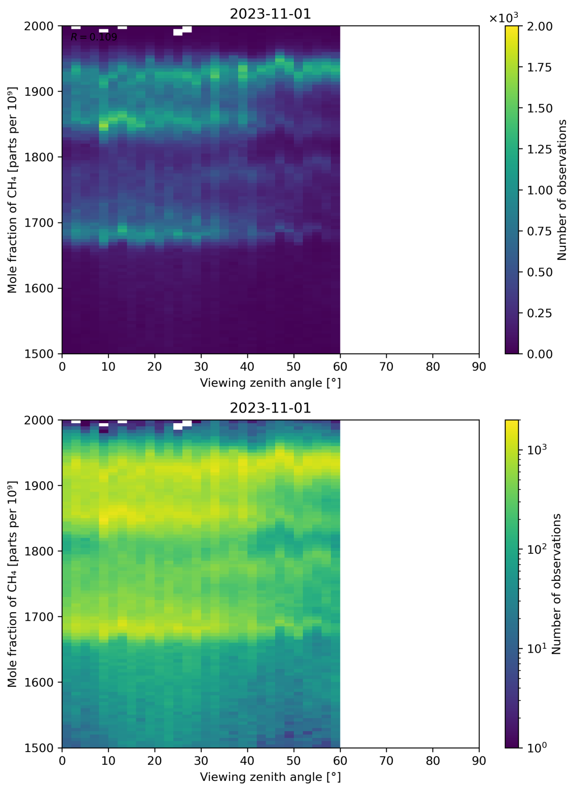
Figure 110: Scatter density plot of “Viewing zenith angle” against “Mole fraction of CH 4 ” for 2023-10-31 to 2023-11-02.
