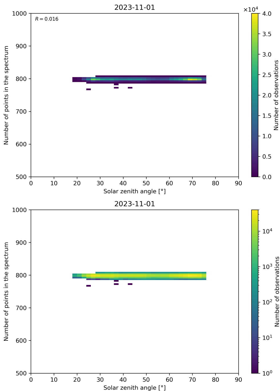
Figure 103: Scatter density plot of “Solar zenith angle” against “Number of points in the spectrum” for 2023-10-31 to 2023-11-02.
