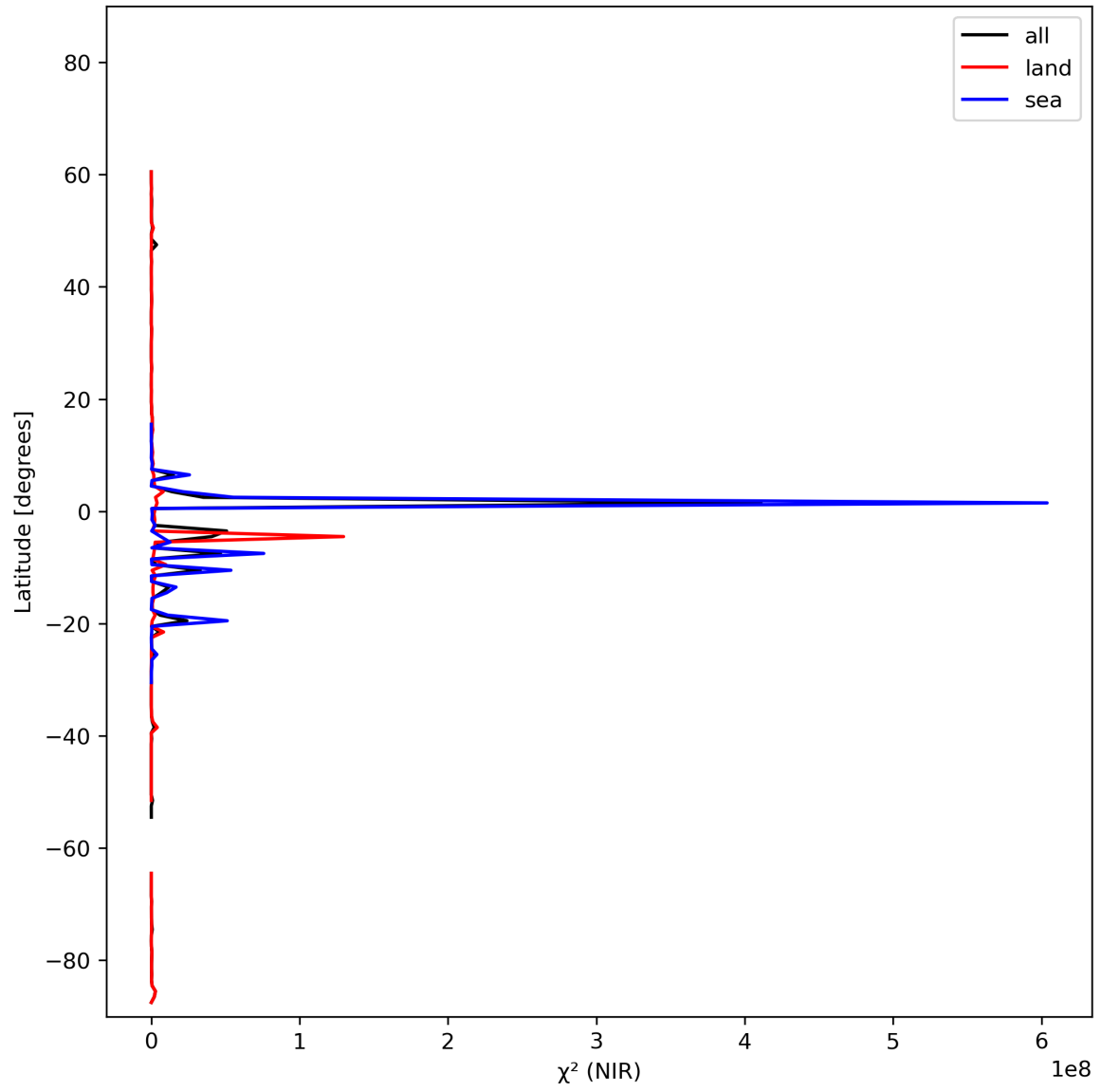
Figure 18: Zonal average of “ \chi^2 (NIR)” for 2023-10-31 to 2023-11-02.
