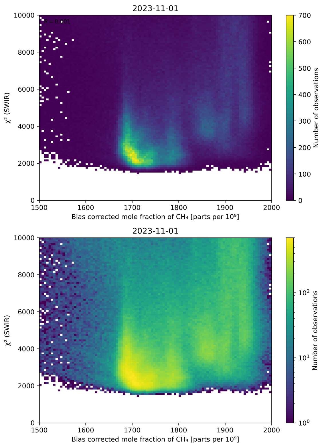
Figure 64: Scatter density plot of “Bias corrected mole fraction of \text{CH}_4 ” against “ \chi^2 (SWIR)” for 2023-10-31 to 2023-11-02.
