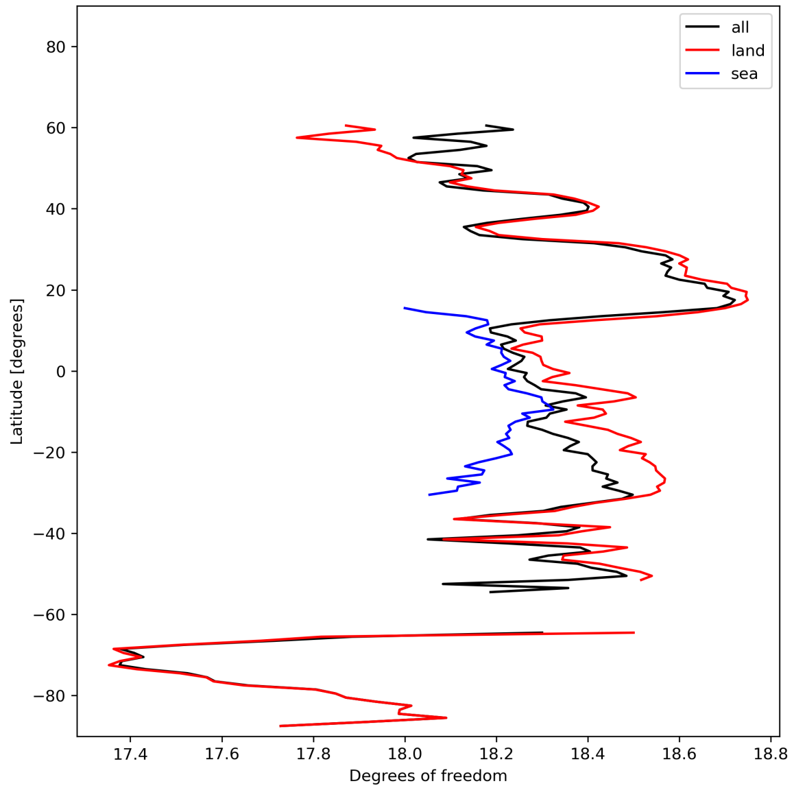
Figure 19: Zonal average of “Degrees of freedom” for 2023-10-31 to 2023-11-02.
