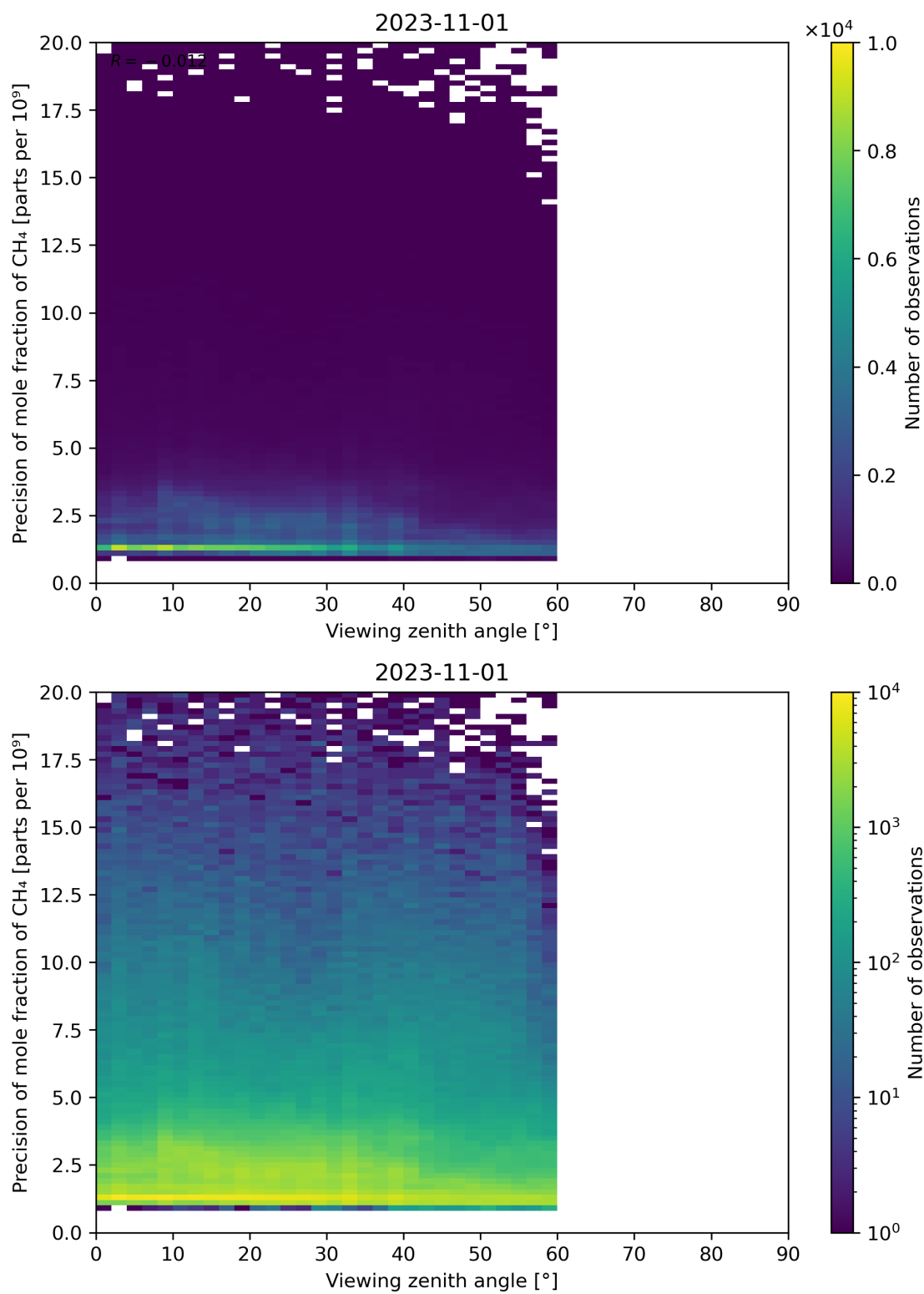
Figure 112: Scatter density plot of “Viewing zenith angle” against “Precision of mole fraction of CH 4 ” for 2023-10-31 to 2023-11-02.
