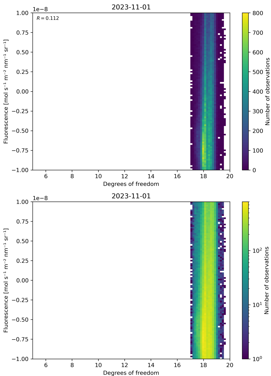
Figure 51: Scatter density plot of “Degrees of freedom” against “Fluorescence” for 2023-10-31 to 2023-11-02.
