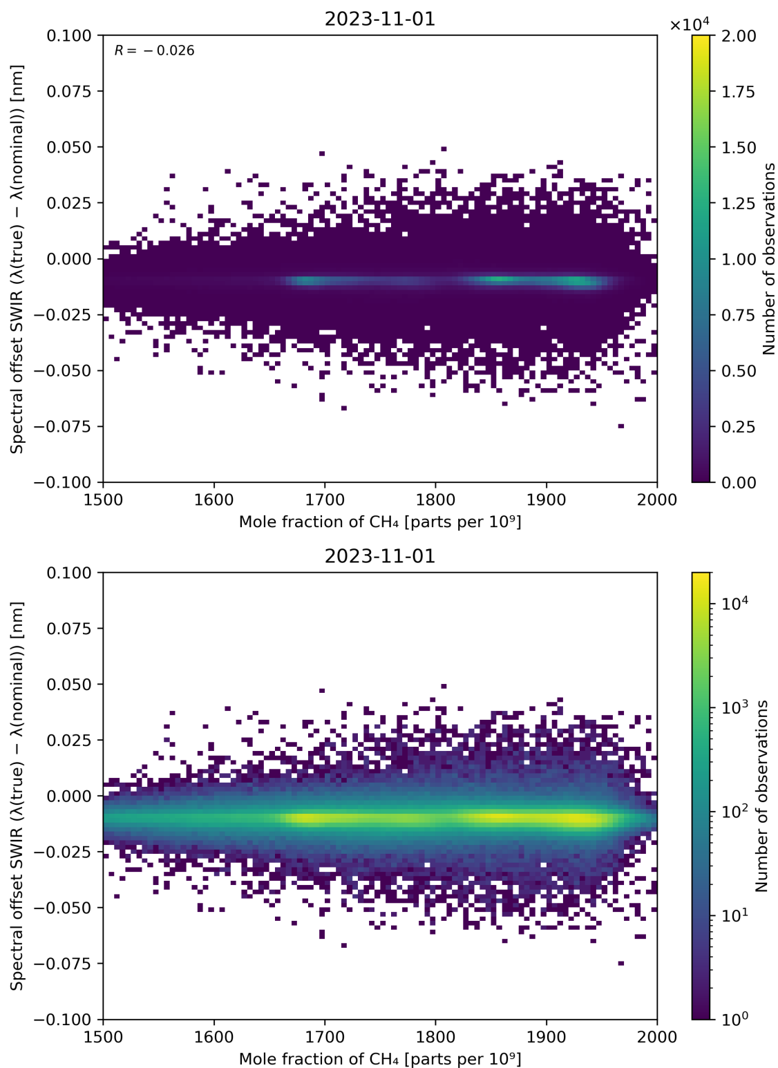
Figure 86: Scatter density plot of “Mole fraction of CH 4 ” against “Spectral offset SWIR ( \lambda(\text{true}) - \lambda(\text{nominal}) )” for 2023-10-31 to 2023-11-02.
