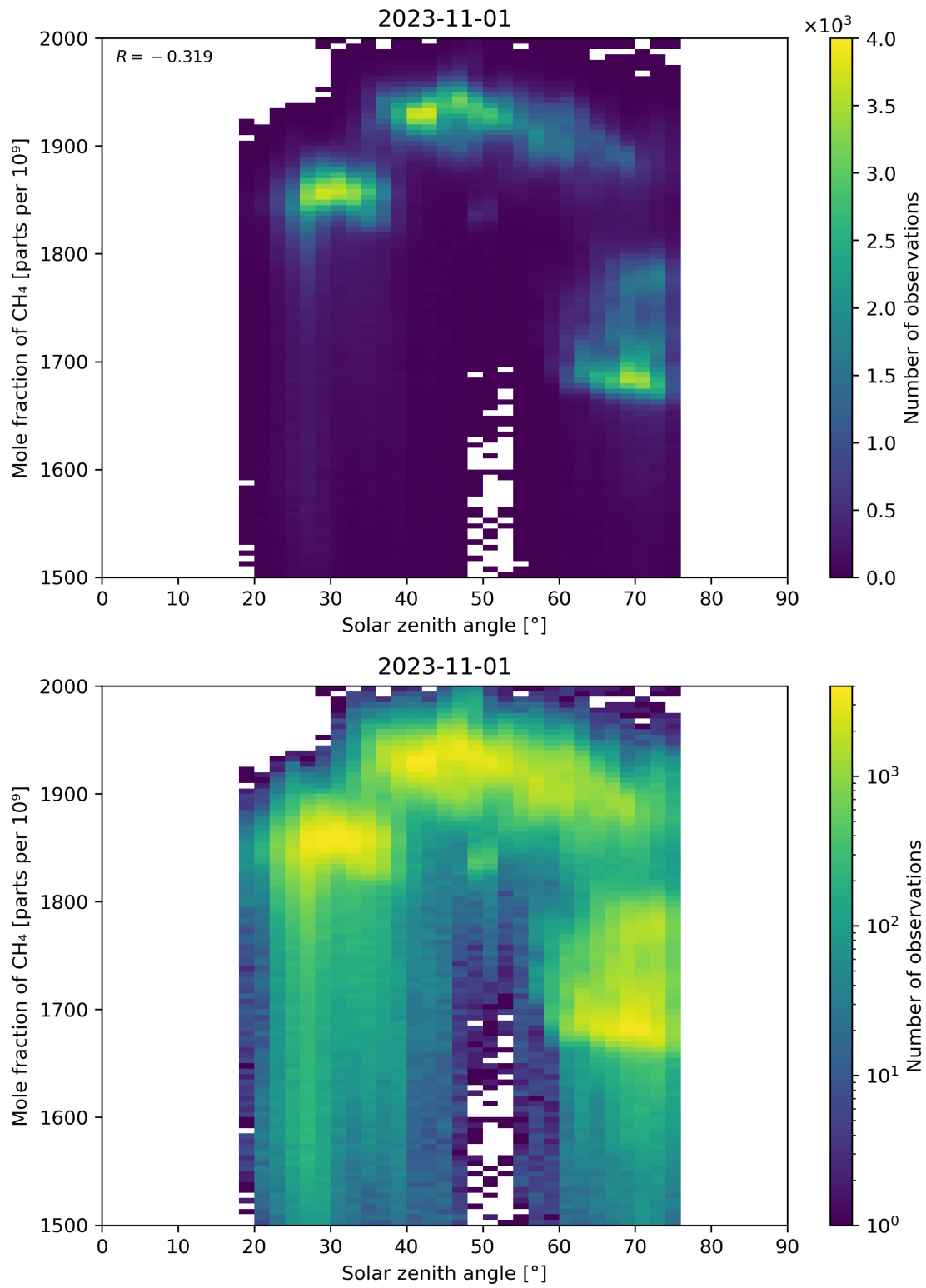
Figure 99: Scatter density plot of “Solar zenith angle” against “Mole fraction of \text{CH}_4 ” for 2023-10-31 to 2023-11-02.
