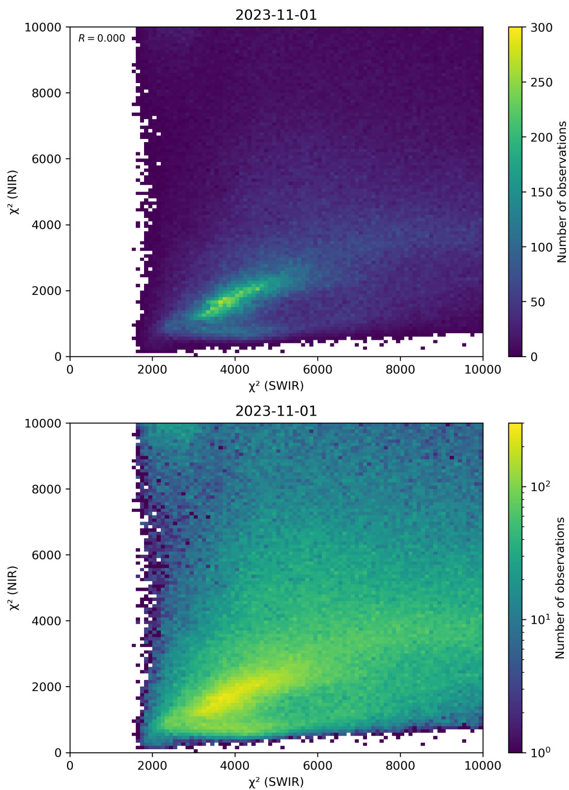
Figure 47: Scatter density plot of “ \chi^2 (SWIR)” against “ \chi^2 (NIR)” for 2023-10-31 to 2023-11-02.
