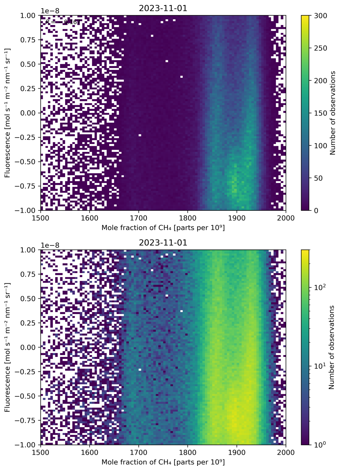
Figure 73: Scatter density plot of “Mole fraction of CH 4 ” against “Fluorescence” for 2023-10-31 to 2023-11-02.
