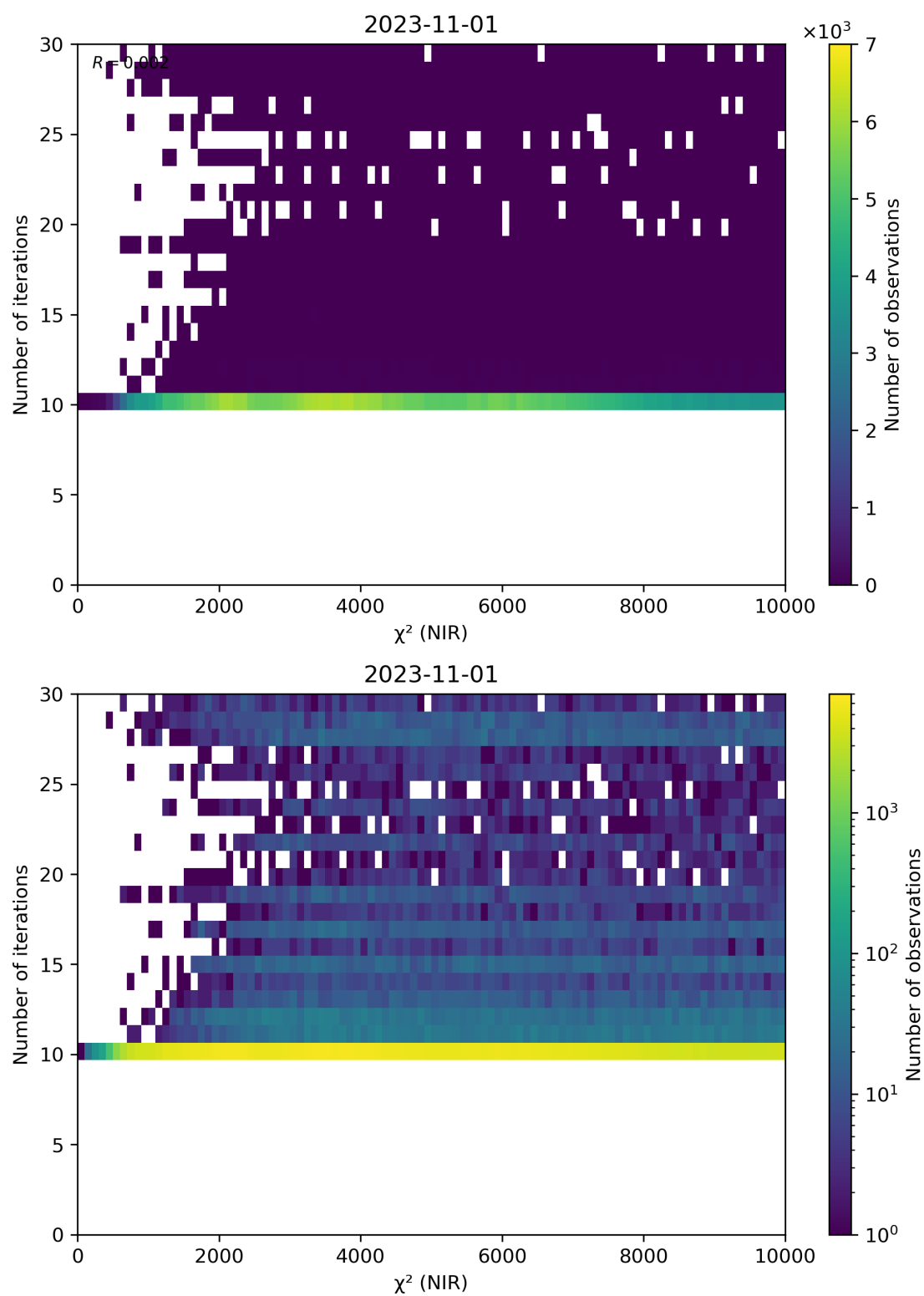
Figure 46: Scatter density plot of “ \chi^2 (NIR)” against “Number of iterations” for 2023-10-31 to 2023-11-02.
