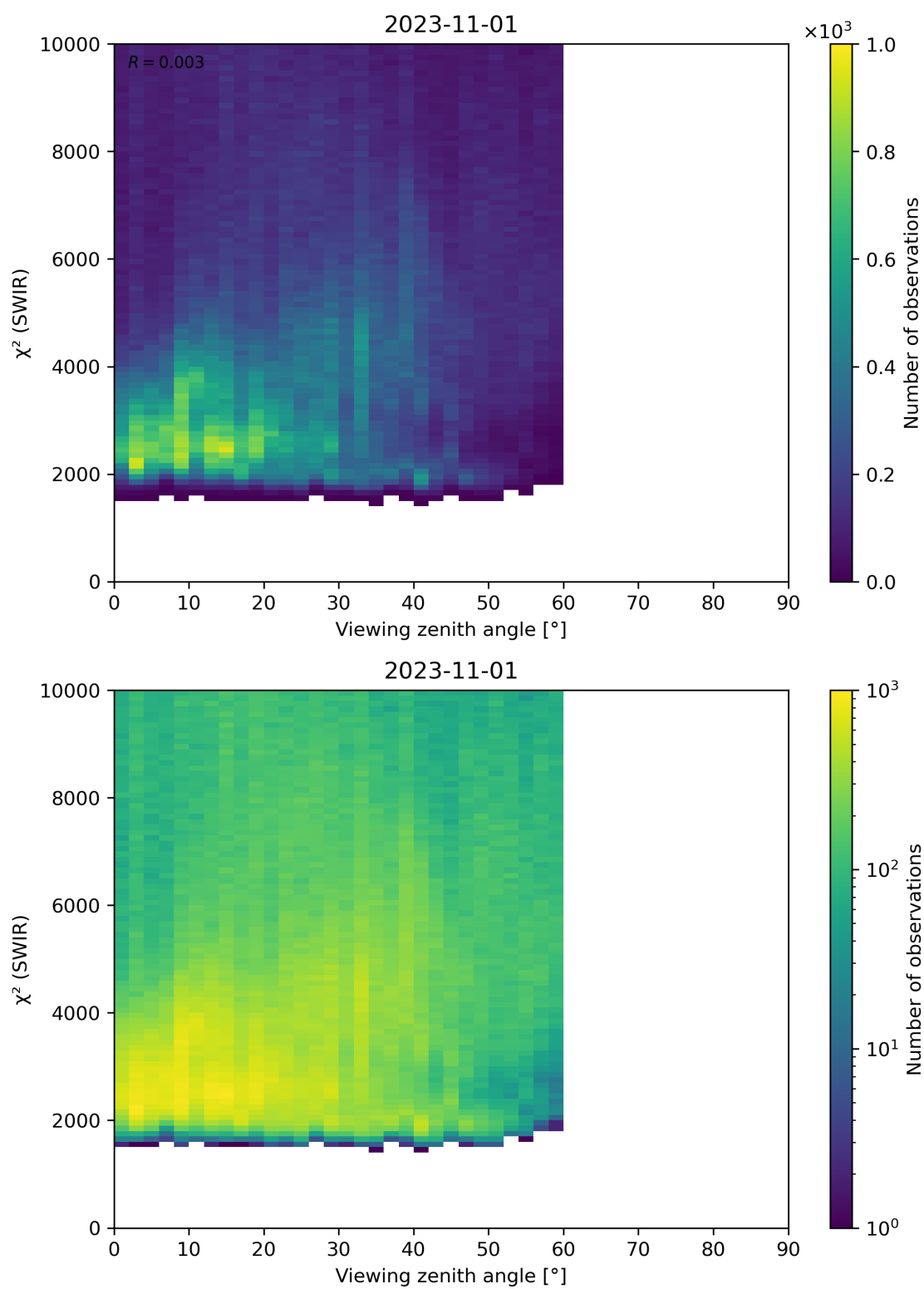
Figure 106: Scatter density plot of “Viewing zenith angle” against “ \chi^2 (SWIR)” for 2023-10-31 to 2023-11-02.
