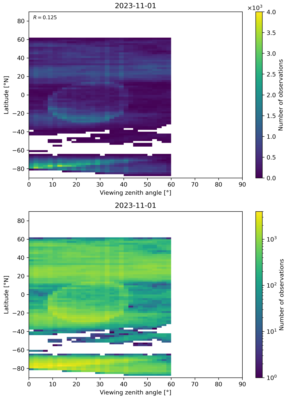
Figure 109: Scatter density plot of “Viewing zenith angle” against “Latitude” for 2023-10-31 to 2023-11-02.
