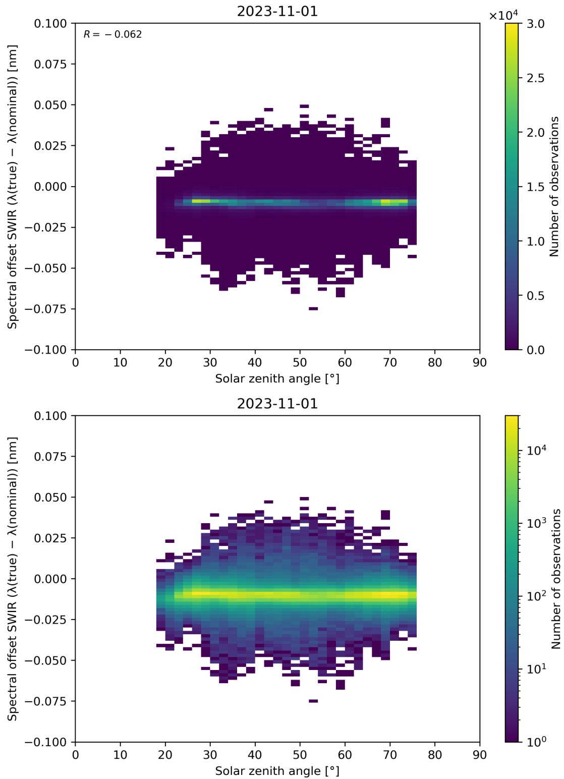
Figure 104: Scatter density plot of “Solar zenith angle” against “Spectral offset SWIR ( \lambda(\text{true}) - \lambda(\text{nominal}) )” for 2023-10-31 to 2023-11-02.
