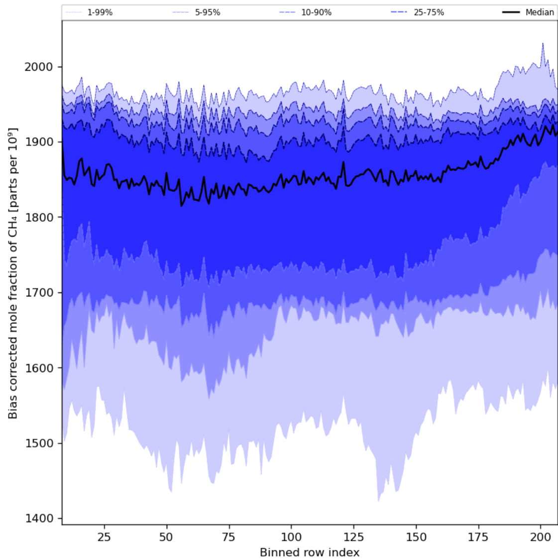
Figure 36: Along track statistics of “Bias corrected mole fraction of CH 4 ” for 2023-10-31 to 2023-11-02
