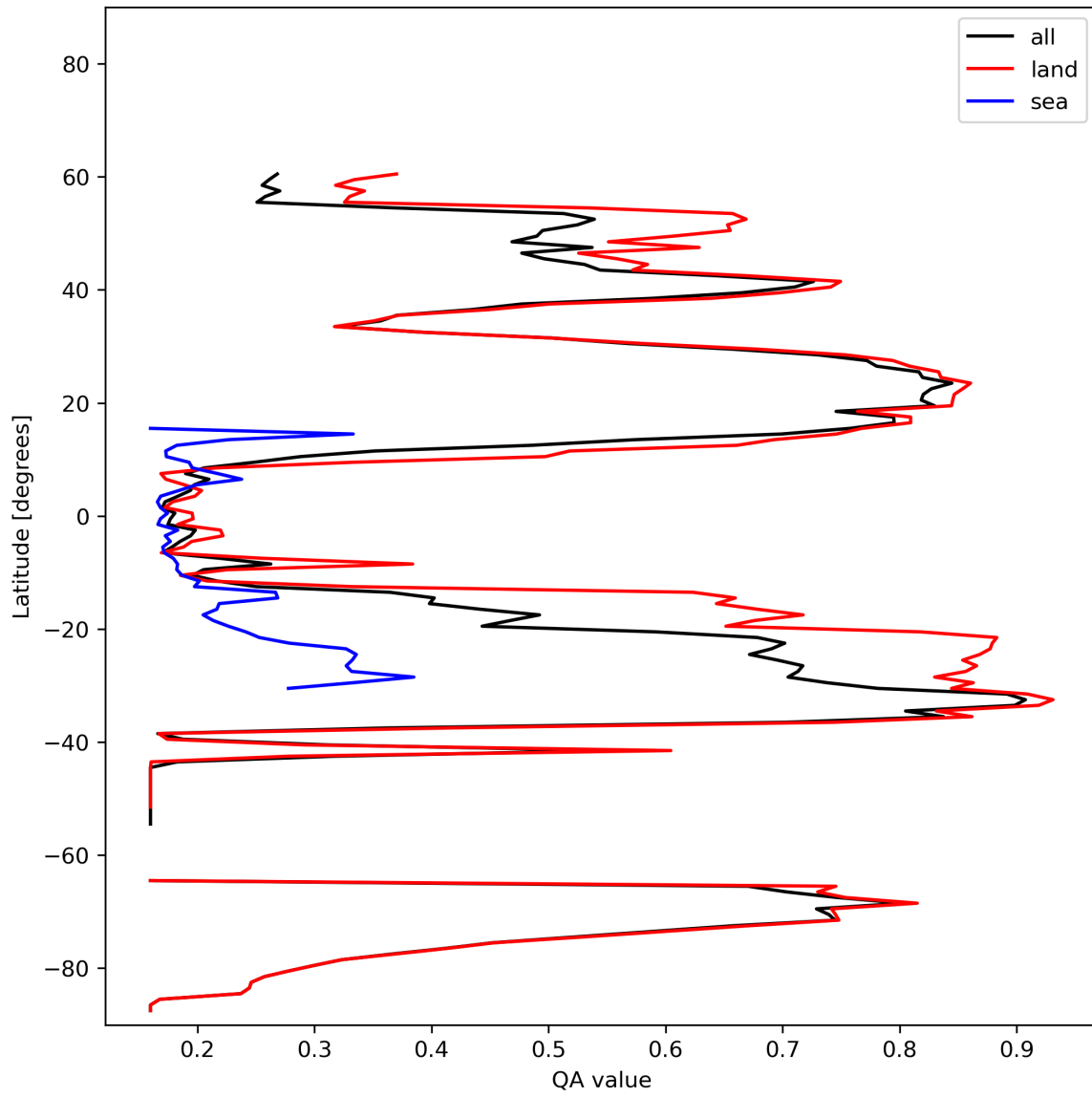
Figure 11: Zonal average of “QA value” for 2023-10-31 to 2023-11-02.
