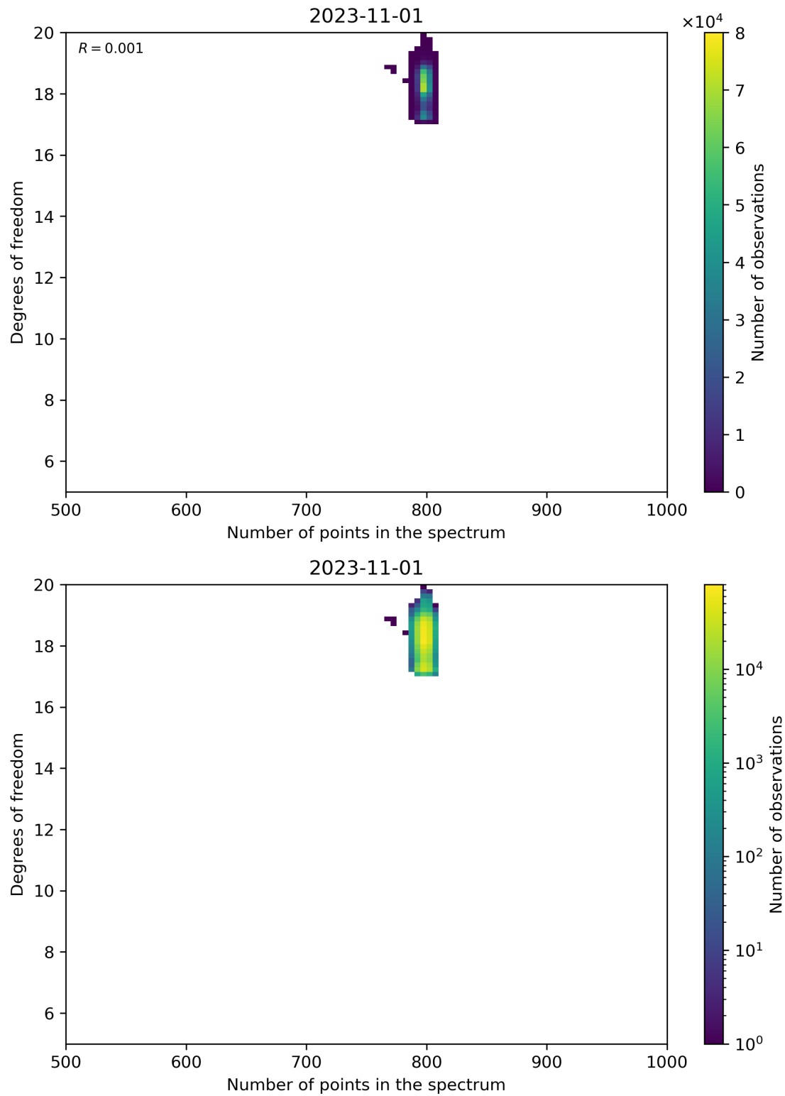
Figure 90: Scatter density plot of “Number of points in the spectrum” against “Degrees of freedom” for 2023-10-31 to 2023-11-02.
