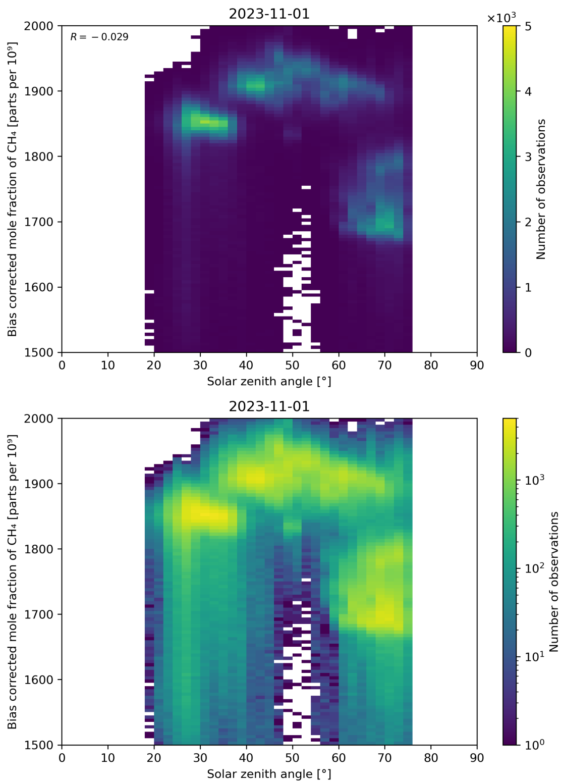
Figure 100: Scatter density plot of “Solar zenith angle” against “Bias corrected mole fraction of CH 4 ” for 2023-10-31 to 2023-11-02.
