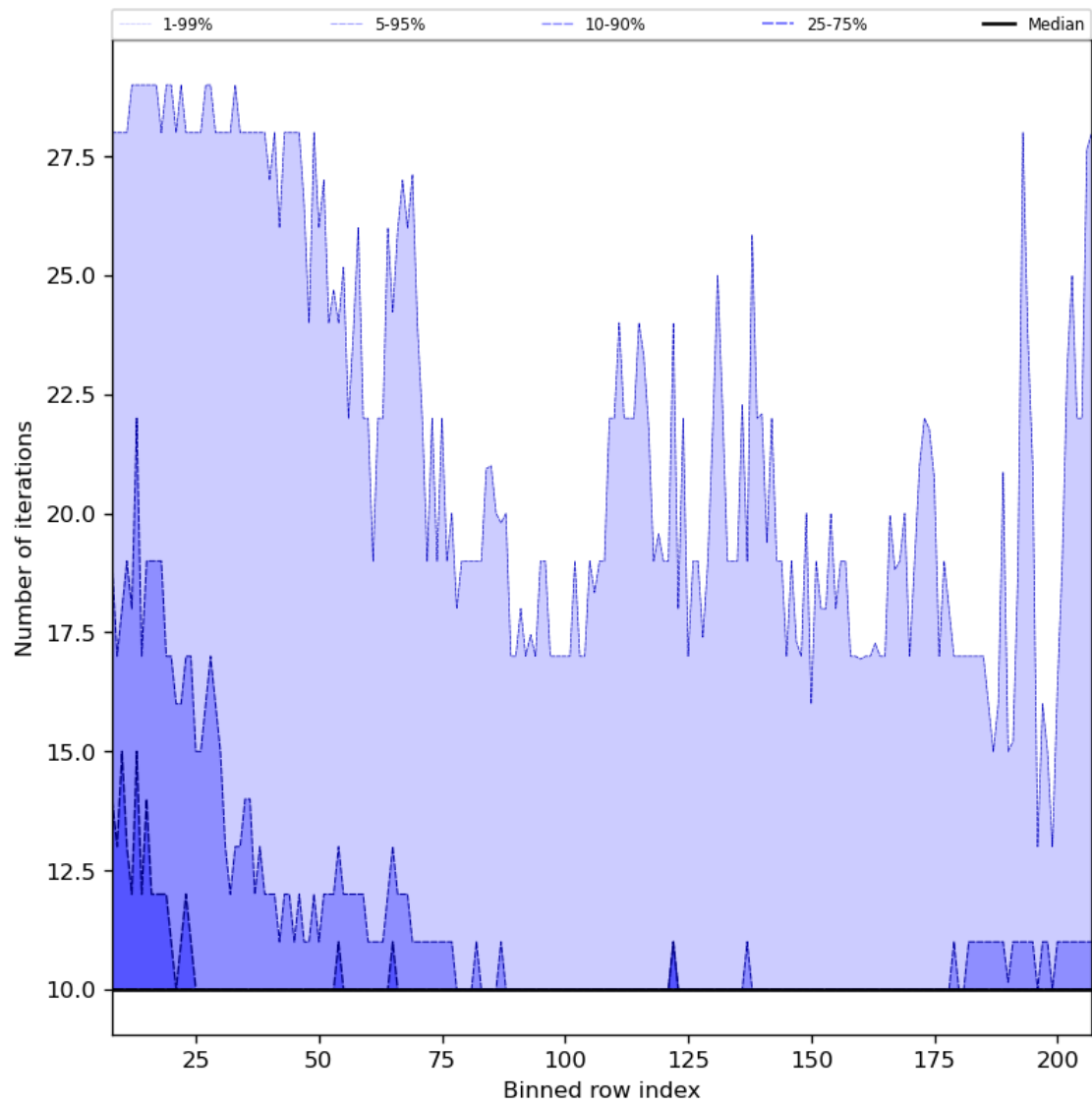
Figure 42: Along track statistics of “Number of iterations” for 2023-10-31 to 2023-11-02
