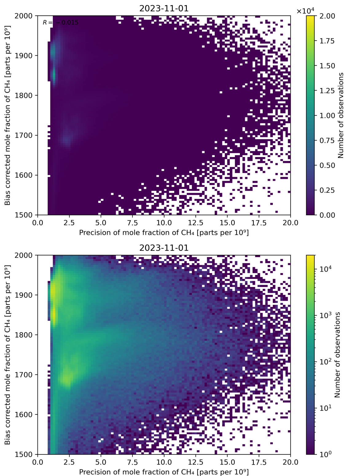
Figure 82: Scatter density plot of “Precision of mole fraction of CH 4 ” against “Bias corrected mole fraction of CH 4 ” for 2023-10-31 to 2023-11-02.
