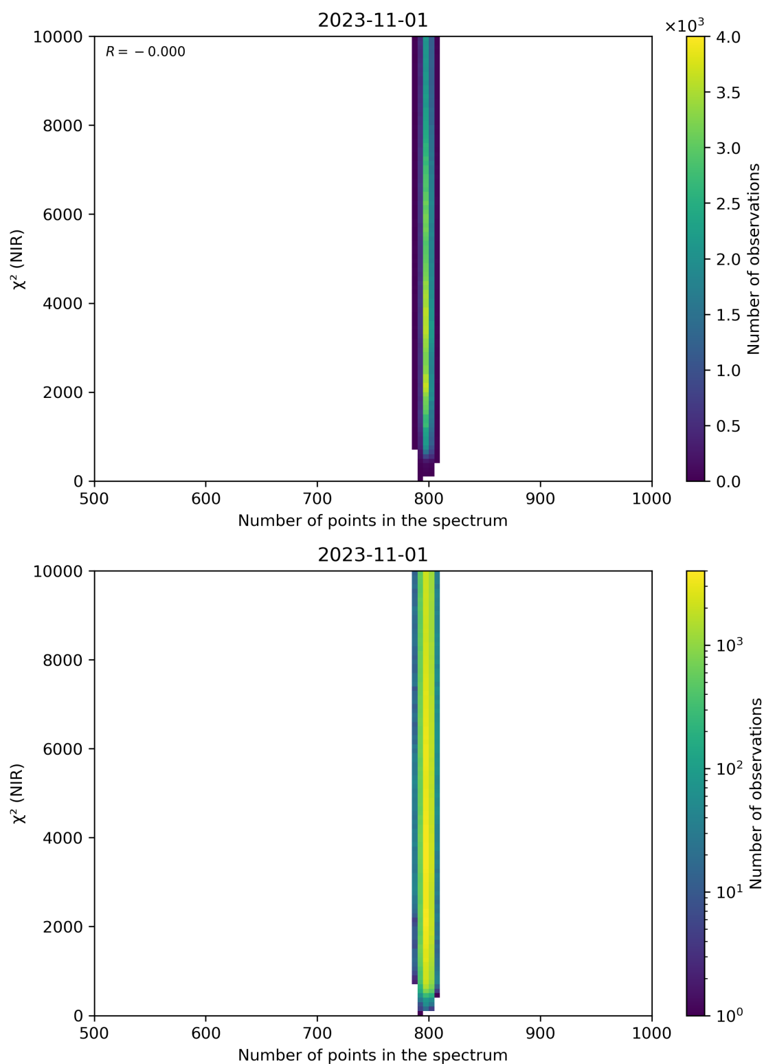
Figure 88: Scatter density plot of “Number of points in the spectrum” against “ \chi^2 (NIR)” for 2023-10-31 to 2023-11-02.
