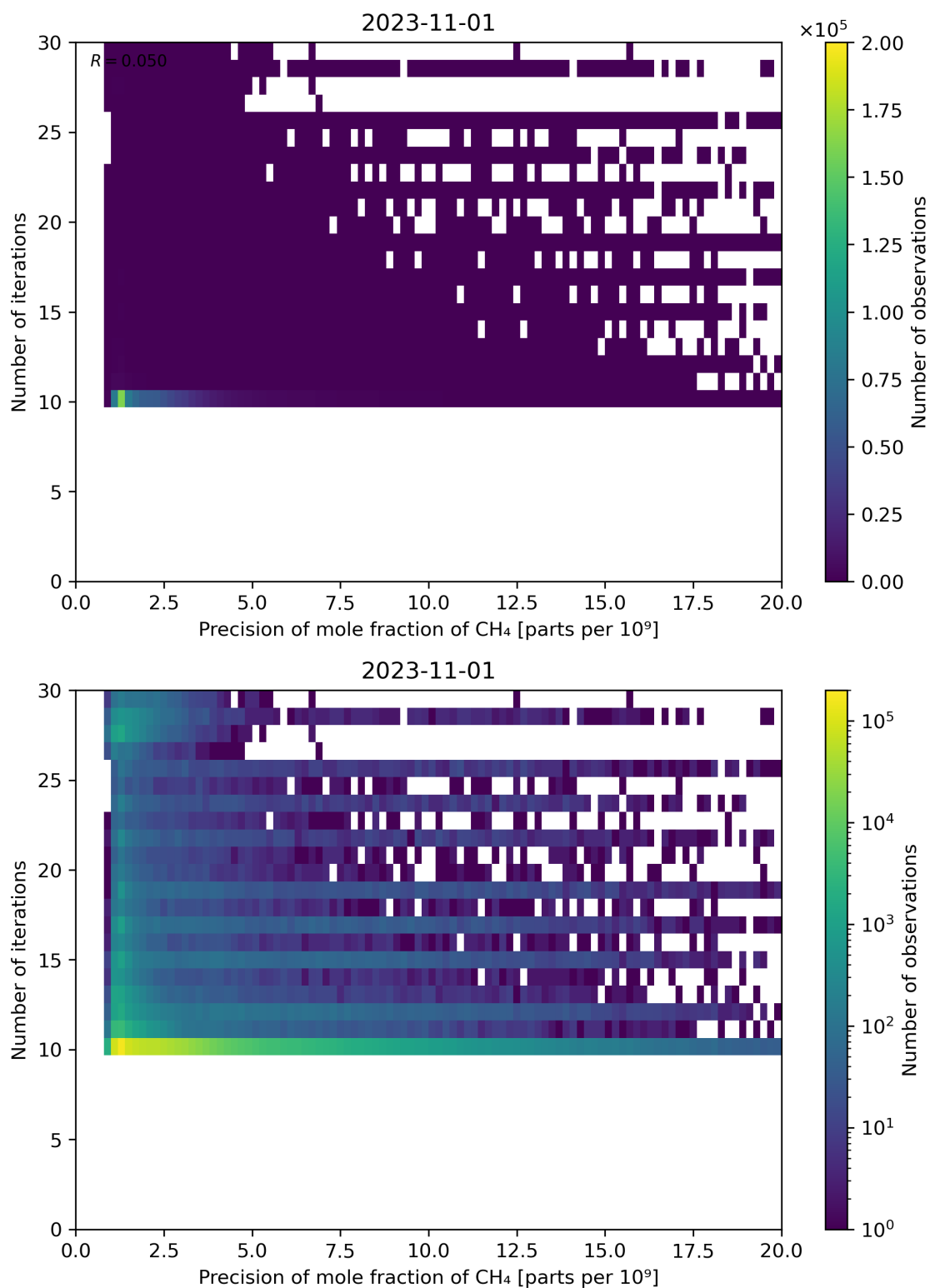
Figure 83: Scatter density plot of “Precision of mole fraction of CH 4 ” against “Number of iterations” for 2023-10-31 to 2023-11-02.
