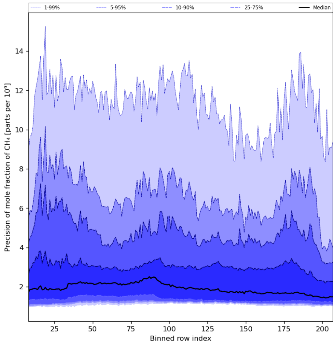
Figure 35: Along track statistics of “Precision of mole fraction of CH 4 ” for 2023-10-31 to 2023-11-02
