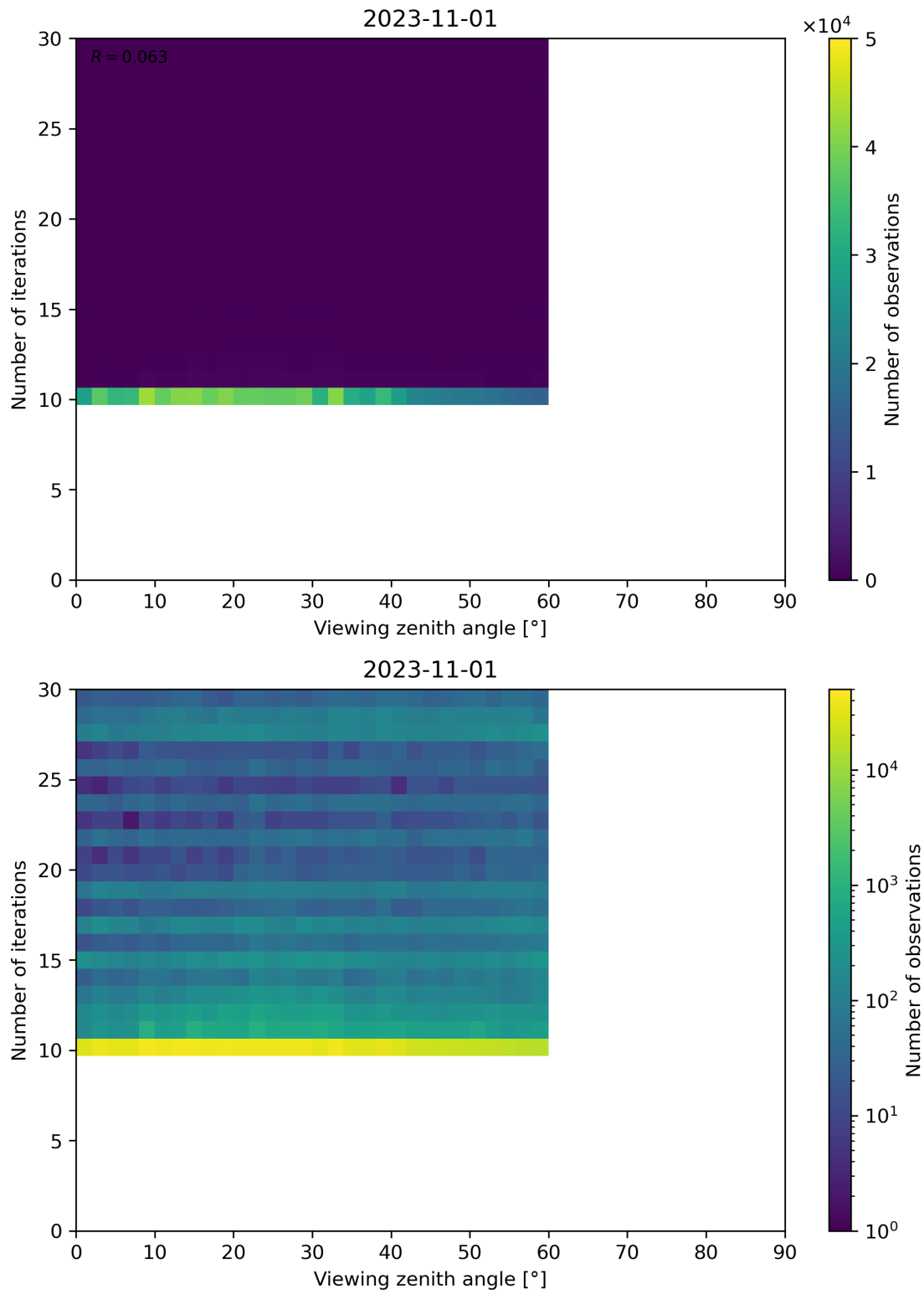
Figure 113: Scatter density plot of “Viewing zenith angle” against “Number of iterations” for 2023-10-31 to 2023-11-02.
