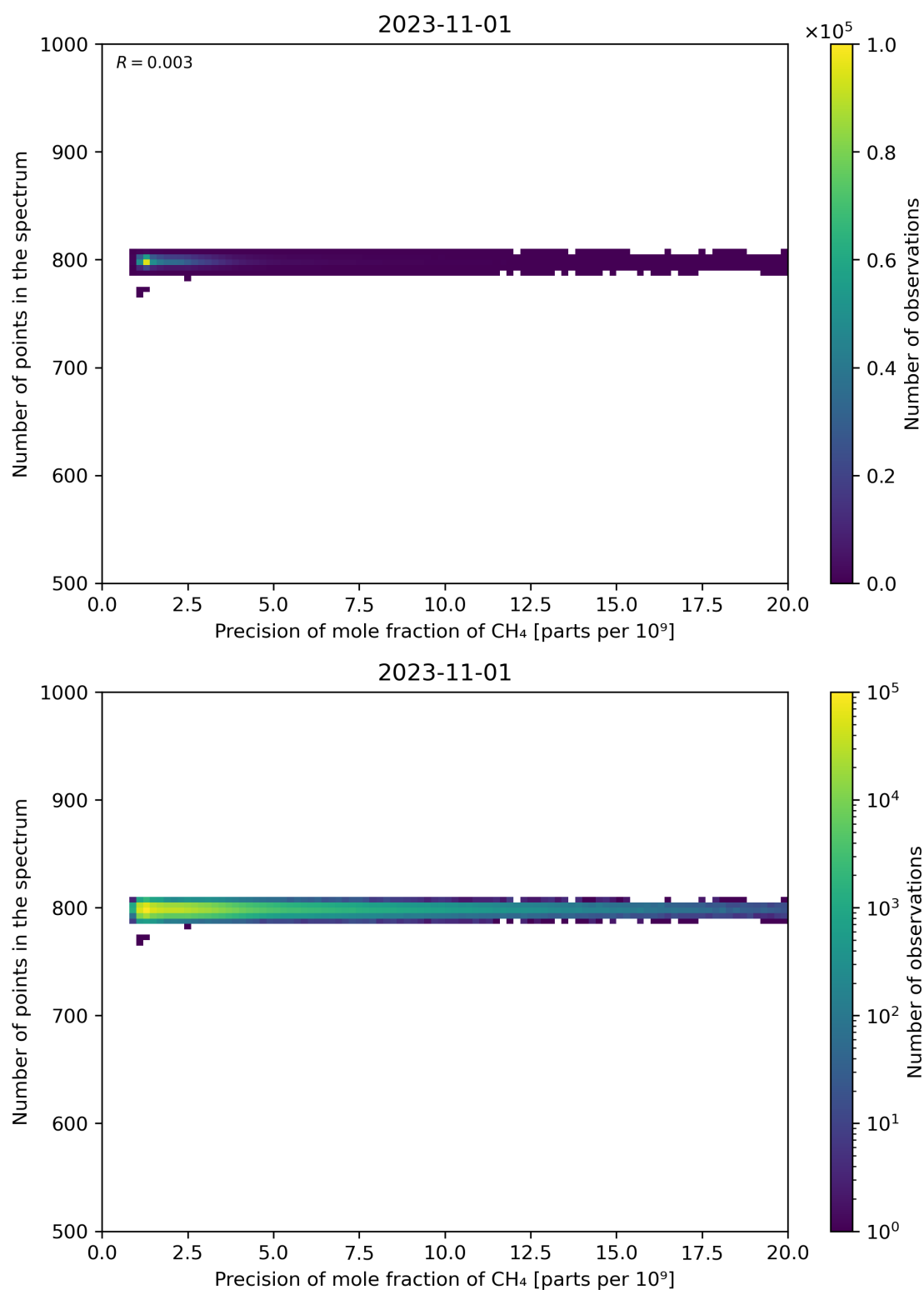
Figure 84: Scatter density plot of “Precision of mole fraction of CH 4 ” against “Number of points in the spectrum” for 2023-10-31 to 2023-11-02.
