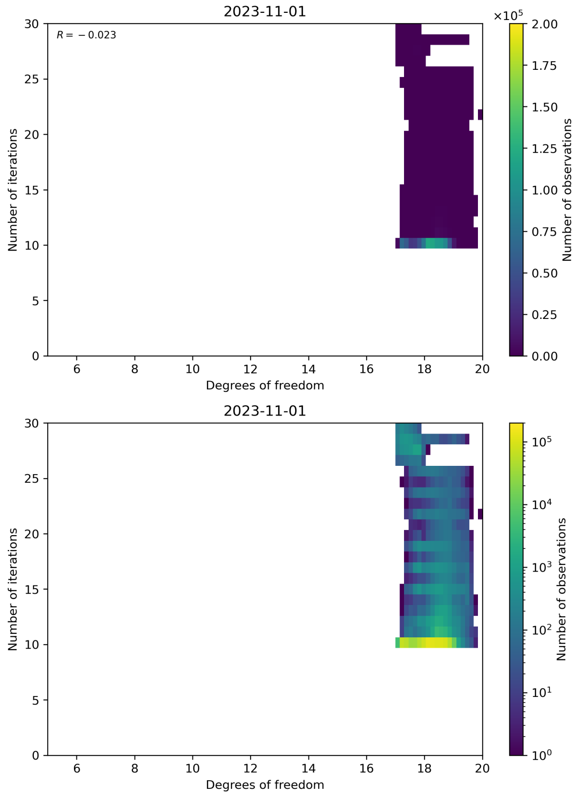
Figure 52: Scatter density plot of “Degrees of freedom” against “Number of iterations” for 2023-10-31 to 2023-11-02.
