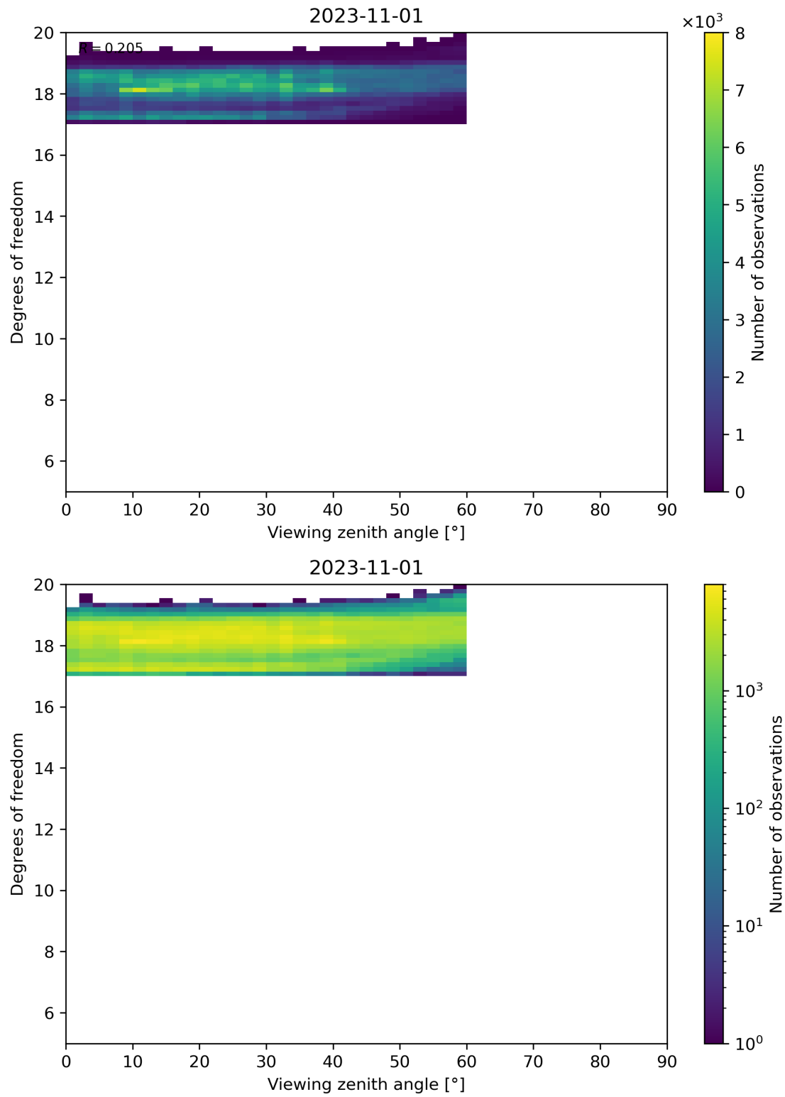
Figure 107: Scatter density plot of “Viewing zenith angle” against “Degrees of freedom” for 2023-10-31 to 2023-11-02.
