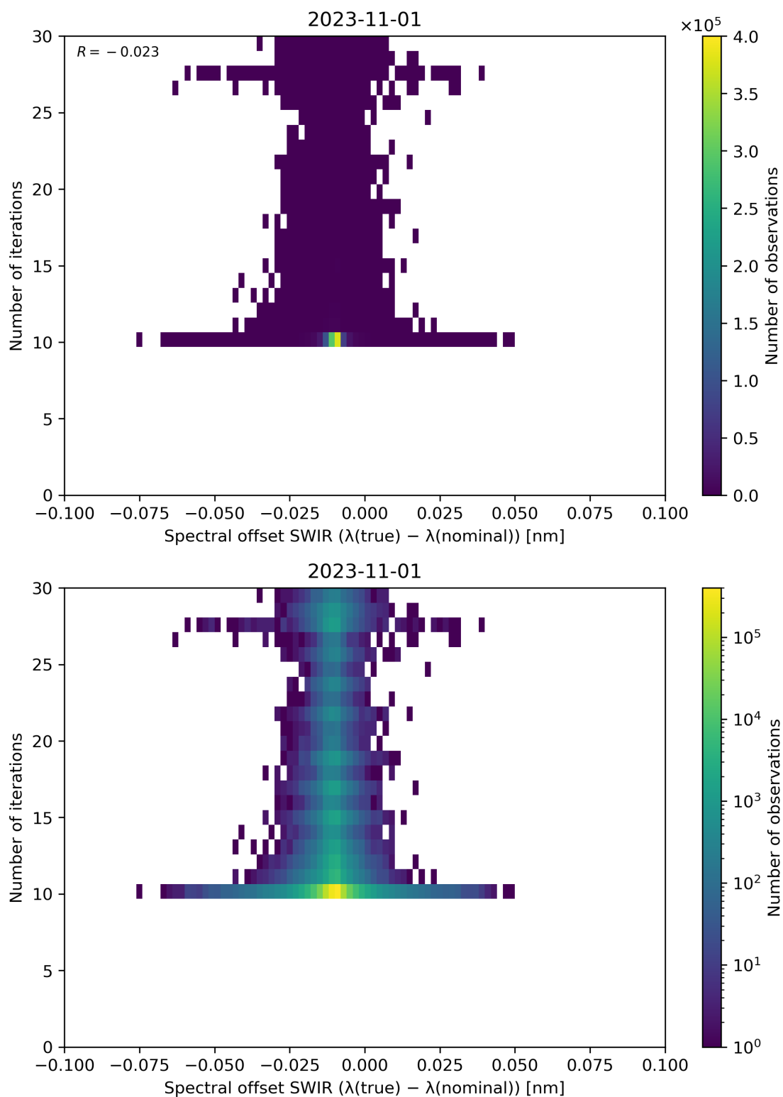
Figure 121: Scatter density plot of “Spectral offset SWIR ( \lambda(\text{true}) - \lambda(\text{nominal}) )” against “Number of iterations” for 2023-10-31 to 2023-11-02.
