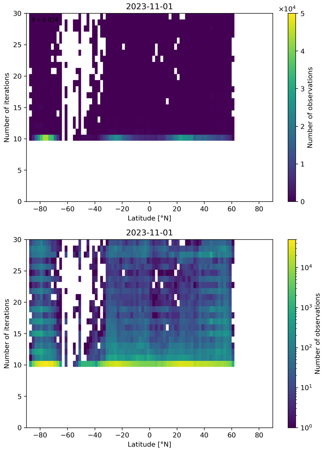
Figure 60: Scatter density plot of “Latitude” against “Number of iterations” for 2023-10-31 to 2023-11-02.
