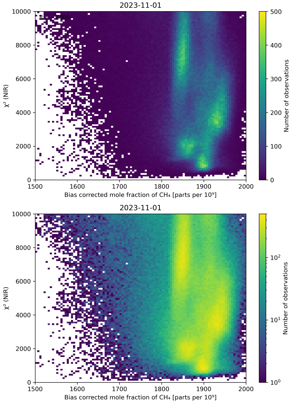
Figure 63: Scatter density plot of “Bias corrected mole fraction of \text{CH}_4 ” against “ \chi^2 (NIR)” for 2023-10-31 to 2023-11-02.
