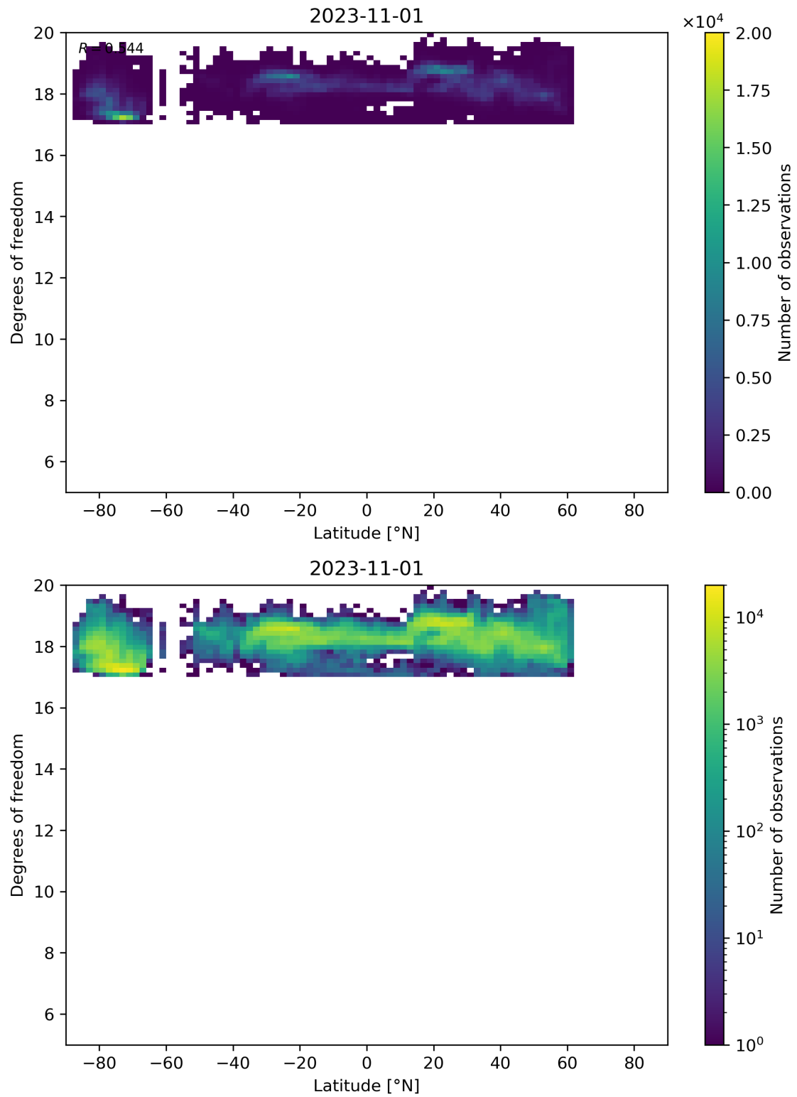
Figure 55: Scatter density plot of “Latitude” against “Degrees of freedom” for 2023-10-31 to 2023-11-02.
