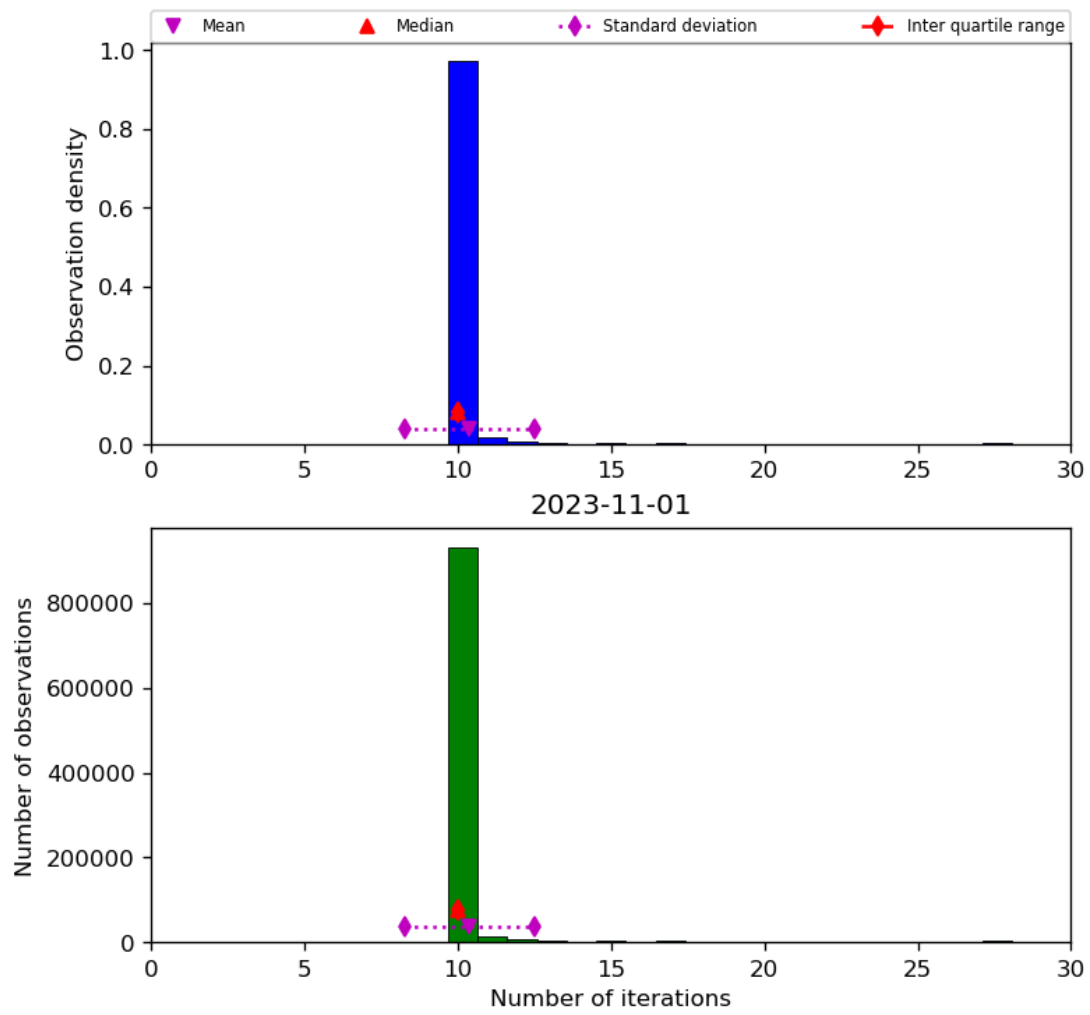
Figure 31: Histogram of “Number of iterations” for 2023-10-31 to 2023-11-02
