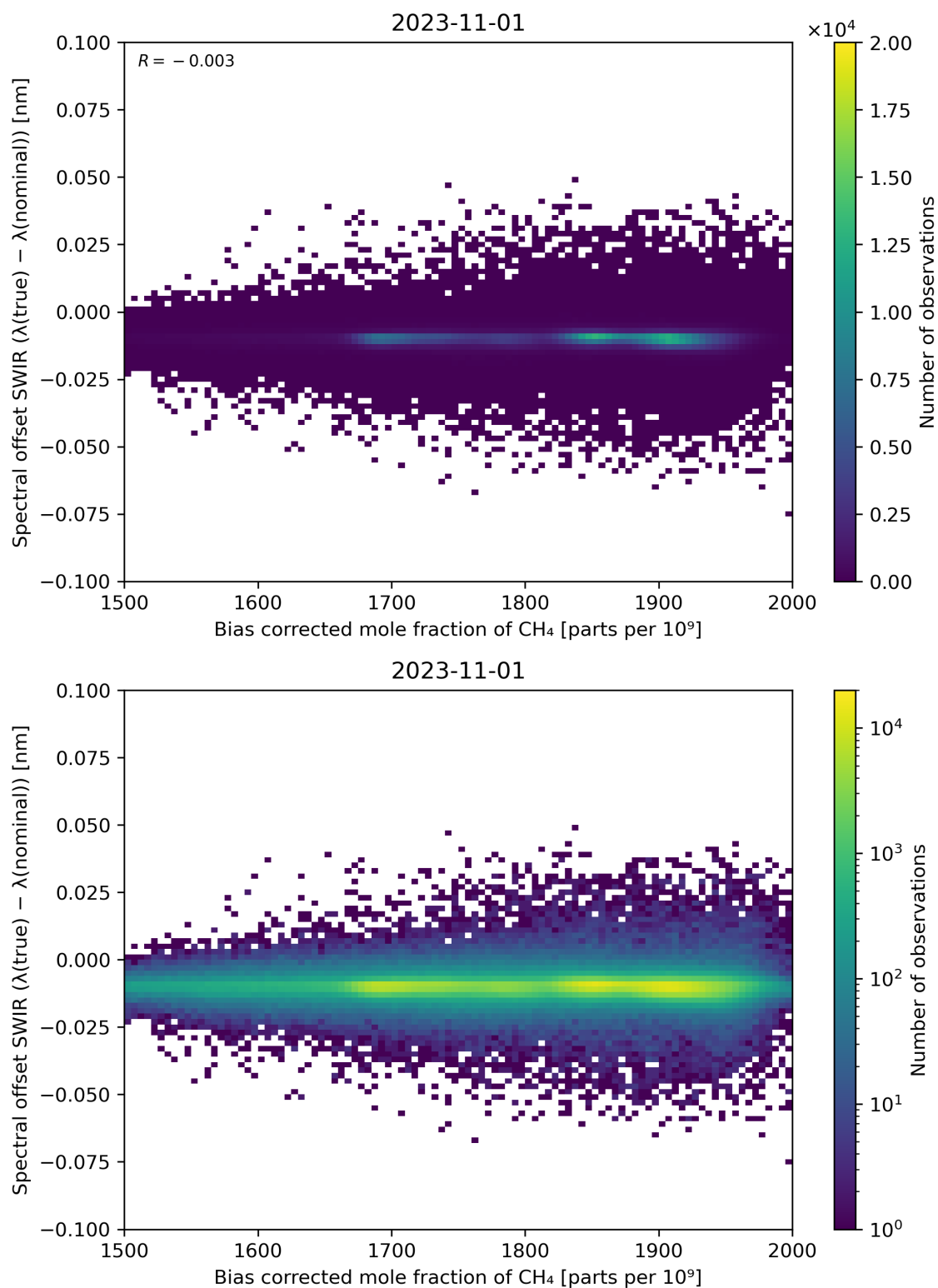
Figure 69: Scatter density plot of “Bias corrected mole fraction of \text{CH}_4 ” against “Spectral offset SWIR ( \lambda(\text{true}) - \lambda(\text{nominal}) )” for 2023-10-31 to 2023-11-02.
