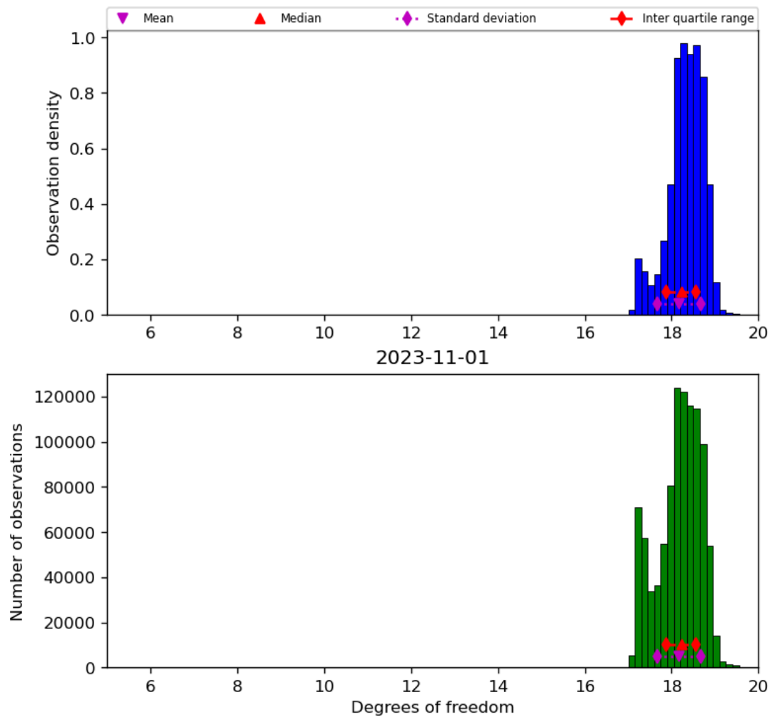
Figure 30: Histogram of “Degrees of freedom” for 2023-10-31 to 2023-11-02
