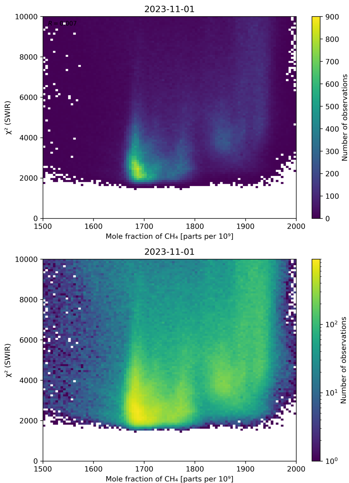
Figure 71: Scatter density plot of “Mole fraction of CH 4 ” against “ \chi^2 (SWIR)” for 2023-10-31 to 2023-11-02.
