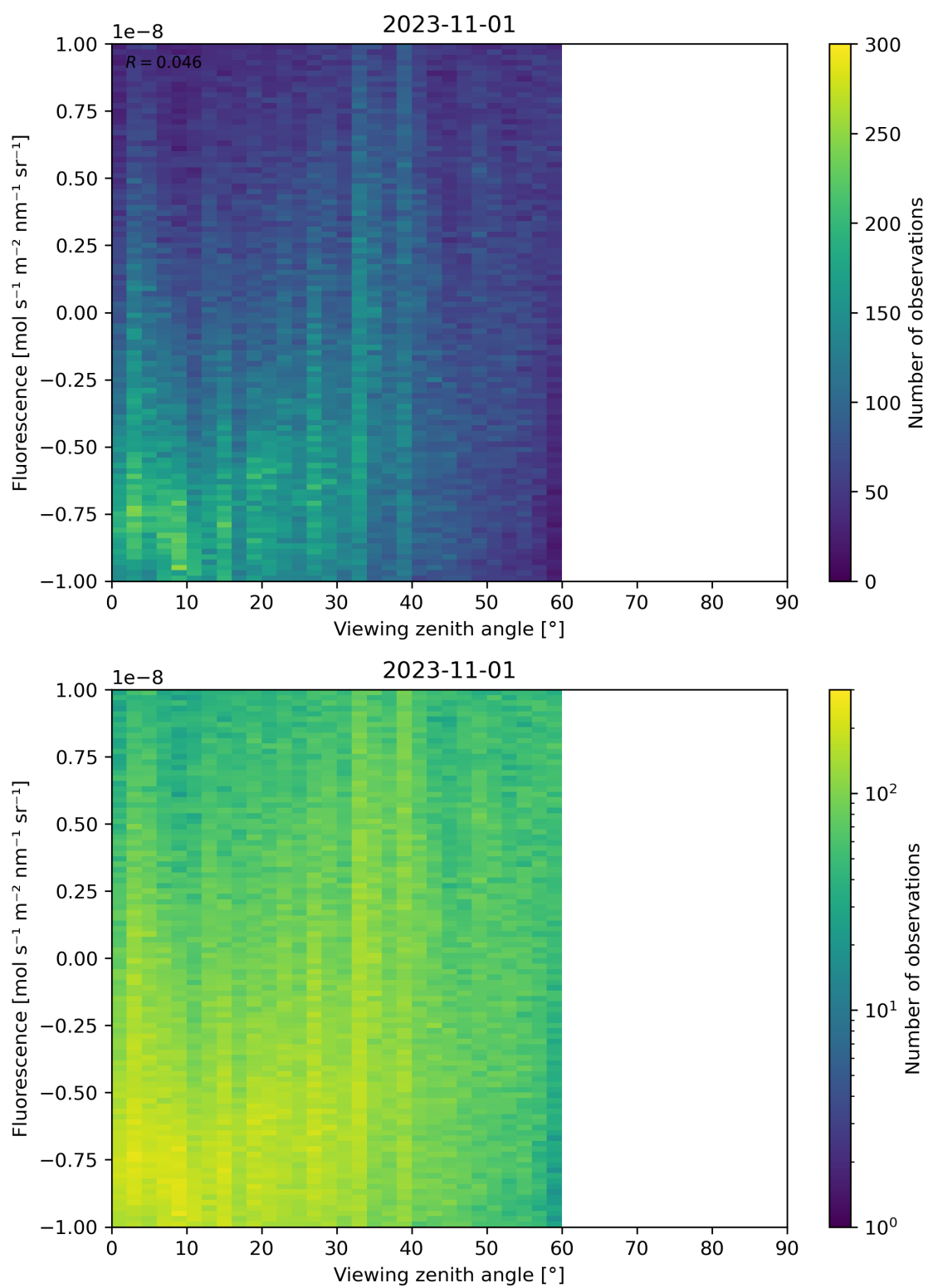
Figure 108: Scatter density plot of “Viewing zenith angle” against “Fluorescence” for 2023-10-31 to 2023-11-02.
