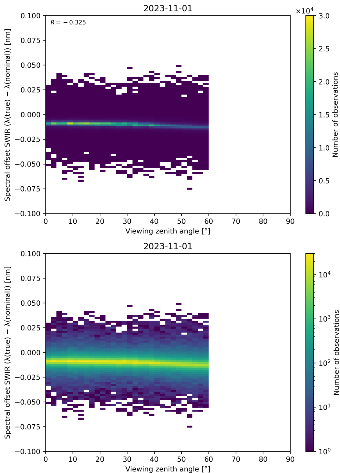
Figure 116: Scatter density plot of “Viewing zenith angle” against “Spectral offset SWIR ( \lambda(\text{true}) - \lambda(\text{nominal}) )” for 2023-10-31 to 2023-11-02.
