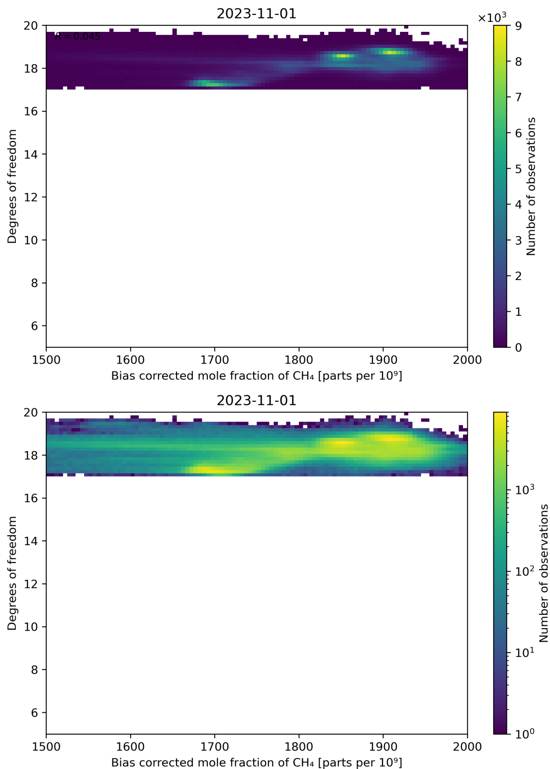
Figure 65: Scatter density plot of “Bias corrected mole fraction of CH 4 ” against “Degrees of freedom” for 2023-10-31 to 2023-11-02.
