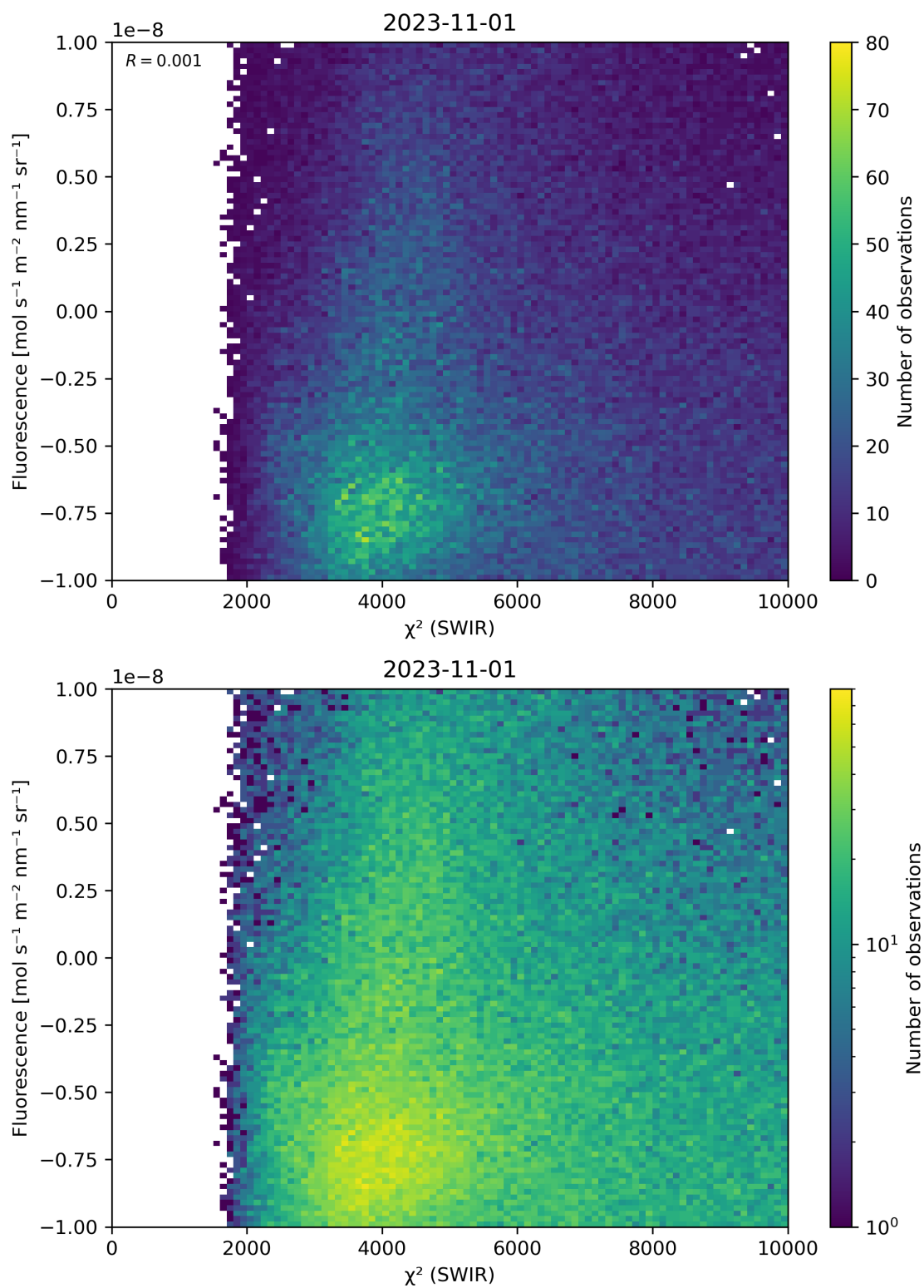
Figure 49: Scatter density plot of “ \chi^2 (SWIR)” against “Fluorescence” for 2023-10-31 to 2023-11-02.
