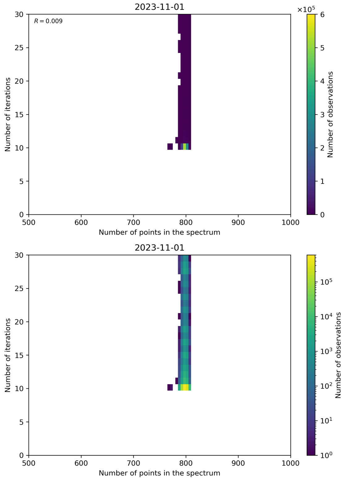
Figure 92: Scatter density plot of “Number of points in the spectrum” against “Number of iterations” for 2023-10-31 to 2023-11-02.
