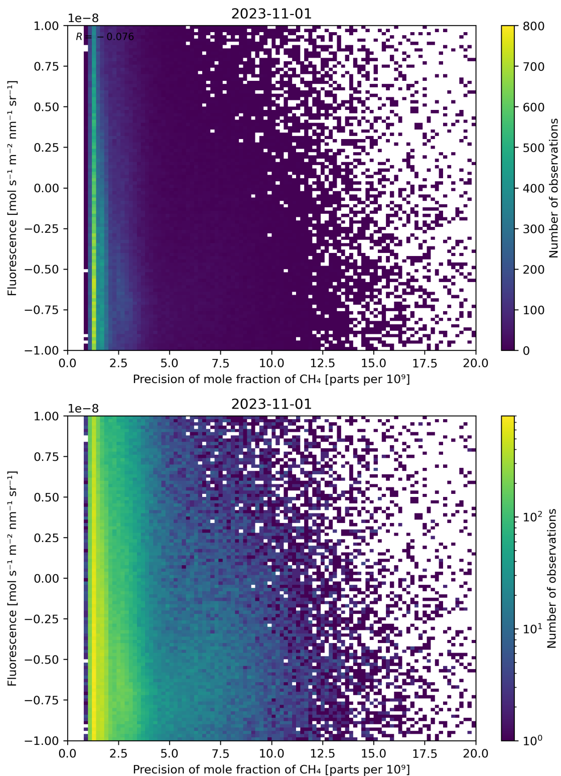
Figure 81: Scatter density plot of “Precision of mole fraction of \text{CH}_4 ” against “Fluorescence” for 2023-10-31 to 2023-11-02.
