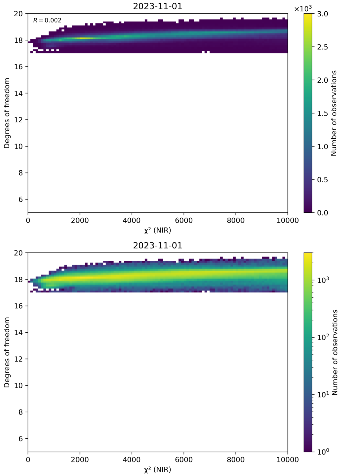
Figure 44: Scatter density plot of “ \chi^2 (NIR)” against “Degrees of freedom” for 2023-10-31 to 2023-11-02.
