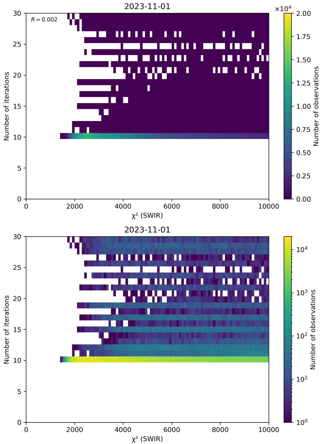
Figure 50: Scatter density plot of “ \chi^2 (SWIR)” against “Number of iterations” for 2023-10-31 to 2023-11-02.
