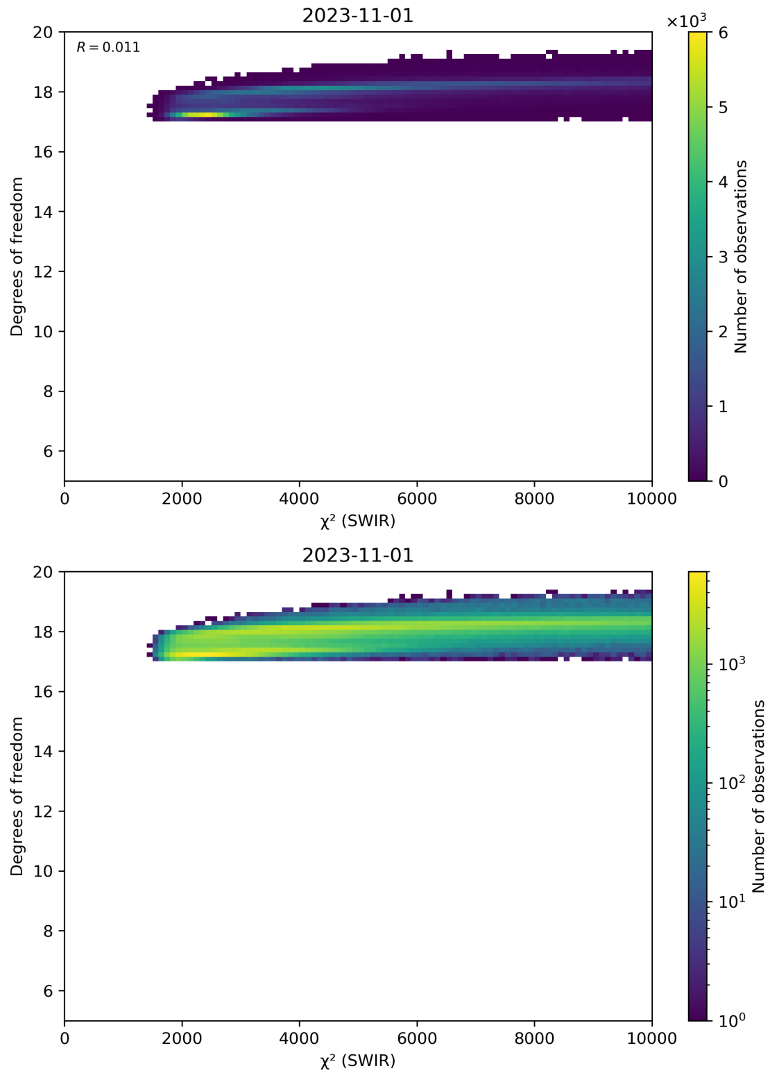
Figure 48: Scatter density plot of “ \chi^2 (SWIR)” against “Degrees of freedom” for 2023-10-31 to 2023-11-02.
