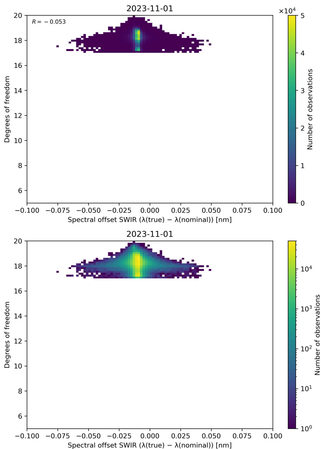
Figure 119: Scatter density plot of “Spectral offset SWIR ( \lambda(\text{true}) - \lambda(\text{nominal}) )” against “Degrees of freedom” for 2023-10-31 to 2023-11-02.
