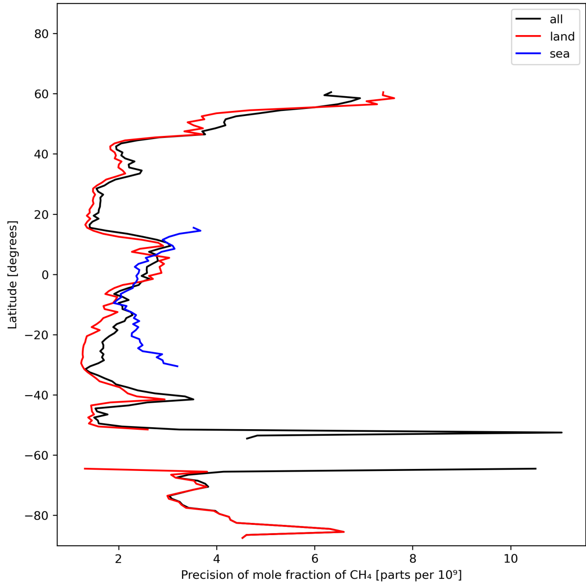
Figure 13: Zonal average of “Precision of mole fraction of CH 4 ” for 2023-10-31 to 2023-11-02.
