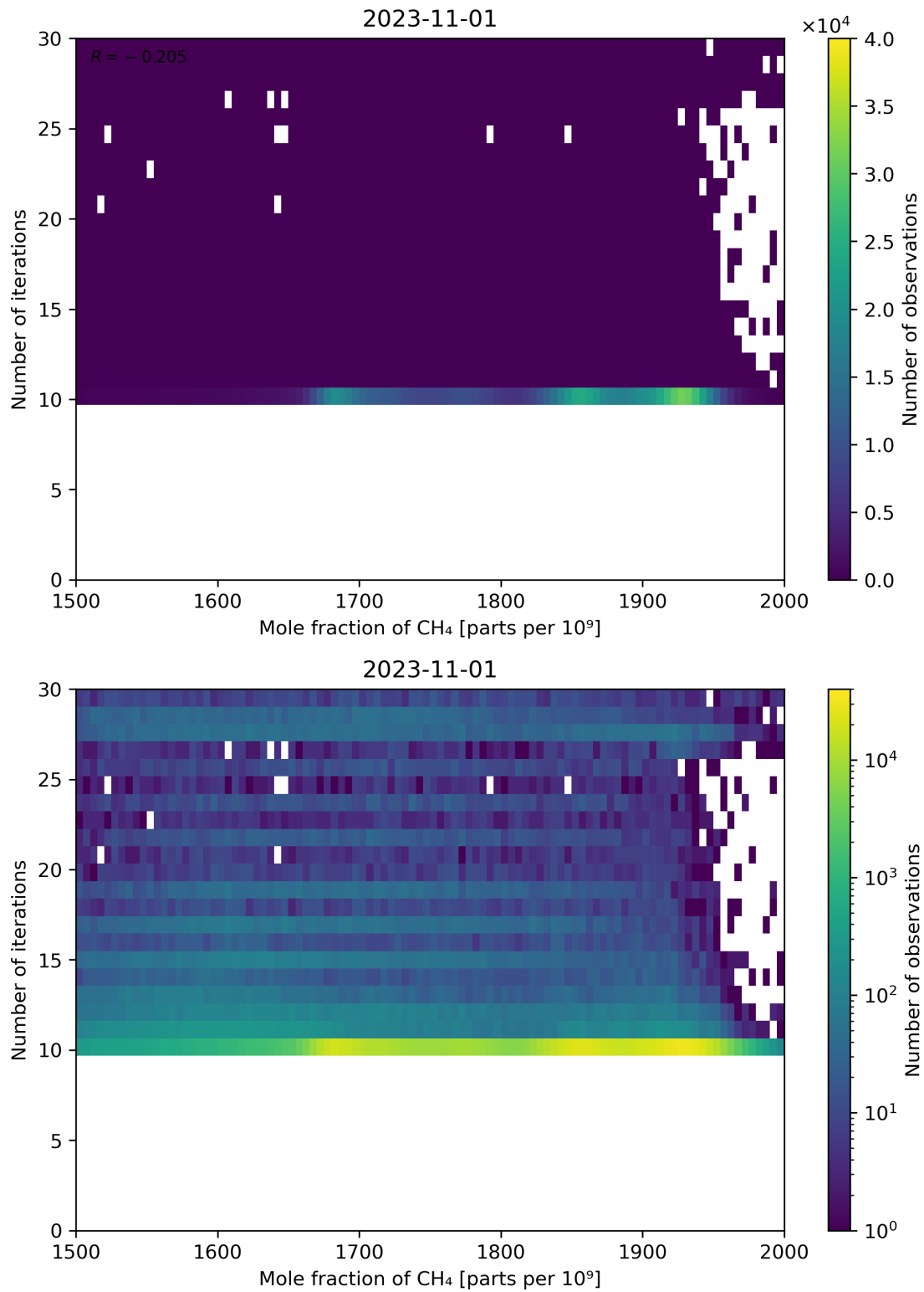
Figure 76: Scatter density plot of “Mole fraction of CH 4 ” against “Number of iterations” for 2023-10-31 to 2023-11-02.
