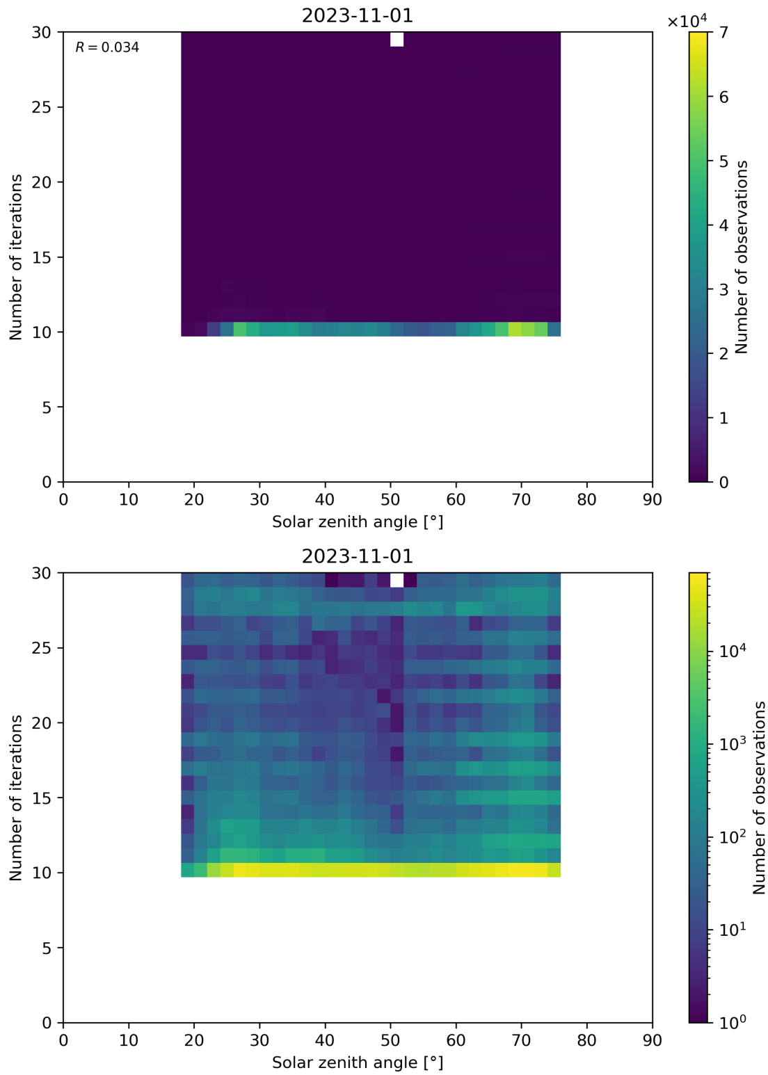
Figure 102: Scatter density plot of “Solar zenith angle” against “Number of iterations” for 2023-10-31 to 2023-11-02.
