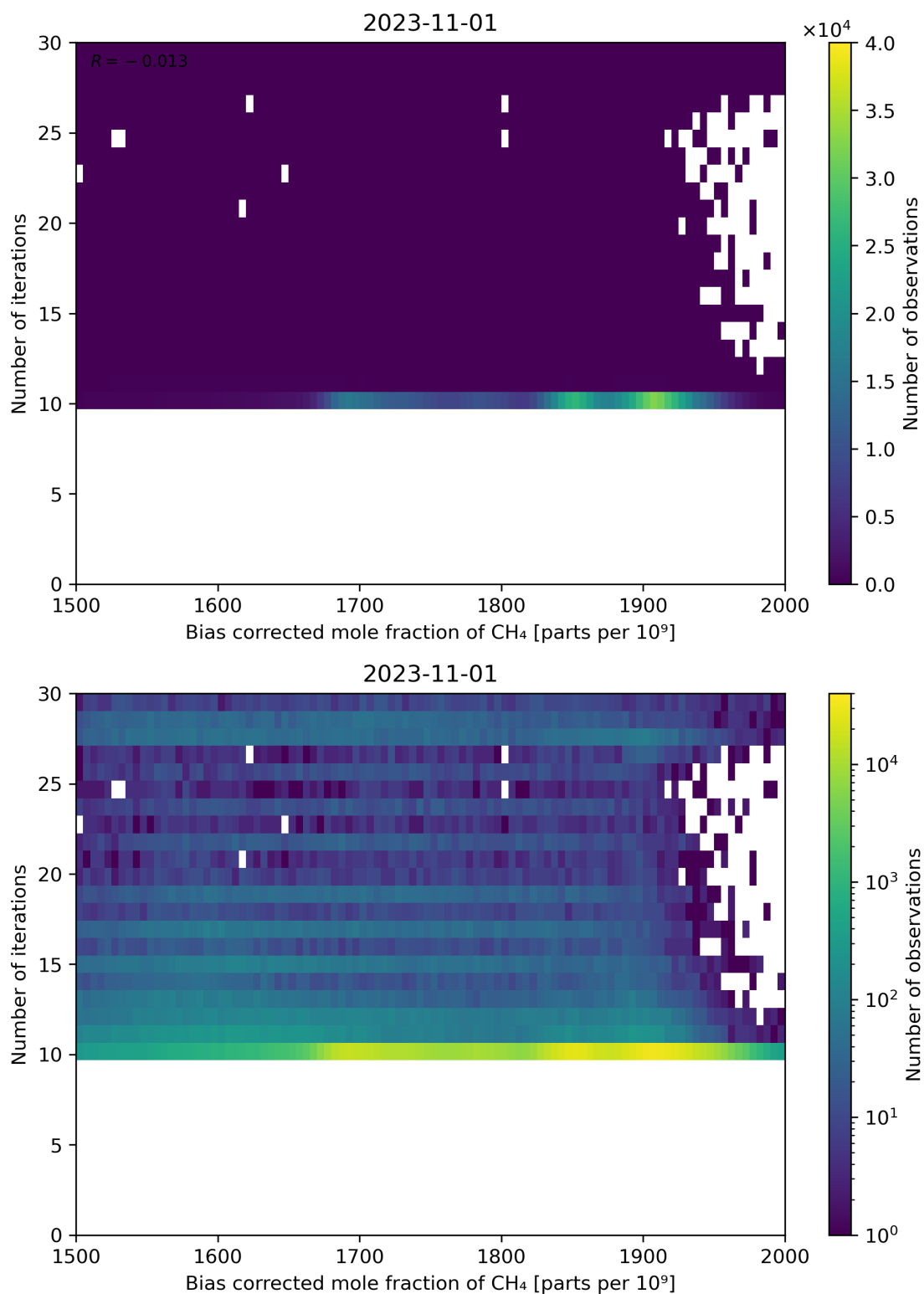
Figure 67: Scatter density plot of “Bias corrected mole fraction of CH 4 ” against “Number of iterations” for 2023-10-31 to 2023-11-02.
