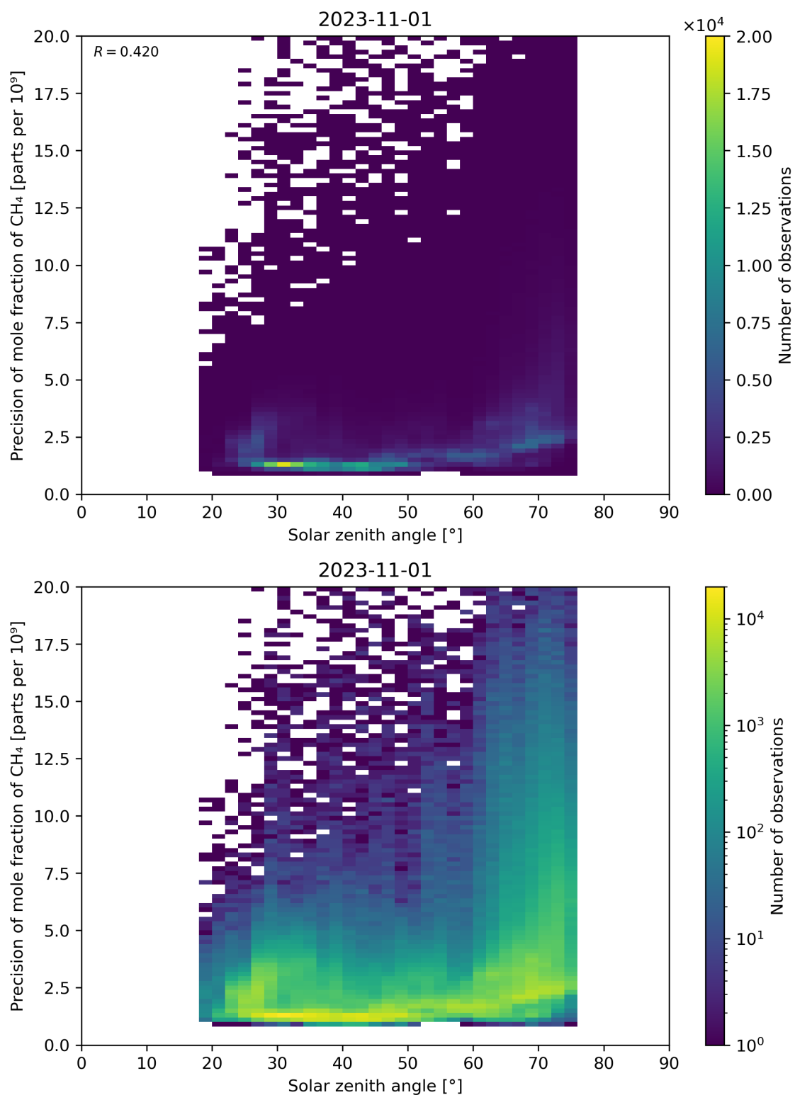
Figure 101: Scatter density plot of “Solar zenith angle” against “Precision of mole fraction of \text{CH}_4 ” for 2023-10-31 to 2023-11-02.
