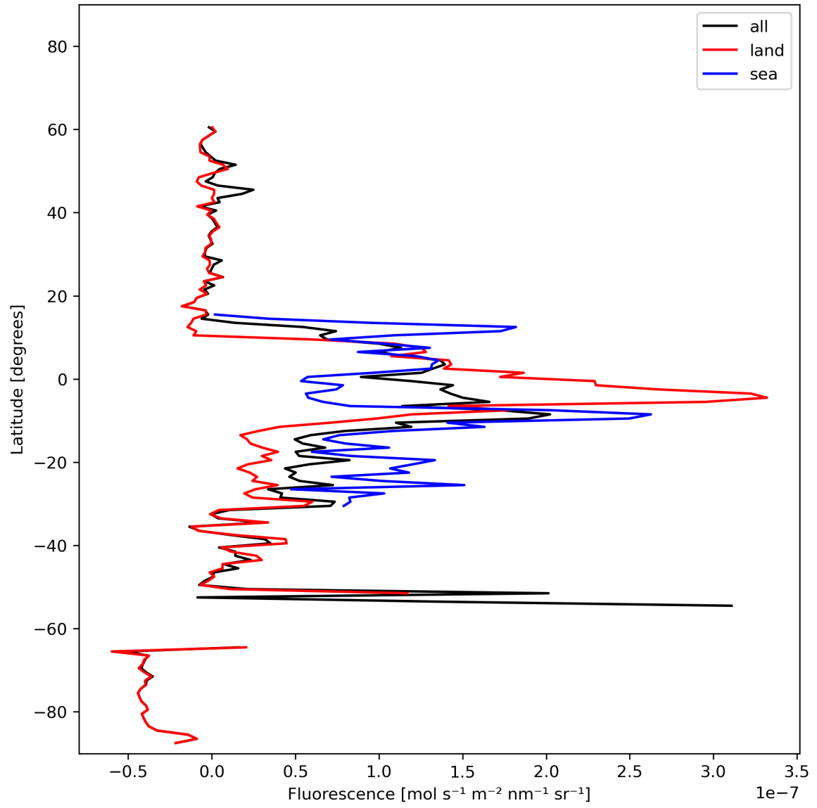
Figure 21: Zonal average of “Fluorescence” for 2023-10-31 to 2023-11-02.
