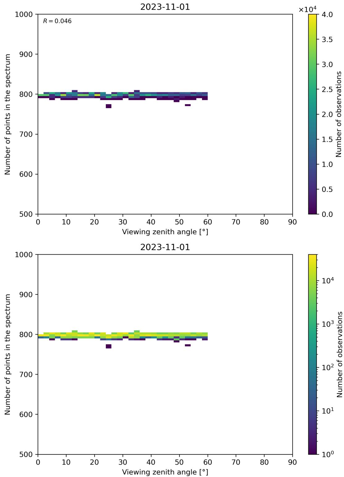
Figure 114: Scatter density plot of “Viewing zenith angle” against “Number of points in the spectrum” for 2023-10-31 to 2023-11-02.
