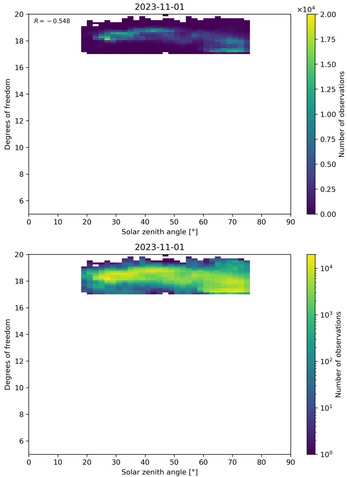
Figure 96: Scatter density plot of “Solar zenith angle” against “Degrees of freedom” for 2023-10-31 to 2023-11-02.
