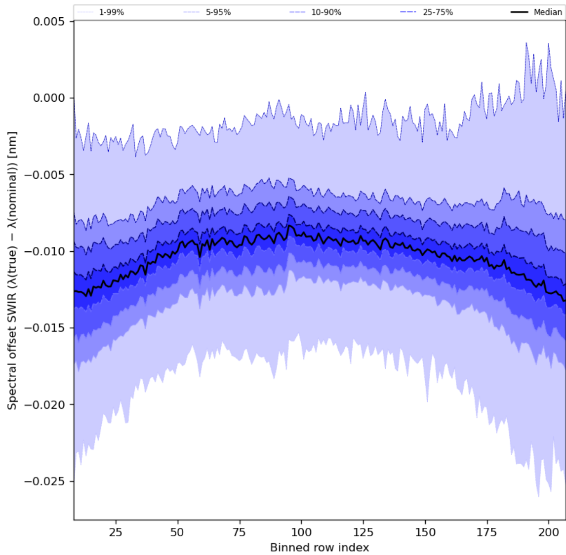
Figure 38: Along track statistics of “Spectral offset SWIR ( \lambda(\text{true}) - \lambda(\text{nominal}) )” for 2023-10-31 to 2023-11-02
