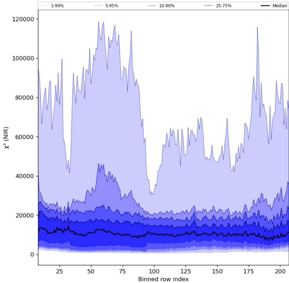
Figure 40: Along track statistics of “ \chi^2 (NIR)” for 2023-10-31 to 2023-11-02
