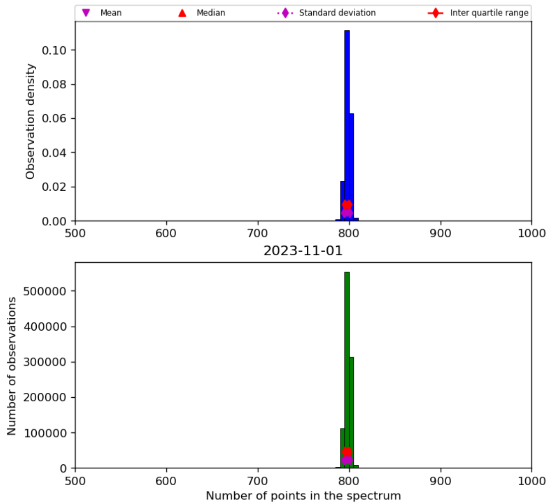
Figure 26: Histogram of “Number of points in the spectrum” for 2023-10-31 to 2023-11-02
