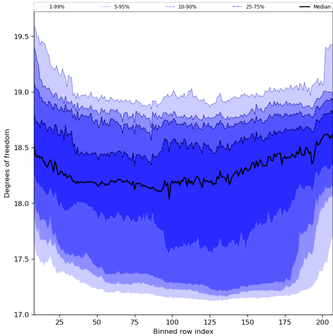
Figure 41: Along track statistics of “Degrees of freedom” for 2023-10-31 to 2023-11-02
