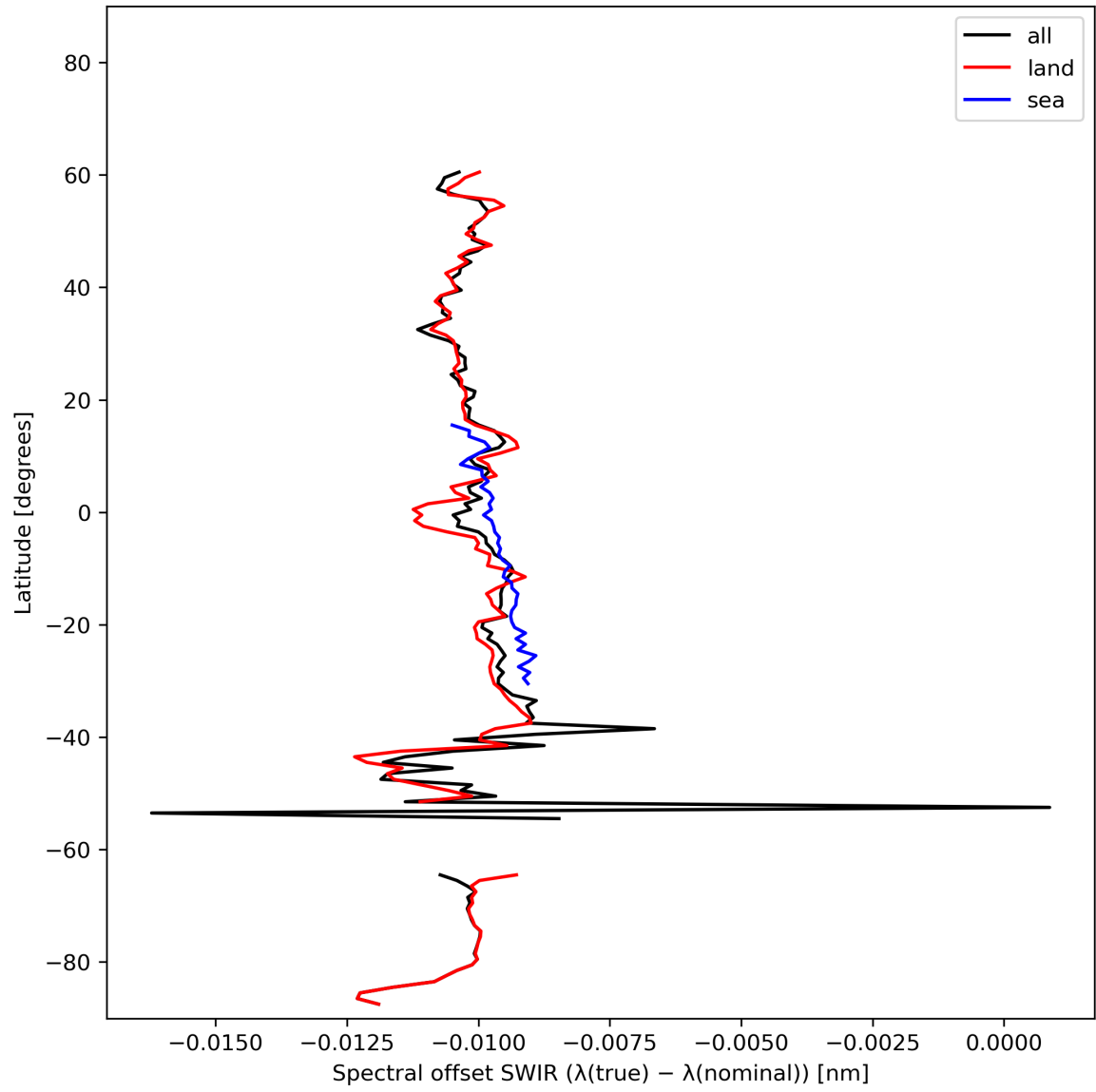
Figure 16: Zonal average of “Spectral offset SWIR ( \lambda(\text{true}) - \lambda(\text{nominal}) )” for 2023-10-31 to 2023-11-02.
