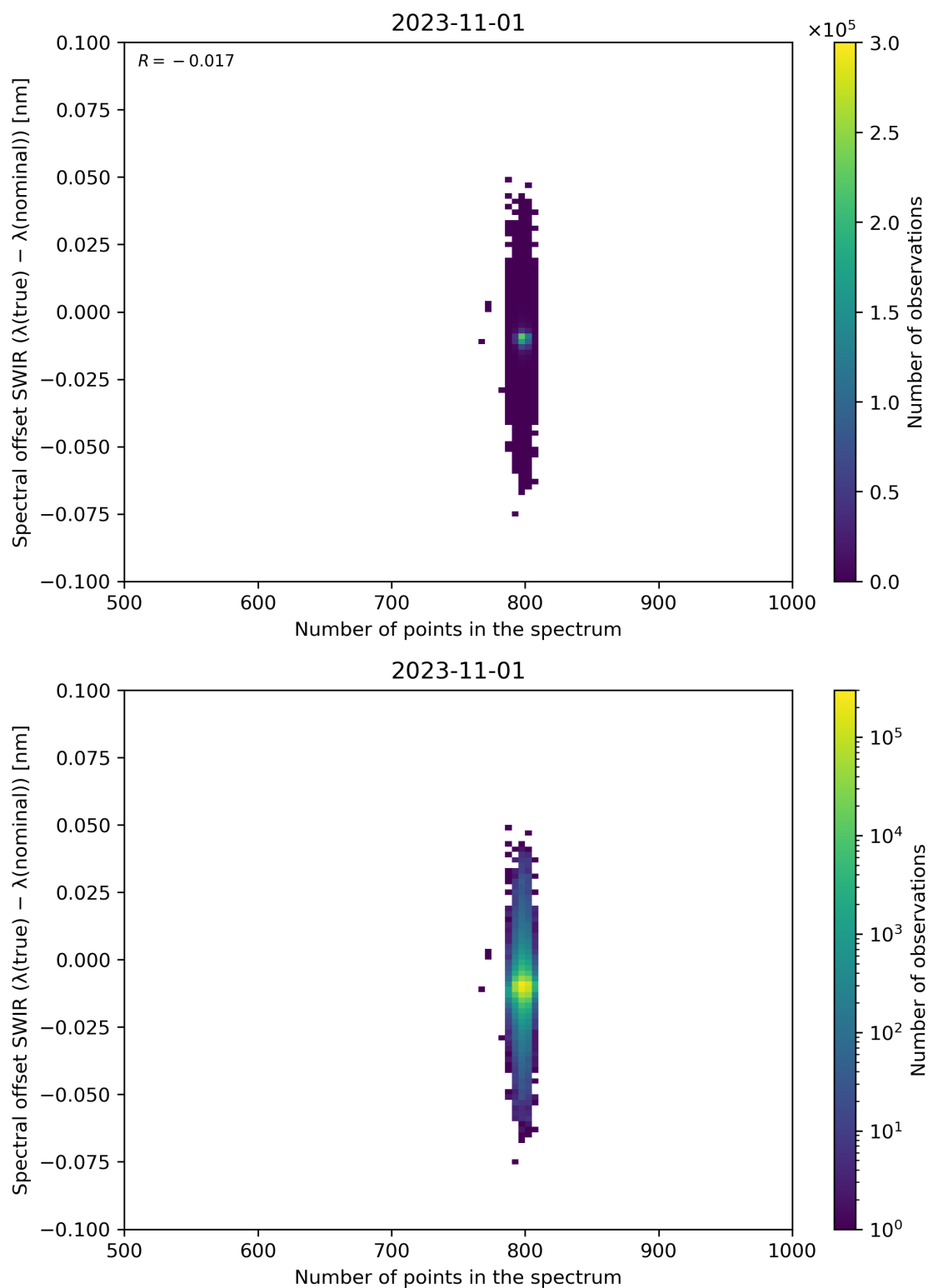
Figure 93: Scatter density plot of “Number of points in the spectrum” against “Spectral offset SWIR ( \lambda(\text{true}) - \lambda(\text{nominal}) )” for 2023-10-31 to 2023-11-02.
