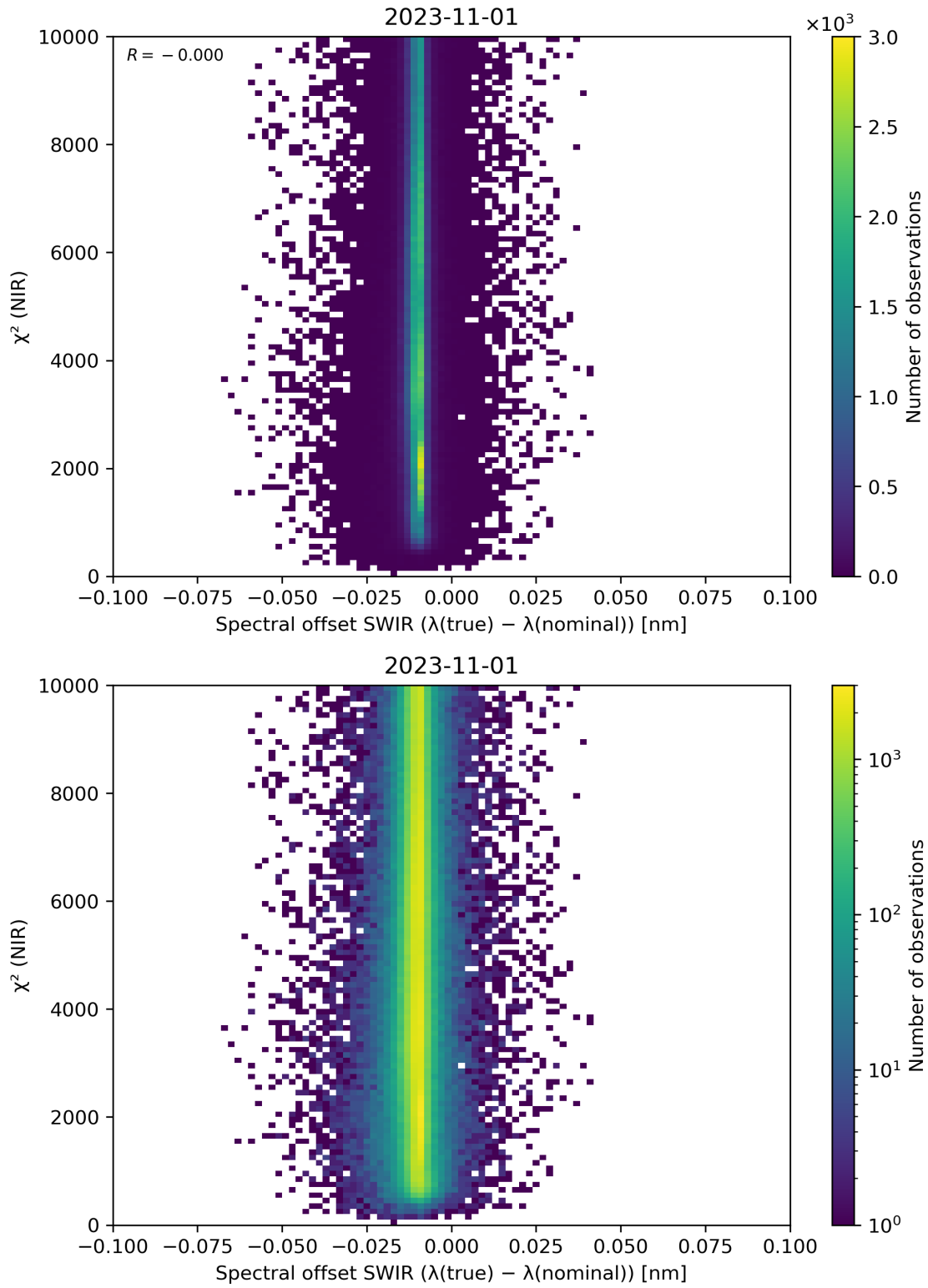
Figure 117: Scatter density plot of “Spectral offset SWIR ( \lambda(\text{true}) - \lambda(\text{nominal}) )” against “ \chi^2 (NIR)” for 2023-10-31 to 2023-11-02.
