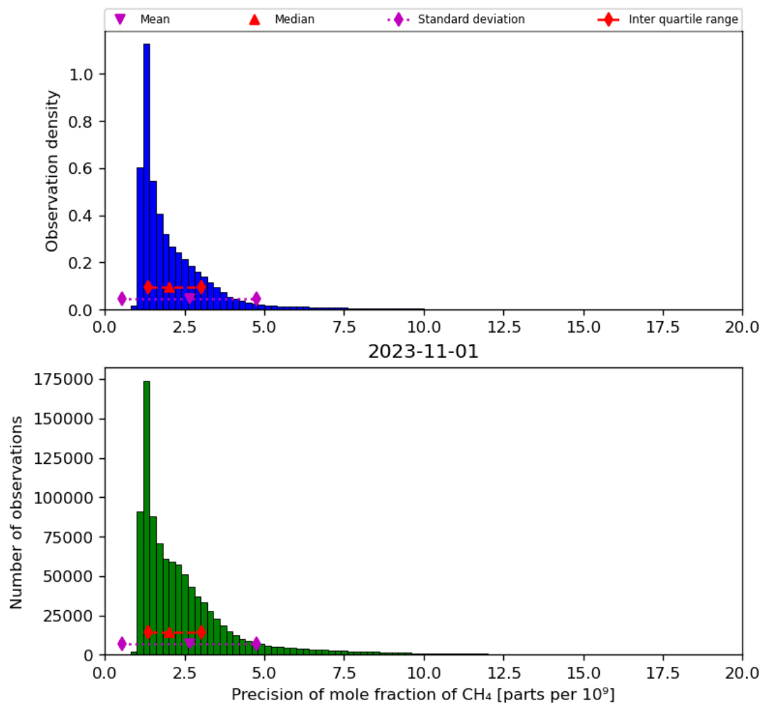
Figure 24: Histogram of “Precision of mole fraction of CH 4 ” for 2023-10-31 to 2023-11-02
