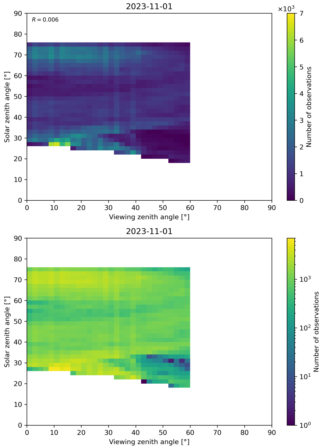
Figure 115: Scatter density plot of “Viewing zenith angle” against “Solar zenith angle” for 2023-10-31 to 2023-11-02.
