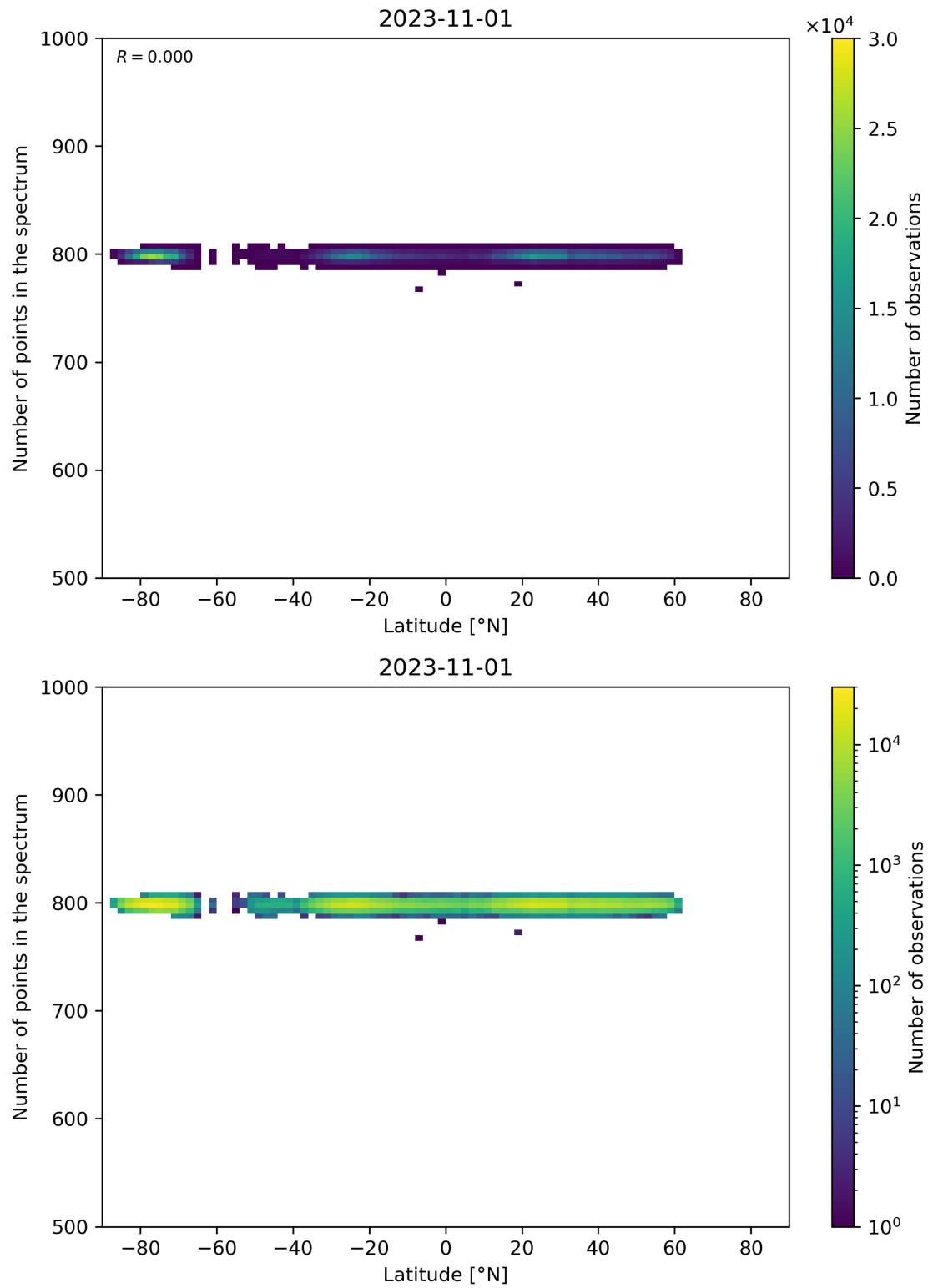
Figure 61: Scatter density plot of “Latitude” against “Number of points in the spectrum” for 2023-10-31 to 2023-11-02.
