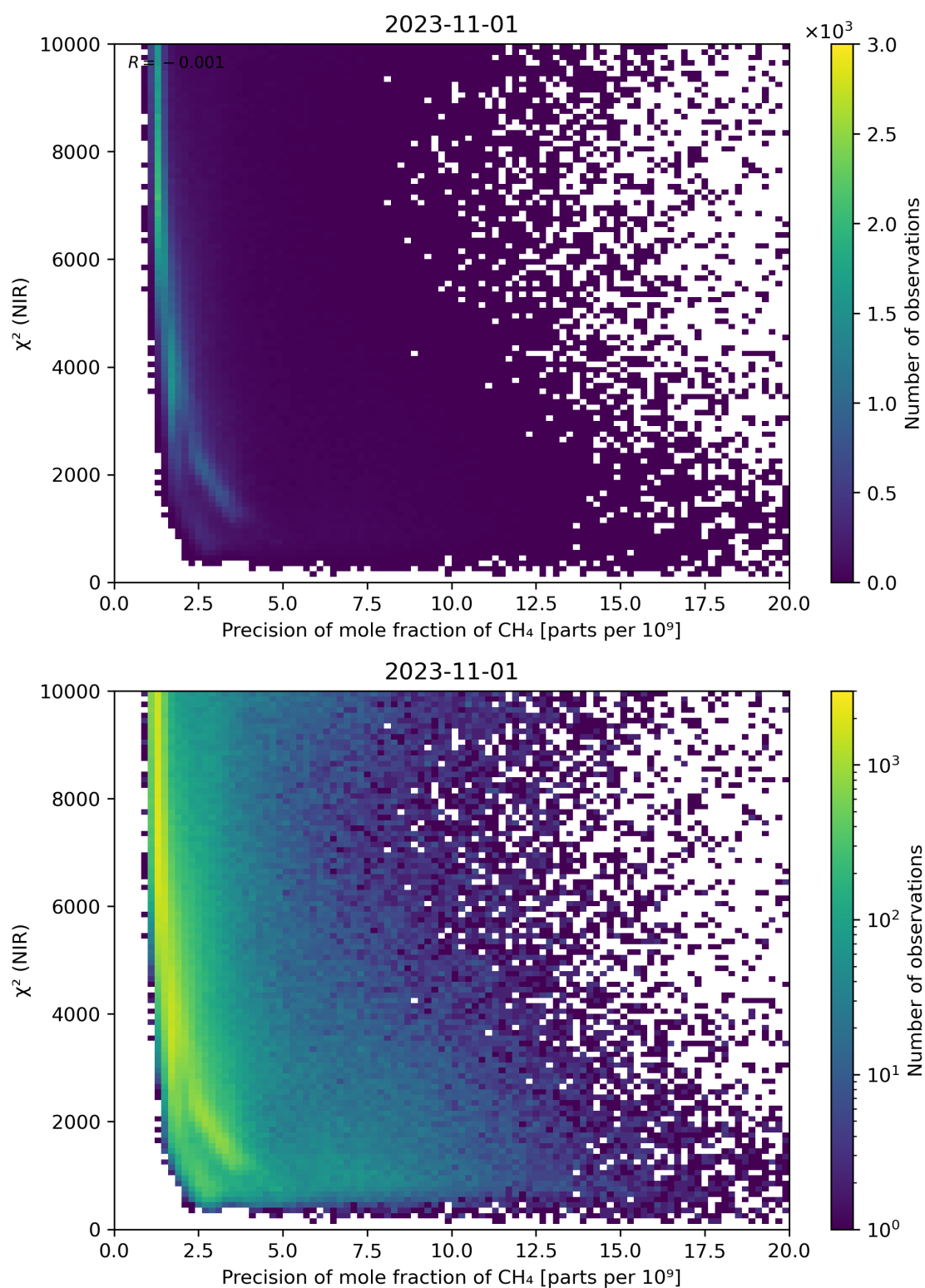
Figure 78: Scatter density plot of “Precision of mole fraction of CH 4 ” against “ \chi^2 (NIR)” for 2023-10-31 to 2023-11-02.
