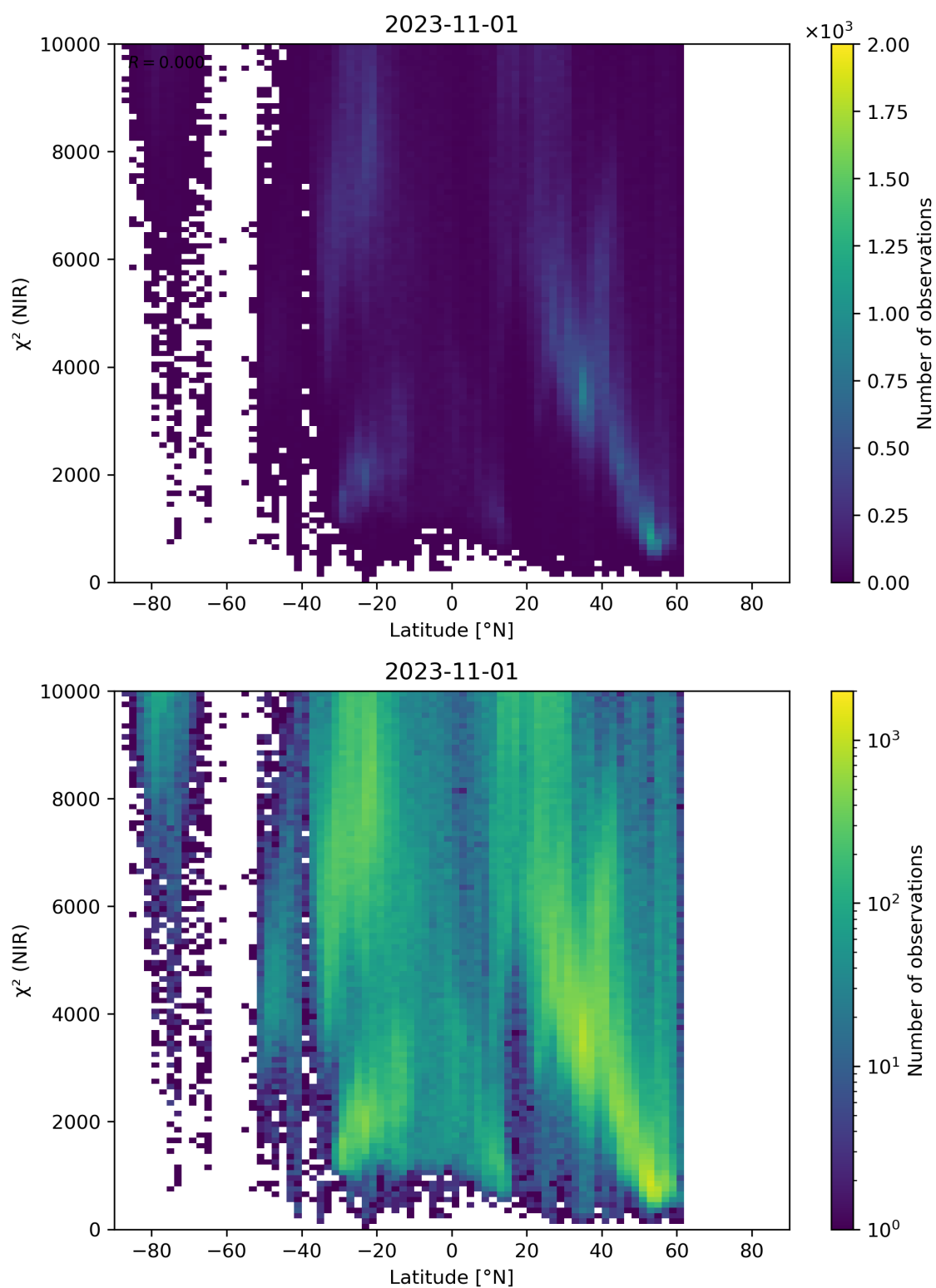
Figure 53: Scatter density plot of “Latitude” against “ \chi^2 (NIR)” for 2023-10-31 to 2023-11-02.
