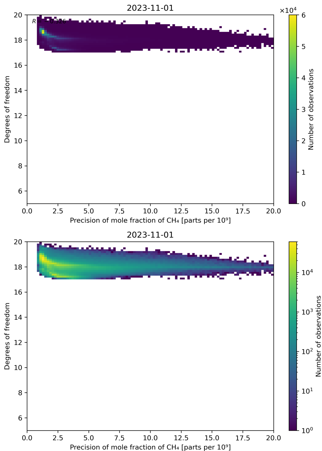
Figure 80: Scatter density plot of “Precision of mole fraction of CH 4 ” against “Degrees of freedom” for 2023-10-31 to 2023-11-02.
