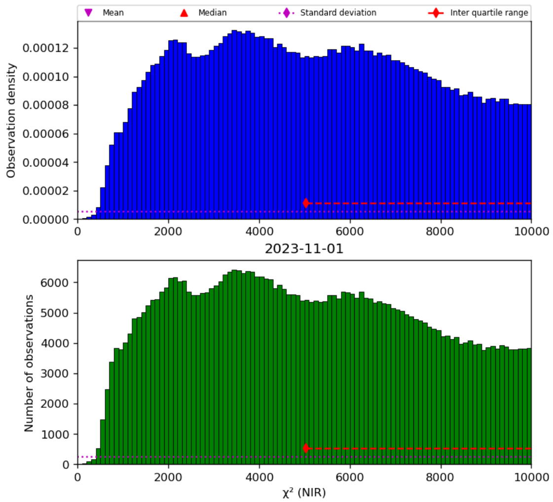
Figure 29: Histogram of “ \chi^2 (NIR)” for 2023-10-31 to 2023-11-02
