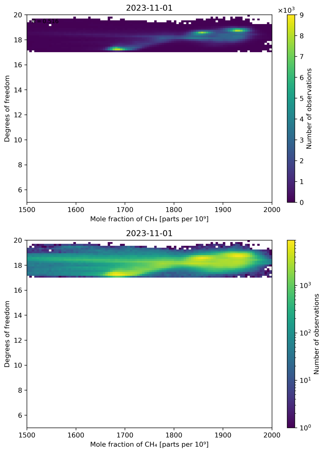
Figure 72: Scatter density plot of “Mole fraction of CH 4 ” against “Degrees of freedom” for 2023-10-31 to 2023-11-02.
