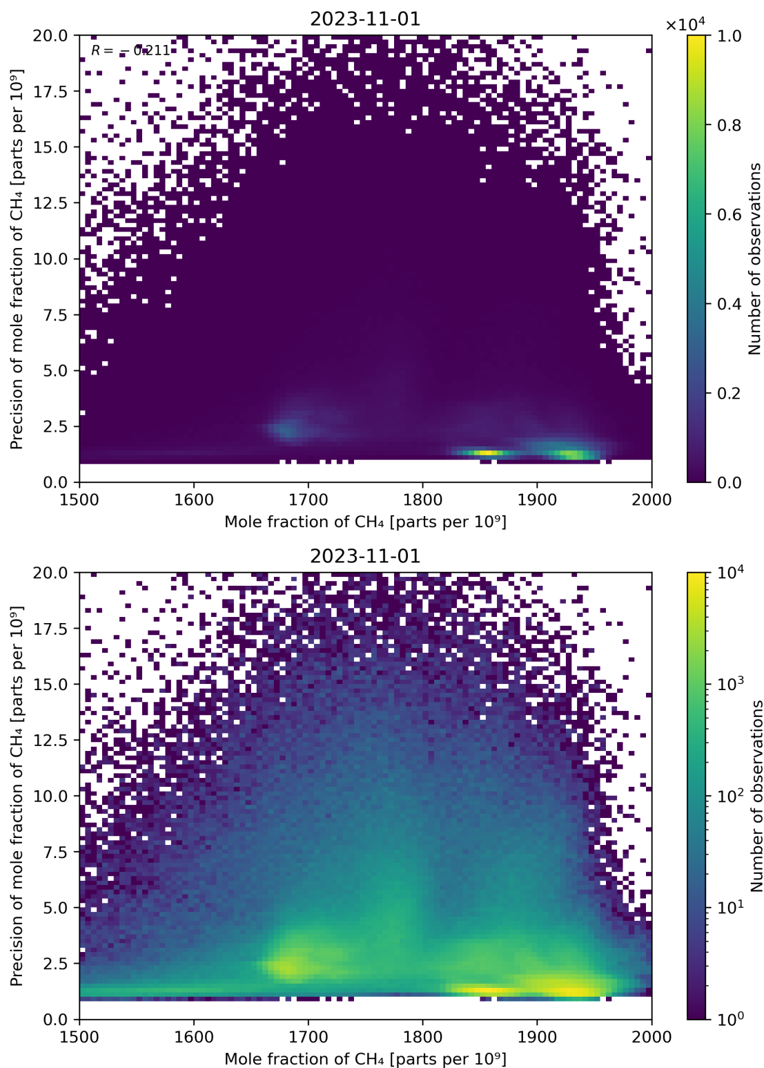
Figure 75: Scatter density plot of “Mole fraction of CH 4 ” against “Precision of mole fraction of CH 4 ” for 2023-10-31 to 2023-11-02.
