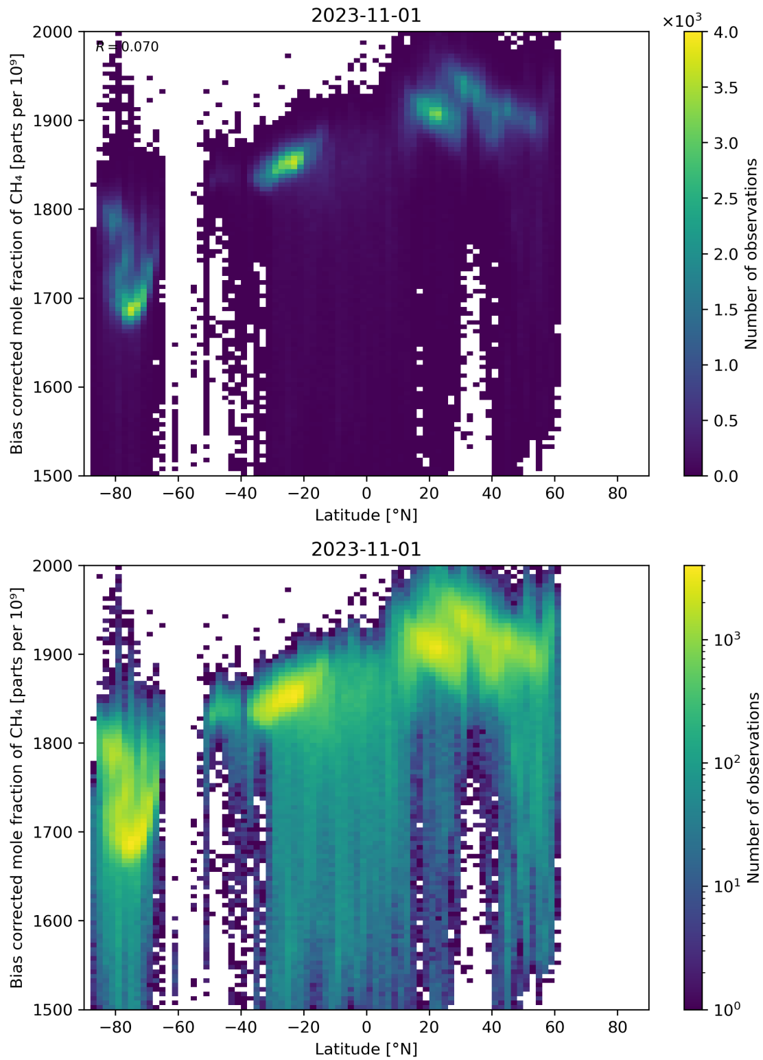
Figure 58: Scatter density plot of “Latitude” against “Bias corrected mole fraction of CH 4 ” for 2023-10-31 to 2023-11-02.
