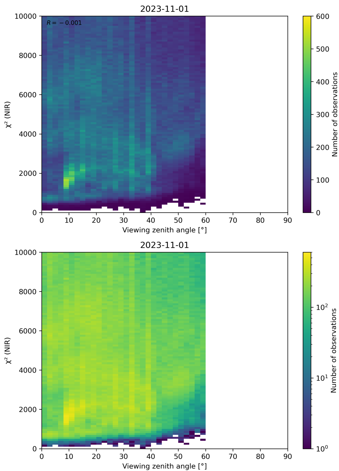
Figure 105: Scatter density plot of “Viewing zenith angle” against “ \chi^2 (NIR)” for 2023-10-31 to 2023-11-02.
