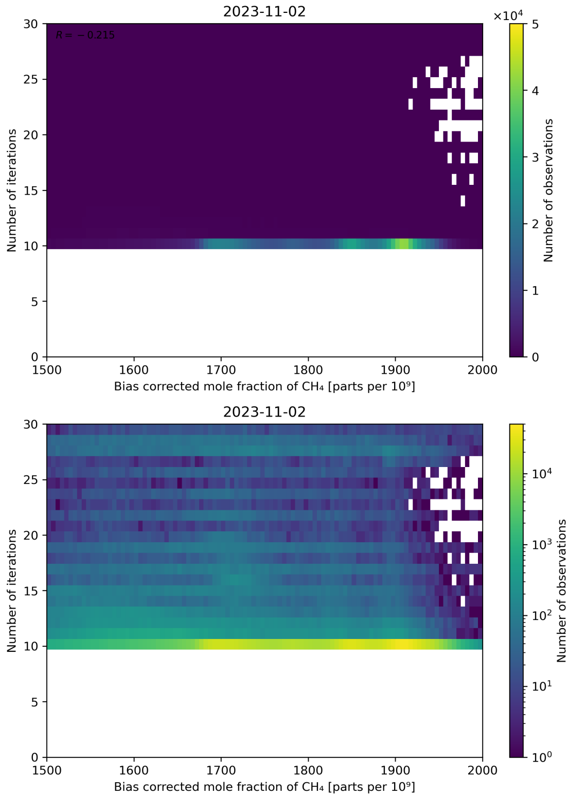
Figure 67: Scatter density plot of “Bias corrected mole fraction of CH 4 ” against “Number of iterations” for 2023-11-02 to 2023-11-03.
