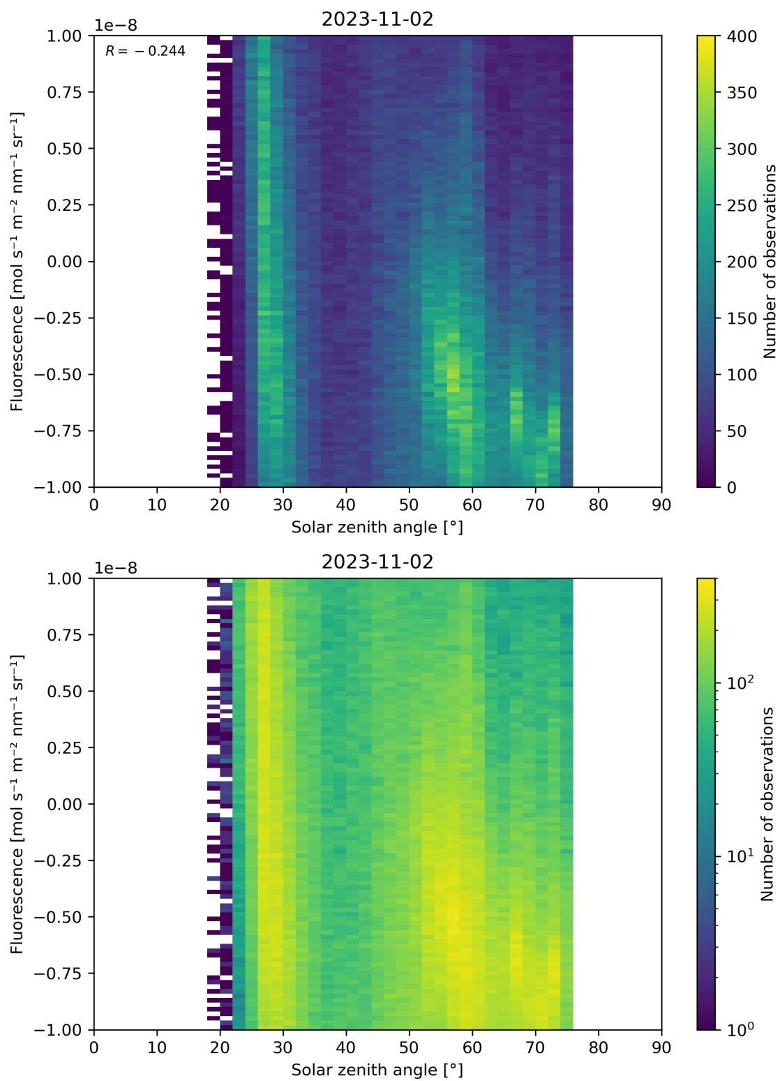
Figure 97: Scatter density plot of “Solar zenith angle” against “Fluorescence” for 2023-11-02 to 2023-11-03.
