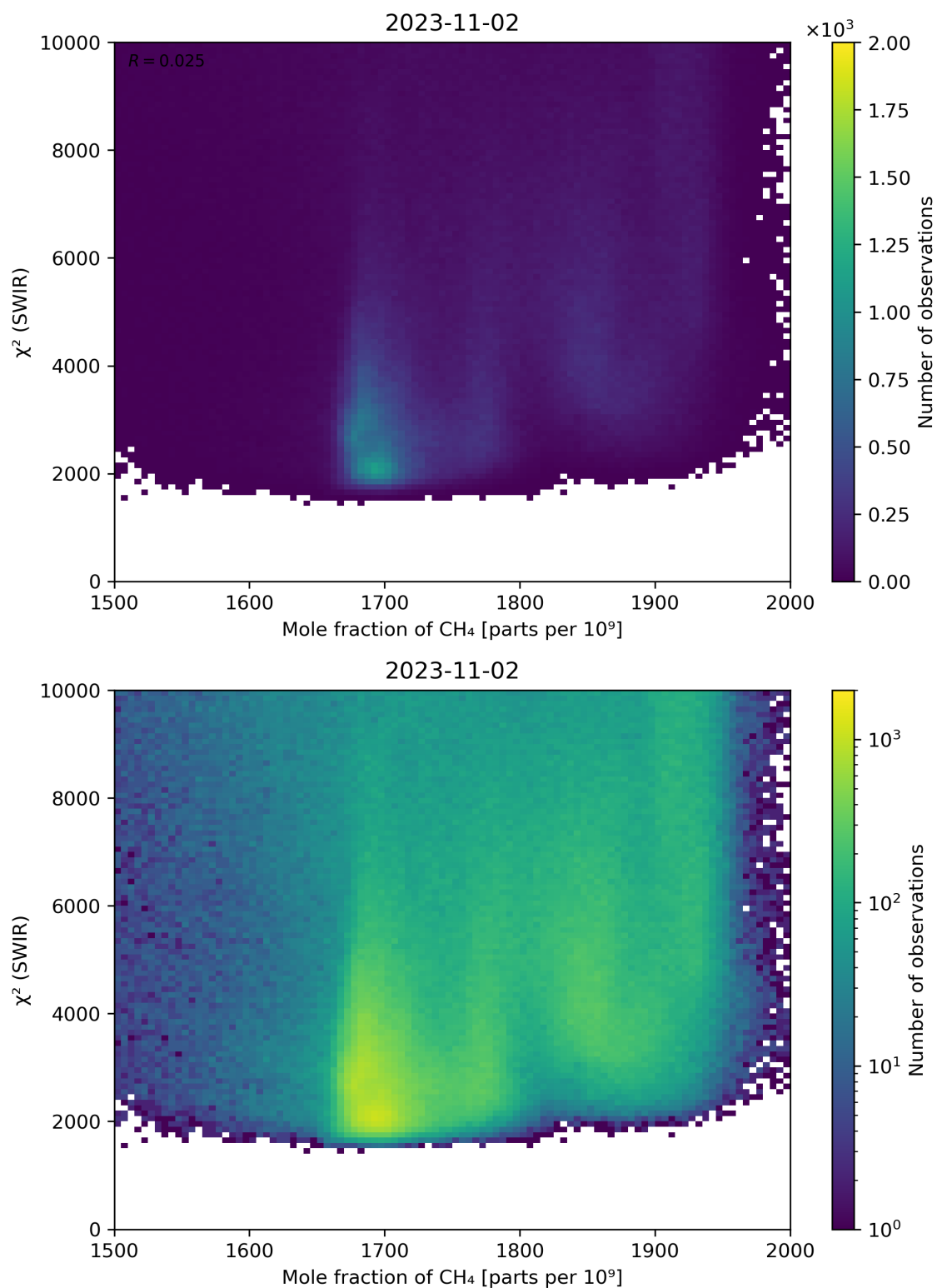
Figure 71: Scatter density plot of “Mole fraction of \text{CH}_4 ” against “ \chi^2 (SWIR)” for 2023-11-02 to 2023-11-03.
