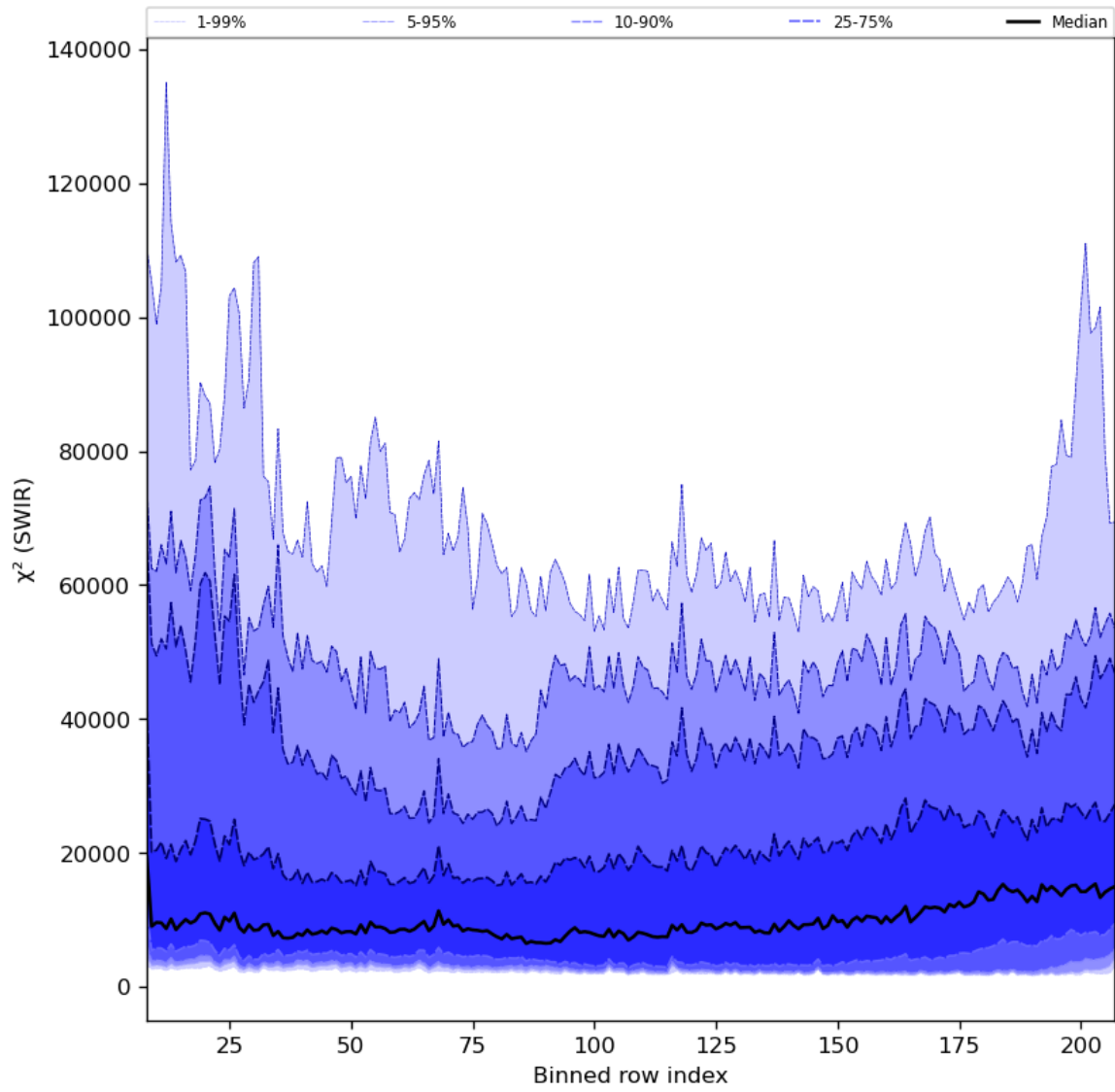
Figure 39: Along track statistics of “ \chi^2 (SWIR)” for 2023-11-02 to 2023-11-03
