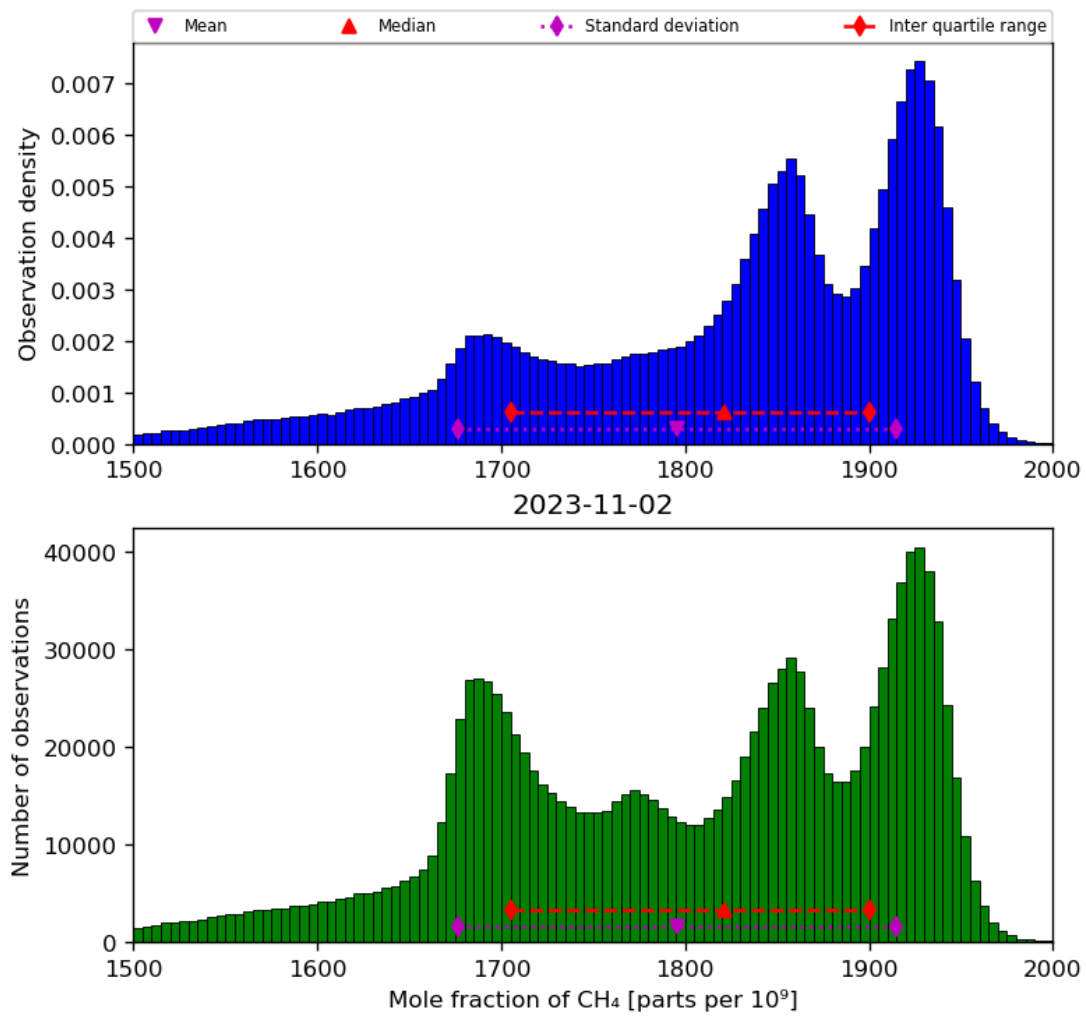
Figure 23: Histogram of “Mole fraction of CH 4 ” for 2023-11-02 to 2023-11-03
