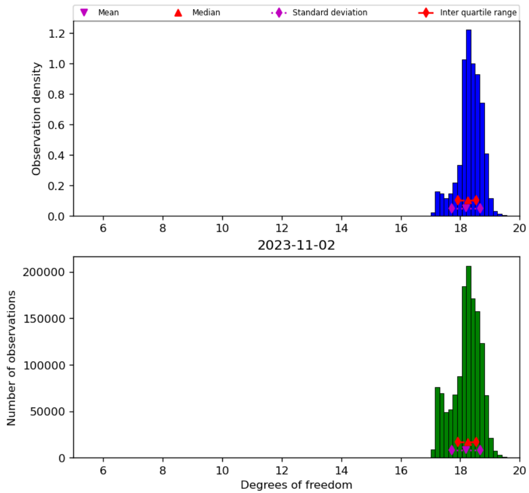
Figure 30: Histogram of “Degrees of freedom” for 2023-11-02 to 2023-11-03
