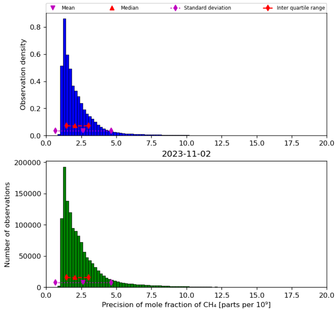
Figure 24: Histogram of “Precision of mole fraction of CH 4 ” for 2023-11-02 to 2023-11-03
