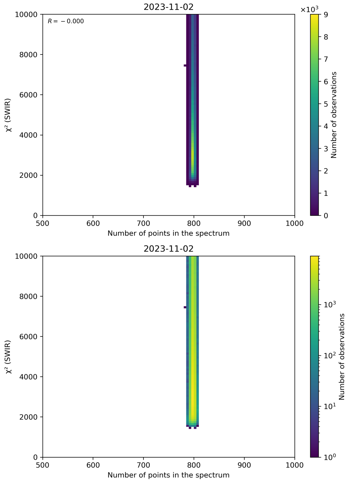
Figure 89: Scatter density plot of “Number of points in the spectrum” against “ \chi^2 (SWIR)” for 2023-11-02 to 2023-11-03.
