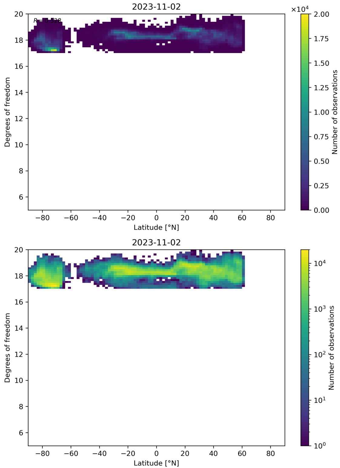
Figure 55: Scatter density plot of “Latitude” against “Degrees of freedom” for 2023-11-02 to 2023-11-03.
