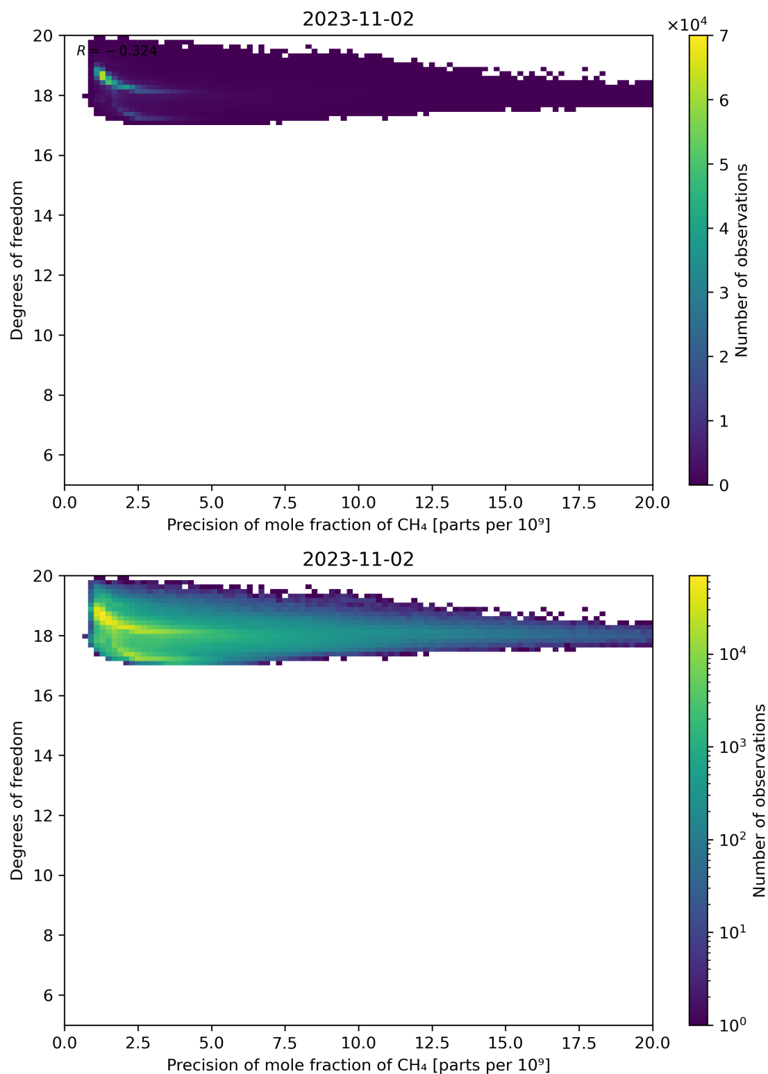
Figure 80: Scatter density plot of “Precision of mole fraction of CH 4 ” against “Degrees of freedom” for 2023-11-02 to 2023-11-03.
