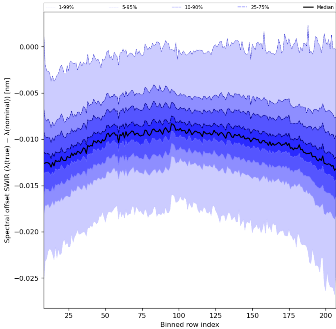
Figure 38: Along track statistics of “Spectral offset SWIR ( \lambda(\text{true}) - \lambda(\text{nominal}) )” for 2023-11-02 to 2023-11-03
