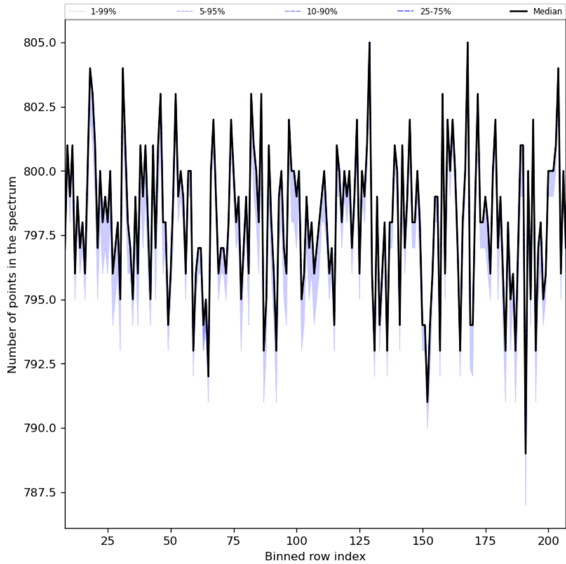
Figure 37: Along track statistics of “Number of points in the spectrum” for 2023-11-02 to 2023-11-03
