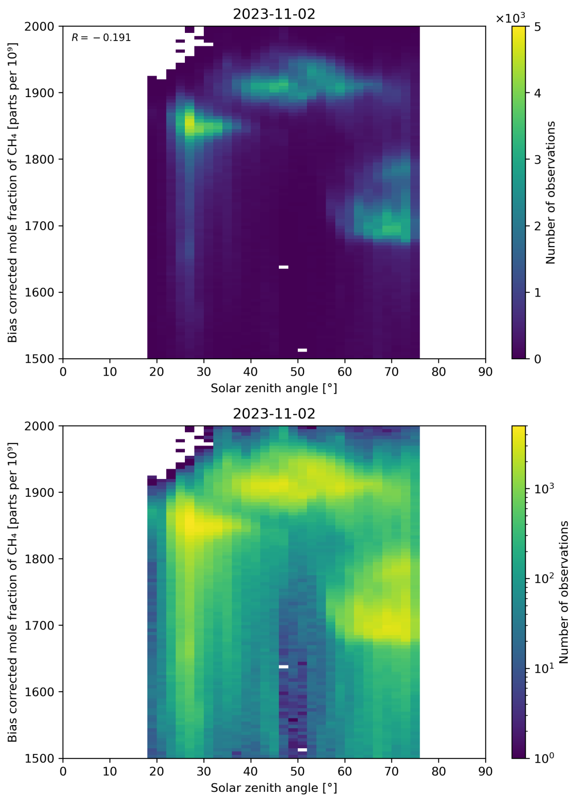
Figure 100: Scatter density plot of “Solar zenith angle” against “Bias corrected mole fraction of CH 4 ” for 2023-11-02 to 2023-11-03.
