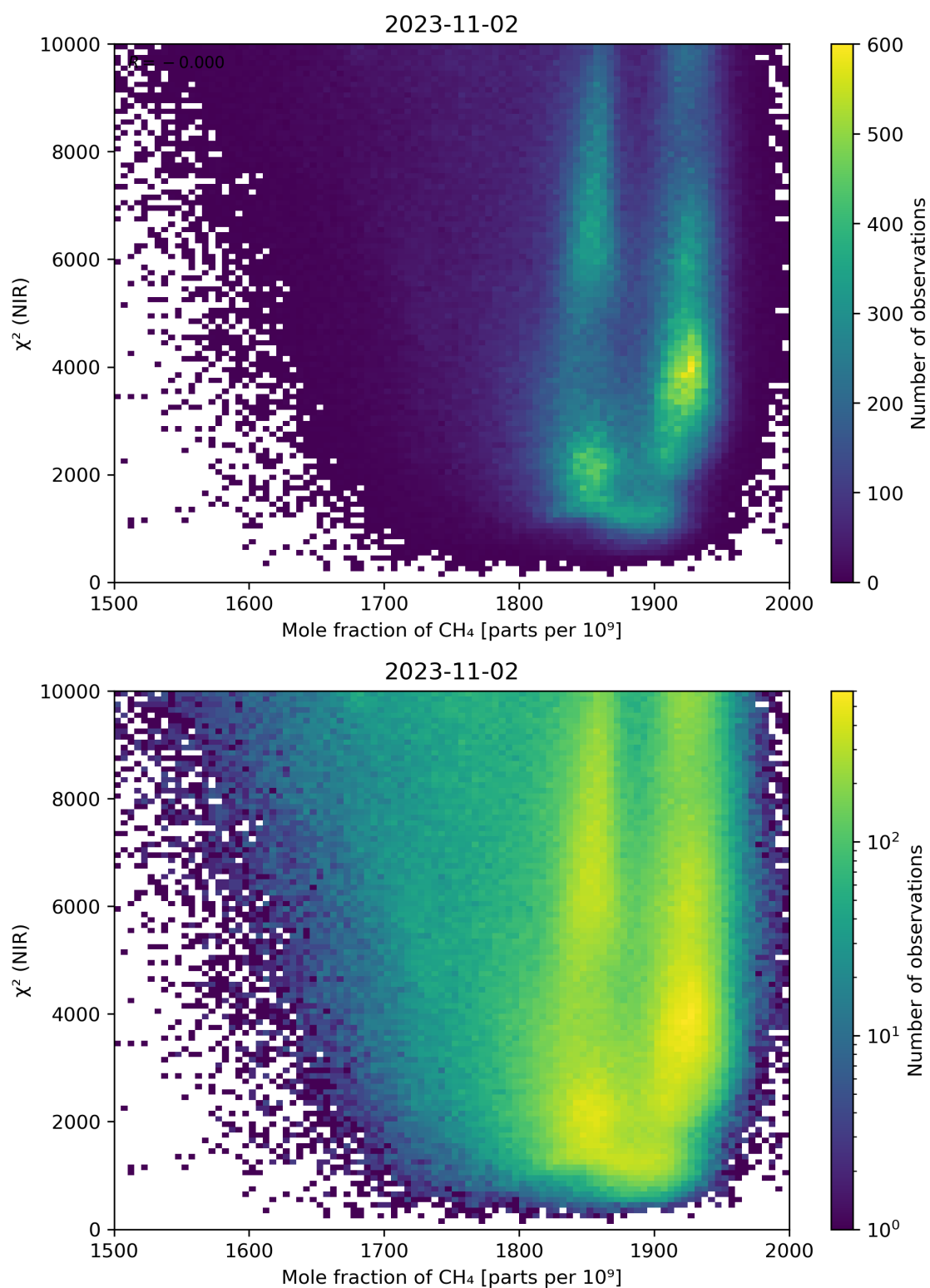
Figure 70: Scatter density plot of “Mole fraction of CH 4 ” against “ \chi^2 (NIR)” for 2023-11-02 to 2023-11-03.
