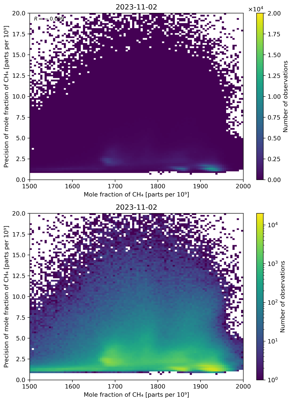
Figure 75: Scatter density plot of “Mole fraction of CH 4 ” against “Precision of mole fraction of CH 4 ” for 2023-11-02 to 2023-11-03.
