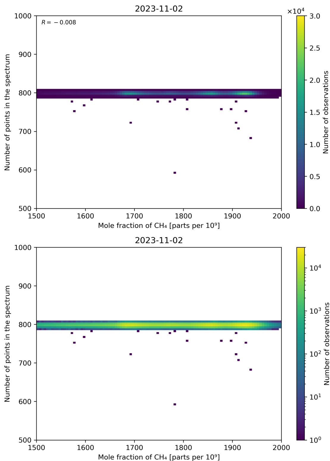
Figure 77: Scatter density plot of “Mole fraction of CH 4 ” against “Number of points in the spectrum” for 2023-11-02 to 2023-11-03.
