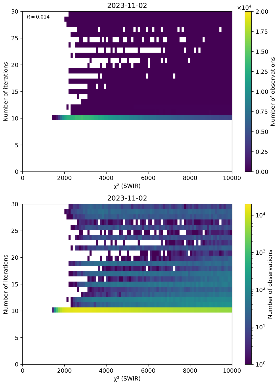
Figure 50: Scatter density plot of “ \chi^2 (SWIR)” against “Number of iterations” for 2023-11-02 to 2023-11-03.
