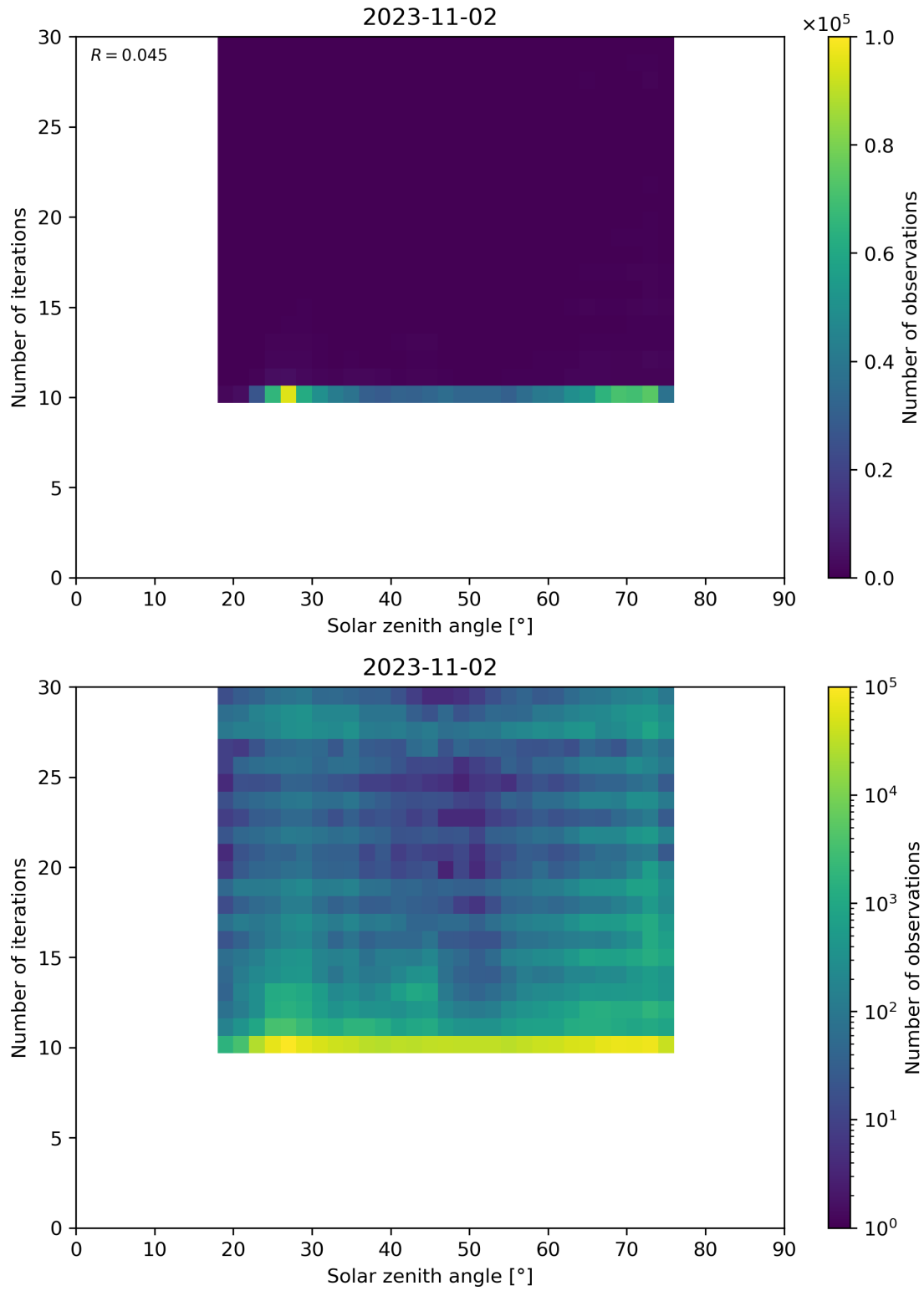
Figure 102: Scatter density plot of “Solar zenith angle” against “Number of iterations” for 2023-11-02 to 2023-11-03.
