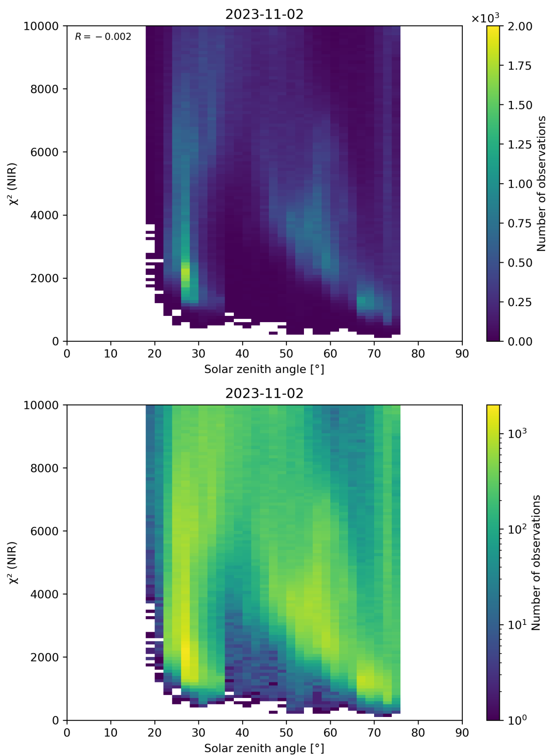
Figure 94: Scatter density plot of “Solar zenith angle” against “ \chi^2 (NIR)” for 2023-11-02 to 2023-11-03.
