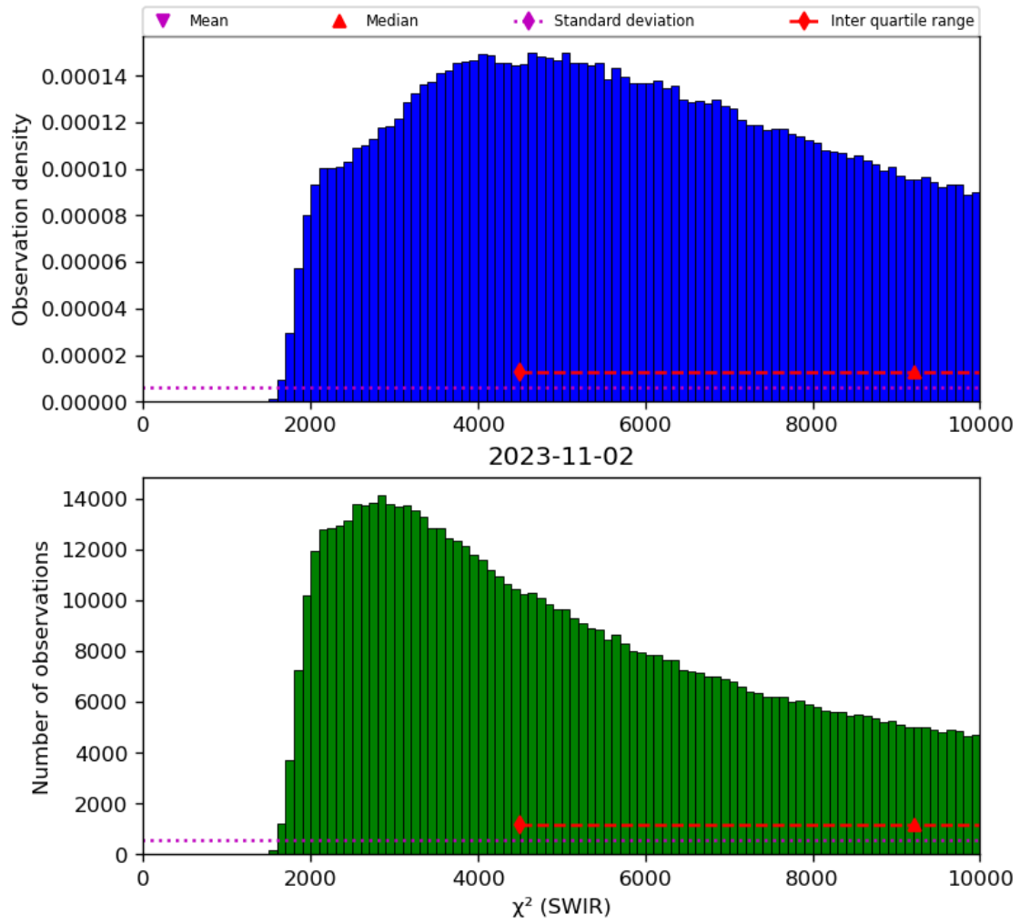
Figure 28: Histogram of “ \chi^2 (SWIR)” for 2023-11-02 to 2023-11-03
