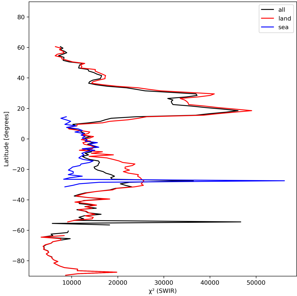
Figure 17: Zonal average of “ \chi^2 (SWIR)” for 2023-11-02 to 2023-11-03.
