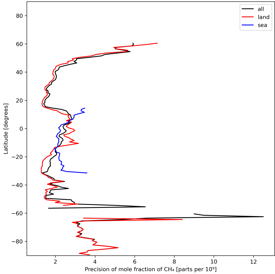
Figure 13: Zonal average of “Precision of mole fraction of CH 4 ” for 2023-11-02 to 2023-11-03.
