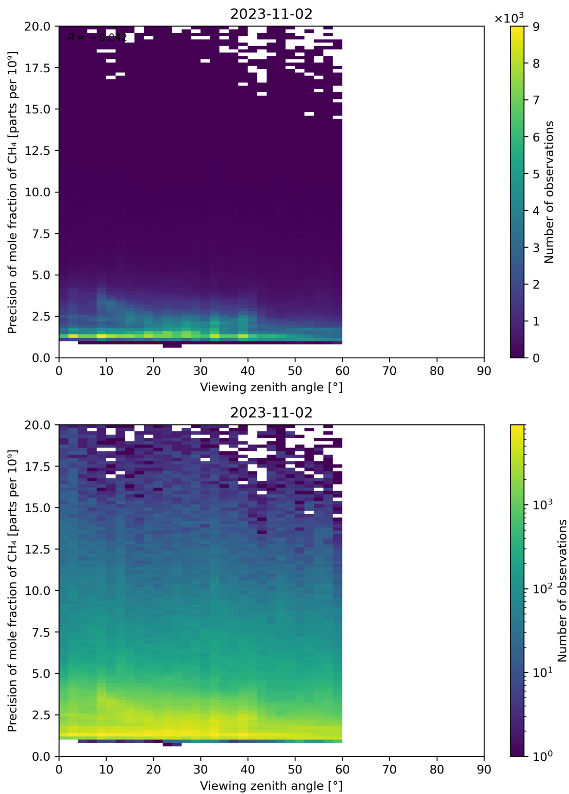
Figure 112: Scatter density plot of “Viewing zenith angle” against “Precision of mole fraction of CH 4 ” for 2023-11-02 to 2023-11-03.
