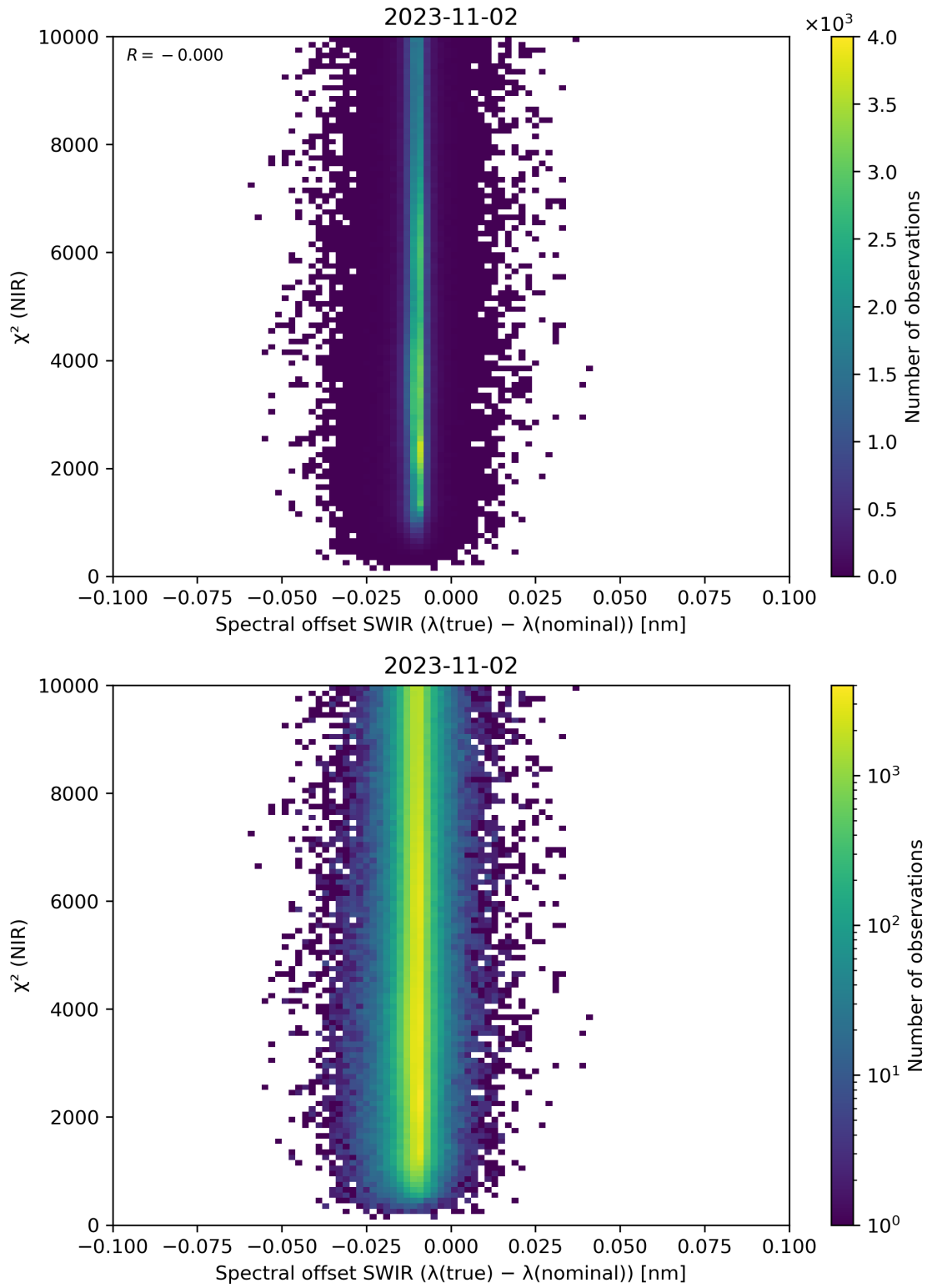
Figure 117: Scatter density plot of “Spectral offset SWIR ( \lambda(\text{true}) - \lambda(\text{nominal}) )” against “ \chi^2 (NIR)” for 2023-11-02 to 2023-11-03.
