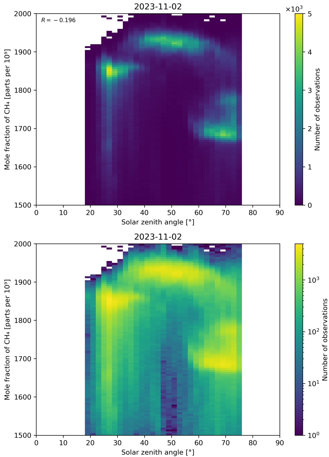
Figure 99: Scatter density plot of “Solar zenith angle” against “Mole fraction of CH 4 ” for 2023-11-02 to 2023-11-03.
