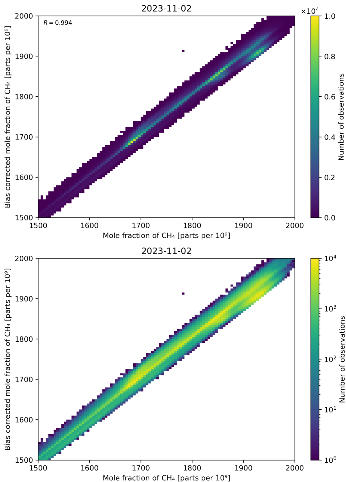
Figure 74: Scatter density plot of “Mole fraction of CH 4 ” against “Bias corrected mole fraction of CH 4 ” for 2023-11-02 to 2023-11-03.
