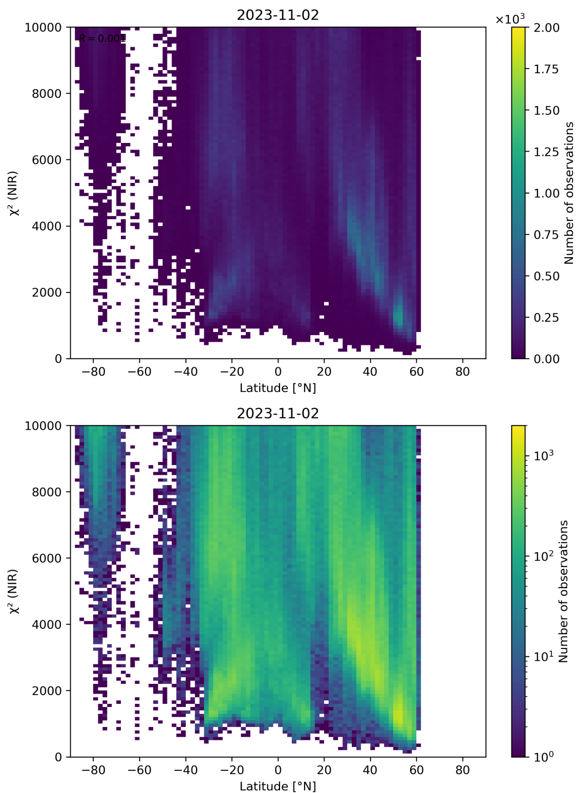
Figure 53: Scatter density plot of “Latitude” against “ \chi^2 (NIR)” for 2023-11-02 to 2023-11-03.
