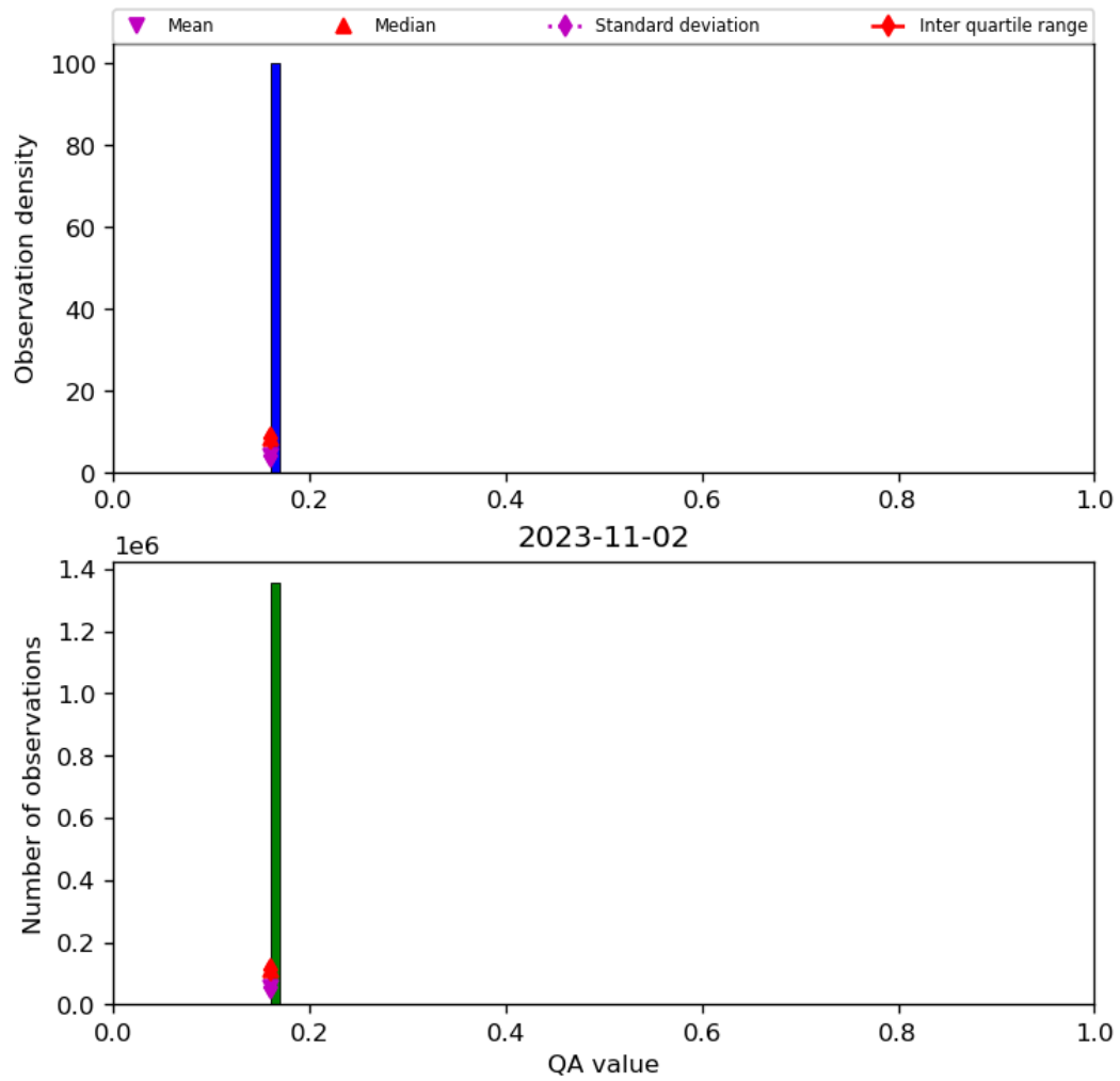
Figure 22: Histogram of “QA value” for 2023-11-02 to 2023-11-03
