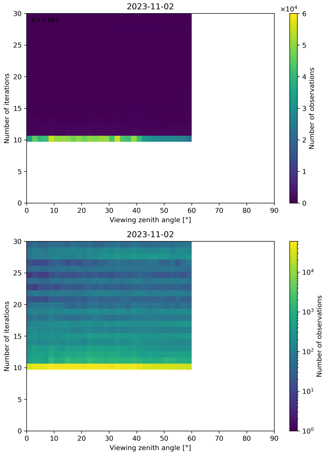
Figure 113: Scatter density plot of “Viewing zenith angle” against “Number of iterations” for 2023-11-02 to 2023-11-03.
