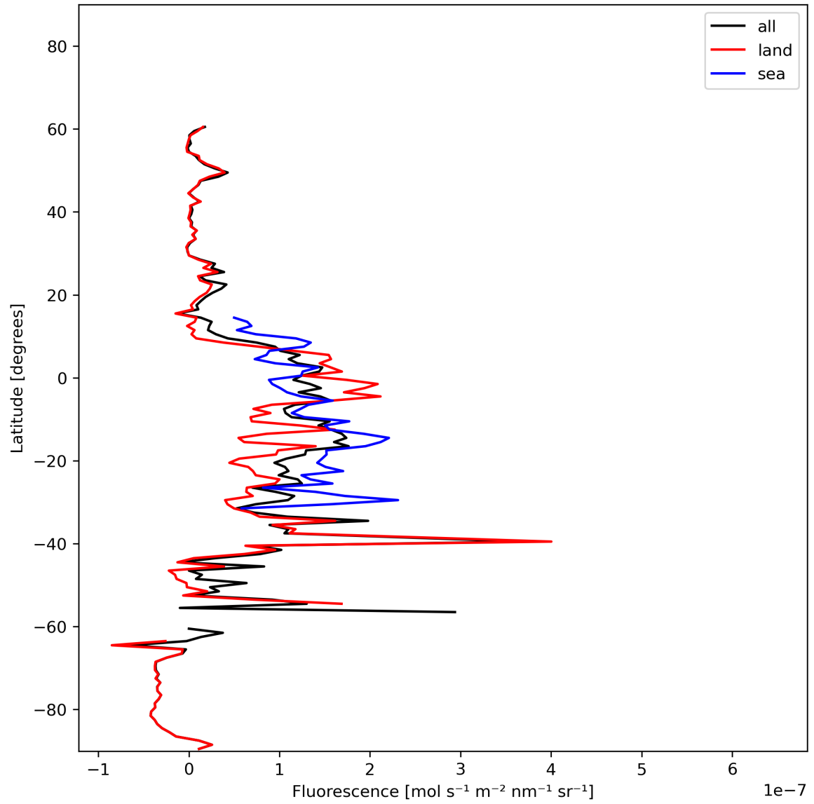
Figure 21: Zonal average of “Fluorescence” for 2023-11-02 to 2023-11-03.
