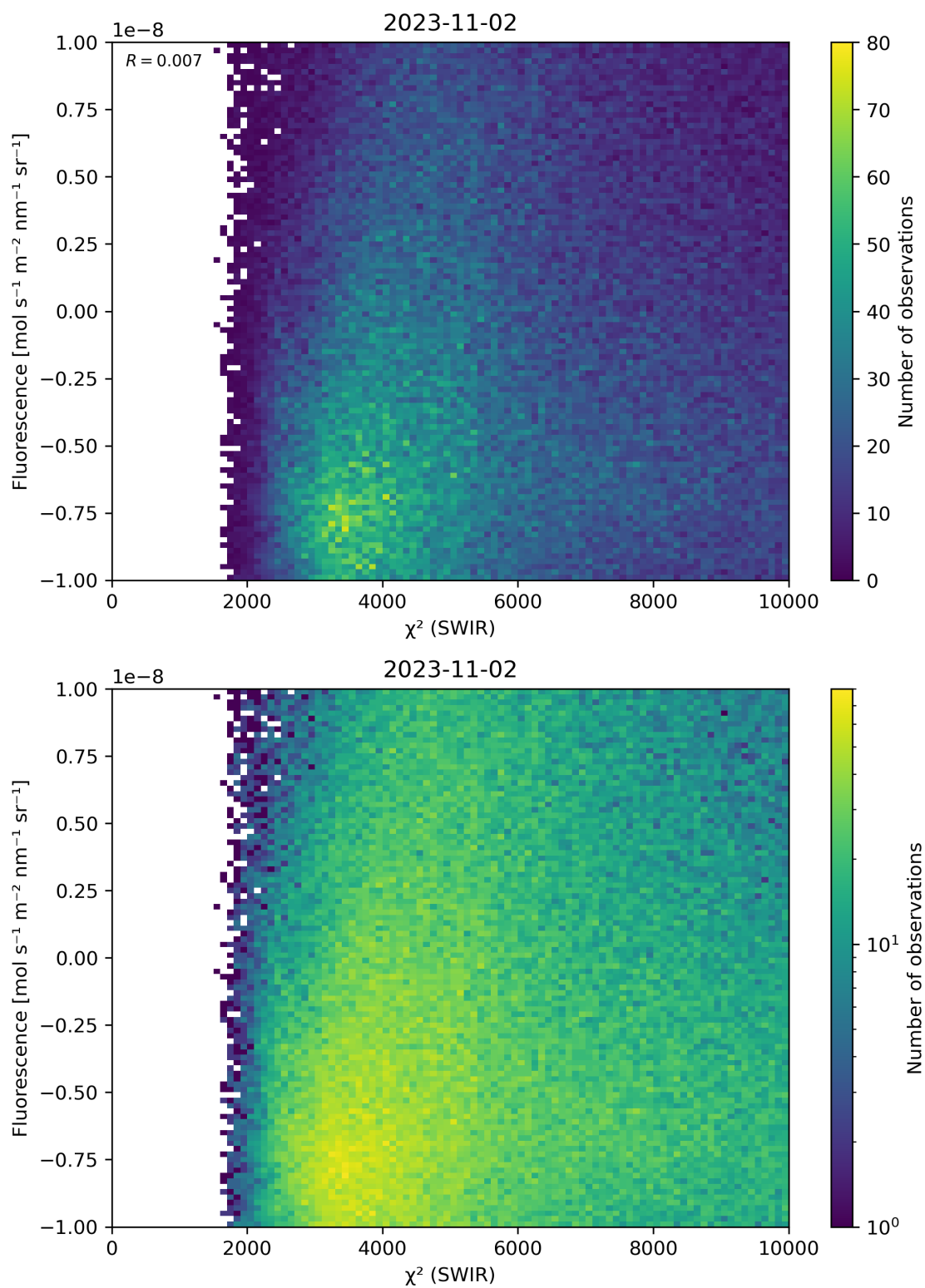
Figure 49: Scatter density plot of “ \chi^2 (SWIR)” against “Fluorescence” for 2023-11-02 to 2023-11-03.
