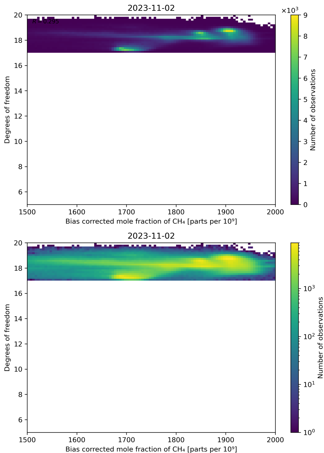
Figure 65: Scatter density plot of “Bias corrected mole fraction of CH 4 ” against “Degrees of freedom” for 2023-11-02 to 2023-11-03.
