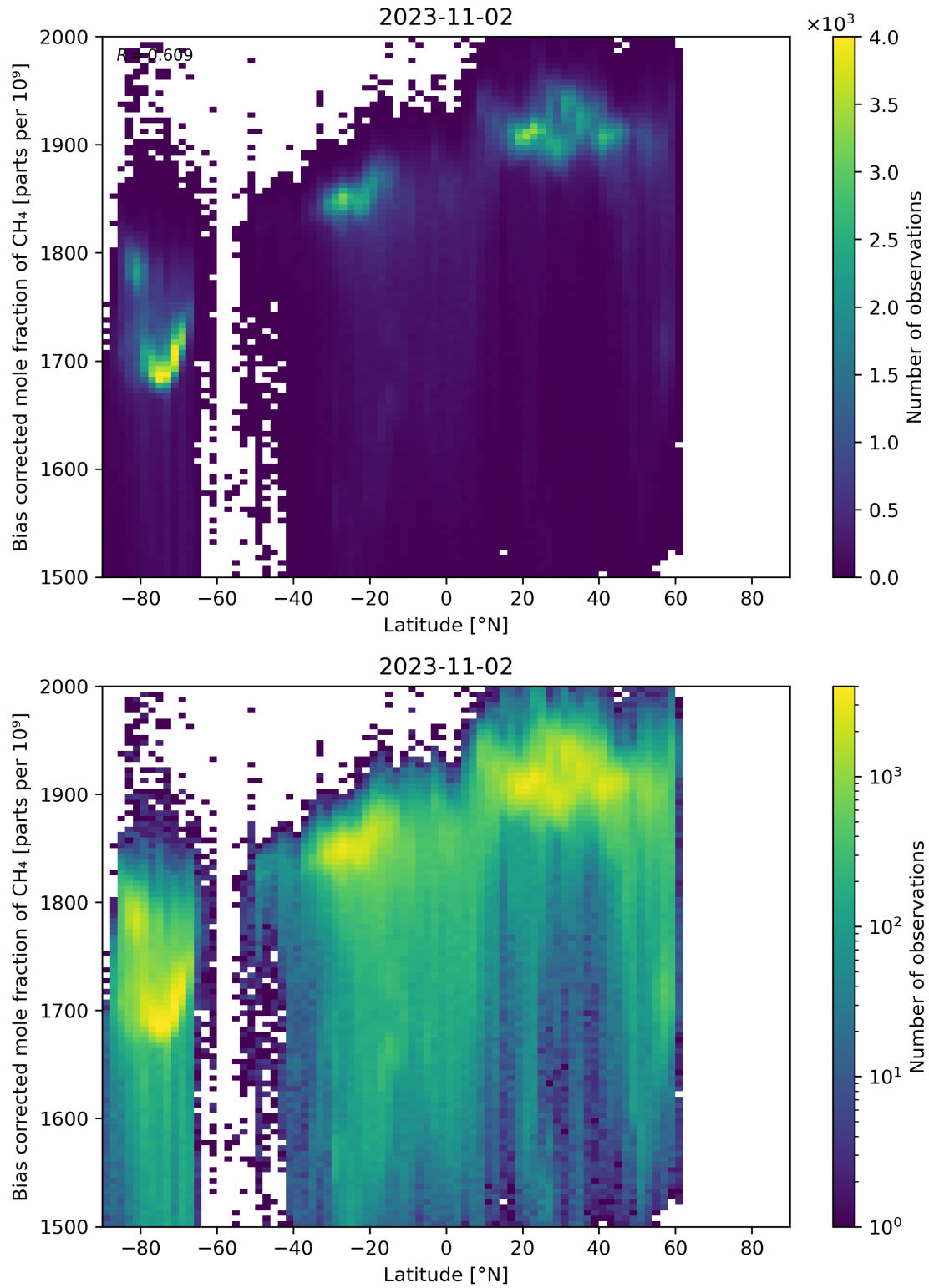
Figure 58: Scatter density plot of “Latitude” against “Bias corrected mole fraction of CH 4 ” for 2023-11-02 to 2023-11-03.
