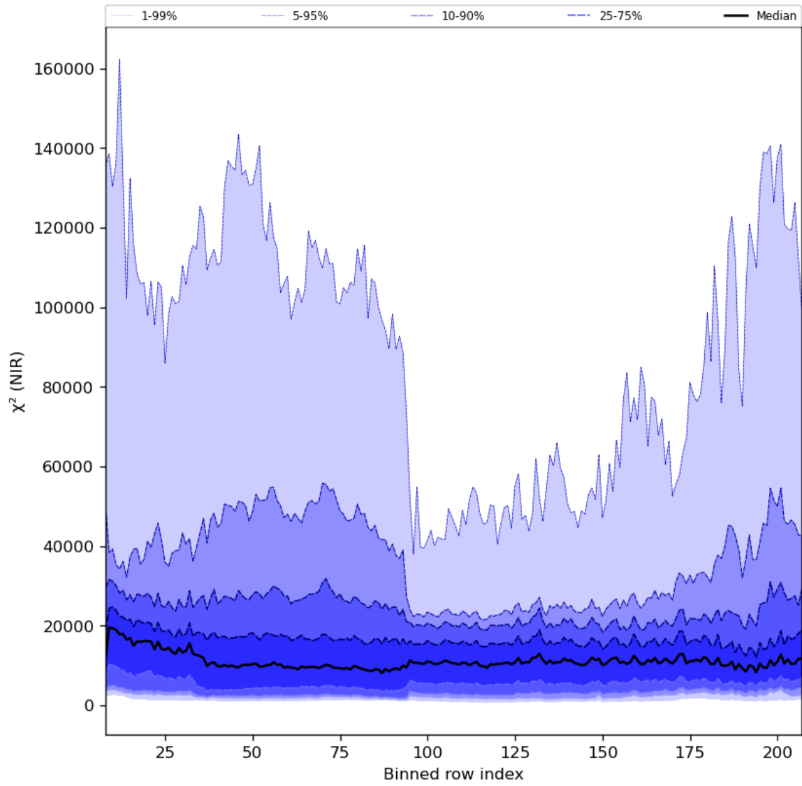
Figure 40: Along track statistics of " \chi^2 (NIR)" for 2023-11-02 to 2023-11-03
