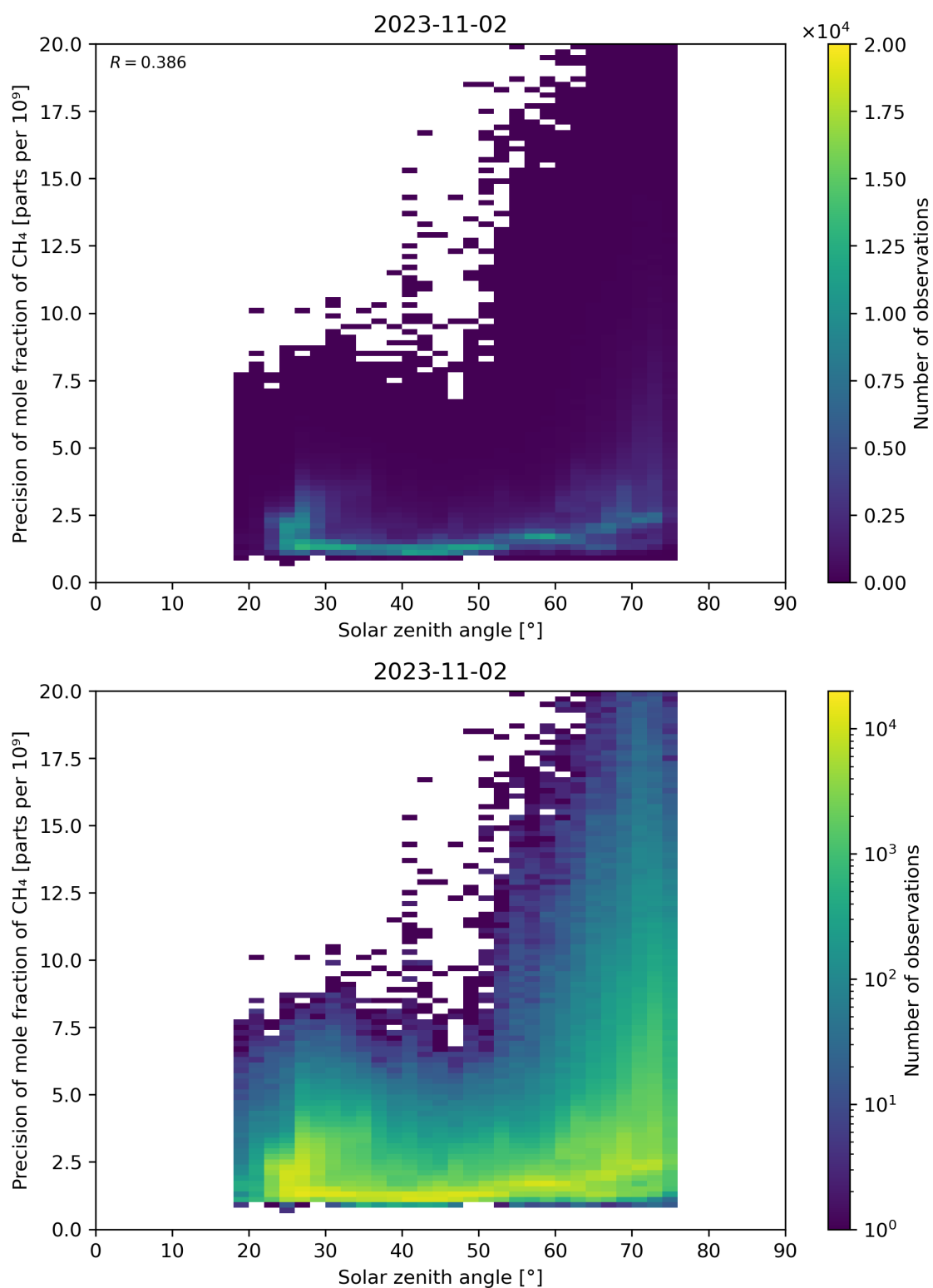
Figure 101: Scatter density plot of “Solar zenith angle” against “Precision of mole fraction of CH 4 ” for 2023-11-02 to 2023-11-03.
