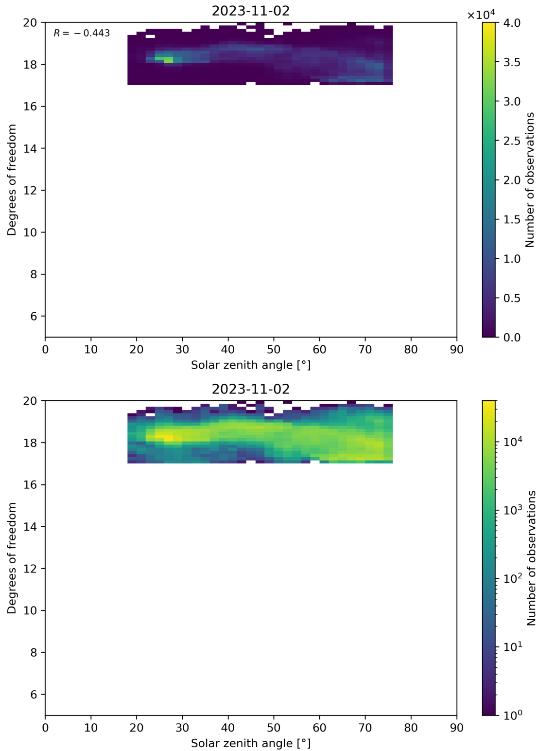
Figure 96: Scatter density plot of “Solar zenith angle” against “Degrees of freedom” for 2023-11-02 to 2023-11-03.
