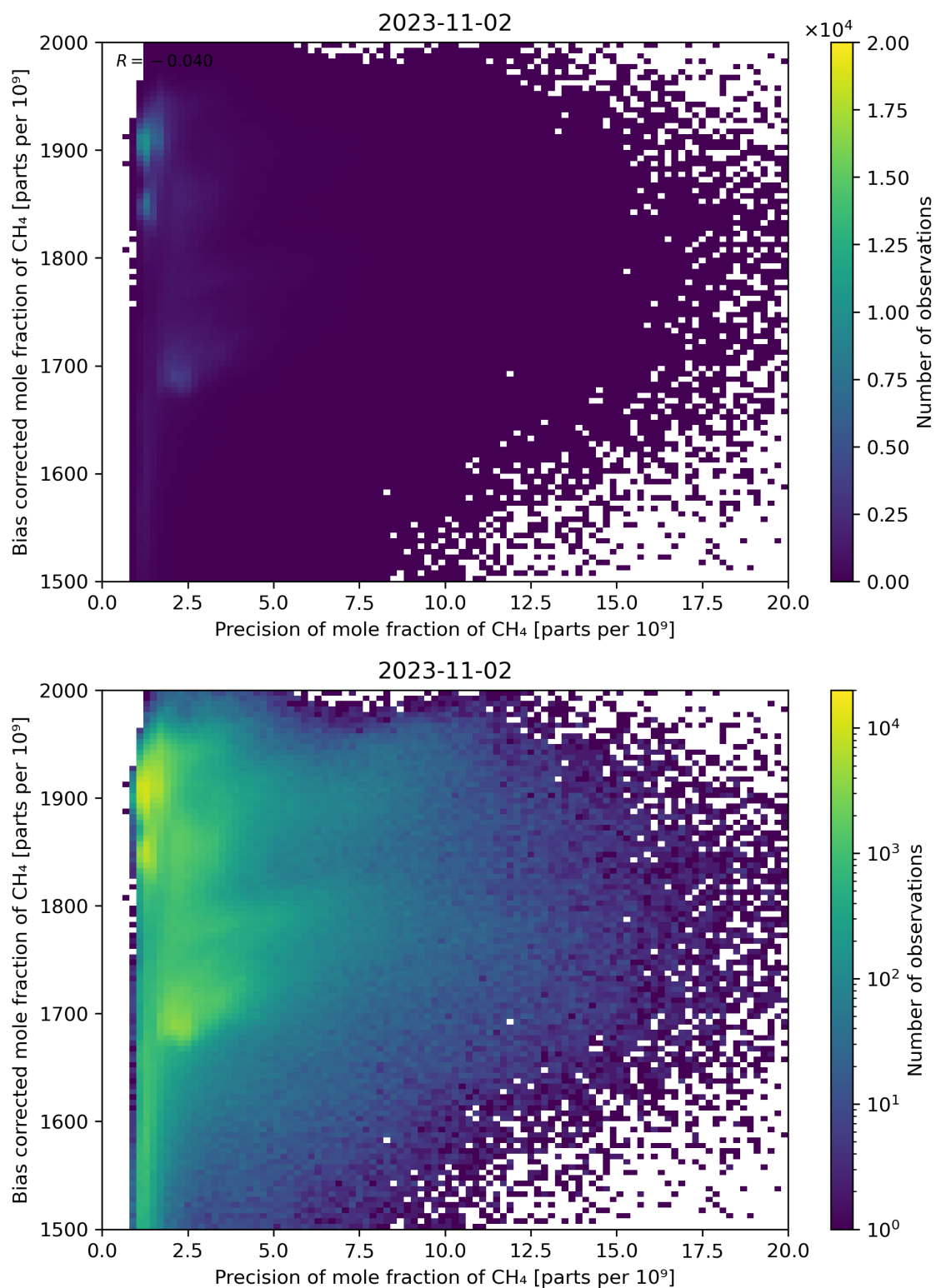
Figure 82: Scatter density plot of “Precision of mole fraction of CH 4 ” against “Bias corrected mole fraction of CH 4 ” for 2023-11-02 to 2023-11-03.
