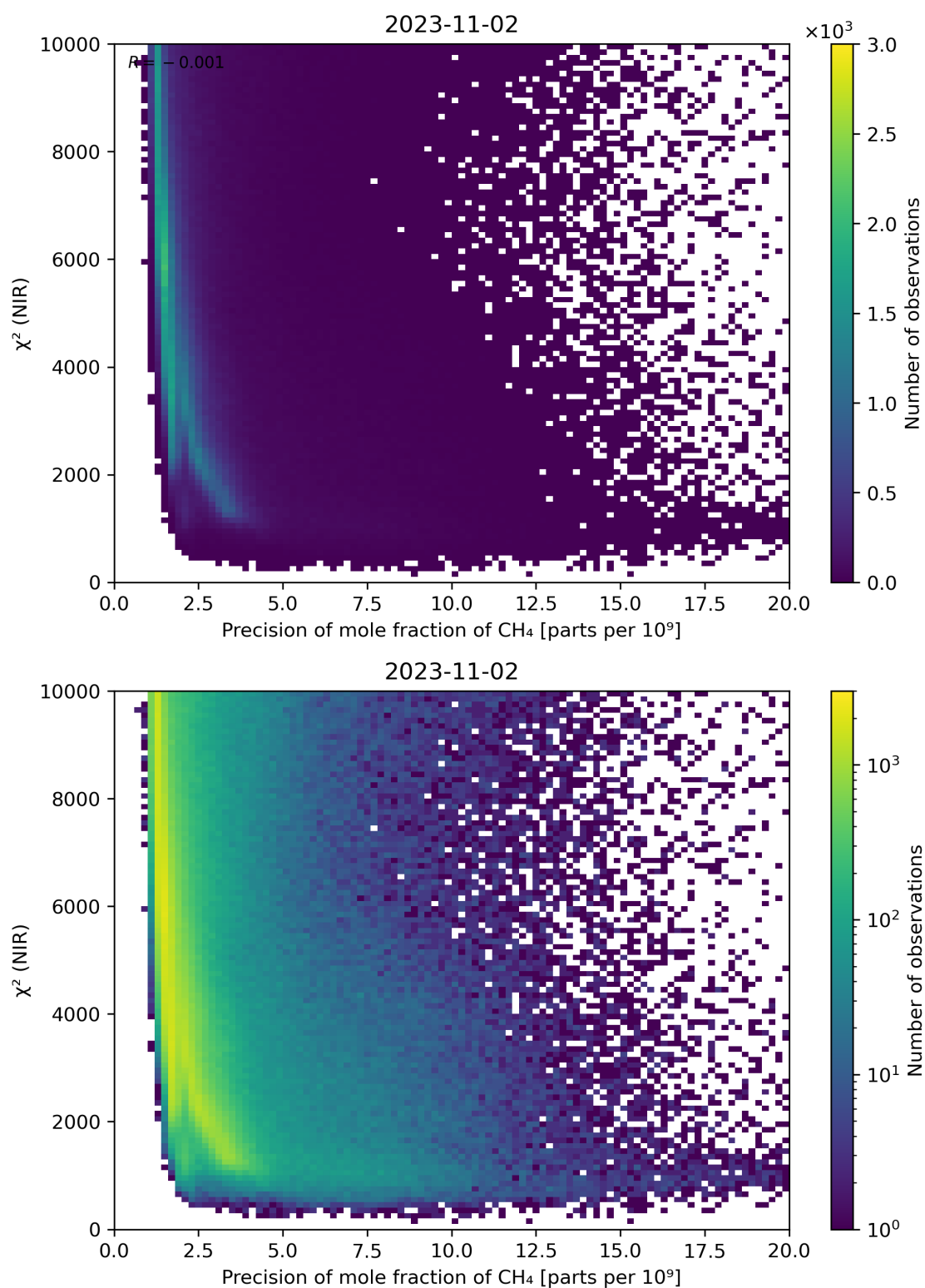
Figure 78: Scatter density plot of “Precision of mole fraction of CH 4 ” against “ \chi^2 (NIR)” for 2023-11-02 to 2023-11-03.
