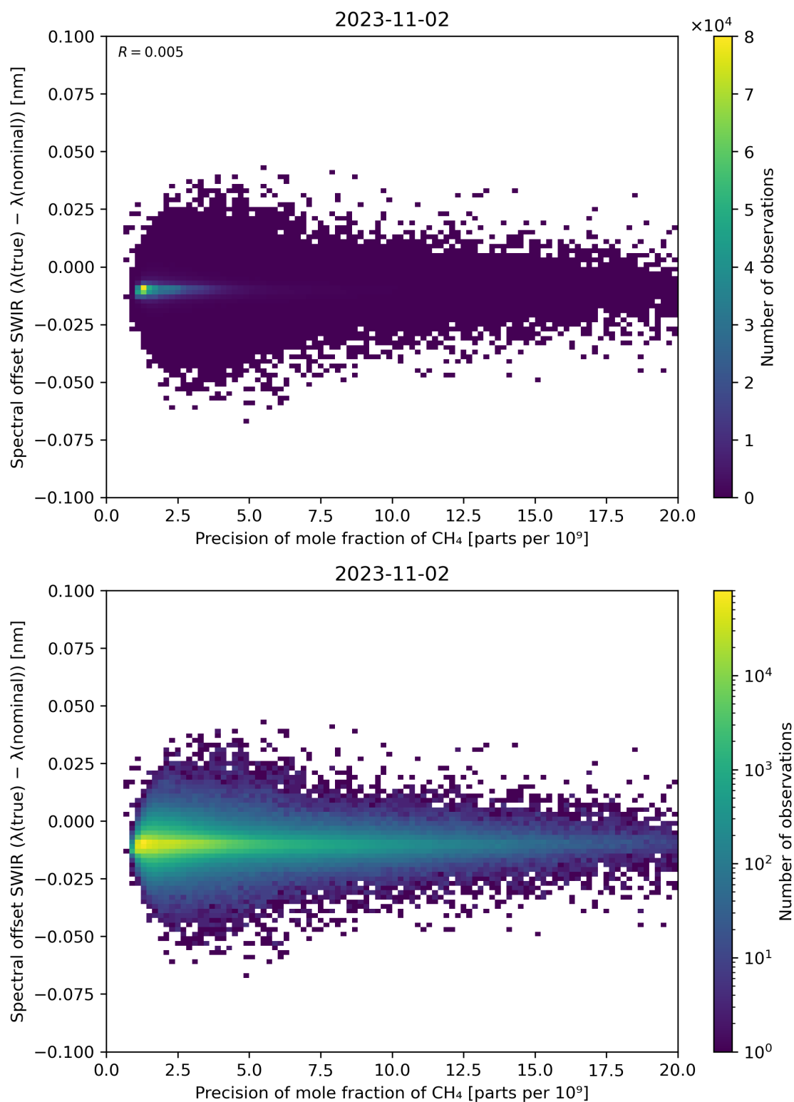
Figure 85: Scatter density plot of “Precision of mole fraction of CH 4 ” against “Spectral offset SWIR ( \lambda(\text{true}) - \lambda(\text{nominal}) )” for 2023-11-02 to 2023-11-03.
