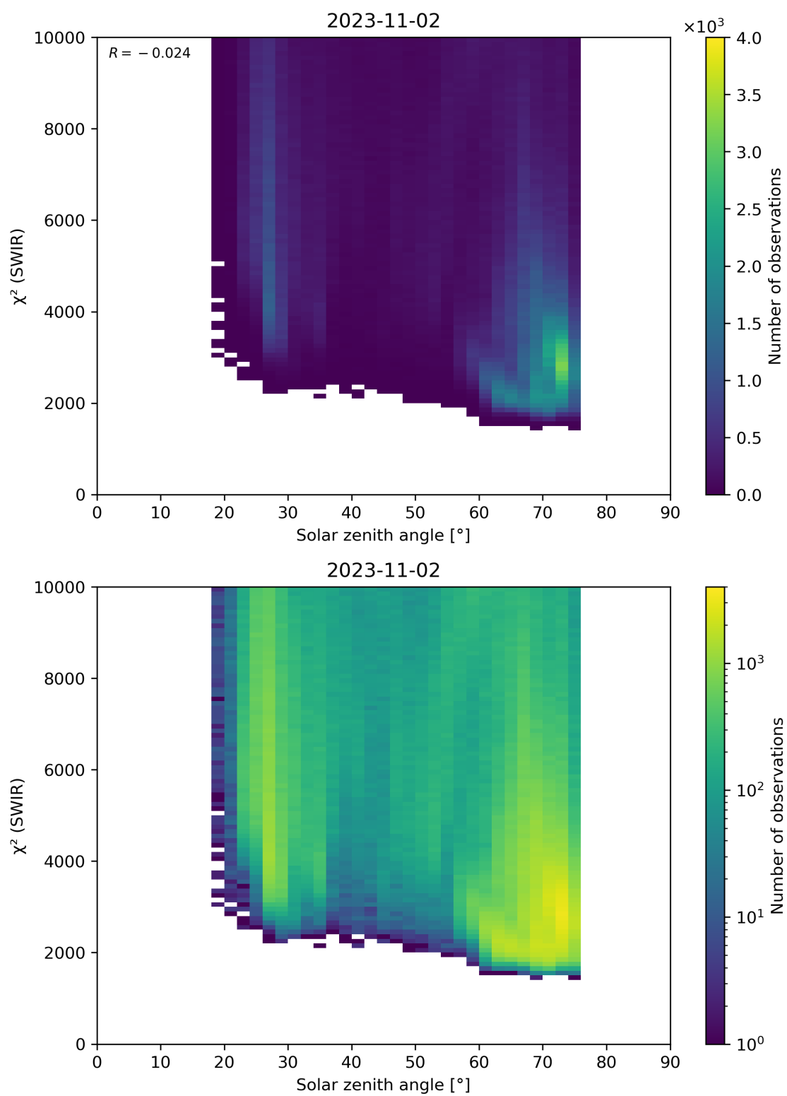
Figure 95: Scatter density plot of “Solar zenith angle” against “ \chi^2 (SWIR)” for 2023-11-02 to 2023-11-03.
