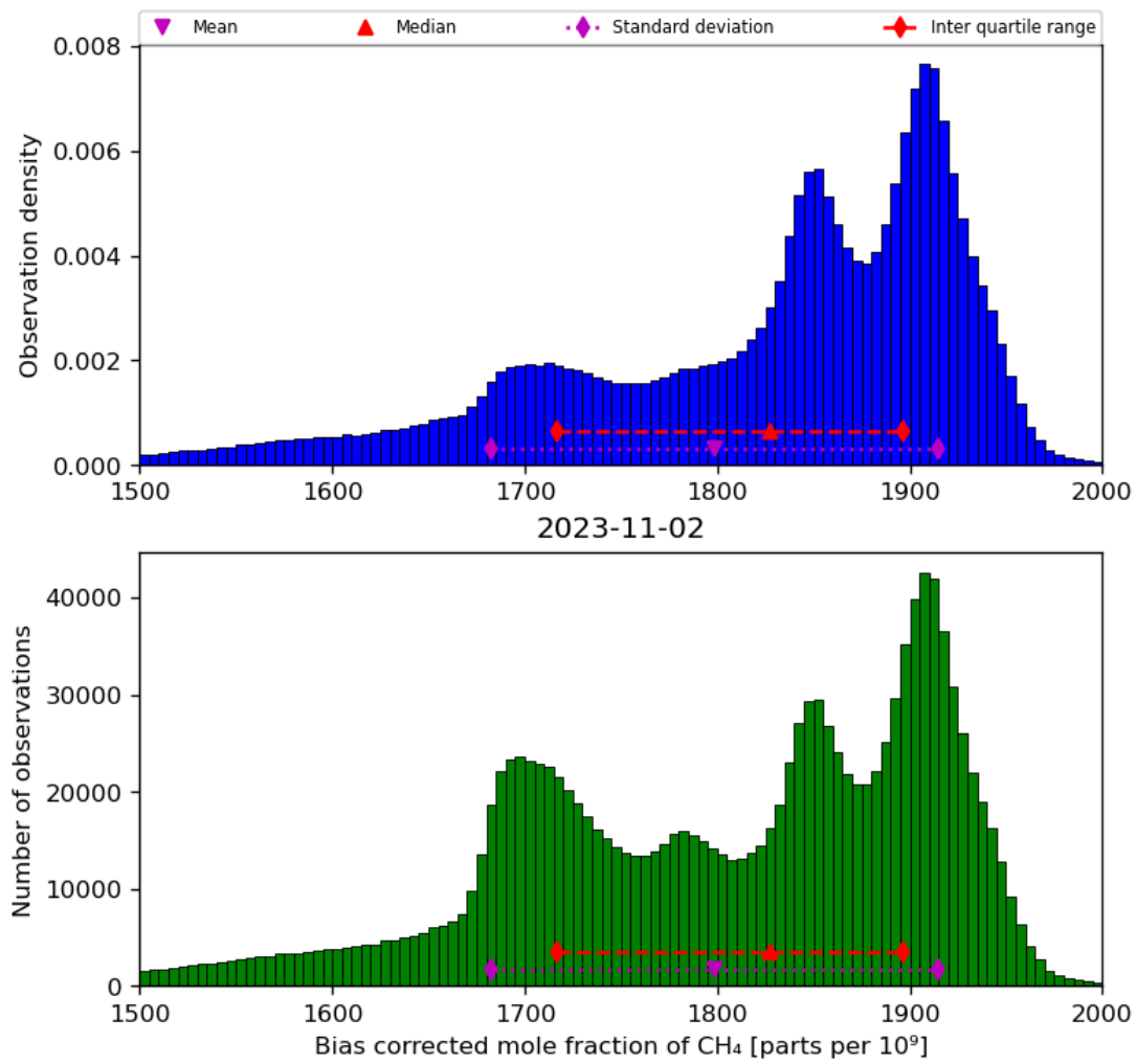
Figure 25: Histogram of “Bias corrected mole fraction of CH 4 ” for 2023-11-02 to 2023-11-03
