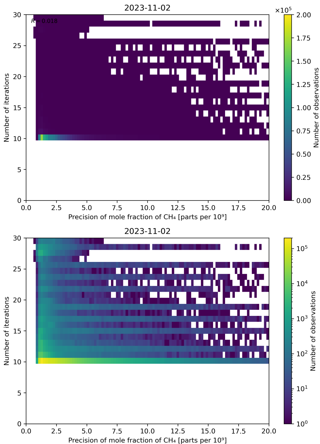
Figure 83: Scatter density plot of “Precision of mole fraction of CH 4 ” against “Number of iterations” for 2023-11-02 to 2023-11-03.
