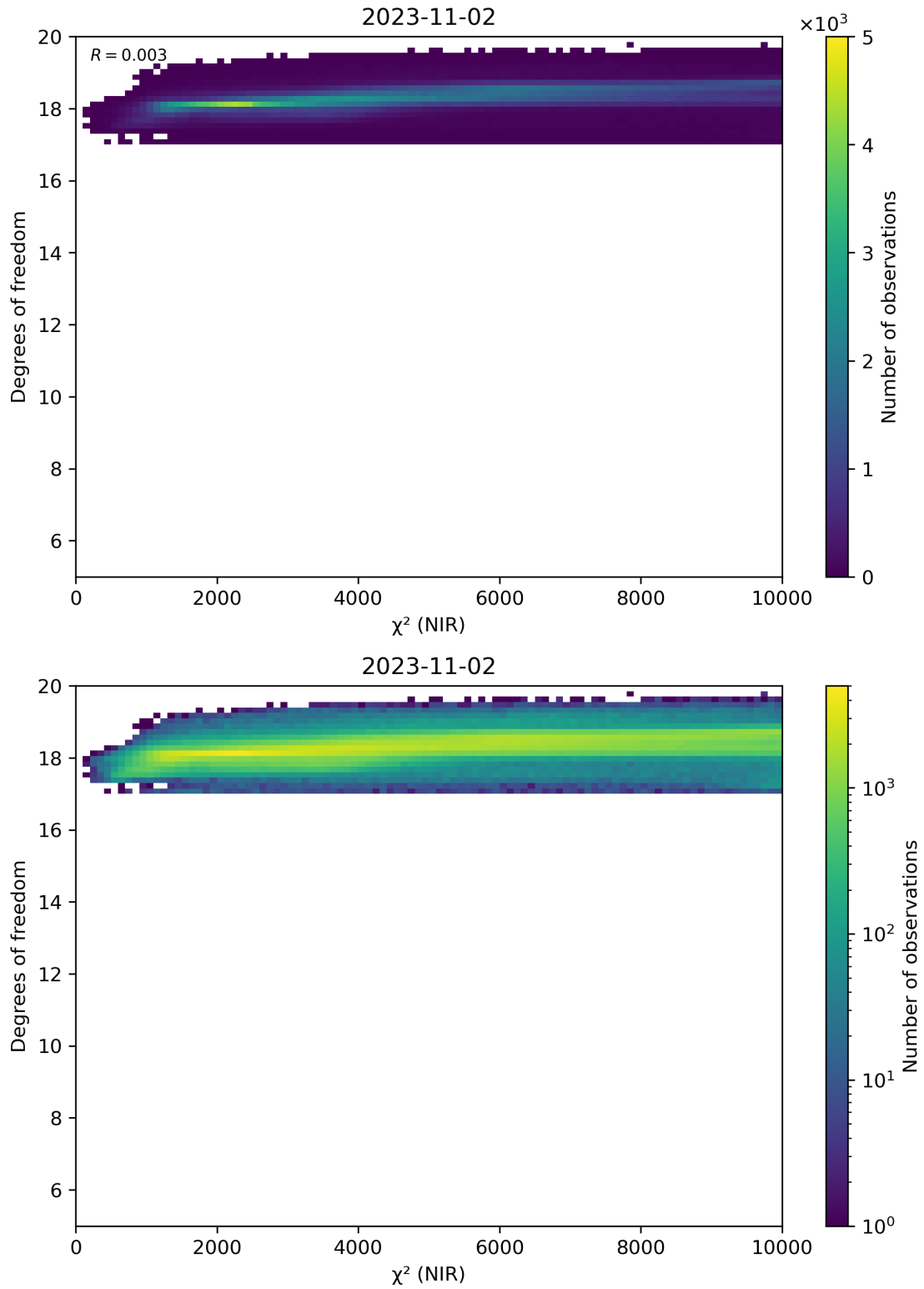
Figure 44: Scatter density plot of “ \chi^2 (NIR)” against “Degrees of freedom” for 2023-11-02 to 2023-11-03.
