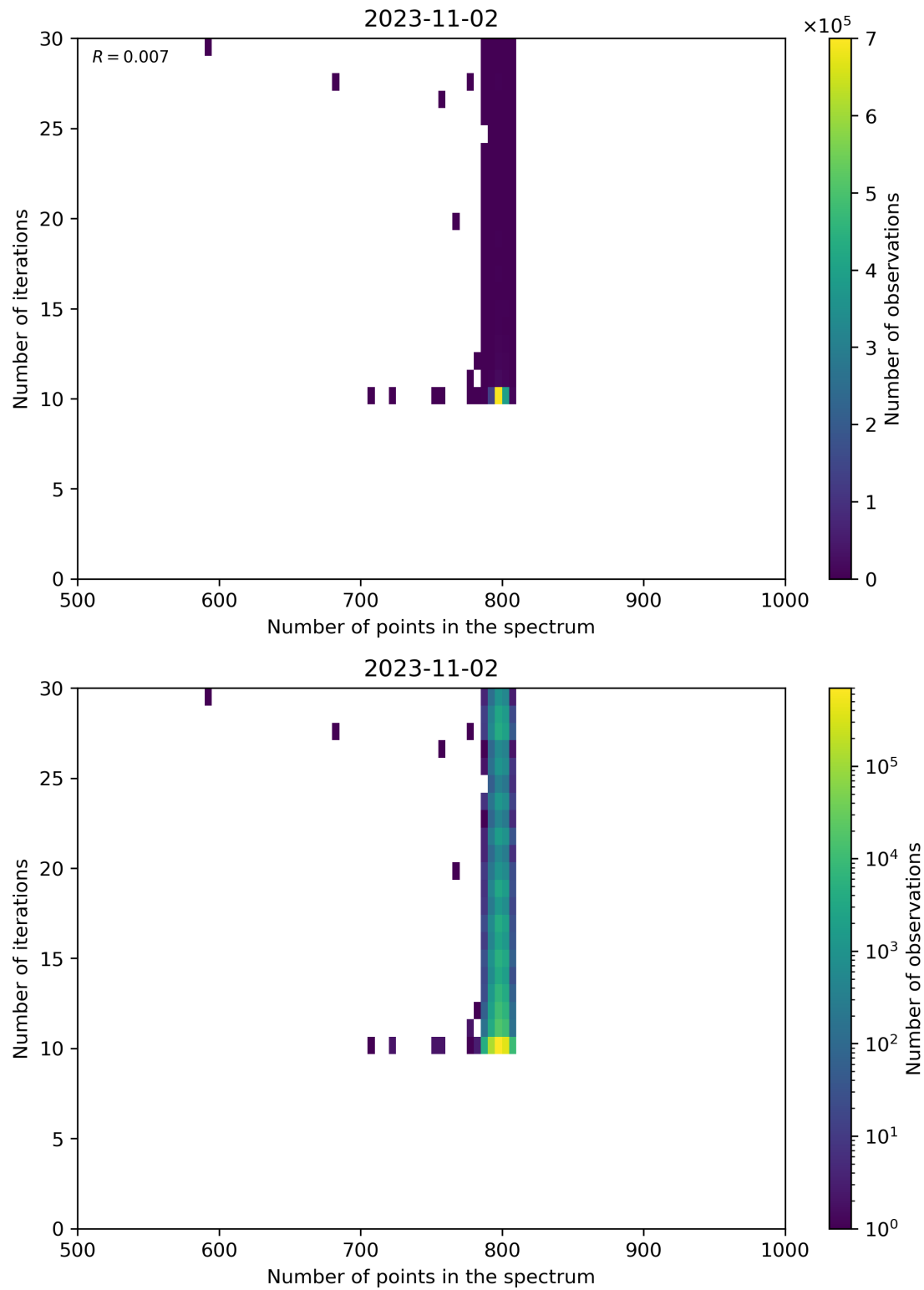
Figure 92: Scatter density plot of “Number of points in the spectrum” against “Number of iterations” for 2023-11-02 to 2023-11-03.
