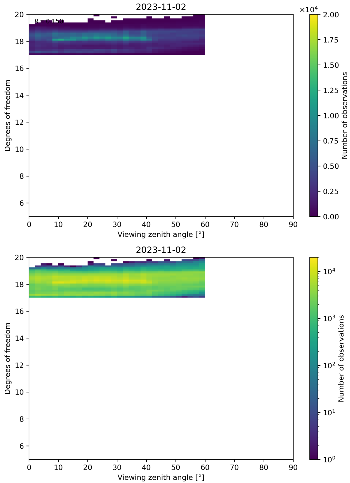
Figure 107: Scatter density plot of “Viewing zenith angle” against “Degrees of freedom” for 2023-11-02 to 2023-11-03.
