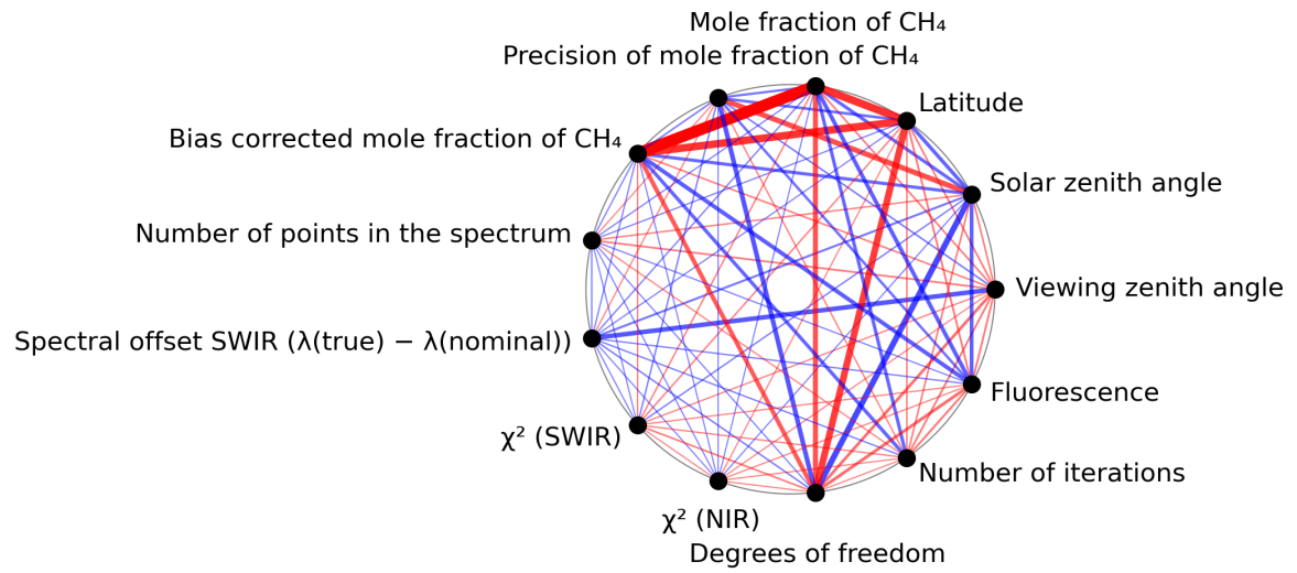
Figure 1: Map of correlation graph for 2023-11-02 to 2023-11-03.
