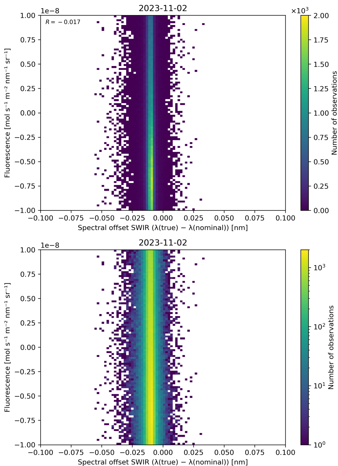
Figure 120: Scatter density plot of “Spectral offset SWIR ( \lambda(\text{true}) - \lambda(\text{nominal}) )” against “Fluorescence” for 2023-11-02 to 2023-11-03.
