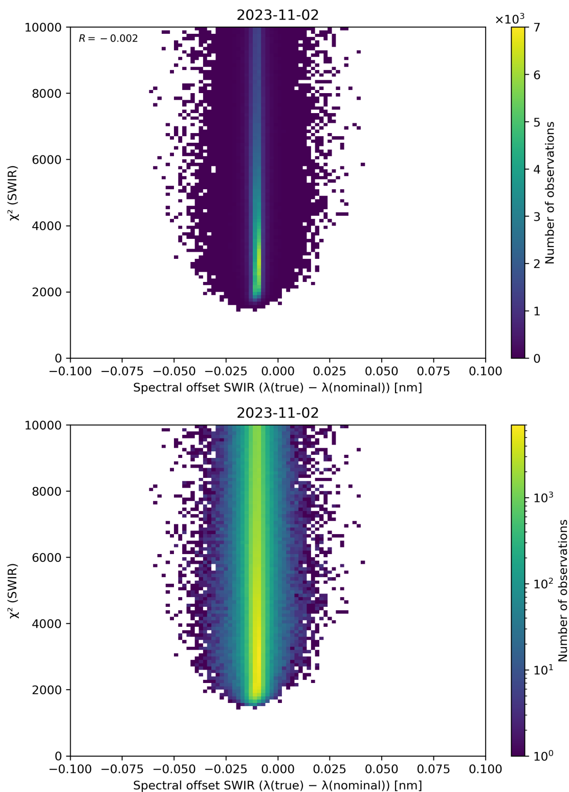
Figure 118: Scatter density plot of “Spectral offset SWIR ( \lambda(\text{true}) - \lambda(\text{nominal}) )” against “ \chi^2 (SWIR)” for 2023-11-02 to 2023-11-03.
