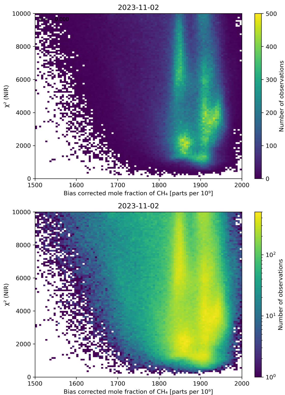
Figure 63: Scatter density plot of “Bias corrected mole fraction of CH 4 ” against “ \chi^2 (NIR)” for 2023-11-02 to 2023-11-03.
