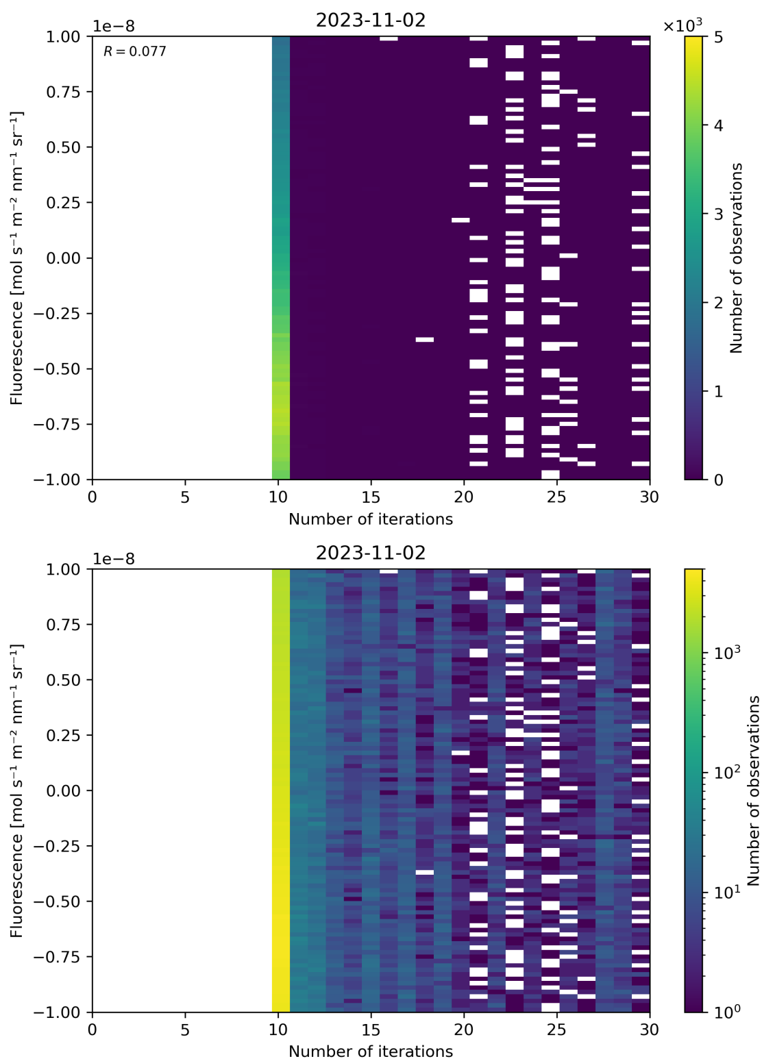
Figure 87: Scatter density plot of “Number of iterations” against “Fluorescence” for 2023-11-02 to 2023-11-03.
