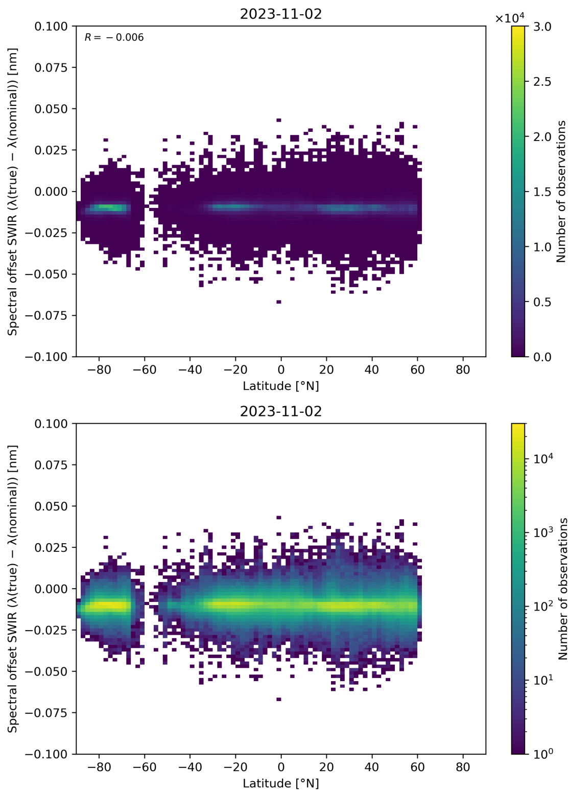
Figure 62: Scatter density plot of “Latitude” against “Spectral offset SWIR ( \lambda(\text{true}) - \lambda(\text{nominal}) )” for 2023-11-02 to 2023-11-03.
