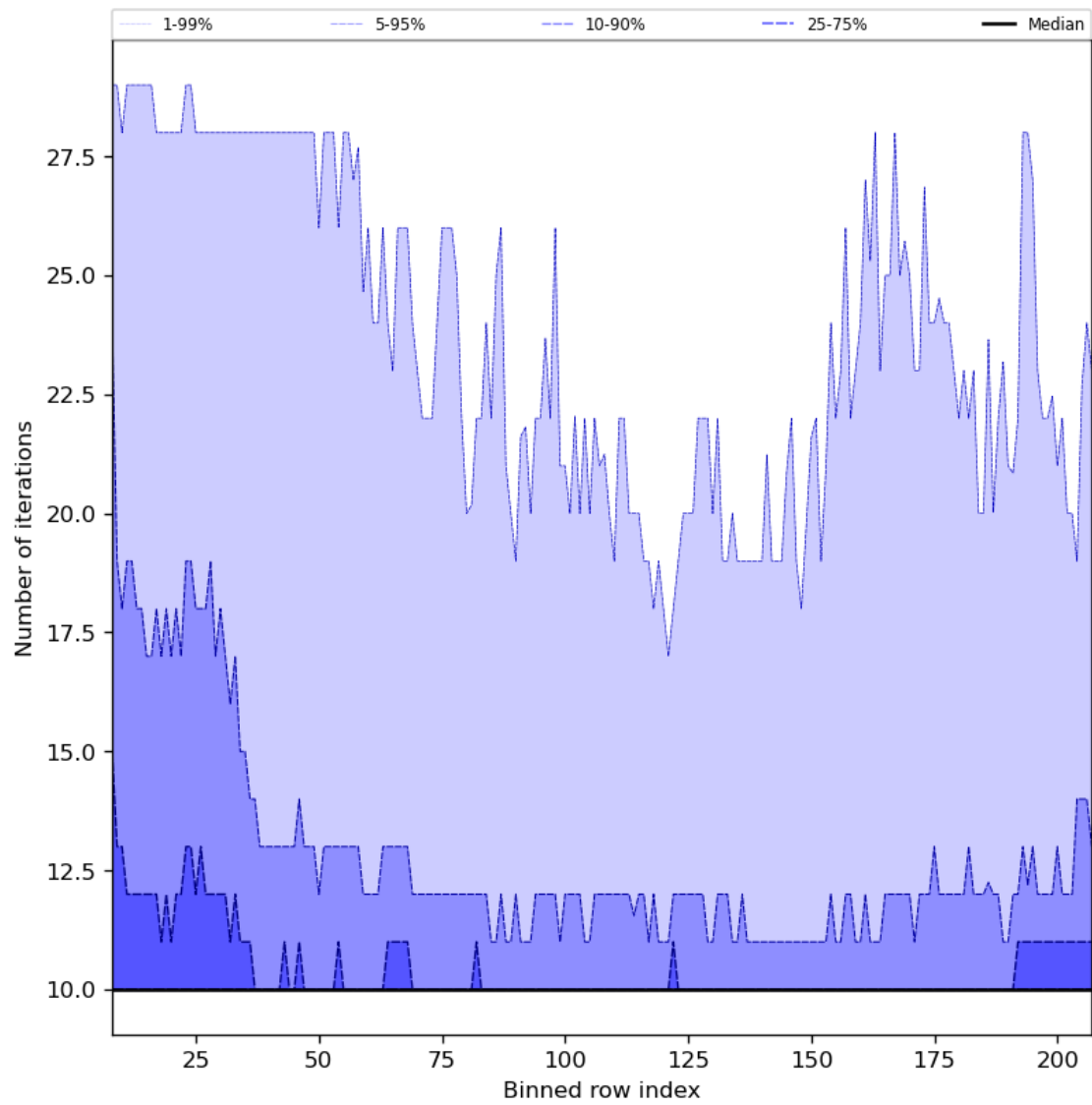
Figure 42: Along track statistics of “Number of iterations” for 2023-11-02 to 2023-11-03
