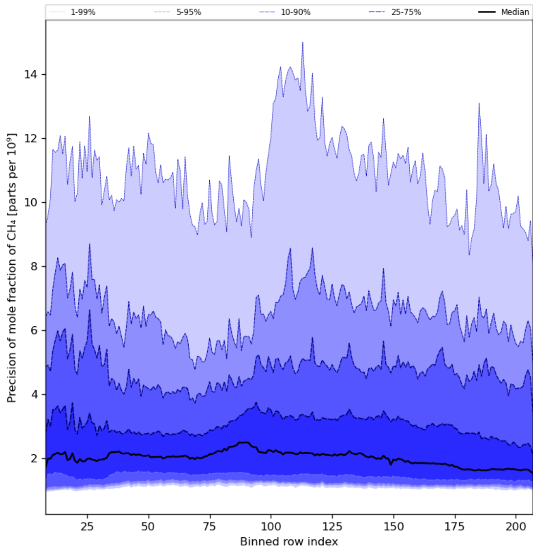
Figure 35: Along track statistics of “Precision of mole fraction of CH 4 ” for 2023-11-02 to 2023-11-03
