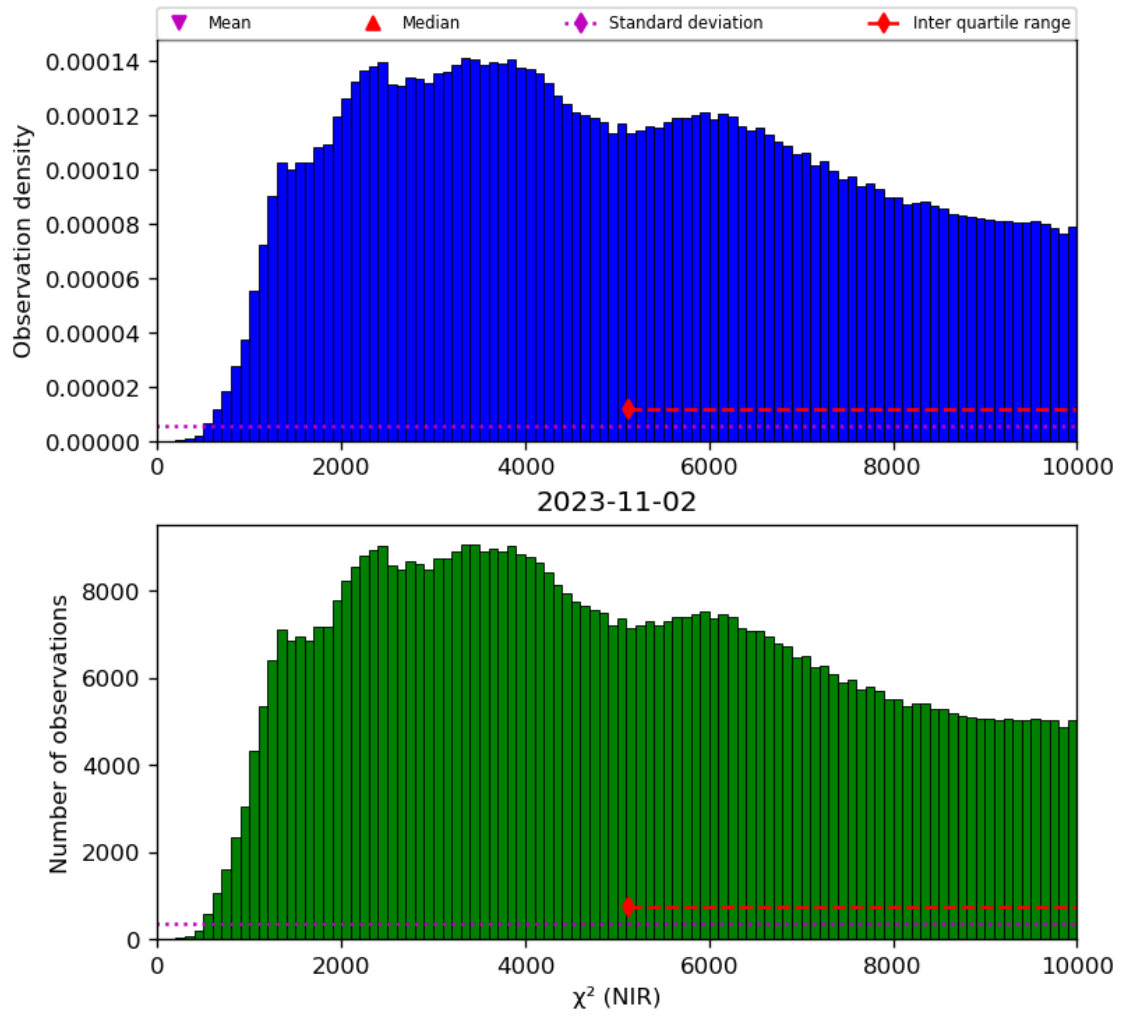
Figure 29: Histogram of “ \chi^2 (NIR)” for 2023-11-02 to 2023-11-03
