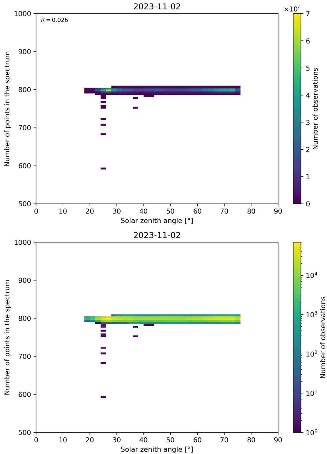
Figure 103: Scatter density plot of “Solar zenith angle” against “Number of points in the spectrum” for 2023-11-02 to 2023-11-03.
