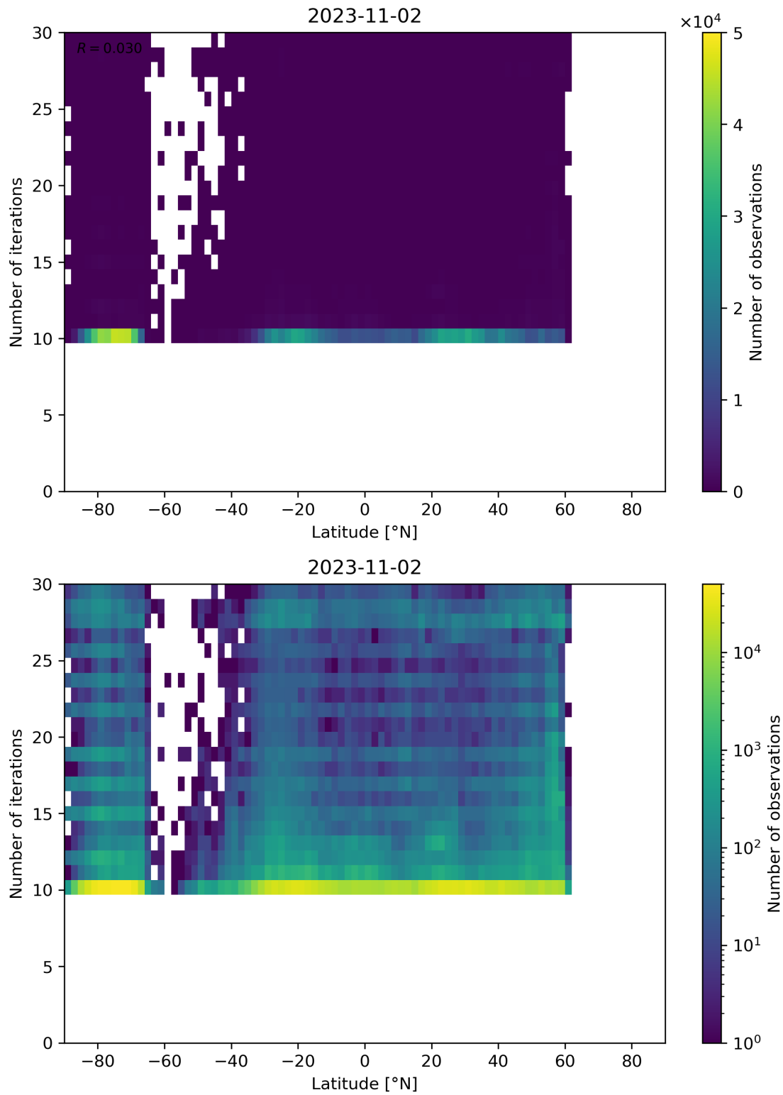
Figure 60: Scatter density plot of “Latitude” against “Number of iterations” for 2023-11-02 to 2023-11-03.
