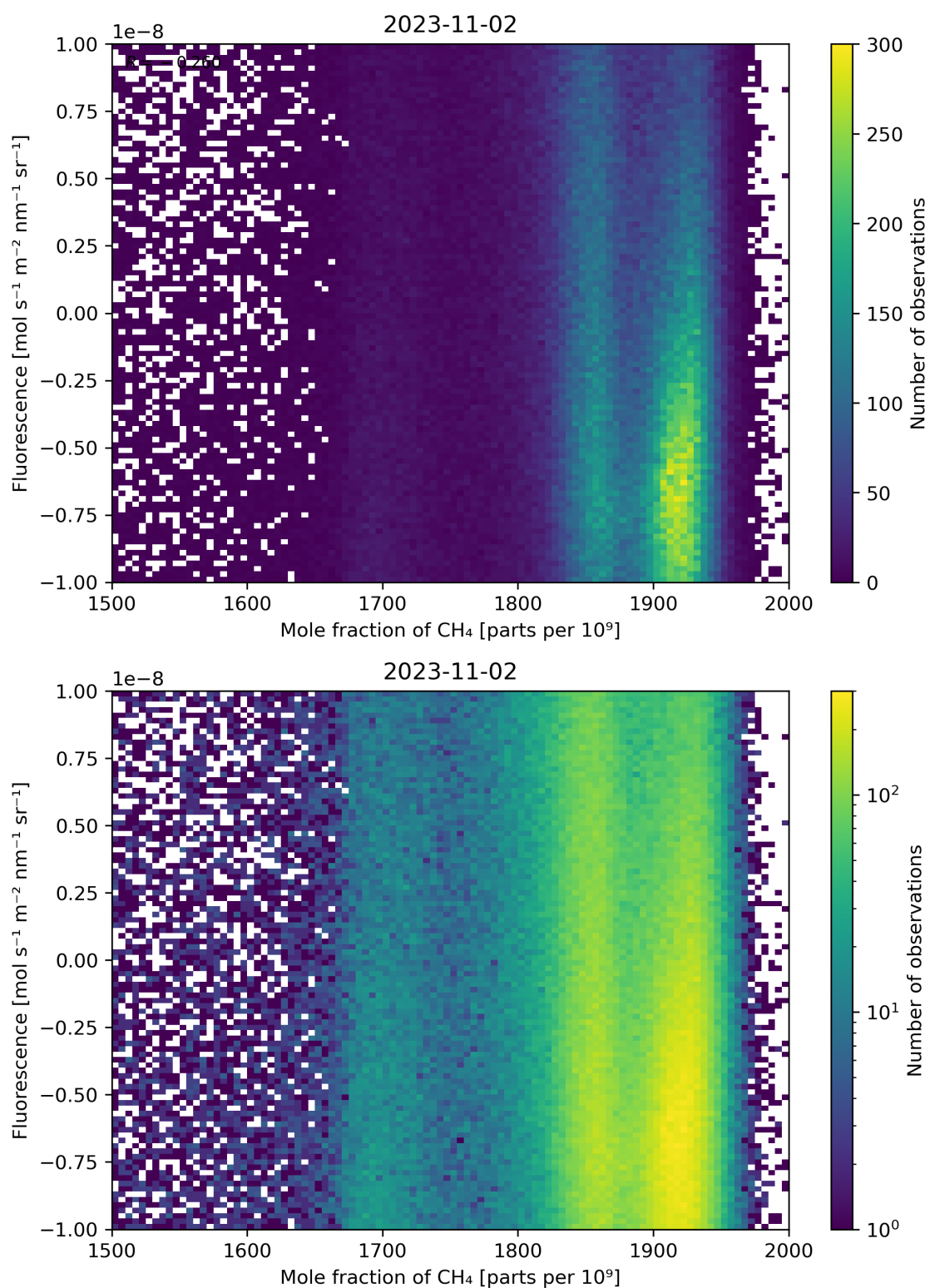
Figure 73: Scatter density plot of “Mole fraction of \text{CH}_4 ” against “Fluorescence” for 2023-11-02 to 2023-11-03.
