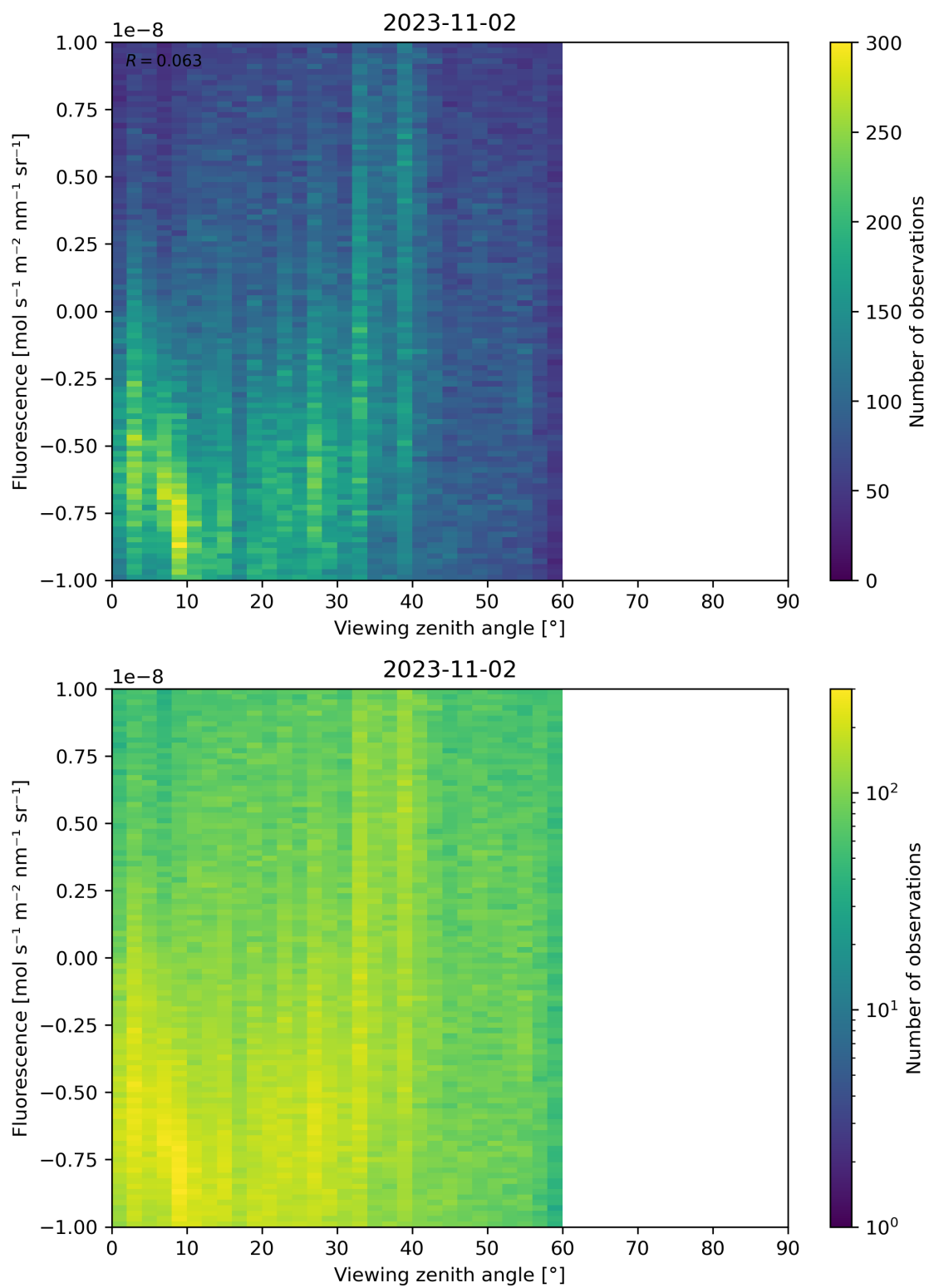
Figure 108: Scatter density plot of “Viewing zenith angle” against “Fluorescence” for 2023-11-02 to 2023-11-03.
