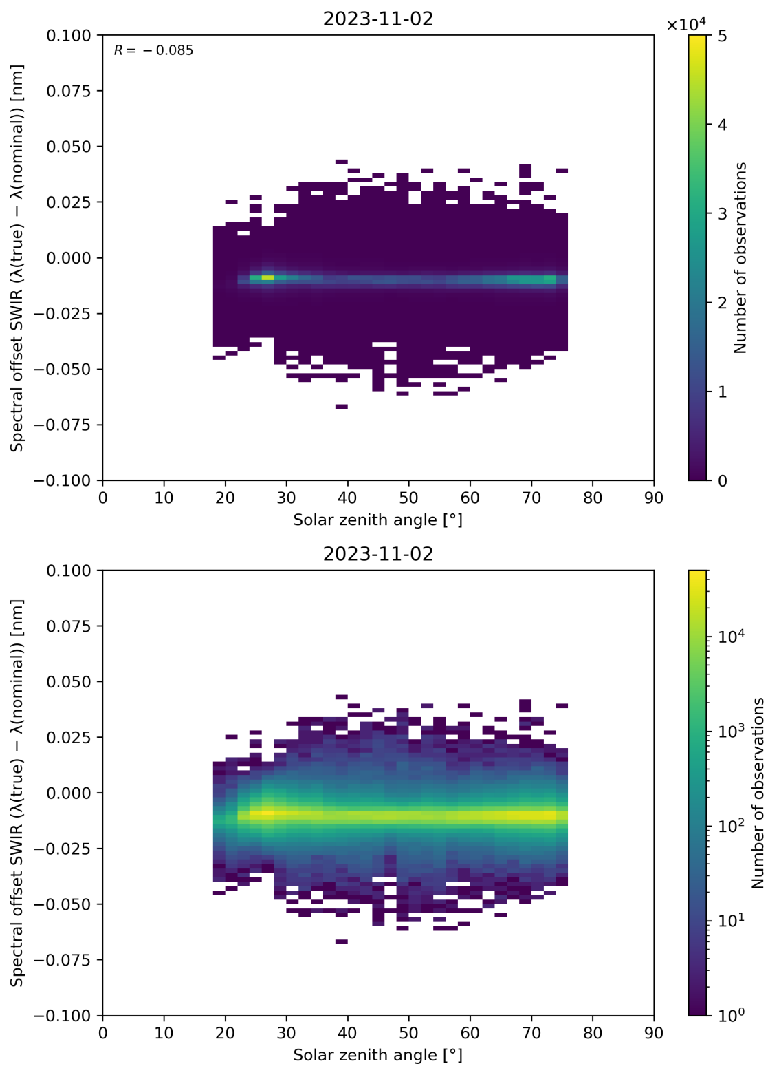
Figure 104: Scatter density plot of “Solar zenith angle” against “Spectral offset SWIR ( \lambda(\text{true}) - \lambda(\text{nominal}) )” for 2023-11-02 to 2023-11-03.
