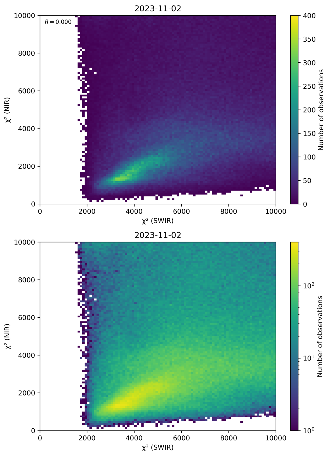
Figure 47: Scatter density plot of “ \chi^2 (SWIR)” against “ \chi^2 (NIR)” for 2023-11-02 to 2023-11-03.
