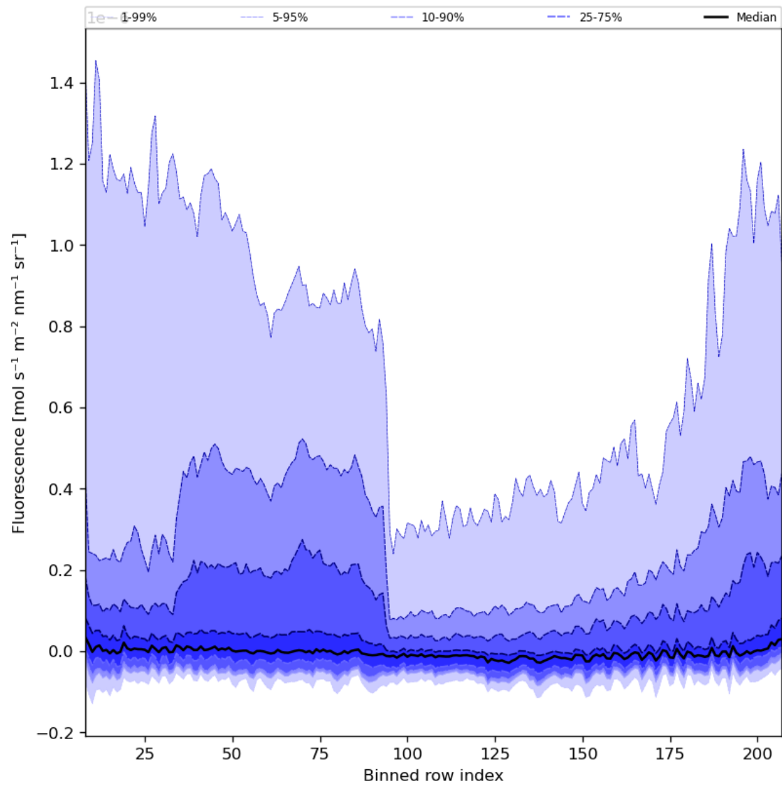
Figure 43: Along track statistics of “Fluorescence” for 2023-11-02 to 2023-11-03
