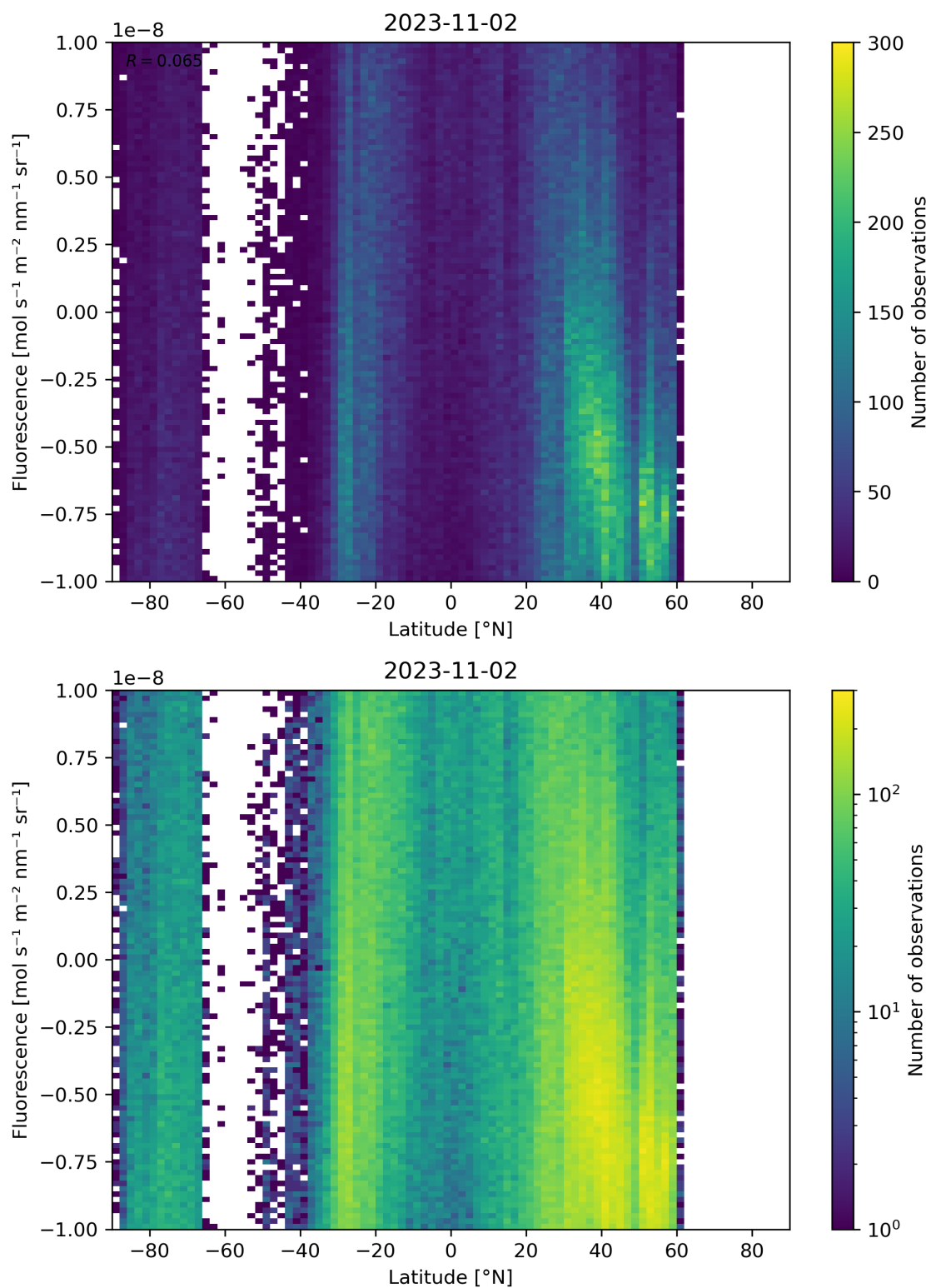
Figure 56: Scatter density plot of “Latitude” against “Fluorescence” for 2023-11-02 to 2023-11-03.
