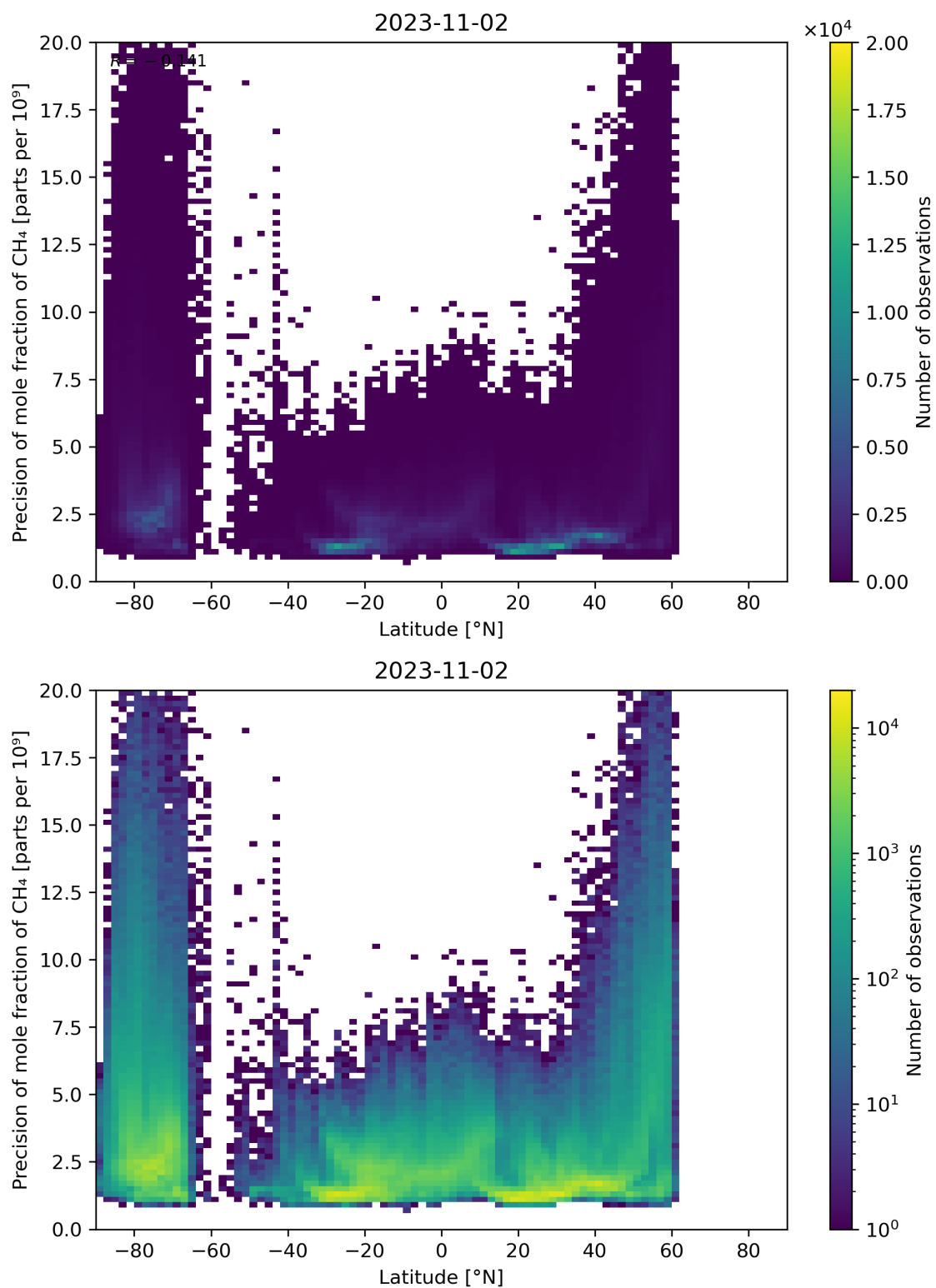
Figure 59: Scatter density plot of “Latitude” against “Precision of mole fraction of CH 4 ” for 2023-11-02 to 2023-11-03.
