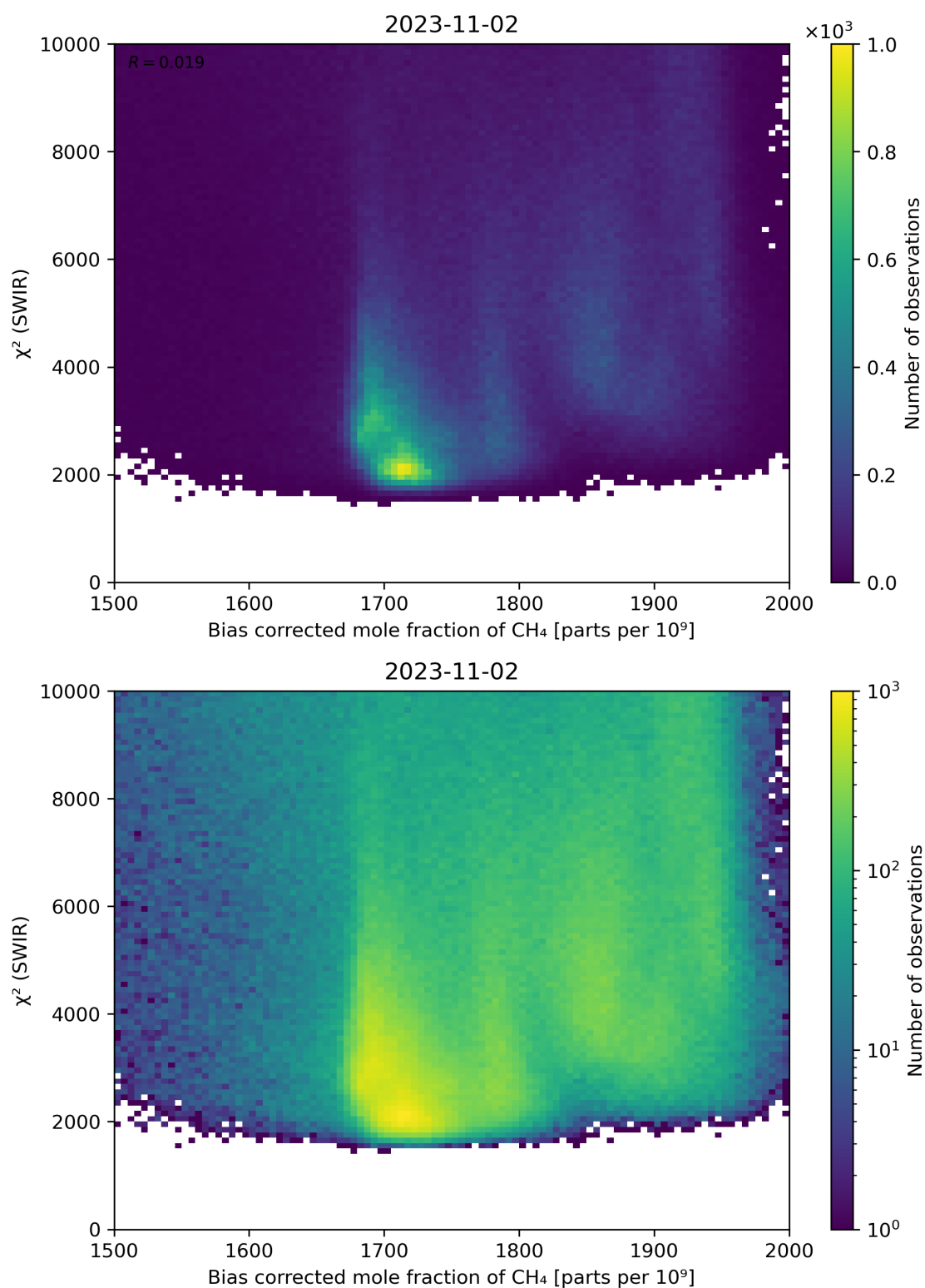
Figure 64: Scatter density plot of “Bias corrected mole fraction of CH 4 ” against “ \chi^2 (SWIR)” for 2023-11-02 to 2023-11-03.
