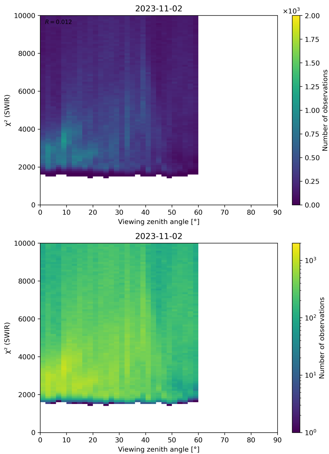
Figure 106: Scatter density plot of “Viewing zenith angle” against “ \chi^2 (SWIR)” for 2023-11-02 to 2023-11-03.
