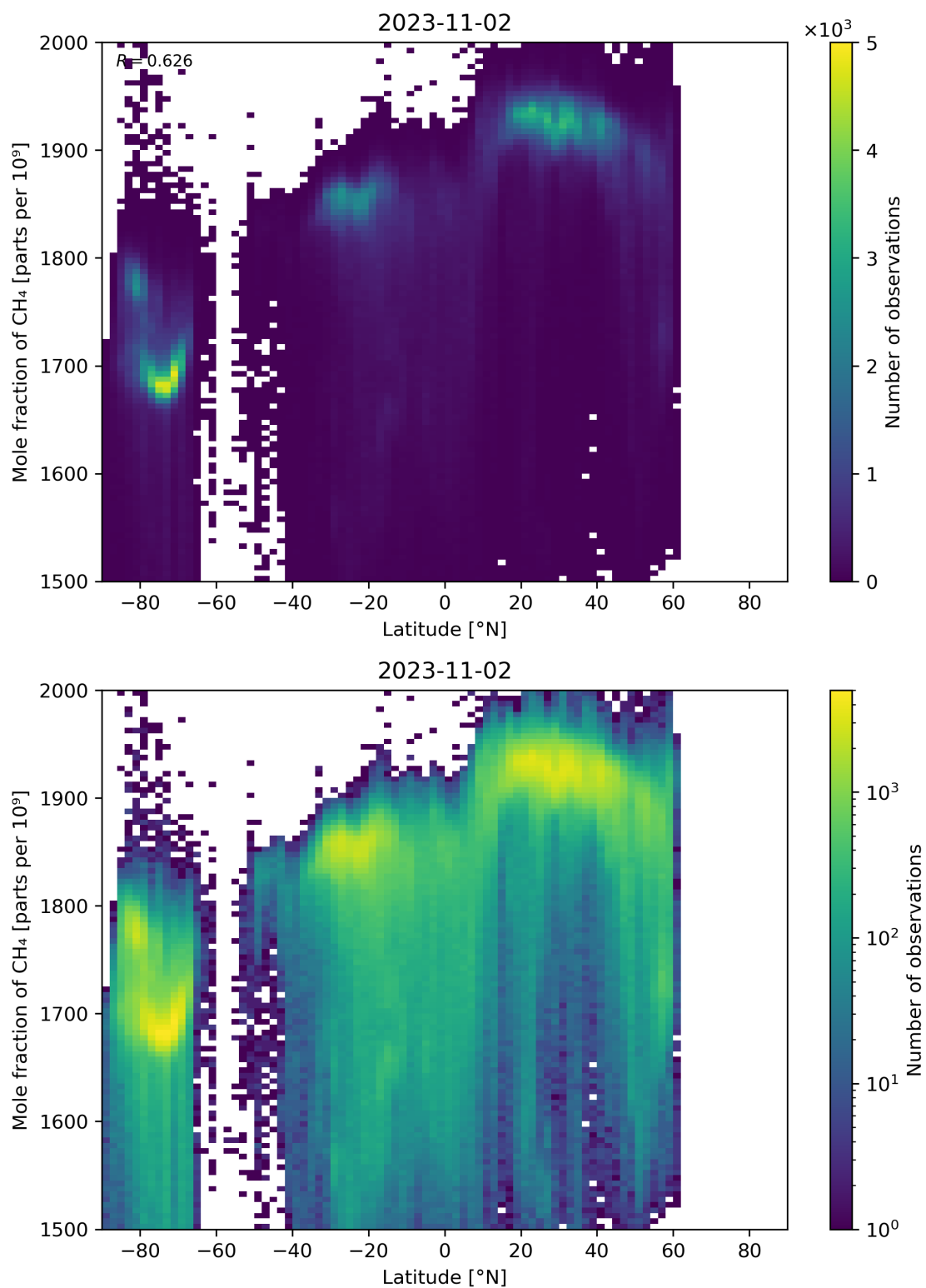
Figure 57: Scatter density plot of “Latitude” against “Mole fraction of CH 4 ” for 2023-11-02 to 2023-11-03.
