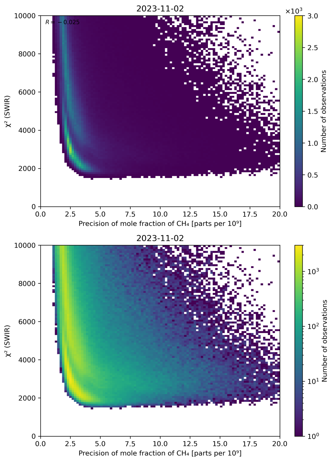
Figure 79: Scatter density plot of “Precision of mole fraction of \text{CH}_4 ” against “ \chi^2 (SWIR)” for 2023-11-02 to 2023-11-03.
