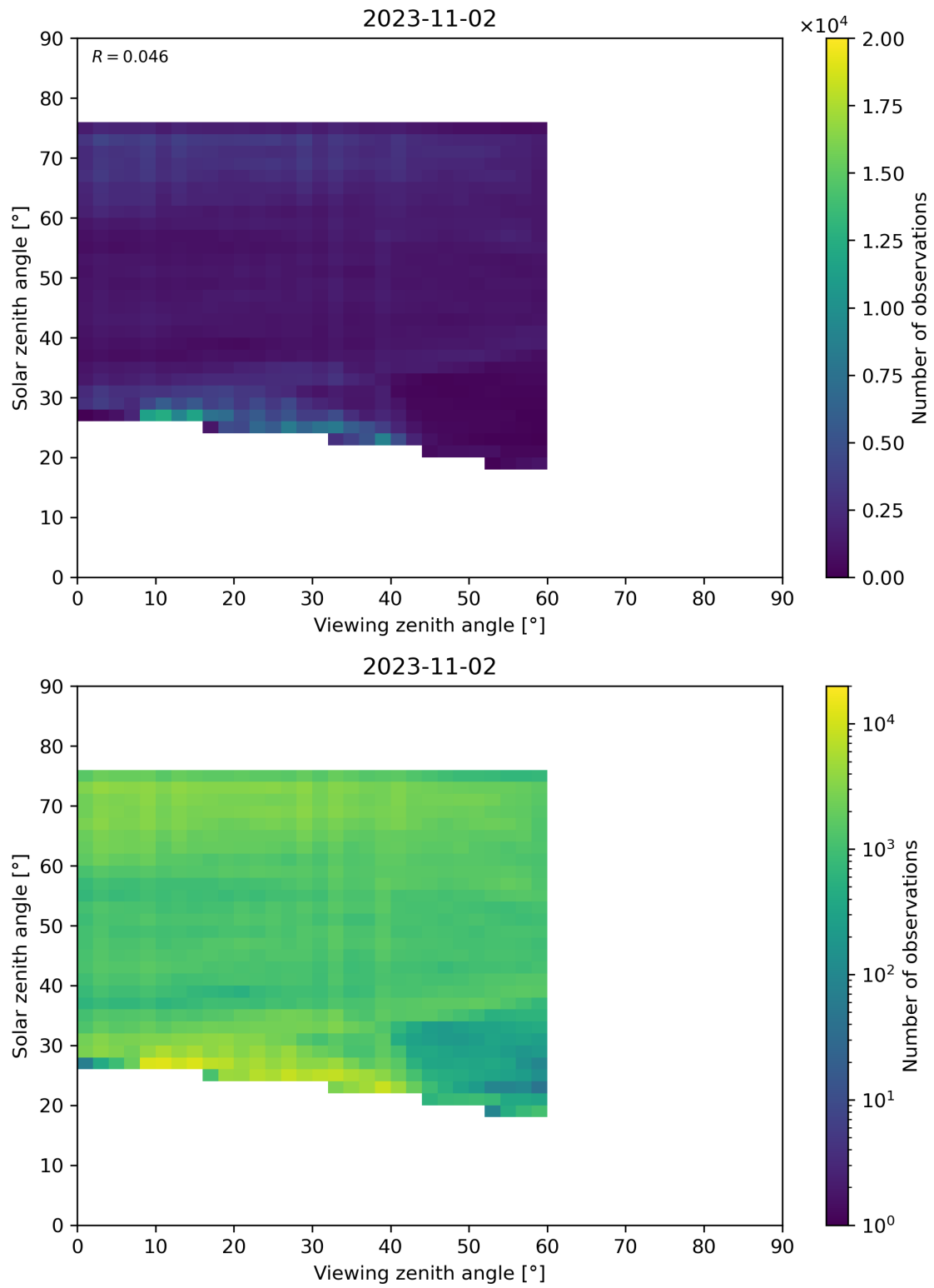
Figure 115: Scatter density plot of “Viewing zenith angle” against “Solar zenith angle” for 2023-11-02 to 2023-11-03.
