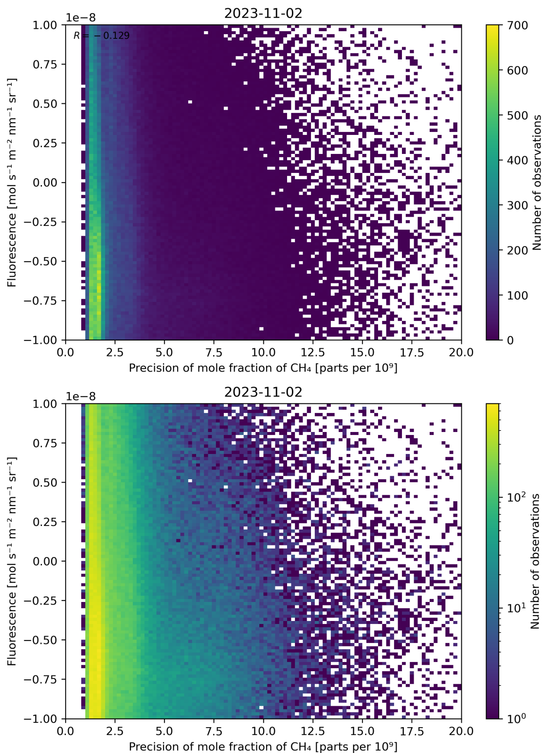
Figure 81: Scatter density plot of “Precision of mole fraction of \text{CH}_4 ” against “Fluorescence” for 2023-11-02 to 2023-11-03.
