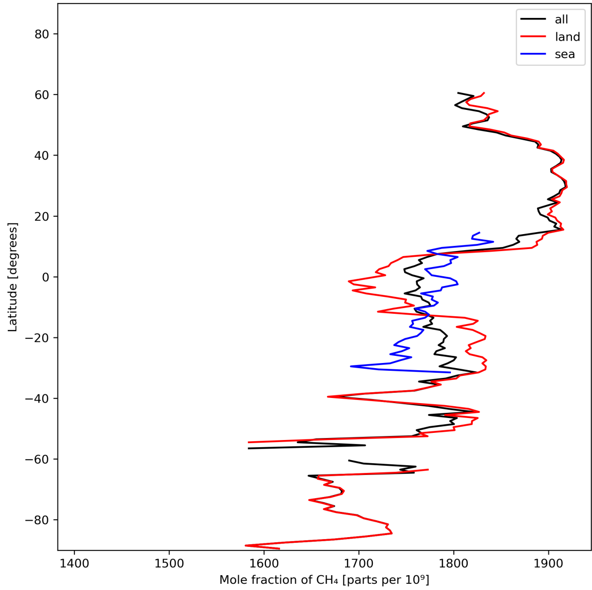
Figure 12: Zonal average of “Mole fraction of CH 4 ” for 2023-11-02 to 2023-11-03.
