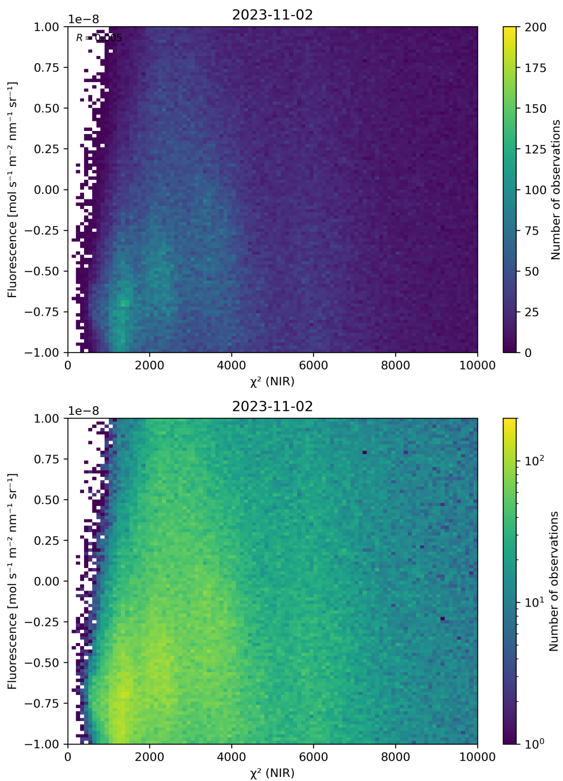
Figure 45: Scatter density plot of “ \chi^2 (NIR)” against “Fluorescence” for 2023-11-02 to 2023-11-03.
