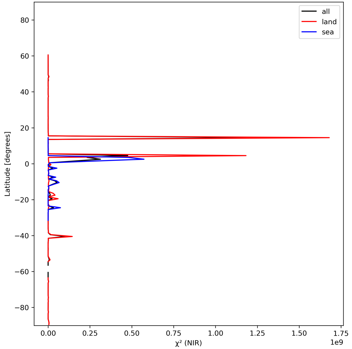
Figure 18: Zonal average of “ \chi^2 (NIR)” for 2023-11-02 to 2023-11-03.
