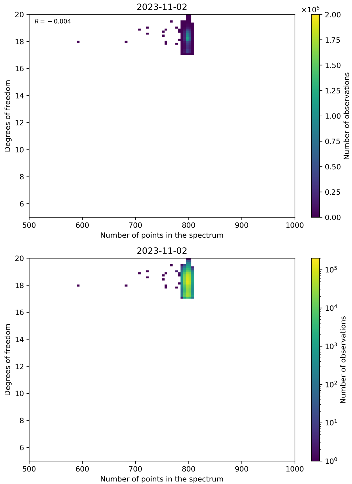
Figure 90: Scatter density plot of “Number of points in the spectrum” against “Degrees of freedom” for 2023-11-02 to 2023-11-03.
