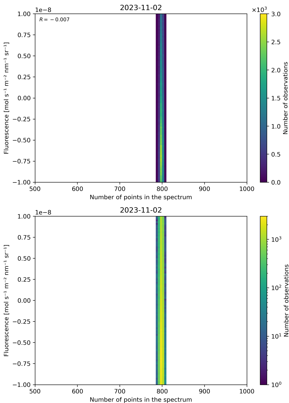
Figure 91: Scatter density plot of “Number of points in the spectrum” against “Fluorescence” for 2023-11-02 to 2023-11-03.
