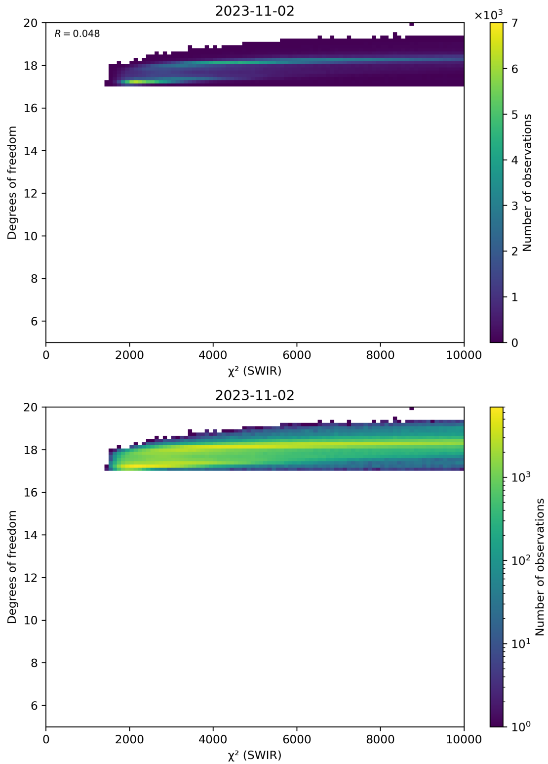
Figure 48: Scatter density plot of “ \chi^2 (SWIR)” against “Degrees of freedom” for 2023-11-02 to 2023-11-03.
