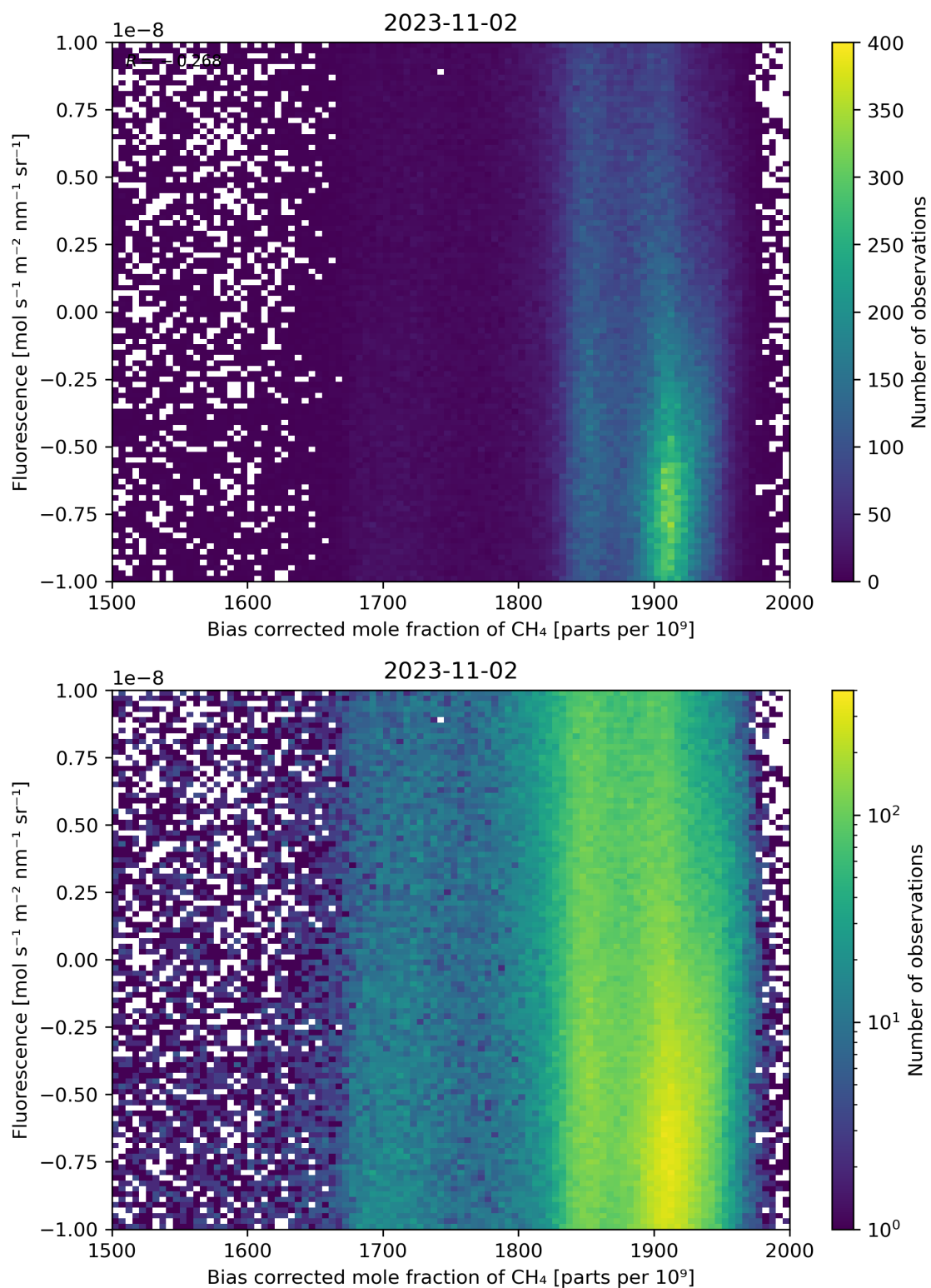
Figure 66: Scatter density plot of “Bias corrected mole fraction of CH 4 ” against “Fluorescence” for 2023-11-02 to 2023-11-03.
