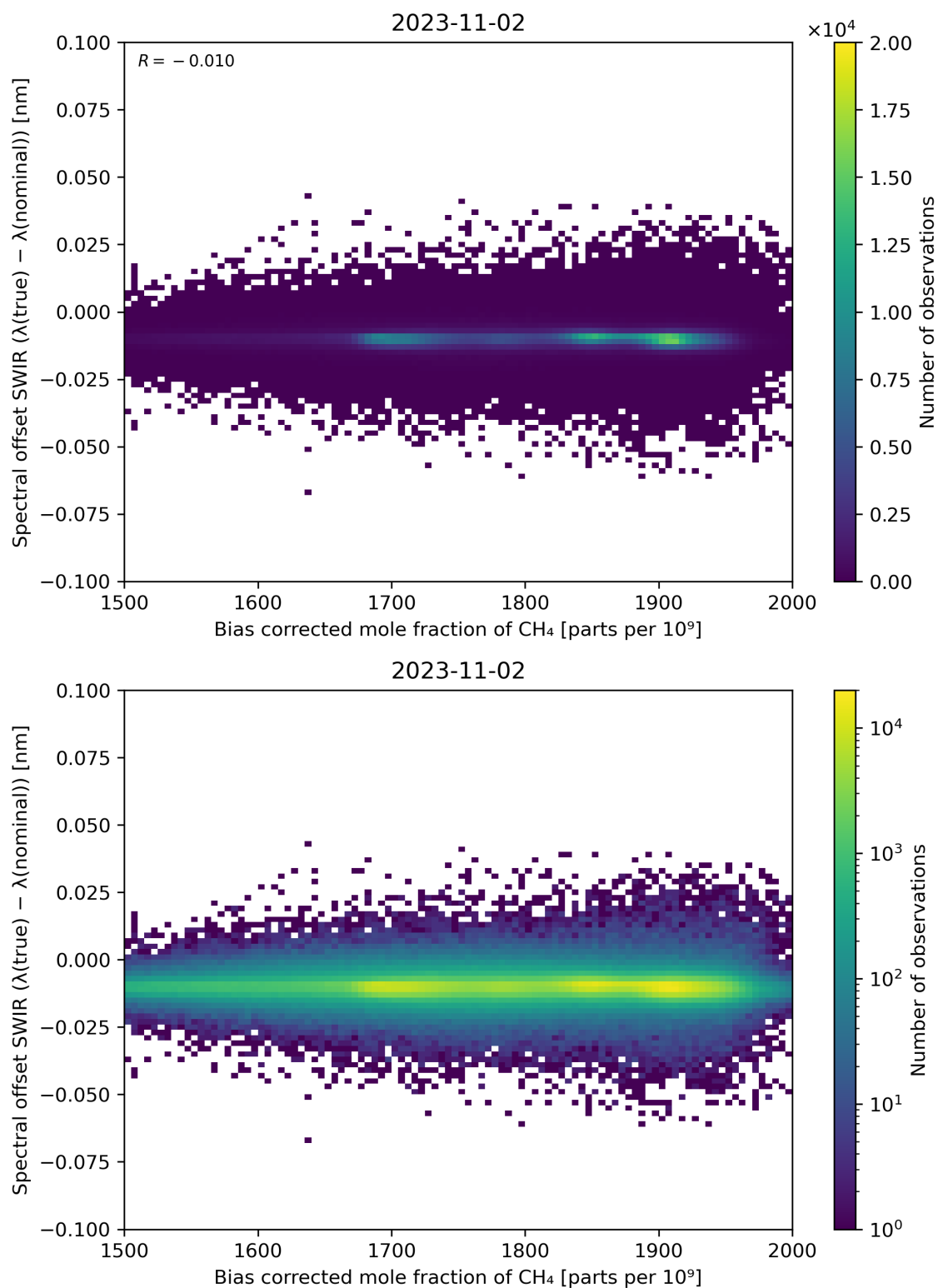
Figure 69: Scatter density plot of “Bias corrected mole fraction of \text{CH}_4 ” against “Spectral offset SWIR ( \lambda(\text{true}) - \lambda(\text{nominal}) )” for 2023-11-02 to 2023-11-03.
