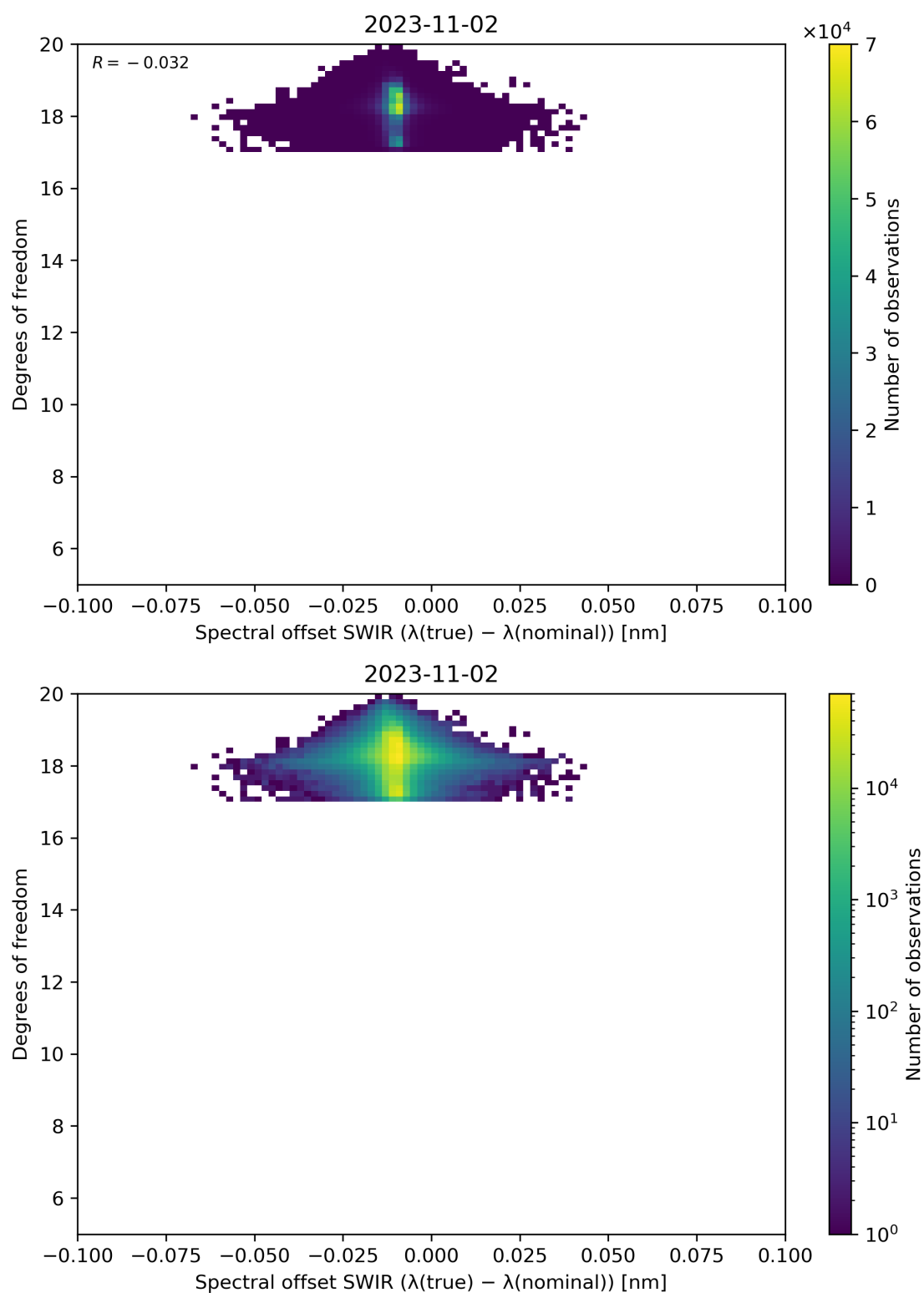
Figure 119: Scatter density plot of “Spectral offset SWIR ( \lambda(\text{true}) - \lambda(\text{nominal}) )” against “Degrees of freedom” for 2023-11-02 to 2023-11-03.
