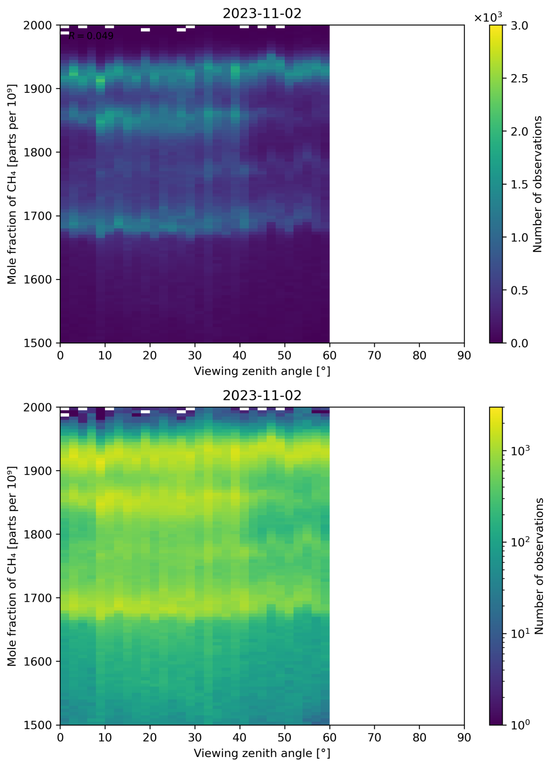
Figure 110: Scatter density plot of “Viewing zenith angle” against “Mole fraction of CH 4 ” for 2023-11-02 to 2023-11-03.
