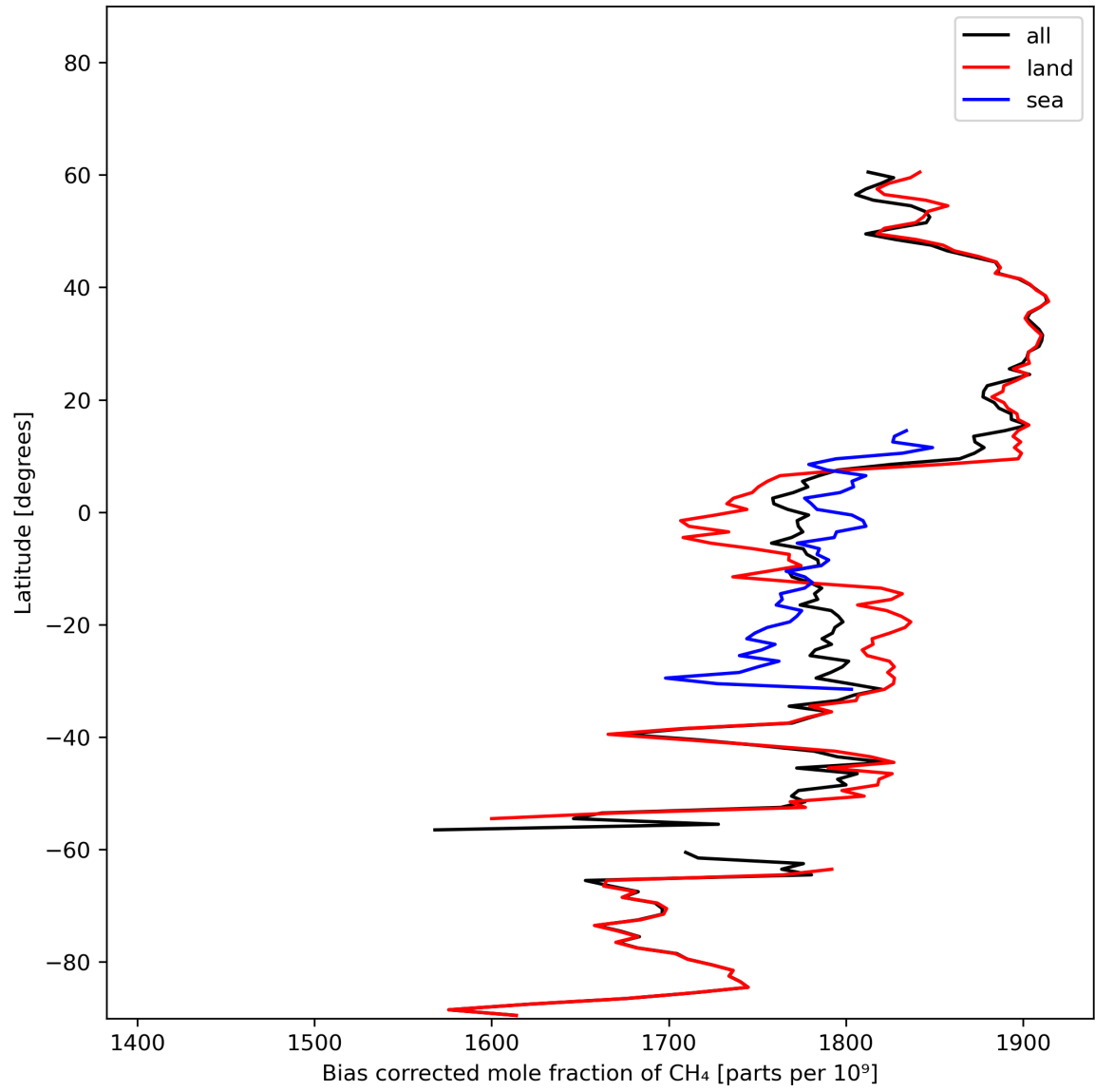
Figure 14: Zonal average of “Bias corrected mole fraction of CH 4 ” for 2023-11-02 to 2023-11-03.
