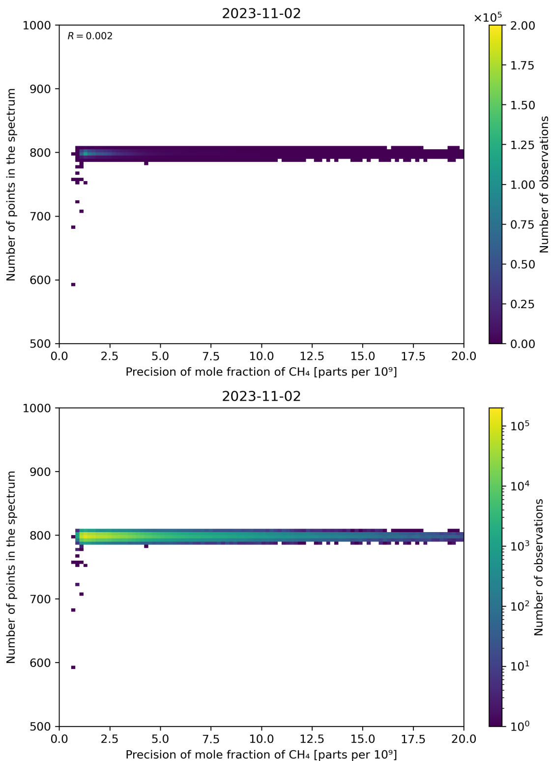
Figure 84: Scatter density plot of “Precision of mole fraction of \text{CH}_4 ” against “Number of points in the spectrum” for 2023-11-02 to 2023-11-03.
