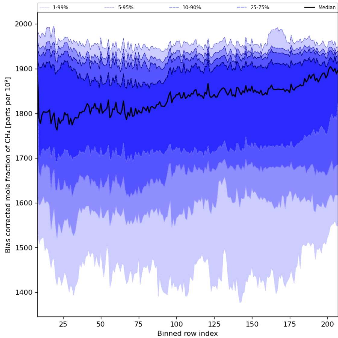
Figure 36: Along track statistics of “Bias corrected mole fraction of CH 4 ” for 2023-11-02 to 2023-11-03
