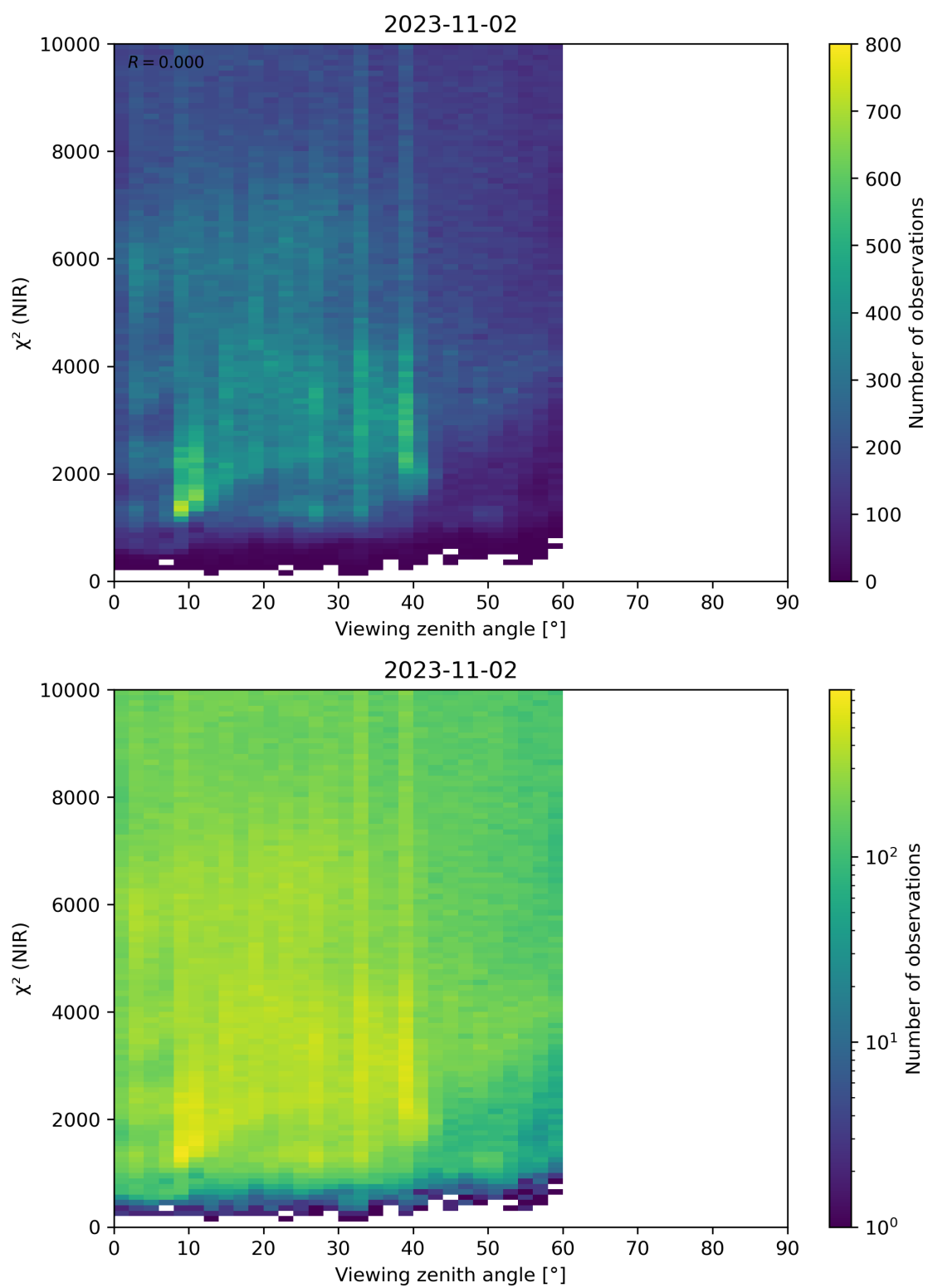
Figure 105: Scatter density plot of “Viewing zenith angle” against “ \chi^2 (NIR)” for 2023-11-02 to 2023-11-03.
