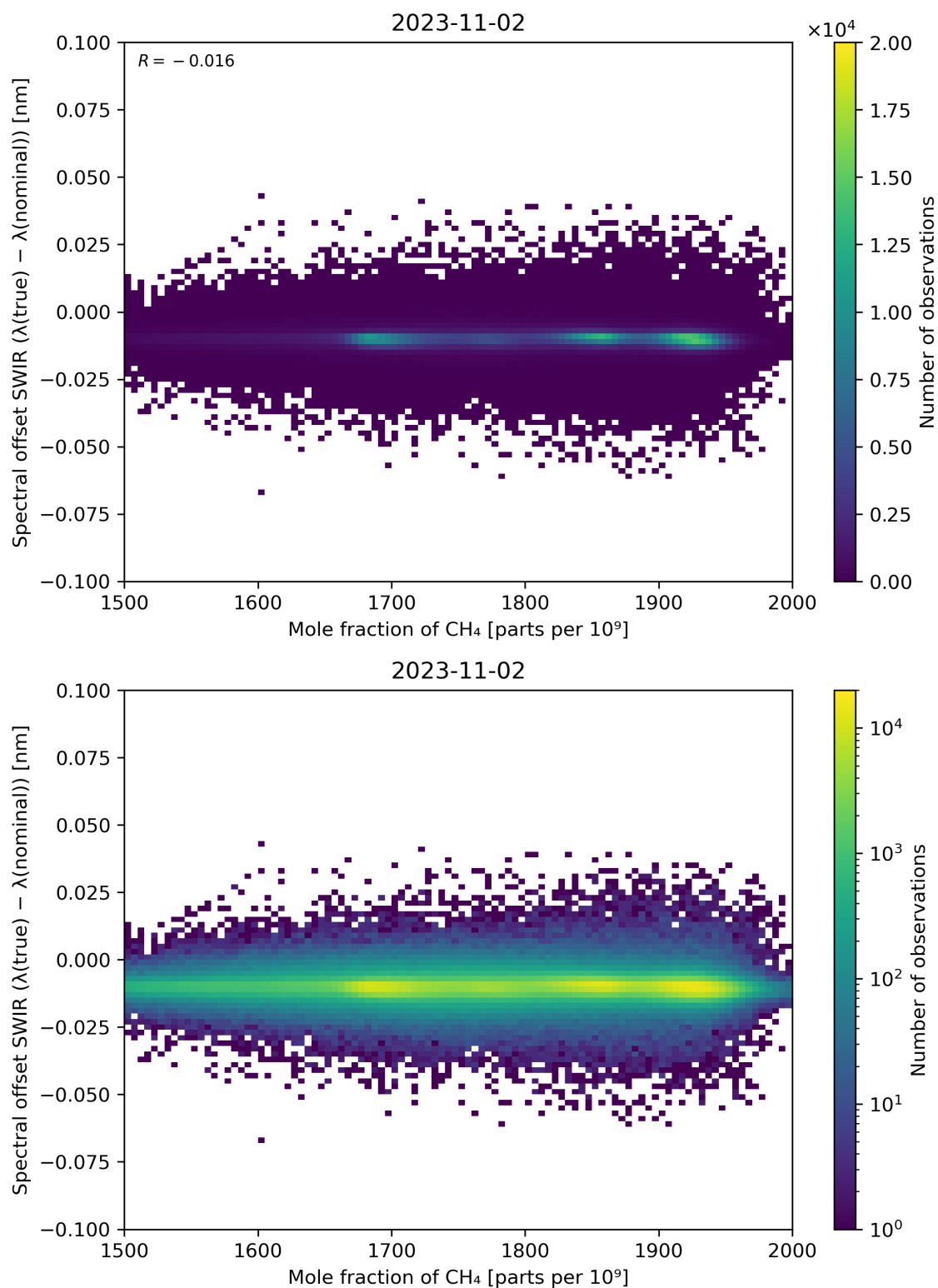
Figure 86: Scatter density plot of “Mole fraction of CH 4 ” against “Spectral offset SWIR ( \lambda(\text{true}) - \lambda(\text{nominal}) )” for 2023-11-02 to 2023-11-03.
