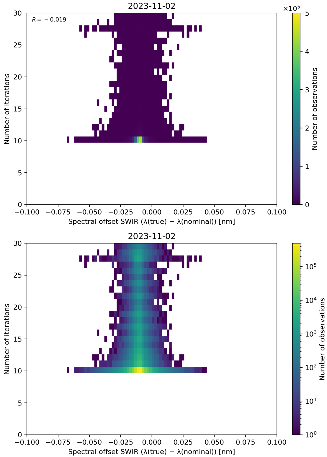
Figure 121: Scatter density plot of “Spectral offset SWIR ( \lambda(\text{true}) - \lambda(\text{nominal}) )” against “Number of iterations” for 2023-11-02 to 2023-11-03.
