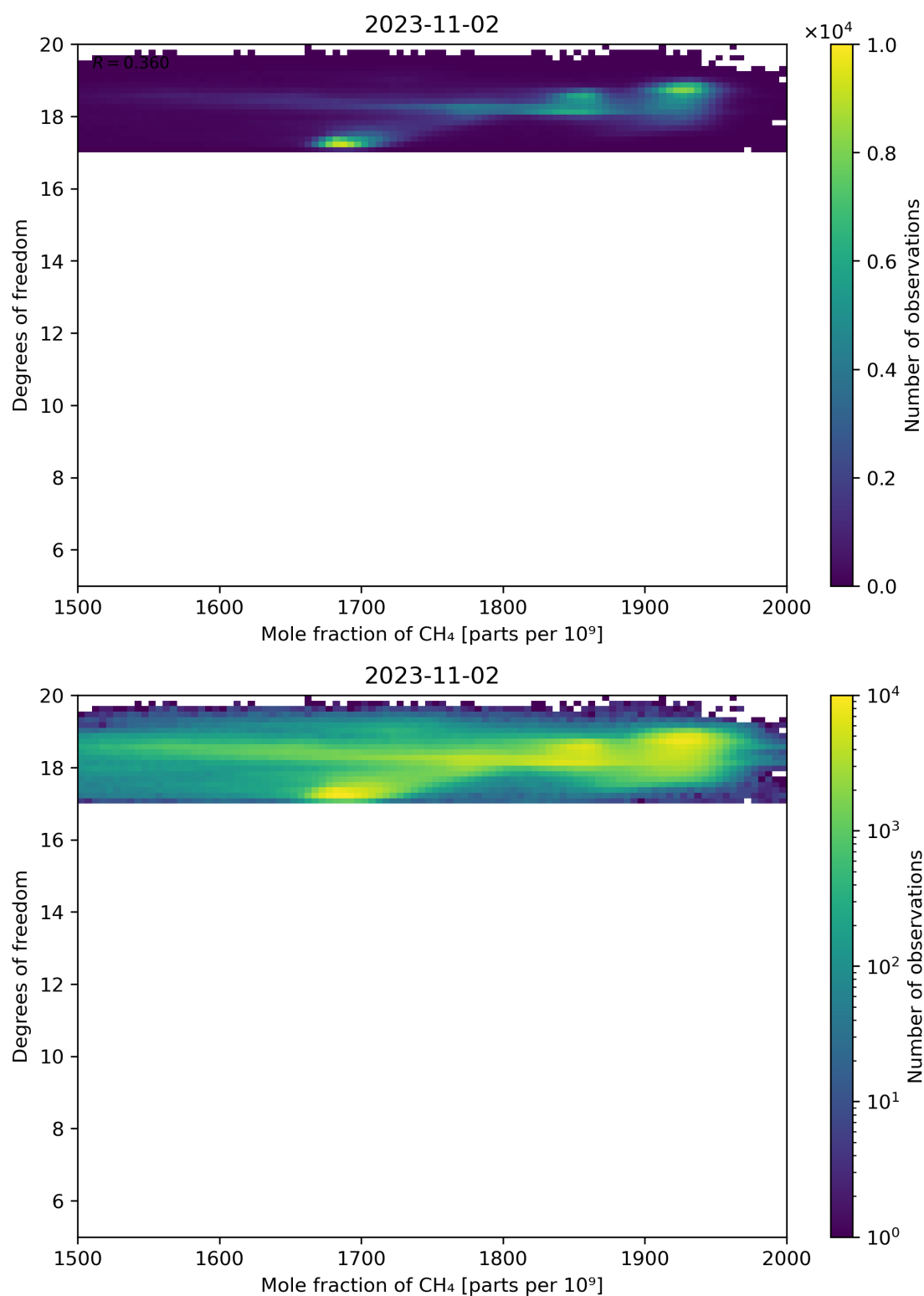
Figure 72: Scatter density plot of “Mole fraction of CH 4 ” against “Degrees of freedom” for 2023-11-02 to 2023-11-03.
