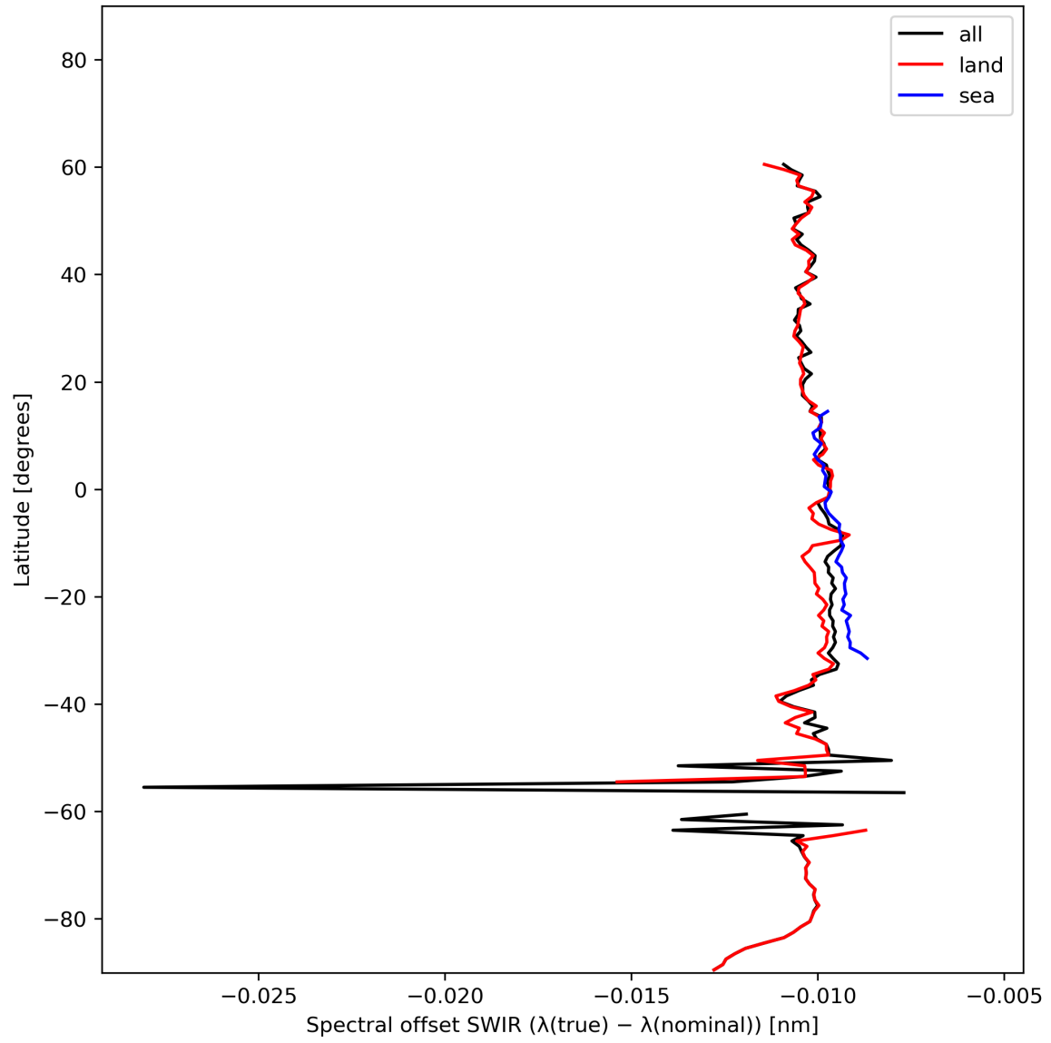
Figure 16: Zonal average of “Spectral offset SWIR ( \lambda(\text{true}) - \lambda(\text{nominal}) )” for 2023-11-02 to 2023-11-03.
