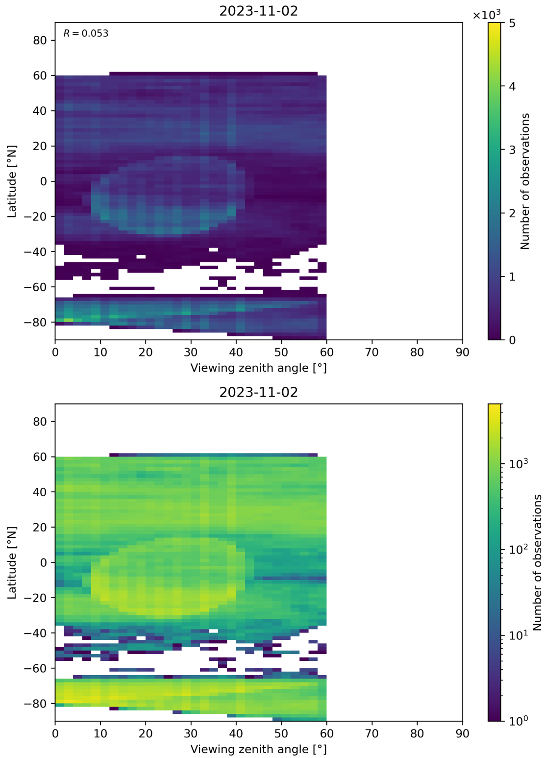
Figure 109: Scatter density plot of “Viewing zenith angle” against “Latitude” for 2023-11-02 to 2023-11-03.
