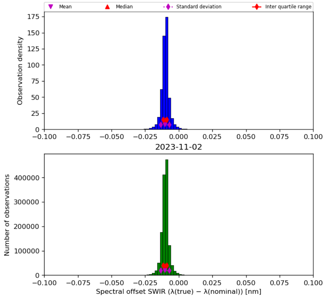
Figure 27: Histogram of “Spectral offset SWIR ( \lambda(\text{true}) - \lambda(\text{nominal}) )” for 2023-11-02 to 2023-11-03
