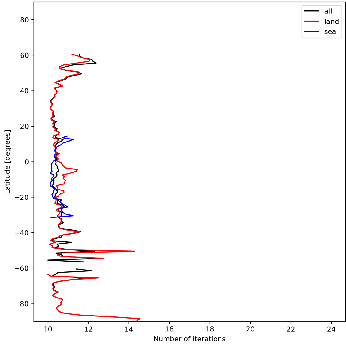
Figure 20: Zonal average of “Number of iterations” for 2023-11-02 to 2023-11-03.
