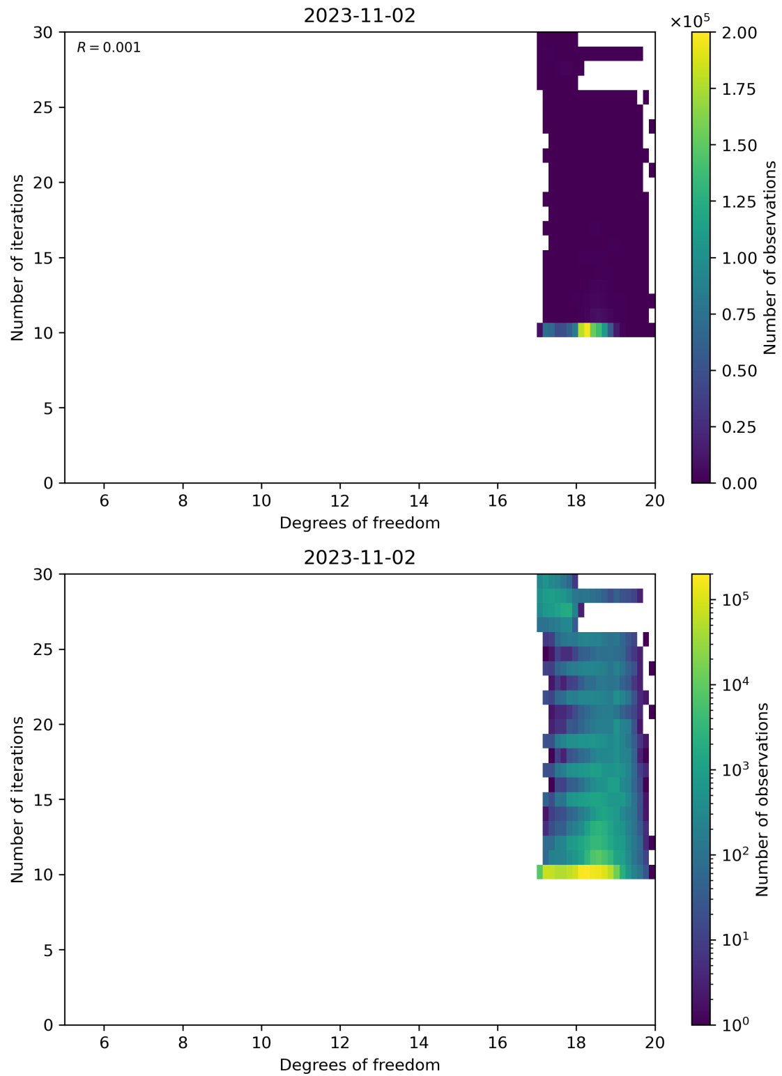
Figure 52: Scatter density plot of “Degrees of freedom” against “Number of iterations” for 2023-11-02 to 2023-11-03.
