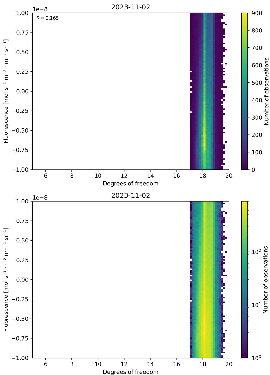
Figure 51: Scatter density plot of “Degrees of freedom” against “Fluorescence” for 2023-11-02 to 2023-11-03.
