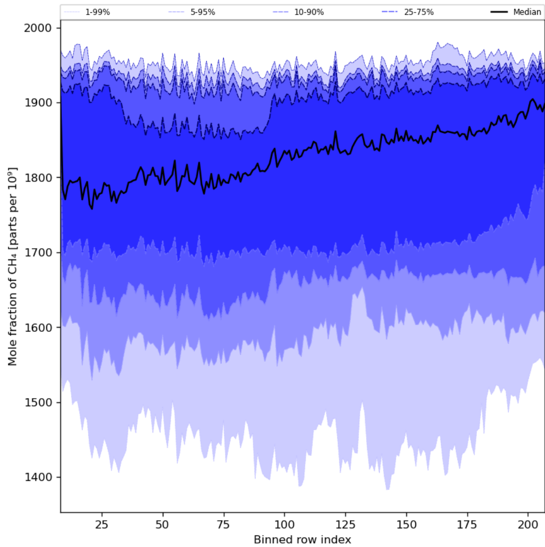
Figure 34: Along track statistics of “Mole fraction of CH 4 ” for 2023-11-02 to 2023-11-03
