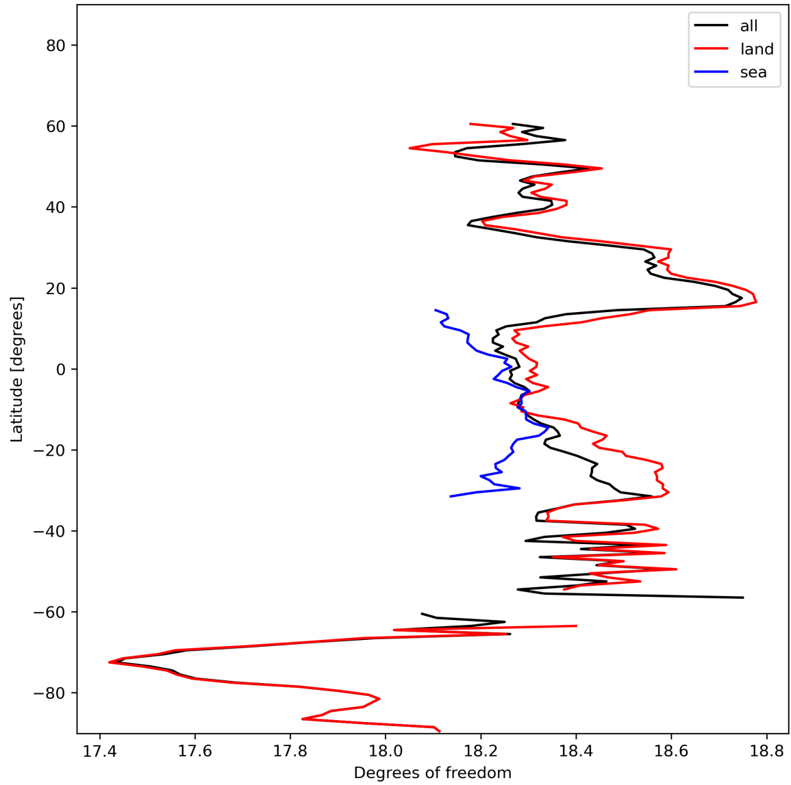
Figure 19: Zonal average of “Degrees of freedom” for 2023-11-02 to 2023-11-03.
