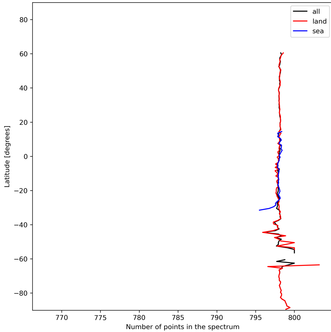
Figure 15: Zonal average of “Number of points in the spectrum” for 2023-11-02 to 2023-11-03.
