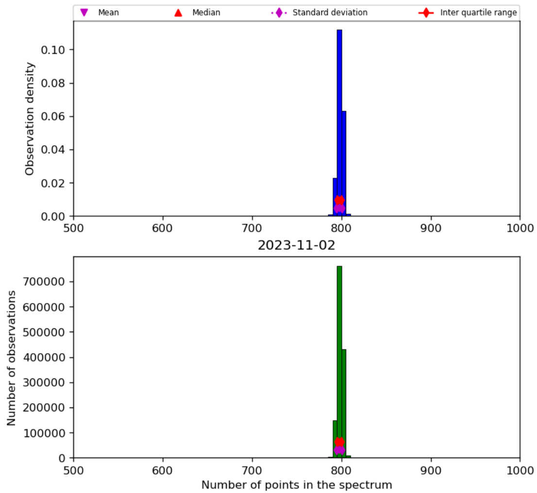
Figure 26: Histogram of “Number of points in the spectrum” for 2023-11-02 to 2023-11-03
