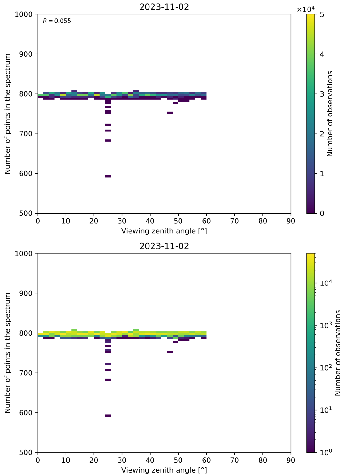
Figure 114: Scatter density plot of “Viewing zenith angle” against “Number of points in the spectrum” for 2023-11-02 to 2023-11-03.
