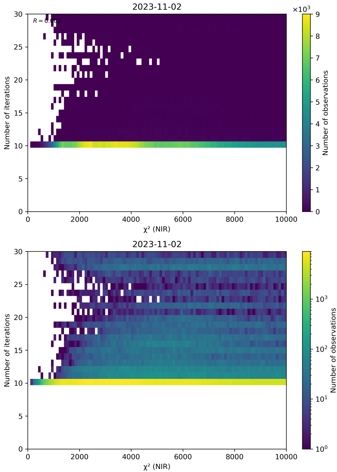
Figure 46: Scatter density plot of “ \chi^2 (NIR)” against “Number of iterations” for 2023-11-02 to 2023-11-03.
