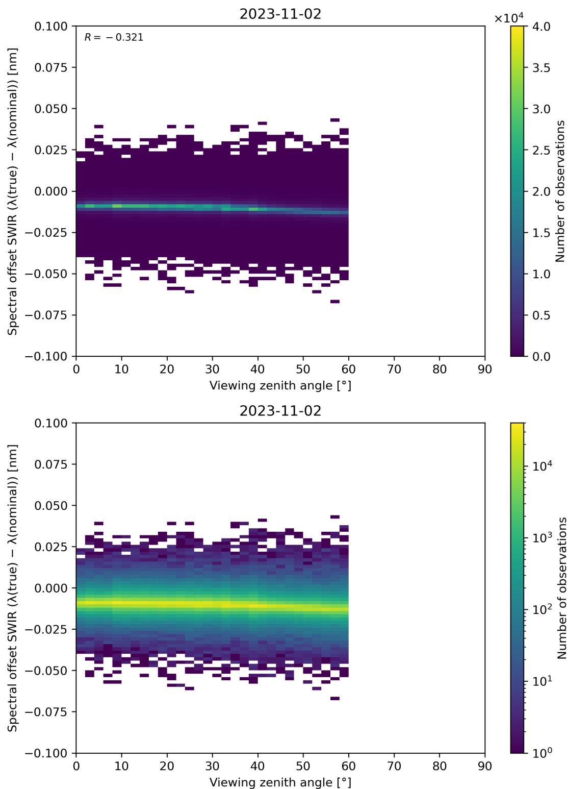
Figure 116: Scatter density plot of “Viewing zenith angle” against “Spectral offset SWIR ( \lambda(\text{true}) - \lambda(\text{nominal}) )” for 2023-11-02 to 2023-11-03.
