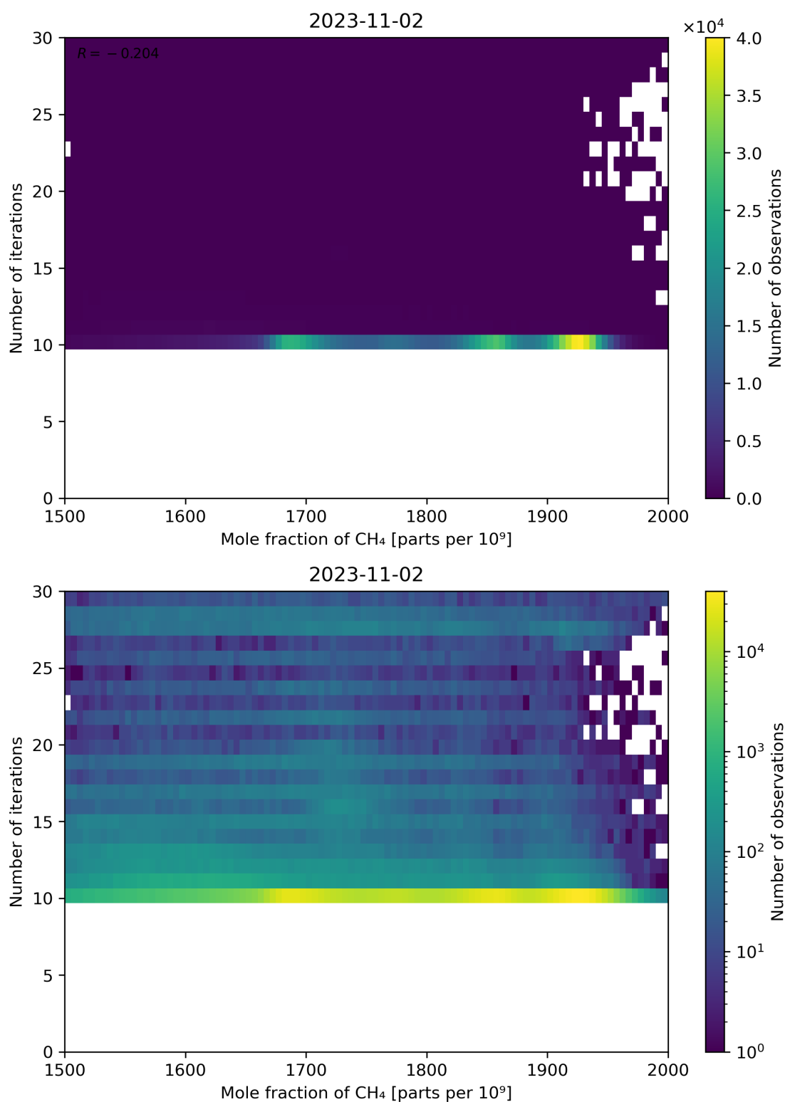
Figure 76: Scatter density plot of “Mole fraction of CH 4 ” against “Number of iterations” for 2023-11-02 to 2023-11-03.
