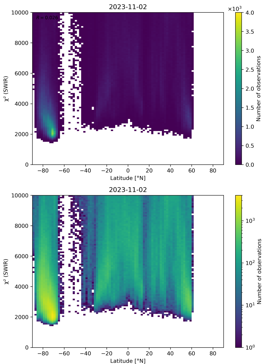
Figure 54: Scatter density plot of “Latitude” against “ \chi^2 (SWIR)” for 2023-11-02 to 2023-11-03.
