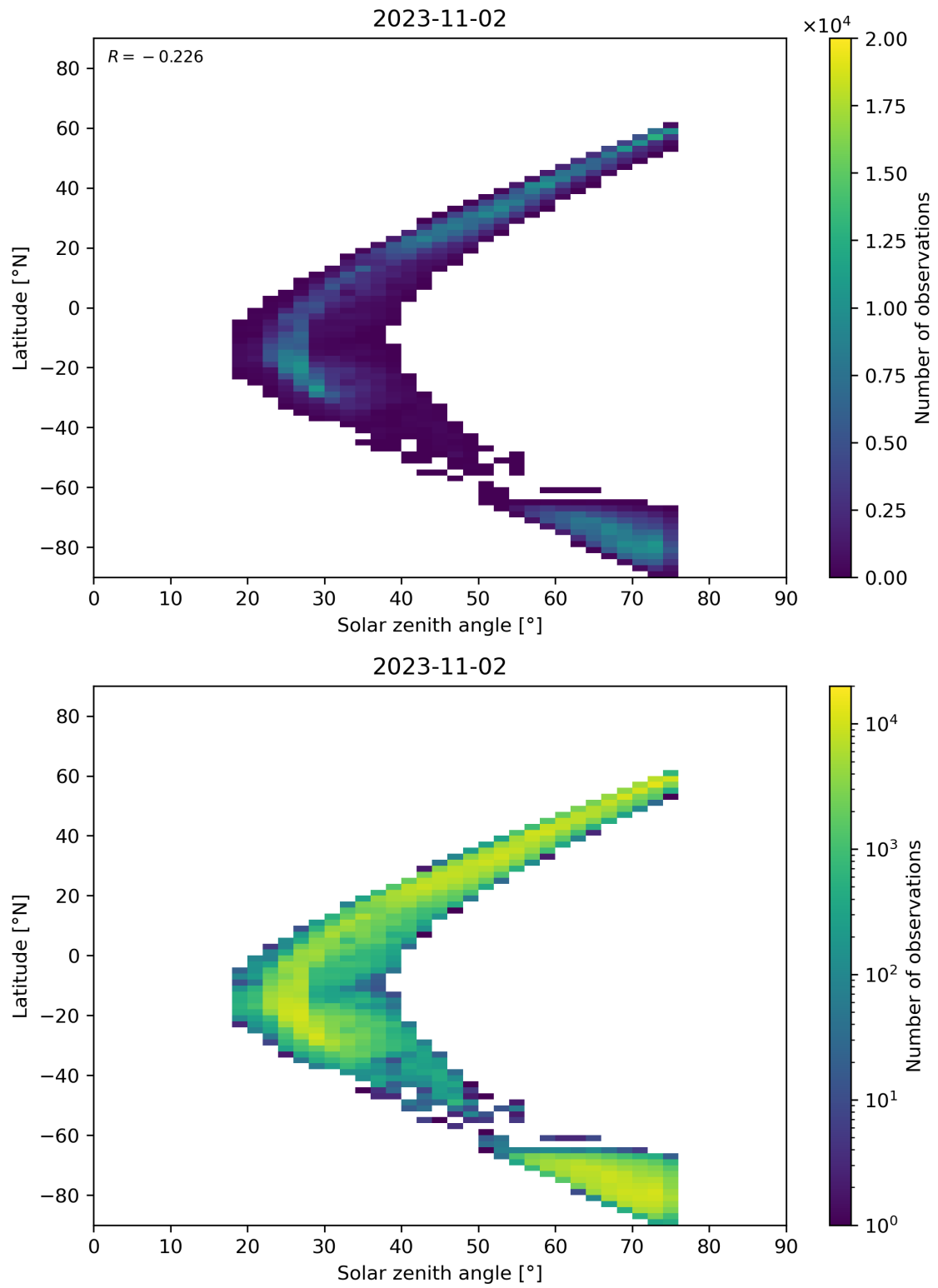
Figure 98: Scatter density plot of “Solar zenith angle” against “Latitude” for 2023-11-02 to 2023-11-03.
