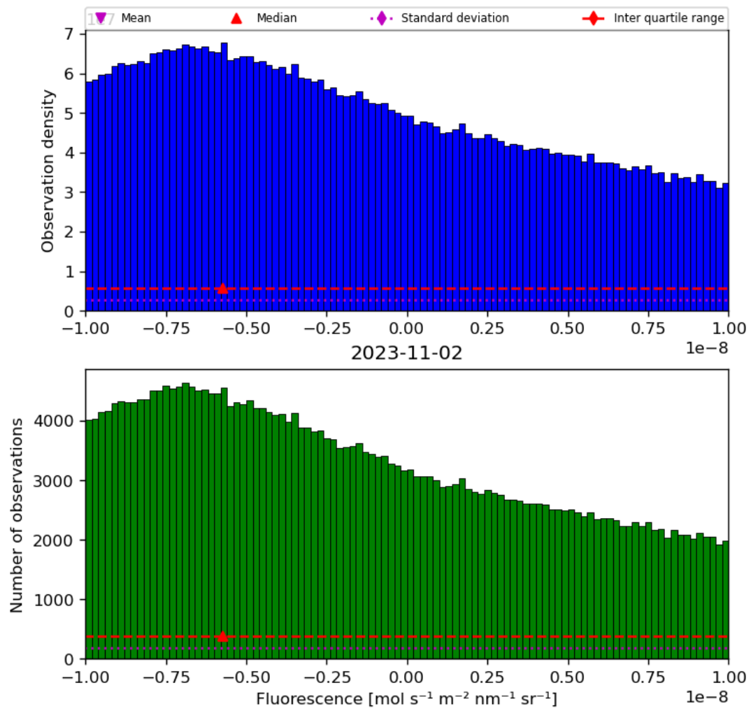
Figure 32: Histogram of “Fluorescence” for 2023-11-02 to 2023-11-03
