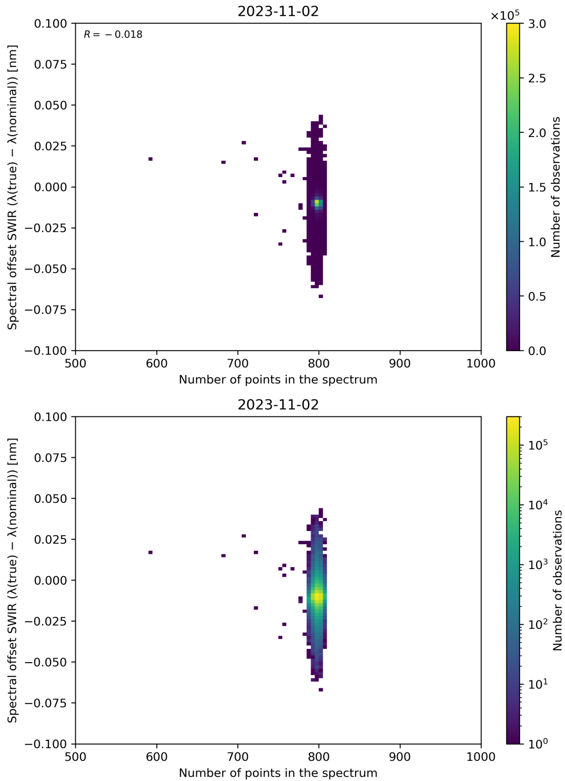
Figure 93: Scatter density plot of “Number of points in the spectrum” against “Spectral offset SWIR ( \lambda(\text{true}) - \lambda(\text{nominal}) )” for 2023-11-02 to 2023-11-03.
