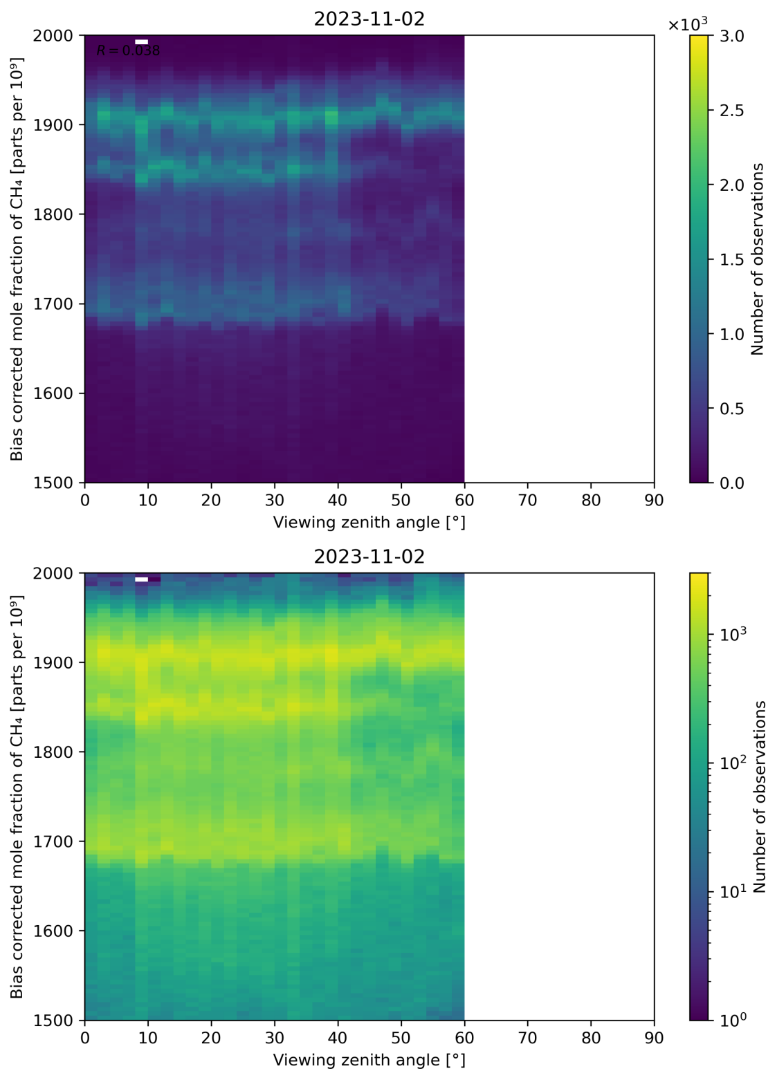
Figure 111: Scatter density plot of “Viewing zenith angle” against “Bias corrected mole fraction of CH 4 ” for 2023-11-02 to 2023-11-03.
