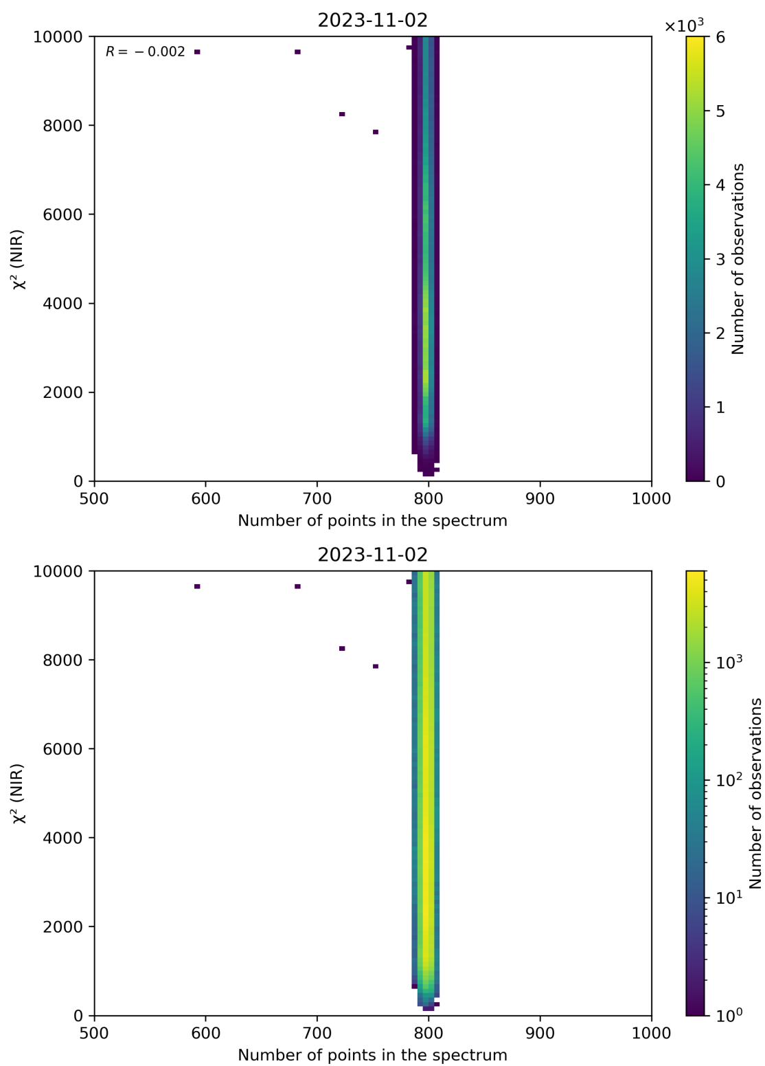
Figure 88: Scatter density plot of “Number of points in the spectrum” against “ \chi^2 (NIR)” for 2023-11-02 to 2023-11-03.
