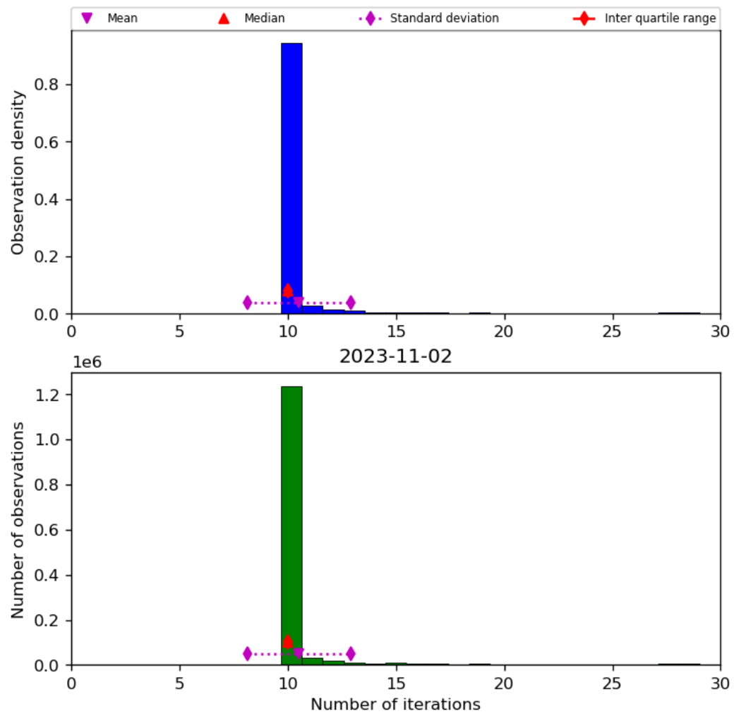
Figure 31: Histogram of “Number of iterations” for 2023-11-02 to 2023-11-03
