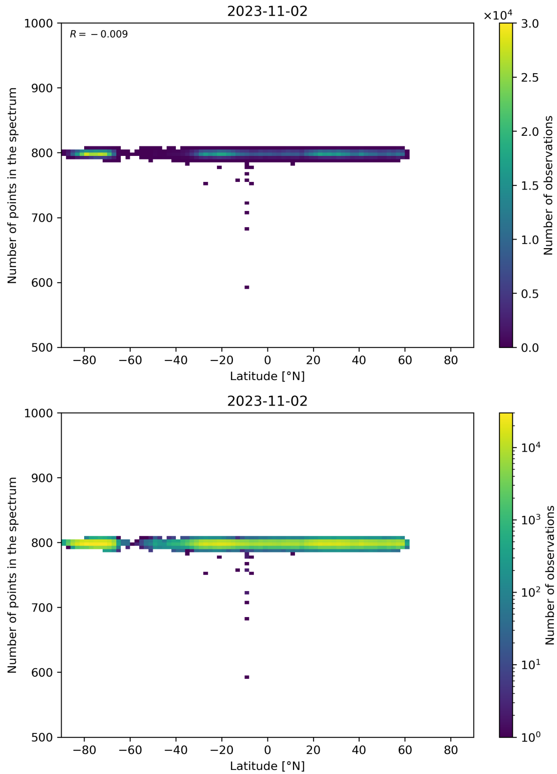
Figure 61: Scatter density plot of “Latitude” against “Number of points in the spectrum” for 2023-11-02 to 2023-11-03.
