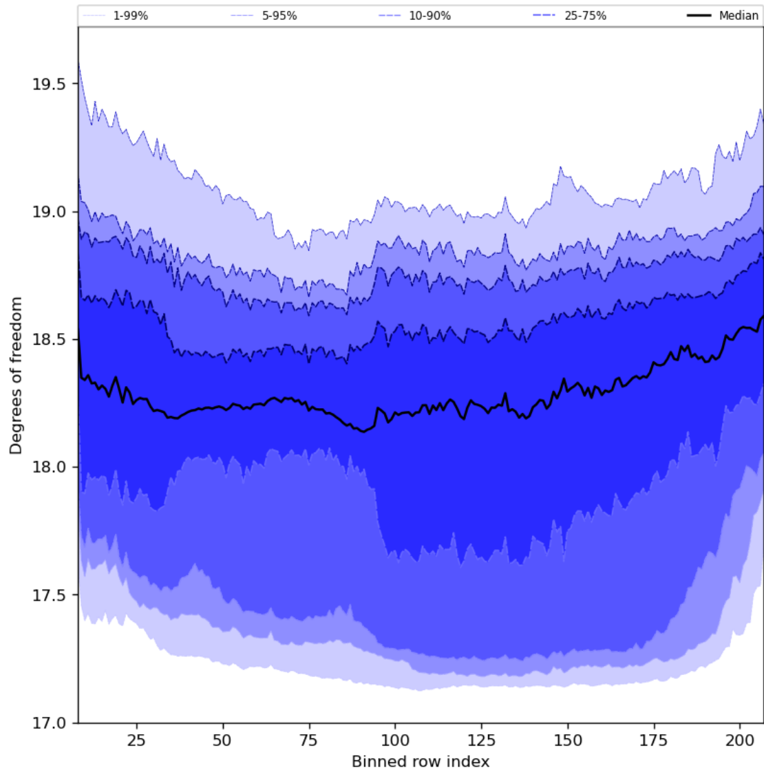
Figure 41: Along track statistics of “Degrees of freedom” for 2023-11-02 to 2023-11-03
