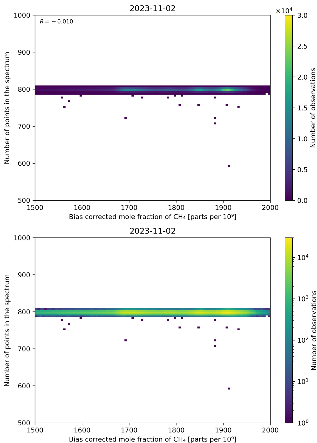
Figure 68: Scatter density plot of “Bias corrected mole fraction of CH 4 ” against “Number of points in the spectrum” for 2023-11-02 to 2023-11-03.
