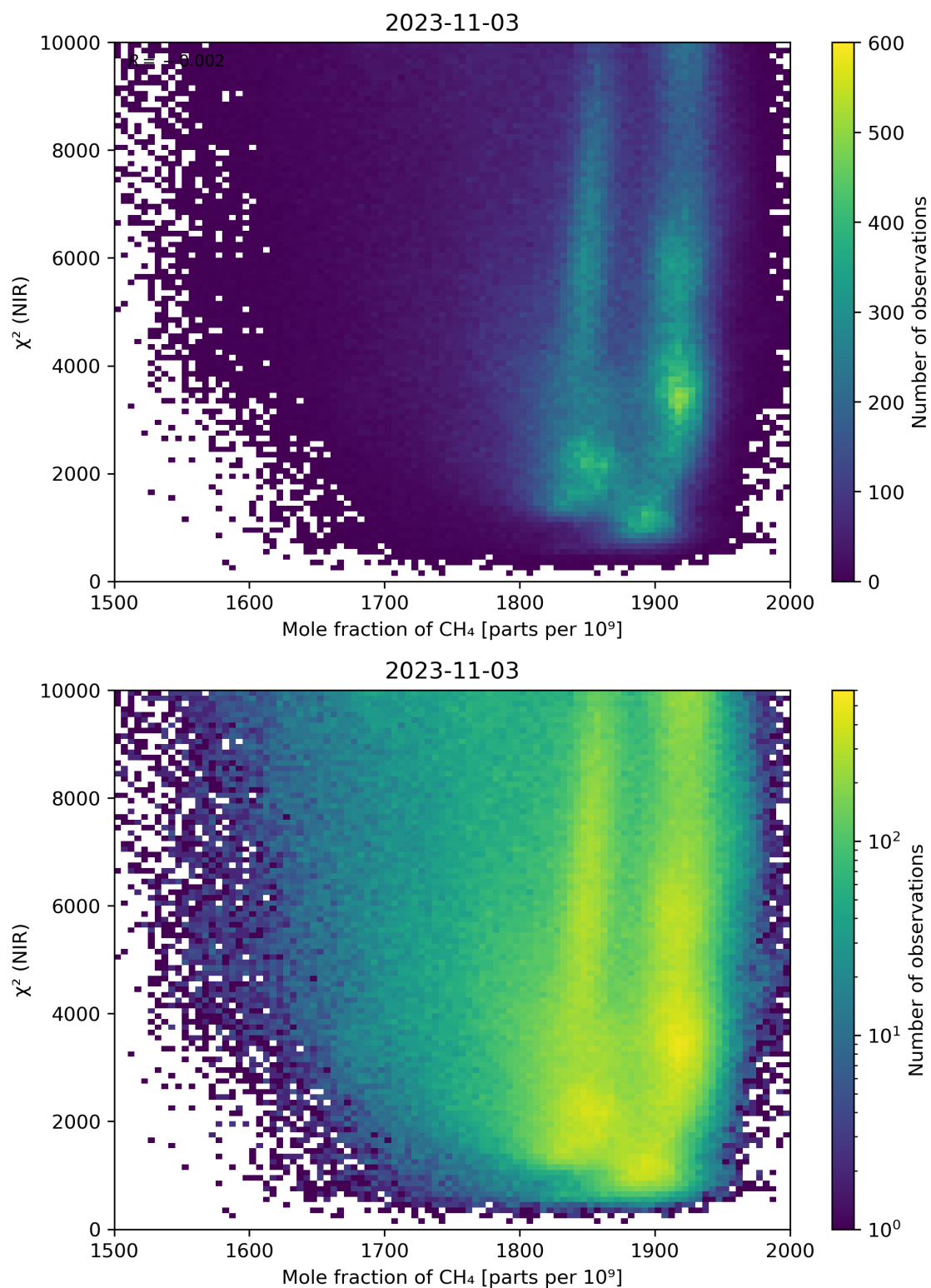
Figure 70: Scatter density plot of “Mole fraction of CH 4 ” against “ \chi^2 (NIR)” for 2023-11-02 to 2023-11-04.
