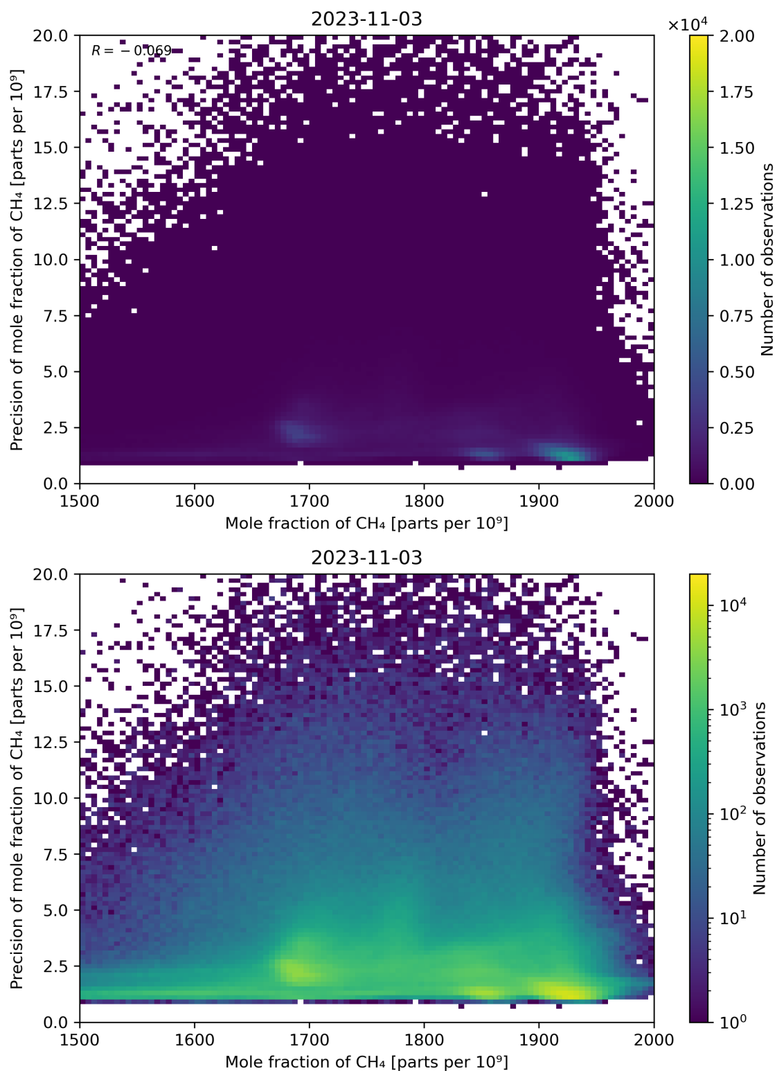
Figure 75: Scatter density plot of “Mole fraction of CH 4 ” against “Precision of mole fraction of CH 4 ” for 2023-11-02 to 2023-11-04.
