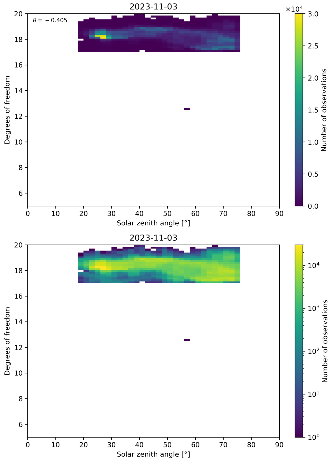
Figure 96: Scatter density plot of “Solar zenith angle” against “Degrees of freedom” for 2023-11-02 to 2023-11-04.
