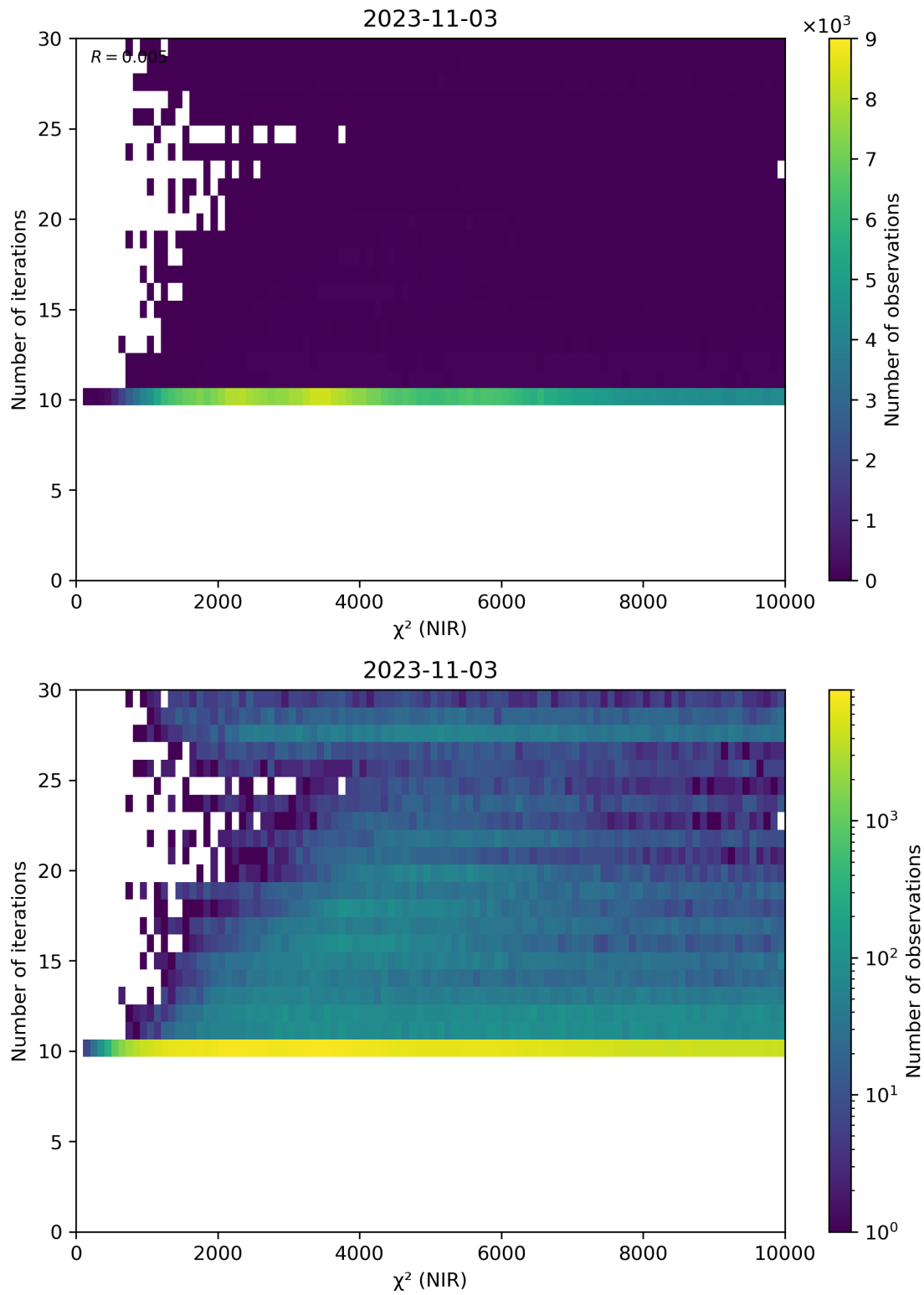
Figure 46: Scatter density plot of “ \chi^2 (NIR)” against “Number of iterations” for 2023-11-02 to 2023-11-04.
