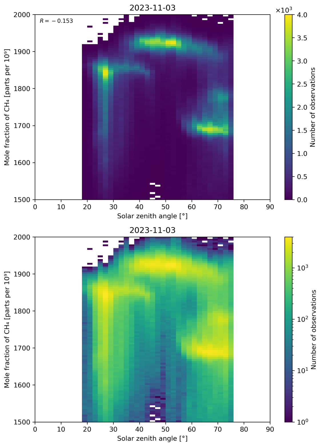
Figure 99: Scatter density plot of “Solar zenith angle” against “Mole fraction of CH 4 ” for 2023-11-02 to 2023-11-04.
