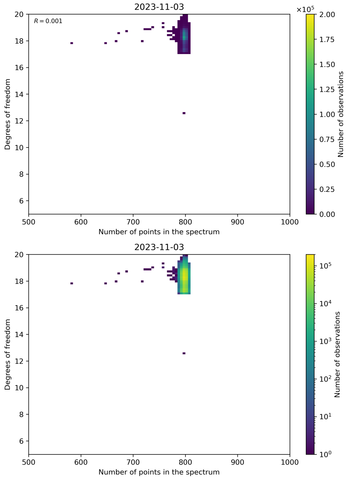
Figure 90: Scatter density plot of “Number of points in the spectrum” against “Degrees of freedom” for 2023-11-02 to 2023-11-04.
