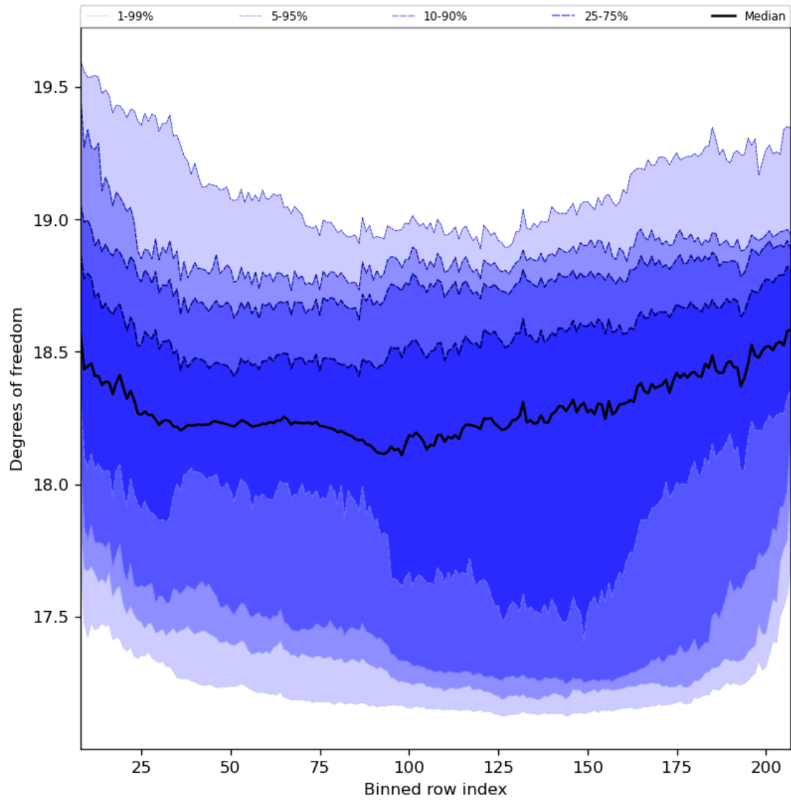
Figure 41: Along track statistics of “Degrees of freedom” for 2023-11-02 to 2023-11-04
