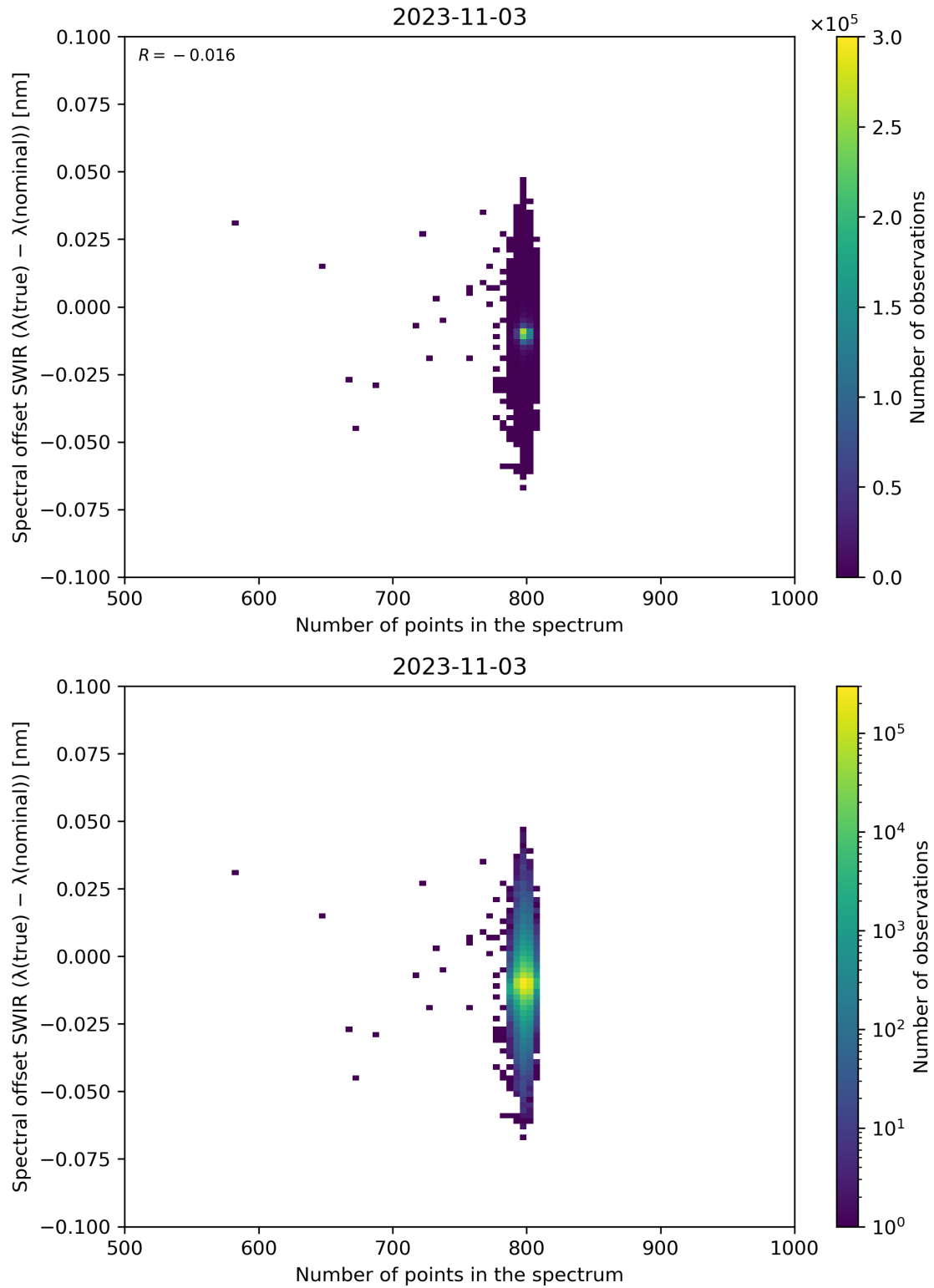
Figure 93: Scatter density plot of “Number of points in the spectrum” against “Spectral offset SWIR ( \lambda(\text{true}) - \lambda(\text{nominal}) )” for 2023-11-02 to 2023-11-04.
