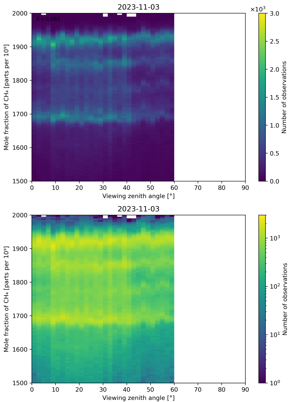
Figure 110: Scatter density plot of “Viewing zenith angle” against “Mole fraction of CH 4 ” for 2023-11-02 to 2023-11-04.
