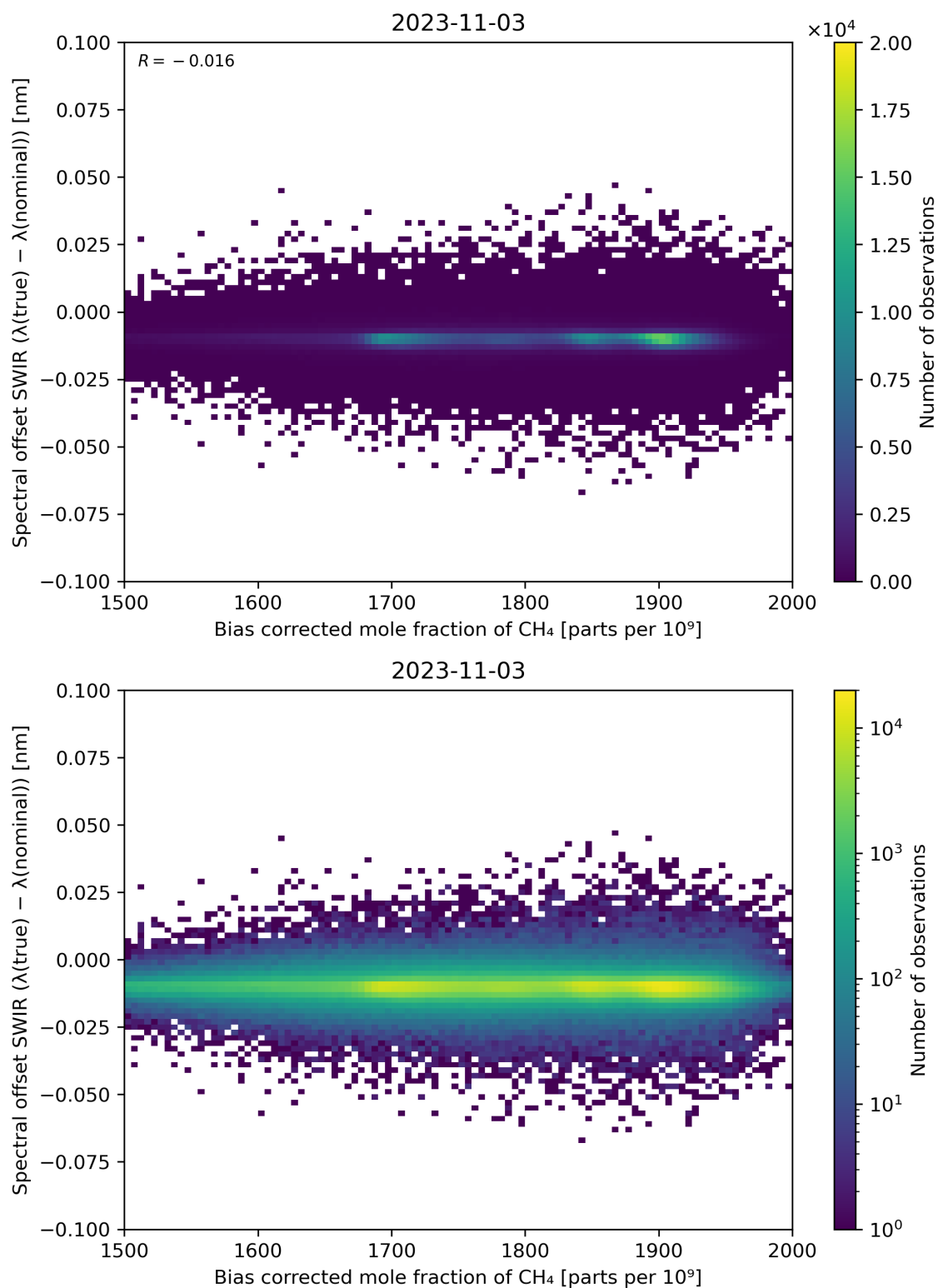
Figure 69: Scatter density plot of “Bias corrected mole fraction of \text{CH}_4 ” against “Spectral offset SWIR ( \lambda(\text{true}) - \lambda(\text{nominal}) )” for 2023-11-02 to 2023-11-04.
