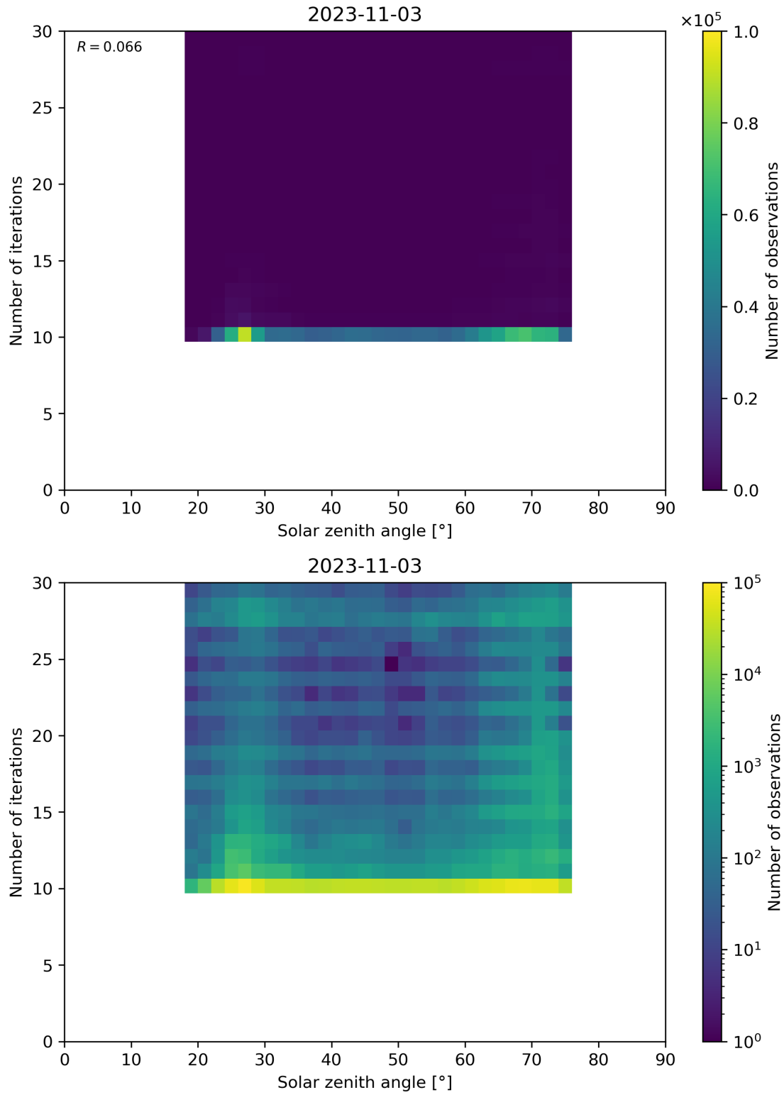
Figure 102: Scatter density plot of “Solar zenith angle” against “Number of iterations” for 2023-11-02 to 2023-11-04.
