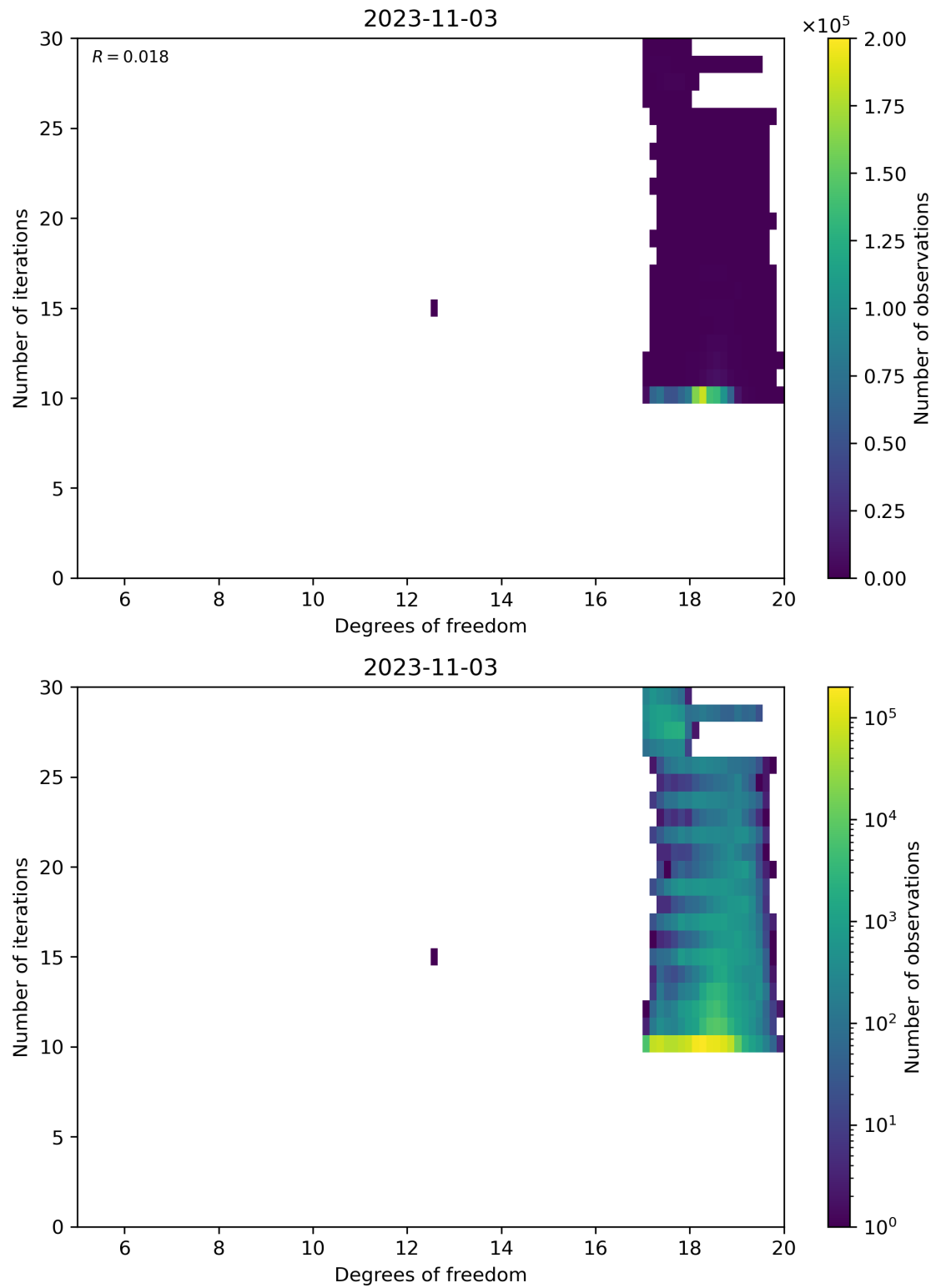
Figure 52: Scatter density plot of “Degrees of freedom” against “Number of iterations” for 2023-11-02 to 2023-11-04.
