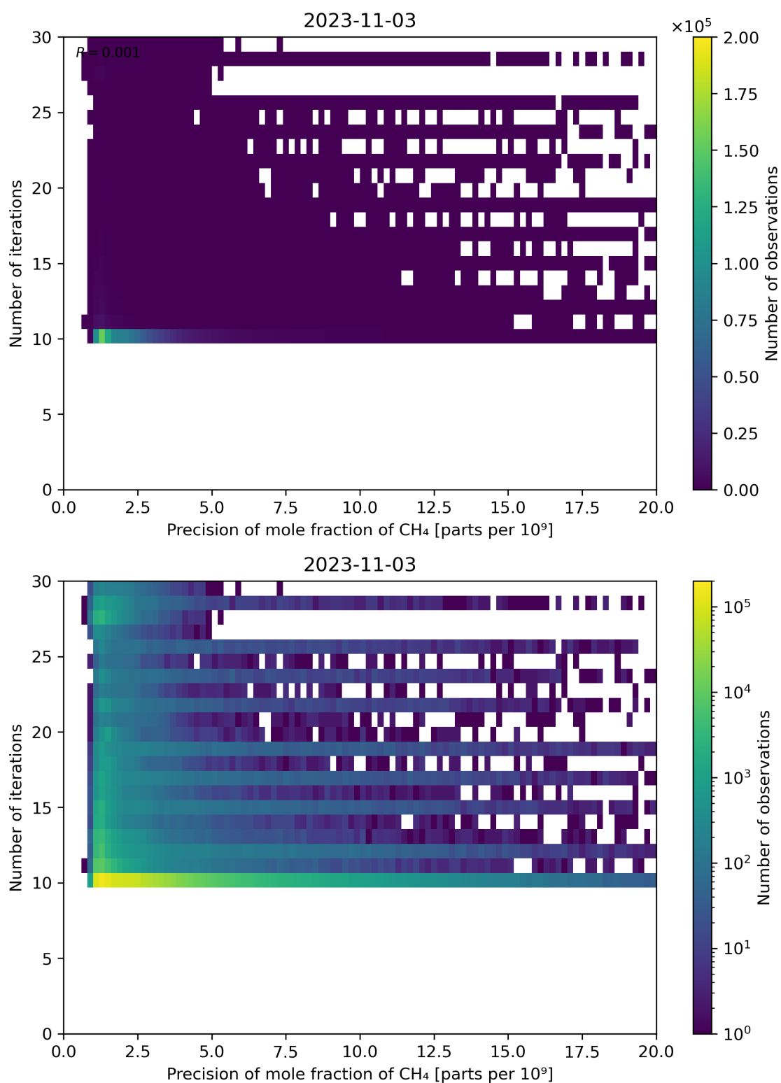
Figure 83: Scatter density plot of “Precision of mole fraction of CH 4 ” against “Number of iterations” for 2023-11-02 to 2023-11-04.
