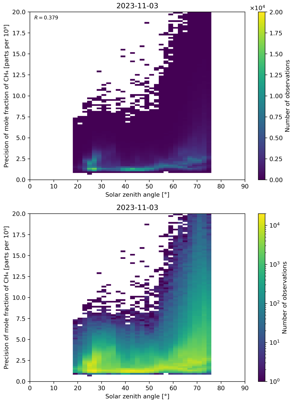
Figure 101: Scatter density plot of “Solar zenith angle” against “Precision of mole fraction of CH 4 ” for 2023-11-02 to 2023-11-04.
