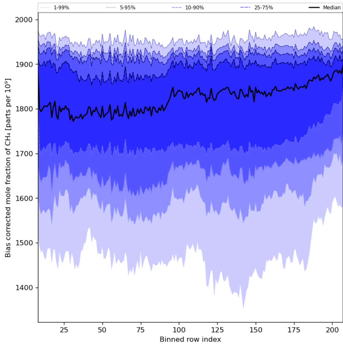
Figure 36: Along track statistics of “Bias corrected mole fraction of CH 4 ” for 2023-11-02 to 2023-11-04
