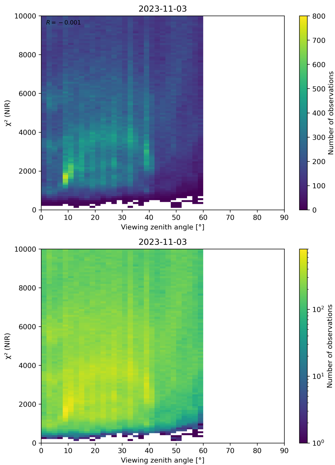
Figure 105: Scatter density plot of “Viewing zenith angle” against “ \chi^2 (NIR)” for 2023-11-02 to 2023-11-04.
