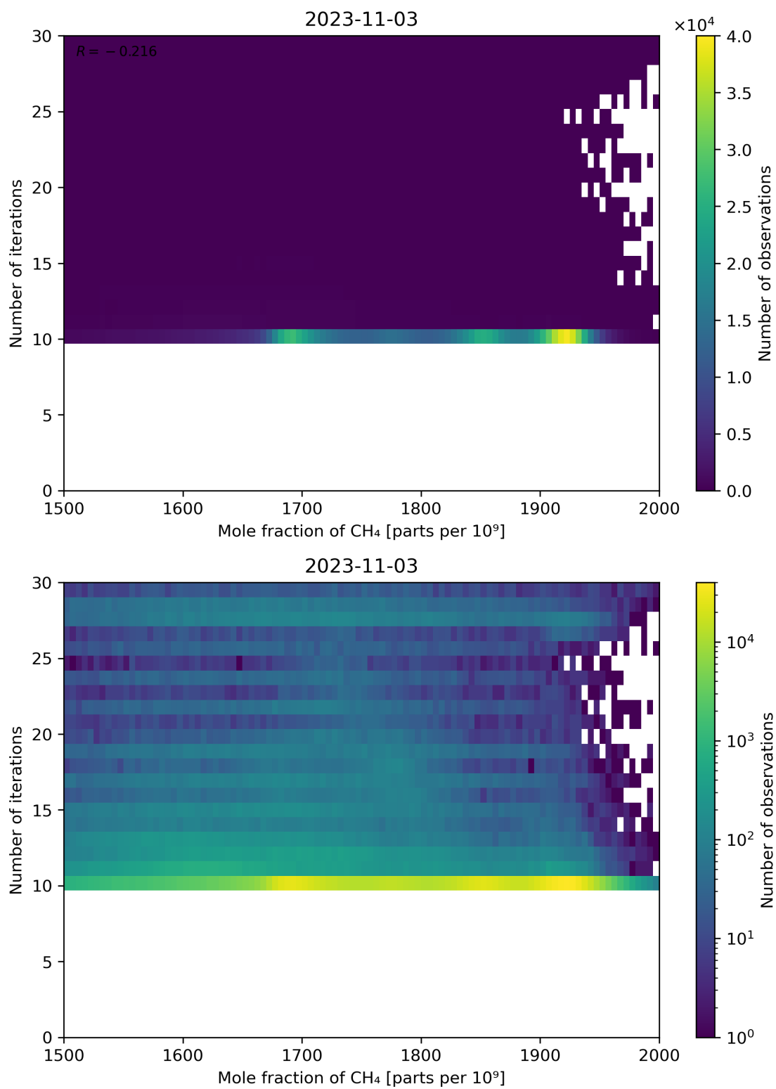
Figure 76: Scatter density plot of “Mole fraction of CH 4 ” against “Number of iterations” for 2023-11-02 to 2023-11-04.
