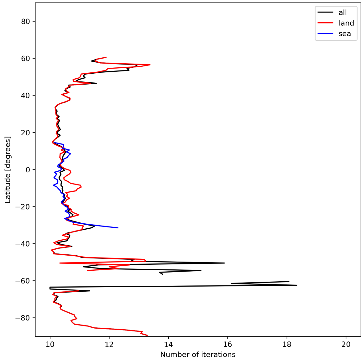
Figure 20: Zonal average of “Number of iterations” for 2023-11-02 to 2023-11-04.
