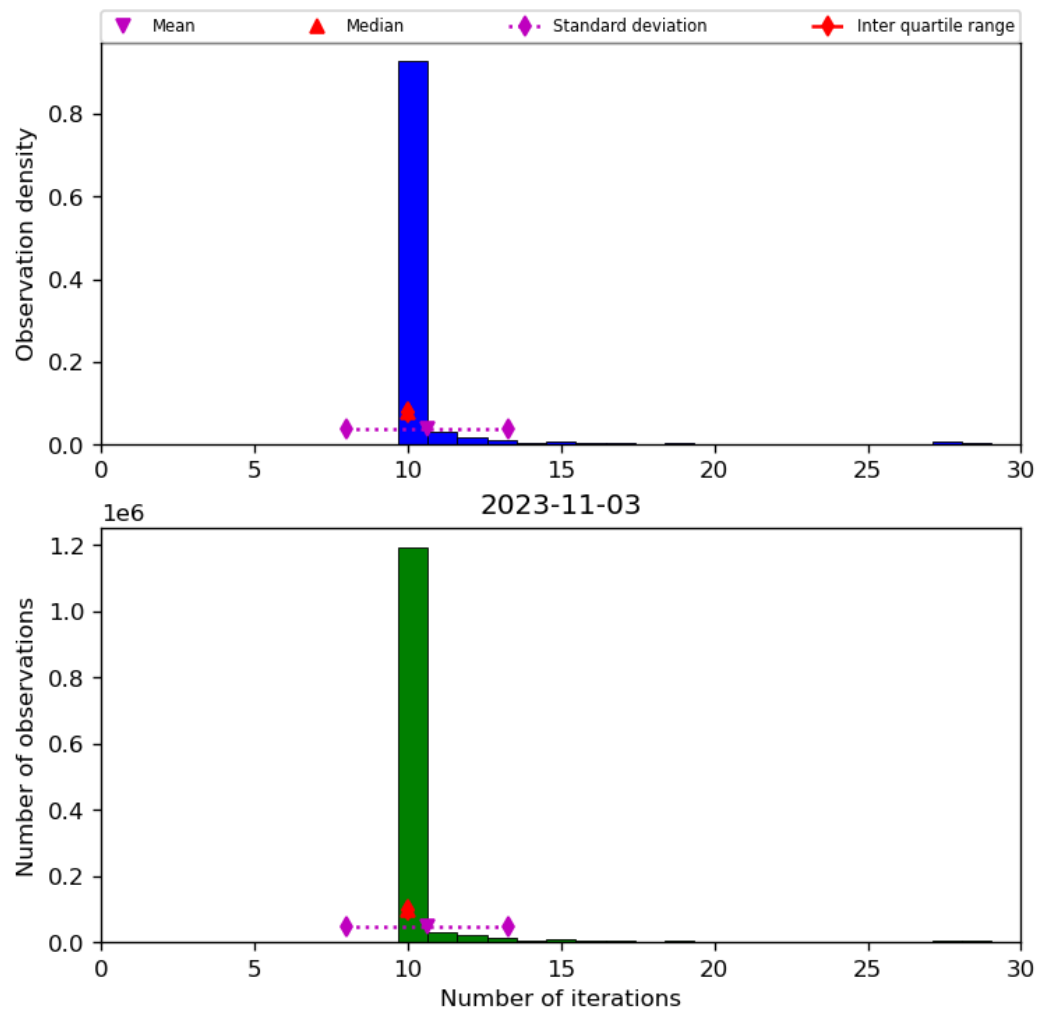
Figure 31: Histogram of “Number of iterations” for 2023-11-02 to 2023-11-04
