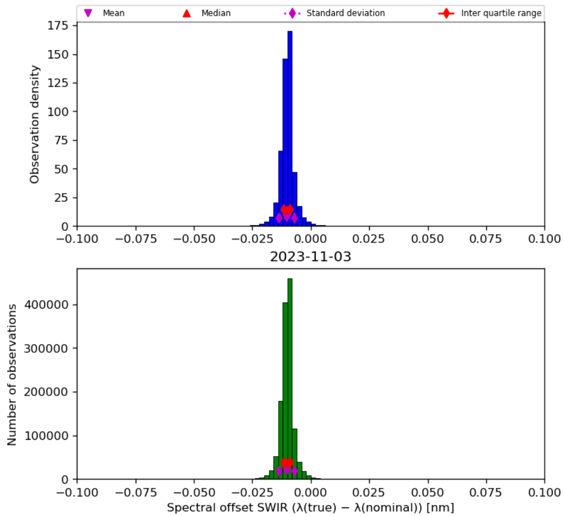
Figure 27: Histogram of “Spectral offset SWIR ( \lambda(\text{true}) - \lambda(\text{nominal}) )” for 2023-11-02 to 2023-11-04
