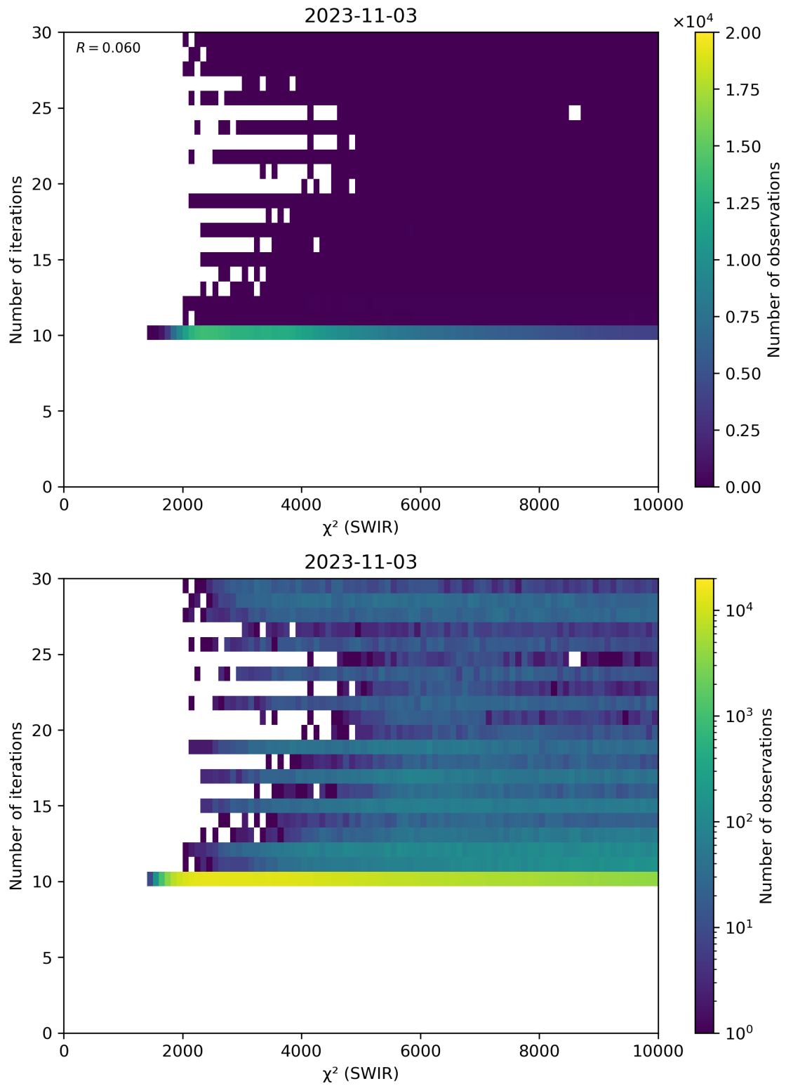
Figure 50: Scatter density plot of “ \chi^2 (SWIR)” against “Number of iterations” for 2023-11-02 to 2023-11-04.
