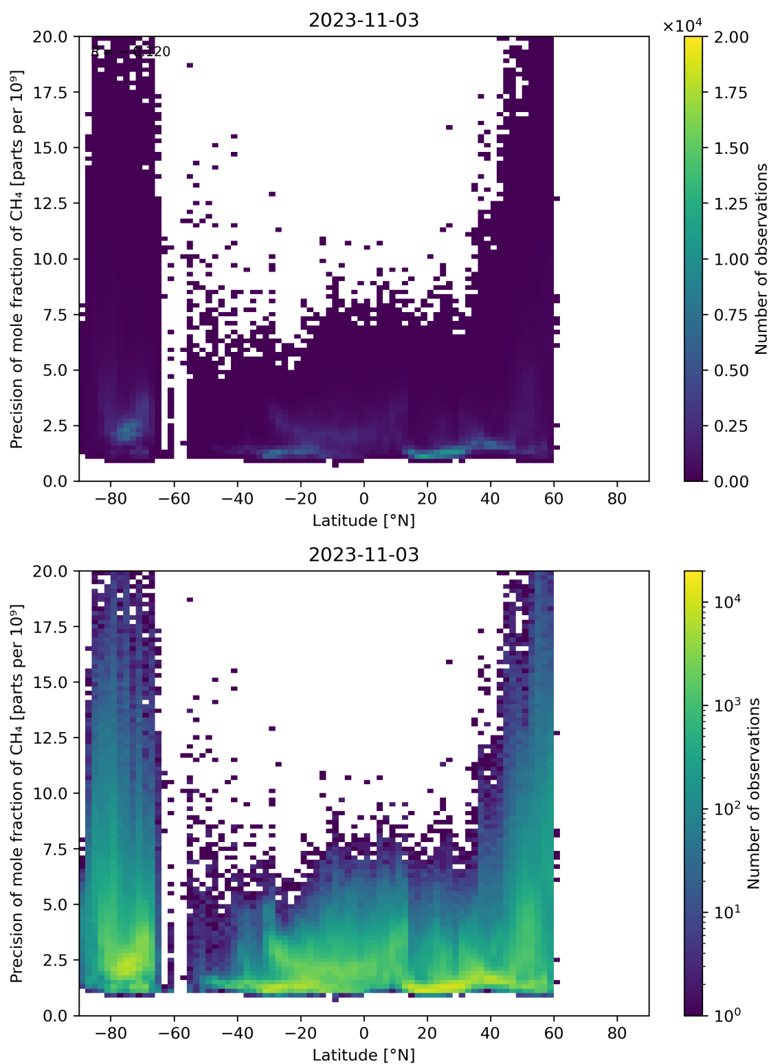
Figure 59: Scatter density plot of “Latitude” against “Precision of mole fraction of CH 4 ” for 2023-11-02 to 2023-11-04.
