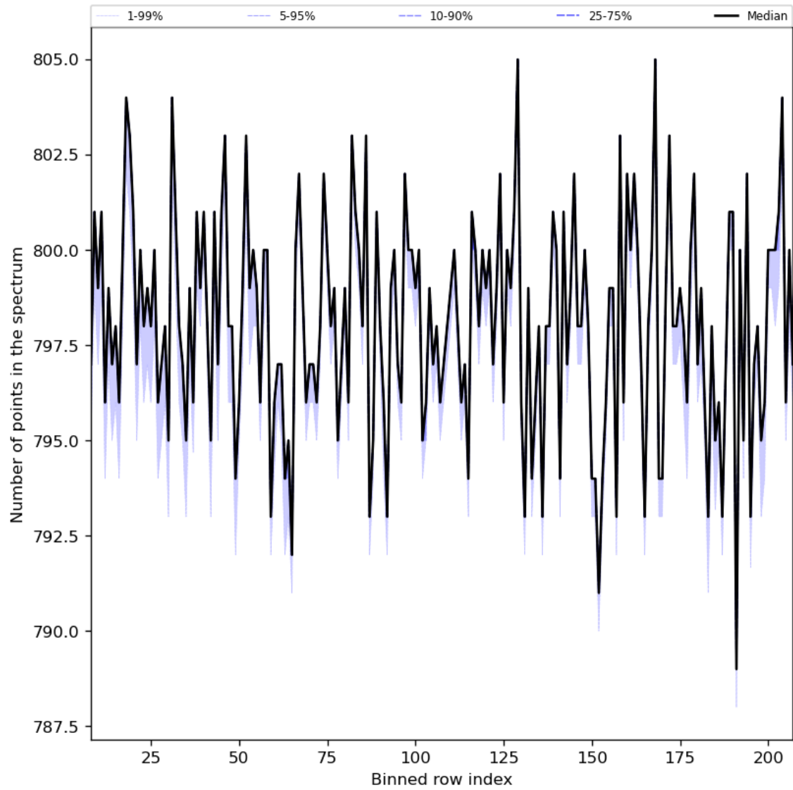
Figure 37: Along track statistics of “Number of points in the spectrum” for 2023-11-02 to 2023-11-04
