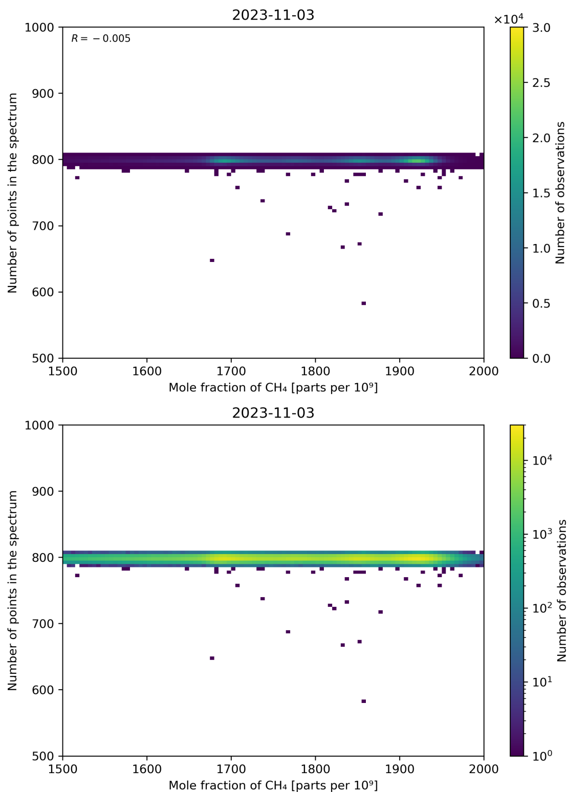
Figure 77: Scatter density plot of “Mole fraction of CH 4 ” against “Number of points in the spectrum” for 2023-11-02 to 2023-11-04.
