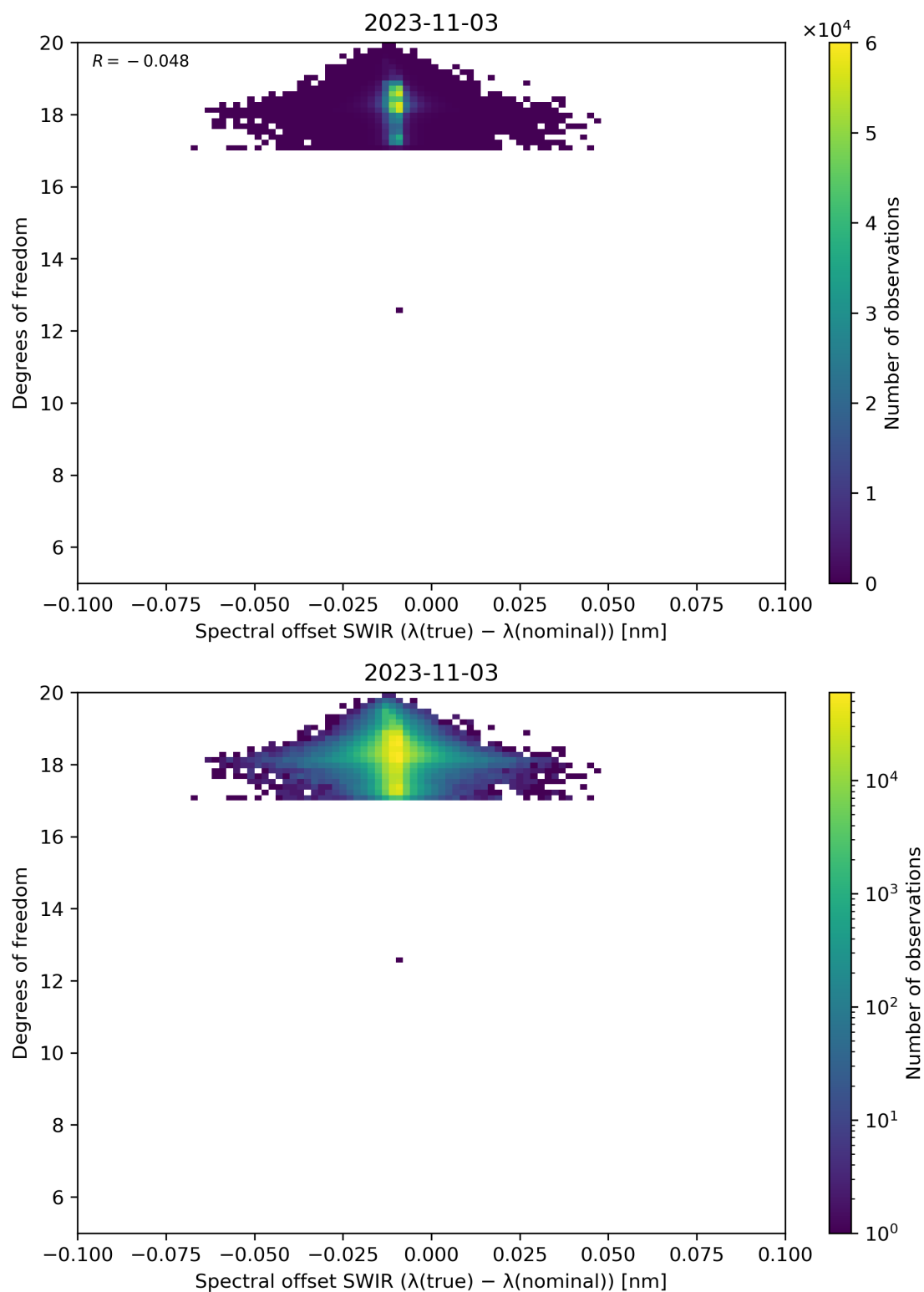
Figure 119: Scatter density plot of “Spectral offset SWIR ( \lambda(\text{true}) - \lambda(\text{nominal}) )” against “Degrees of freedom” for 2023-11-02 to 2023-11-04.
