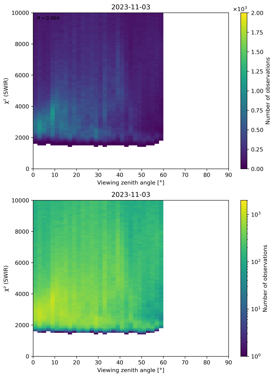
Figure 106: Scatter density plot of “Viewing zenith angle” against “ \chi^2 (SWIR)” for 2023-11-02 to 2023-11-04.
