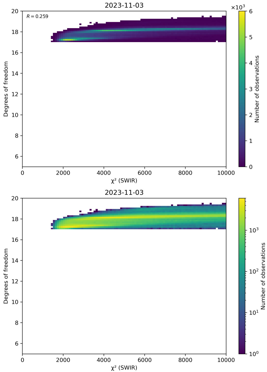
Figure 48: Scatter density plot of “ \chi^2 (SWIR)” against “Degrees of freedom” for 2023-11-02 to 2023-11-04.
