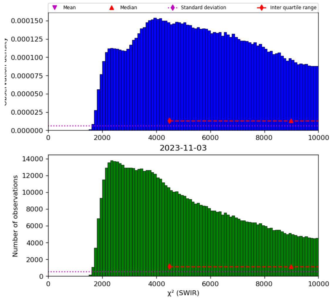
Figure 28: Histogram of “ \chi^2 (SWIR)” for 2023-11-02 to 2023-11-04
