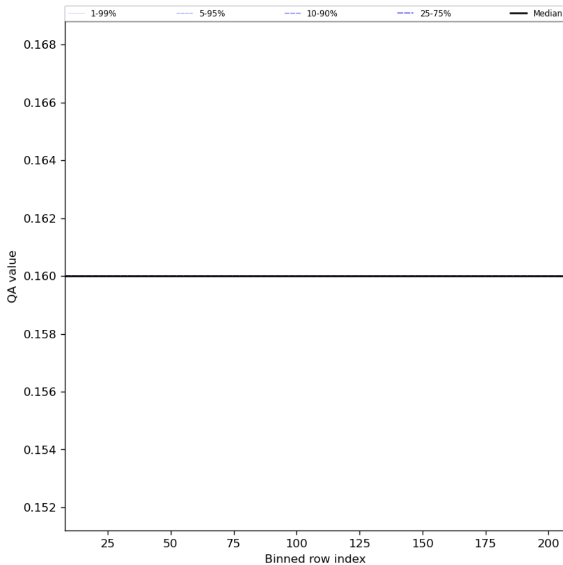
Figure 33: Along track statistics of “QA value” for 2023-11-02 to 2023-11-04
