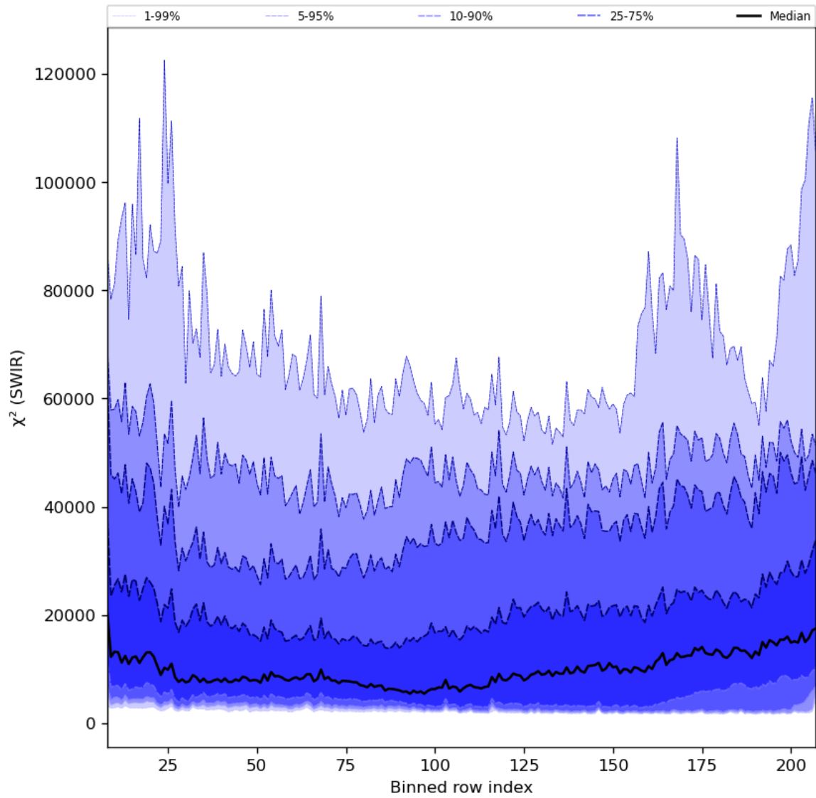
Figure 39: Along track statistics of “ \chi^2 (SWIR)” for 2023-11-02 to 2023-11-04
