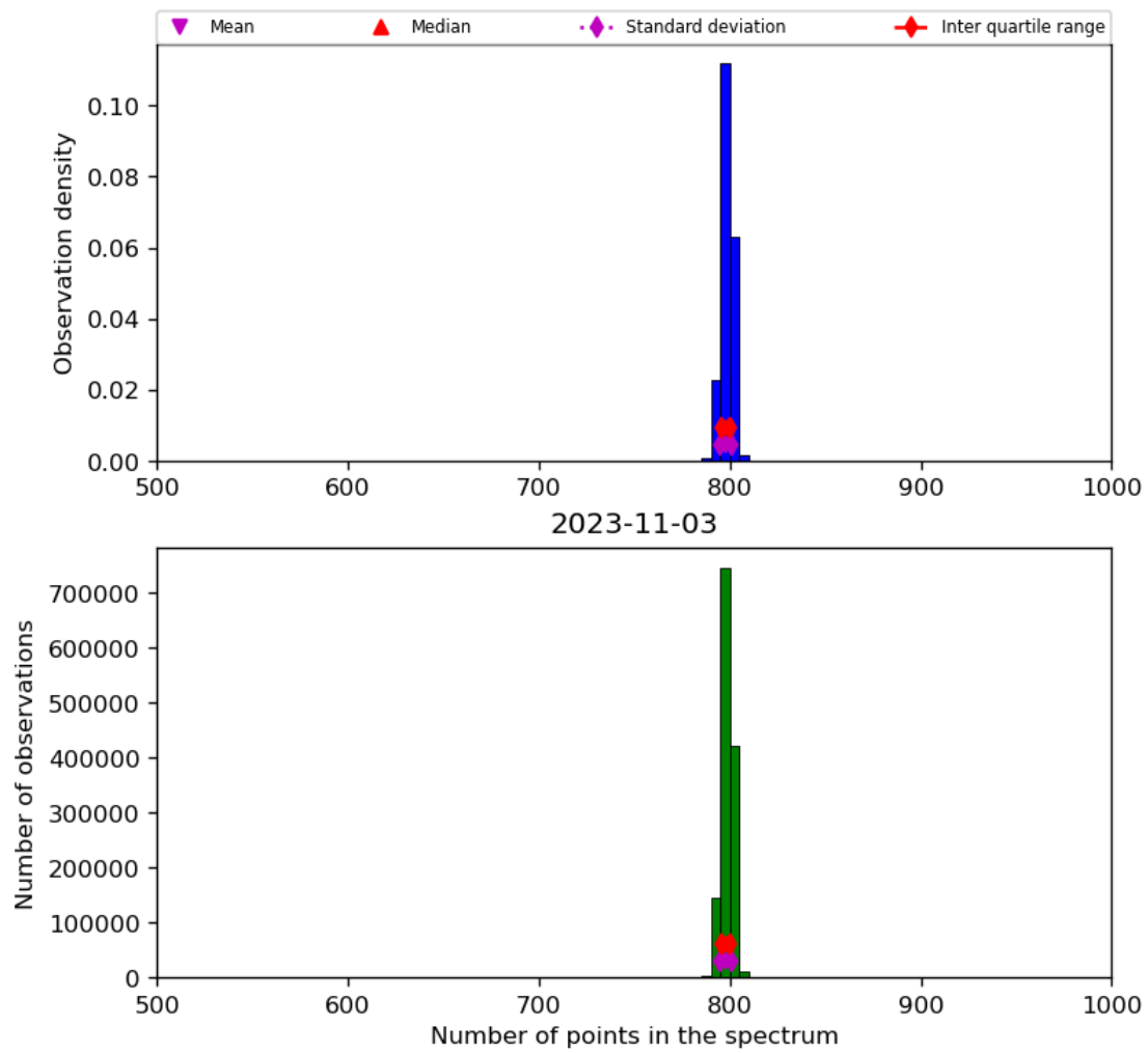
Figure 26: Histogram of “Number of points in the spectrum” for 2023-11-02 to 2023-11-04
