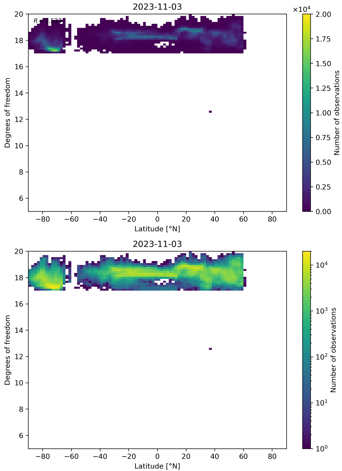
Figure 55: Scatter density plot of “Latitude” against “Degrees of freedom” for 2023-11-02 to 2023-11-04.
