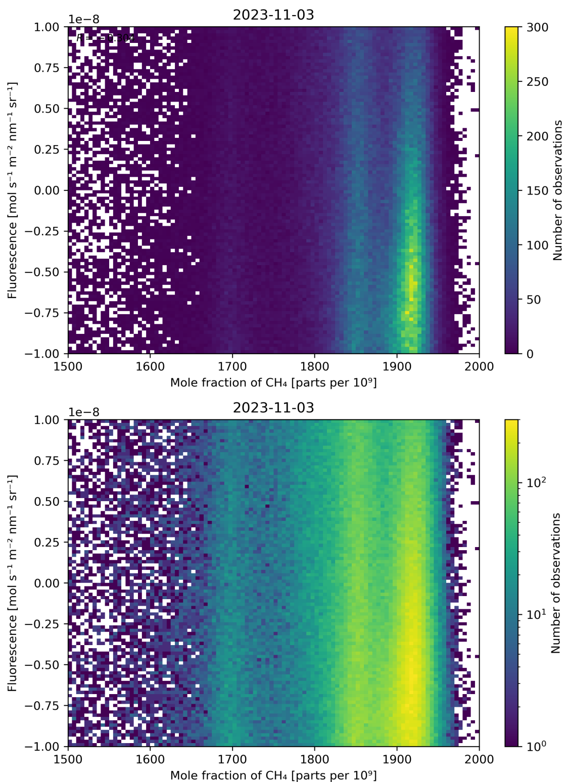
Figure 73: Scatter density plot of “Mole fraction of \text{CH}_4 ” against “Fluorescence” for 2023-11-02 to 2023-11-04.
