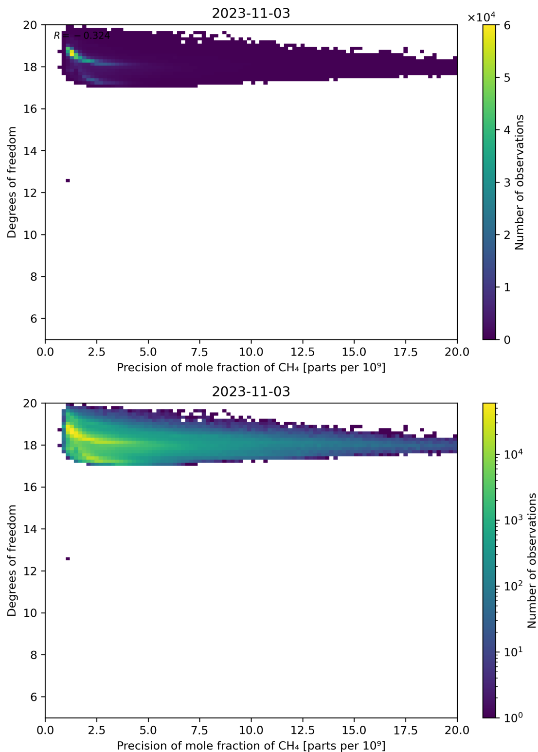
Figure 80: Scatter density plot of “Precision of mole fraction of CH 4 ” against “Degrees of freedom” for 2023-11-02 to 2023-11-04.
