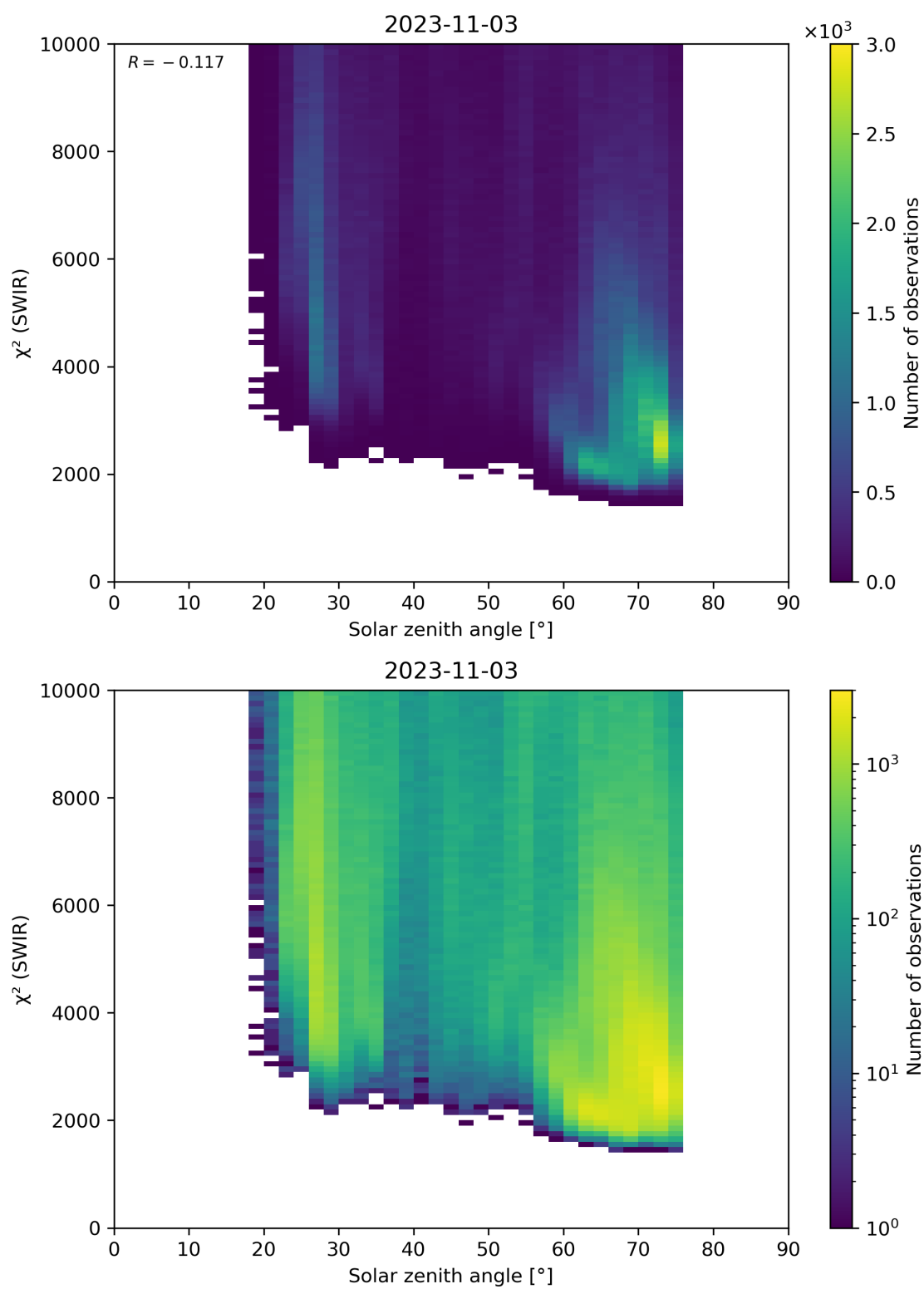
Figure 95: Scatter density plot of “Solar zenith angle” against “ \chi^2 (SWIR)” for 2023-11-02 to 2023-11-04.
