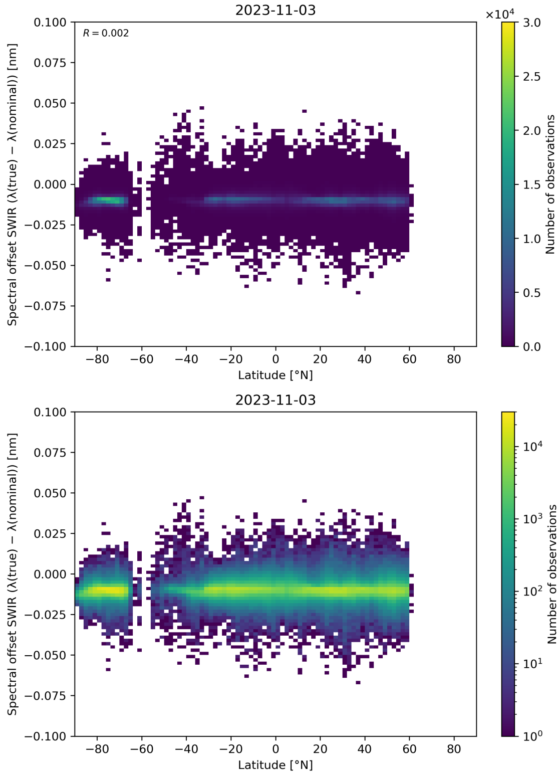
Figure 62: Scatter density plot of “Latitude” against “Spectral offset SWIR ( \lambda(\text{true}) - \lambda(\text{nominal}) )” for 2023-11-02 to 2023-11-04.
