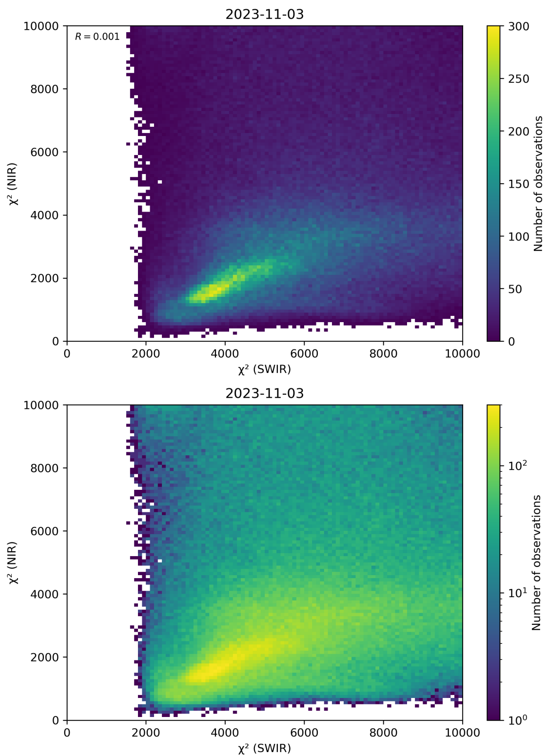
Figure 47: Scatter density plot of “ \chi^2 (SWIR)” against “ \chi^2 (NIR)” for 2023-11-02 to 2023-11-04.
