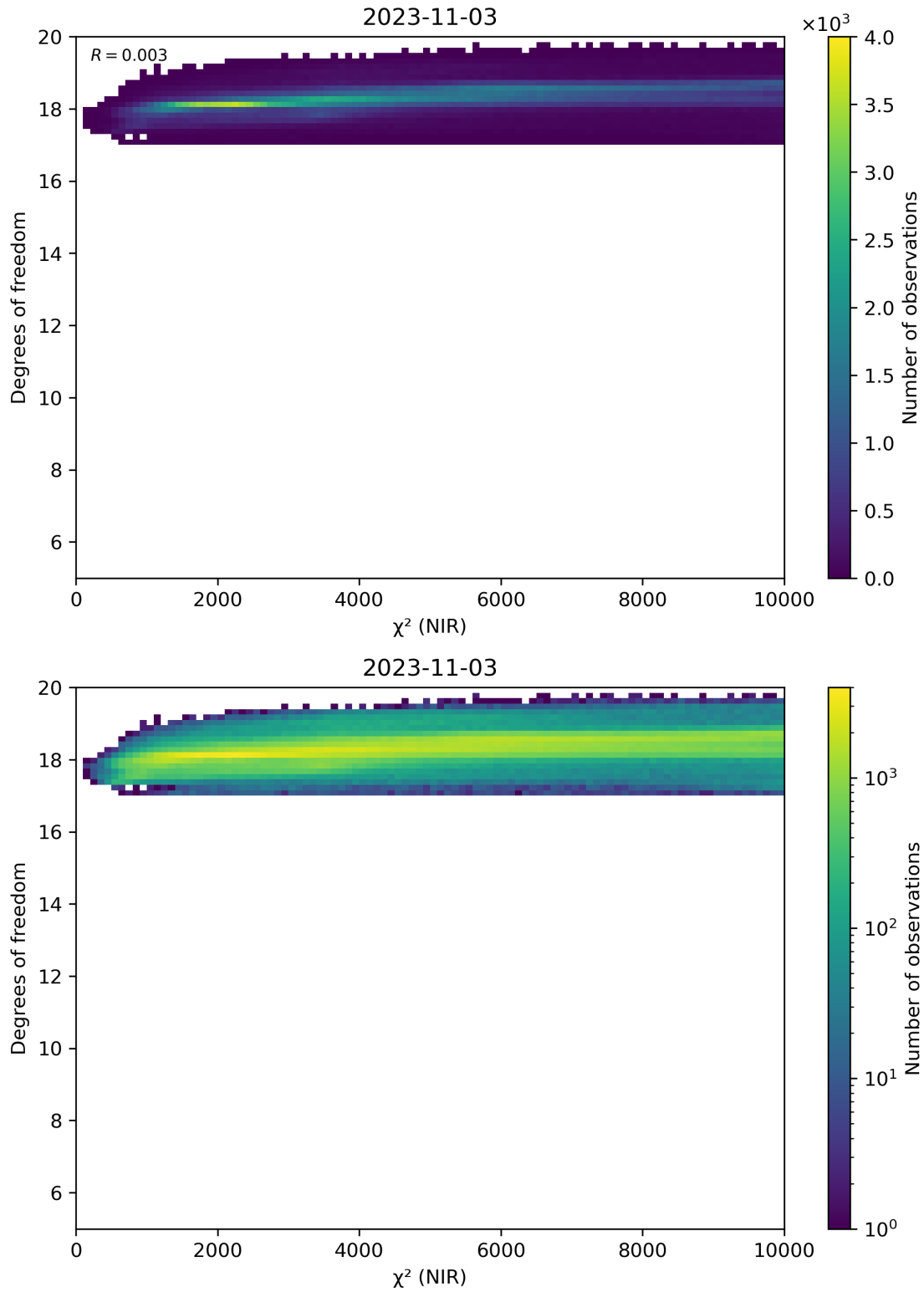
Figure 44: Scatter density plot of “ \chi^2 (NIR)” against “Degrees of freedom” for 2023-11-02 to 2023-11-04.
