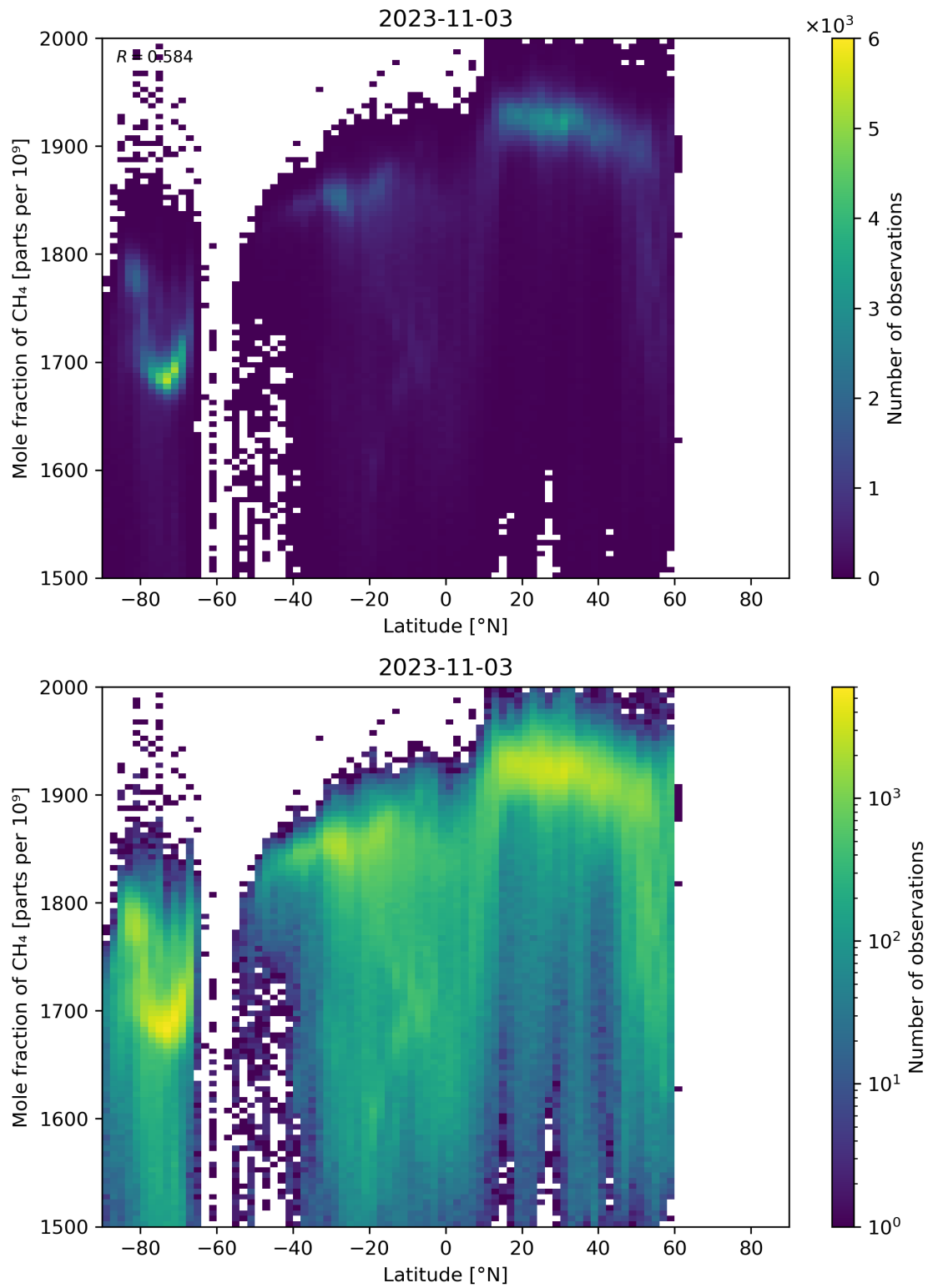
Figure 57: Scatter density plot of “Latitude” against “Mole fraction of CH 4 ” for 2023-11-02 to 2023-11-04.
