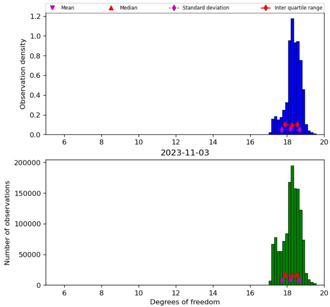
Figure 30: Histogram of “Degrees of freedom” for 2023-11-02 to 2023-11-04
