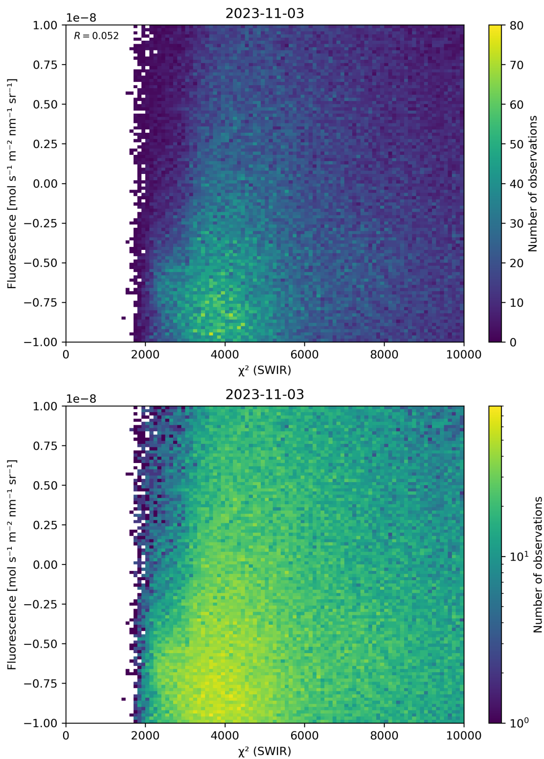
Figure 49: Scatter density plot of “ \chi^2 (SWIR)” against “Fluorescence” for 2023-11-02 to 2023-11-04.
