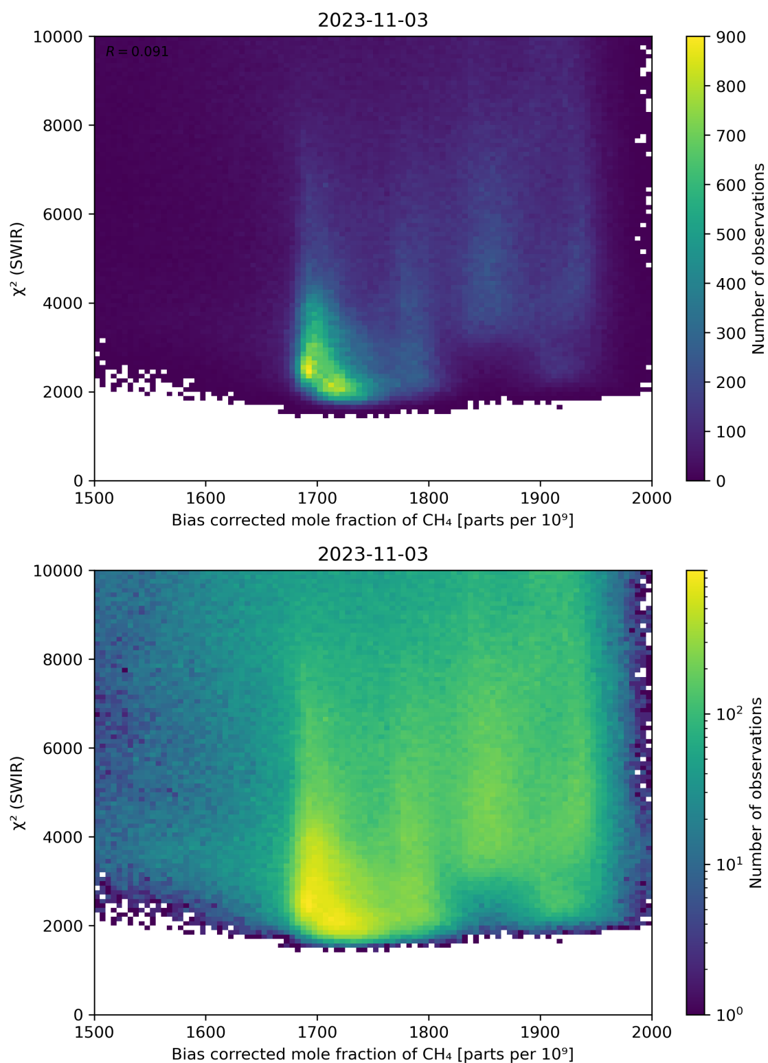
Figure 64: Scatter density plot of “Bias corrected mole fraction of \text{CH}_4 ” against “ \chi^2 (SWIR)” for 2023-11-02 to 2023-11-04.
