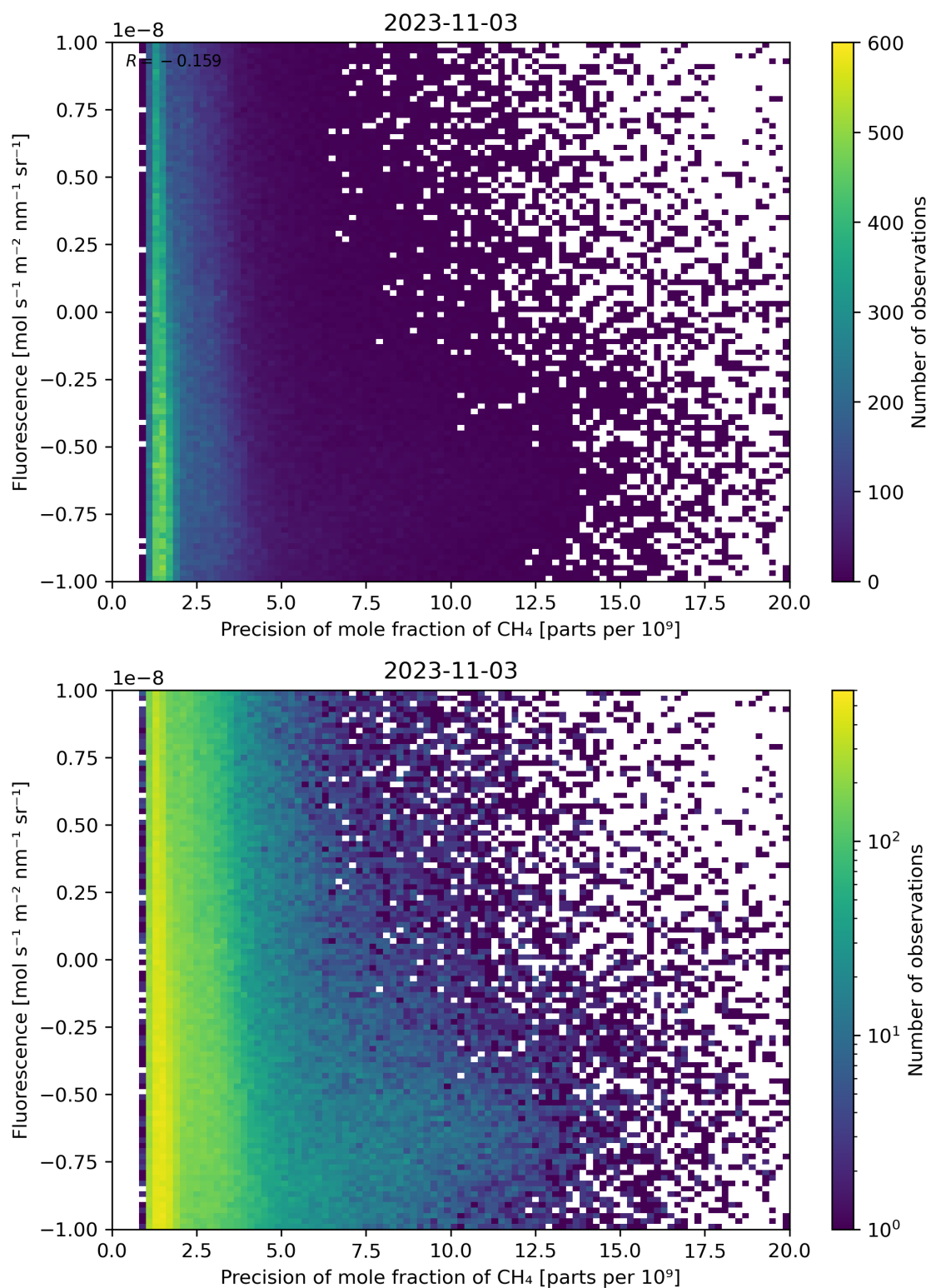
Figure 81: Scatter density plot of “Precision of mole fraction of \text{CH}_4 ” against “Fluorescence” for 2023-11-02 to 2023-11-04.
