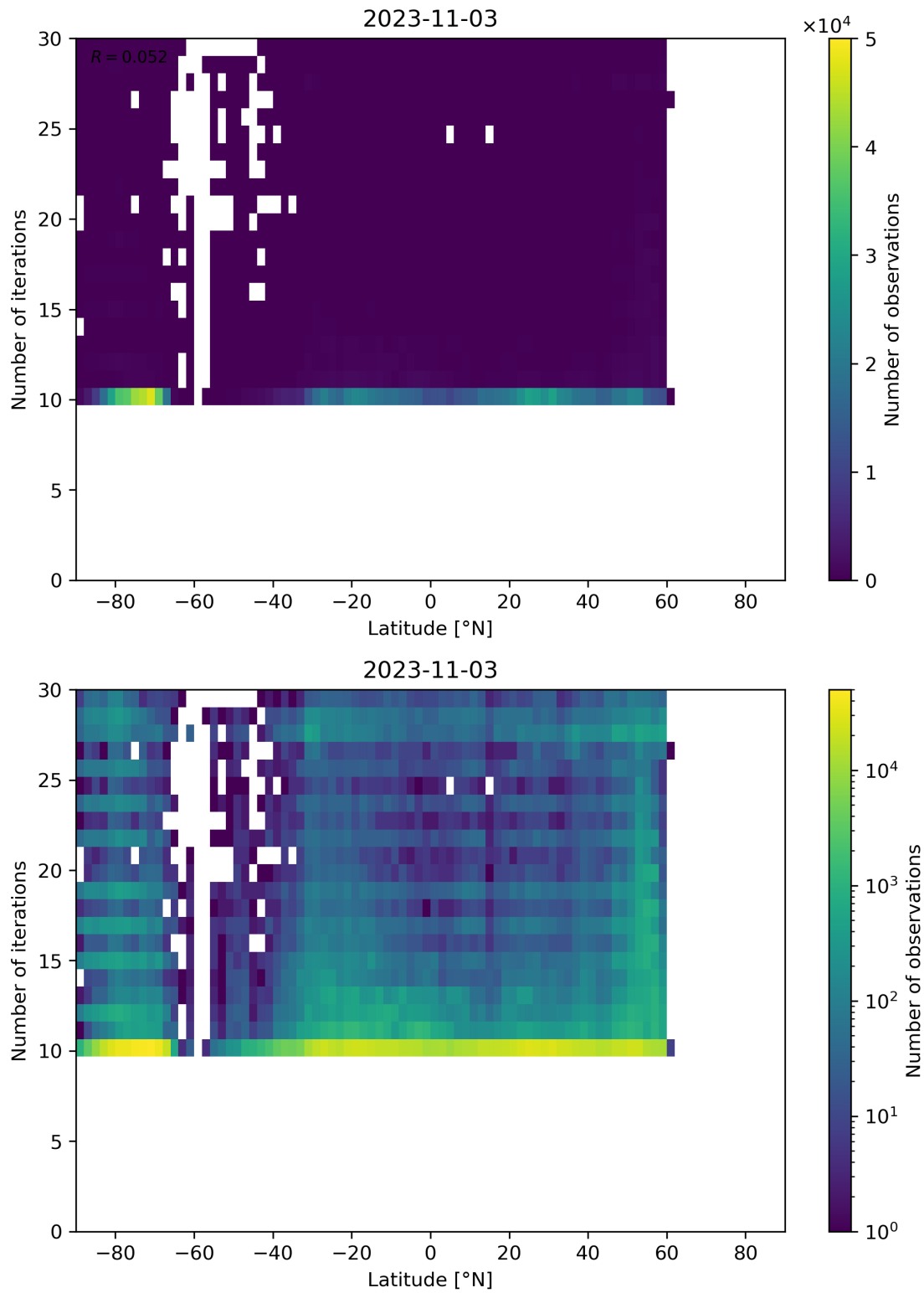
Figure 60: Scatter density plot of “Latitude” against “Number of iterations” for 2023-11-02 to 2023-11-04.
