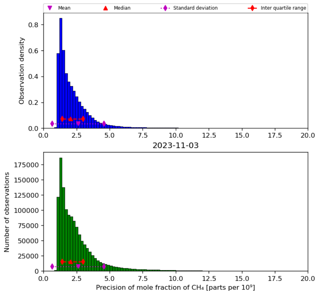
Figure 24: Histogram of “Precision of mole fraction of CH 4 ” for 2023-11-02 to 2023-11-04
