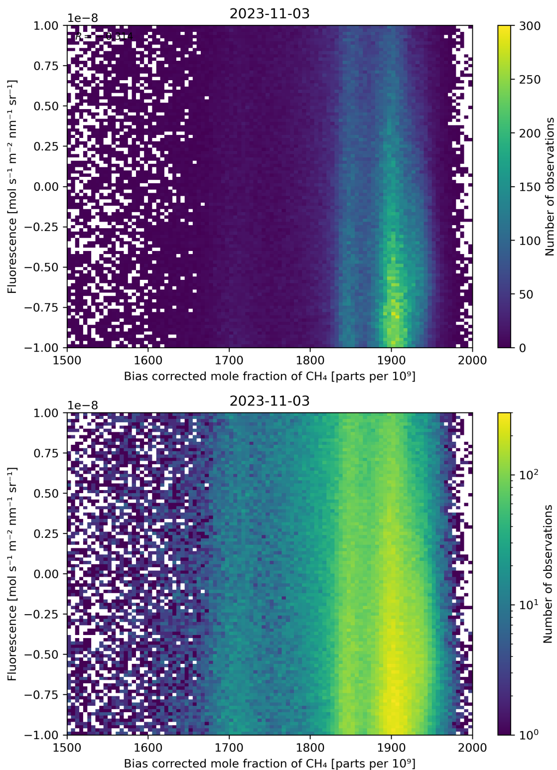
Figure 66: Scatter density plot of “Bias corrected mole fraction of \text{CH}_4 ” against “Fluorescence” for 2023-11-02 to 2023-11-04.
