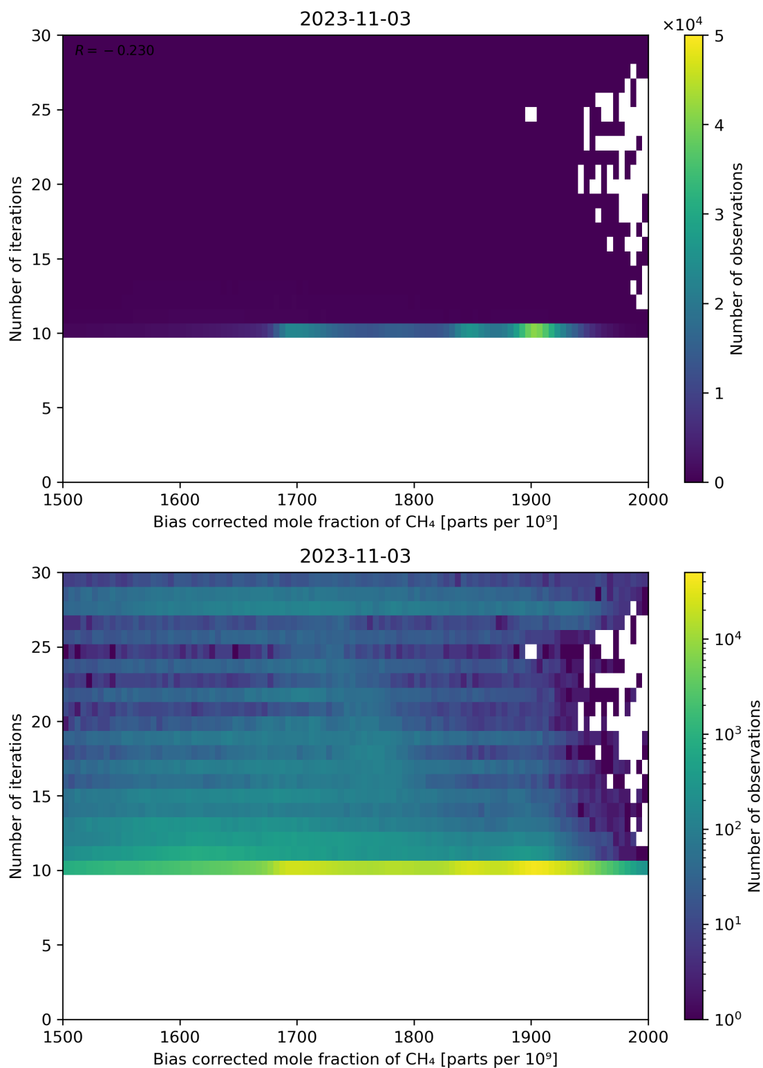
Figure 67: Scatter density plot of “Bias corrected mole fraction of \text{CH}_4 ” against “Number of iterations” for 2023-11-02 to 2023-11-04.
