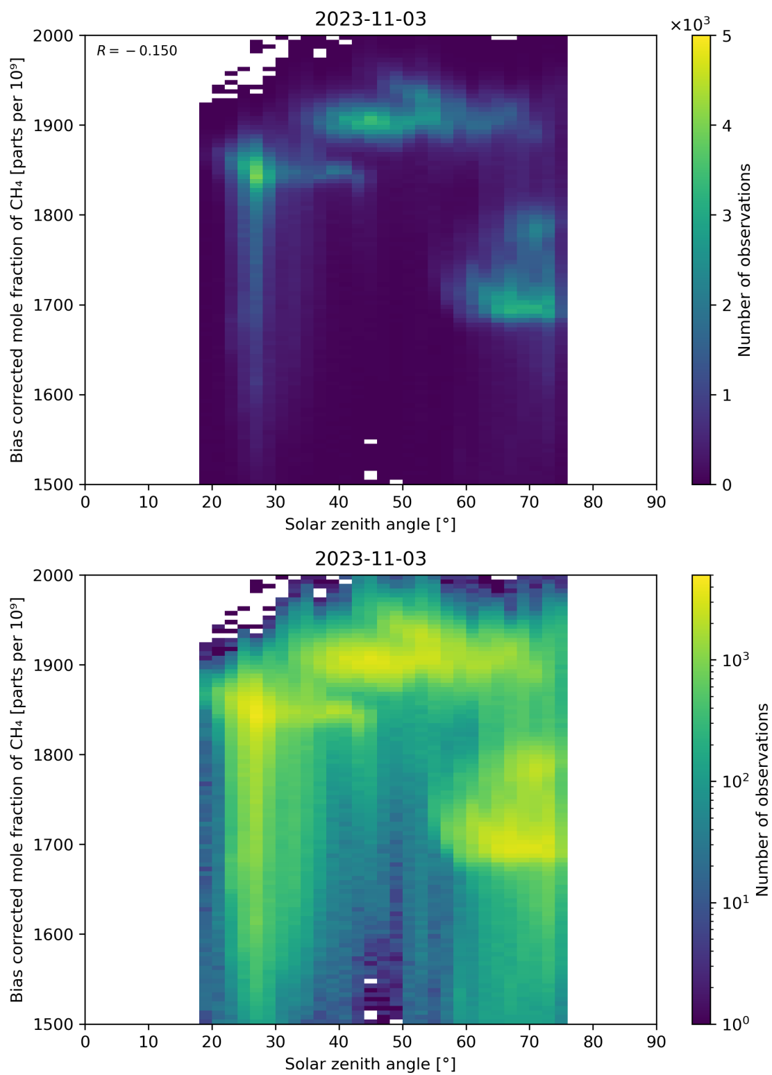
Figure 100: Scatter density plot of “Solar zenith angle” against “Bias corrected mole fraction of CH 4 ” for 2023-11-02 to 2023-11-04.
