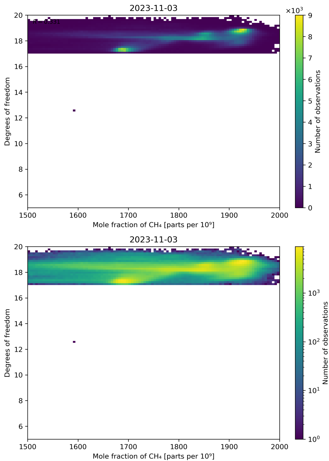
Figure 72: Scatter density plot of “Mole fraction of CH 4 ” against “Degrees of freedom” for 2023-11-02 to 2023-11-04.
