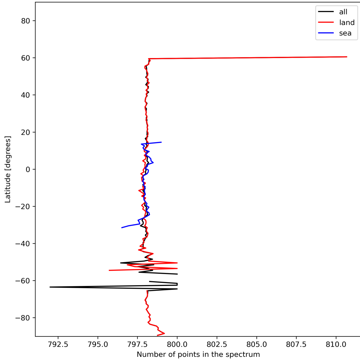
Figure 15: Zonal average of “Number of points in the spectrum” for 2023-11-02 to 2023-11-04.
