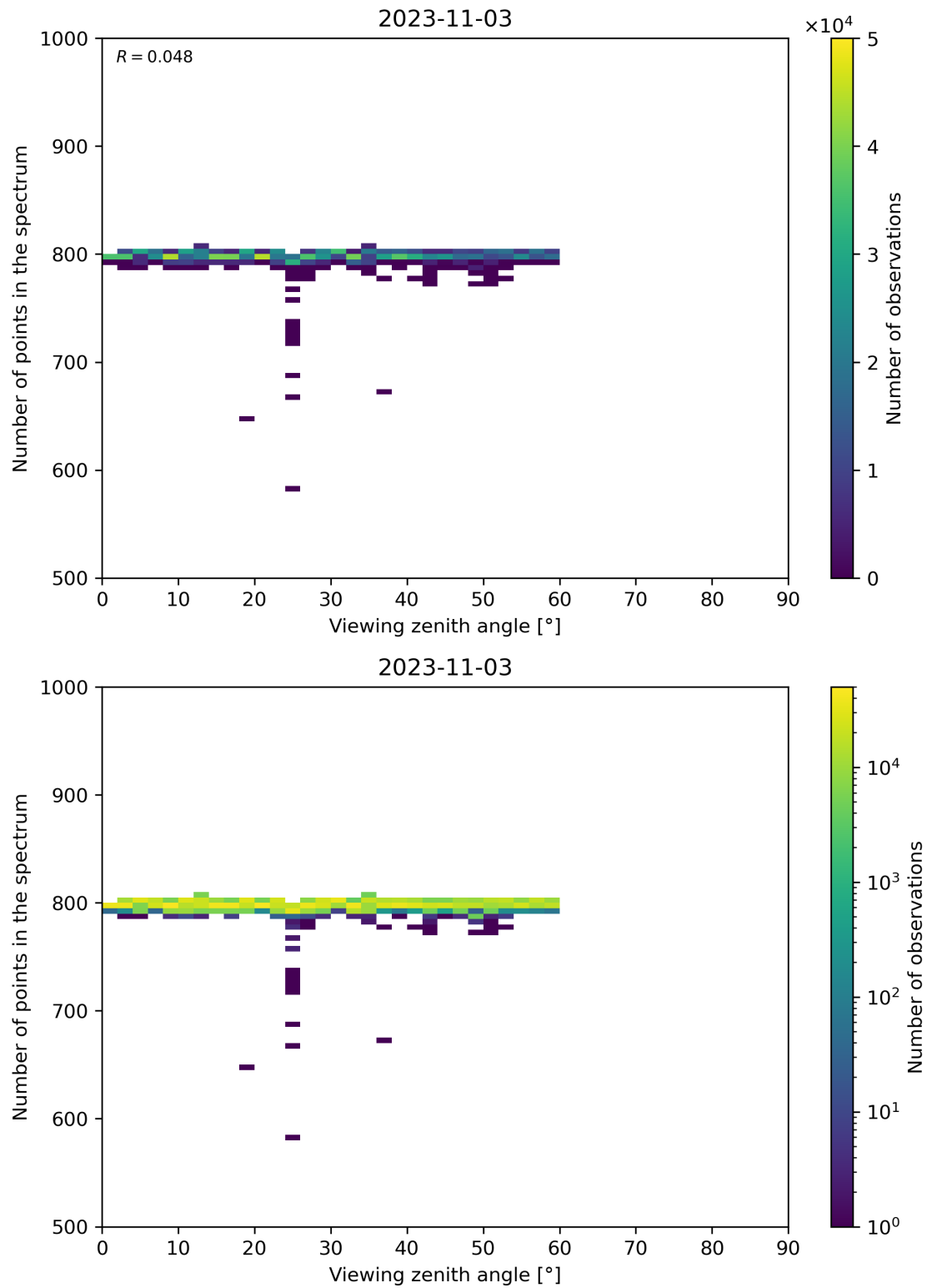
Figure 114: Scatter density plot of “Viewing zenith angle” against “Number of points in the spectrum” for 2023-11-02 to 2023-11-04.
