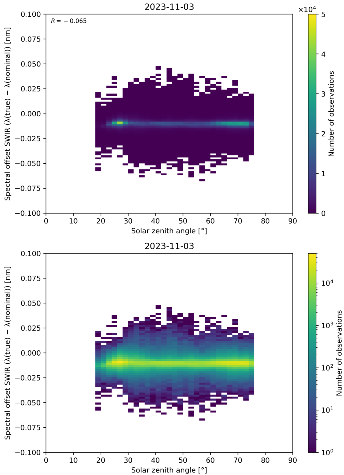
Figure 104: Scatter density plot of “Solar zenith angle” against “Spectral offset SWIR ( \lambda(\text{true}) - \lambda(\text{nominal}) )” for 2023-11-02 to 2023-11-04.
