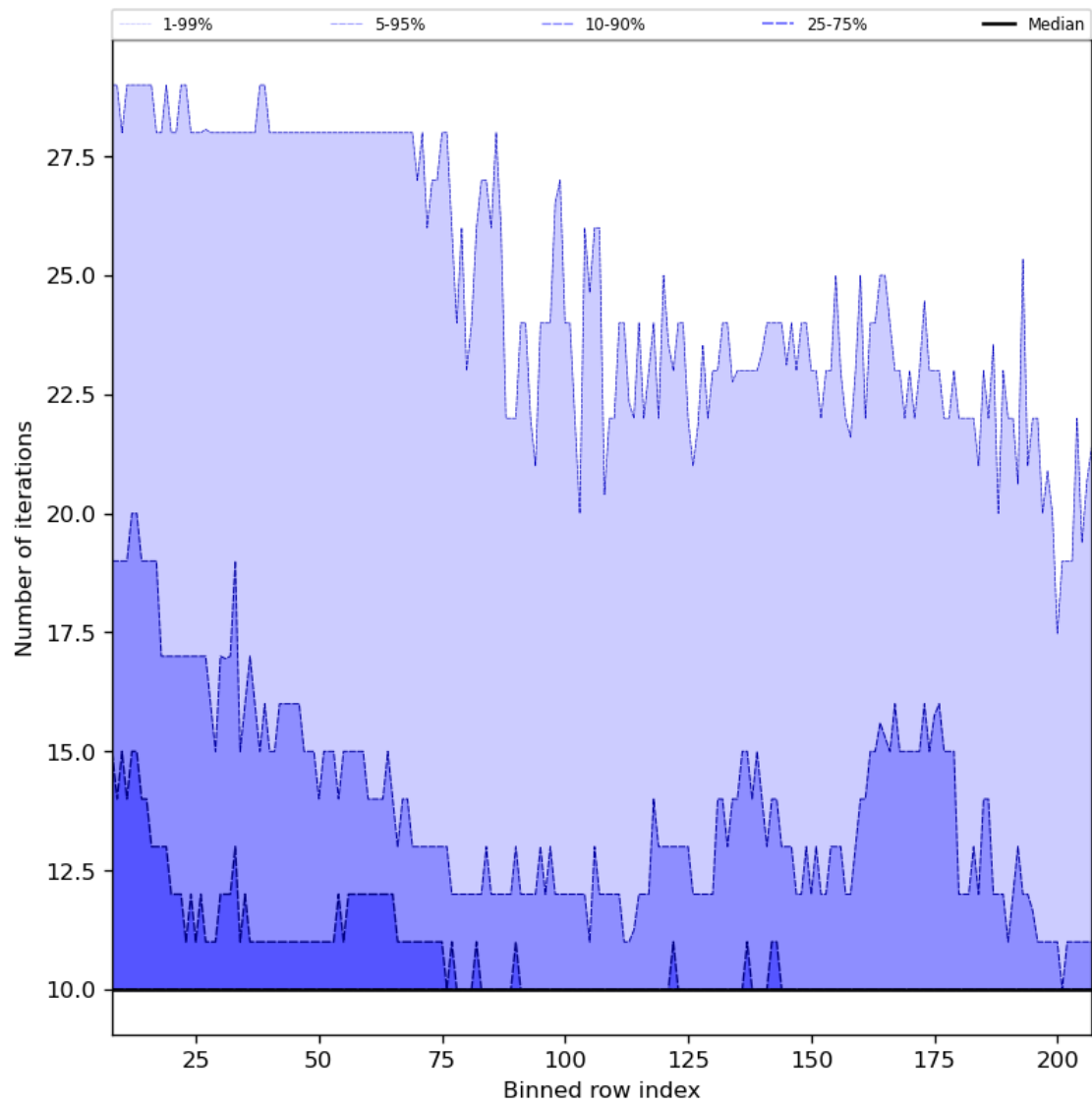
Figure 42: Along track statistics of “Number of iterations” for 2023-11-02 to 2023-11-04
