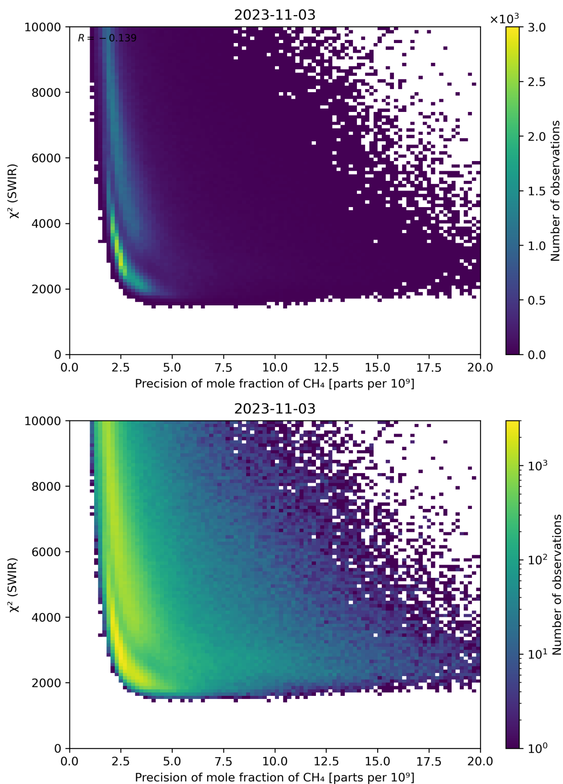
Figure 79: Scatter density plot of “Precision of mole fraction of CH 4 ” against “ \chi^2 (SWIR)” for 2023-11-02 to 2023-11-04.
