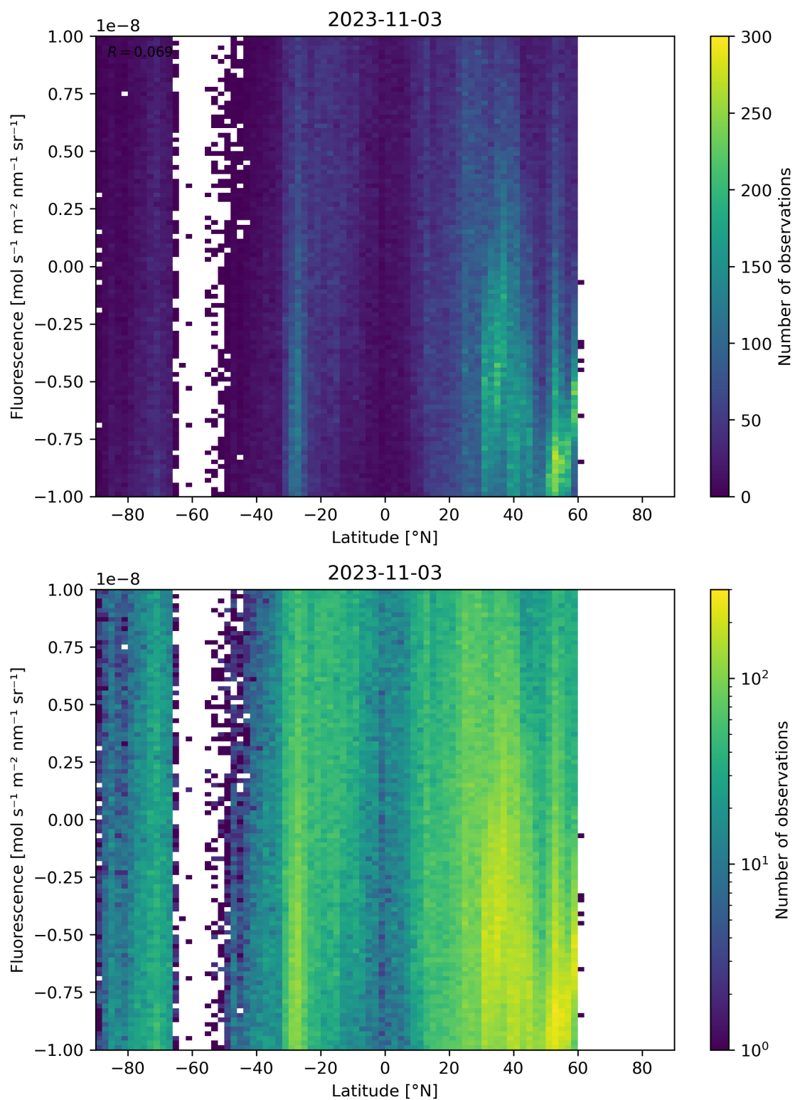
Figure 56: Scatter density plot of “Latitude” against “Fluorescence” for 2023-11-02 to 2023-11-04.
