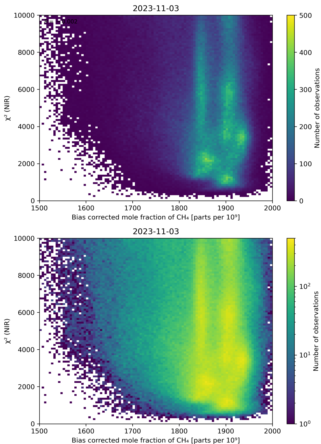
Figure 63: Scatter density plot of “Bias corrected mole fraction of CH 4 ” against “ \chi^2 (NIR)” for 2023-11-02 to 2023-11-04.
