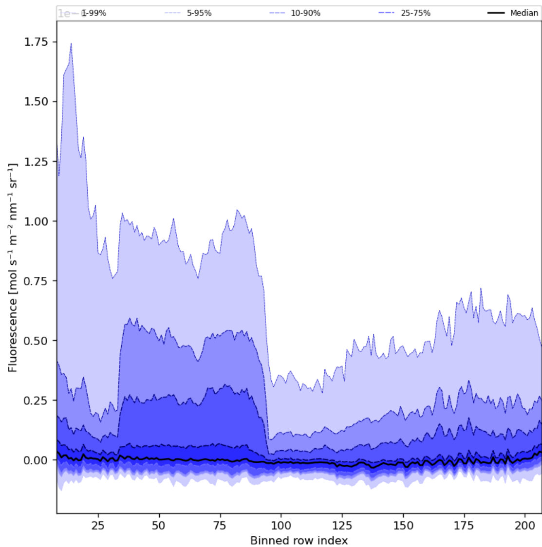
Figure 43: Along track statistics of “Fluorescence” for 2023-11-02 to 2023-11-04
