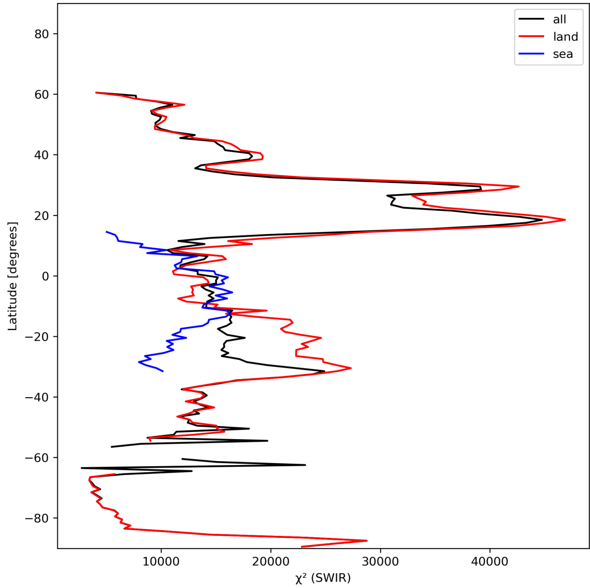
Figure 17: Zonal average of “ \chi^2 (SWIR)” for 2023-11-02 to 2023-11-04.
