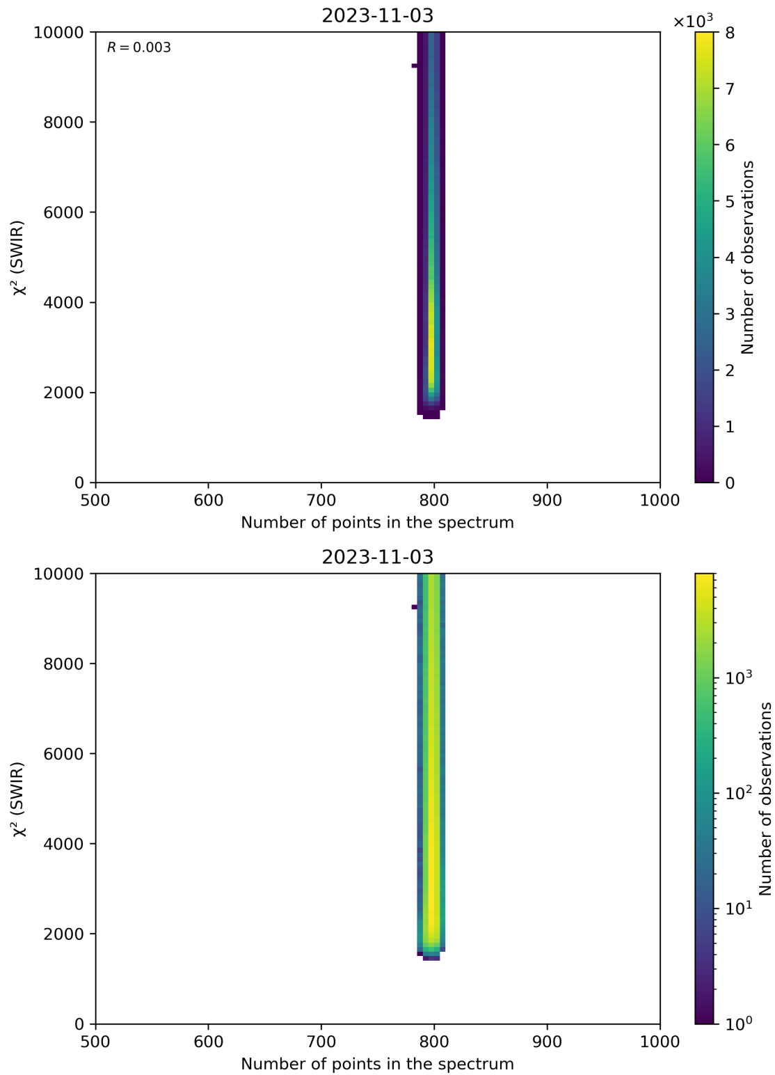
Figure 89: Scatter density plot of “Number of points in the spectrum” against “ \chi^2 (SWIR)” for 2023-11-02 to 2023-11-04.
