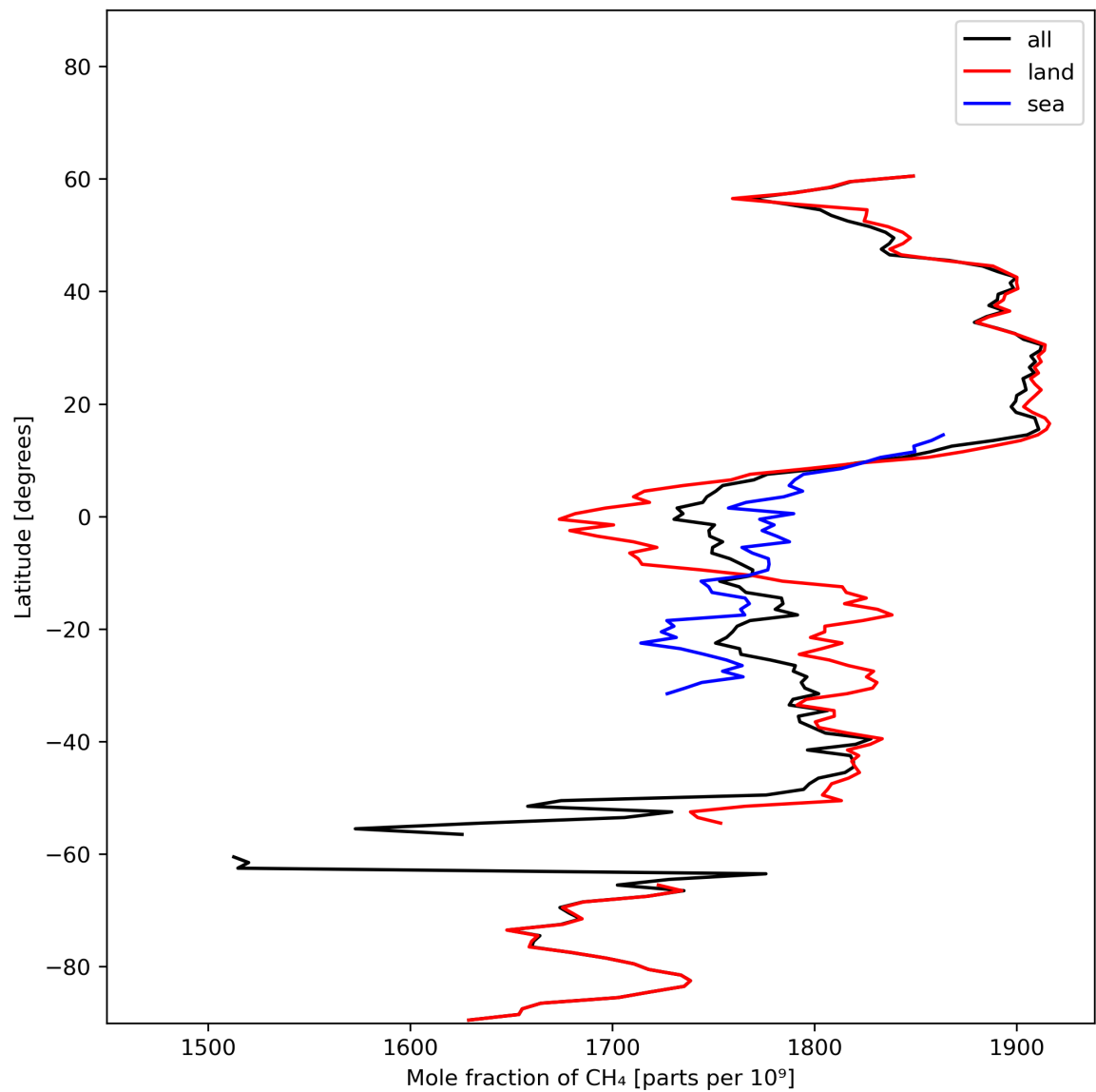
Figure 12: Zonal average of “Mole fraction of \text{CH}_4 ” for 2023-11-02 to 2023-11-04.
