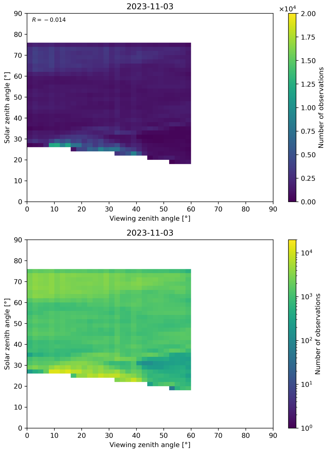
Figure 115: Scatter density plot of “Viewing zenith angle” against “Solar zenith angle” for 2023-11-02 to 2023-11-04.
