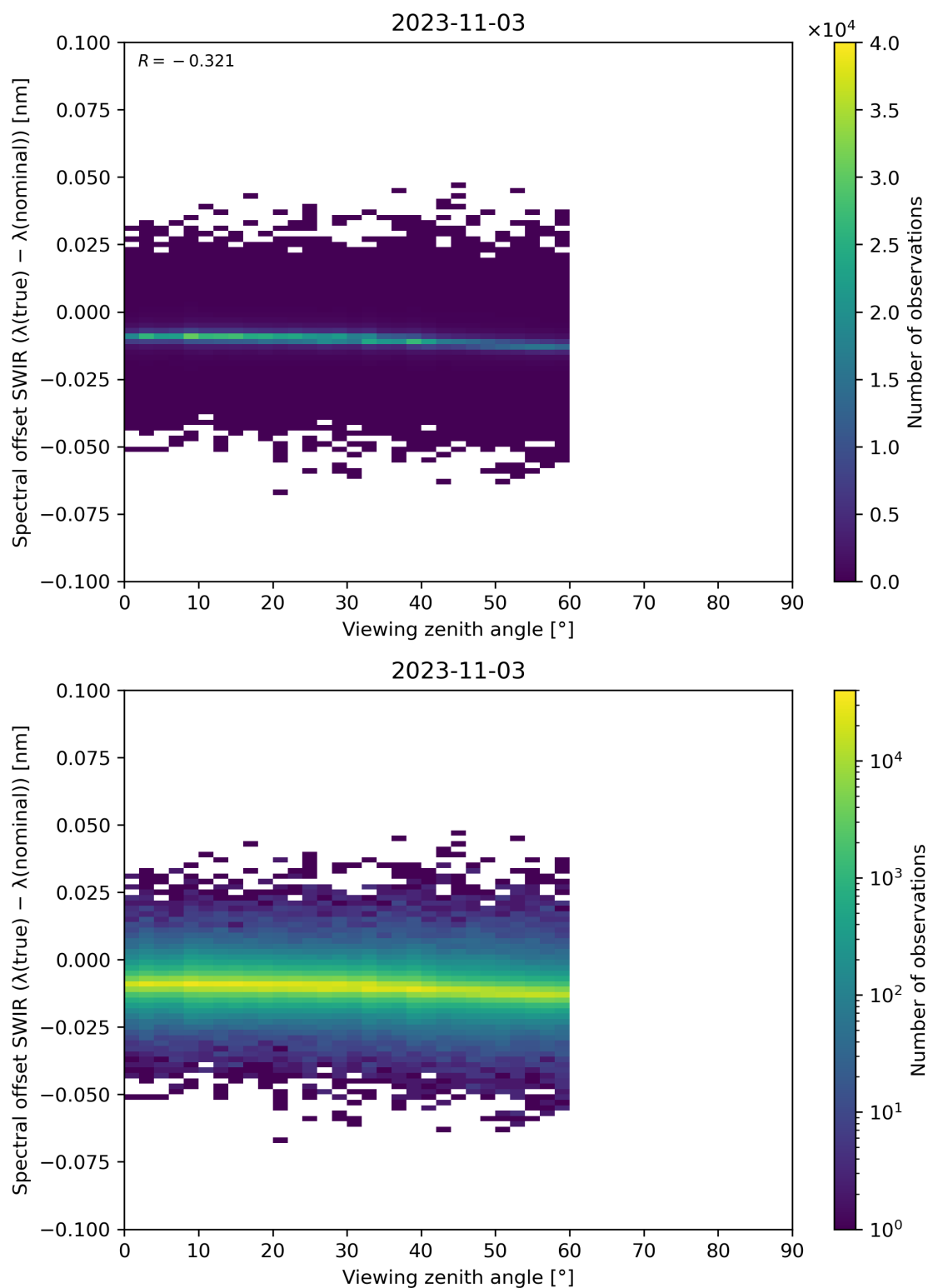
Figure 116: Scatter density plot of “Viewing zenith angle” against “Spectral offset SWIR ( \lambda(\text{true}) - \lambda(\text{nominal}) )” for 2023-11-02 to 2023-11-04.
