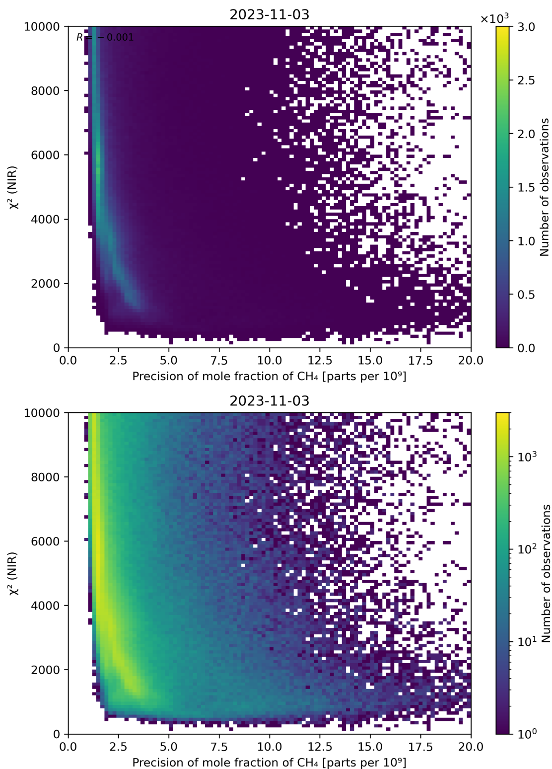
Figure 78: Scatter density plot of “Precision of mole fraction of \text{CH}_4 ” against “ \chi^2 (NIR)” for 2023-11-02 to 2023-11-04.
