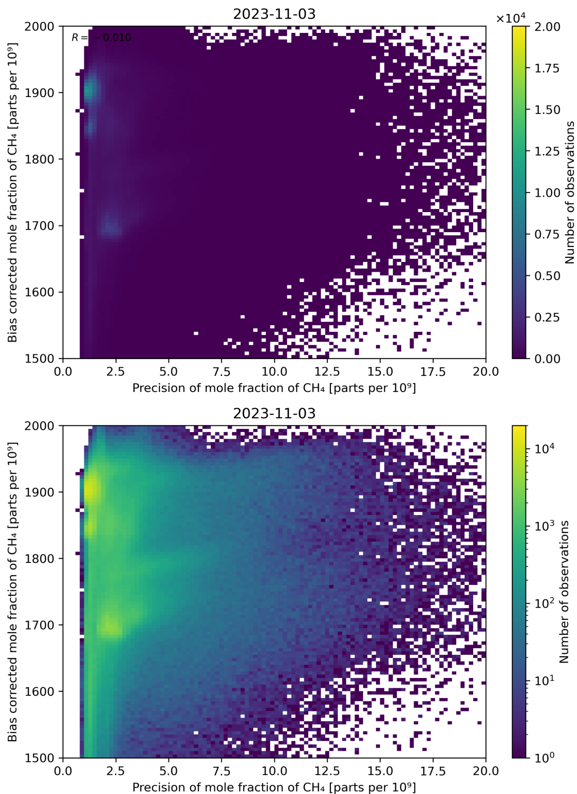
Figure 82: Scatter density plot of “Precision of mole fraction of CH 4 ” against “Bias corrected mole fraction of CH 4 ” for 2023-11-02 to 2023-11-04.
