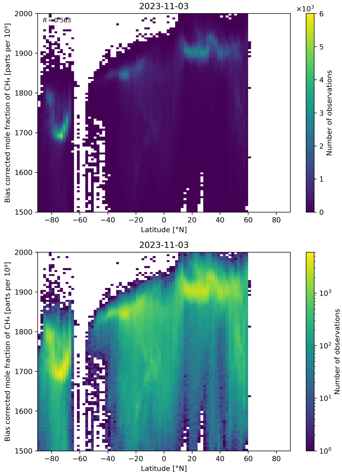
Figure 58: Scatter density plot of “Latitude” against “Bias corrected mole fraction of \text{CH}_4 ” for 2023-11-02 to 2023-11-04.
