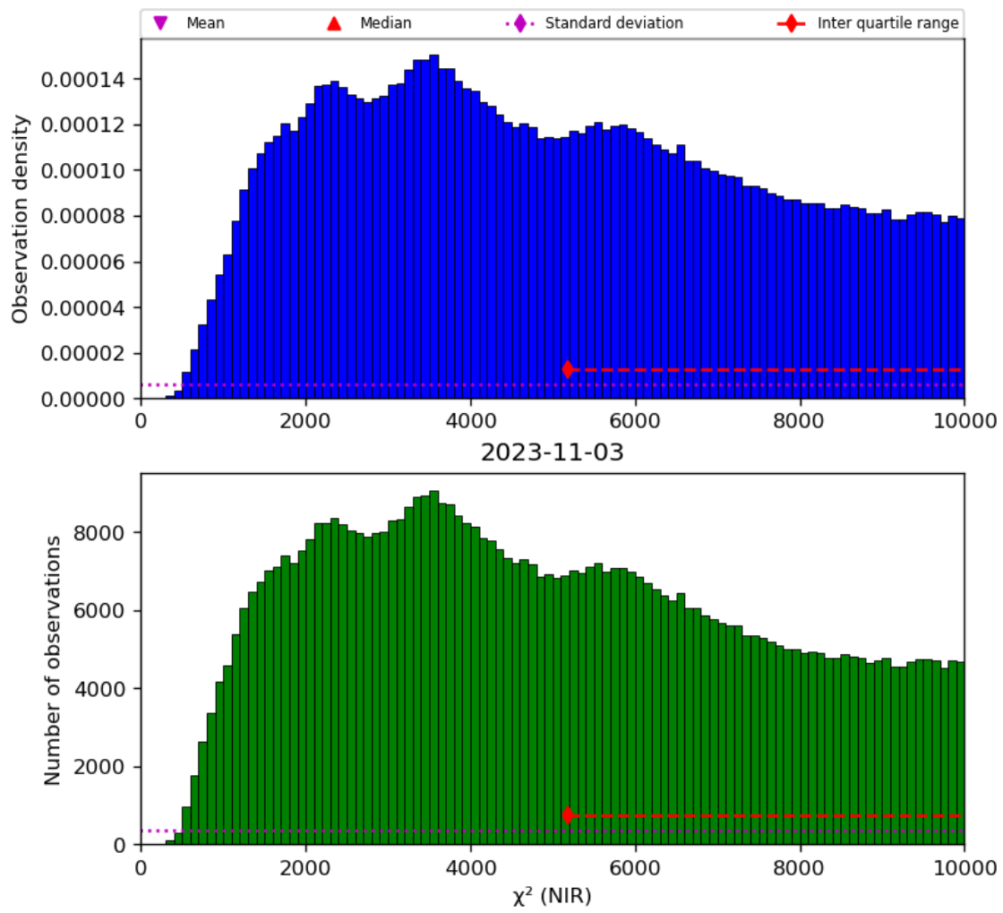
Figure 29: Histogram of " \chi^2 (NIR)" for 2023-11-02 to 2023-11-04
