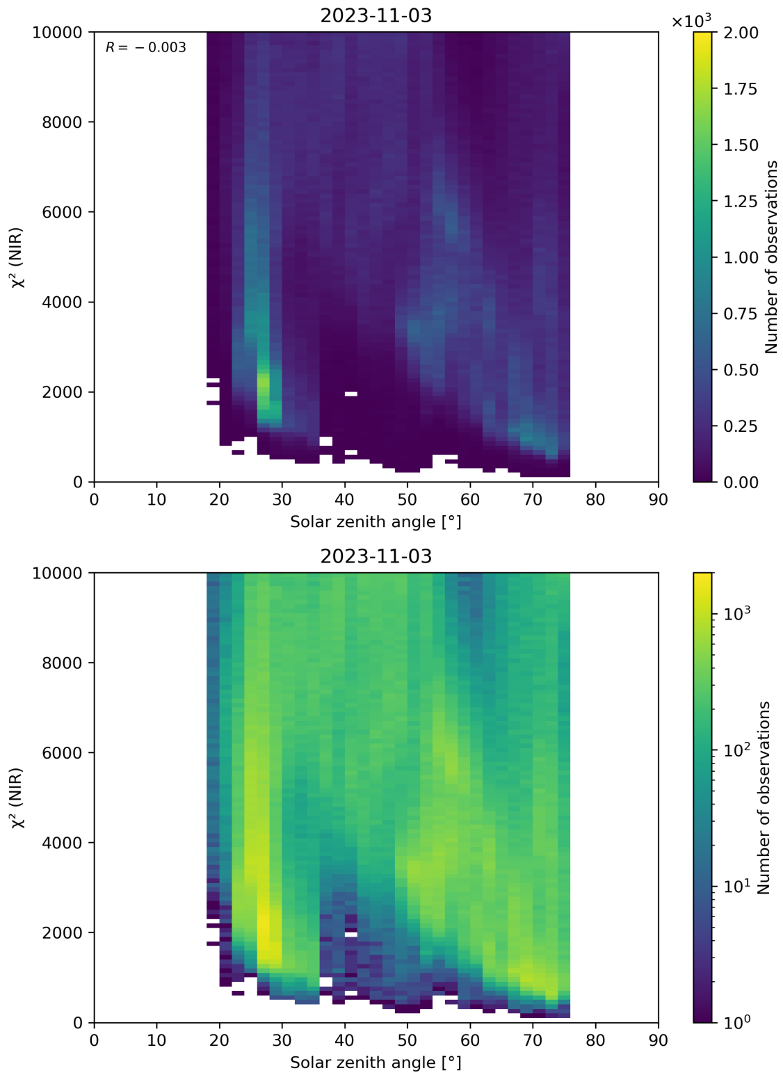
Figure 94: Scatter density plot of “Solar zenith angle” against “ \chi^2 (NIR)” for 2023-11-02 to 2023-11-04.
