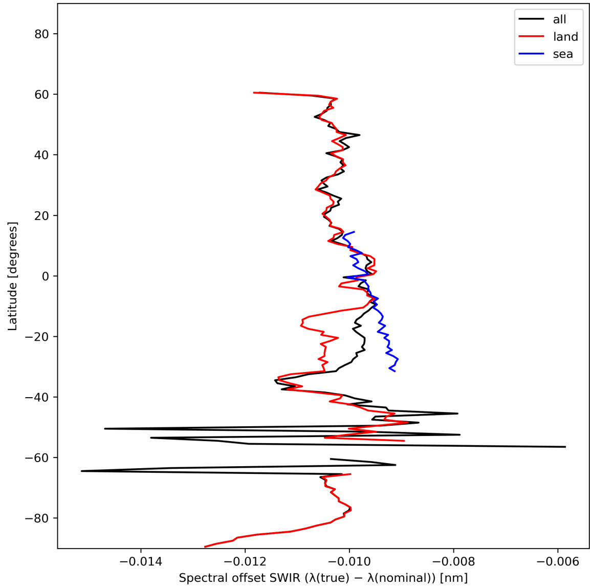
Figure 16: Zonal average of “Spectral offset SWIR ( \lambda(\text{true}) - \lambda(\text{nominal}) )” for 2023-11-02 to 2023-11-04.
