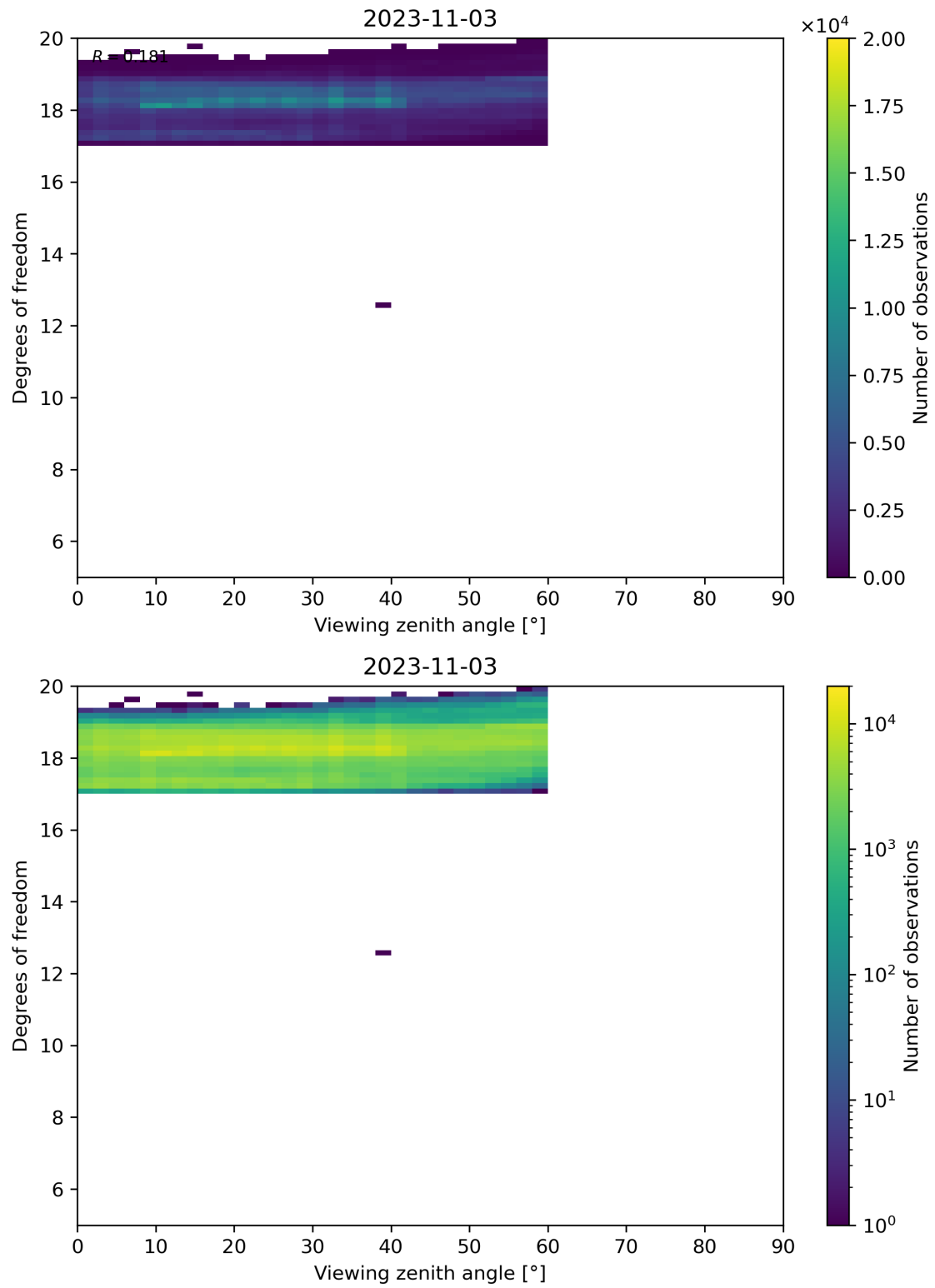
Figure 107: Scatter density plot of “Viewing zenith angle” against “Degrees of freedom” for 2023-11-02 to 2023-11-04.
