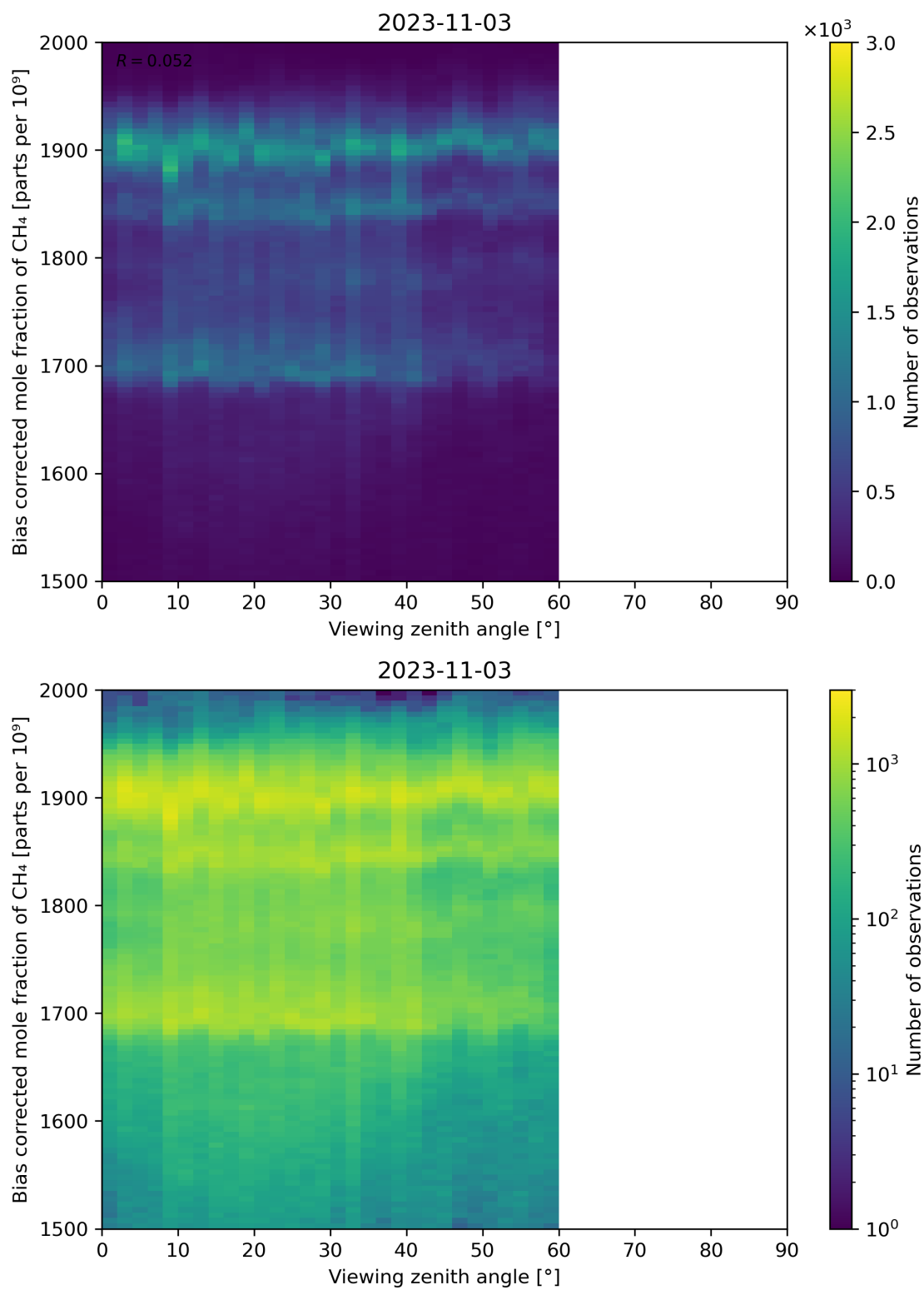
Figure 111: Scatter density plot of “Viewing zenith angle” against “Bias corrected mole fraction of CH 4 ” for 2023-11-02 to 2023-11-04.
