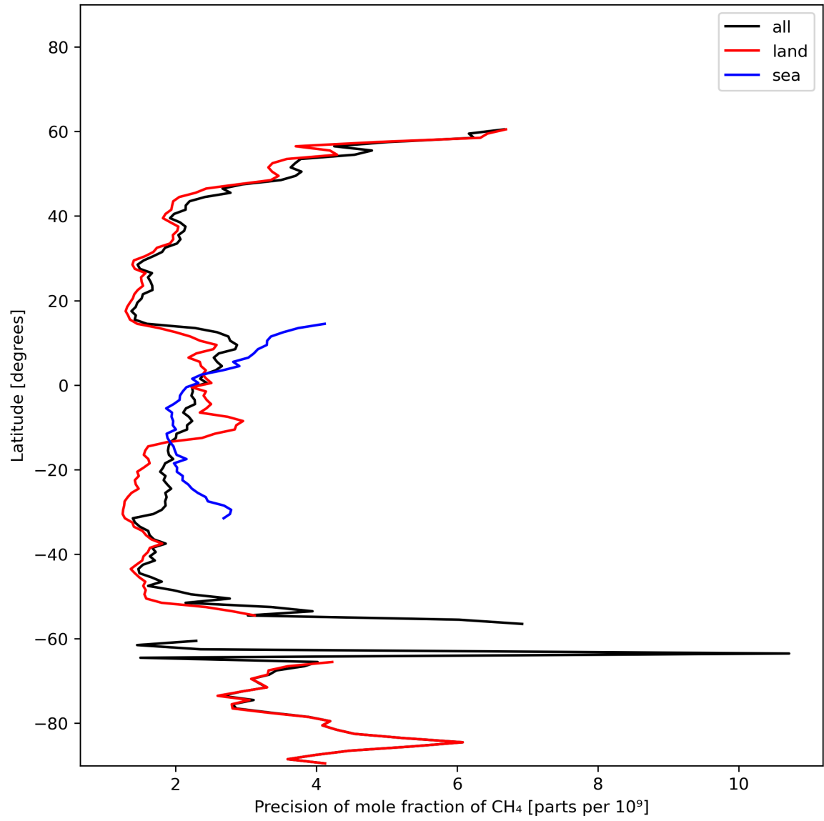
Figure 13: Zonal average of “Precision of mole fraction of CH 4 ” for 2023-11-02 to 2023-11-04.
