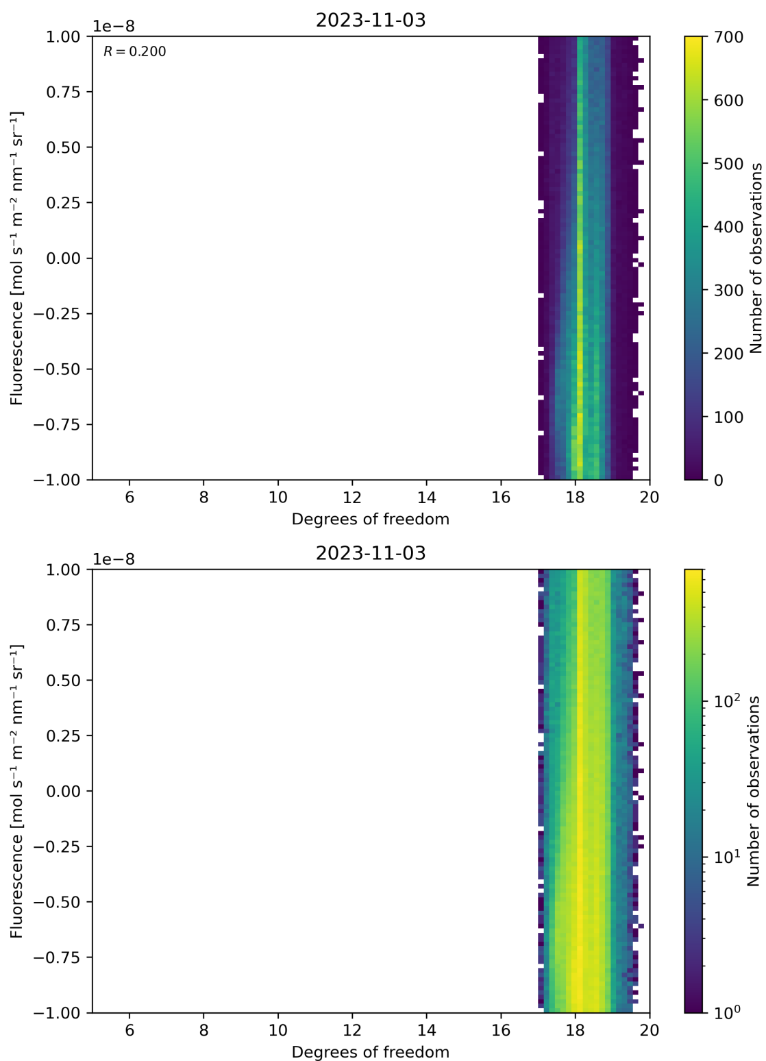
Figure 51: Scatter density plot of “Degrees of freedom” against “Fluorescence” for 2023-11-02 to 2023-11-04.
