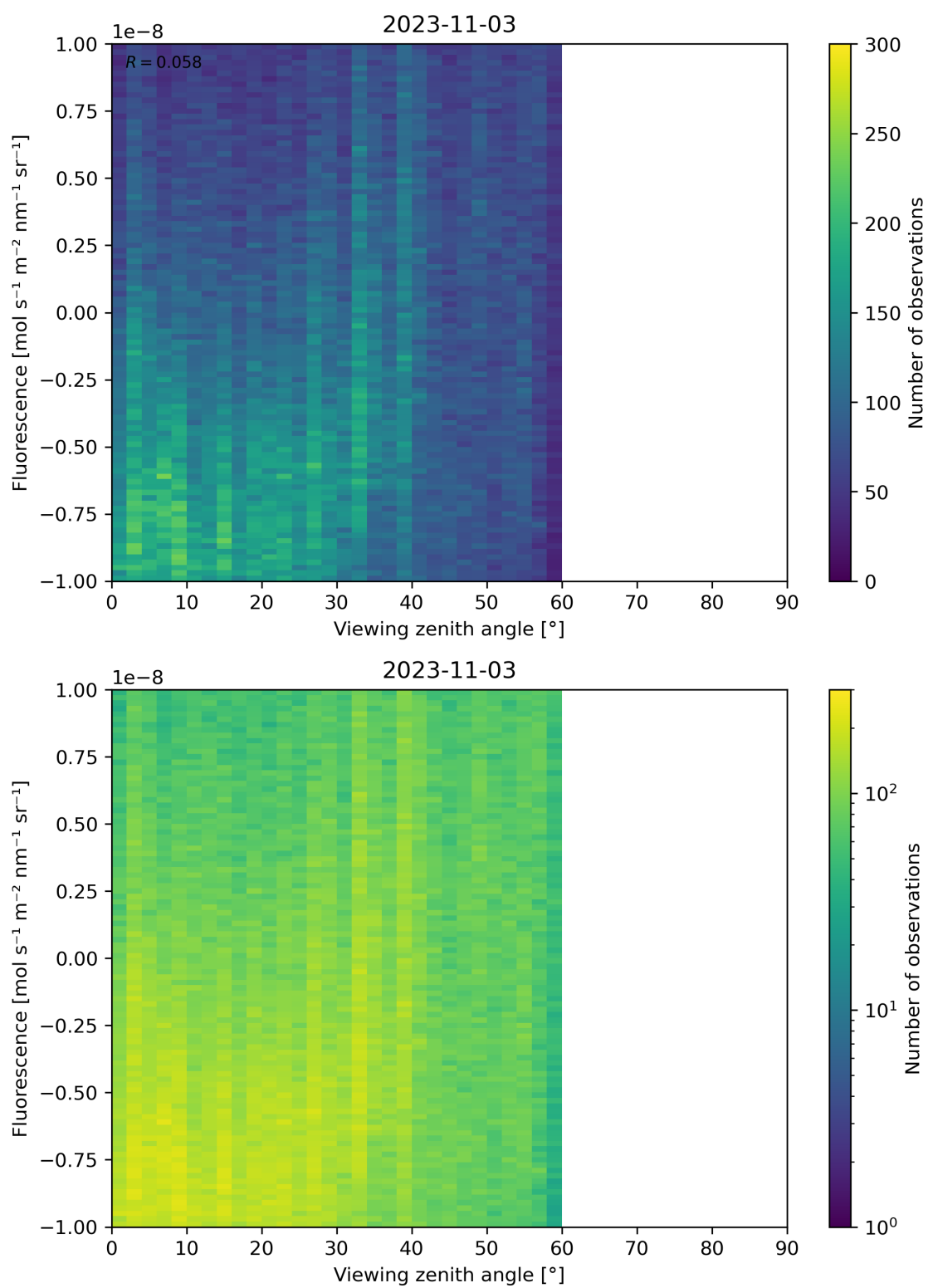
Figure 108: Scatter density plot of “Viewing zenith angle” against “Fluorescence” for 2023-11-02 to 2023-11-04.
