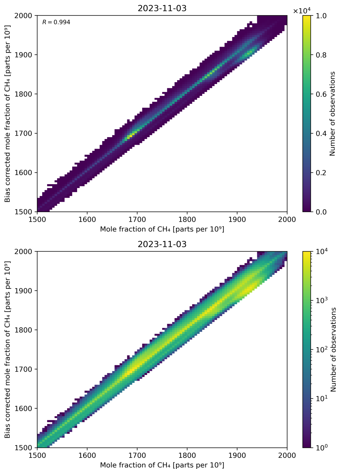
Figure 74: Scatter density plot of “Mole fraction of CH 4 ” against “Bias corrected mole fraction of CH 4 ” for 2023-11-02 to 2023-11-04.
