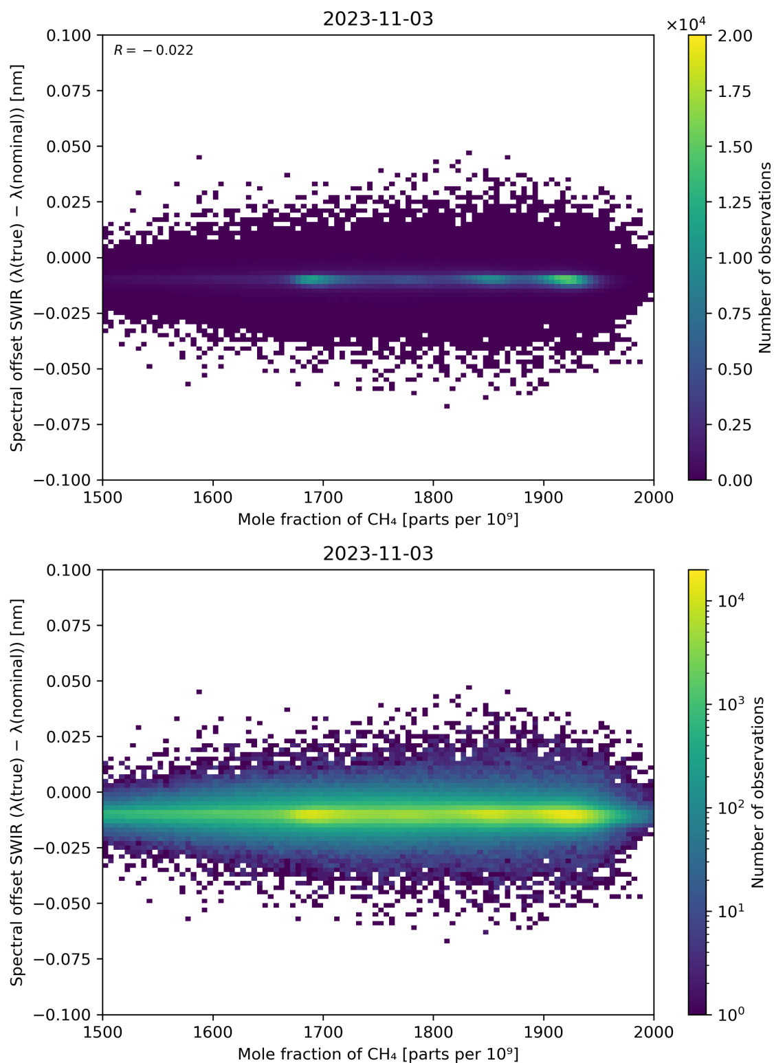
Figure 86: Scatter density plot of “Mole fraction of CH 4 ” against “Spectral offset SWIR ( \lambda(\text{true}) - \lambda(\text{nominal}) )” for 2023-11-02 to 2023-11-04.
