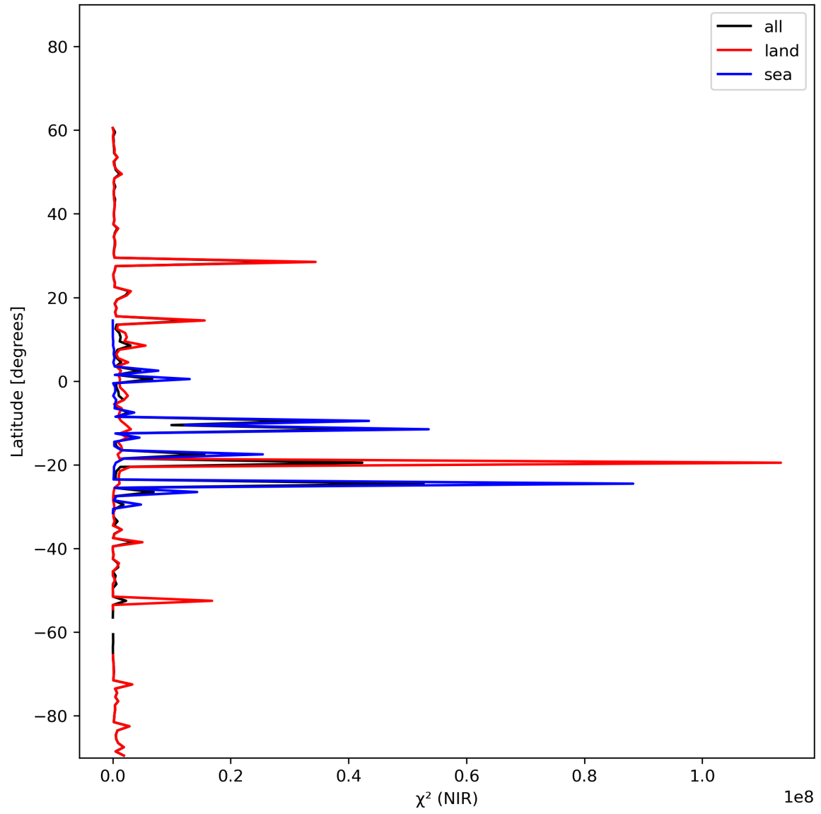
Figure 18: Zonal average of “ \chi^2 (NIR)” for 2023-11-02 to 2023-11-04.
