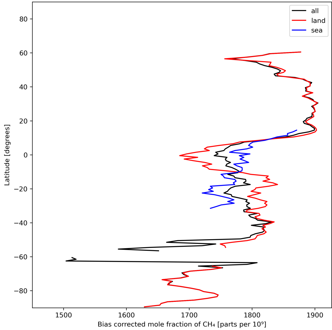
Figure 14: Zonal average of “Bias corrected mole fraction of CH 4 ” for 2023-11-02 to 2023-11-04.
