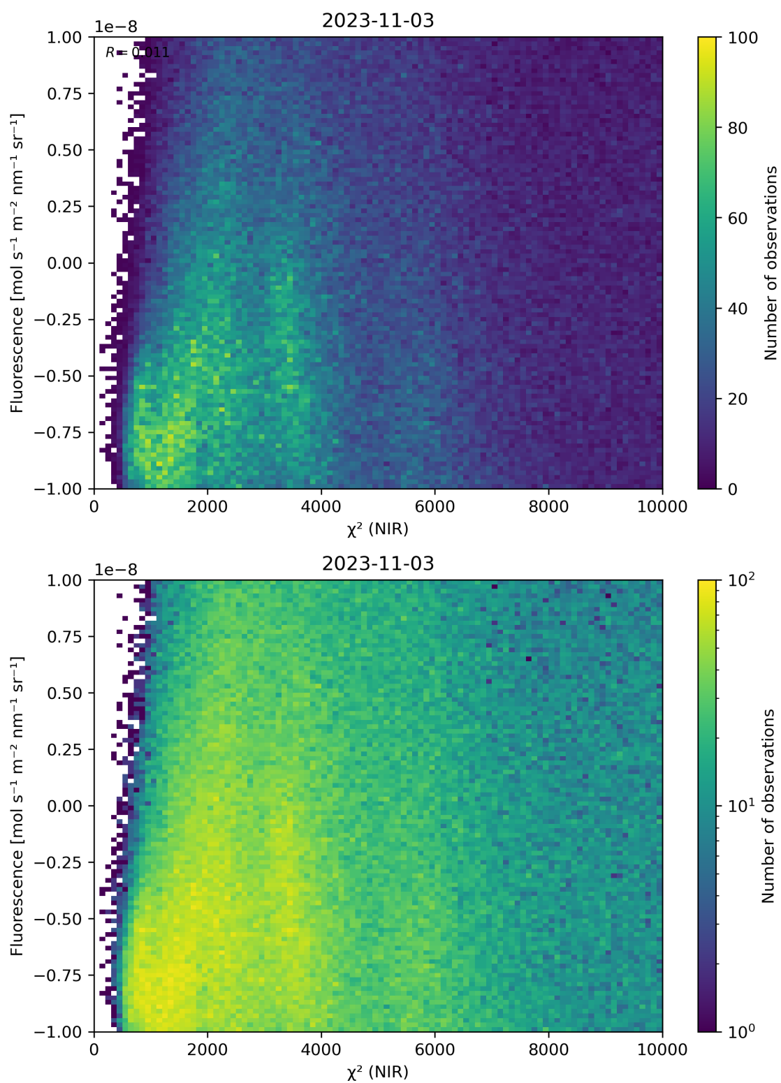
Figure 45: Scatter density plot of “ \chi^2 (NIR)” against “Fluorescence” for 2023-11-02 to 2023-11-04.
