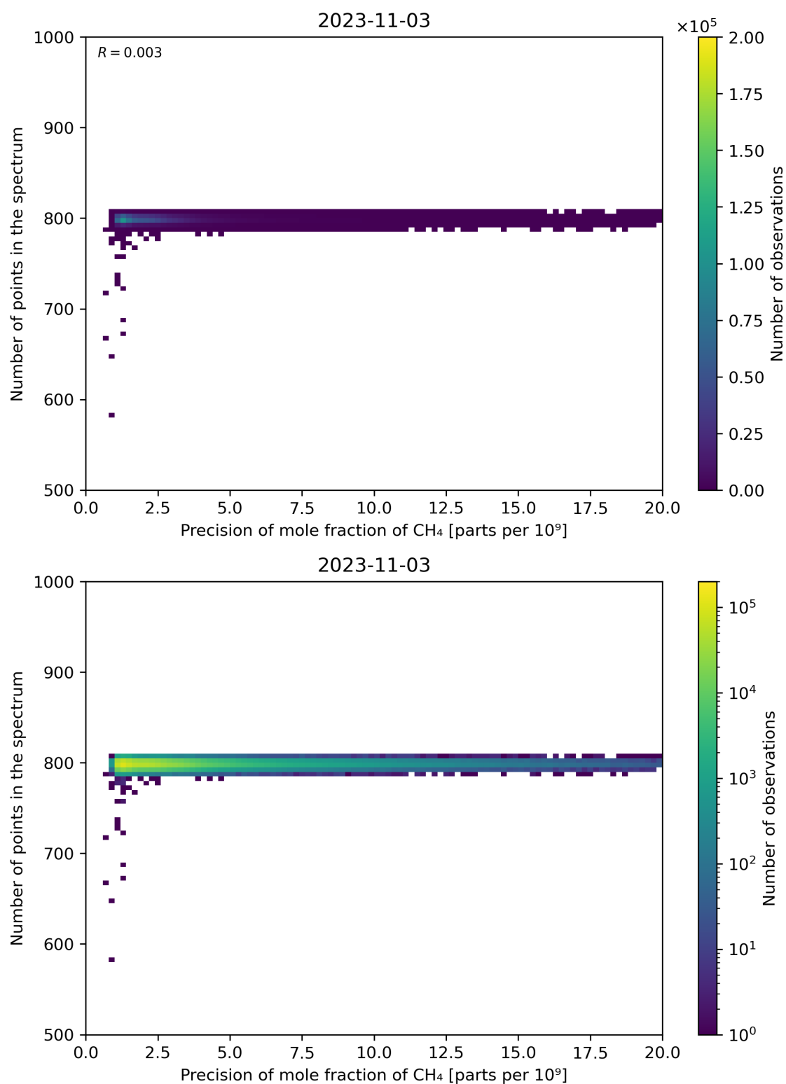
Figure 84: Scatter density plot of “Precision of mole fraction of CH 4 ” against “Number of points in the spectrum” for 2023-11-02 to 2023-11-04.
