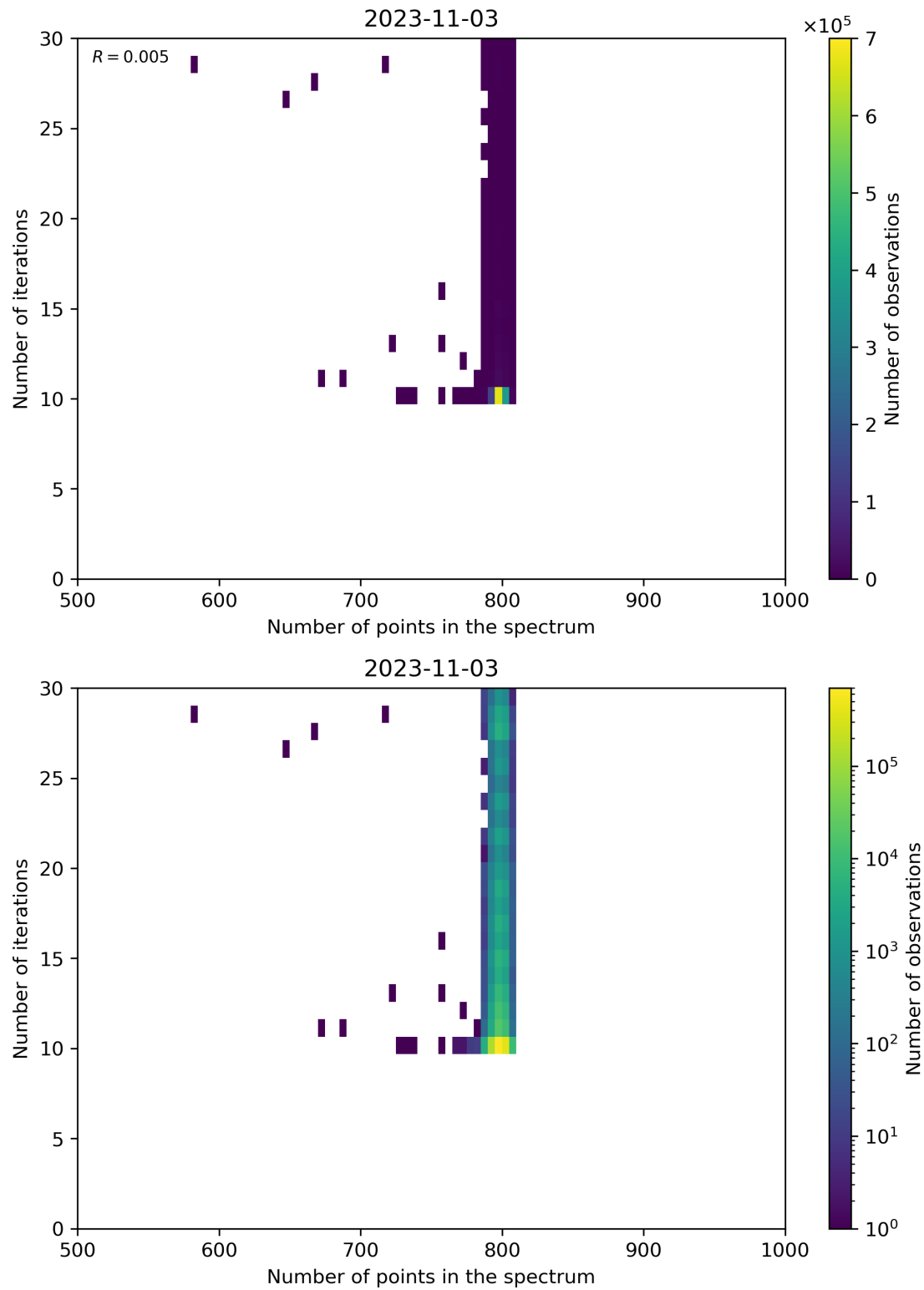
Figure 92: Scatter density plot of “Number of points in the spectrum” against “Number of iterations” for 2023-11-02 to 2023-11-04.
