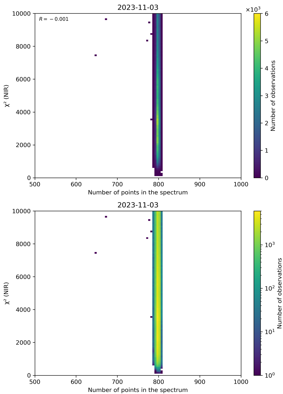
Figure 88: Scatter density plot of “Number of points in the spectrum” against “ \chi^2 (NIR)” for 2023-11-02 to 2023-11-04.
