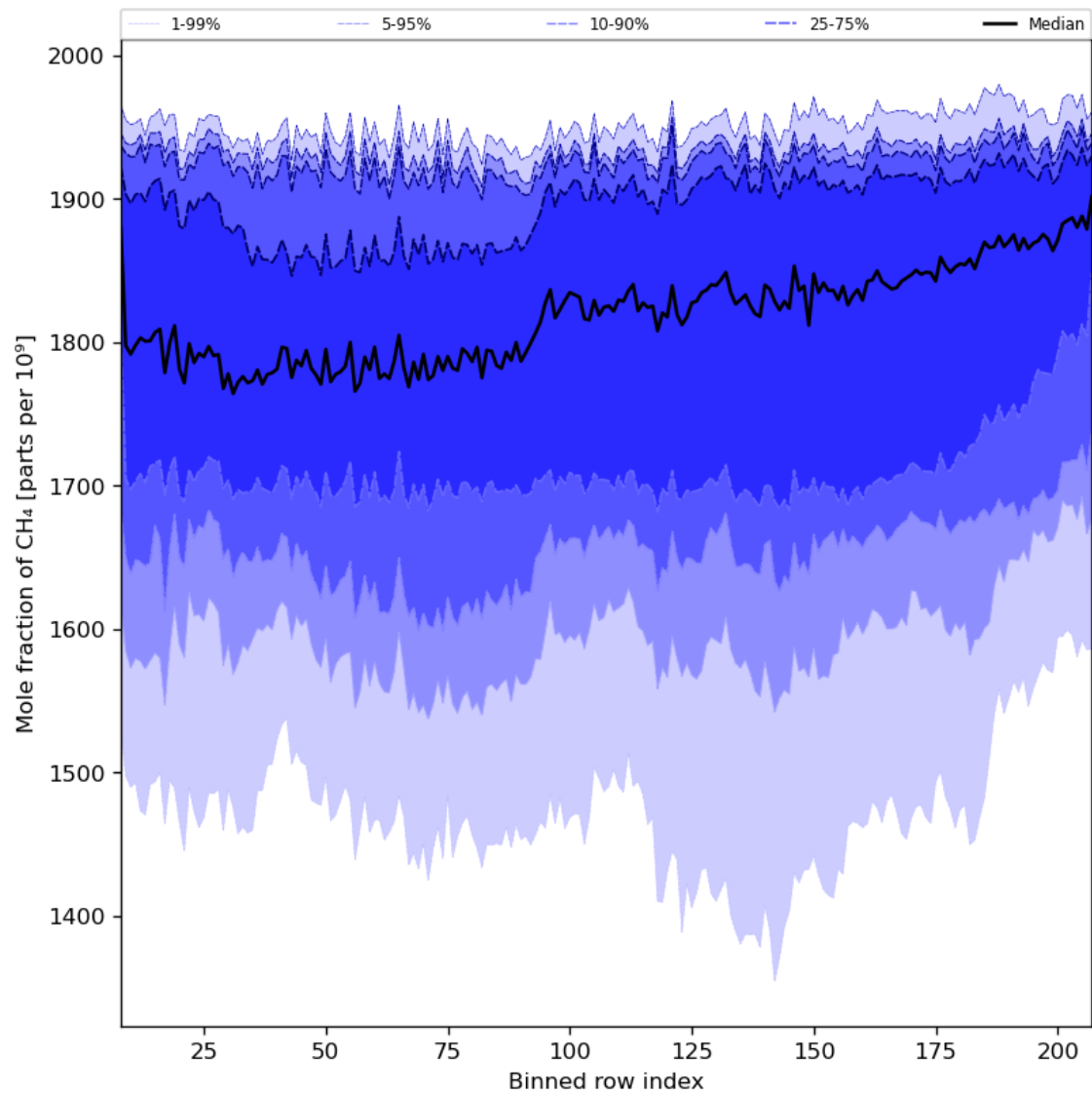
Figure 34: Along track statistics of “Mole fraction of CH 4 ” for 2023-11-02 to 2023-11-04
