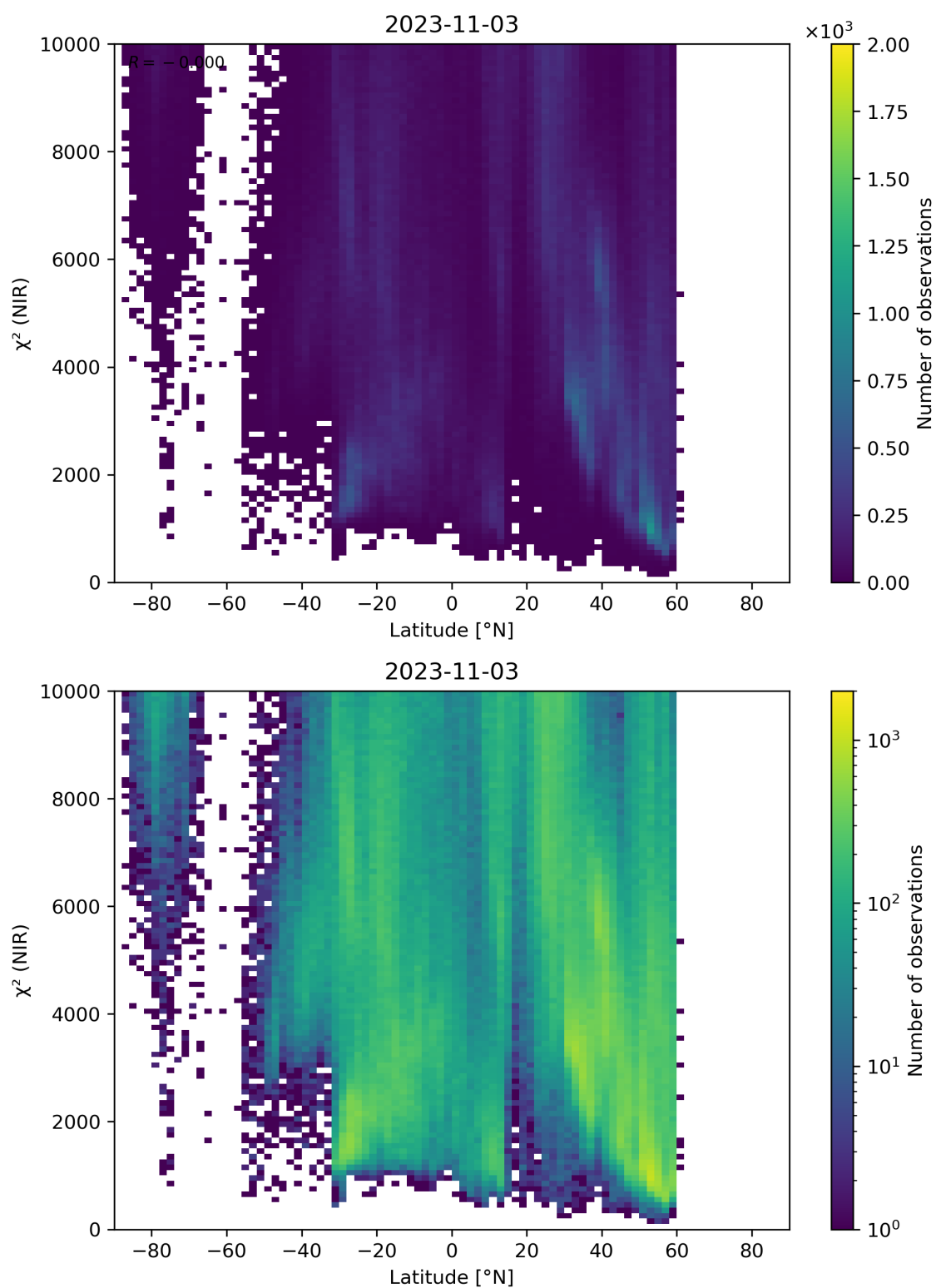
Figure 53: Scatter density plot of “Latitude” against “ \chi^2 (NIR)” for 2023-11-02 to 2023-11-04.
