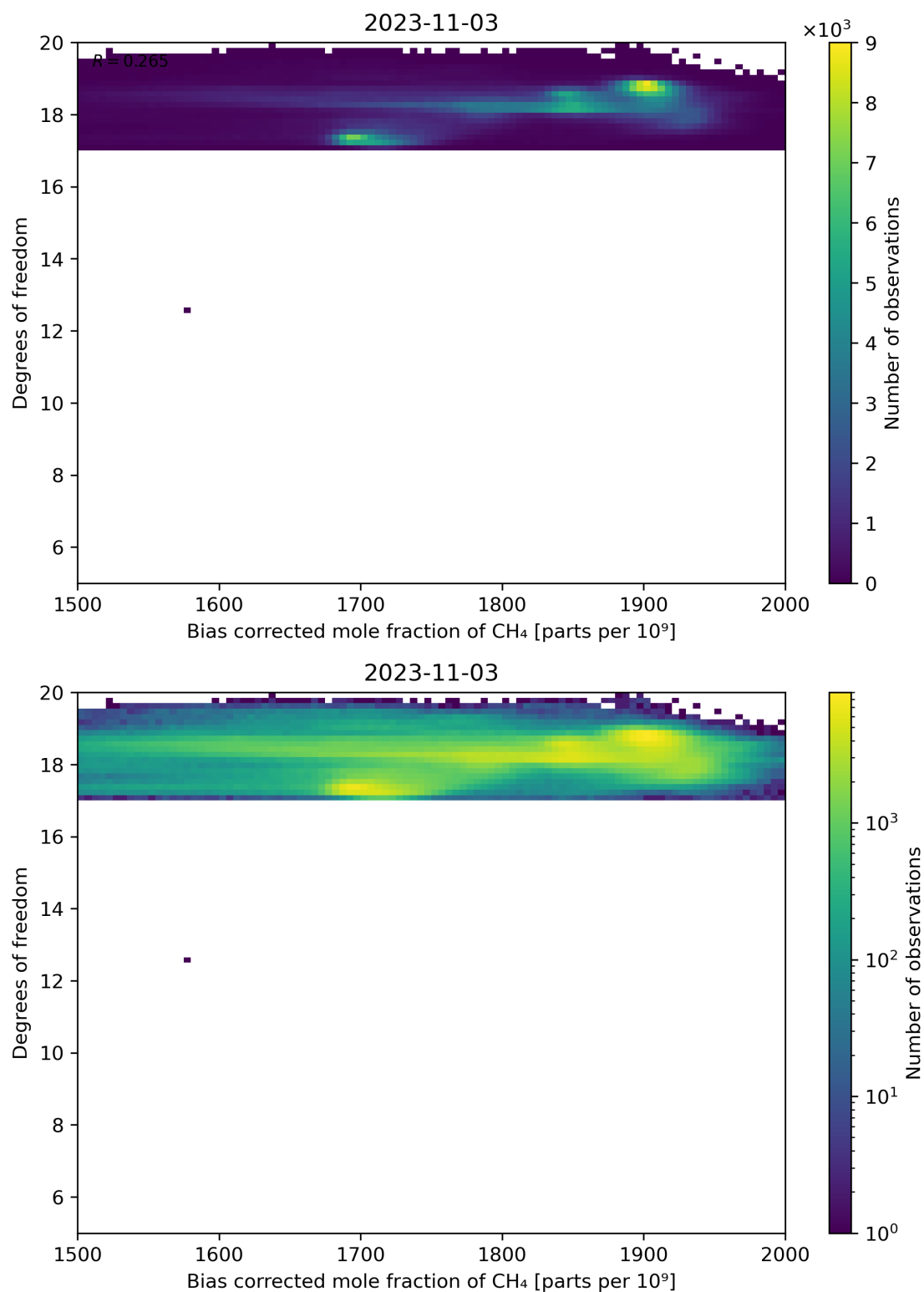
Figure 65: Scatter density plot of “Bias corrected mole fraction of CH 4 ” against “Degrees of freedom” for 2023-11-02 to 2023-11-04.
