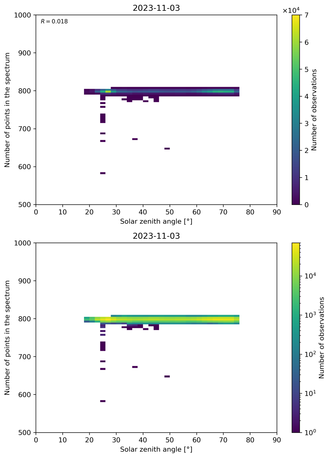
Figure 103: Scatter density plot of “Solar zenith angle” against “Number of points in the spectrum” for 2023-11-02 to 2023-11-04.
