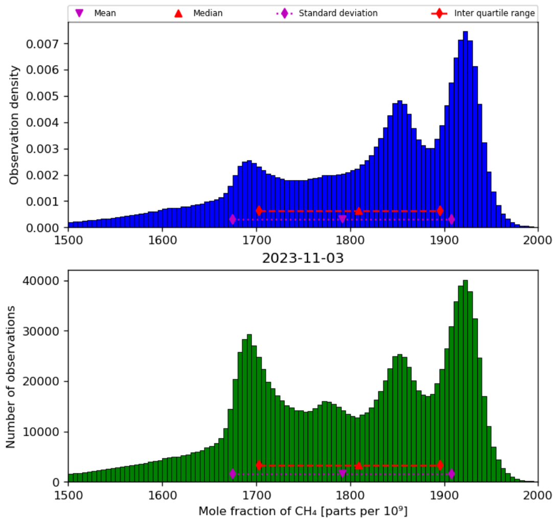
Figure 23: Histogram of “Mole fraction of CH 4 ” for 2023-11-02 to 2023-11-04
