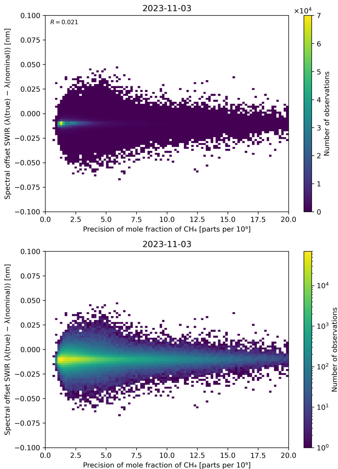
Figure 85: Scatter density plot of “Precision of mole fraction of CH 4 ” against “Spectral offset SWIR ( \lambda(\text{true}) - \lambda(\text{nominal}) )” for 2023-11-02 to 2023-11-04.
