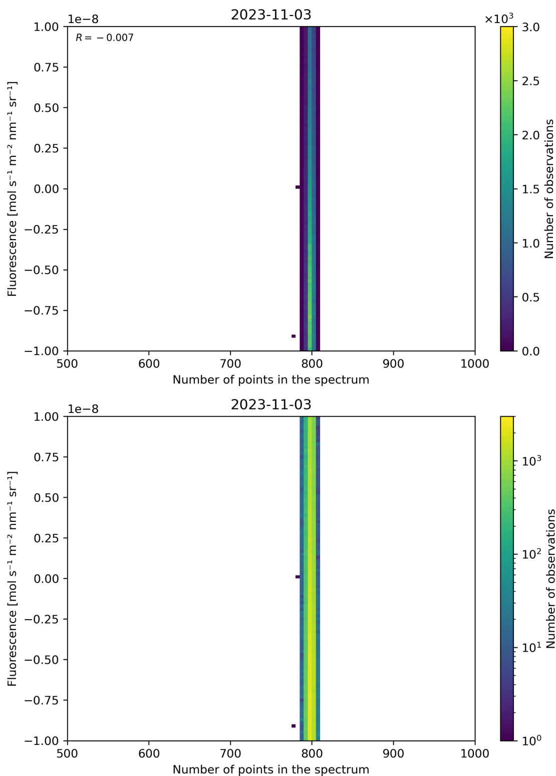
Figure 91: Scatter density plot of “Number of points in the spectrum” against “Fluorescence” for 2023-11-02 to 2023-11-04.
