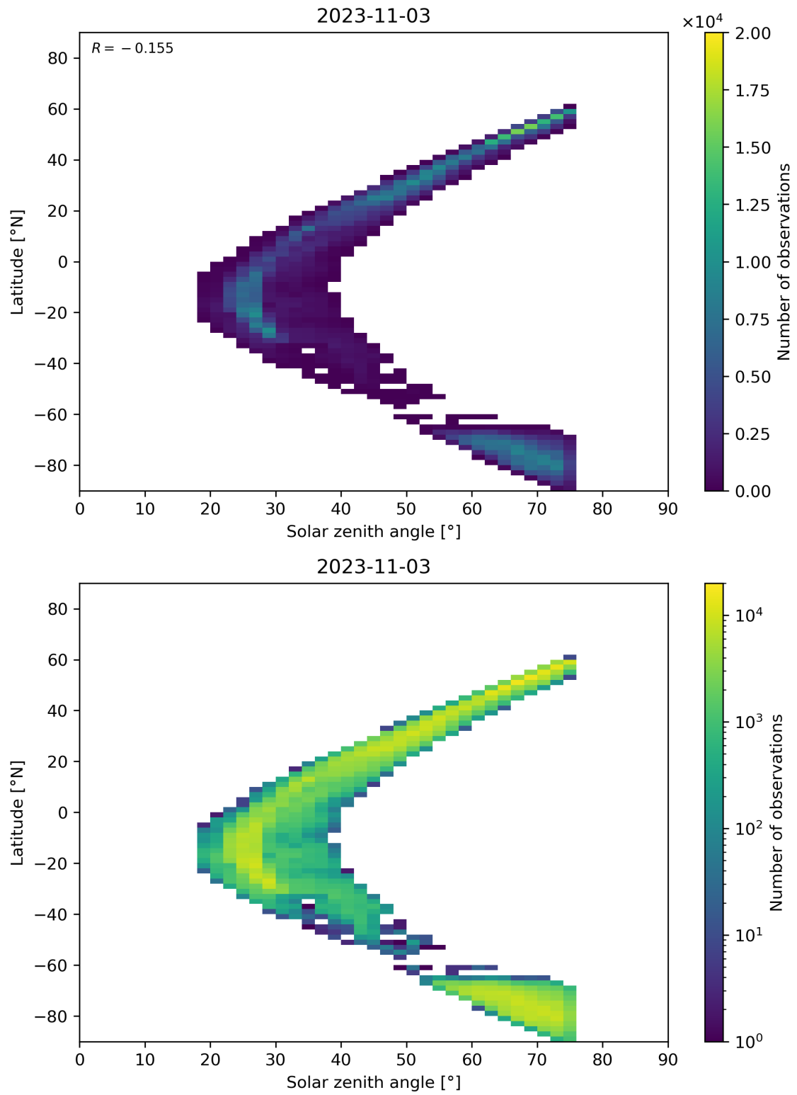
Figure 98: Scatter density plot of “Solar zenith angle” against “Latitude” for 2023-11-02 to 2023-11-04.
