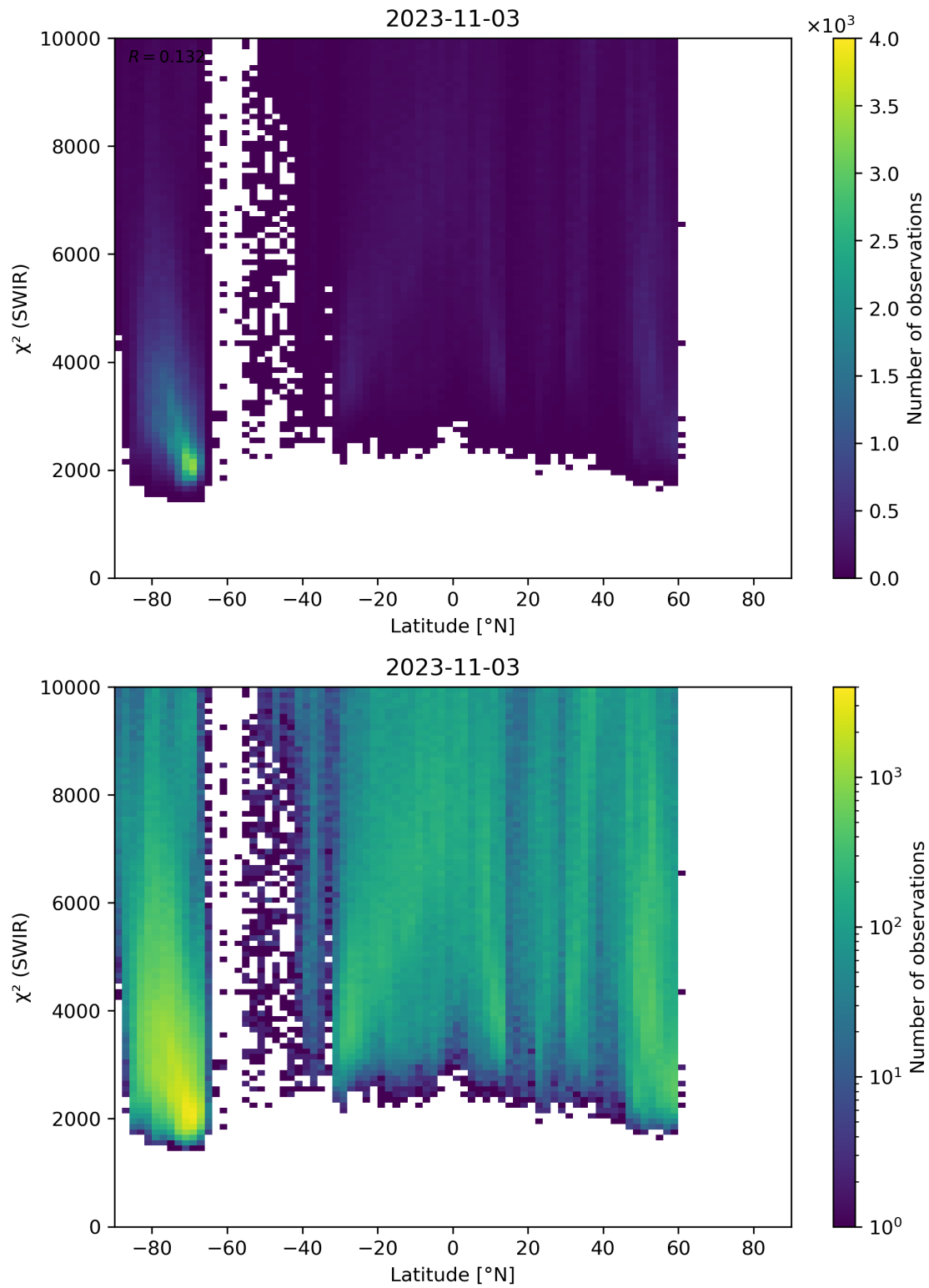
Figure 54: Scatter density plot of “Latitude” against “ \chi^2 (SWIR)” for 2023-11-02 to 2023-11-04.
