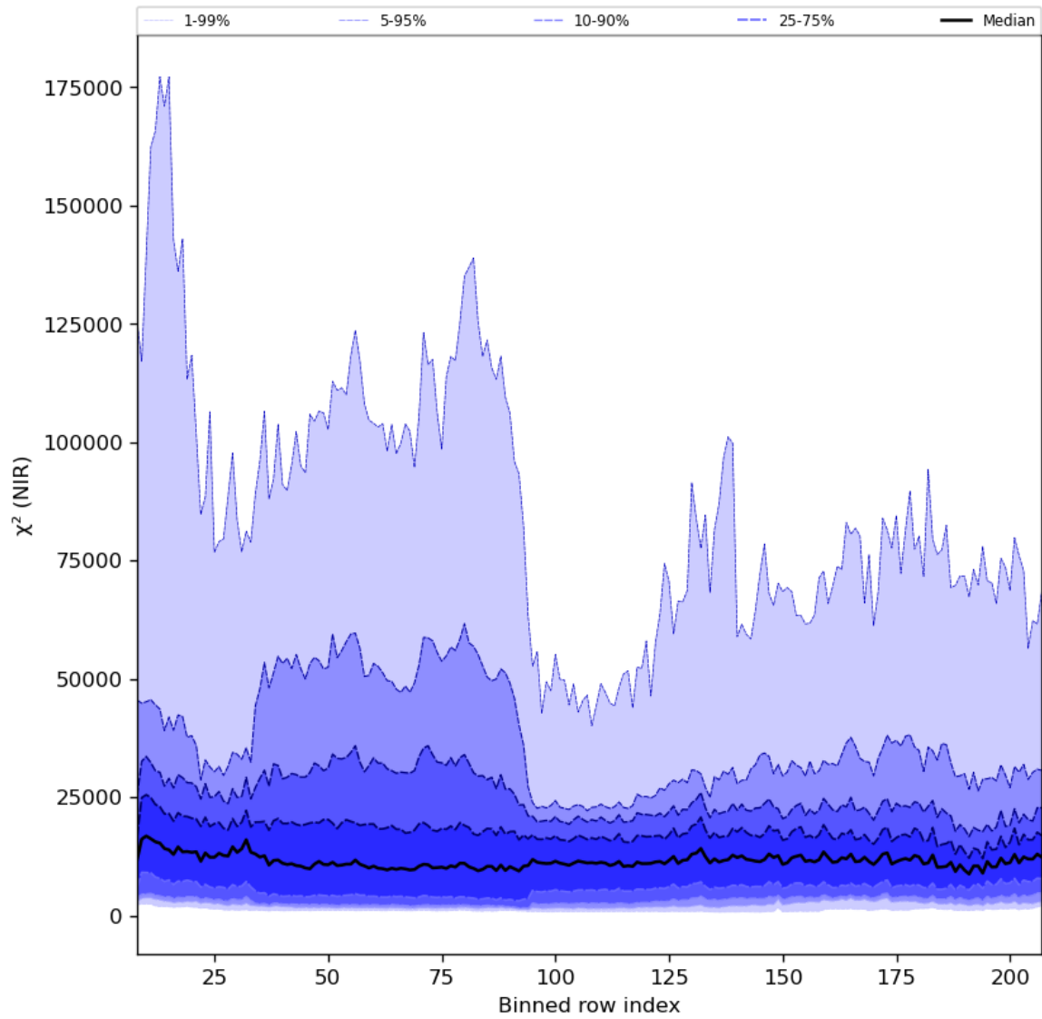
Figure 40: Along track statistics of “ \chi^2 (NIR)” for 2023-11-02 to 2023-11-04
