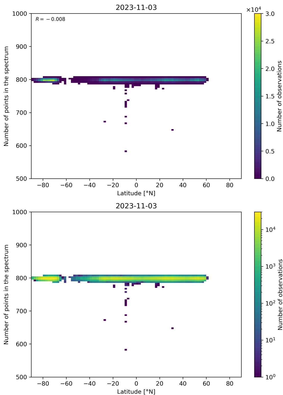
Figure 61: Scatter density plot of “Latitude” against “Number of points in the spectrum” for 2023-11-02 to 2023-11-04.
