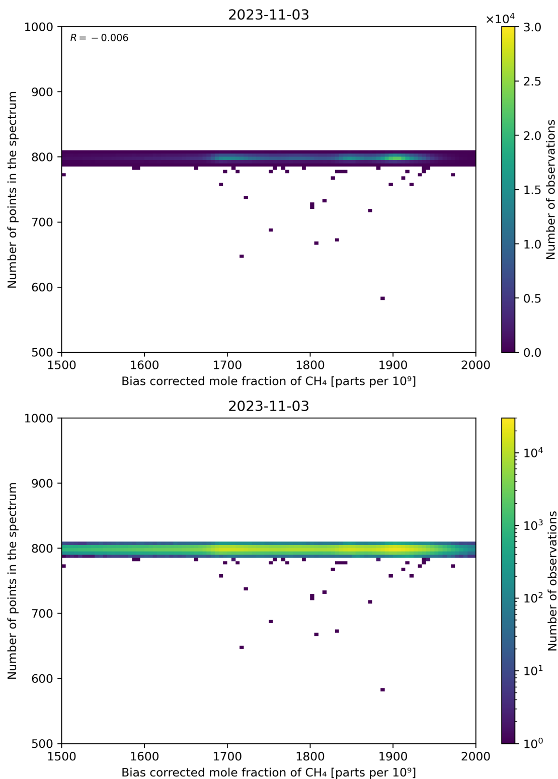
Figure 68: Scatter density plot of “Bias corrected mole fraction of CH 4 ” against “Number of points in the spectrum” for 2023-11-02 to 2023-11-04.
