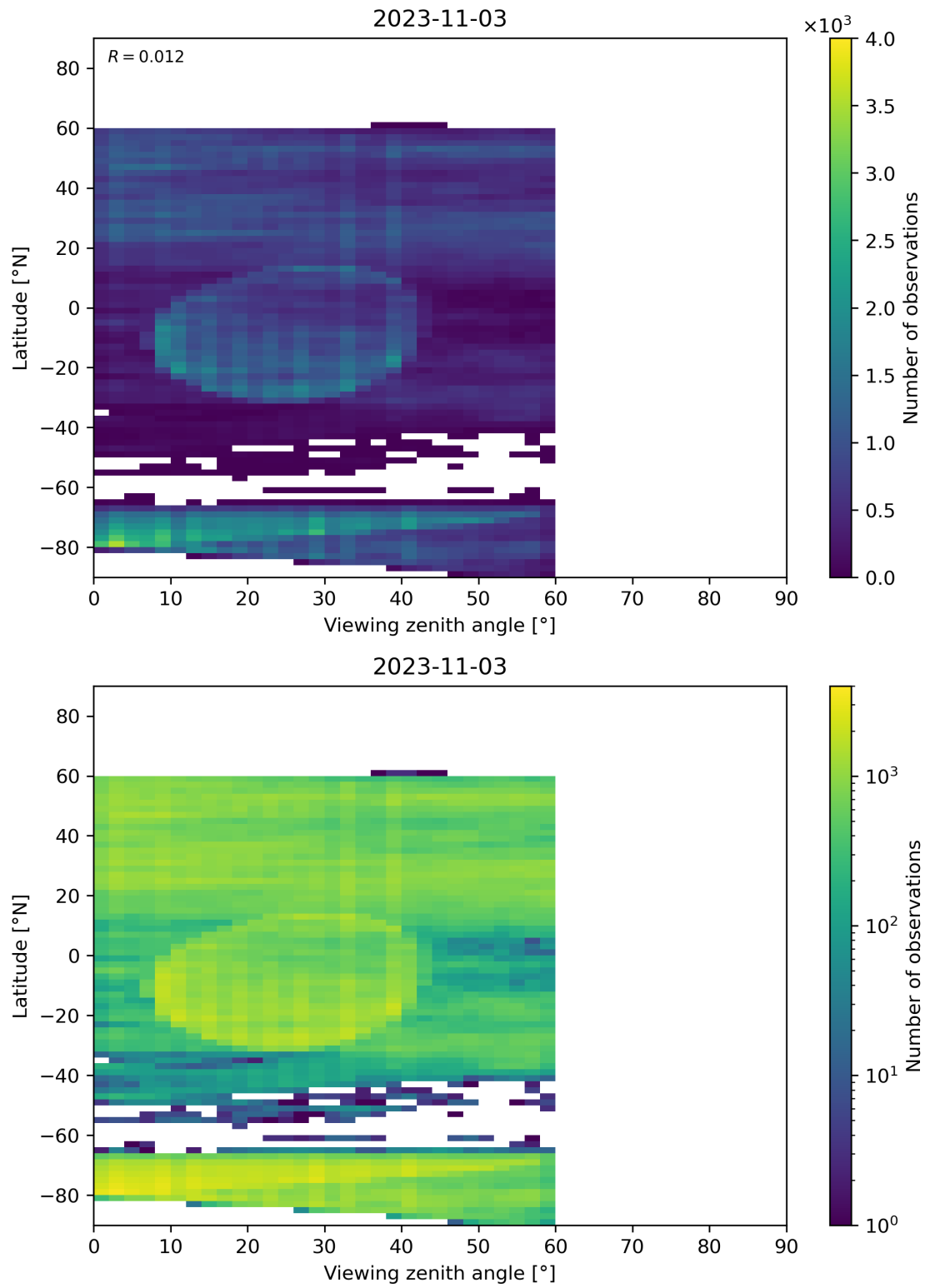
Figure 109: Scatter density plot of “Viewing zenith angle” against “Latitude” for 2023-11-02 to 2023-11-04.
