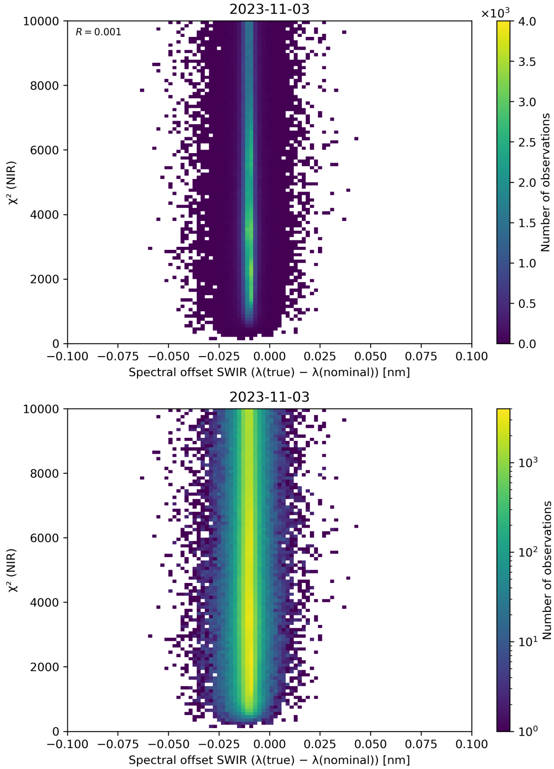
Figure 117: Scatter density plot of “Spectral offset SWIR ( \lambda(\text{true}) - \lambda(\text{nominal}) )” against “ \chi^2 (NIR)” for 2023-11-02 to 2023-11-04.
