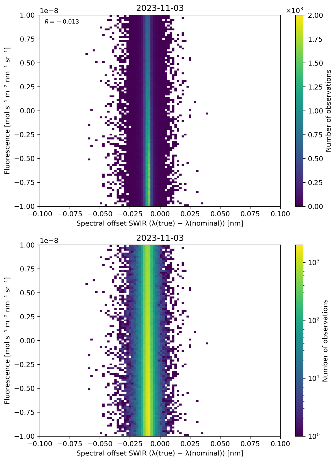
Figure 120: Scatter density plot of “Spectral offset SWIR ( \lambda(\text{true}) - \lambda(\text{nominal}) )” against “Fluorescence” for 2023-11-02 to 2023-11-04.
