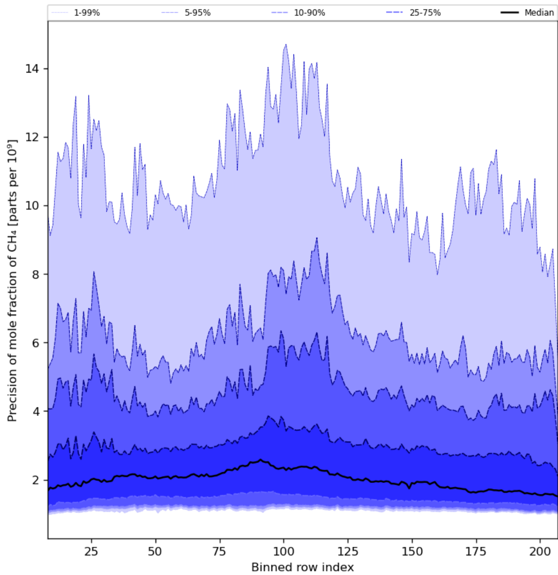
Figure 35: Along track statistics of “Precision of mole fraction of CH 4 ” for 2023-11-02 to 2023-11-04
