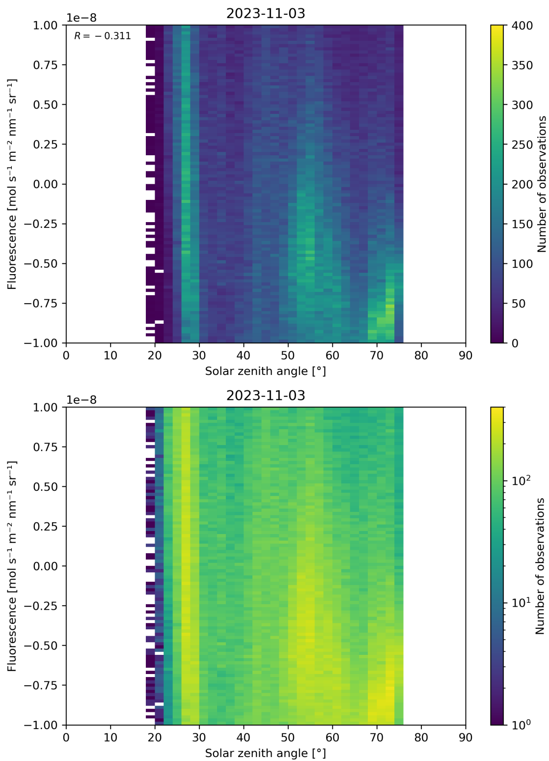
Figure 97: Scatter density plot of “Solar zenith angle” against “Fluorescence” for 2023-11-02 to 2023-11-04.
