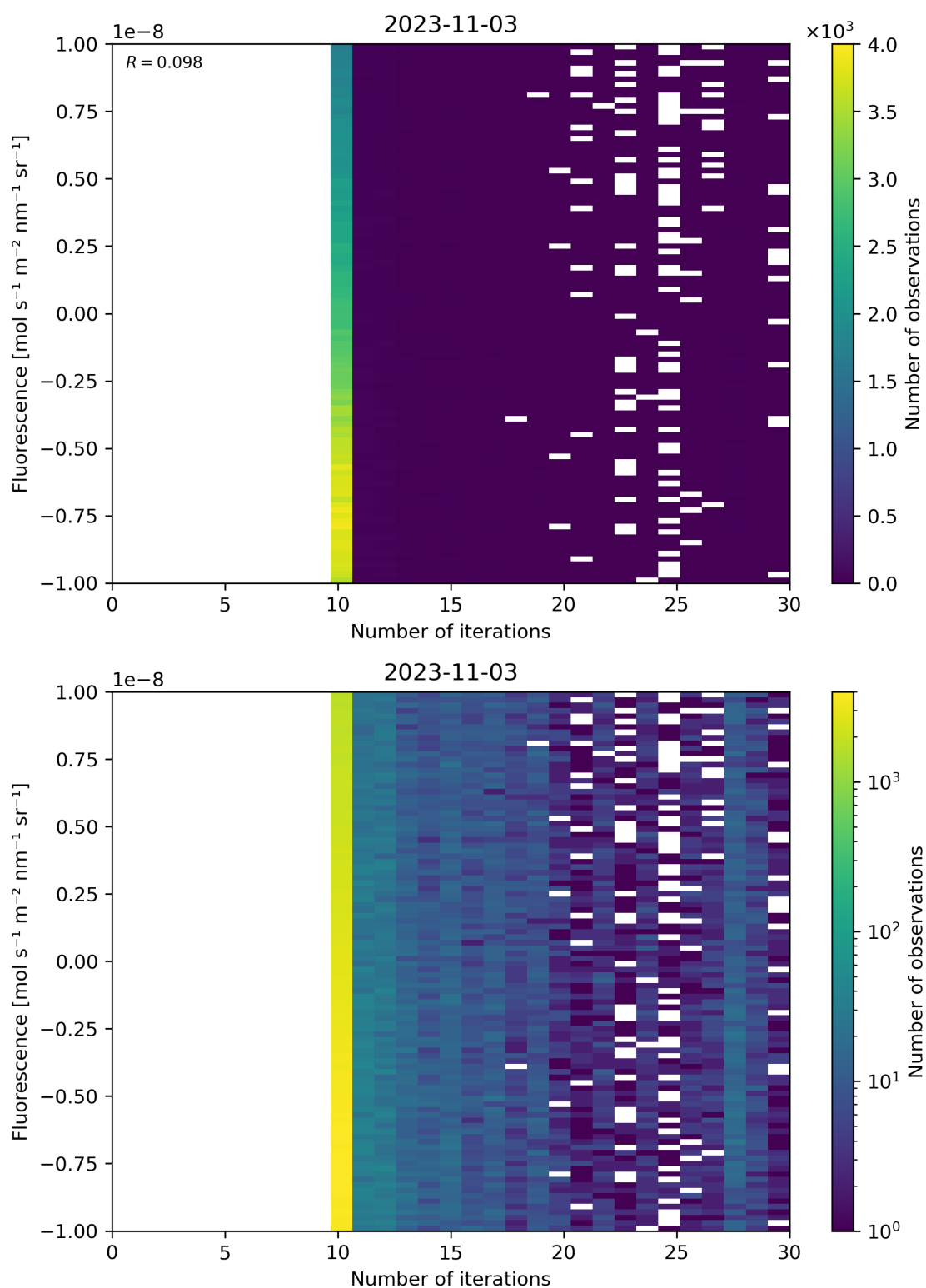
Figure 87: Scatter density plot of “Number of iterations” against “Fluorescence” for 2023-11-02 to 2023-11-04.
