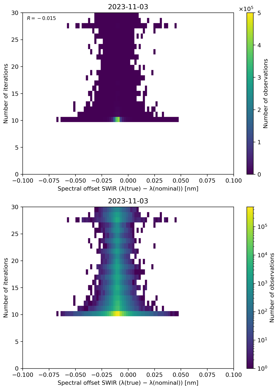
Figure 121: Scatter density plot of “Spectral offset SWIR ( \lambda(\text{true}) - \lambda(\text{nominal}) )” against “Number of iterations” for 2023-11-02 to 2023-11-04.
