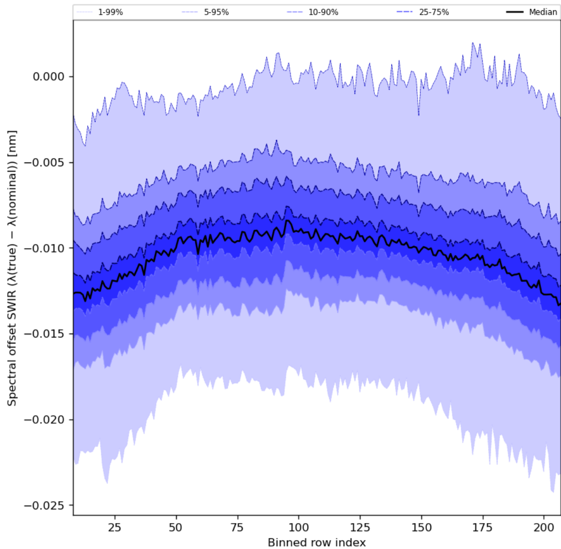
Figure 38: Along track statistics of “Spectral offset SWIR ( \lambda(\text{true}) - \lambda(\text{nominal}) )” for 2023-11-02 to 2023-11-04
