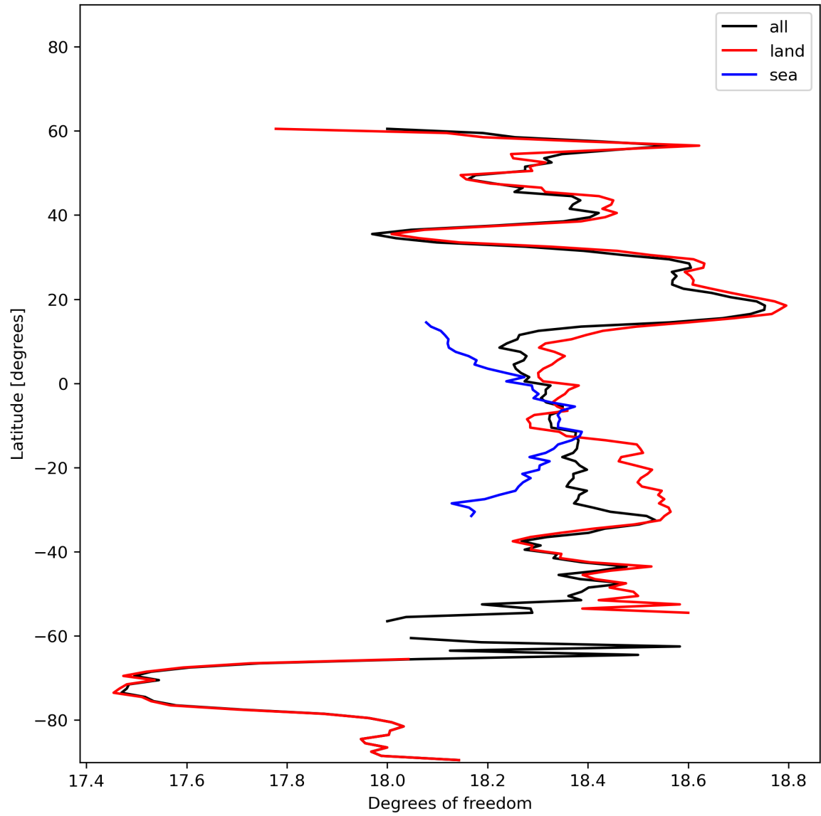
Figure 19: Zonal average of “Degrees of freedom” for 2023-11-02 to 2023-11-04.
