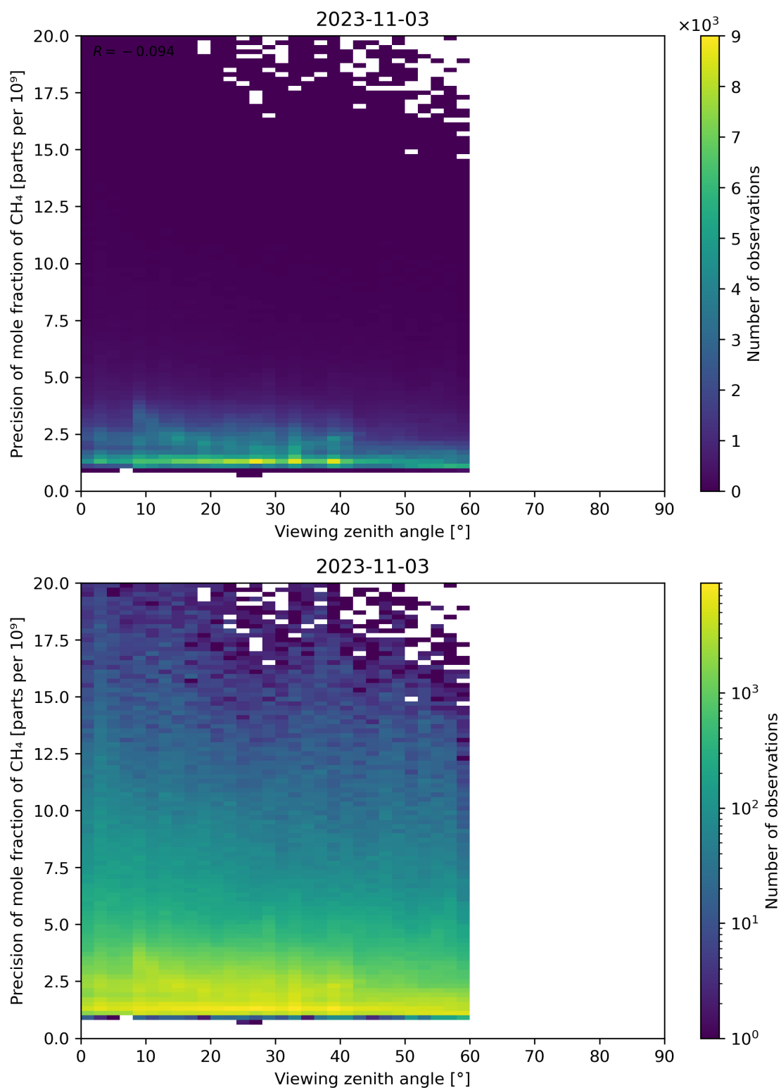
Figure 112: Scatter density plot of “Viewing zenith angle” against “Precision of mole fraction of CH 4 ” for 2023-11-02 to 2023-11-04.
