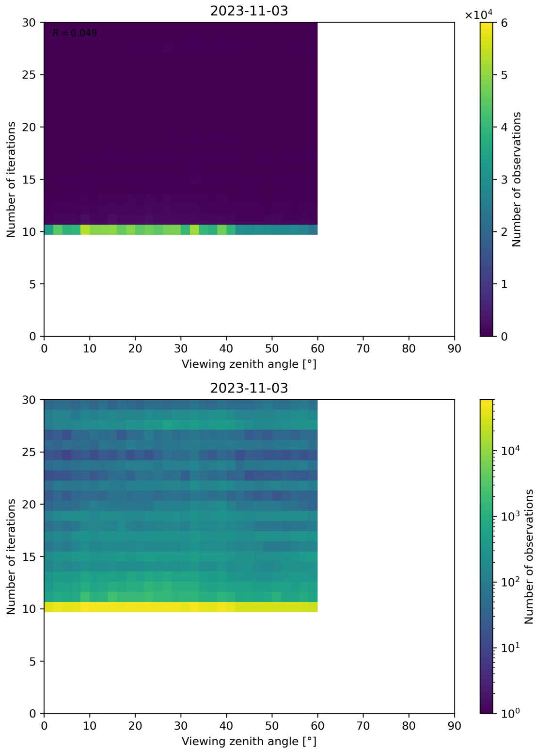
Figure 113: Scatter density plot of “Viewing zenith angle” against “Number of iterations” for 2023-11-02 to 2023-11-04.
