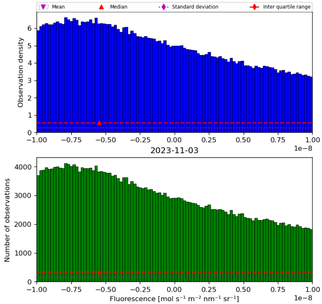
Figure 32: Histogram of “Fluorescence” for 2023-11-02 to 2023-11-04
