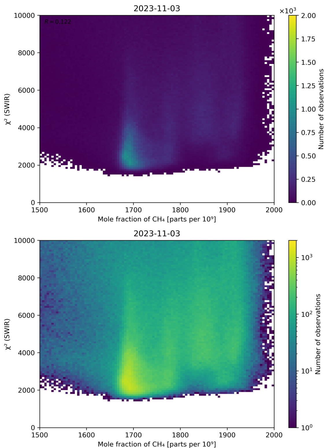
Figure 71: Scatter density plot of “Mole fraction of \text{CH}_4 ” against “ \chi^2 (SWIR)” for 2023-11-02 to 2023-11-04.
