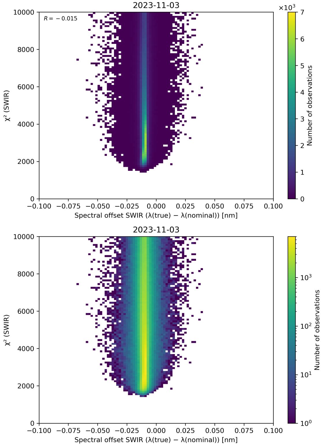
Figure 118: Scatter density plot of “Spectral offset SWIR ( \lambda(\text{true}) - \lambda(\text{nominal}) )” against “ \chi^2 (SWIR)” for 2023-11-02 to 2023-11-04.
