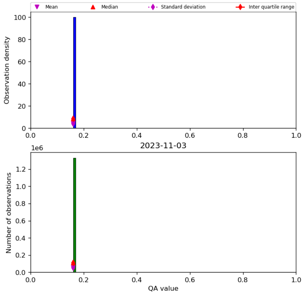
Figure 22: Histogram of “QA value” for 2023-11-02 to 2023-11-04
