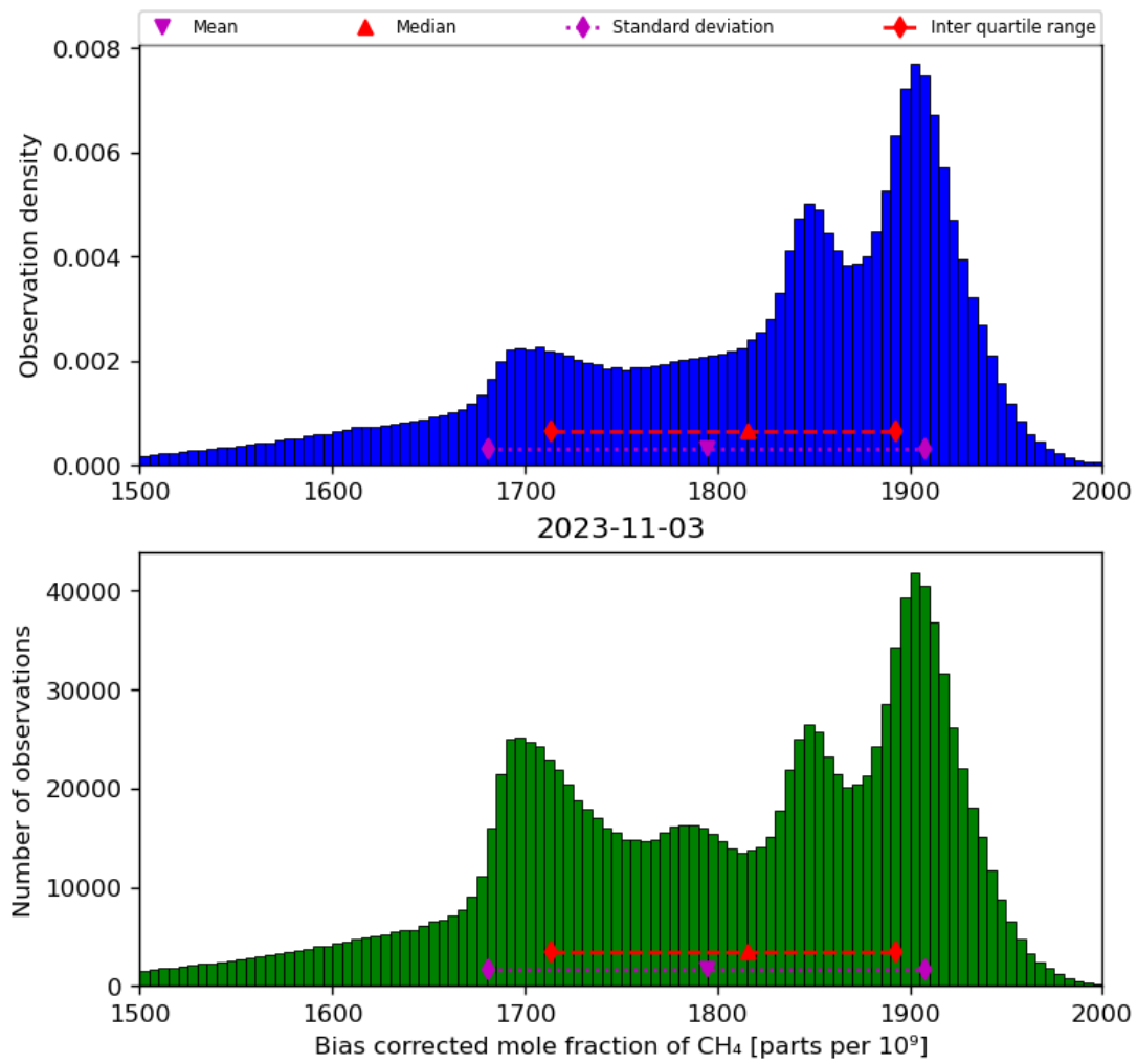
Figure 25: Histogram of “Bias corrected mole fraction of CH 4 ” for 2023-11-02 to 2023-11-04
