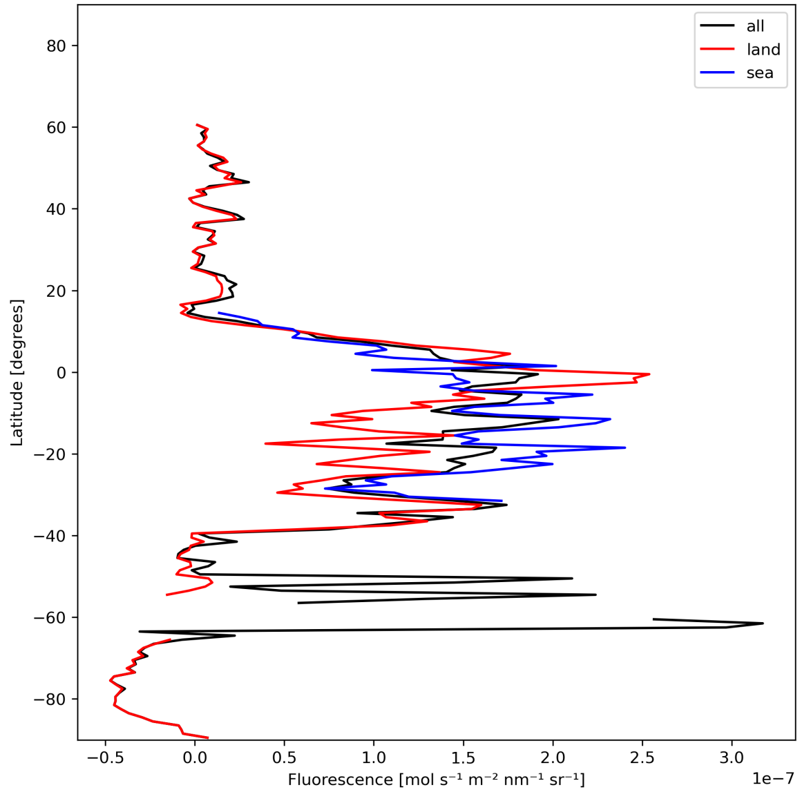
Figure 21: Zonal average of “Fluorescence” for 2023-11-02 to 2023-11-04.
