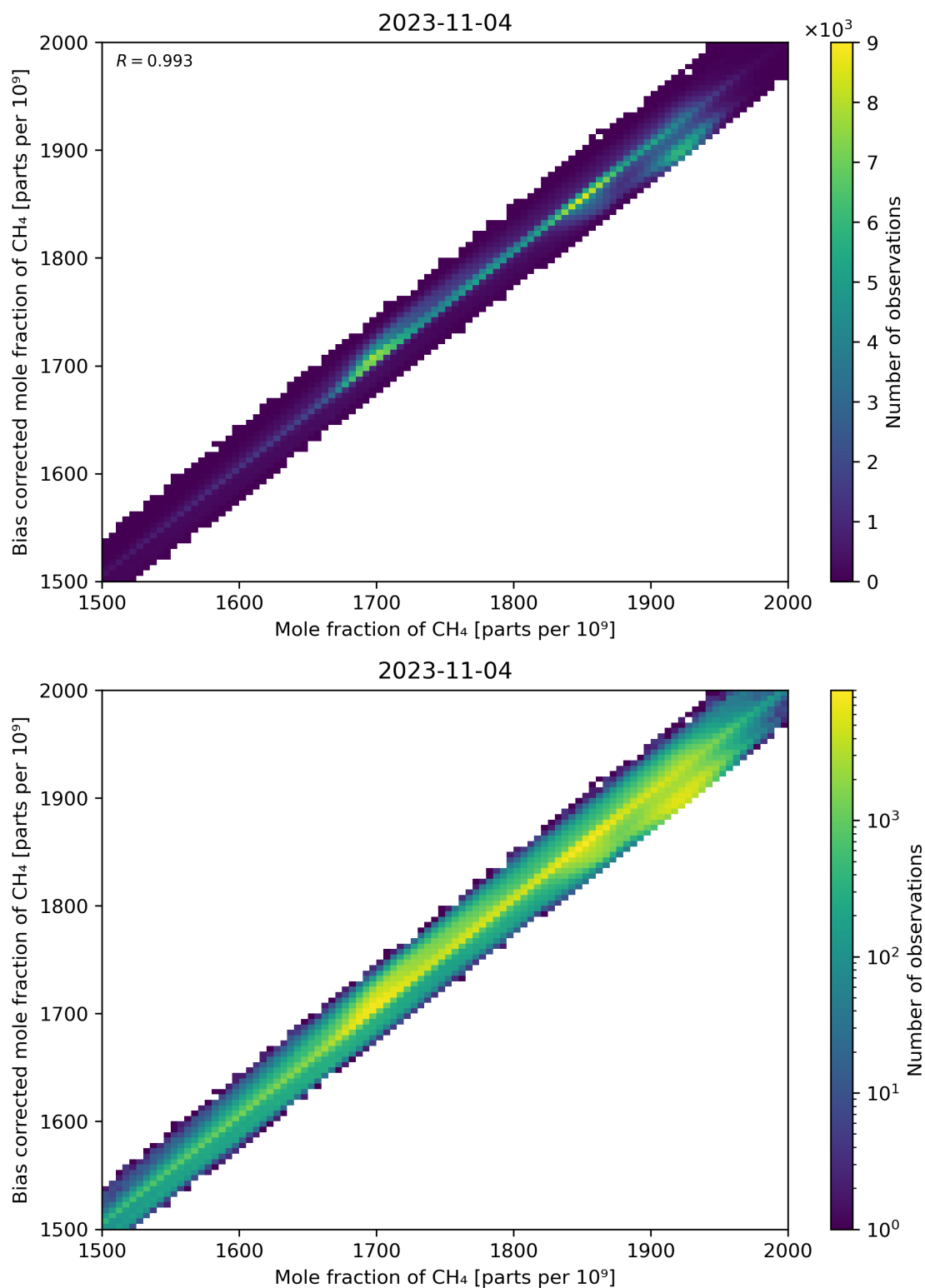
Figure 74: Scatter density plot of “Mole fraction of CH 4 ” against “Bias corrected mole fraction of CH 4 ” for 2023-11-03 to 2023-11-05.
