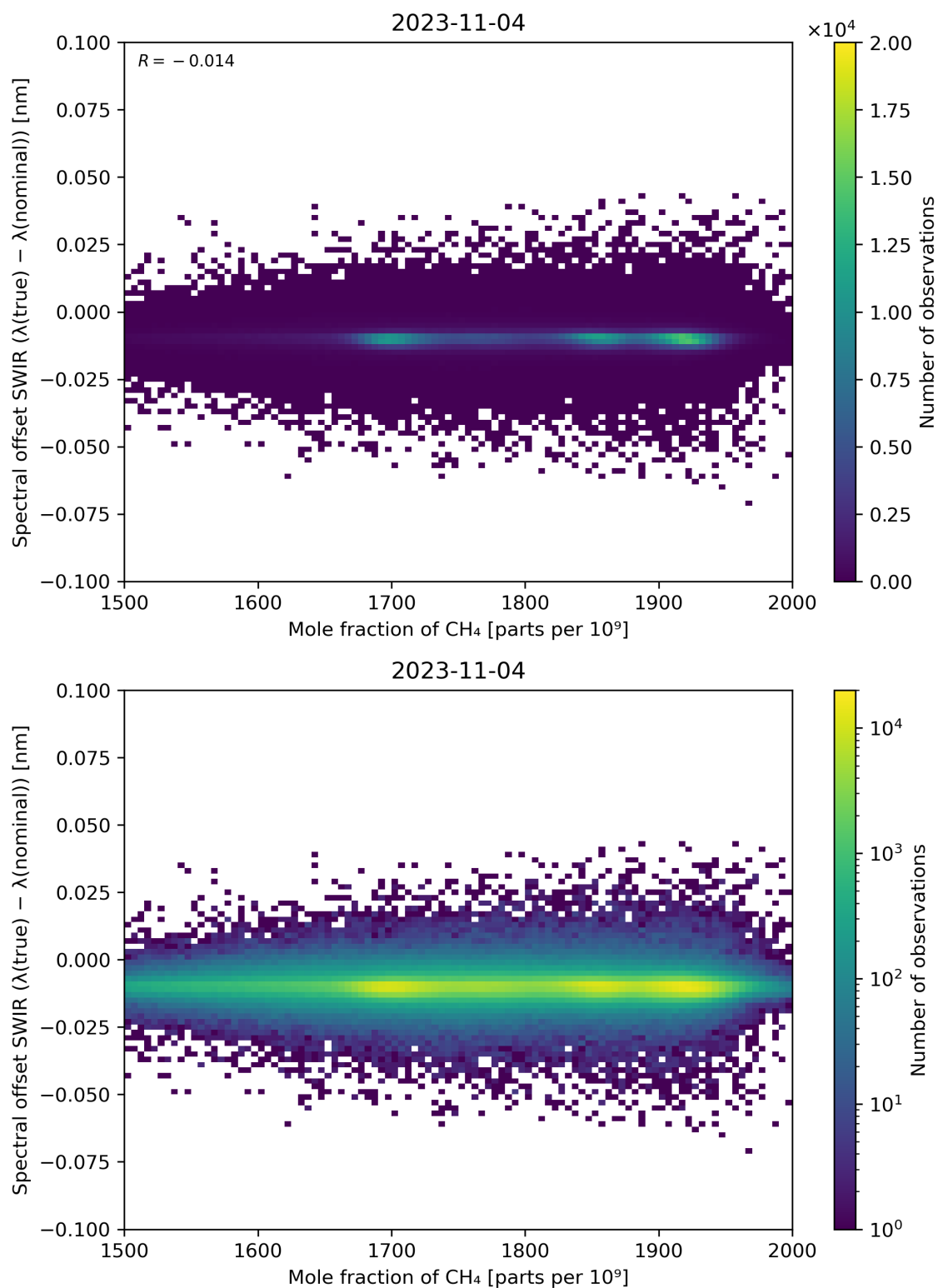
Figure 86: Scatter density plot of “Mole fraction of \text{CH}_4 ” against “Spectral offset SWIR ( \lambda(\text{true}) - \lambda(\text{nominal}) )” for 2023-11-03 to 2023-11-05.
