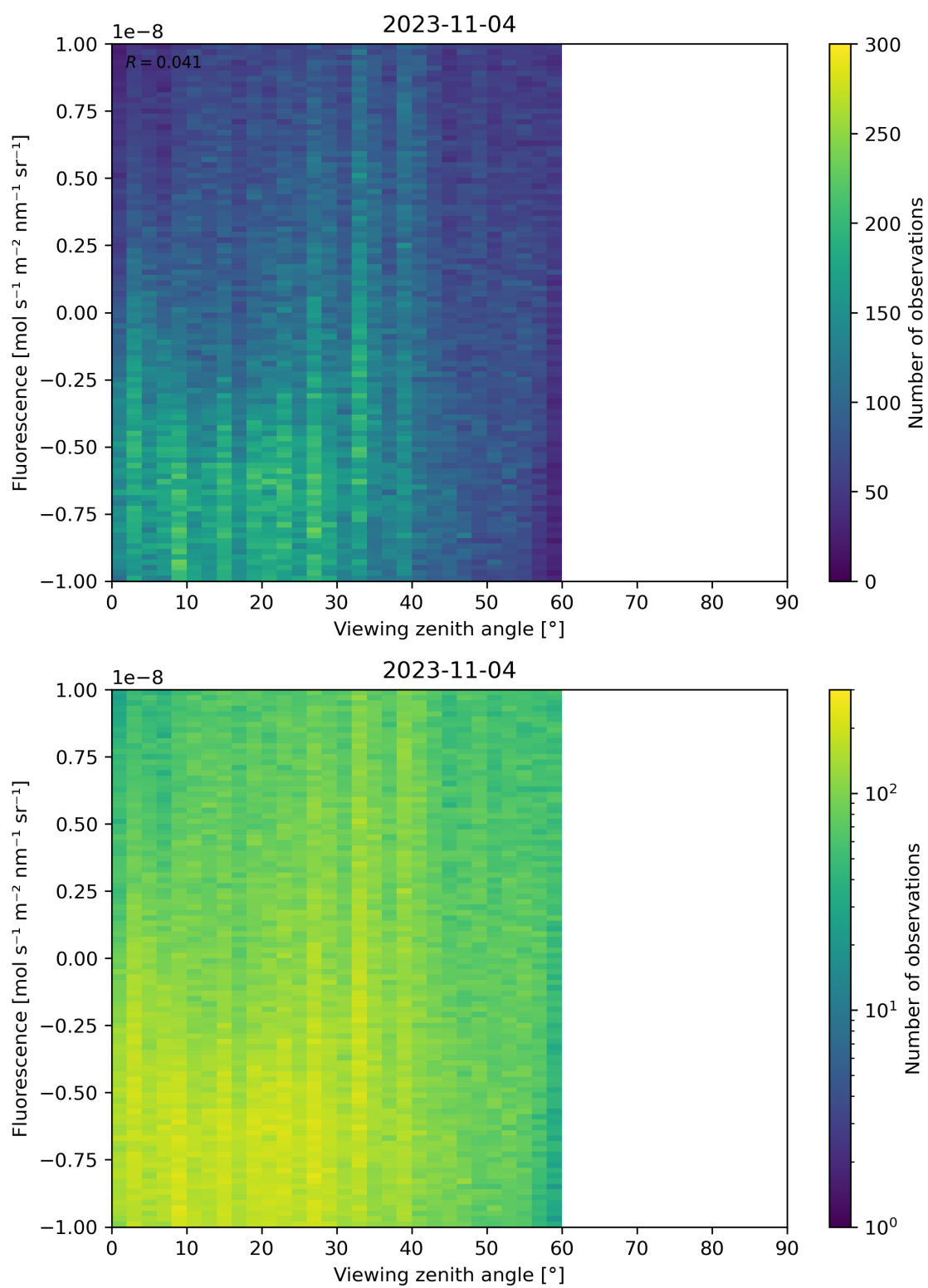
Figure 108: Scatter density plot of “Viewing zenith angle” against “Fluorescence” for 2023-11-03 to 2023-11-05.
