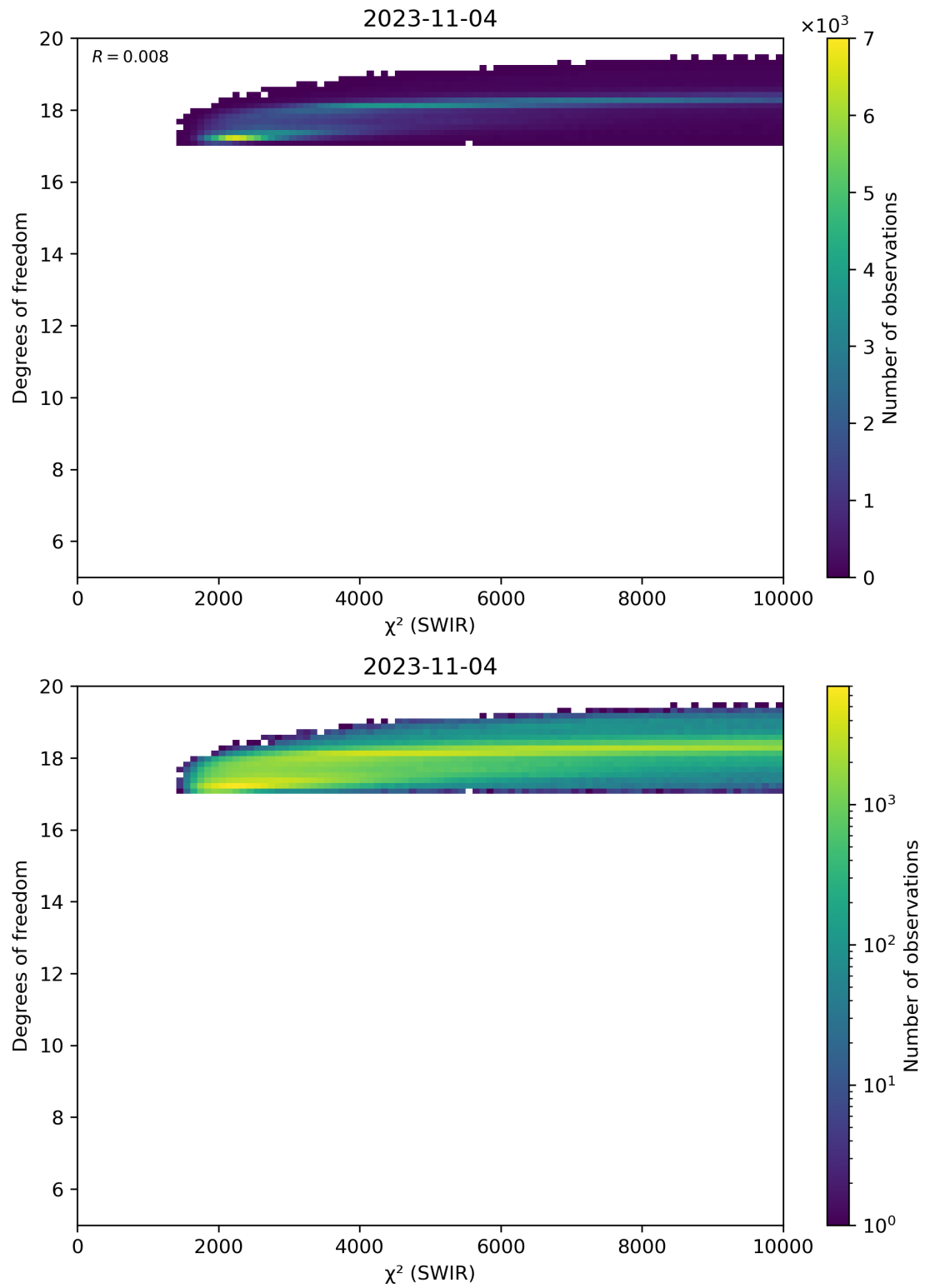
Figure 48: Scatter density plot of “ \chi^2 (SWIR)” against “Degrees of freedom” for 2023-11-03 to 2023-11-05.
