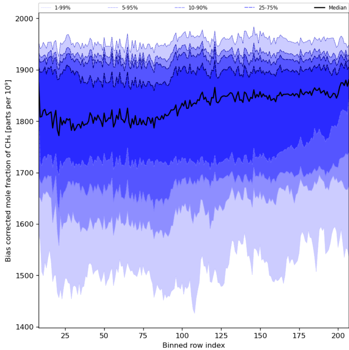
Figure 36: Along track statistics of “Bias corrected mole fraction of CH 4 ” for 2023-11-03 to 2023-11-05
