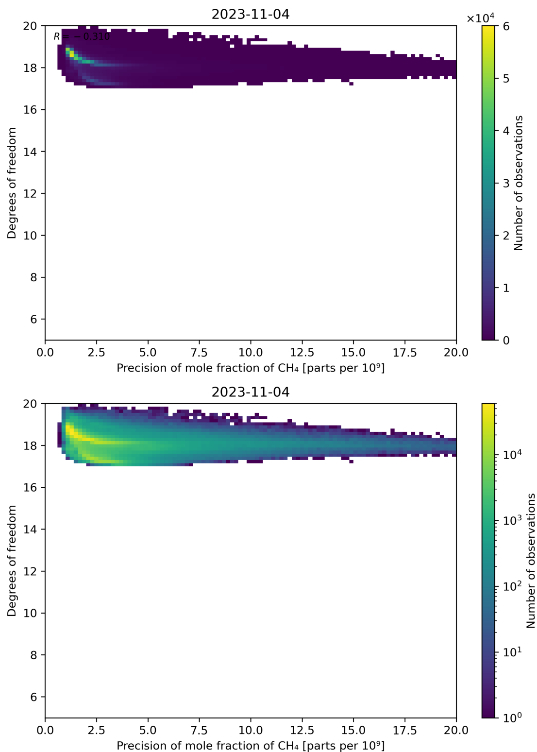
Figure 80: Scatter density plot of “Precision of mole fraction of CH 4 ” against “Degrees of freedom” for 2023-11-03 to 2023-11-05.
