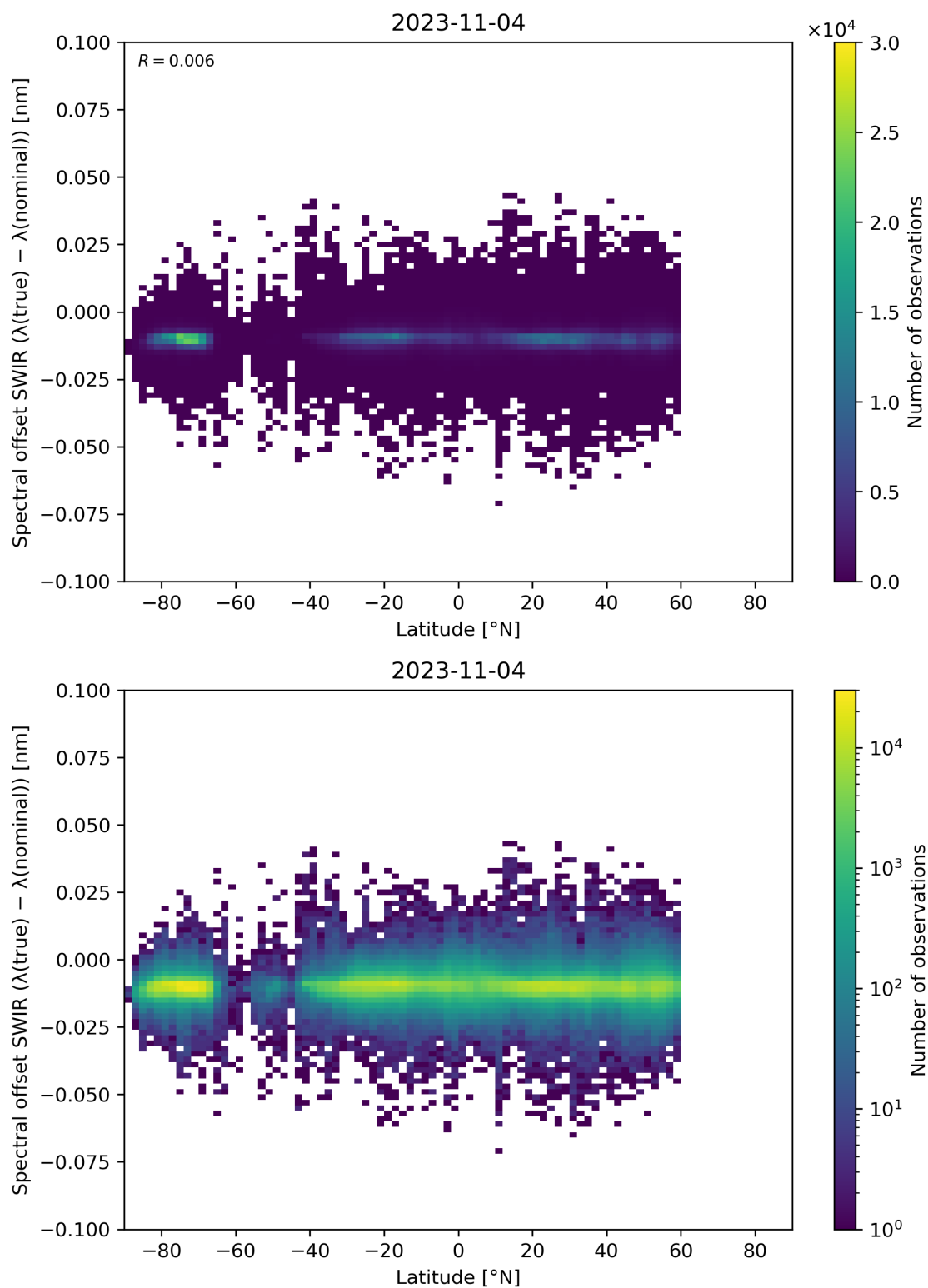
Figure 62: Scatter density plot of “Latitude” against “Spectral offset SWIR ( \lambda(\text{true}) - \lambda(\text{nominal}) )” for 2023-11-03 to 2023-11-05.
