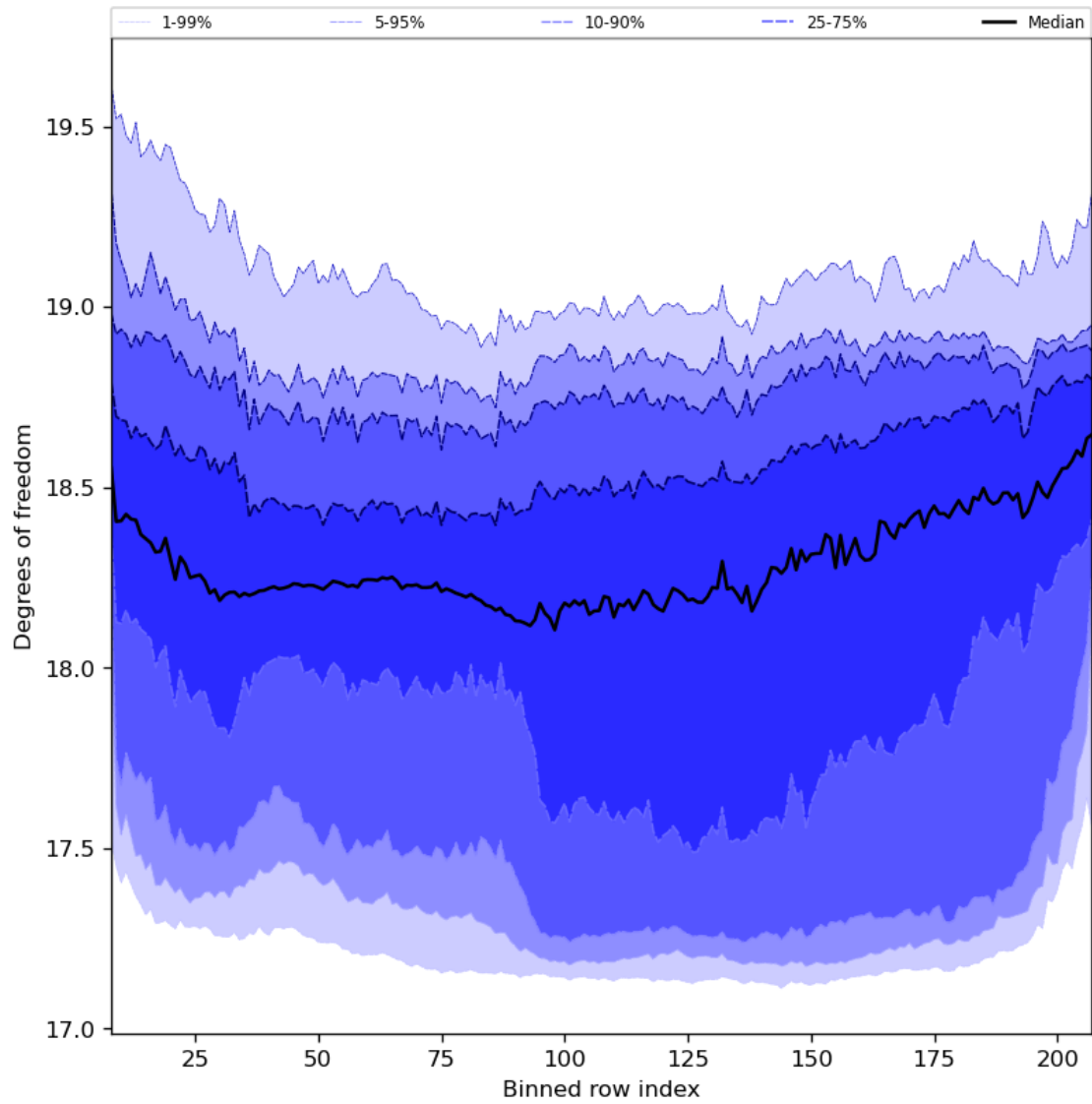
Figure 41: Along track statistics of “Degrees of freedom” for 2023-11-03 to 2023-11-05
