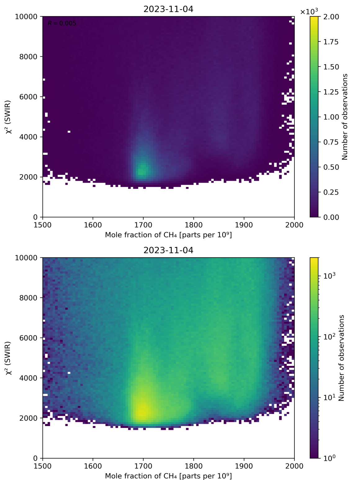
Figure 71: Scatter density plot of “Mole fraction of CH 4 ” against “ \chi^2 (SWIR)” for 2023-11-03 to 2023-11-05.
