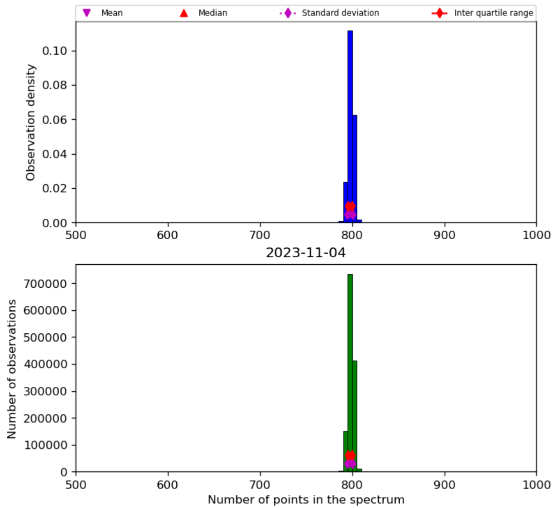
Figure 26: Histogram of “Number of points in the spectrum” for 2023-11-03 to 2023-11-05
