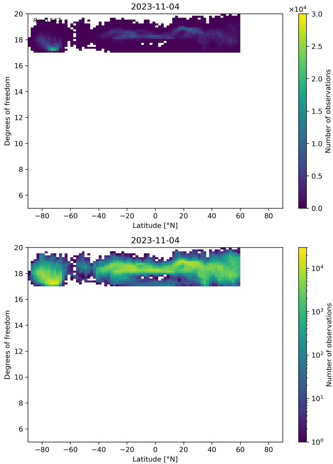
Figure 55: Scatter density plot of “Latitude” against “Degrees of freedom” for 2023-11-03 to 2023-11-05.
