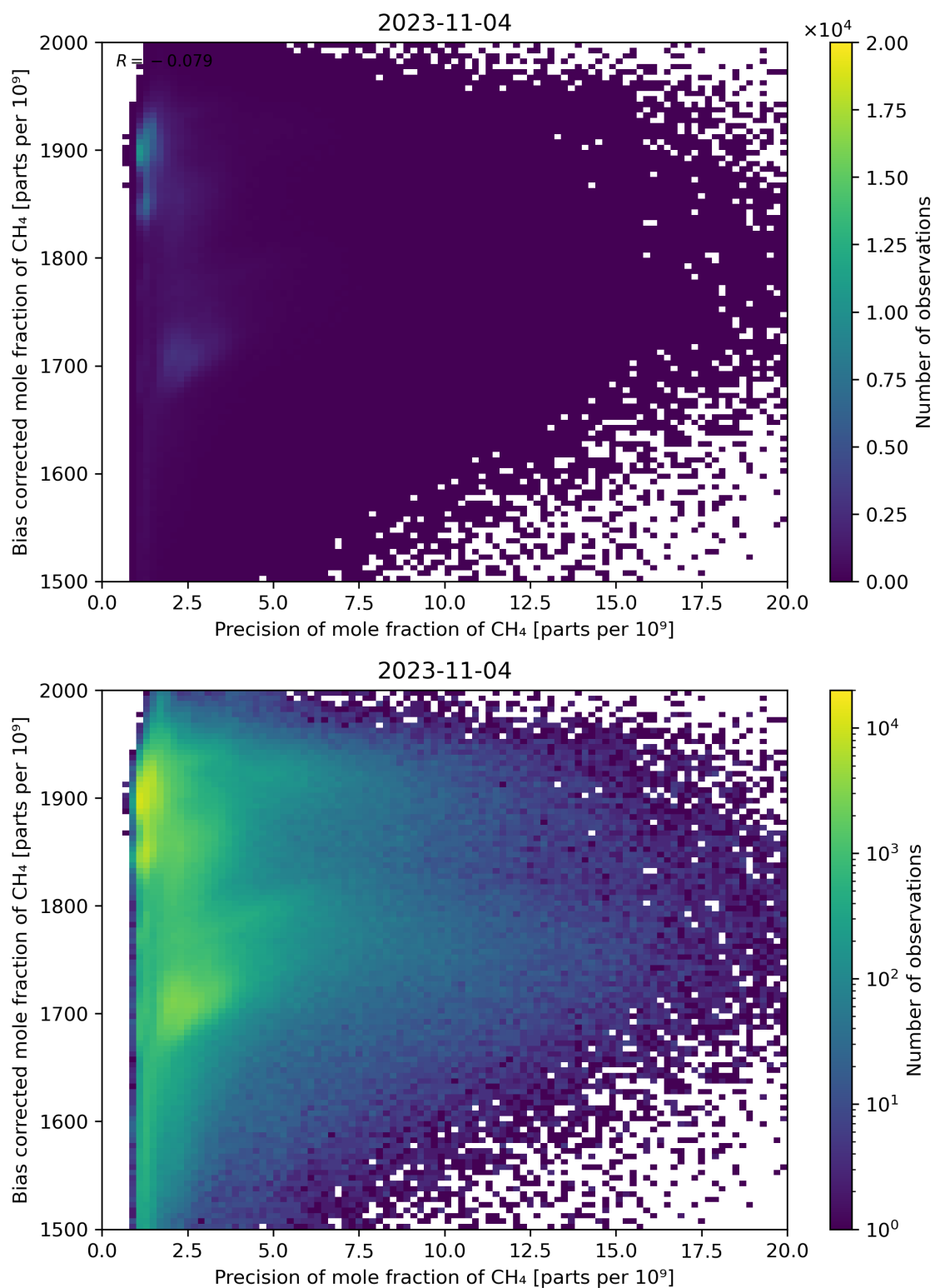
Figure 82: Scatter density plot of “Precision of mole fraction of CH 4 ” against “Bias corrected mole fraction of CH 4 ” for 2023-11-03 to 2023-11-05.
