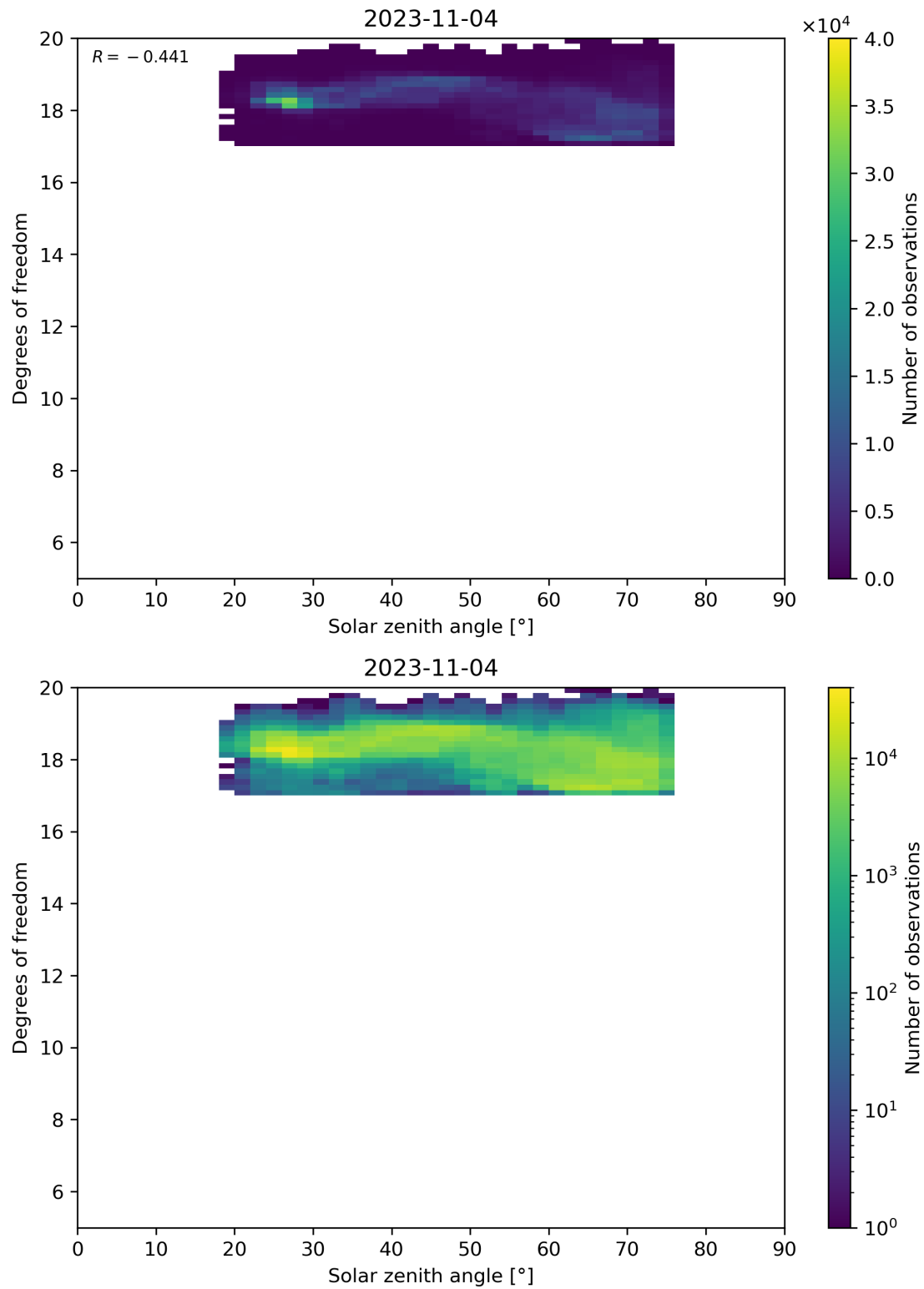
Figure 96: Scatter density plot of “Solar zenith angle” against “Degrees of freedom” for 2023-11-03 to 2023-11-05.
