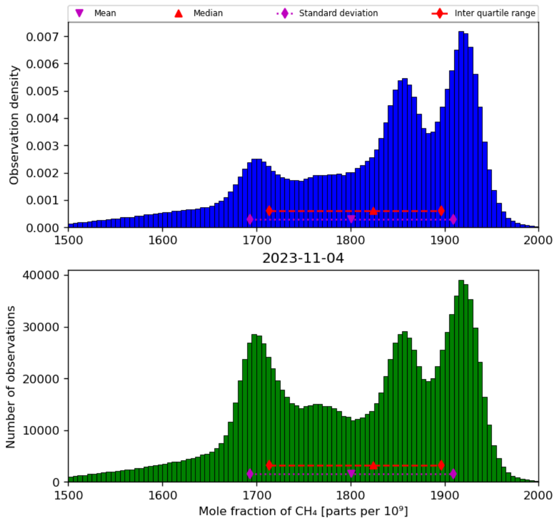
Figure 23: Histogram of “Mole fraction of CH 4 ” for 2023-11-03 to 2023-11-05
