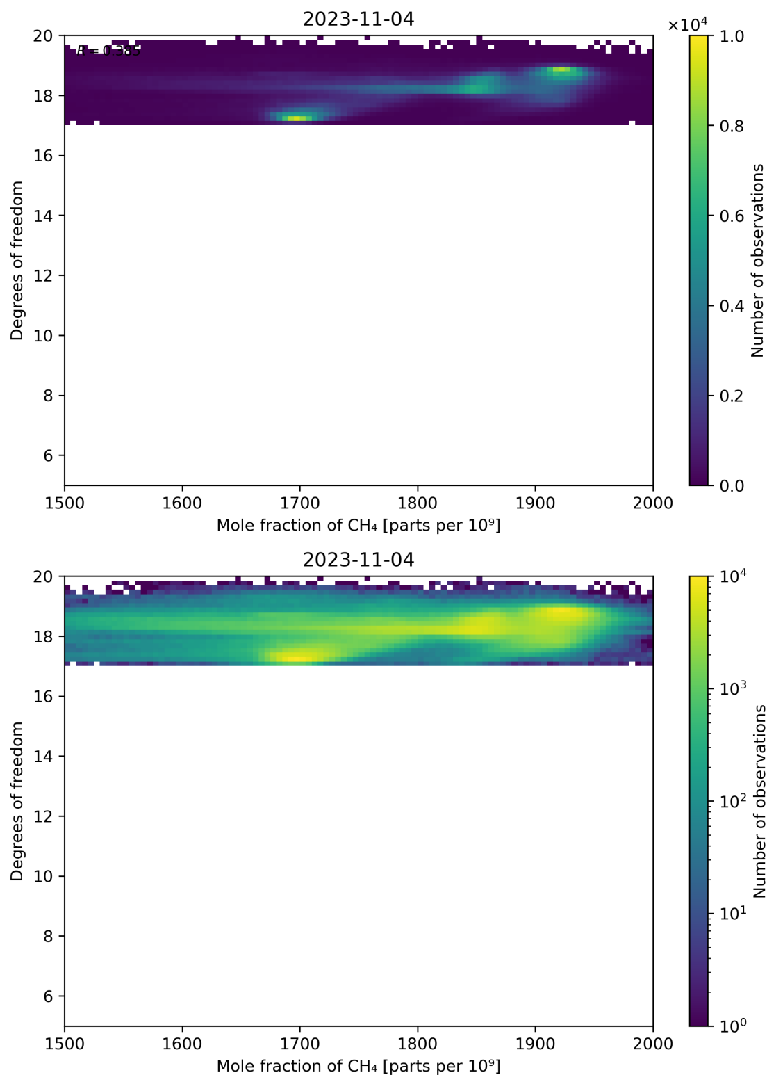
Figure 72: Scatter density plot of “Mole fraction of CH 4 ” against “Degrees of freedom” for 2023-11-03 to 2023-11-05.
