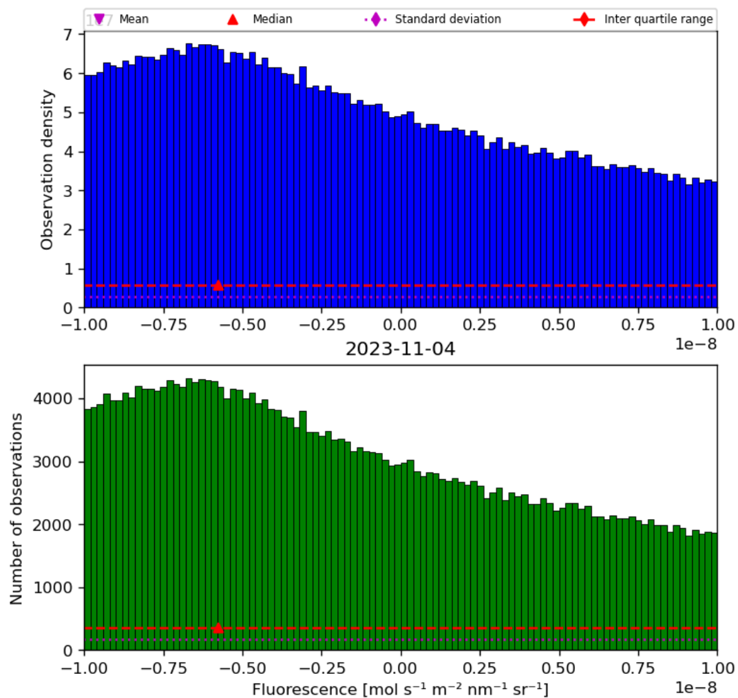
Figure 32: Histogram of “Fluorescence” for 2023-11-03 to 2023-11-05
