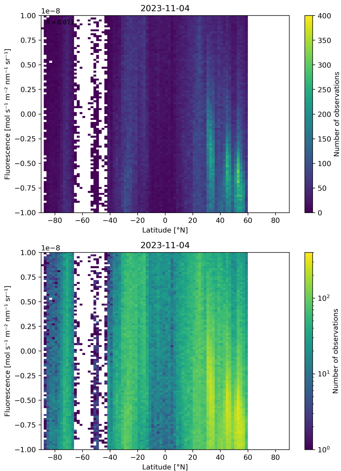
Figure 56: Scatter density plot of “Latitude” against “Fluorescence” for 2023-11-03 to 2023-11-05.
