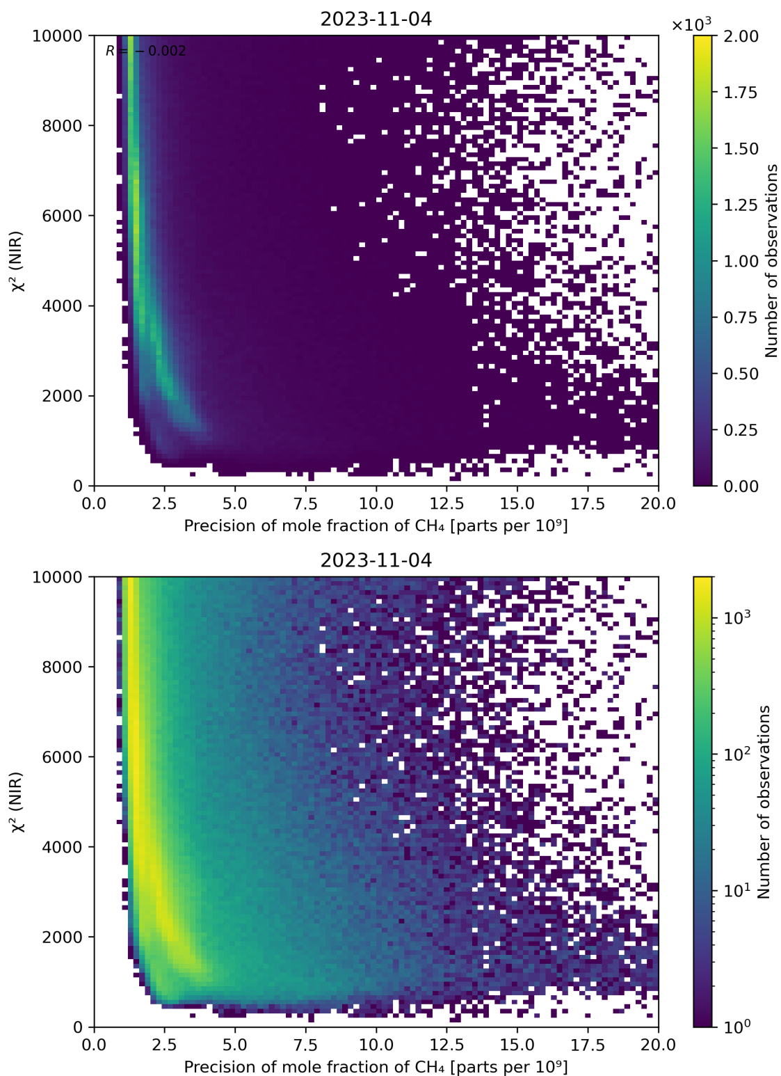
Figure 78: Scatter density plot of “Precision of mole fraction of \text{CH}_4 ” against “ \chi^2 (NIR)” for 2023-11-03 to 2023-11-05.
