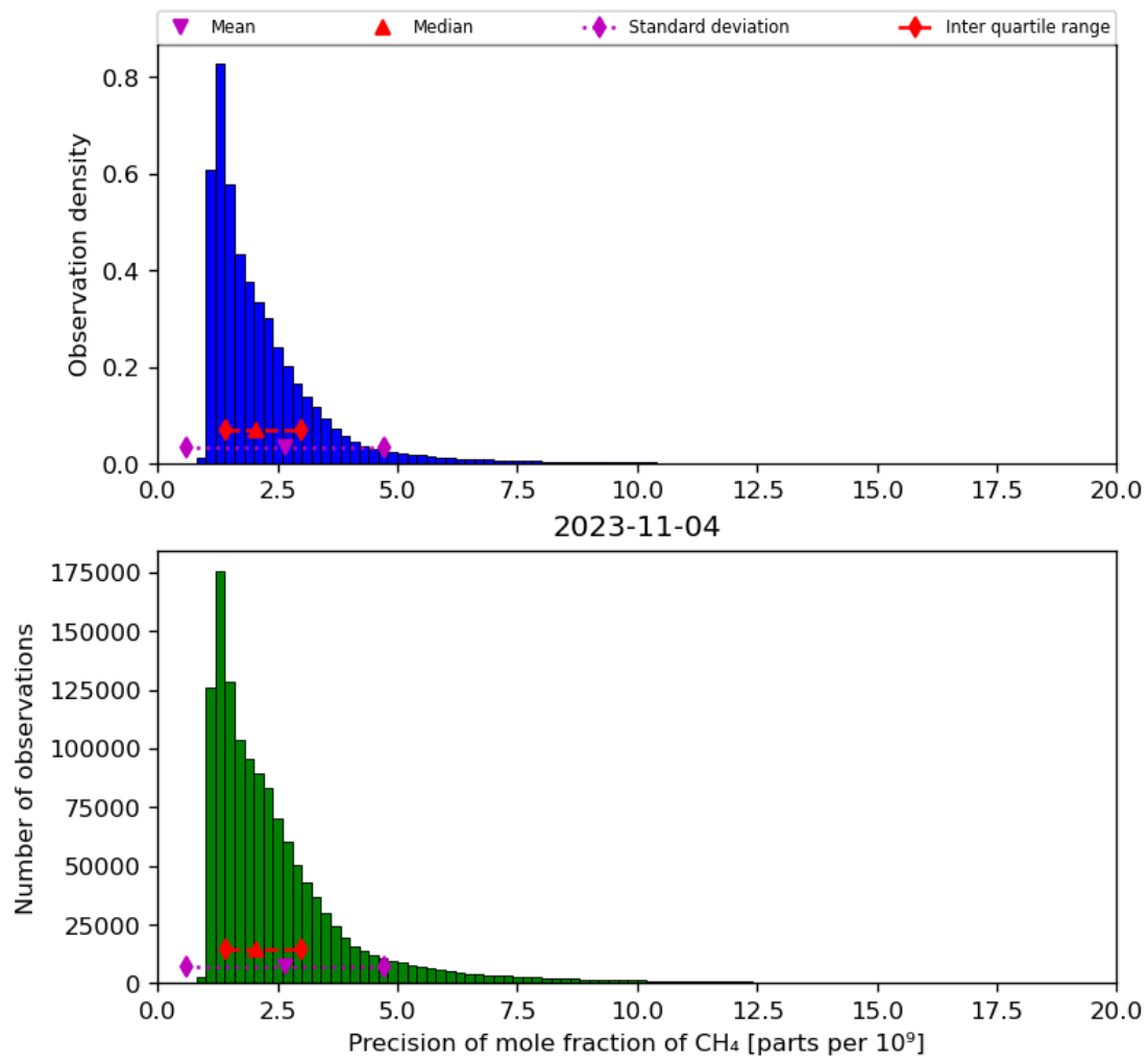
Figure 24: Histogram of “Precision of mole fraction of CH 4 ” for 2023-11-03 to 2023-11-05
