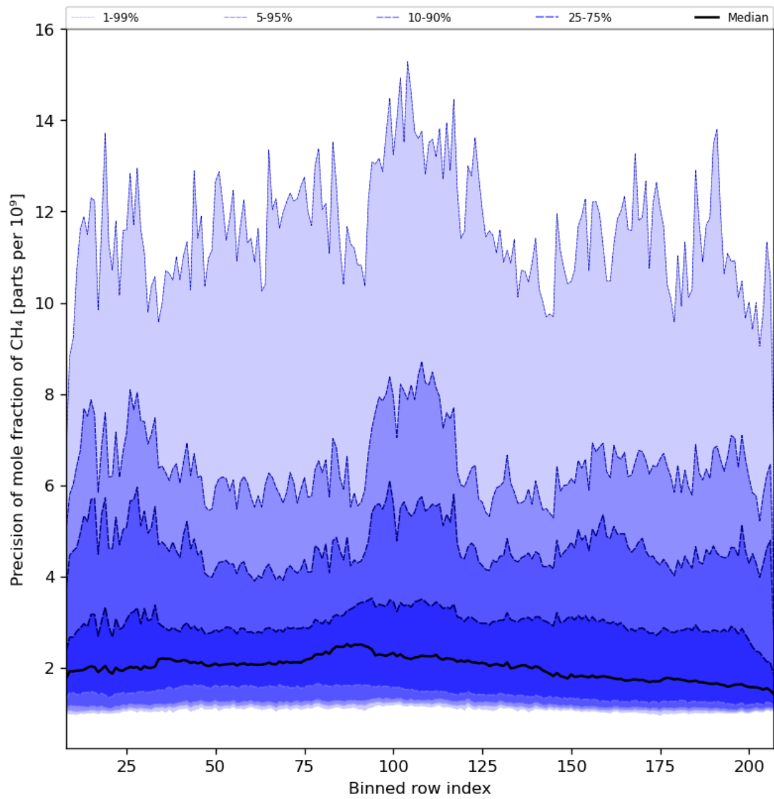
Figure 35: Along track statistics of “Precision of mole fraction of CH 4 ” for 2023-11-03 to 2023-11-05
