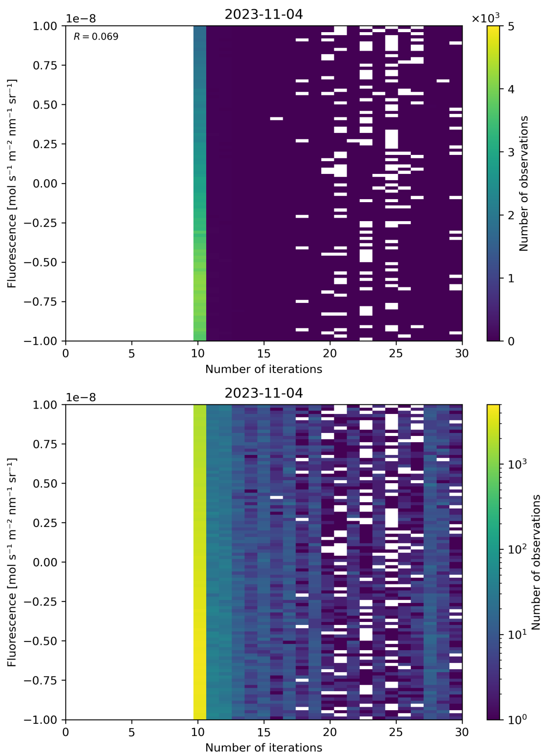
Figure 87: Scatter density plot of “Number of iterations” against “Fluorescence” for 2023-11-03 to 2023-11-05.
