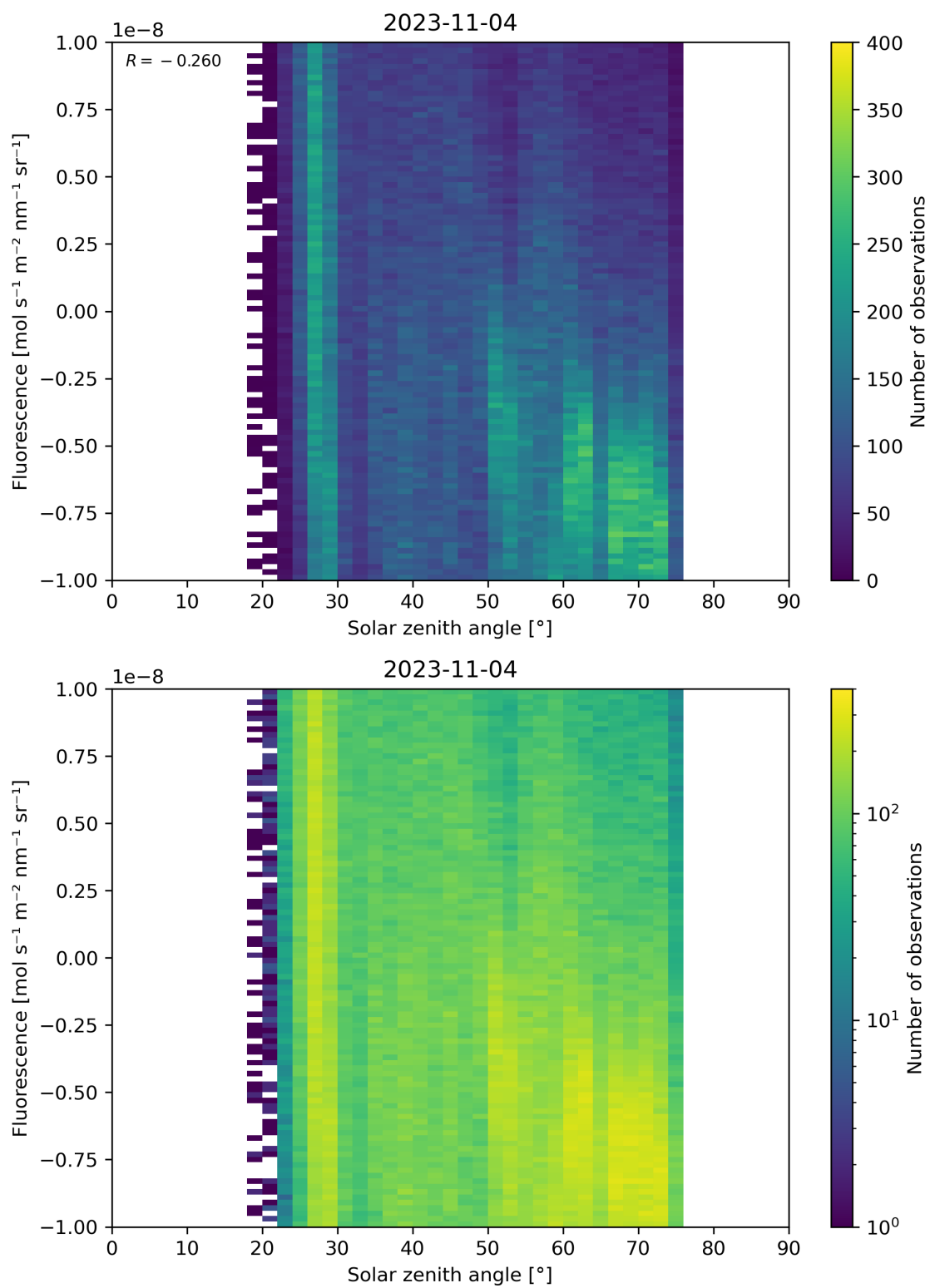
Figure 97: Scatter density plot of “Solar zenith angle” against “Fluorescence” for 2023-11-03 to 2023-11-05.
