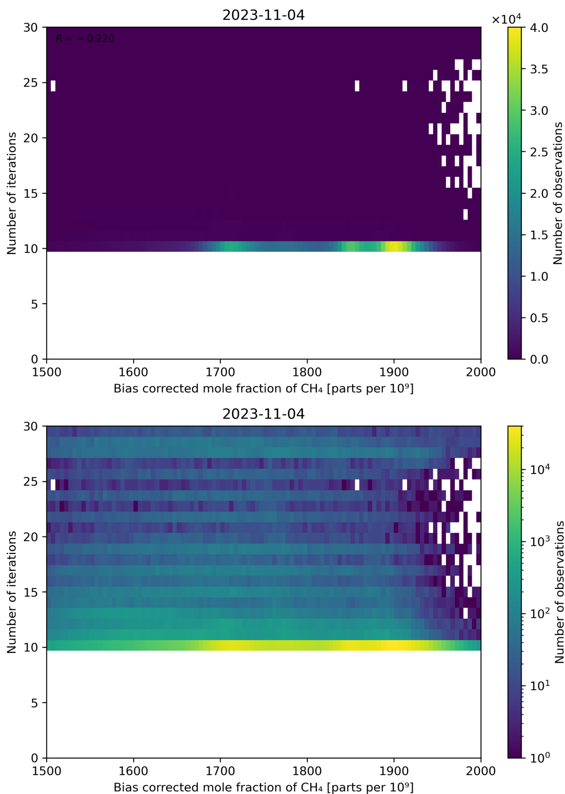
Figure 67: Scatter density plot of “Bias corrected mole fraction of CH 4 ” against “Number of iterations” for 2023-11-03 to 2023-11-05.
