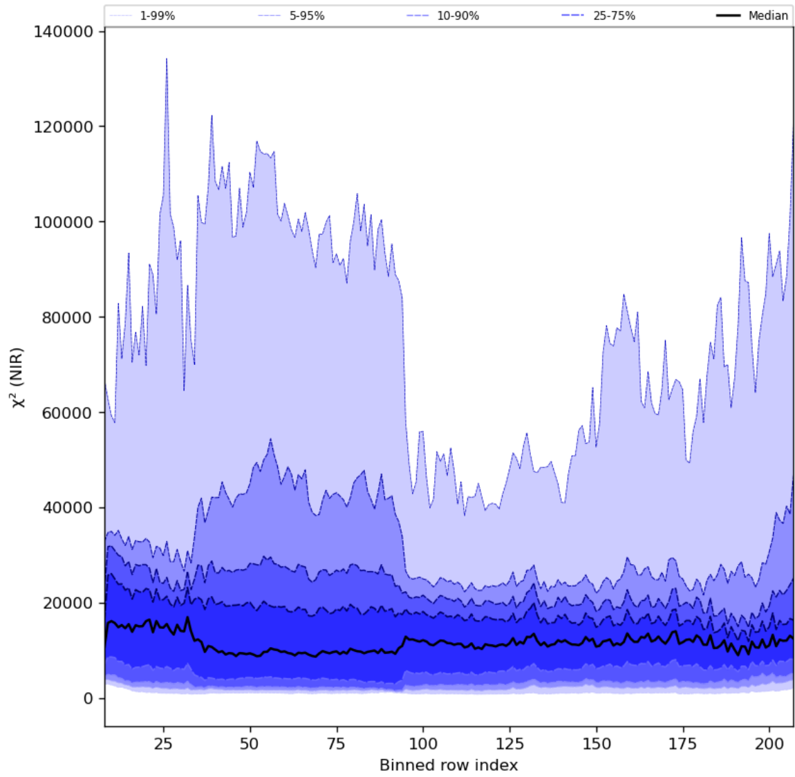
Figure 40: Along track statistics of “ \chi^2 (NIR)” for 2023-11-03 to 2023-11-05
