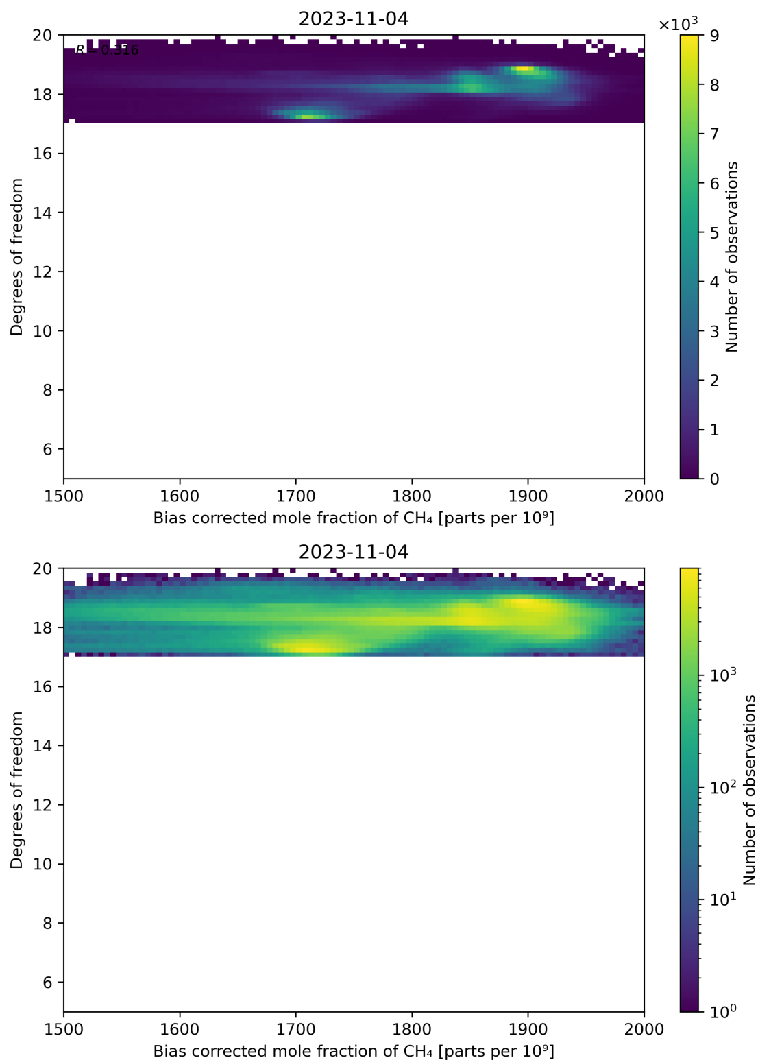
Figure 65: Scatter density plot of “Bias corrected mole fraction of CH 4 ” against “Degrees of freedom” for 2023-11-03 to 2023-11-05.
