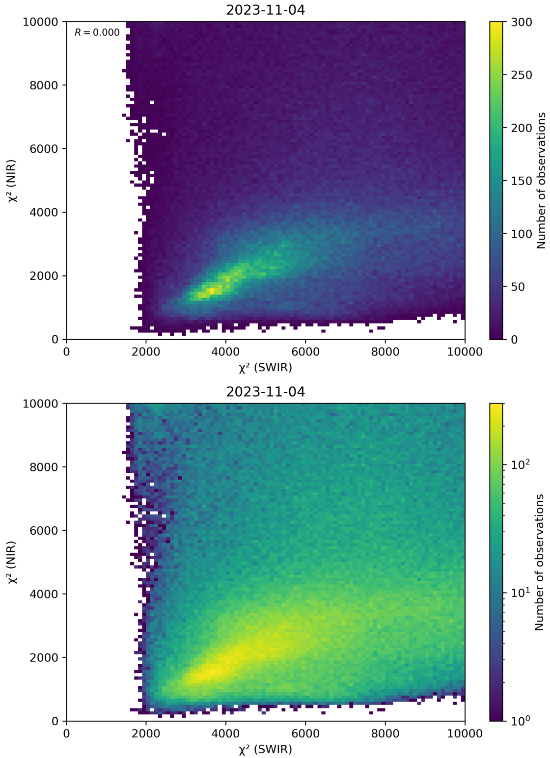
Figure 47: Scatter density plot of “ \chi^2 (SWIR)” against “ \chi^2 (NIR)” for 2023-11-03 to 2023-11-05.
