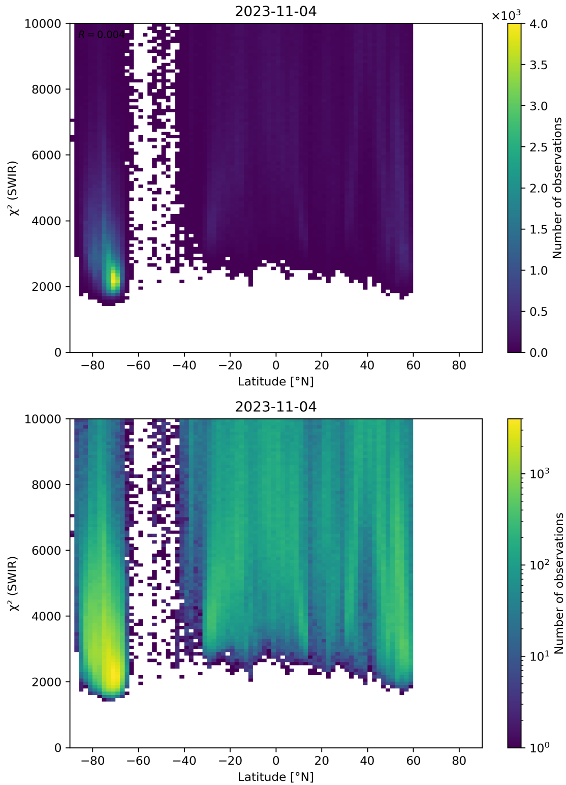
Figure 54: Scatter density plot of “Latitude” against “ \chi^2 (SWIR)” for 2023-11-03 to 2023-11-05.
