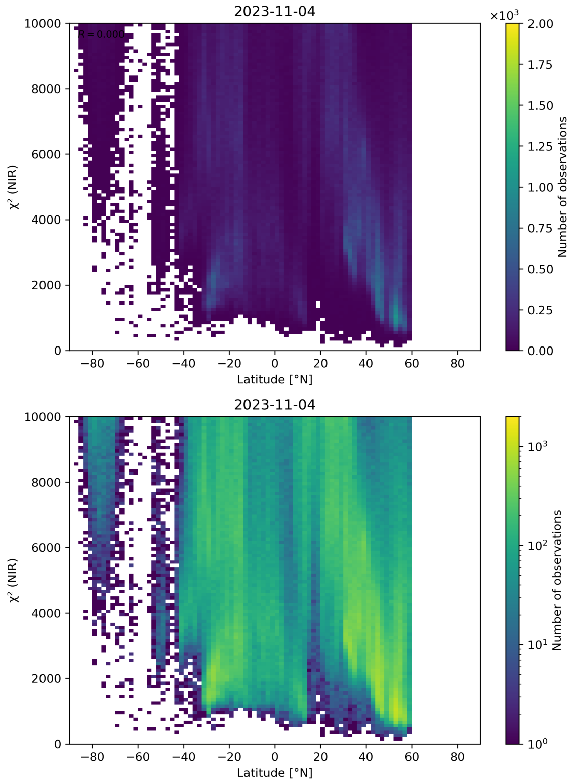
Figure 53: Scatter density plot of “Latitude” against “ \chi^2 (NIR)” for 2023-11-03 to 2023-11-05.
