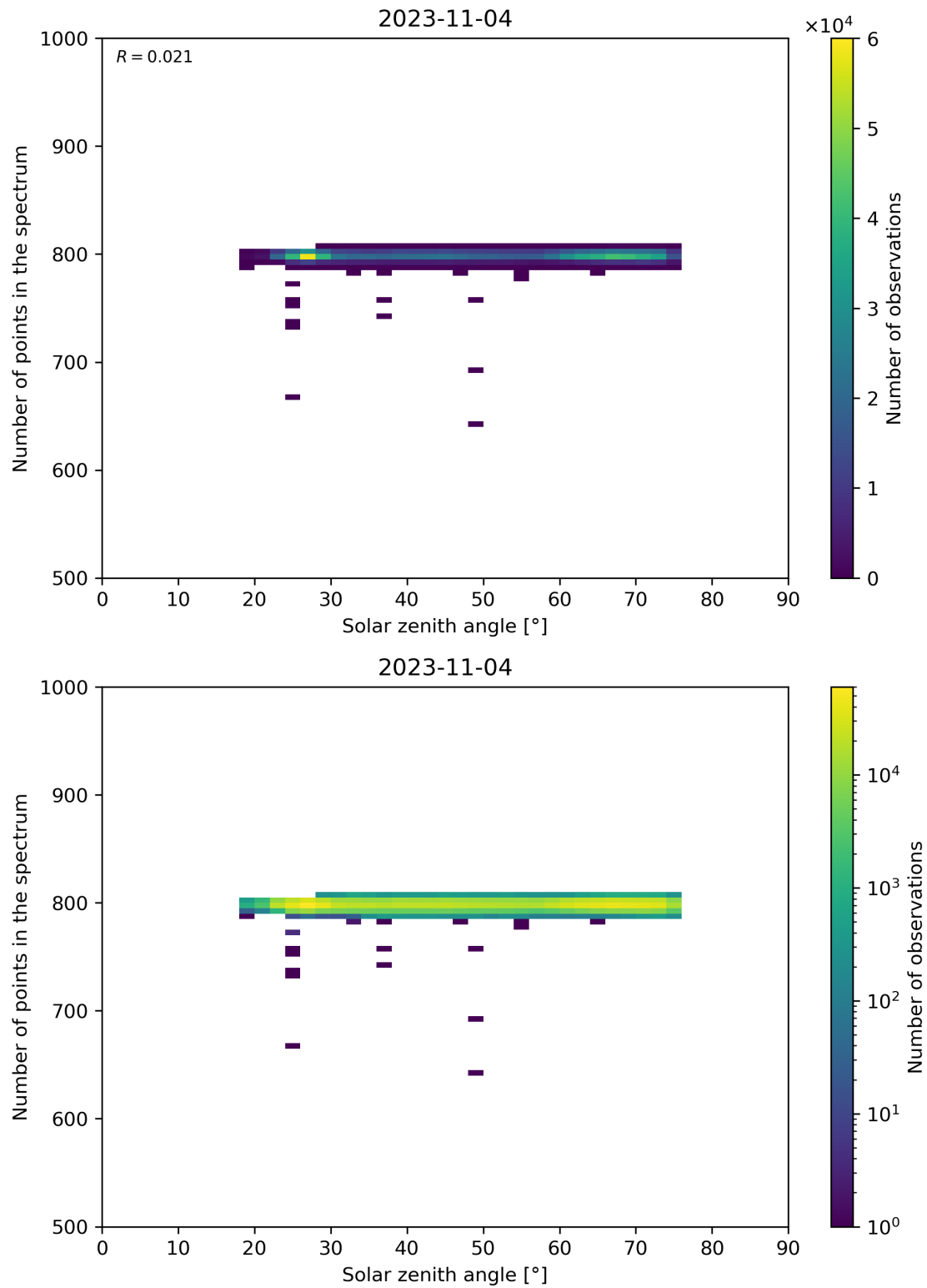
Figure 103: Scatter density plot of “Solar zenith angle” against “Number of points in the spectrum” for 2023-11-03 to 2023-11-05.
