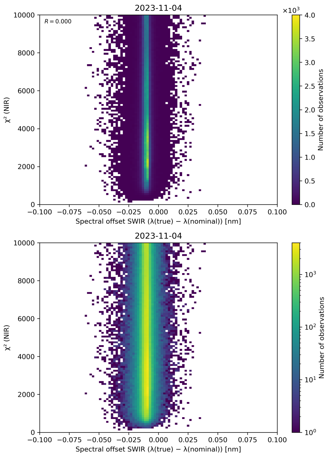
Figure 117: Scatter density plot of “Spectral offset SWIR ( \lambda(\text{true}) - \lambda(\text{nominal}) )” against “ \chi^2 (NIR)” for 2023-11-03 to 2023-11-05.
