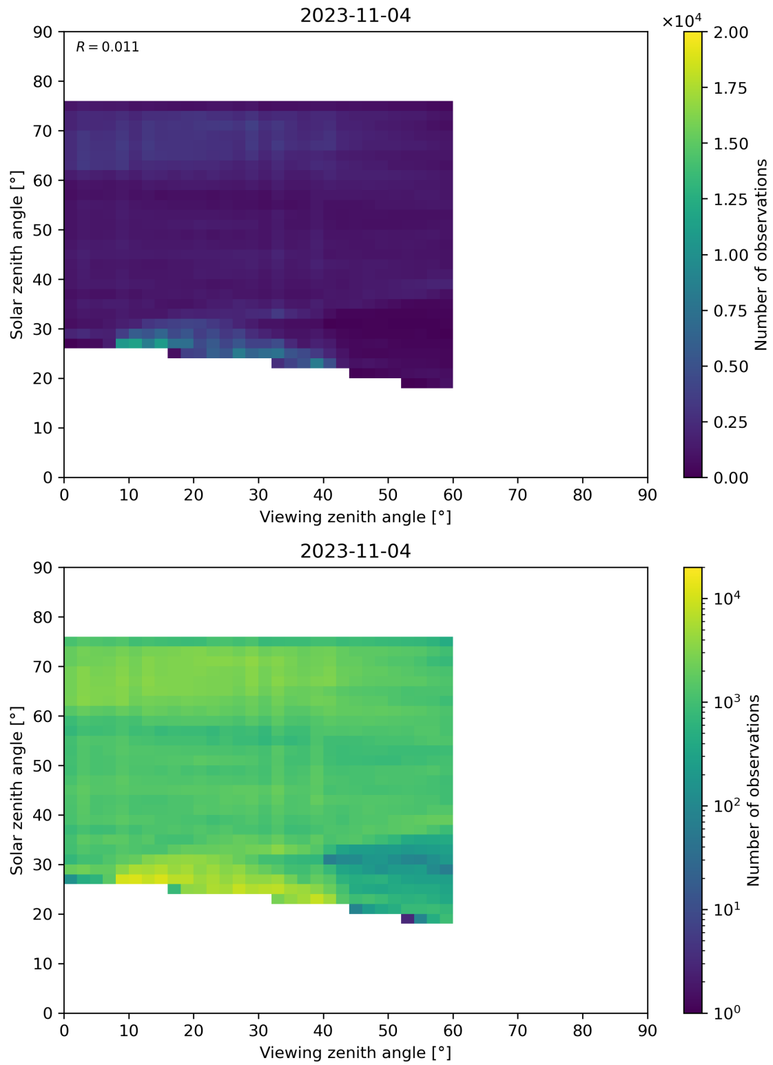
Figure 115: Scatter density plot of “Viewing zenith angle” against “Solar zenith angle” for 2023-11-03 to 2023-11-05.
