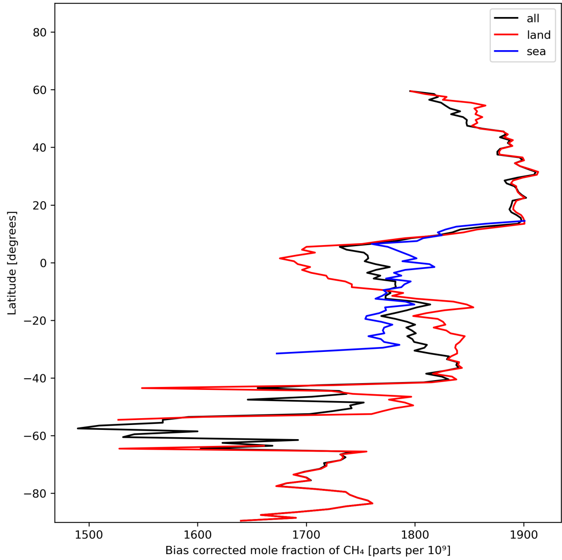
Figure 14: Zonal average of “Bias corrected mole fraction of CH 4 ” for 2023-11-03 to 2023-11-05.
