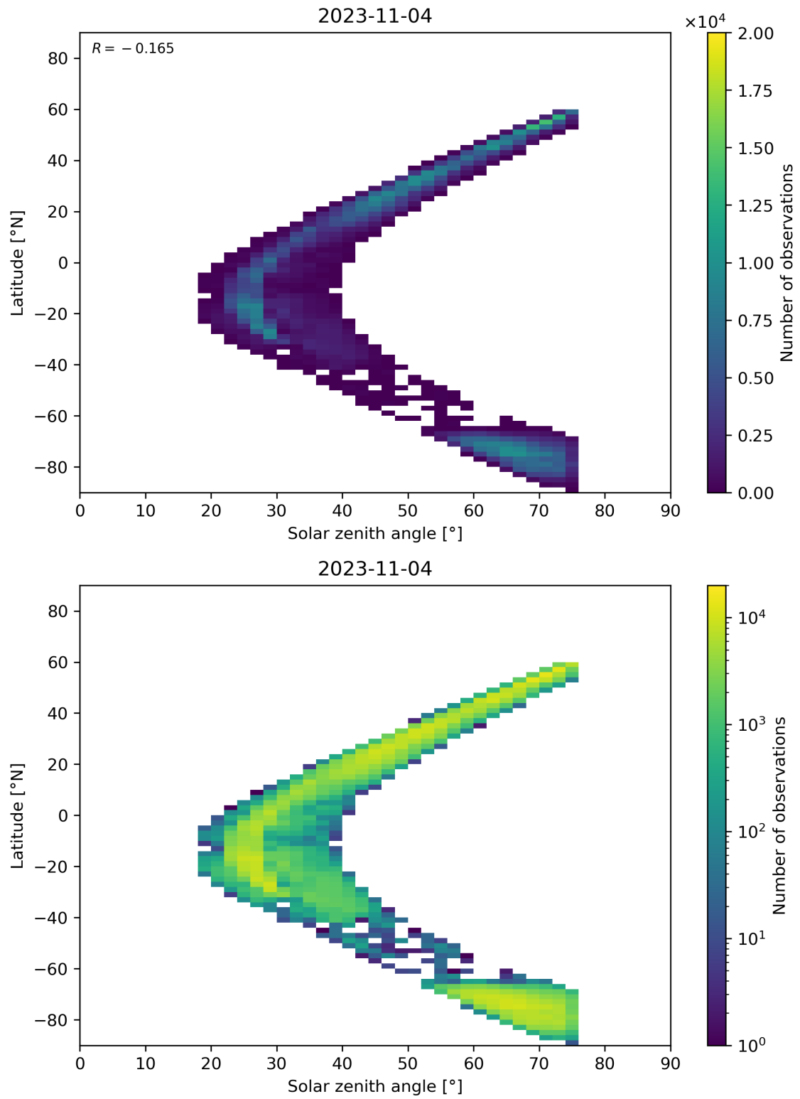
Figure 98: Scatter density plot of “Solar zenith angle” against “Latitude” for 2023-11-03 to 2023-11-05.
