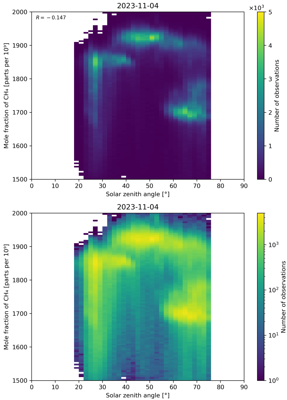
Figure 99: Scatter density plot of “Solar zenith angle” against “Mole fraction of \text{CH}_4 ” for 2023-11-03 to 2023-11-05.
