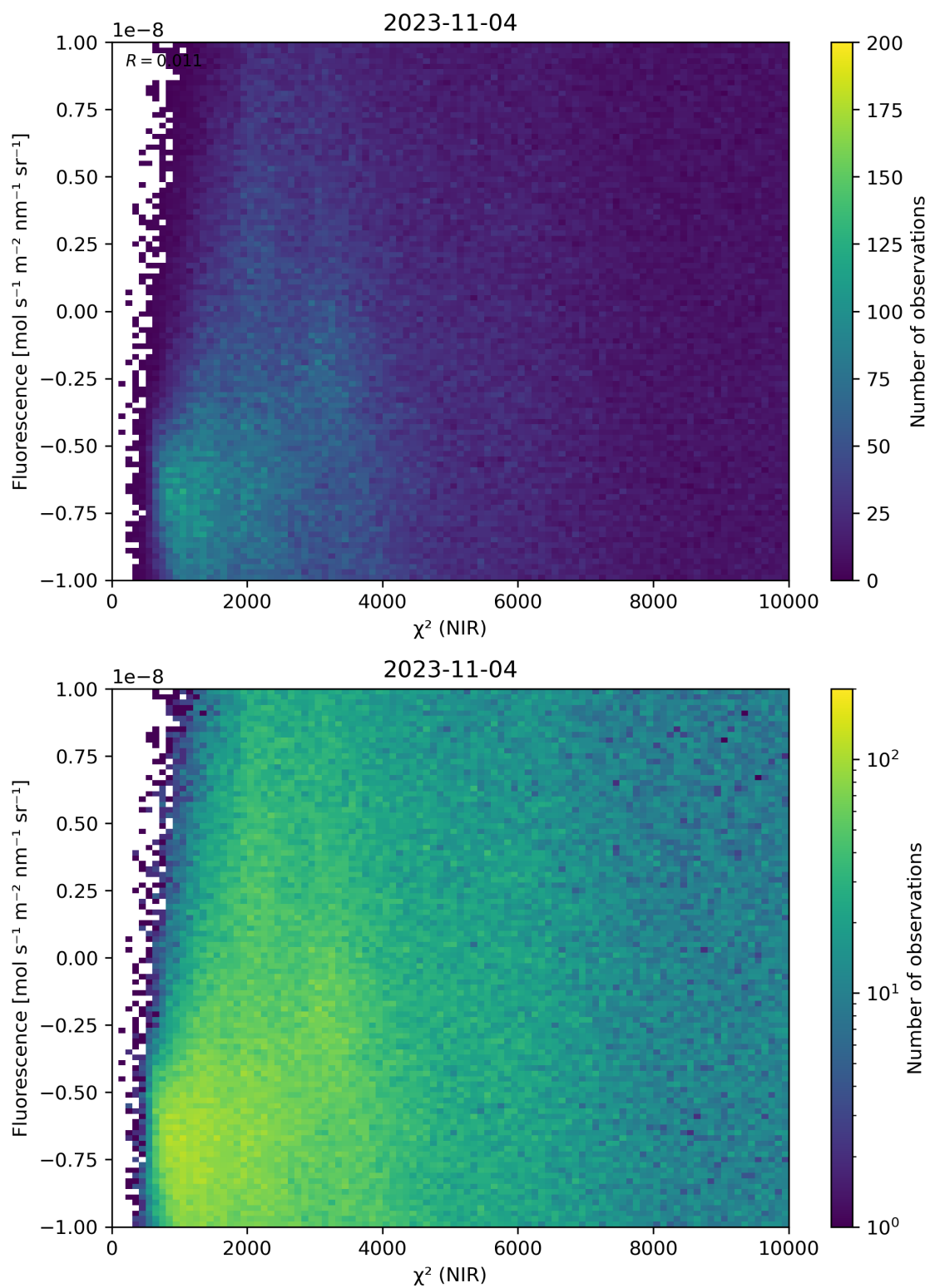
Figure 45: Scatter density plot of “ \chi^2 (NIR)” against “Fluorescence” for 2023-11-03 to 2023-11-05.
