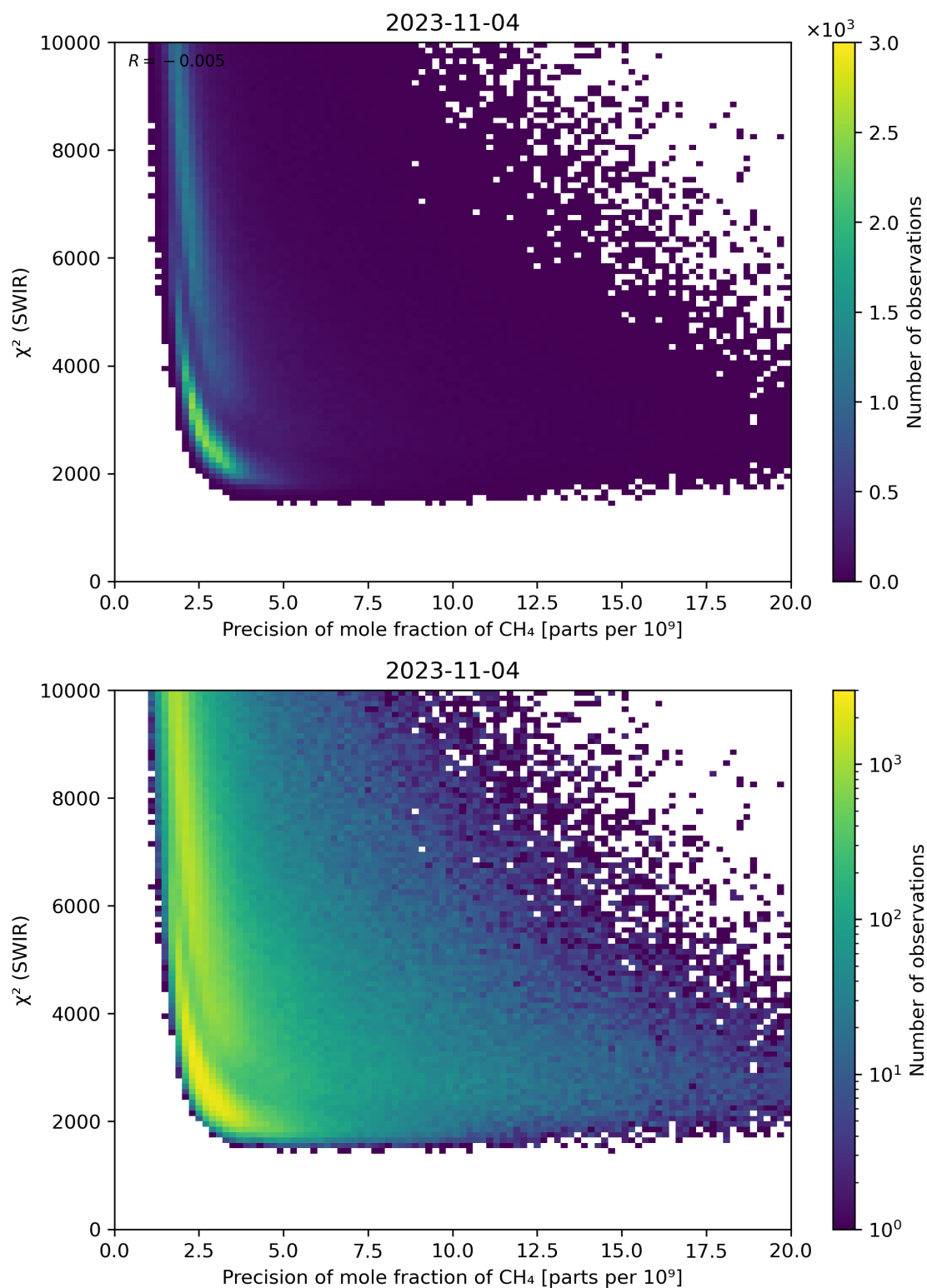
Figure 79: Scatter density plot of “Precision of mole fraction of CH 4 ” against “ \chi^2 (SWIR)” for 2023-11-03 to 2023-11-05.
