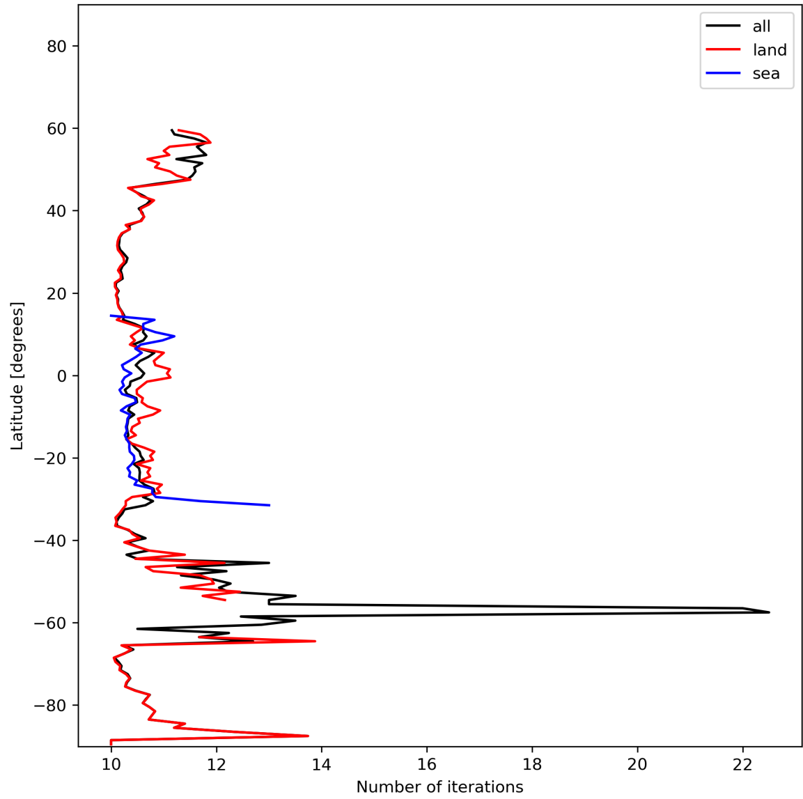
Figure 20: Zonal average of “Number of iterations” for 2023-11-03 to 2023-11-05.
