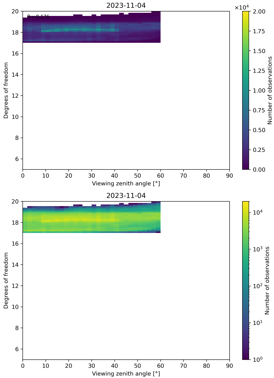
Figure 107: Scatter density plot of “Viewing zenith angle” against “Degrees of freedom” for 2023-11-03 to 2023-11-05.
