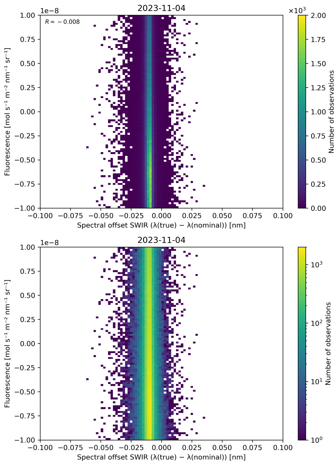
Figure 120: Scatter density plot of “Spectral offset SWIR ( \lambda(\text{true}) - \lambda(\text{nominal}) )” against “Fluorescence” for 2023-11-03 to 2023-11-05.
