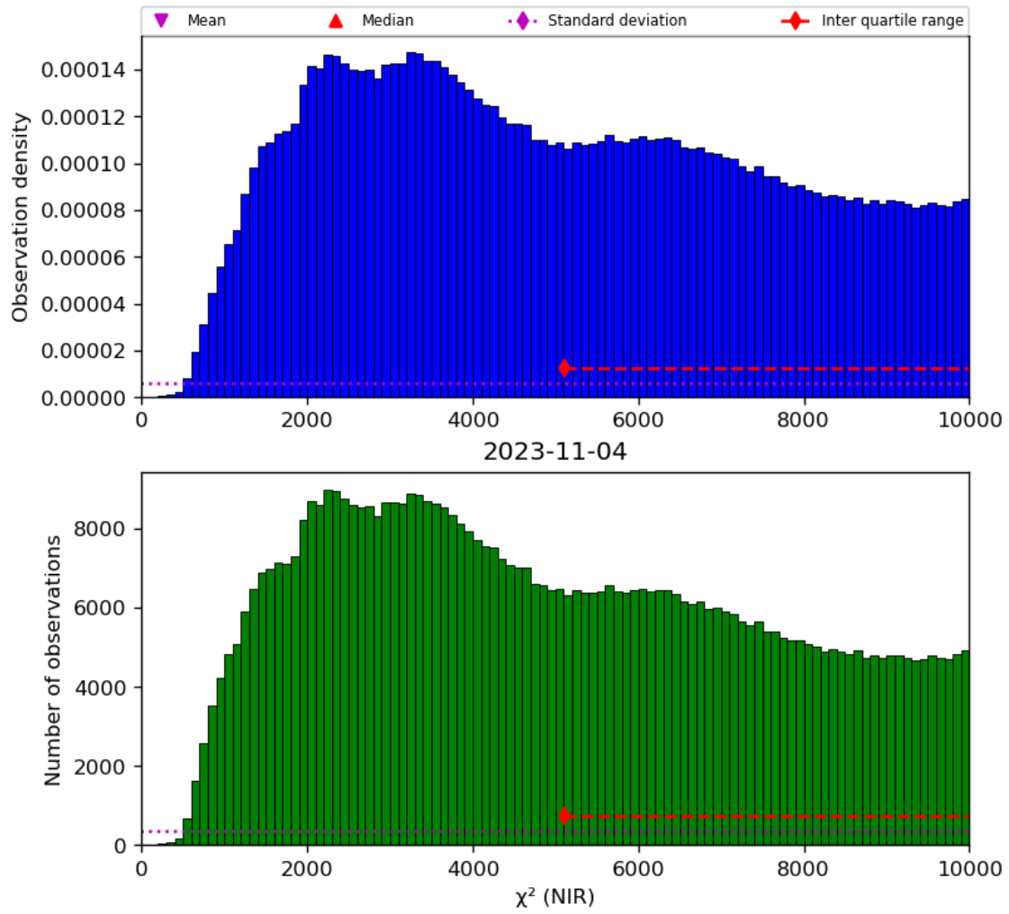
Figure 29: Histogram of “ \chi^2 (NIR)” for 2023-11-03 to 2023-11-05
