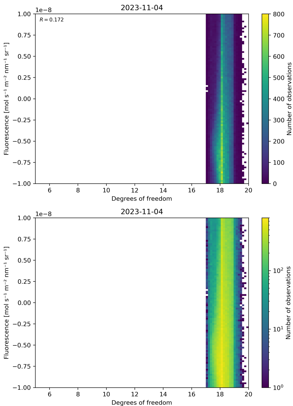
Figure 51: Scatter density plot of “Degrees of freedom” against “Fluorescence” for 2023-11-03 to 2023-11-05.
