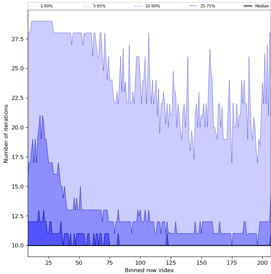
Figure 42: Along track statistics of “Number of iterations” for 2023-11-03 to 2023-11-05
