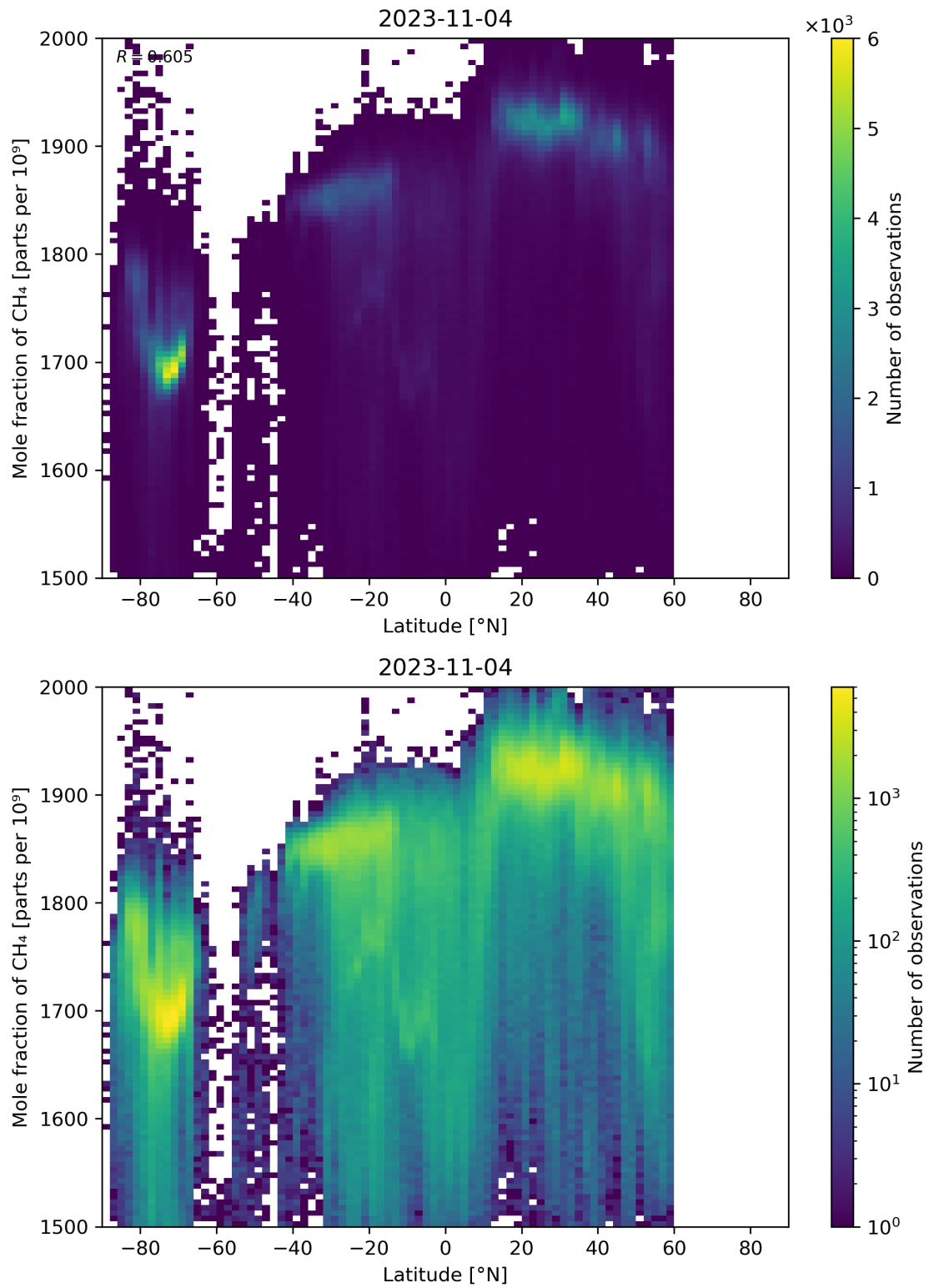
Figure 57: Scatter density plot of “Latitude” against “Mole fraction of CH 4 ” for 2023-11-03 to 2023-11-05.
