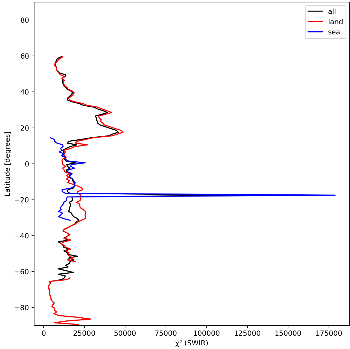
Figure 17: Zonal average of “ \chi^2 (SWIR)” for 2023-11-03 to 2023-11-05.
