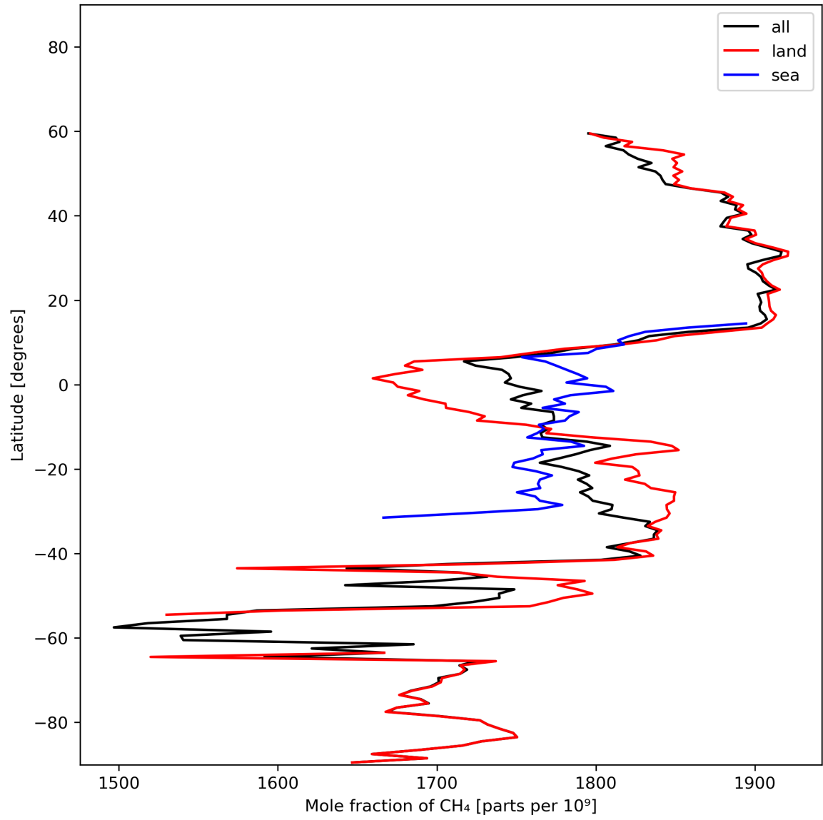
Figure 12: Zonal average of “Mole fraction of \text{CH}_4 ” for 2023-11-03 to 2023-11-05.
