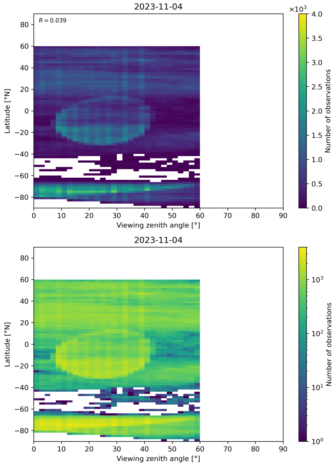
Figure 109: Scatter density plot of “Viewing zenith angle” against “Latitude” for 2023-11-03 to 2023-11-05.
