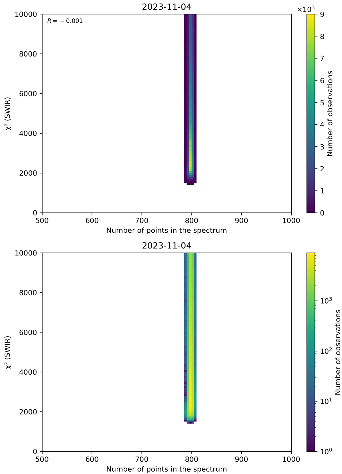
Figure 89: Scatter density plot of “Number of points in the spectrum” against “ \chi^2 (SWIR)” for 2023-11-03 to 2023-11-05.
