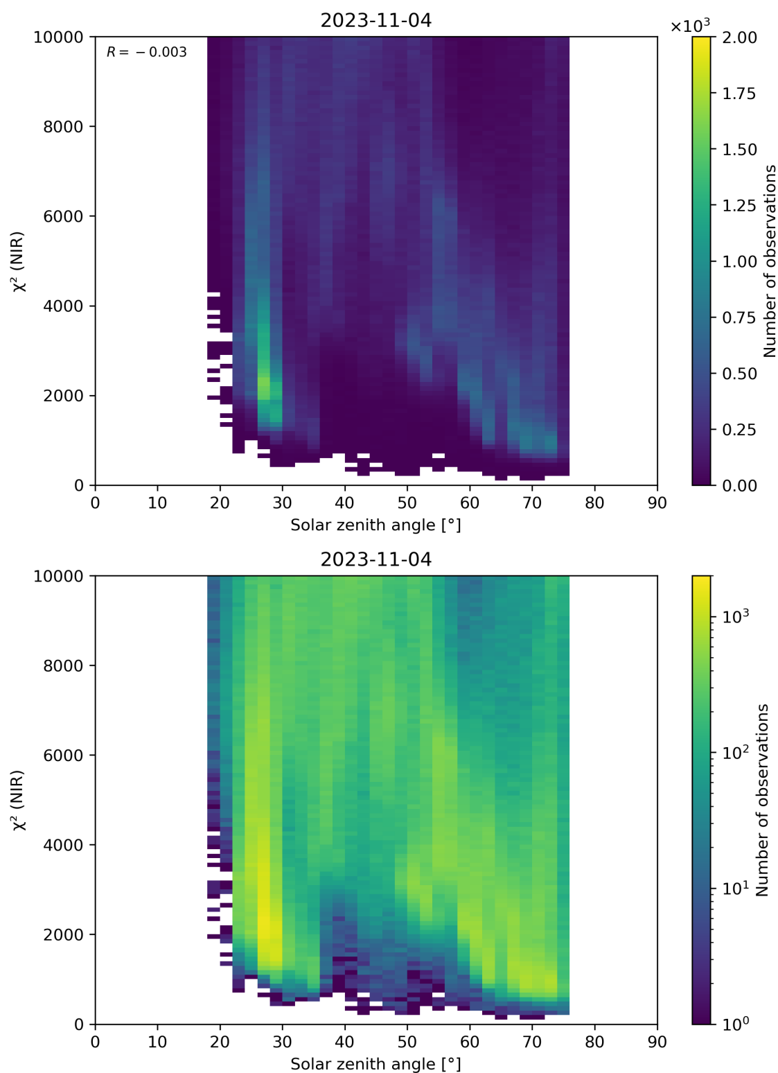
Figure 94: Scatter density plot of “Solar zenith angle” against “ \chi^2 (NIR)” for 2023-11-03 to 2023-11-05.
