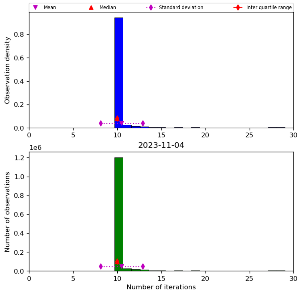
Figure 31: Histogram of “Number of iterations” for 2023-11-03 to 2023-11-05
