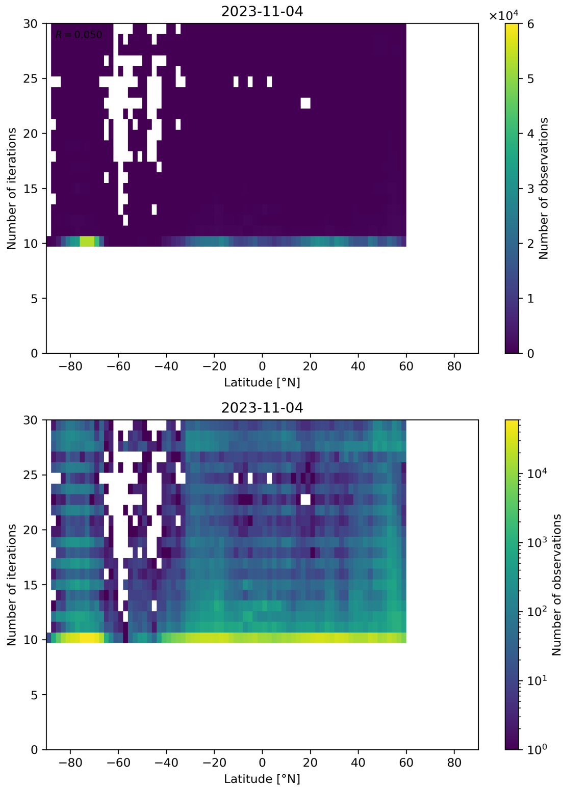
Figure 60: Scatter density plot of “Latitude” against “Number of iterations” for 2023-11-03 to 2023-11-05.
