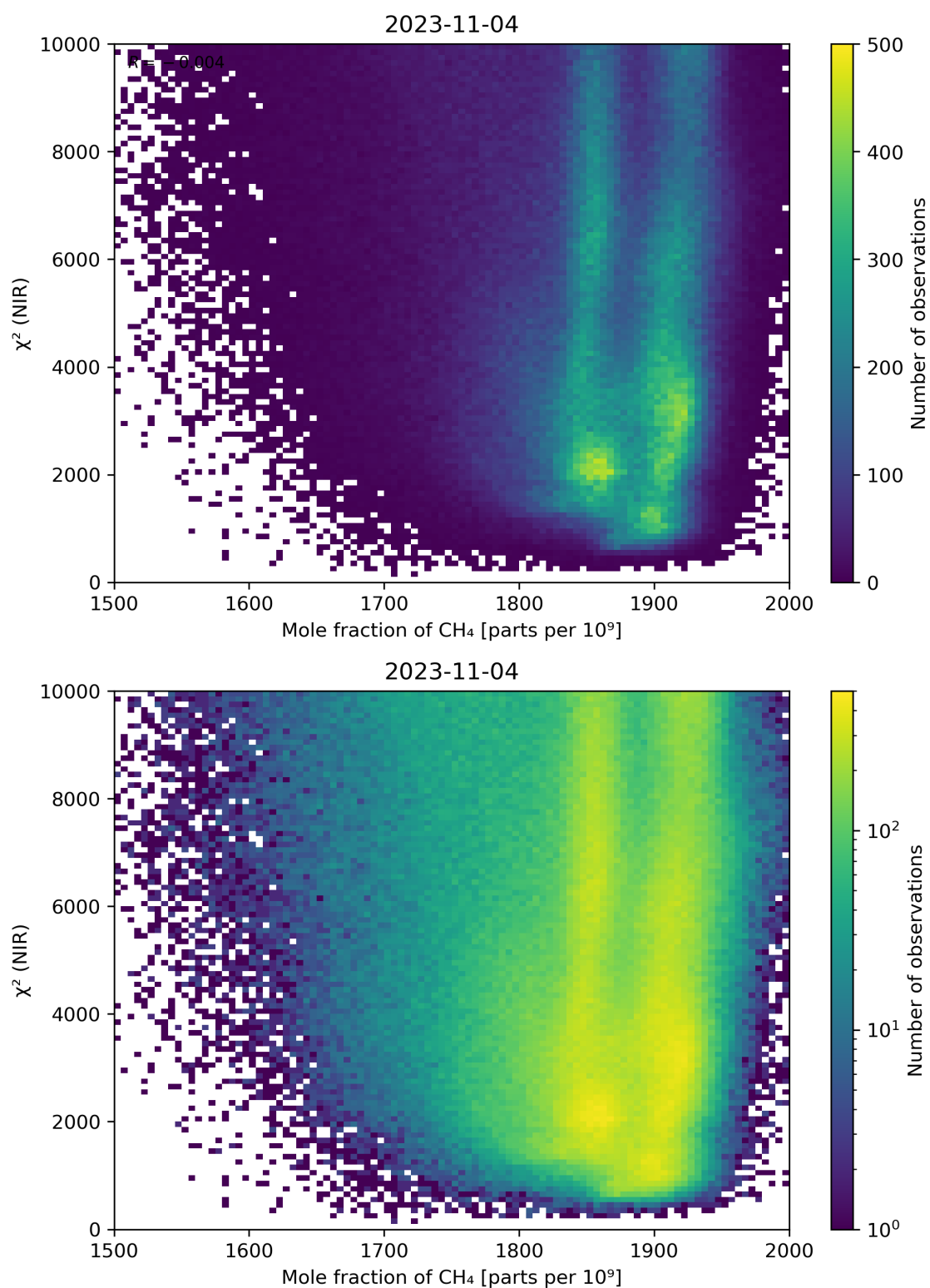
Figure 70: Scatter density plot of “Mole fraction of CH 4 ” against “ \chi^2 (NIR)” for 2023-11-03 to 2023-11-05.
