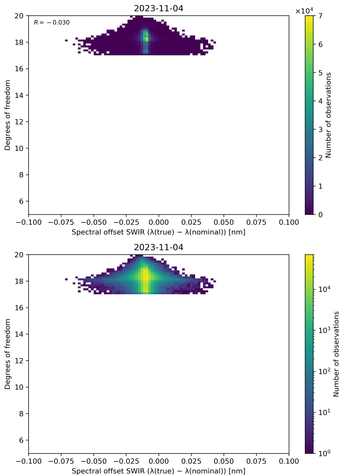
Figure 119: Scatter density plot of “Spectral offset SWIR ( \lambda(\text{true}) - \lambda(\text{nominal}) )” against “Degrees of freedom” for 2023-11-03 to 2023-11-05.
