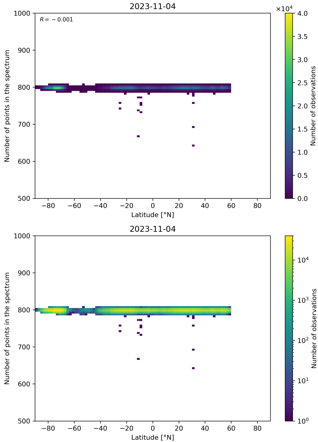
Figure 61: Scatter density plot of “Latitude” against “Number of points in the spectrum” for 2023-11-03 to 2023-11-05.
