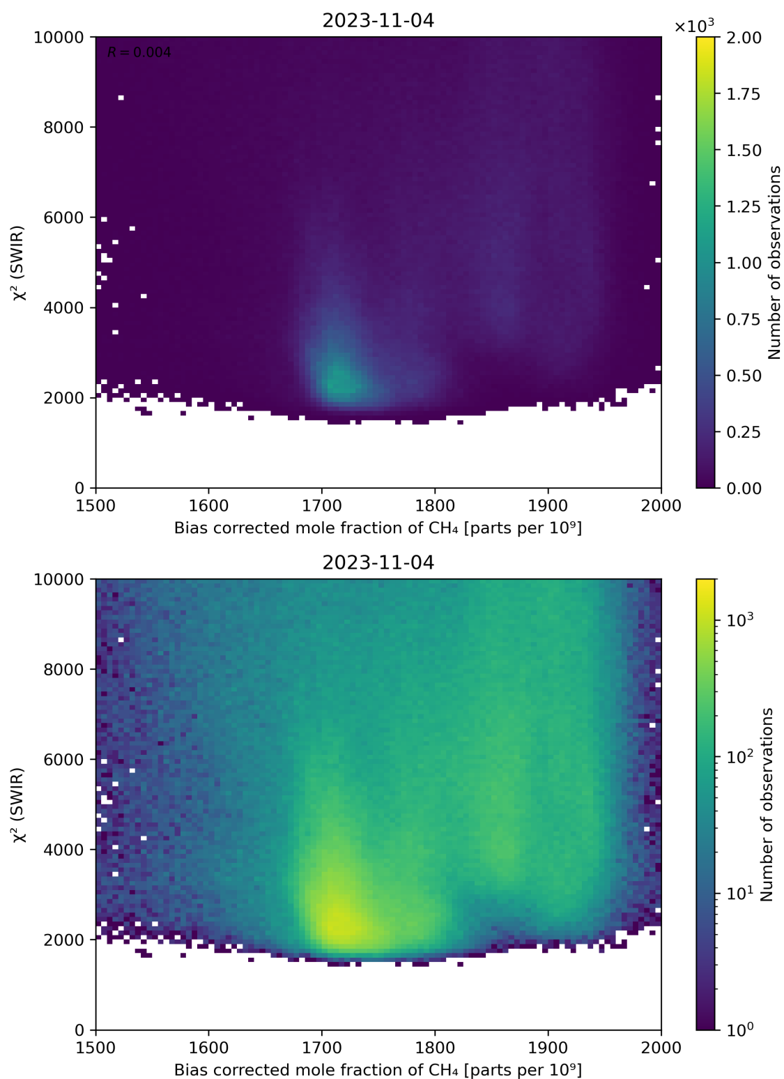
Figure 64: Scatter density plot of “Bias corrected mole fraction of CH 4 ” against “ \chi^2 (SWIR)” for 2023-11-03 to 2023-11-05.
