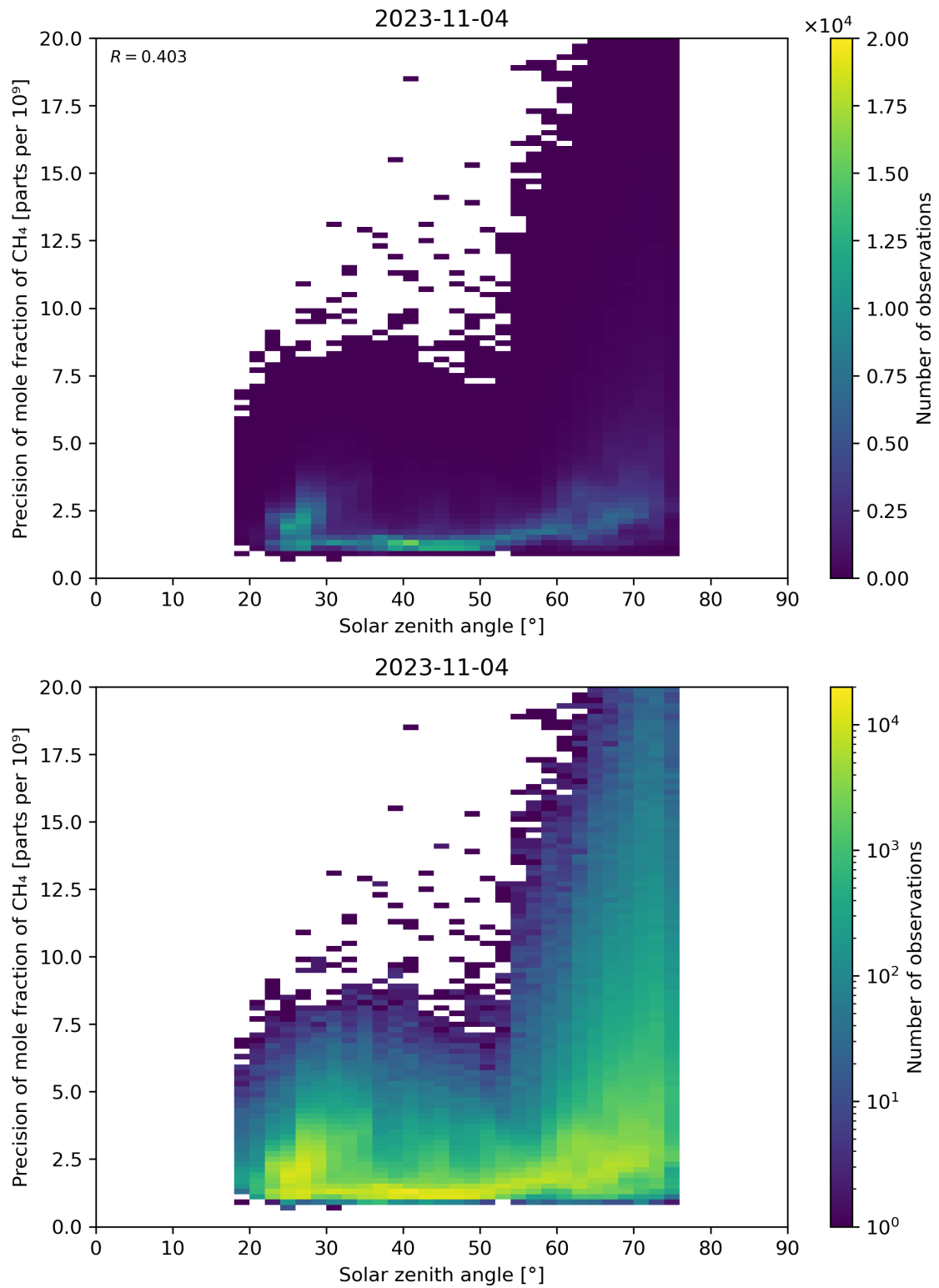
Figure 101: Scatter density plot of “Solar zenith angle” against “Precision of mole fraction of CH 4 ” for 2023-11-03 to 2023-11-05.
