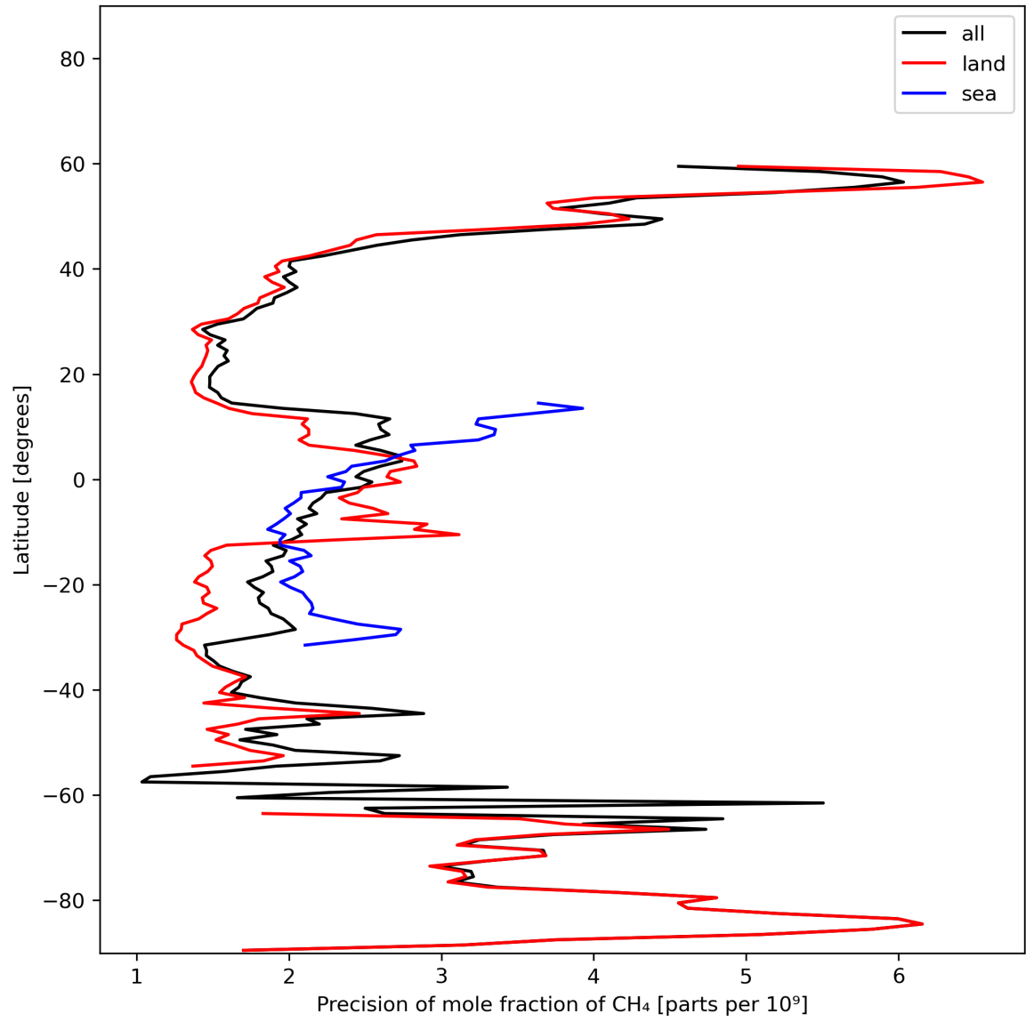
Figure 13: Zonal average of “Precision of mole fraction of CH 4 ” for 2023-11-03 to 2023-11-05.
