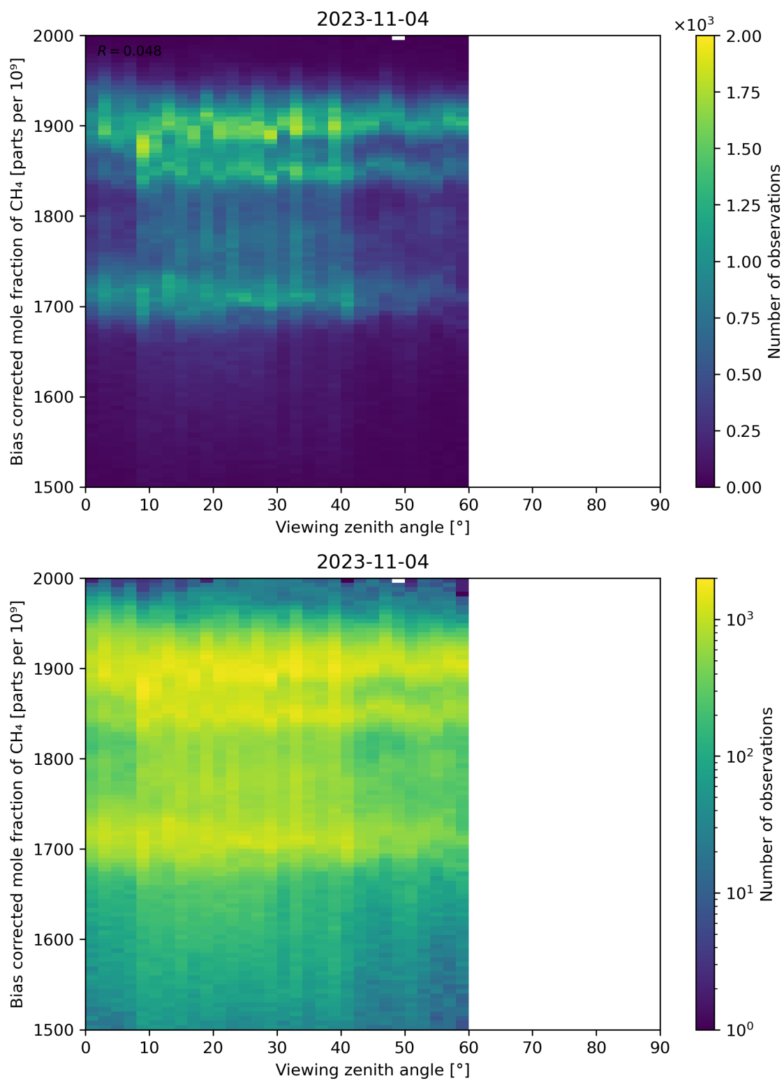
Figure 111: Scatter density plot of “Viewing zenith angle” against “Bias corrected mole fraction of CH 4 ” for 2023-11-03 to 2023-11-05.
