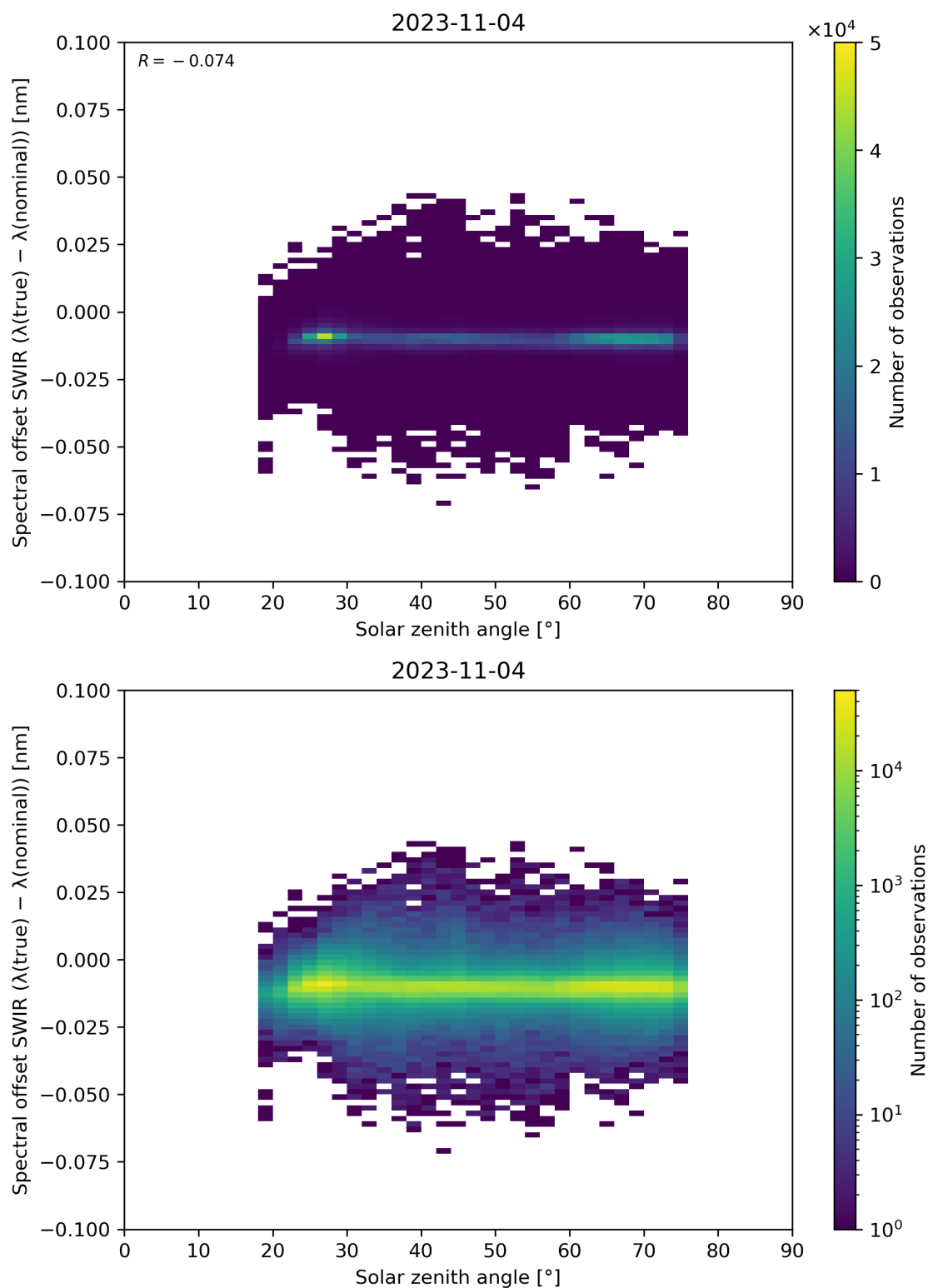
Figure 104: Scatter density plot of “Solar zenith angle” against “Spectral offset SWIR ( \lambda(\text{true}) - \lambda(\text{nominal}) )” for 2023-11-03 to 2023-11-05.
