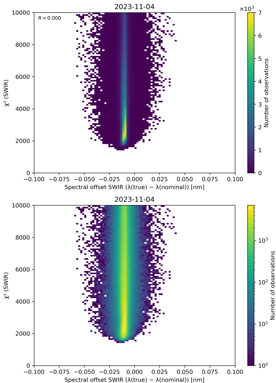
Figure 118: Scatter density plot of “Spectral offset SWIR ( \lambda(\text{true}) - \lambda(\text{nominal}) )” against “ \chi^2 (SWIR)” for 2023-11-03 to 2023-11-05.
