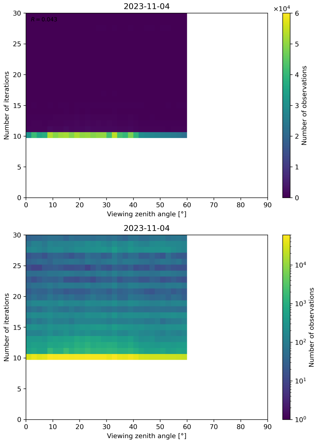
Figure 113: Scatter density plot of “Viewing zenith angle” against “Number of iterations” for 2023-11-03 to 2023-11-05.
