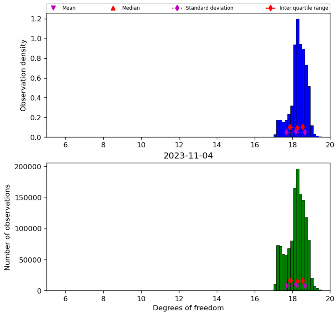
Figure 30: Histogram of “Degrees of freedom” for 2023-11-03 to 2023-11-05
