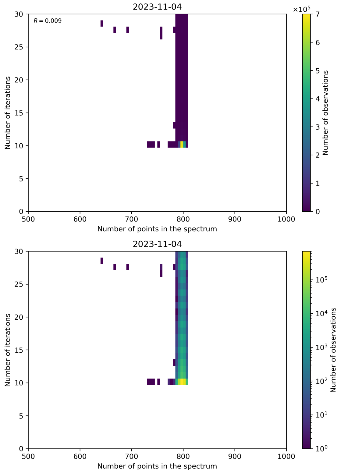
Figure 92: Scatter density plot of “Number of points in the spectrum” against “Number of iterations” for 2023-11-03 to 2023-11-05.
