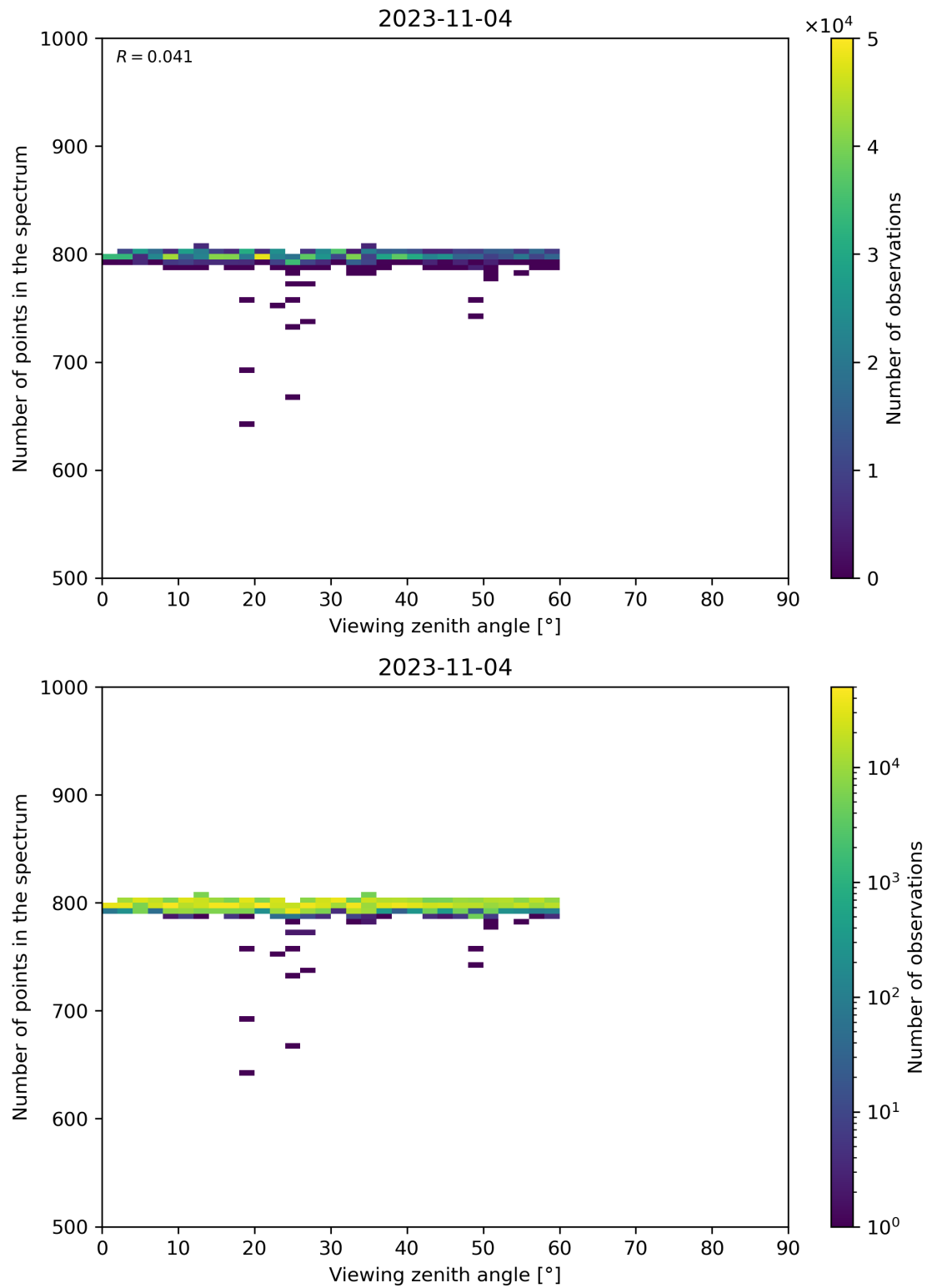
Figure 114: Scatter density plot of “Viewing zenith angle” against “Number of points in the spectrum” for 2023-11-03 to 2023-11-05.
