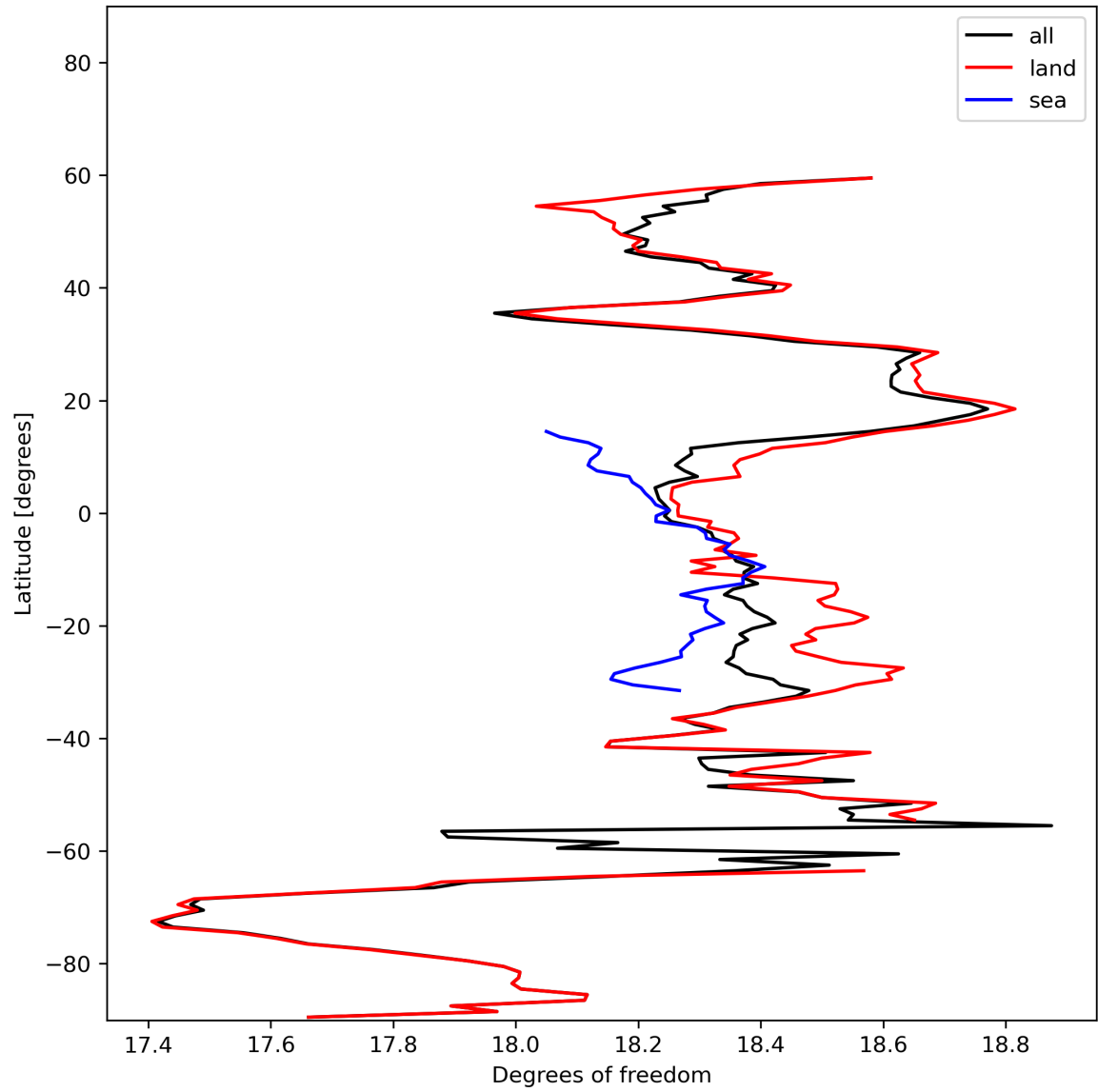
Figure 19: Zonal average of “Degrees of freedom” for 2023-11-03 to 2023-11-05.
