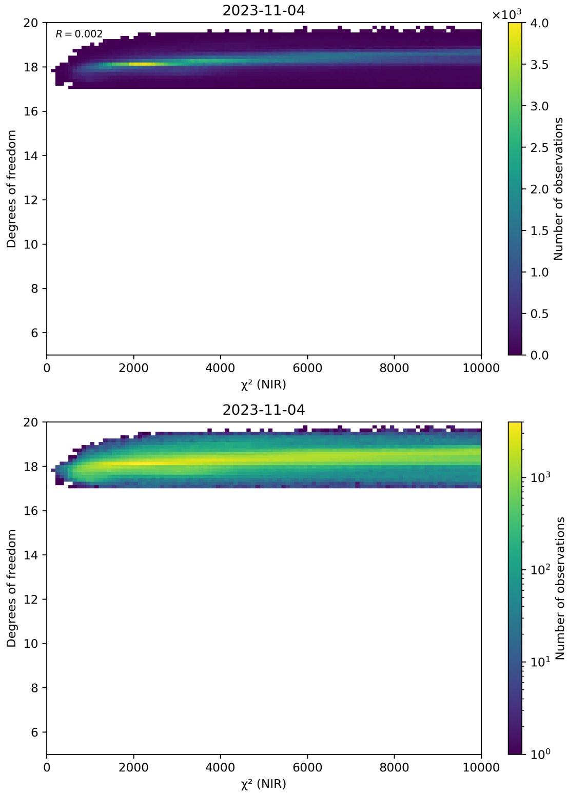
Figure 44: Scatter density plot of “ \chi^2 (NIR)” against “Degrees of freedom” for 2023-11-03 to 2023-11-05.
