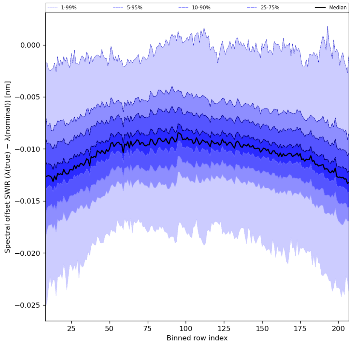
Figure 38: Along track statistics of “Spectral offset SWIR ( \lambda(\text{true}) - \lambda(\text{nominal}) )” for 2023-11-03 to 2023-11-05
