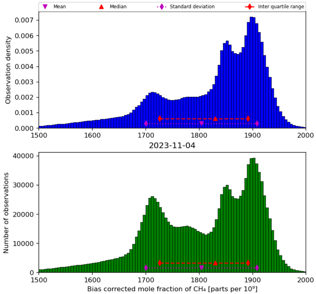
Figure 25: Histogram of “Bias corrected mole fraction of CH 4 ” for 2023-11-03 to 2023-11-05
