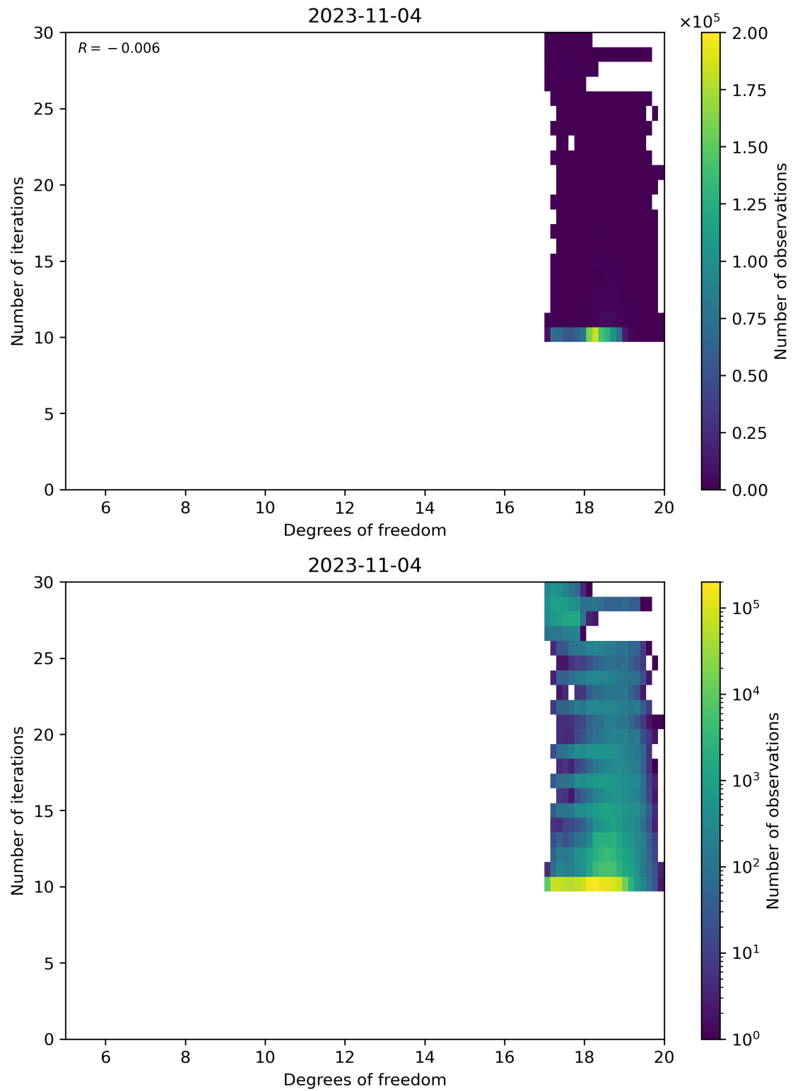
Figure 52: Scatter density plot of “Degrees of freedom” against “Number of iterations” for 2023-11-03 to 2023-11-05.
