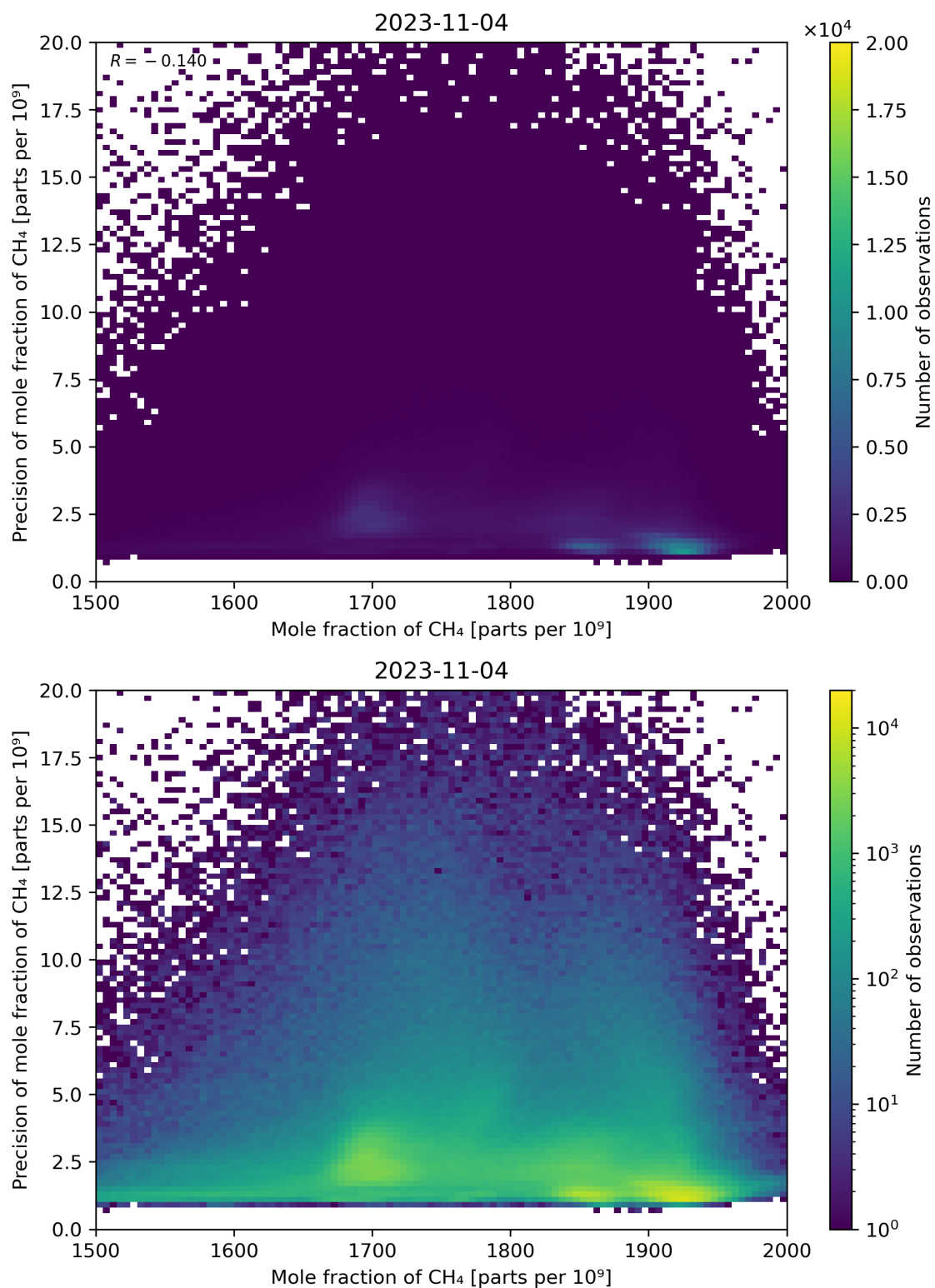
Figure 75: Scatter density plot of “Mole fraction of CH 4 ” against “Precision of mole fraction of CH 4 ” for 2023-11-03 to 2023-11-05.
