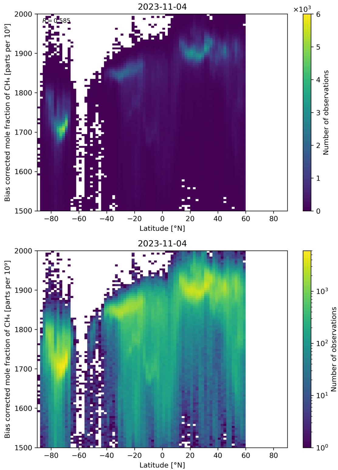
Figure 58: Scatter density plot of “Latitude” against “Bias corrected mole fraction of CH 4 ” for 2023-11-03 to 2023-11-05.
