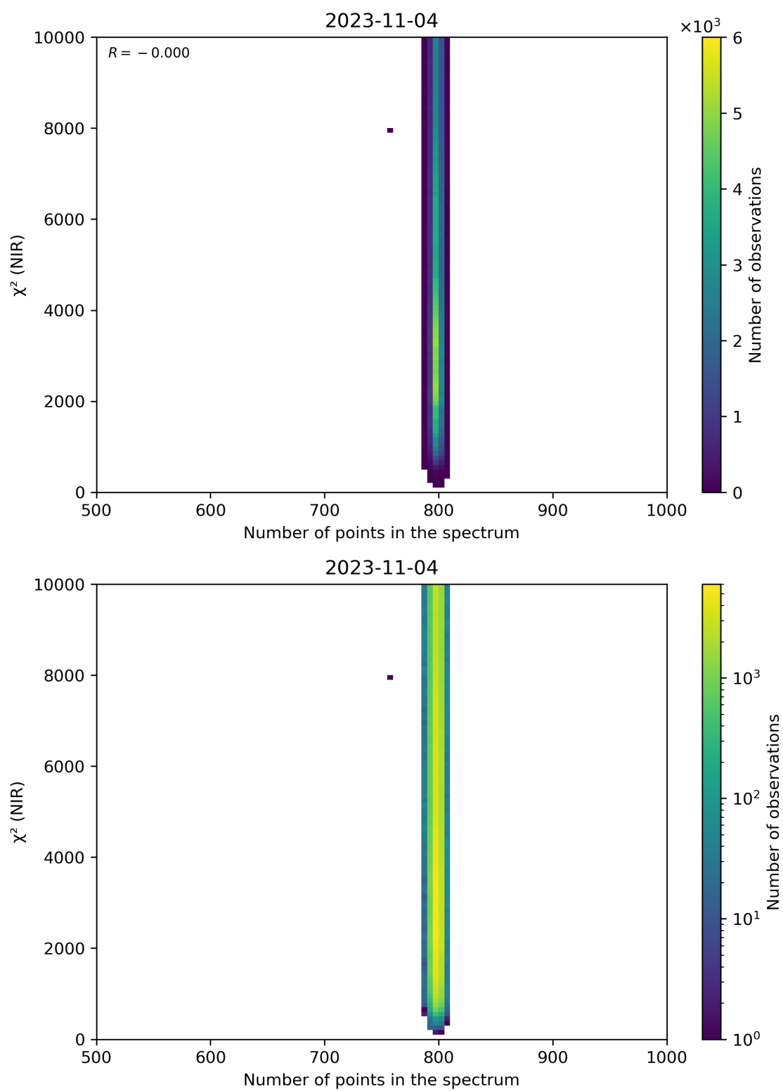
Figure 88: Scatter density plot of “Number of points in the spectrum” against “ \chi^2 (NIR)” for 2023-11-03 to 2023-11-05.
