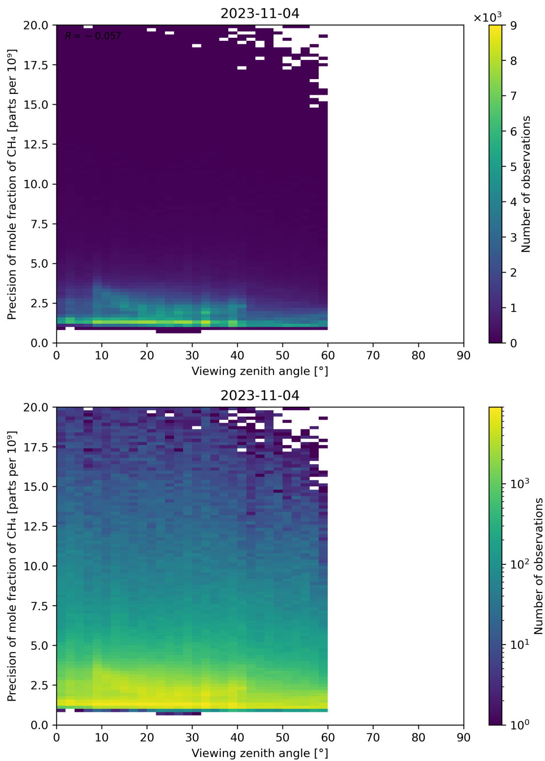
Figure 112: Scatter density plot of “Viewing zenith angle” against “Precision of mole fraction of CH 4 ” for 2023-11-03 to 2023-11-05.
