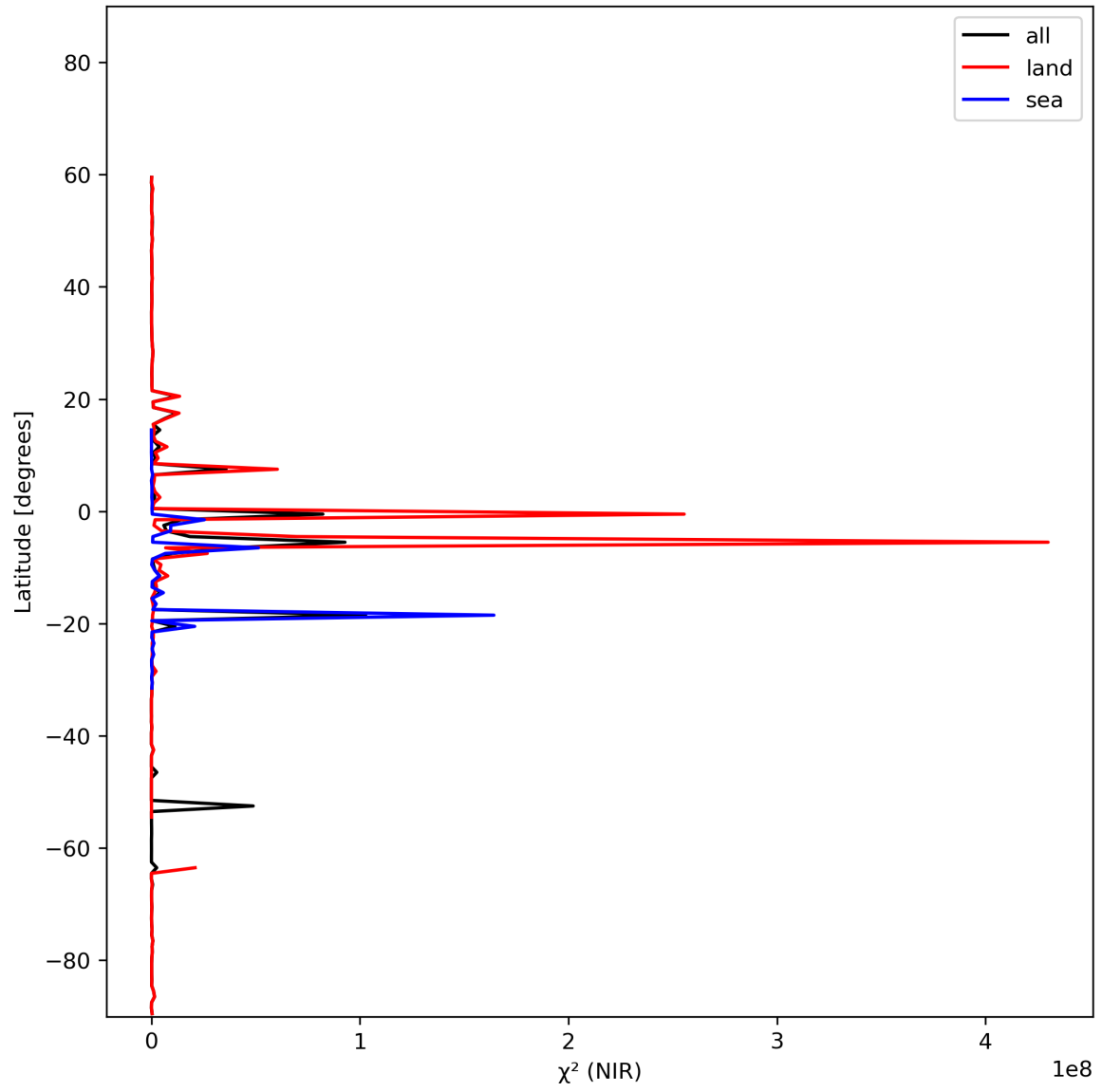
Figure 18: Zonal average of “ \chi^2 (NIR)” for 2023-11-03 to 2023-11-05.
