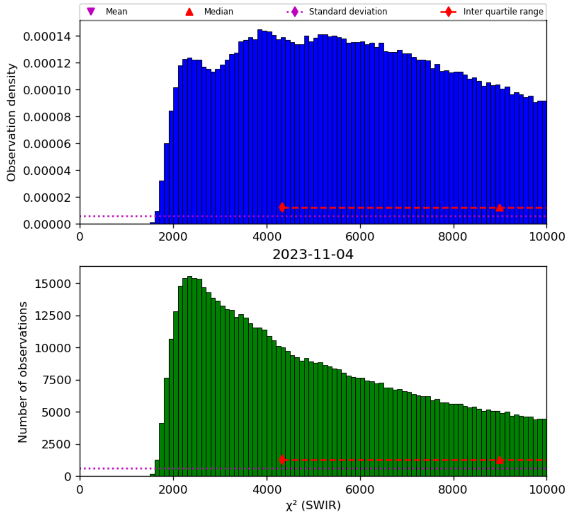
Figure 28: Histogram of “ \chi^2 (SWIR)” for 2023-11-03 to 2023-11-05
