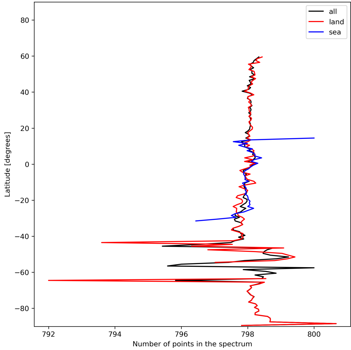
Figure 15: Zonal average of “Number of points in the spectrum” for 2023-11-03 to 2023-11-05.
