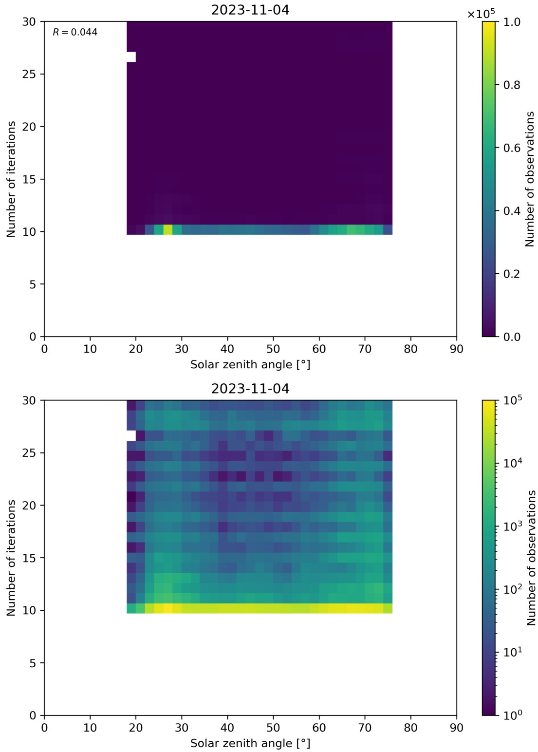
Figure 102: Scatter density plot of “Solar zenith angle” against “Number of iterations” for 2023-11-03 to 2023-11-05.
