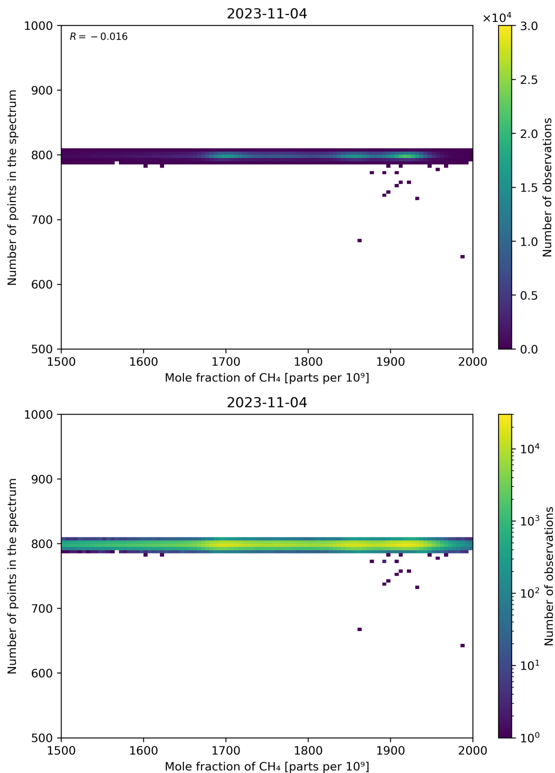
Figure 77: Scatter density plot of “Mole fraction of CH 4 ” against “Number of points in the spectrum” for 2023-11-03 to 2023-11-05.
