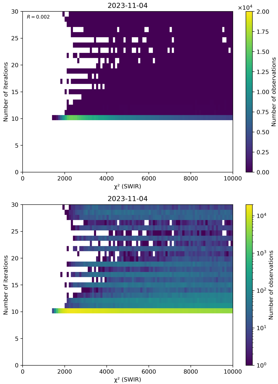
Figure 50: Scatter density plot of “ \chi^2 (SWIR)” against “Number of iterations” for 2023-11-03 to 2023-11-05.
