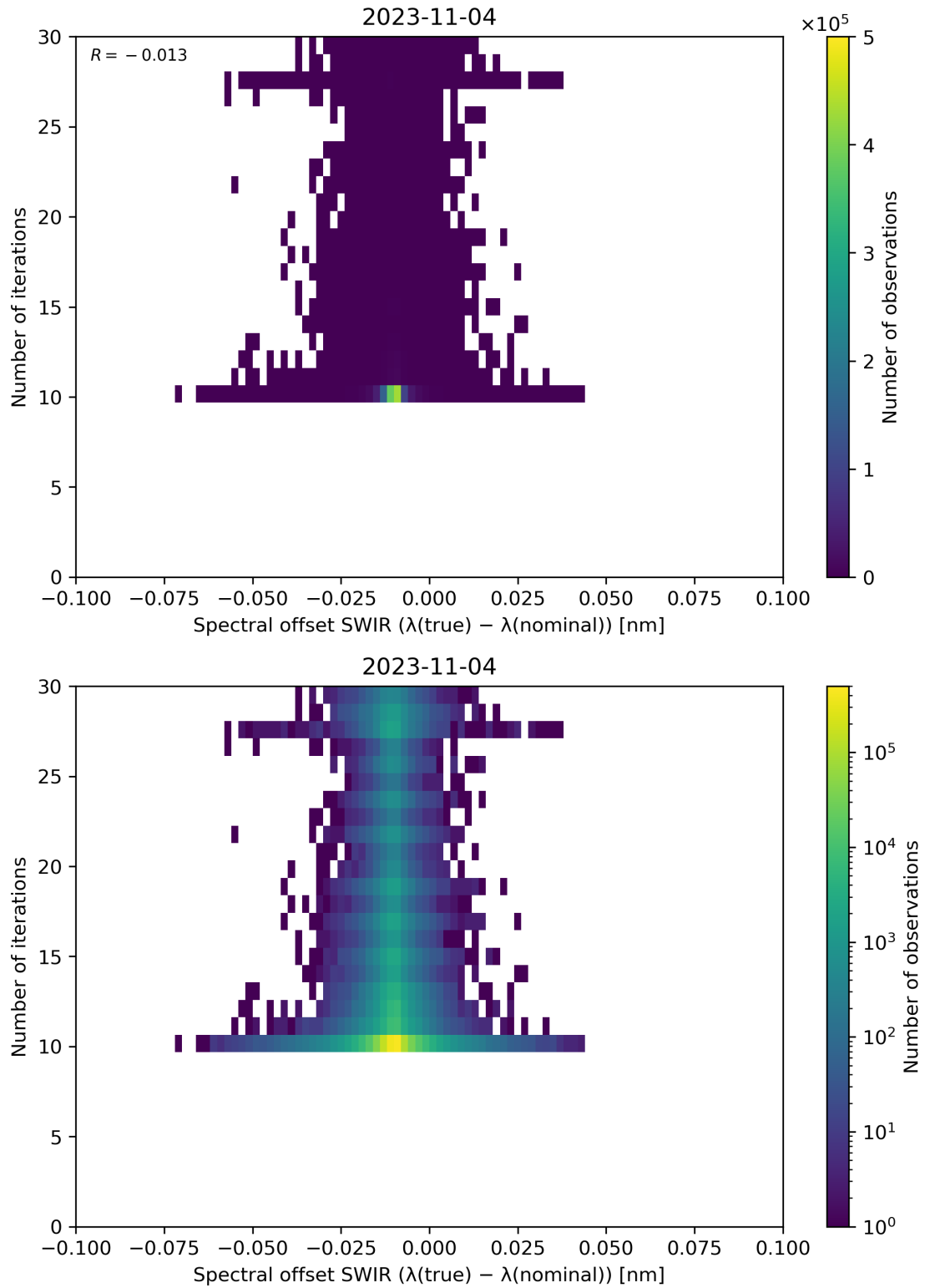
Figure 121: Scatter density plot of “Spectral offset SWIR ( \lambda(\text{true}) - \lambda(\text{nominal}) )” against “Number of iterations” for 2023-11-03 to 2023-11-05.
