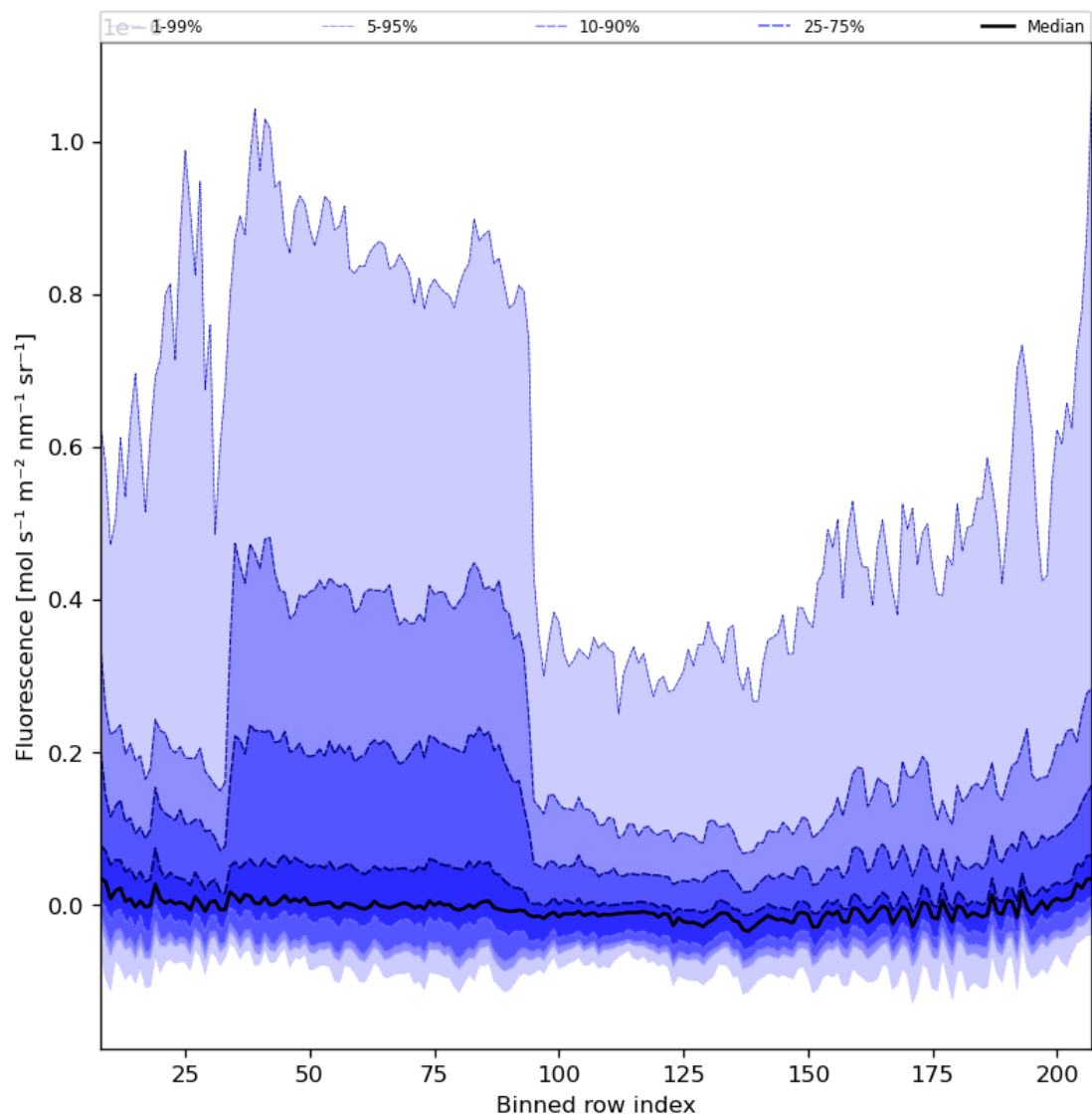
Figure 43: Along track statistics of “Fluorescence” for 2023-11-03 to 2023-11-05
