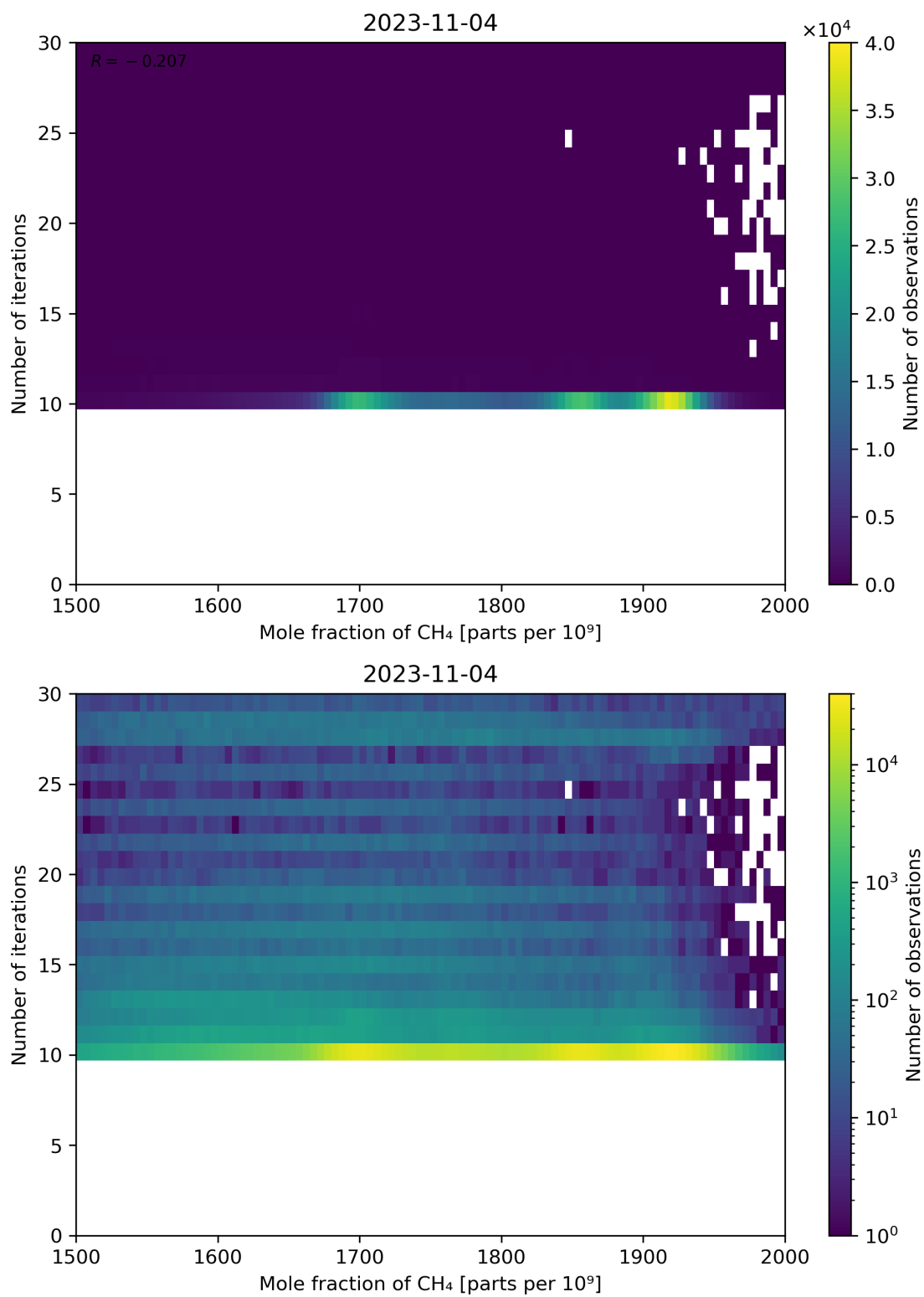
Figure 76: Scatter density plot of “Mole fraction of CH 4 ” against “Number of iterations” for 2023-11-03 to 2023-11-05.
