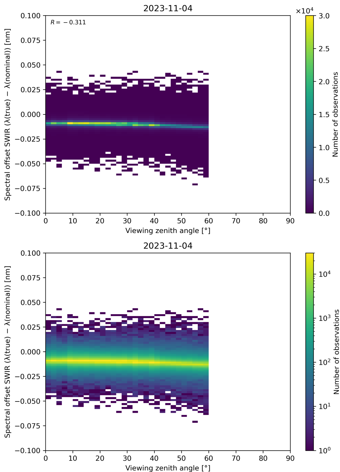
Figure 116: Scatter density plot of “Viewing zenith angle” against “Spectral offset SWIR ( \lambda(\text{true}) - \lambda(\text{nominal}) )” for 2023-11-03 to 2023-11-05.
