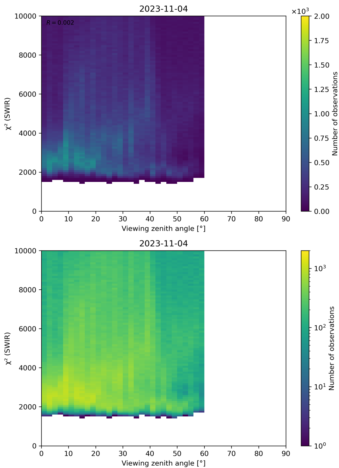
Figure 106: Scatter density plot of “Viewing zenith angle” against “ \chi^2 (SWIR)” for 2023-11-03 to 2023-11-05.
