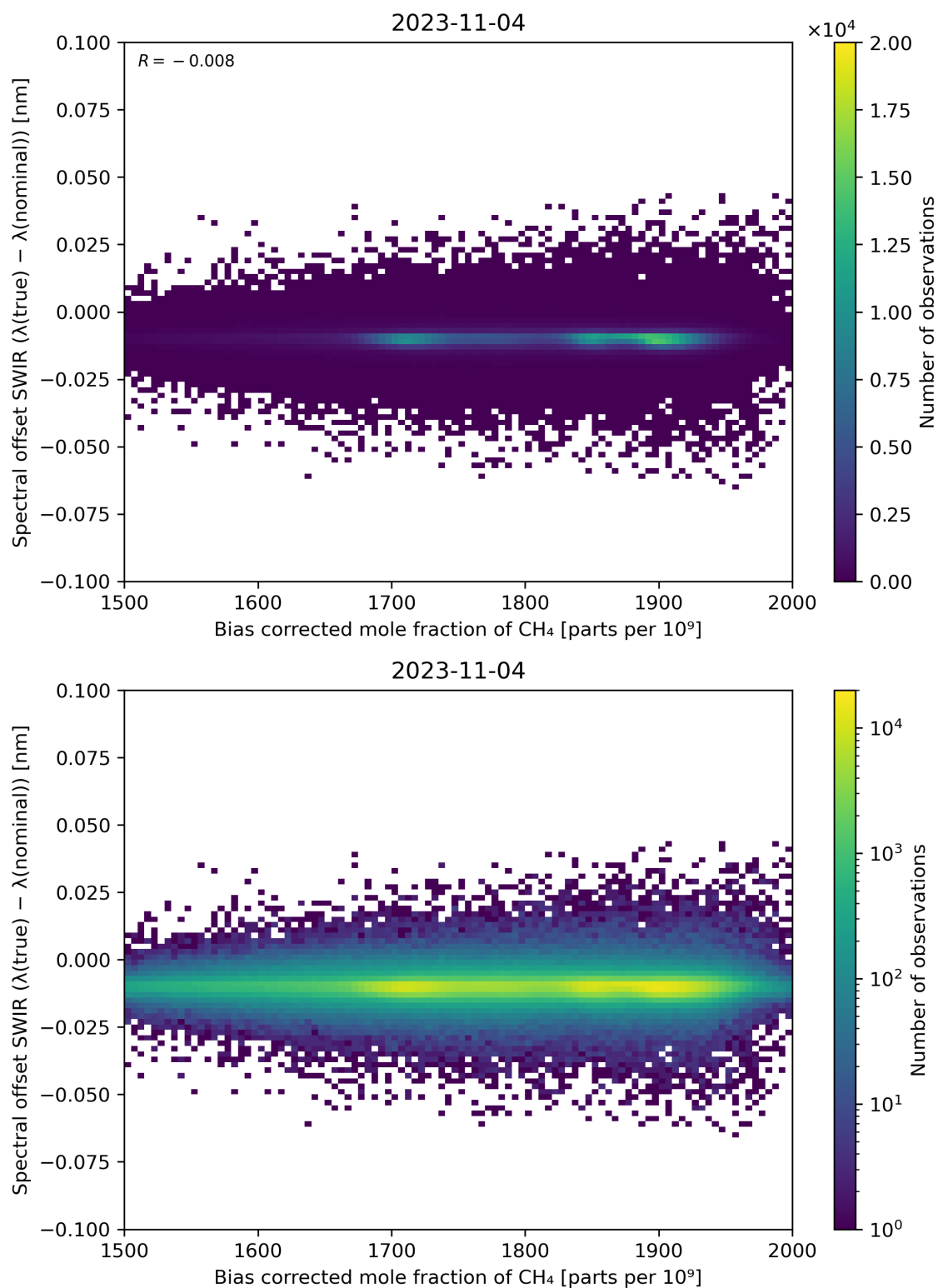
Figure 69: Scatter density plot of “Bias corrected mole fraction of \text{CH}_4 ” against “Spectral offset SWIR ( \lambda(\text{true}) - \lambda(\text{nominal}) )” for 2023-11-03 to 2023-11-05.
