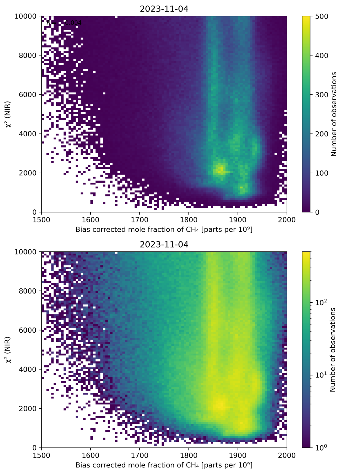
Figure 63: Scatter density plot of “Bias corrected mole fraction of \text{CH}_4 ” against “ \chi^2 (NIR)” for 2023-11-03 to 2023-11-05.
