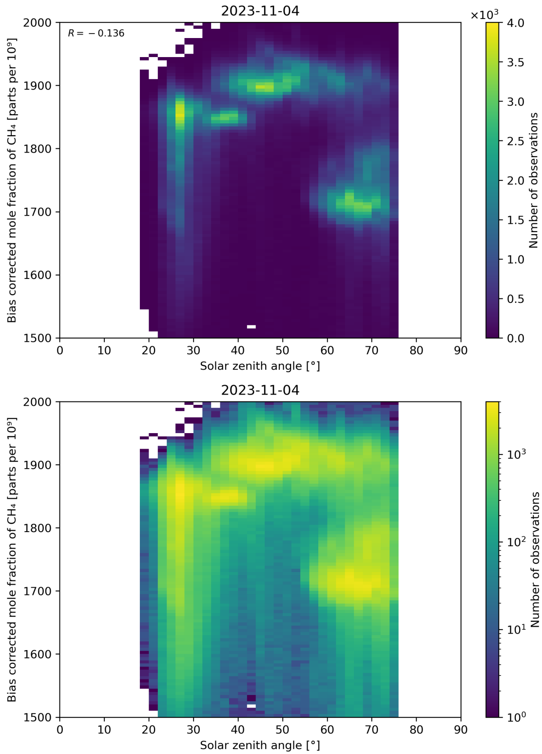
Figure 100: Scatter density plot of “Solar zenith angle” against “Bias corrected mole fraction of \text{CH}_4 ” for 2023-11-03 to 2023-11-05.
