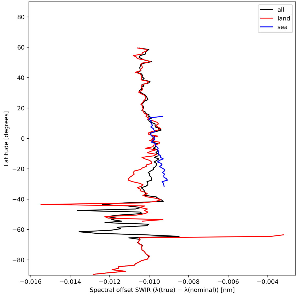
Figure 16: Zonal average of “Spectral offset SWIR ( \lambda(\text{true}) - \lambda(\text{nominal}) )” for 2023-11-03 to 2023-11-05.
