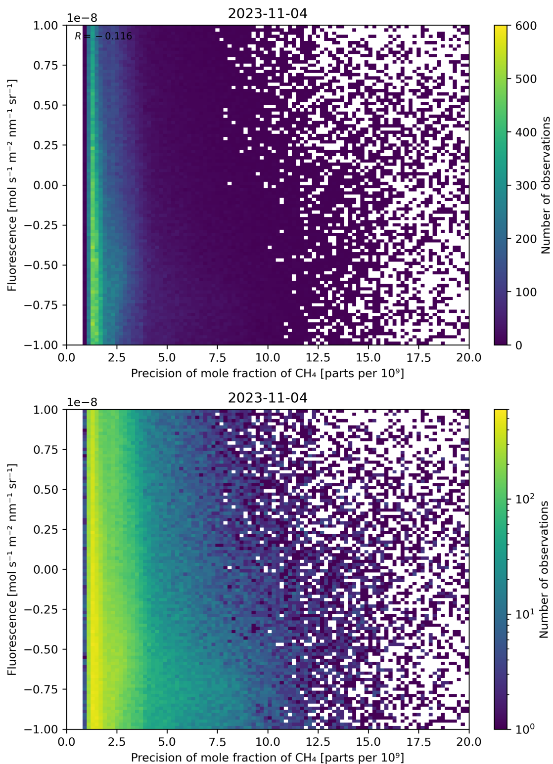
Figure 81: Scatter density plot of “Precision of mole fraction of \text{CH}_4 ” against “Fluorescence” for 2023-11-03 to 2023-11-05.
