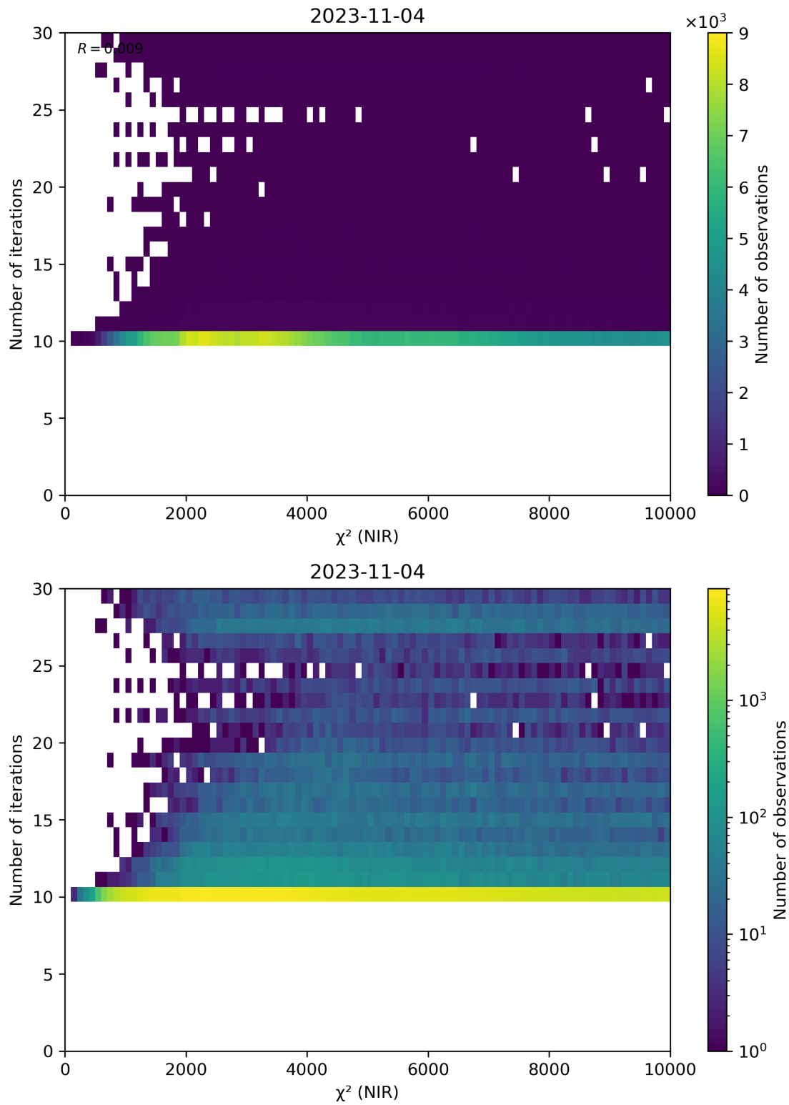
Figure 46: Scatter density plot of “ \chi^2 (NIR)” against “Number of iterations” for 2023-11-03 to 2023-11-05.
