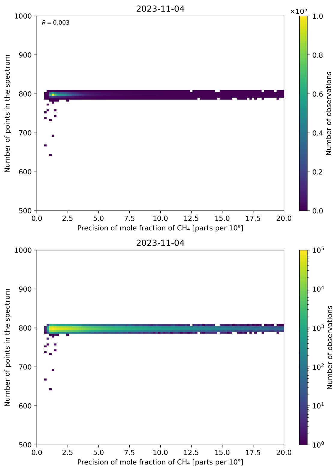
Figure 84: Scatter density plot of “Precision of mole fraction of \text{CH}_4 ” against “Number of points in the spectrum” for 2023-11-03 to 2023-11-05.
