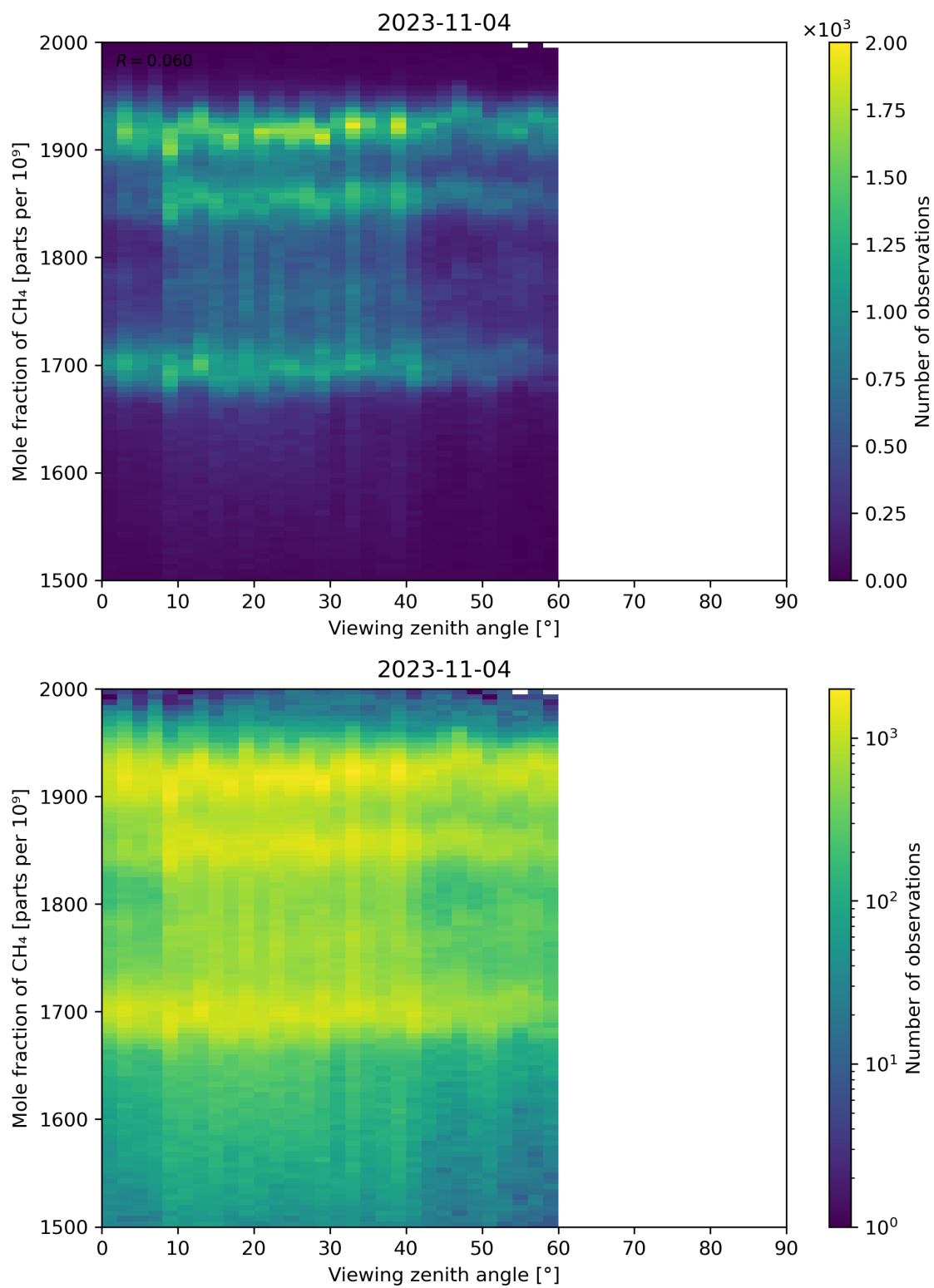
Figure 110: Scatter density plot of “Viewing zenith angle” against “Mole fraction of CH 4 ” for 2023-11-03 to 2023-11-05.
