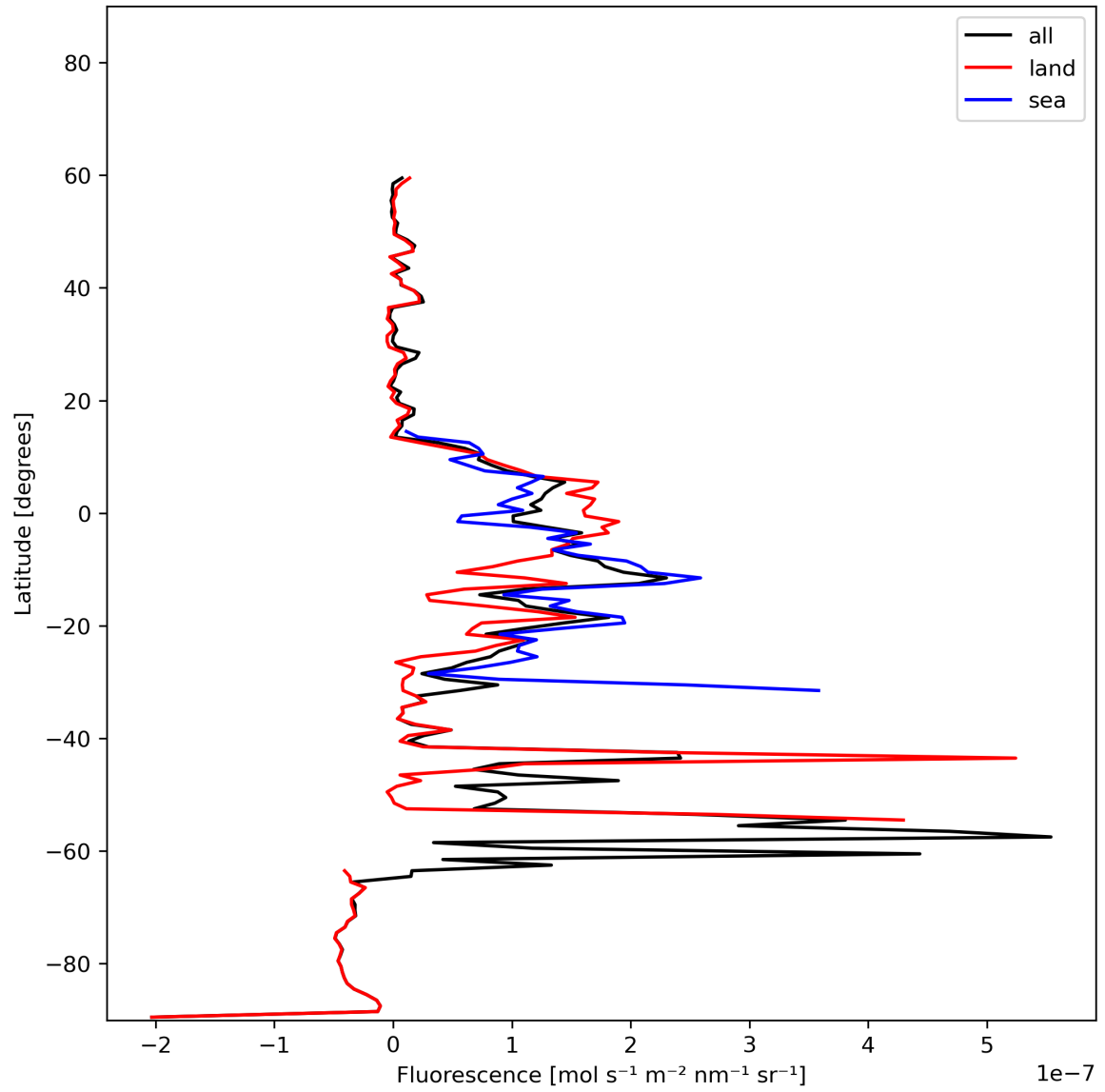
Figure 21: Zonal average of “Fluorescence” for 2023-11-03 to 2023-11-05.
