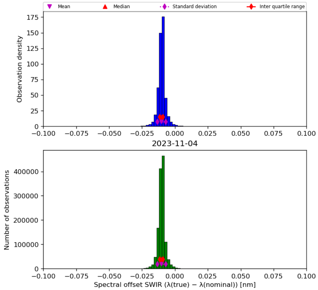
Figure 27: Histogram of “Spectral offset SWIR ( \lambda(\text{true}) - \lambda(\text{nominal}) )” for 2023-11-03 to 2023-11-05
