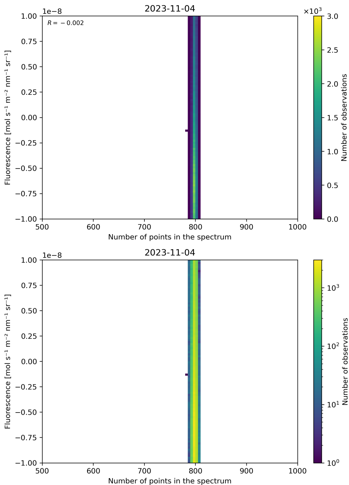
Figure 91: Scatter density plot of “Number of points in the spectrum” against “Fluorescence” for 2023-11-03 to 2023-11-05.
