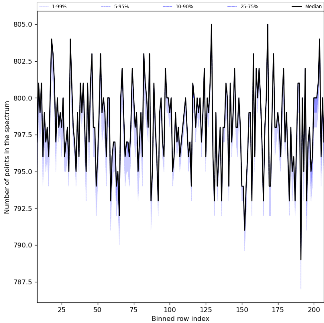
Figure 37: Along track statistics of “Number of points in the spectrum” for 2023-11-03 to 2023-11-05
