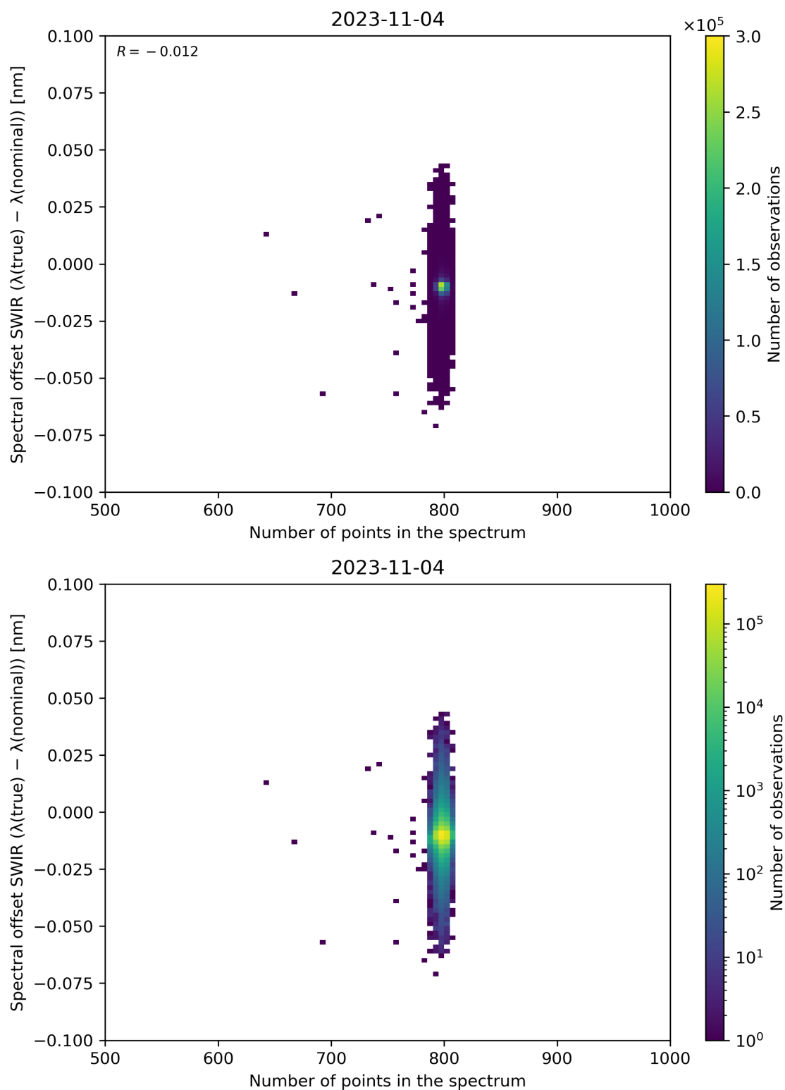
Figure 93: Scatter density plot of “Number of points in the spectrum” against “Spectral offset SWIR ( \lambda(\text{true}) - \lambda(\text{nominal}) )” for 2023-11-03 to 2023-11-05.
