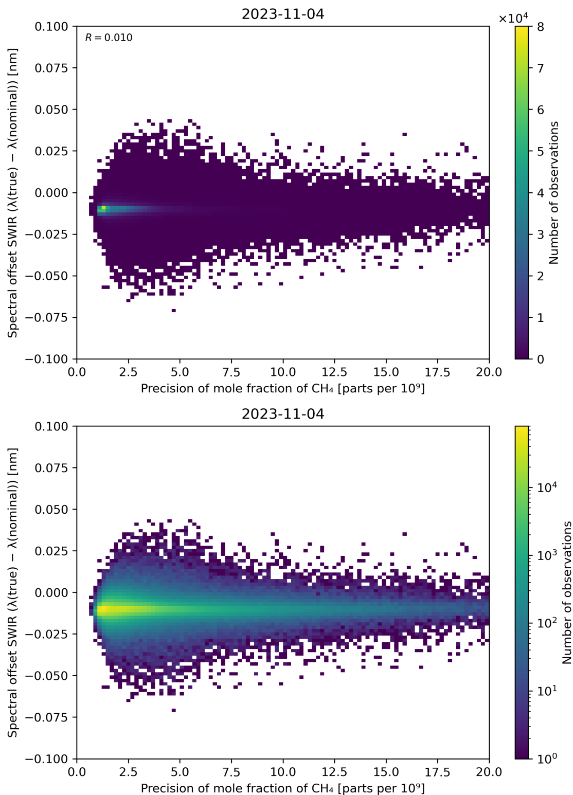
Figure 85: Scatter density plot of “Precision of mole fraction of CH 4 ” against “Spectral offset SWIR ( \lambda(\text{true}) - \lambda(\text{nominal}) )” for 2023-11-03 to 2023-11-05.
