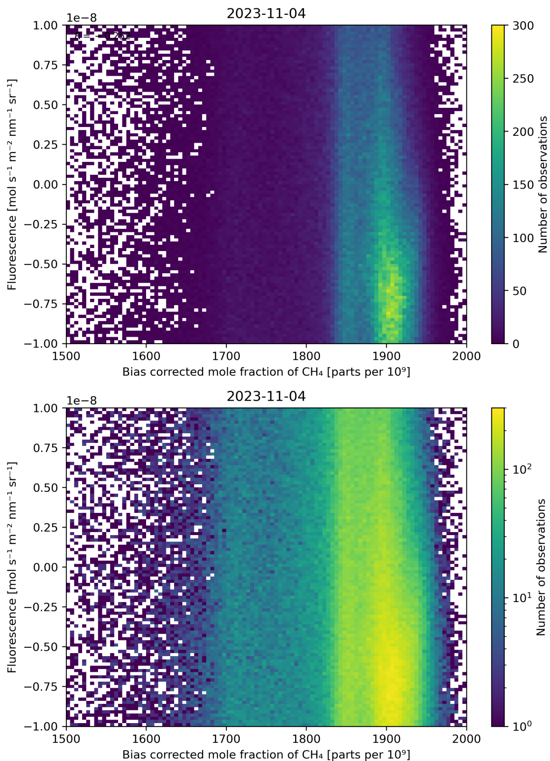
Figure 66: Scatter density plot of “Bias corrected mole fraction of \text{CH}_4 ” against “Fluorescence” for 2023-11-03 to 2023-11-05.
