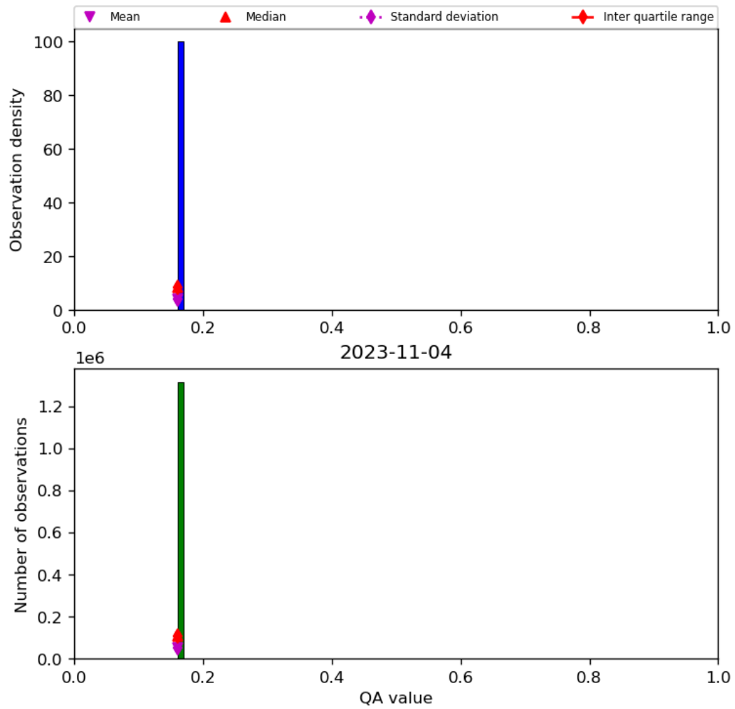
Figure 22: Histogram of “QA value” for 2023-11-03 to 2023-11-05
