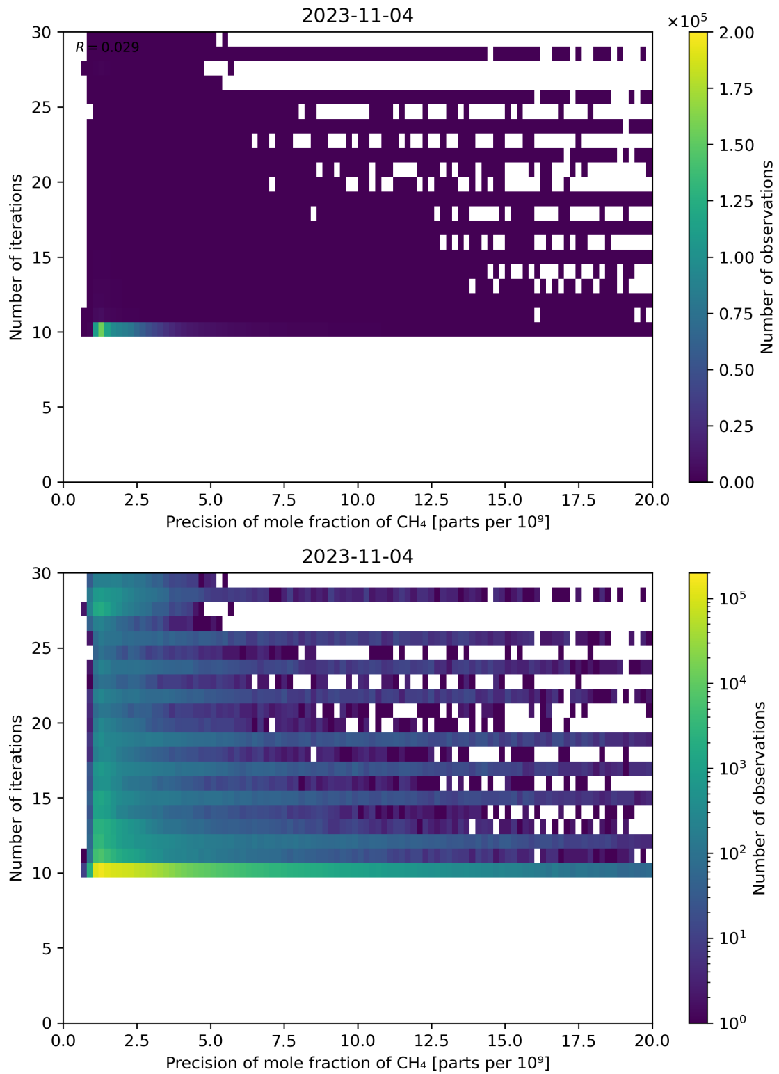
Figure 83: Scatter density plot of “Precision of mole fraction of CH 4 ” against “Number of iterations” for 2023-11-03 to 2023-11-05.
