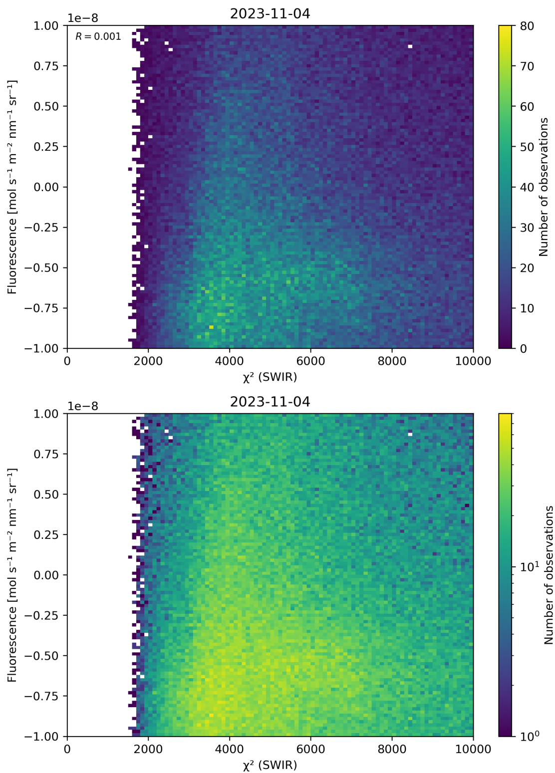
Figure 49: Scatter density plot of “ \chi^2 (SWIR)” against “Fluorescence” for 2023-11-03 to 2023-11-05.
