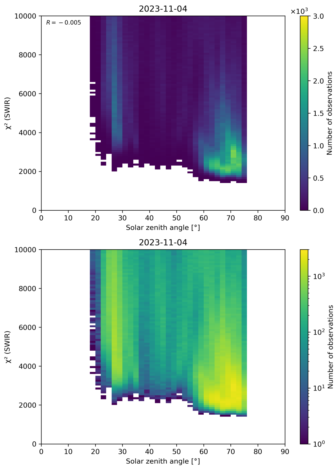
Figure 95: Scatter density plot of “Solar zenith angle” against “ \chi^2 (SWIR)” for 2023-11-03 to 2023-11-05.
