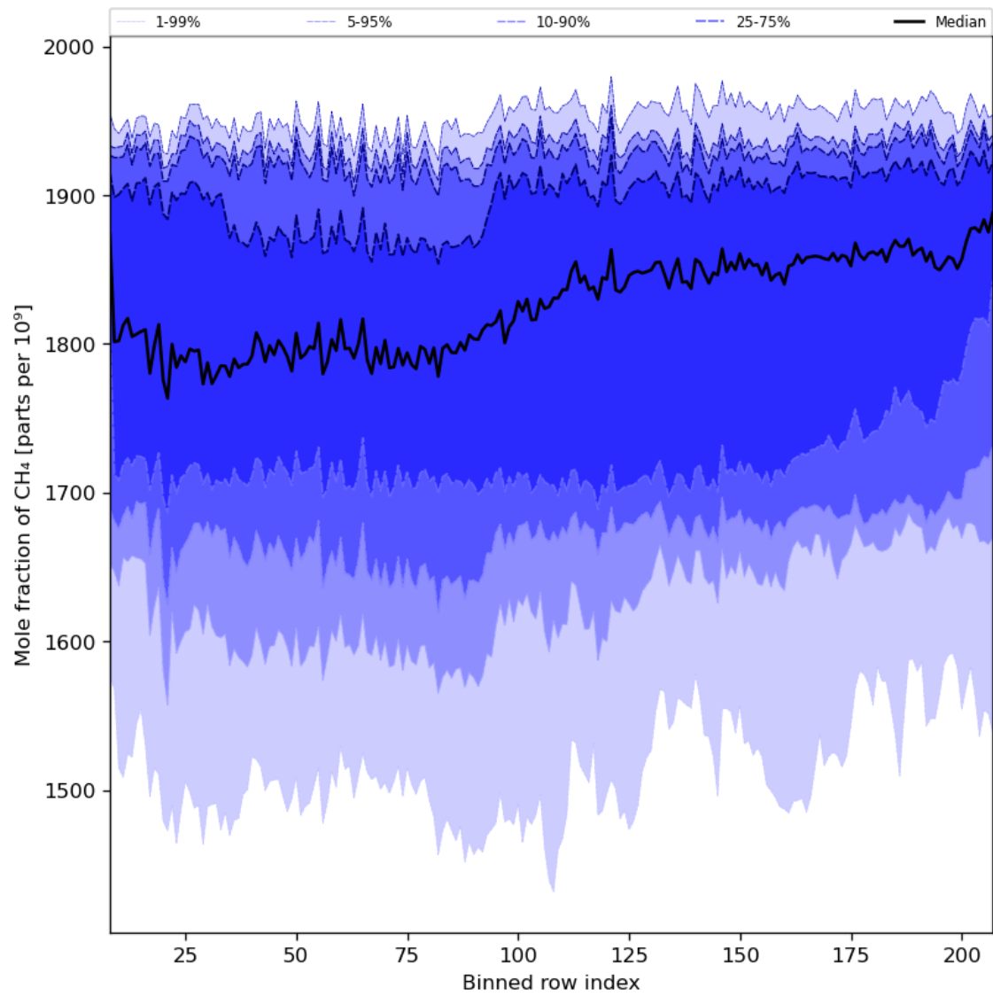
Figure 34: Along track statistics of “Mole fraction of CH 4 ” for 2023-11-03 to 2023-11-05
