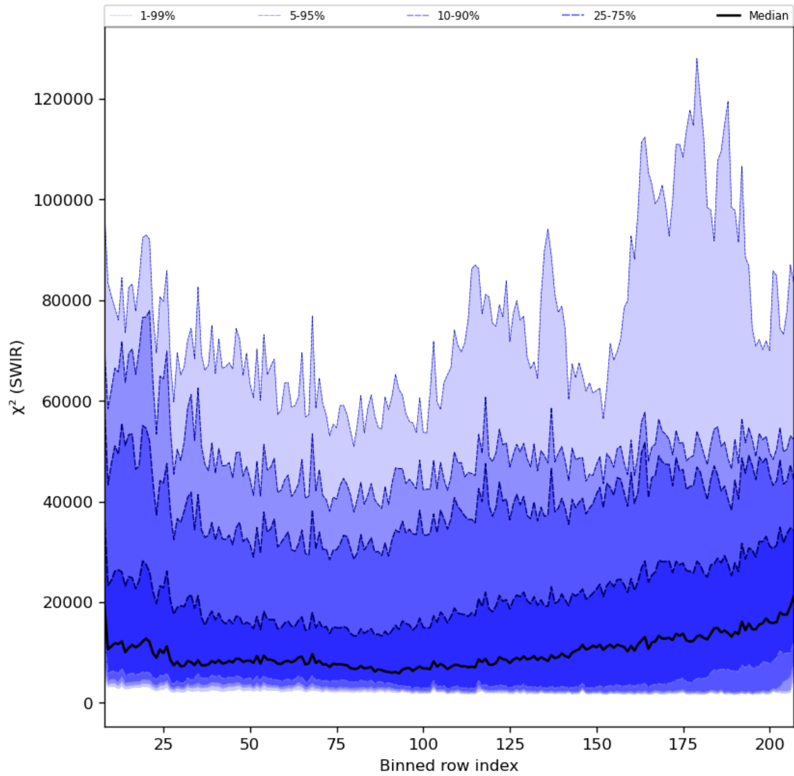
Figure 39: Along track statistics of “ \chi^2 (SWIR)” for 2023-11-03 to 2023-11-05
