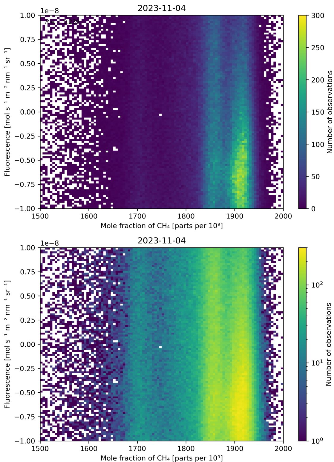
Figure 73: Scatter density plot of “Mole fraction of \text{CH}_4 ” against “Fluorescence” for 2023-11-03 to 2023-11-05.
