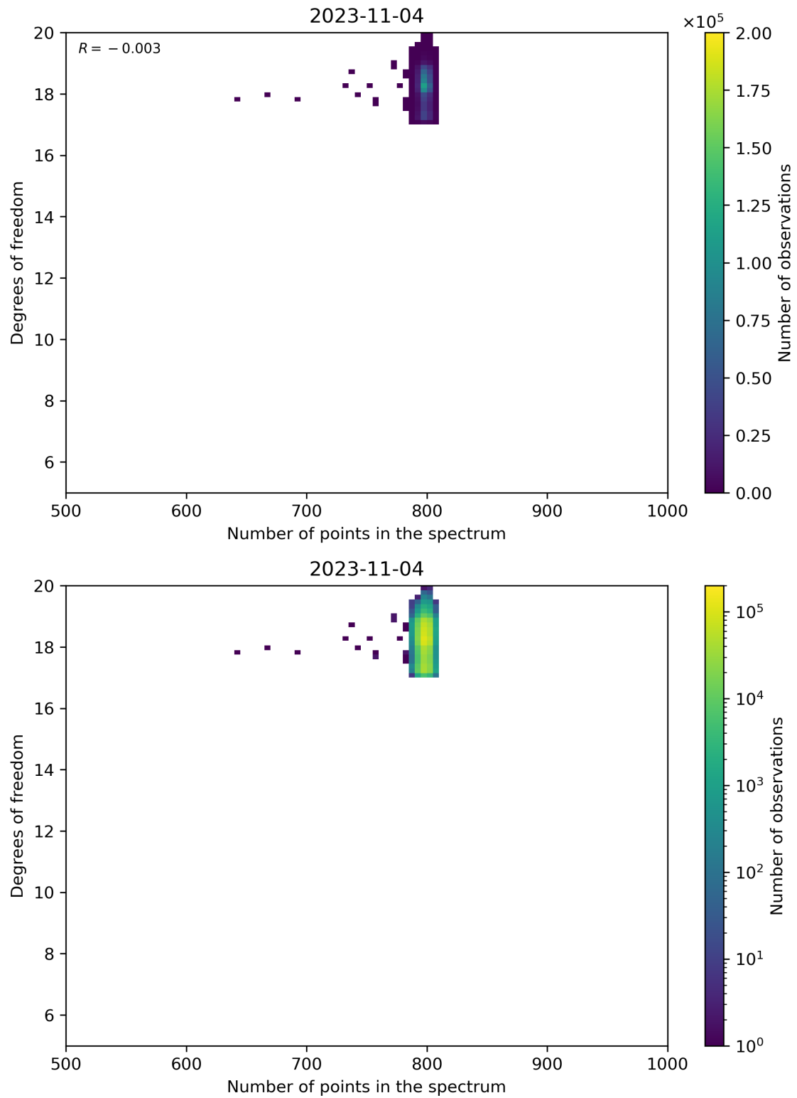
Figure 90: Scatter density plot of “Number of points in the spectrum” against “Degrees of freedom” for 2023-11-03 to 2023-11-05.
