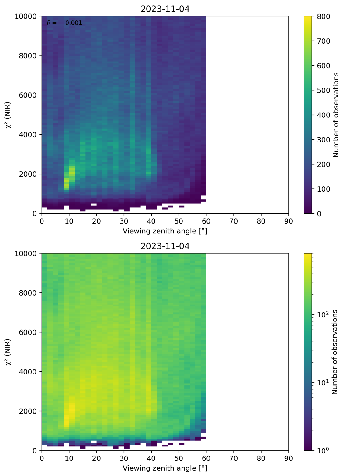
Figure 105: Scatter density plot of “Viewing zenith angle” against “ \chi^2 (NIR)” for 2023-11-03 to 2023-11-05.
