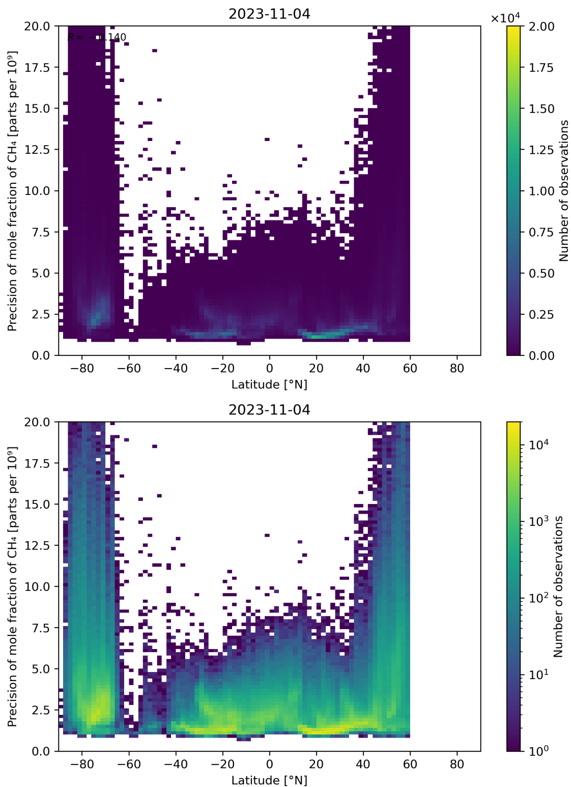
Figure 59: Scatter density plot of “Latitude” against “Precision of mole fraction of CH 4 ” for 2023-11-03 to 2023-11-05.
