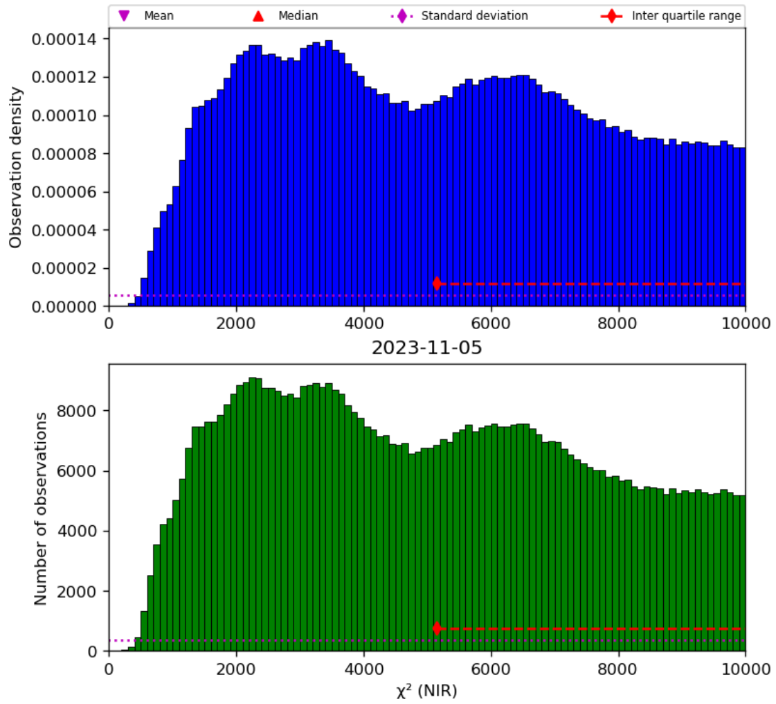
Figure 29: Histogram of " \chi^2 (NIR)" for 2023-11-04 to 2023-11-06
