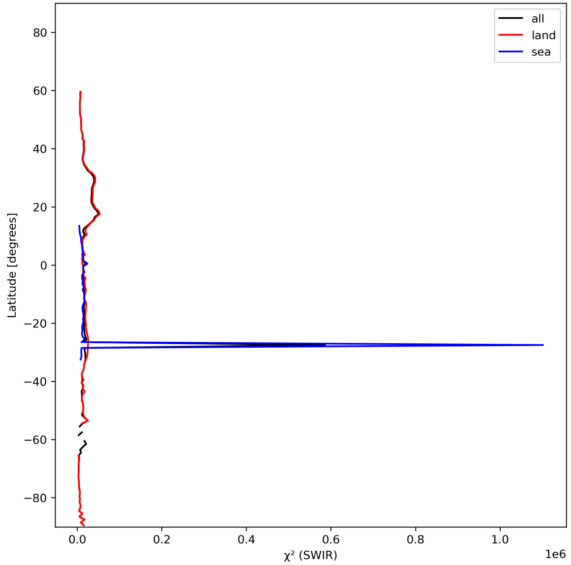
Figure 17: Zonal average of “ \chi^2 (SWIR)” for 2023-11-04 to 2023-11-06.
