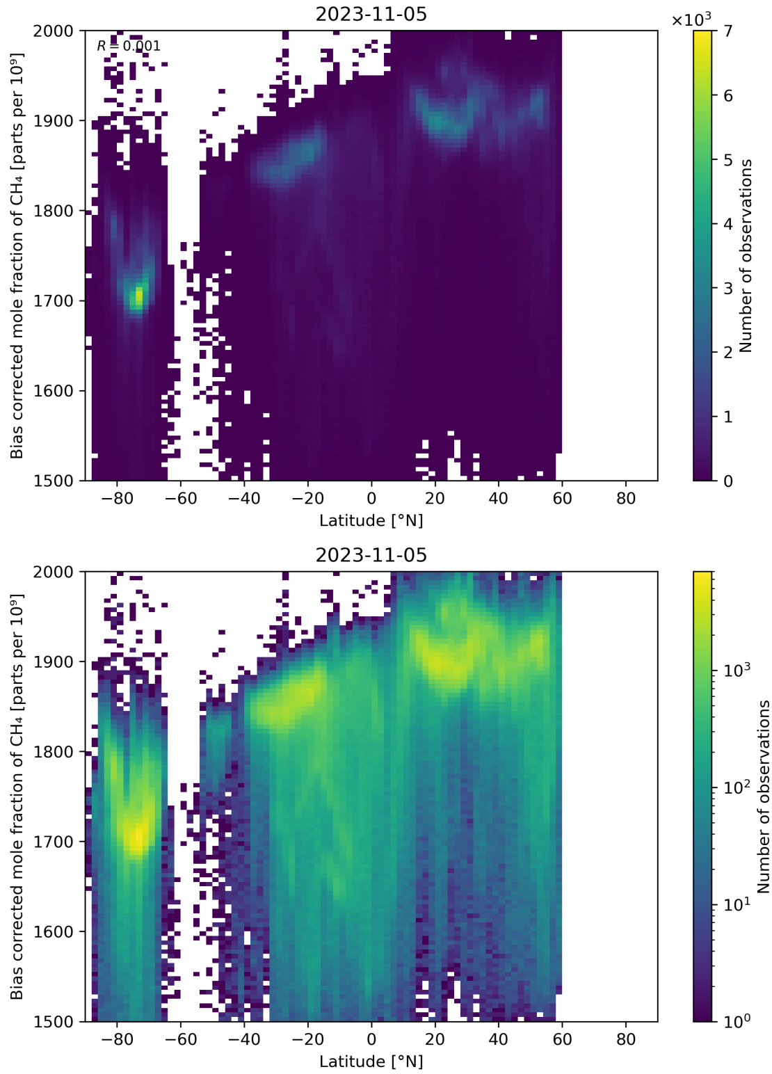
Figure 58: Scatter density plot of “Latitude” against “Bias corrected mole fraction of CH 4 ” for 2023-11-04 to 2023-11-06.
