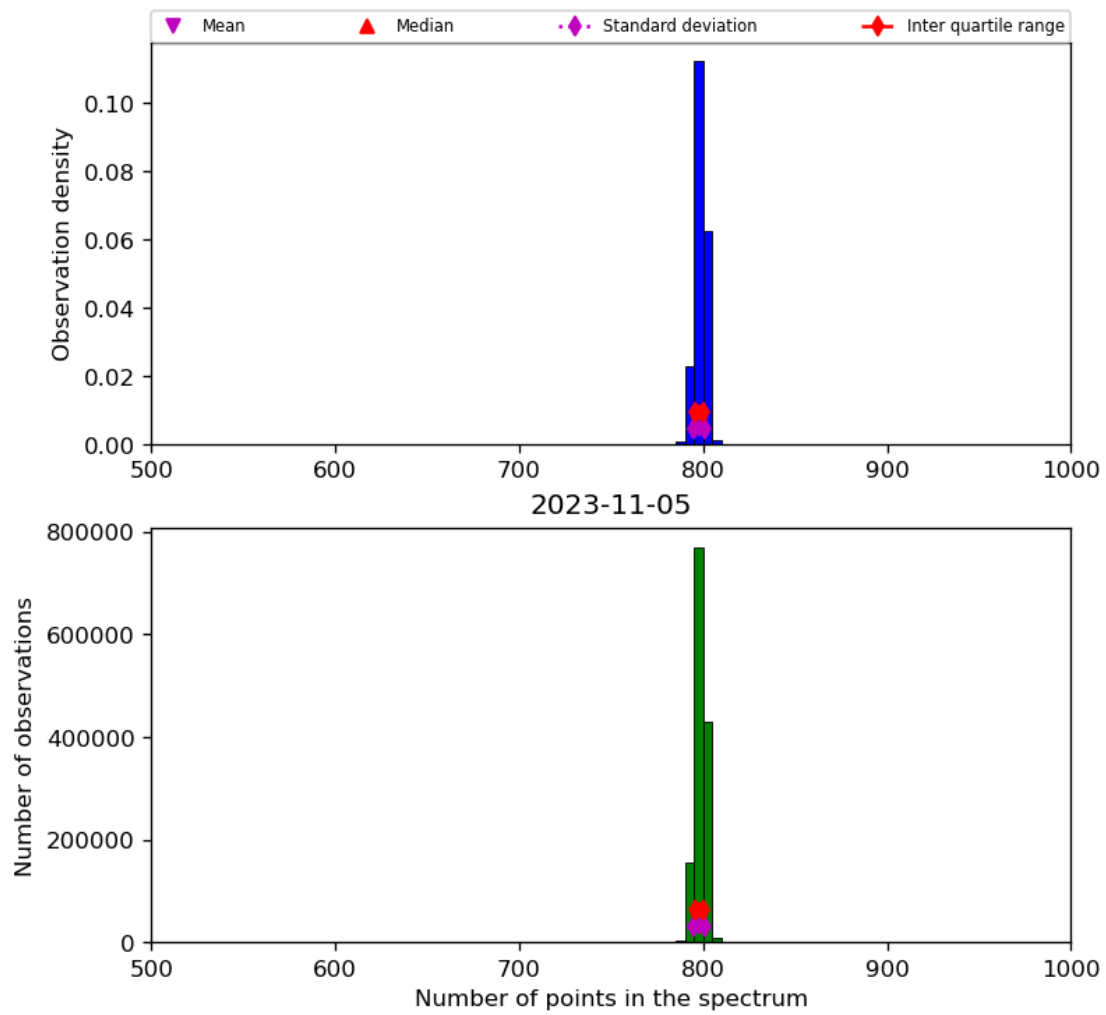
Figure 26: Histogram of “Number of points in the spectrum” for 2023-11-04 to 2023-11-06
