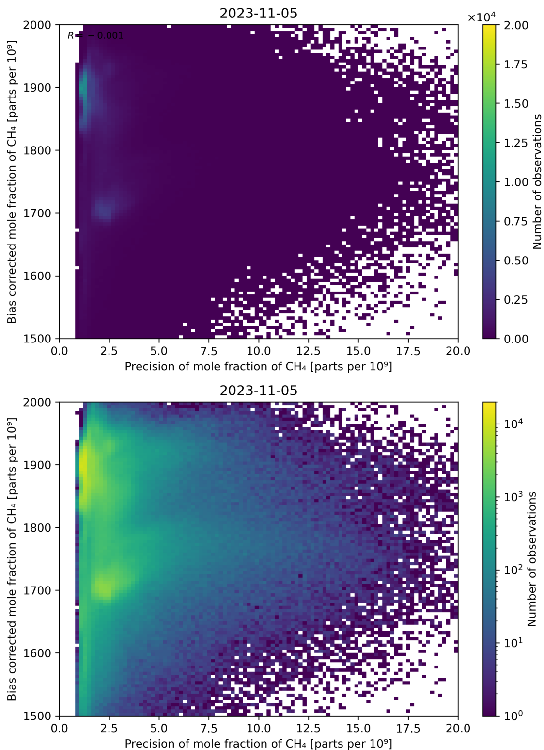
Figure 82: Scatter density plot of “Precision of mole fraction of CH 4 ” against “Bias corrected mole fraction of CH 4 ” for 2023-11-04 to 2023-11-06.
