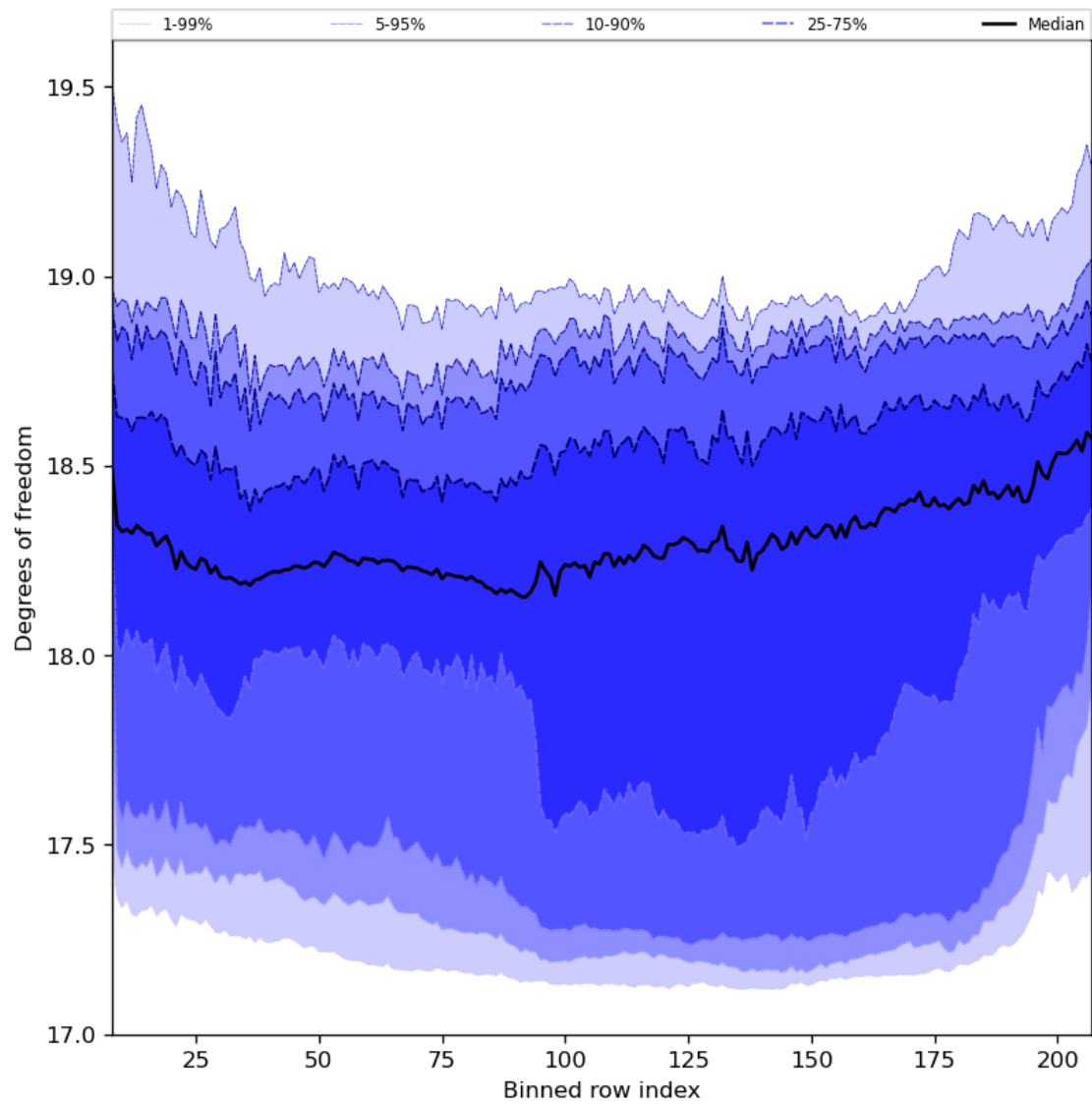
Figure 41: Along track statistics of “Degrees of freedom” for 2023-11-04 to 2023-11-06
