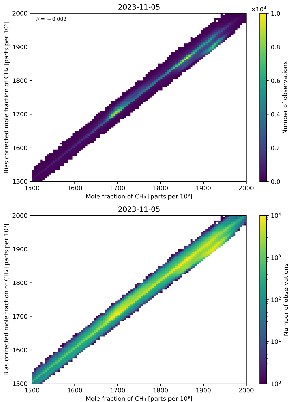
Figure 74: Scatter density plot of “Mole fraction of CH 4 ” against “Bias corrected mole fraction of CH 4 ” for 2023-11-04 to 2023-11-06.
