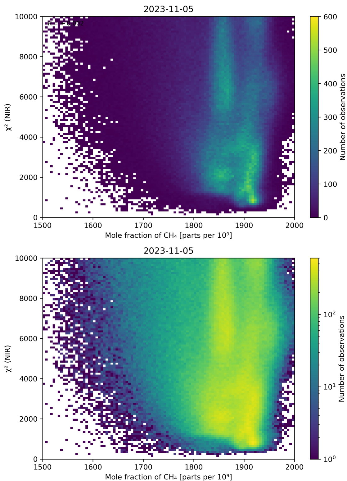
Figure 70: Scatter density plot of “Mole fraction of \text{CH}_4 ” against “ \chi^2 (NIR)” for 2023-11-04 to 2023-11-06.
