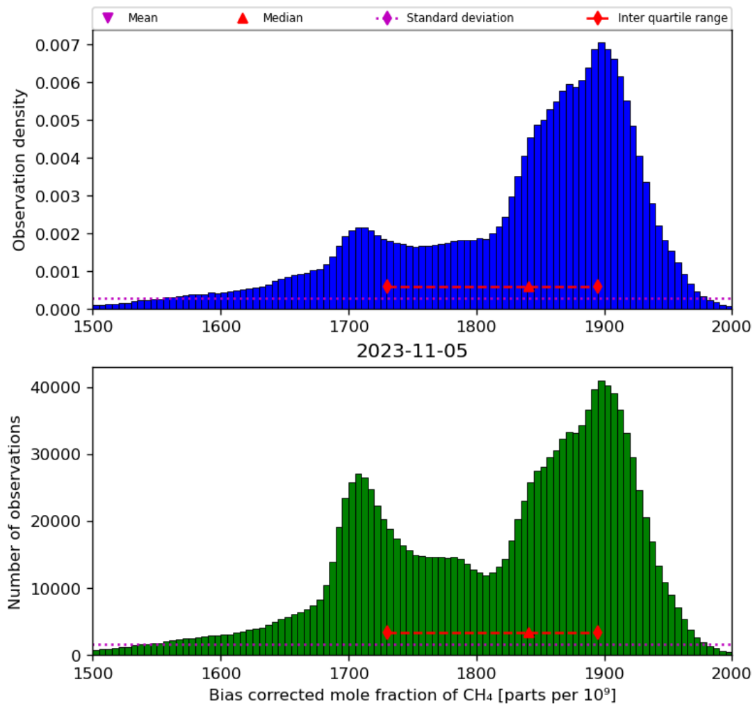
Figure 25: Histogram of “Bias corrected mole fraction of CH 4 ” for 2023-11-04 to 2023-11-06
