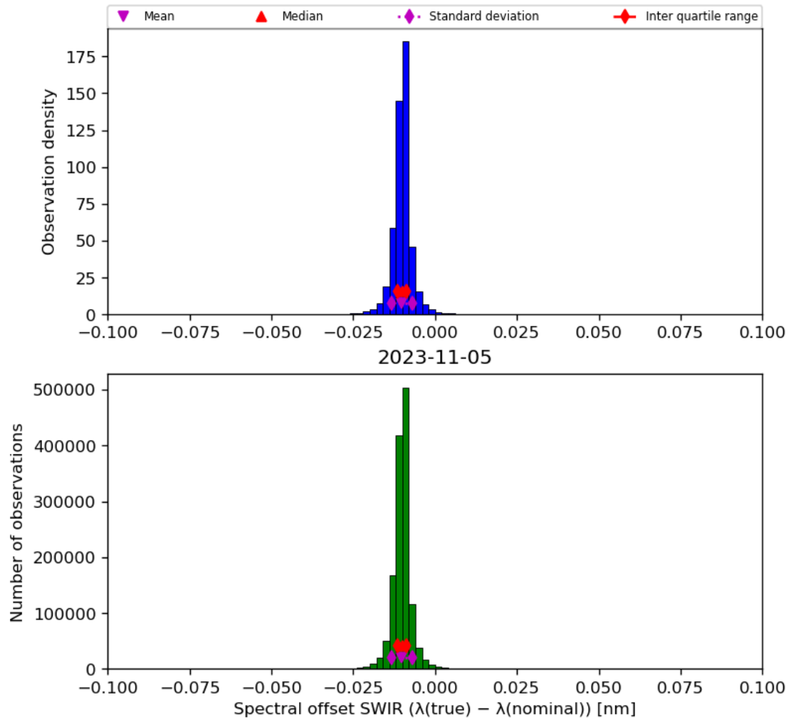
Figure 27: Histogram of “Spectral offset SWIR ( \lambda(\text{true}) - \lambda(\text{nominal}) )” for 2023-11-04 to 2023-11-06
