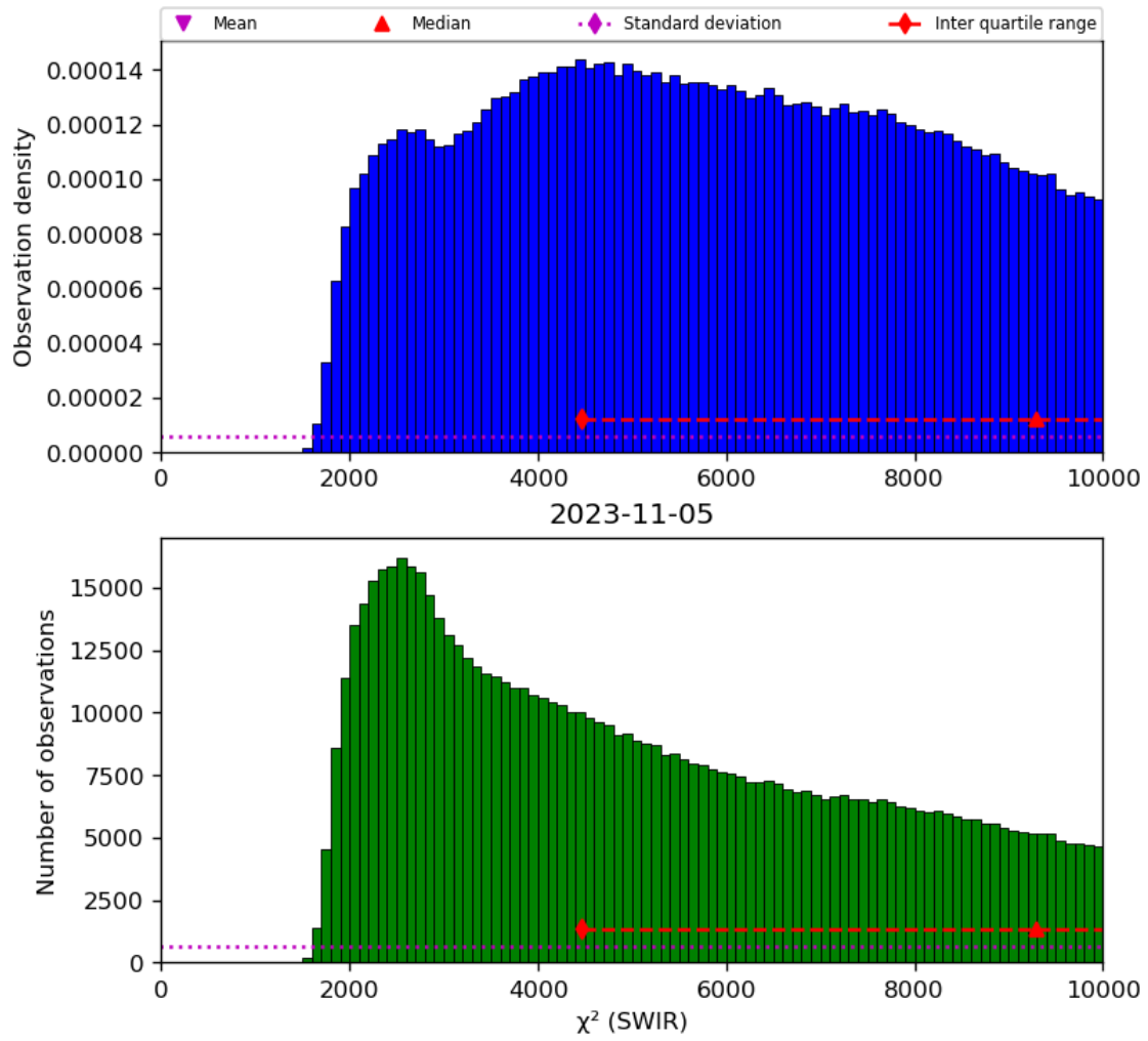
Figure 28: Histogram of “ \chi^2 (SWIR)” for 2023-11-04 to 2023-11-06
