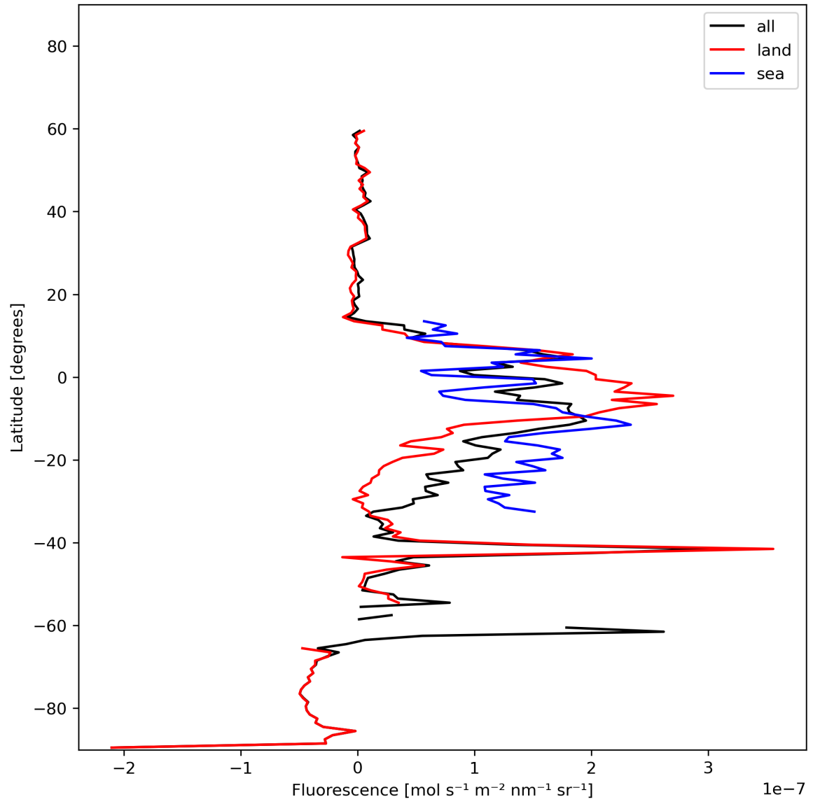
Figure 21: Zonal average of “Fluorescence” for 2023-11-04 to 2023-11-06.
