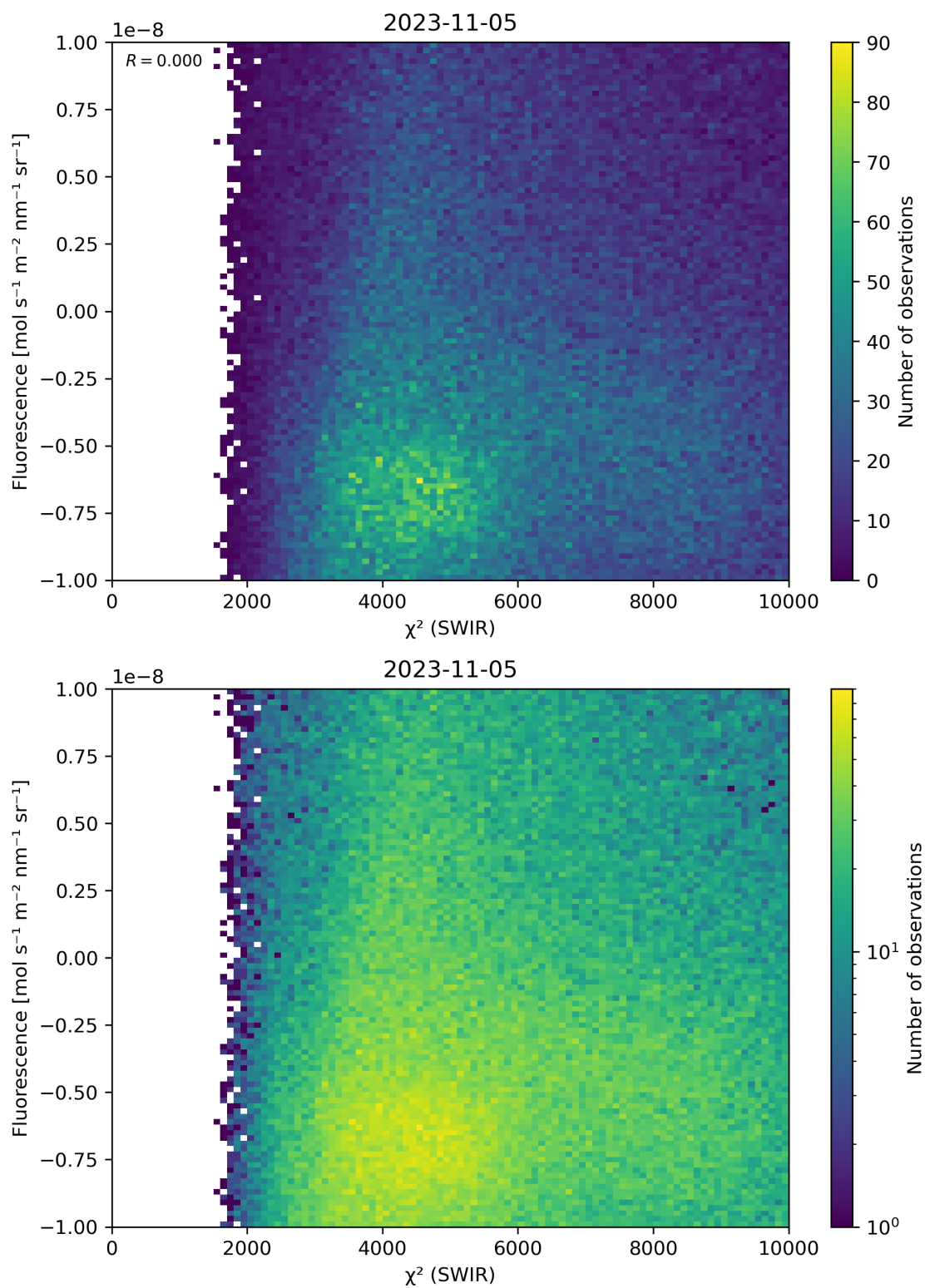
Figure 49: Scatter density plot of “ \chi^2 (SWIR)” against “Fluorescence” for 2023-11-04 to 2023-11-06.
