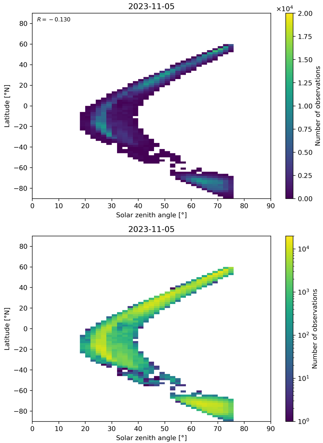
Figure 98: Scatter density plot of “Solar zenith angle” against “Latitude” for 2023-11-04 to 2023-11-06.
