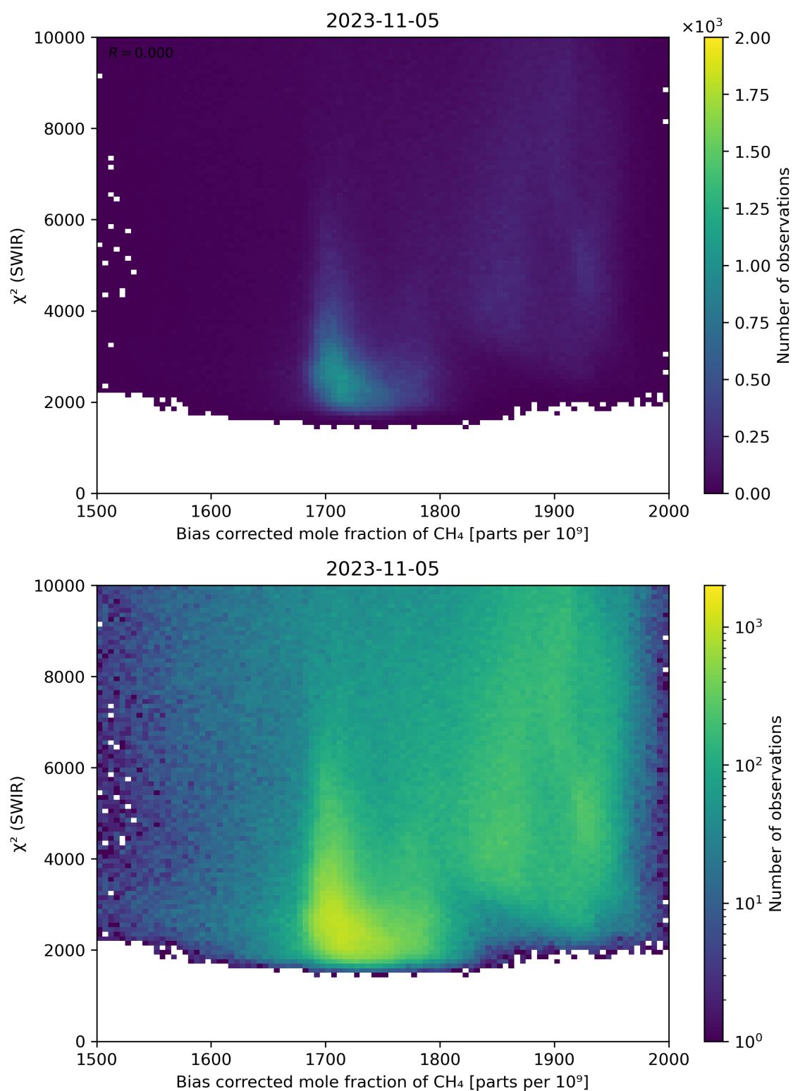
Figure 64: Scatter density plot of “Bias corrected mole fraction of CH 4 ” against “ \chi^2 (SWIR)” for 2023-11-04 to 2023-11-06.
