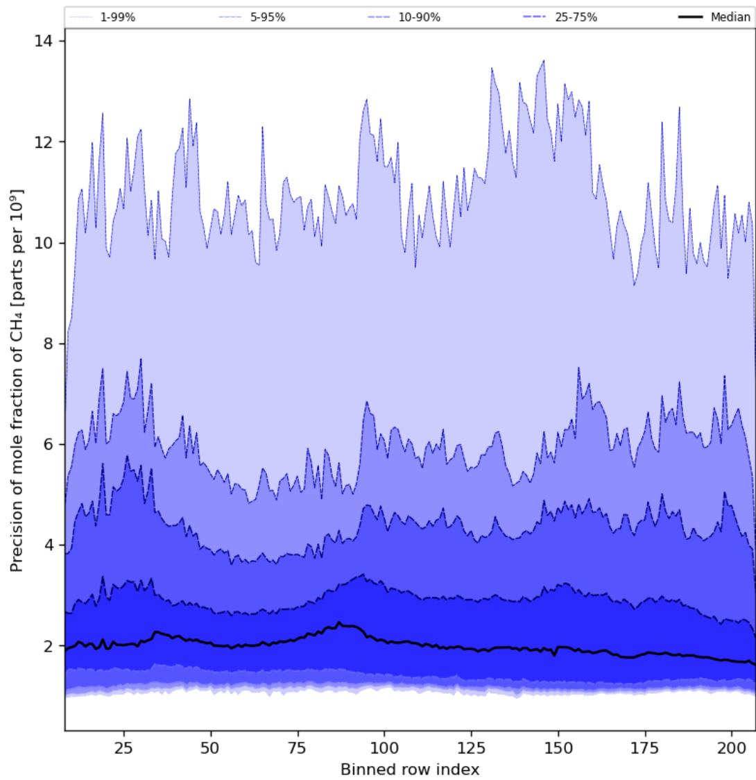
Figure 35: Along track statistics of “Precision of mole fraction of CH 4 ” for 2023-11-04 to 2023-11-06
