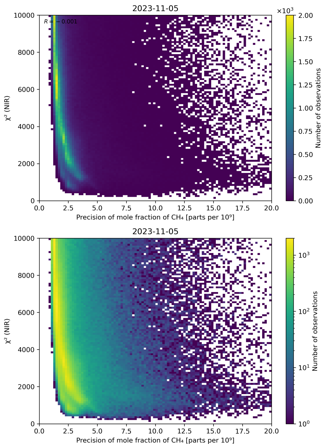
Figure 78: Scatter density plot of “Precision of mole fraction of CH 4 ” against “ \chi^2 (NIR)” for 2023-11-04 to 2023-11-06.
