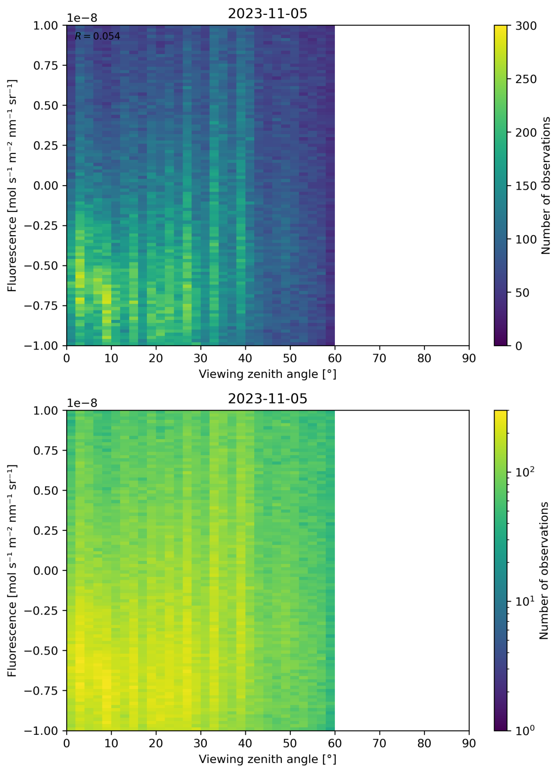
Figure 108: Scatter density plot of “Viewing zenith angle” against “Fluorescence” for 2023-11-04 to 2023-11-06.
