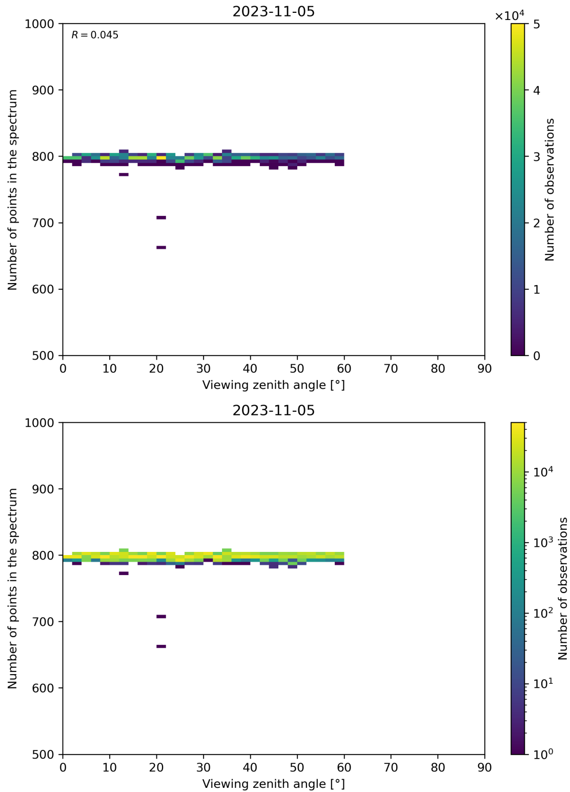
Figure 114: Scatter density plot of “Viewing zenith angle” against “Number of points in the spectrum” for 2023-11-04 to 2023-11-06.
