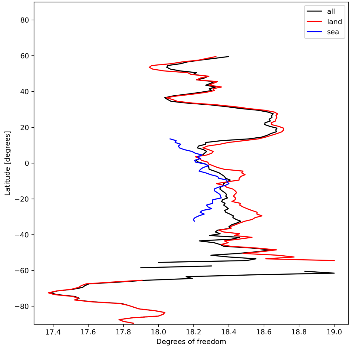
Figure 19: Zonal average of “Degrees of freedom” for 2023-11-04 to 2023-11-06.
