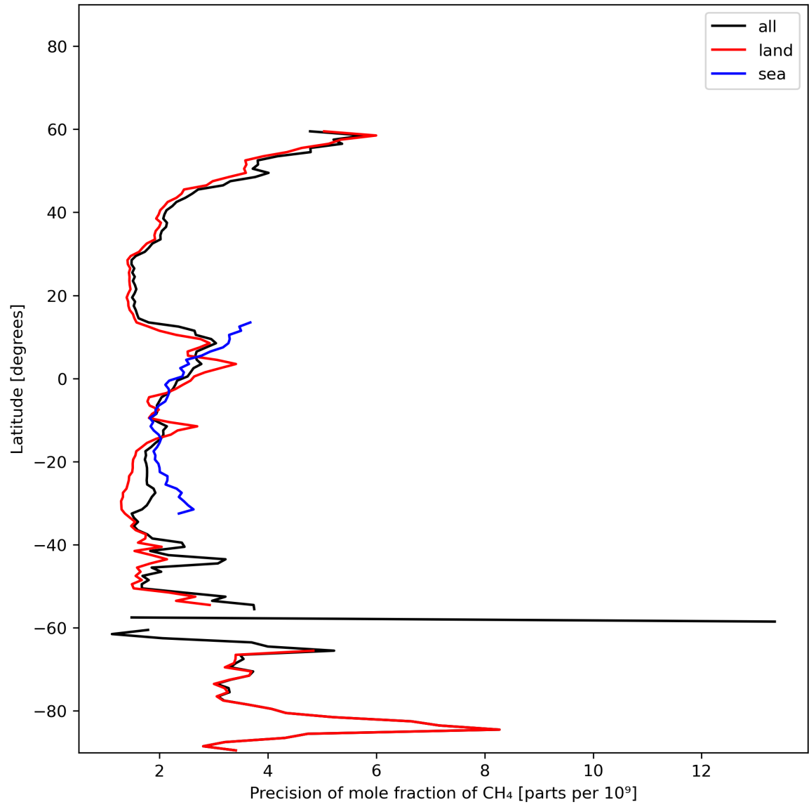
Figure 13: Zonal average of “Precision of mole fraction of CH 4 ” for 2023-11-04 to 2023-11-06.
