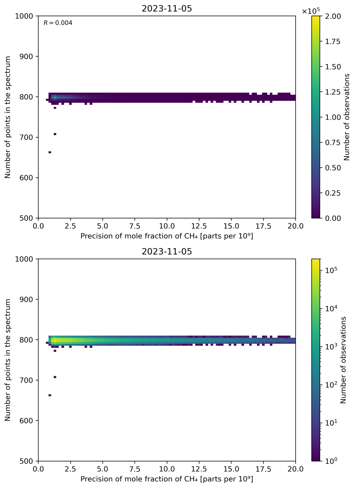
Figure 84: Scatter density plot of “Precision of mole fraction of \text{CH}_4 ” against “Number of points in the spectrum” for 2023-11-04 to 2023-11-06.
