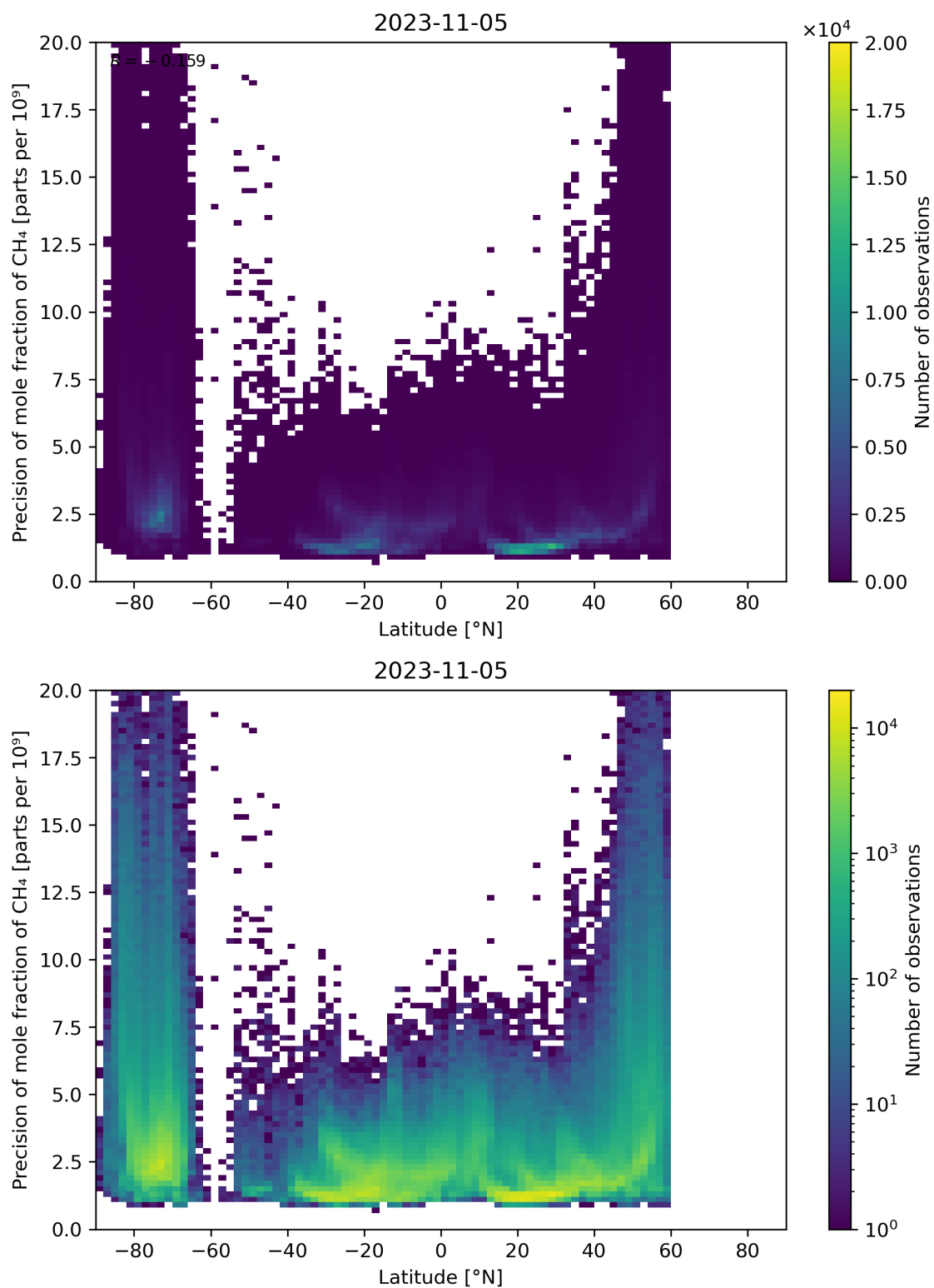
Figure 59: Scatter density plot of “Latitude” against “Precision of mole fraction of CH 4 ” for 2023-11-04 to 2023-11-06.
