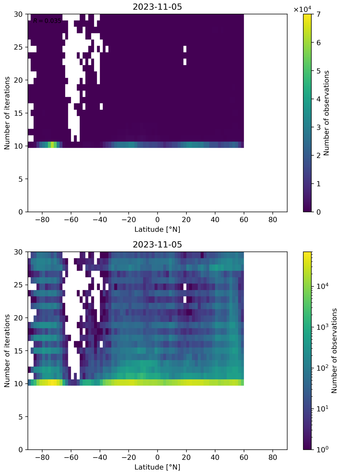
Figure 60: Scatter density plot of “Latitude” against “Number of iterations” for 2023-11-04 to 2023-11-06.
