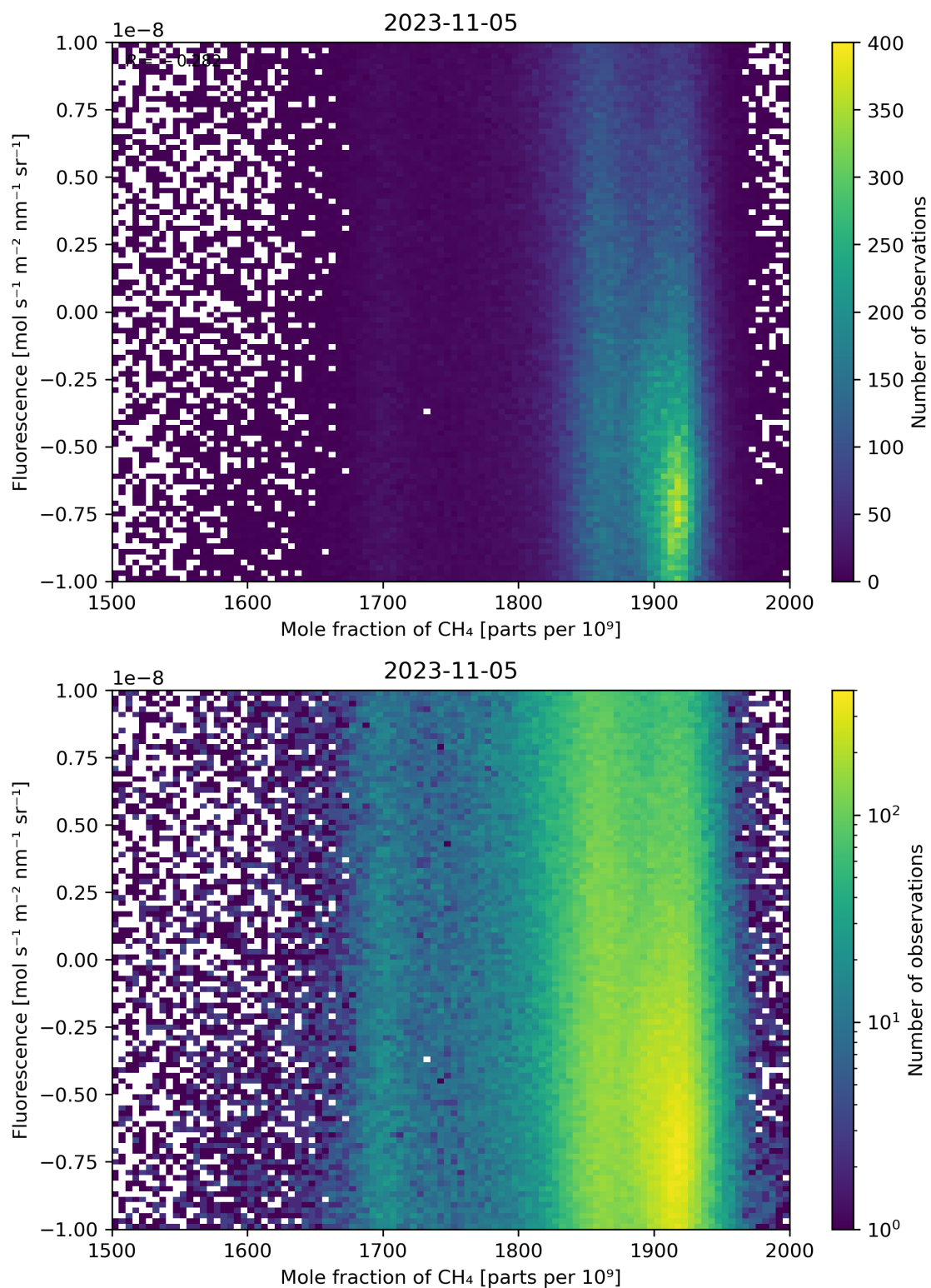
Figure 73: Scatter density plot of “Mole fraction of \text{CH}_4 ” against “Fluorescence” for 2023-11-04 to 2023-11-06.
