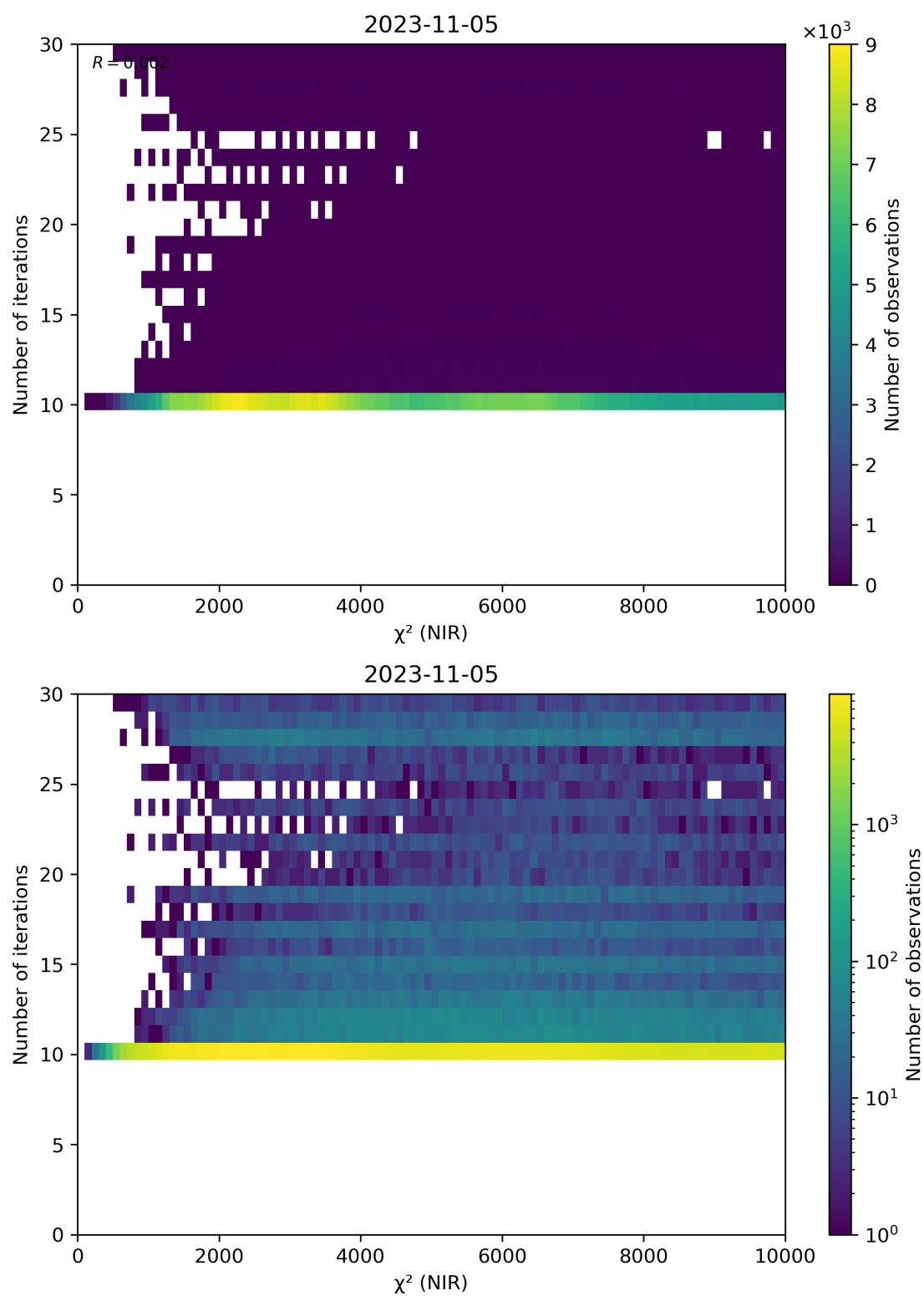
Figure 46: Scatter density plot of “ \chi^2 (NIR)” against “Number of iterations” for 2023-11-04 to 2023-11-06.
