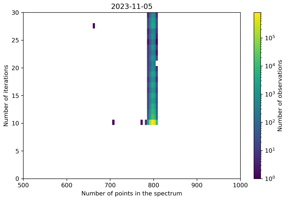
Figure 92: Scatter density plot of “Number of points in the spectrum” against “Number of iterations” for 2023-11-04 to 2023-11-06.
