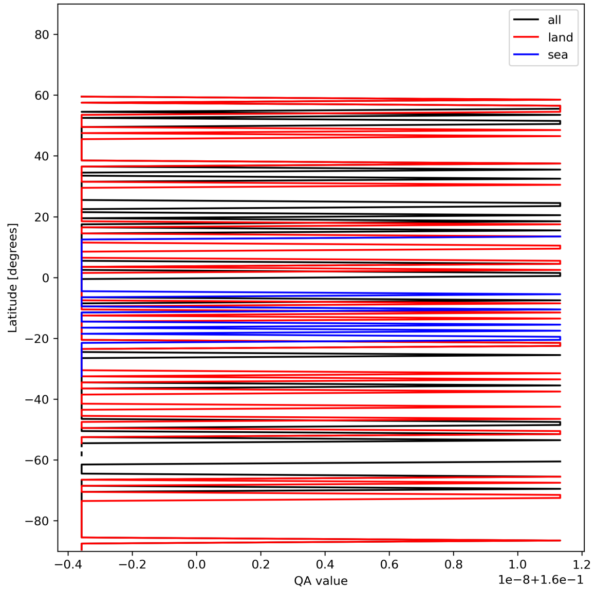
Figure 11: Zonal average of “QA value” for 2023-11-04 to 2023-11-06.
