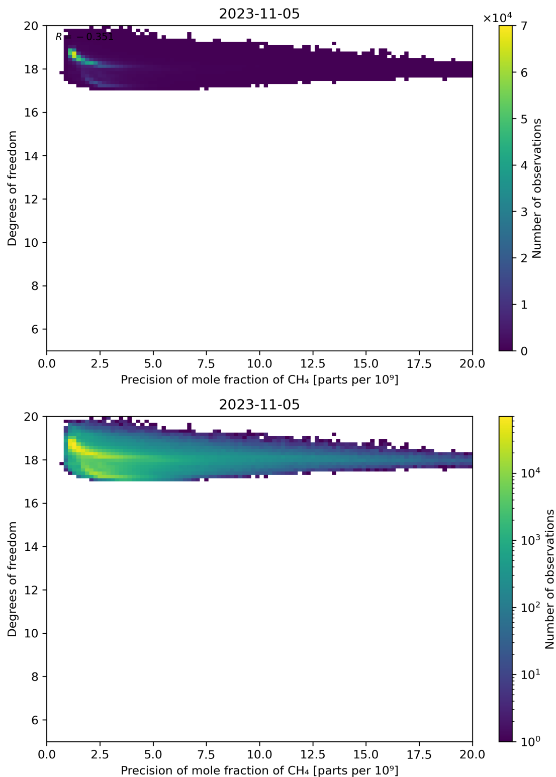
Figure 80: Scatter density plot of “Precision of mole fraction of CH 4 ” against “Degrees of freedom” for 2023-11-04 to 2023-11-06.
