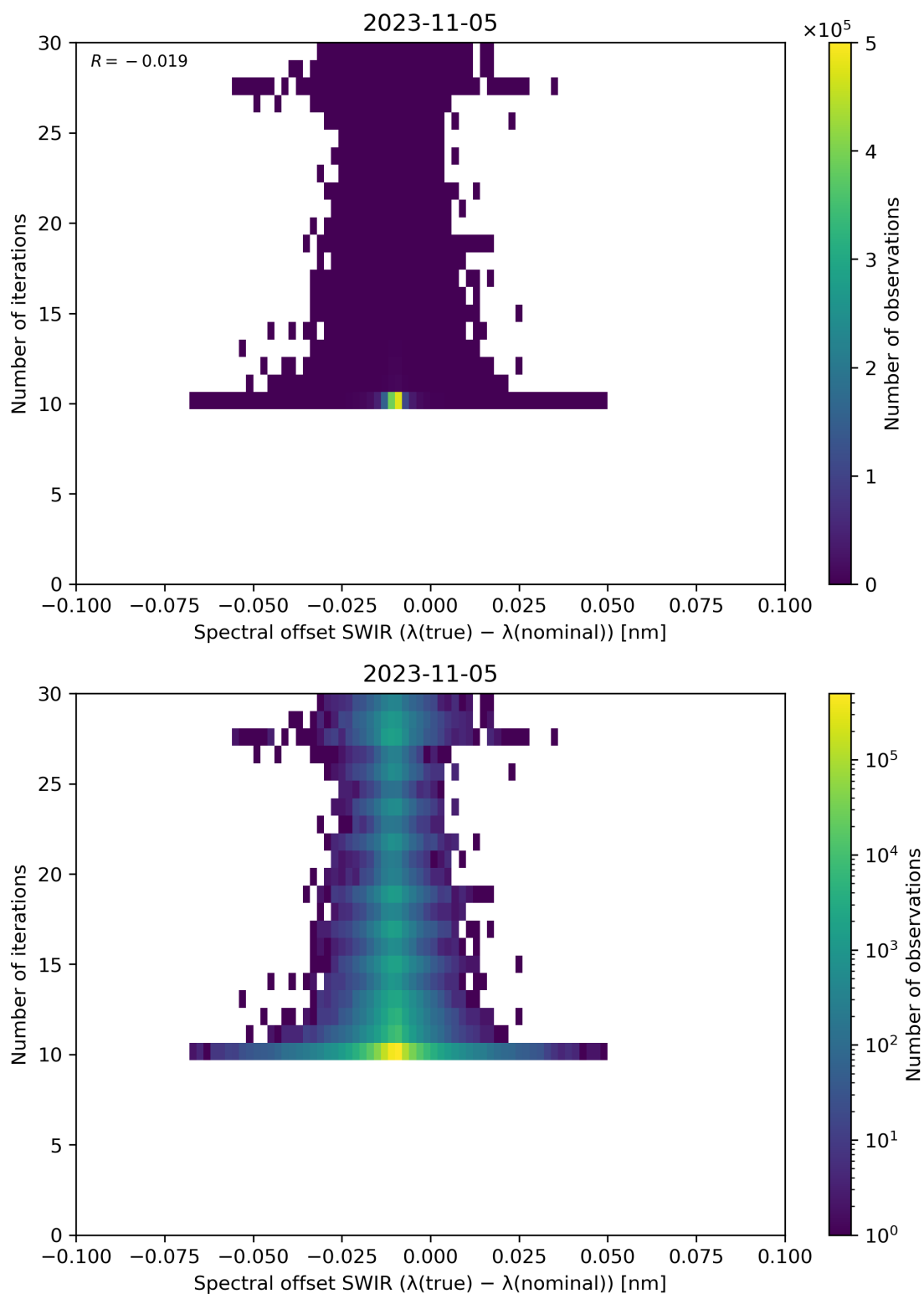
Figure 121: Scatter density plot of “Spectral offset SWIR ( \lambda(\text{true}) - \lambda(\text{nominal}) )” against “Number of iterations” for 2023-11-04 to 2023-11-06.
