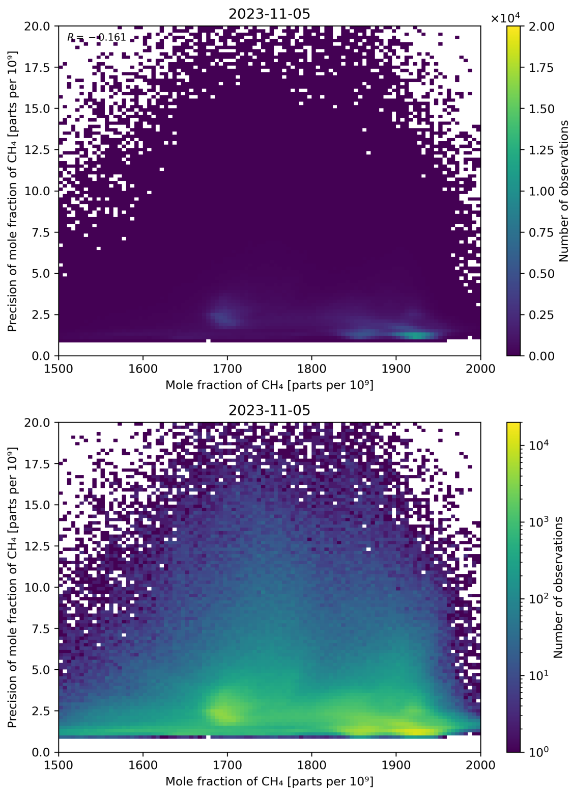
Figure 75: Scatter density plot of “Mole fraction of CH 4 ” against “Precision of mole fraction of CH 4 ” for 2023-11-04 to 2023-11-06.
