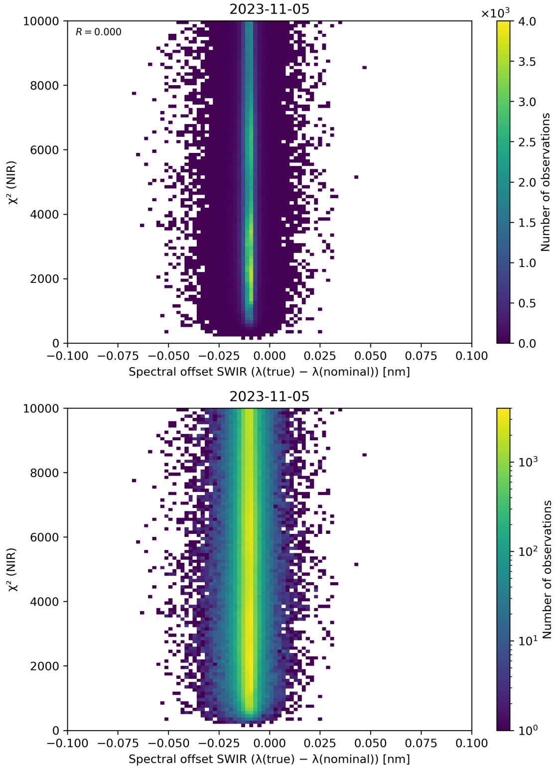
Figure 117: Scatter density plot of “Spectral offset SWIR ( \lambda(\text{true}) - \lambda(\text{nominal}) )” against “ \chi^2 (NIR)” for 2023-11-04 to 2023-11-06.
