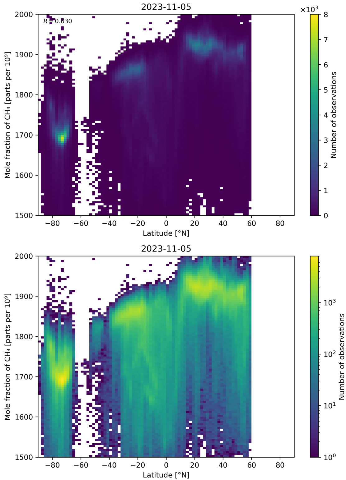
Figure 57: Scatter density plot of “Latitude” against “Mole fraction of CH 4 ” for 2023-11-04 to 2023-11-06.
