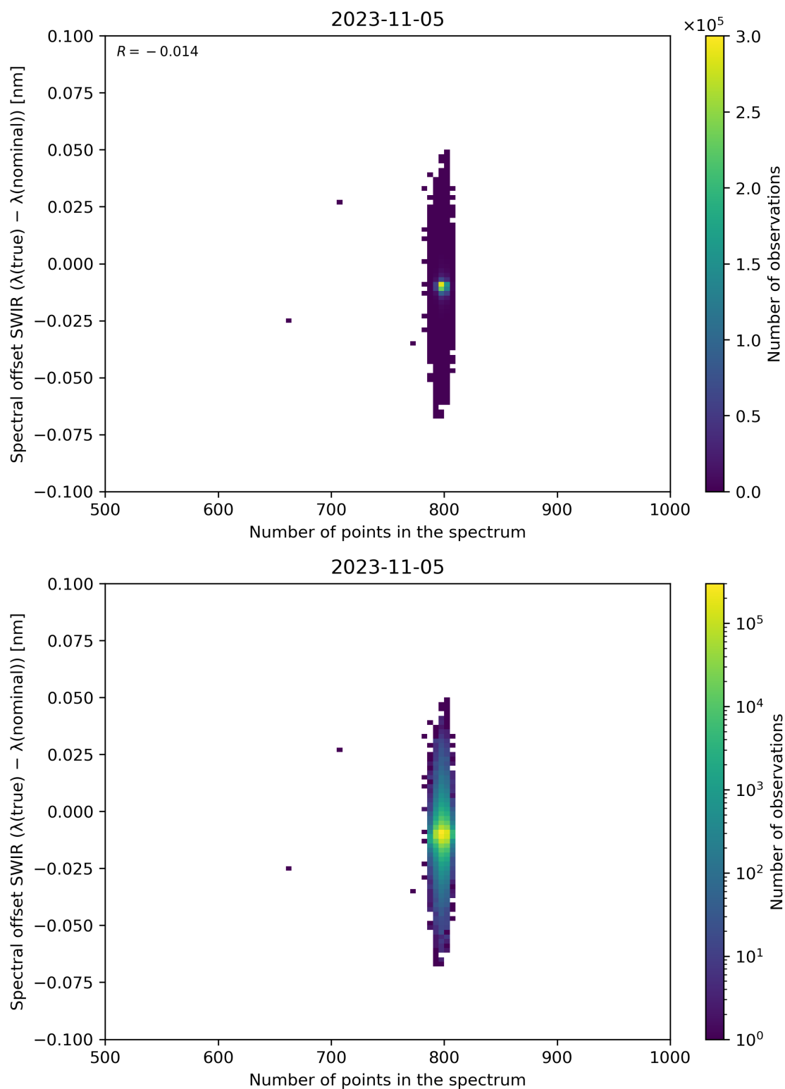
Figure 93: Scatter density plot of “Number of points in the spectrum” against “Spectral offset SWIR ( \lambda(\text{true}) - \lambda(\text{nominal}) )” for 2023-11-04 to 2023-11-06.
