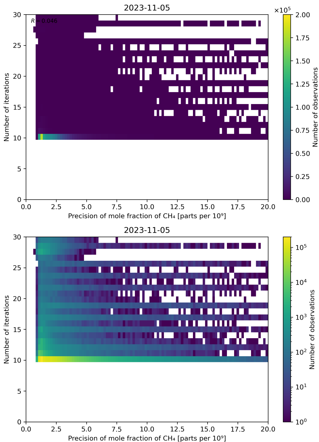
Figure 83: Scatter density plot of “Precision of mole fraction of CH 4 ” against “Number of iterations” for 2023-11-04 to 2023-11-06.
