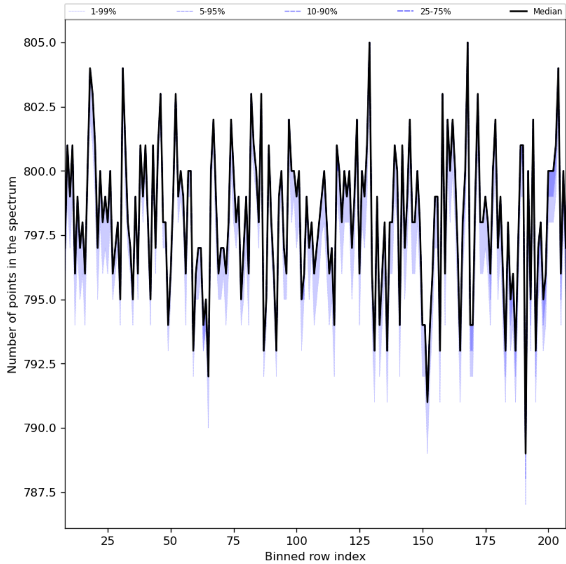
Figure 37: Along track statistics of “Number of points in the spectrum” for 2023-11-04 to 2023-11-06
