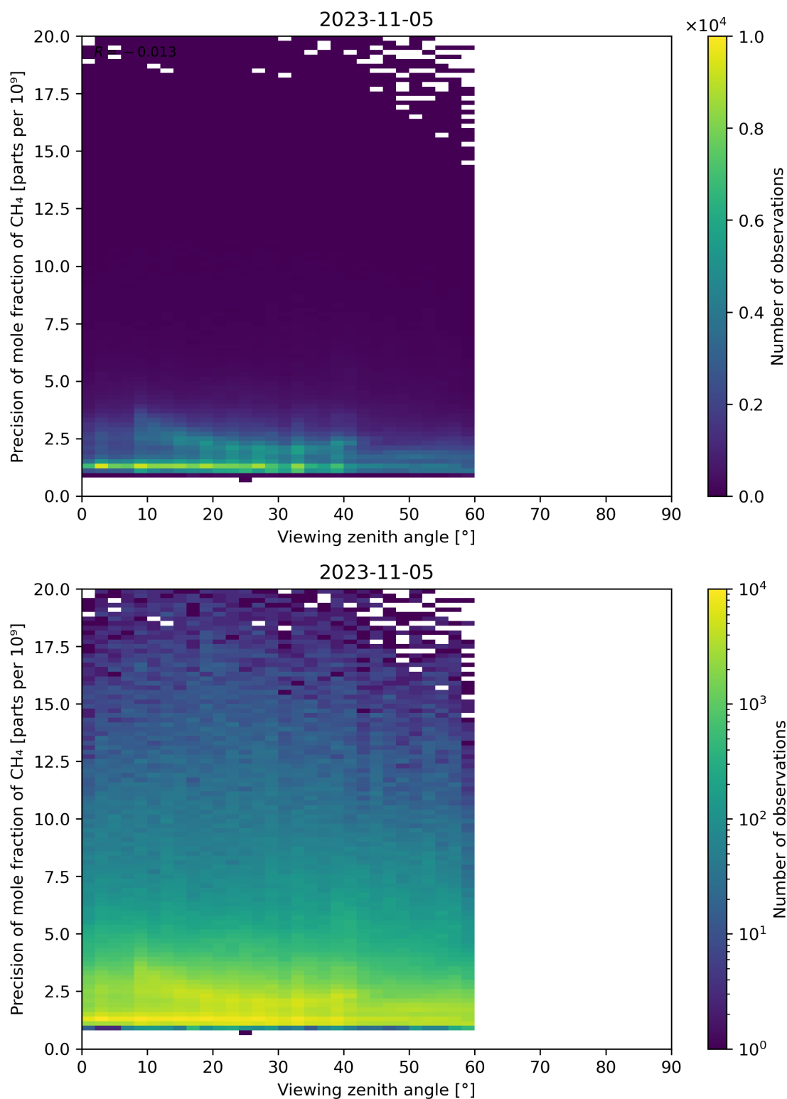
Figure 112: Scatter density plot of “Viewing zenith angle” against “Precision of mole fraction of CH 4 ” for 2023-11-04 to 2023-11-06.
