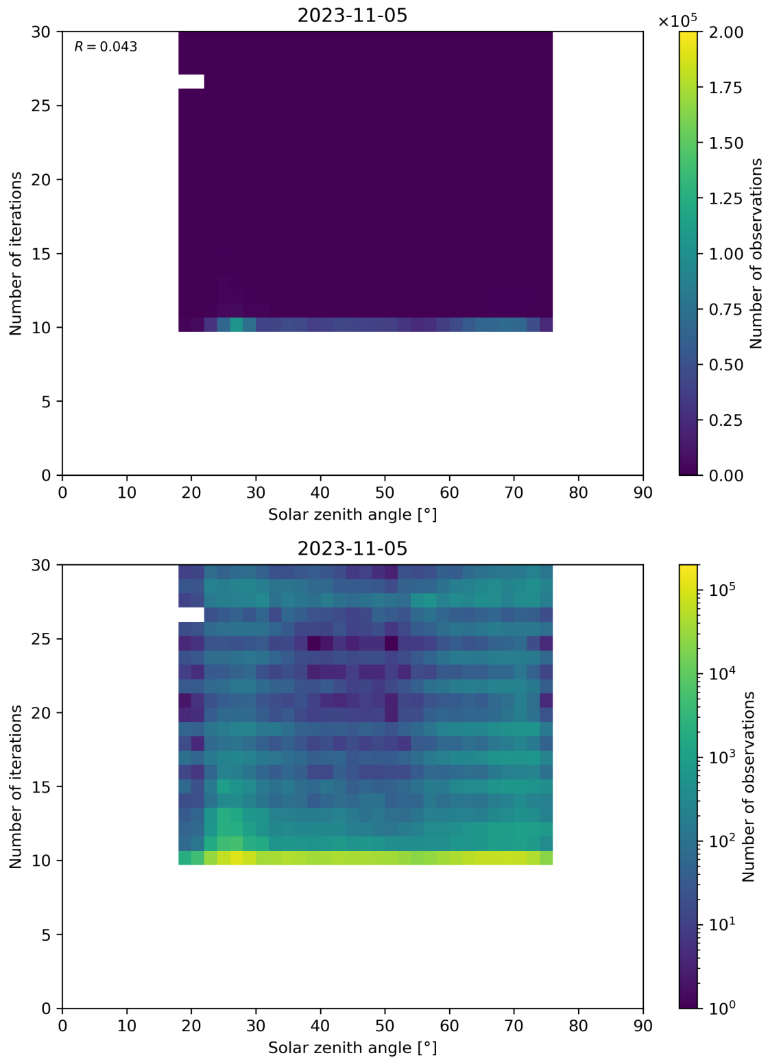
Figure 102: Scatter density plot of “Solar zenith angle” against “Number of iterations” for 2023-11-04 to 2023-11-06.
