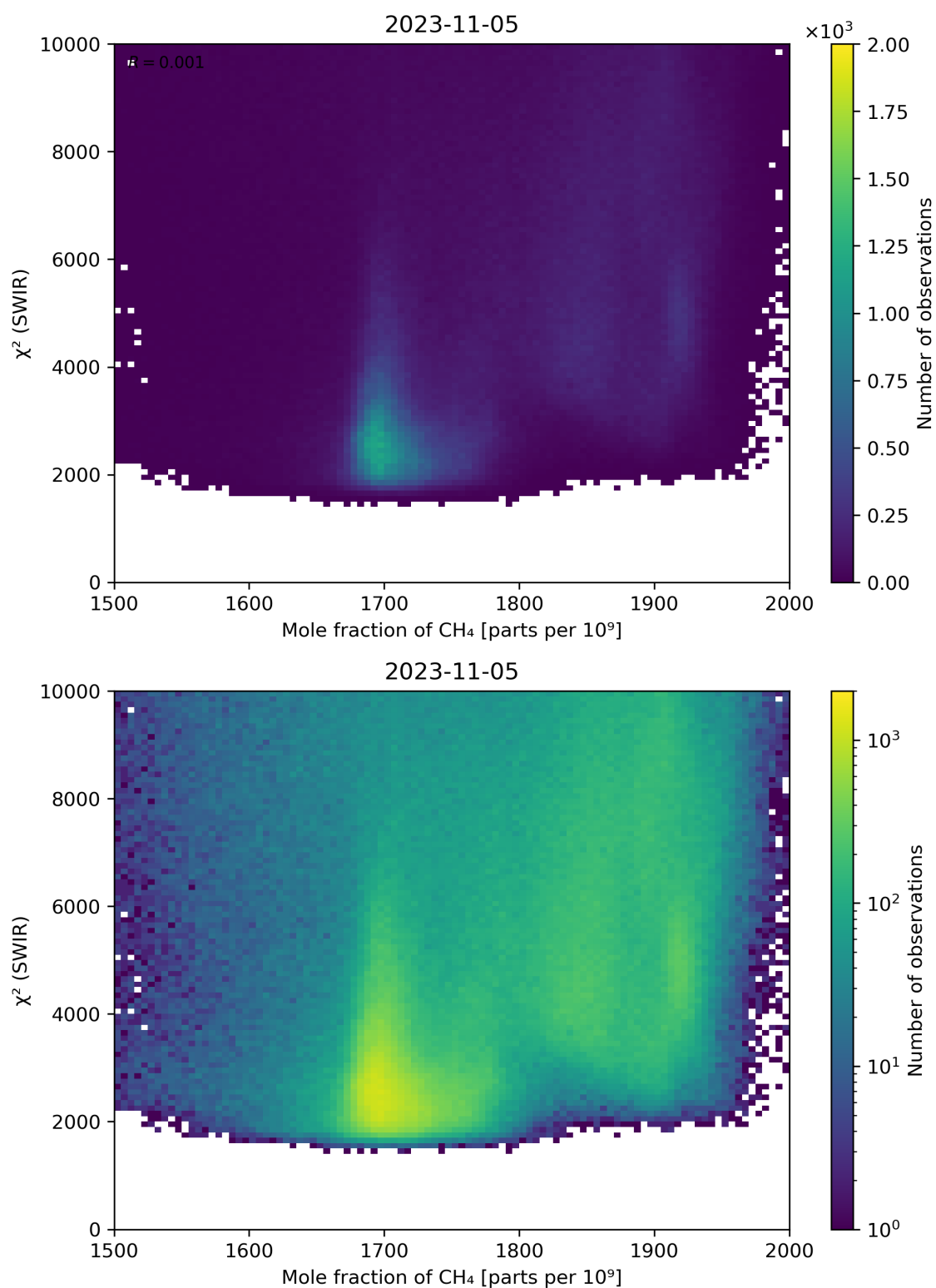
Figure 71: Scatter density plot of “Mole fraction of CH 4 ” against “ \chi^2 (SWIR)” for 2023-11-04 to 2023-11-06.
