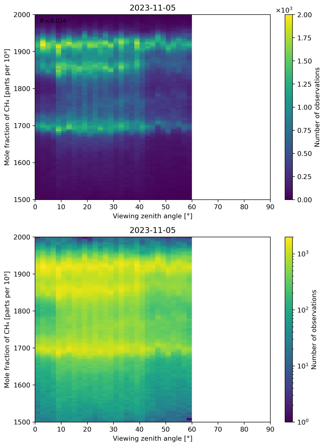
Figure 110: Scatter density plot of “Viewing zenith angle” against “Mole fraction of CH 4 ” for 2023-11-04 to 2023-11-06.
