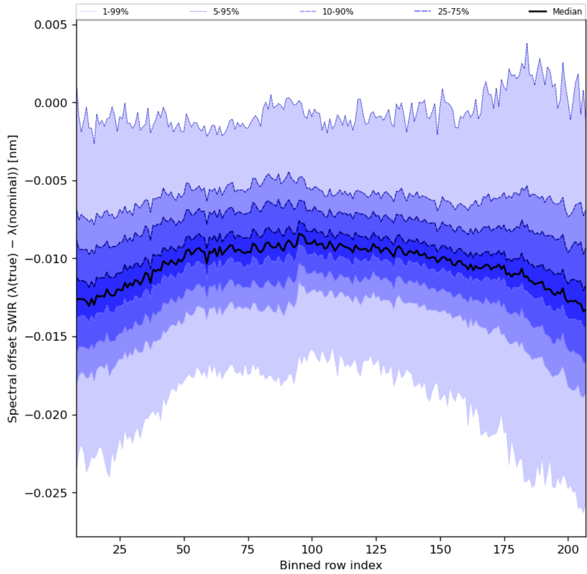
Figure 38: Along track statistics of “Spectral offset SWIR ( \lambda(\text{true}) - \lambda(\text{nominal}) )” for 2023-11-04 to 2023-11-06
