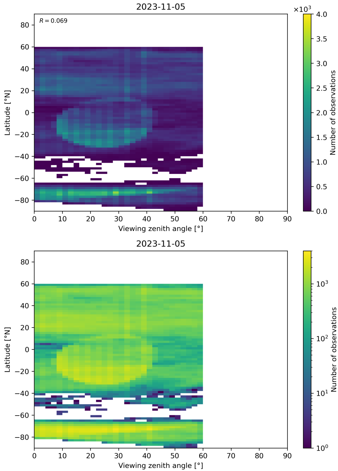
Figure 109: Scatter density plot of “Viewing zenith angle” against “Latitude” for 2023-11-04 to 2023-11-06.
