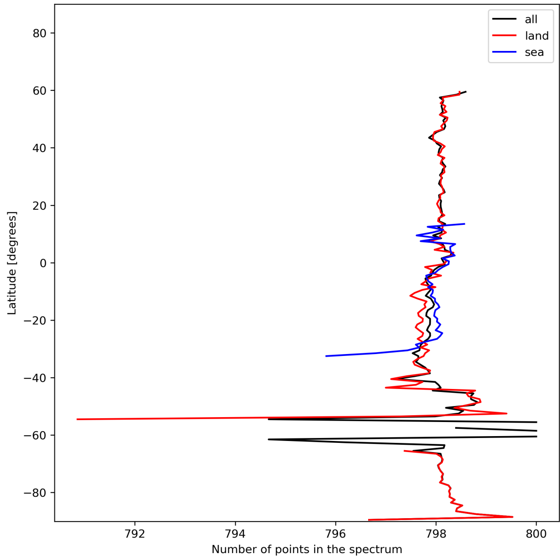
Figure 15: Zonal average of “Number of points in the spectrum” for 2023-11-04 to 2023-11-06.
