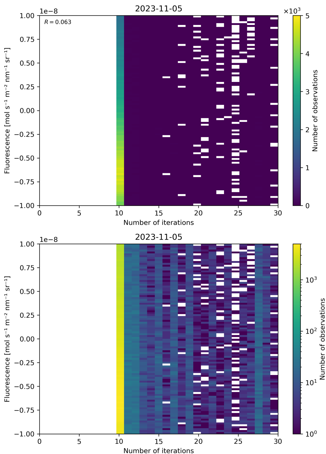
Figure 87: Scatter density plot of “Number of iterations” against “Fluorescence” for 2023-11-04 to 2023-11-06.
