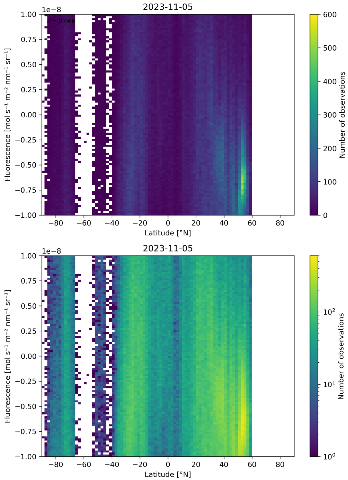
Figure 56: Scatter density plot of “Latitude” against “Fluorescence” for 2023-11-04 to 2023-11-06.
