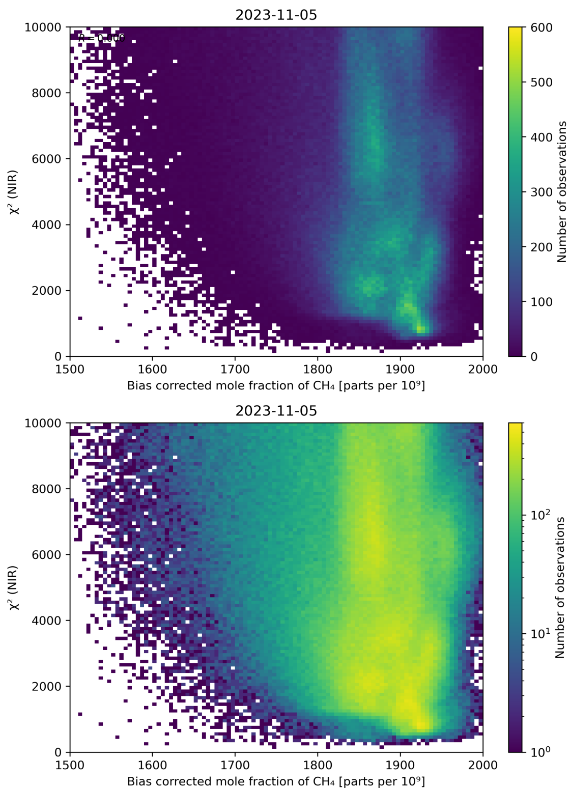
Figure 63: Scatter density plot of “Bias corrected mole fraction of CH 4 ” against “ \chi^2 (NIR)” for 2023-11-04 to 2023-11-06.
