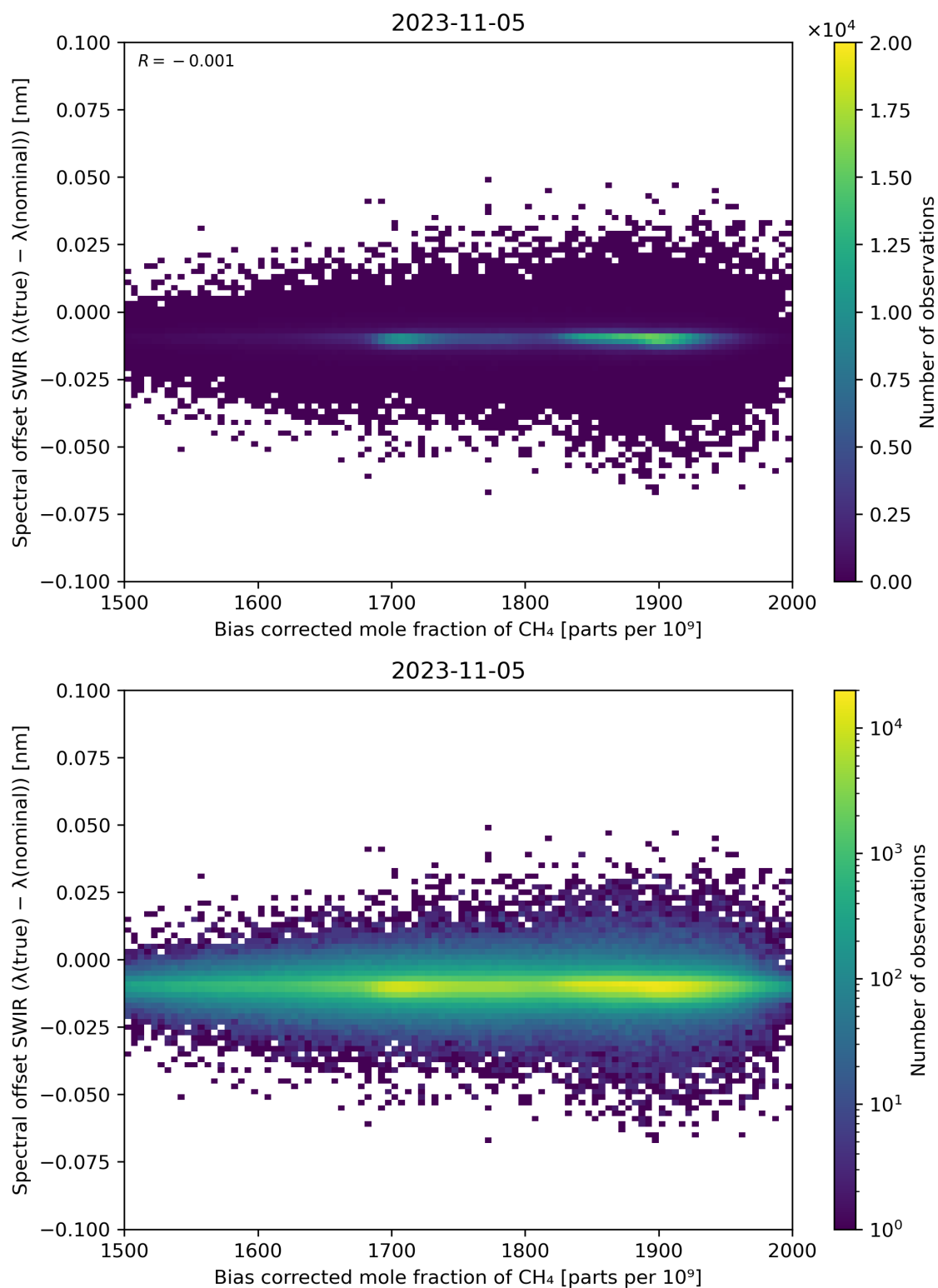
Figure 69: Scatter density plot of “Bias corrected mole fraction of \text{CH}_4 ” against “Spectral offset SWIR ( \lambda(\text{true}) - \lambda(\text{nominal}) )” for 2023-11-04 to 2023-11-06.
