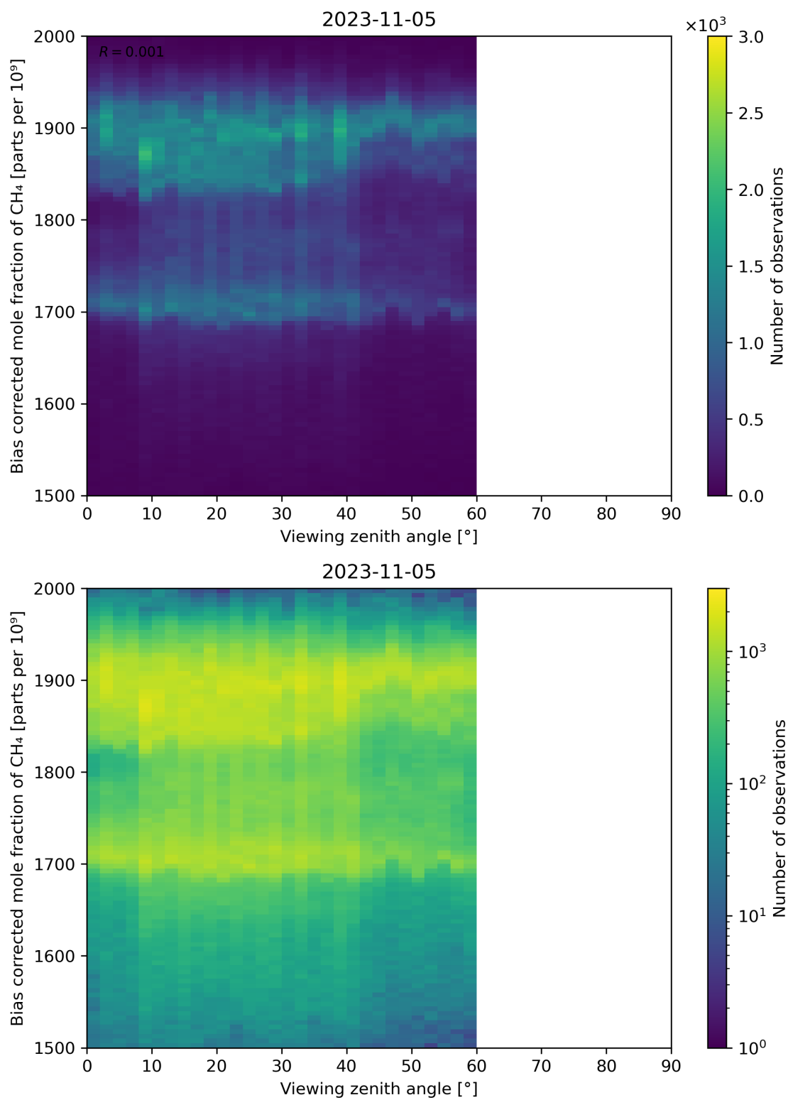
Figure 111: Scatter density plot of “Viewing zenith angle” against “Bias corrected mole fraction of CH 4 ” for 2023-11-04 to 2023-11-06.
