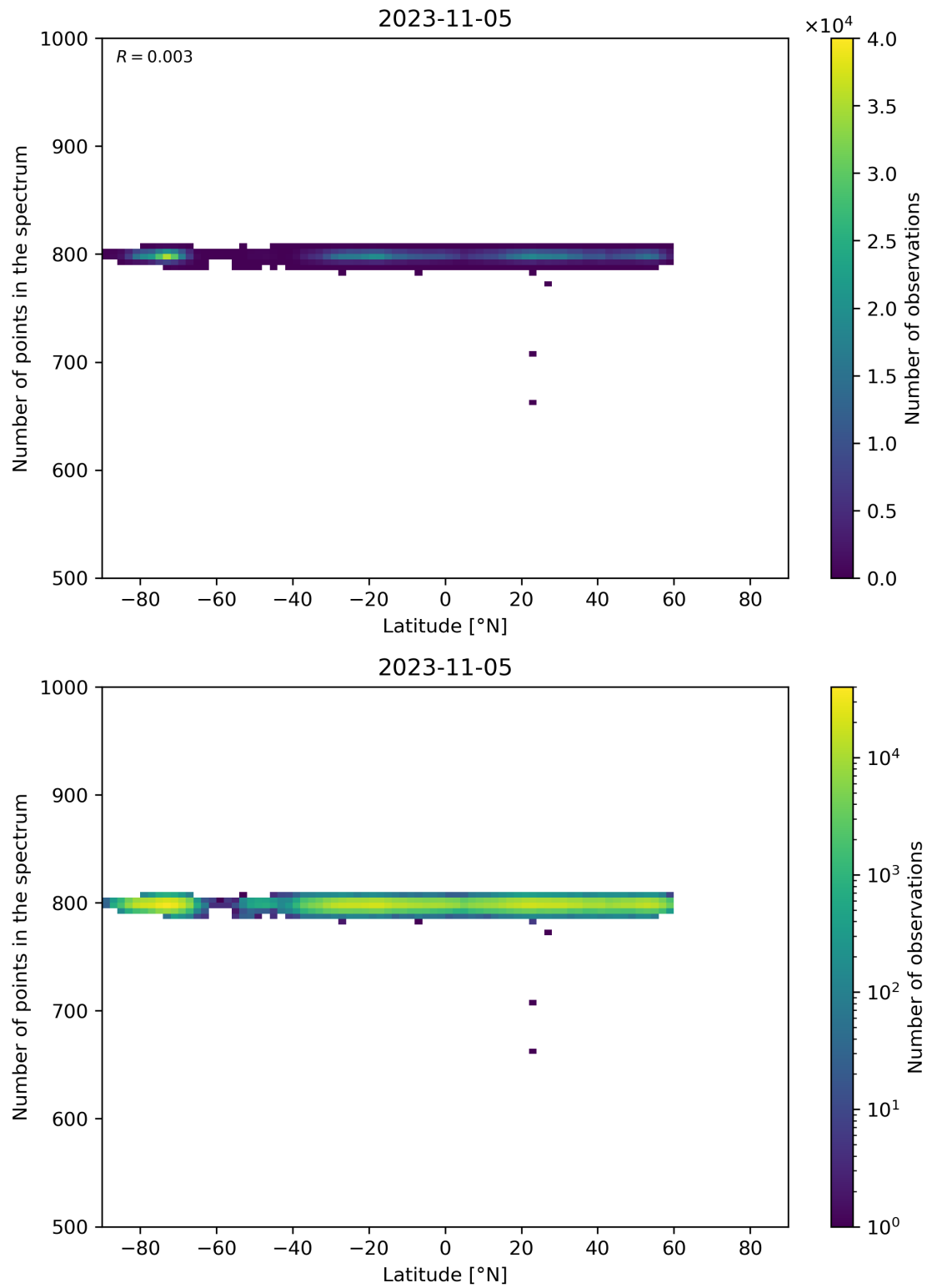
Figure 61: Scatter density plot of “Latitude” against “Number of points in the spectrum” for 2023-11-04 to 2023-11-06.
