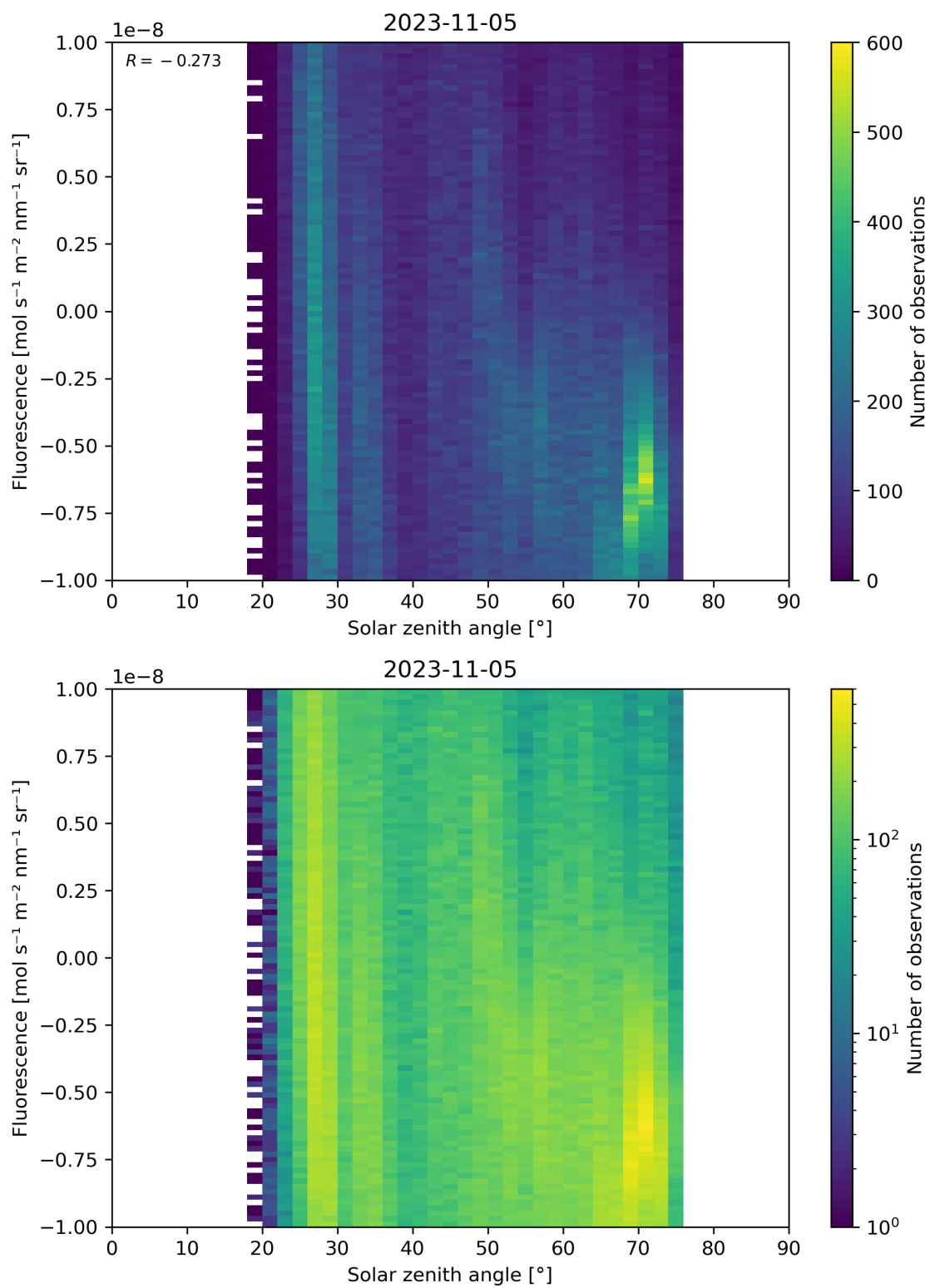
Figure 97: Scatter density plot of “Solar zenith angle” against “Fluorescence” for 2023-11-04 to 2023-11-06.
