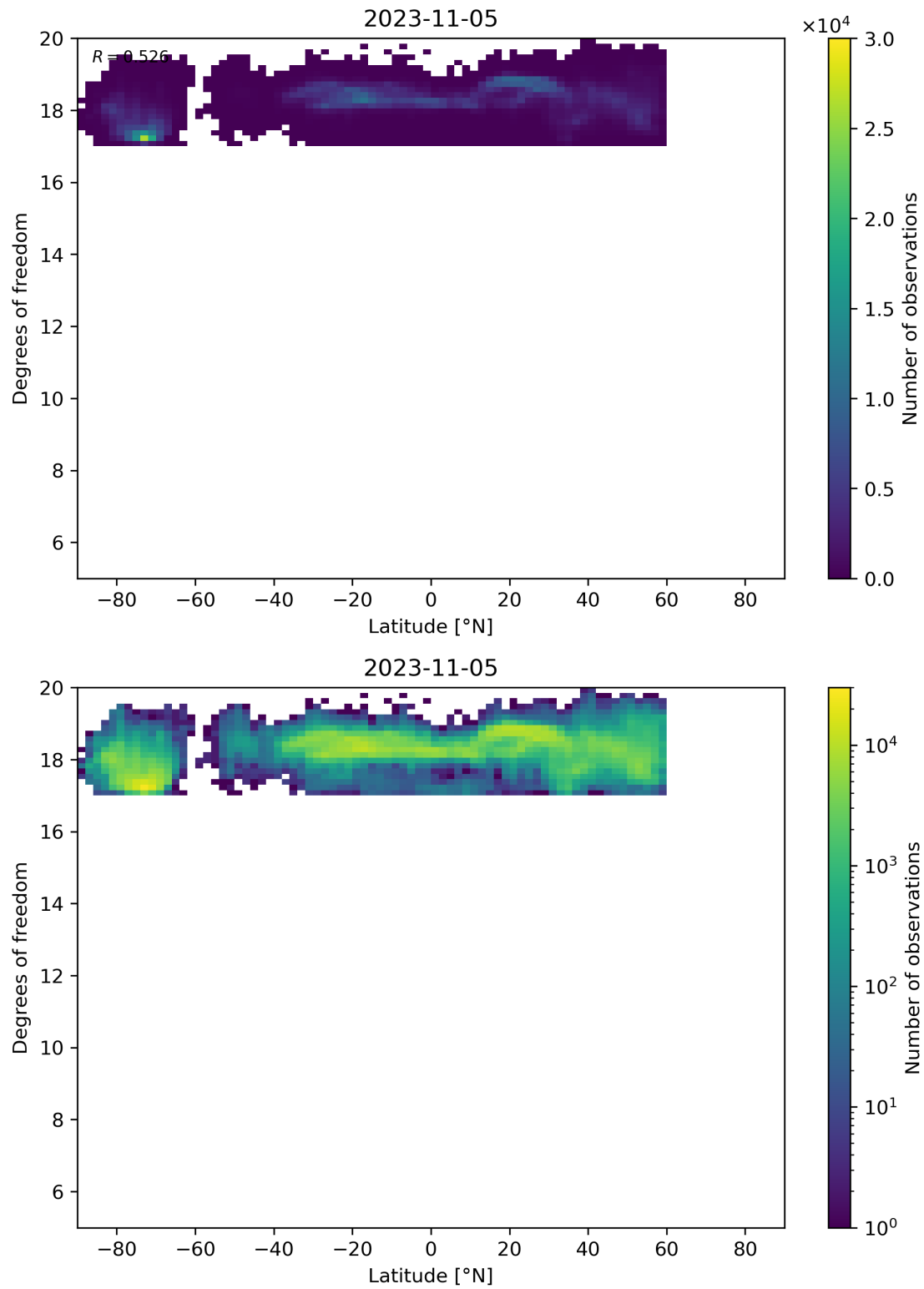
Figure 55: Scatter density plot of “Latitude” against “Degrees of freedom” for 2023-11-04 to 2023-11-06.
