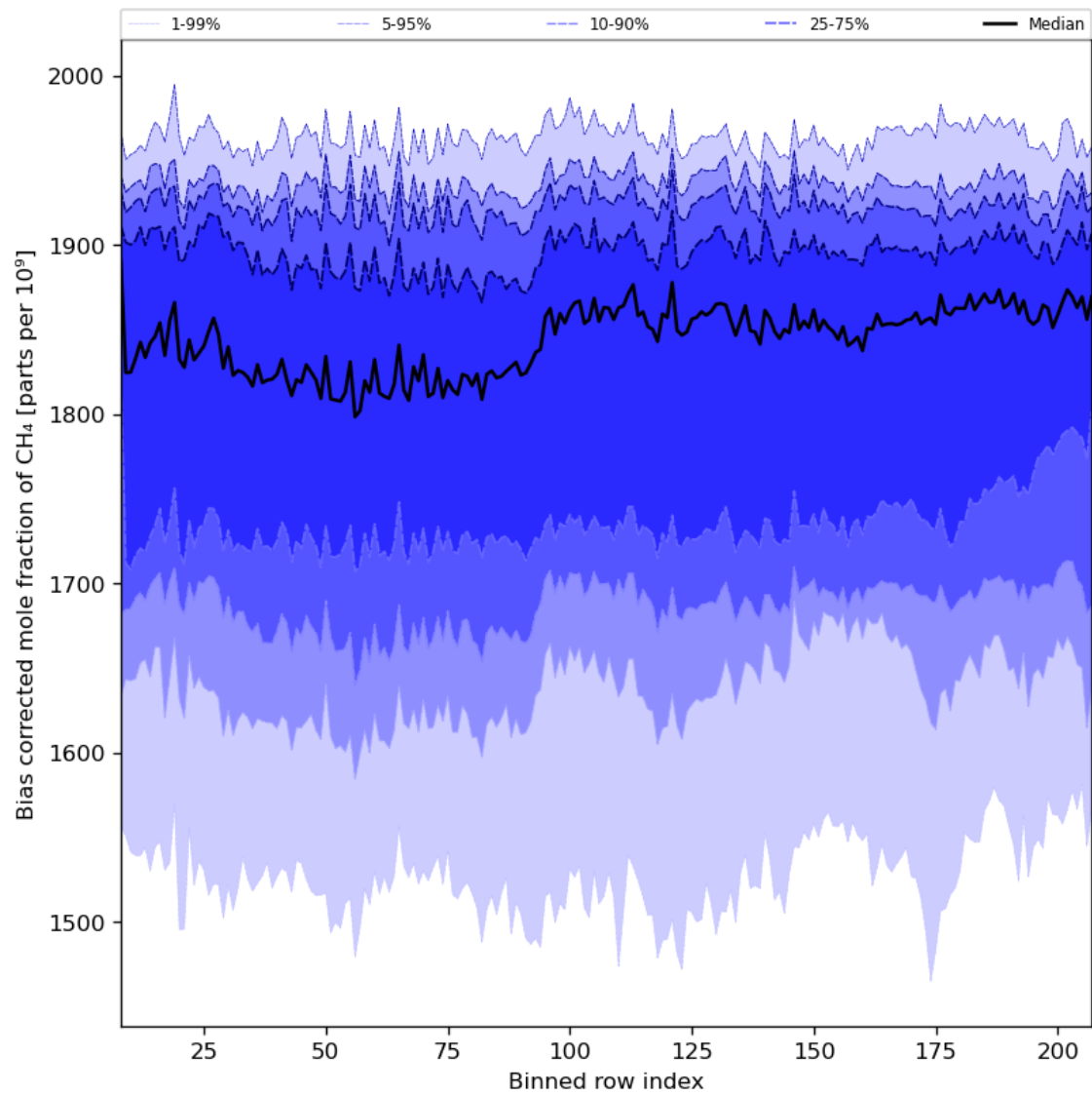
Figure 36: Along track statistics of “Bias corrected mole fraction of CH 4 ” for 2023-11-04 to 2023-11-06
