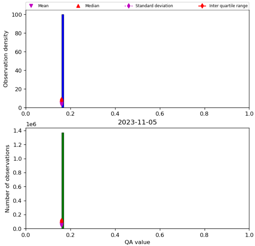
Figure 22: Histogram of “QA value” for 2023-11-04 to 2023-11-06
