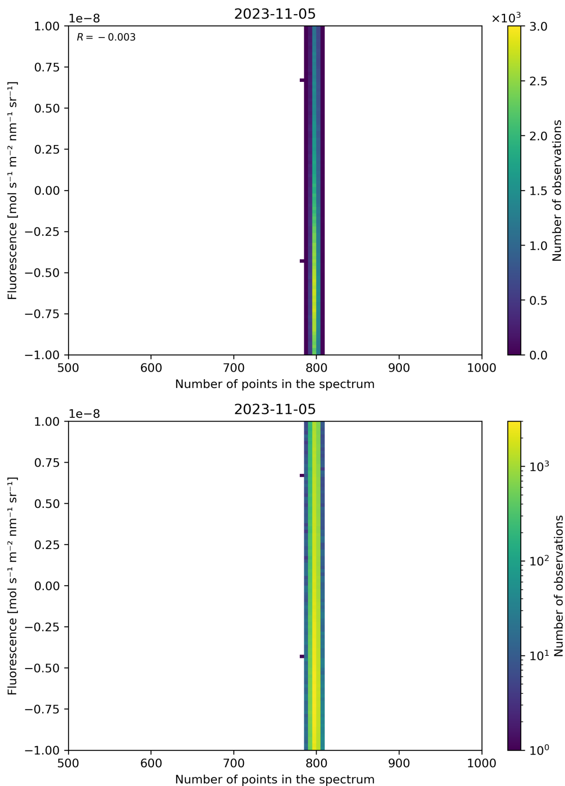
Figure 91: Scatter density plot of “Number of points in the spectrum” against “Fluorescence” for 2023-11-04 to 2023-11-06.
