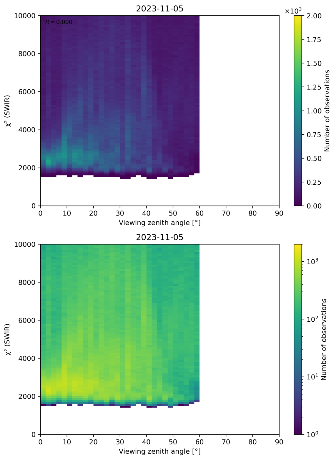
Figure 106: Scatter density plot of “Viewing zenith angle” against “ \chi^2 (SWIR)” for 2023-11-04 to 2023-11-06.
