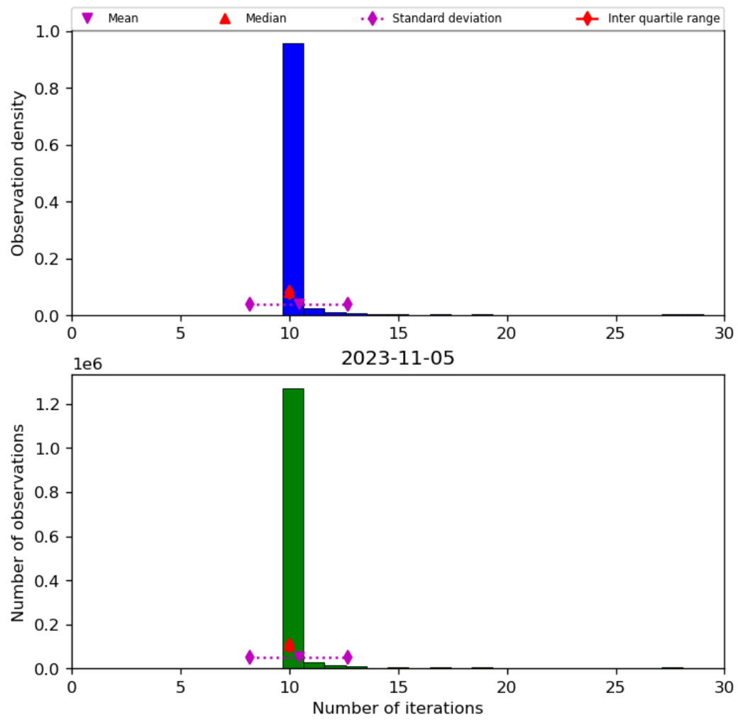
Figure 31: Histogram of “Number of iterations” for 2023-11-04 to 2023-11-06
