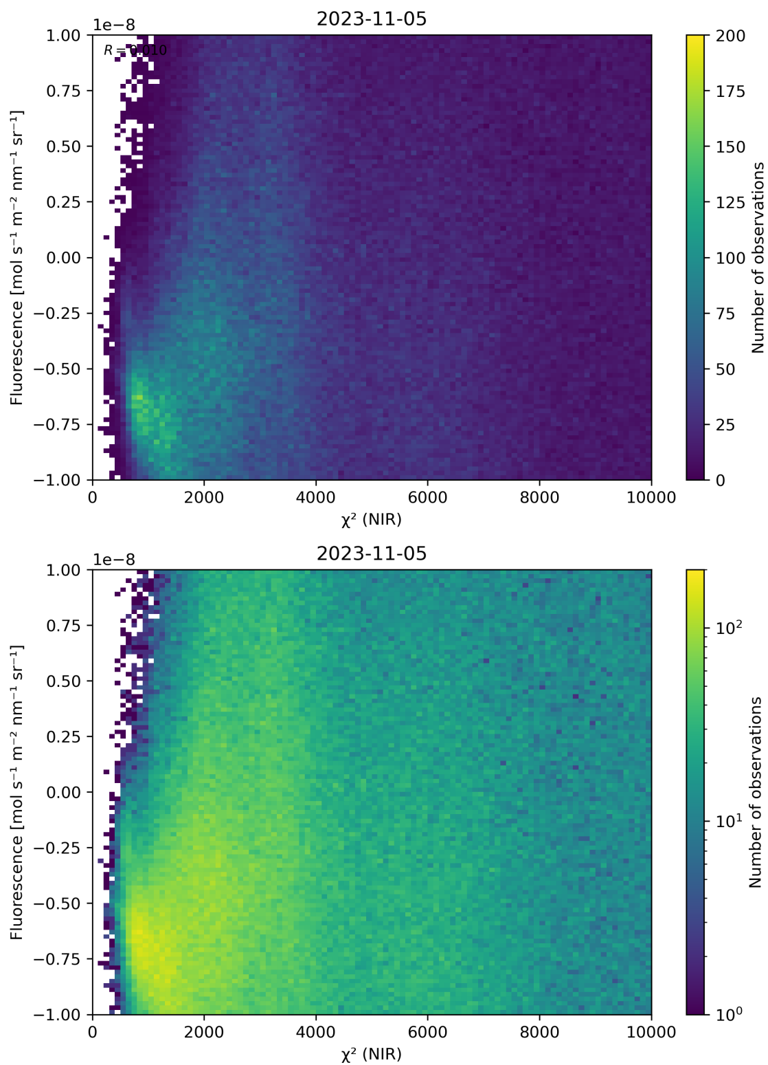
Figure 45: Scatter density plot of “ \chi^2 (NIR)” against “Fluorescence” for 2023-11-04 to 2023-11-06.
