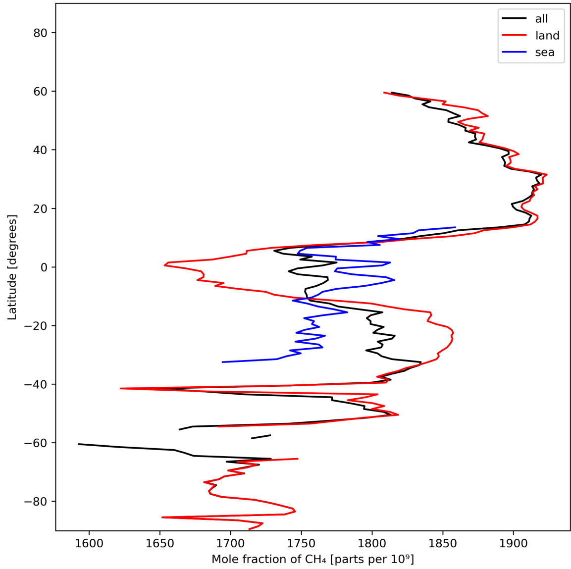
Figure 12: Zonal average of “Mole fraction of \text{CH}_4 ” for 2023-11-04 to 2023-11-06.
