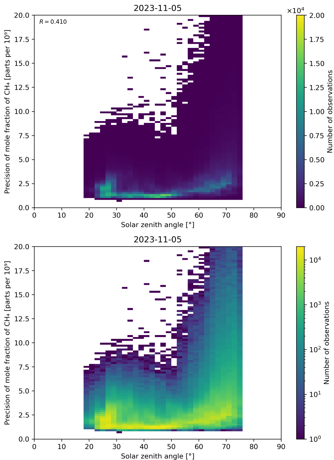
Figure 101: Scatter density plot of “Solar zenith angle” against “Precision of mole fraction of CH 4 ” for 2023-11-04 to 2023-11-06.
