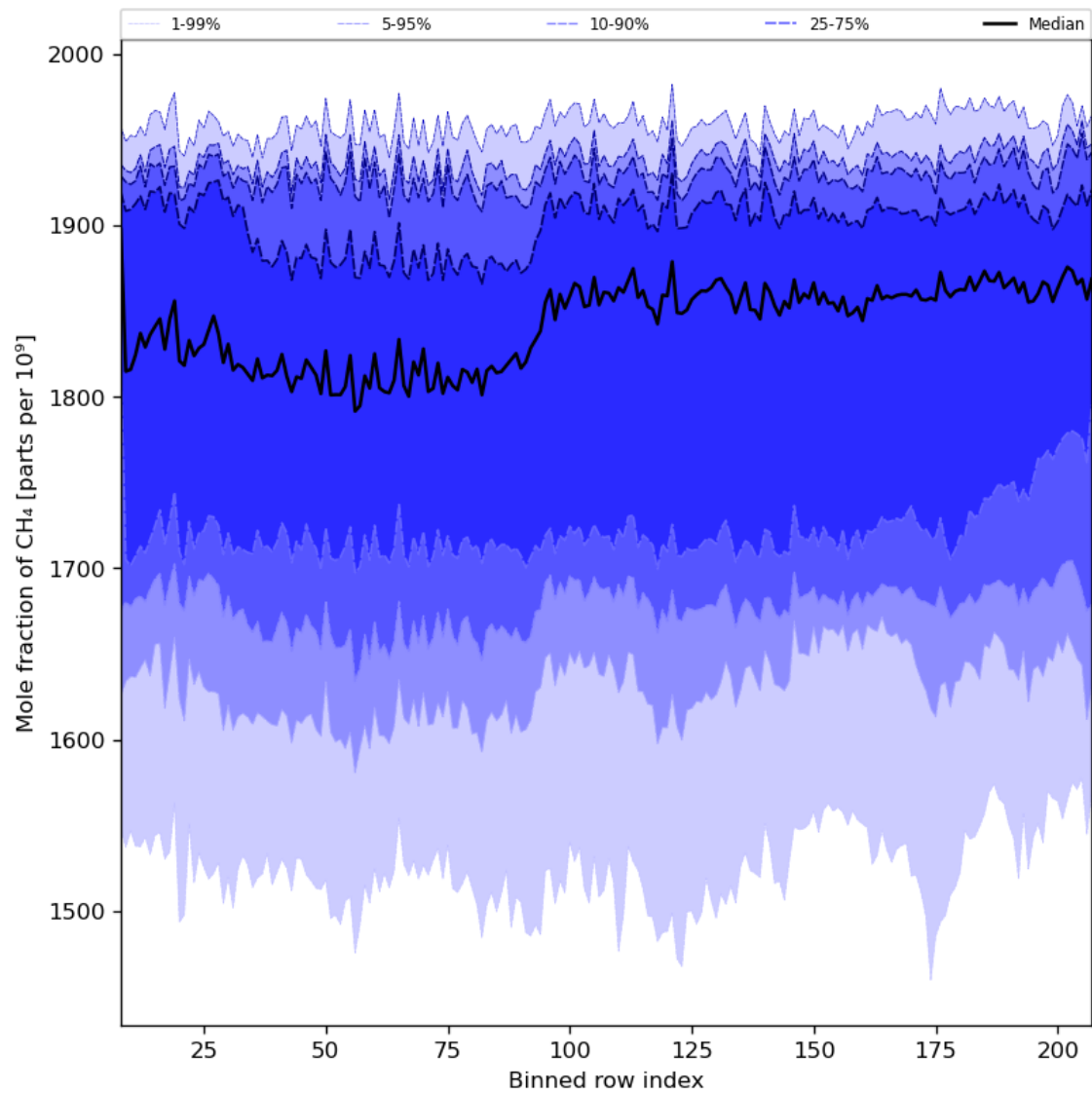
Figure 34: Along track statistics of “Mole fraction of CH 4 ” for 2023-11-04 to 2023-11-06
