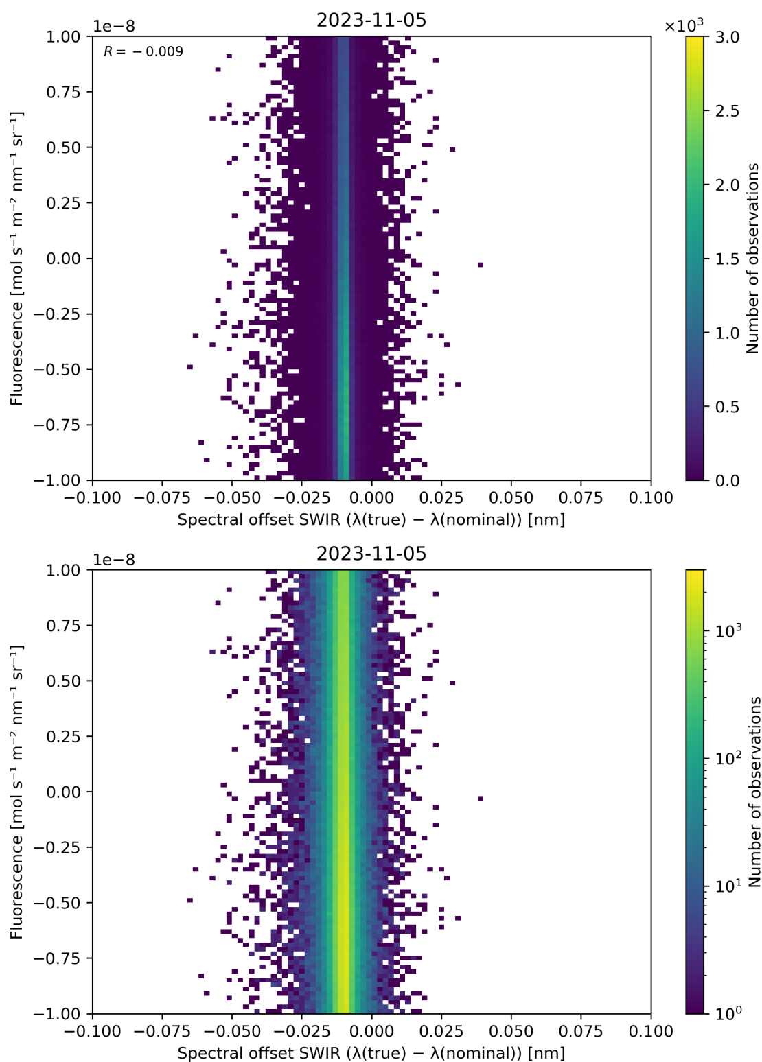
Figure 120: Scatter density plot of “Spectral offset SWIR ( \lambda(\text{true}) - \lambda(\text{nominal}) )” against “Fluorescence” for 2023-11-04 to 2023-11-06.
