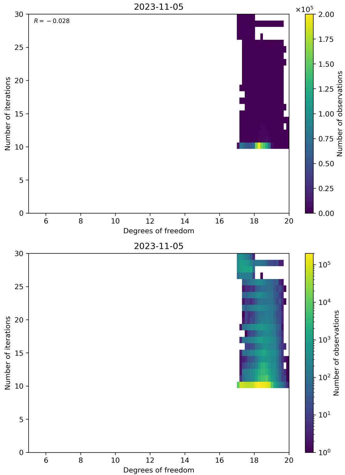
Figure 52: Scatter density plot of “Degrees of freedom” against “Number of iterations” for 2023-11-04 to 2023-11-06.
