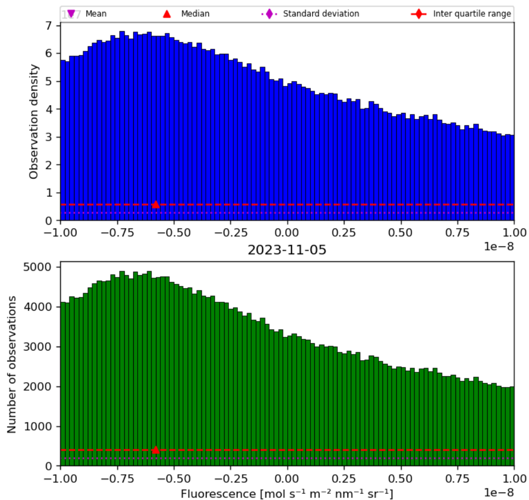
Figure 32: Histogram of “Fluorescence” for 2023-11-04 to 2023-11-06
