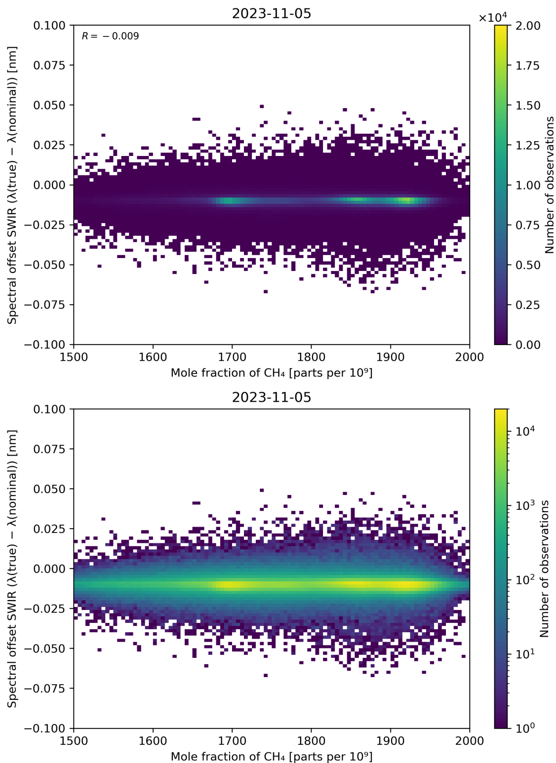
Figure 86: Scatter density plot of “Mole fraction of CH 4 ” against “Spectral offset SWIR ( \lambda(\text{true}) - \lambda(\text{nominal}) )” for 2023-11-04 to 2023-11-06.
