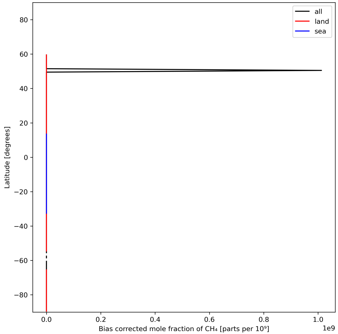
Figure 14: Zonal average of “Bias corrected mole fraction of CH 4 ” for 2023-11-04 to 2023-11-06.
