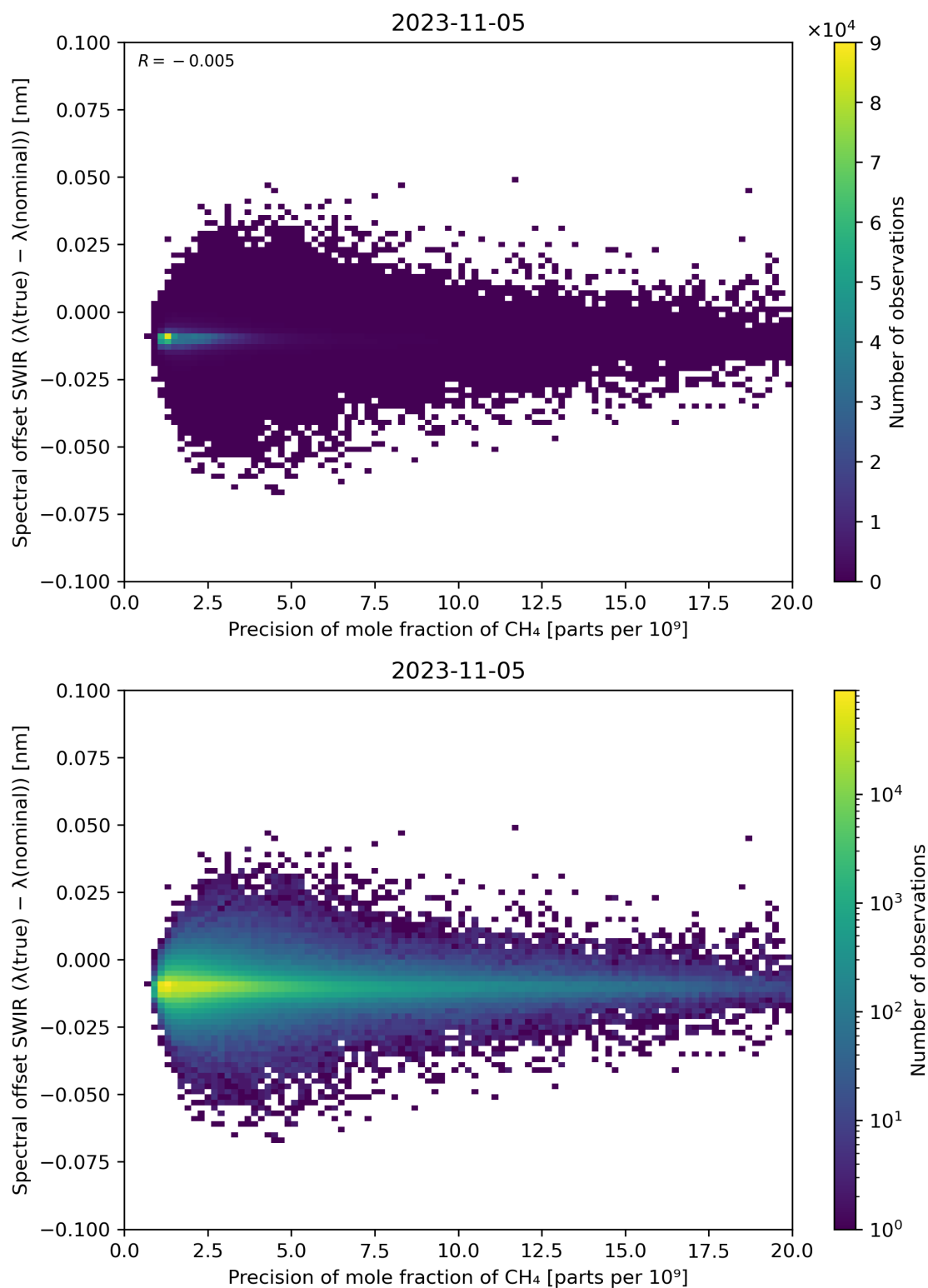
Figure 85: Scatter density plot of “Precision of mole fraction of CH 4 ” against “Spectral offset SWIR ( \lambda(\text{true}) - \lambda(\text{nominal}) )” for 2023-11-04 to 2023-11-06.
