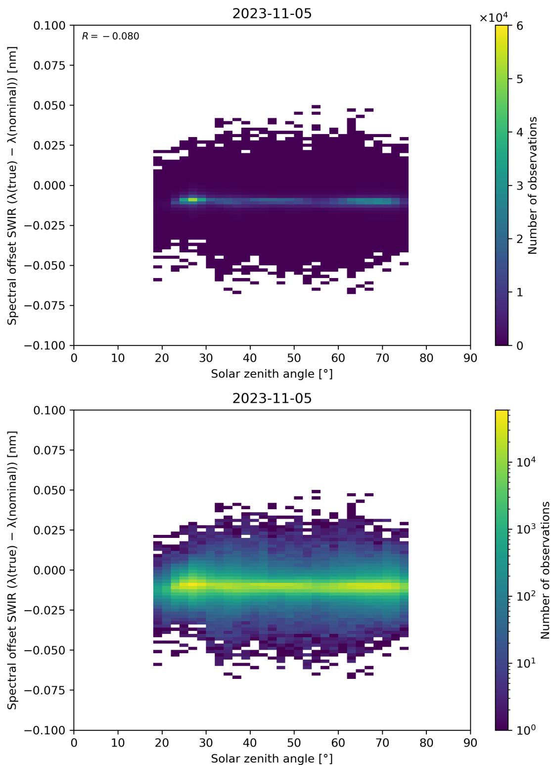
Figure 104: Scatter density plot of “Solar zenith angle” against “Spectral offset SWIR ( \lambda(\text{true}) - \lambda(\text{nominal}) )” for 2023-11-04 to 2023-11-06.
