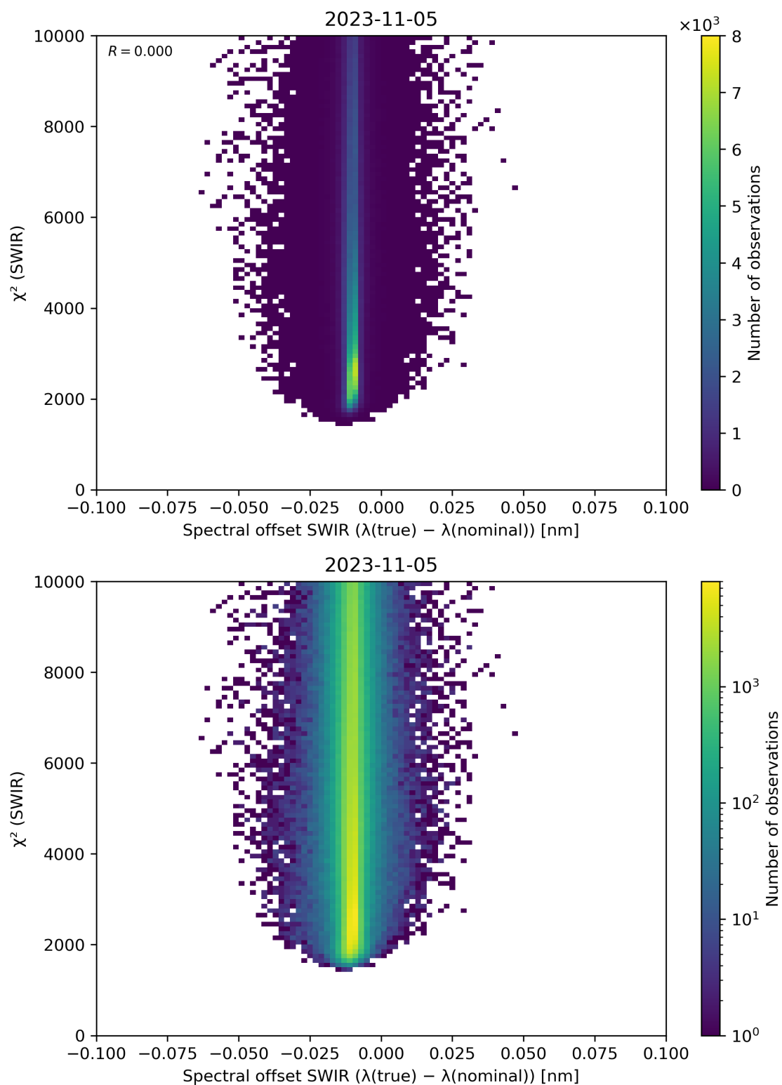
Figure 118: Scatter density plot of “Spectral offset SWIR ( \lambda(\text{true}) - \lambda(\text{nominal}) )” against “ \chi^2 (SWIR)” for 2023-11-04 to 2023-11-06.
