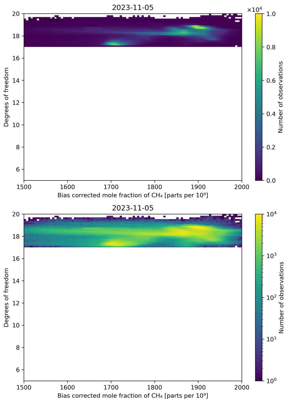
Figure 65: Scatter density plot of “Bias corrected mole fraction of CH 4 ” against “Degrees of freedom” for 2023-11-04 to 2023-11-06.
