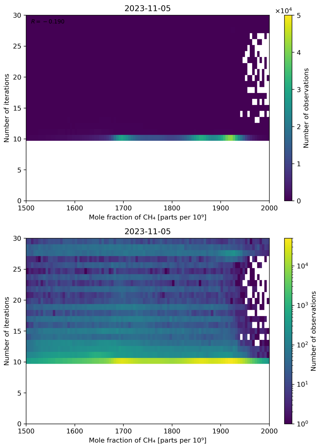
Figure 76: Scatter density plot of “Mole fraction of CH 4 ” against “Number of iterations” for 2023-11-04 to 2023-11-06.
