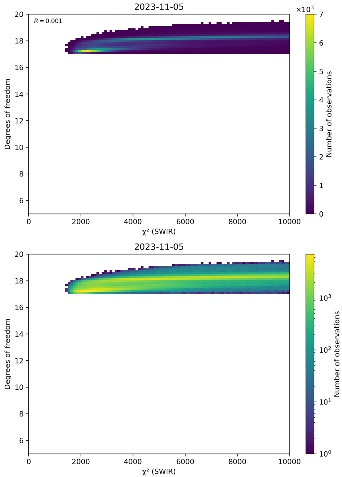
Figure 48: Scatter density plot of “ \chi^2 (SWIR)” against “Degrees of freedom” for 2023-11-04 to 2023-11-06.
