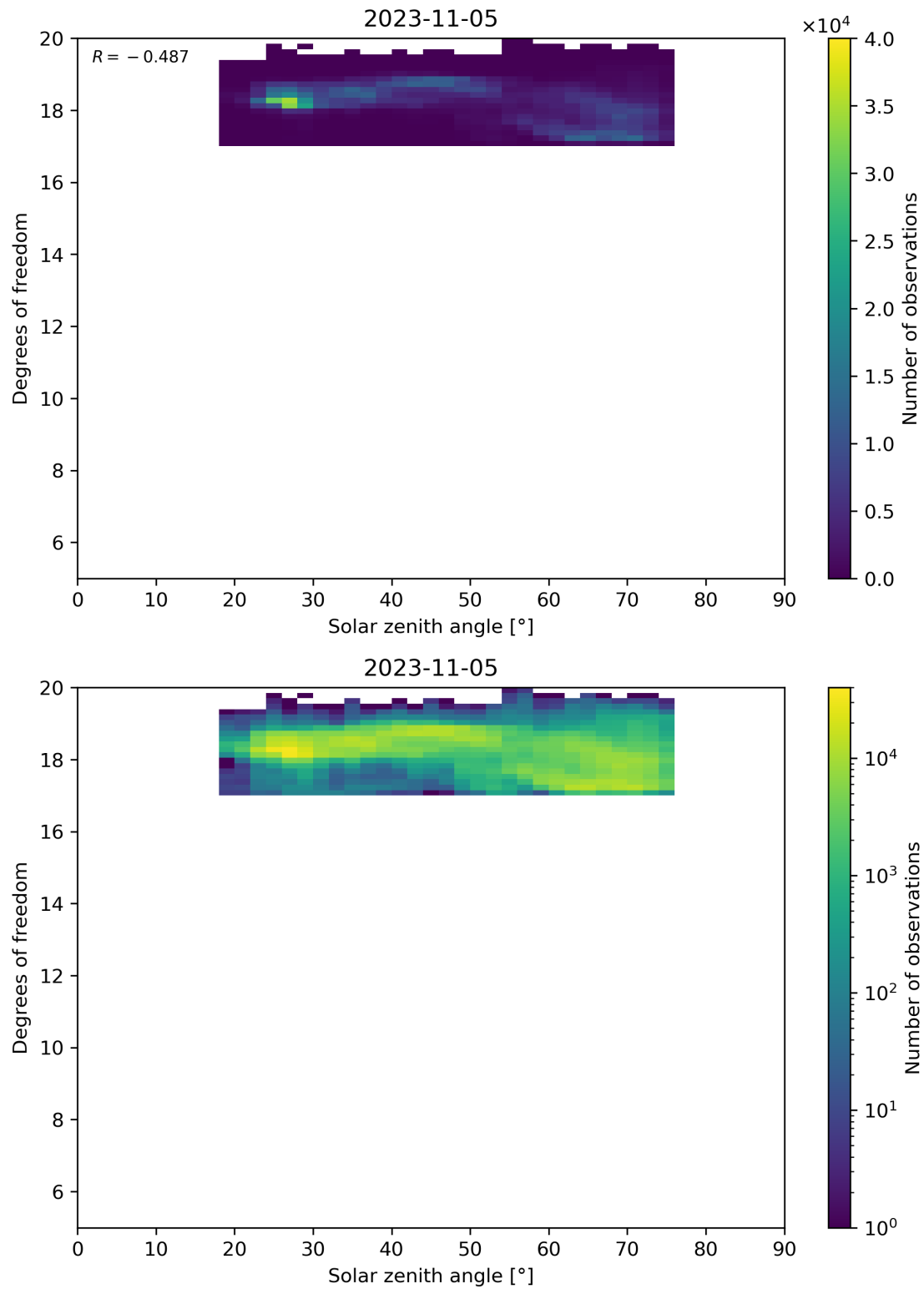
Figure 96: Scatter density plot of “Solar zenith angle” against “Degrees of freedom” for 2023-11-04 to 2023-11-06.
