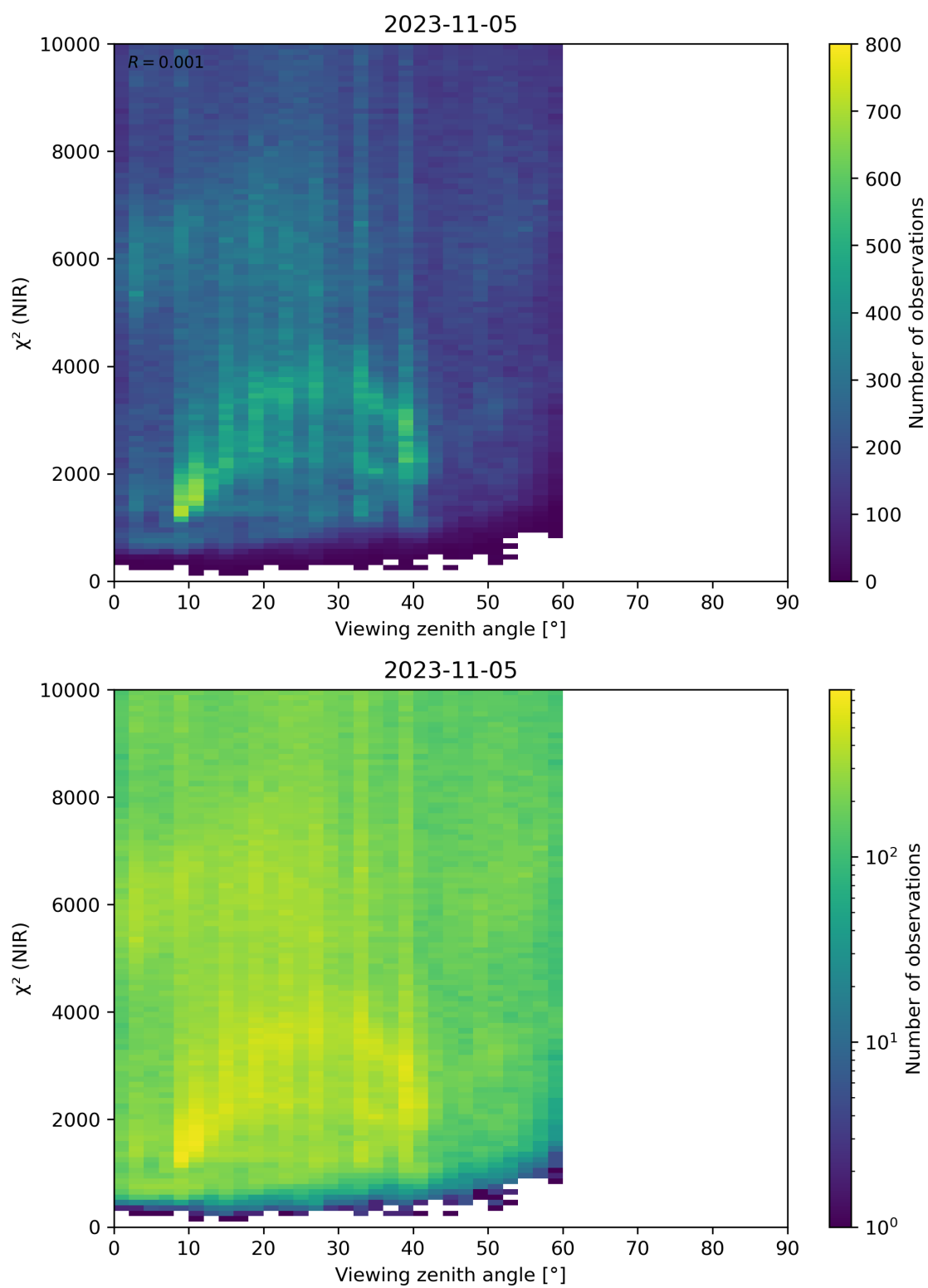
Figure 105: Scatter density plot of “Viewing zenith angle” against “ \chi^2 (NIR)” for 2023-11-04 to 2023-11-06.
