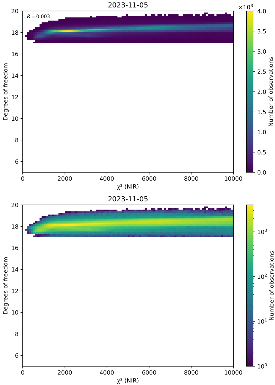
Figure 44: Scatter density plot of “ \chi^2 (NIR)” against “Degrees of freedom” for 2023-11-04 to 2023-11-06.
