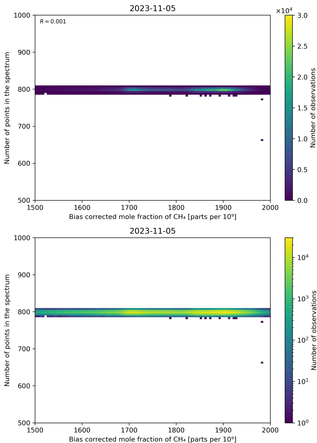
Figure 68: Scatter density plot of “Bias corrected mole fraction of CH 4 ” against “Number of points in the spectrum” for 2023-11-04 to 2023-11-06.
