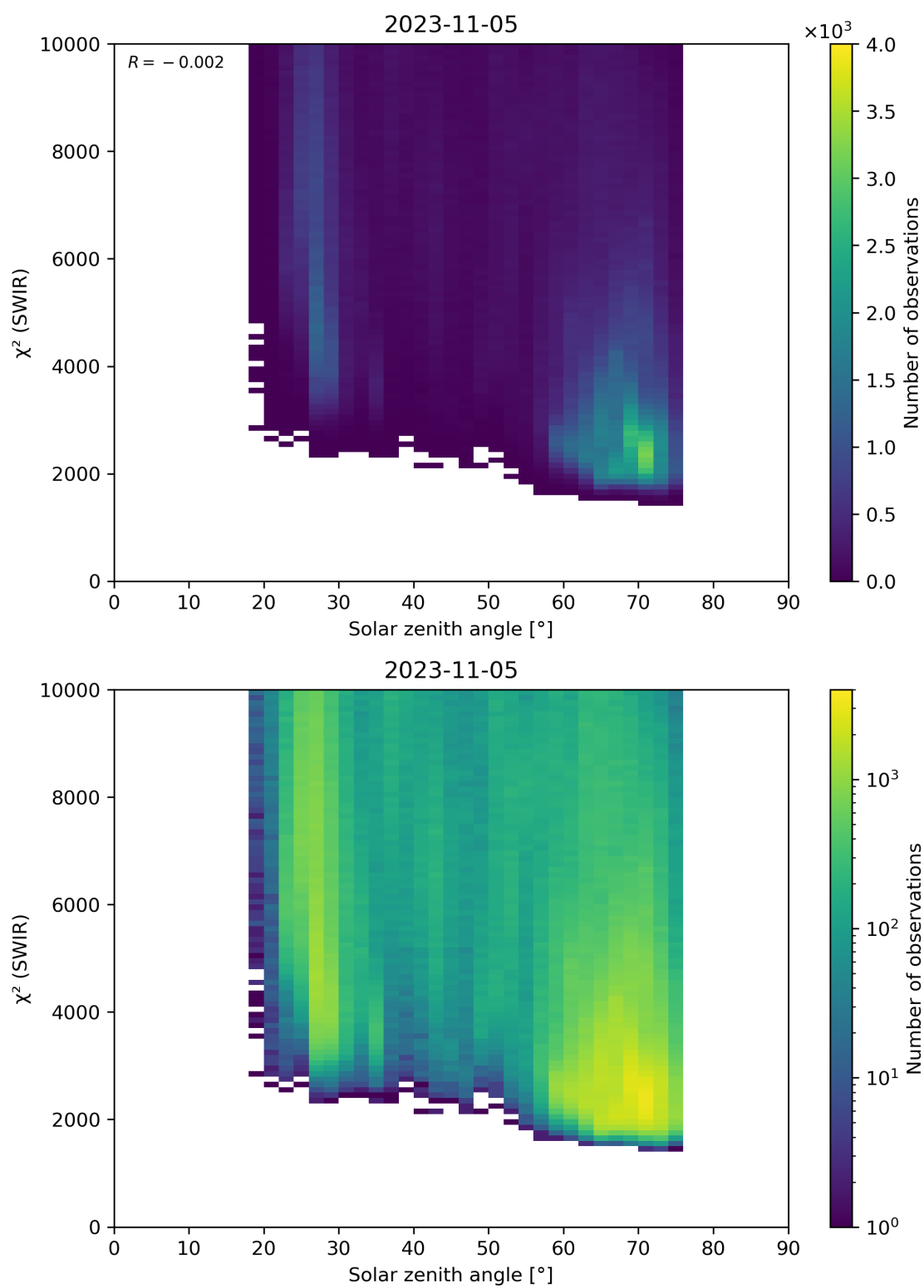
Figure 95: Scatter density plot of “Solar zenith angle” against “ \chi^2 (SWIR)” for 2023-11-04 to 2023-11-06.
