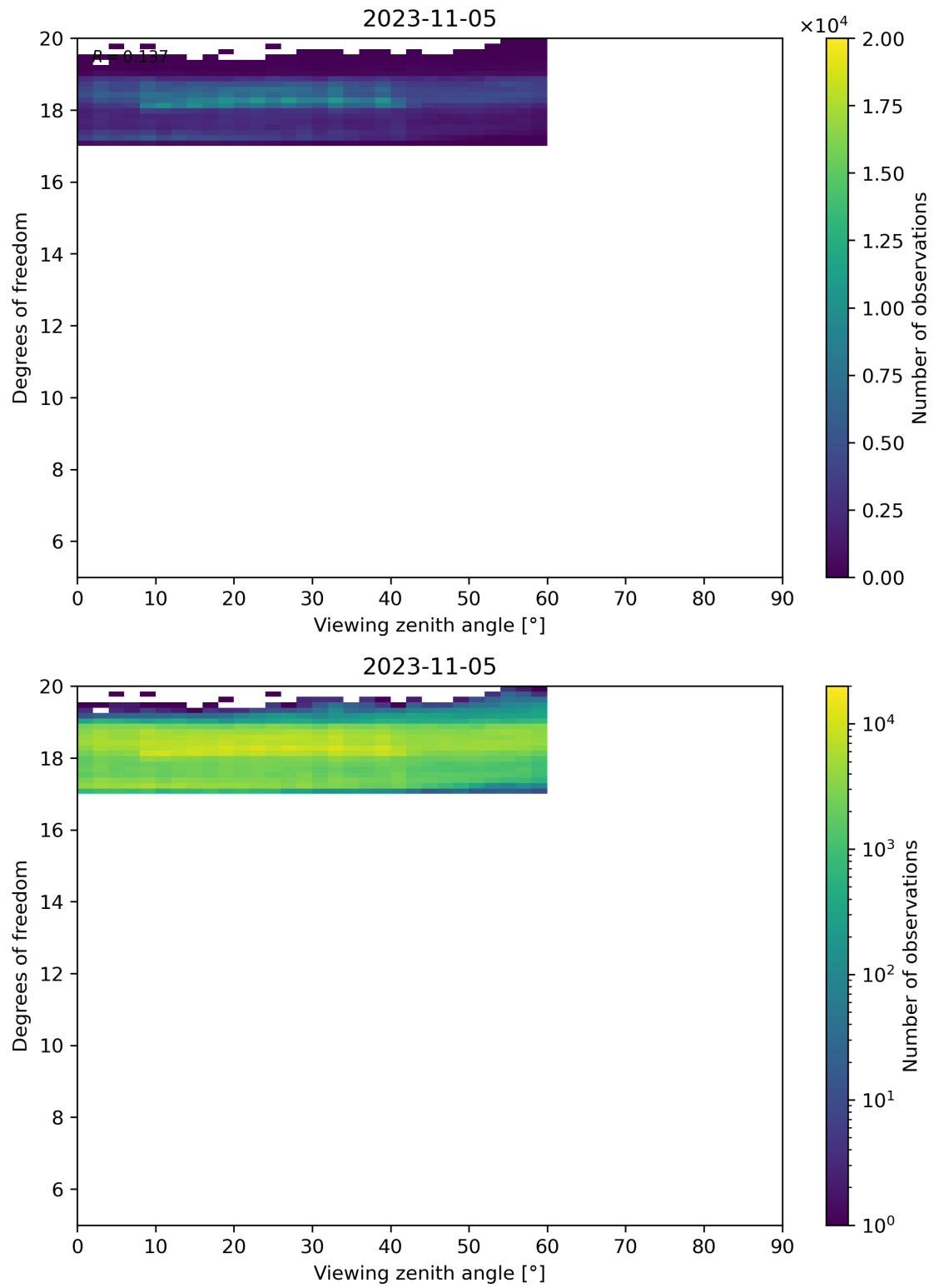
Figure 107: Scatter density plot of “Viewing zenith angle” against “Degrees of freedom” for 2023-11-04 to 2023-11-06.
