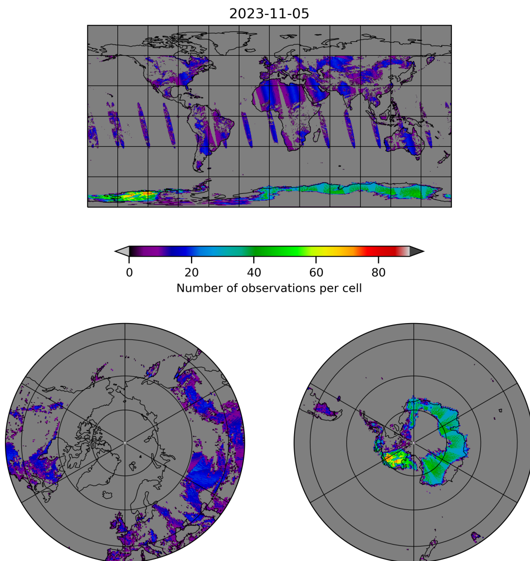
Figure 10: Map of the number of observations for 2023-11-04 to 2023-11-06
