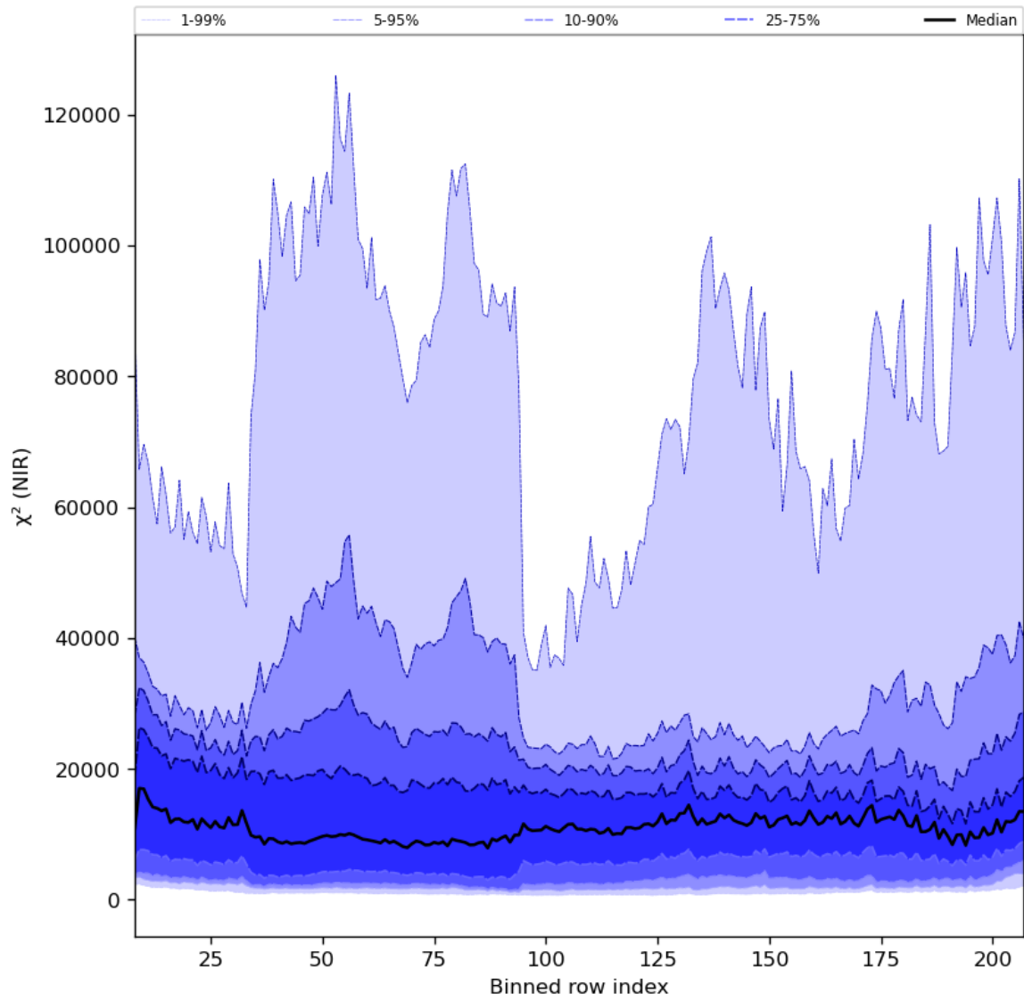
Figure 40: Along track statistics of " \chi^2 (NIR)" for 2023-11-04 to 2023-11-06
