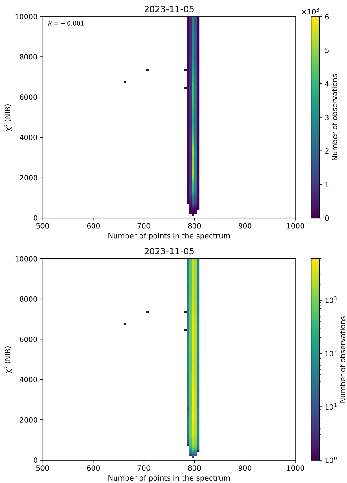
Figure 88: Scatter density plot of “Number of points in the spectrum” against “ \chi^2 (NIR)” for 2023-11-04 to 2023-11-06.
