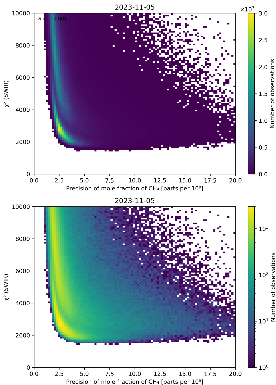
Figure 79: Scatter density plot of “Precision of mole fraction of CH 4 ” against “ \chi^2 (SWIR)” for 2023-11-04 to 2023-11-06.
