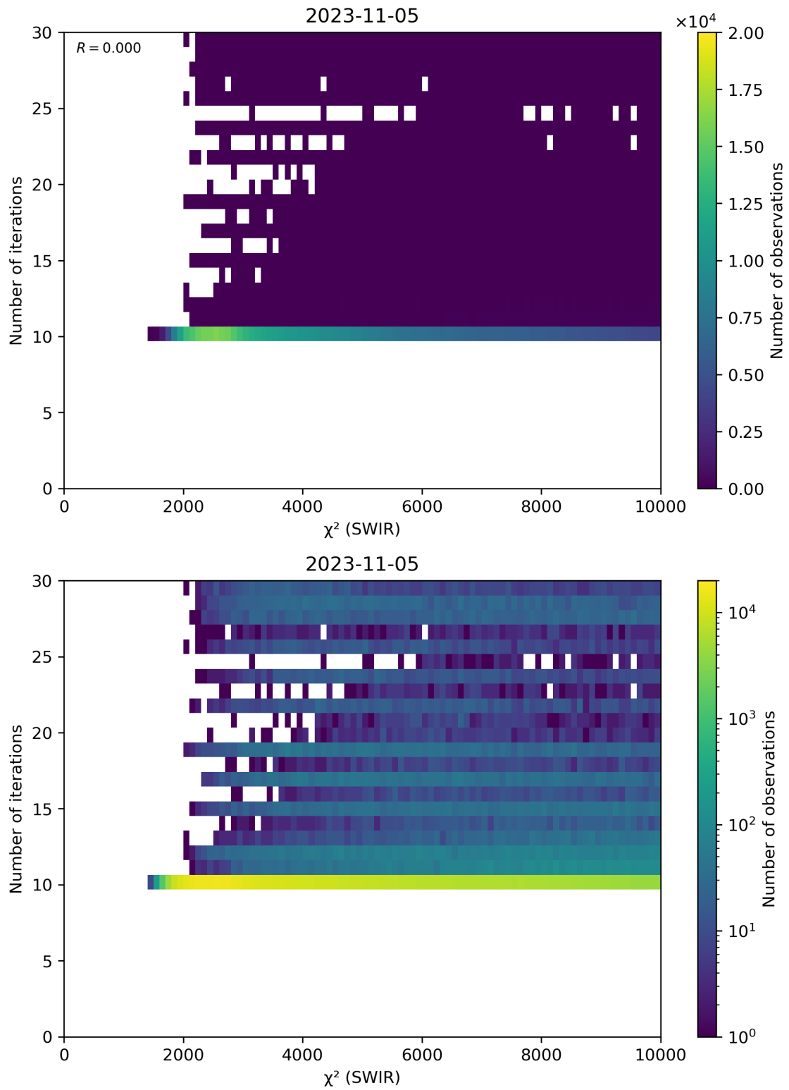
Figure 50: Scatter density plot of “ \chi^2 (SWIR)” against “Number of iterations” for 2023-11-04 to 2023-11-06.
