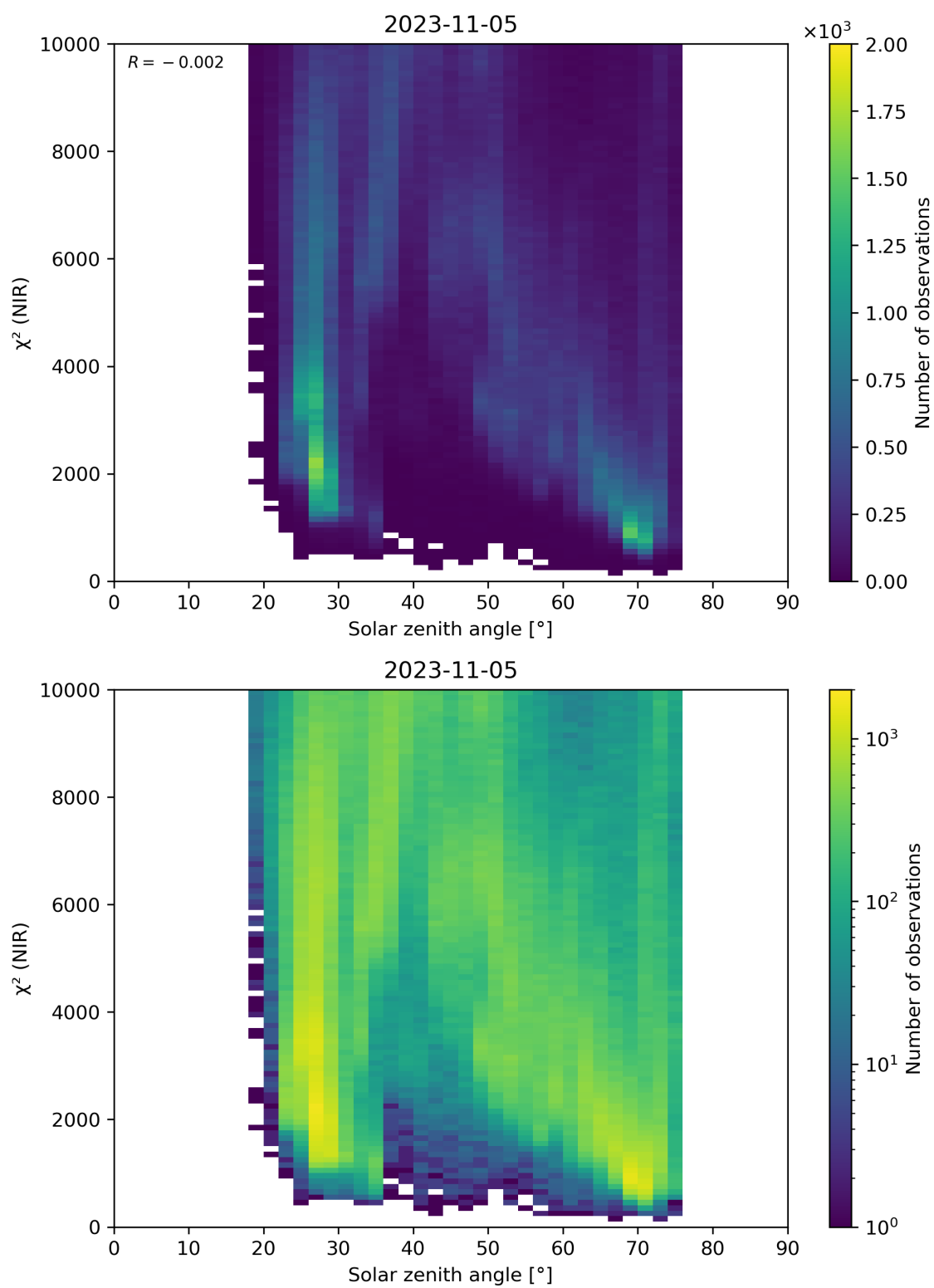
Figure 94: Scatter density plot of “Solar zenith angle” against “ \chi^2 (NIR)” for 2023-11-04 to 2023-11-06.
