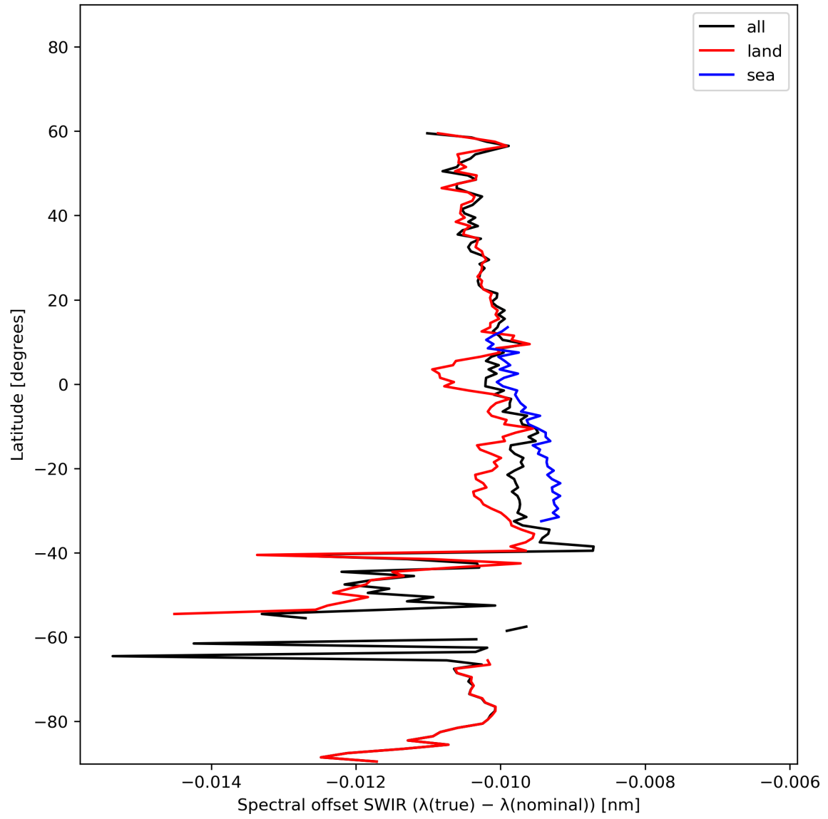
Figure 16: Zonal average of “Spectral offset SWIR ( \lambda(\text{true}) - \lambda(\text{nominal}) )” for 2023-11-04 to 2023-11-06.
