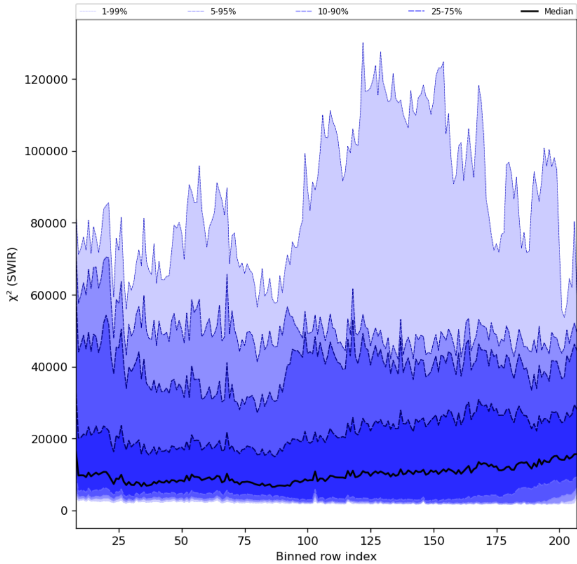
Figure 39: Along track statistics of “ \chi^2 (SWIR)” for 2023-11-04 to 2023-11-06
