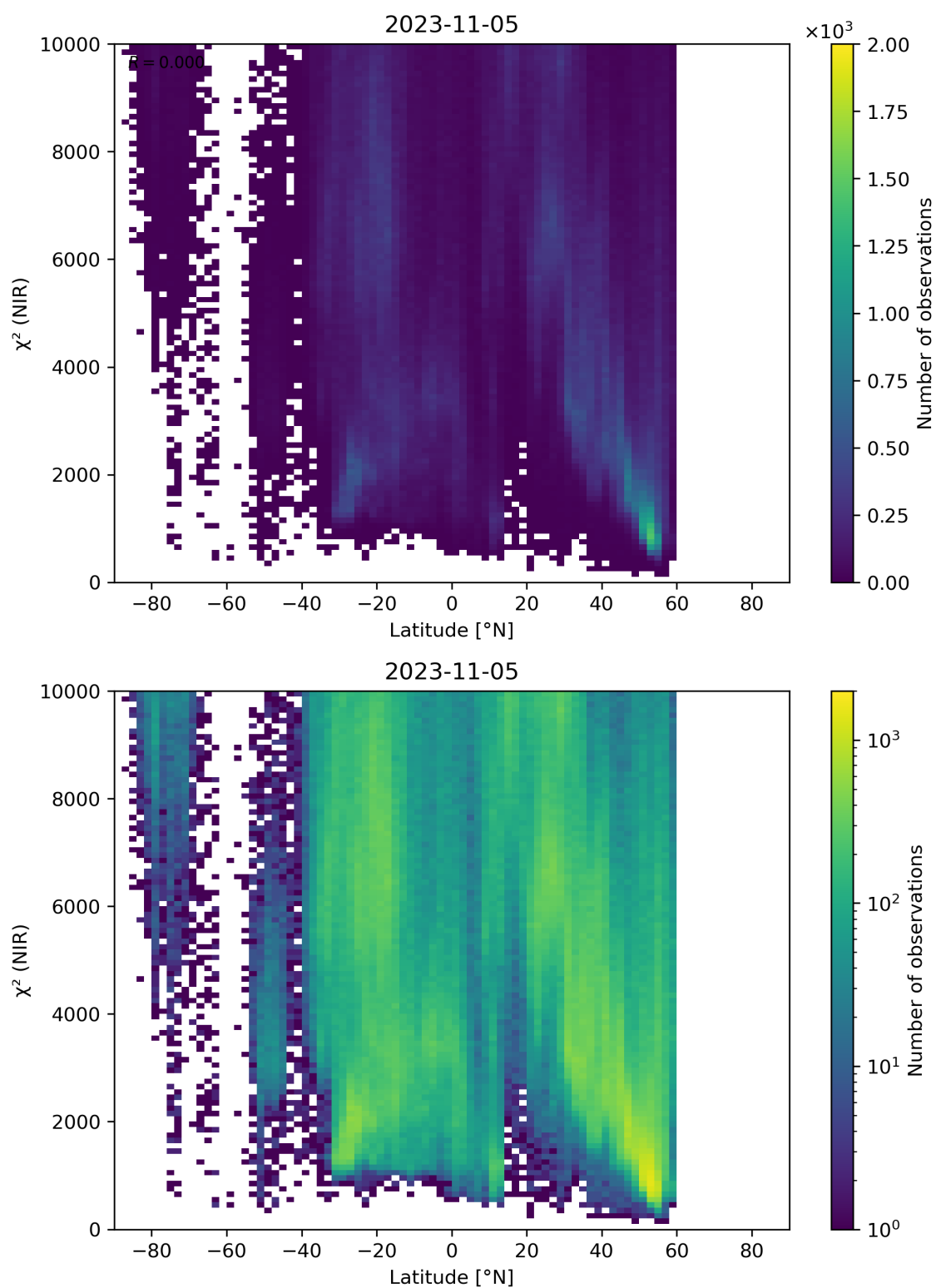
Figure 53: Scatter density plot of “Latitude” against “ \chi^2 (NIR)” for 2023-11-04 to 2023-11-06.
