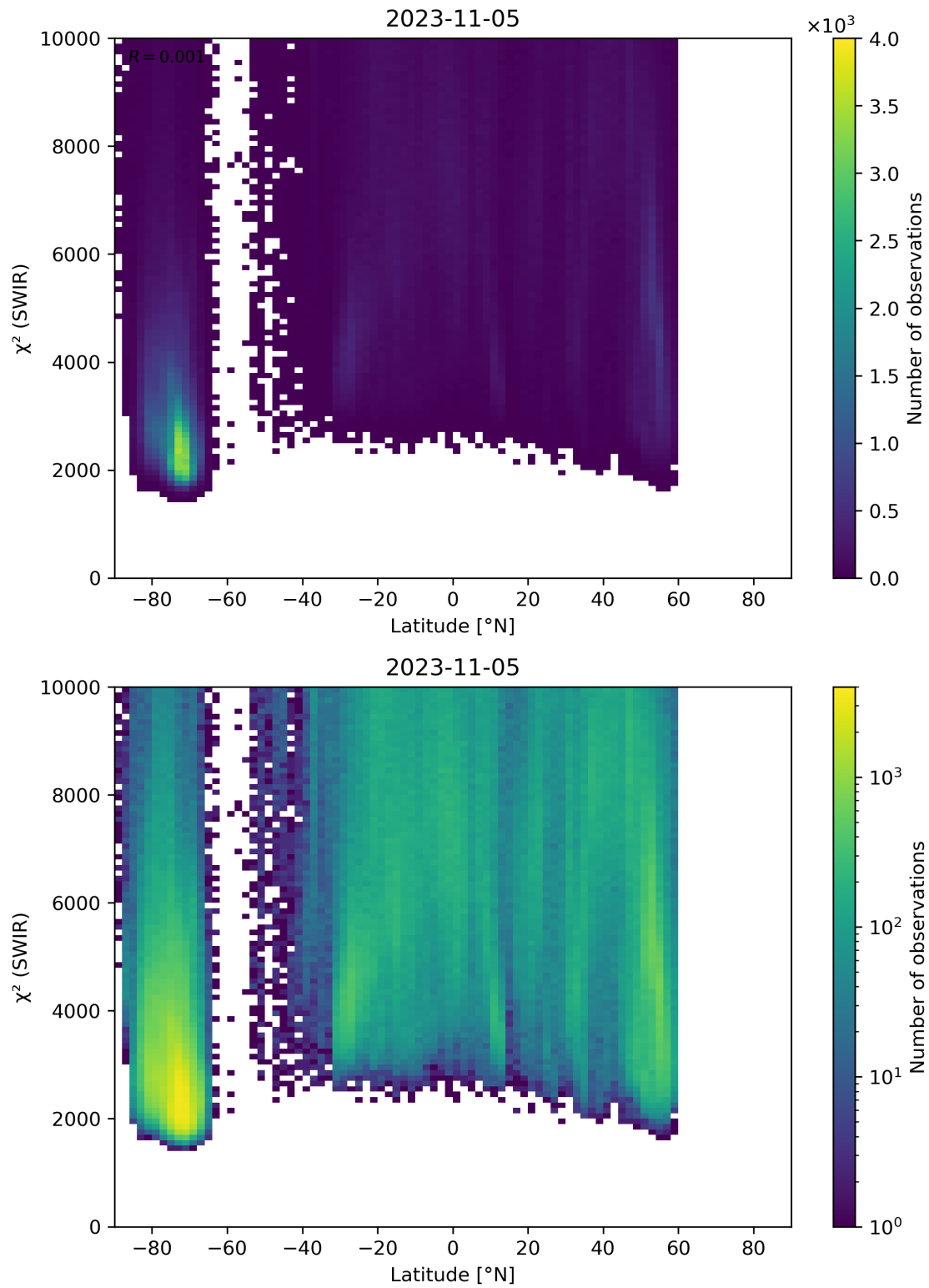
Figure 54: Scatter density plot of “Latitude” against “ \chi^2 (SWIR)” for 2023-11-04 to 2023-11-06.
