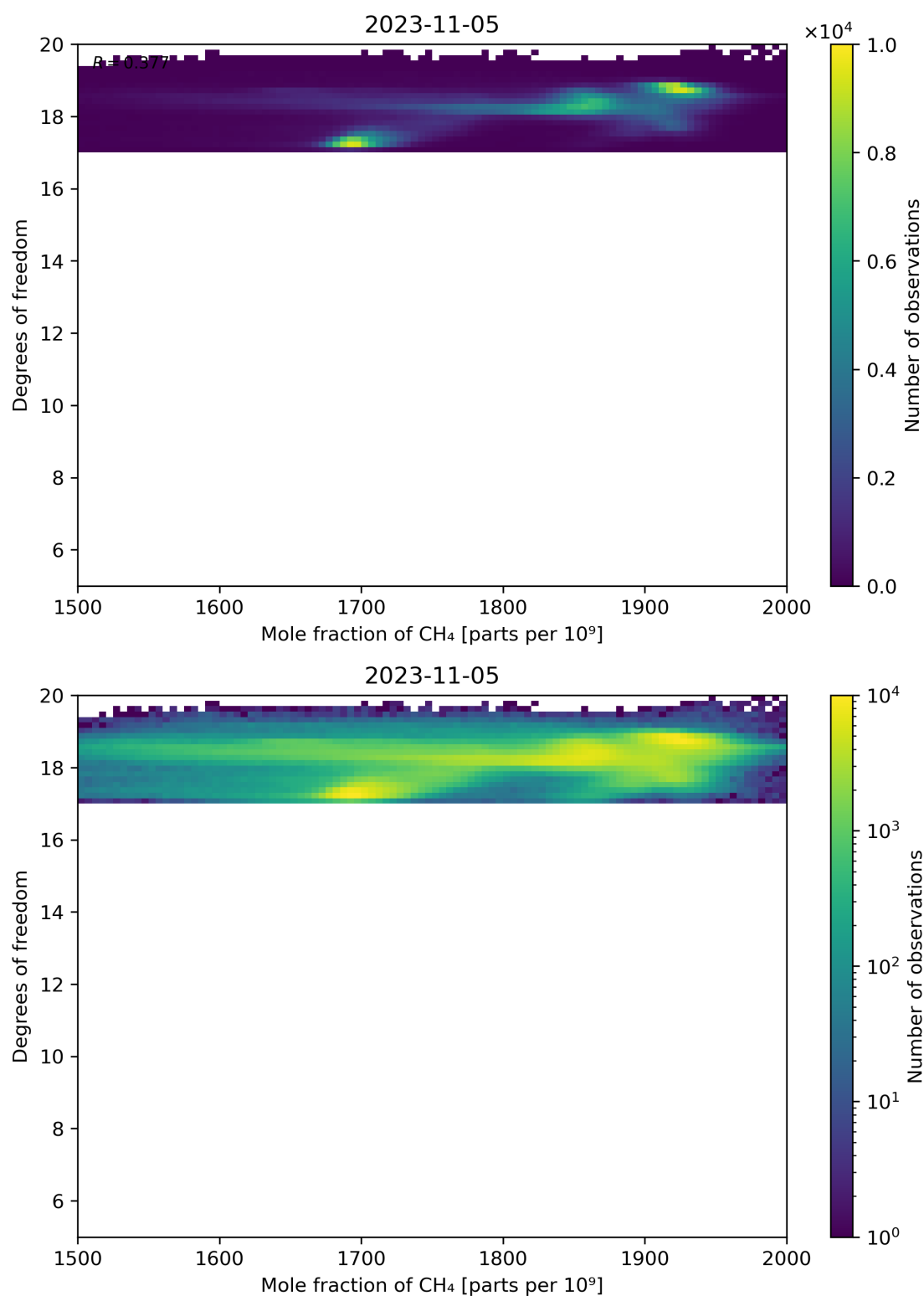
Figure 72: Scatter density plot of “Mole fraction of CH 4 ” against “Degrees of freedom” for 2023-11-04 to 2023-11-06.
