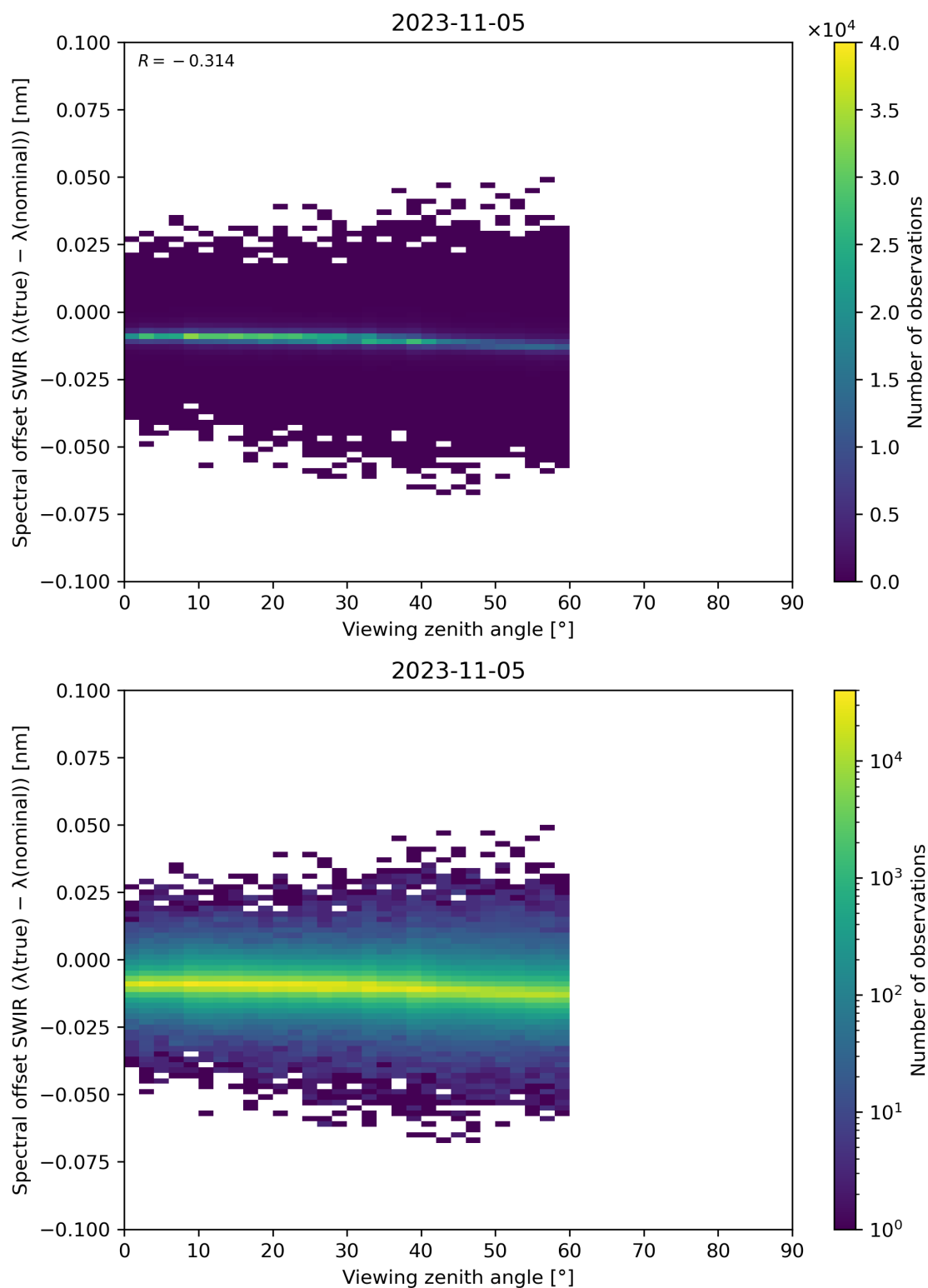
Figure 116: Scatter density plot of “Viewing zenith angle” against “Spectral offset SWIR ( \lambda(\text{true}) - \lambda(\text{nominal}) )” for 2023-11-04 to 2023-11-06.
