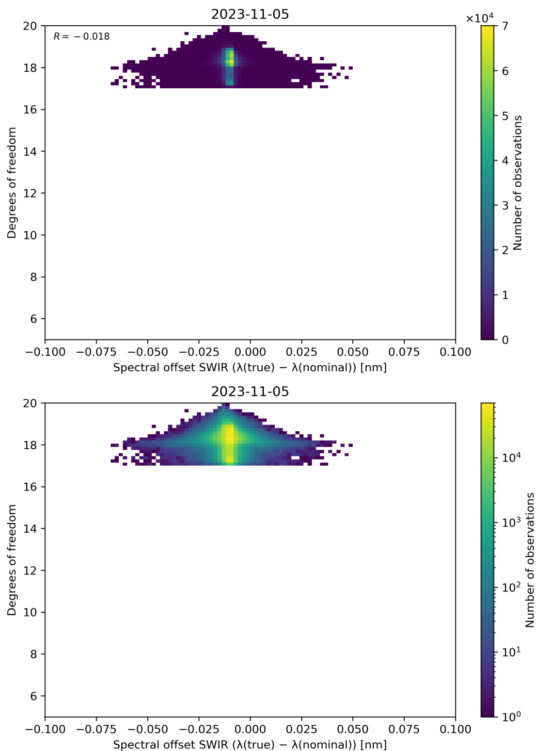
Figure 119: Scatter density plot of “Spectral offset SWIR ( \lambda(\text{true}) - \lambda(\text{nominal}) )” against “Degrees of freedom” for 2023-11-04 to 2023-11-06.
