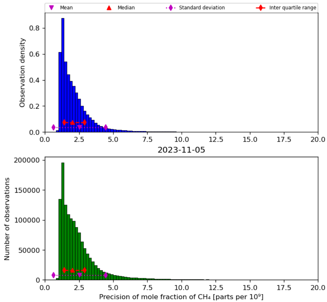
Figure 24: Histogram of “Precision of mole fraction of CH 4 ” for 2023-11-04 to 2023-11-06
