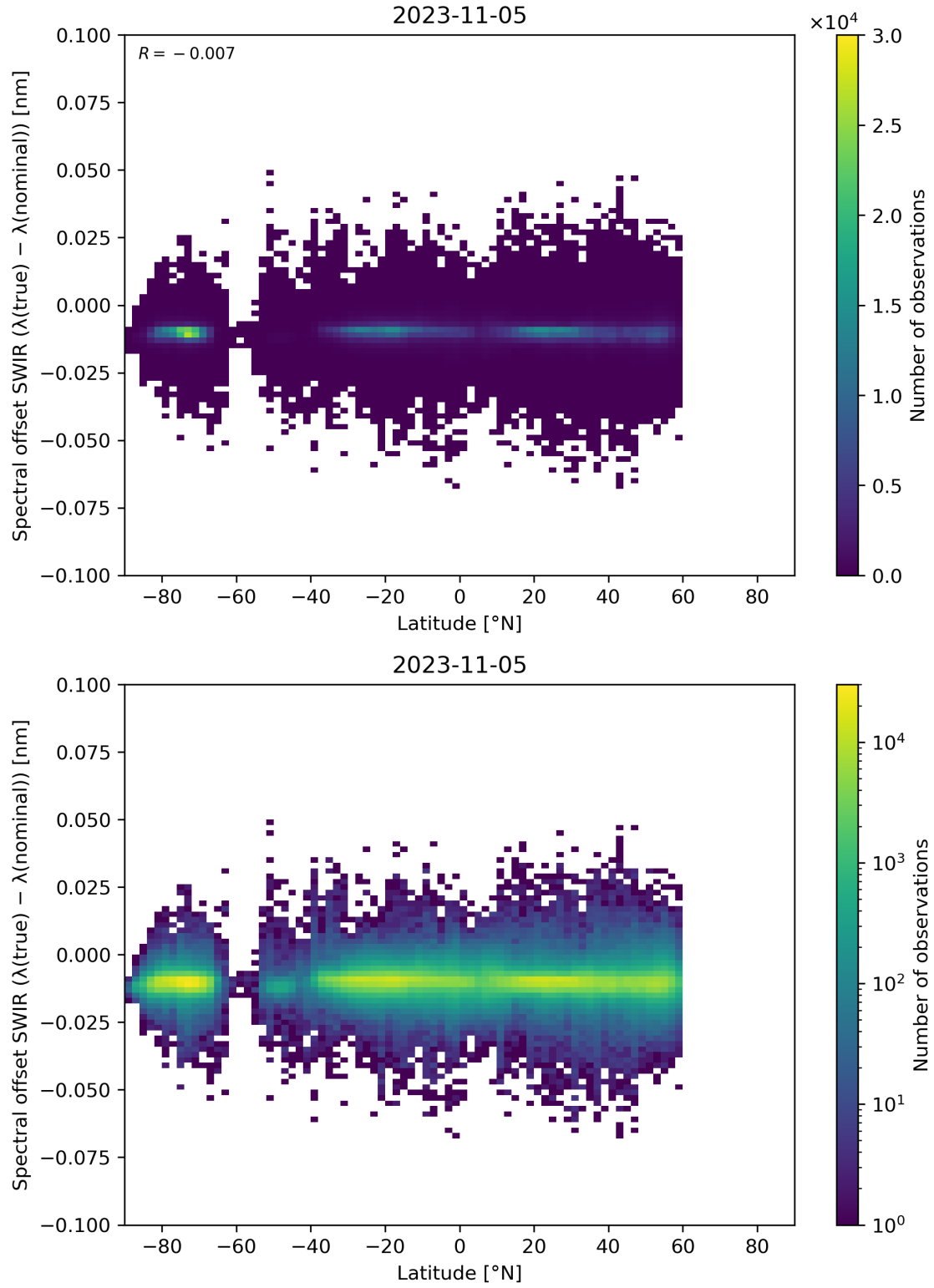
Figure 62: Scatter density plot of “Latitude” against “Spectral offset SWIR ( \lambda(\text{true}) - \lambda(\text{nominal}) )” for 2023-11-04 to 2023-11-06.
