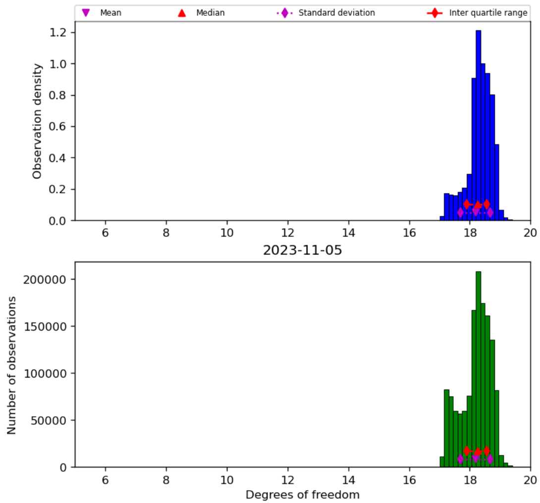
Figure 30: Histogram of “Degrees of freedom” for 2023-11-04 to 2023-11-06
