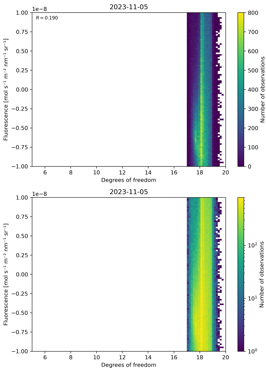
Figure 51: Scatter density plot of “Degrees of freedom” against “Fluorescence” for 2023-11-04 to 2023-11-06.
