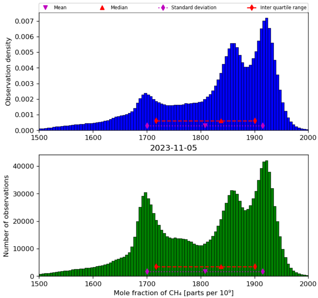
Figure 23: Histogram of “Mole fraction of CH 4 ” for 2023-11-04 to 2023-11-06
