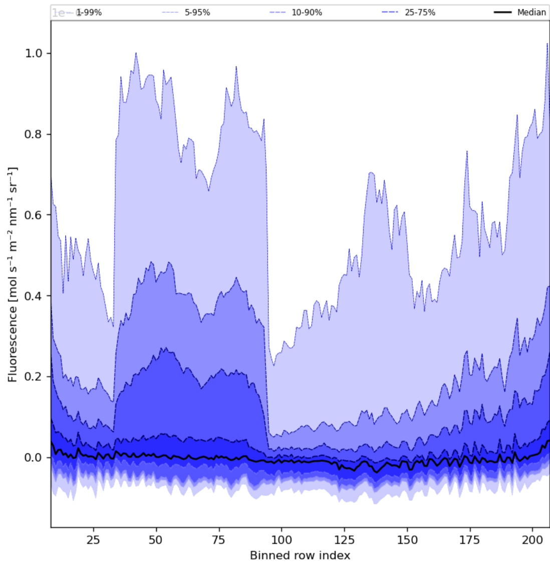
Figure 43: Along track statistics of “Fluorescence” for 2023-11-04 to 2023-11-06
