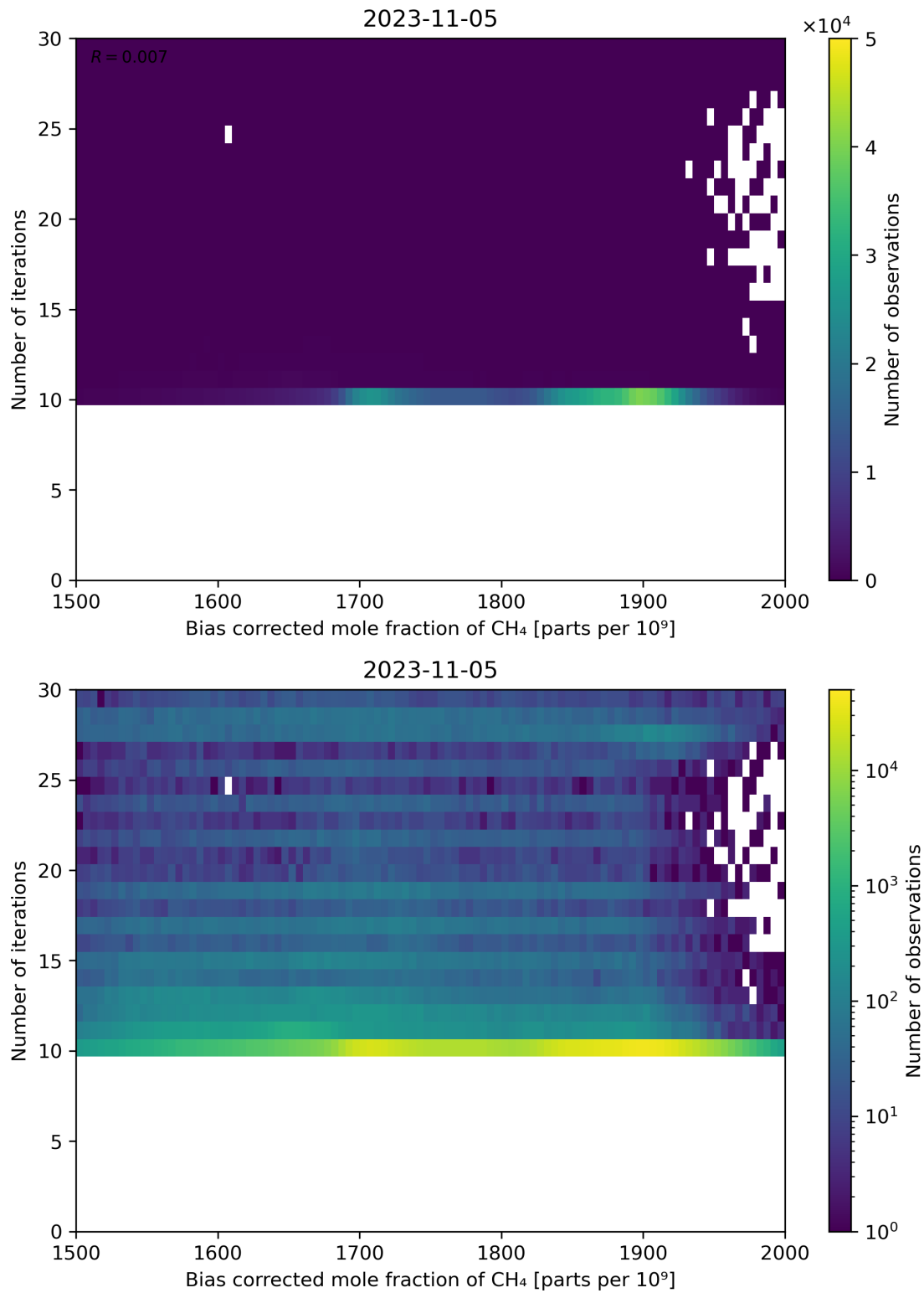
Figure 67: Scatter density plot of “Bias corrected mole fraction of CH 4 ” against “Number of iterations” for 2023-11-04 to 2023-11-06.
