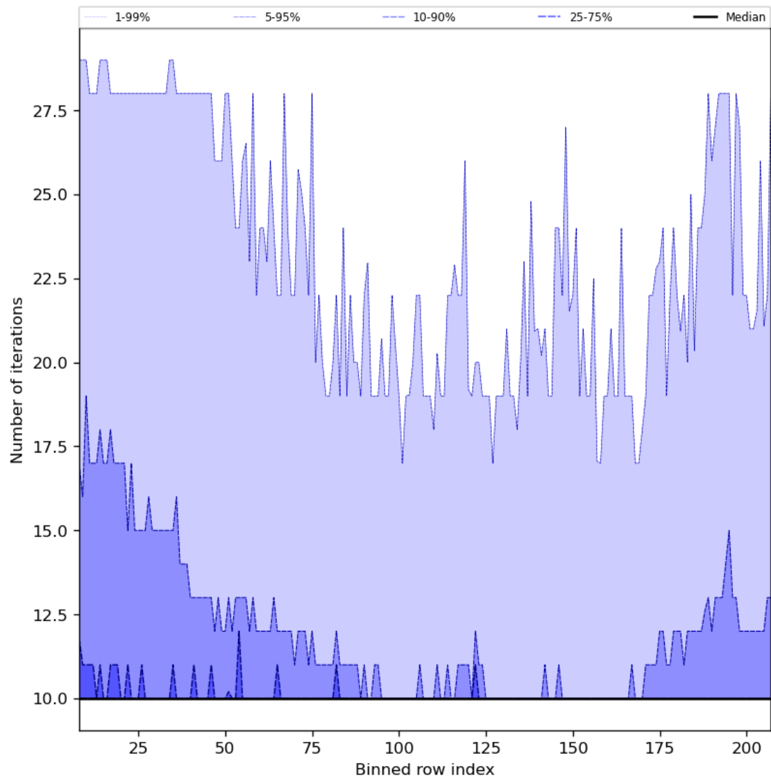
Figure 42: Along track statistics of “Number of iterations” for 2023-11-04 to 2023-11-06
