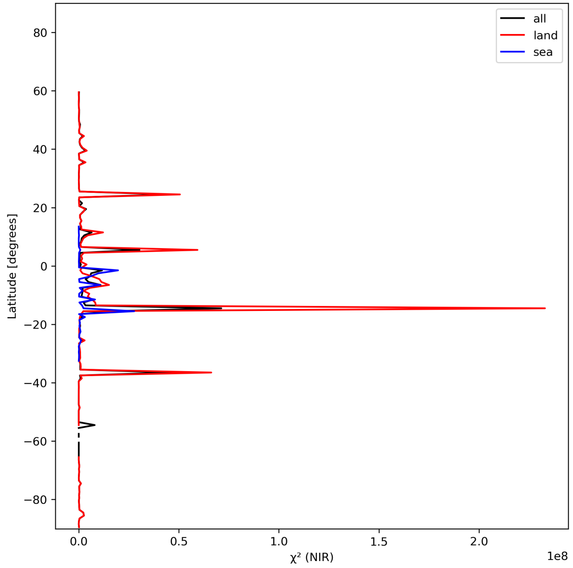
Figure 18: Zonal average of “ \chi^2 (NIR)” for 2023-11-04 to 2023-11-06.
