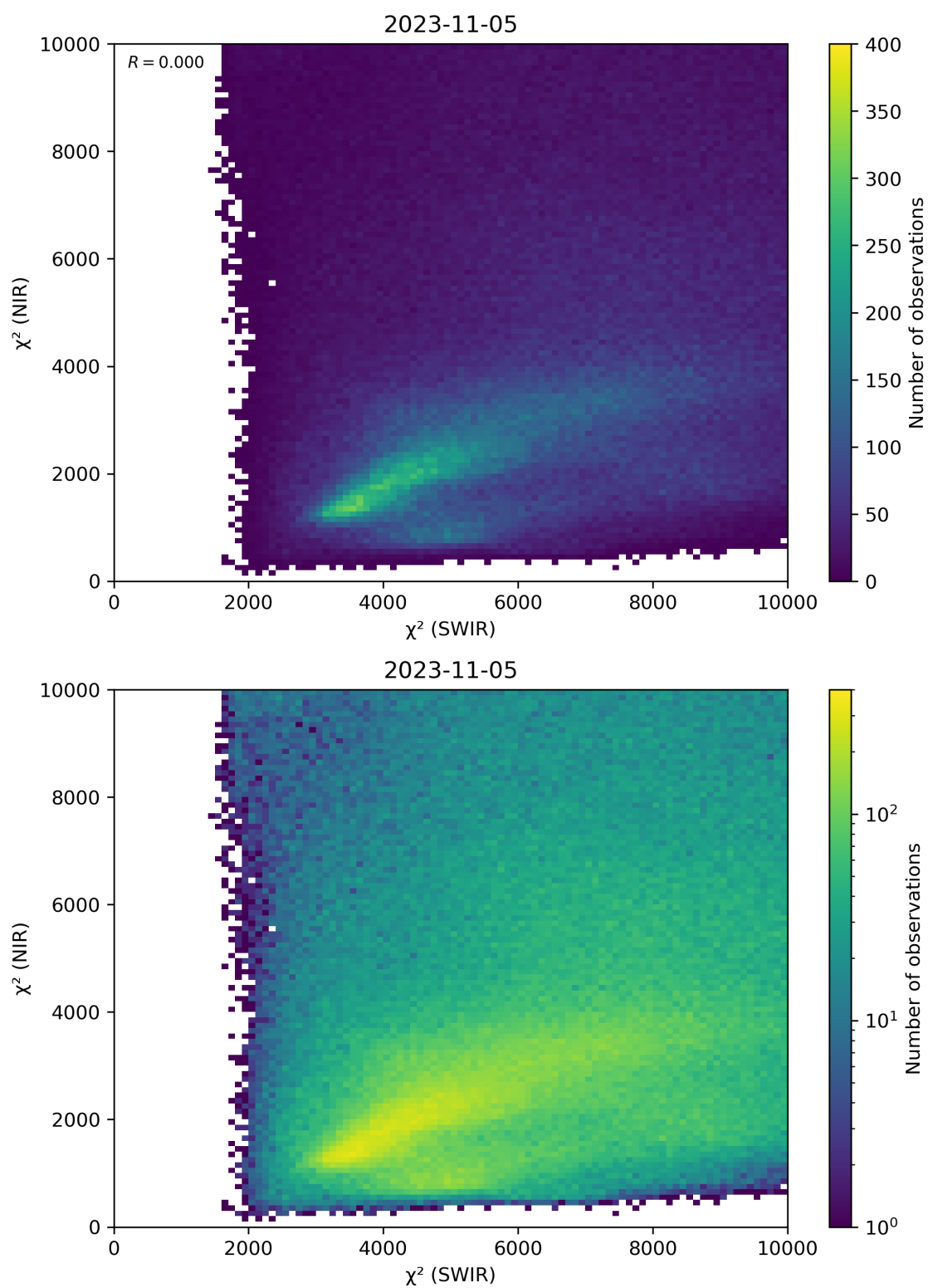
Figure 47: Scatter density plot of “ \chi^2 (SWIR)” against “ \chi^2 (NIR)” for 2023-11-04 to 2023-11-06.
