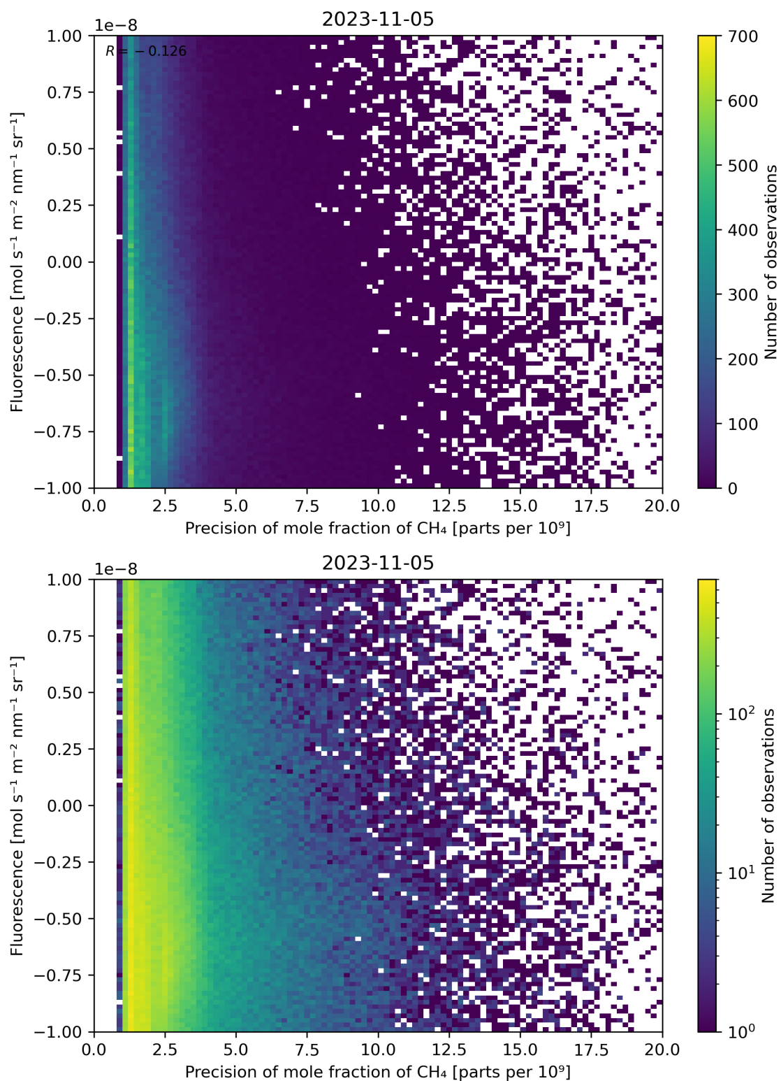
Figure 81: Scatter density plot of “Precision of mole fraction of \text{CH}_4 ” against “Fluorescence” for 2023-11-04 to 2023-11-06.
