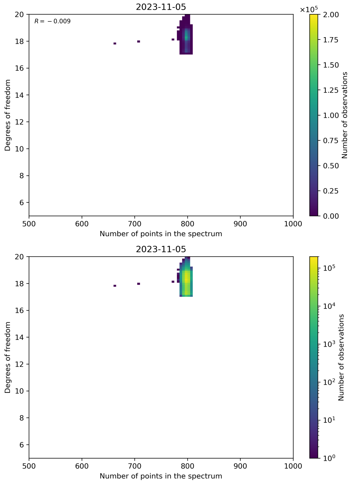
Figure 90: Scatter density plot of “Number of points in the spectrum” against “Degrees of freedom” for 2023-11-04 to 2023-11-06.
