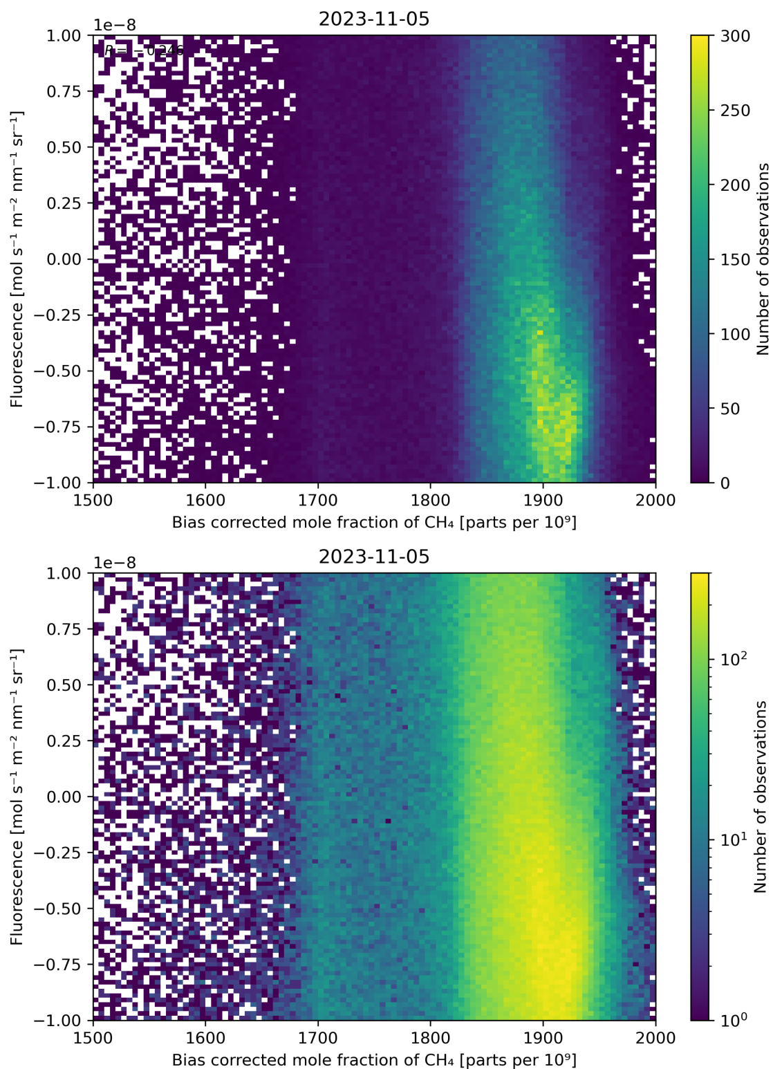
Figure 66: Scatter density plot of “Bias corrected mole fraction of \text{CH}_4 ” against “Fluorescence” for 2023-11-04 to 2023-11-06.
