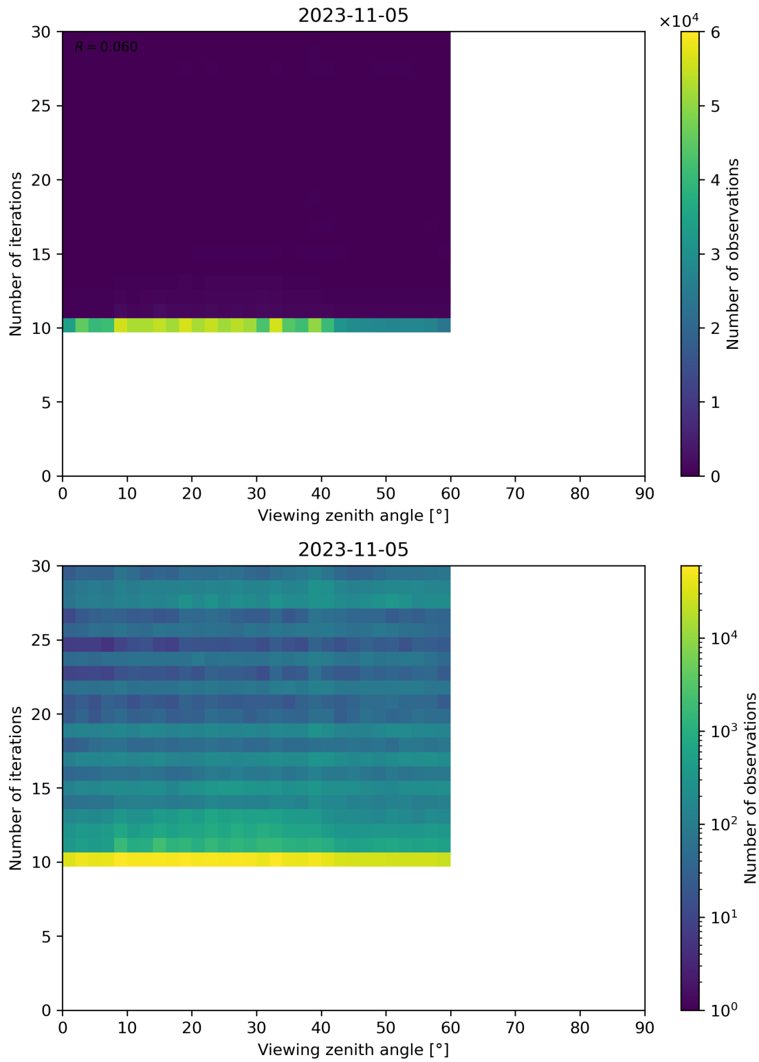
Figure 113: Scatter density plot of “Viewing zenith angle” against “Number of iterations” for 2023-11-04 to 2023-11-06.
