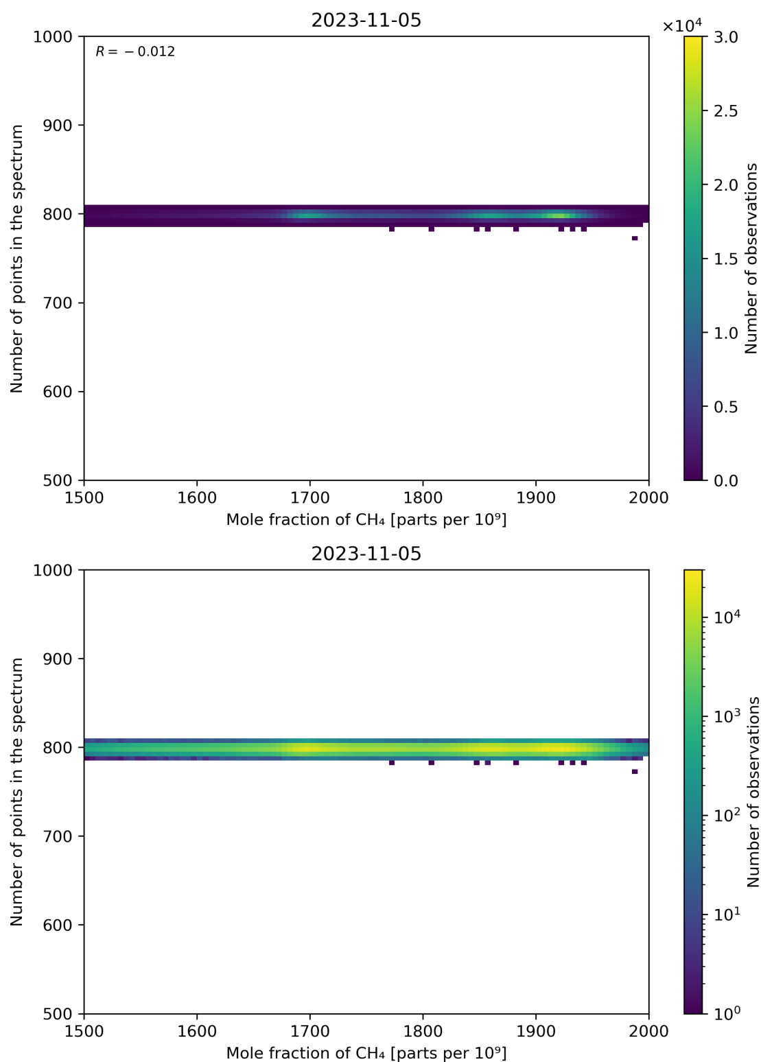
Figure 77: Scatter density plot of “Mole fraction of CH 4 ” against “Number of points in the spectrum” for 2023-11-04 to 2023-11-06.
