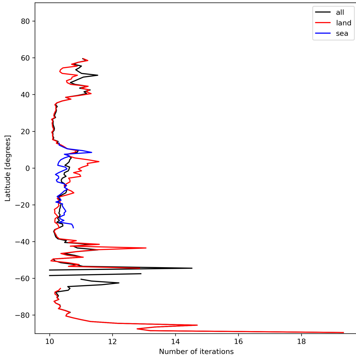
Figure 20: Zonal average of “Number of iterations” for 2023-11-04 to 2023-11-06.
