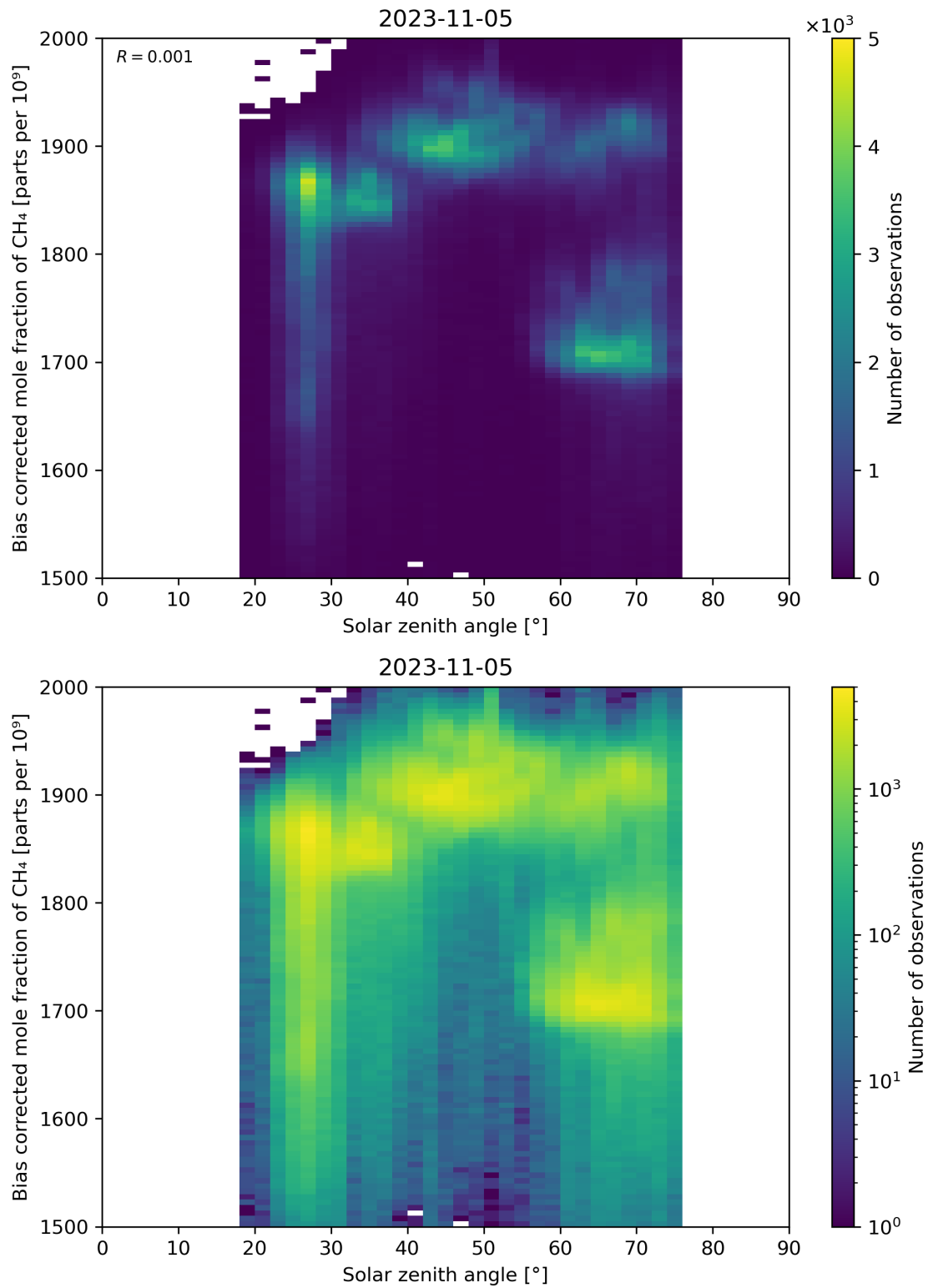
Figure 100: Scatter density plot of “Solar zenith angle” against “Bias corrected mole fraction of \text{CH}_4 ” for 2023-11-04 to 2023-11-06.
