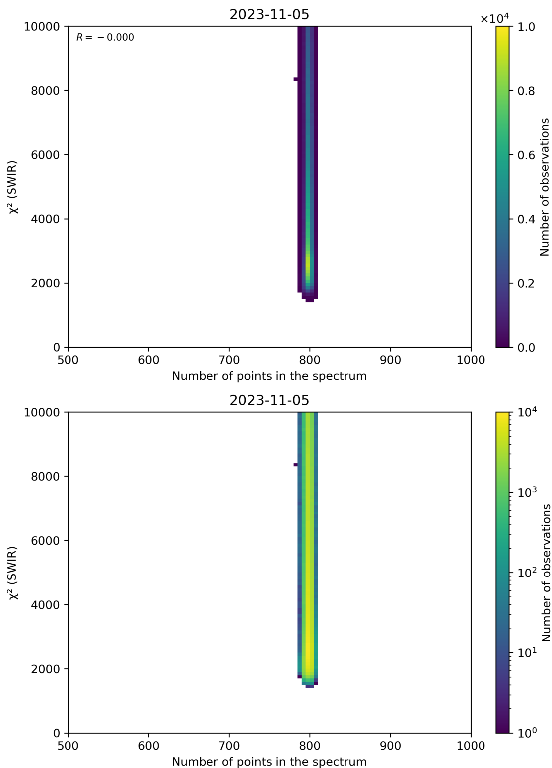
Figure 89: Scatter density plot of “Number of points in the spectrum” against “ \chi^2 (SWIR)” for 2023-11-04 to 2023-11-06.
