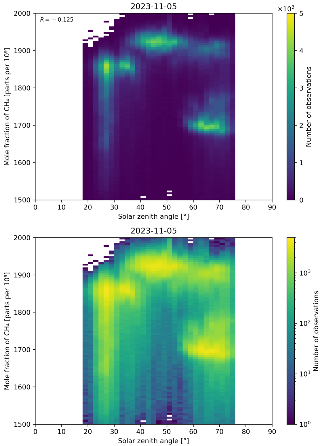
Figure 99: Scatter density plot of “Solar zenith angle” against “Mole fraction of \text{CH}_4 ” for 2023-11-04 to 2023-11-06.
