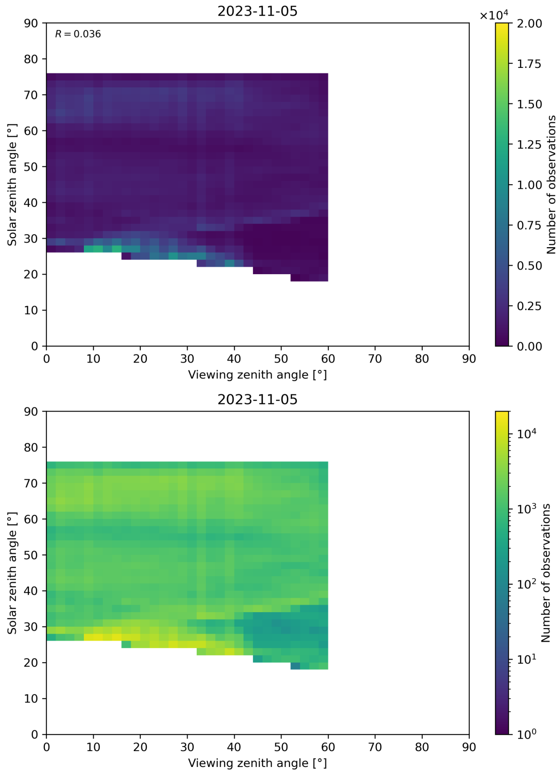
Figure 115: Scatter density plot of “Viewing zenith angle” against “Solar zenith angle” for 2023-11-04 to 2023-11-06.
