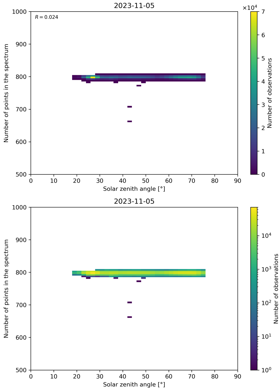
Figure 103: Scatter density plot of “Solar zenith angle” against “Number of points in the spectrum” for 2023-11-04 to 2023-11-06.
