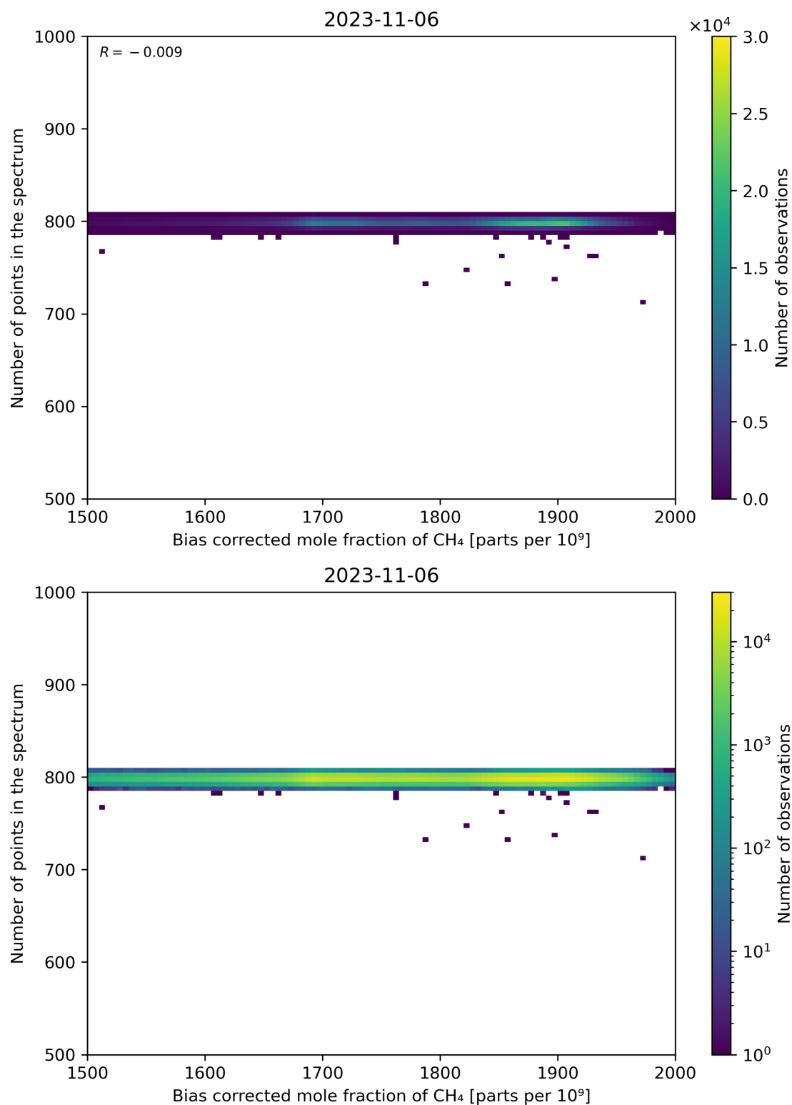
Figure 68: Scatter density plot of “Bias corrected mole fraction of CH 4 ” against “Number of points in the spectrum” for 2023-11-05 to 2023-11-07.
