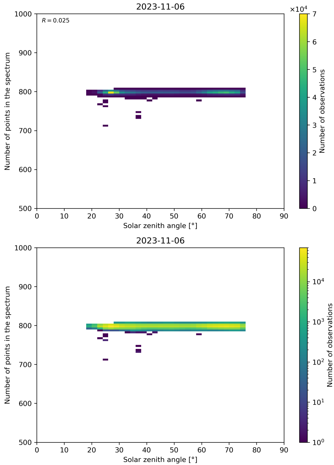
Figure 103: Scatter density plot of “Solar zenith angle” against “Number of points in the spectrum” for 2023-11-05 to 2023-11-07.
