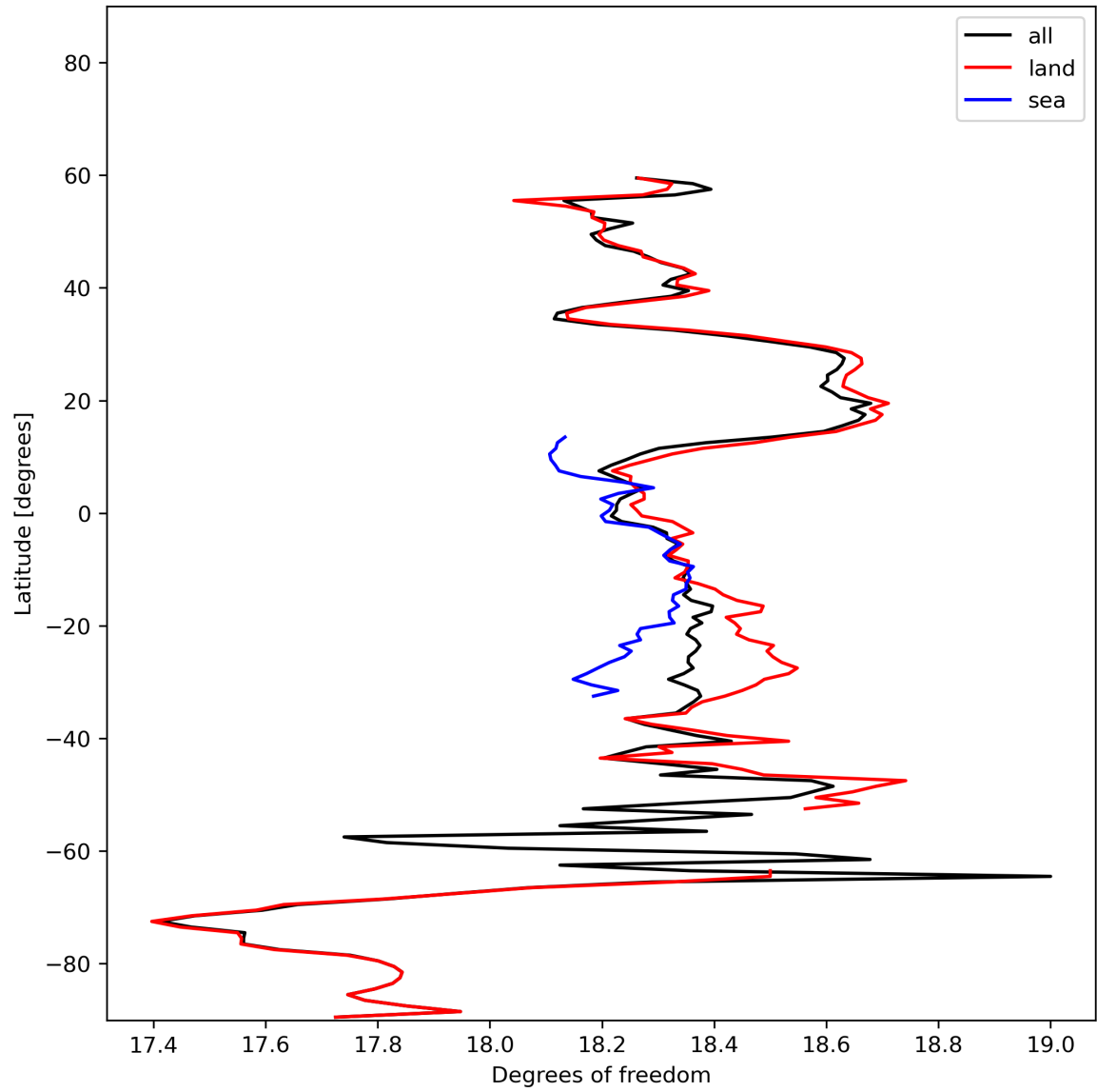
Figure 19: Zonal average of “Degrees of freedom” for 2023-11-05 to 2023-11-07.
