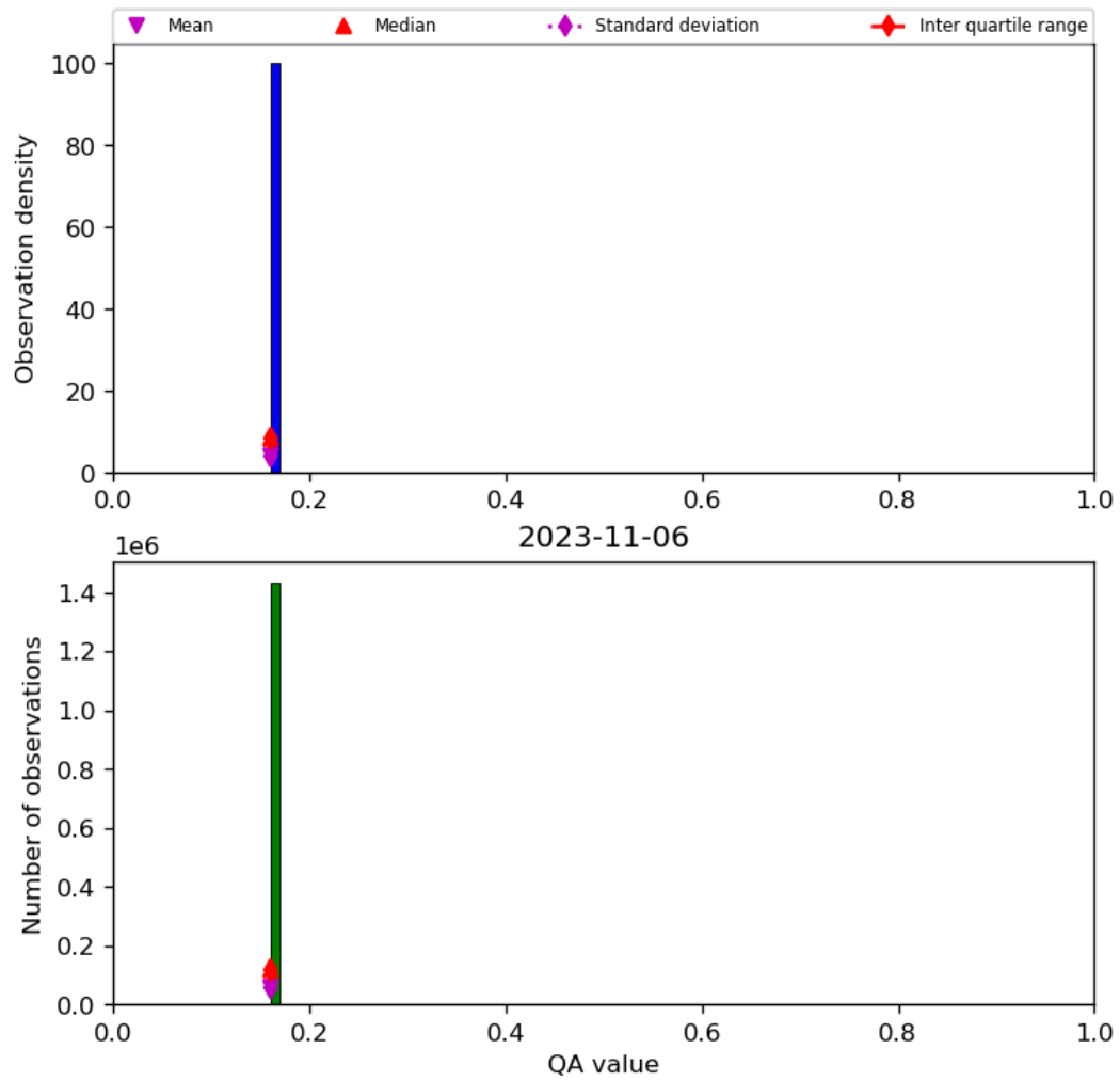
Figure 22: Histogram of “QA value” for 2023-11-05 to 2023-11-07
