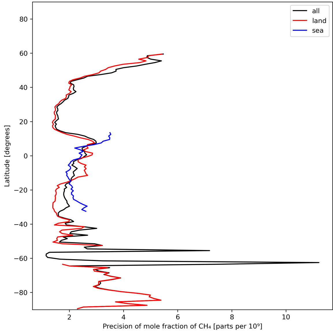
Figure 13: Zonal average of “Precision of mole fraction of CH 4 ” for 2023-11-05 to 2023-11-07.
