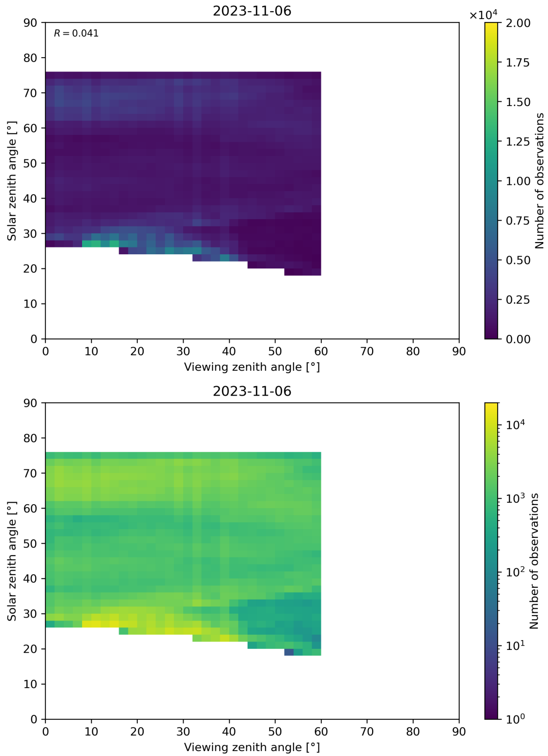
Figure 115: Scatter density plot of “Viewing zenith angle” against “Solar zenith angle” for 2023-11-05 to 2023-11-07.
