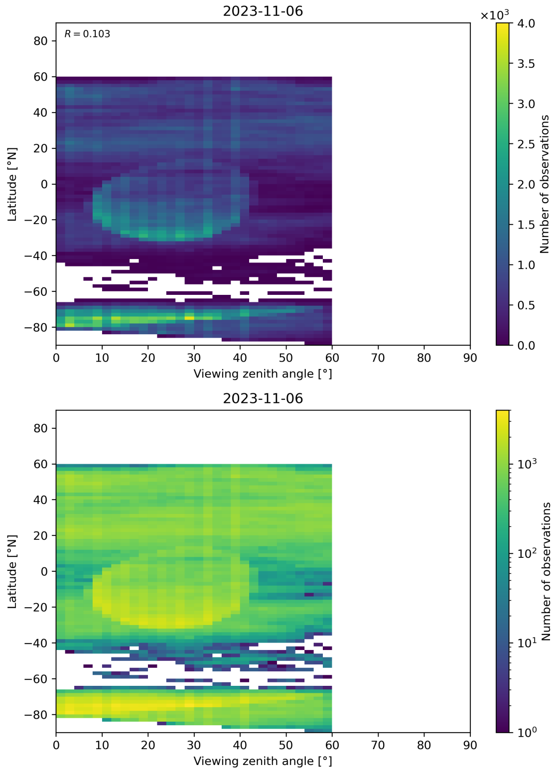
Figure 109: Scatter density plot of “Viewing zenith angle” against “Latitude” for 2023-11-05 to 2023-11-07.
