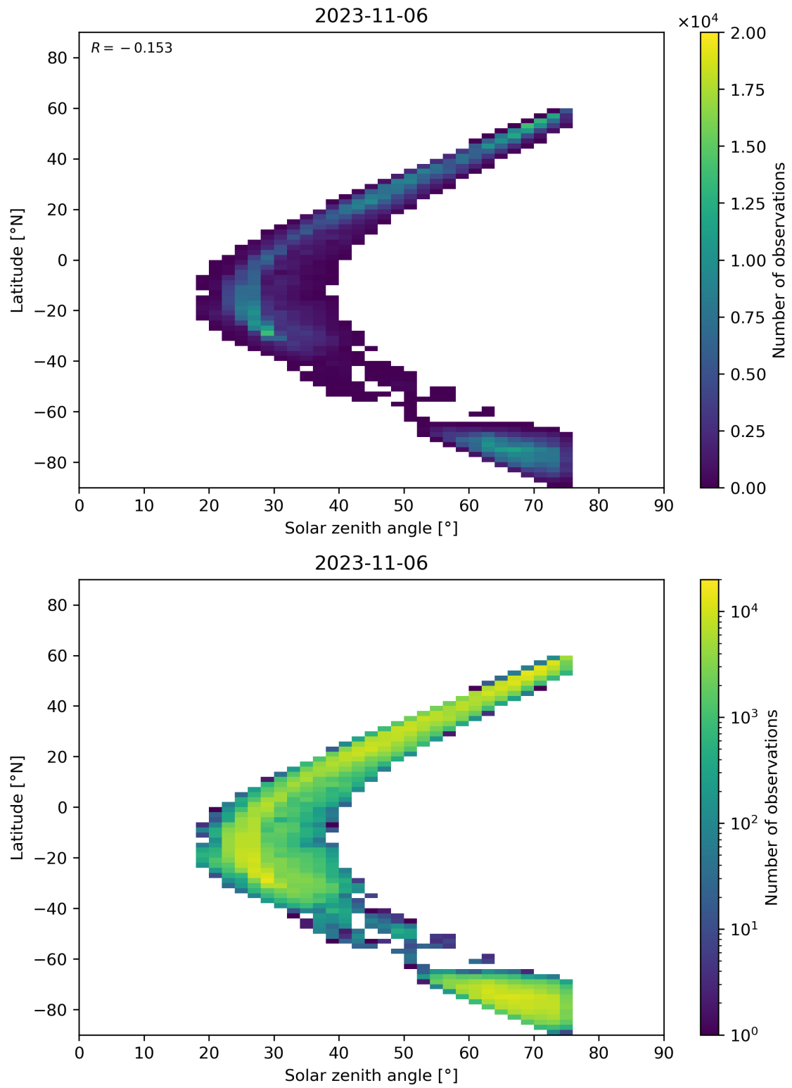
Figure 98: Scatter density plot of “Solar zenith angle” against “Latitude” for 2023-11-05 to 2023-11-07.
