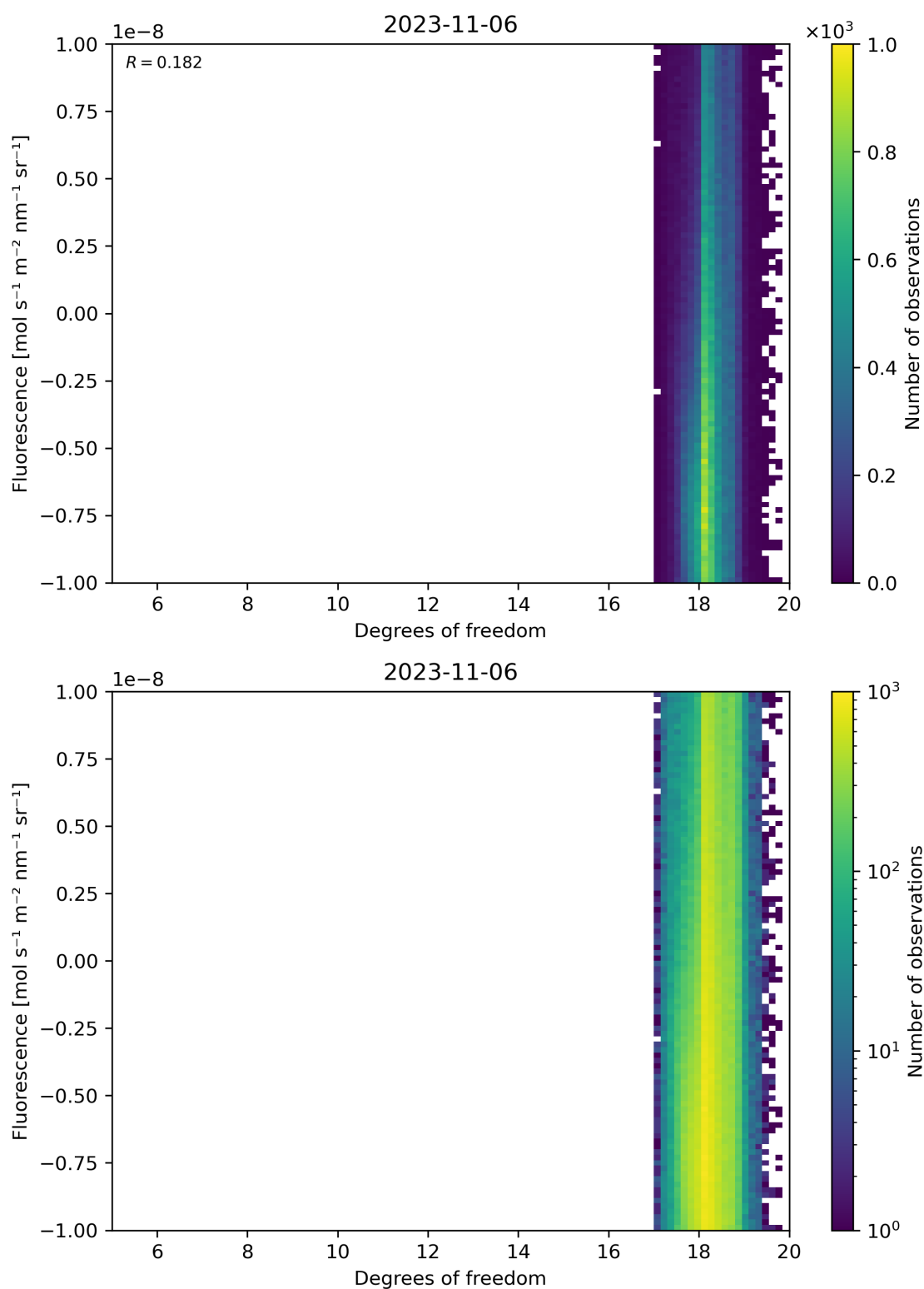
Figure 51: Scatter density plot of “Degrees of freedom” against “Fluorescence” for 2023-11-05 to 2023-11-07.
