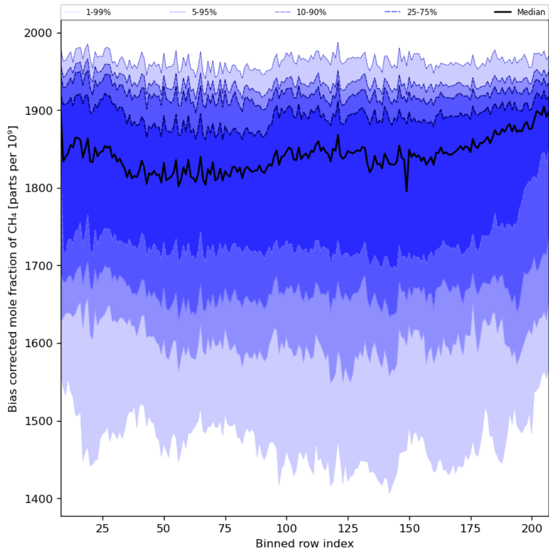
Figure 36: Along track statistics of “Bias corrected mole fraction of CH 4 ” for 2023-11-05 to 2023-11-07
