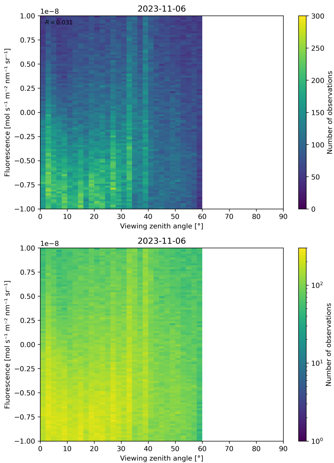
Figure 108: Scatter density plot of “Viewing zenith angle” against “Fluorescence” for 2023-11-05 to 2023-11-07.
