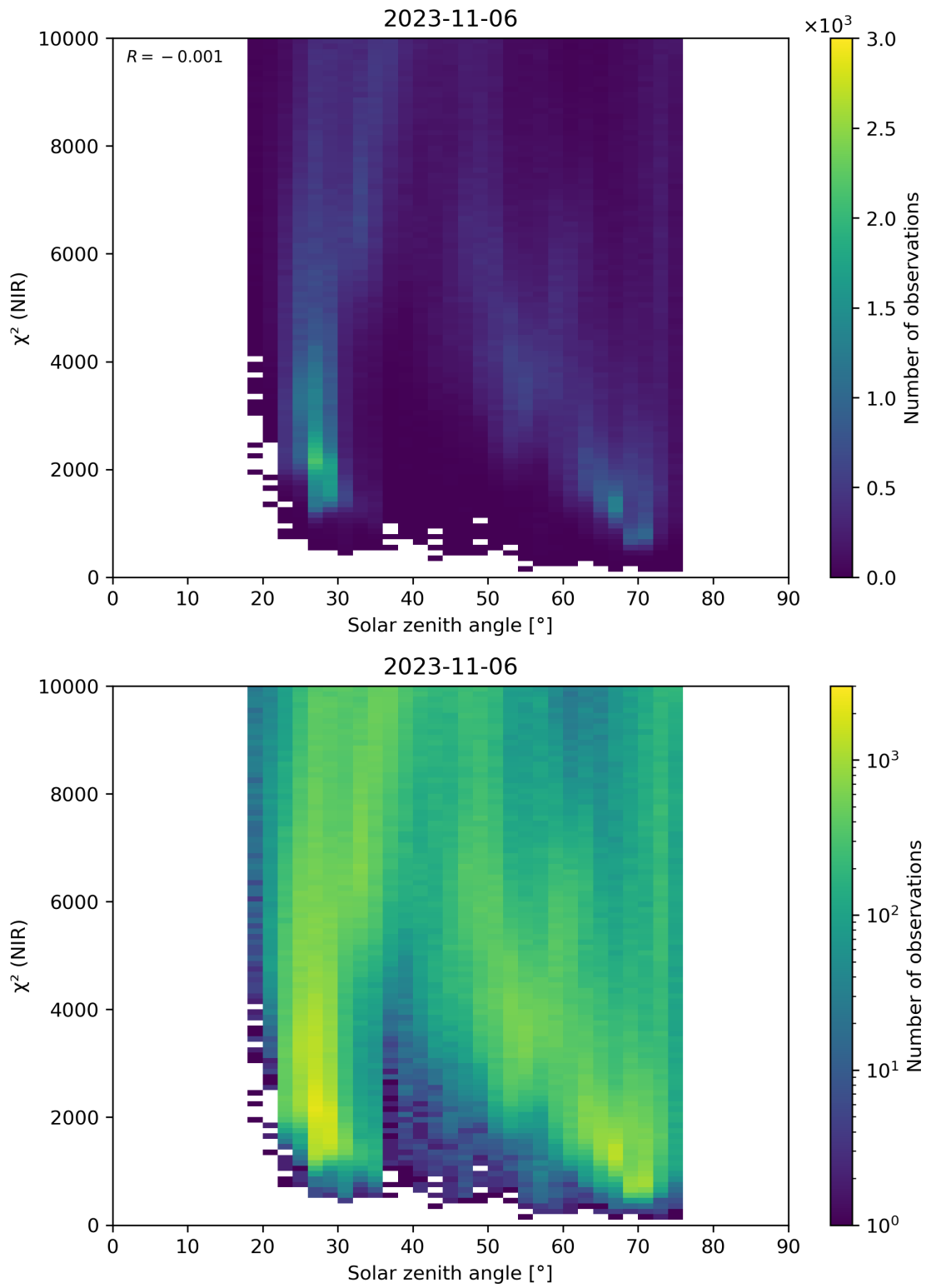
Figure 94: Scatter density plot of “Solar zenith angle” against “ \chi^2 (NIR)” for 2023-11-05 to 2023-11-07.
