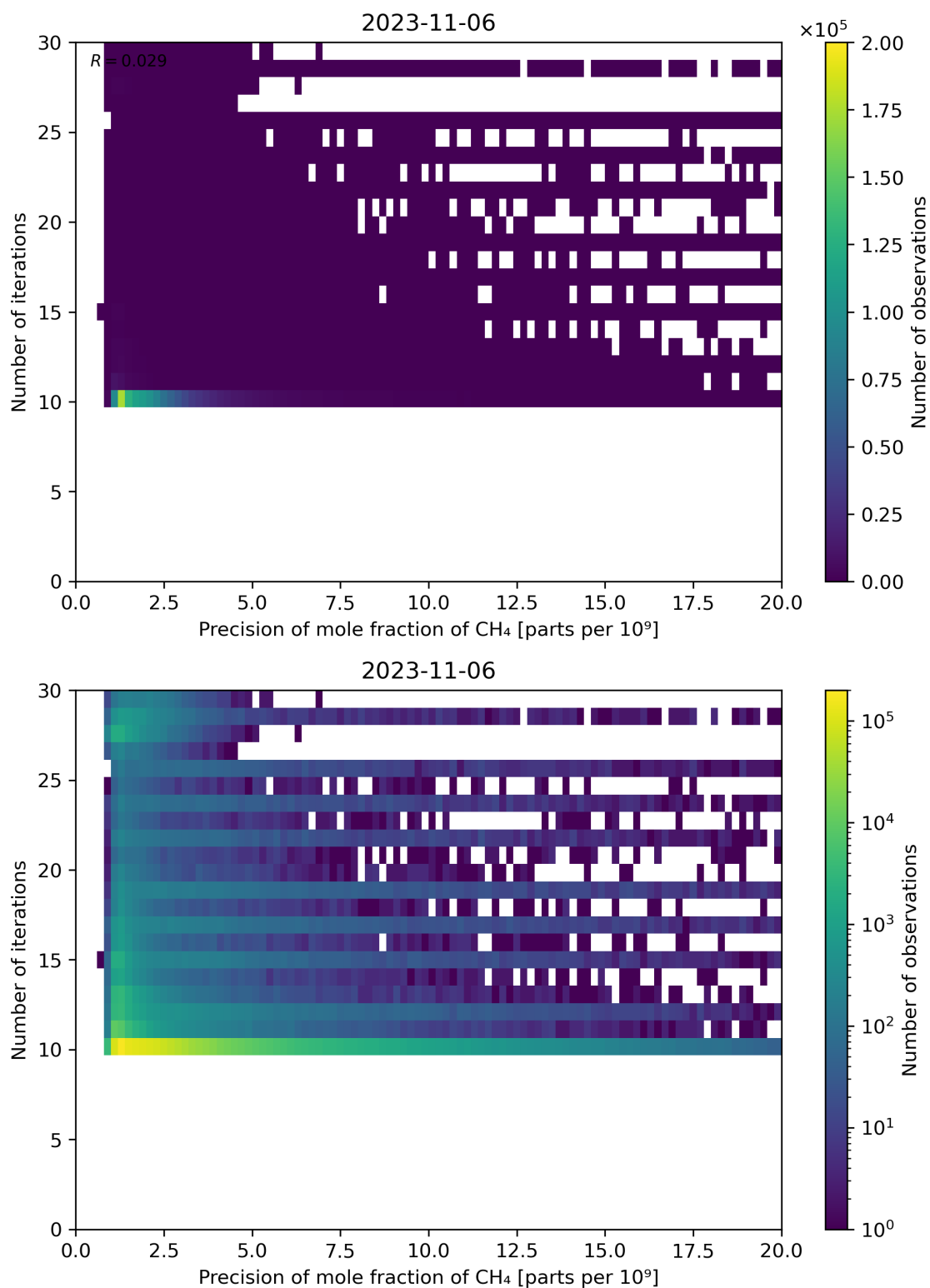
Figure 83: Scatter density plot of “Precision of mole fraction of CH 4 ” against “Number of iterations” for 2023-11-05 to 2023-11-07.
