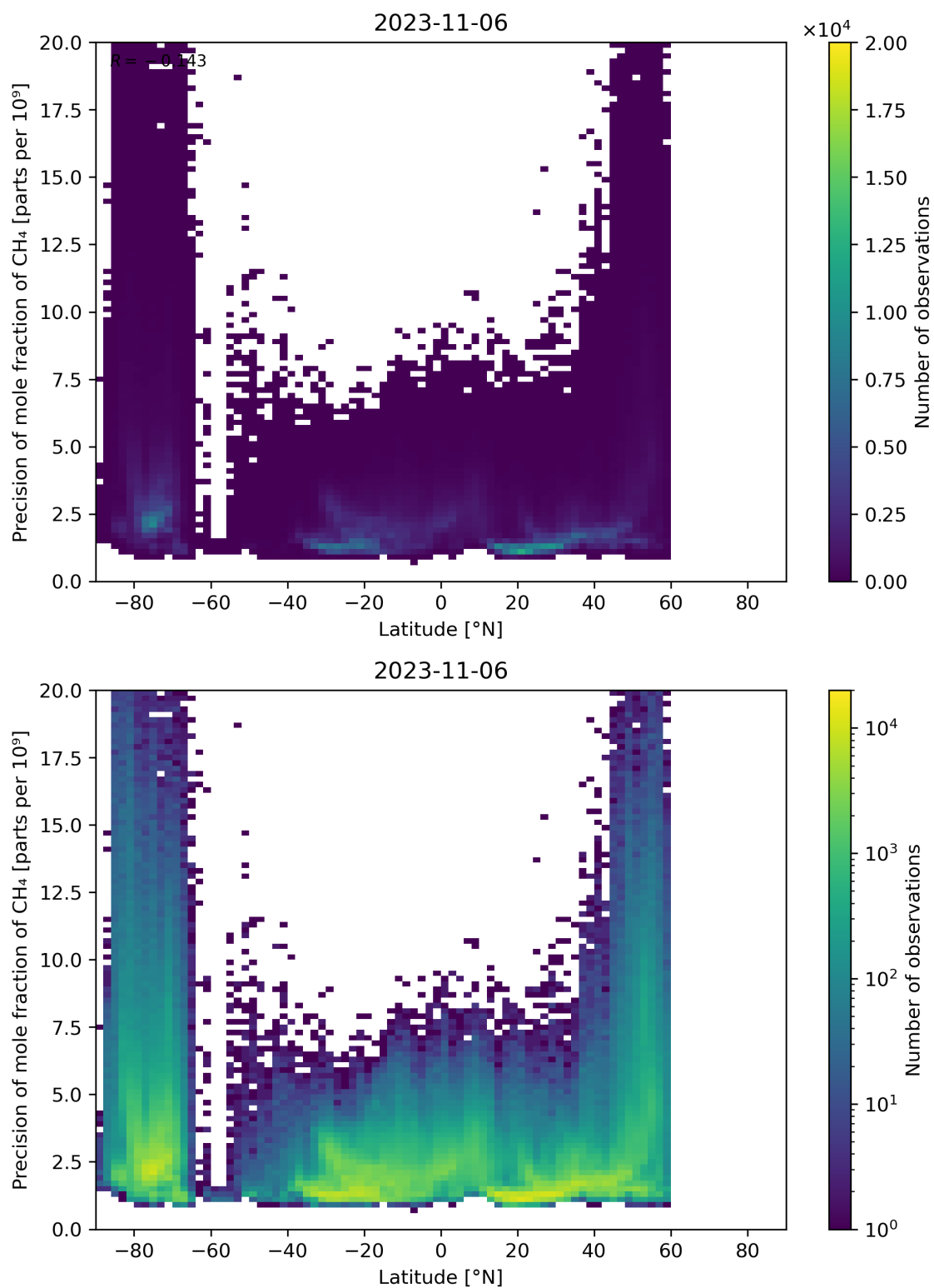
Figure 59: Scatter density plot of “Latitude” against “Precision of mole fraction of CH 4 ” for 2023-11-05 to 2023-11-07.
