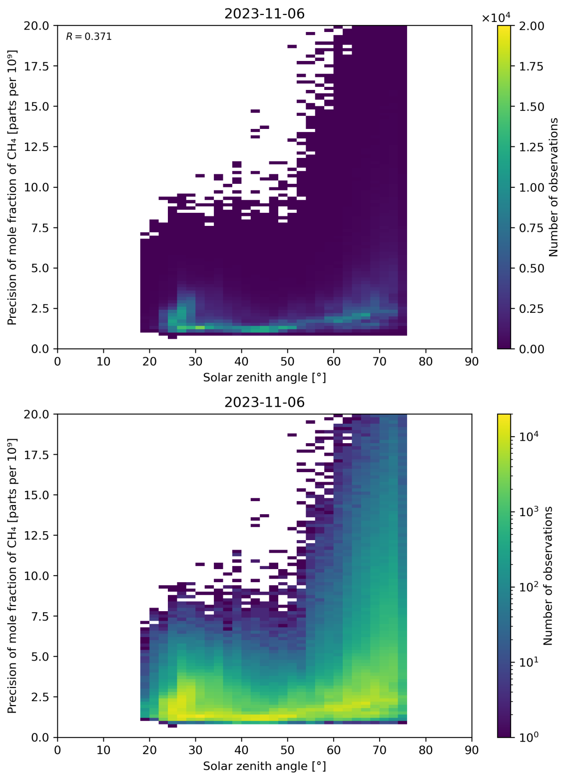
Figure 101: Scatter density plot of “Solar zenith angle” against “Precision of mole fraction of CH 4 ” for 2023-11-05 to 2023-11-07.
