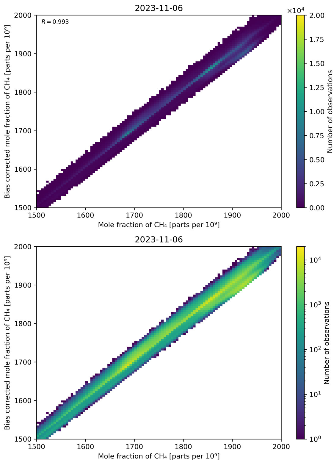
Figure 74: Scatter density plot of “Mole fraction of CH 4 ” against “Bias corrected mole fraction of CH 4 ” for 2023-11-05 to 2023-11-07.
