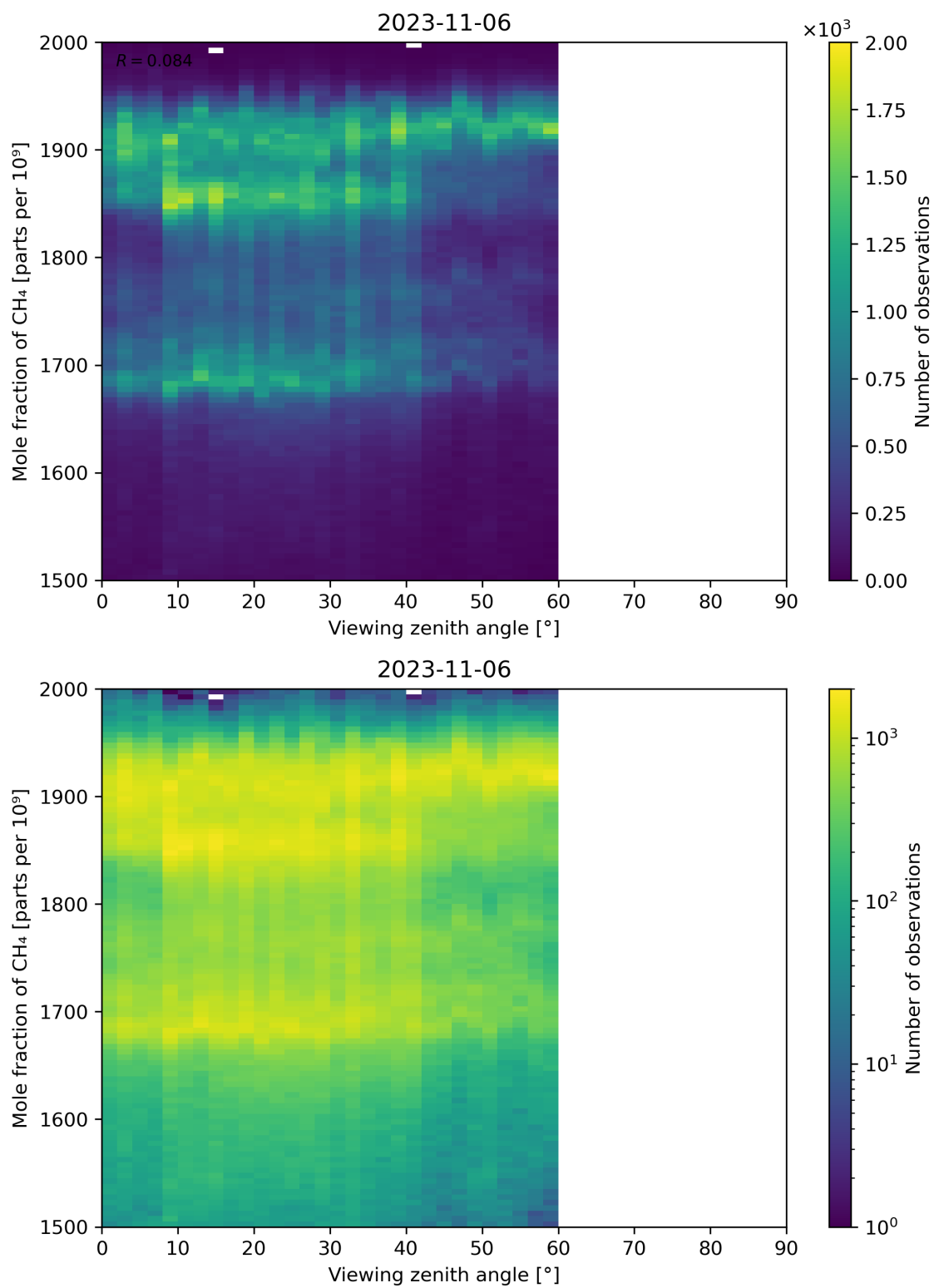
Figure 110: Scatter density plot of “Viewing zenith angle” against “Mole fraction of CH 4 ” for 2023-11-05 to 2023-11-07.
