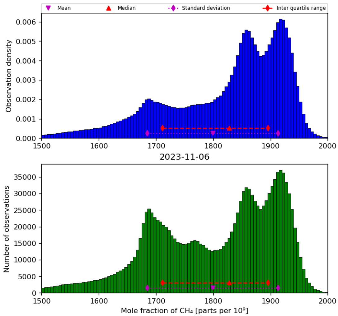
Figure 23: Histogram of “Mole fraction of CH 4 ” for 2023-11-05 to 2023-11-07
