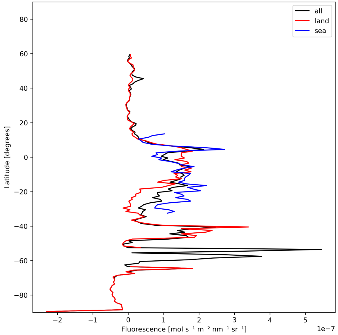
Figure 21: Zonal average of “Fluorescence” for 2023-11-05 to 2023-11-07.
