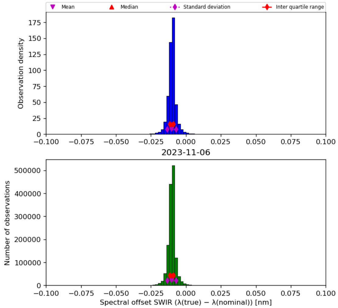
Figure 27: Histogram of “Spectral offset SWIR ( \lambda(\text{true}) - \lambda(\text{nominal}) )” for 2023-11-05 to 2023-11-07
