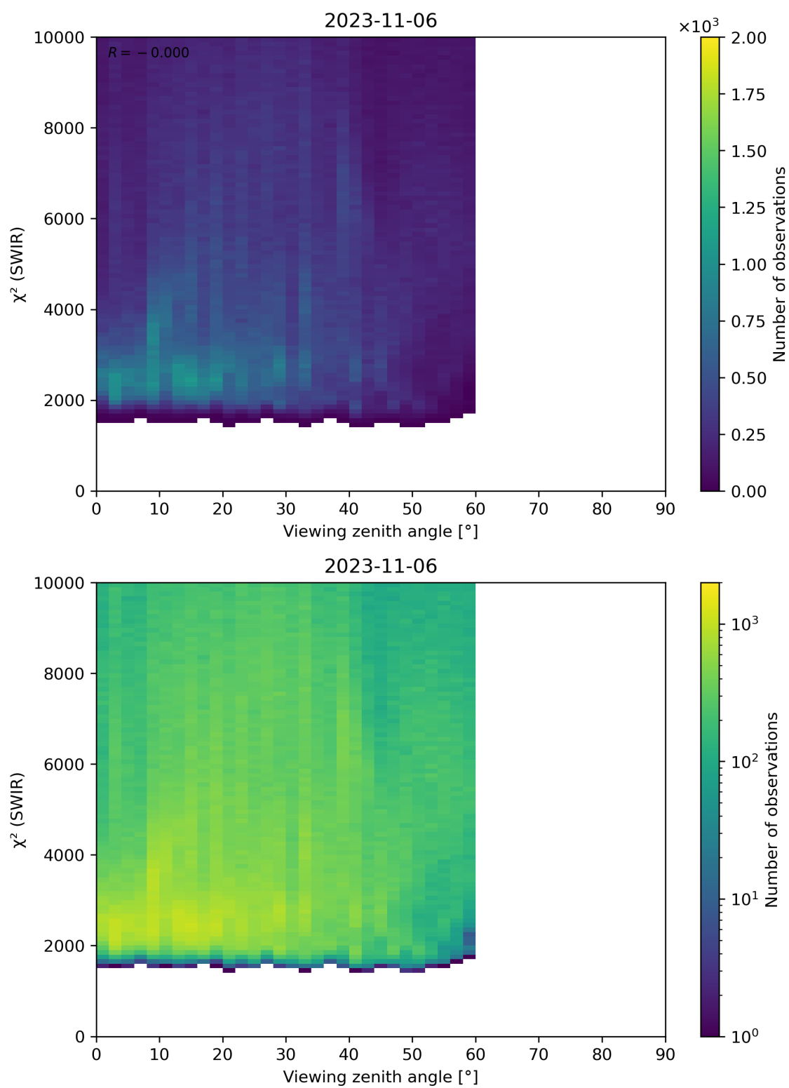
Figure 106: Scatter density plot of “Viewing zenith angle” against “ \chi^2 (SWIR)” for 2023-11-05 to 2023-11-07.
