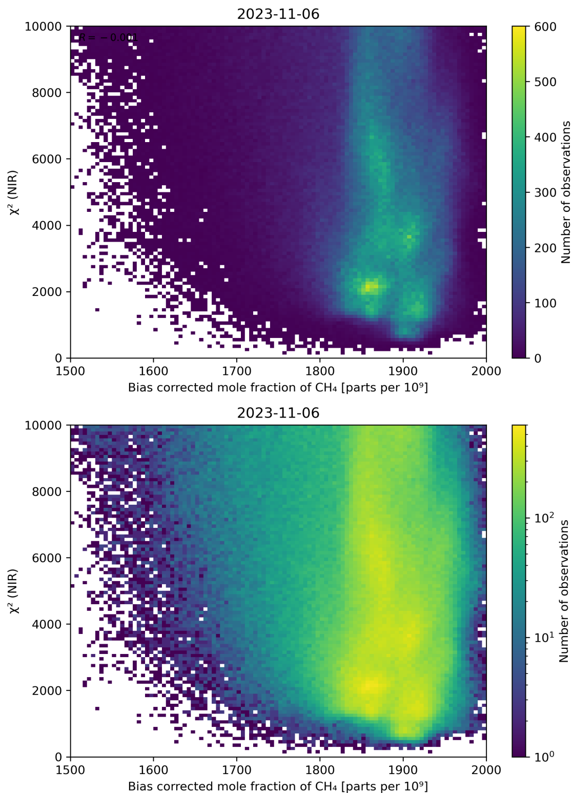
Figure 63: Scatter density plot of “Bias corrected mole fraction of CH 4 ” against “ \chi^2 (NIR)” for 2023-11-05 to 2023-11-07.
