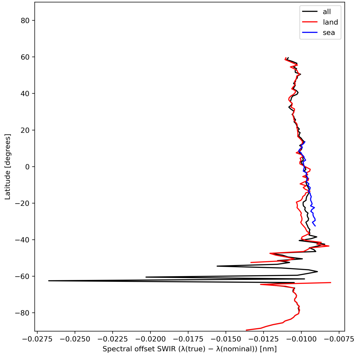
Figure 16: Zonal average of “Spectral offset SWIR ( \lambda(\text{true}) - \lambda(\text{nominal}) )” for 2023-11-05 to 2023-11-07.
