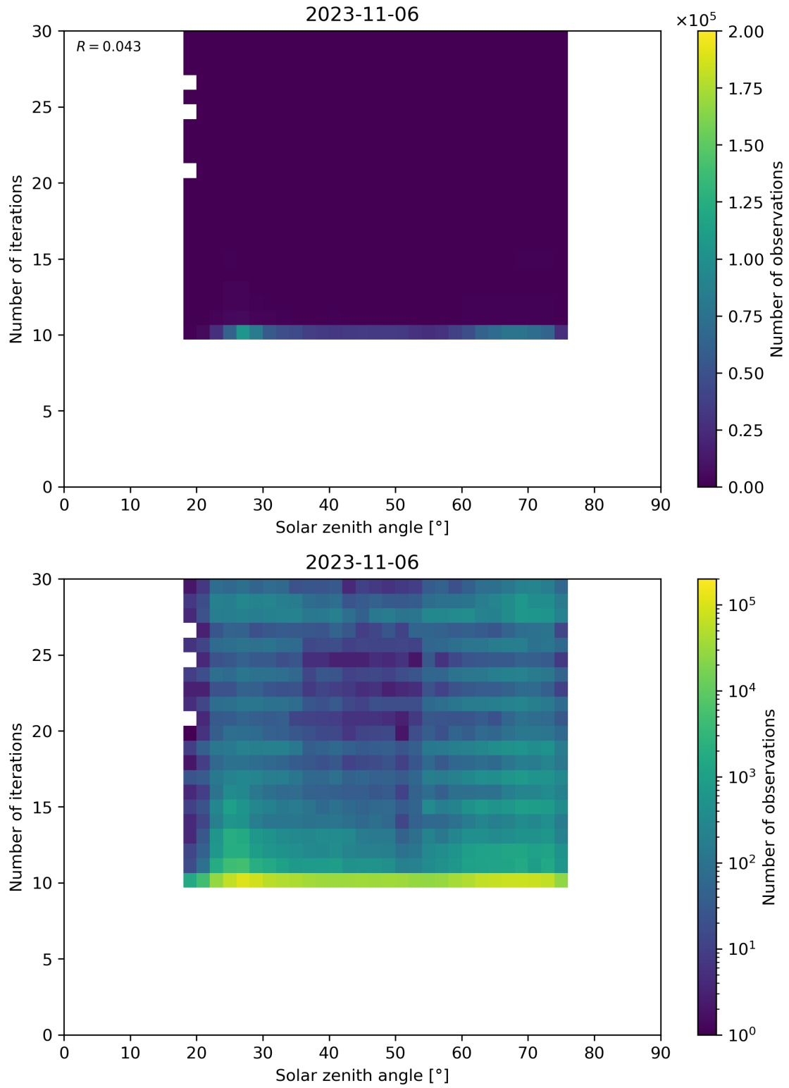
Figure 102: Scatter density plot of “Solar zenith angle” against “Number of iterations” for 2023-11-05 to 2023-11-07.
