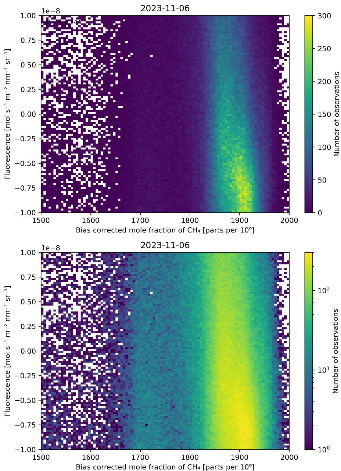
Figure 66: Scatter density plot of “Bias corrected mole fraction of \text{CH}_4 ” against “Fluorescence” for 2023-11-05 to 2023-11-07.
