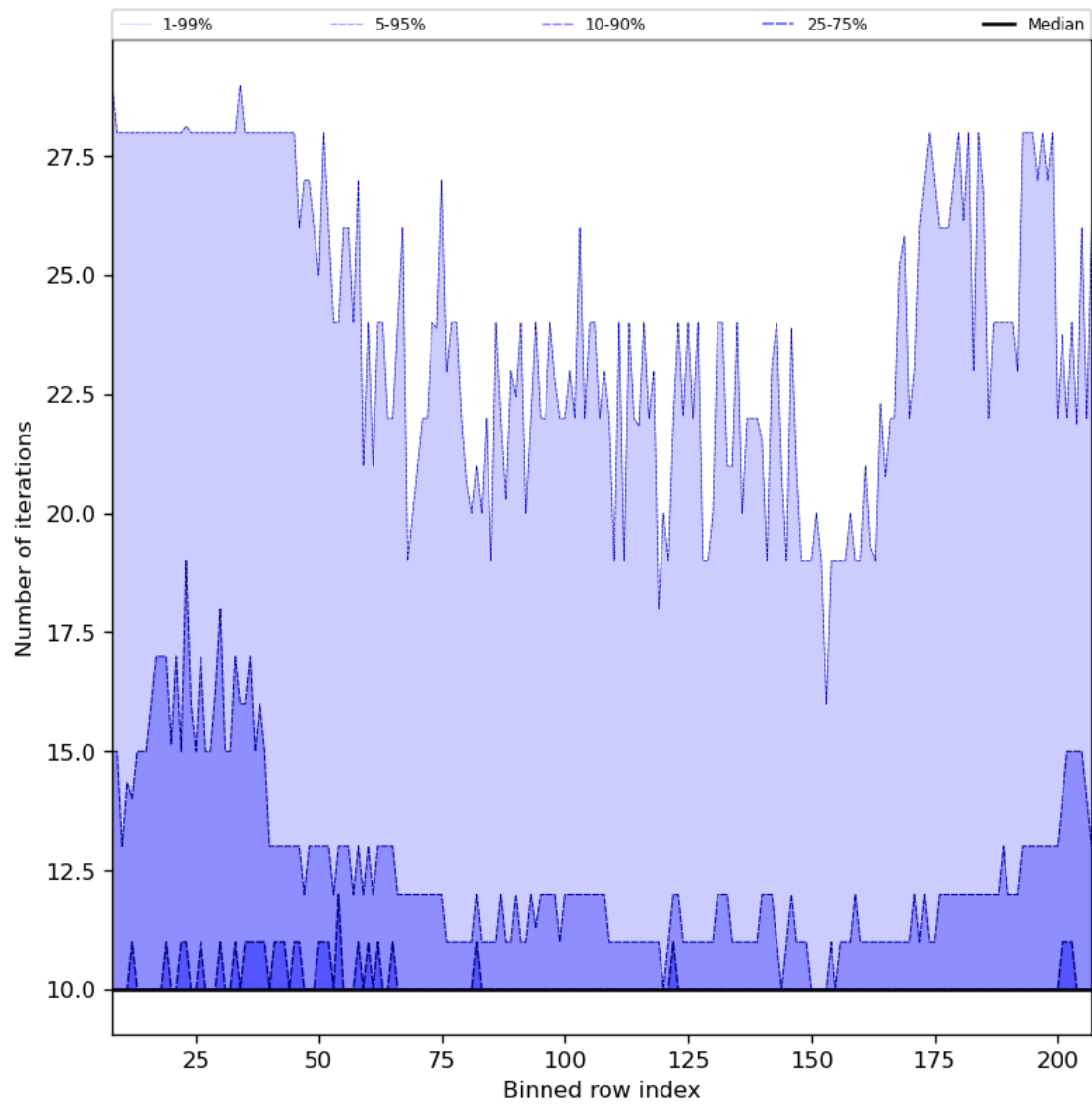
Figure 42: Along track statistics of “Number of iterations” for 2023-11-05 to 2023-11-07
