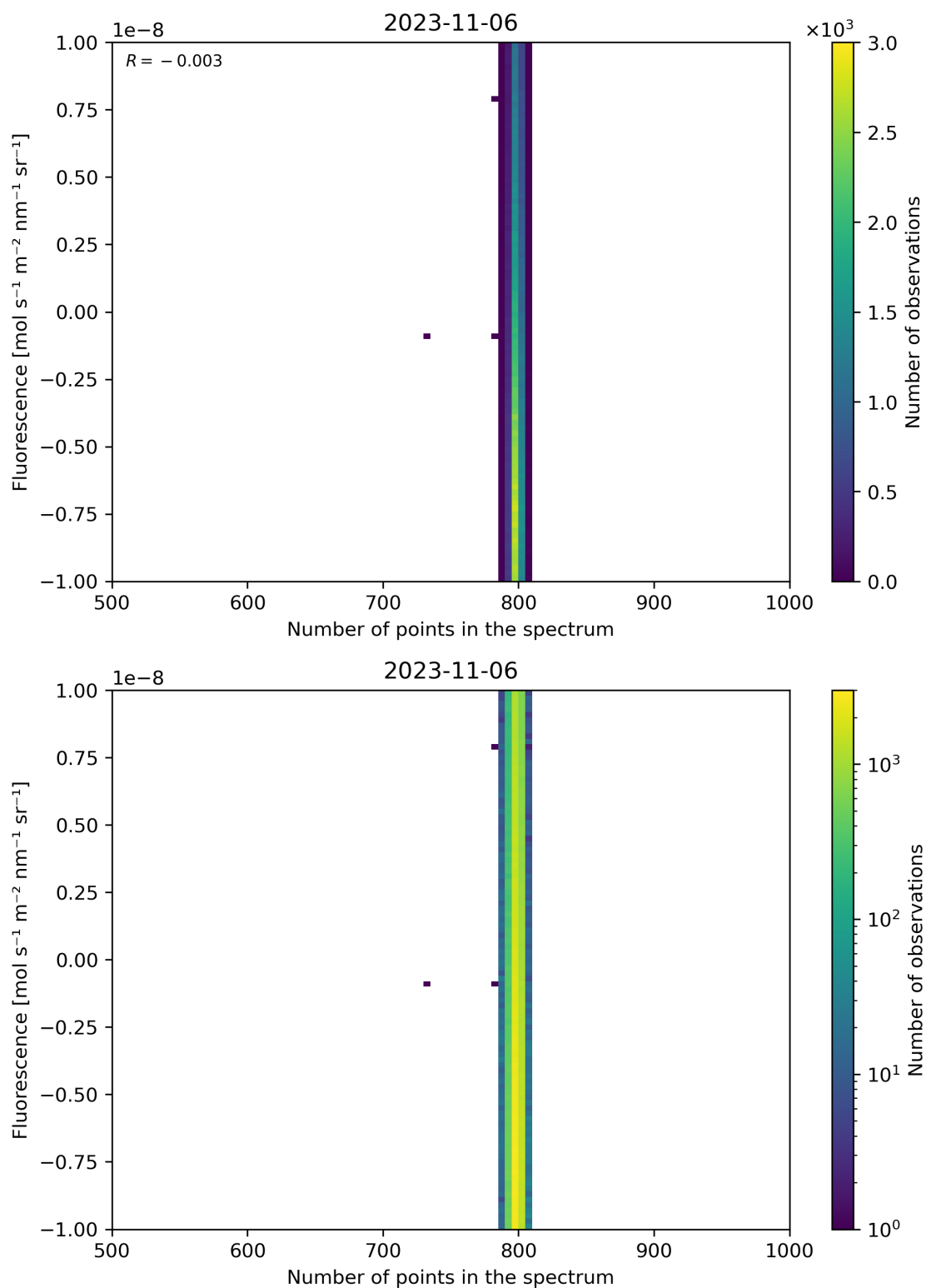
Figure 91: Scatter density plot of “Number of points in the spectrum” against “Fluorescence” for 2023-11-05 to 2023-11-07.
