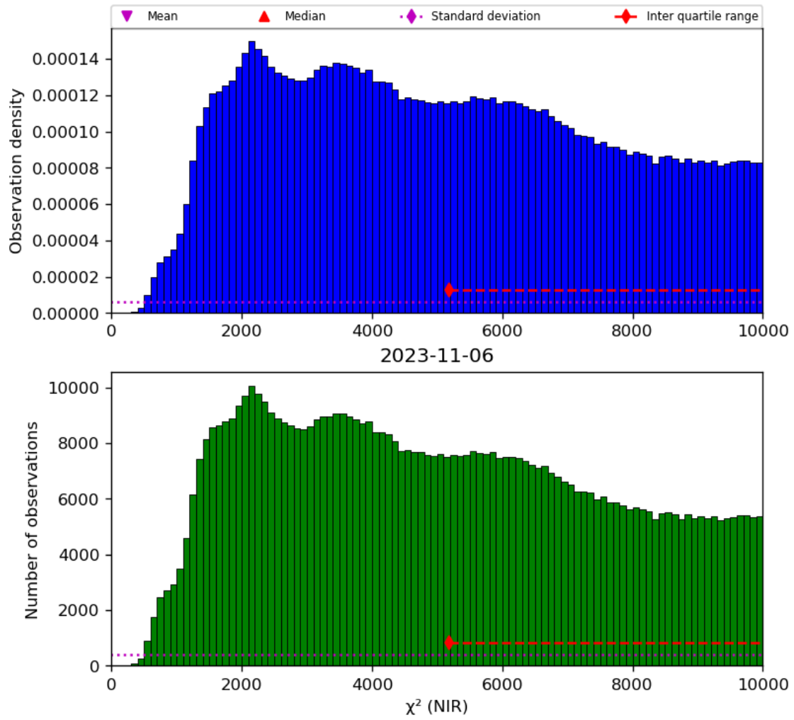
Figure 29: Histogram of “ \chi^2 (NIR)” for 2023-11-05 to 2023-11-07
