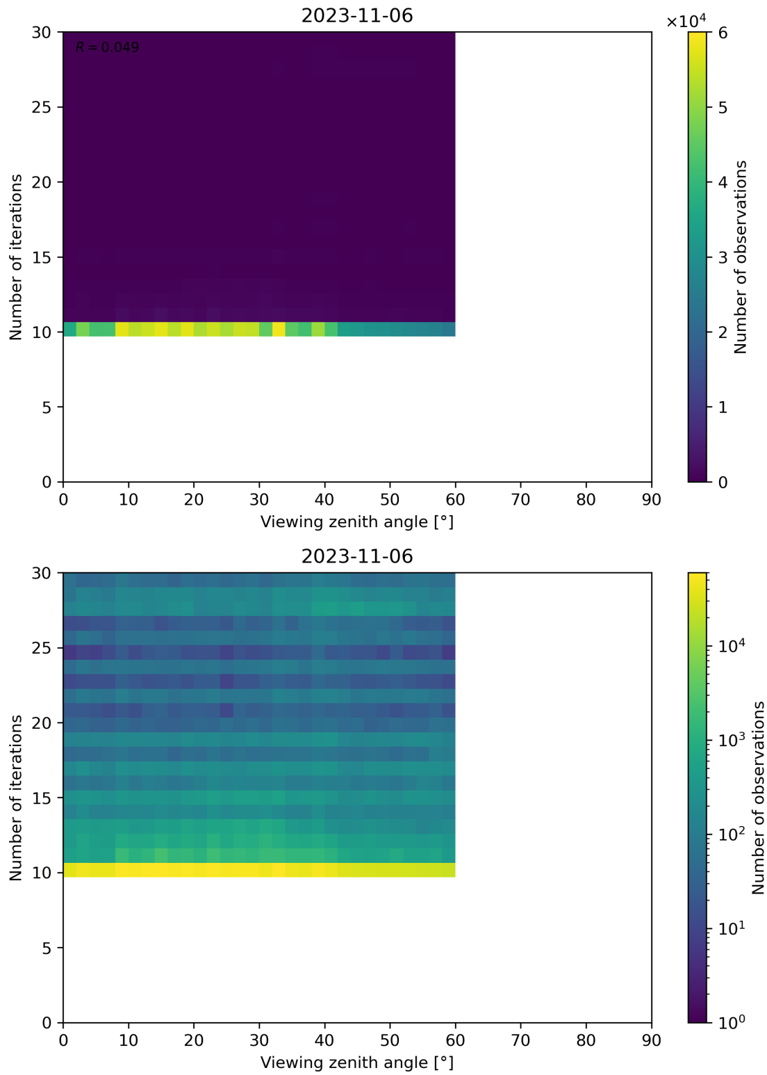
Figure 113: Scatter density plot of “Viewing zenith angle” against “Number of iterations” for 2023-11-05 to 2023-11-07.
