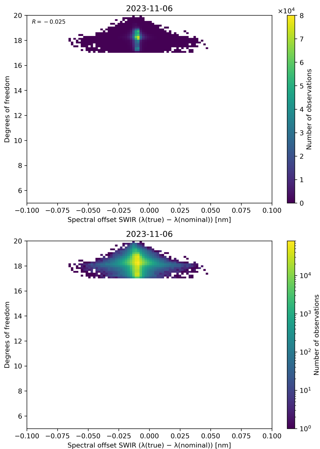
Figure 119: Scatter density plot of “Spectral offset SWIR ( \lambda(\text{true}) - \lambda(\text{nominal}) )” against “Degrees of freedom” for 2023-11-05 to 2023-11-07.
