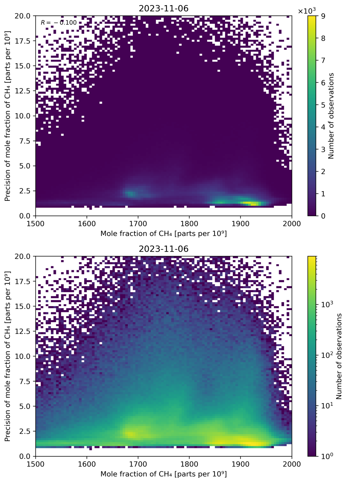
Figure 75: Scatter density plot of “Mole fraction of CH 4 ” against “Precision of mole fraction of CH 4 ” for 2023-11-05 to 2023-11-07.
