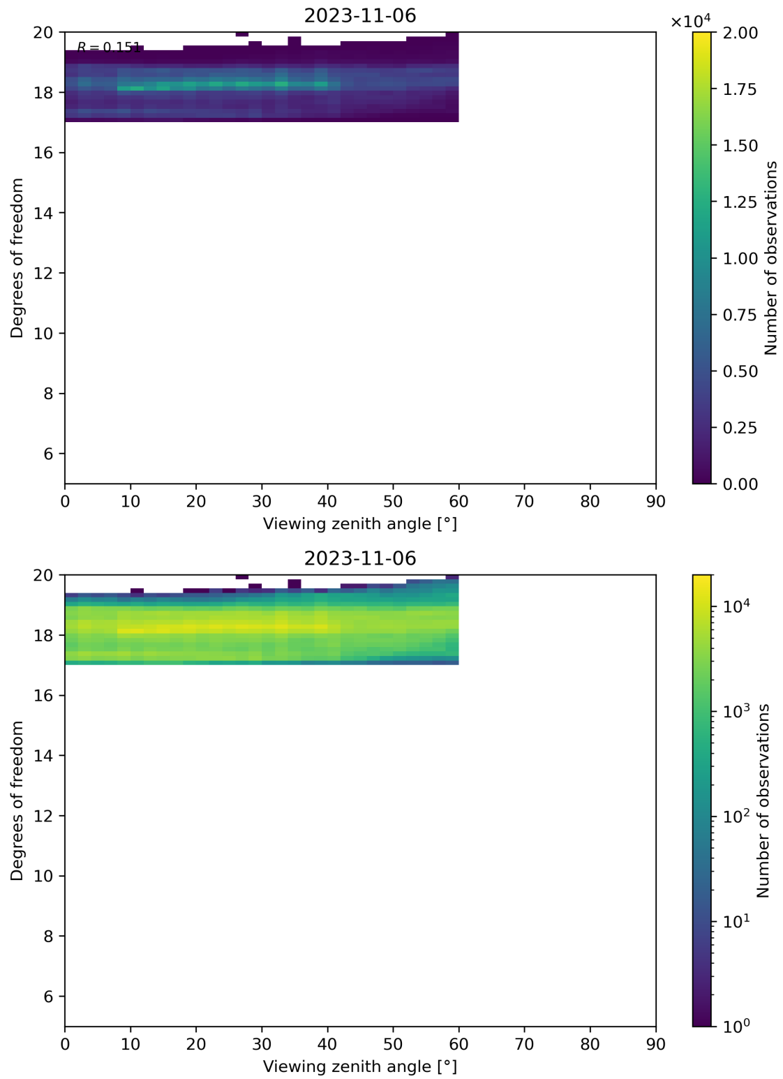
Figure 107: Scatter density plot of “Viewing zenith angle” against “Degrees of freedom” for 2023-11-05 to 2023-11-07.
