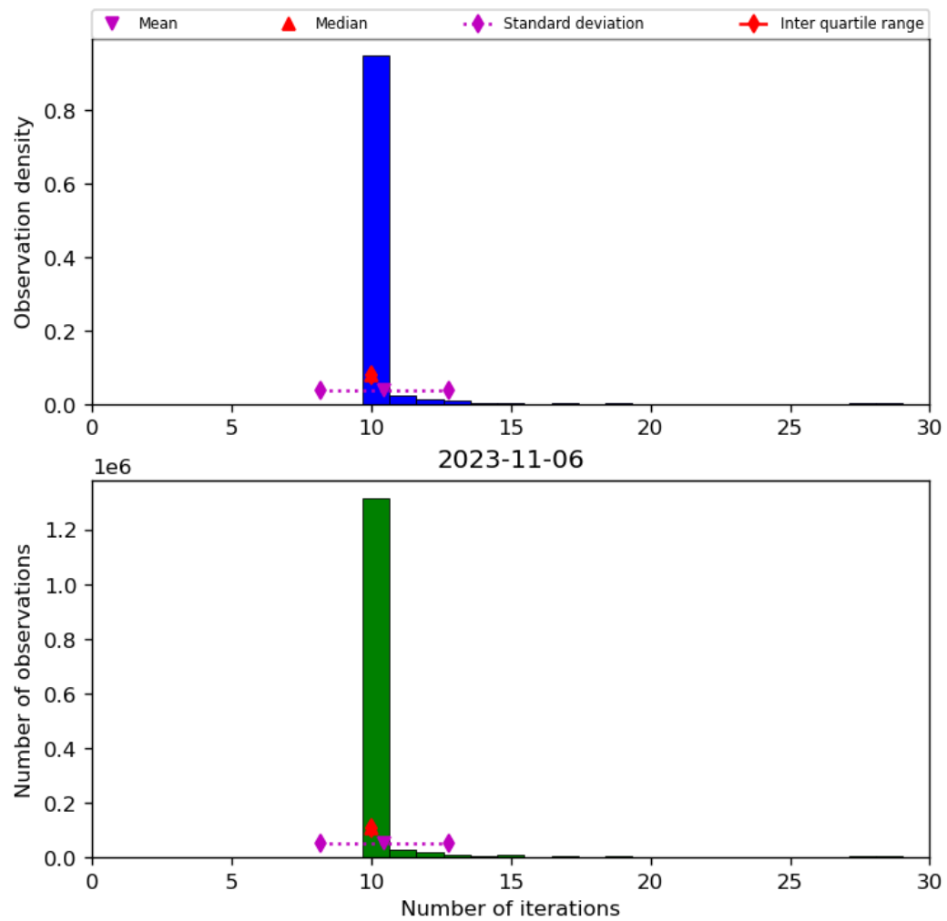
Figure 31: Histogram of “Number of iterations” for 2023-11-05 to 2023-11-07
