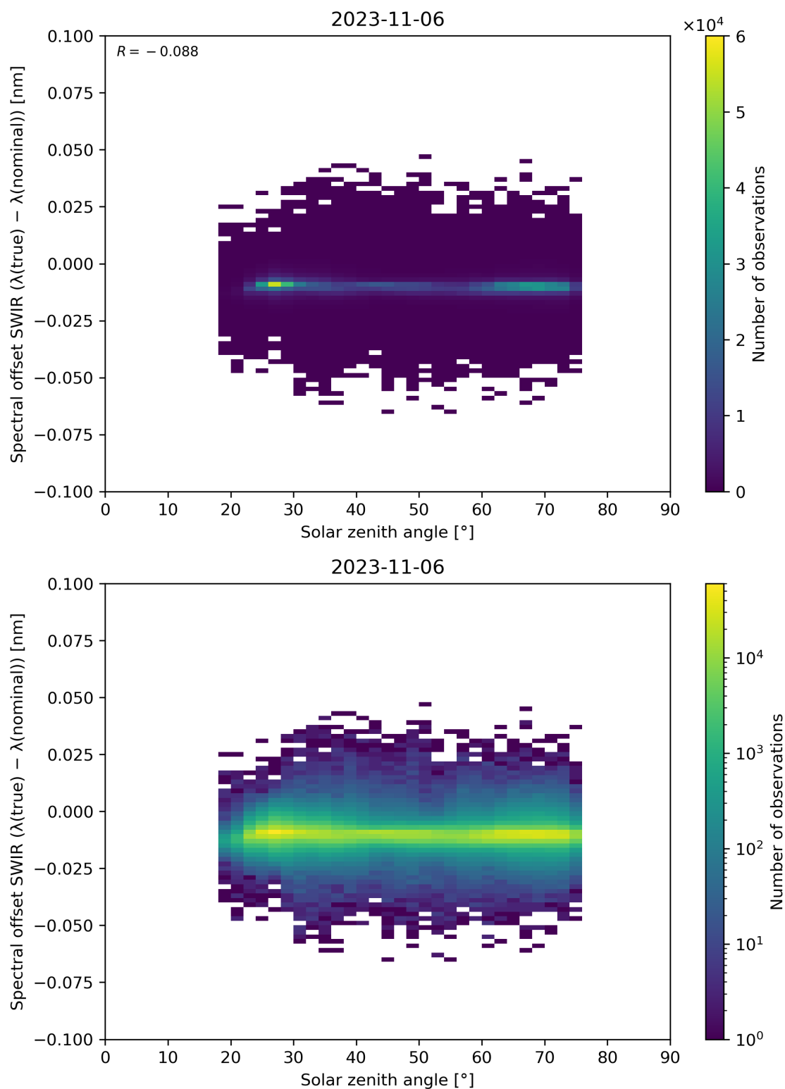
Figure 104: Scatter density plot of “Solar zenith angle” against “Spectral offset SWIR ( \lambda(\text{true}) - \lambda(\text{nominal}) )” for 2023-11-05 to 2023-11-07.
