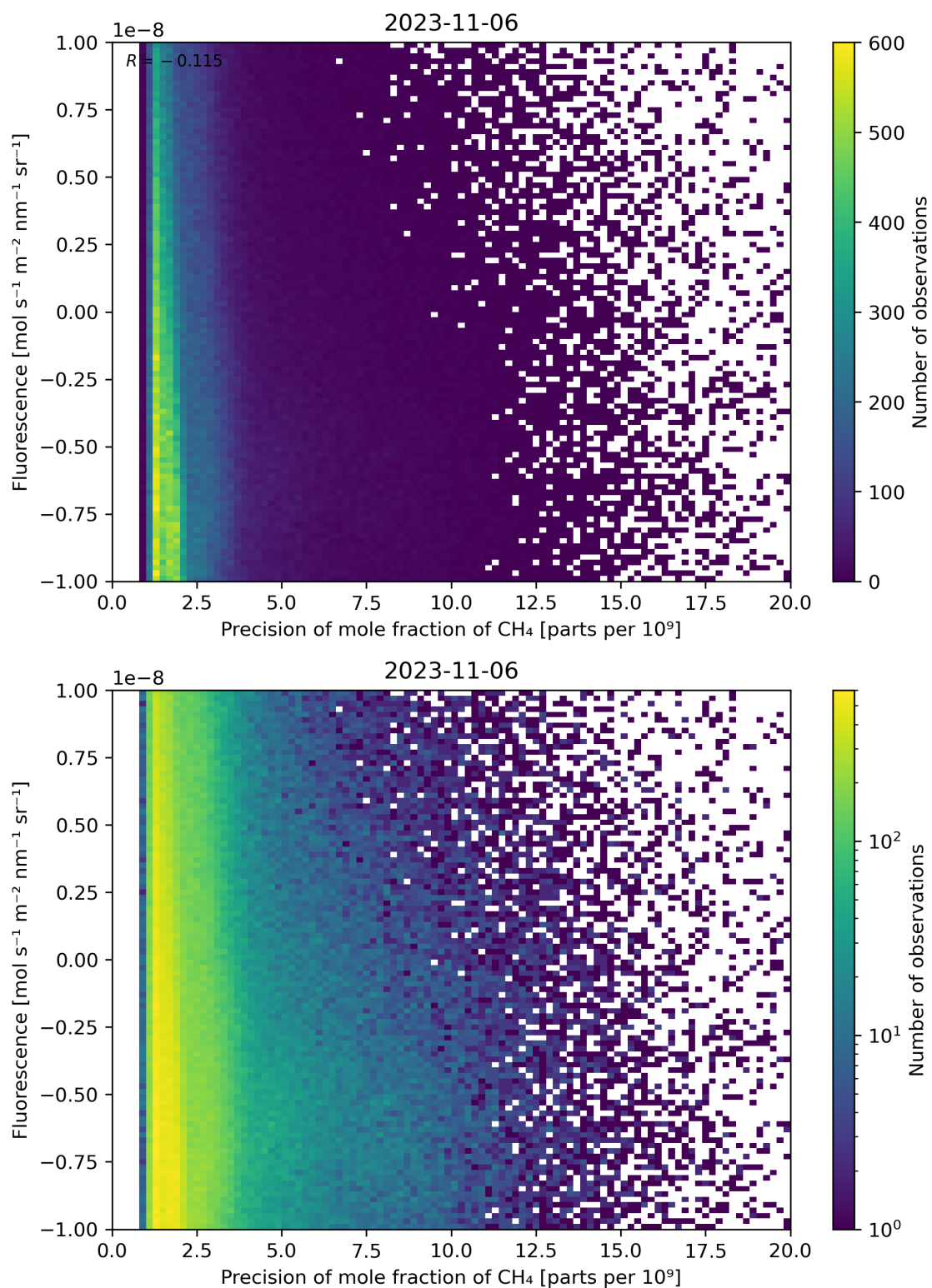
Figure 81: Scatter density plot of “Precision of mole fraction of \text{CH}_4 ” against “Fluorescence” for 2023-11-05 to 2023-11-07.
