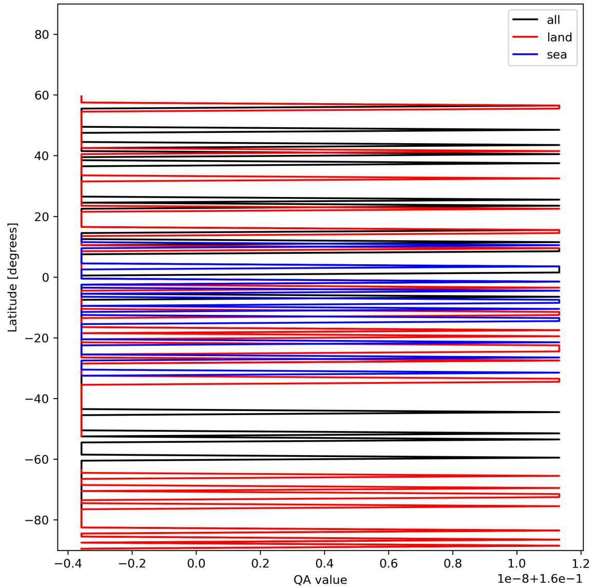
Figure 11: Zonal average of “QA value” for 2023-11-05 to 2023-11-07.
