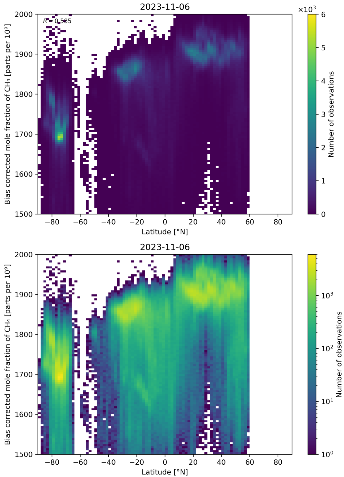
Figure 58: Scatter density plot of “Latitude” against “Bias corrected mole fraction of CH 4 ” for 2023-11-05 to 2023-11-07.
