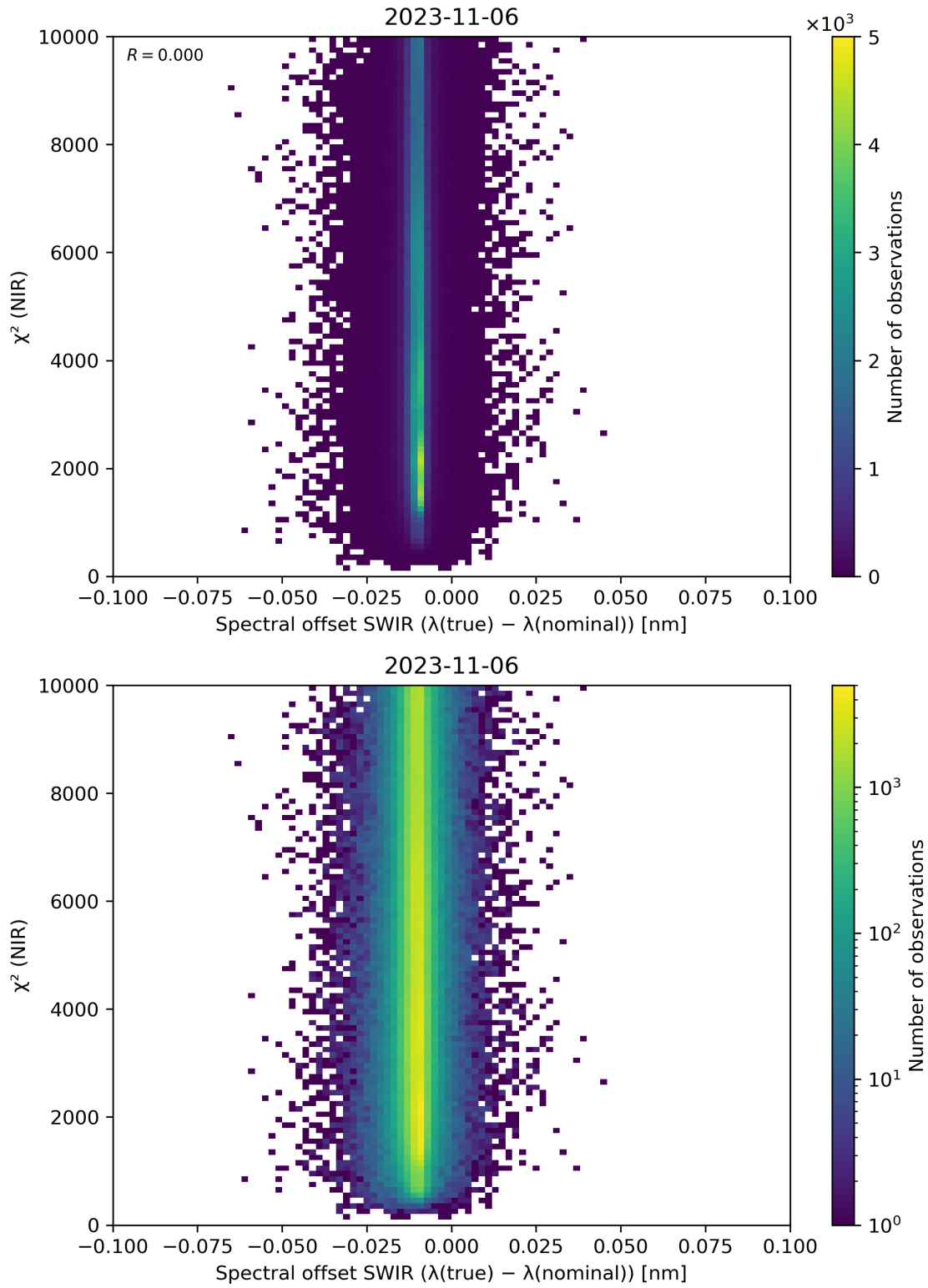
Figure 117: Scatter density plot of “Spectral offset SWIR ( \lambda(\text{true}) - \lambda(\text{nominal}) )” against “ \chi^2 (NIR)” for 2023-11-05 to 2023-11-07.
