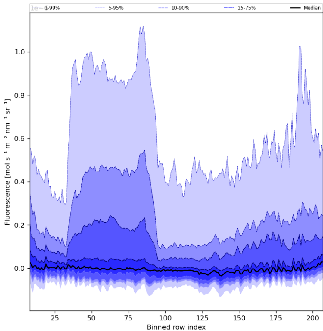
Figure 43: Along track statistics of “Fluorescence” for 2023-11-05 to 2023-11-07
