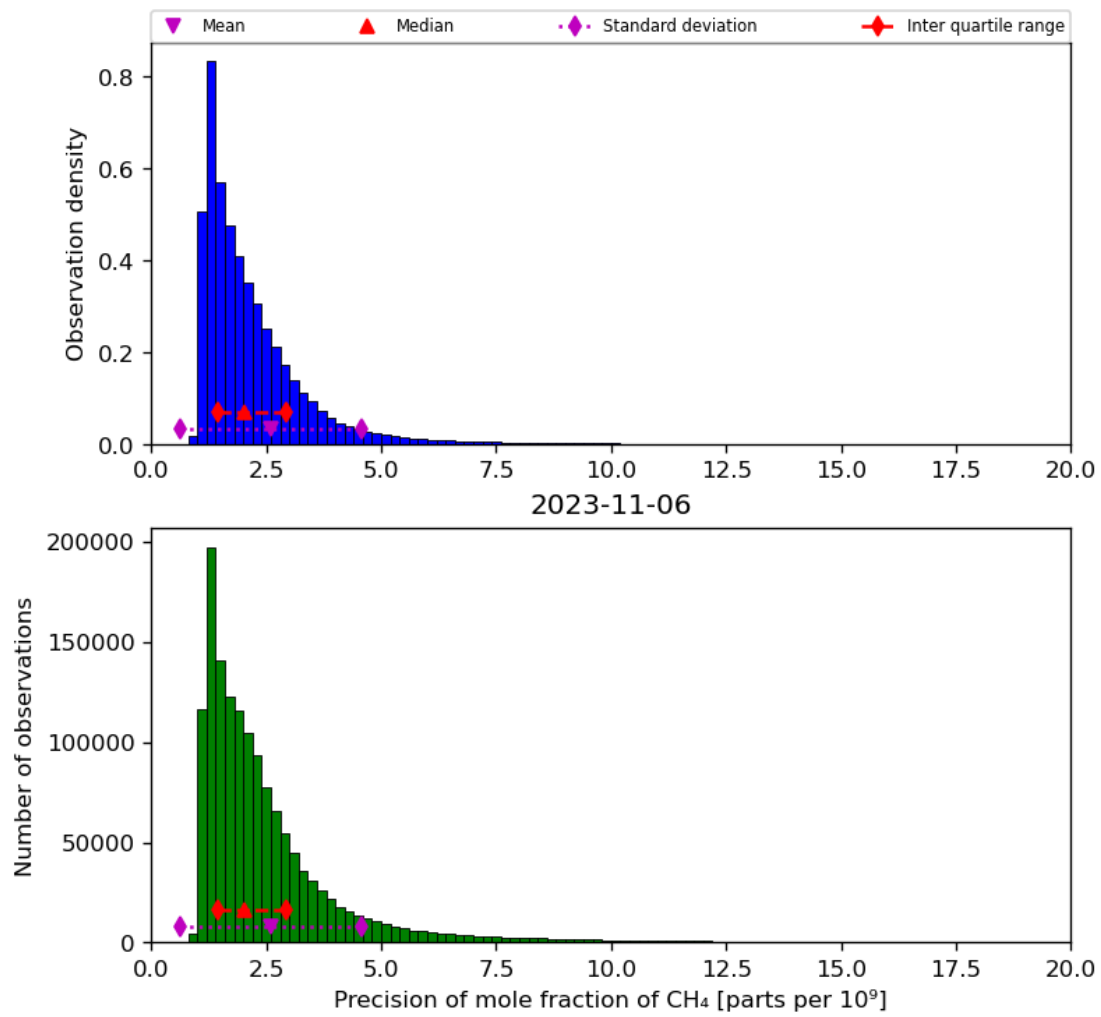
Figure 24: Histogram of “Precision of mole fraction of CH 4 ” for 2023-11-05 to 2023-11-07
