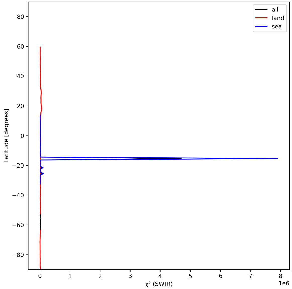
Figure 17: Zonal average of “ \chi^2 (SWIR)” for 2023-11-05 to 2023-11-07.
