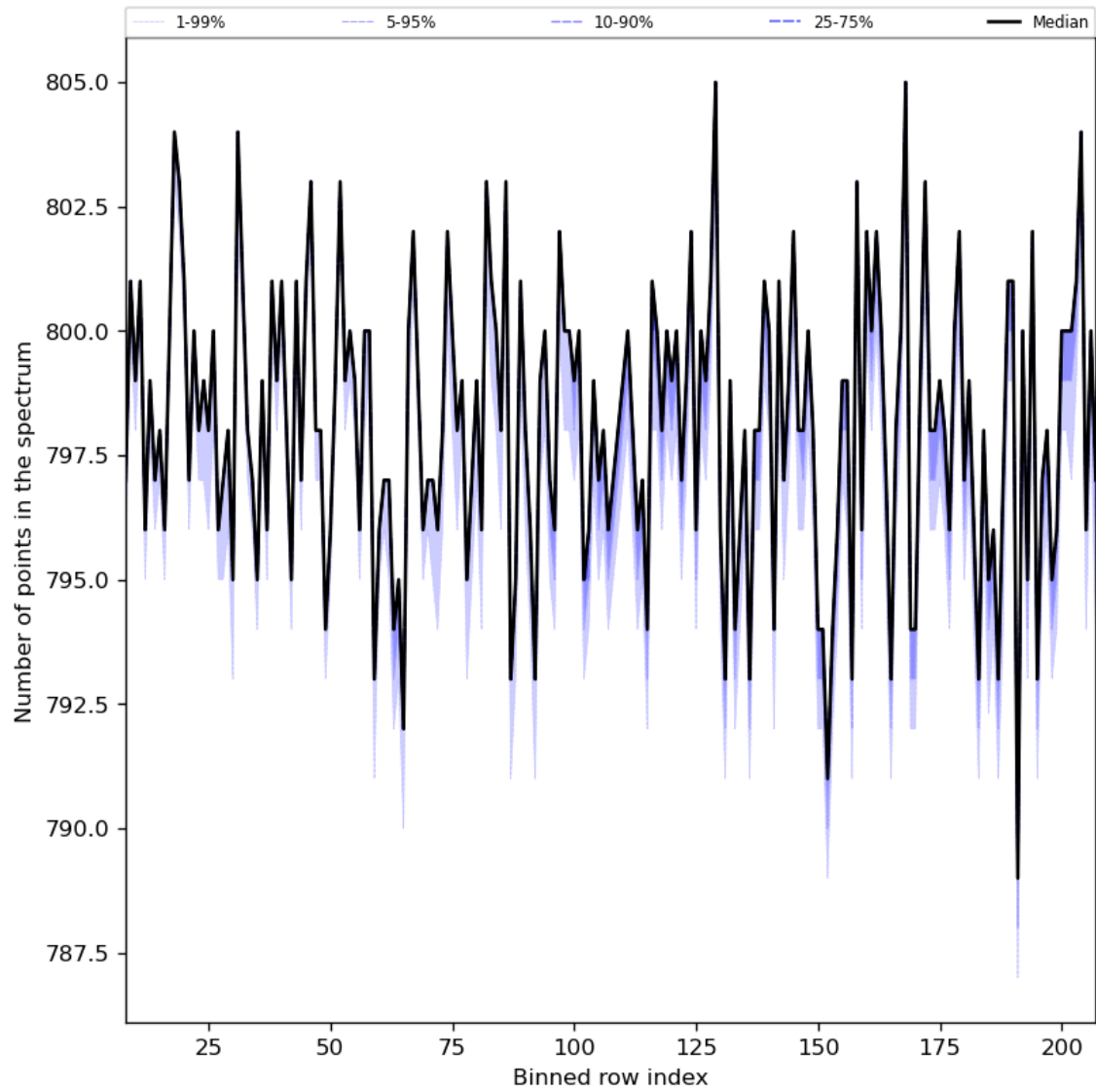
Figure 37: Along track statistics of “Number of points in the spectrum” for 2023-11-05 to 2023-11-07
