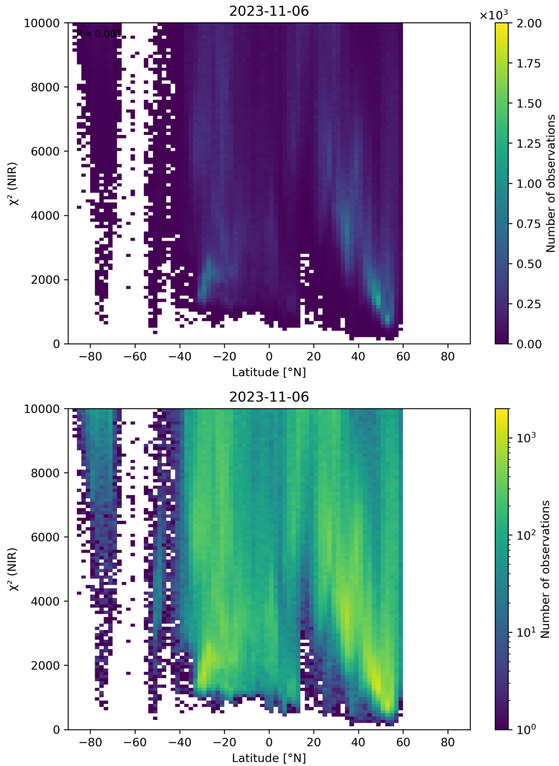
Figure 53: Scatter density plot of “Latitude” against “ \chi^2 (NIR)” for 2023-11-05 to 2023-11-07.
