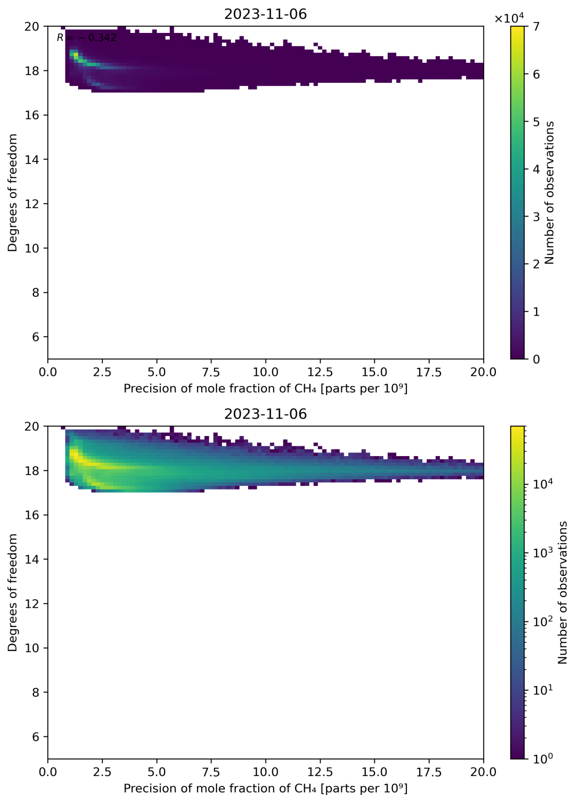
Figure 80: Scatter density plot of “Precision of mole fraction of CH 4 ” against “Degrees of freedom” for 2023-11-05 to 2023-11-07.
