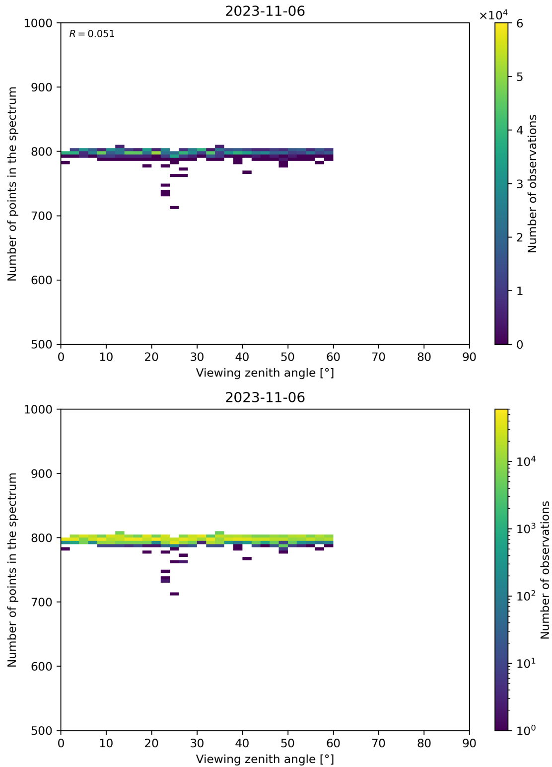
Figure 114: Scatter density plot of “Viewing zenith angle” against “Number of points in the spectrum” for 2023-11-05 to 2023-11-07.
