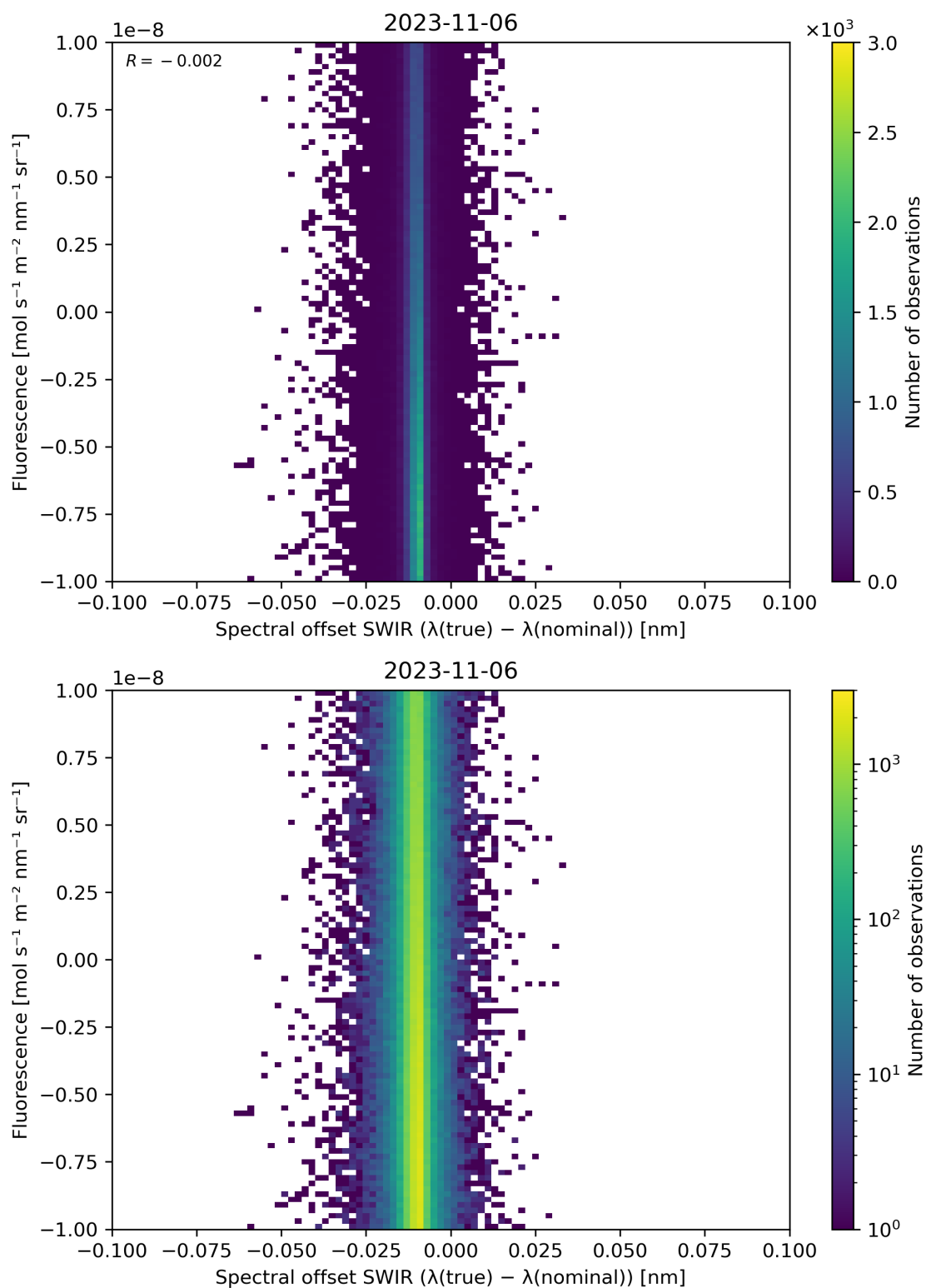
Figure 120: Scatter density plot of “Spectral offset SWIR ( \lambda(\text{true}) - \lambda(\text{nominal}) )” against “Fluorescence” for 2023-11-05 to 2023-11-07.
