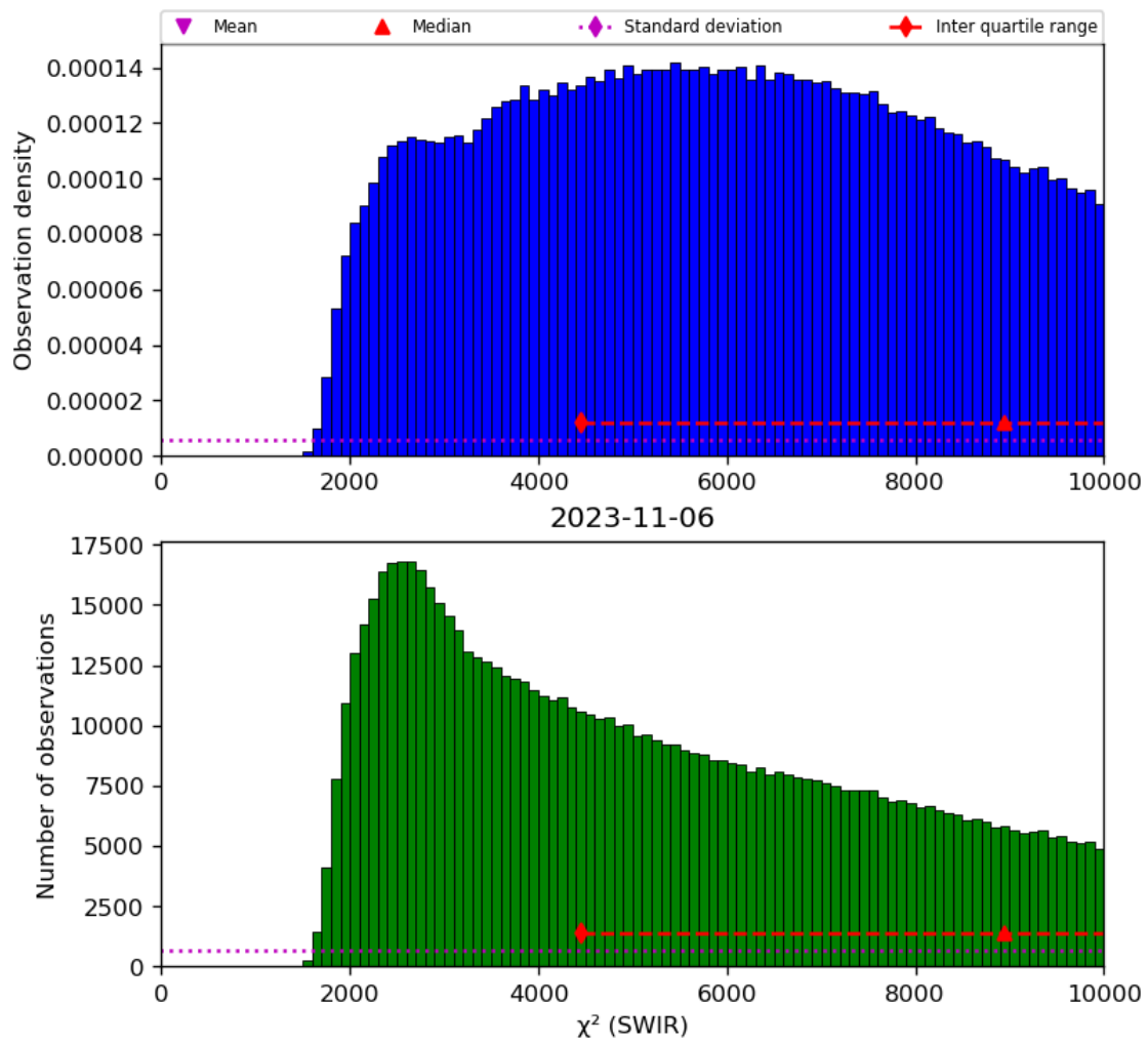
Figure 28: Histogram of “ \chi^2 (SWIR)” for 2023-11-05 to 2023-11-07
