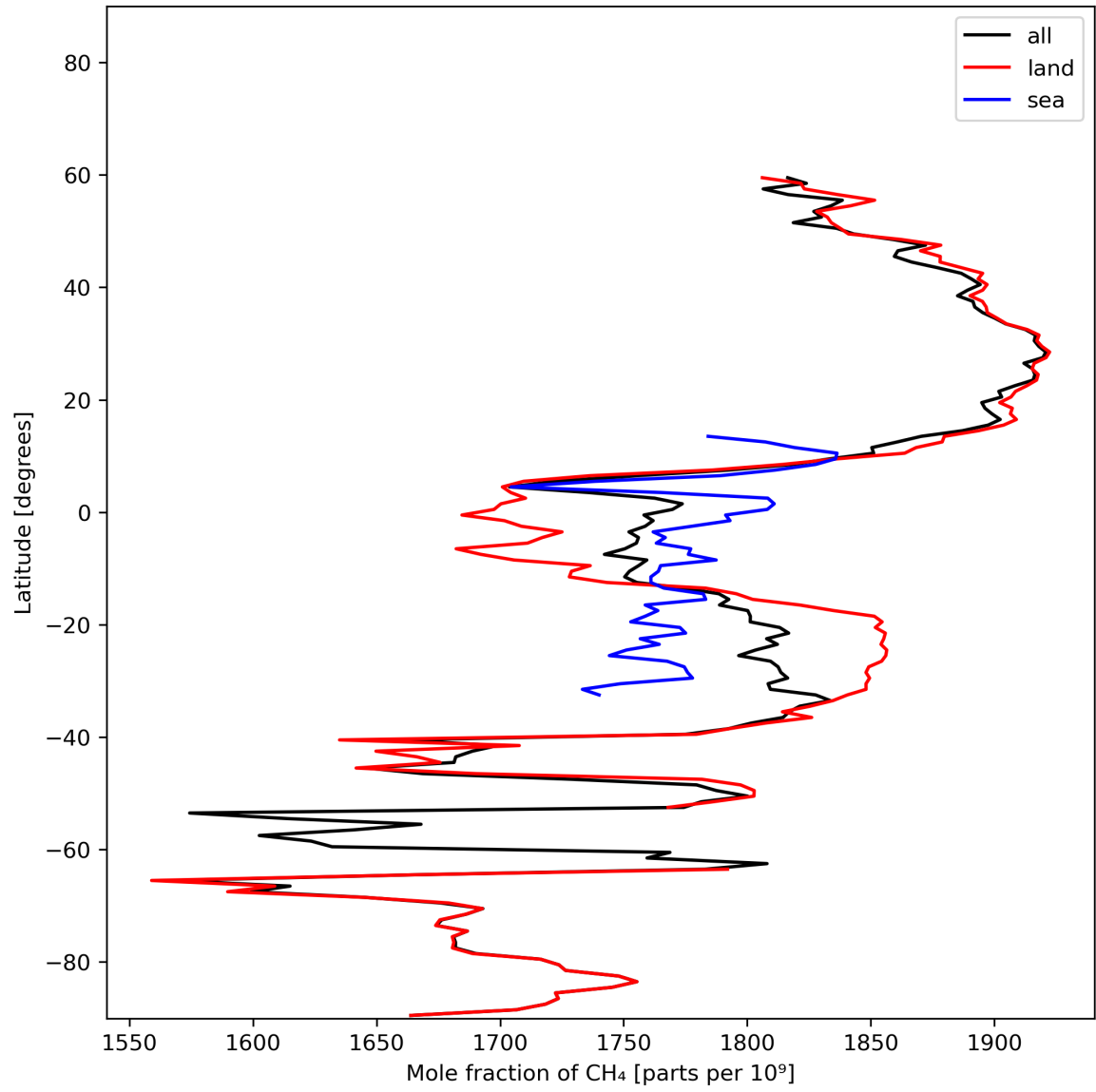
Figure 12: Zonal average of “Mole fraction of \text{CH}_4 ” for 2023-11-05 to 2023-11-07.
