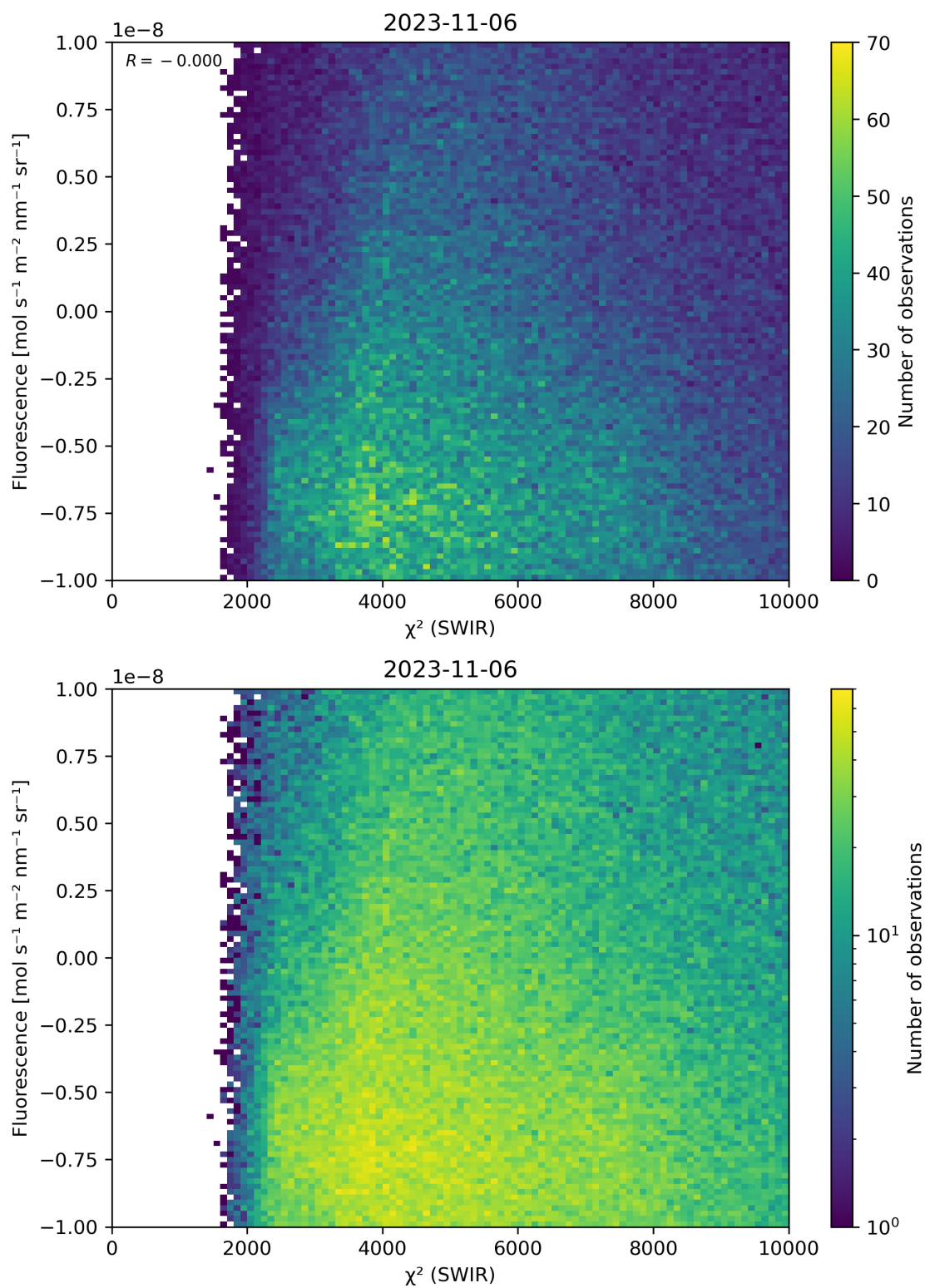
Figure 49: Scatter density plot of “ \chi^2 (SWIR)” against “Fluorescence” for 2023-11-05 to 2023-11-07.
