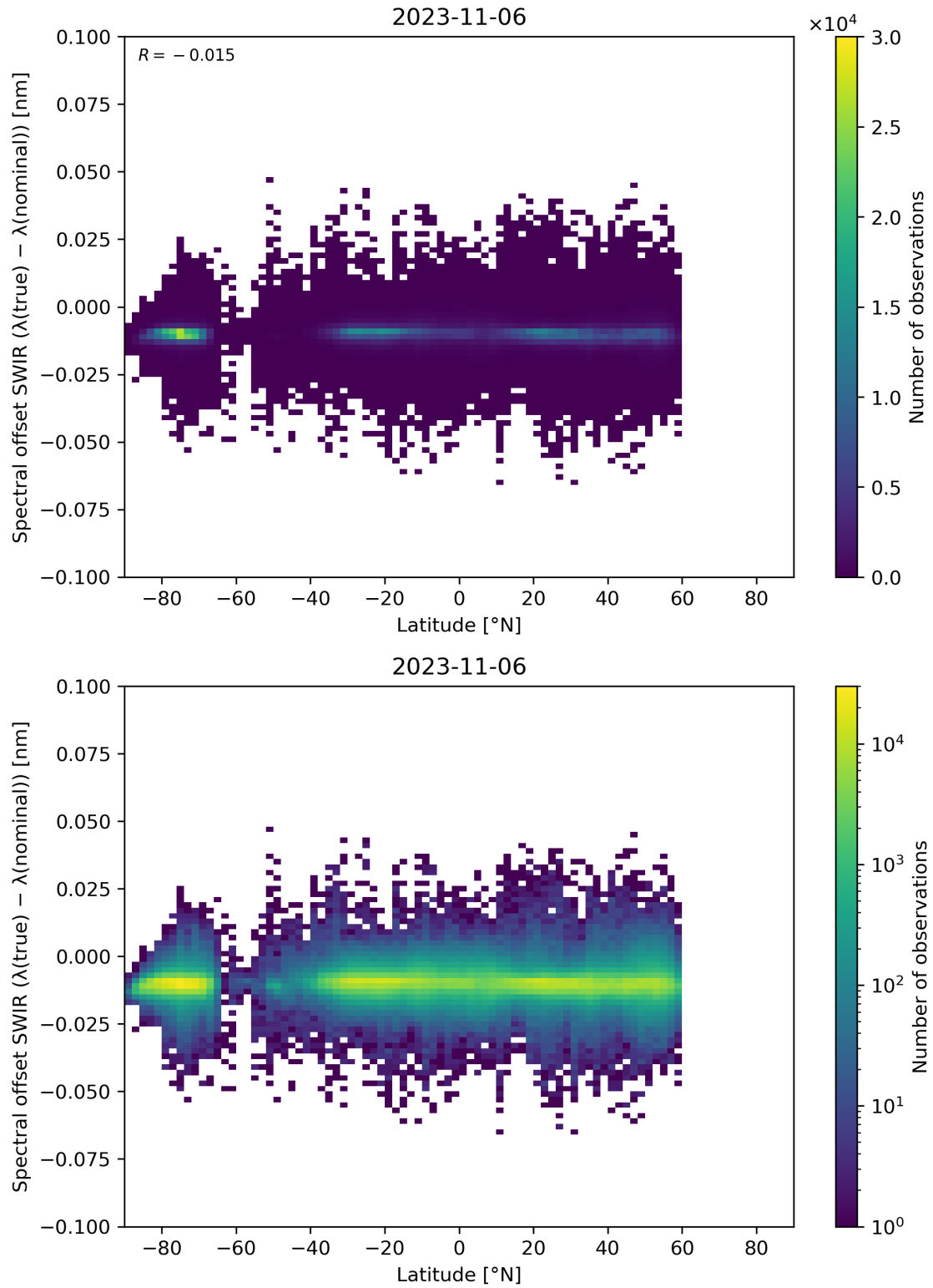
Figure 62: Scatter density plot of “Latitude” against “Spectral offset SWIR ( \lambda(\text{true}) - \lambda(\text{nominal}) )” for 2023-11-05 to 2023-11-07.
