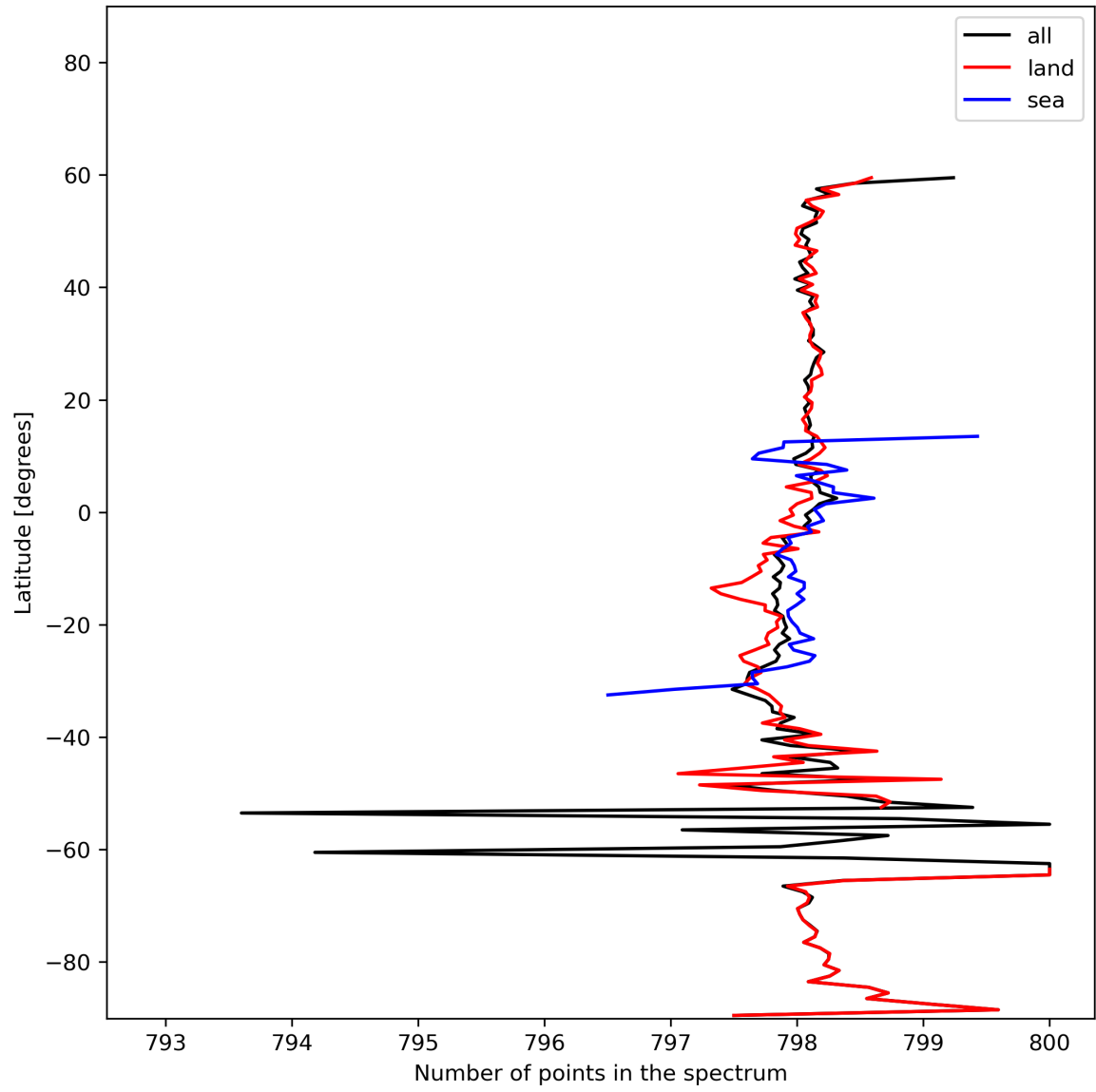
Figure 15: Zonal average of “Number of points in the spectrum” for 2023-11-05 to 2023-11-07.
