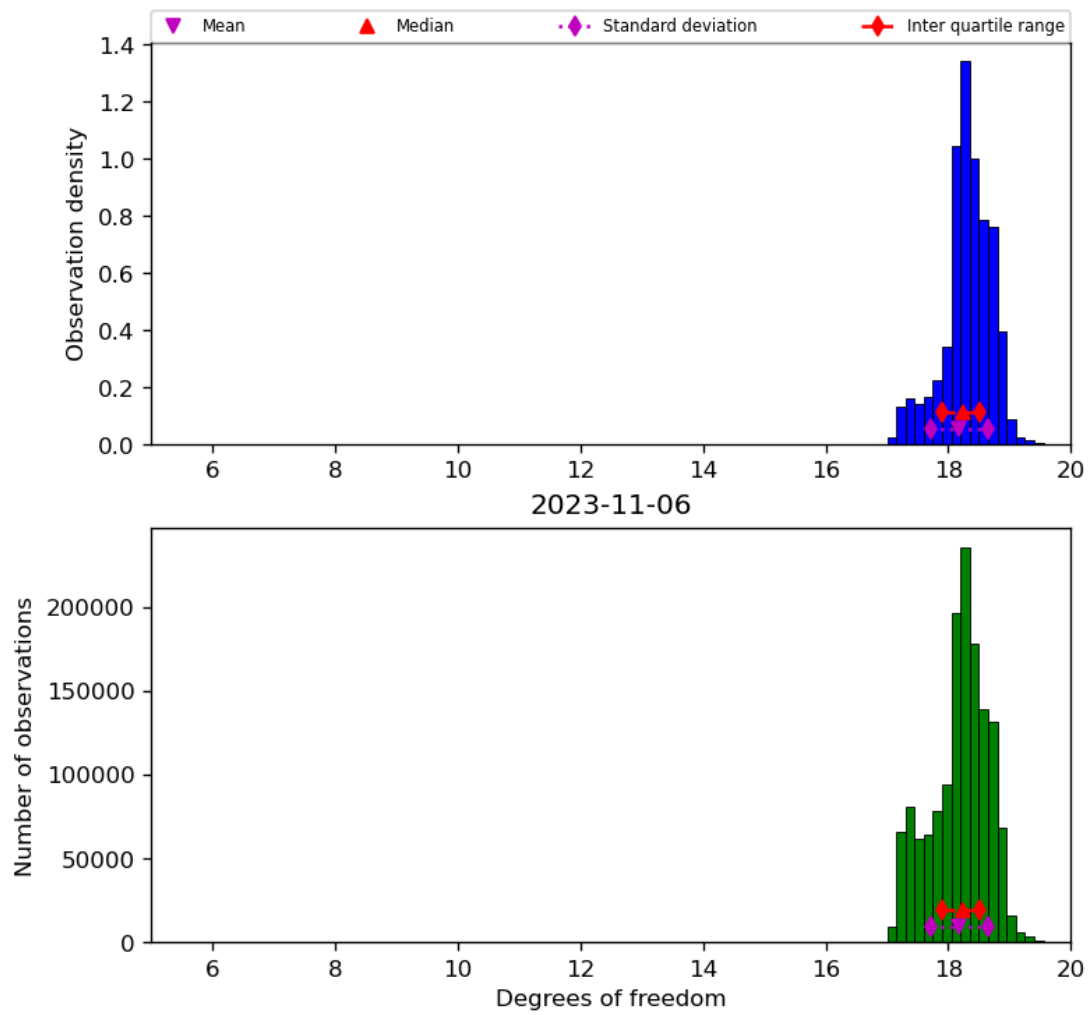
Figure 30: Histogram of “Degrees of freedom” for 2023-11-05 to 2023-11-07
