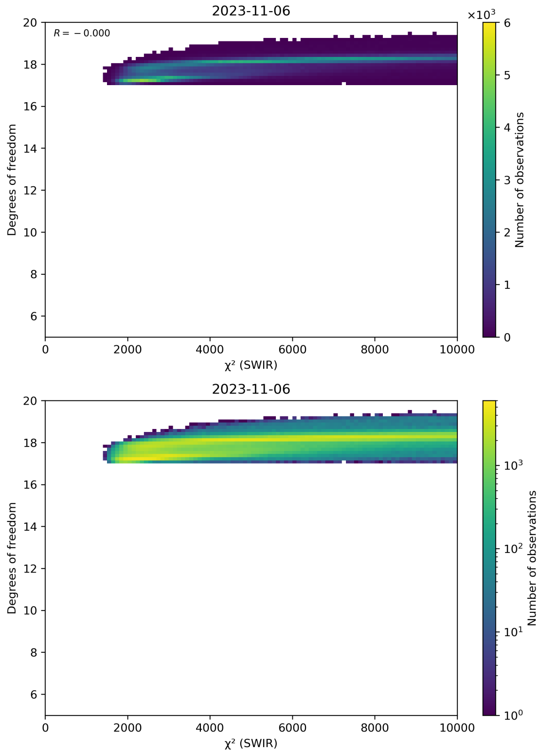
Figure 48: Scatter density plot of “ \chi^2 (SWIR)” against “Degrees of freedom” for 2023-11-05 to 2023-11-07.
