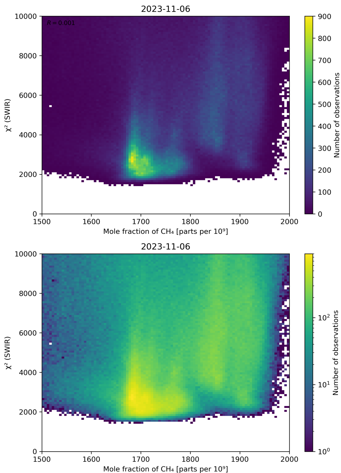
Figure 71: Scatter density plot of “Mole fraction of CH 4 ” against “ \chi^2 (SWIR)” for 2023-11-05 to 2023-11-07.
