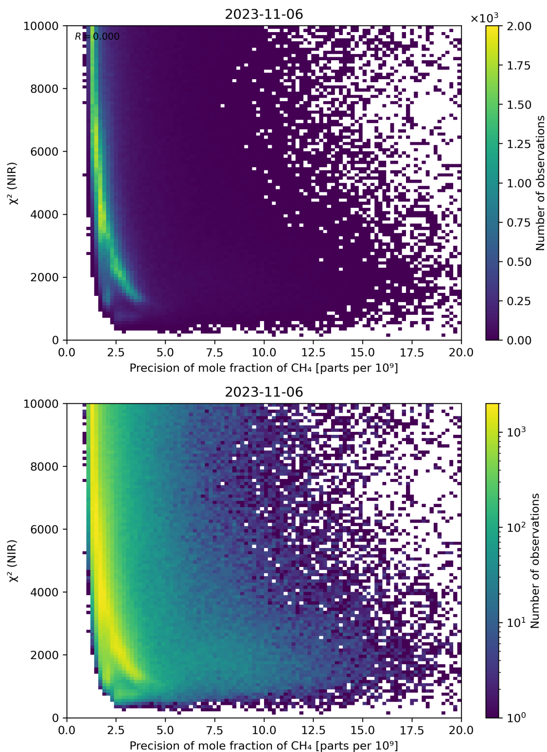
Figure 78: Scatter density plot of “Precision of mole fraction of \text{CH}_4 ” against “ \chi^2 (NIR)” for 2023-11-05 to 2023-11-07.
