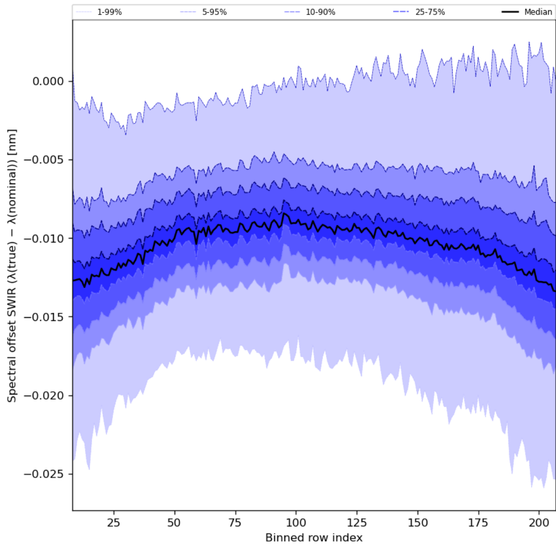
Figure 38: Along track statistics of “Spectral offset SWIR ( \lambda(\text{true}) - \lambda(\text{nominal}) )” for 2023-11-05 to 2023-11-07
