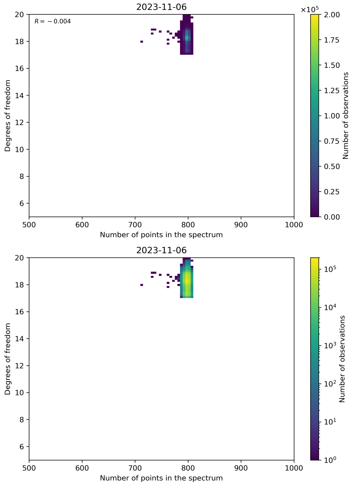
Figure 90: Scatter density plot of “Number of points in the spectrum” against “Degrees of freedom” for 2023-11-05 to 2023-11-07.
