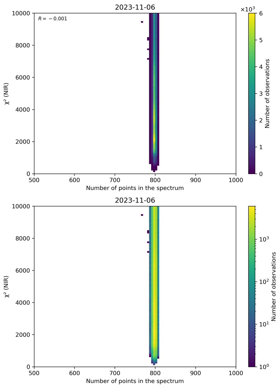
Figure 88: Scatter density plot of “Number of points in the spectrum” against “ \chi^2 (NIR)” for 2023-11-05 to 2023-11-07.
