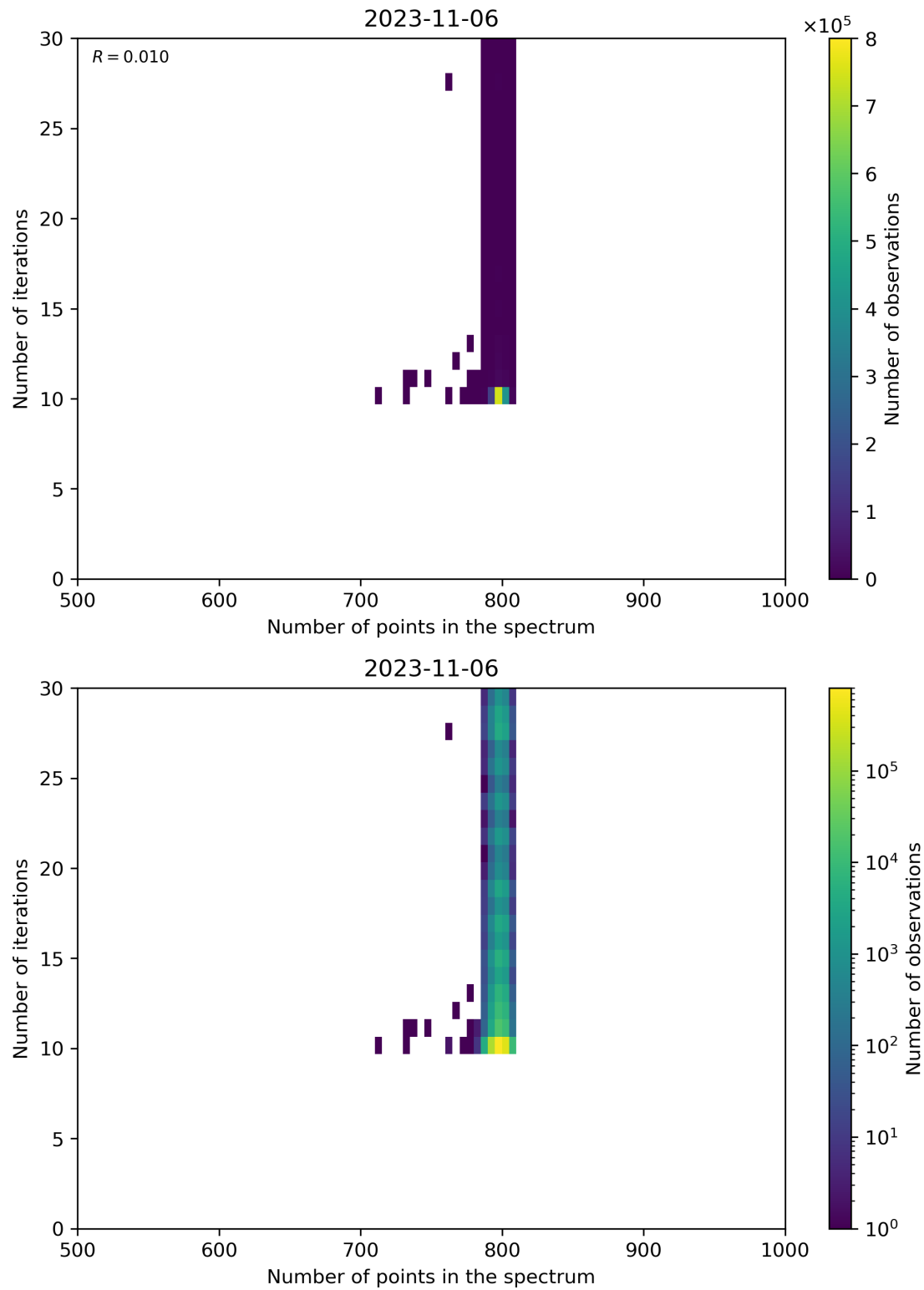
Figure 92: Scatter density plot of “Number of points in the spectrum” against “Number of iterations” for 2023-11-05 to 2023-11-07.
