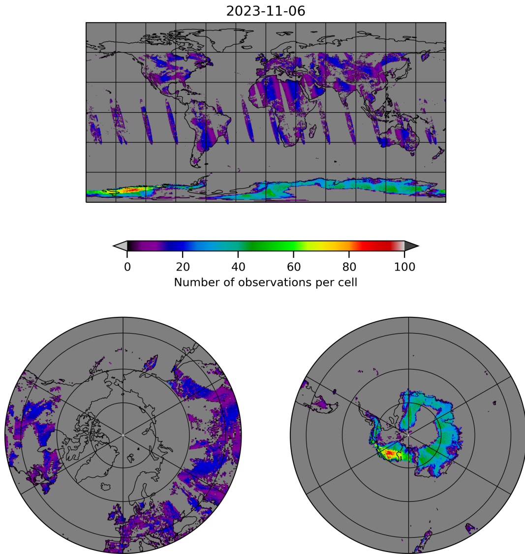
Figure 10: Map of the number of observations for 2023-11-05 to 2023-11-07
