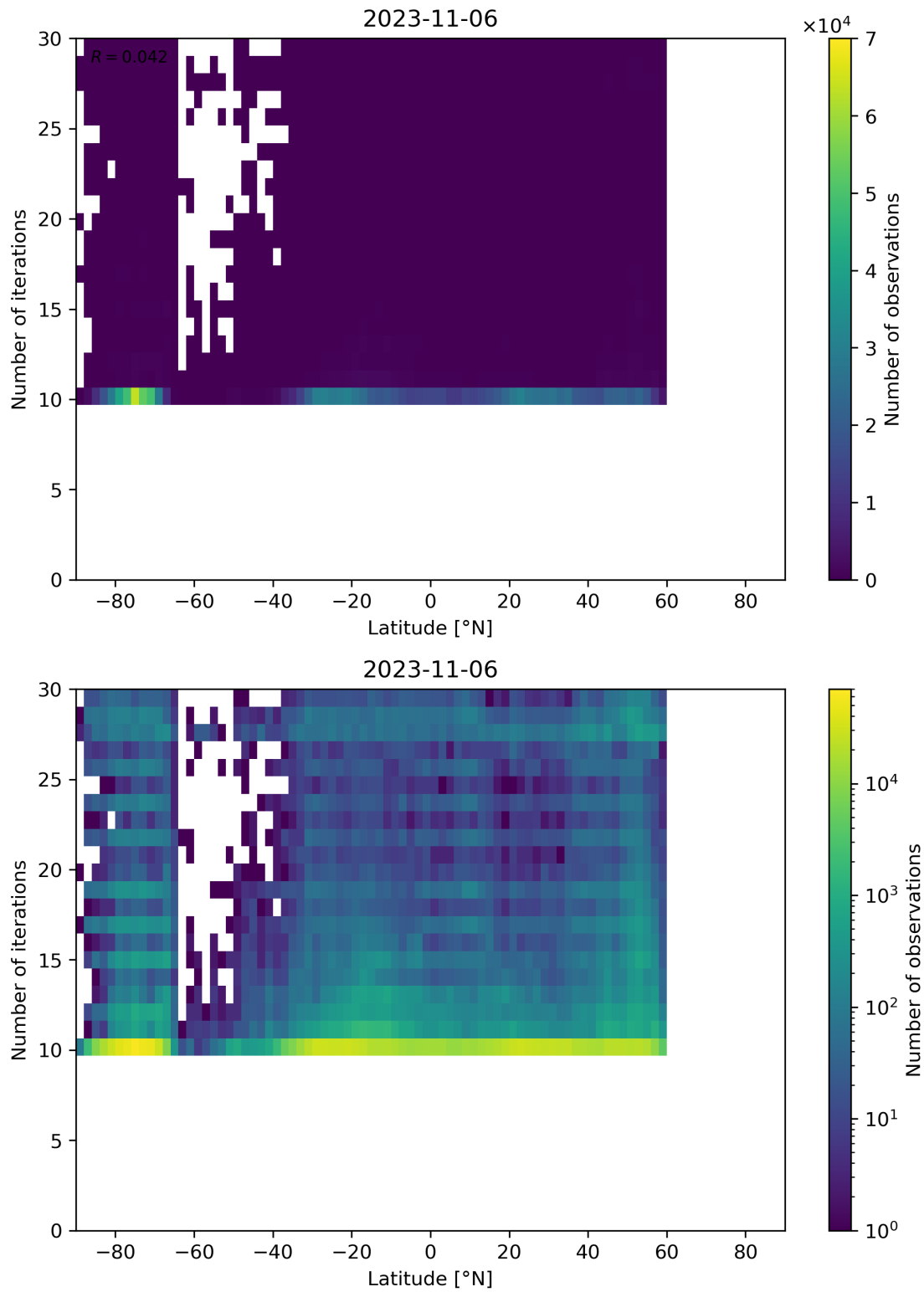
Figure 60: Scatter density plot of “Latitude” against “Number of iterations” for 2023-11-05 to 2023-11-07.
