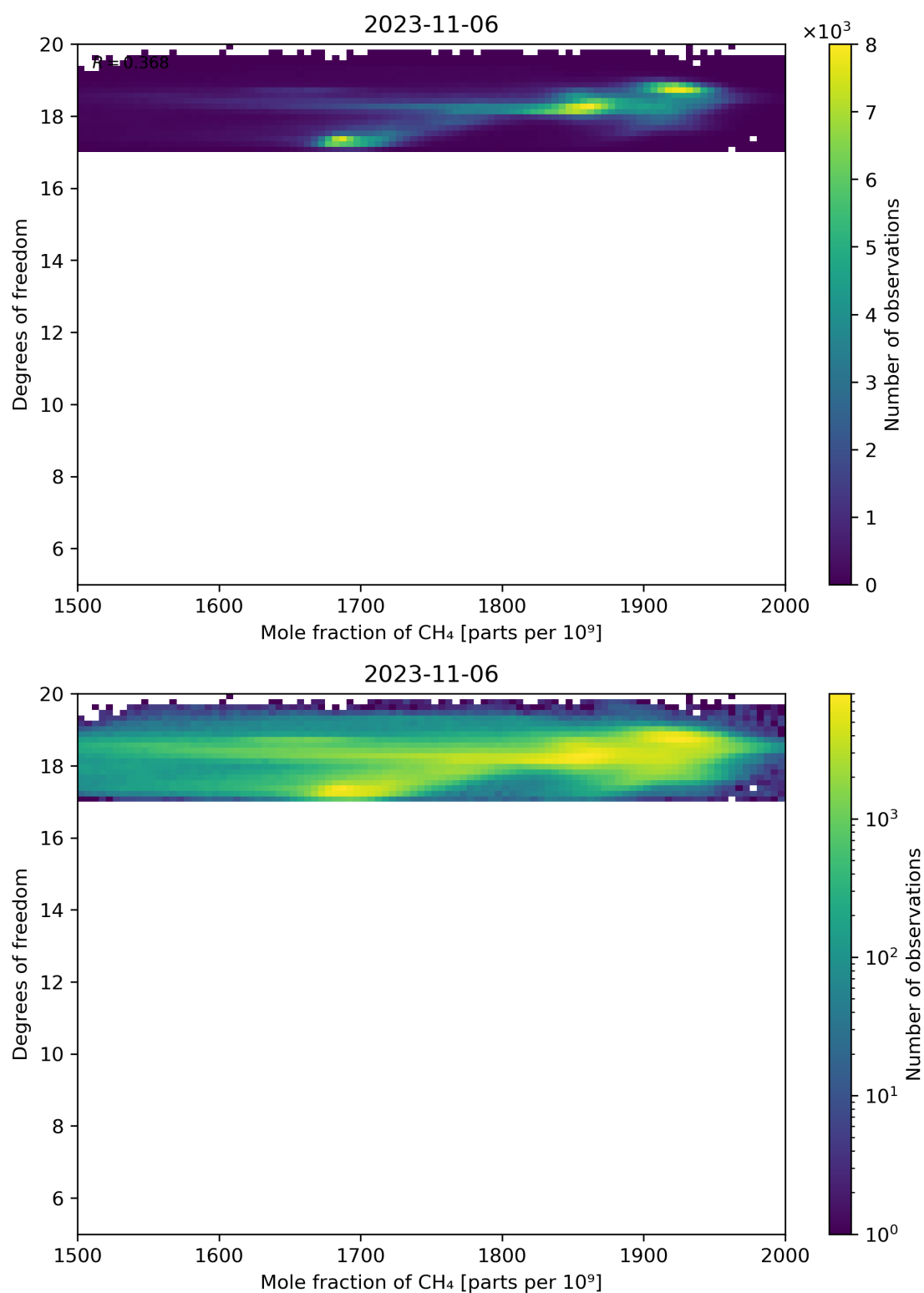
Figure 72: Scatter density plot of “Mole fraction of CH 4 ” against “Degrees of freedom” for 2023-11-05 to 2023-11-07.
