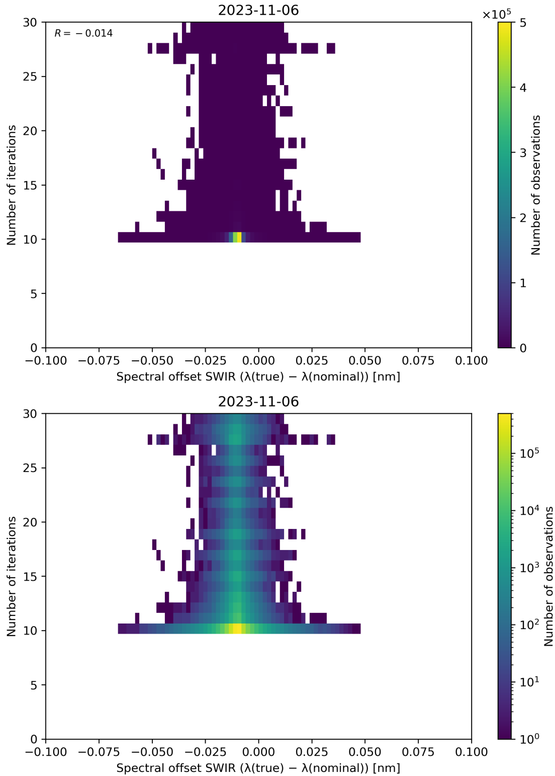
Figure 121: Scatter density plot of “Spectral offset SWIR ( \lambda(\text{true}) - \lambda(\text{nominal}) )” against “Number of iterations” for 2023-11-05 to 2023-11-07.
