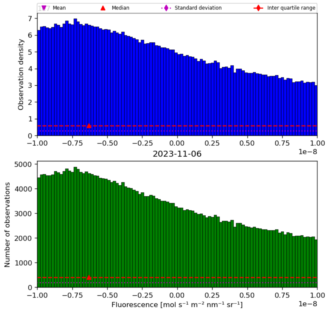
Figure 32: Histogram of “Fluorescence” for 2023-11-05 to 2023-11-07
