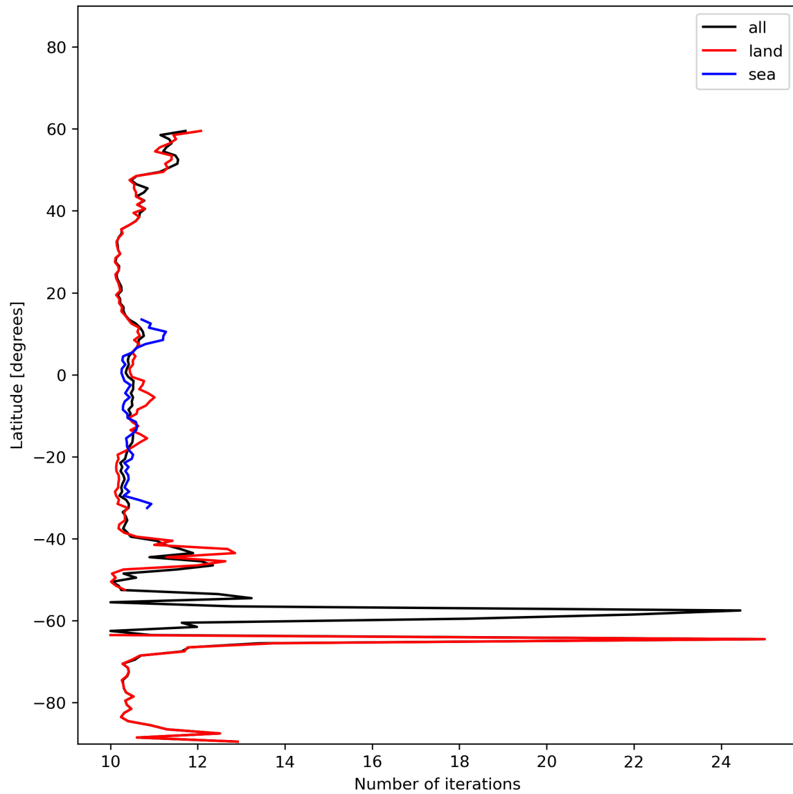
Figure 20: Zonal average of “Number of iterations” for 2023-11-05 to 2023-11-07.
