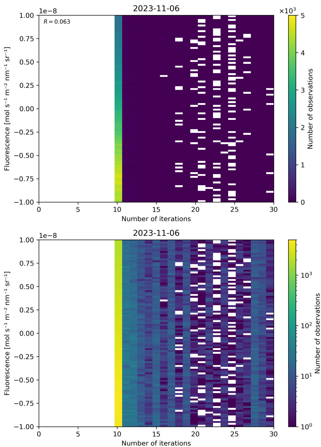
Figure 87: Scatter density plot of “Number of iterations” against “Fluorescence” for 2023-11-05 to 2023-11-07.
