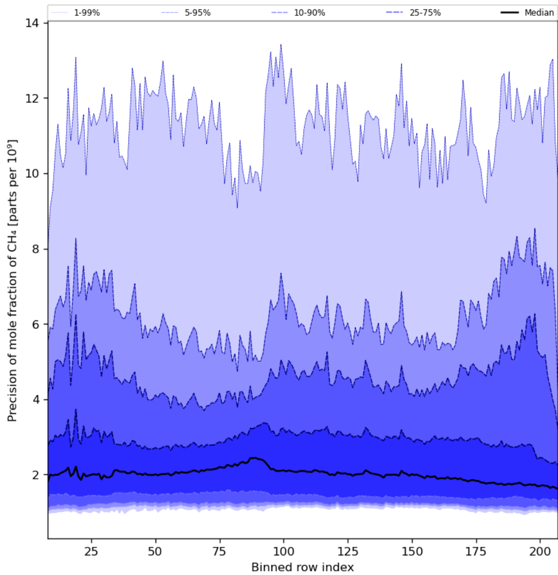
Figure 35: Along track statistics of “Precision of mole fraction of CH 4 ” for 2023-11-05 to 2023-11-07
