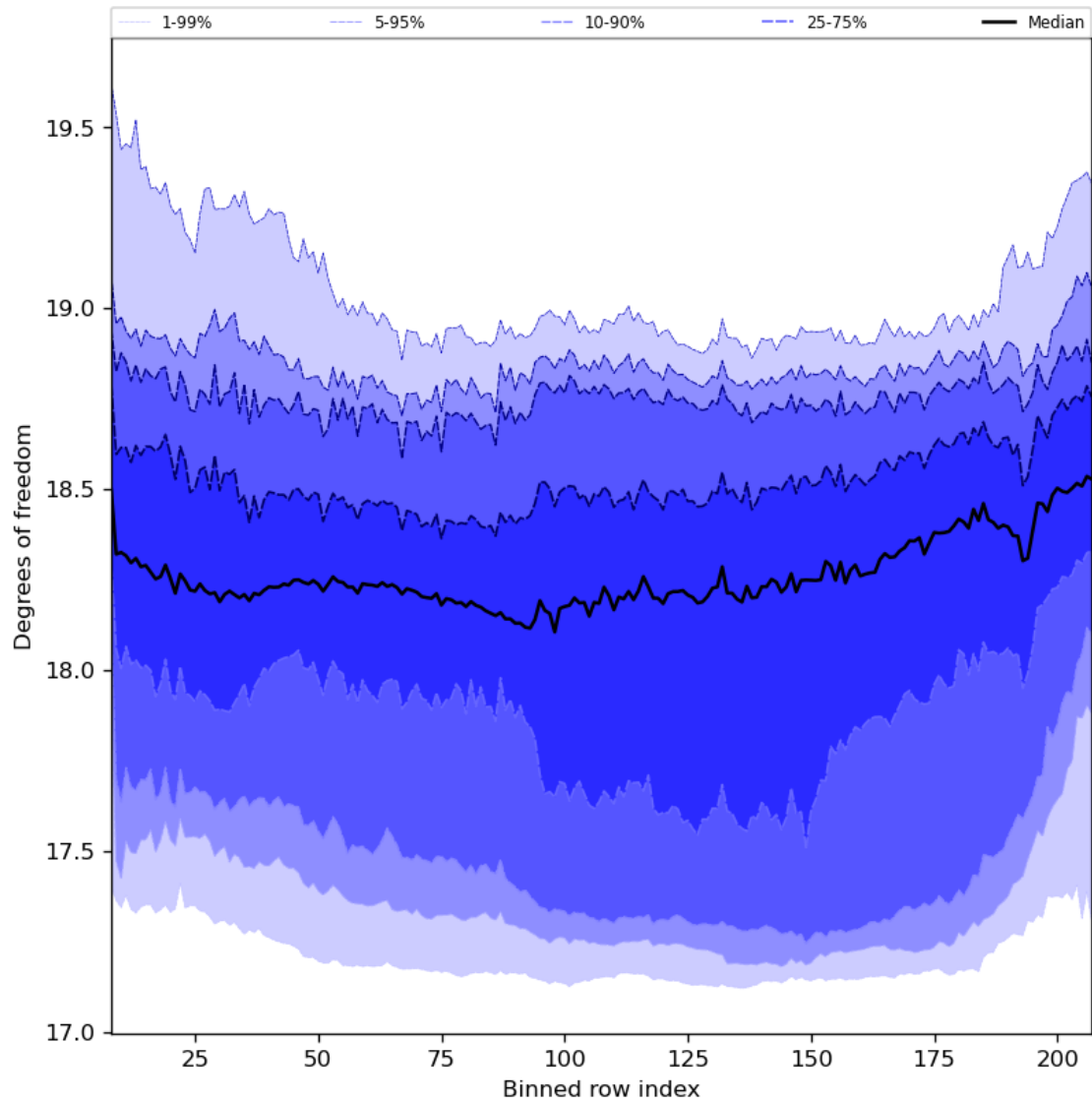
Figure 41: Along track statistics of “Degrees of freedom” for 2023-11-05 to 2023-11-07
