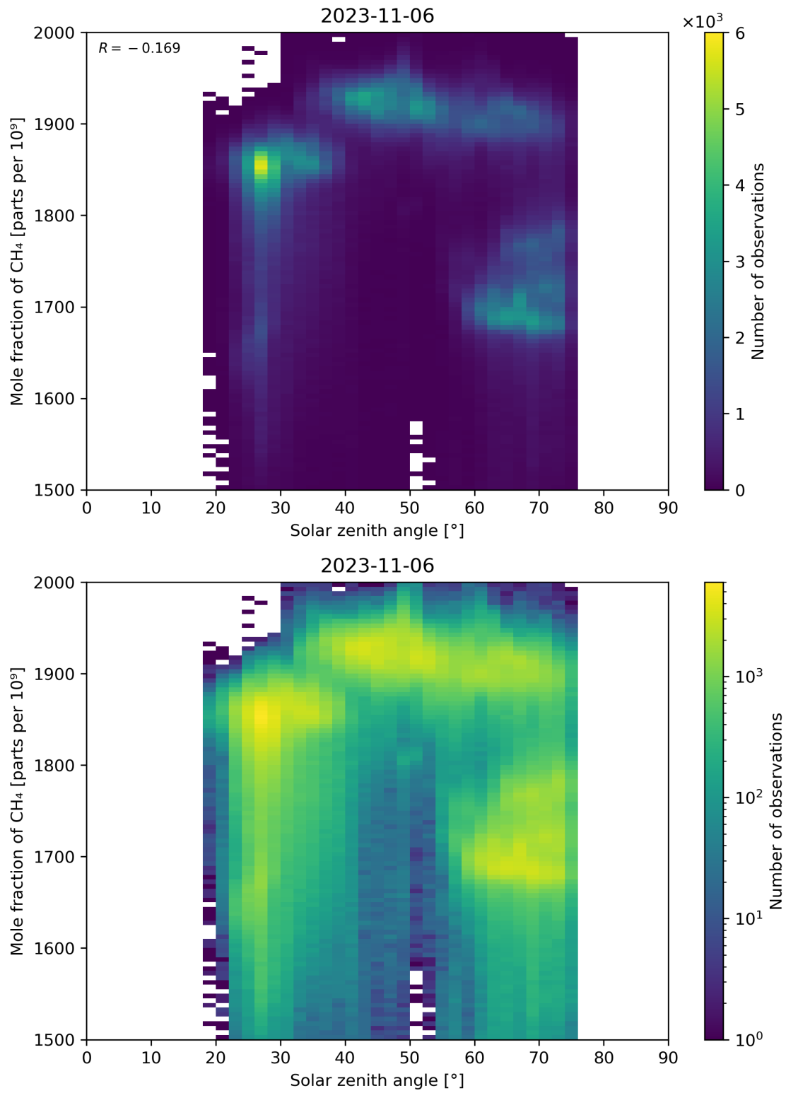
Figure 99: Scatter density plot of “Solar zenith angle” against “Mole fraction of CH 4 ” for 2023-11-05 to 2023-11-07.
