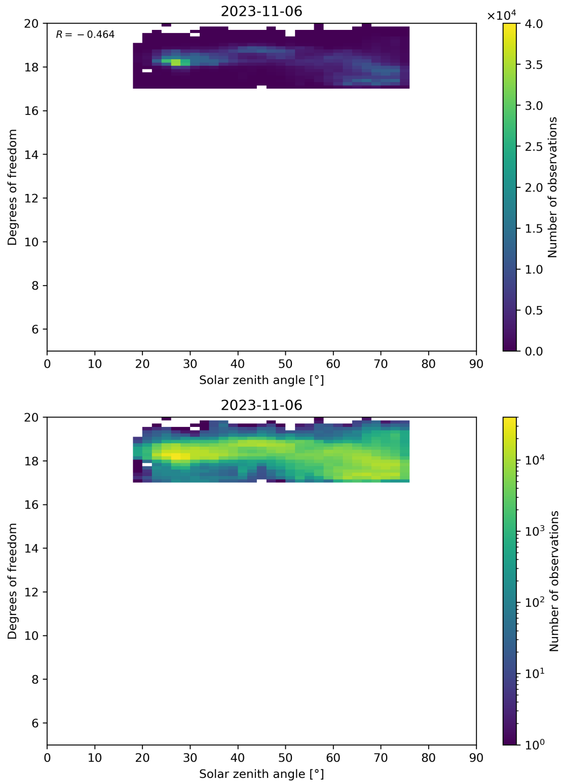
Figure 96: Scatter density plot of “Solar zenith angle” against “Degrees of freedom” for 2023-11-05 to 2023-11-07.
