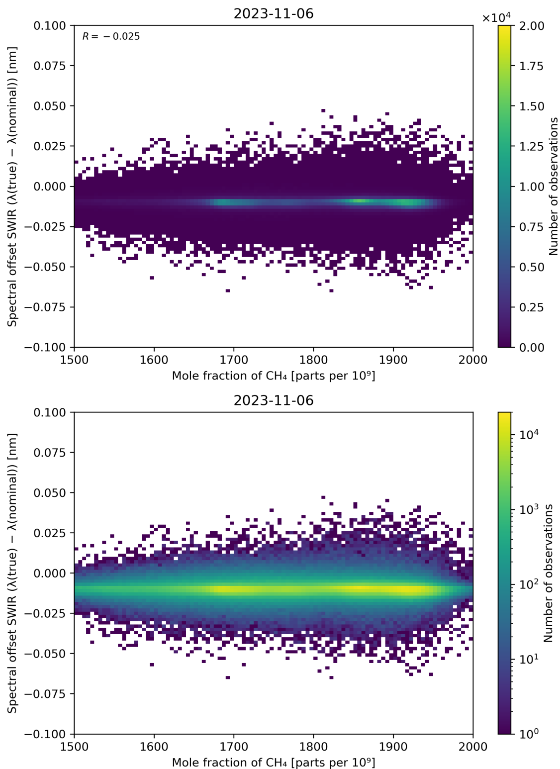
Figure 86: Scatter density plot of “Mole fraction of CH 4 ” against “Spectral offset SWIR ( \lambda(\text{true}) - \lambda(\text{nominal}) )” for 2023-11-05 to 2023-11-07.
