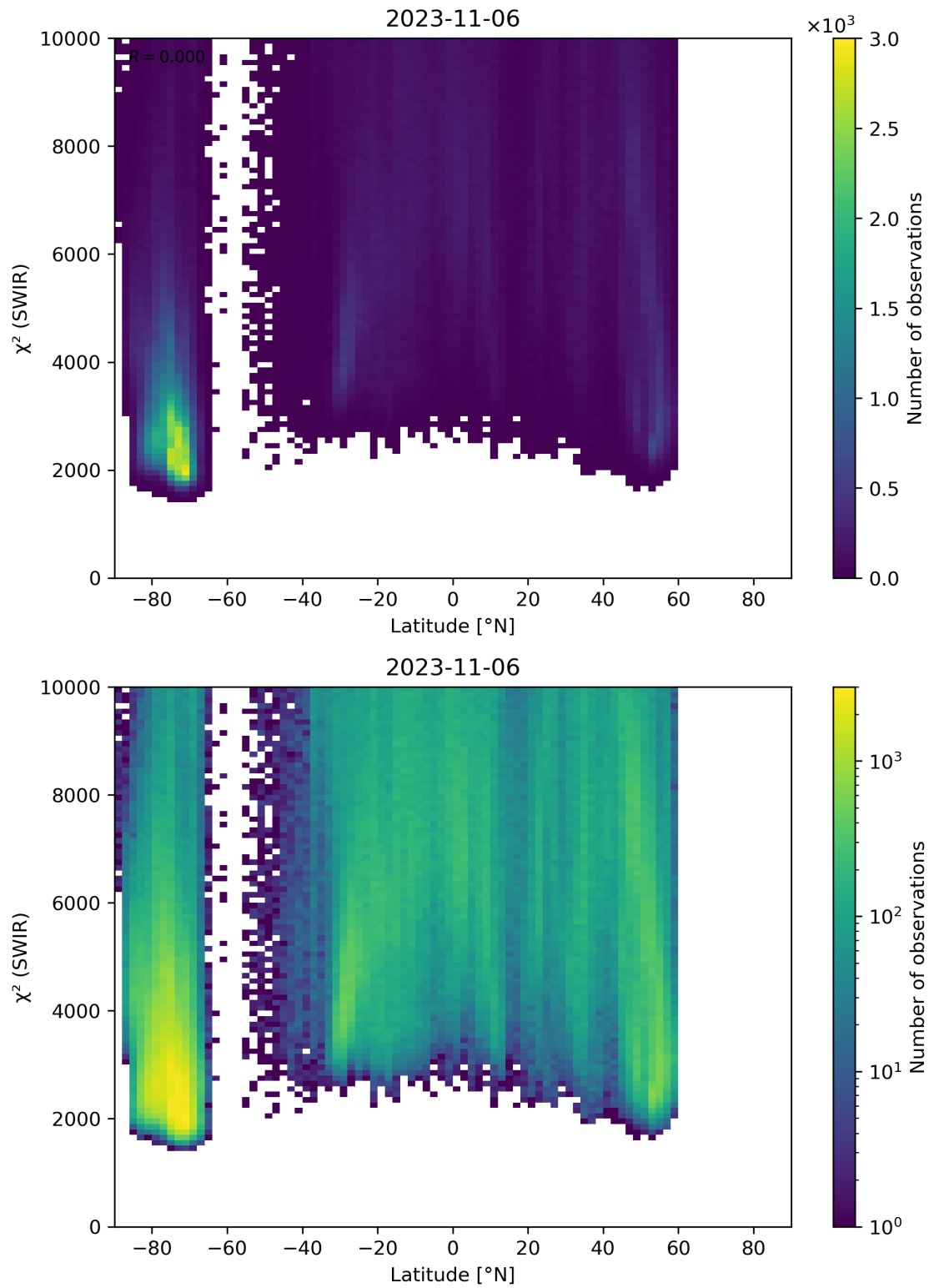
Figure 54: Scatter density plot of “Latitude” against “ \chi^2 (SWIR)” for 2023-11-05 to 2023-11-07.
