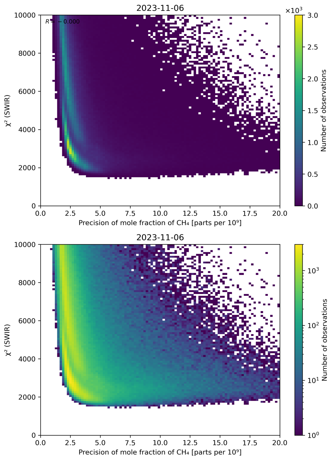
Figure 79: Scatter density plot of “Precision of mole fraction of CH 4 ” against “ \chi^2 (SWIR)” for 2023-11-05 to 2023-11-07.
