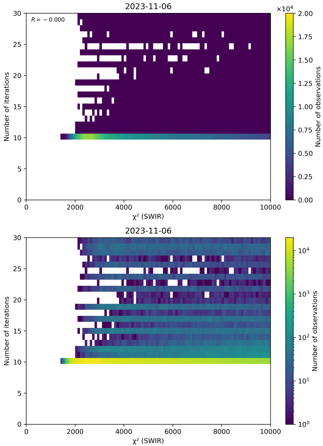
Figure 50: Scatter density plot of “ \chi^2 (SWIR)” against “Number of iterations” for 2023-11-05 to 2023-11-07.
