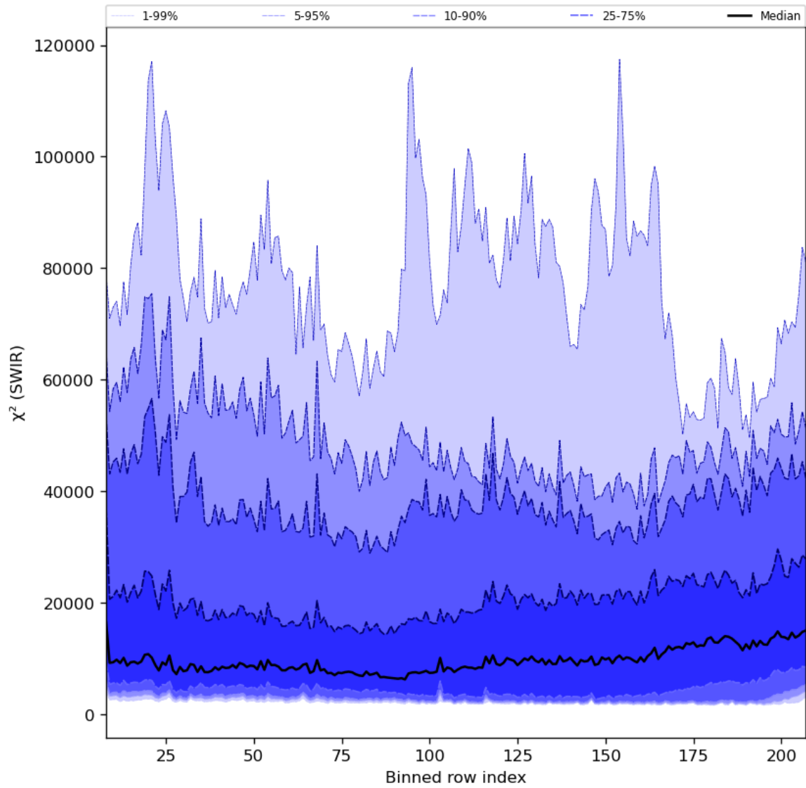
Figure 39: Along track statistics of “ \chi^2 (SWIR)” for 2023-11-05 to 2023-11-07
