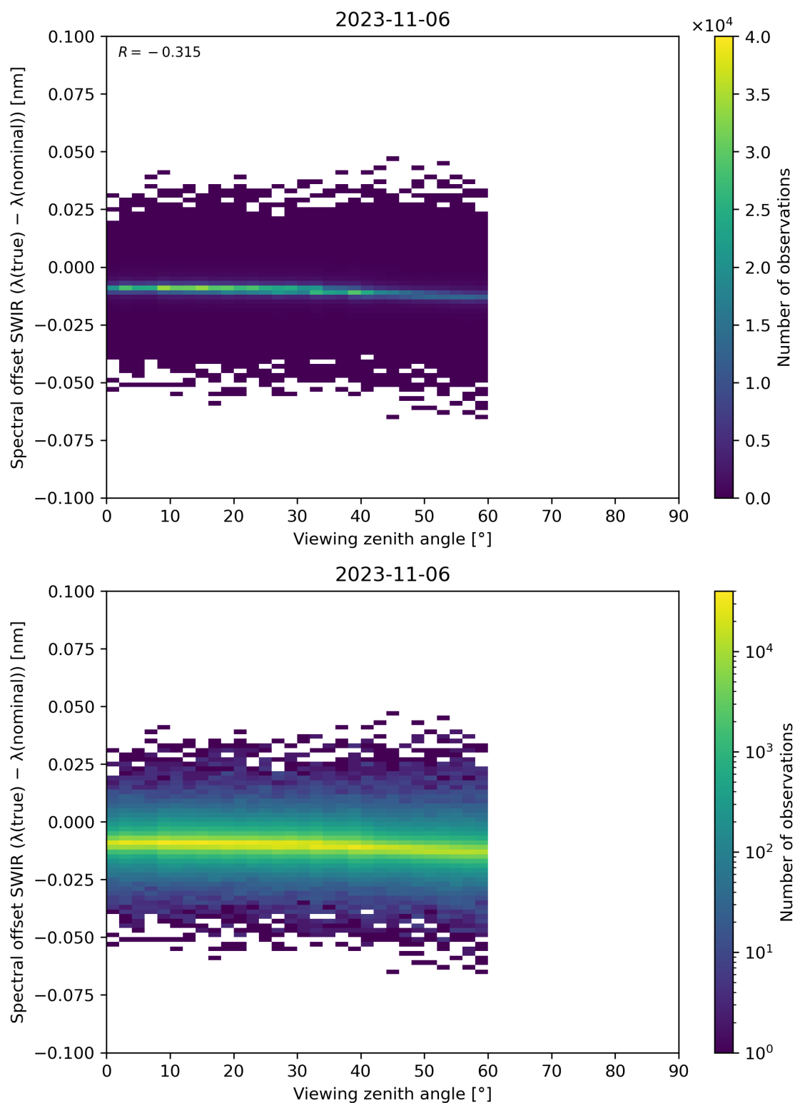
Figure 116: Scatter density plot of “Viewing zenith angle” against “Spectral offset SWIR ( \lambda(\text{true}) - \lambda(\text{nominal}) )” for 2023-11-05 to 2023-11-07.
