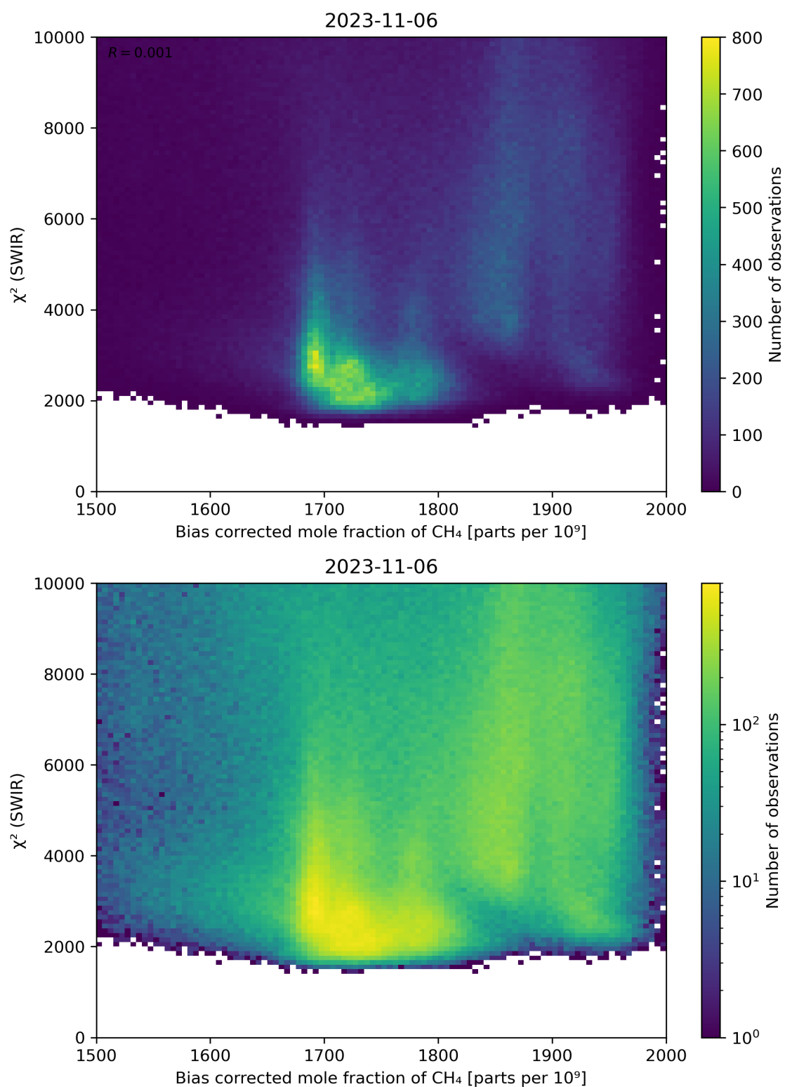
Figure 64: Scatter density plot of “Bias corrected mole fraction of \text{CH}_4 ” against “ \chi^2 (SWIR)” for 2023-11-05 to 2023-11-07.
