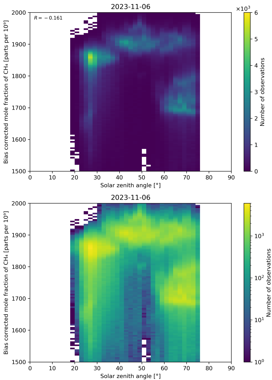
Figure 100: Scatter density plot of “Solar zenith angle” against “Bias corrected mole fraction of \text{CH}_4 ” for 2023-11-05 to 2023-11-07.
