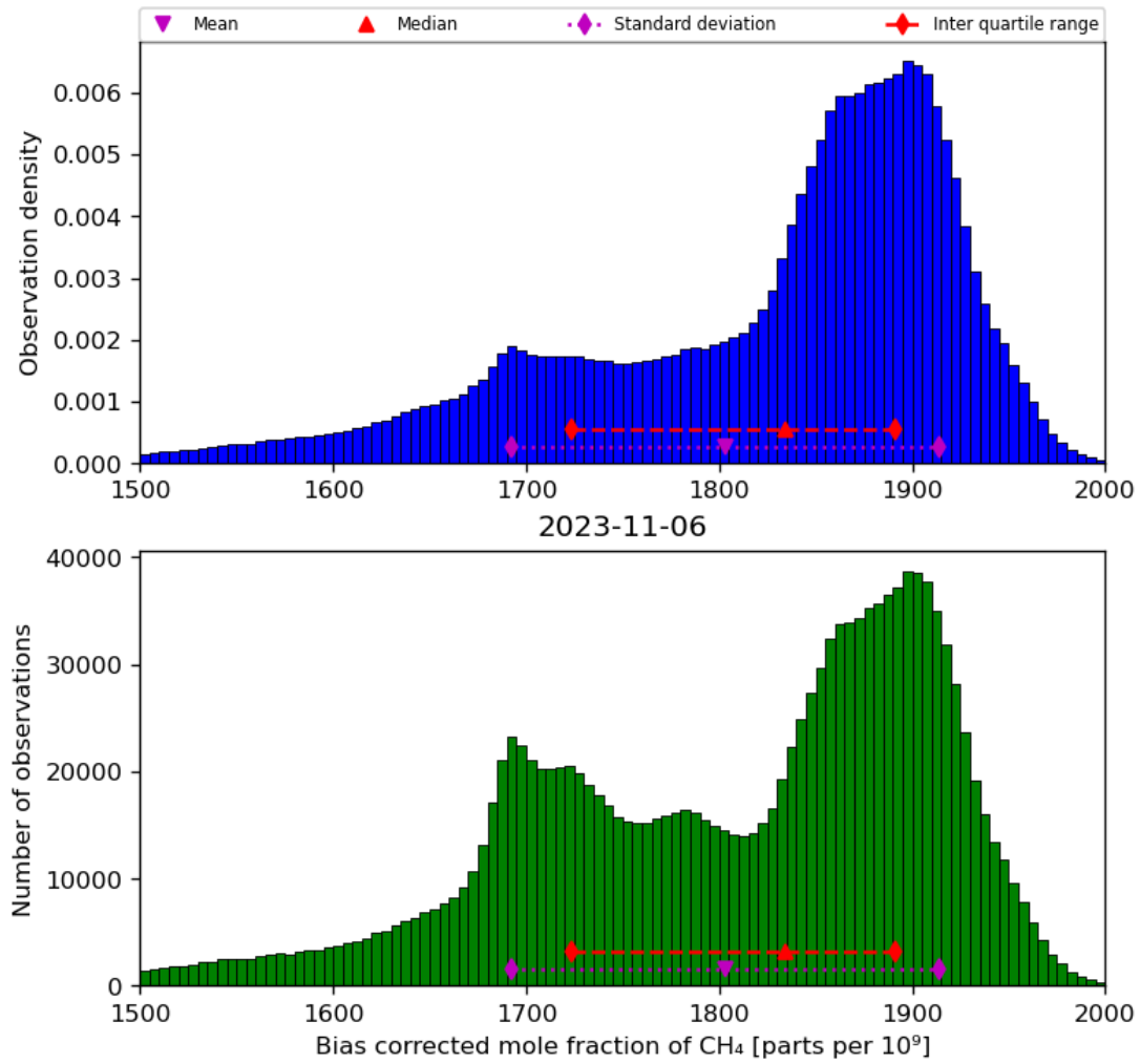
Figure 25: Histogram of “Bias corrected mole fraction of CH 4 ” for 2023-11-05 to 2023-11-07
