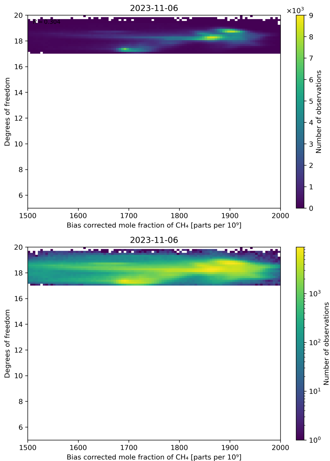
Figure 65: Scatter density plot of “Bias corrected mole fraction of CH 4 ” against “Degrees of freedom” for 2023-11-05 to 2023-11-07.
