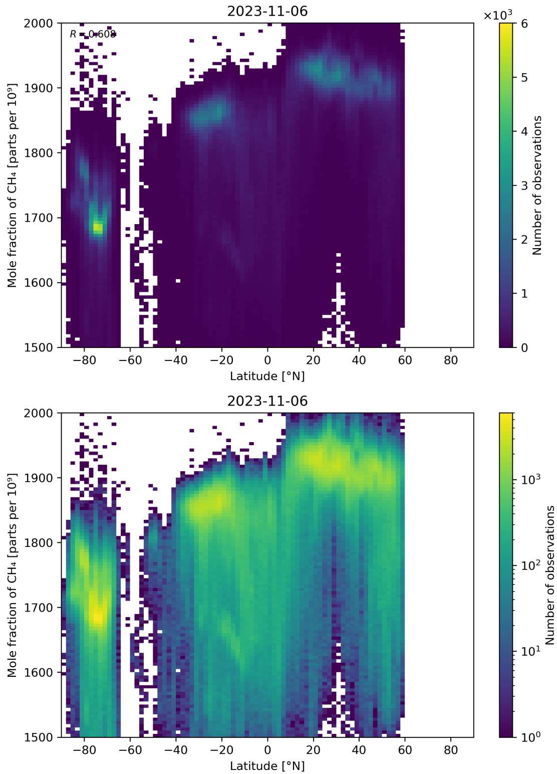
Figure 57: Scatter density plot of “Latitude” against “Mole fraction of CH 4 ” for 2023-11-05 to 2023-11-07.
