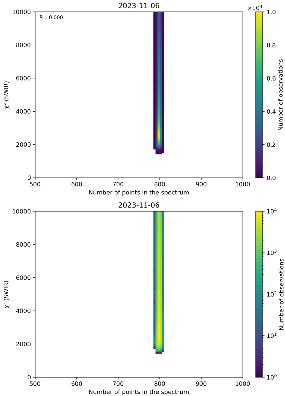
Figure 89: Scatter density plot of “Number of points in the spectrum” against “ \chi^2 (SWIR)” for 2023-11-05 to 2023-11-07.
