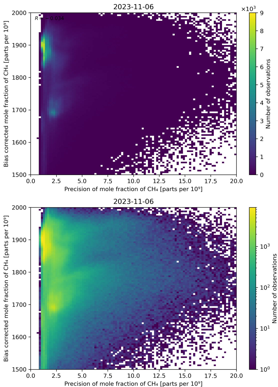
Figure 82: Scatter density plot of “Precision of mole fraction of CH 4 ” against “Bias corrected mole fraction of CH 4 ” for 2023-11-05 to 2023-11-07.
