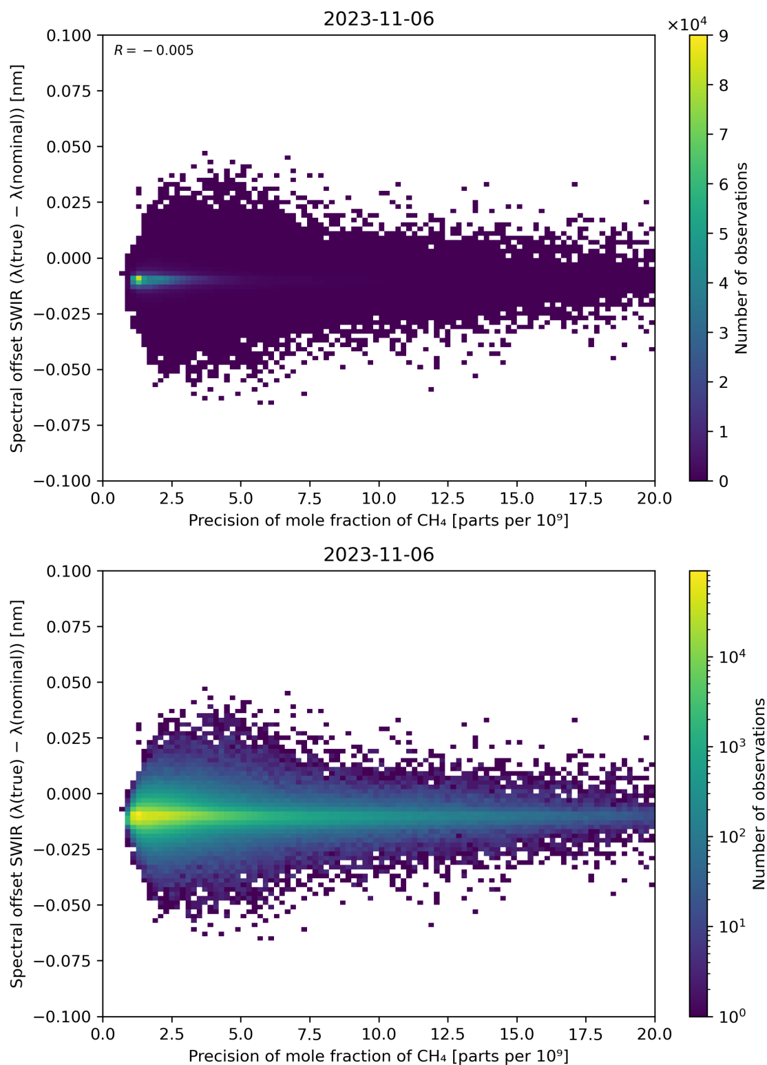
Figure 85: Scatter density plot of “Precision of mole fraction of CH 4 ” against “Spectral offset SWIR ( \lambda(\text{true}) - \lambda(\text{nominal}) )” for 2023-11-05 to 2023-11-07.
