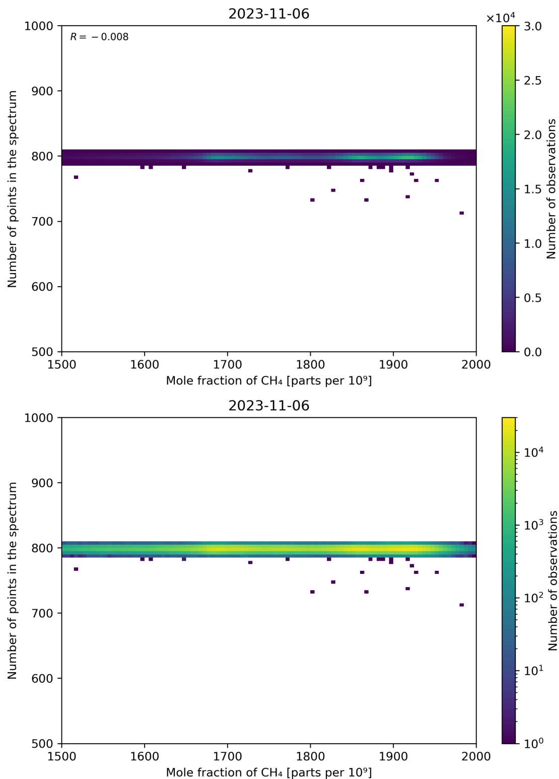
Figure 77: Scatter density plot of “Mole fraction of CH 4 ” against “Number of points in the spectrum” for 2023-11-05 to 2023-11-07.
