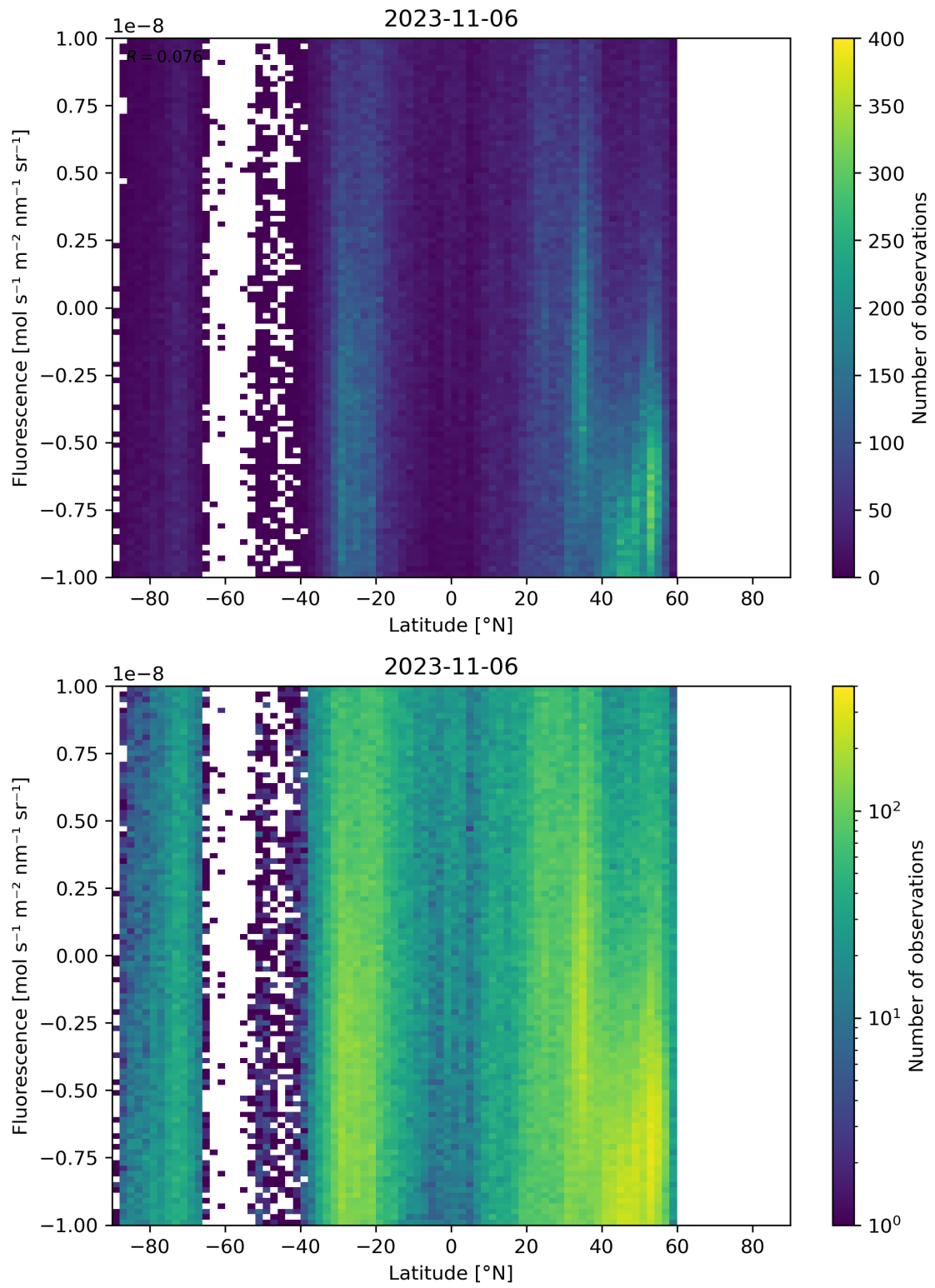
Figure 56: Scatter density plot of “Latitude” against “Fluorescence” for 2023-11-05 to 2023-11-07.
