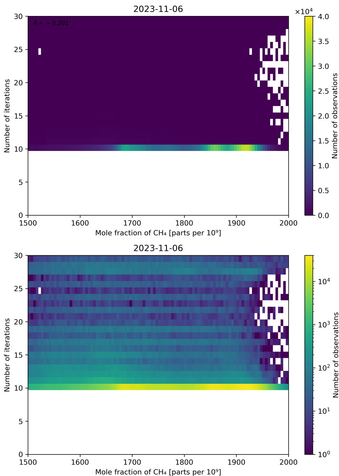
Figure 76: Scatter density plot of “Mole fraction of CH 4 ” against “Number of iterations” for 2023-11-05 to 2023-11-07.
