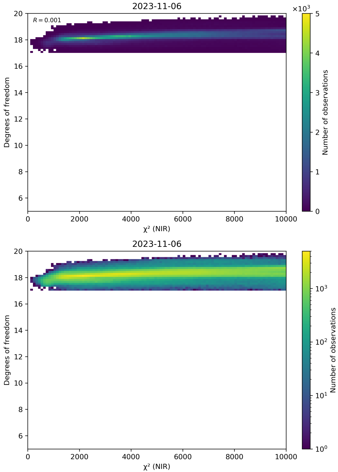
Figure 44: Scatter density plot of “ \chi^2 (NIR)” against “Degrees of freedom” for 2023-11-05 to 2023-11-07.
