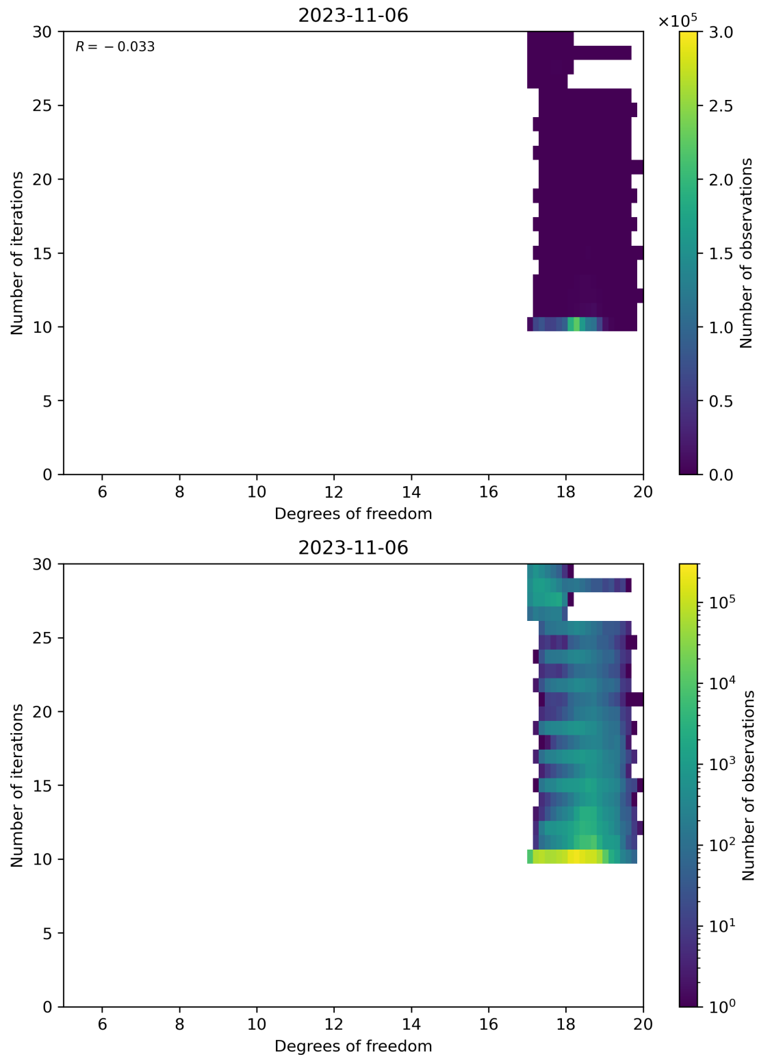
Figure 52: Scatter density plot of “Degrees of freedom” against “Number of iterations” for 2023-11-05 to 2023-11-07.
