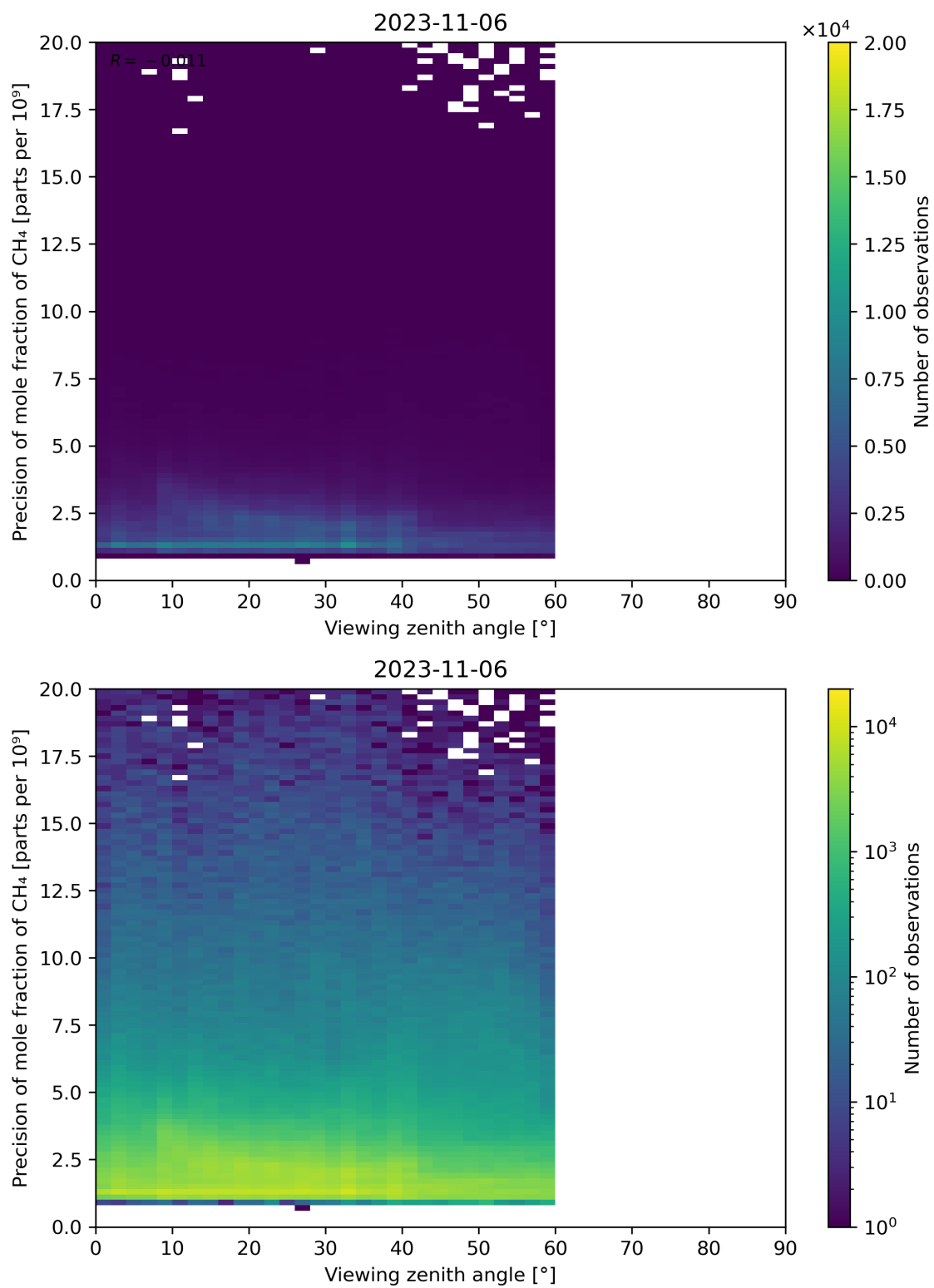
Figure 112: Scatter density plot of “Viewing zenith angle” against “Precision of mole fraction of CH 4 ” for 2023-11-05 to 2023-11-07.
