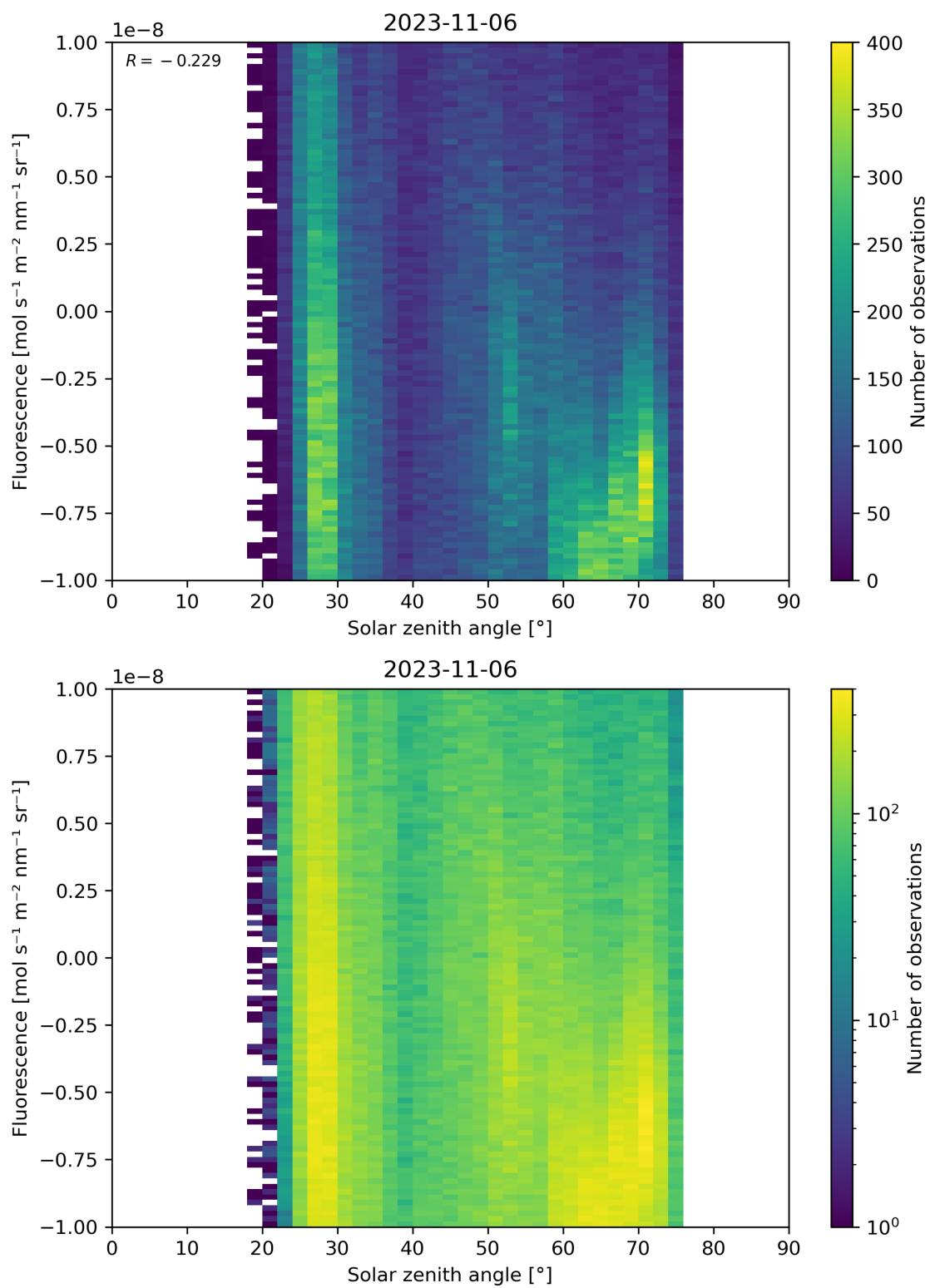
Figure 97: Scatter density plot of “Solar zenith angle” against “Fluorescence” for 2023-11-05 to 2023-11-07.
