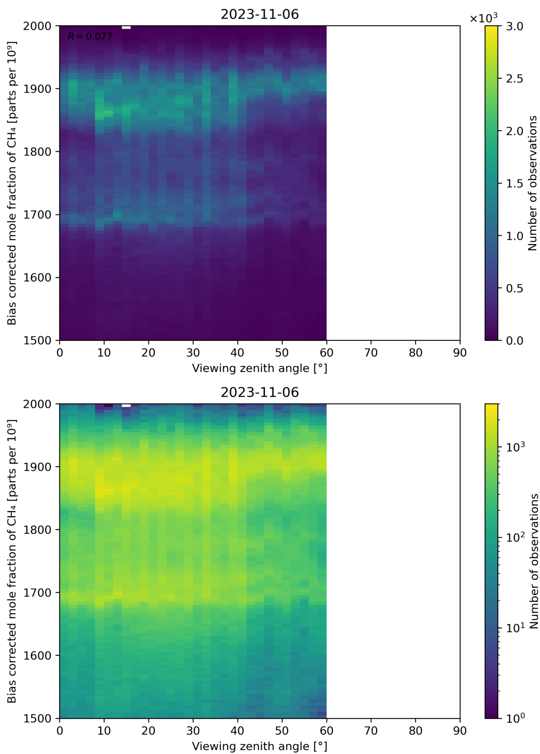
Figure 111: Scatter density plot of “Viewing zenith angle” against “Bias corrected mole fraction of CH 4 ” for 2023-11-05 to 2023-11-07.
