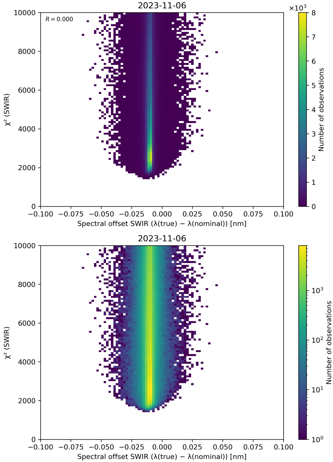
Figure 118: Scatter density plot of “Spectral offset SWIR ( \lambda(\text{true}) - \lambda(\text{nominal}) )” against “ \chi^2 (SWIR)” for 2023-11-05 to 2023-11-07.
