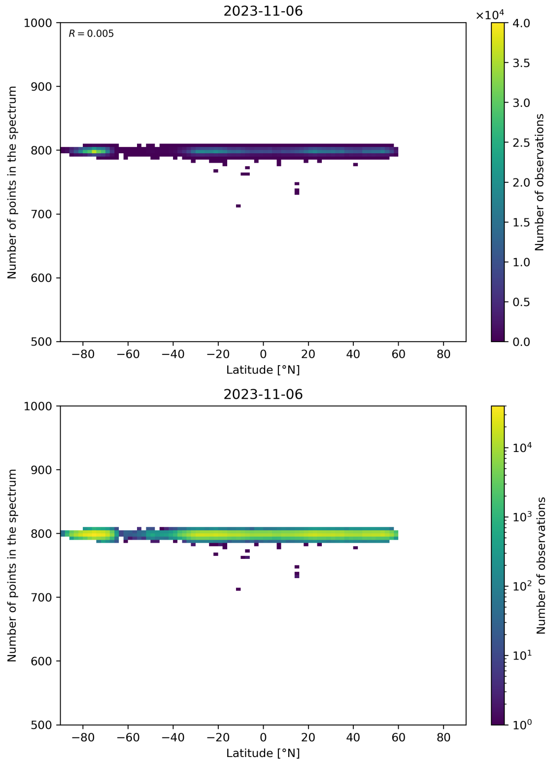
Figure 61: Scatter density plot of “Latitude” against “Number of points in the spectrum” for 2023-11-05 to 2023-11-07.
