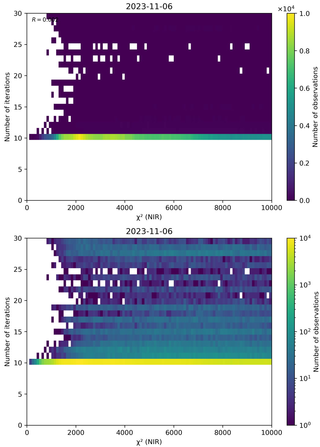
Figure 46: Scatter density plot of “ \chi^2 (NIR)” against “Number of iterations” for 2023-11-05 to 2023-11-07.
