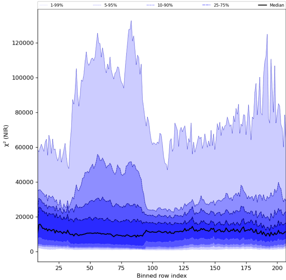
Figure 40: Along track statistics of “ \chi^2 (NIR)” for 2023-11-05 to 2023-11-07
