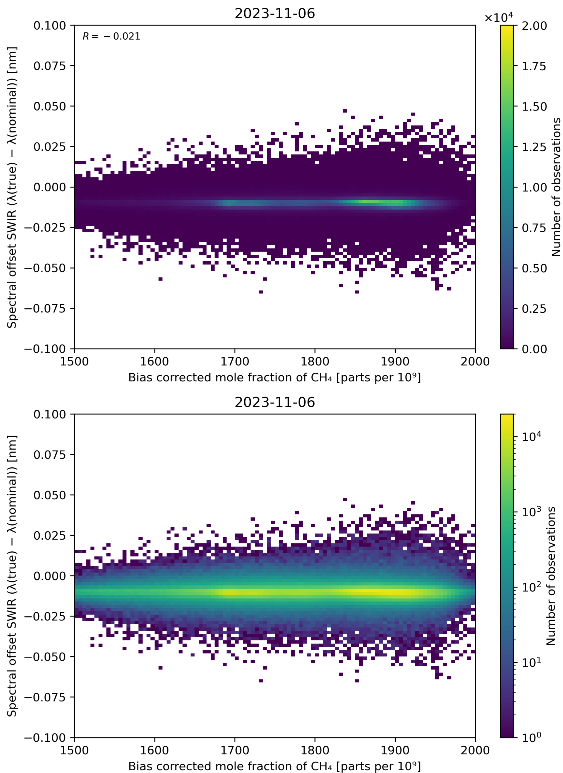
Figure 69: Scatter density plot of “Bias corrected mole fraction of \text{CH}_4 ” against “Spectral offset SWIR ( \lambda(\text{true}) - \lambda(\text{nominal}) )” for 2023-11-05 to 2023-11-07.
