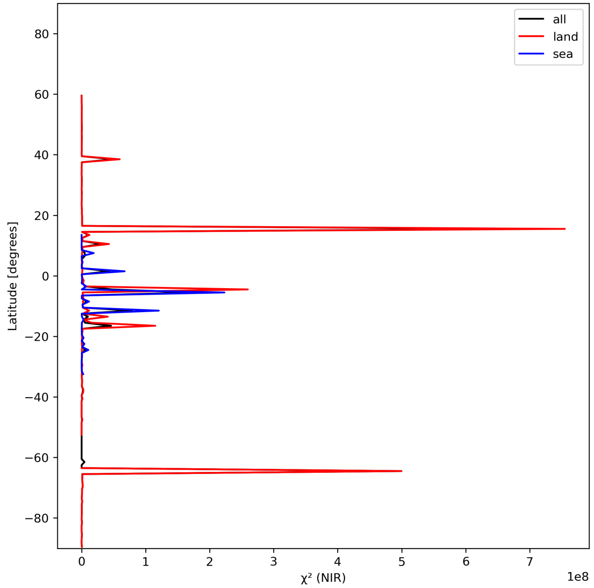
Figure 18: Zonal average of “ \chi^2 (NIR)” for 2023-11-05 to 2023-11-07.
