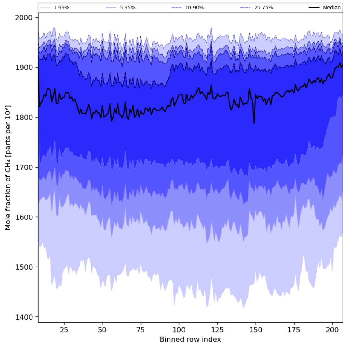
Figure 34: Along track statistics of “Mole fraction of CH 4 ” for 2023-11-05 to 2023-11-07
