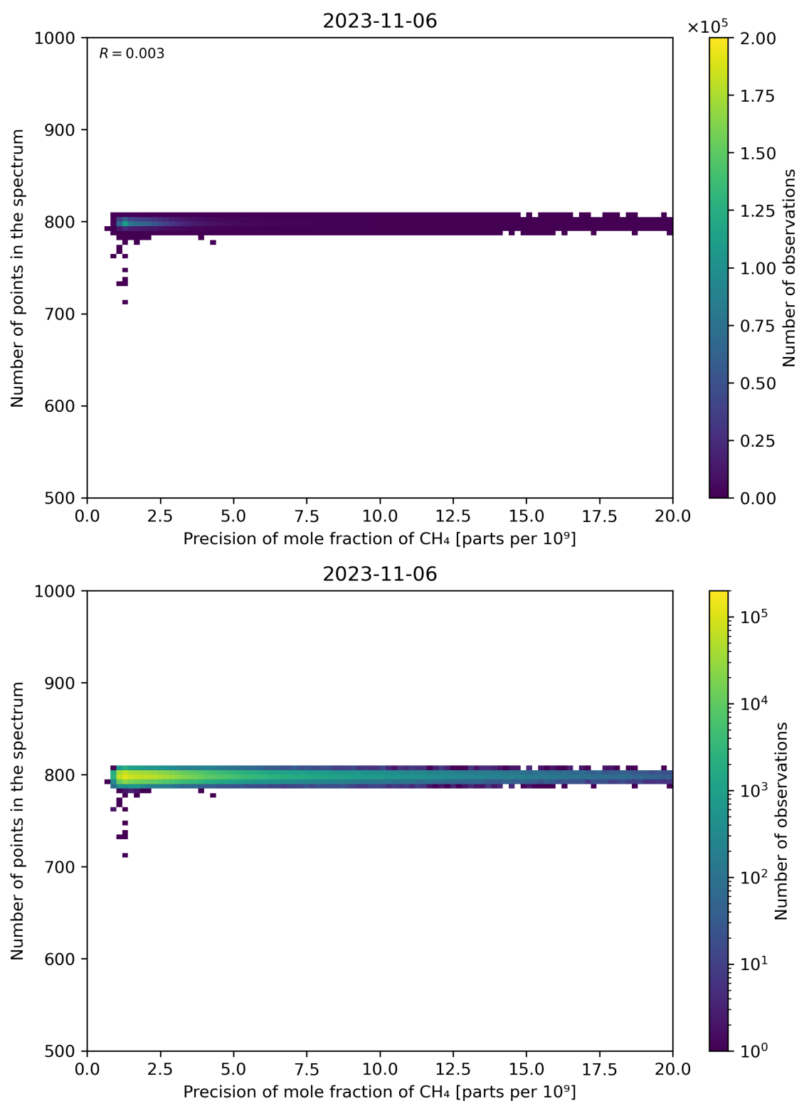
Figure 84: Scatter density plot of “Precision of mole fraction of CH 4 ” against “Number of points in the spectrum” for 2023-11-05 to 2023-11-07.
