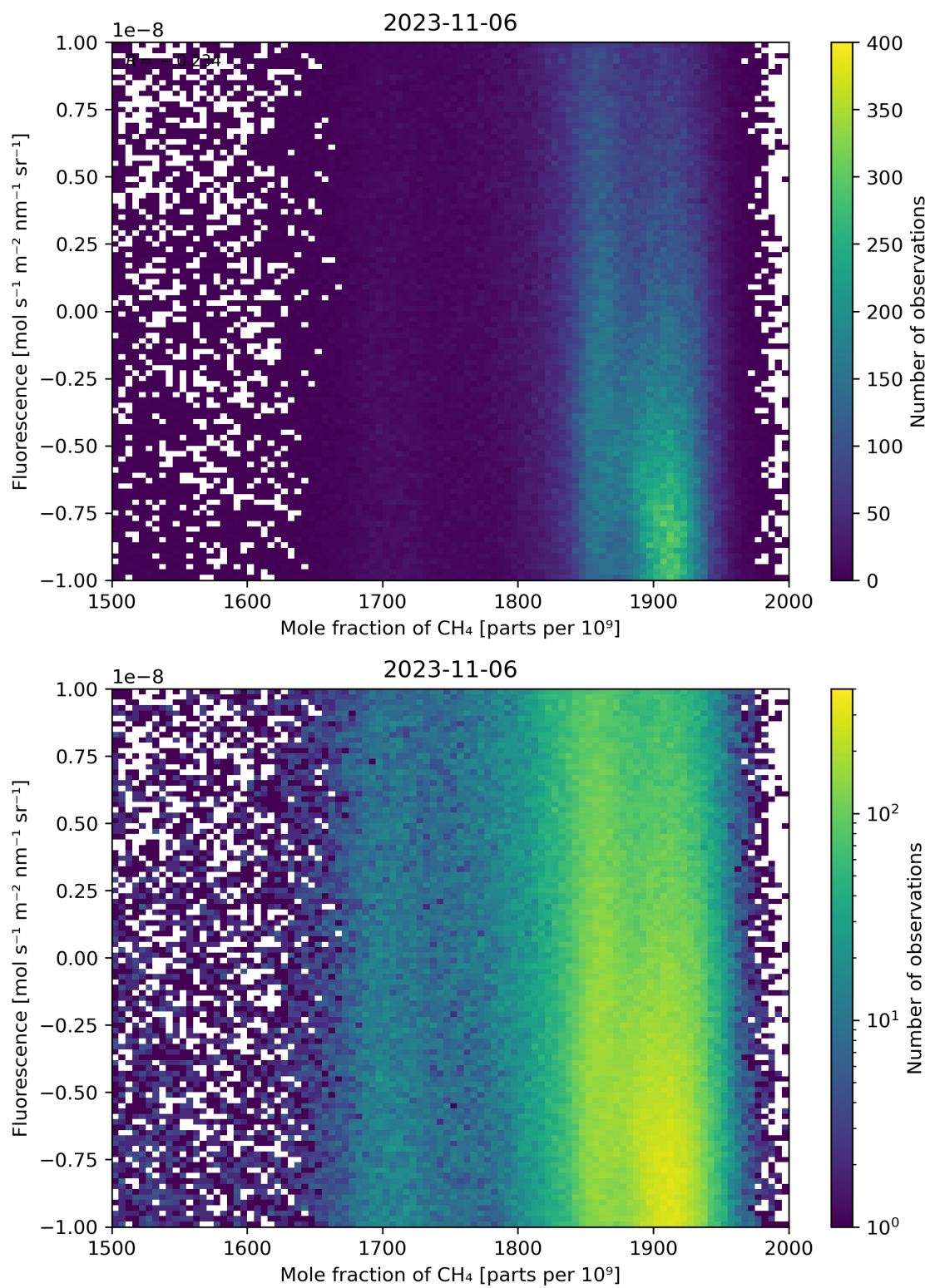
Figure 73: Scatter density plot of “Mole fraction of \text{CH}_4 ” against “Fluorescence” for 2023-11-05 to 2023-11-07.
