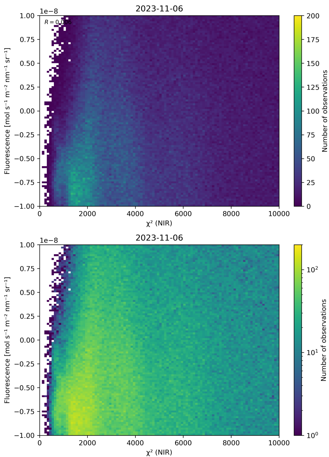
Figure 45: Scatter density plot of “ \chi^2 (NIR)” against “Fluorescence” for 2023-11-05 to 2023-11-07.
