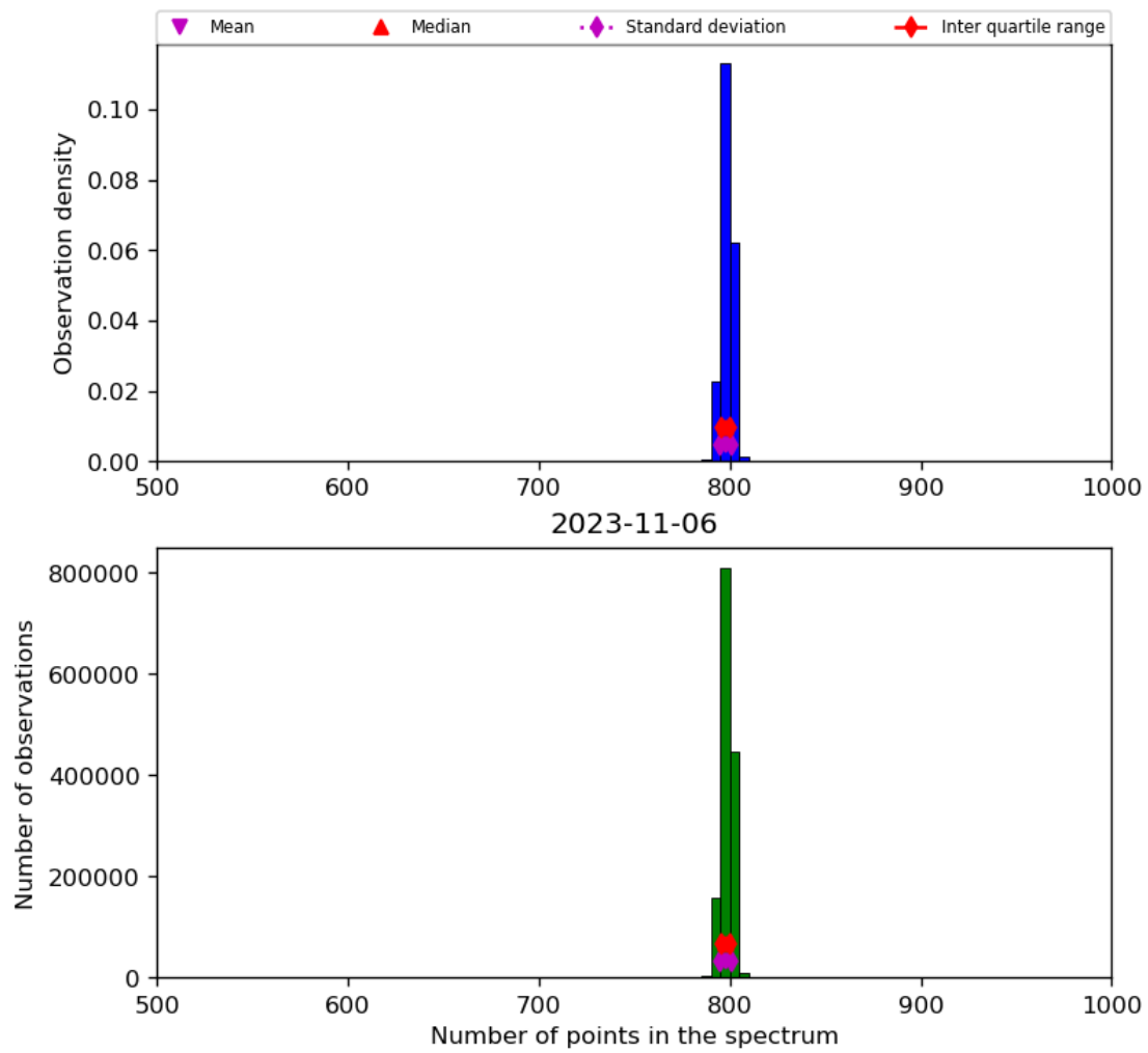
Figure 26: Histogram of “Number of points in the spectrum” for 2023-11-05 to 2023-11-07
