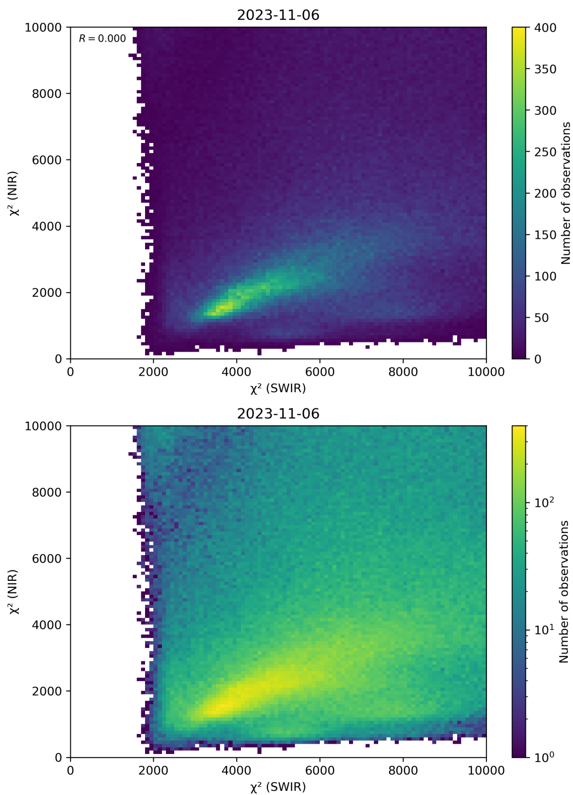
Figure 47: Scatter density plot of “ \chi^2 (SWIR)” against “ \chi^2 (NIR)” for 2023-11-05 to 2023-11-07.
