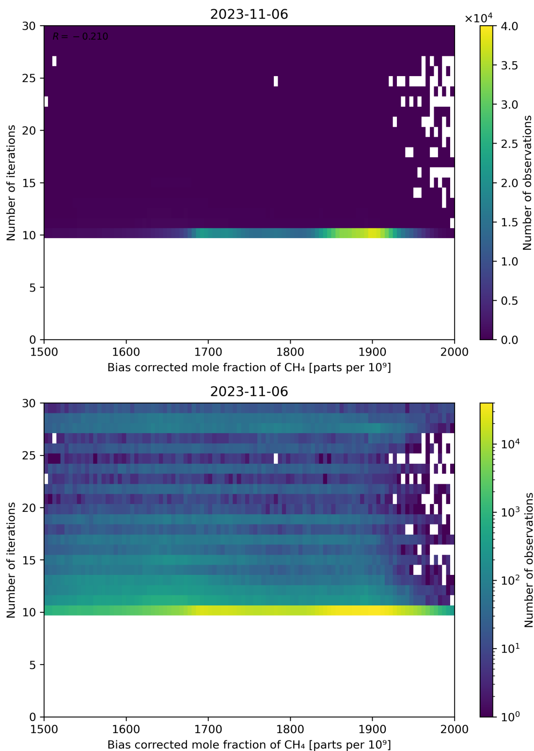
Figure 67: Scatter density plot of “Bias corrected mole fraction of \text{CH}_4 ” against “Number of iterations” for 2023-11-05 to 2023-11-07.
