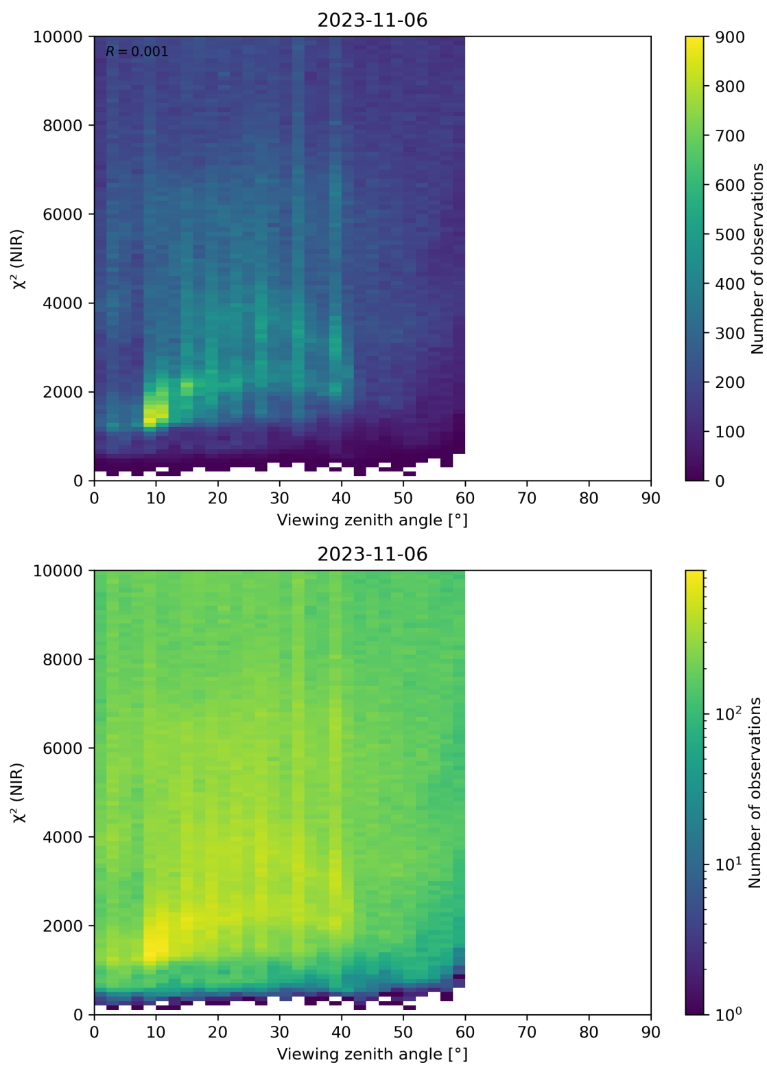
Figure 105: Scatter density plot of “Viewing zenith angle” against “ \chi^2 (NIR)” for 2023-11-05 to 2023-11-07.
