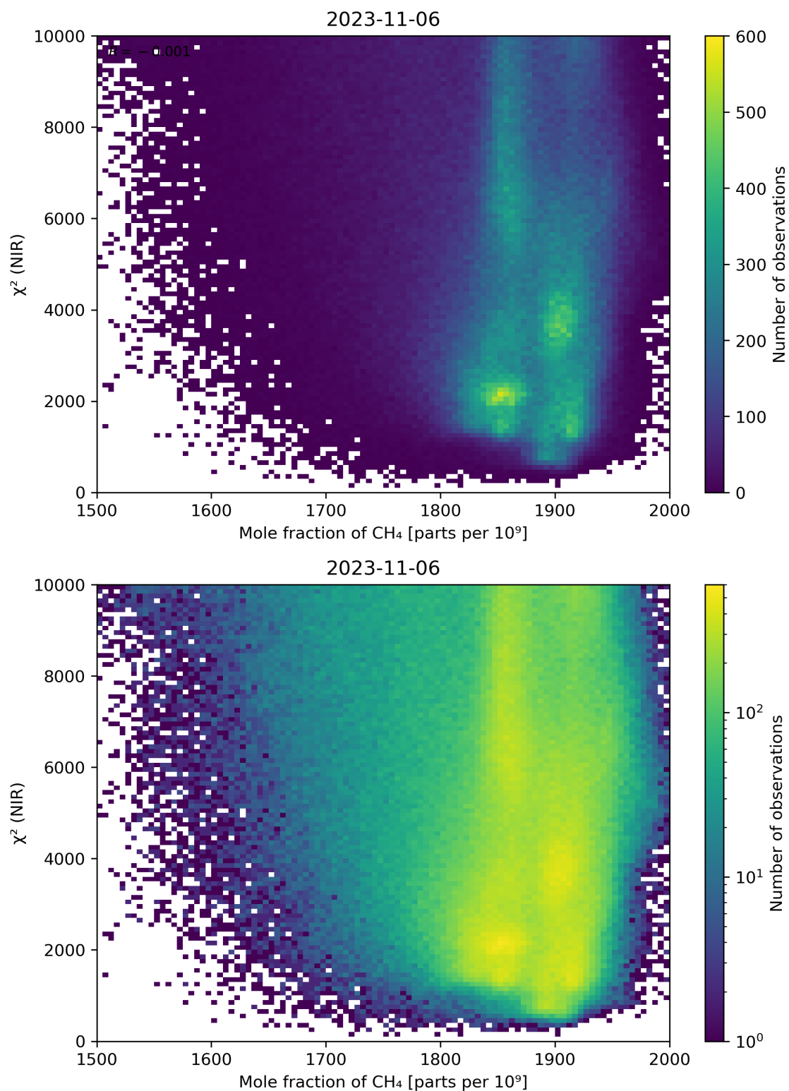
Figure 70: Scatter density plot of “Mole fraction of \text{CH}_4 ” against “ \chi^2 (NIR)” for 2023-11-05 to 2023-11-07.
