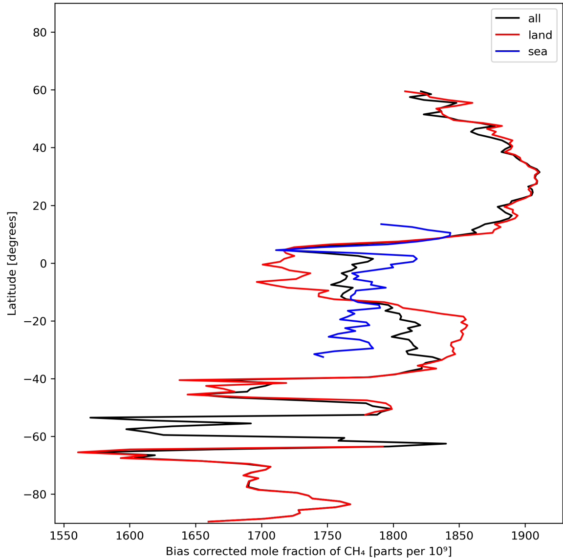
Figure 14: Zonal average of “Bias corrected mole fraction of \text{CH}_4 ” for 2023-11-05 to 2023-11-07.
