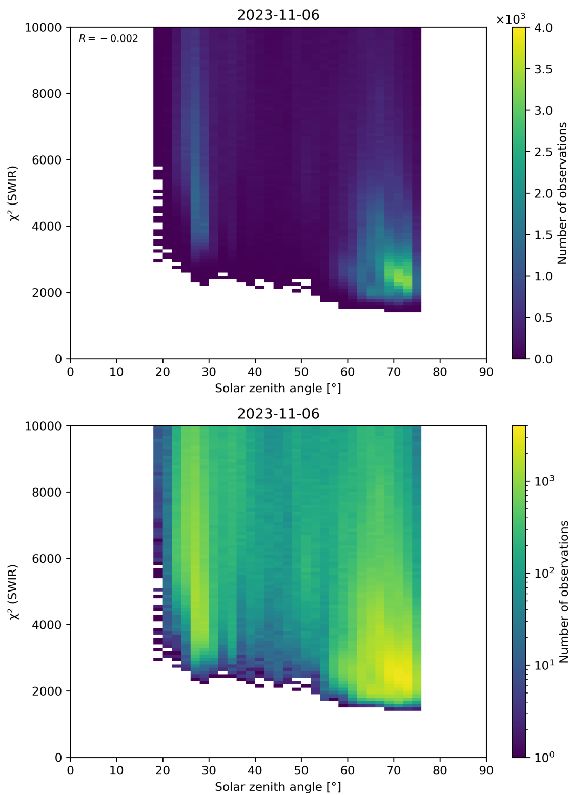
Figure 95: Scatter density plot of “Solar zenith angle” against “ \chi^2 (SWIR)” for 2023-11-05 to 2023-11-07.
