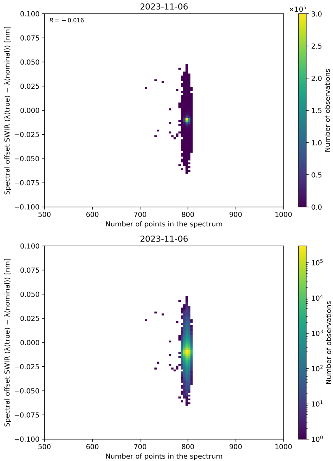
Figure 93: Scatter density plot of “Number of points in the spectrum” against “Spectral offset SWIR ( \lambda(\text{true}) - \lambda(\text{nominal}) )” for 2023-11-05 to 2023-11-07.
