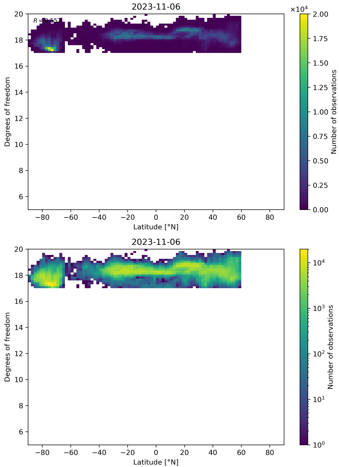
Figure 55: Scatter density plot of “Latitude” against “Degrees of freedom” for 2023-11-05 to 2023-11-07.
