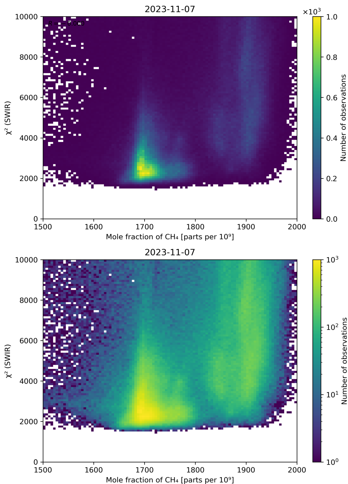
Figure 71: Scatter density plot of “Mole fraction of \text{CH}_4 ” against “ \chi^2 (SWIR)” for 2023-11-07 to 2023-11-08.
