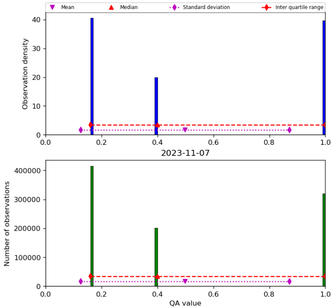
Figure 22: Histogram of “QA value” for 2023-11-07 to 2023-11-08
