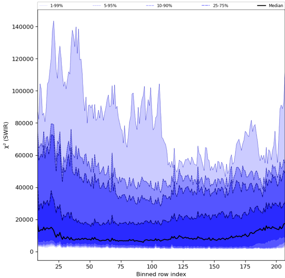
Figure 39: Along track statistics of “ \chi^2 (SWIR)” for 2023-11-07 to 2023-11-08
