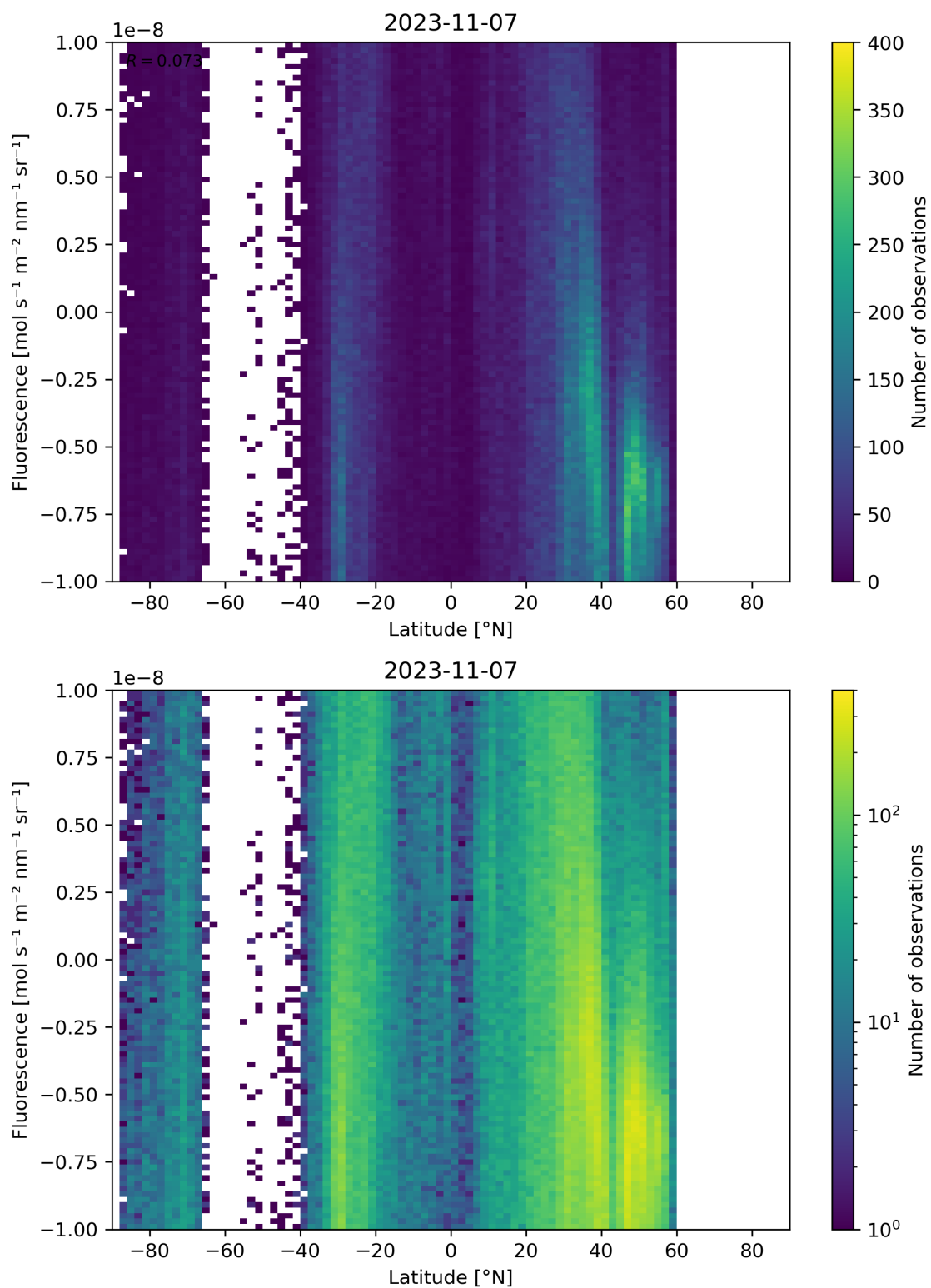
Figure 56: Scatter density plot of “Latitude” against “Fluorescence” for 2023-11-07 to 2023-11-08.
