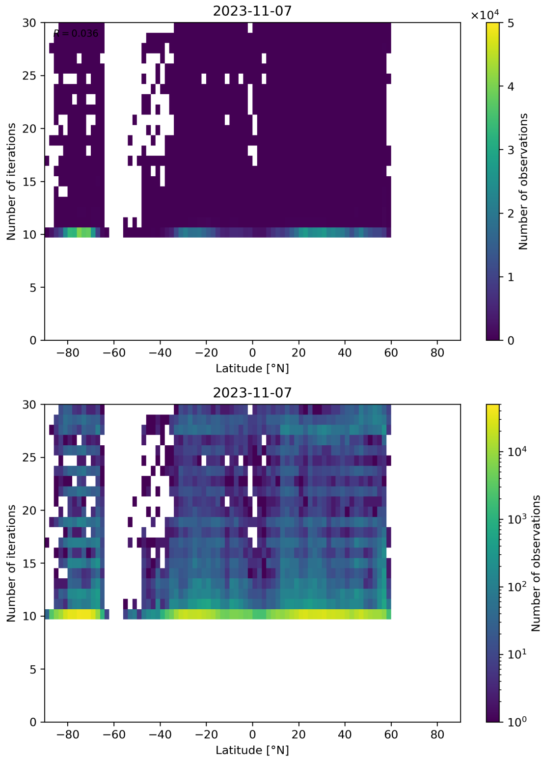
Figure 60: Scatter density plot of “Latitude” against “Number of iterations” for 2023-11-07 to 2023-11-08.
