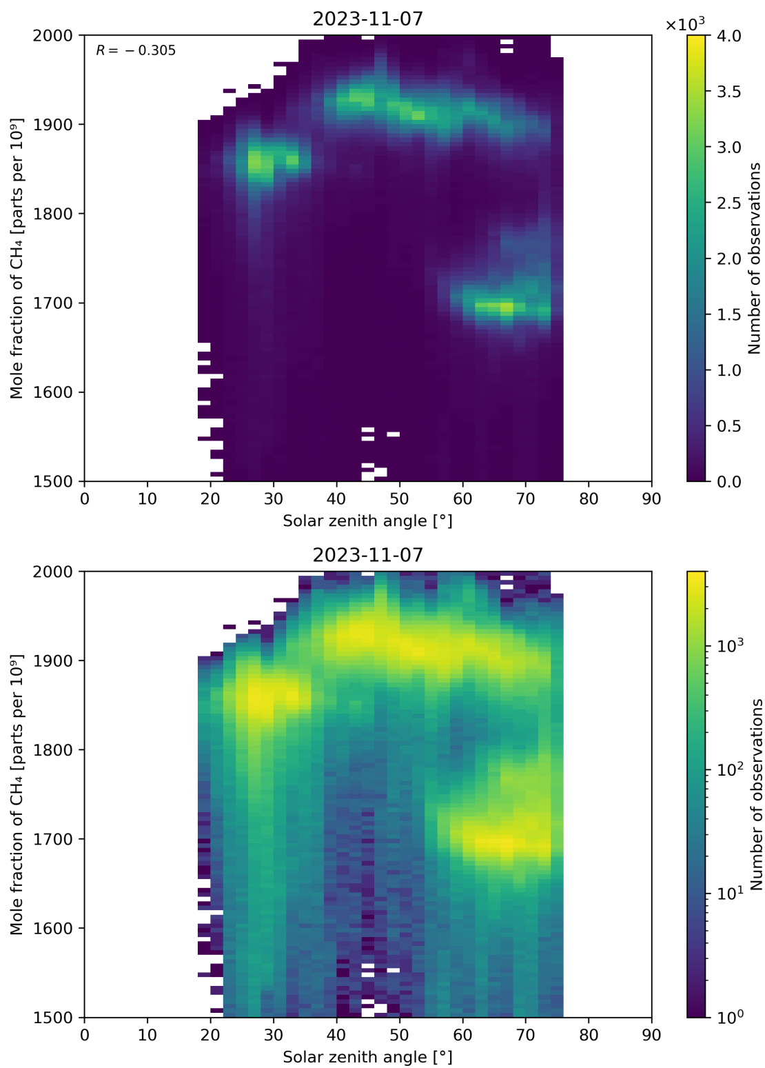
Figure 99: Scatter density plot of “Solar zenith angle” against “Mole fraction of \text{CH}_4 ” for 2023-11-07 to 2023-11-08.
