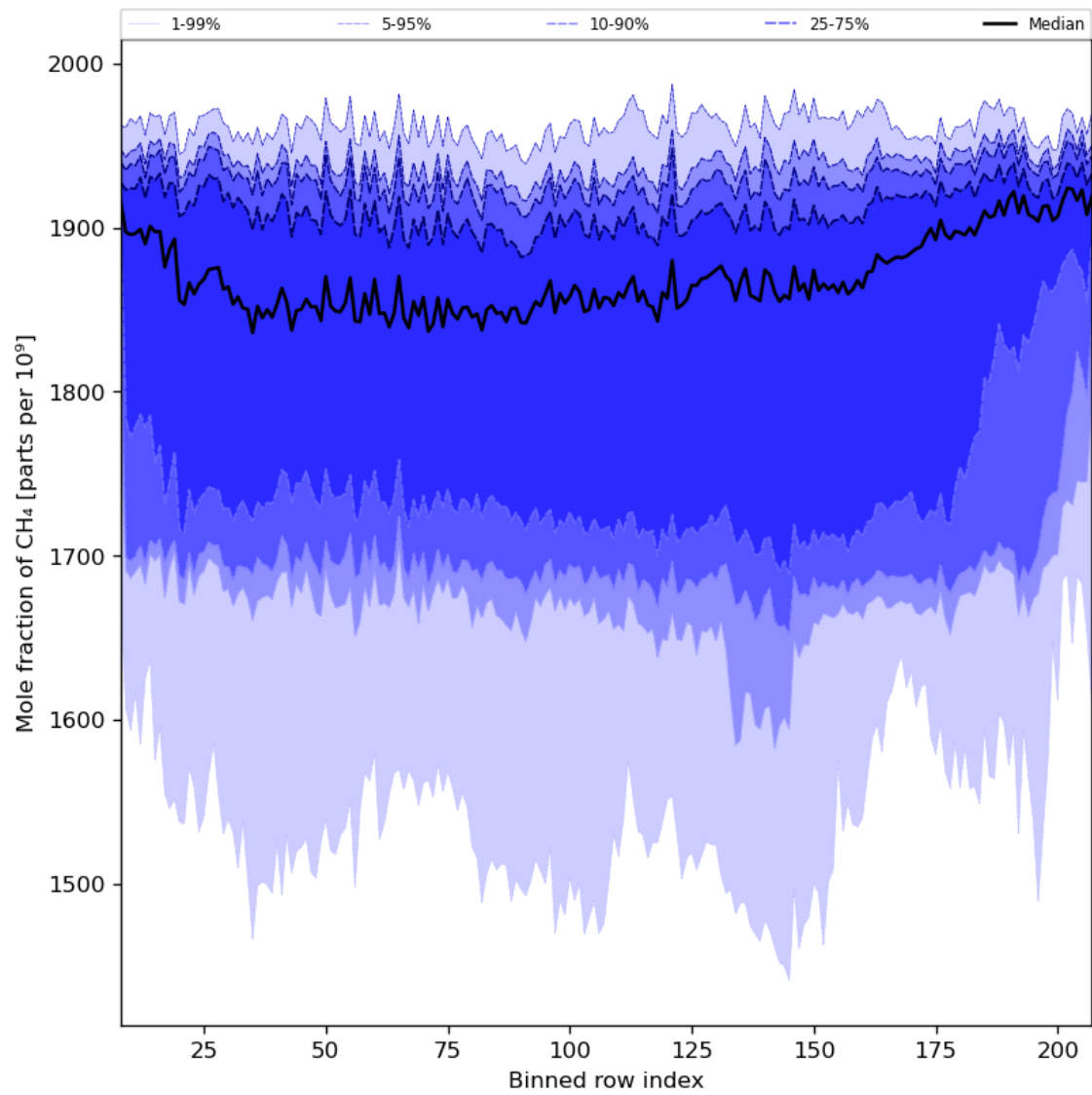
Figure 34: Along track statistics of “Mole fraction of CH 4 ” for 2023-11-07 to 2023-11-08
