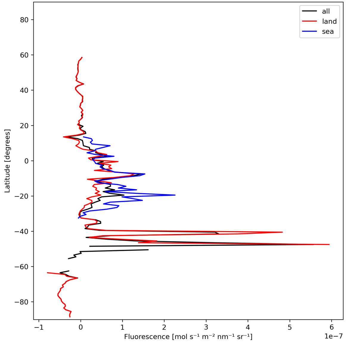
Figure 21: Zonal average of “Fluorescence” for 2023-11-07 to 2023-11-08.
