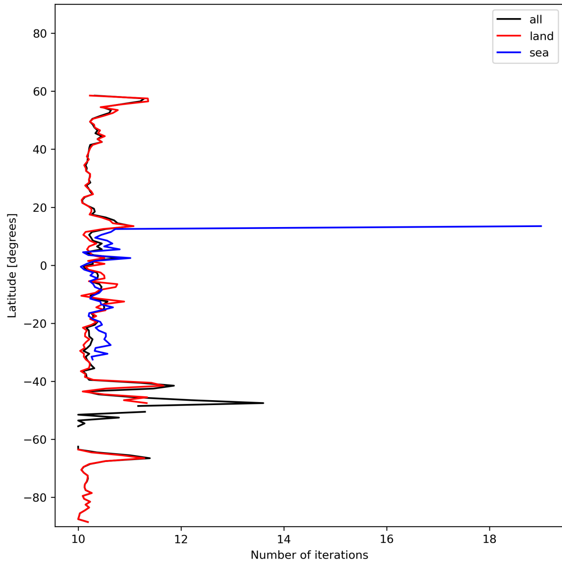
Figure 20: Zonal average of “Number of iterations” for 2023-11-07 to 2023-11-08.
