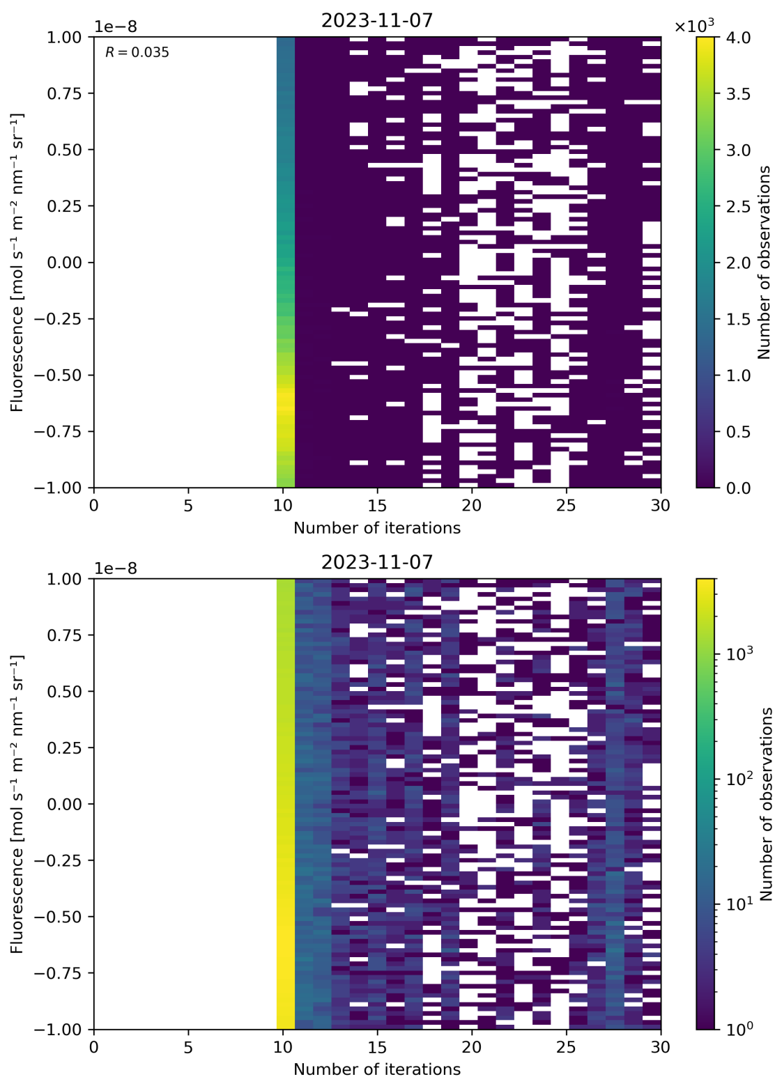
Figure 87: Scatter density plot of “Number of iterations” against “Fluorescence” for 2023-11-07 to 2023-11-08.
