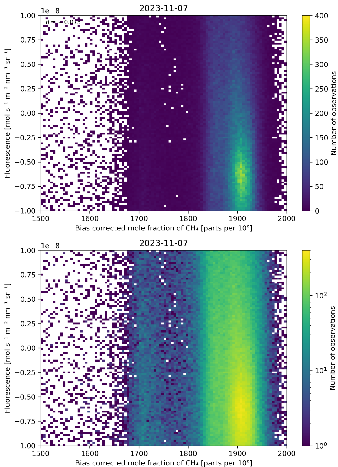
Figure 66: Scatter density plot of “Bias corrected mole fraction of CH 4 ” against “Fluorescence” for 2023-11-07 to 2023-11-08.
