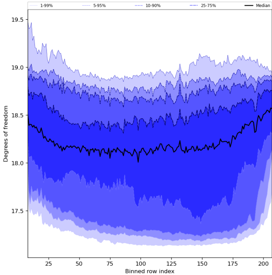
Figure 41: Along track statistics of “Degrees of freedom” for 2023-11-07 to 2023-11-08
