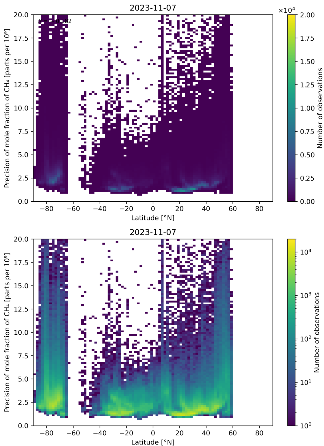
Figure 59: Scatter density plot of “Latitude” against “Precision of mole fraction of CH 4 ” for 2023-11-07 to 2023-11-08.
