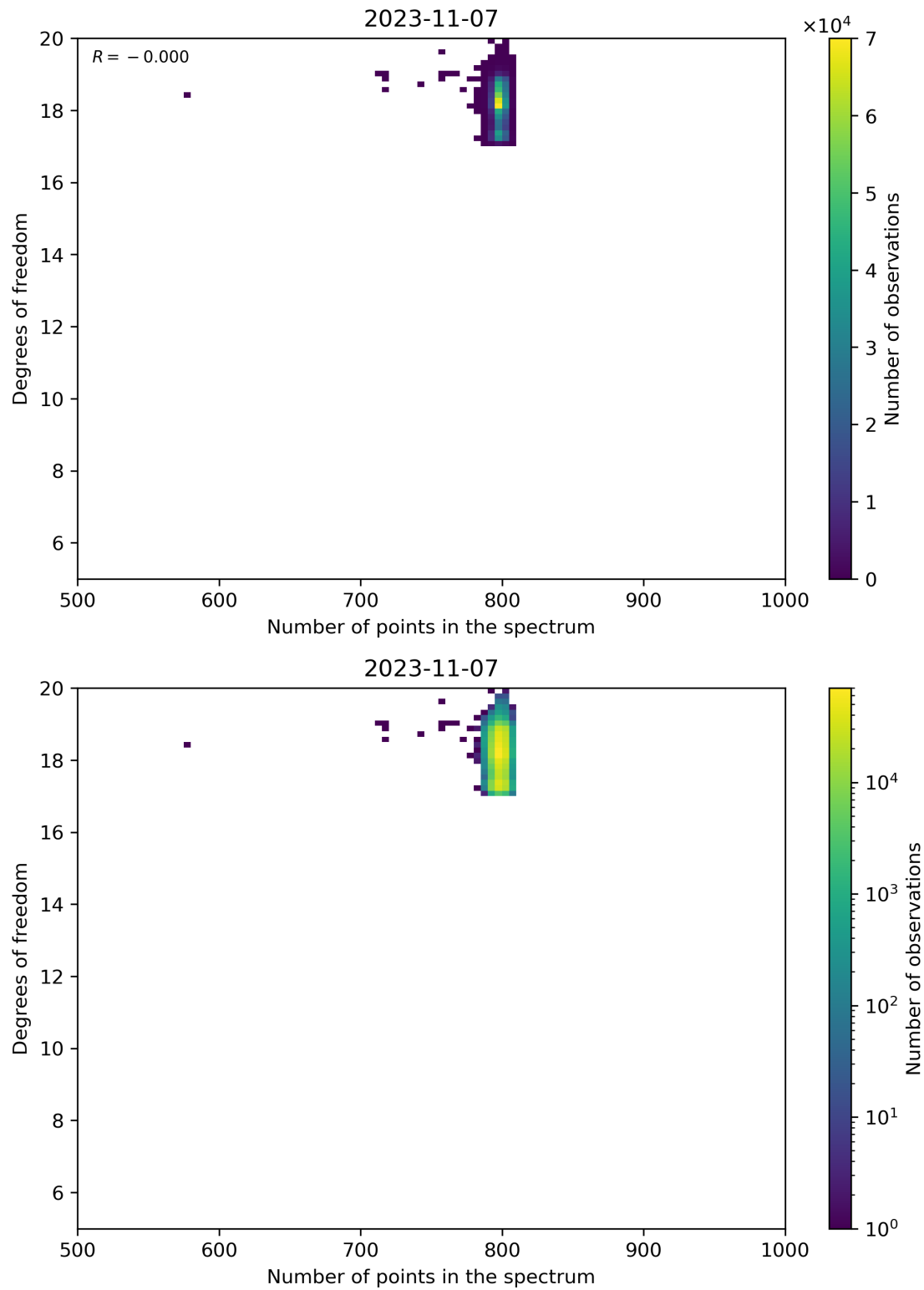
Figure 90: Scatter density plot of “Number of points in the spectrum” against “Degrees of freedom” for 2023-11-07 to 2023-11-08.
