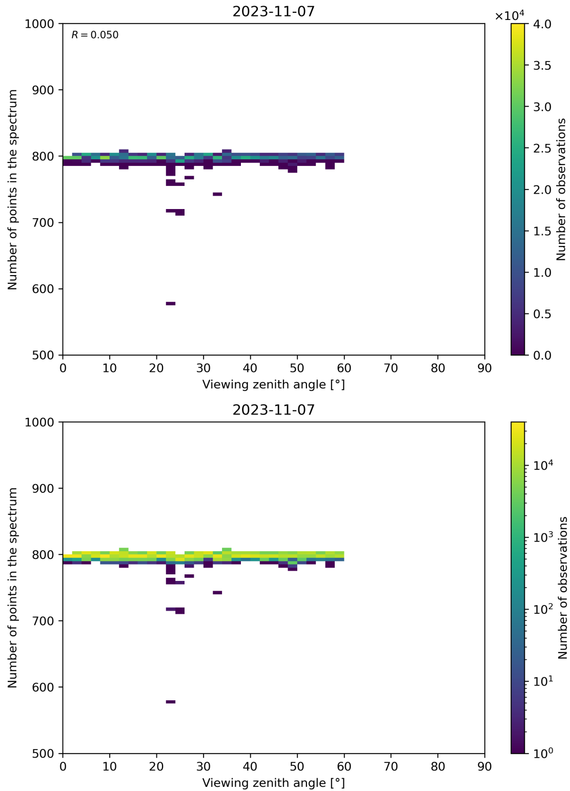
Figure 114: Scatter density plot of “Viewing zenith angle” against “Number of points in the spectrum” for 2023-11-07 to 2023-11-08.
