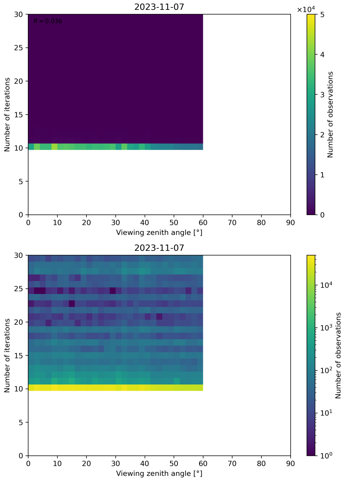
Figure 113: Scatter density plot of “Viewing zenith angle” against “Number of iterations” for 2023-11-07 to 2023-11-08.
