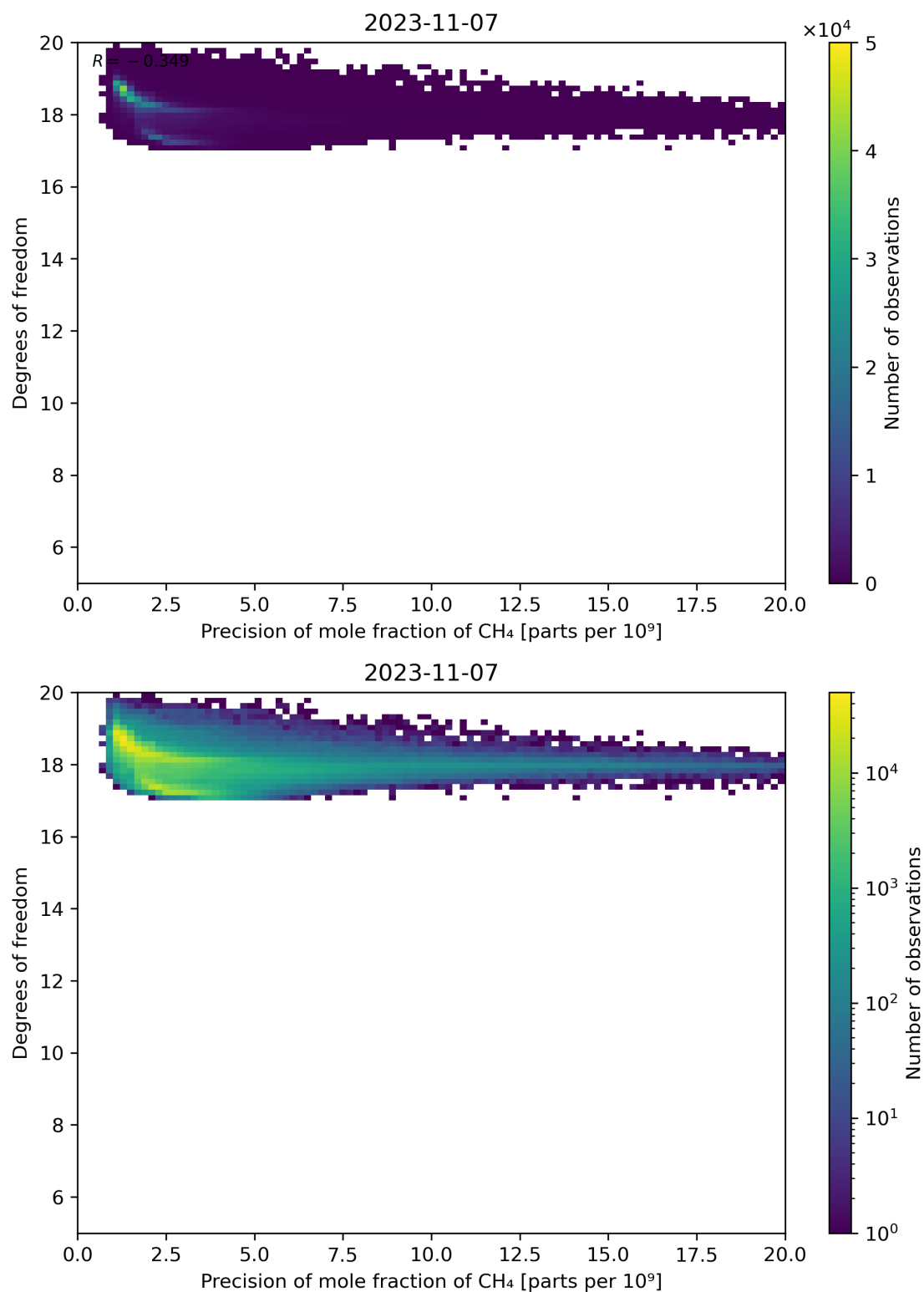
Figure 80: Scatter density plot of “Precision of mole fraction of CH 4 ” against “Degrees of freedom” for 2023-11-07 to 2023-11-08.
