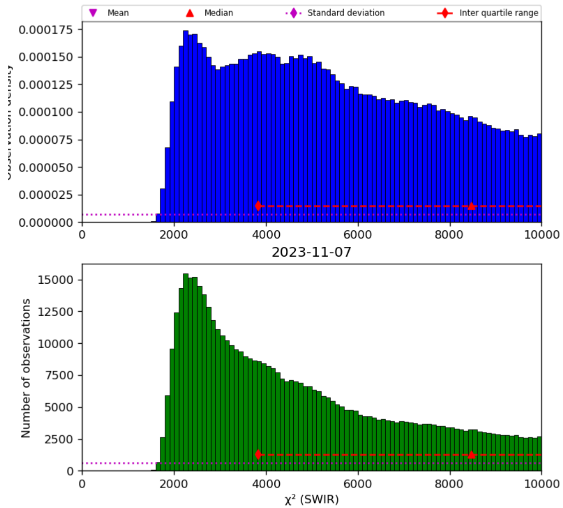
Figure 28: Histogram of “ \chi^2 (SWIR)” for 2023-11-07 to 2023-11-08
