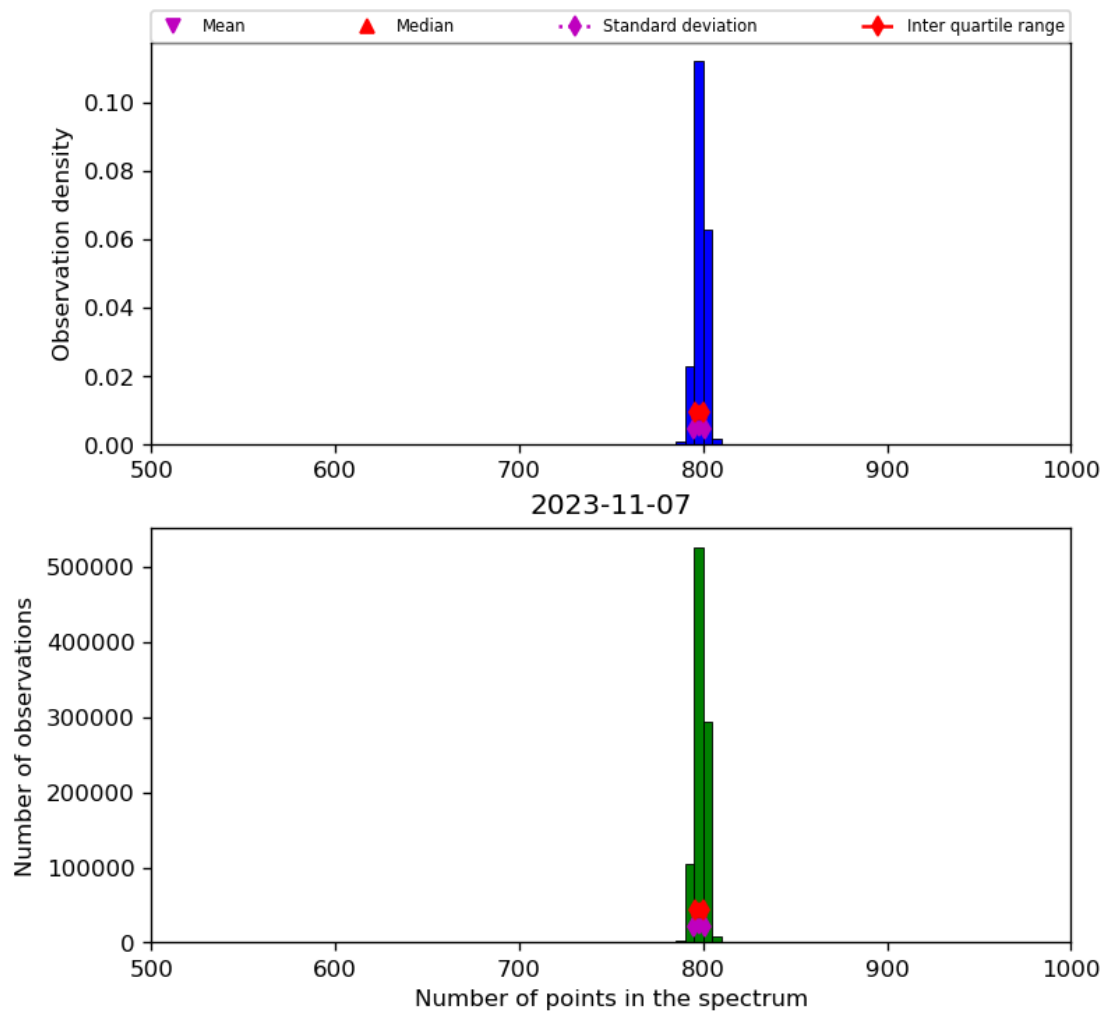
Figure 26: Histogram of “Number of points in the spectrum” for 2023-11-07 to 2023-11-08
