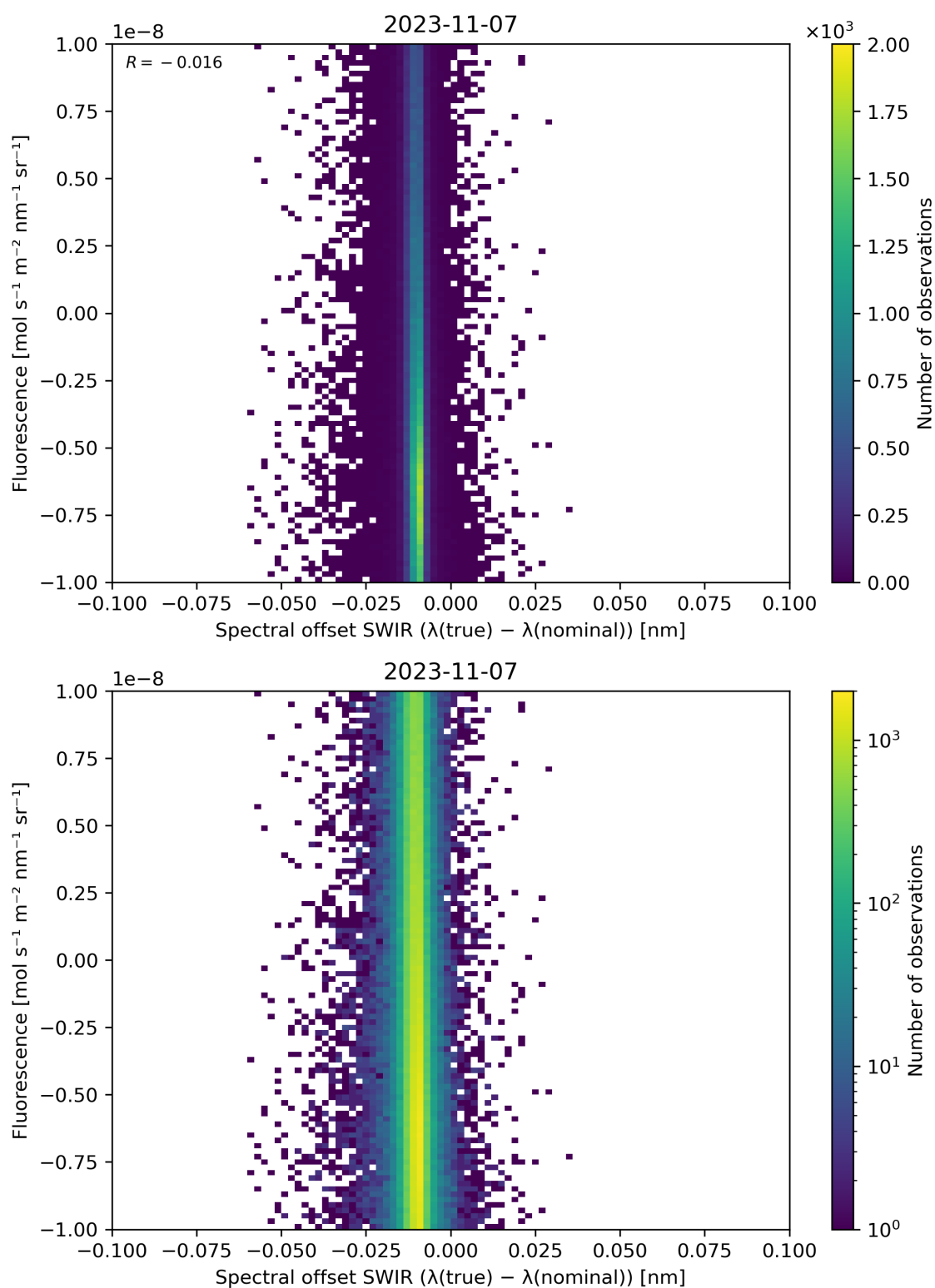
Figure 120: Scatter density plot of “Spectral offset SWIR ( \lambda(\text{true}) - \lambda(\text{nominal}) )” against “Fluorescence” for 2023-11-07 to 2023-11-08.
