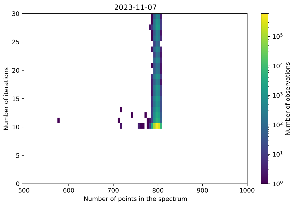
Figure 92: Scatter density plot of “Number of points in the spectrum” against “Number of iterations” for 2023-11-07 to 2023-11-08.
