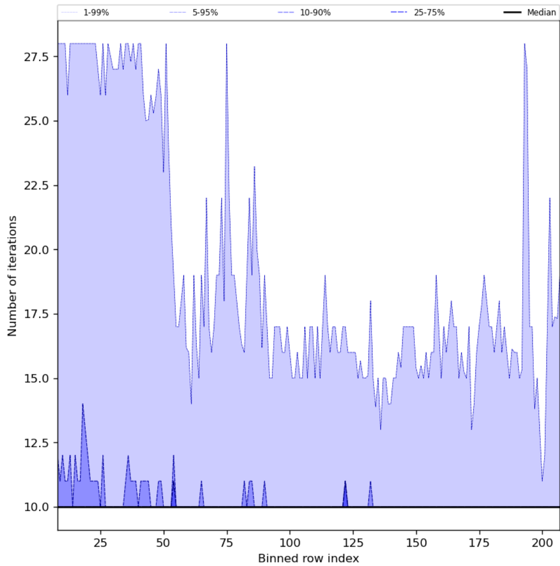
Figure 42: Along track statistics of “Number of iterations” for 2023-11-07 to 2023-11-08
