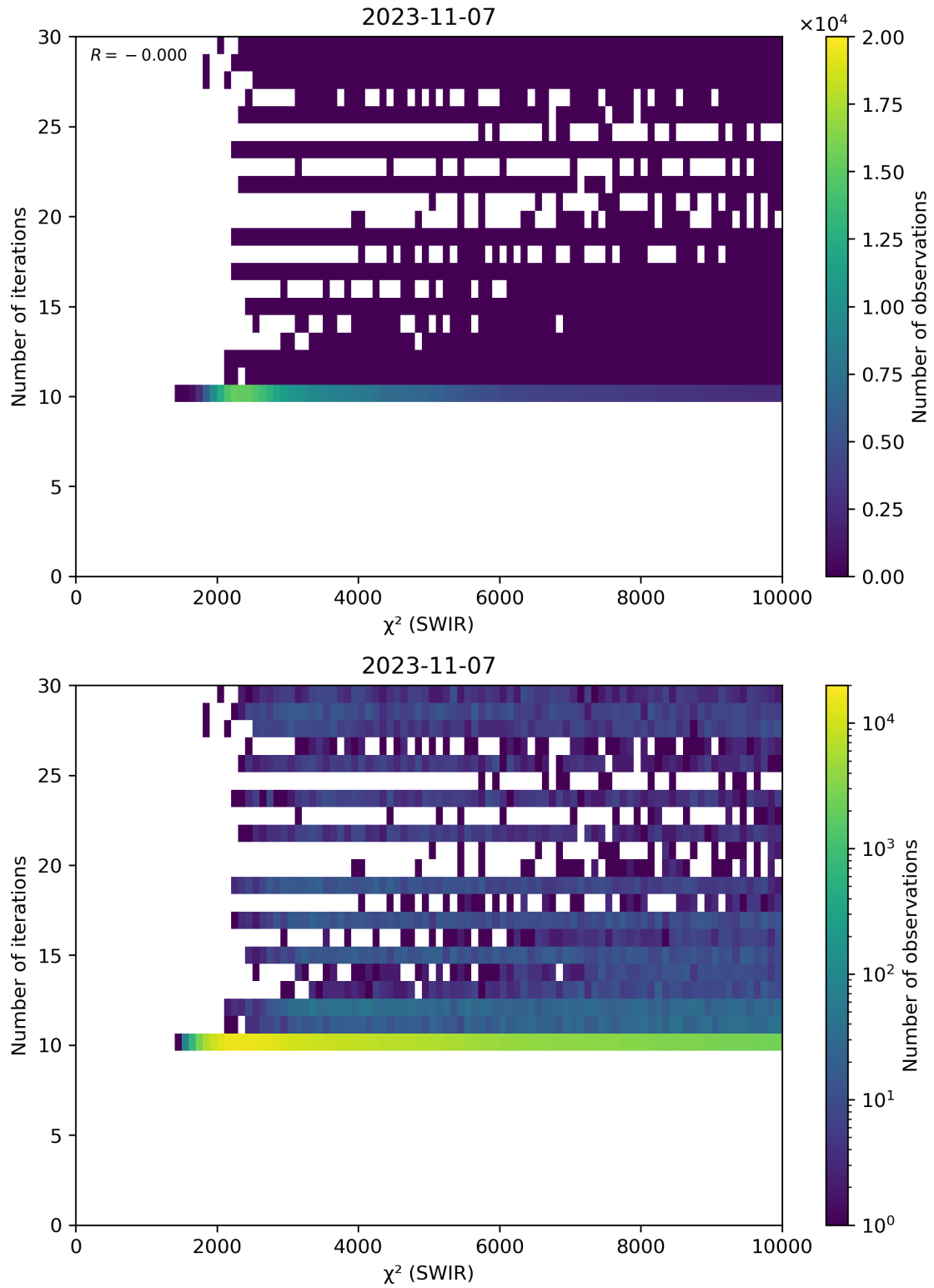
Figure 50: Scatter density plot of “ \chi^2 (SWIR)” against “Number of iterations” for 2023-11-07 to 2023-11-08.
