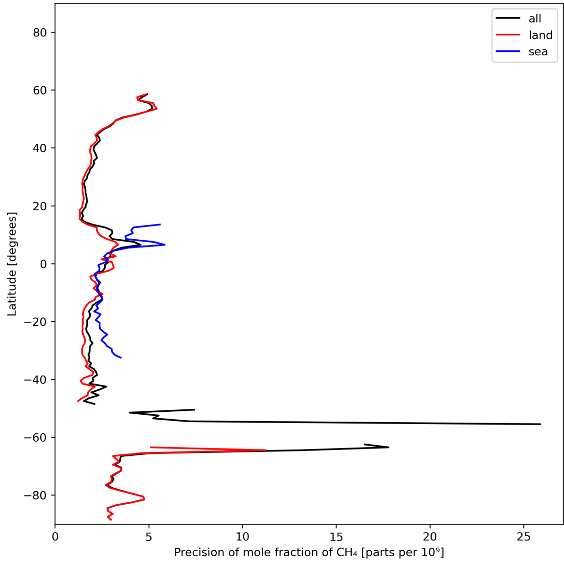
Figure 13: Zonal average of “Precision of mole fraction of CH 4 ” for 2023-11-07 to 2023-11-08.
