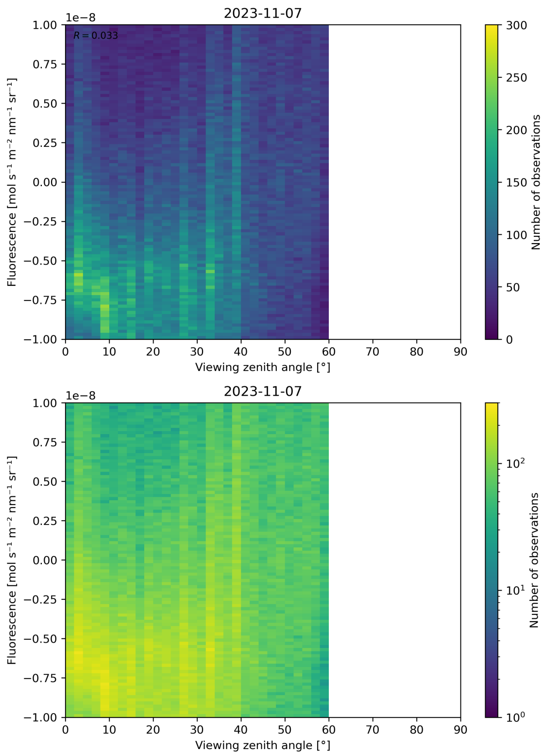
Figure 108: Scatter density plot of “Viewing zenith angle” against “Fluorescence” for 2023-11-07 to 2023-11-08.
