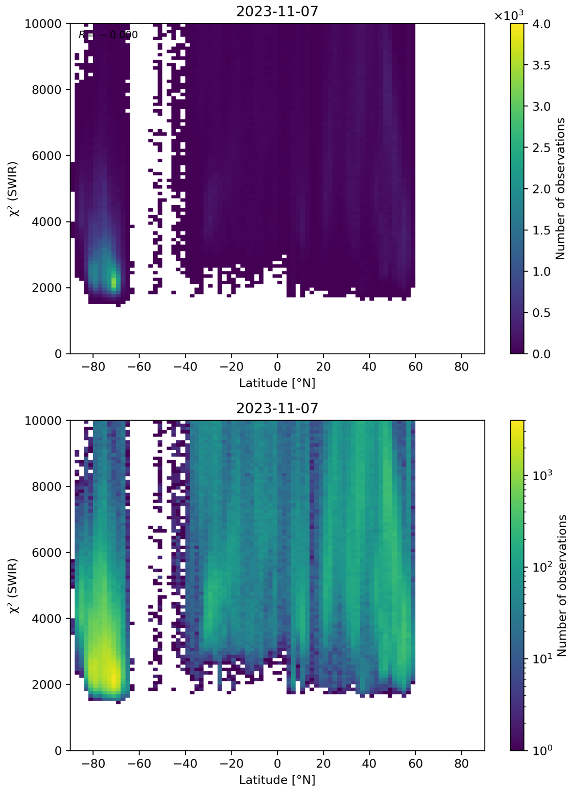
Figure 54: Scatter density plot of “Latitude” against “ \chi^2 (SWIR)” for 2023-11-07 to 2023-11-08.
