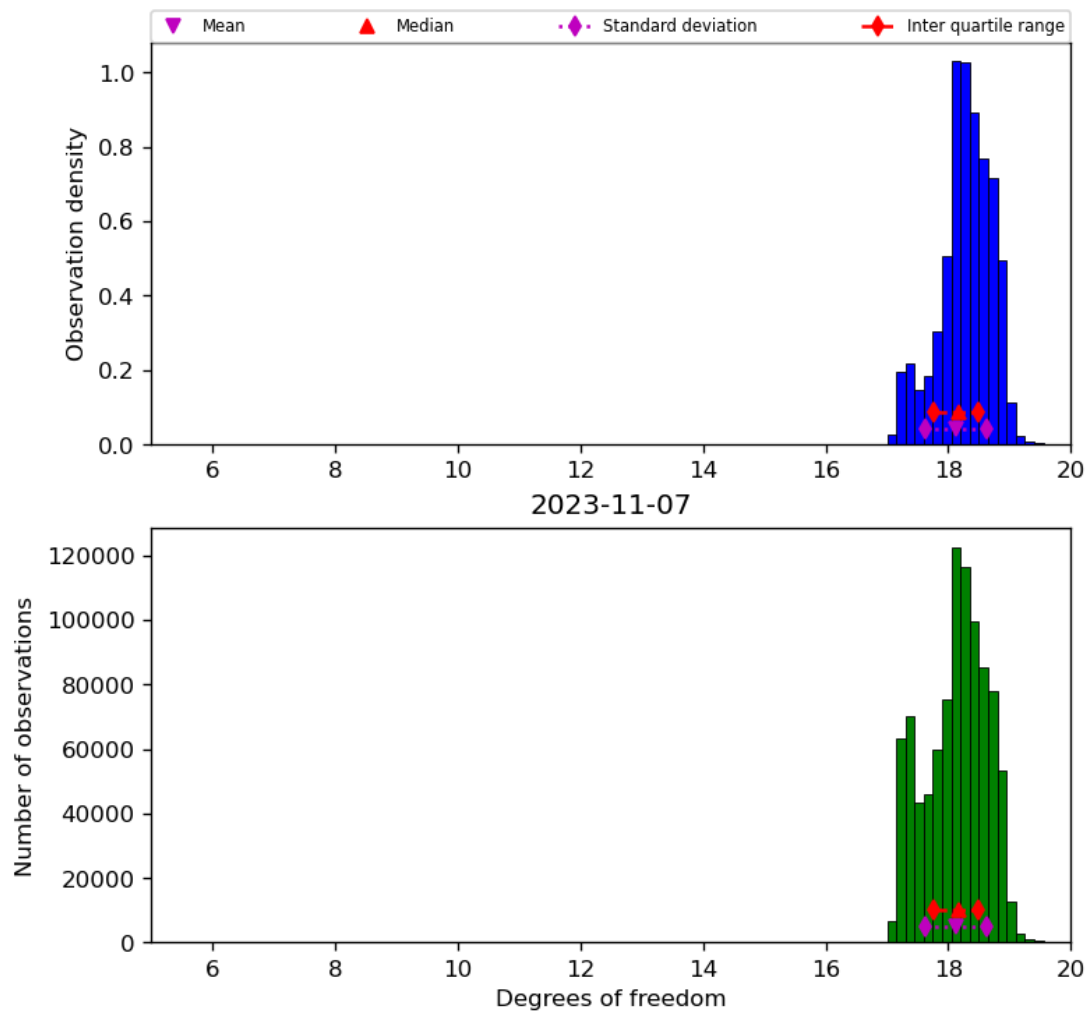
Figure 30: Histogram of “Degrees of freedom” for 2023-11-07 to 2023-11-08
