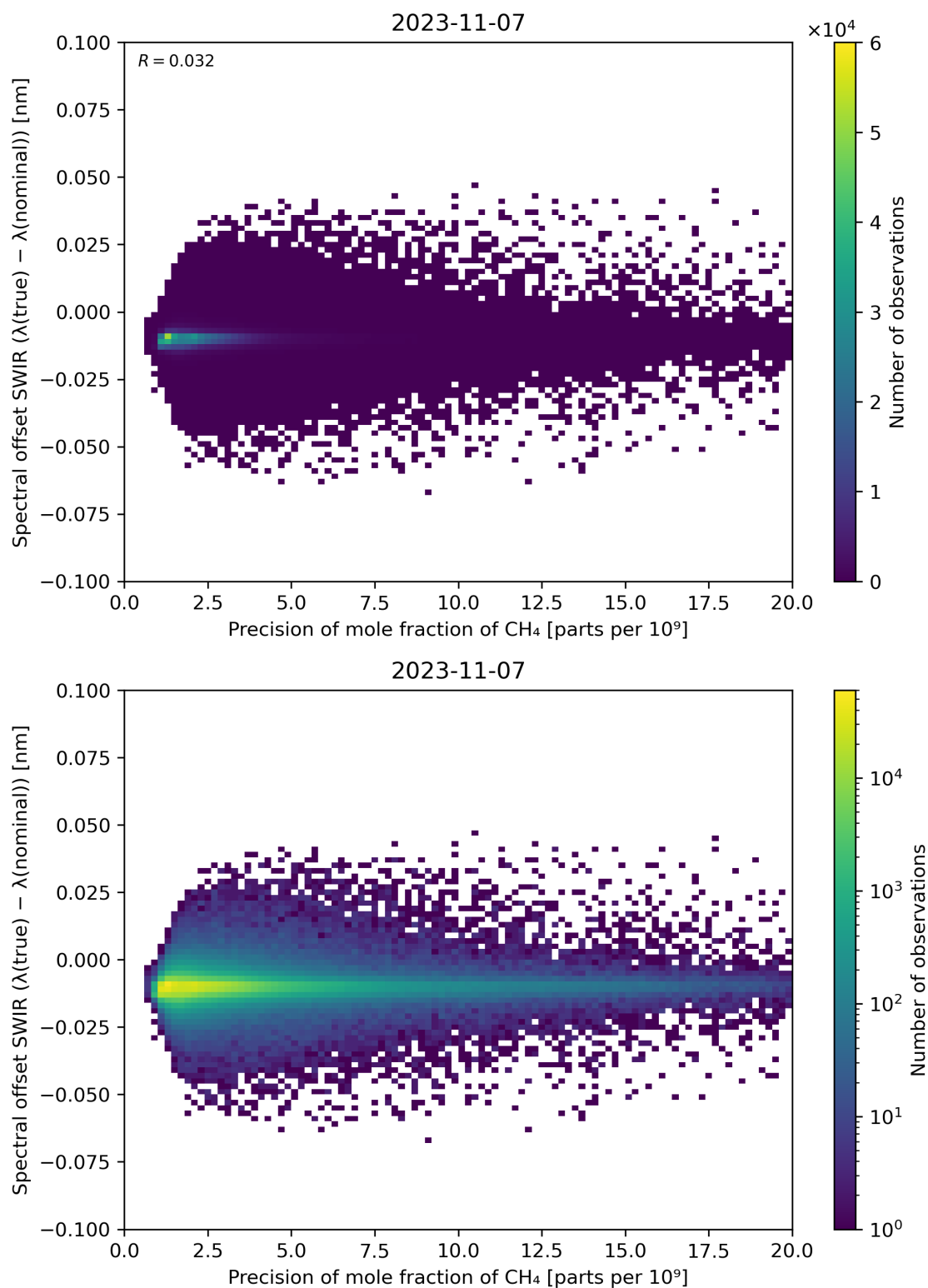
Figure 85: Scatter density plot of “Precision of mole fraction of \text{CH}_4 ” against “Spectral offset SWIR ( \lambda(\text{true}) - \lambda(\text{nominal}) )” for 2023-11-07 to 2023-11-08.
