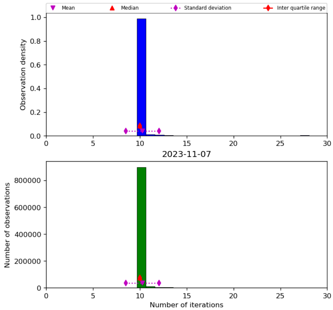
Figure 31: Histogram of “Number of iterations” for 2023-11-07 to 2023-11-08
