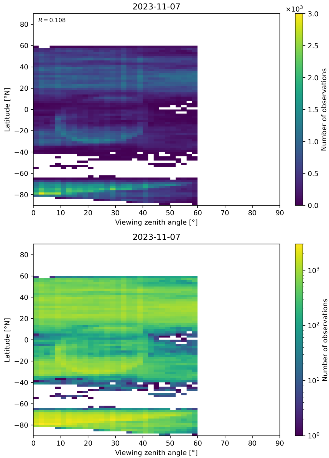
Figure 109: Scatter density plot of “Viewing zenith angle” against “Latitude” for 2023-11-07 to 2023-11-08.
