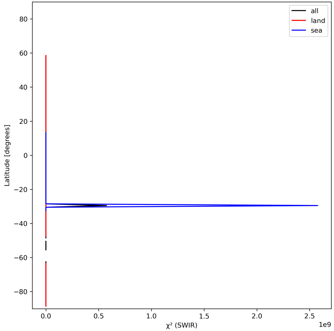
Figure 17: Zonal average of “ \chi^2 (SWIR)” for 2023-11-07 to 2023-11-08.
