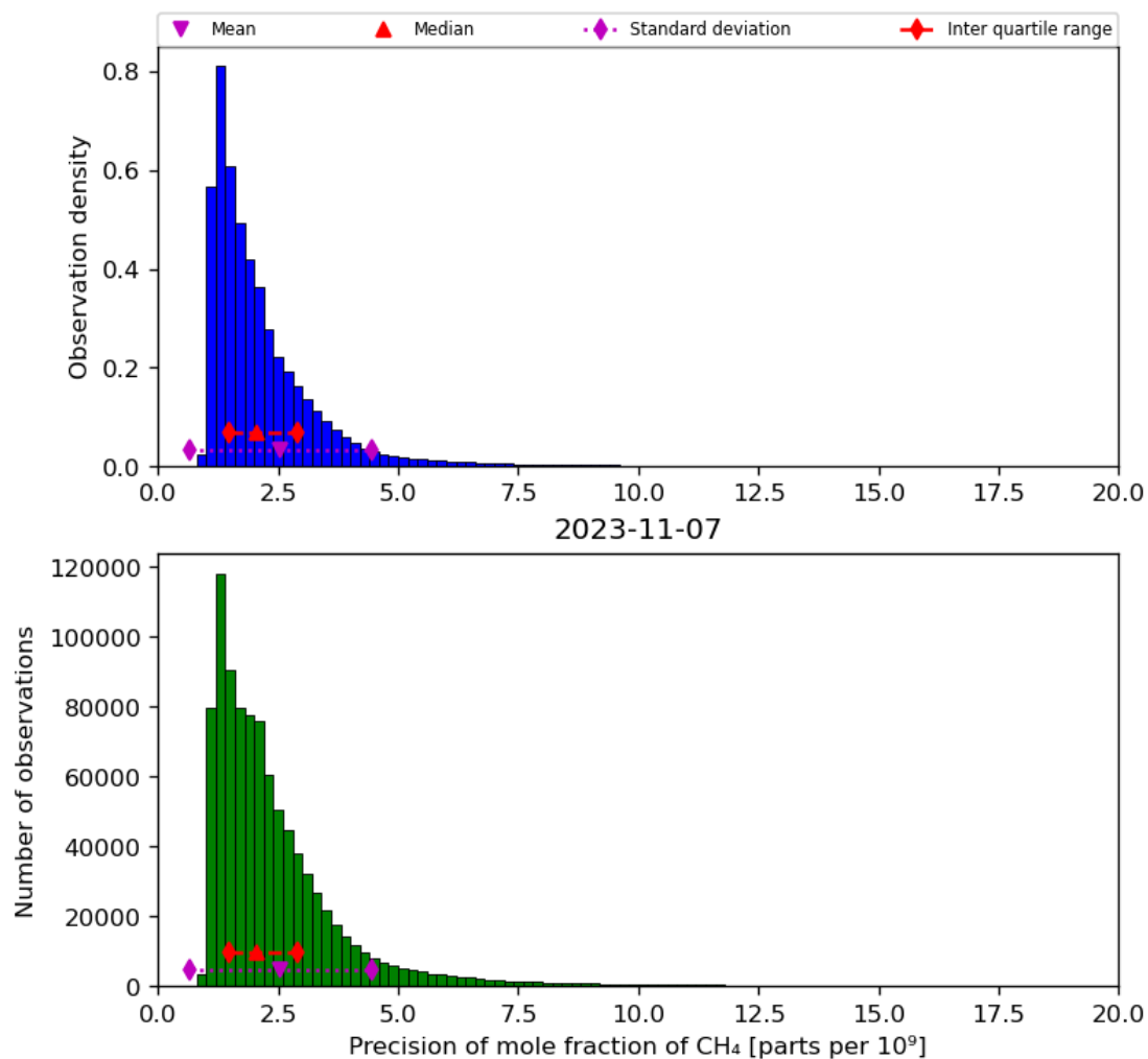
Figure 24: Histogram of “Precision of mole fraction of CH 4 ” for 2023-11-07 to 2023-11-08
