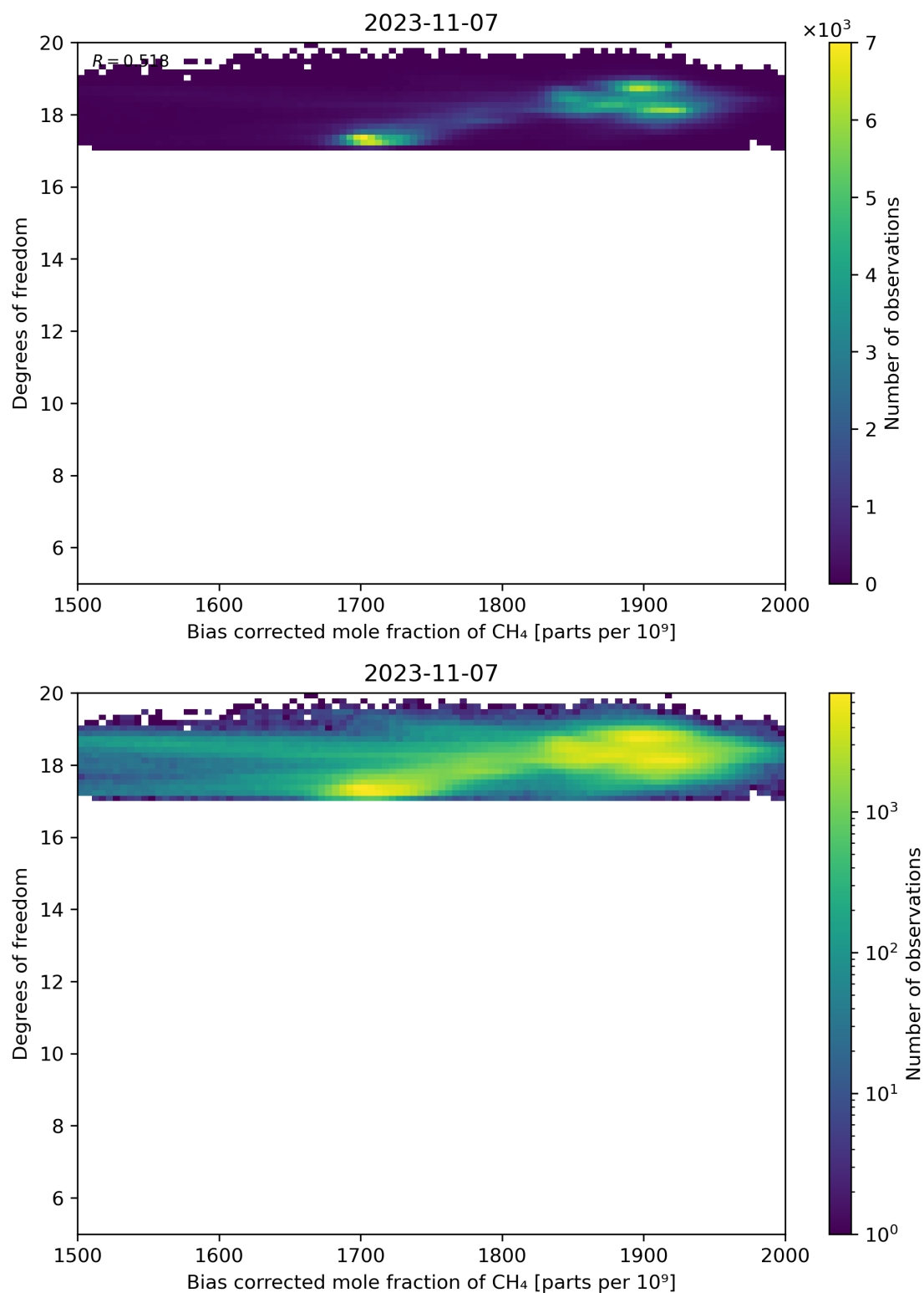
Figure 65: Scatter density plot of “Bias corrected mole fraction of CH 4 ” against “Degrees of freedom” for 2023-11-07 to 2023-11-08.
