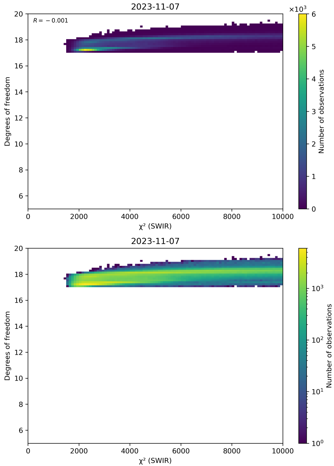
Figure 48: Scatter density plot of “ \chi^2 (SWIR)” against “Degrees of freedom” for 2023-11-07 to 2023-11-08.
