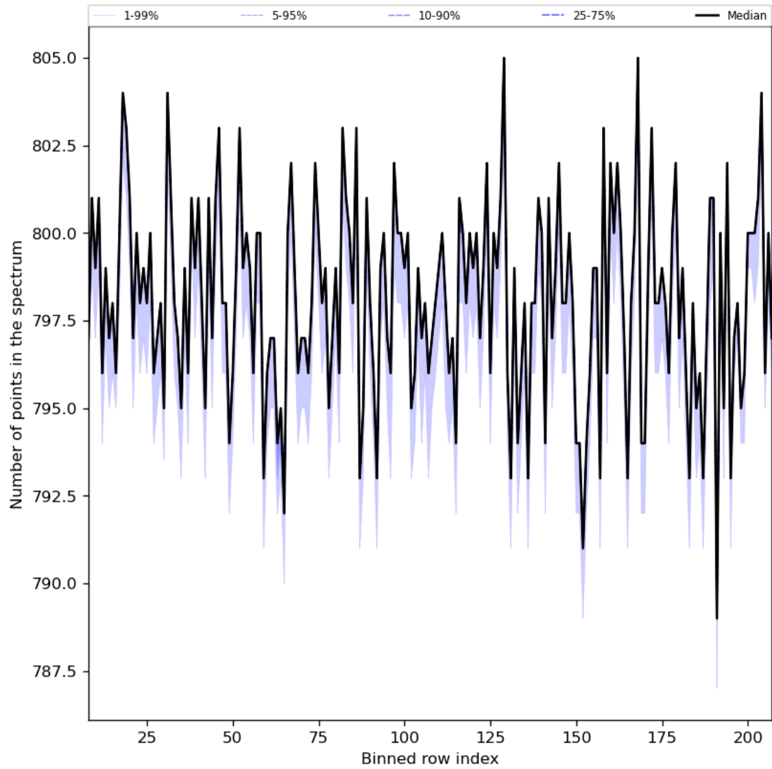
Figure 37: Along track statistics of “Number of points in the spectrum” for 2023-11-07 to 2023-11-08
