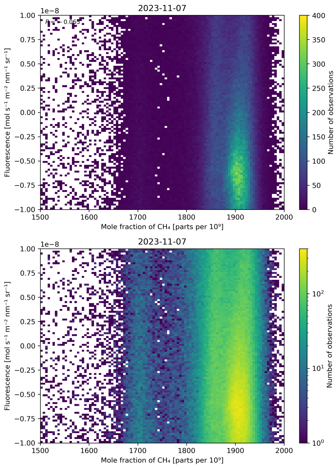
Figure 73: Scatter density plot of “Mole fraction of CH 4 ” against “Fluorescence” for 2023-11-07 to 2023-11-08.
