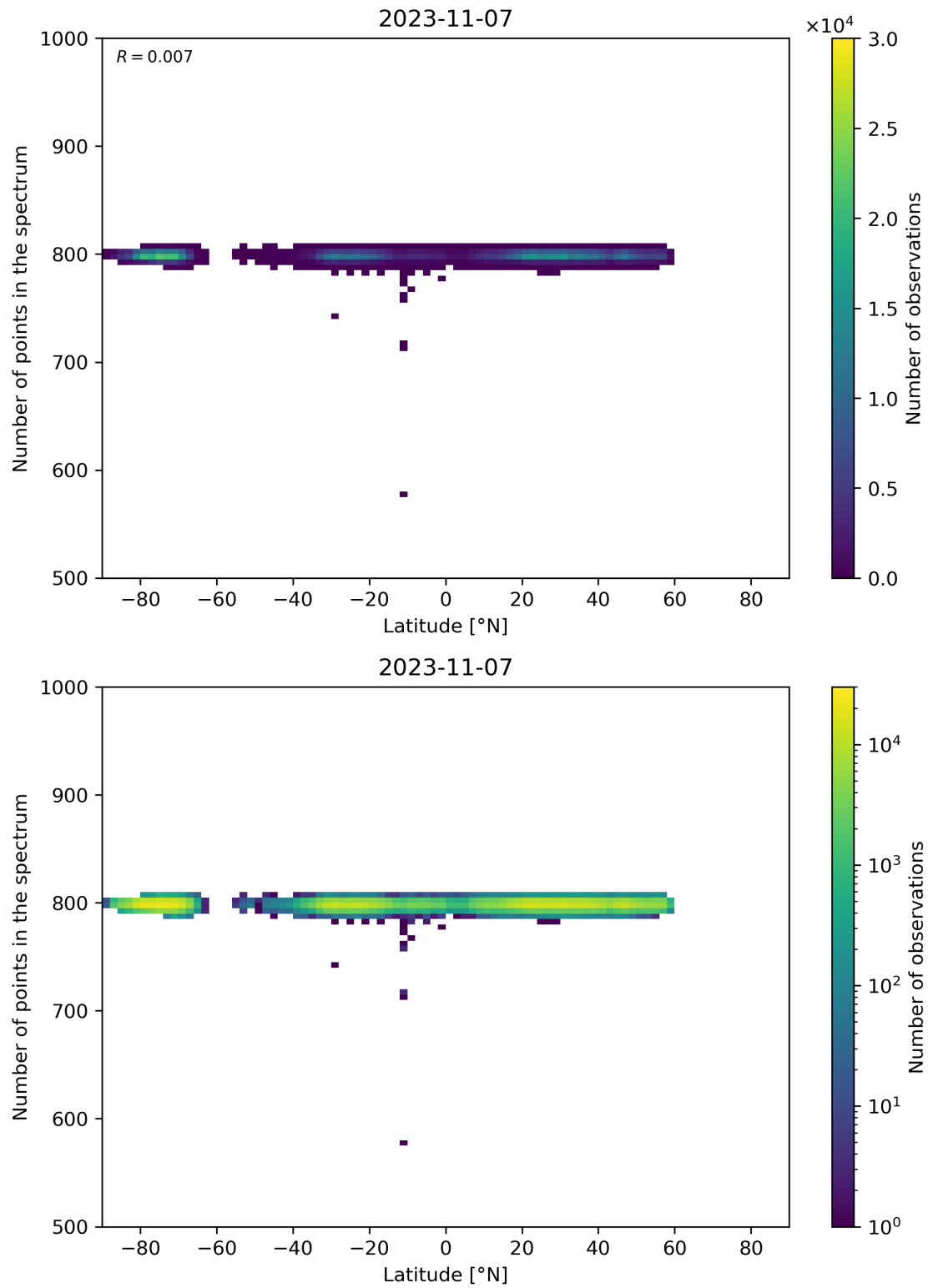
Figure 61: Scatter density plot of “Latitude” against “Number of points in the spectrum” for 2023-11-07 to 2023-11-08.
