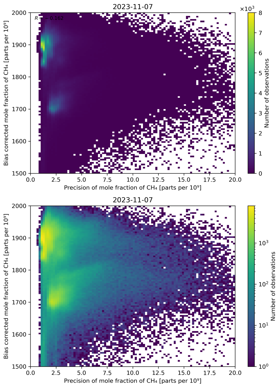
Figure 82: Scatter density plot of “Precision of mole fraction of CH 4 ” against “Bias corrected mole fraction of CH 4 ” for 2023-11-07 to 2023-11-08.
