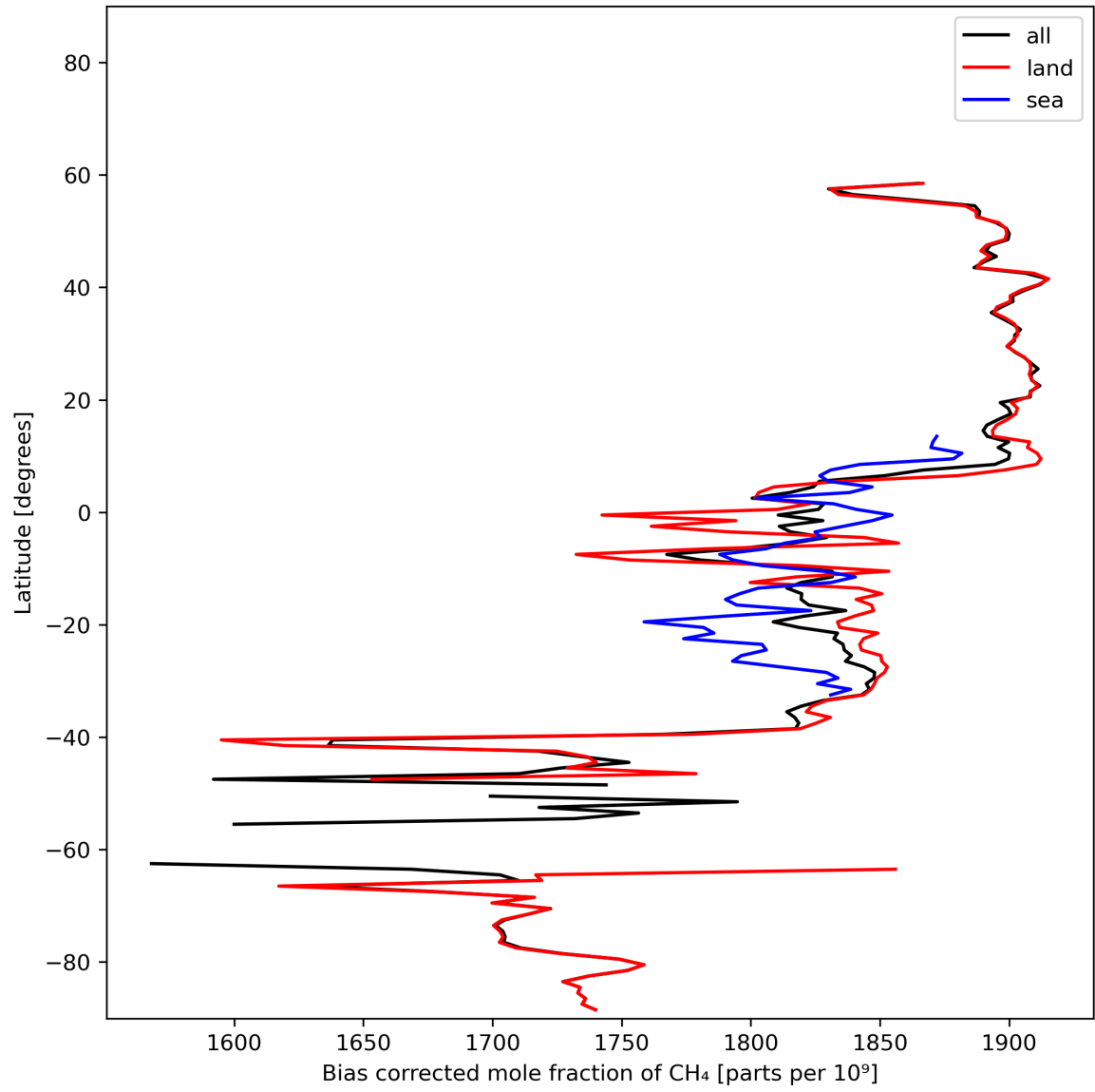
Figure 14: Zonal average of “Bias corrected mole fraction of \text{CH}_4 ” for 2023-11-07 to 2023-11-08.
