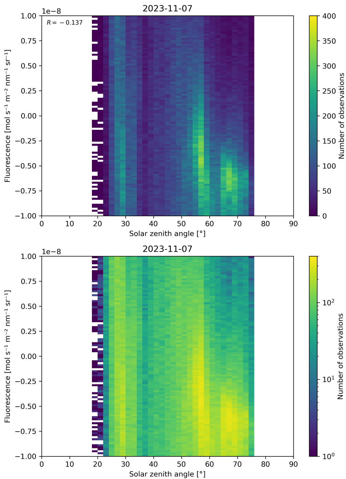
Figure 97: Scatter density plot of “Solar zenith angle” against “Fluorescence” for 2023-11-07 to 2023-11-08.
