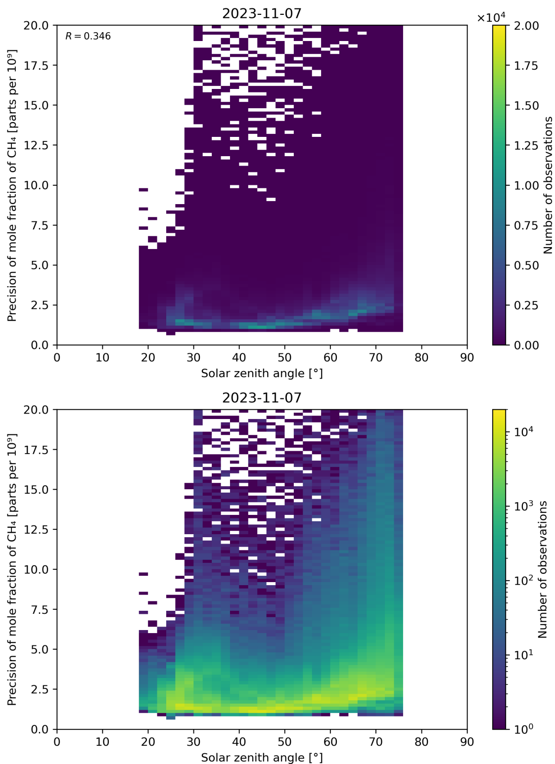
Figure 101: Scatter density plot of “Solar zenith angle” against “Precision of mole fraction of CH 4 ” for 2023-11-07 to 2023-11-08.
