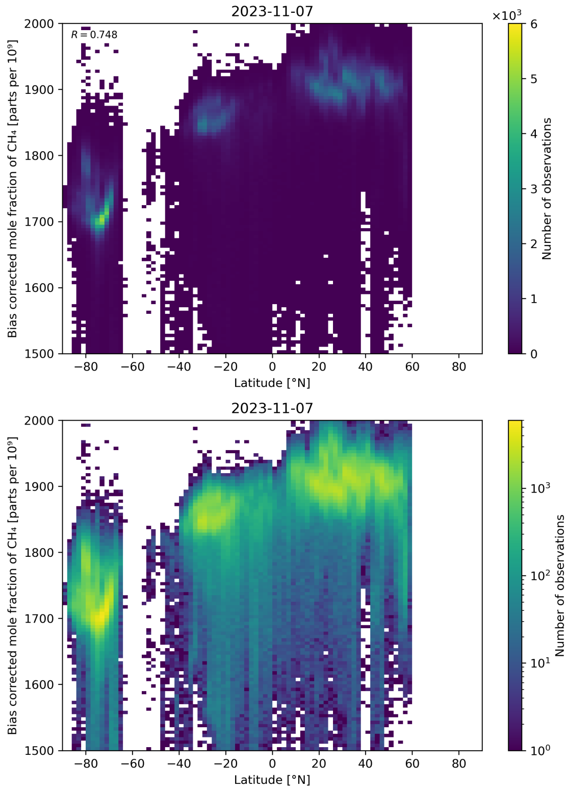
Figure 58: Scatter density plot of “Latitude” against “Bias corrected mole fraction of CH 4 ” for 2023-11-07 to 2023-11-08.
