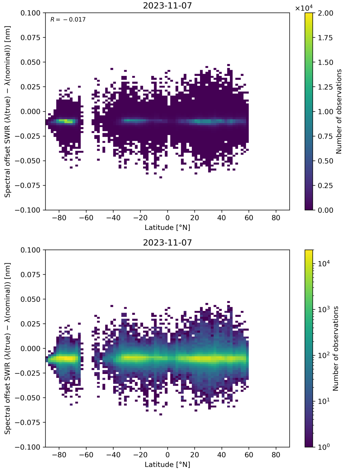
Figure 62: Scatter density plot of “Latitude” against “Spectral offset SWIR ( \lambda(\text{true}) - \lambda(\text{nominal}) )” for 2023-11-07 to 2023-11-08.
