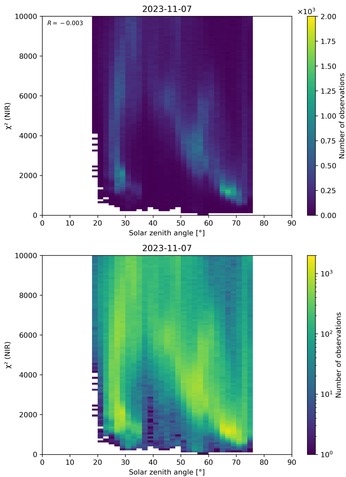
Figure 94: Scatter density plot of “Solar zenith angle” against “ \chi^2 (NIR)” for 2023-11-07 to 2023-11-08.
