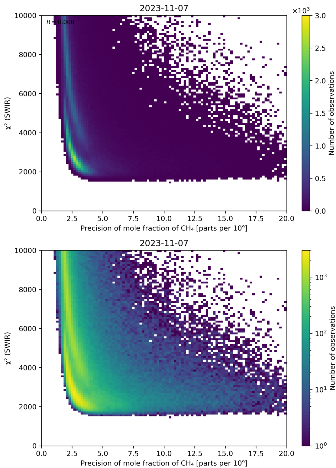
Figure 79: Scatter density plot of “Precision of mole fraction of CH 4 ” against “ \chi^2 (SWIR)” for 2023-11-07 to 2023-11-08.
