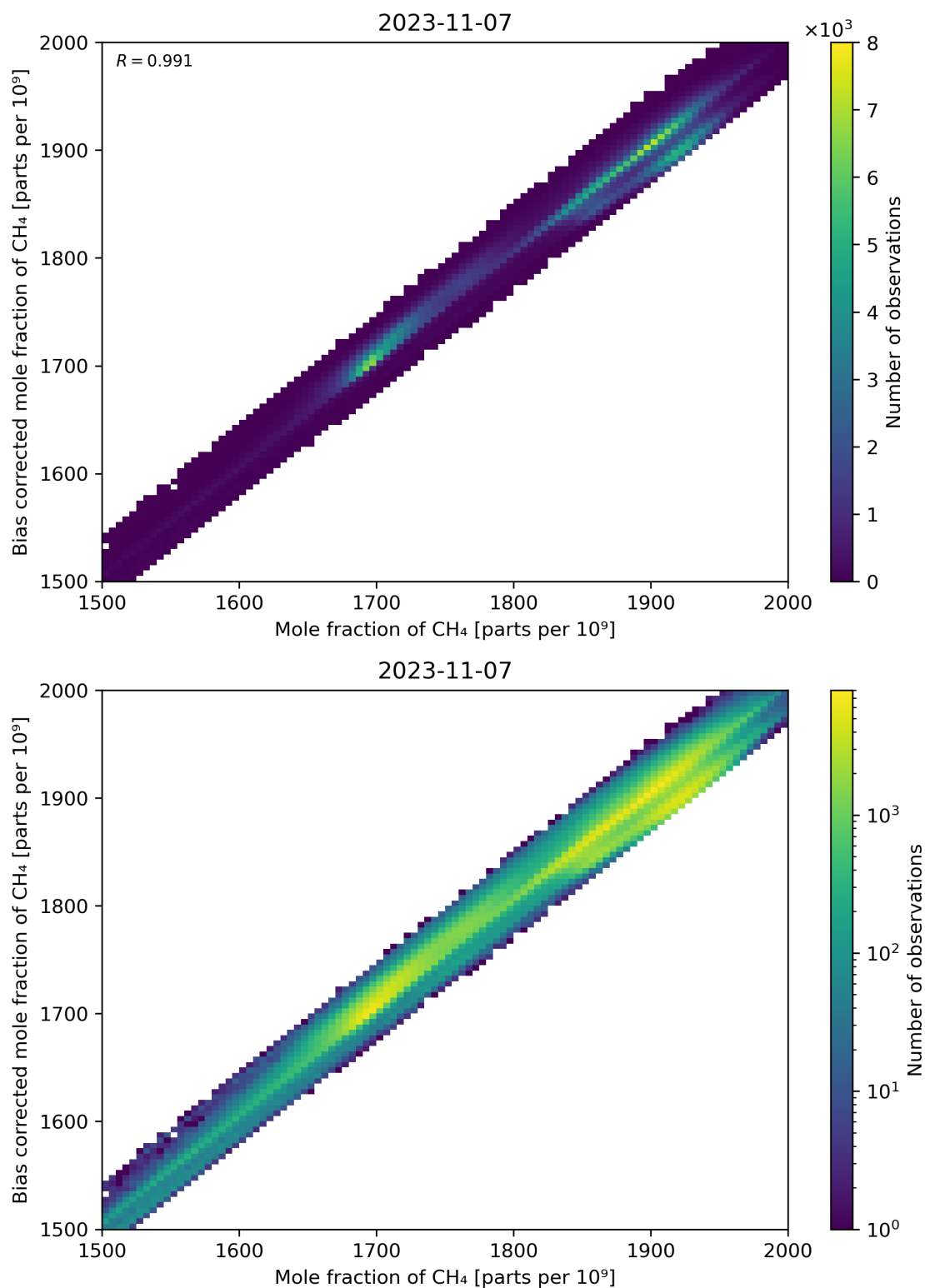
Figure 74: Scatter density plot of “Mole fraction of CH 4 ” against “Bias corrected mole fraction of CH 4 ” for 2023-11-07 to 2023-11-08.
