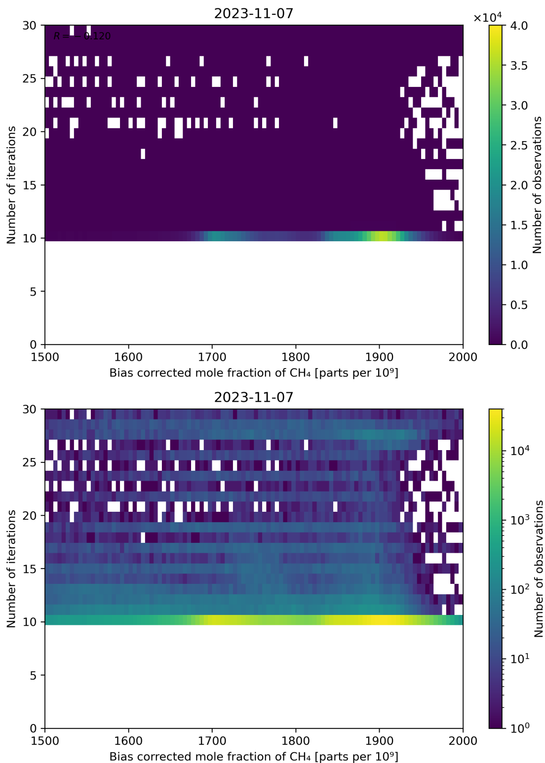
Figure 67: Scatter density plot of “Bias corrected mole fraction of CH 4 ” against “Number of iterations” for 2023-11-07 to 2023-11-08.
