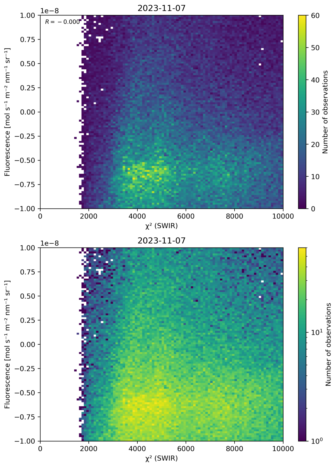
Figure 49: Scatter density plot of “ \chi^2 (SWIR)” against “Fluorescence” for 2023-11-07 to 2023-11-08.
