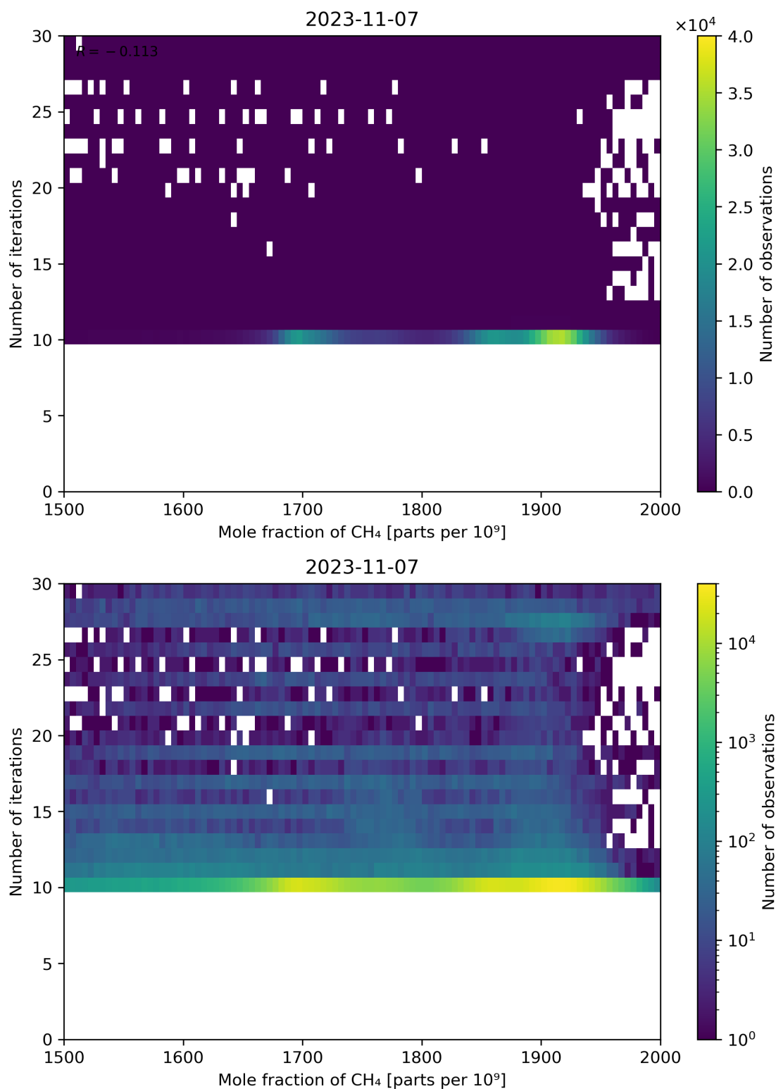
Figure 76: Scatter density plot of “Mole fraction of CH 4 ” against “Number of iterations” for 2023-11-07 to 2023-11-08.
