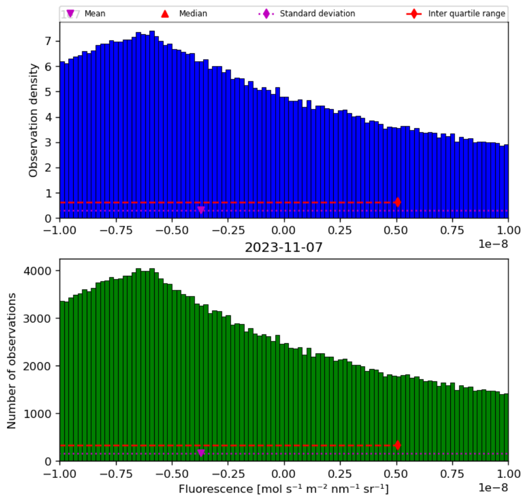
Figure 32: Histogram of “Fluorescence” for 2023-11-07 to 2023-11-08
