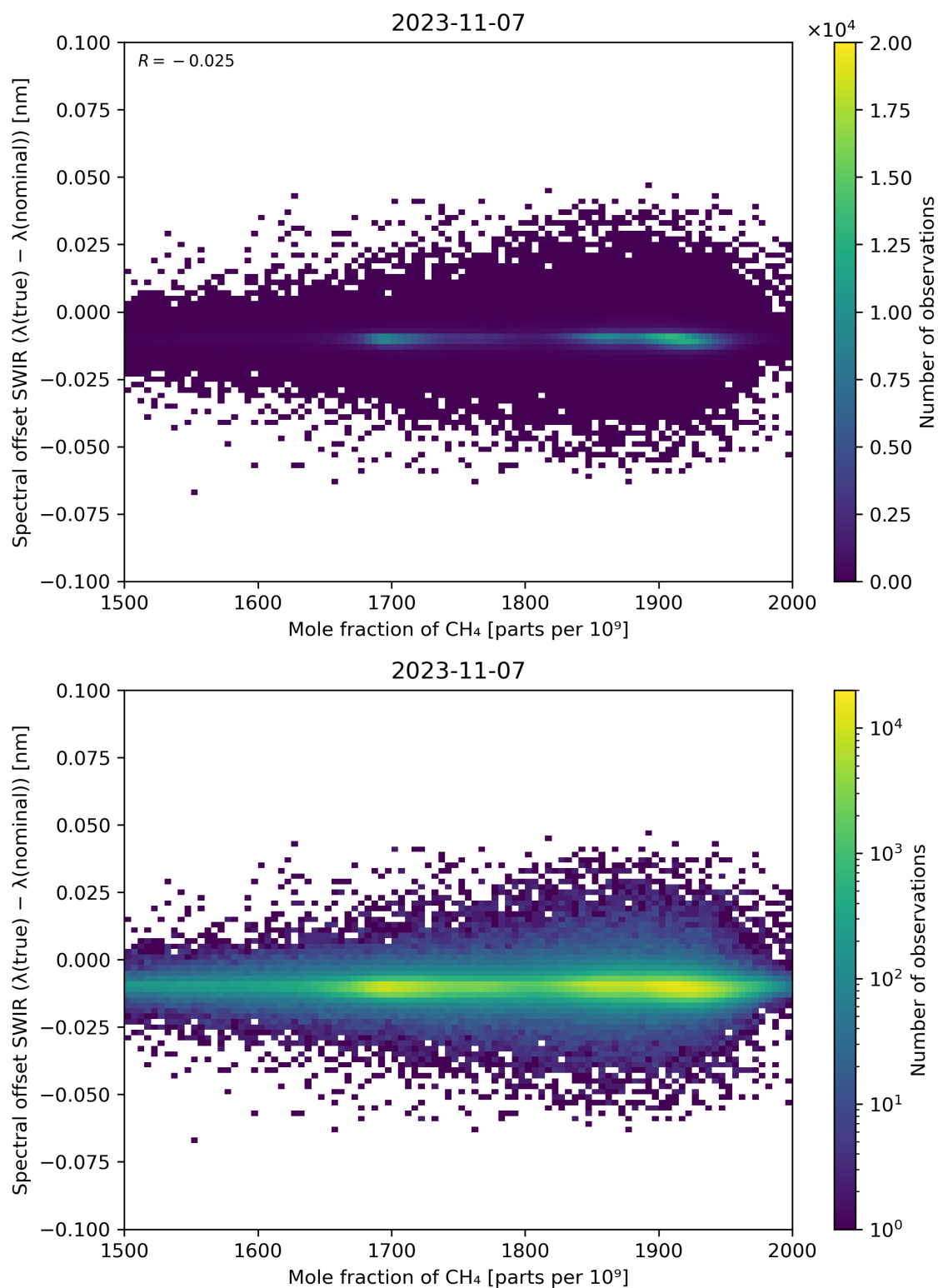
Figure 86: Scatter density plot of “Mole fraction of CH 4 ” against “Spectral offset SWIR ( \lambda(\text{true}) - \lambda(\text{nominal}) )” for 2023-11-07 to 2023-11-08.
