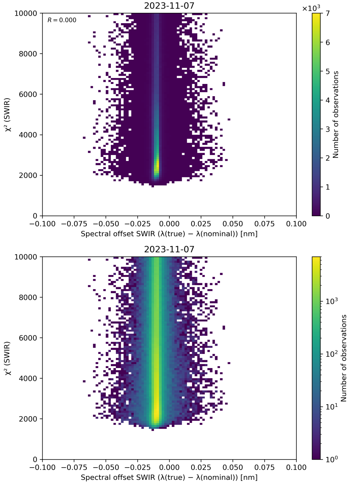
Figure 118: Scatter density plot of “Spectral offset SWIR ( \lambda(\text{true}) - \lambda(\text{nominal}) )” against “ \chi^2 (SWIR)” for 2023-11-07 to 2023-11-08.
