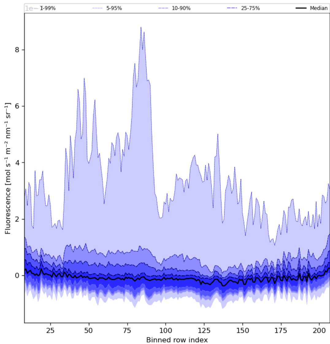
Figure 43: Along track statistics of “Fluorescence” for 2023-11-07 to 2023-11-08
