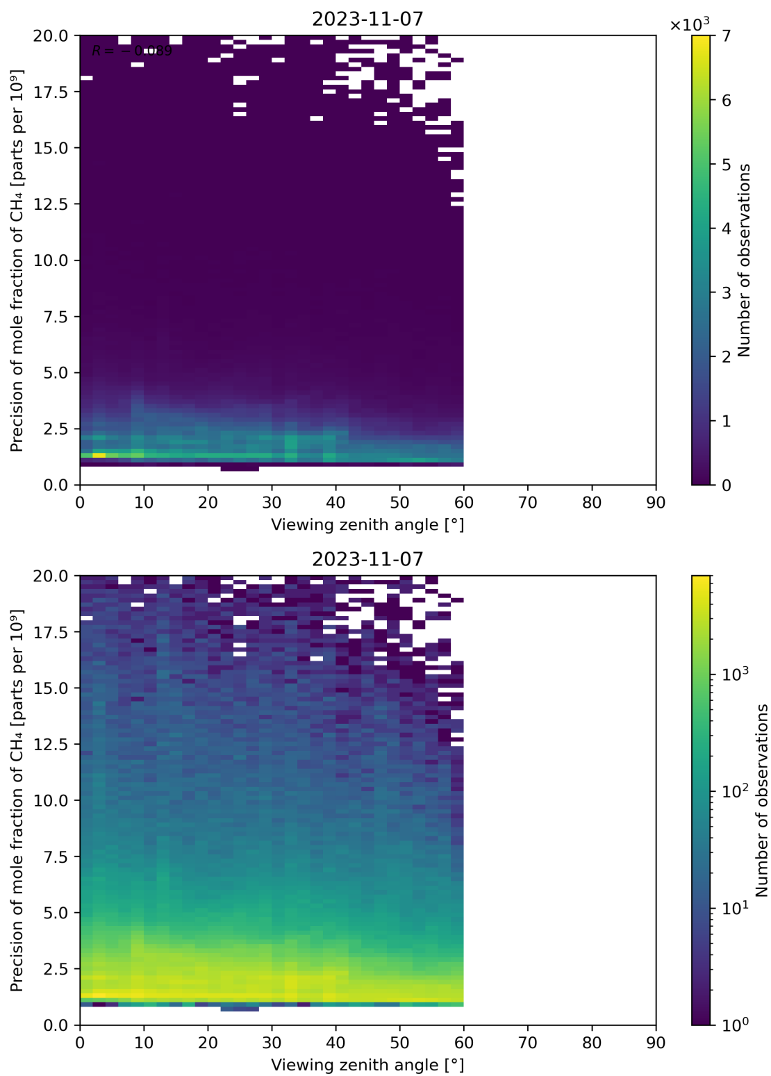
Figure 112: Scatter density plot of “Viewing zenith angle” against “Precision of mole fraction of CH 4 ” for 2023-11-07 to 2023-11-08.
