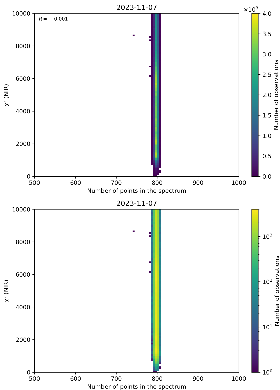
Figure 88: Scatter density plot of “Number of points in the spectrum” against “ \chi^2 (NIR)” for 2023-11-07 to 2023-11-08.
