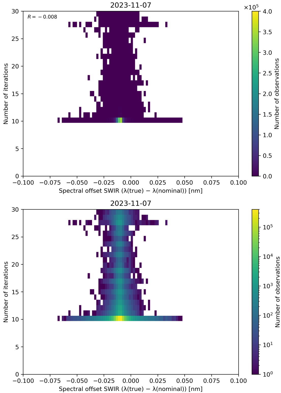
Figure 121: Scatter density plot of “Spectral offset SWIR ( \lambda(\text{true}) - \lambda(\text{nominal}) )” against “Number of iterations” for 2023-11-07 to 2023-11-08.
