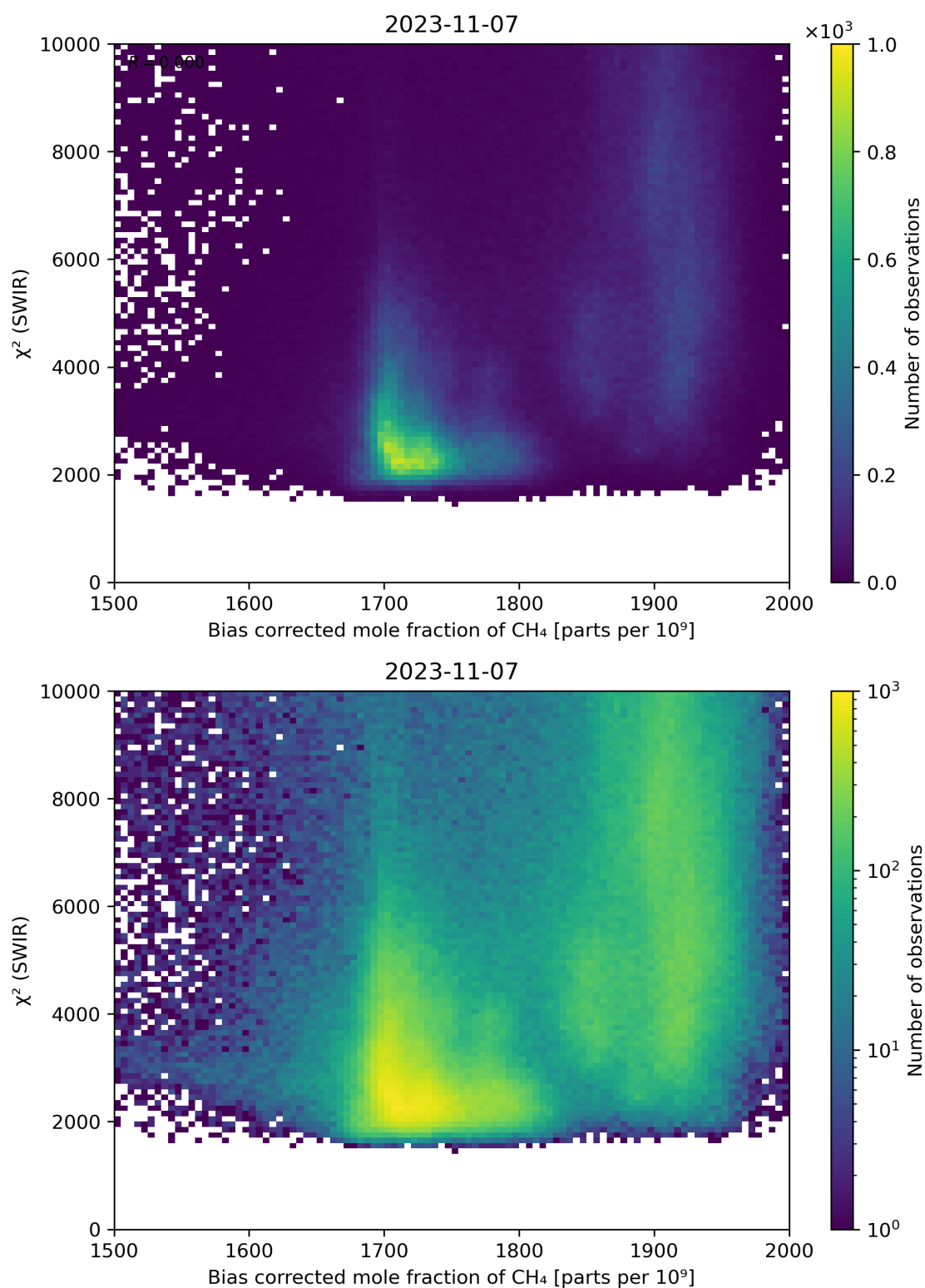
Figure 64: Scatter density plot of “Bias corrected mole fraction of CH 4 ” against “ \chi^2 (SWIR)” for 2023-11-07 to 2023-11-08.
