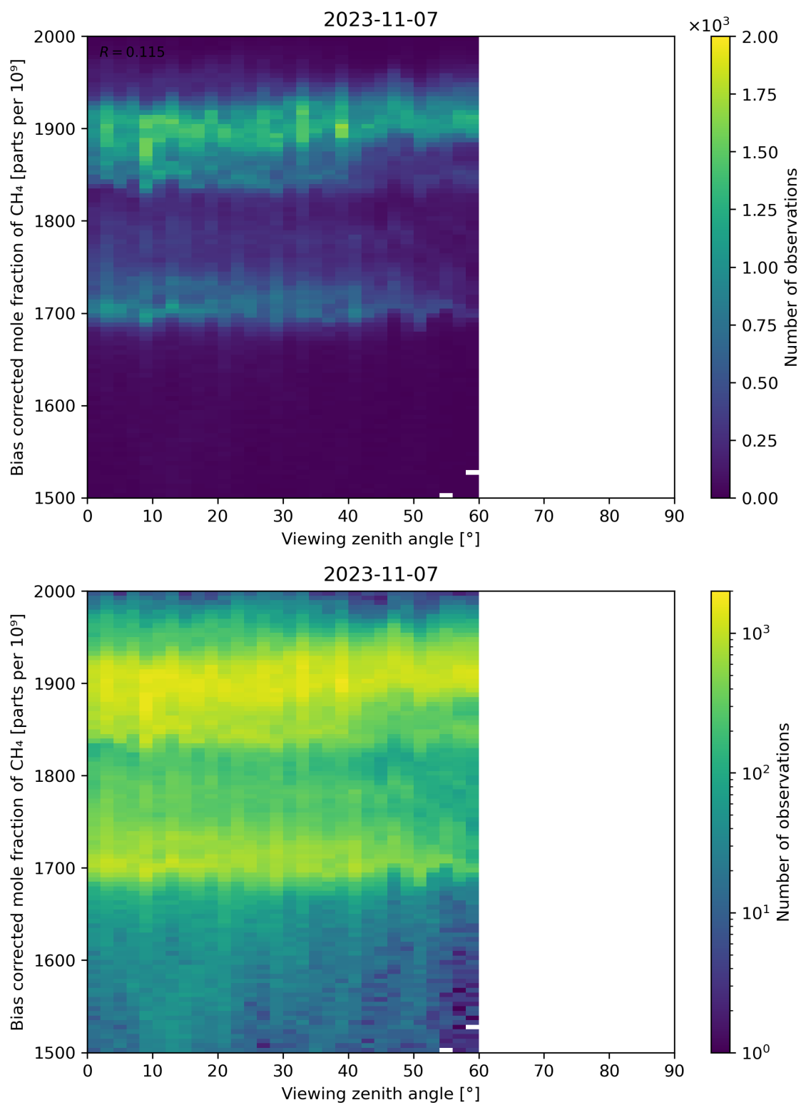
Figure 111: Scatter density plot of “Viewing zenith angle” against “Bias corrected mole fraction of CH 4 ” for 2023-11-07 to 2023-11-08.
