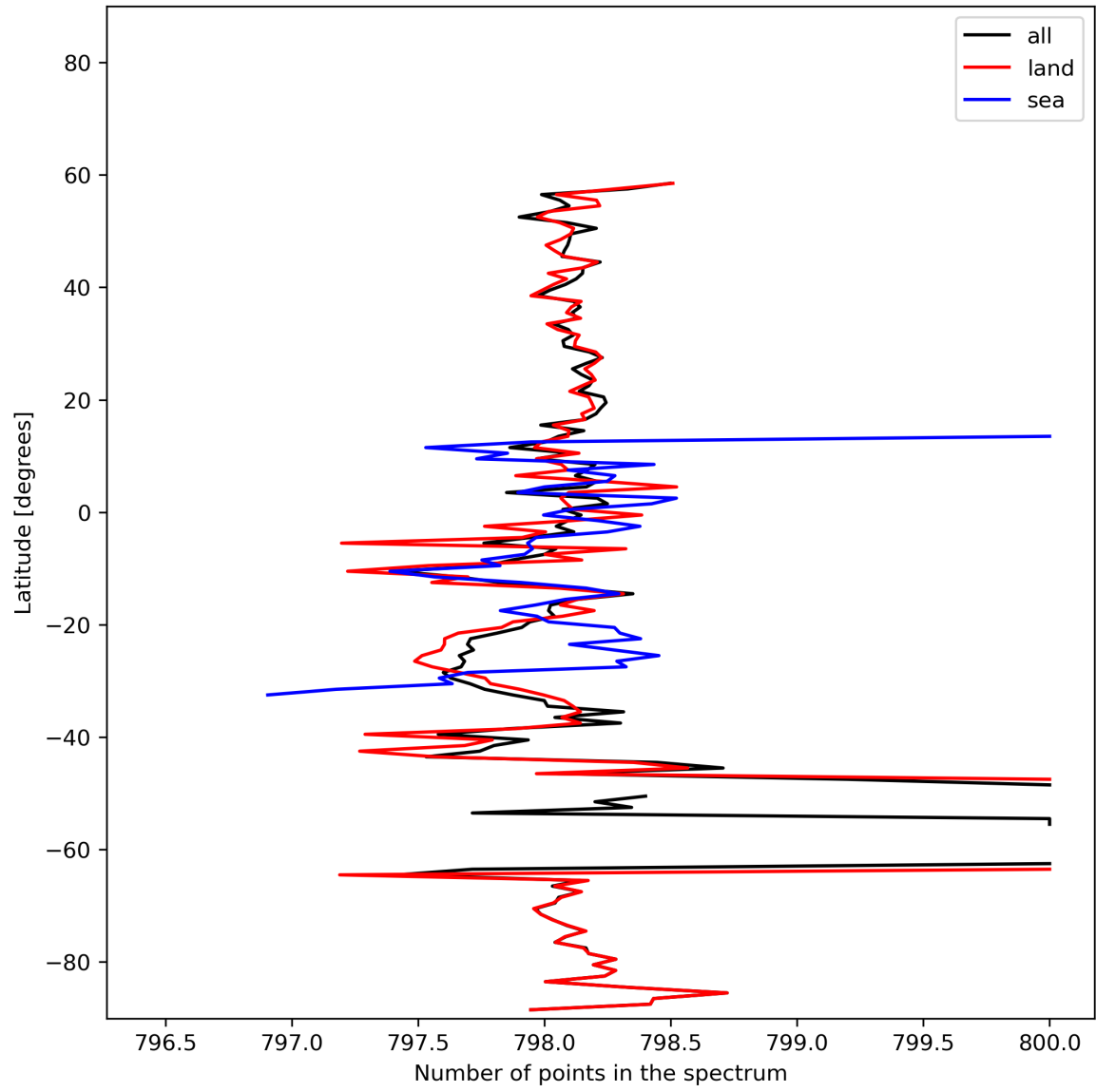
Figure 15: Zonal average of “Number of points in the spectrum” for 2023-11-07 to 2023-11-08.
