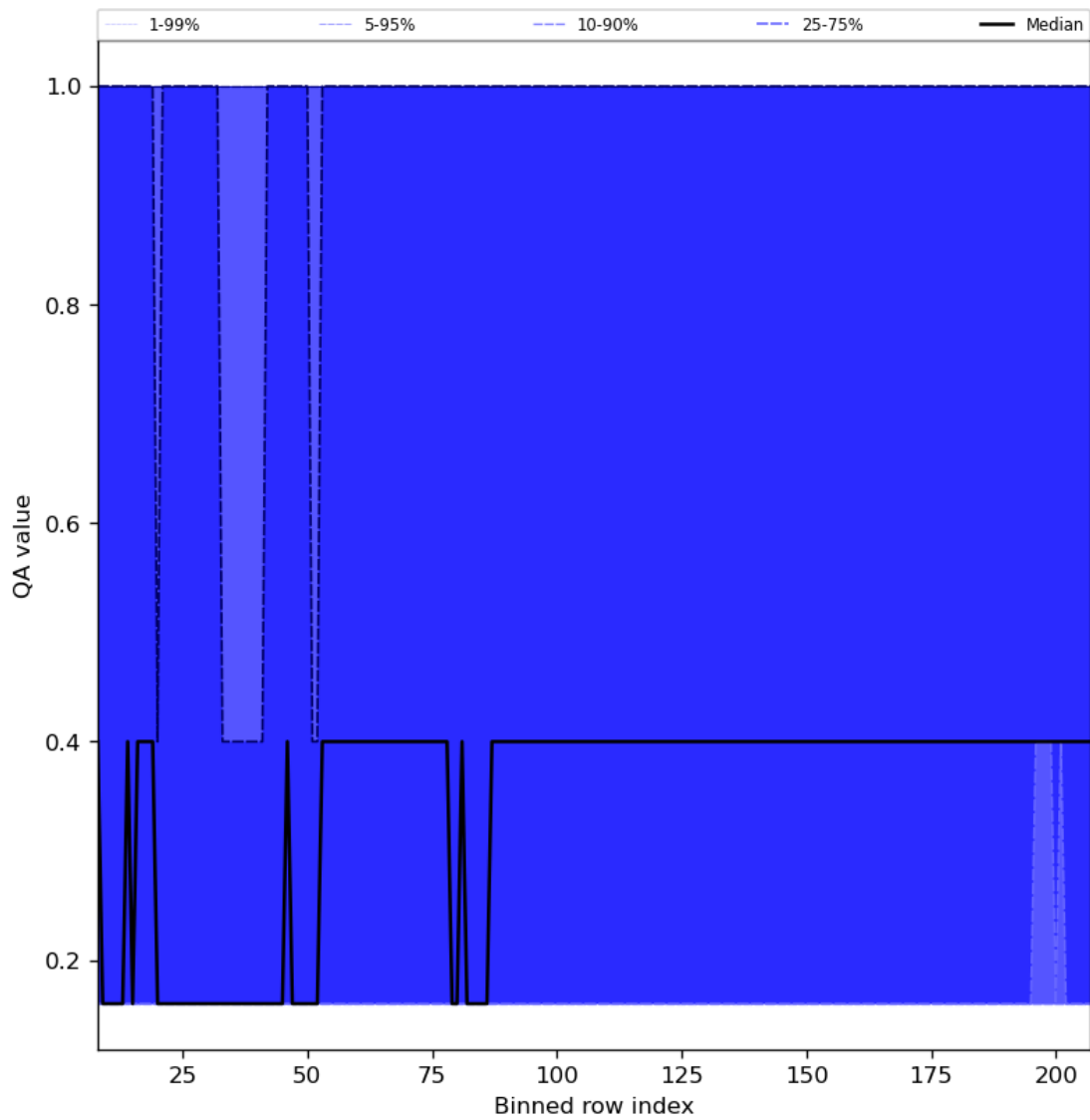
Figure 33: Along track statistics of “QA value” for 2023-11-07 to 2023-11-08
