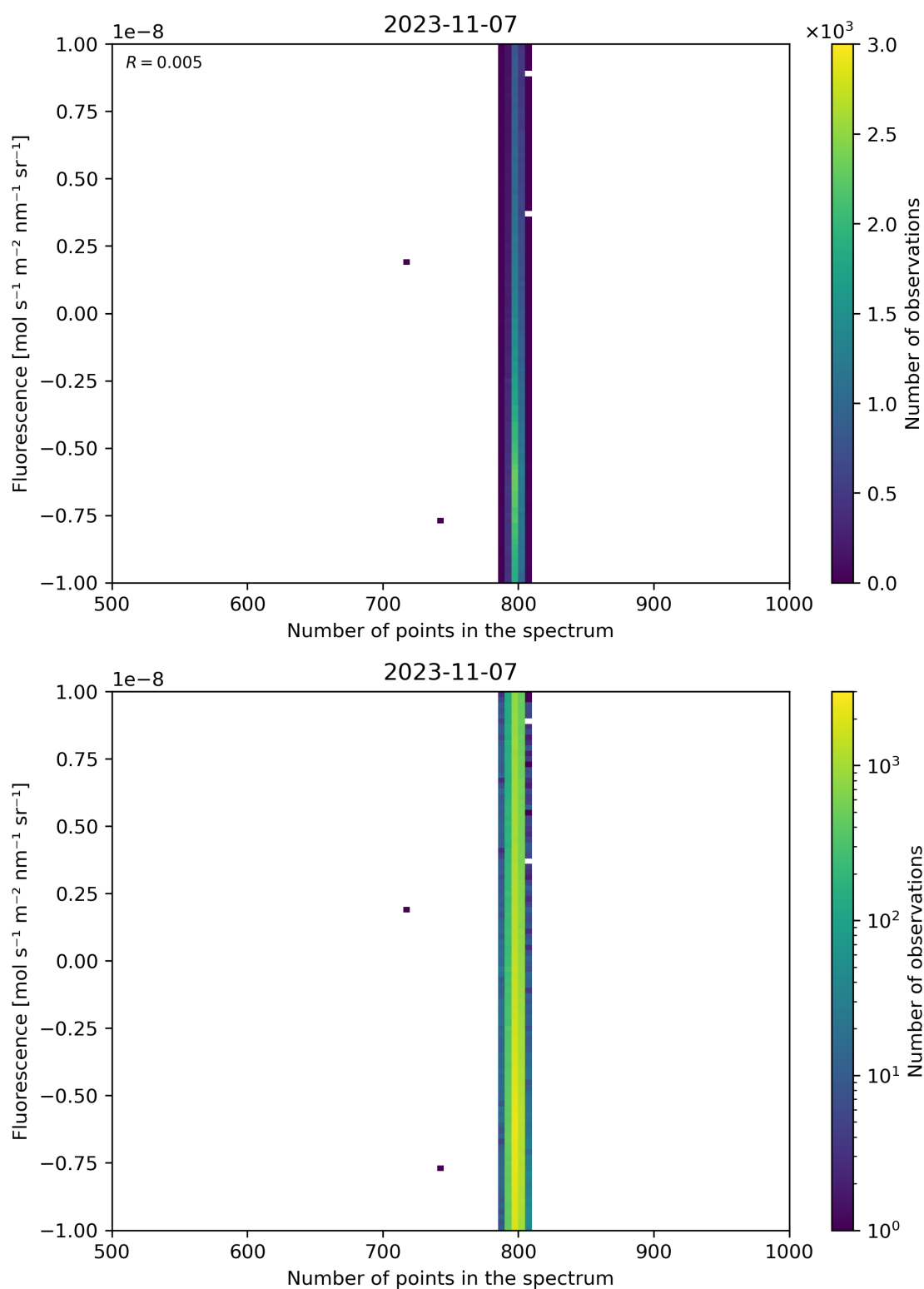
Figure 91: Scatter density plot of “Number of points in the spectrum” against “Fluorescence” for 2023-11-07 to 2023-11-08.
