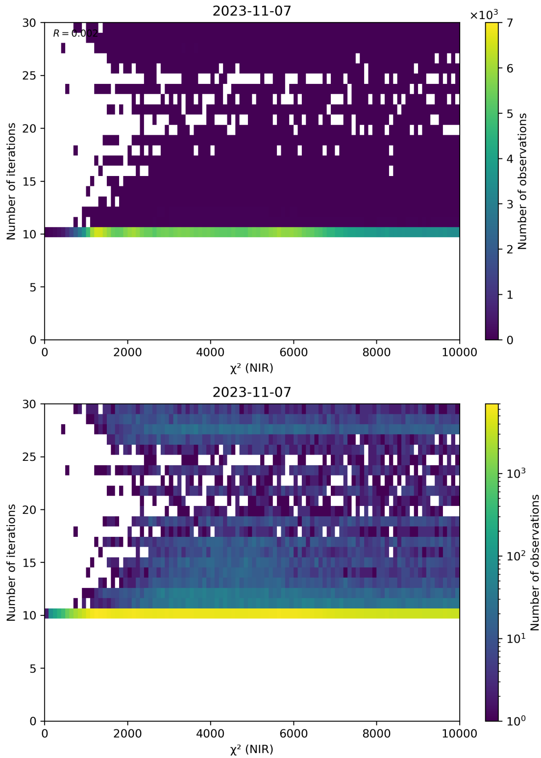
Figure 46: Scatter density plot of “ \chi^2 (NIR)” against “Number of iterations” for 2023-11-07 to 2023-11-08.
