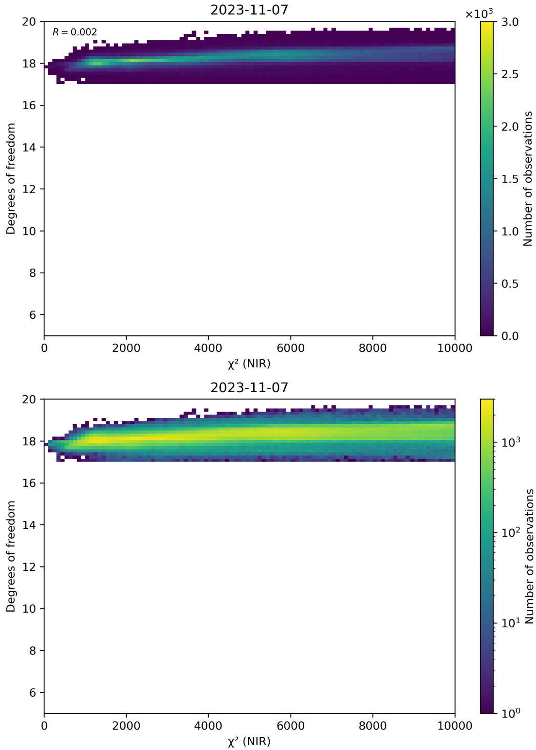
Figure 44: Scatter density plot of “ \chi^2 (NIR)” against “Degrees of freedom” for 2023-11-07 to 2023-11-08.
