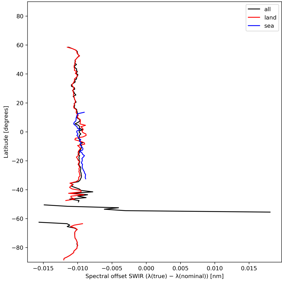
Figure 16: Zonal average of “Spectral offset SWIR ( \lambda(\text{true}) - \lambda(\text{nominal}) )” for 2023-11-07 to 2023-11-08.
