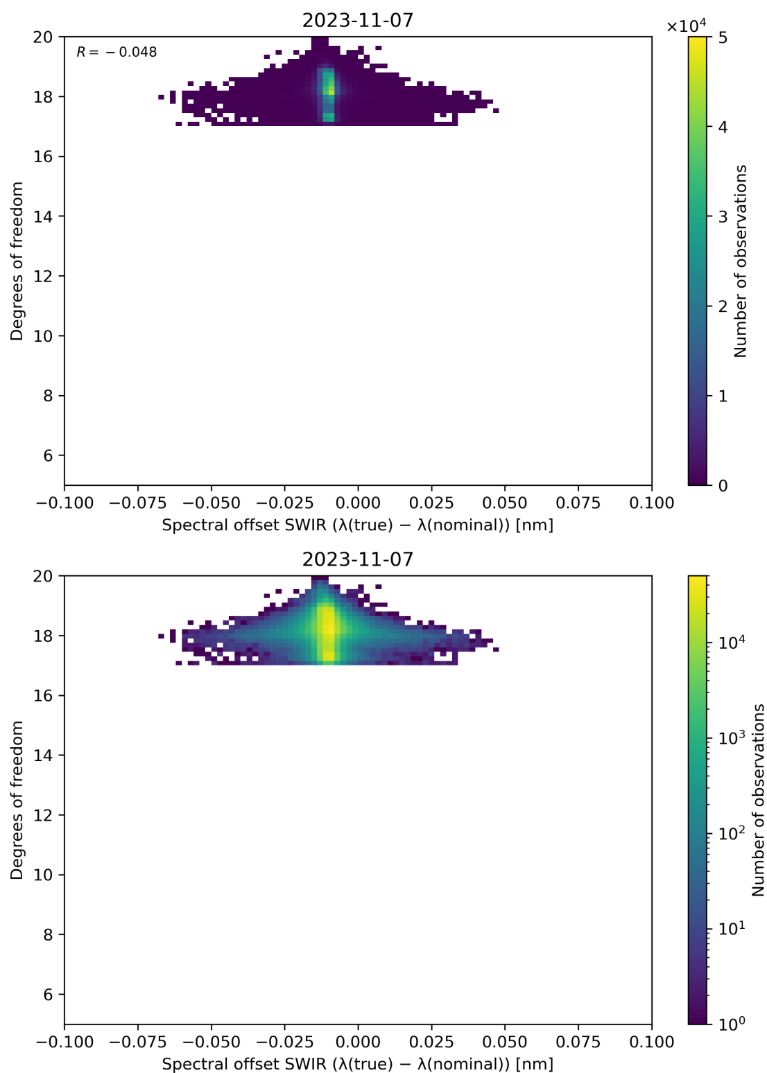
Figure 119: Scatter density plot of “Spectral offset SWIR ( \lambda(\text{true}) - \lambda(\text{nominal}) )” against “Degrees of freedom” for 2023-11-07 to 2023-11-08.
