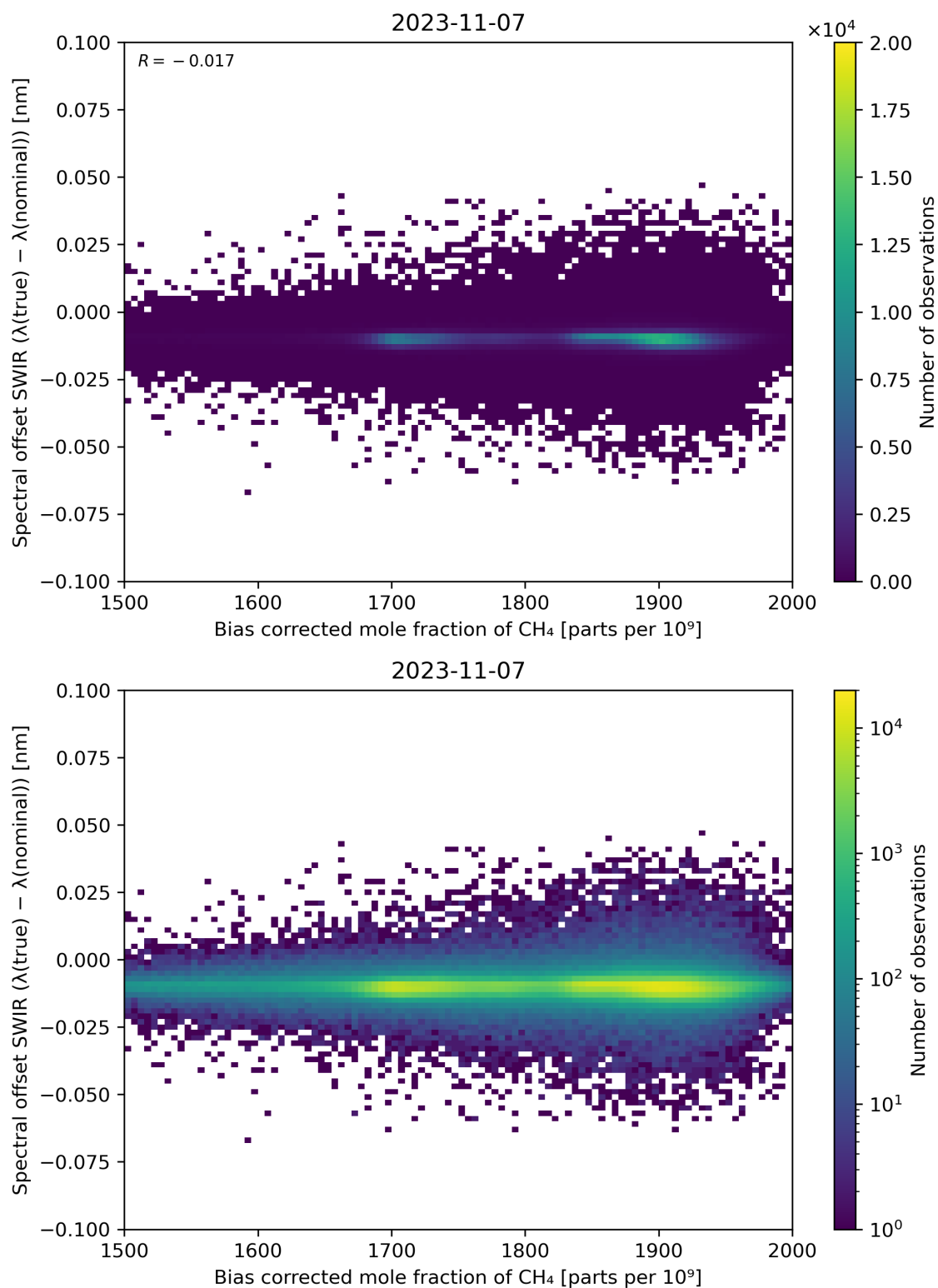
Figure 69: Scatter density plot of “Bias corrected mole fraction of \text{CH}_4 ” against “Spectral offset SWIR ( \lambda(\text{true}) - \lambda(\text{nominal}) )” for 2023-11-07 to 2023-11-08.
