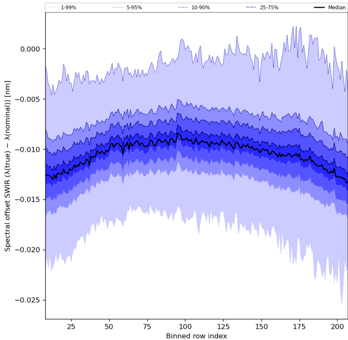
Figure 38: Along track statistics of “Spectral offset SWIR ( \lambda(\text{true}) - \lambda(\text{nominal}) )” for 2023-11-07 to 2023-11-08
