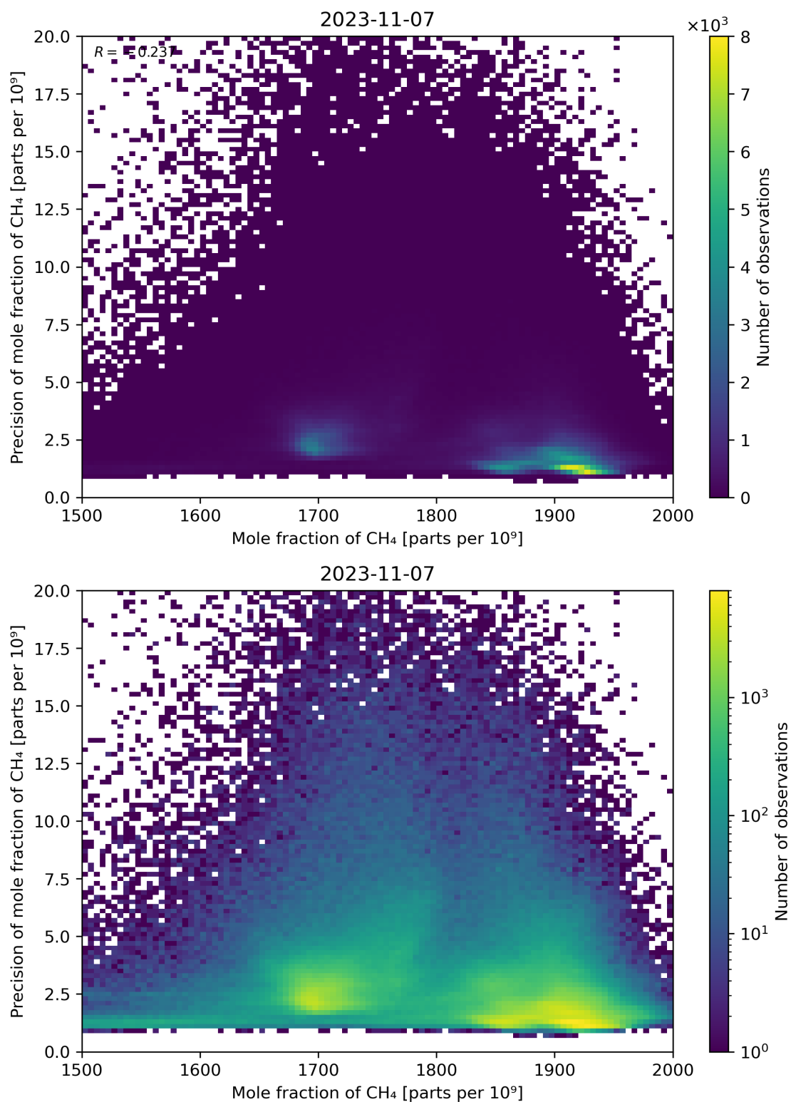
Figure 75: Scatter density plot of “Mole fraction of CH 4 ” against “Precision of mole fraction of CH 4 ” for 2023-11-07 to 2023-11-08.
