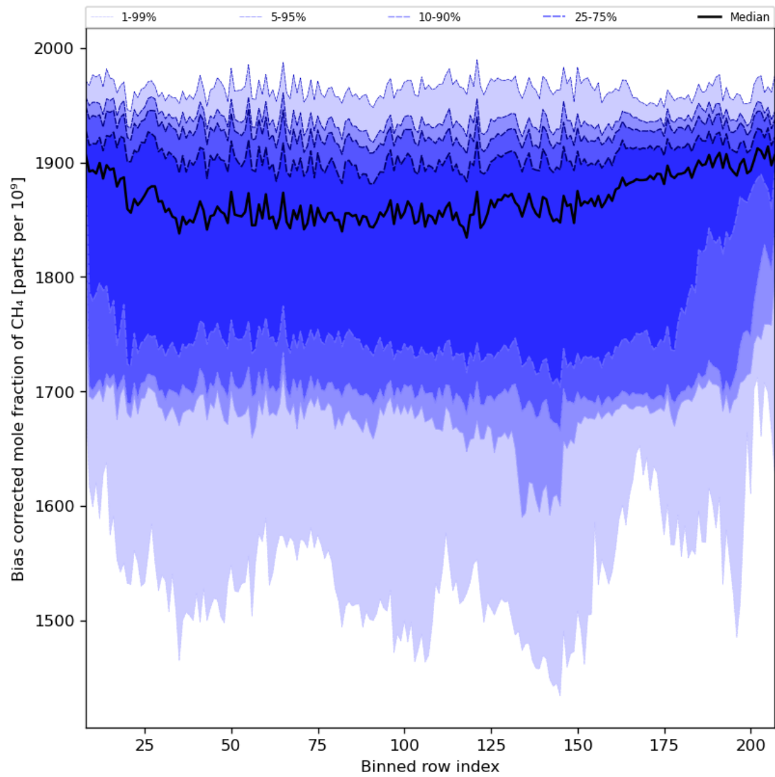
Figure 36: Along track statistics of “Bias corrected mole fraction of CH 4 ” for 2023-11-07 to 2023-11-08
