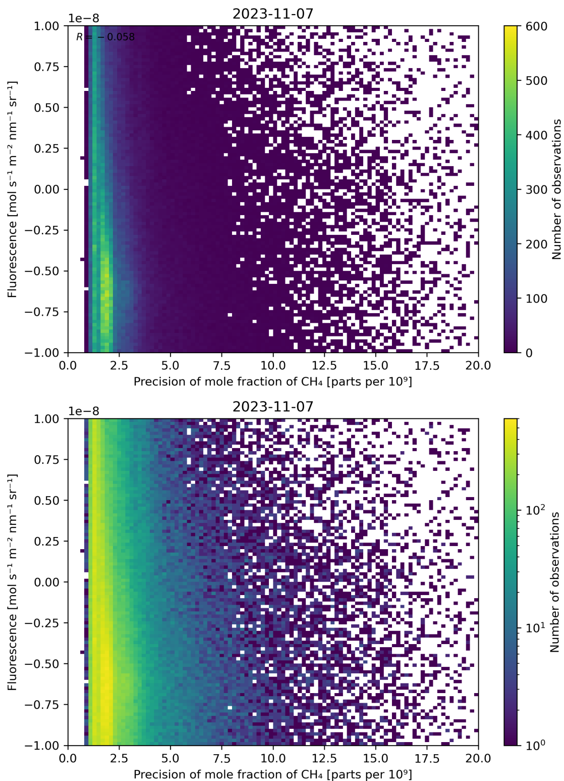
Figure 81: Scatter density plot of “Precision of mole fraction of \text{CH}_4 ” against “Fluorescence” for 2023-11-07 to 2023-11-08.
