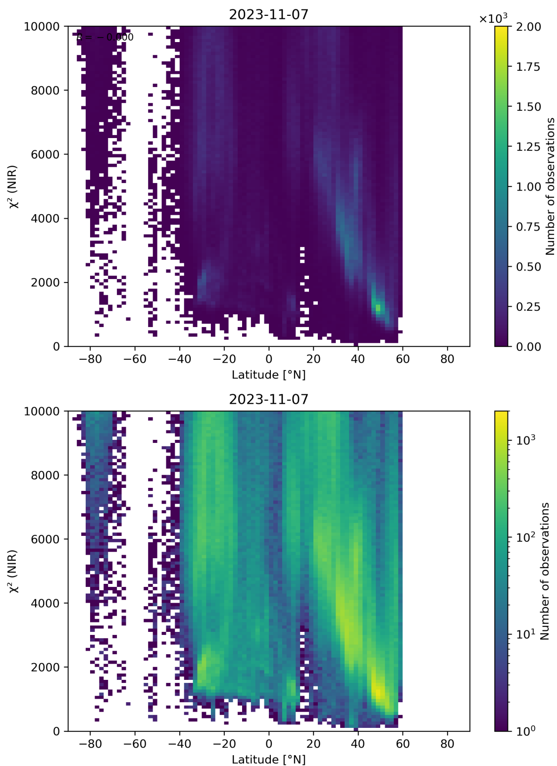
Figure 53: Scatter density plot of “Latitude” against “ \chi^2 (NIR)” for 2023-11-07 to 2023-11-08.
