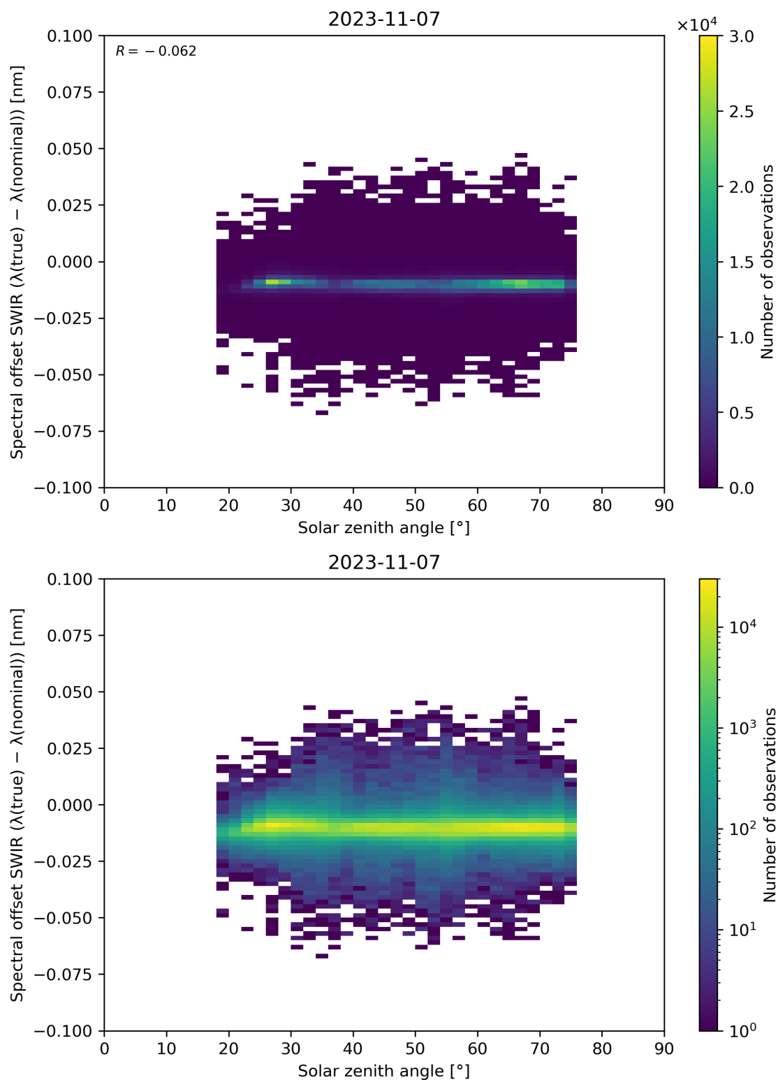
Figure 104: Scatter density plot of “Solar zenith angle” against “Spectral offset SWIR ( \lambda(\text{true}) - \lambda(\text{nominal}) )” for 2023-11-07 to 2023-11-08.
