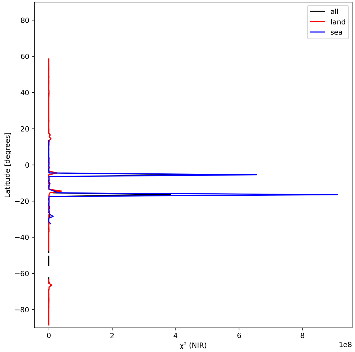
Figure 18: Zonal average of “ \chi^2 (NIR)” for 2023-11-07 to 2023-11-08.
