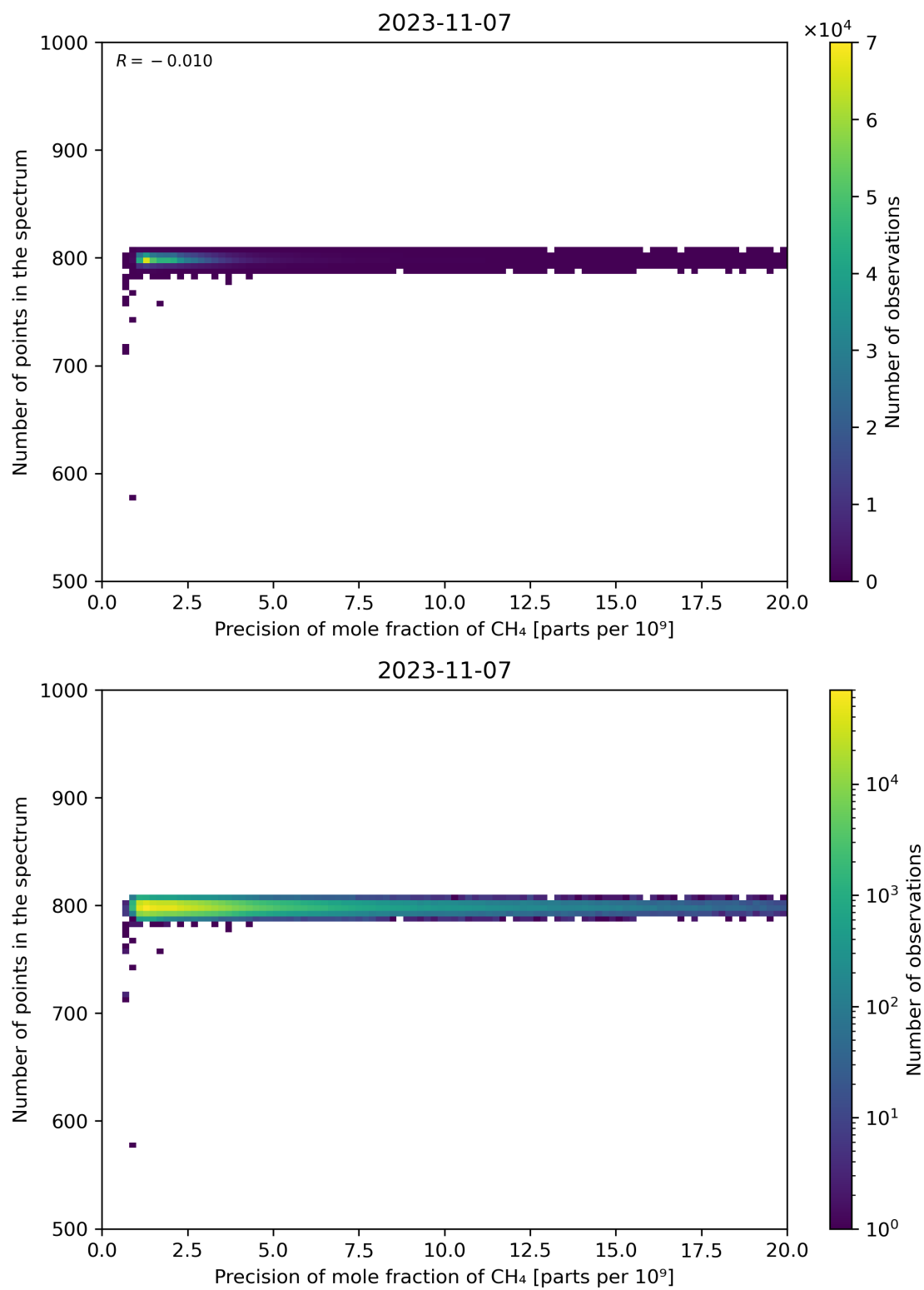
Figure 84: Scatter density plot of “Precision of mole fraction of CH 4 ” against “Number of points in the spectrum” for 2023-11-07 to 2023-11-08.
