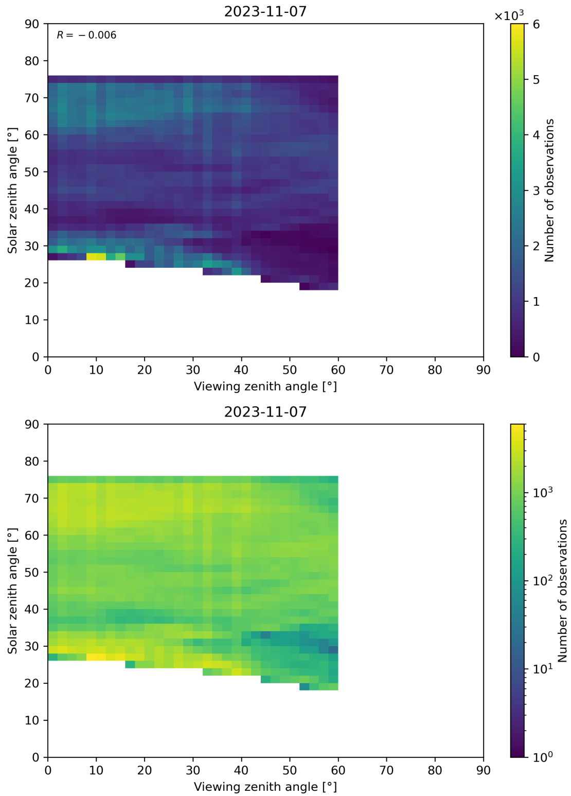
Figure 115: Scatter density plot of “Viewing zenith angle” against “Solar zenith angle” for 2023-11-07 to 2023-11-08.
