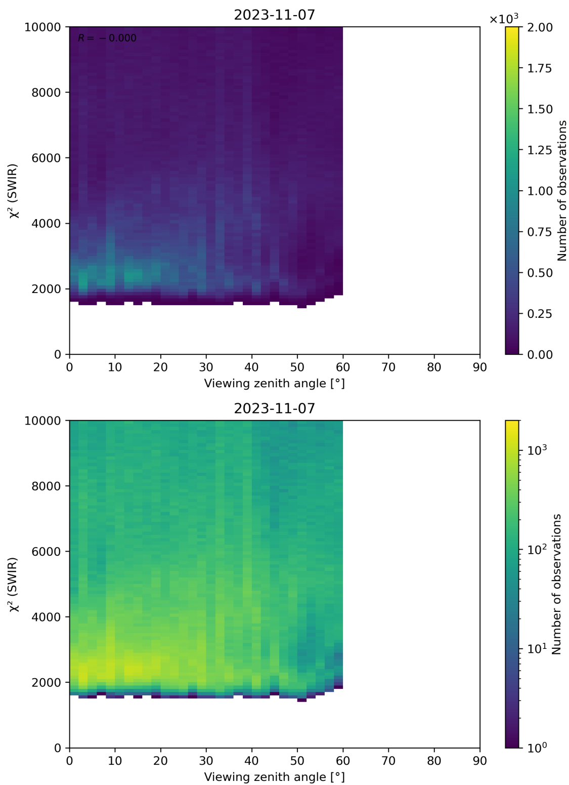
Figure 106: Scatter density plot of “Viewing zenith angle” against “ \chi^2 (SWIR)” for 2023-11-07 to 2023-11-08.
