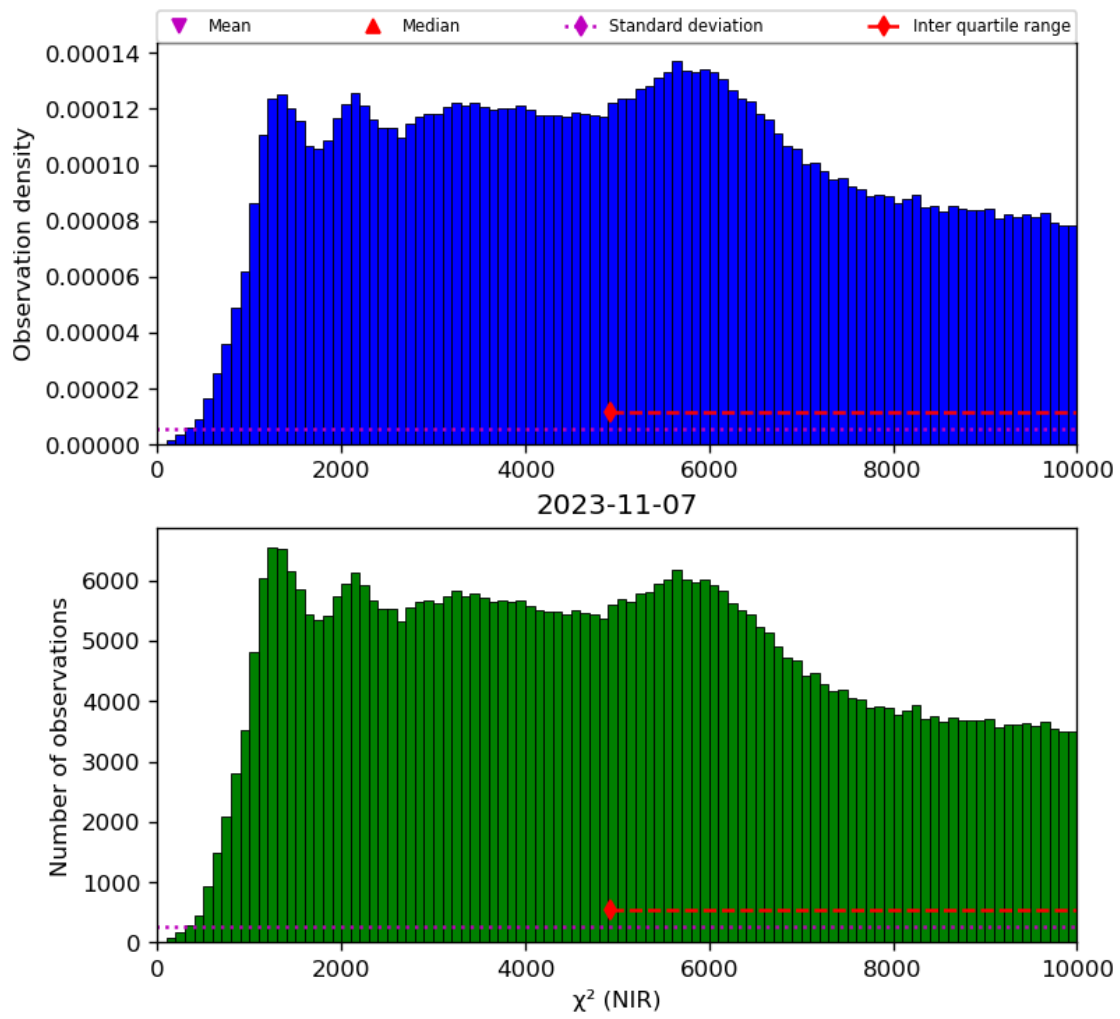
Figure 29: Histogram of “ \chi^2 (NIR)” for 2023-11-07 to 2023-11-08
