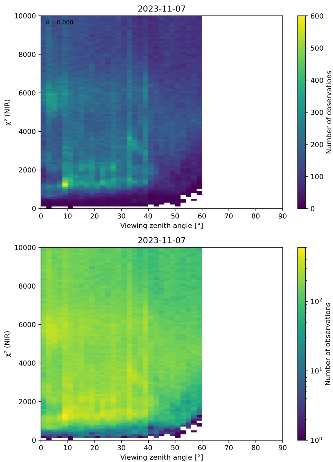
Figure 105: Scatter density plot of “Viewing zenith angle” against “ \chi^2 (NIR)” for 2023-11-07 to 2023-11-08.
