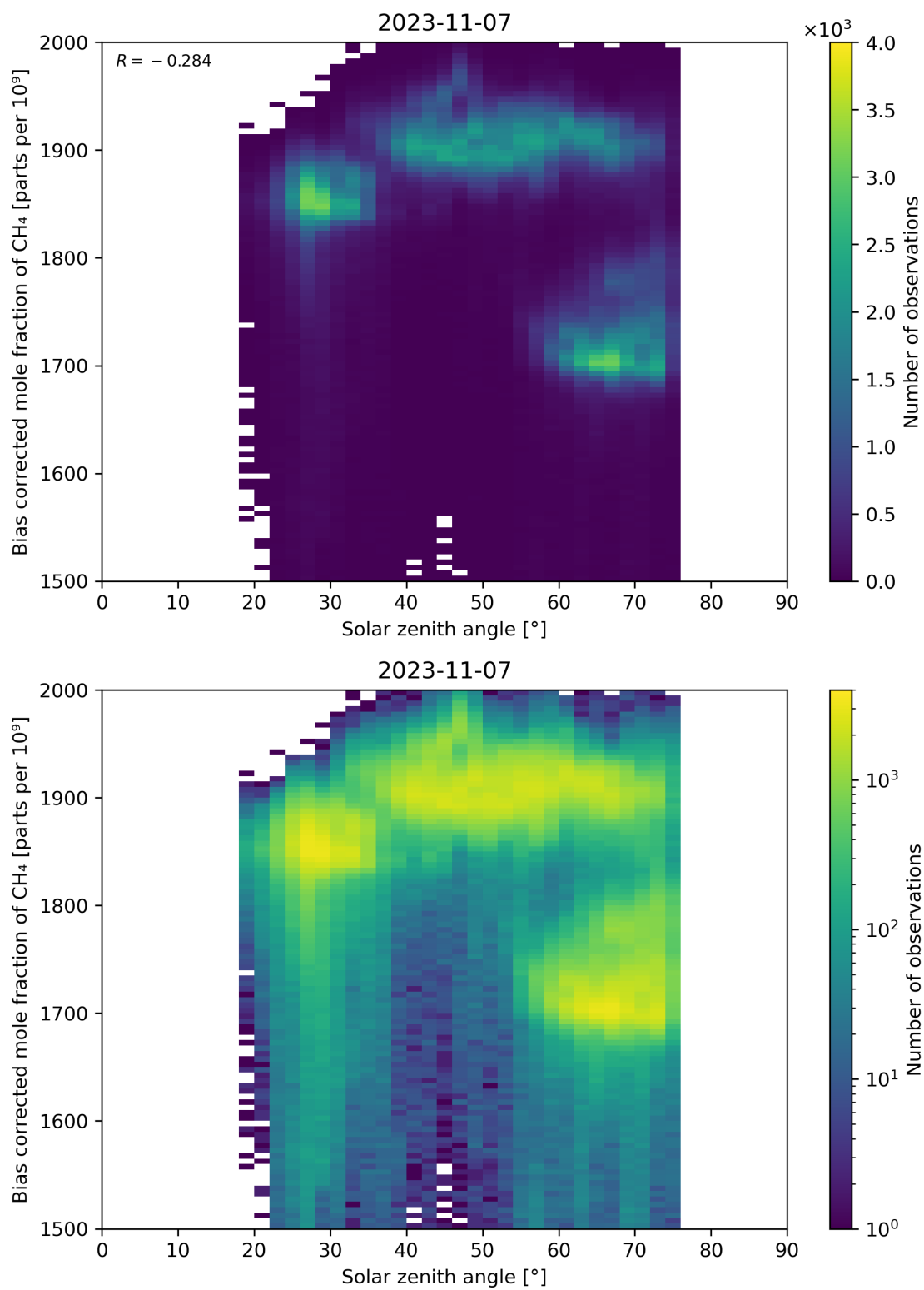
Figure 100: Scatter density plot of “Solar zenith angle” against “Bias corrected mole fraction of CH 4 ” for 2023-11-07 to 2023-11-08.
