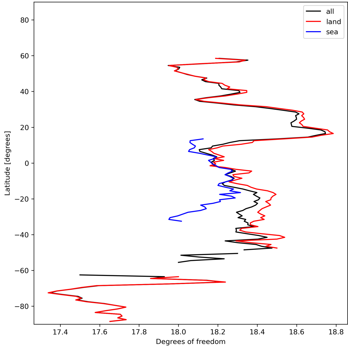
Figure 19: Zonal average of “Degrees of freedom” for 2023-11-07 to 2023-11-08.
