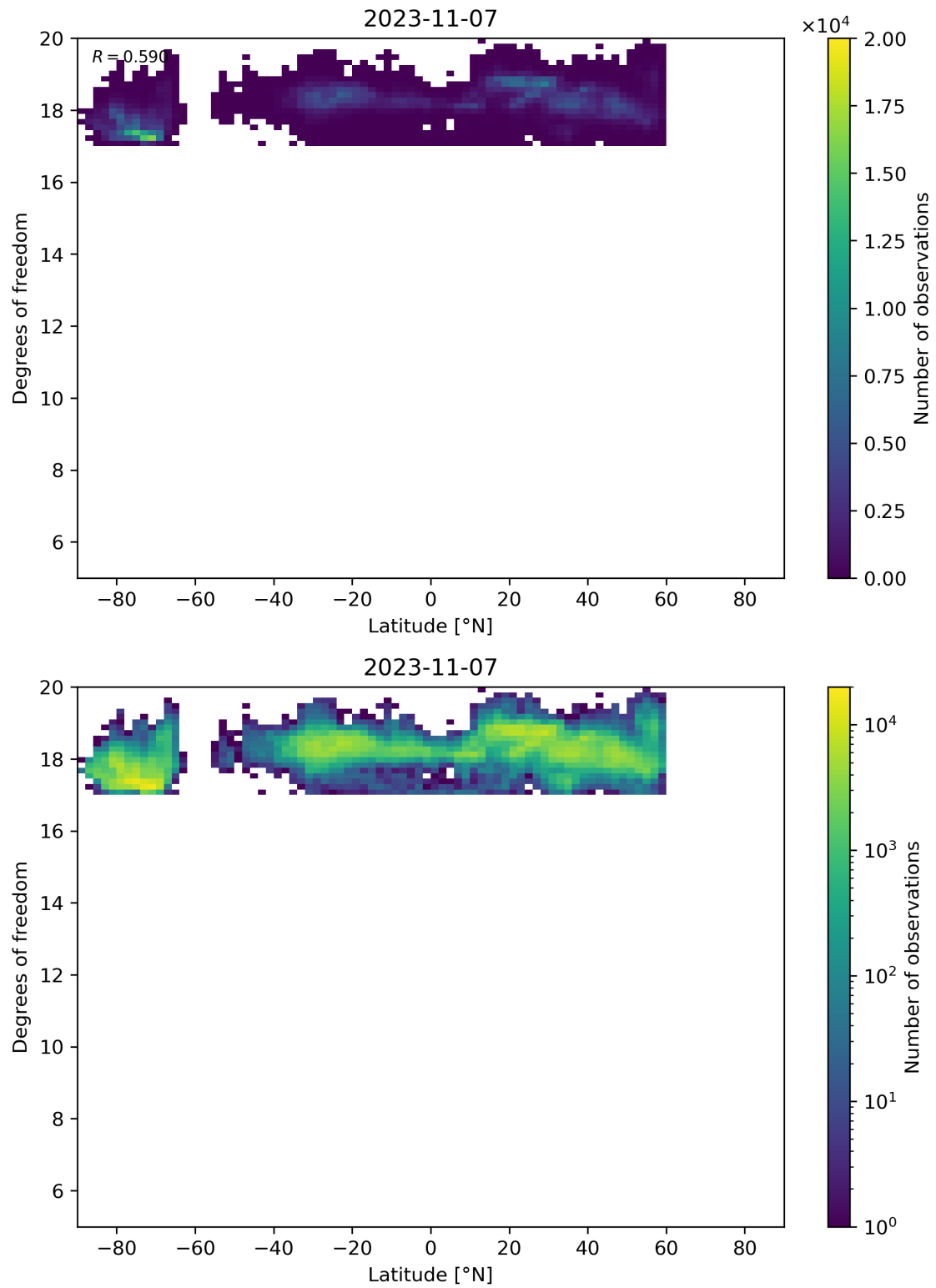
Figure 55: Scatter density plot of “Latitude” against “Degrees of freedom” for 2023-11-07 to 2023-11-08.
