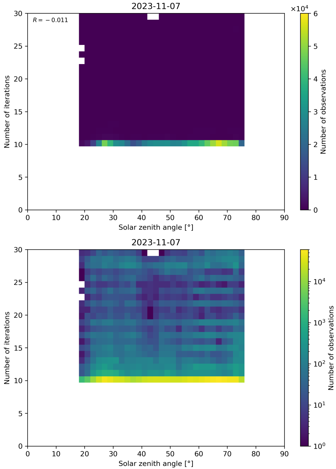
Figure 102: Scatter density plot of “Solar zenith angle” against “Number of iterations” for 2023-11-07 to 2023-11-08.
