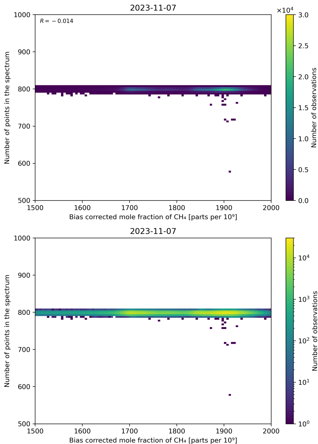
Figure 68: Scatter density plot of “Bias corrected mole fraction of CH 4 ” against “Number of points in the spectrum” for 2023-11-07 to 2023-11-08.
