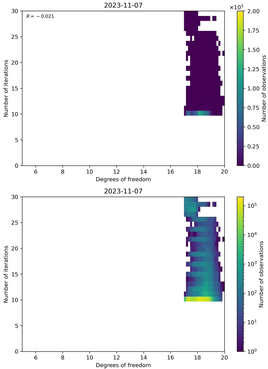
Figure 52: Scatter density plot of “Degrees of freedom” against “Number of iterations” for 2023-11-07 to 2023-11-08.
