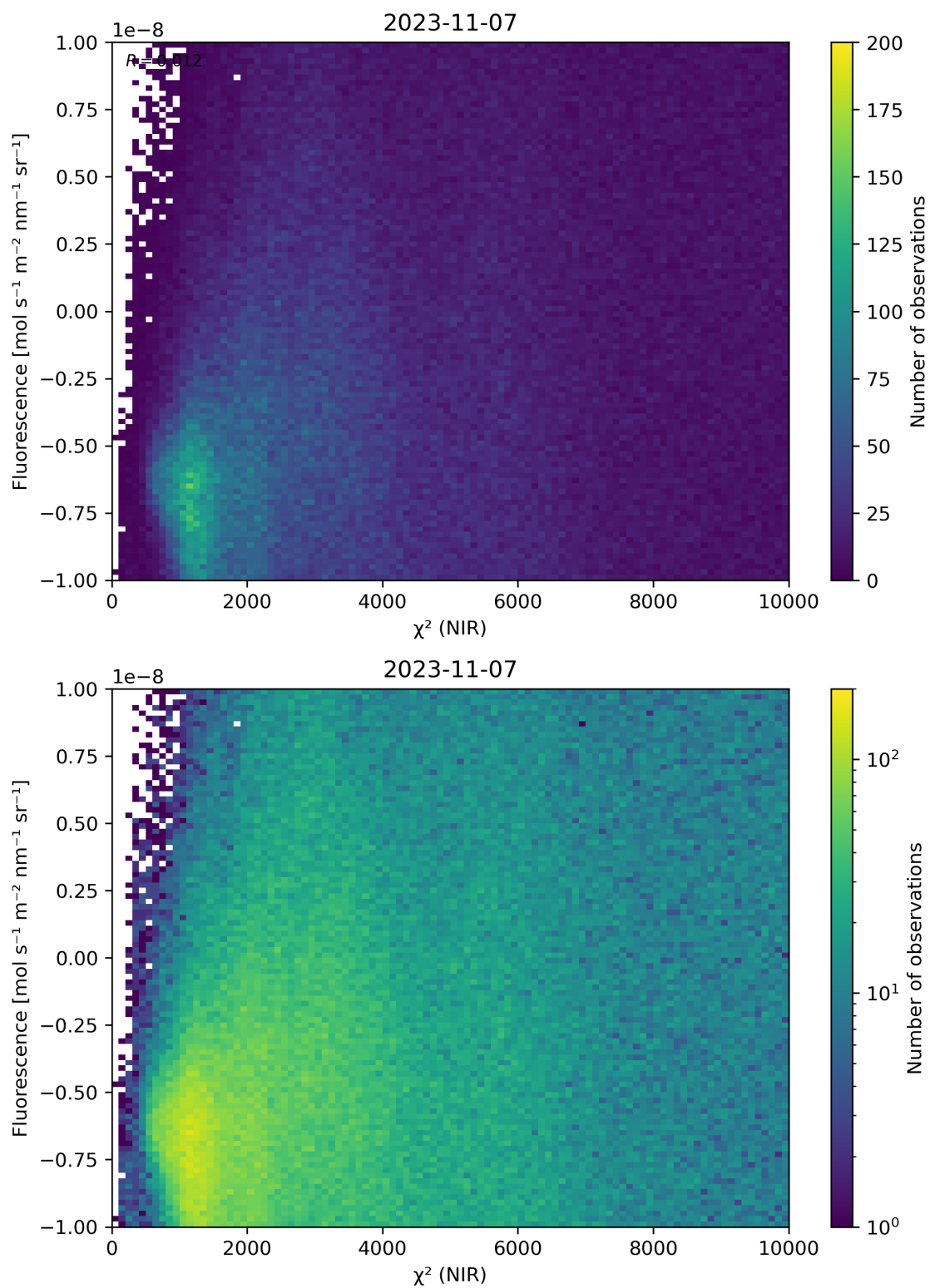
Figure 45: Scatter density plot of “ \chi^2 (NIR)” against “Fluorescence” for 2023-11-07 to 2023-11-08.
