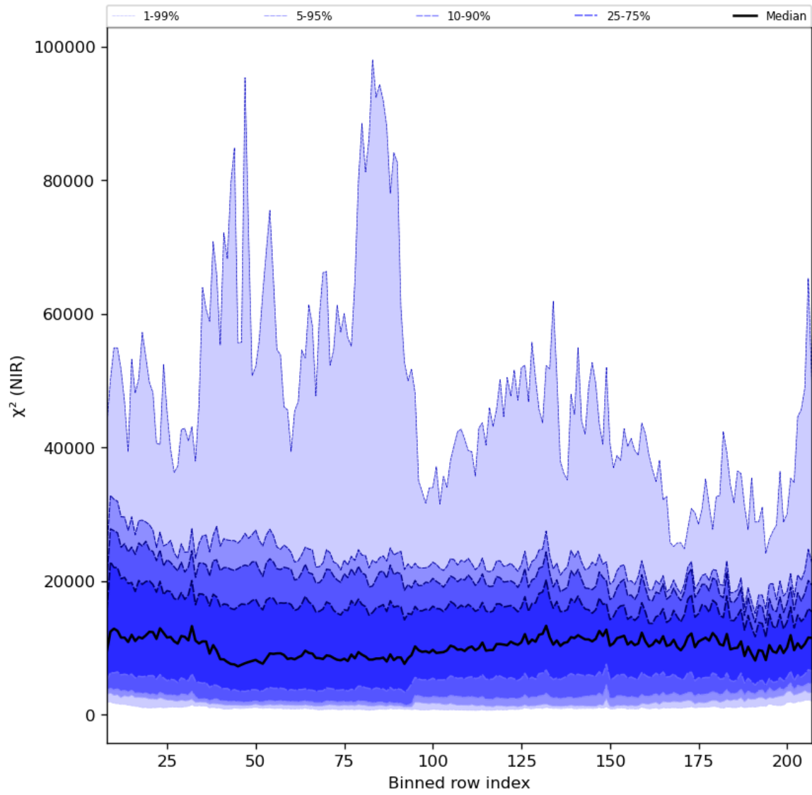
Figure 40: Along track statistics of “ \chi^2 (NIR)” for 2023-11-07 to 2023-11-08
