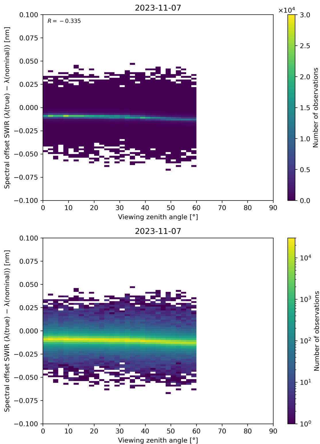
Figure 116: Scatter density plot of “Viewing zenith angle” against “Spectral offset SWIR ( \lambda(\text{true}) - \lambda(\text{nominal}) )” for 2023-11-07 to 2023-11-08.
