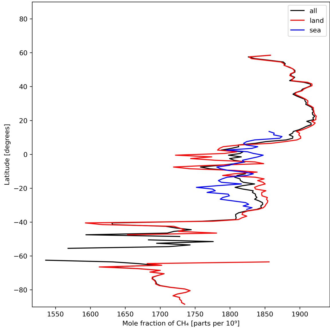
Figure 12: Zonal average of “Mole fraction of CH 4 ” for 2023-11-07 to 2023-11-08.
