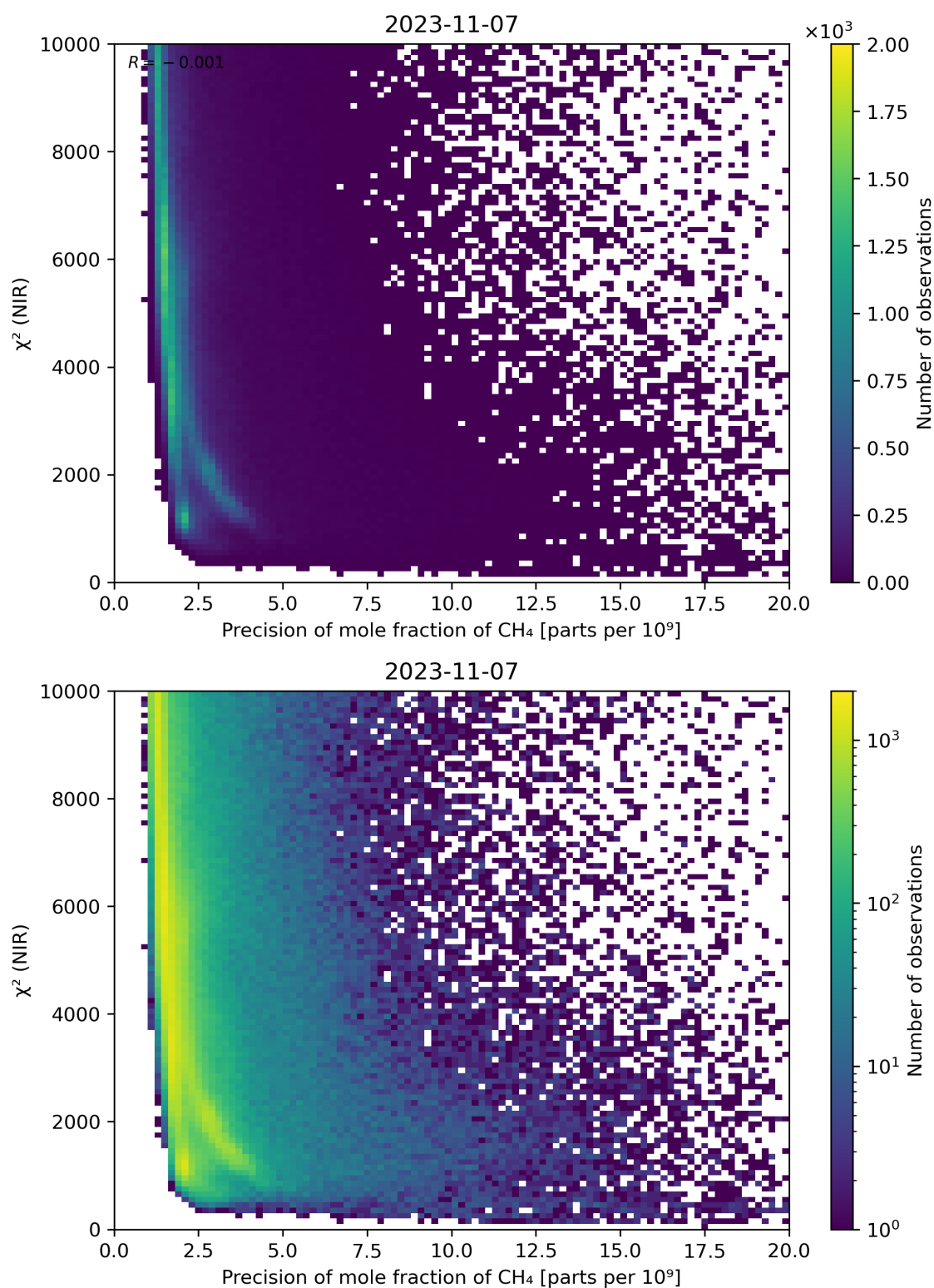
Figure 78: Scatter density plot of “Precision of mole fraction of CH 4 ” against “ \chi^2 (NIR)” for 2023-11-07 to 2023-11-08.
