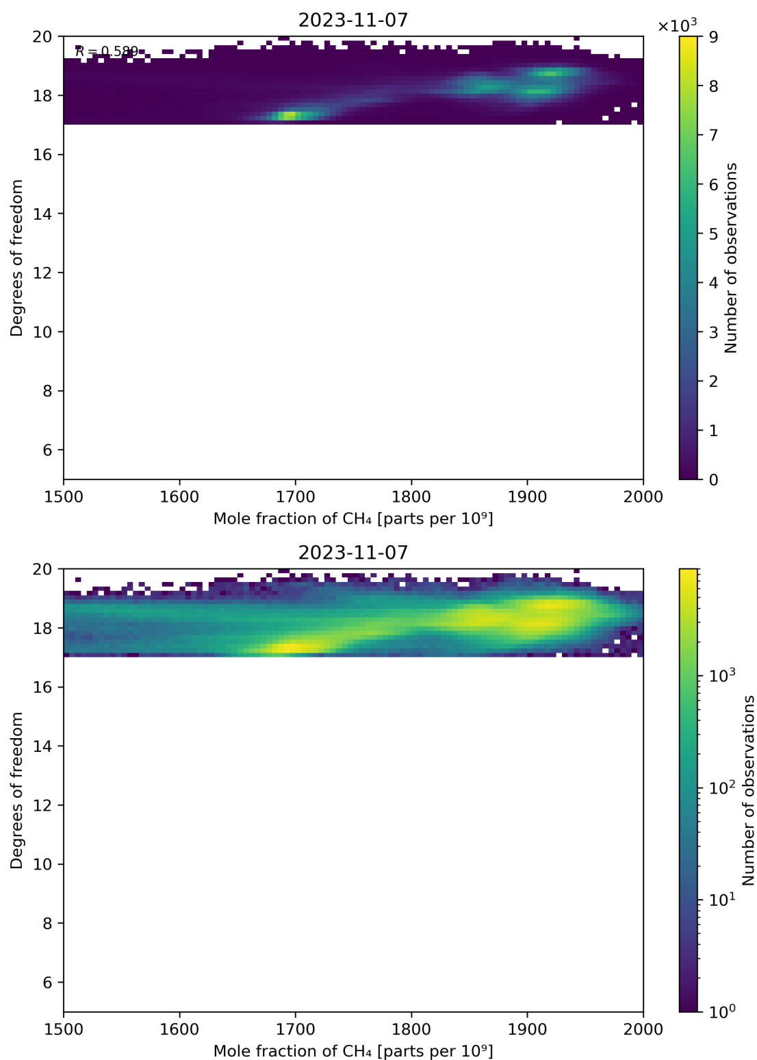
Figure 72: Scatter density plot of “Mole fraction of CH 4 ” against “Degrees of freedom” for 2023-11-07 to 2023-11-08.
