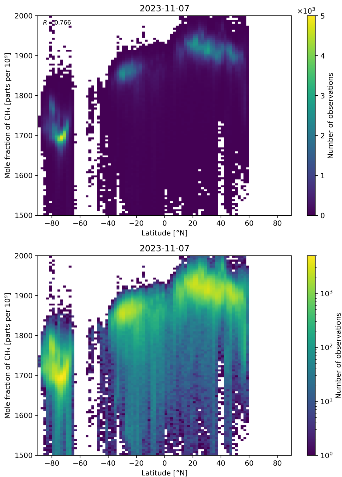
Figure 57: Scatter density plot of “Latitude” against “Mole fraction of CH 4 ” for 2023-11-07 to 2023-11-08.
