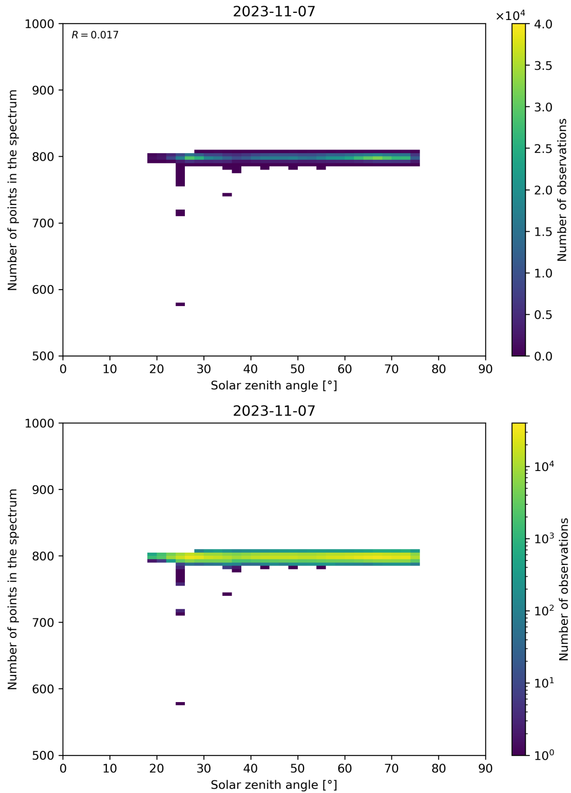
Figure 103: Scatter density plot of “Solar zenith angle” against “Number of points in the spectrum” for 2023-11-07 to 2023-11-08.
