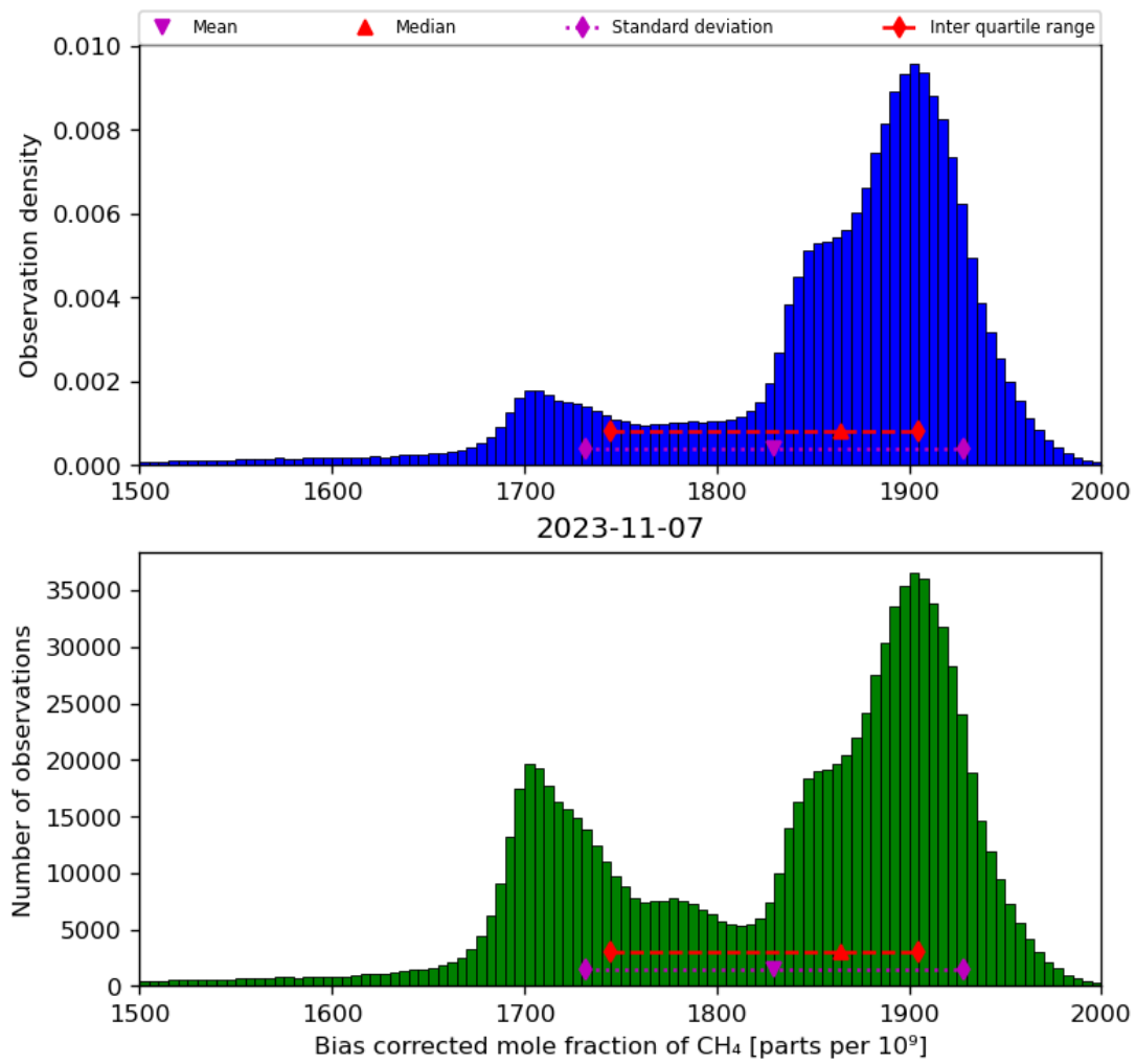
Figure 25: Histogram of “Bias corrected mole fraction of CH 4 ” for 2023-11-07 to 2023-11-08
