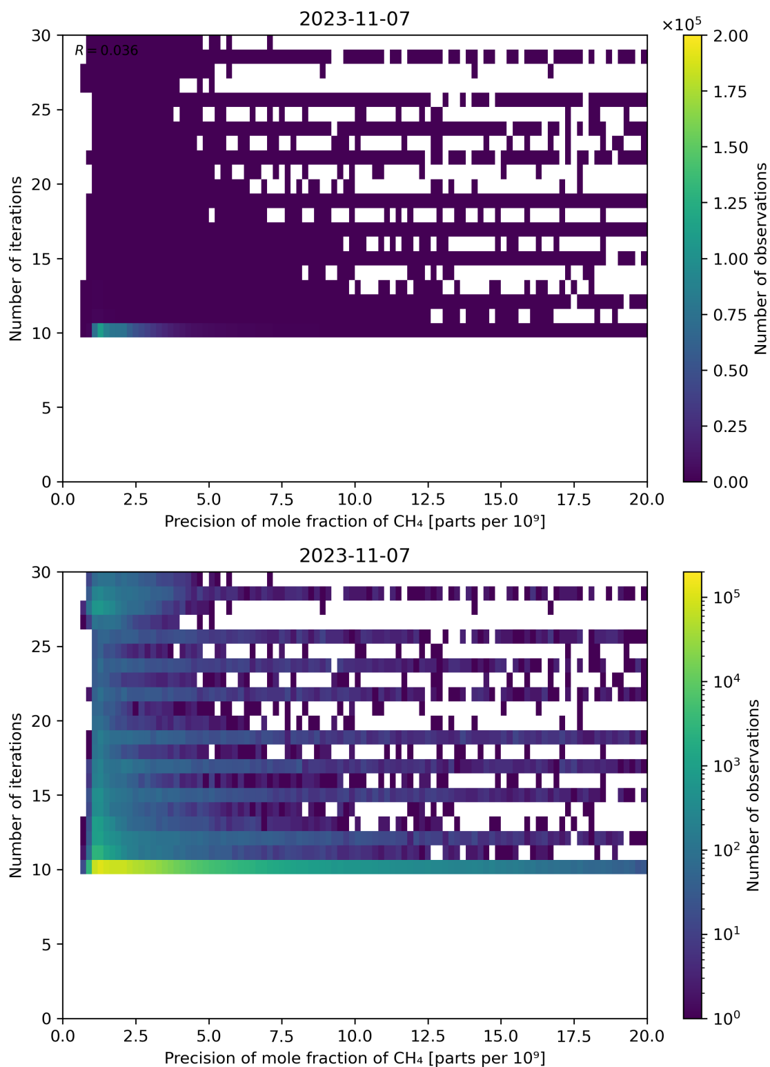
Figure 83: Scatter density plot of “Precision of mole fraction of \text{CH}_4 ” against “Number of iterations” for 2023-11-07 to 2023-11-08.
