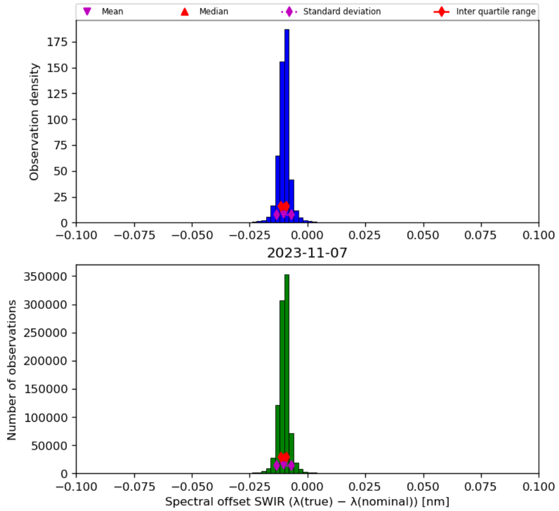
Figure 27: Histogram of “Spectral offset SWIR ( \lambda(\text{true}) - \lambda(\text{nominal}) )” for 2023-11-07 to 2023-11-08
