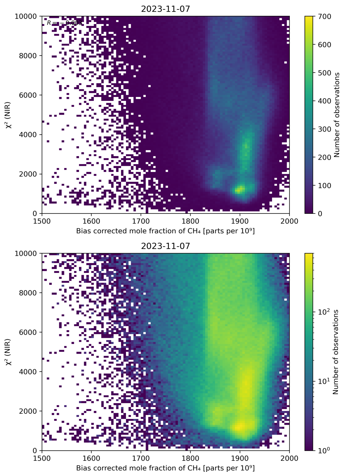
Figure 63: Scatter density plot of “Bias corrected mole fraction of CH 4 ” against “ \chi^2 (NIR)” for 2023-11-07 to 2023-11-08.
