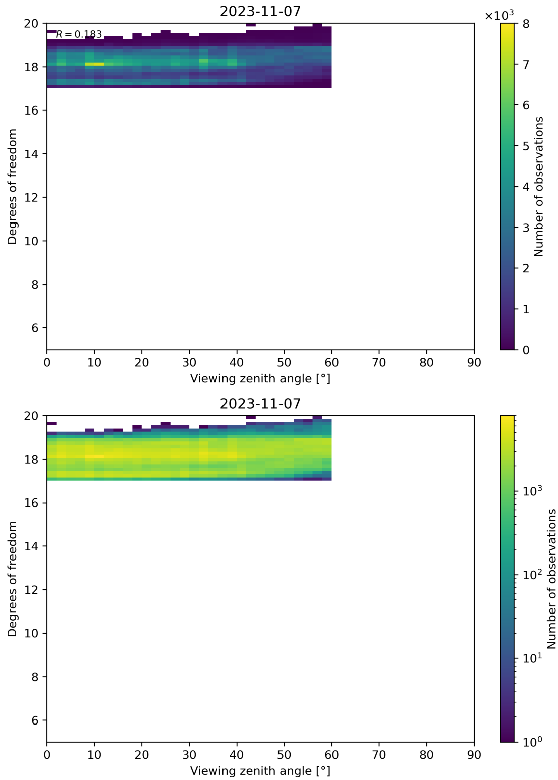
Figure 107: Scatter density plot of “Viewing zenith angle” against “Degrees of freedom” for 2023-11-07 to 2023-11-08.
