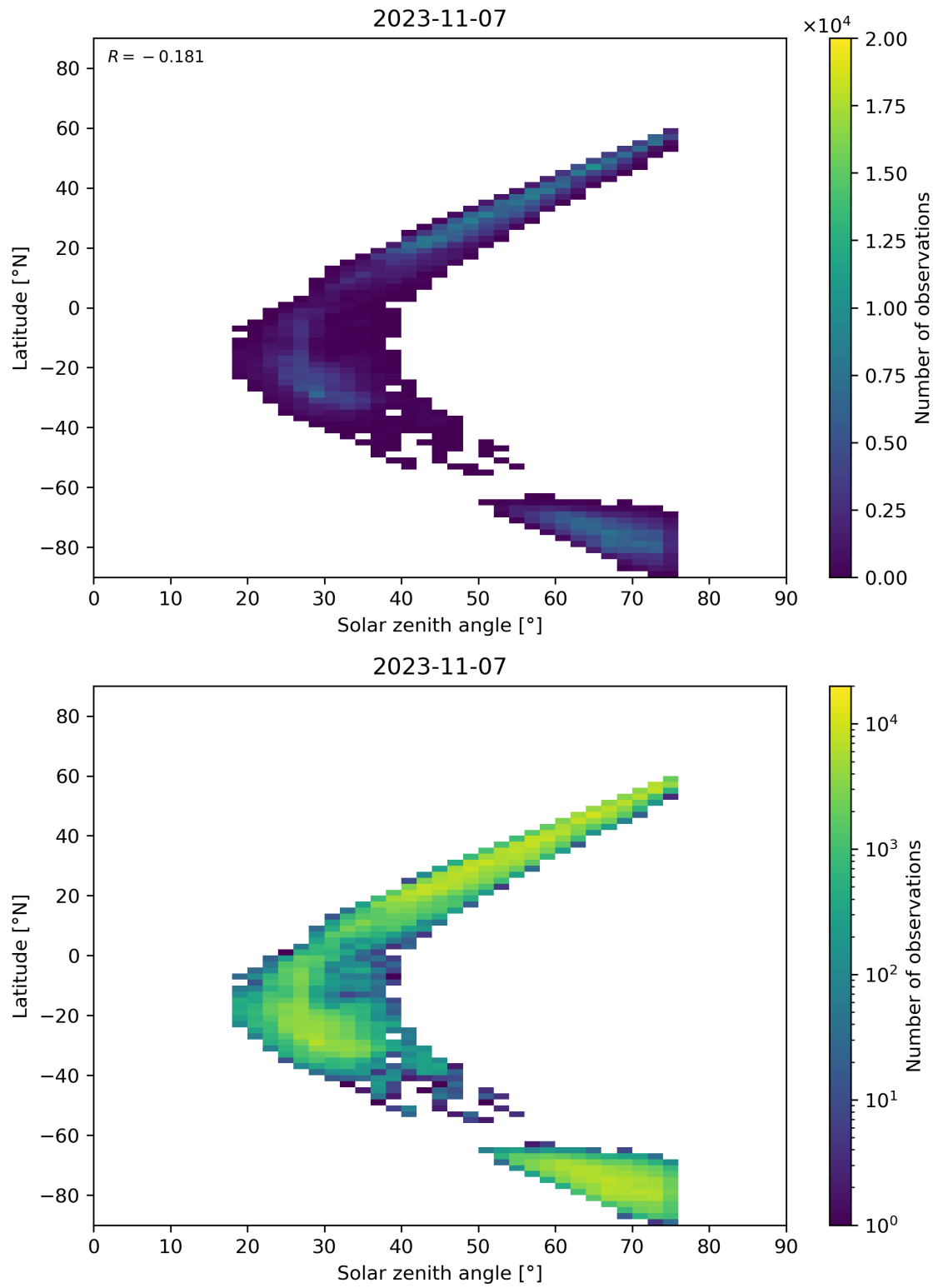
Figure 98: Scatter density plot of “Solar zenith angle” against “Latitude” for 2023-11-07 to 2023-11-08.
