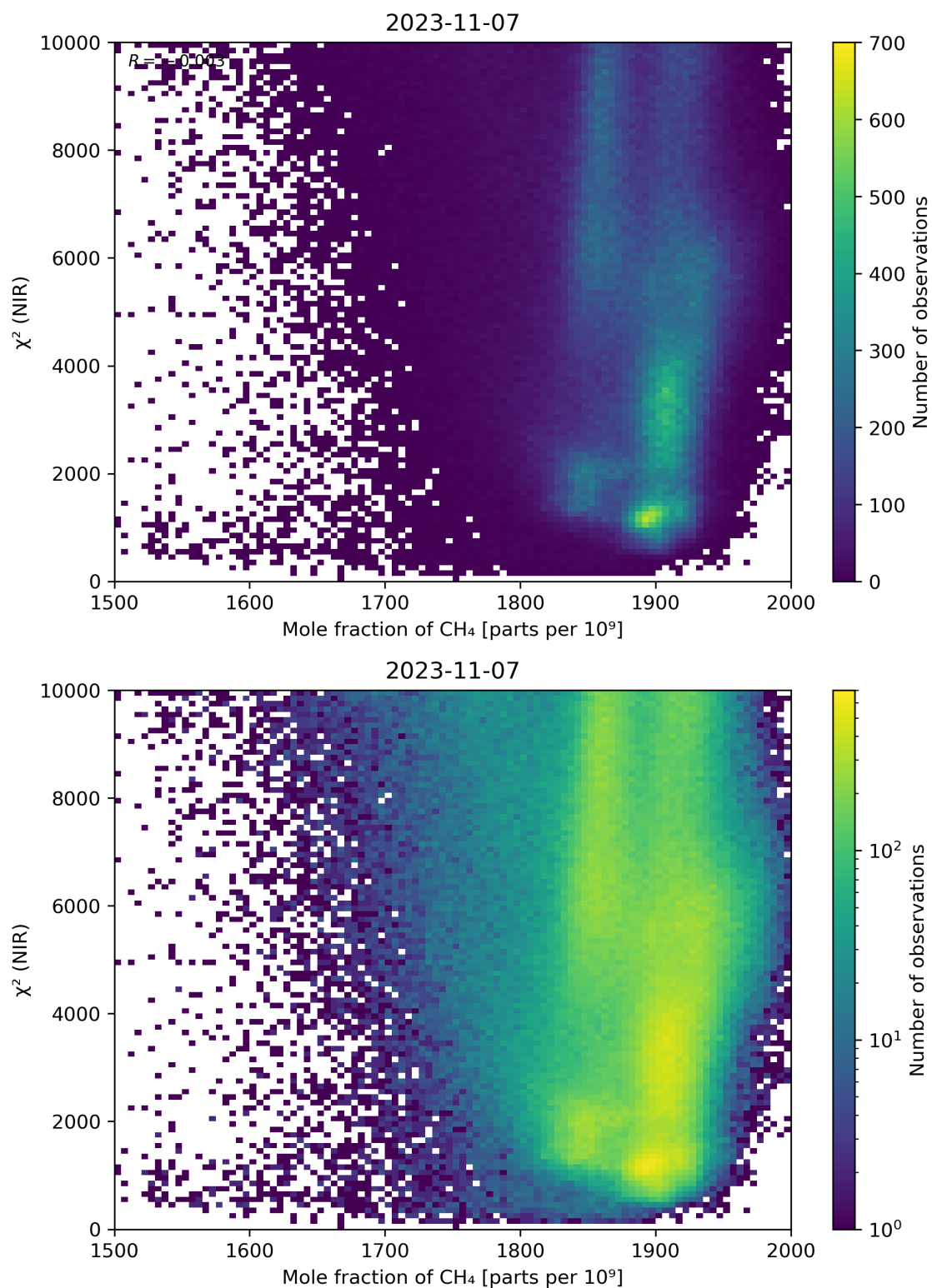
Figure 70: Scatter density plot of “Mole fraction of CH 4 ” against “ \chi^2 (NIR)” for 2023-11-07 to 2023-11-08.
