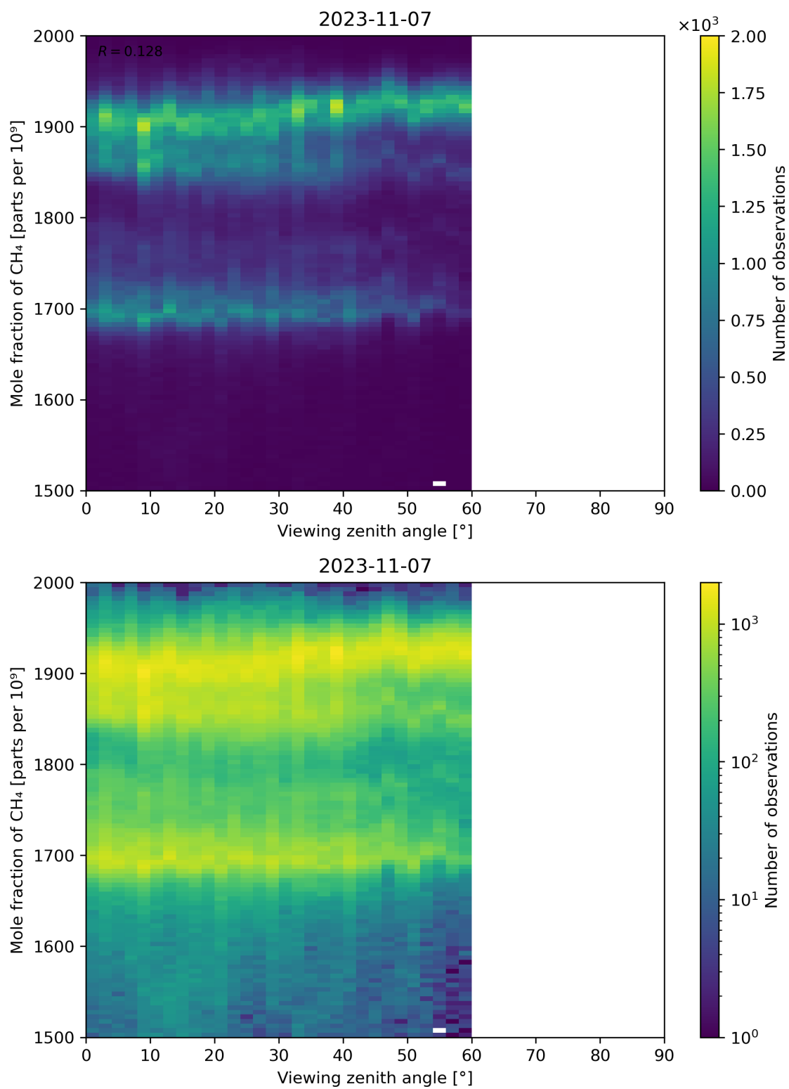
Figure 110: Scatter density plot of “Viewing zenith angle” against “Mole fraction of CH 4 ” for 2023-11-07 to 2023-11-08.
