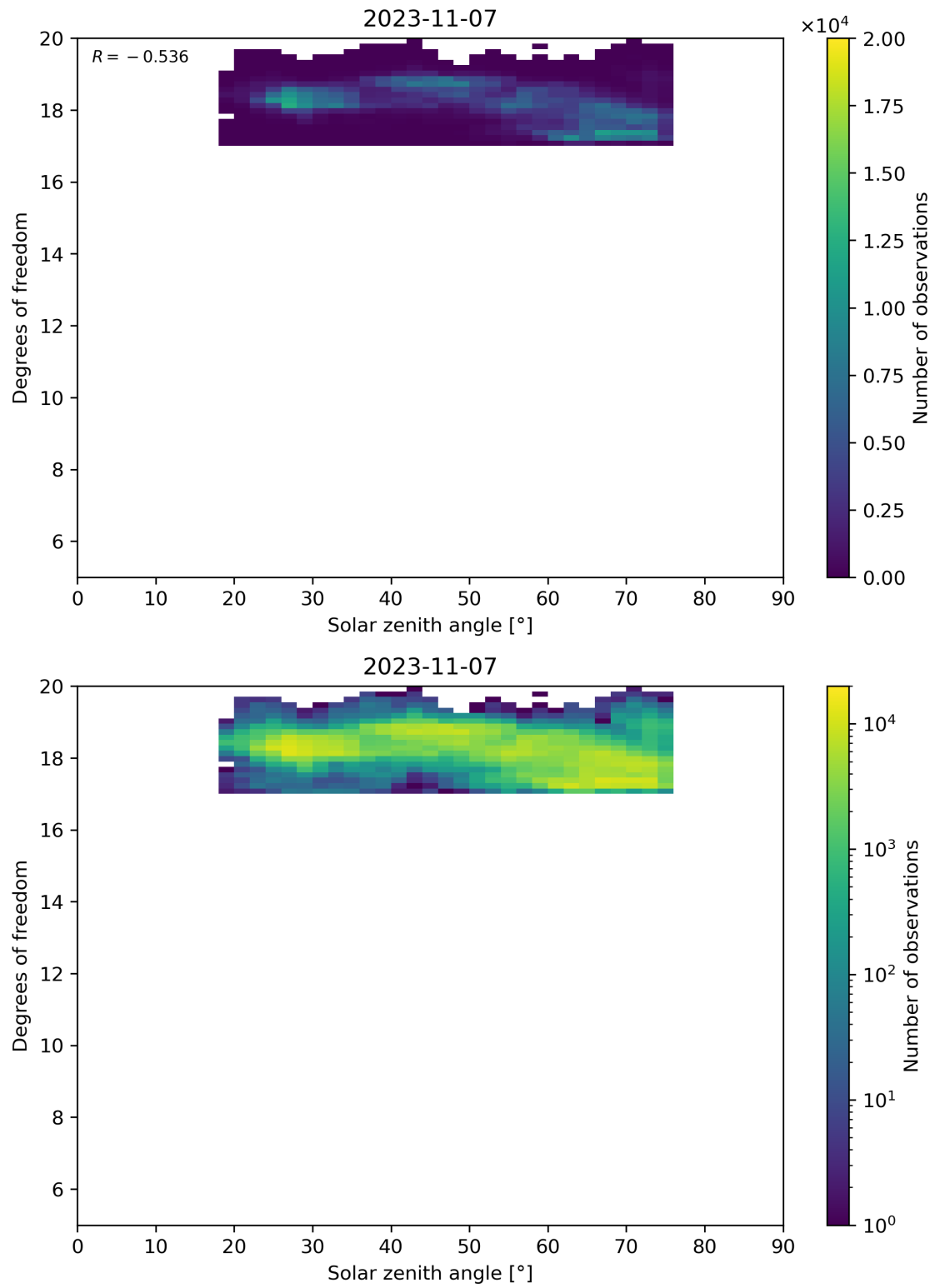
Figure 96: Scatter density plot of “Solar zenith angle” against “Degrees of freedom” for 2023-11-07 to 2023-11-08.
