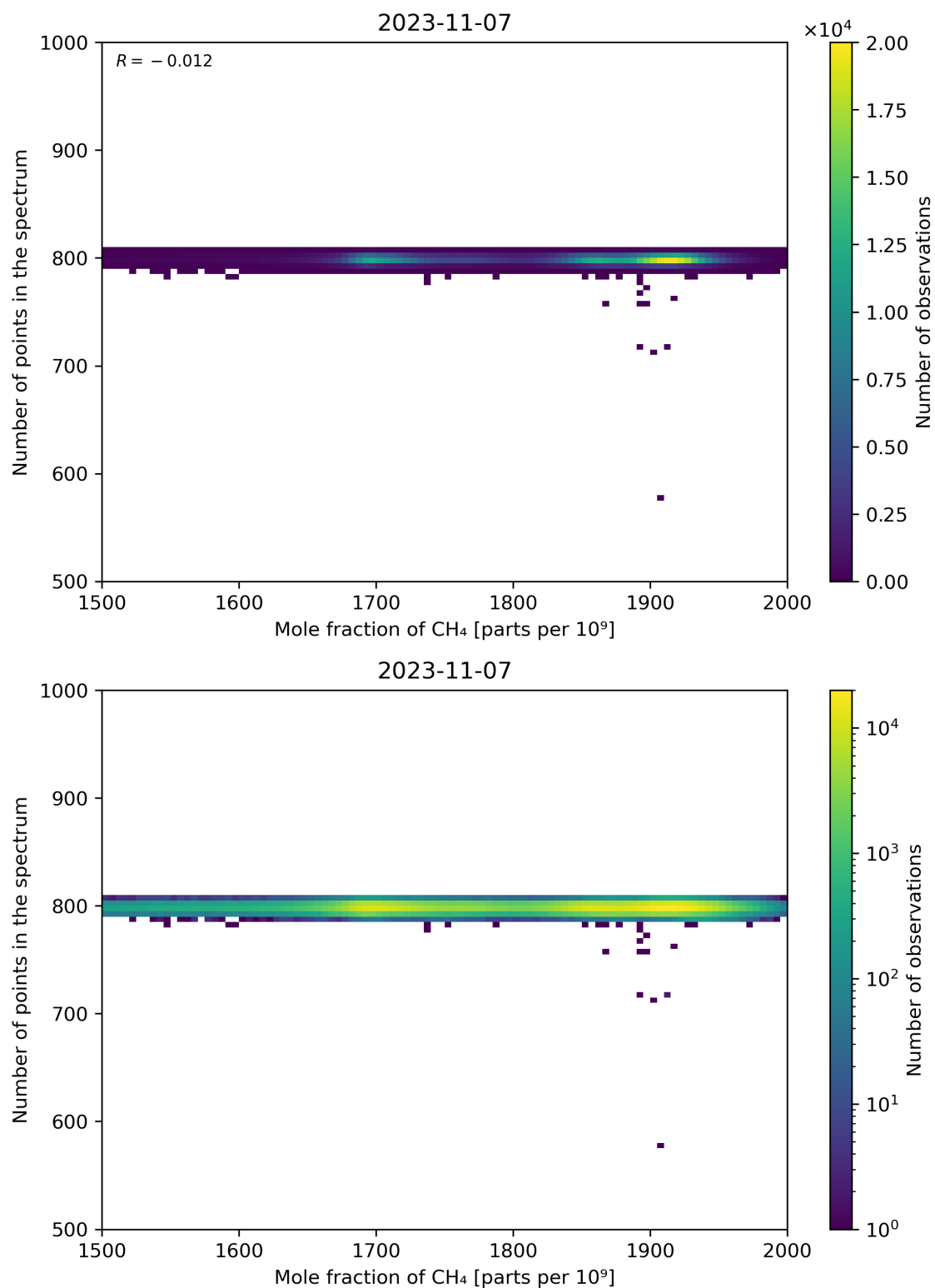
Figure 77: Scatter density plot of “Mole fraction of CH 4 ” against “Number of points in the spectrum” for 2023-11-07 to 2023-11-08.
