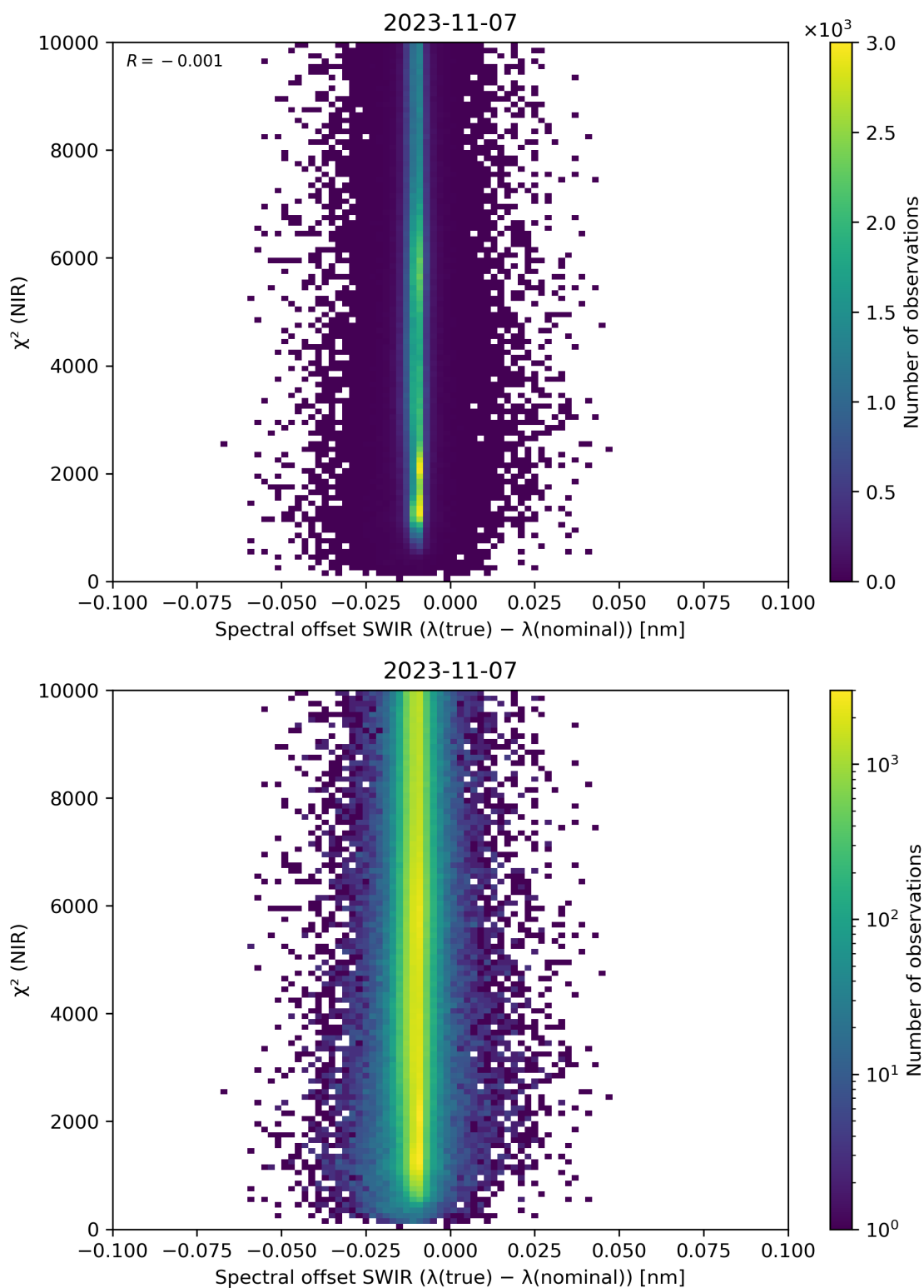
Figure 117: Scatter density plot of “Spectral offset SWIR ( \lambda(\text{true}) - \lambda(\text{nominal}) )” against “ \chi^2 (NIR)” for 2023-11-07 to 2023-11-08.
