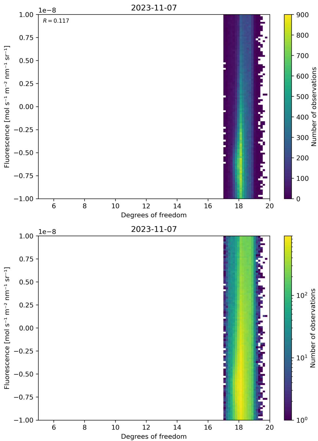
Figure 51: Scatter density plot of “Degrees of freedom” against “Fluorescence” for 2023-11-07 to 2023-11-08.
