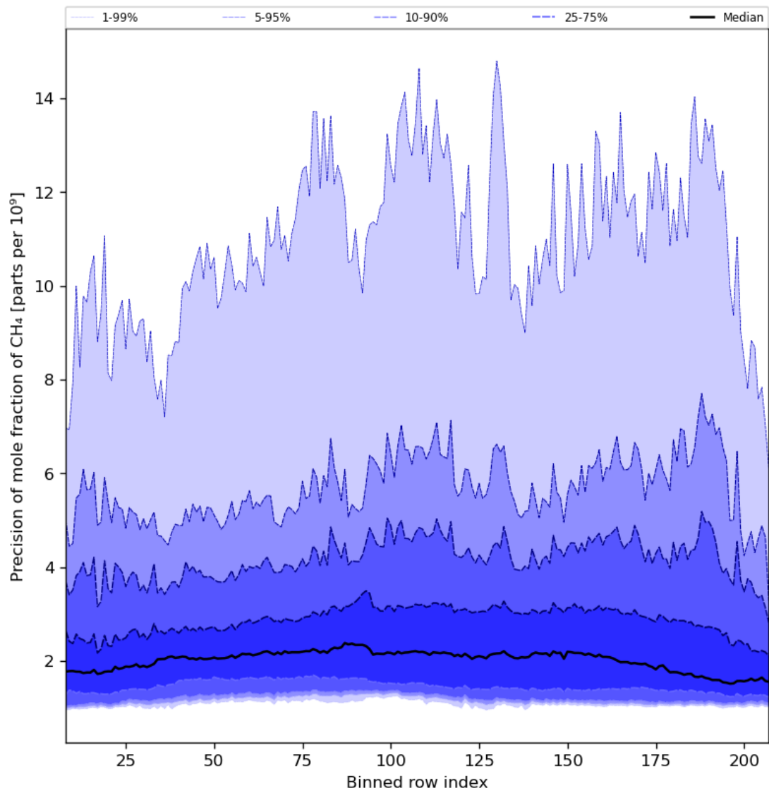
Figure 35: Along track statistics of “Precision of mole fraction of CH 4 ” for 2023-11-07 to 2023-11-08
