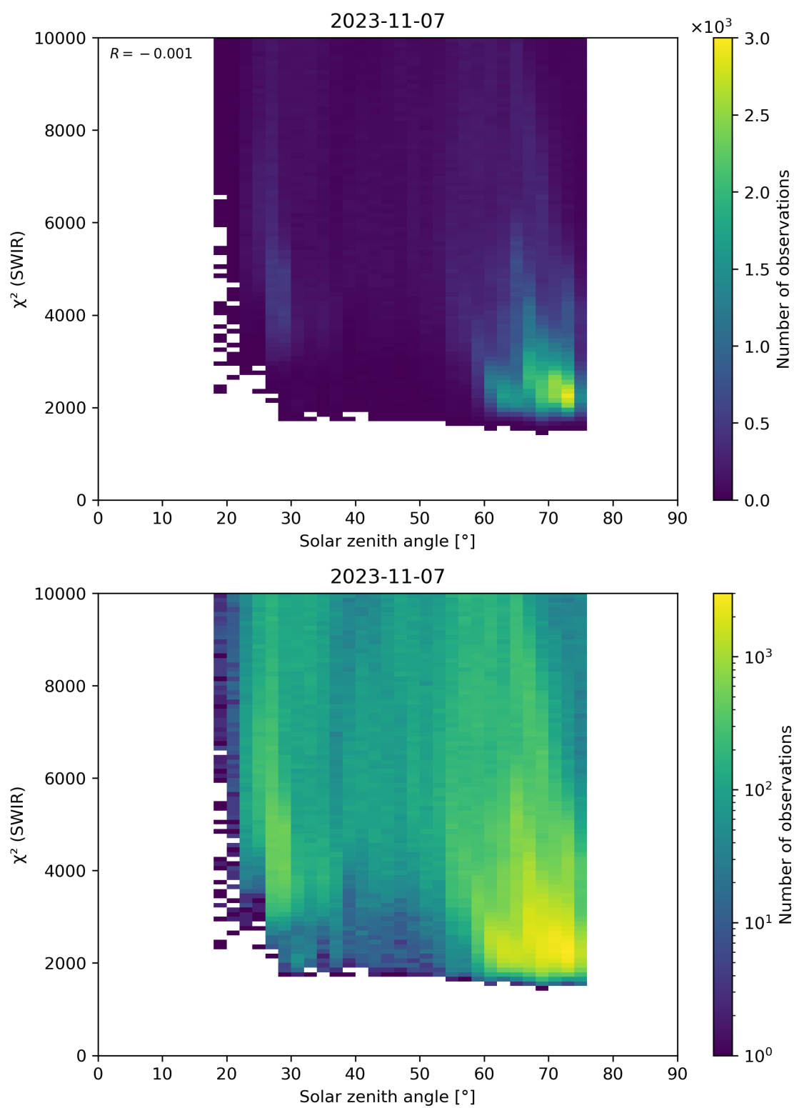
Figure 95: Scatter density plot of “Solar zenith angle” against “ \chi^2 (SWIR)” for 2023-11-07 to 2023-11-08.
