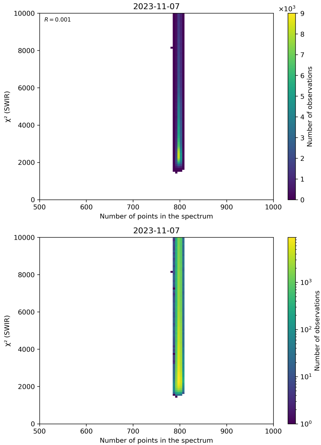
Figure 89: Scatter density plot of “Number of points in the spectrum” against “ \chi^2 (SWIR)” for 2023-11-07 to 2023-11-08.
