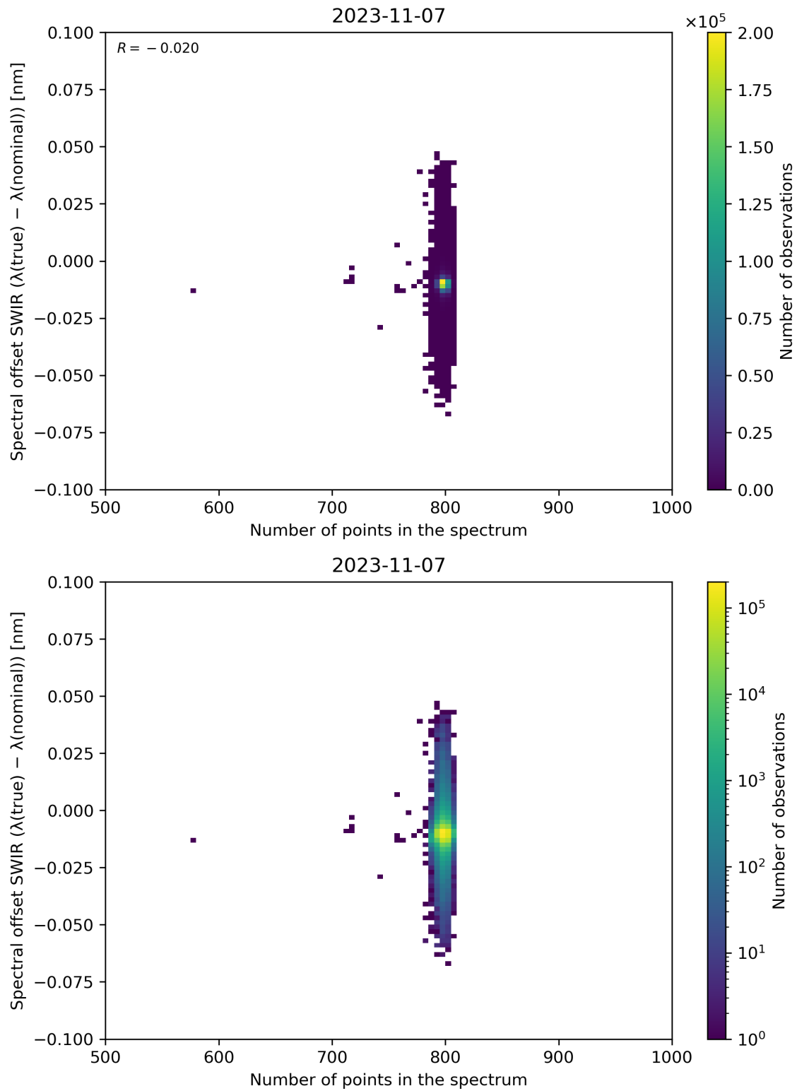
Figure 93: Scatter density plot of “Number of points in the spectrum” against “Spectral offset SWIR ( \lambda(\text{true}) - \lambda(\text{nominal}) )” for 2023-11-07 to 2023-11-08.
