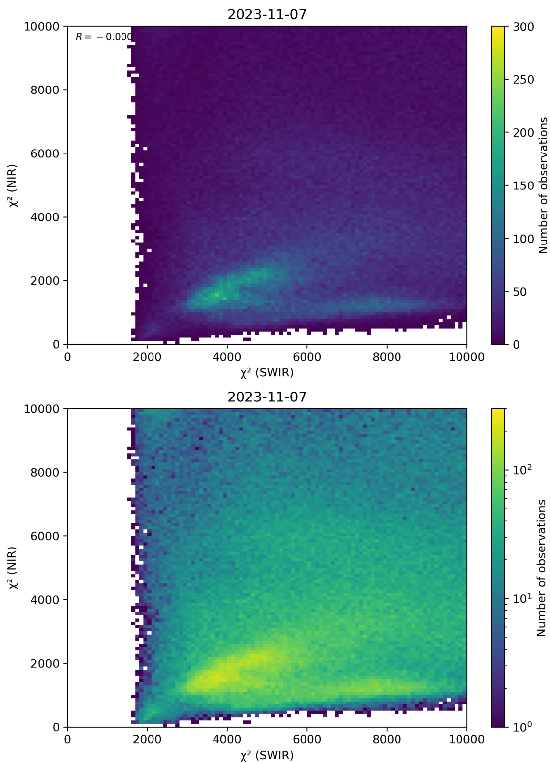
Figure 47: Scatter density plot of “ \chi^2 (SWIR)” against “ \chi^2 (NIR)” for 2023-11-07 to 2023-11-08.
