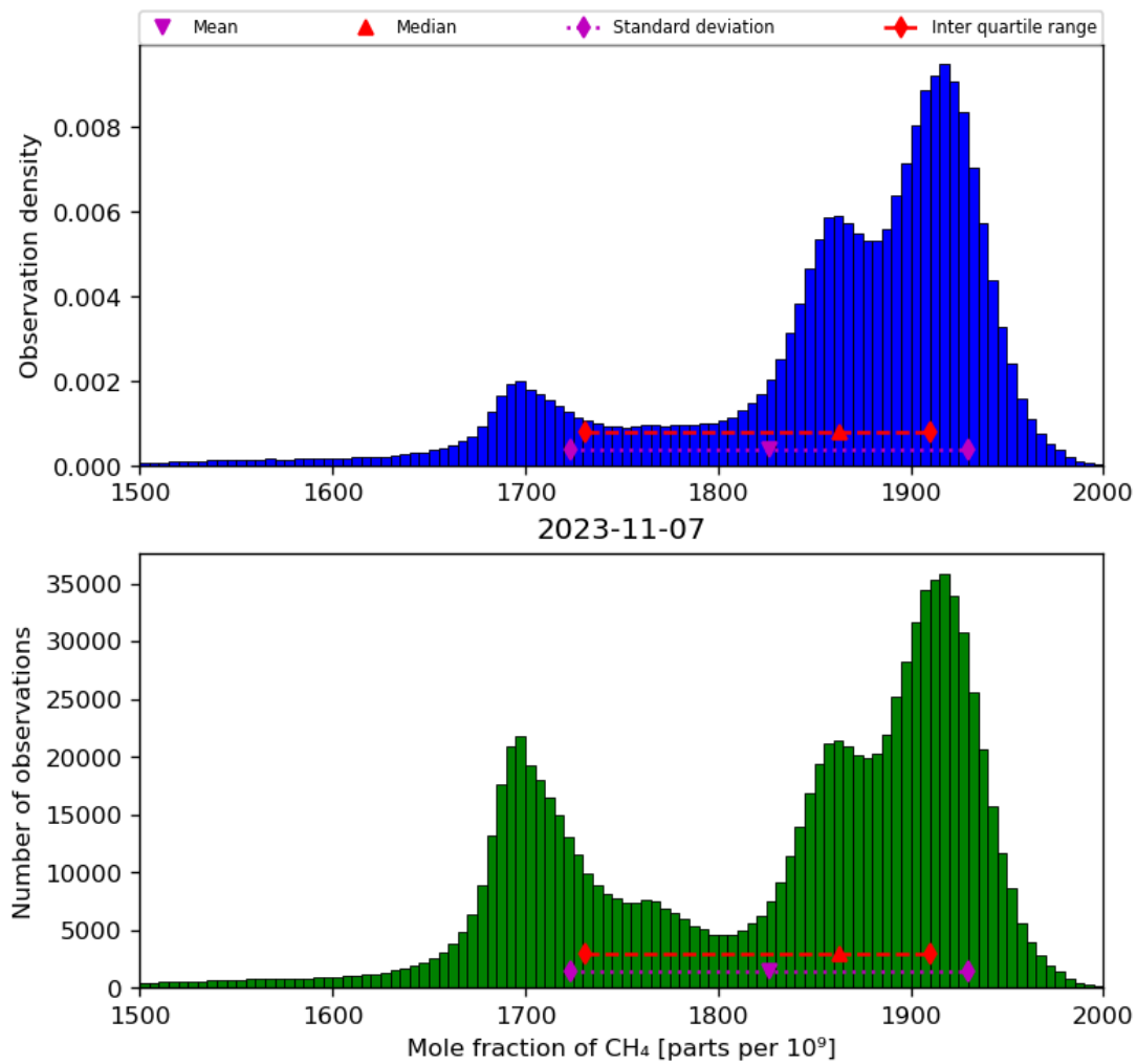
Figure 23: Histogram of “Mole fraction of CH 4 ” for 2023-11-07 to 2023-11-08
