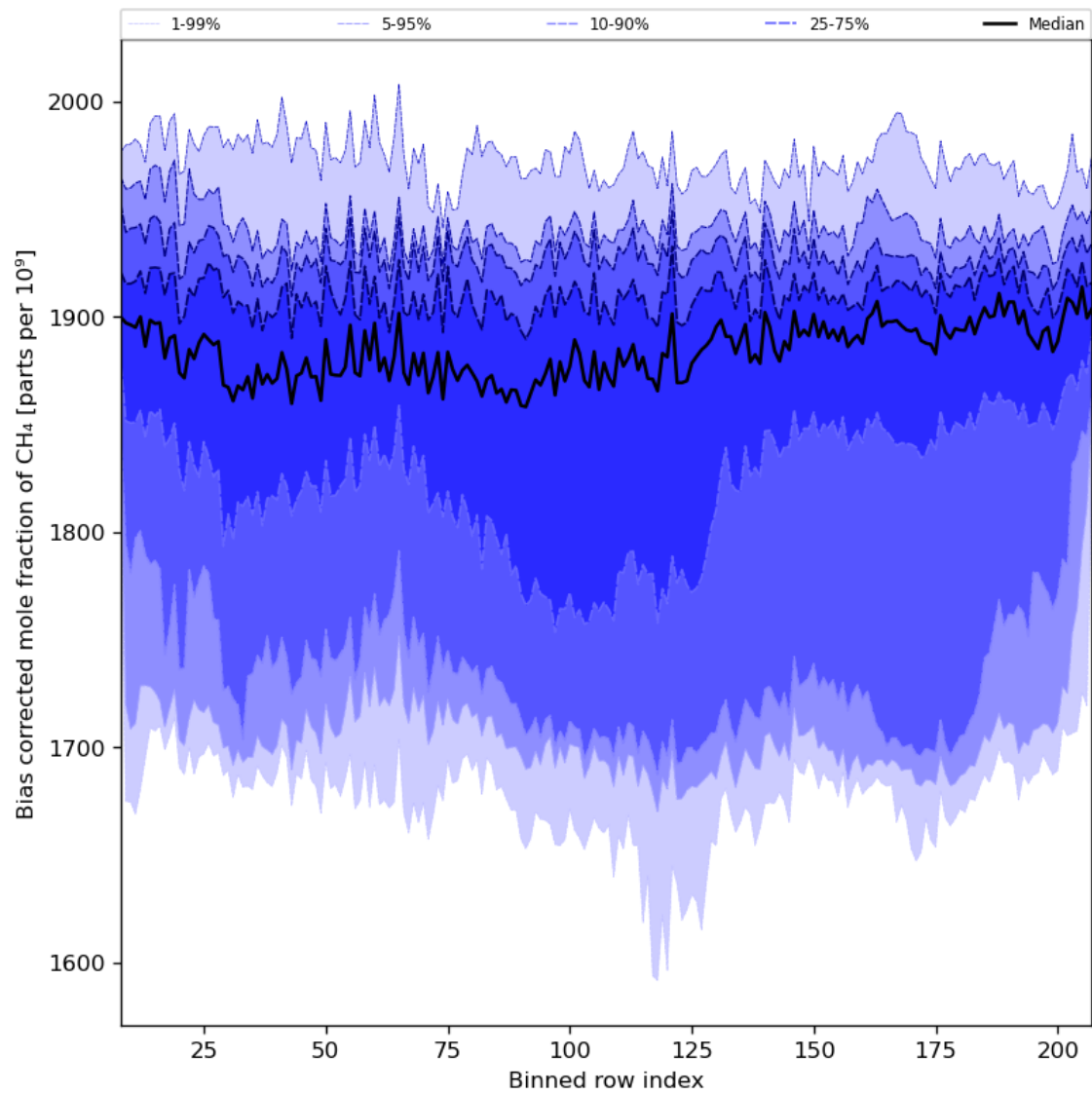
Figure 36: Along track statistics of “Bias corrected mole fraction of \text{CH}_4 ” for 2023-11-08 to 2023-11-10
