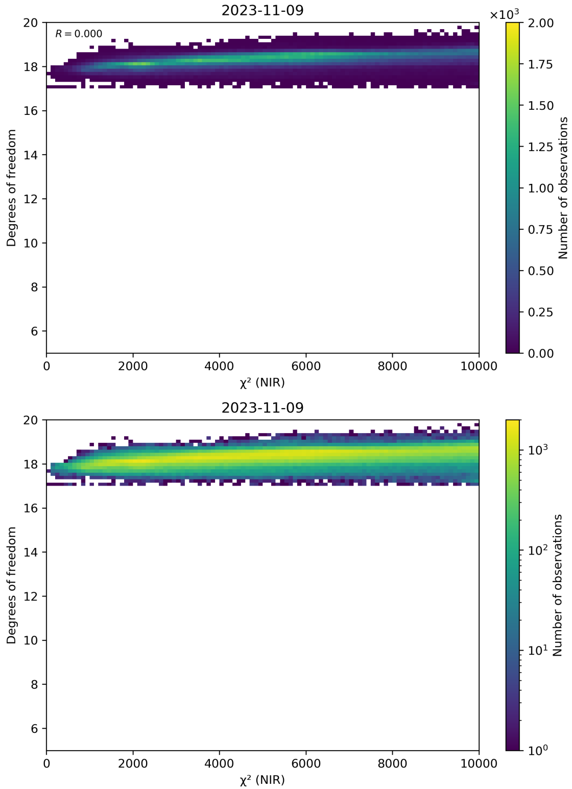
Figure 44: Scatter density plot of “ \chi^2 (NIR)” against “Degrees of freedom” for 2023-11-08 to 2023-11-10.
