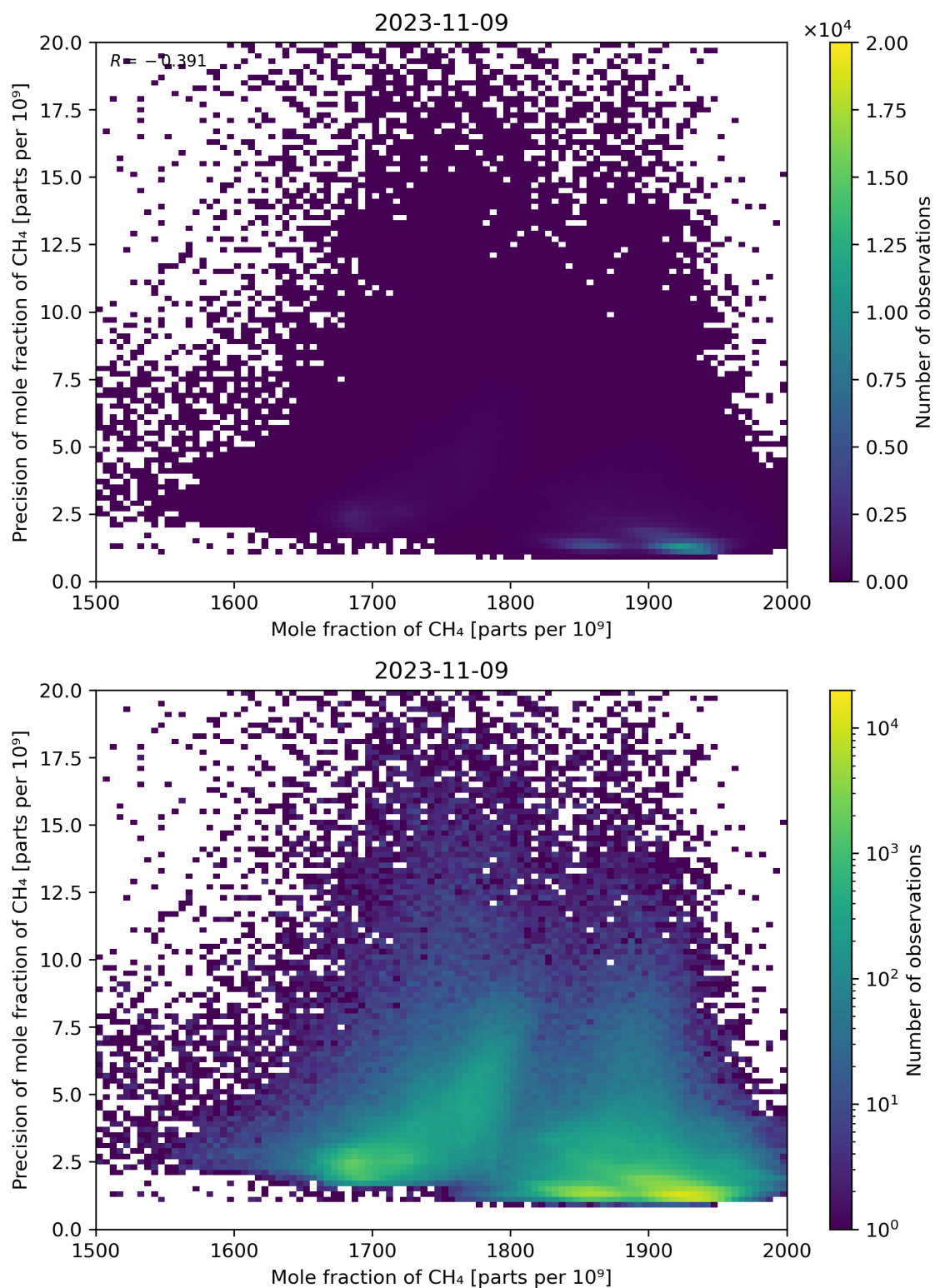
Figure 75: Scatter density plot of “Mole fraction of CH 4 ” against “Precision of mole fraction of CH 4 ” for 2023-11-08 to 2023-11-10.
