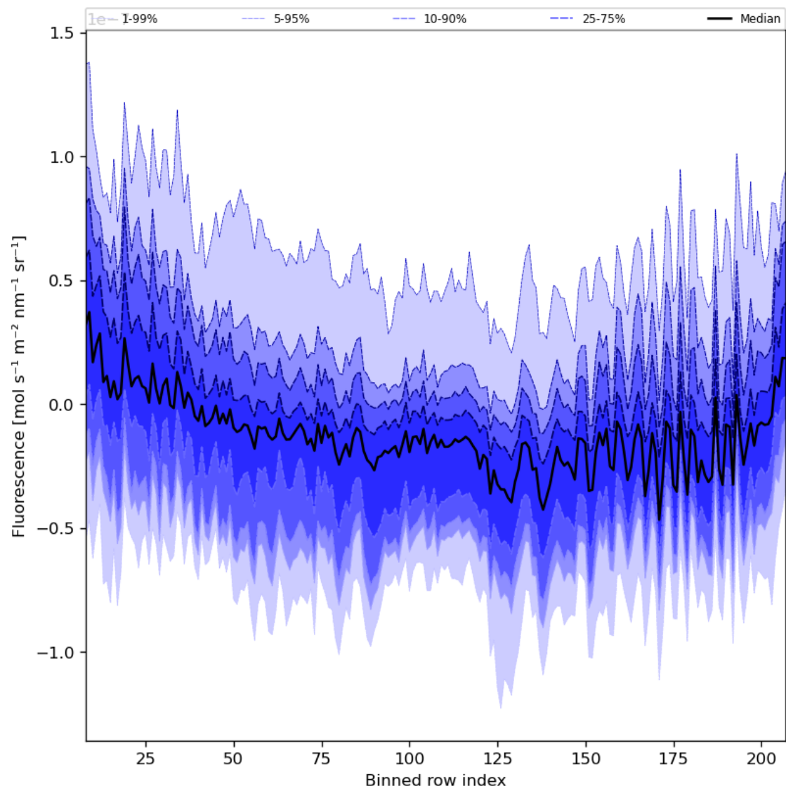
Figure 43: Along track statistics of “Fluorescence” for 2023-11-08 to 2023-11-10
