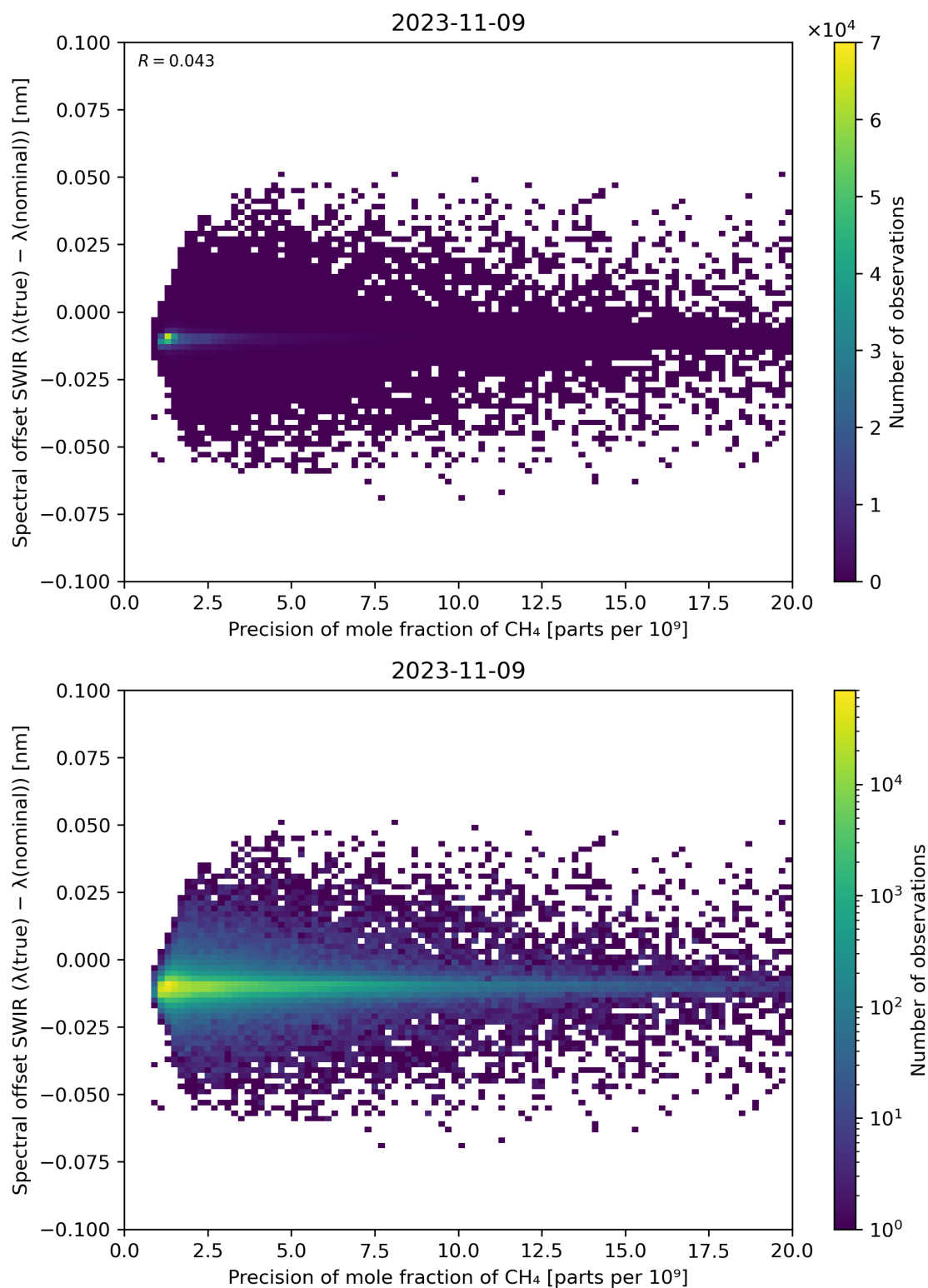
Figure 85: Scatter density plot of “Precision of mole fraction of CH 4 ” against “Spectral offset SWIR ( \lambda(\text{true}) - \lambda(\text{nominal}) )” for 2023-11-08 to 2023-11-10.
