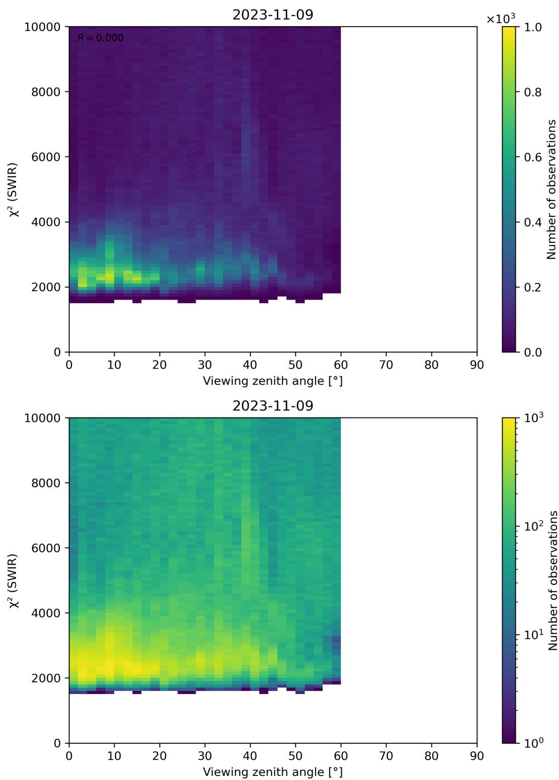
Figure 106: Scatter density plot of “Viewing zenith angle” against “ \chi^2 (SWIR)” for 2023-11-08 to 2023-11-10.
