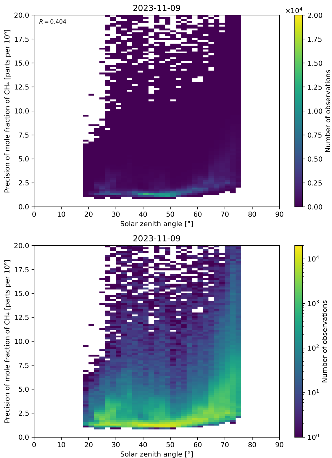
Figure 101: Scatter density plot of “Solar zenith angle” against “Precision of mole fraction of CH 4 ” for 2023-11-08 to 2023-11-10.
