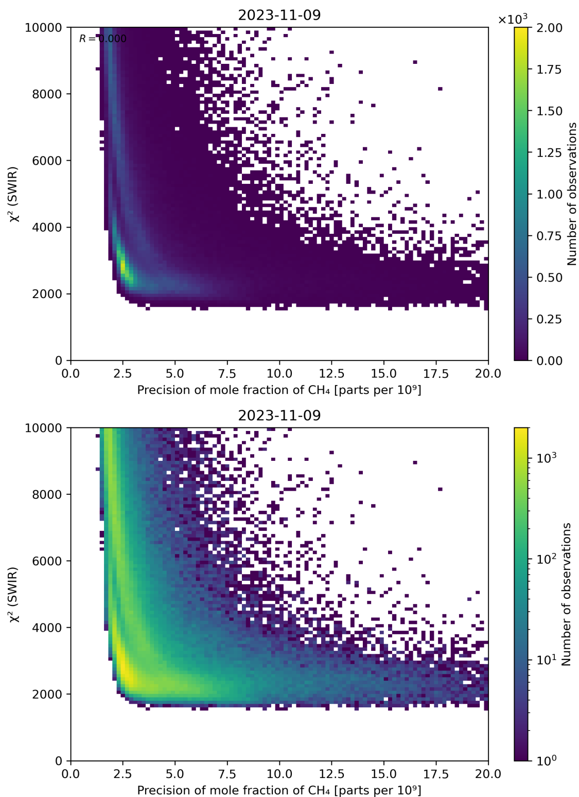
Figure 79: Scatter density plot of “Precision of mole fraction of CH 4 ” against “ \chi^2 (SWIR)” for 2023-11-08 to 2023-11-10.
