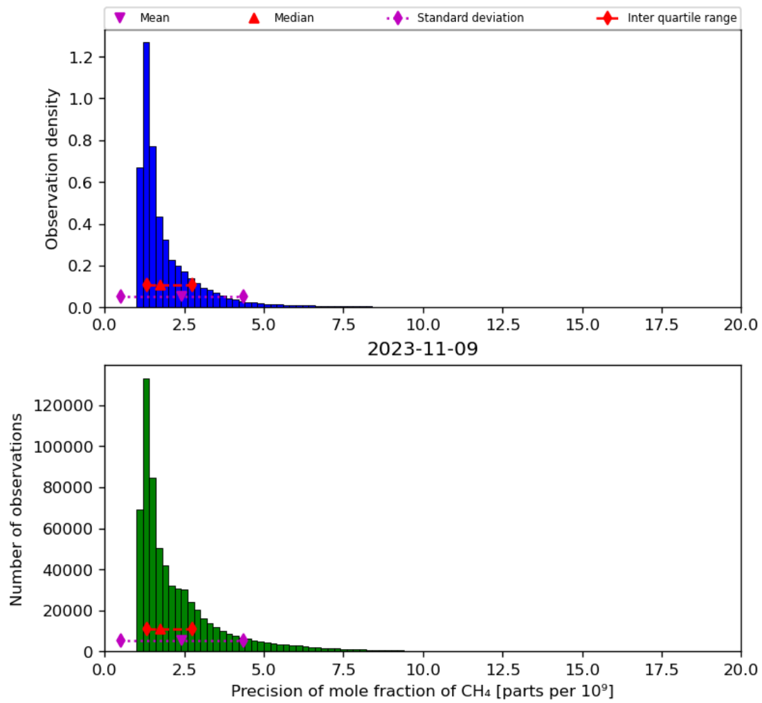
Figure 24: Histogram of “Precision of mole fraction of CH 4 ” for 2023-11-08 to 2023-11-10
