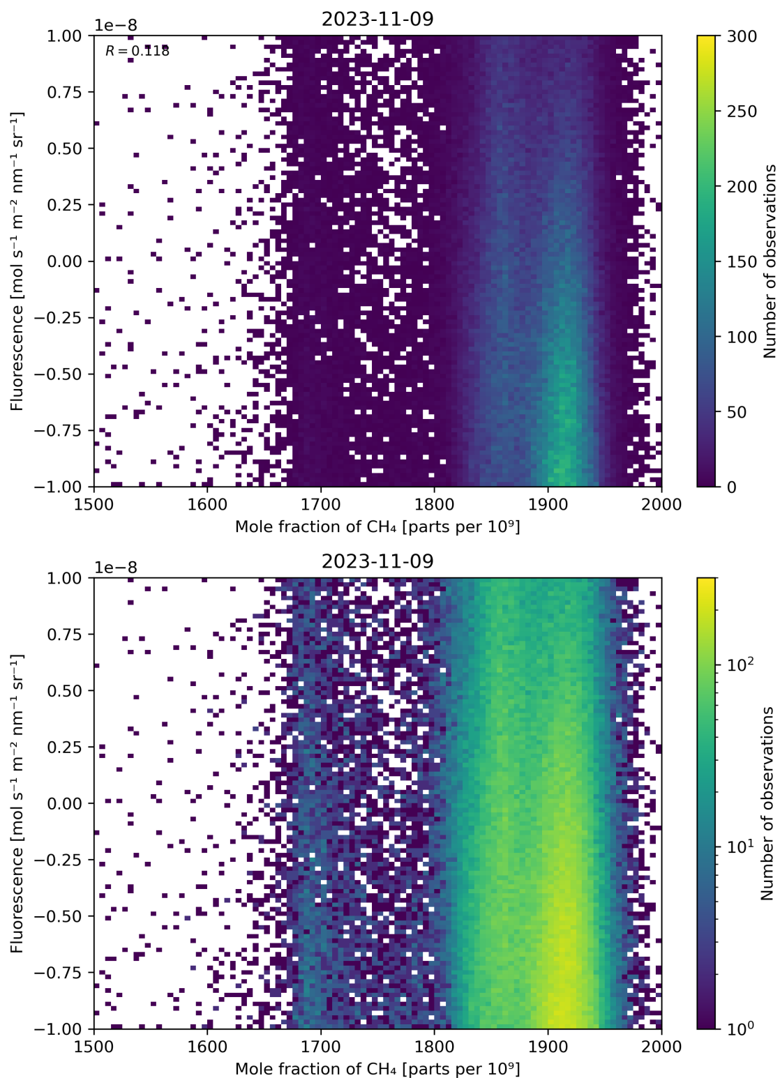
Figure 73: Scatter density plot of “Mole fraction of \text{CH}_4 ” against “Fluorescence” for 2023-11-08 to 2023-11-10.
