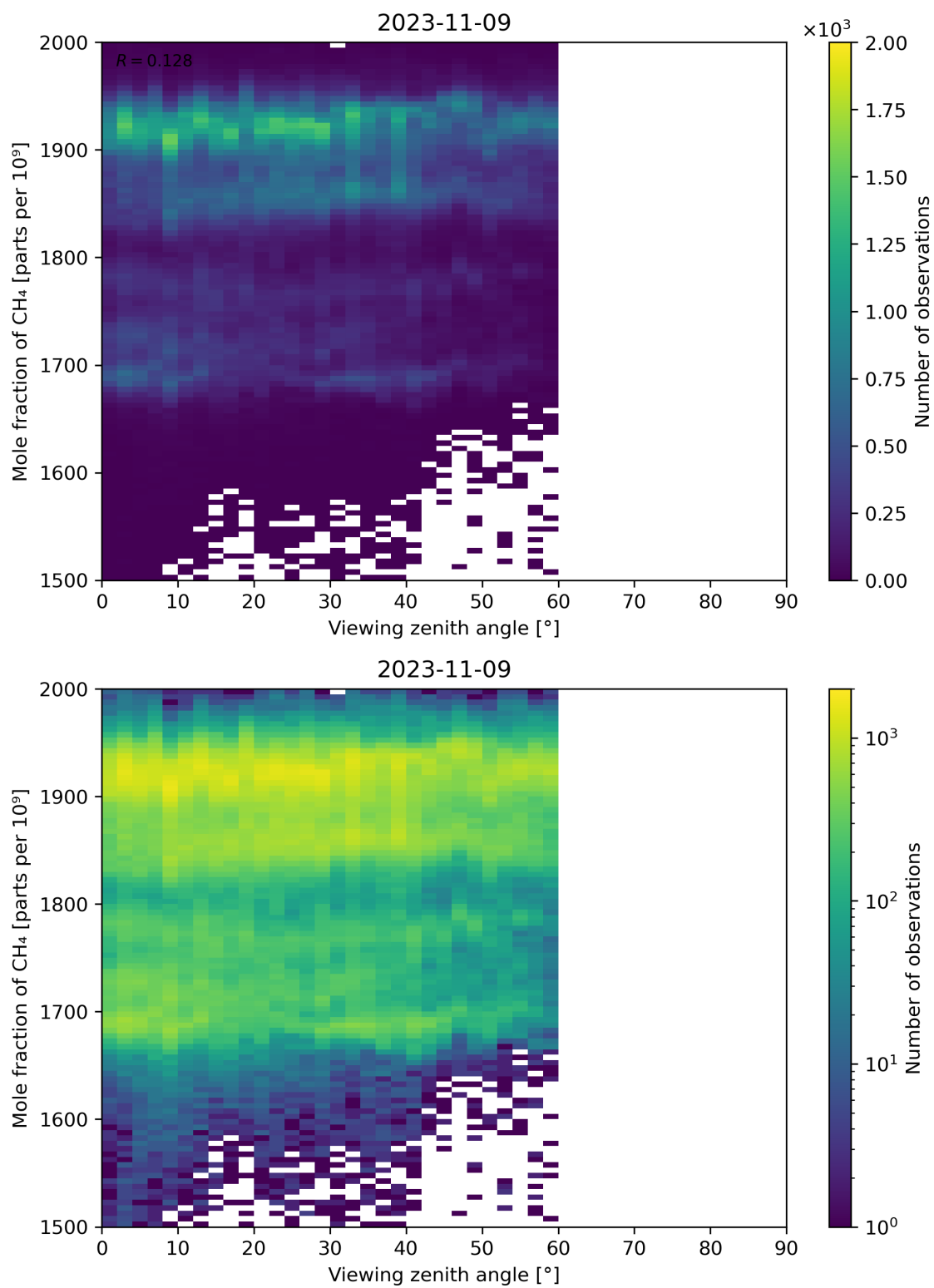
Figure 110: Scatter density plot of “Viewing zenith angle” against “Mole fraction of CH 4 ” for 2023-11-08 to 2023-11-10.
