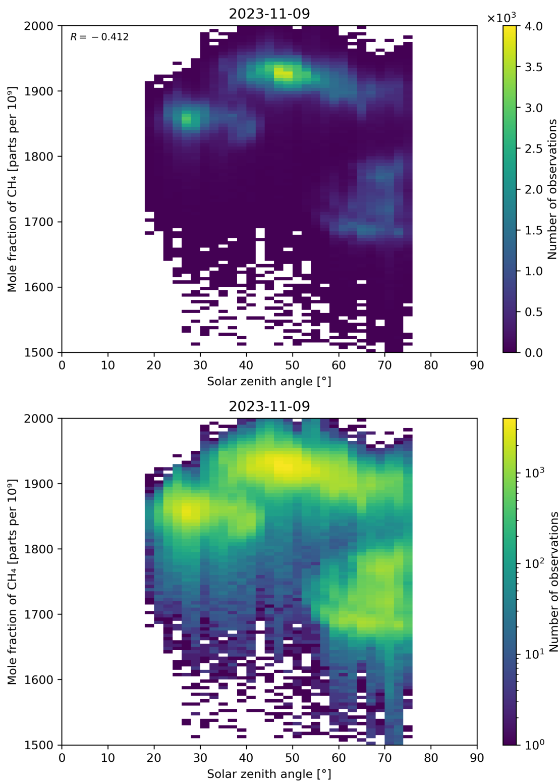
Figure 99: Scatter density plot of “Solar zenith angle” against “Mole fraction of \text{CH}_4 ” for 2023-11-08 to 2023-11-10.
