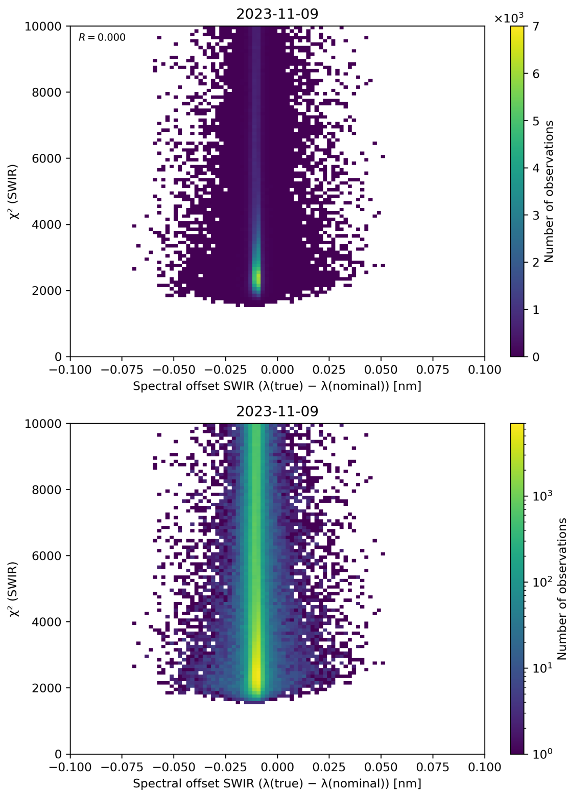
Figure 118: Scatter density plot of “Spectral offset SWIR ( \lambda(\text{true}) - \lambda(\text{nominal}) )” against “ \chi^2 (SWIR)” for 2023-11-08 to 2023-11-10.
