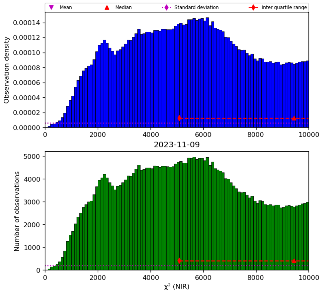
Figure 29: Histogram of “ \chi^2 (NIR)” for 2023-11-08 to 2023-11-10
