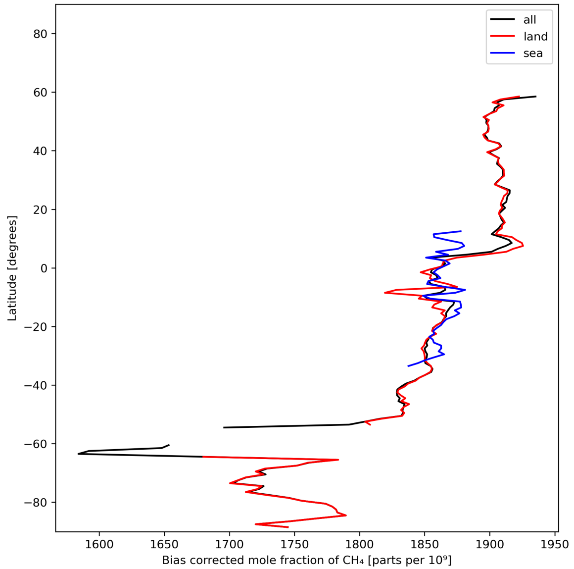
Figure 14: Zonal average of “Bias corrected mole fraction of CH 4 ” for 2023-11-08 to 2023-11-10.
