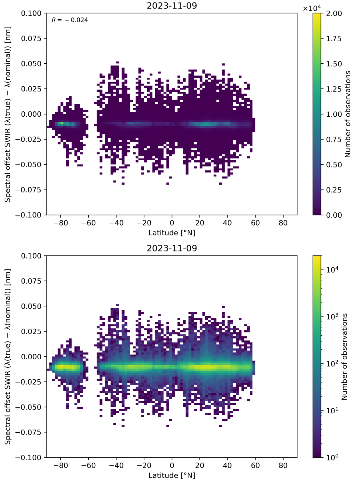
Figure 62: Scatter density plot of “Latitude” against “Spectral offset SWIR ( \lambda(\text{true}) - \lambda(\text{nominal}) )” for 2023-11-08 to 2023-11-10.
