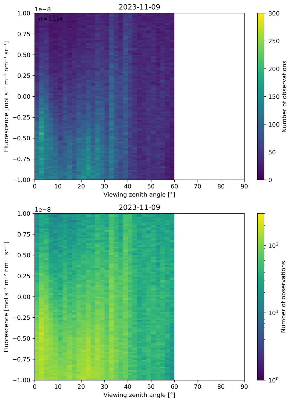
Figure 108: Scatter density plot of “Viewing zenith angle” against “Fluorescence” for 2023-11-08 to 2023-11-10.
