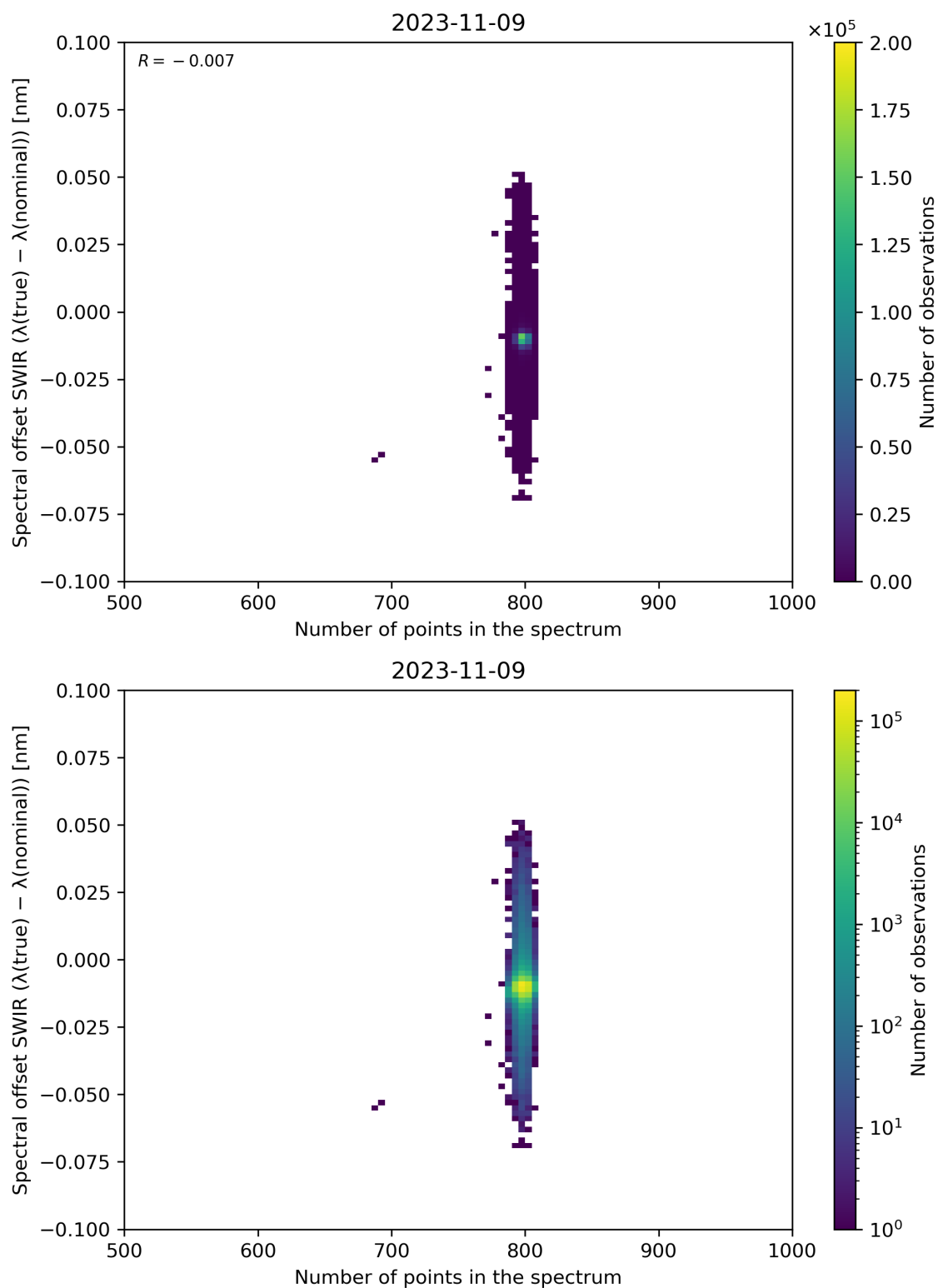
Figure 93: Scatter density plot of “Number of points in the spectrum” against “Spectral offset SWIR ( \lambda(\text{true}) - \lambda(\text{nominal}) )” for 2023-11-08 to 2023-11-10.
