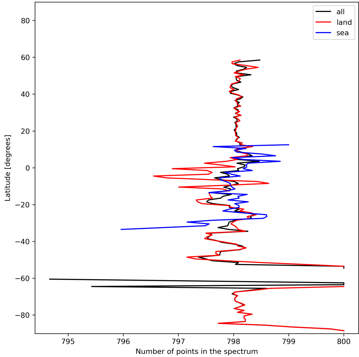
Figure 15: Zonal average of “Number of points in the spectrum” for 2023-11-08 to 2023-11-10.
