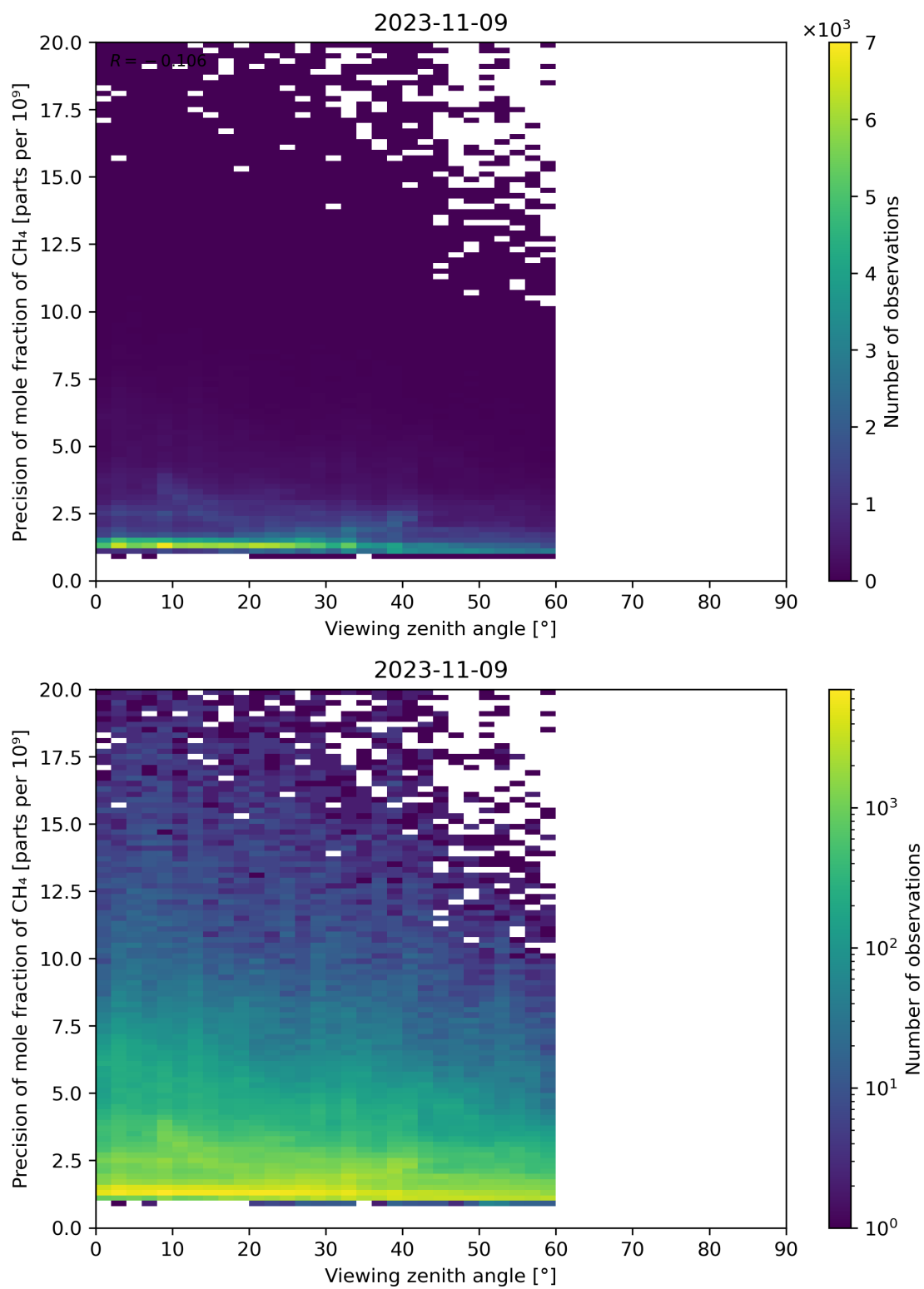
Figure 112: Scatter density plot of “Viewing zenith angle” against “Precision of mole fraction of CH 4 ” for 2023-11-08 to 2023-11-10.
