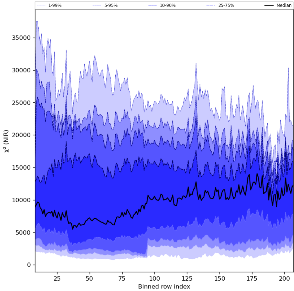
Figure 40: Along track statistics of “ \chi^2 (NIR)” for 2023-11-08 to 2023-11-10
