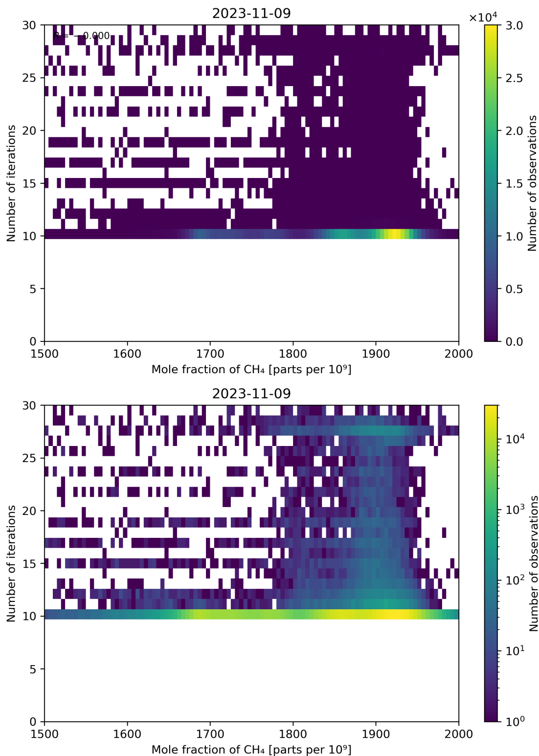
Figure 76: Scatter density plot of “Mole fraction of CH 4 ” against “Number of iterations” for 2023-11-08 to 2023-11-10.
