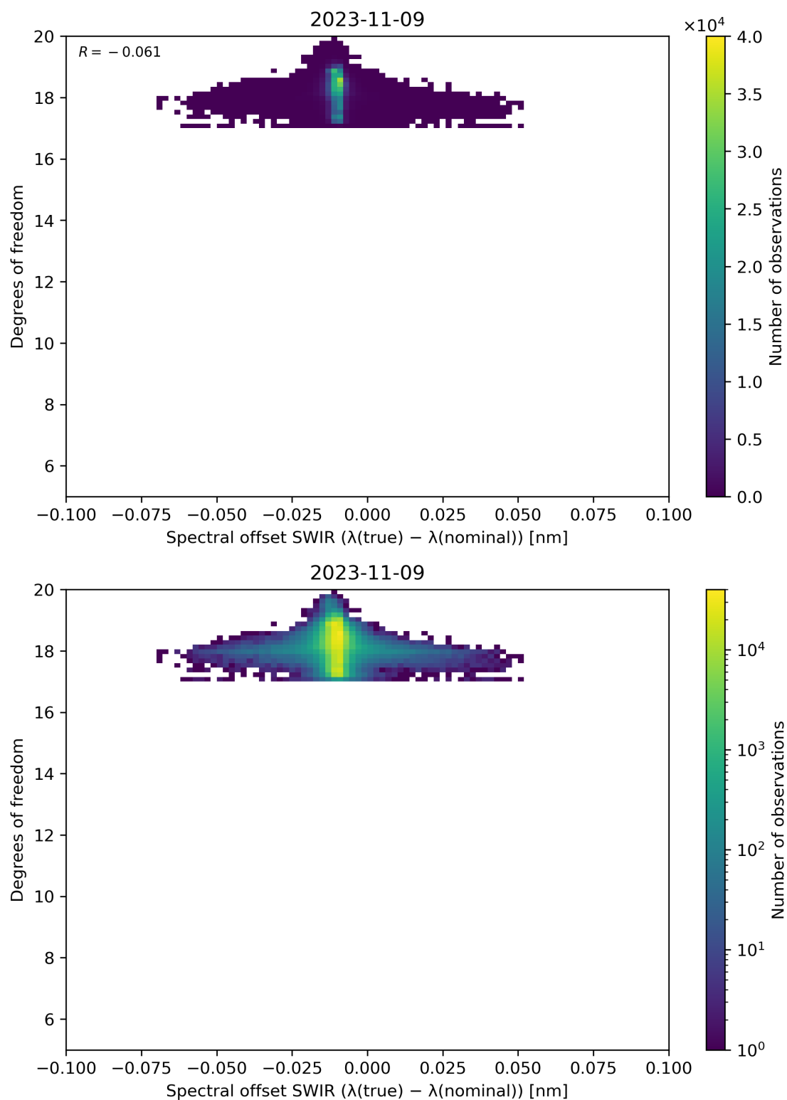
Figure 119: Scatter density plot of “Spectral offset SWIR ( \lambda(\text{true}) - \lambda(\text{nominal}) )” against “Degrees of freedom” for 2023-11-08 to 2023-11-10.
