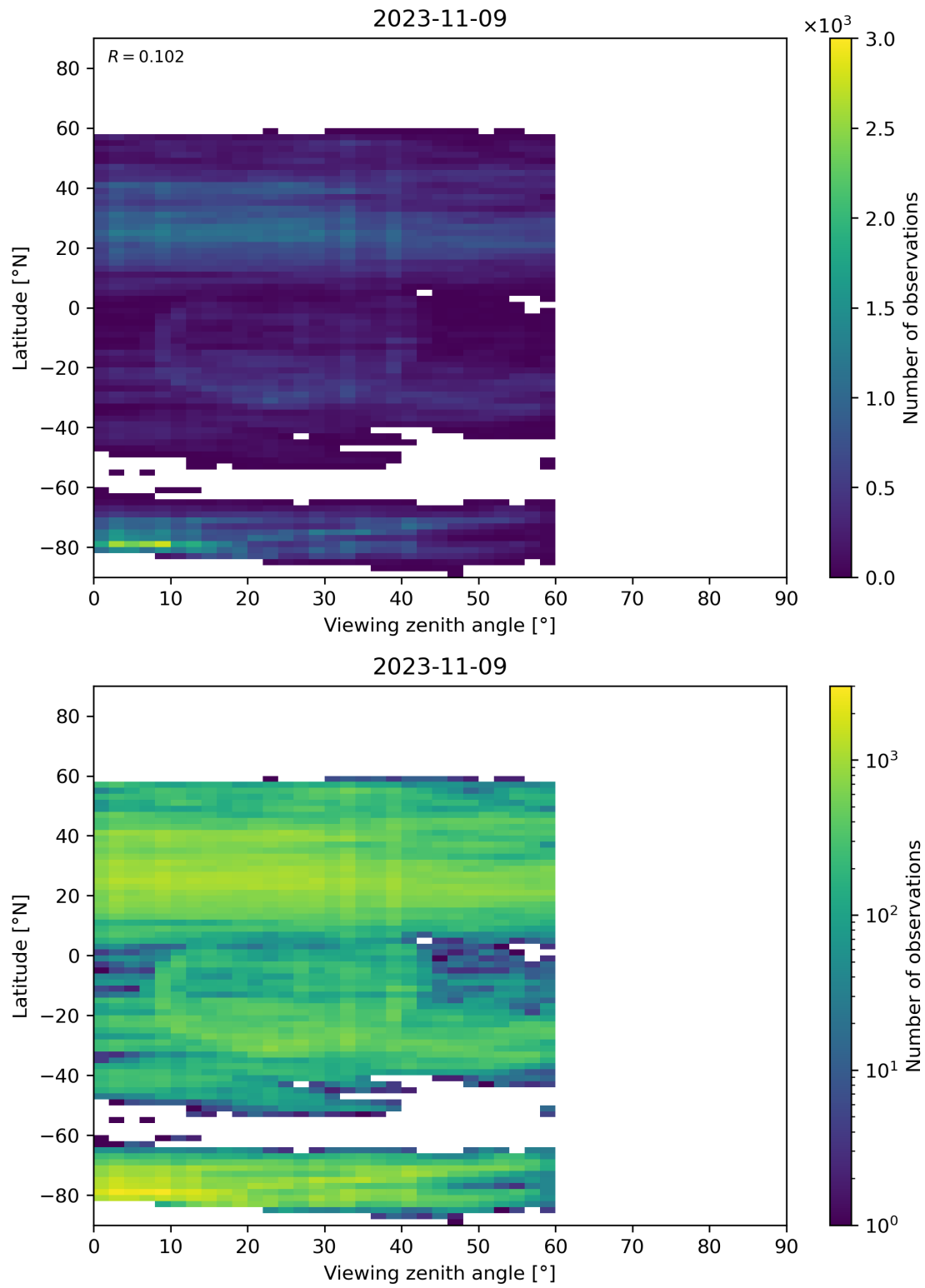
Figure 109: Scatter density plot of “Viewing zenith angle” against “Latitude” for 2023-11-08 to 2023-11-10.
