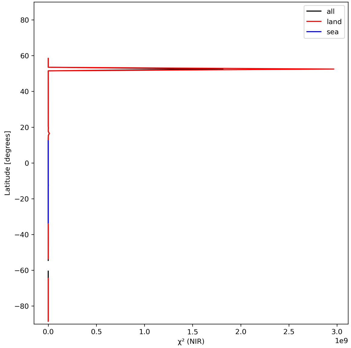
Figure 18: Zonal average of “ \chi^2 (NIR)” for 2023-11-08 to 2023-11-10.
