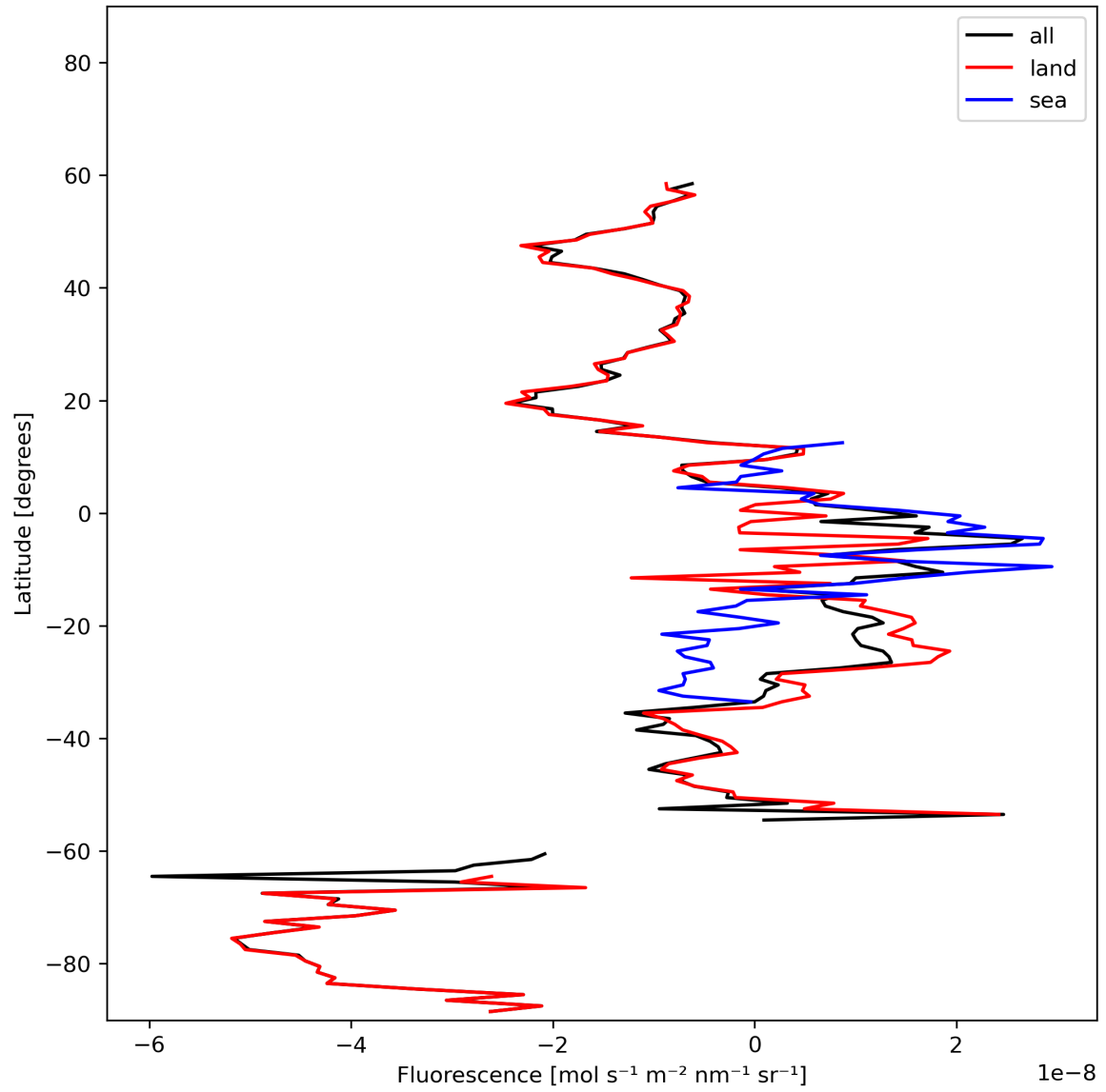
Figure 21: Zonal average of “Fluorescence” for 2023-11-08 to 2023-11-10.
