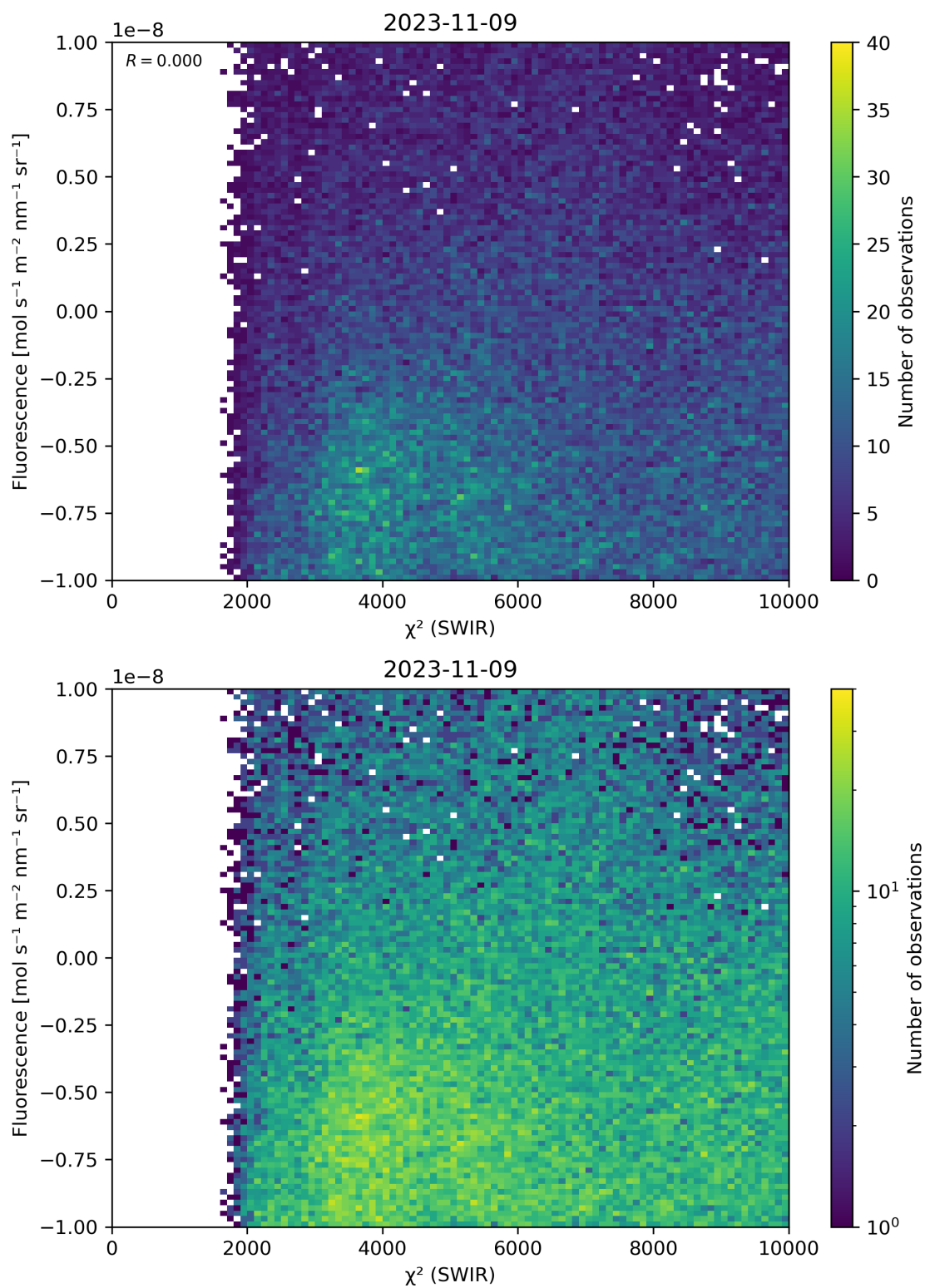
Figure 49: Scatter density plot of “ \chi^2 (SWIR)” against “Fluorescence” for 2023-11-08 to 2023-11-10.
