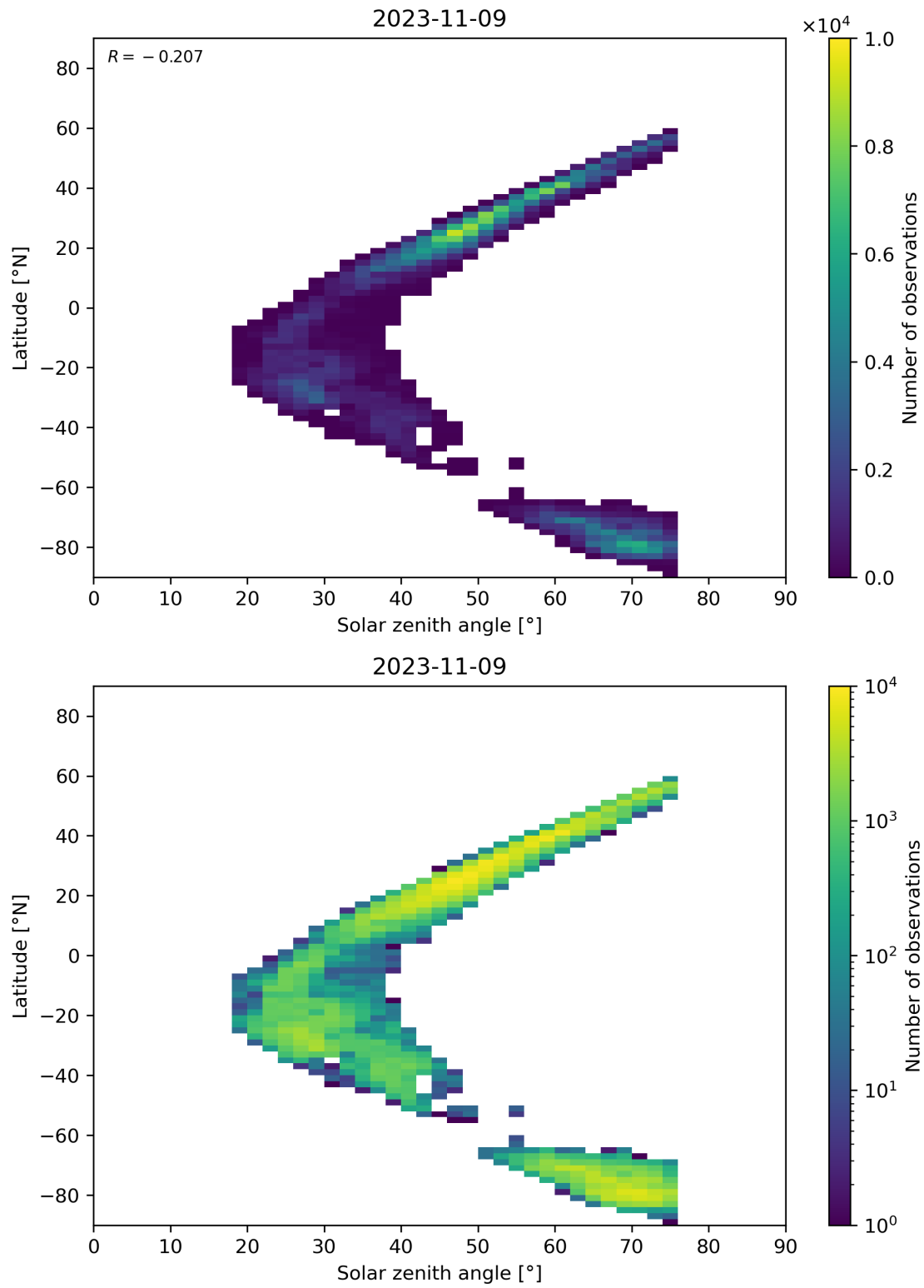
Figure 98: Scatter density plot of “Solar zenith angle” against “Latitude” for 2023-11-08 to 2023-11-10.
