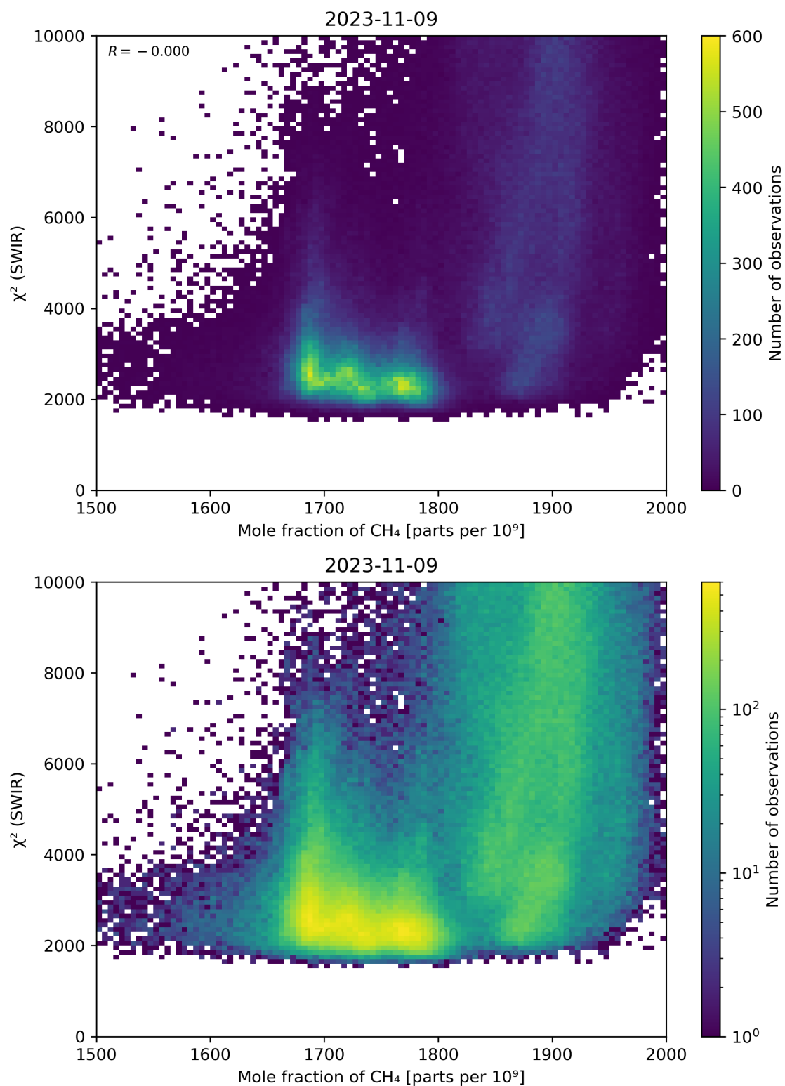
Figure 71: Scatter density plot of “Mole fraction of \text{CH}_4 ” against “ \chi^2 (SWIR)” for 2023-11-08 to 2023-11-10.
