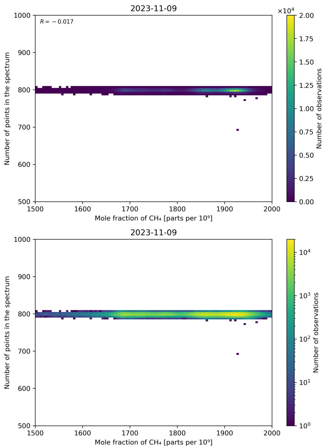
Figure 77: Scatter density plot of “Mole fraction of CH 4 ” against “Number of points in the spectrum” for 2023-11-08 to 2023-11-10.
