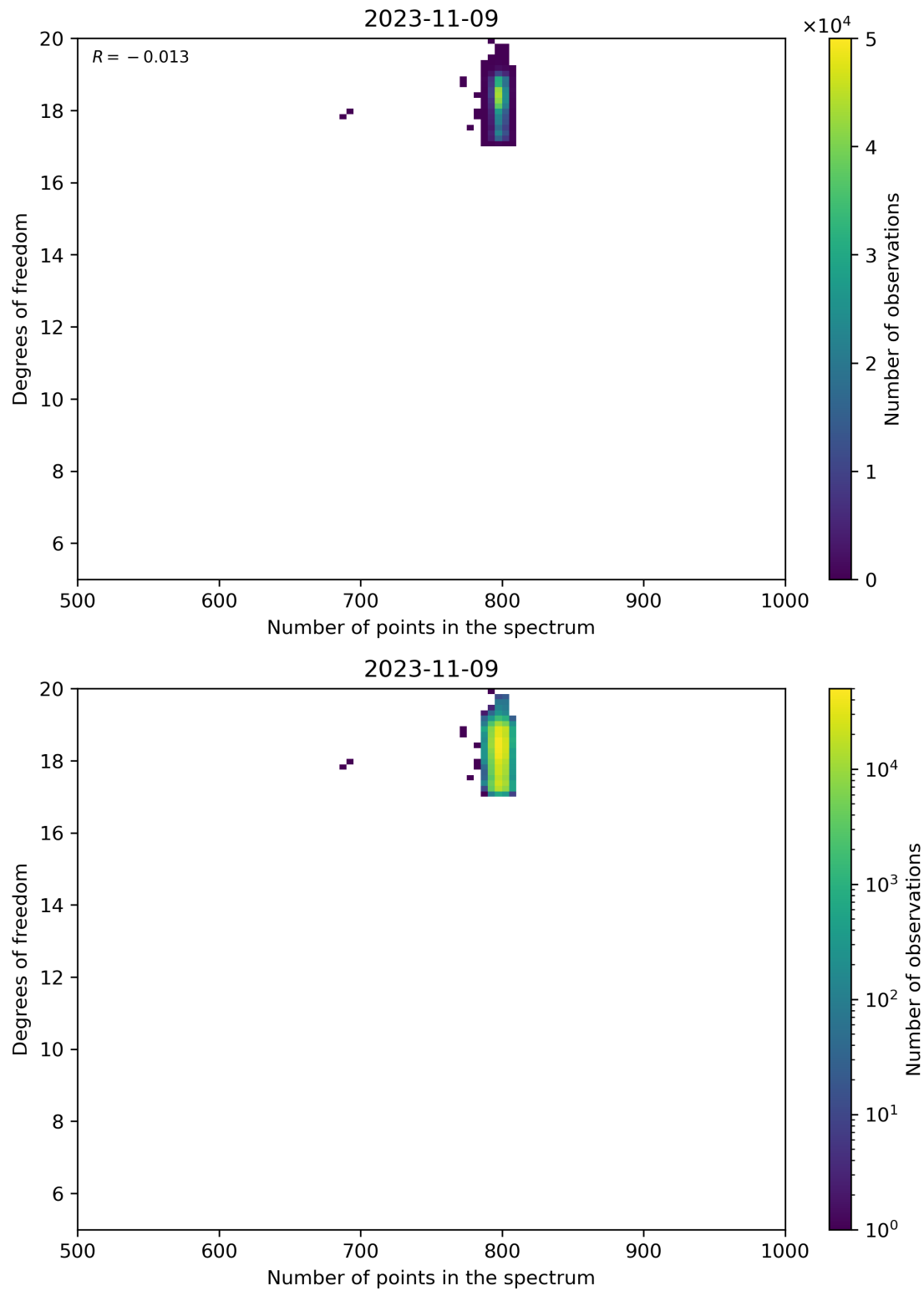
Figure 90: Scatter density plot of “Number of points in the spectrum” against “Degrees of freedom” for 2023-11-08 to 2023-11-10.
