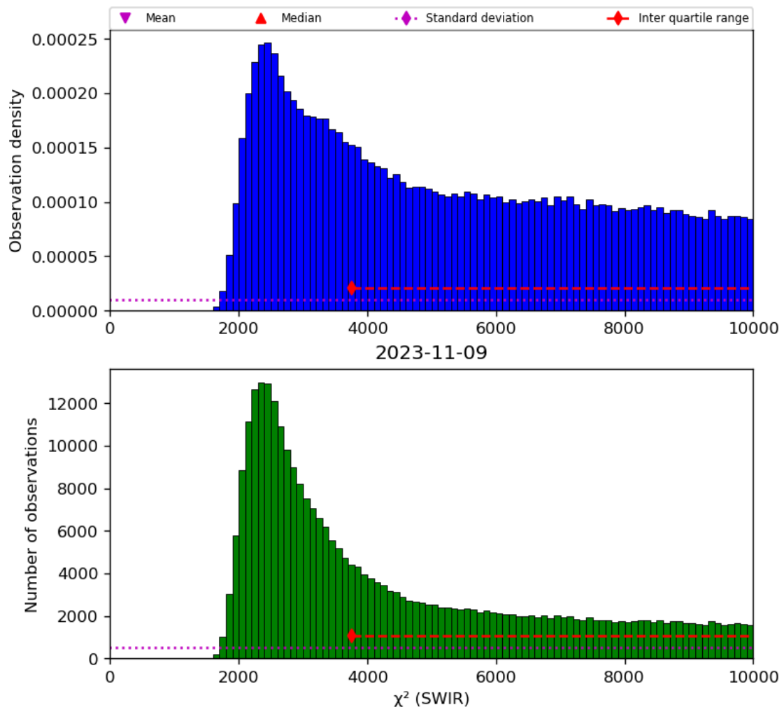
Figure 28: Histogram of “ \chi^2 (SWIR)” for 2023-11-08 to 2023-11-10
