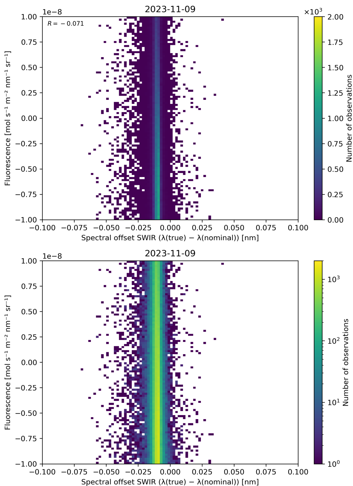
Figure 120: Scatter density plot of “Spectral offset SWIR ( \lambda(\text{true}) - \lambda(\text{nominal}) )” against “Fluorescence” for 2023-11-08 to 2023-11-10.
