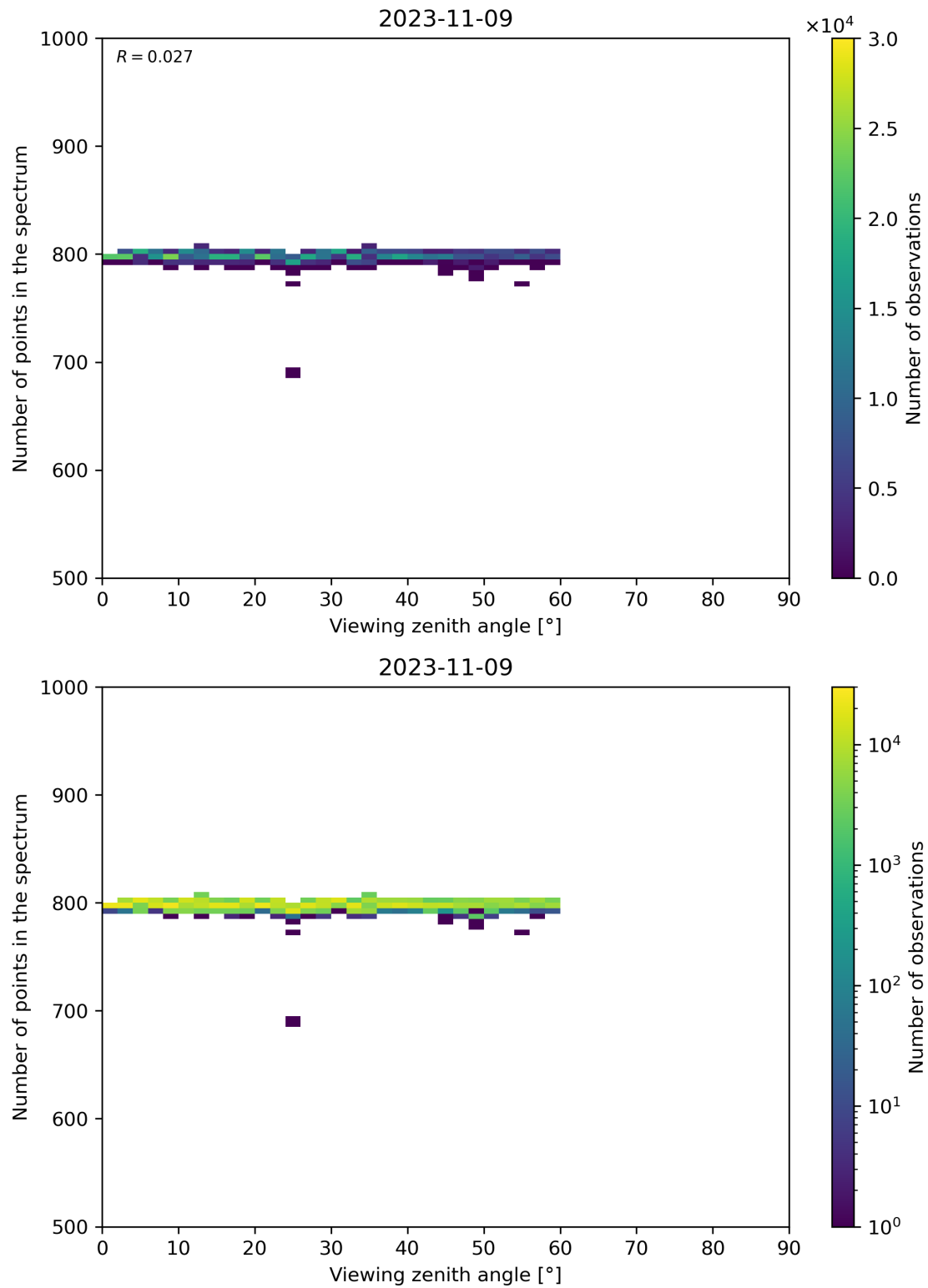
Figure 114: Scatter density plot of “Viewing zenith angle” against “Number of points in the spectrum” for 2023-11-08 to 2023-11-10.
