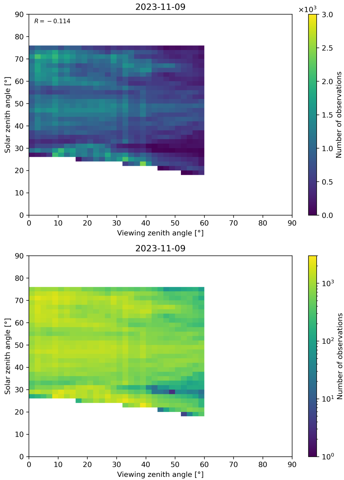
Figure 115: Scatter density plot of “Viewing zenith angle” against “Solar zenith angle” for 2023-11-08 to 2023-11-10.
