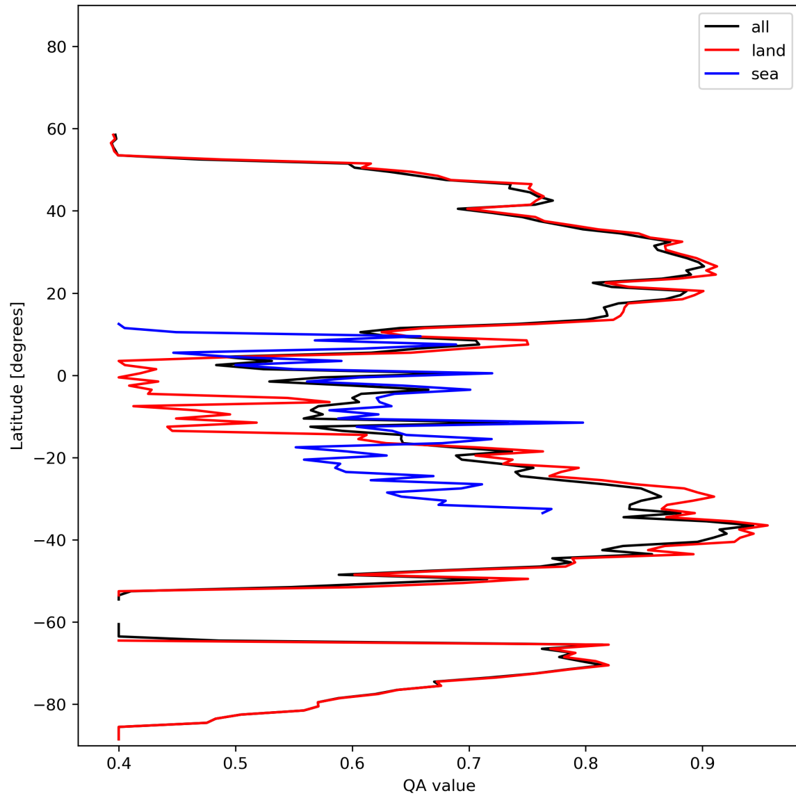
Figure 11: Zonal average of “QA value” for 2023-11-08 to 2023-11-10.
