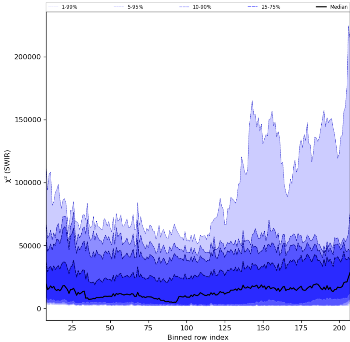
Figure 39: Along track statistics of “ \chi^2 (SWIR)” for 2023-11-08 to 2023-11-10
