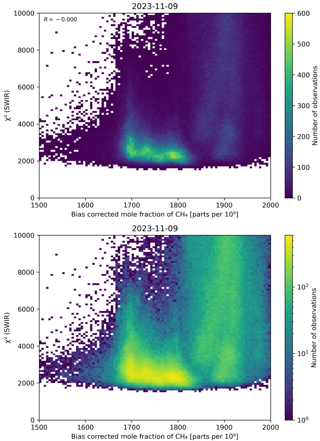
Figure 64: Scatter density plot of “Bias corrected mole fraction of CH 4 ” against “ \chi^2 (SWIR)” for 2023-11-08 to 2023-11-10.
