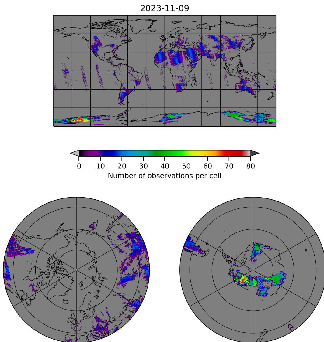
Figure 10: Map of the number of observations for 2023-11-08 to 2023-11-10
