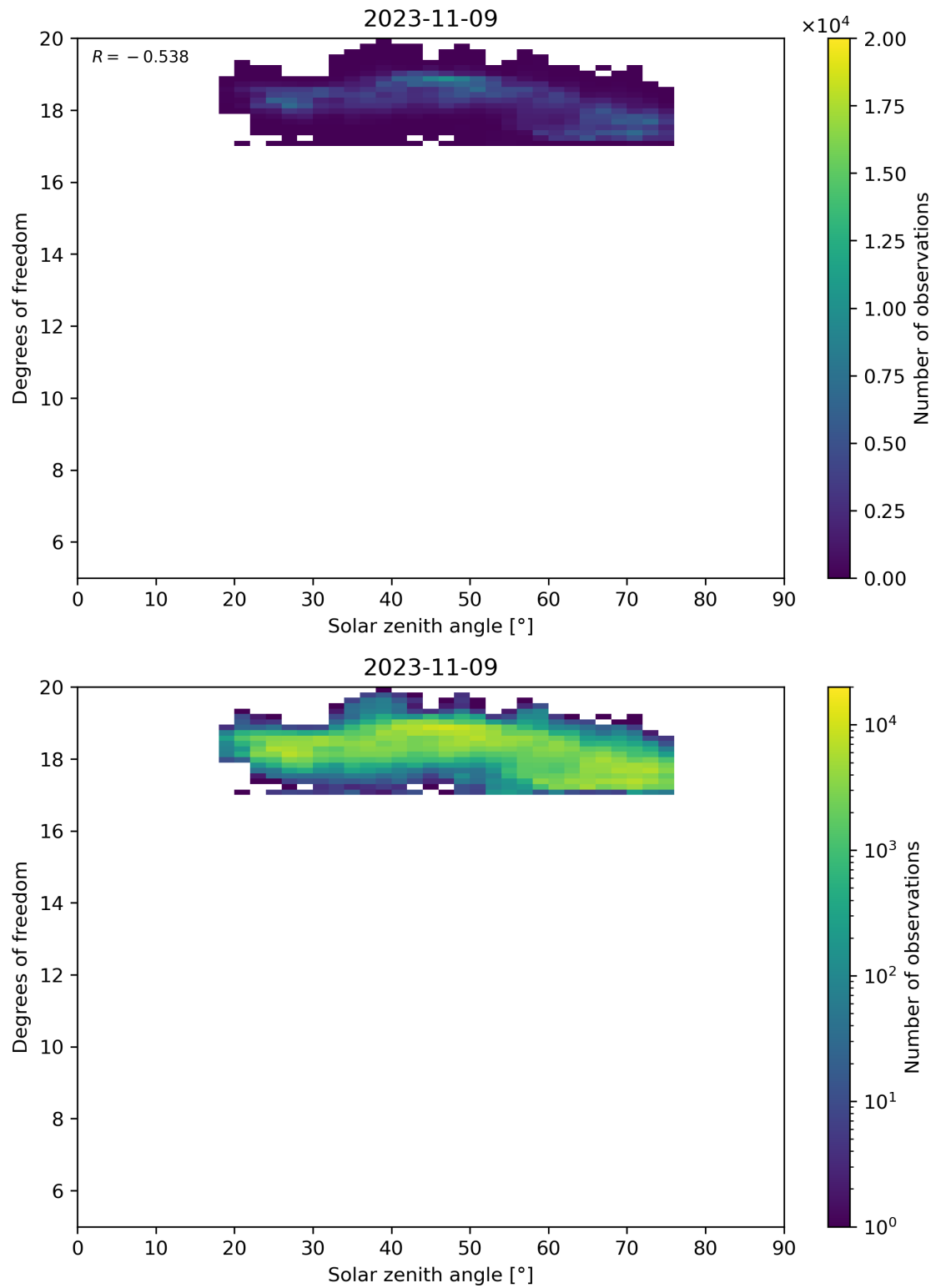
Figure 96: Scatter density plot of “Solar zenith angle” against “Degrees of freedom” for 2023-11-08 to 2023-11-10.
