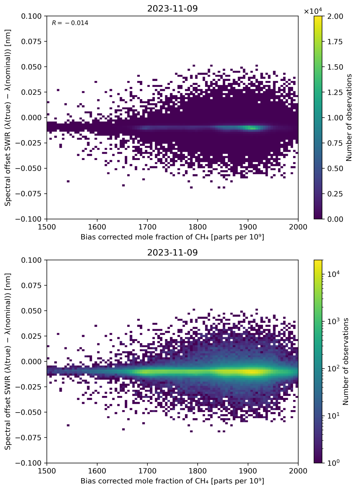
Figure 69: Scatter density plot of “Bias corrected mole fraction of \text{CH}_4 ” against “Spectral offset SWIR ( \lambda(\text{true}) - \lambda(\text{nominal}) )” for 2023-11-08 to 2023-11-10.
