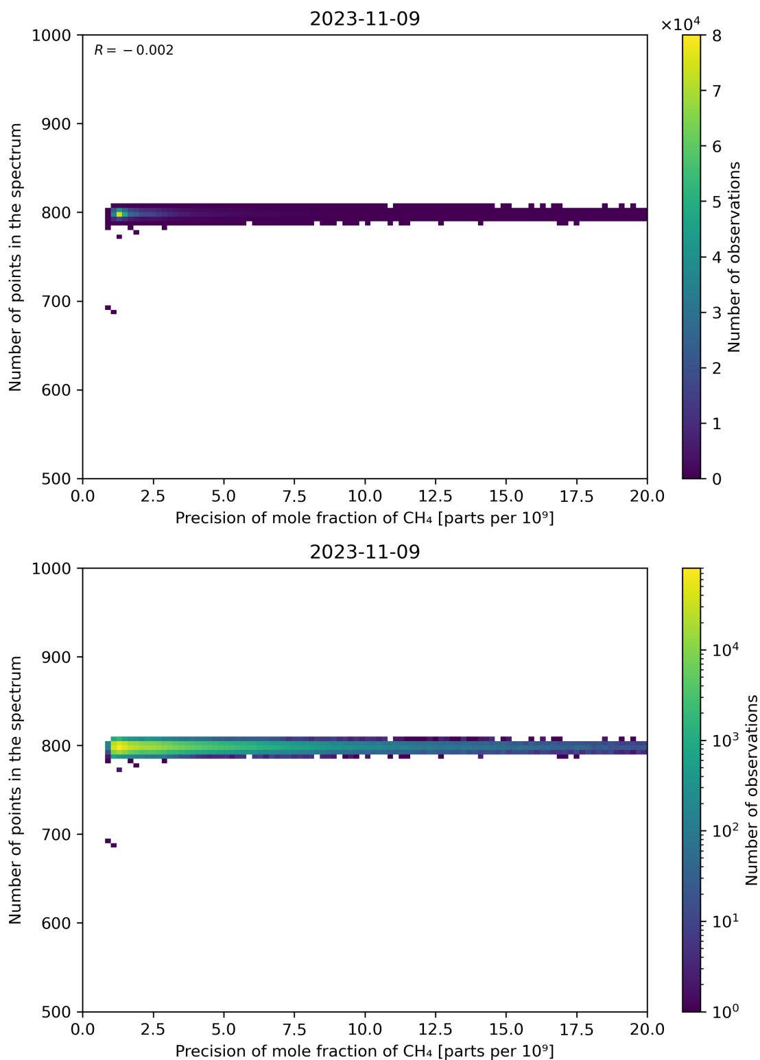
Figure 84: Scatter density plot of “Precision of mole fraction of CH 4 ” against “Number of points in the spectrum” for 2023-11-08 to 2023-11-10.
