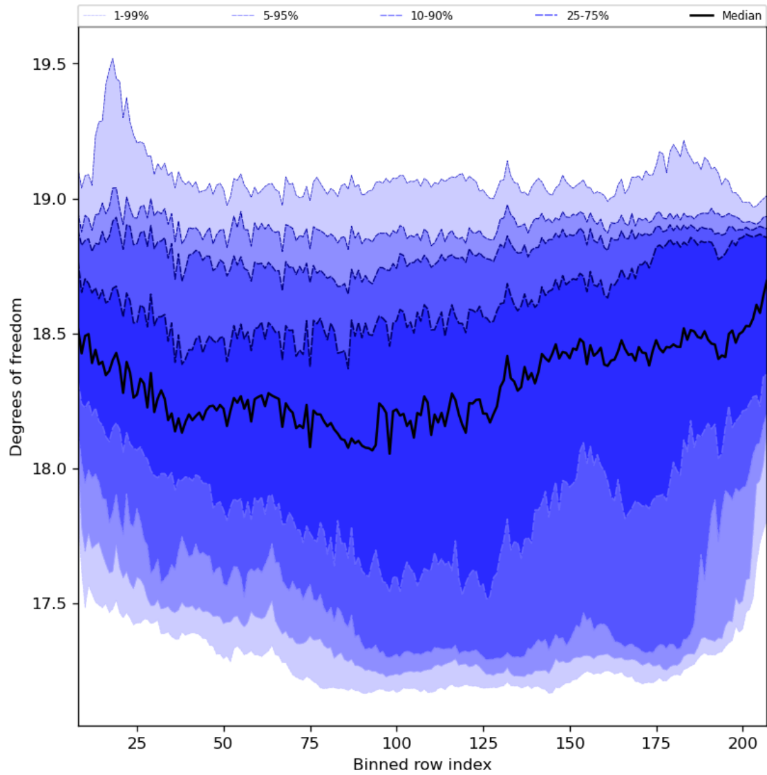
Figure 41: Along track statistics of “Degrees of freedom” for 2023-11-08 to 2023-11-10
