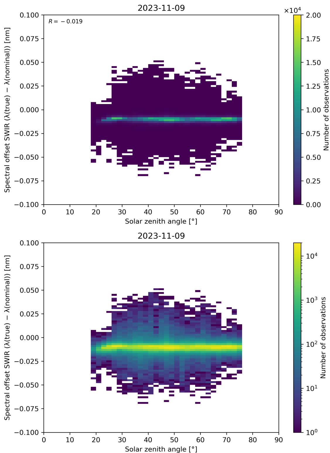
Figure 104: Scatter density plot of “Solar zenith angle” against “Spectral offset SWIR ( \lambda(\text{true}) - \lambda(\text{nominal}) )” for 2023-11-08 to 2023-11-10.
