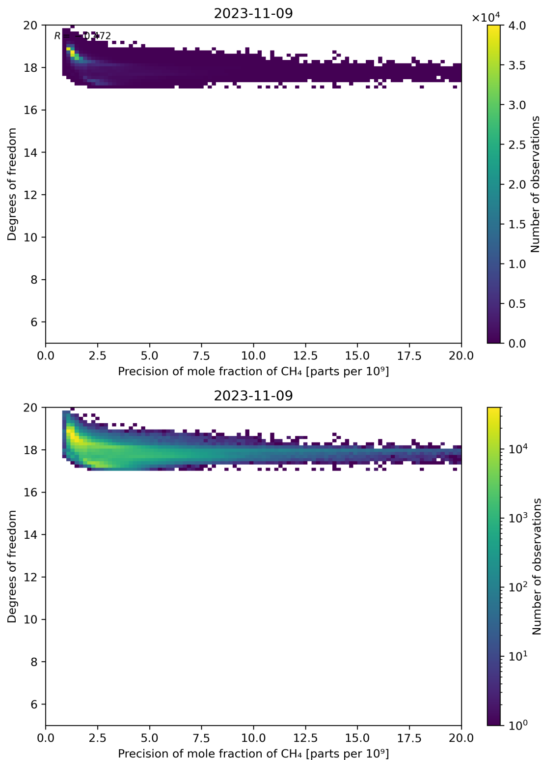
Figure 80: Scatter density plot of “Precision of mole fraction of CH 4 ” against “Degrees of freedom” for 2023-11-08 to 2023-11-10.
