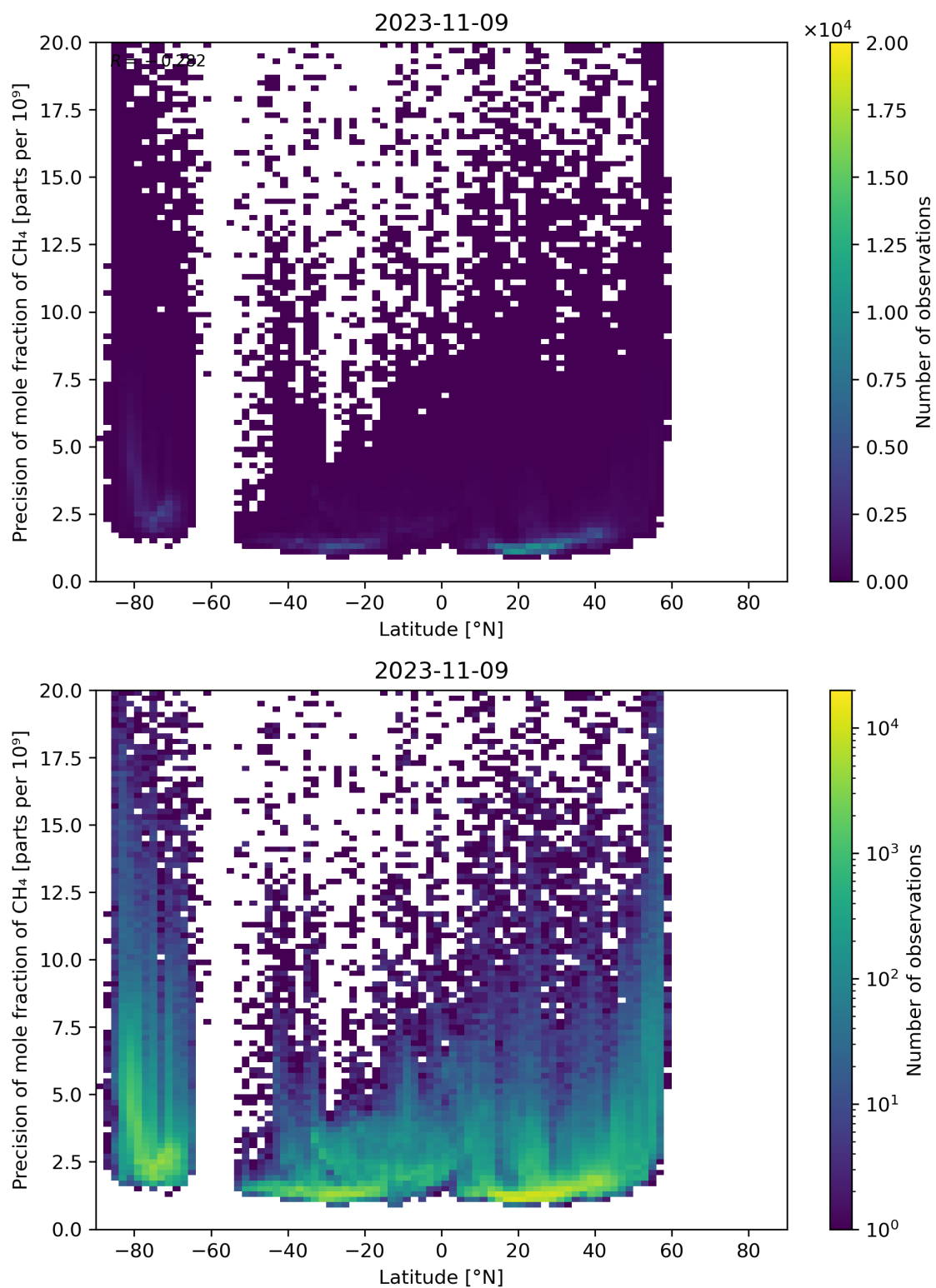
Figure 59: Scatter density plot of “Latitude” against “Precision of mole fraction of CH 4 ” for 2023-11-08 to 2023-11-10.
