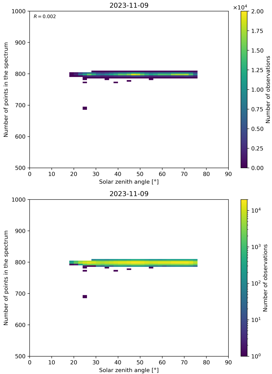
Figure 103: Scatter density plot of “Solar zenith angle” against “Number of points in the spectrum” for 2023-11-08 to 2023-11-10.
