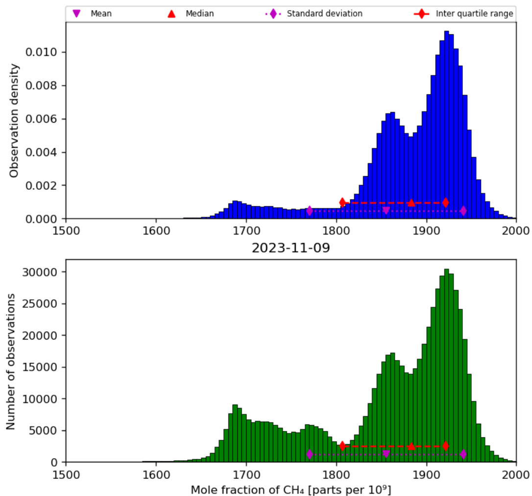
Figure 23: Histogram of “Mole fraction of CH 4 ” for 2023-11-08 to 2023-11-10
