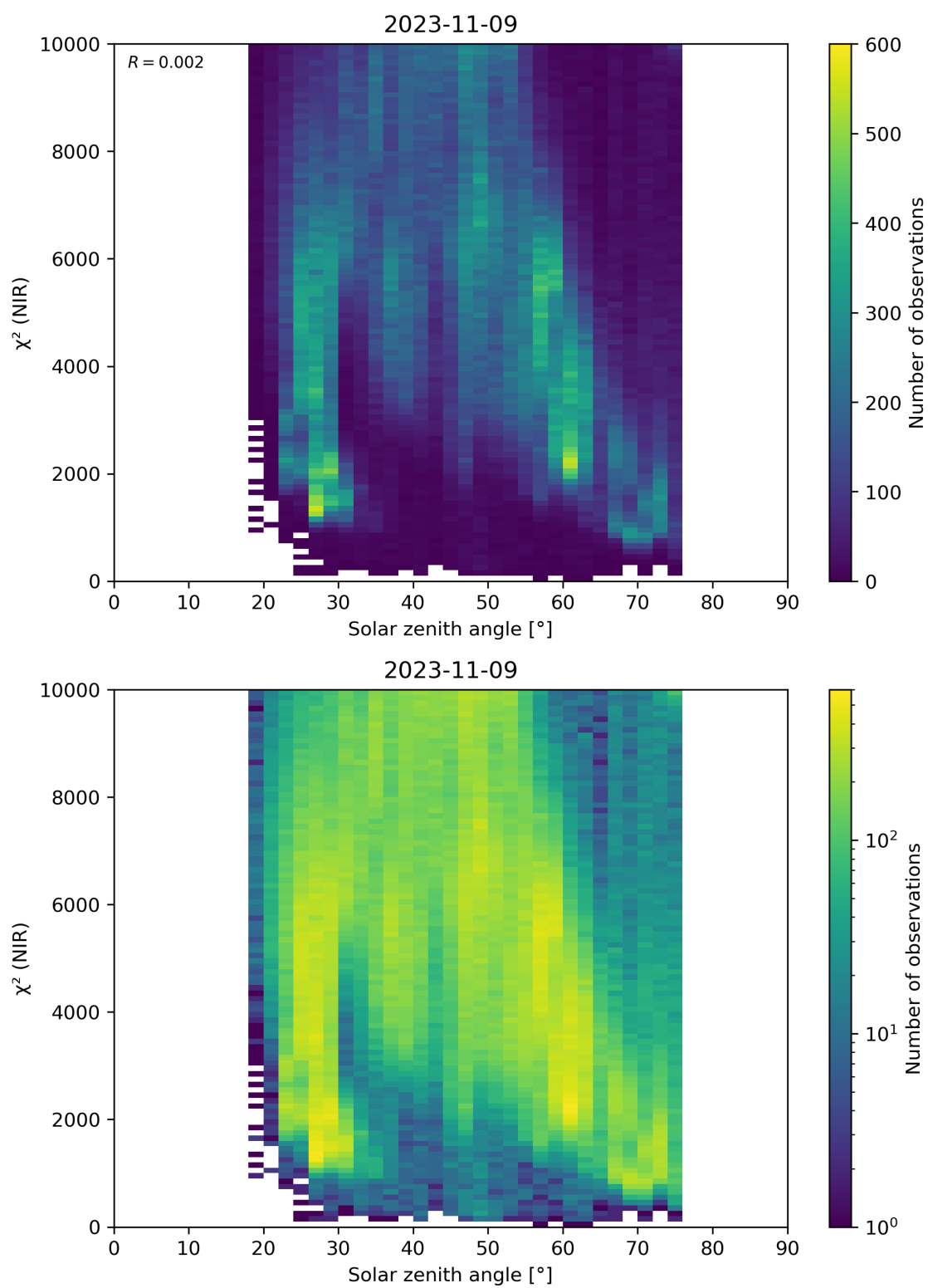
Figure 94: Scatter density plot of “Solar zenith angle” against “ \chi^2 (NIR)” for 2023-11-08 to 2023-11-10.
