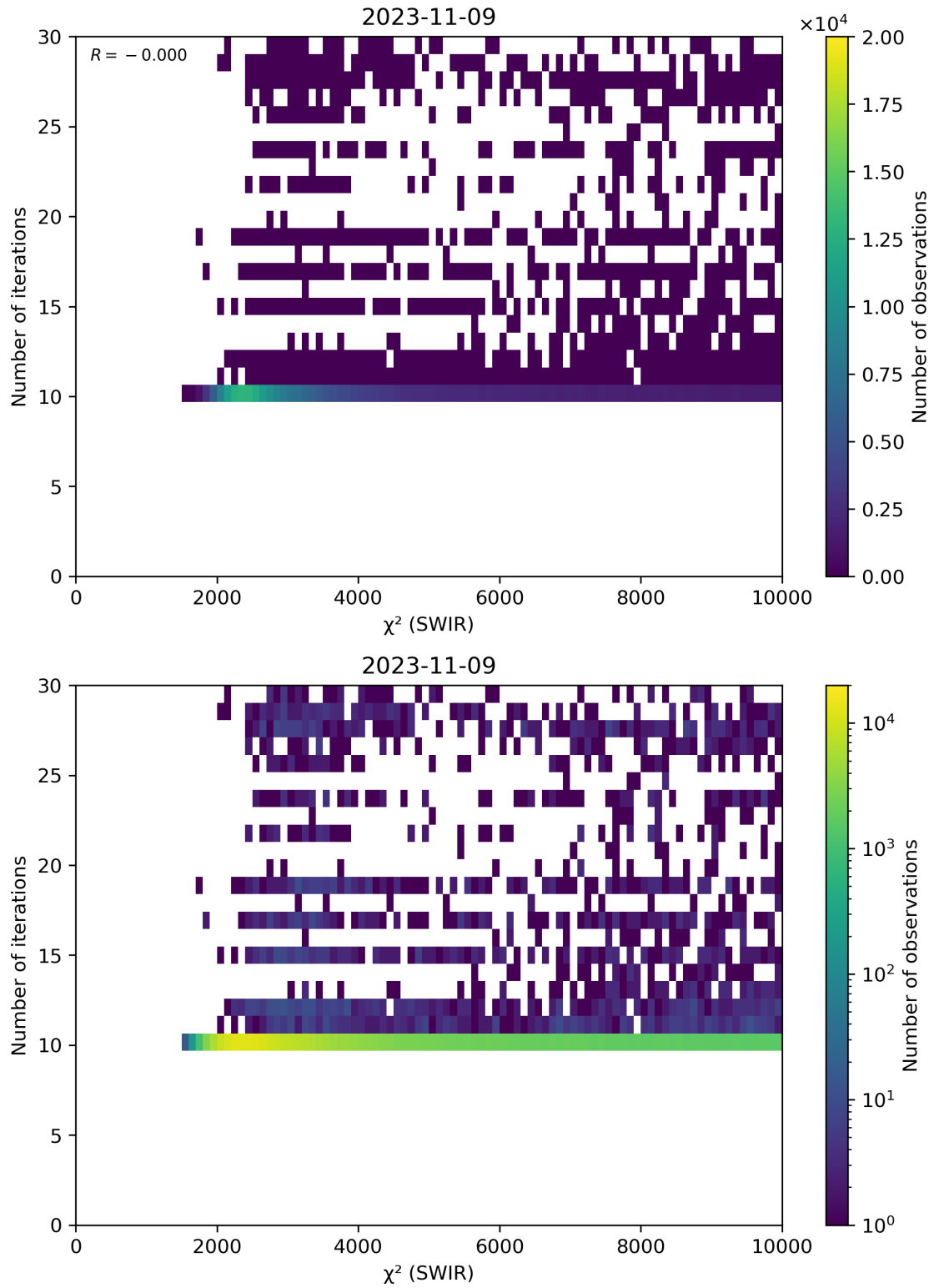
Figure 50: Scatter density plot of “ \chi^2 (SWIR)” against “Number of iterations” for 2023-11-08 to 2023-11-10.
