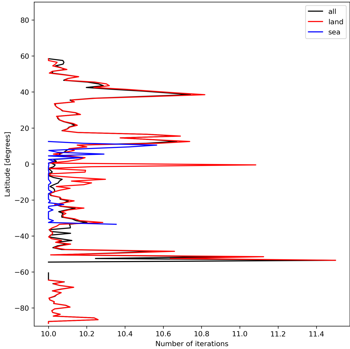
Figure 20: Zonal average of “Number of iterations” for 2023-11-08 to 2023-11-10.
