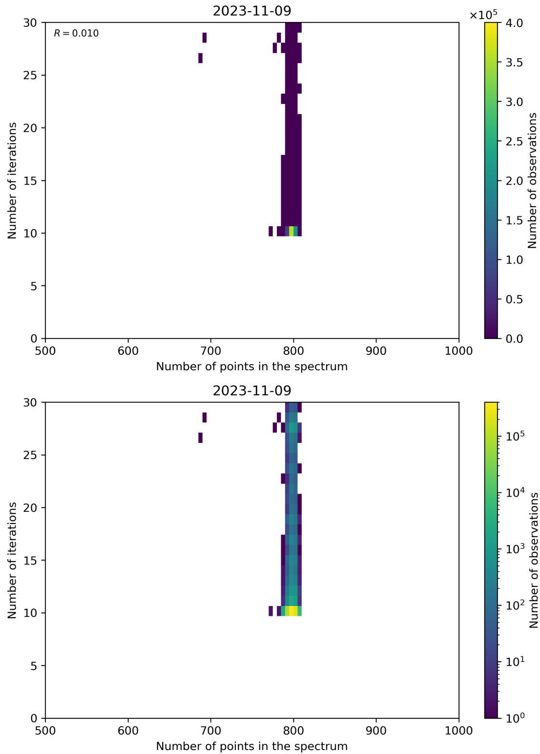
Figure 92: Scatter density plot of “Number of points in the spectrum” against “Number of iterations” for 2023-11-08 to 2023-11-10.
