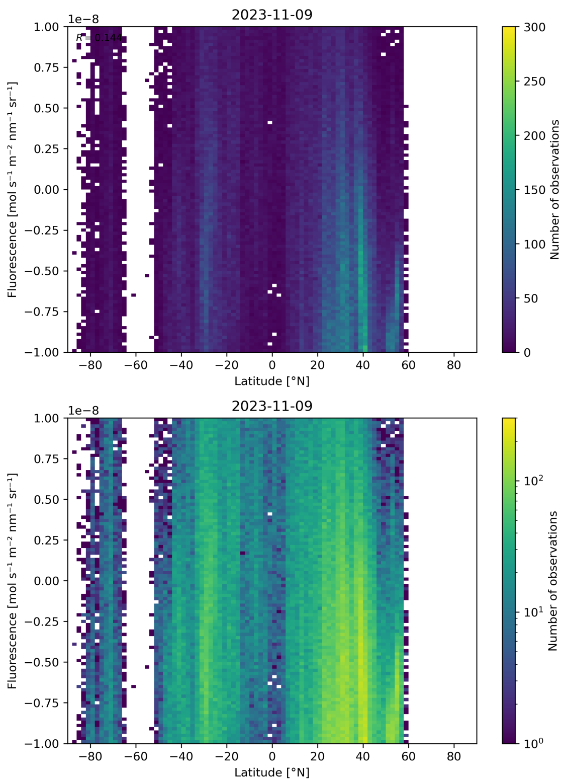
Figure 56: Scatter density plot of “Latitude” against “Fluorescence” for 2023-11-08 to 2023-11-10.
