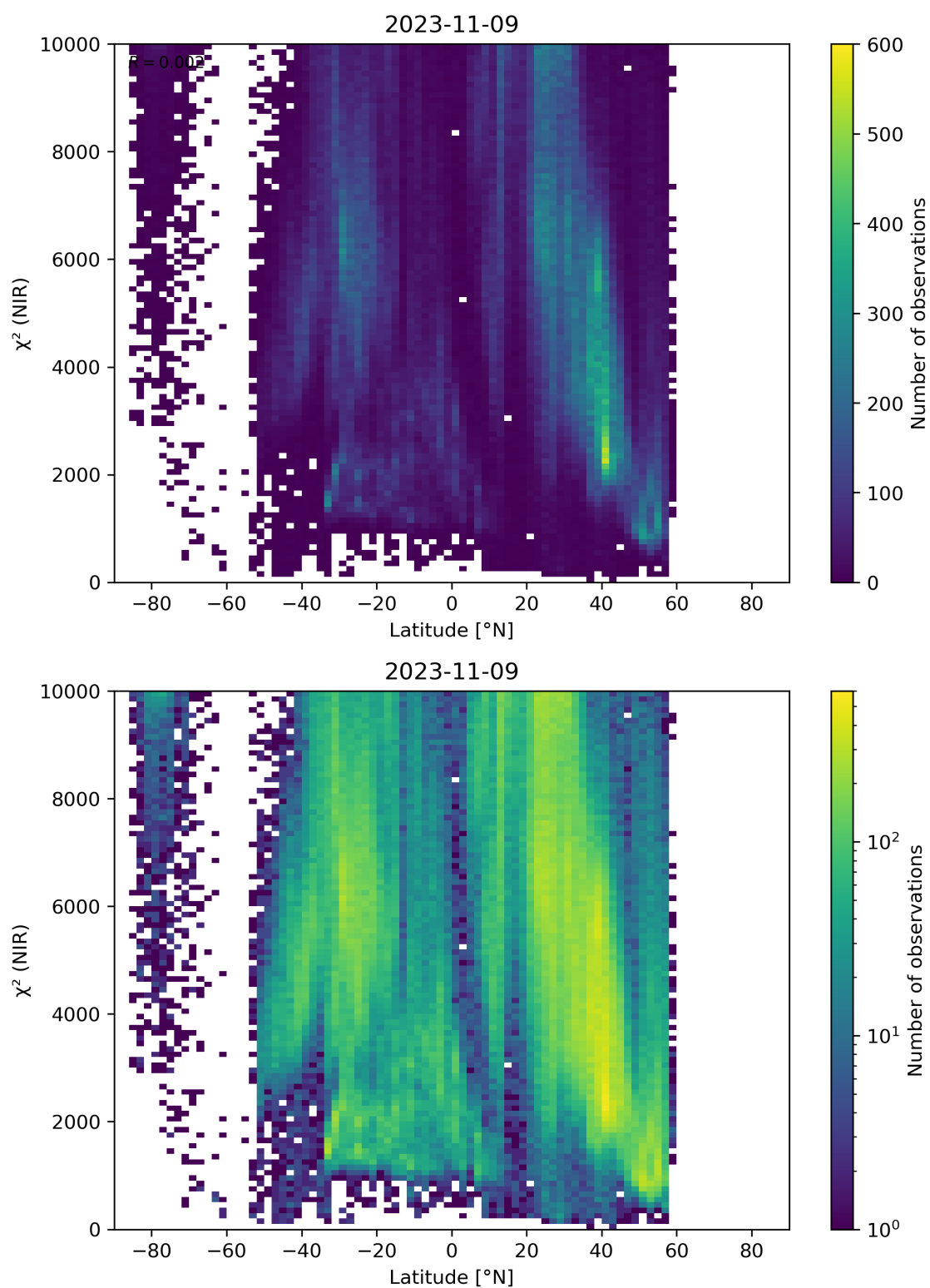
Figure 53: Scatter density plot of “Latitude” against “ \chi^2 (NIR)” for 2023-11-08 to 2023-11-10.
