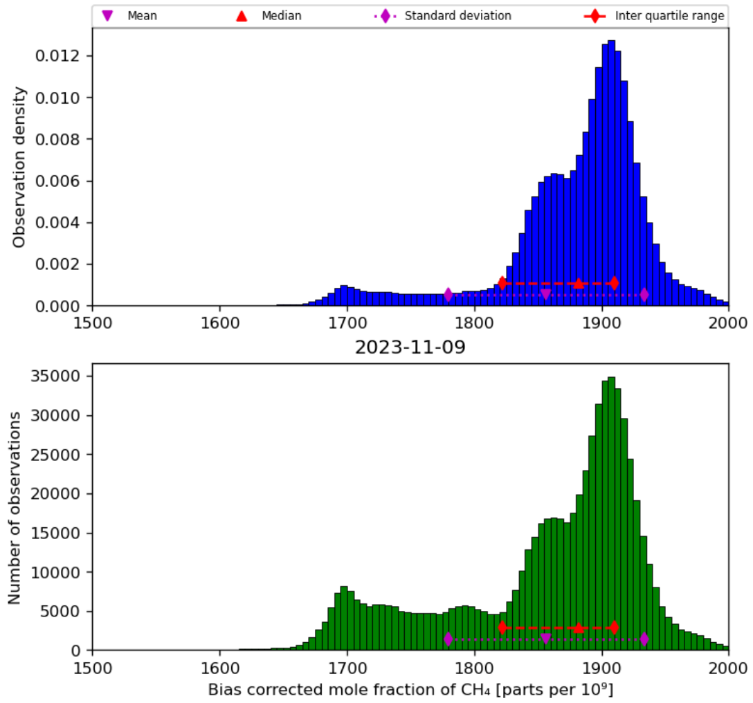
Figure 25: Histogram of “Bias corrected mole fraction of CH 4 ” for 2023-11-08 to 2023-11-10
