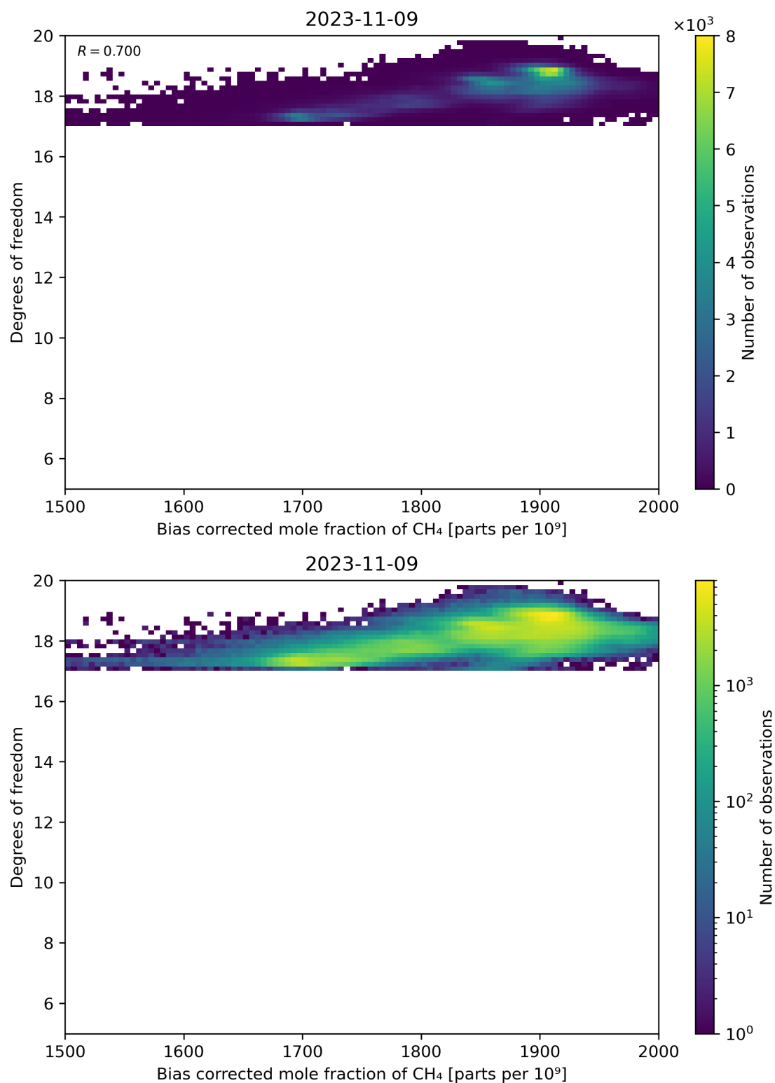
Figure 65: Scatter density plot of “Bias corrected mole fraction of CH 4 ” against “Degrees of freedom” for 2023-11-08 to 2023-11-10.
