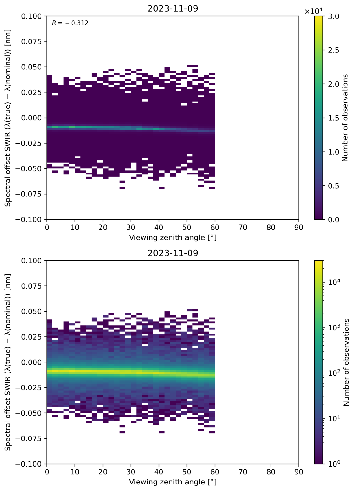
Figure 116: Scatter density plot of “Viewing zenith angle” against “Spectral offset SWIR ( \lambda(\text{true}) - \lambda(\text{nominal}) )” for 2023-11-08 to 2023-11-10.
