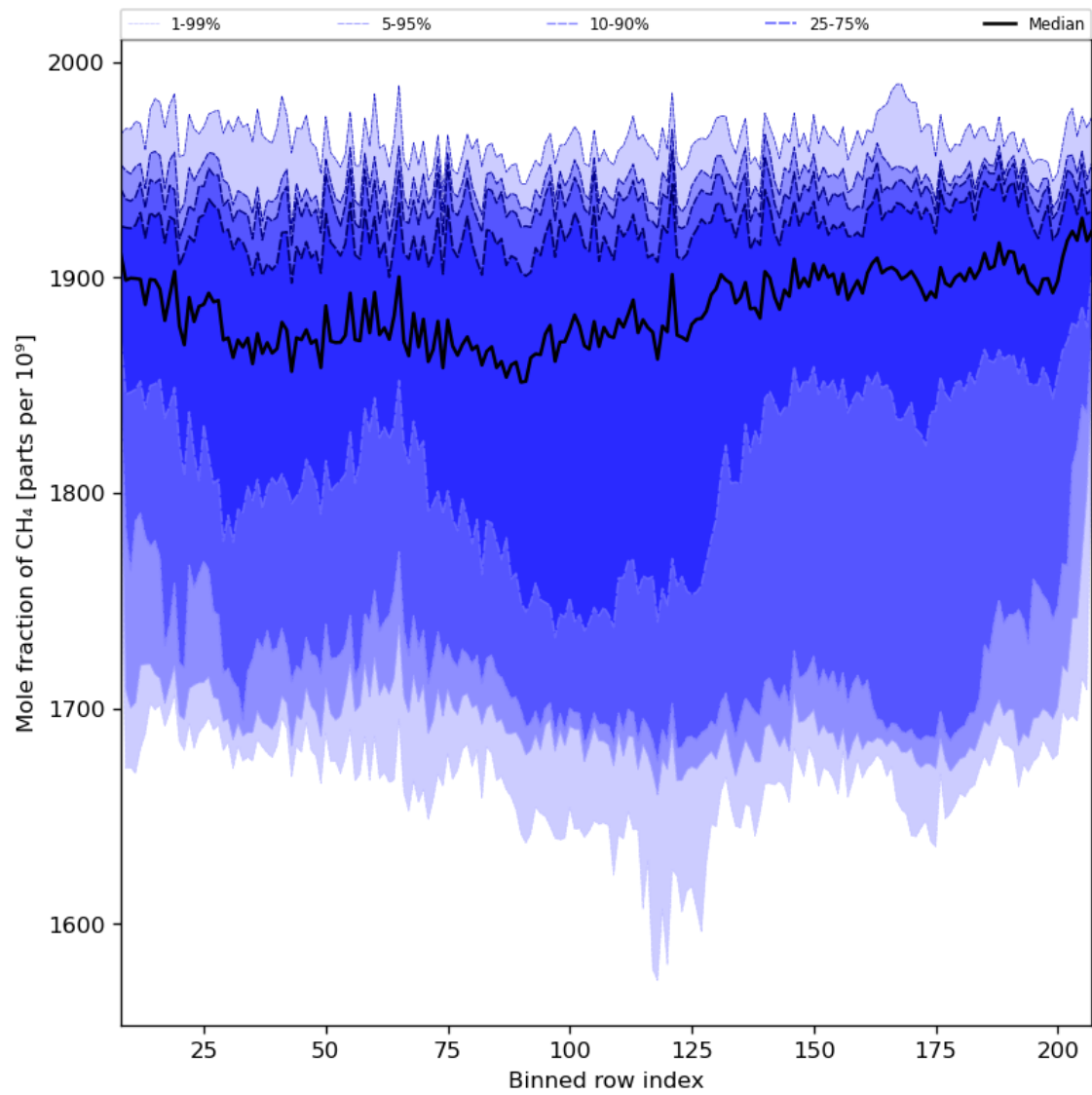
Figure 34: Along track statistics of “Mole fraction of CH 4 ” for 2023-11-08 to 2023-11-10
