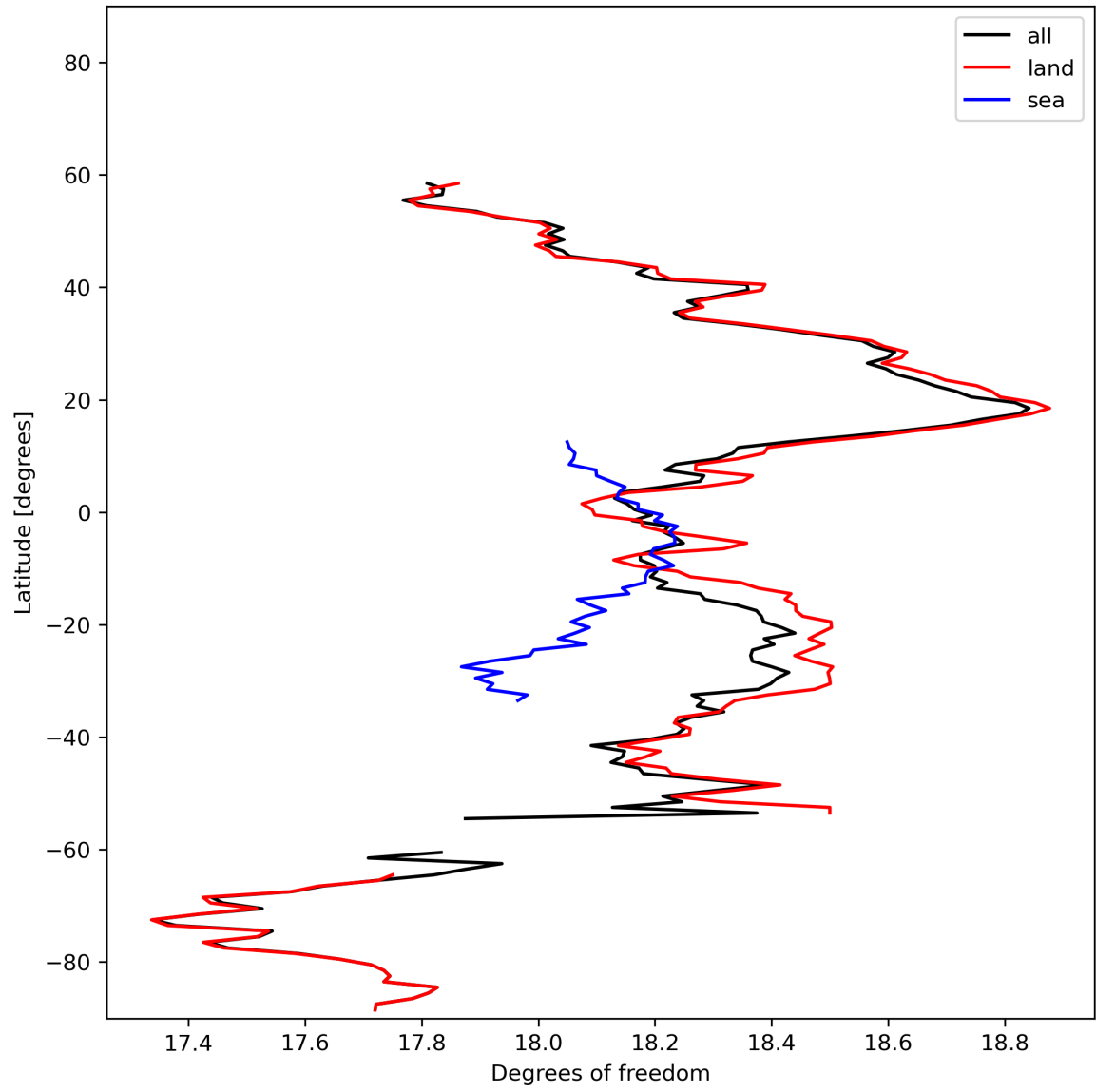
Figure 19: Zonal average of “Degrees of freedom” for 2023-11-08 to 2023-11-10.
