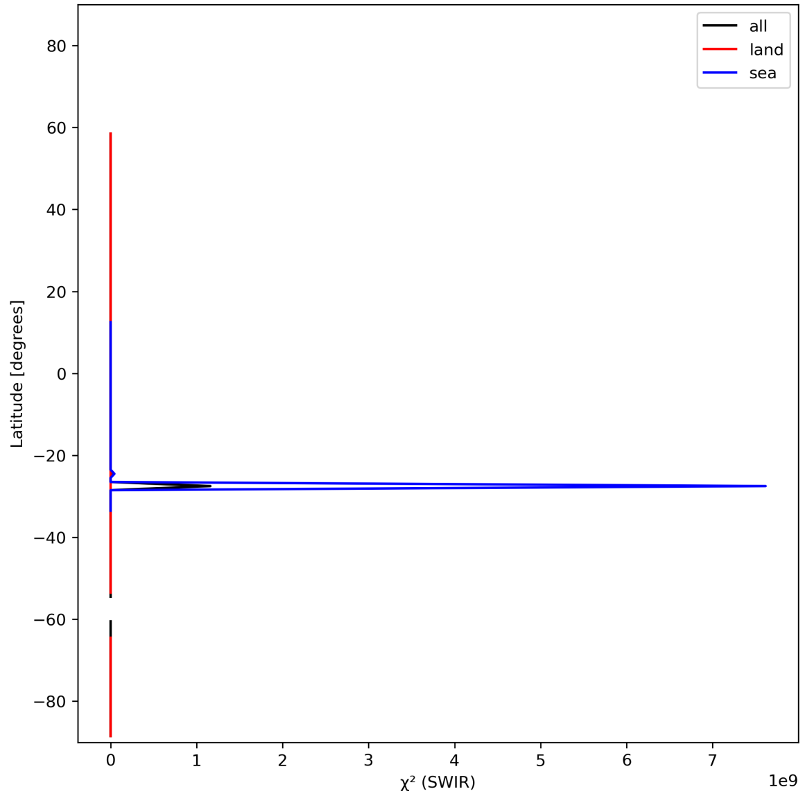
Figure 17: Zonal average of “ \chi^2 (SWIR)” for 2023-11-08 to 2023-11-10.
