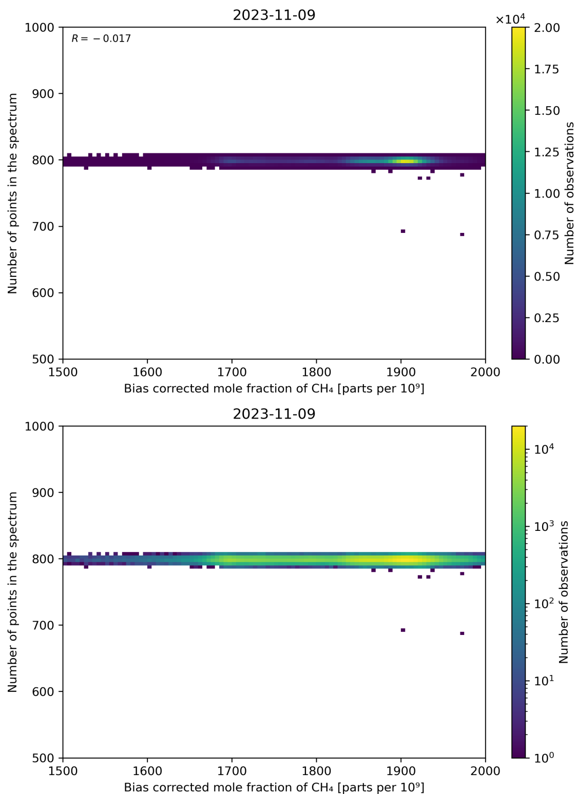
Figure 68: Scatter density plot of “Bias corrected mole fraction of \text{CH}_4 ” against “Number of points in the spectrum” for 2023-11-08 to 2023-11-10.
