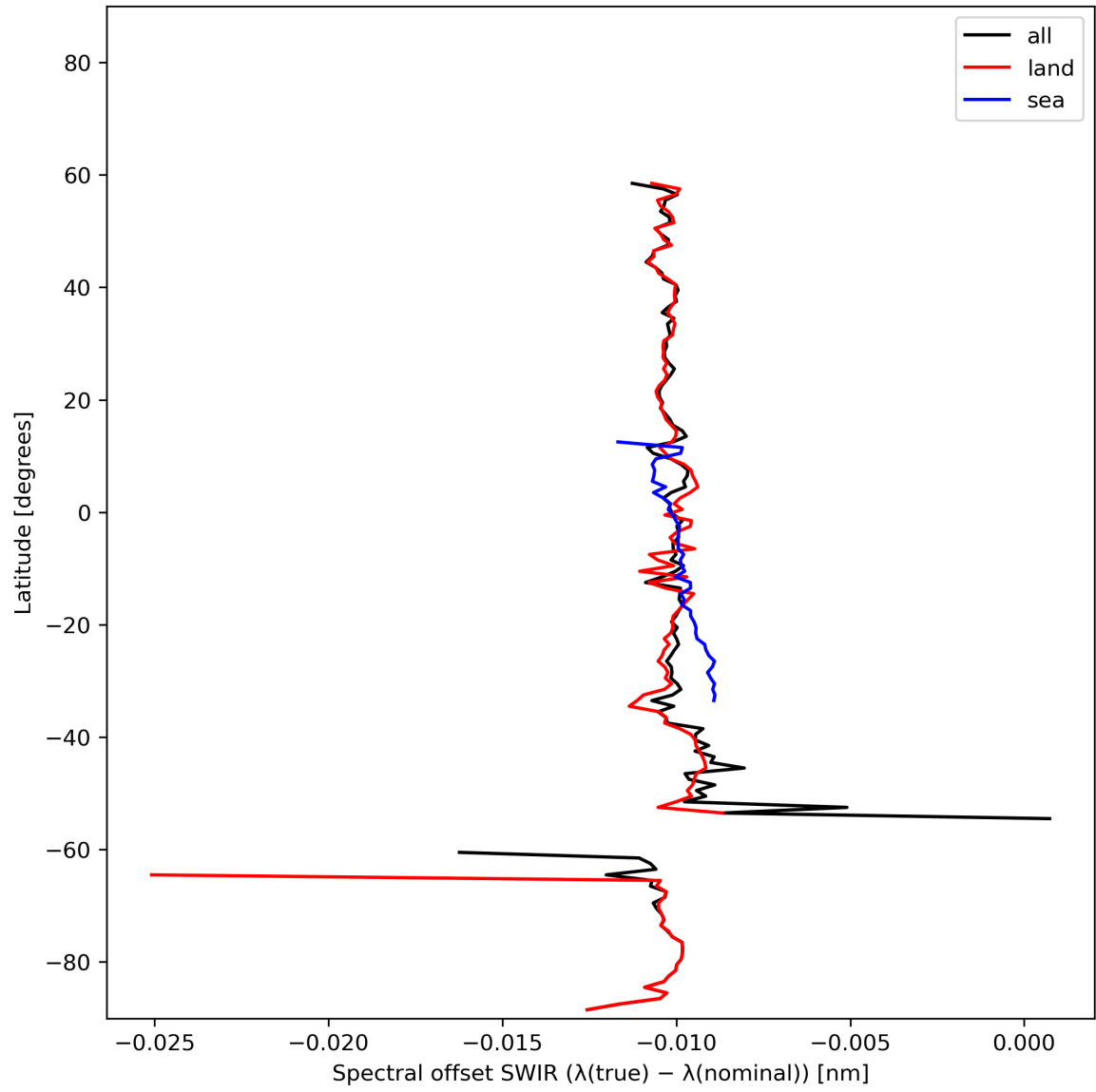
Figure 16: Zonal average of “Spectral offset SWIR ( \lambda(\text{true}) - \lambda(\text{nominal}) )” for 2023-11-08 to 2023-11-10.
