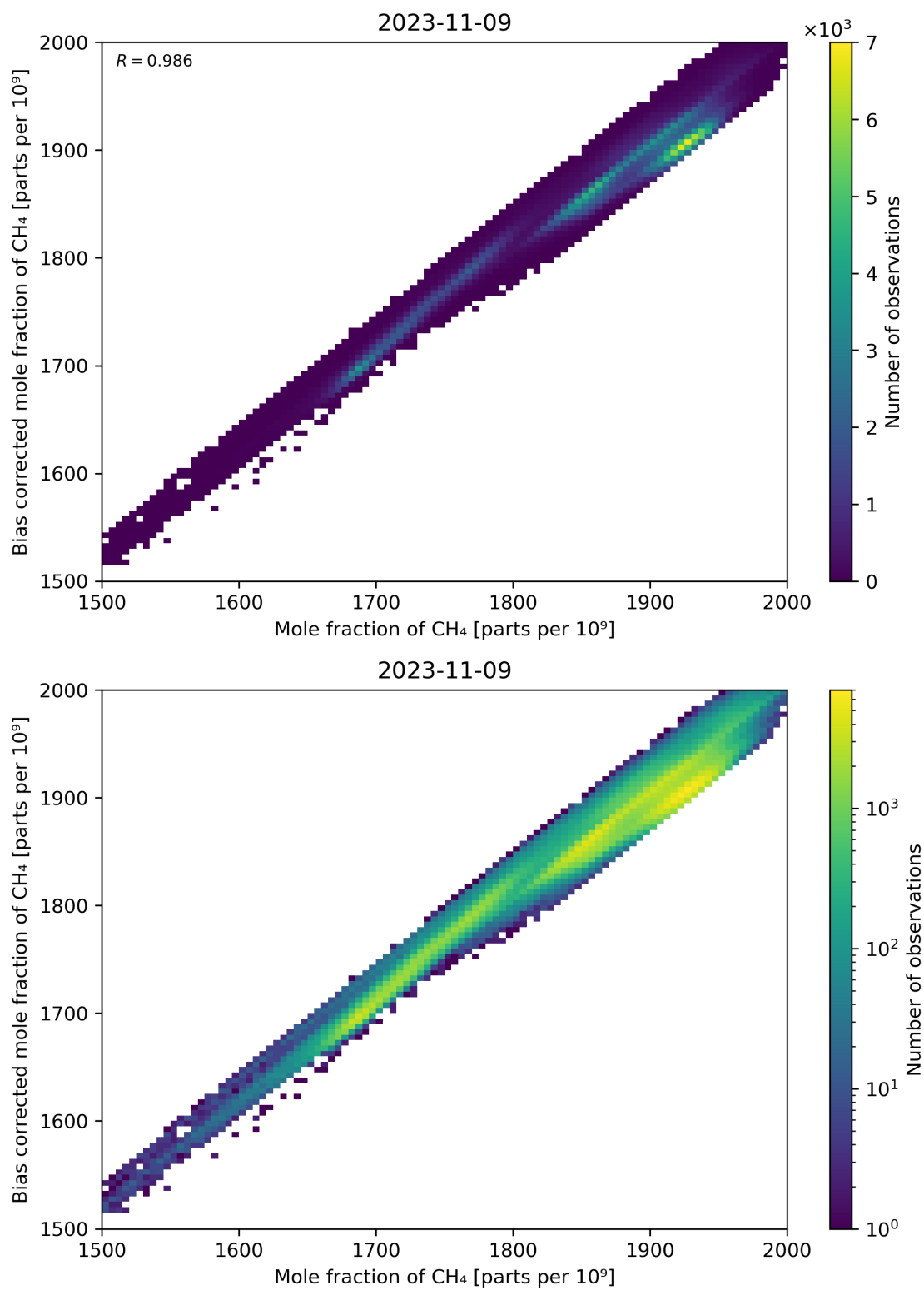
Figure 74: Scatter density plot of “Mole fraction of CH 4 ” against “Bias corrected mole fraction of CH 4 ” for 2023-11-08 to 2023-11-10.
