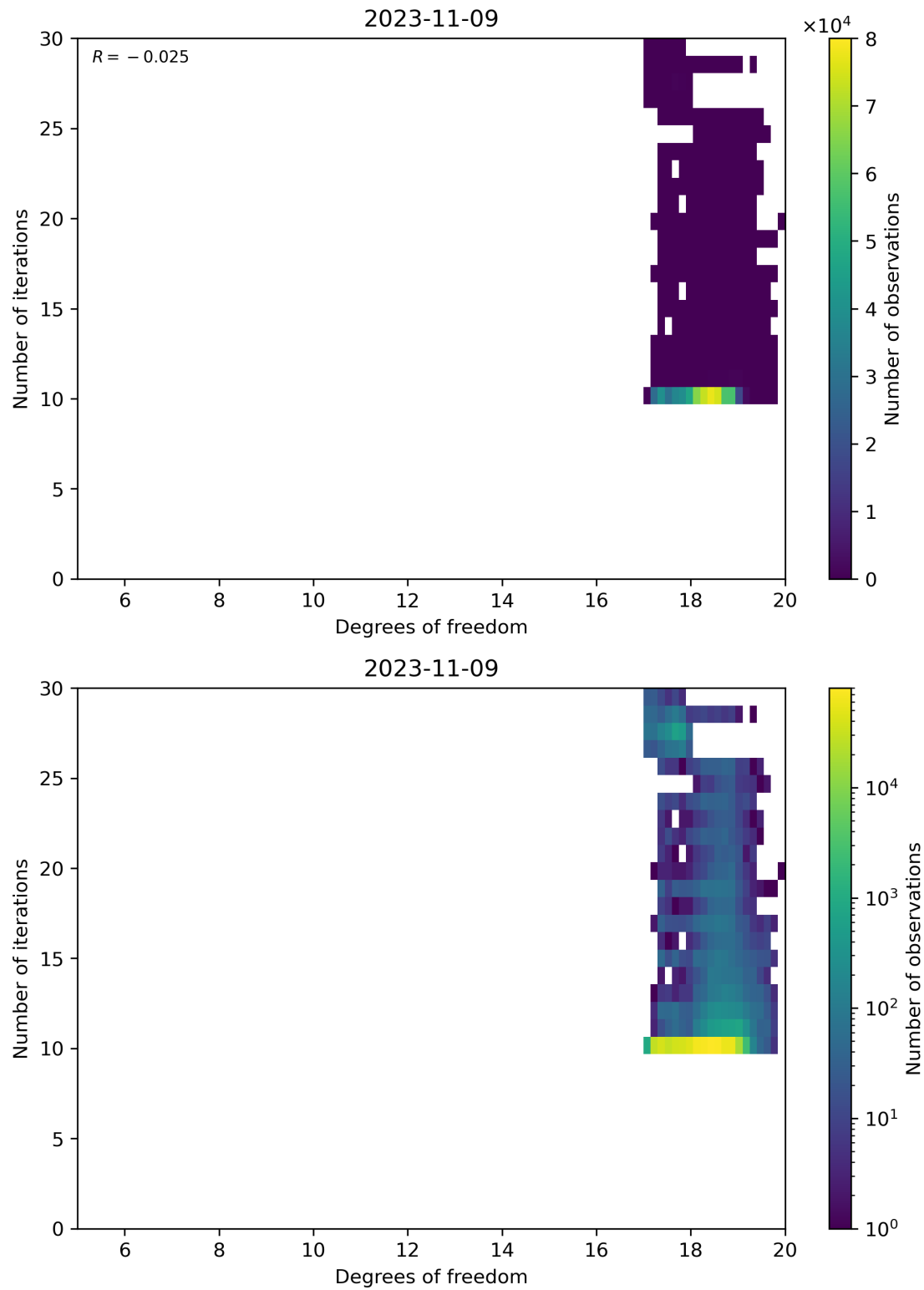
Figure 52: Scatter density plot of “Degrees of freedom” against “Number of iterations” for 2023-11-08 to 2023-11-10.
