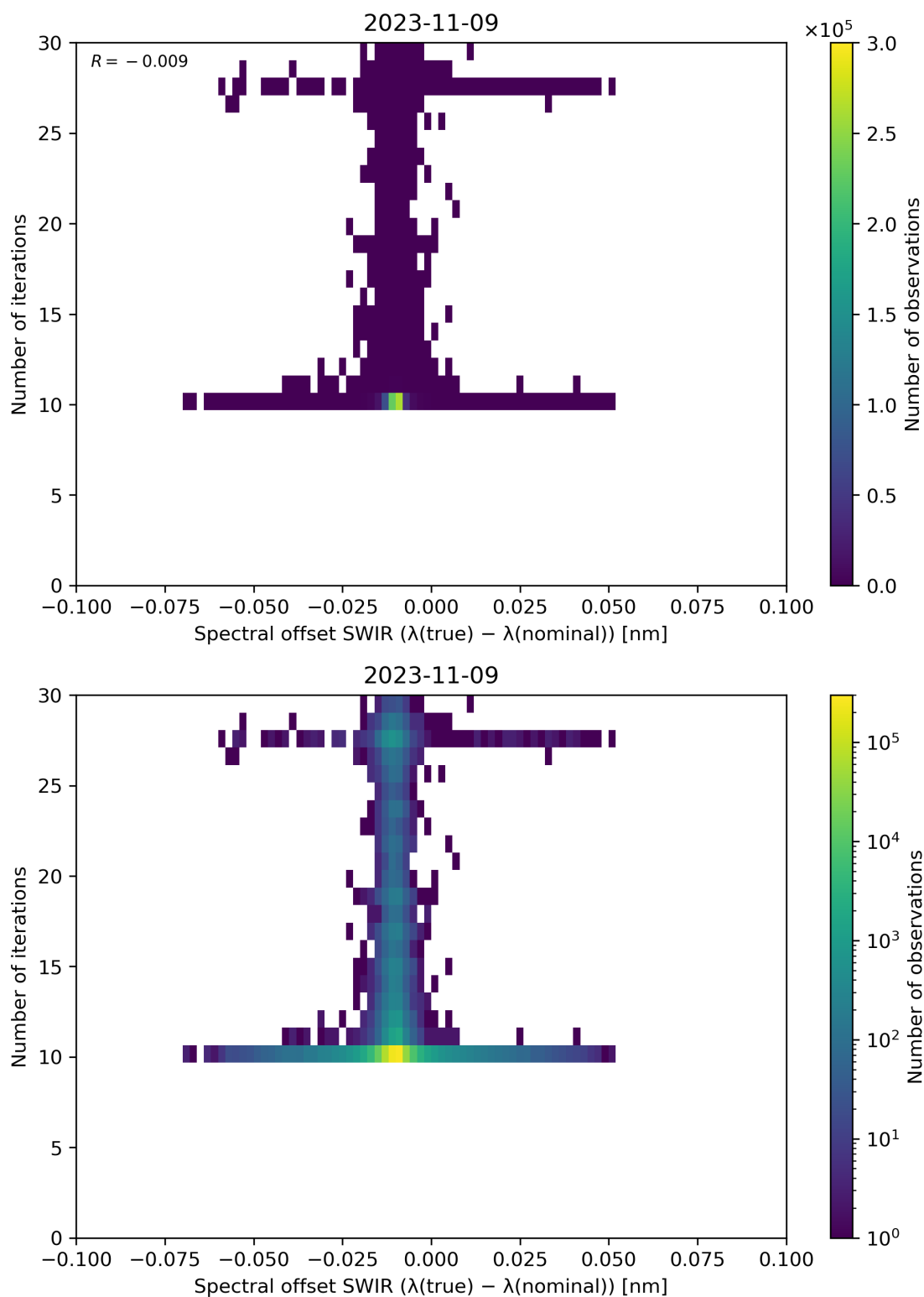
Figure 121: Scatter density plot of “Spectral offset SWIR ( \lambda(\text{true}) - \lambda(\text{nominal}) )” against “Number of iterations” for 2023-11-08 to 2023-11-10.
