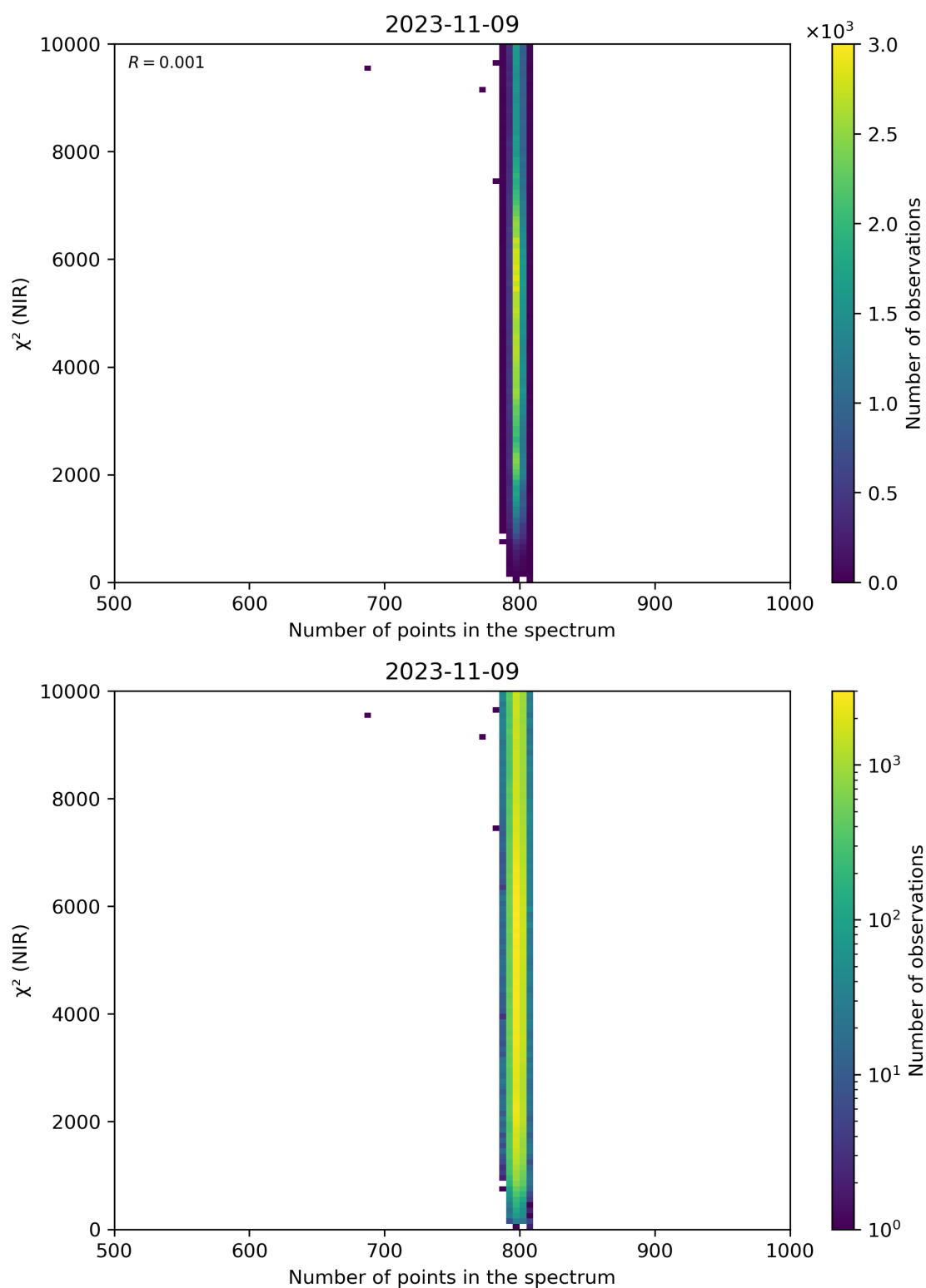
Figure 88: Scatter density plot of “Number of points in the spectrum” against “ \chi^2 (NIR)” for 2023-11-08 to 2023-11-10.
