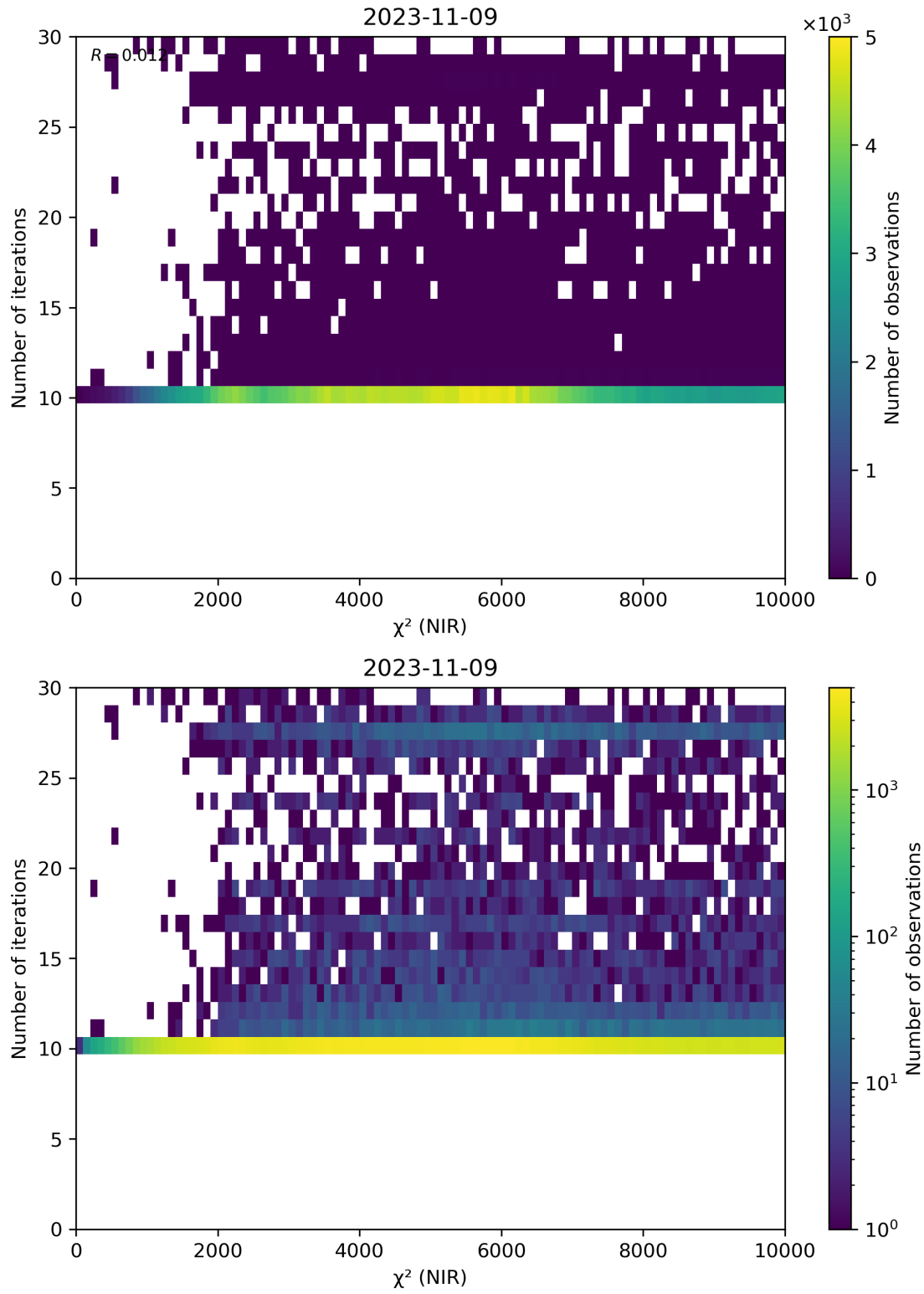
Figure 46: Scatter density plot of “ \chi^2 (NIR)” against “Number of iterations” for 2023-11-08 to 2023-11-10.
