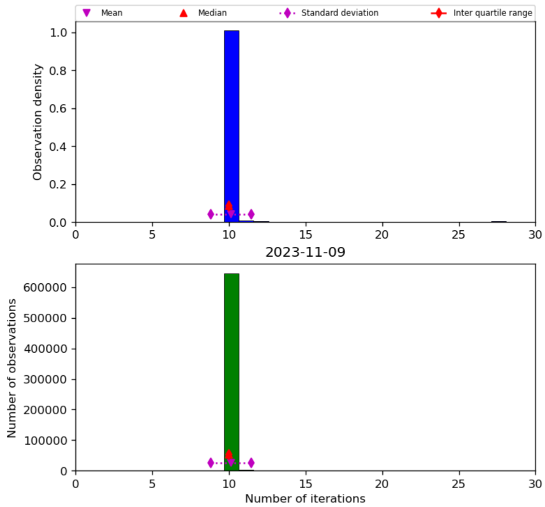
Figure 31: Histogram of “Number of iterations” for 2023-11-08 to 2023-11-10
