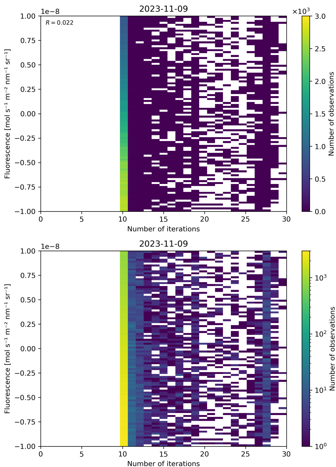
Figure 87: Scatter density plot of “Number of iterations” against “Fluorescence” for 2023-11-08 to 2023-11-10.
