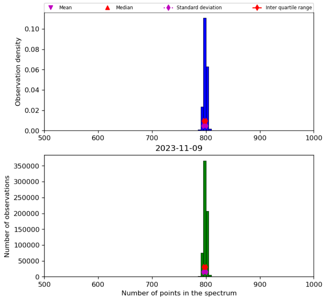
Figure 26: Histogram of “Number of points in the spectrum” for 2023-11-08 to 2023-11-10
