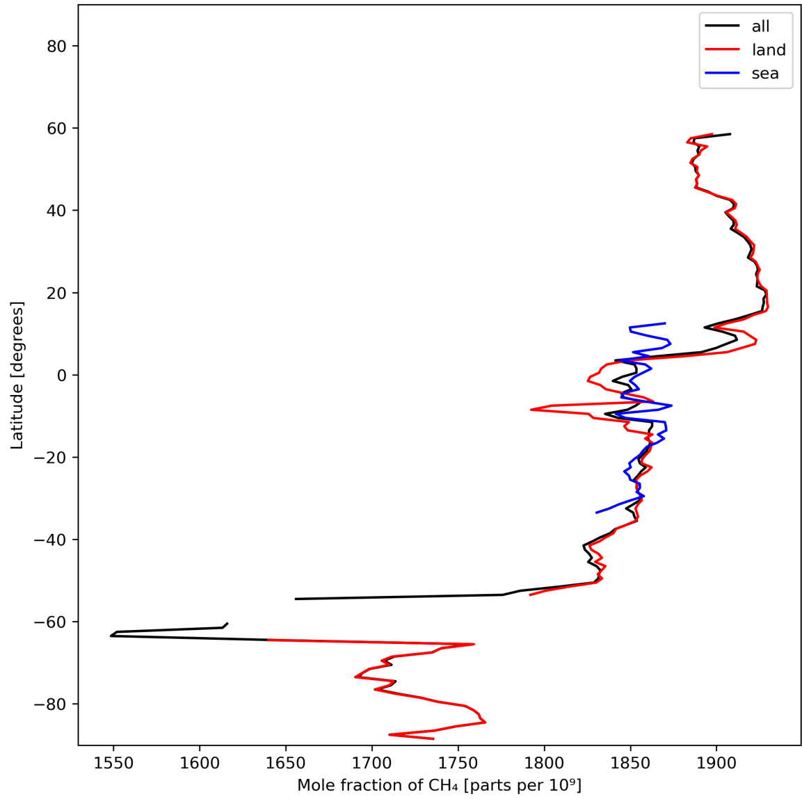
Figure 12: Zonal average of “Mole fraction of CH 4 ” for 2023-11-08 to 2023-11-10.
