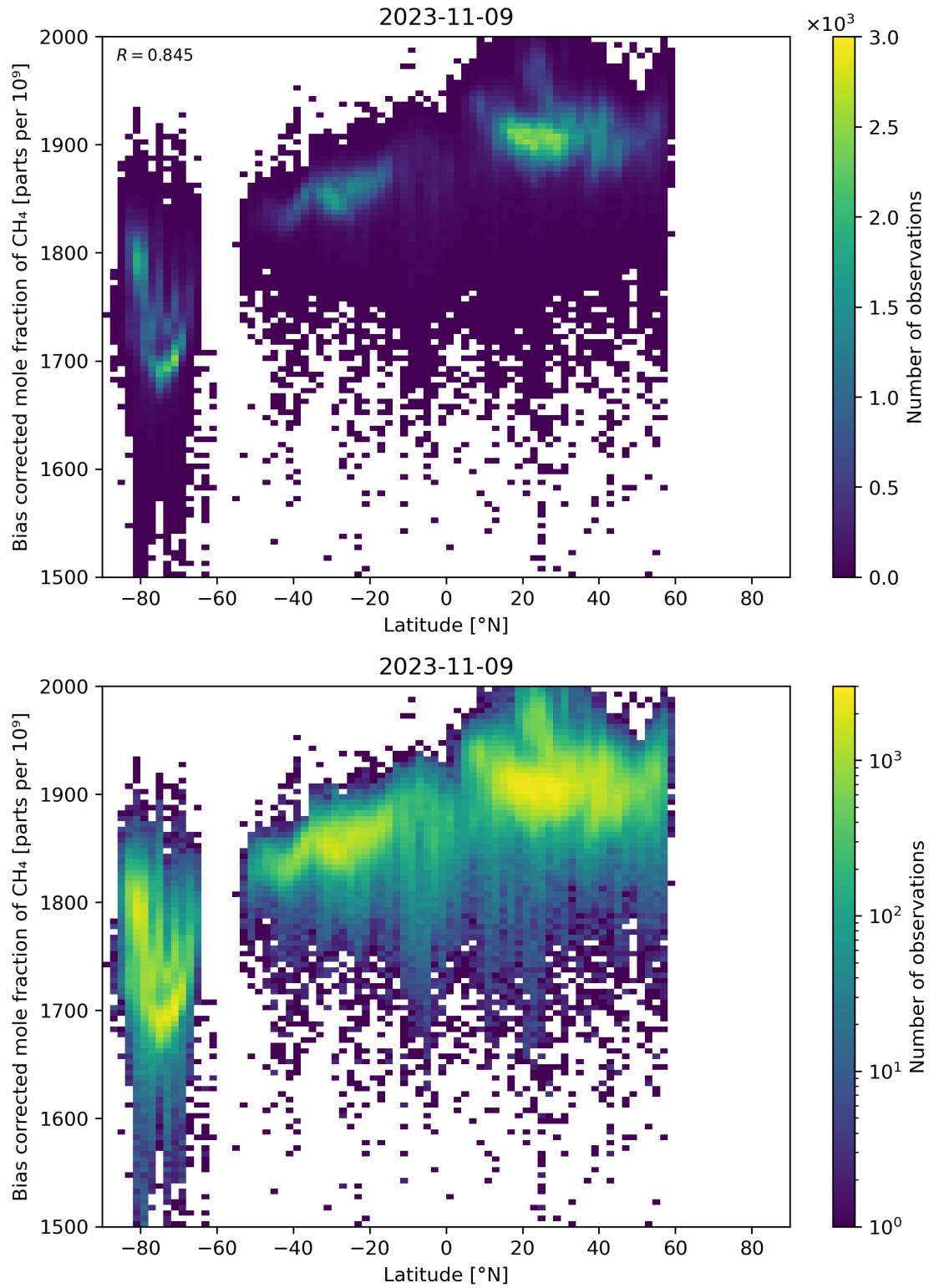
Figure 58: Scatter density plot of “Latitude” against “Bias corrected mole fraction of \text{CH}_4 ” for 2023-11-08 to 2023-11-10.
