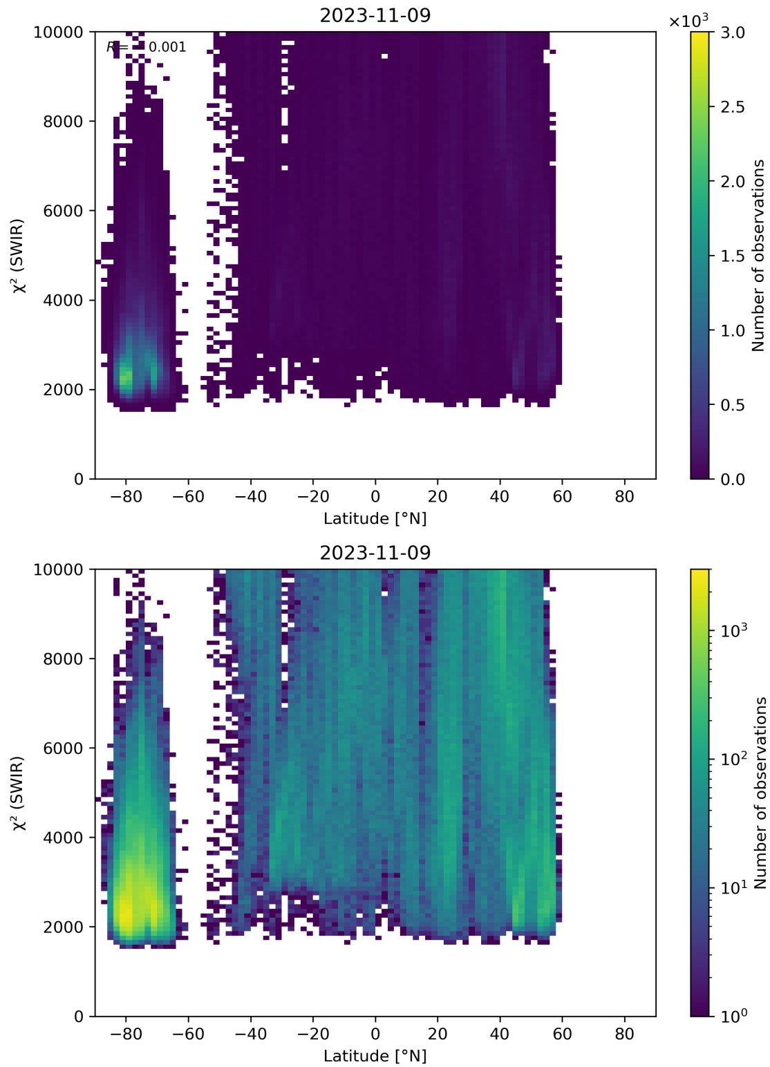
Figure 54: Scatter density plot of “Latitude” against “ \chi^2 (SWIR)” for 2023-11-08 to 2023-11-10.
