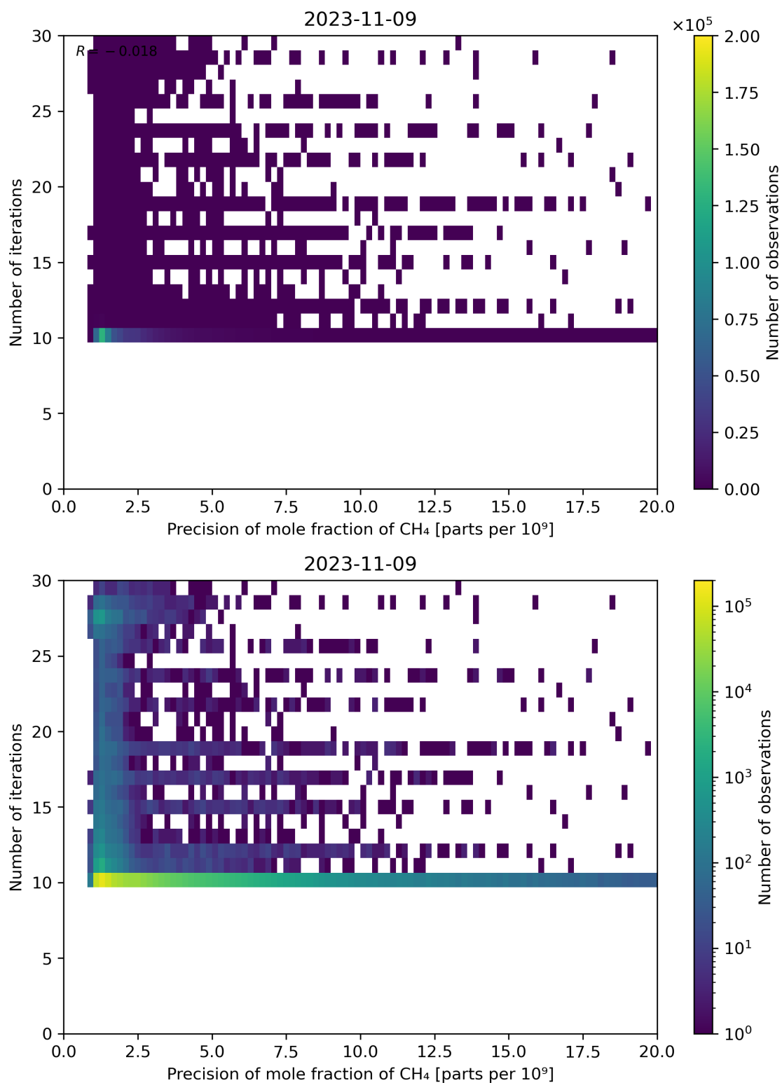
Figure 83: Scatter density plot of “Precision of mole fraction of CH 4 ” against “Number of iterations” for 2023-11-08 to 2023-11-10.
