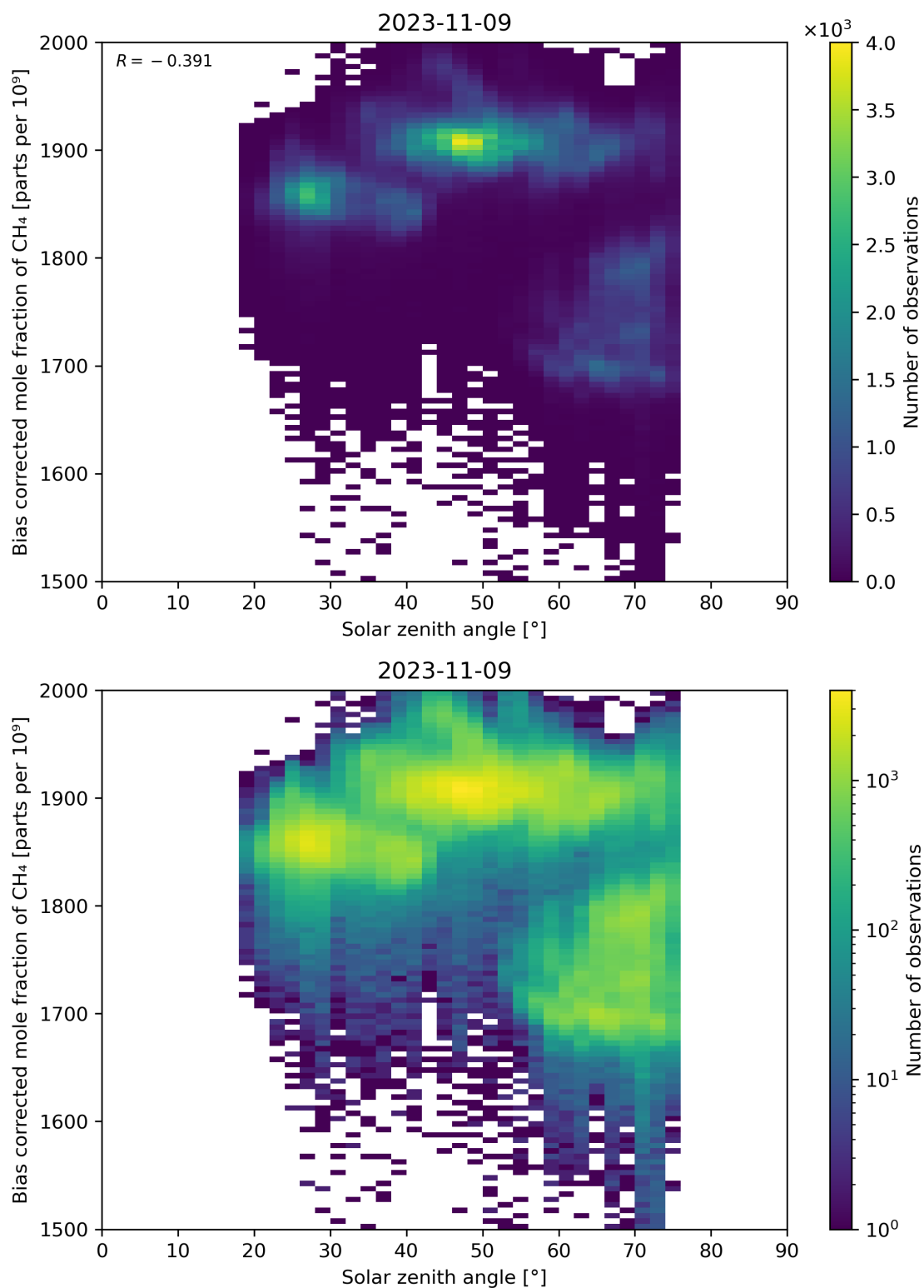
Figure 100: Scatter density plot of “Solar zenith angle” against “Bias corrected mole fraction of CH 4 ” for 2023-11-08 to 2023-11-10.
