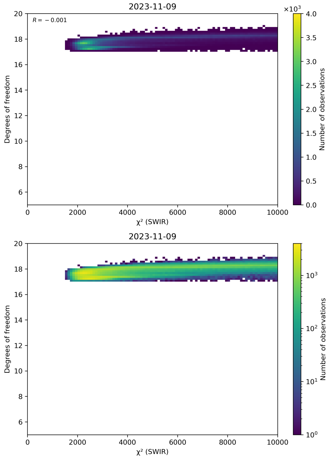
Figure 48: Scatter density plot of “ \chi^2 (SWIR)” against “Degrees of freedom” for 2023-11-08 to 2023-11-10.
