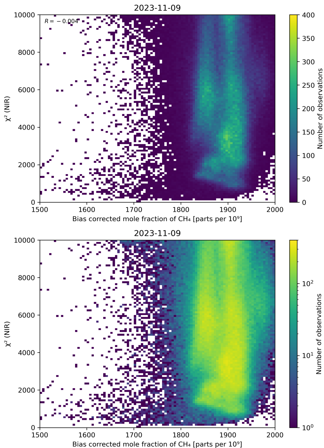
Figure 63: Scatter density plot of “Bias corrected mole fraction of CH 4 ” against “ \chi^2 (NIR)” for 2023-11-08 to 2023-11-10.
