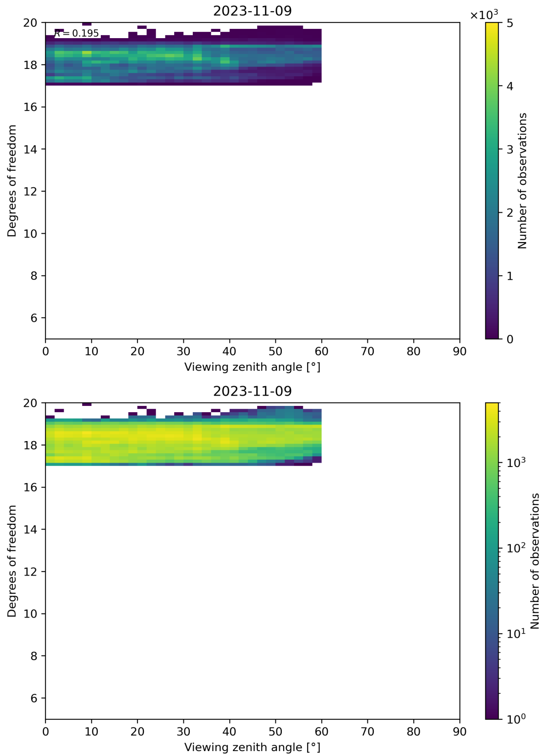
Figure 107: Scatter density plot of “Viewing zenith angle” against “Degrees of freedom” for 2023-11-08 to 2023-11-10.
