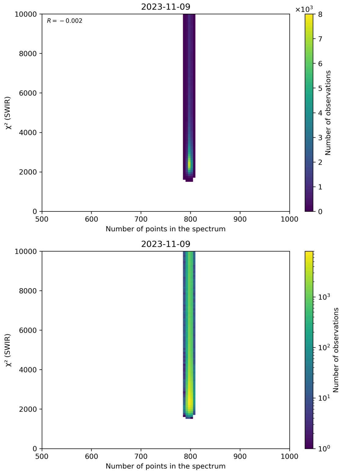
Figure 89: Scatter density plot of “Number of points in the spectrum” against “ \chi^2 (SWIR)” for 2023-11-08 to 2023-11-10.
