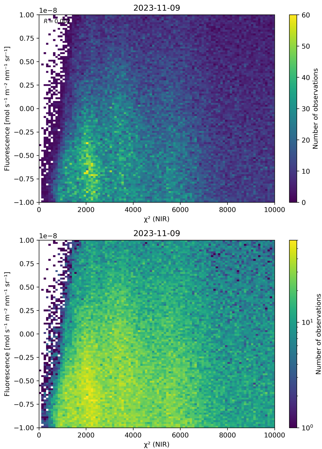
Figure 45: Scatter density plot of “ \chi^2 (NIR)” against “Fluorescence” for 2023-11-08 to 2023-11-10.
