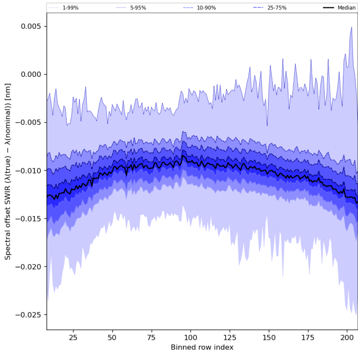
Figure 38: Along track statistics of “Spectral offset SWIR ( \lambda(\text{true}) - \lambda(\text{nominal}) )” for 2023-11-08 to 2023-11-10
