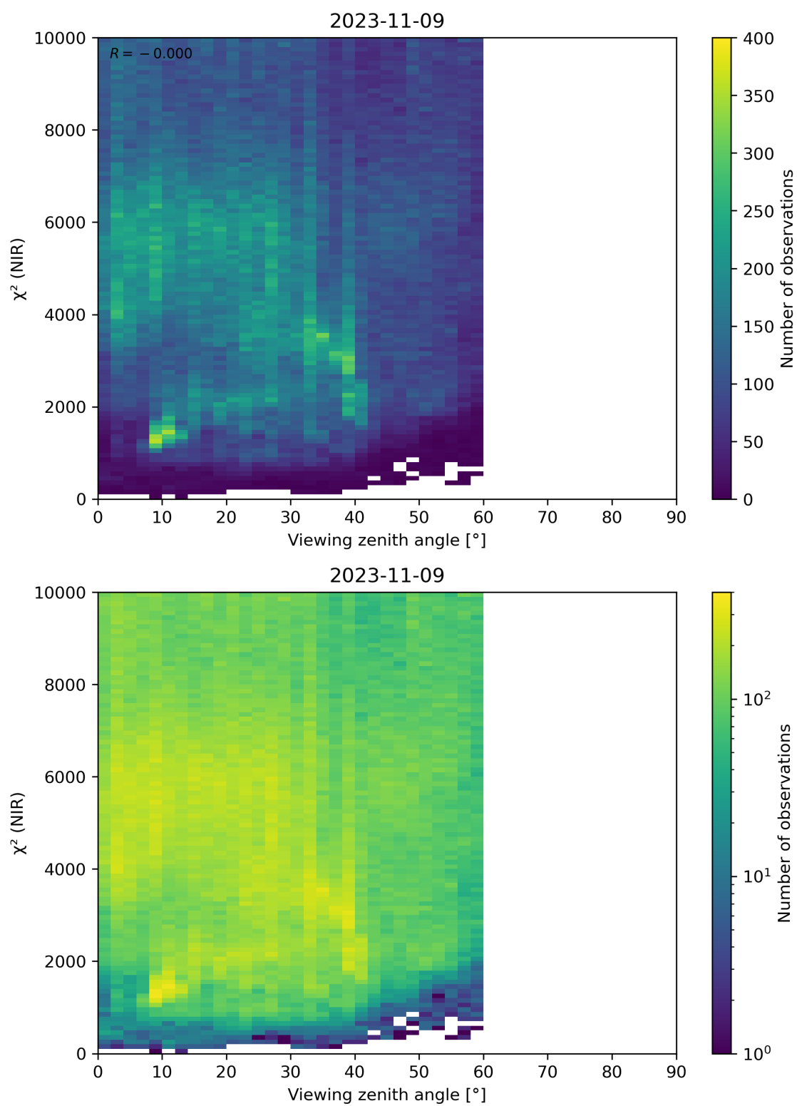
Figure 105: Scatter density plot of “Viewing zenith angle” against “ \chi^2 (NIR)” for 2023-11-08 to 2023-11-10.
