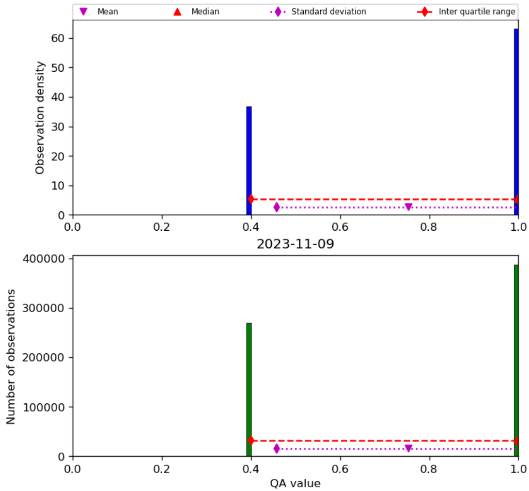
Figure 22: Histogram of “QA value” for 2023-11-08 to 2023-11-10
