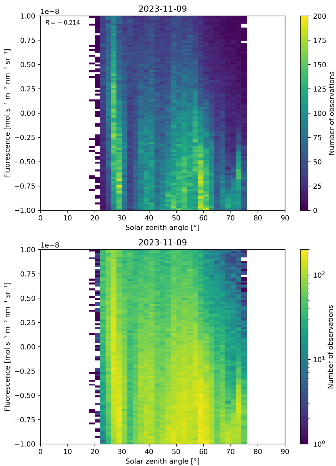
Figure 97: Scatter density plot of “Solar zenith angle” against “Fluorescence” for 2023-11-08 to 2023-11-10.
