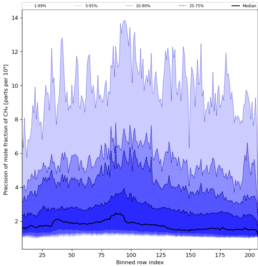
Figure 35: Along track statistics of “Precision of mole fraction of \text{CH}_4 ” for 2023-11-08 to 2023-11-10
