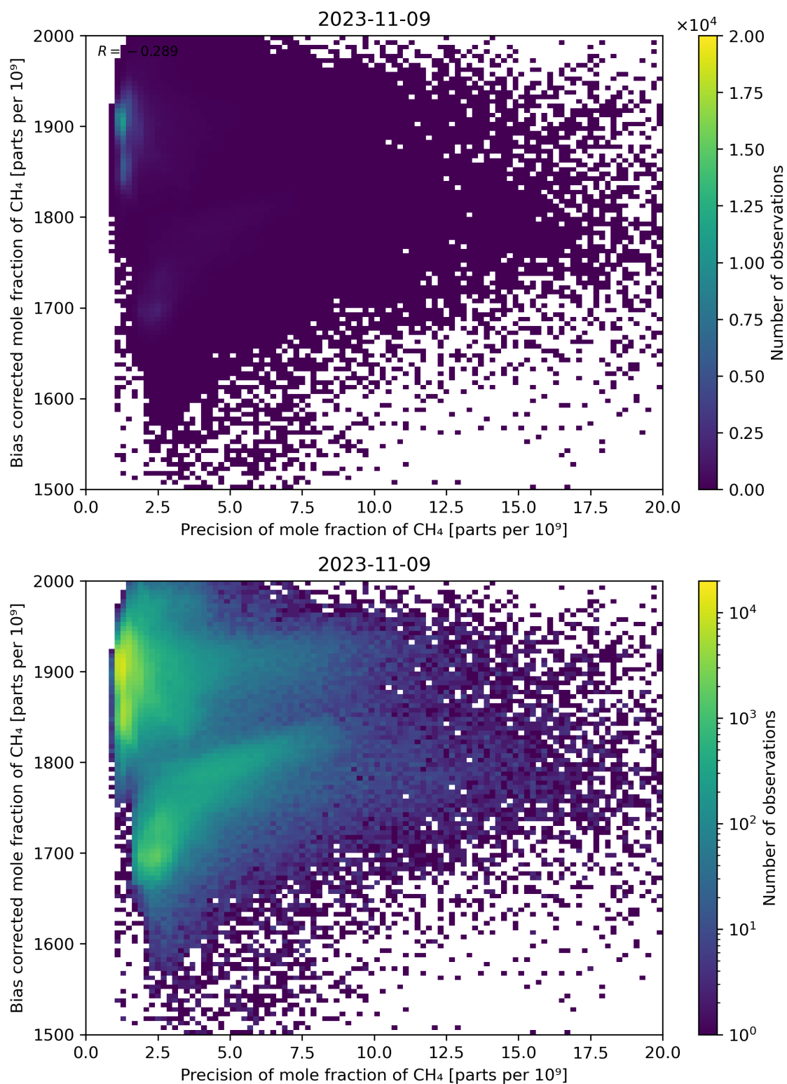
Figure 82: Scatter density plot of “Precision of mole fraction of \text{CH}_4 ” against “Bias corrected mole fraction of \text{CH}_4 ” for 2023-11-08 to 2023-11-10.
