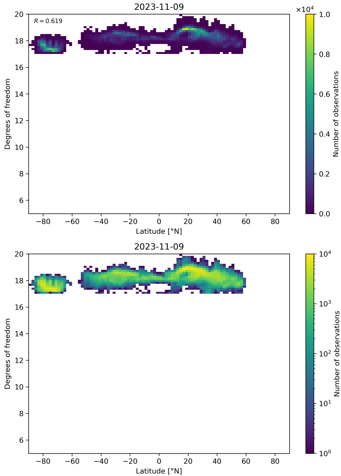
Figure 55: Scatter density plot of “Latitude” against “Degrees of freedom” for 2023-11-08 to 2023-11-10.
