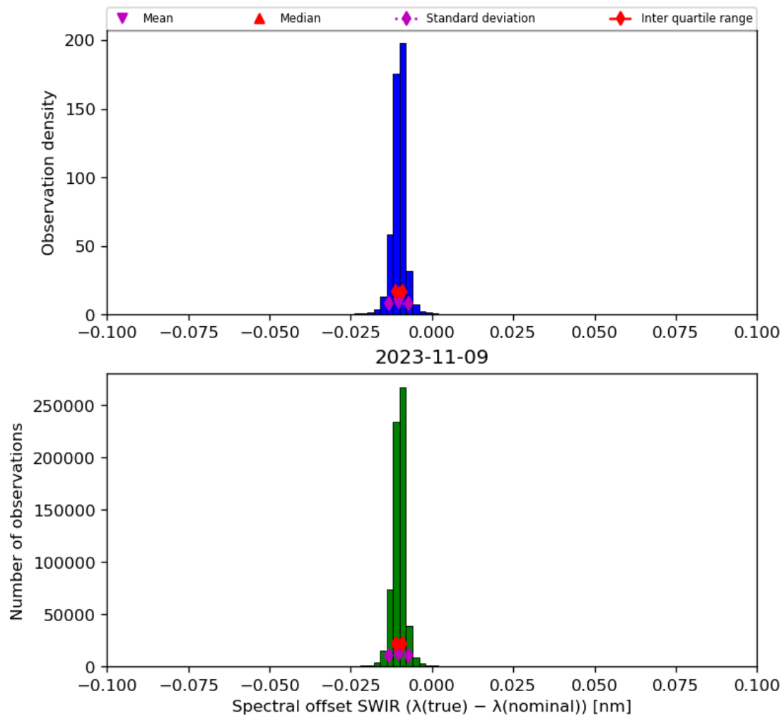
Figure 27: Histogram of “Spectral offset SWIR ( \lambda(\text{true}) - \lambda(\text{nominal}) )” for 2023-11-08 to 2023-11-10
