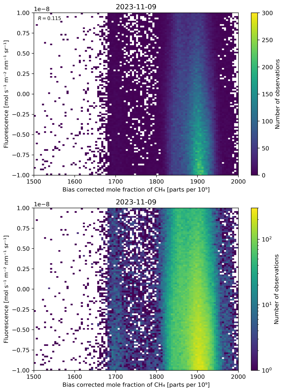
Figure 66: Scatter density plot of “Bias corrected mole fraction of \text{CH}_4 ” against “Fluorescence” for 2023-11-08 to 2023-11-10.
