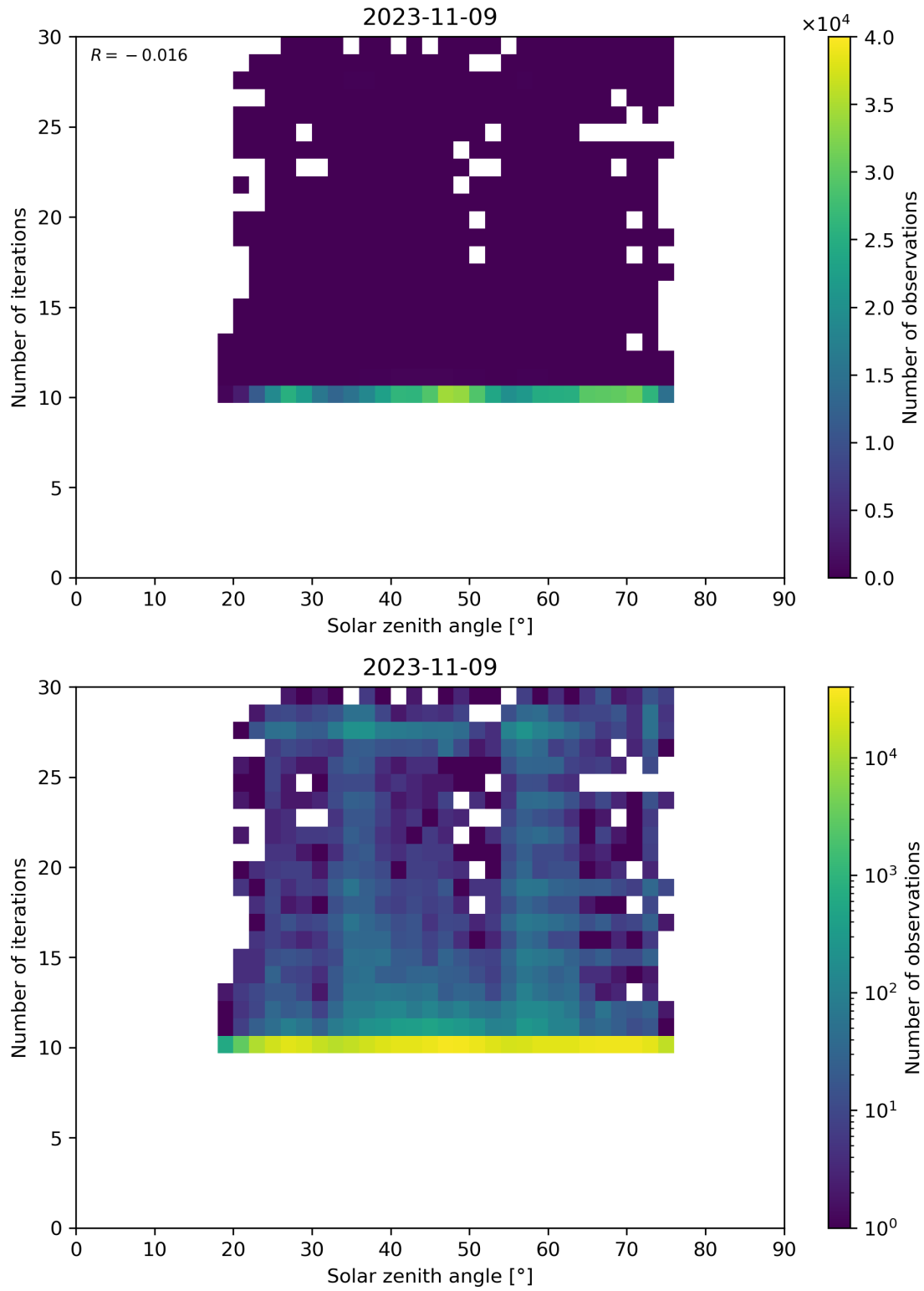
Figure 102: Scatter density plot of “Solar zenith angle” against “Number of iterations” for 2023-11-08 to 2023-11-10.
