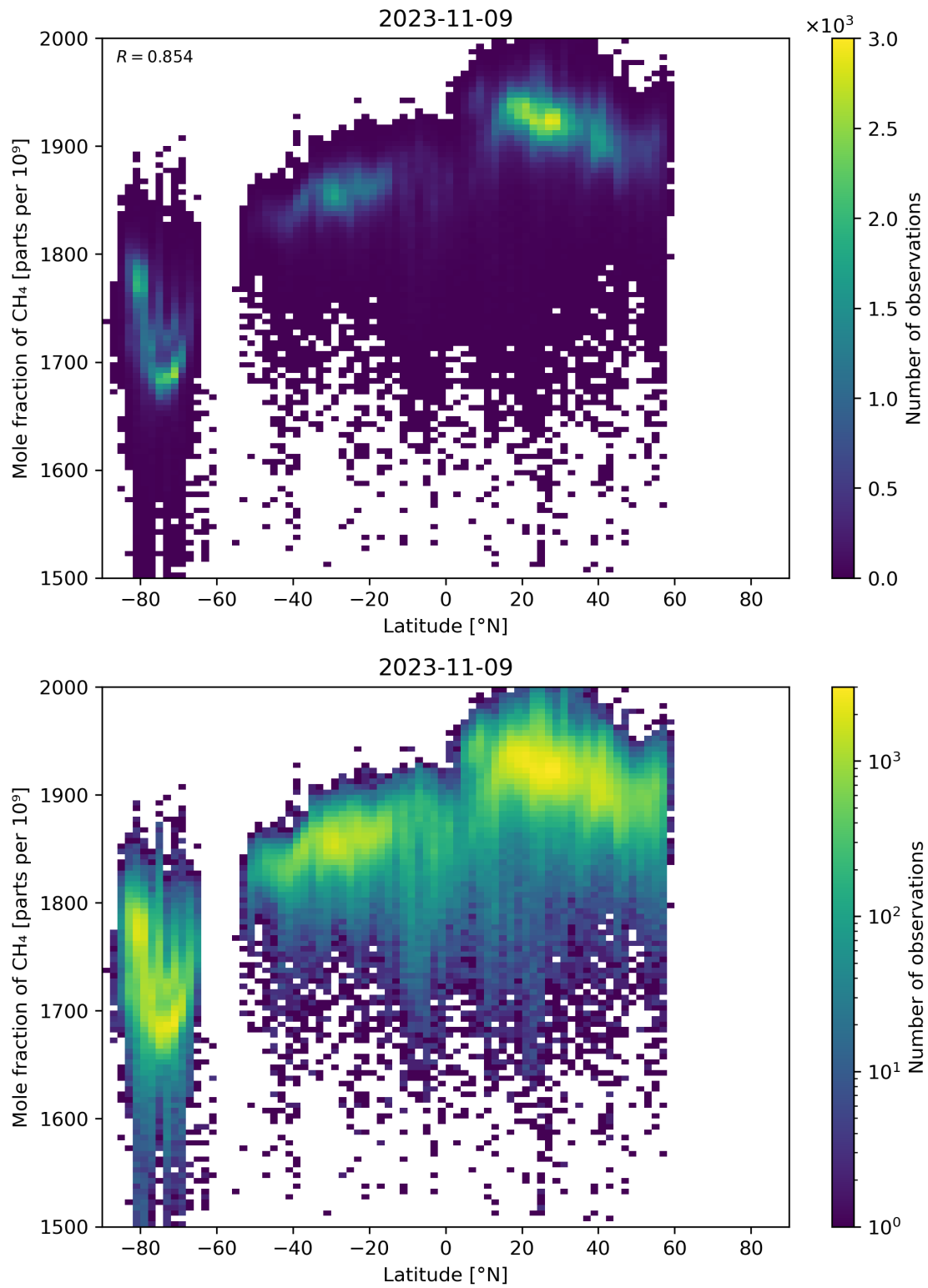
Figure 57: Scatter density plot of “Latitude” against “Mole fraction of CH 4 ” for 2023-11-08 to 2023-11-10.
