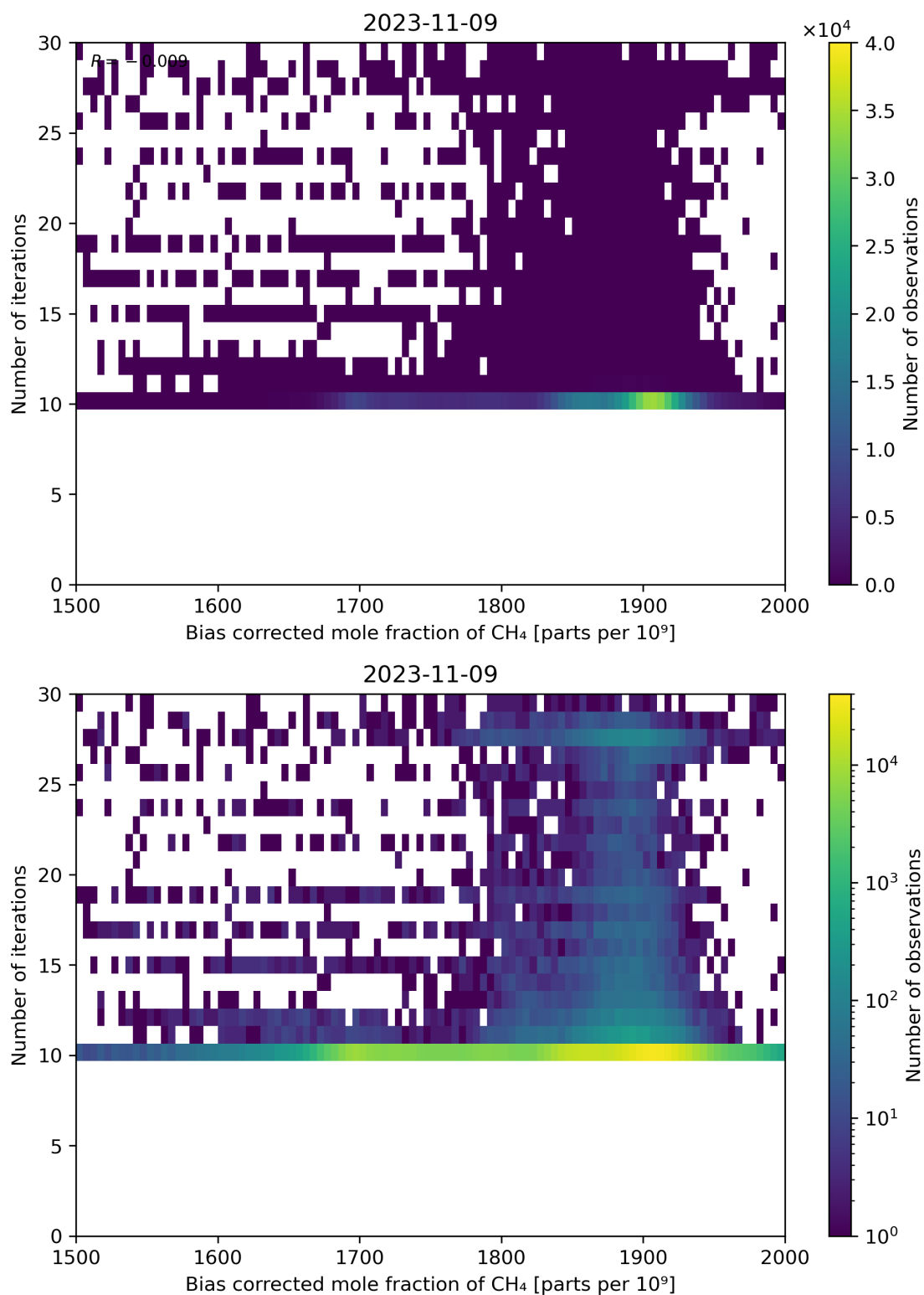
Figure 67: Scatter density plot of “Bias corrected mole fraction of CH 4 ” against “Number of iterations” for 2023-11-08 to 2023-11-10.
