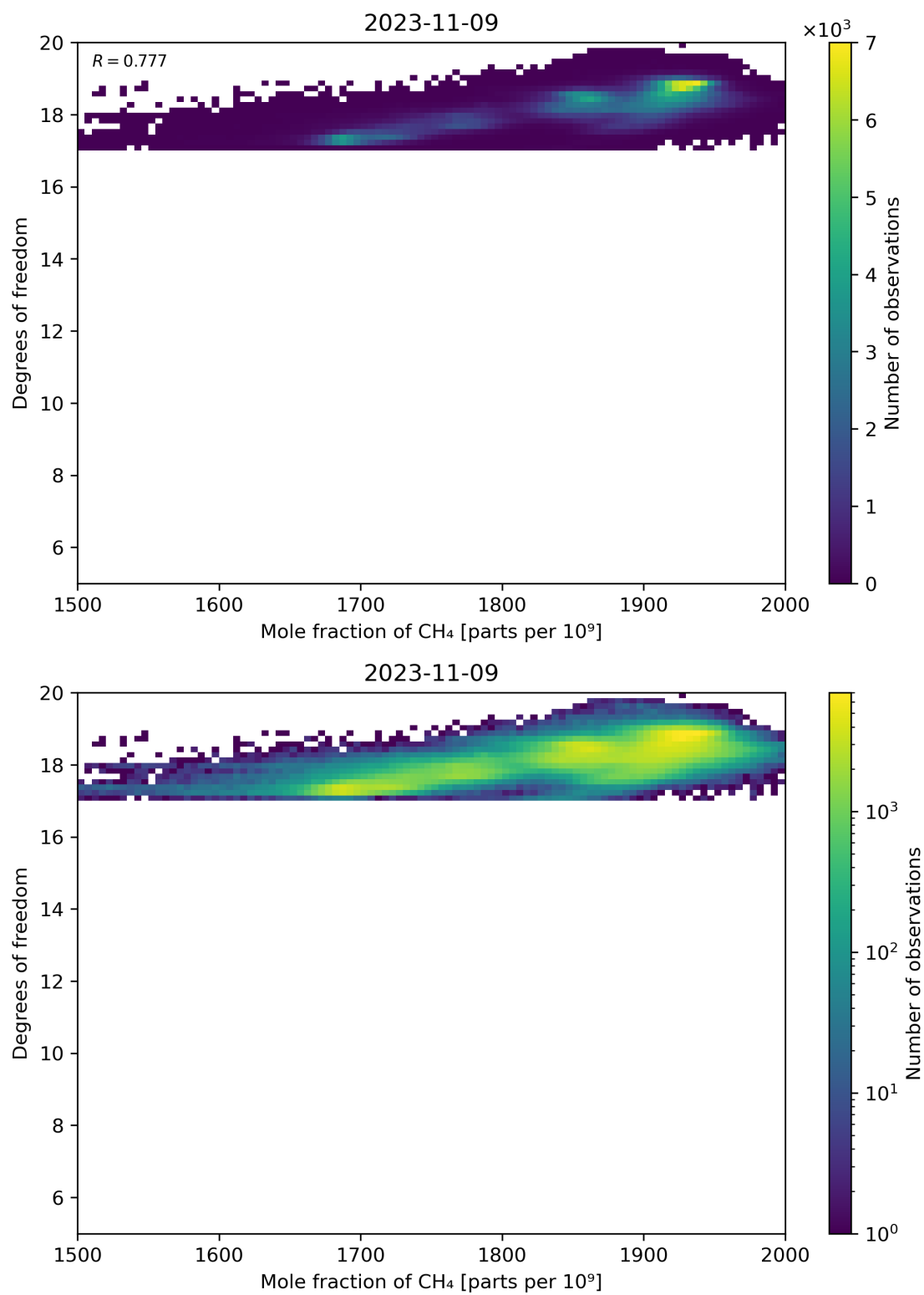
Figure 72: Scatter density plot of “Mole fraction of CH 4 ” against “Degrees of freedom” for 2023-11-08 to 2023-11-10.
