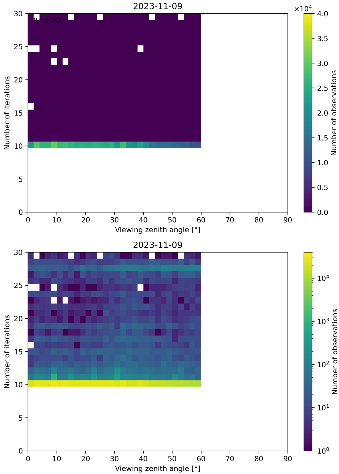
Figure 113: Scatter density plot of “Viewing zenith angle” against “Number of iterations” for 2023-11-08 to 2023-11-10.
