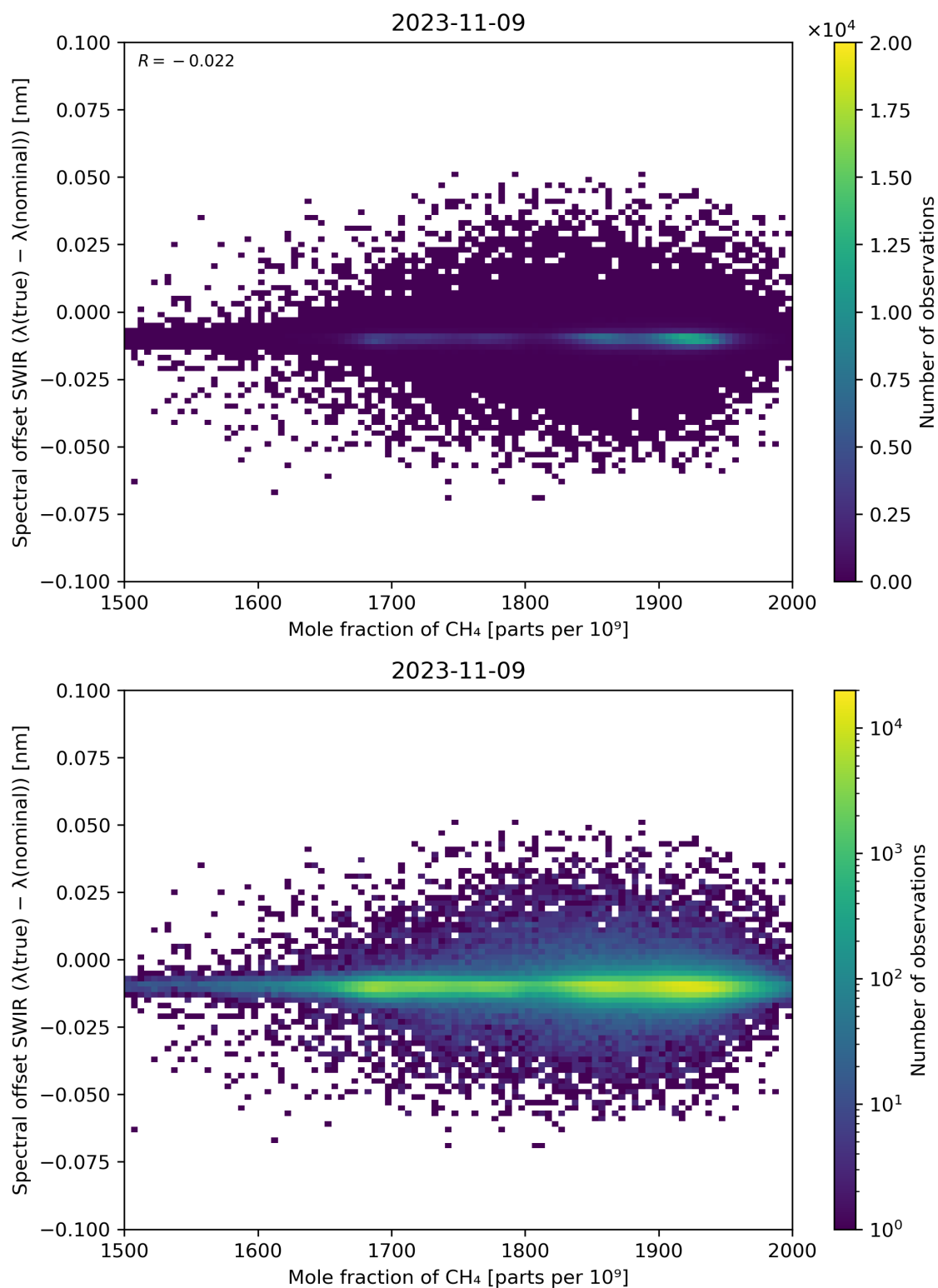
Figure 86: Scatter density plot of “Mole fraction of \text{CH}_4 ” against “Spectral offset SWIR ( \lambda(\text{true}) - \lambda(\text{nominal}) )” for 2023-11-08 to 2023-11-10.
