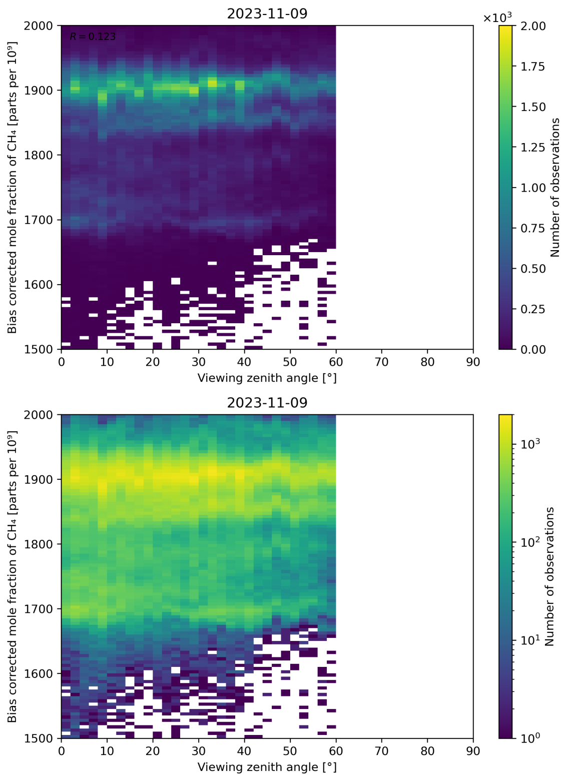
Figure 111: Scatter density plot of “Viewing zenith angle” against “Bias corrected mole fraction of CH 4 ” for 2023-11-08 to 2023-11-10.
