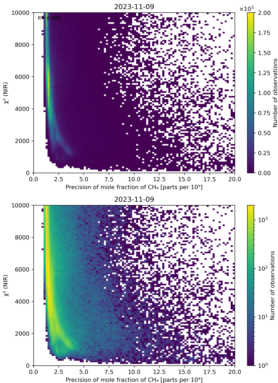
Figure 78: Scatter density plot of “Precision of mole fraction of CH 4 ” against “ \chi^2 (NIR)” for 2023-11-08 to 2023-11-10.
