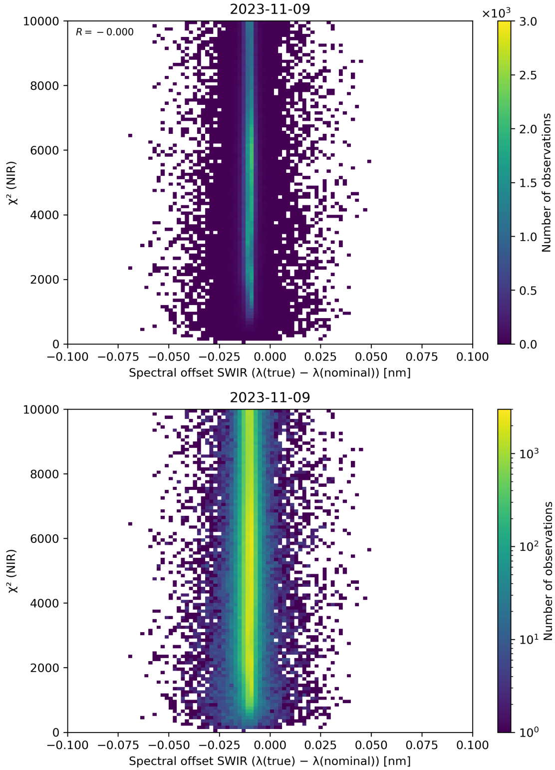
Figure 117: Scatter density plot of “Spectral offset SWIR ( \lambda(\text{true}) - \lambda(\text{nominal}) )” against “ \chi^2 (NIR)” for 2023-11-08 to 2023-11-10.
