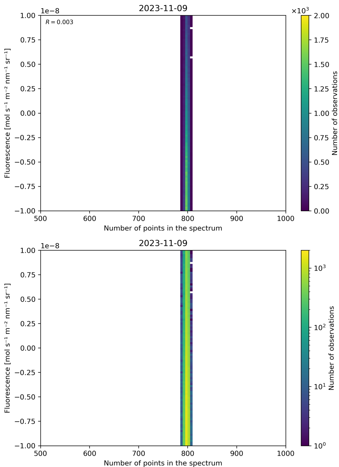
Figure 91: Scatter density plot of “Number of points in the spectrum” against “Fluorescence” for 2023-11-08 to 2023-11-10.
