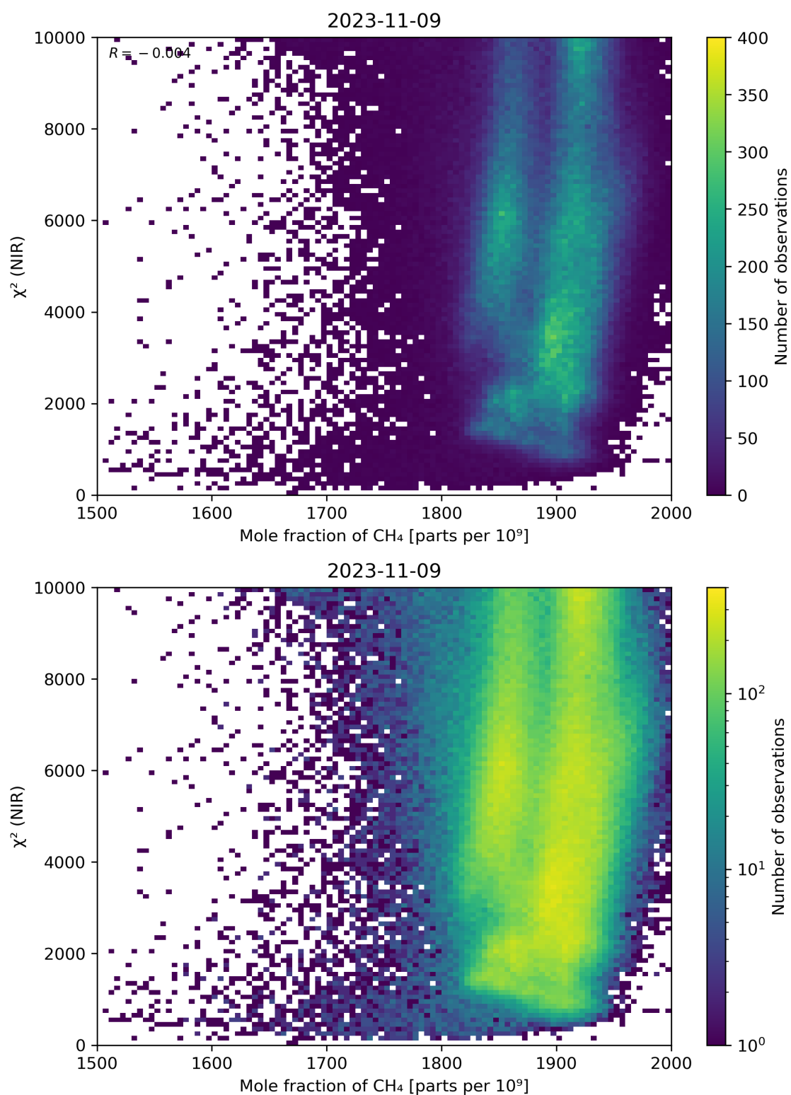
Figure 70: Scatter density plot of “Mole fraction of CH 4 ” against “ \chi^2 (NIR)” for 2023-11-08 to 2023-11-10.
