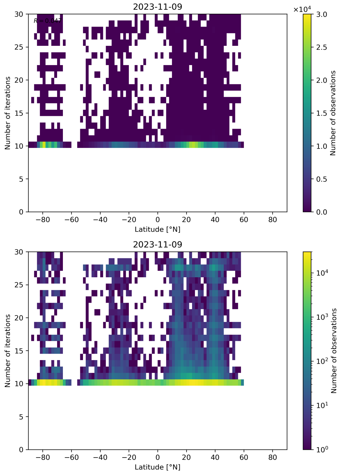
Figure 60: Scatter density plot of “Latitude” against “Number of iterations” for 2023-11-08 to 2023-11-10.
