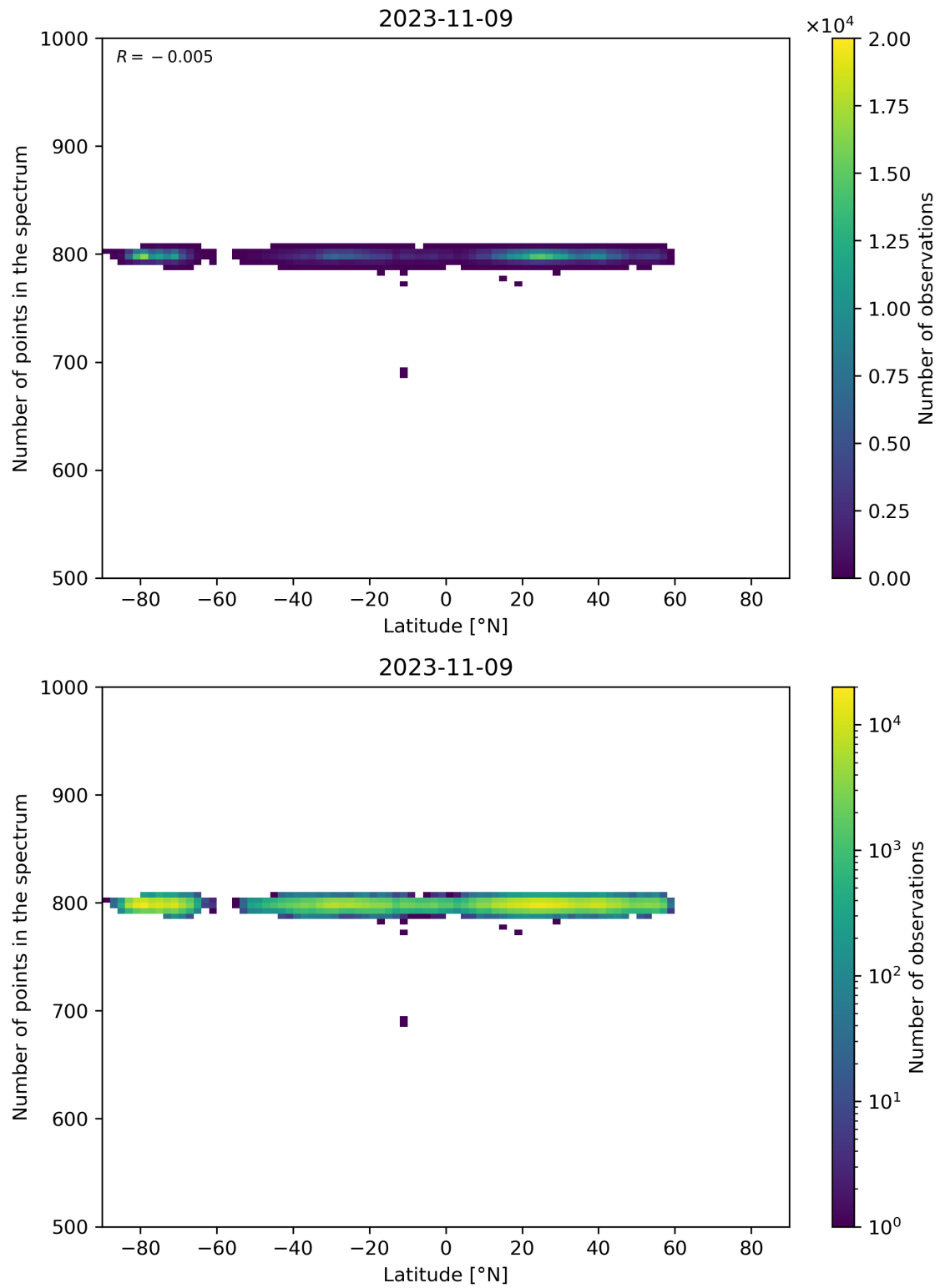
Figure 61: Scatter density plot of “Latitude” against “Number of points in the spectrum” for 2023-11-08 to 2023-11-10.
