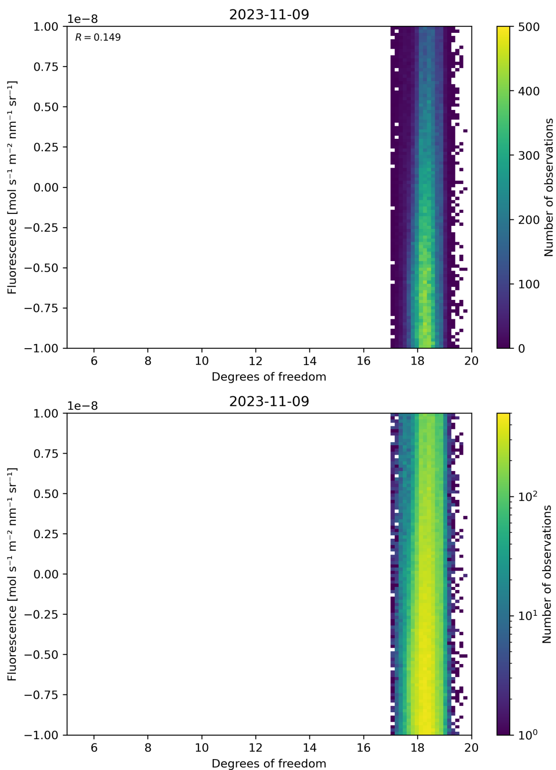
Figure 51: Scatter density plot of “Degrees of freedom” against “Fluorescence” for 2023-11-08 to 2023-11-10.
