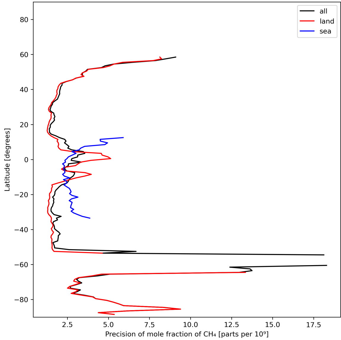
Figure 13: Zonal average of “Precision of mole fraction of CH 4 ” for 2023-11-08 to 2023-11-10.
