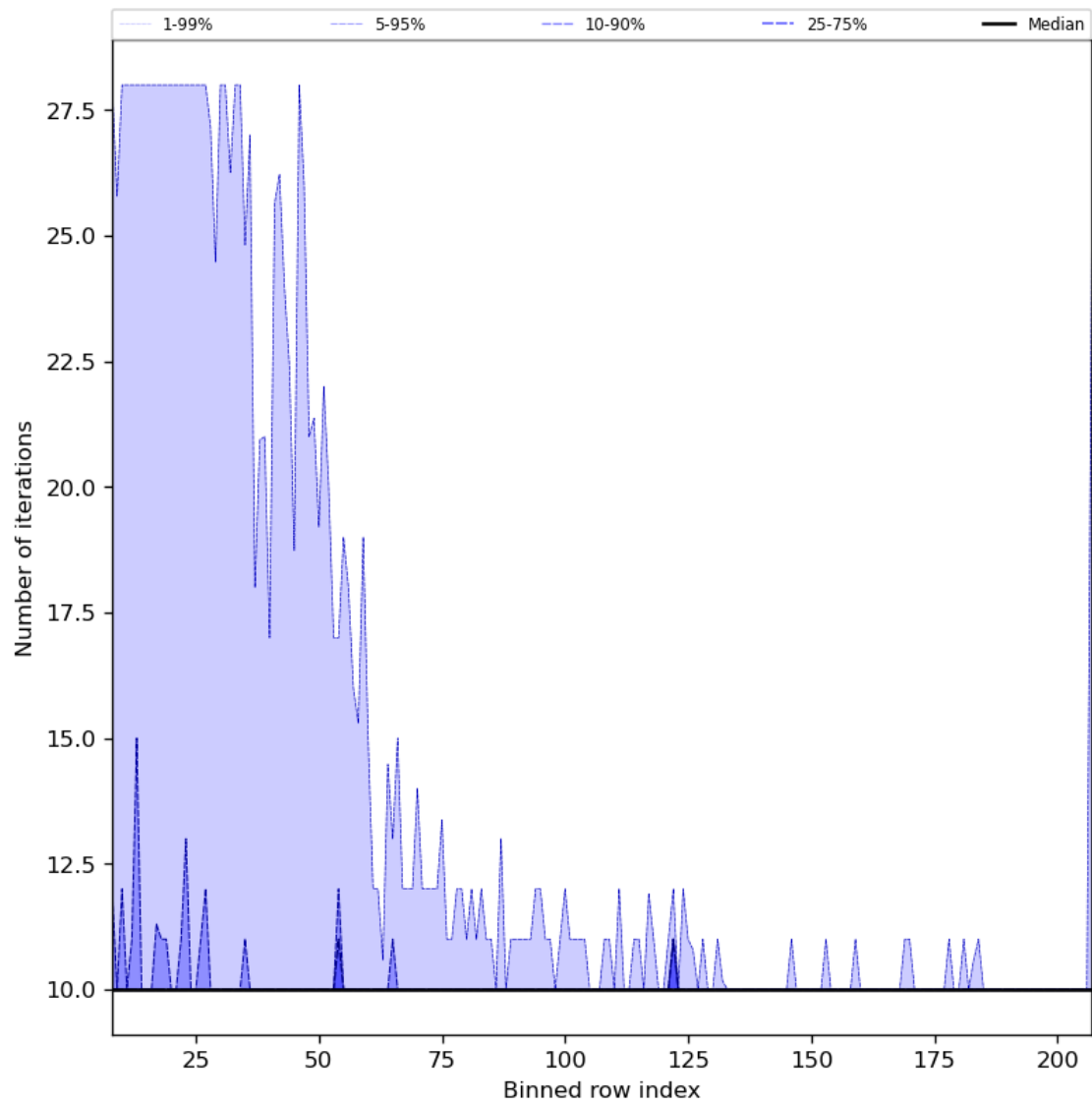
Figure 42: Along track statistics of “Number of iterations” for 2023-11-08 to 2023-11-10
