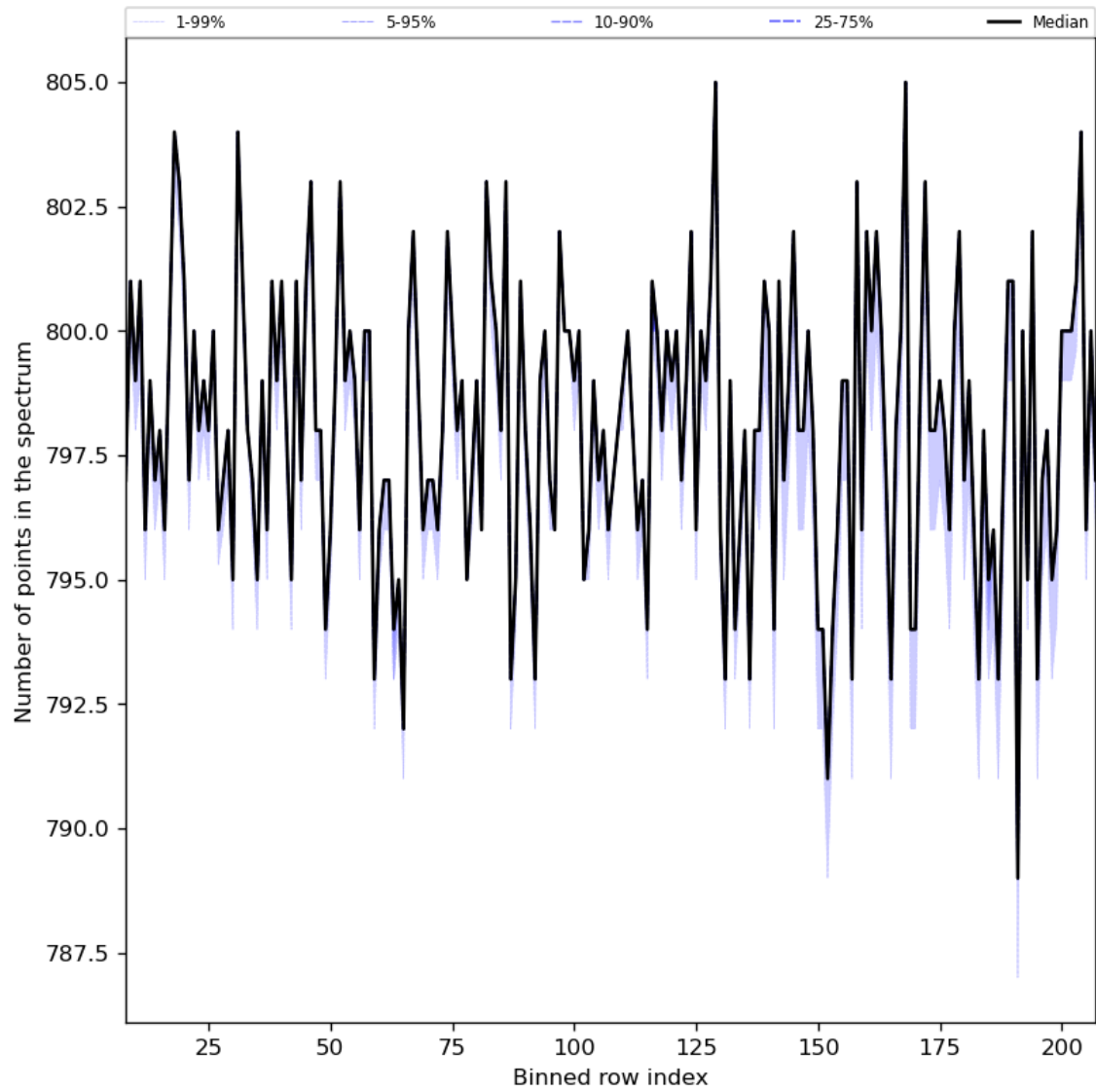
Figure 37: Along track statistics of “Number of points in the spectrum” for 2023-11-08 to 2023-11-10
