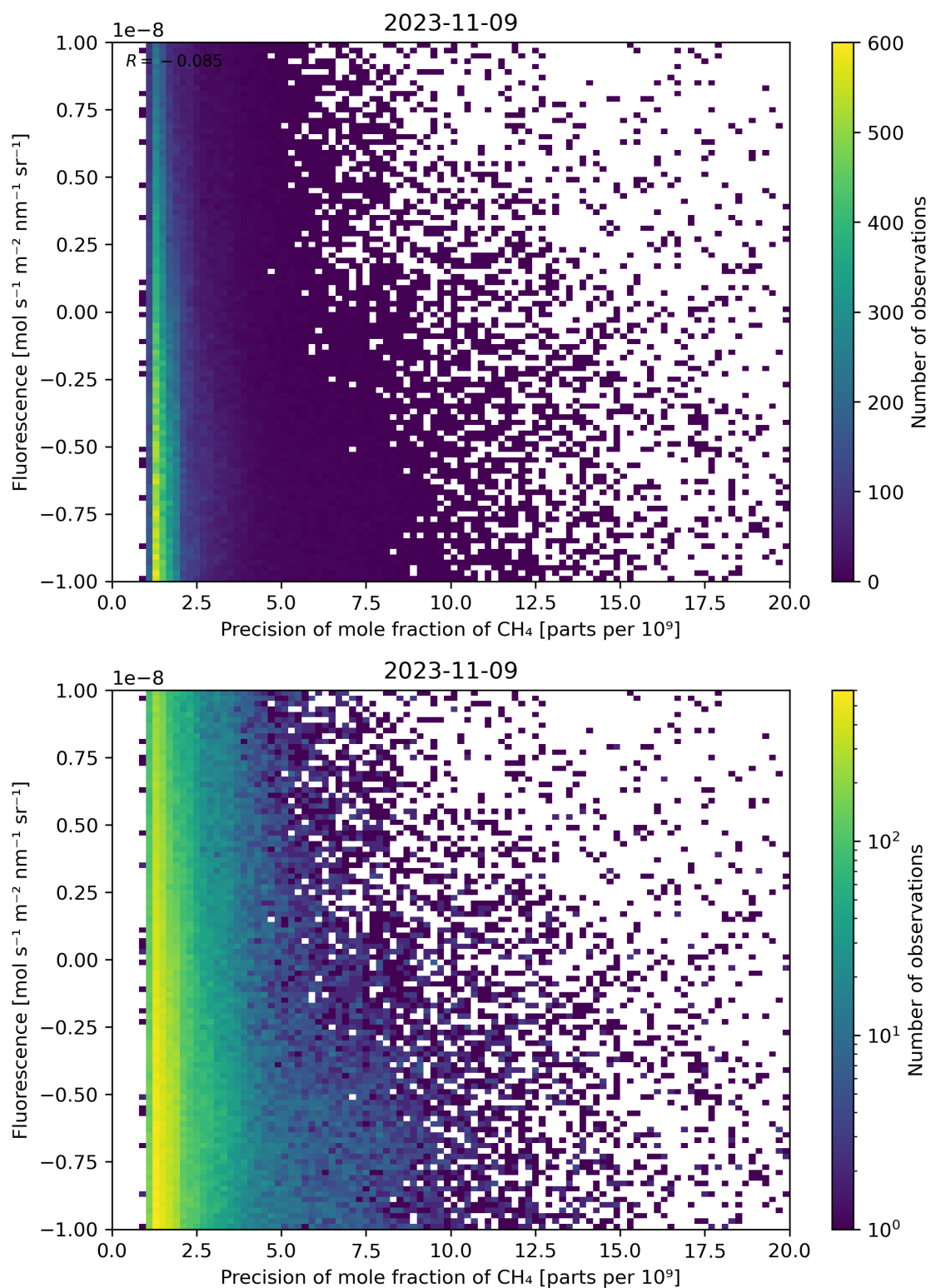
Figure 81: Scatter density plot of “Precision of mole fraction of \text{CH}_4 ” against “Fluorescence” for 2023-11-08 to 2023-11-10.
