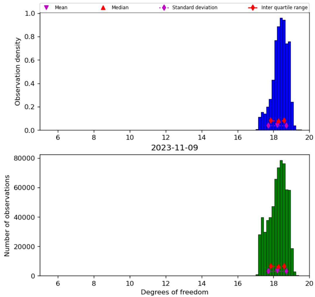
Figure 30: Histogram of “Degrees of freedom” for 2023-11-08 to 2023-11-10
