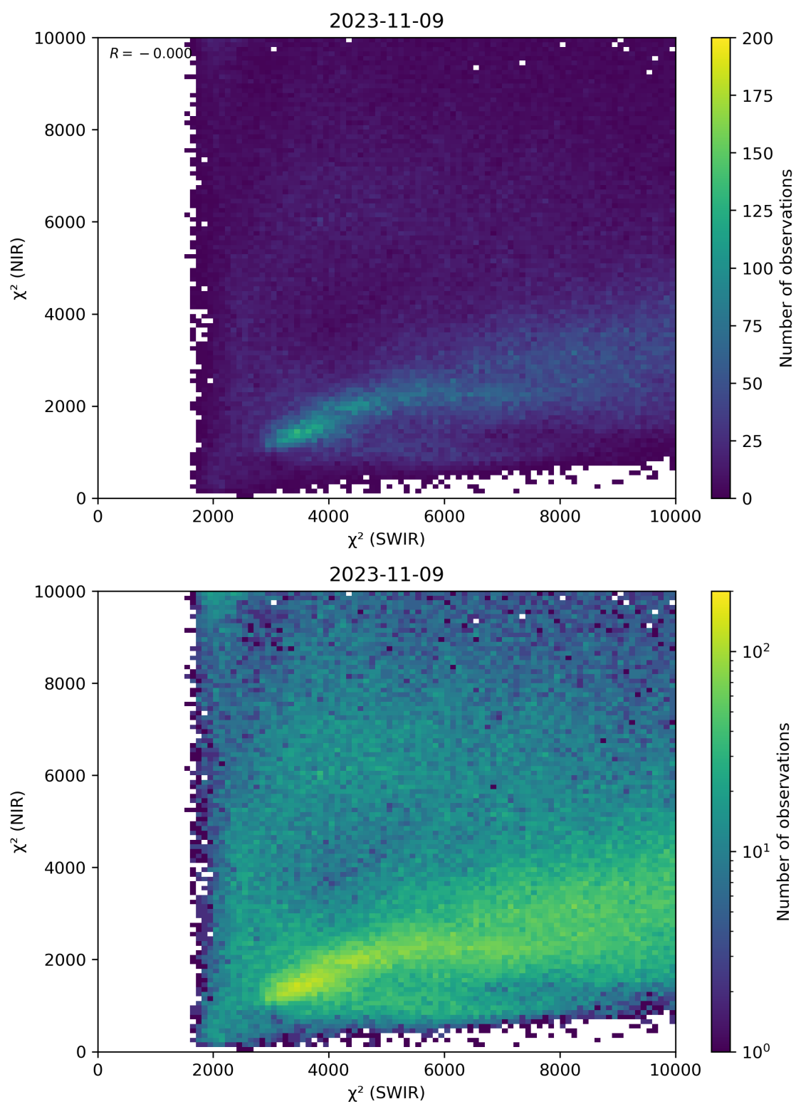
Figure 47: Scatter density plot of “ \chi^2 (SWIR)” against “ \chi^2 (NIR)” for 2023-11-08 to 2023-11-10.
