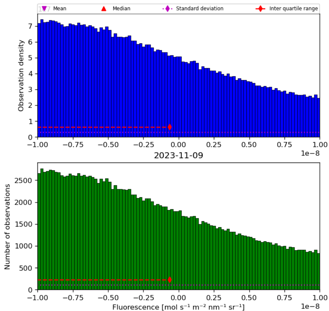
Figure 32: Histogram of “Fluorescence” for 2023-11-08 to 2023-11-10
