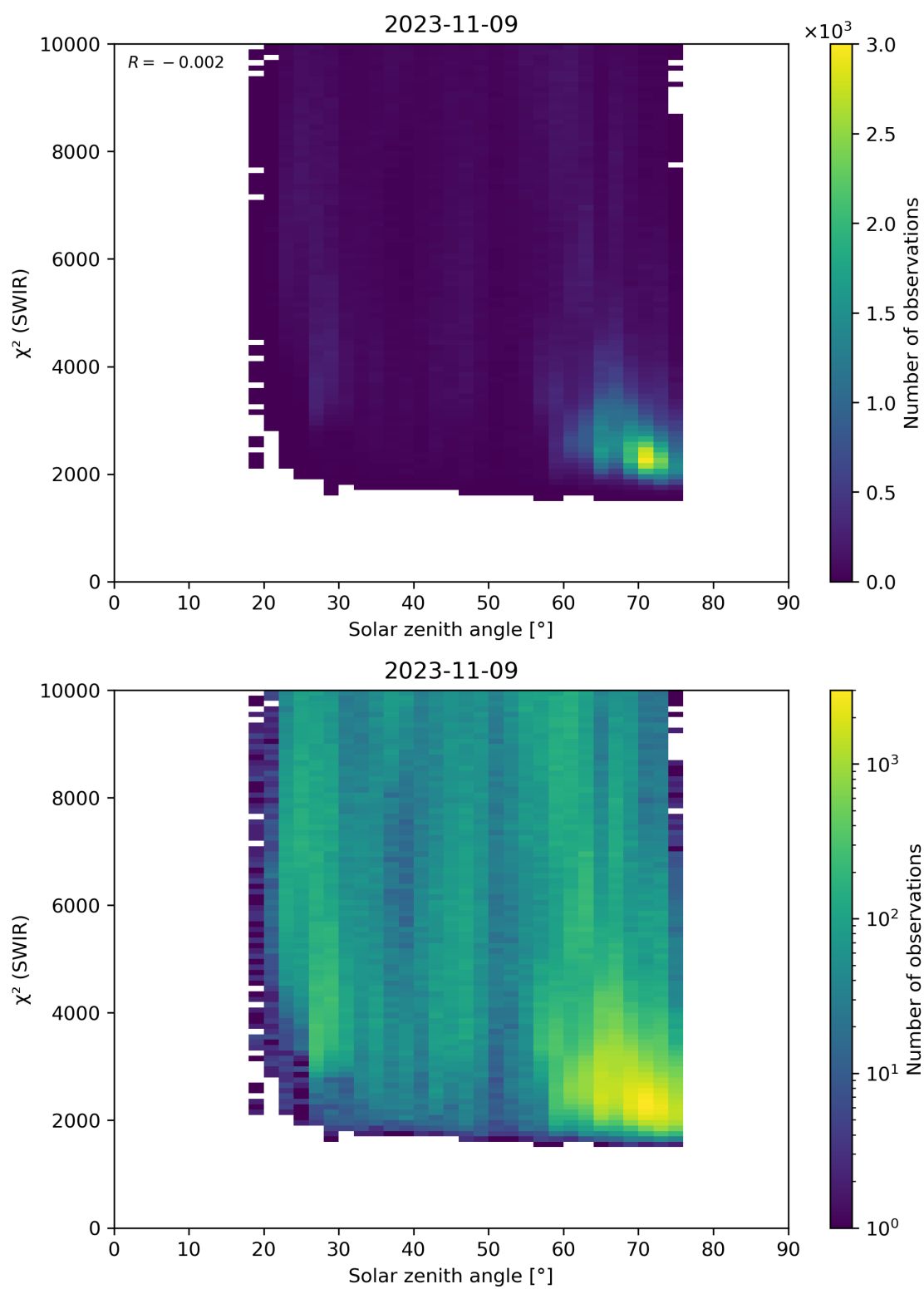
Figure 95: Scatter density plot of “Solar zenith angle” against “ \chi^2 (SWIR)” for 2023-11-08 to 2023-11-10.
