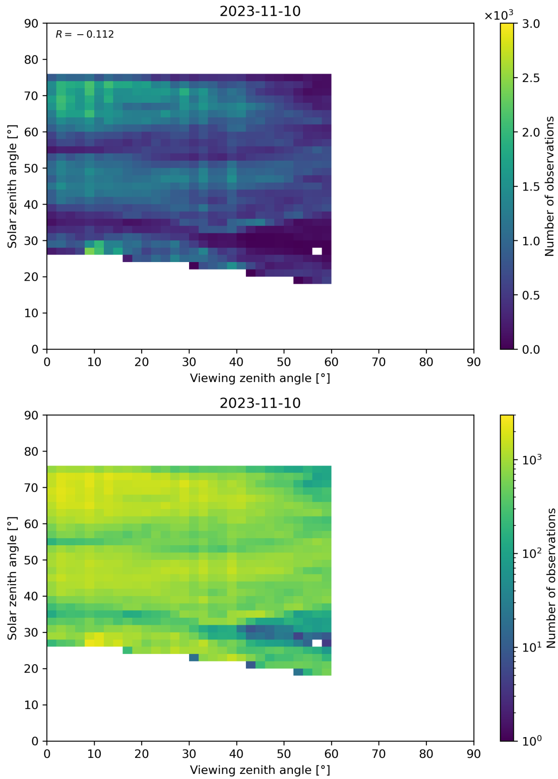
Figure 115: Scatter density plot of “Viewing zenith angle” against “Solar zenith angle” for 2023-11-09 to 2023-11-11.
