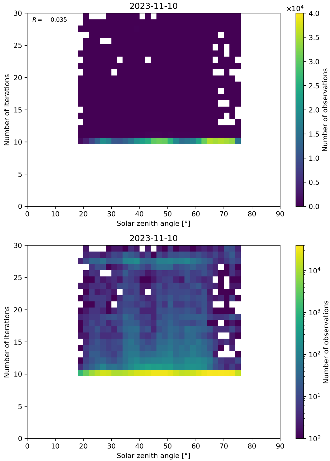
Figure 102: Scatter density plot of “Solar zenith angle” against “Number of iterations” for 2023-11-09 to 2023-11-11.
