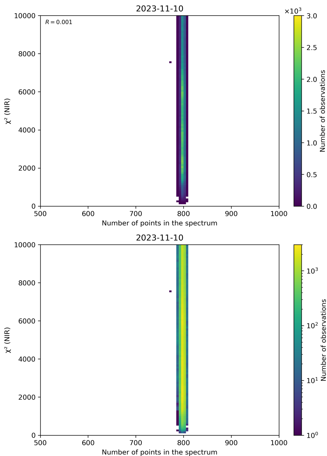
Figure 88: Scatter density plot of “Number of points in the spectrum” against “ \chi^2 (NIR)” for 2023-11-09 to 2023-11-11.
