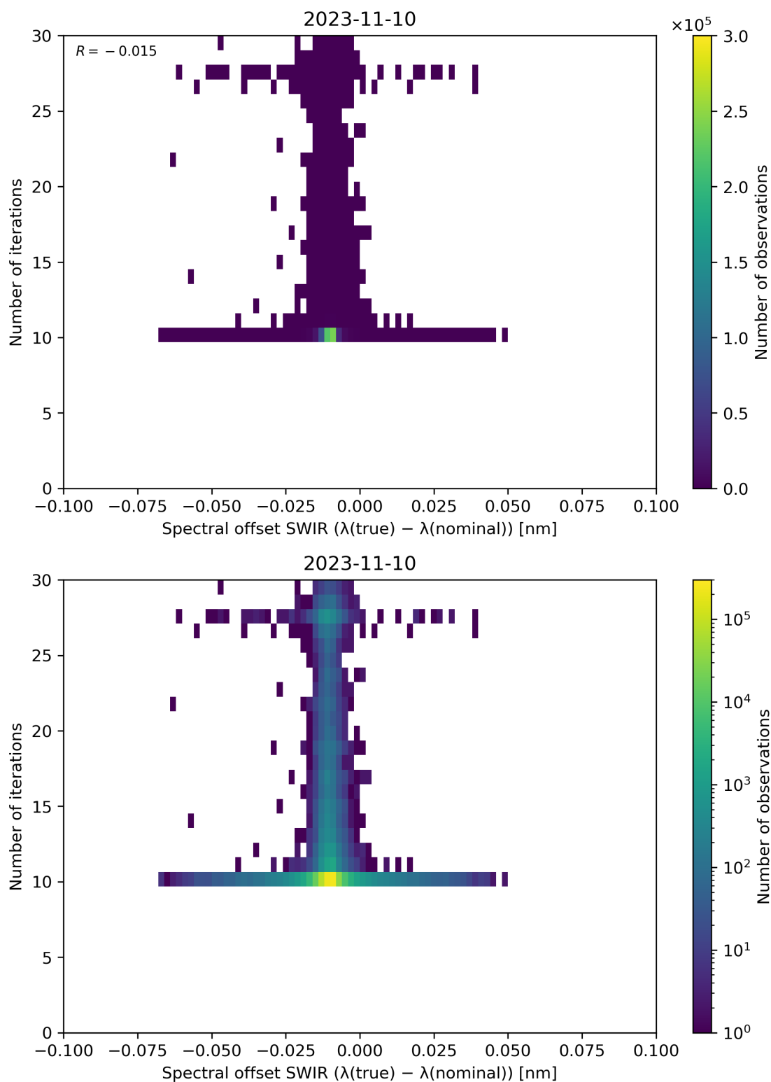
Figure 121: Scatter density plot of “Spectral offset SWIR ( \lambda(\text{true}) - \lambda(\text{nominal}) )” against “Number of iterations” for 2023-11-09 to 2023-11-11.
