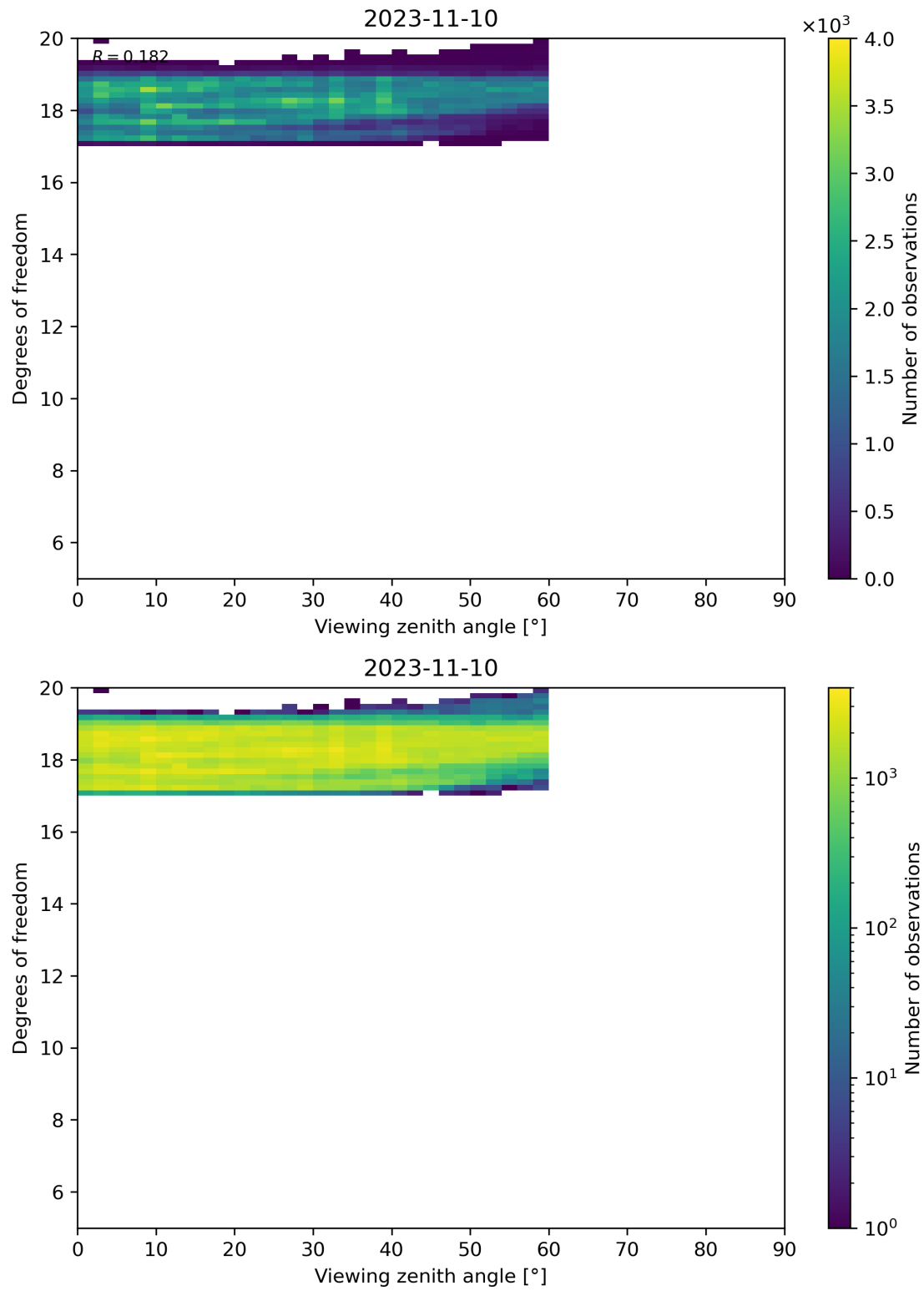
Figure 107: Scatter density plot of “Viewing zenith angle” against “Degrees of freedom” for 2023-11-09 to 2023-11-11.
