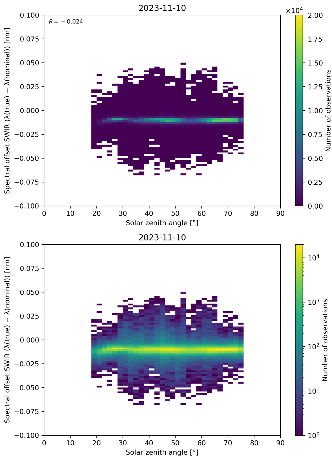
Figure 104: Scatter density plot of “Solar zenith angle” against “Spectral offset SWIR ( \lambda(\text{true}) - \lambda(\text{nominal}) )” for 2023-11-09 to 2023-11-11.
