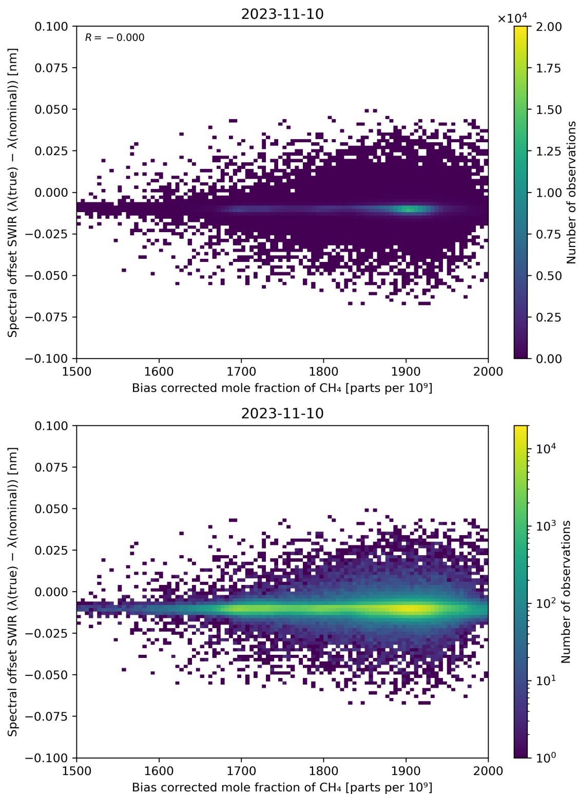
Figure 69: Scatter density plot of “Bias corrected mole fraction of \text{CH}_4 ” against “Spectral offset SWIR ( \lambda(\text{true}) - \lambda(\text{nominal}) )” for 2023-11-09 to 2023-11-11.
