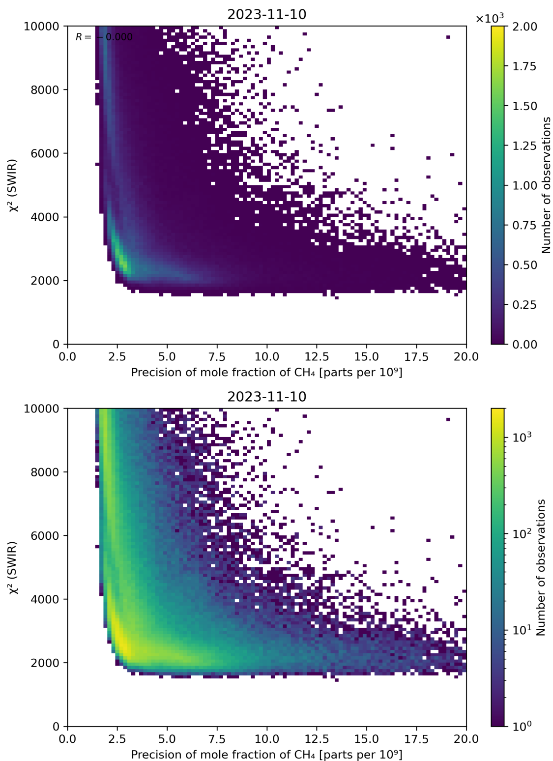
Figure 79: Scatter density plot of “Precision of mole fraction of CH 4 ” against “ \chi^2 (SWIR)” for 2023-11-09 to 2023-11-11.
