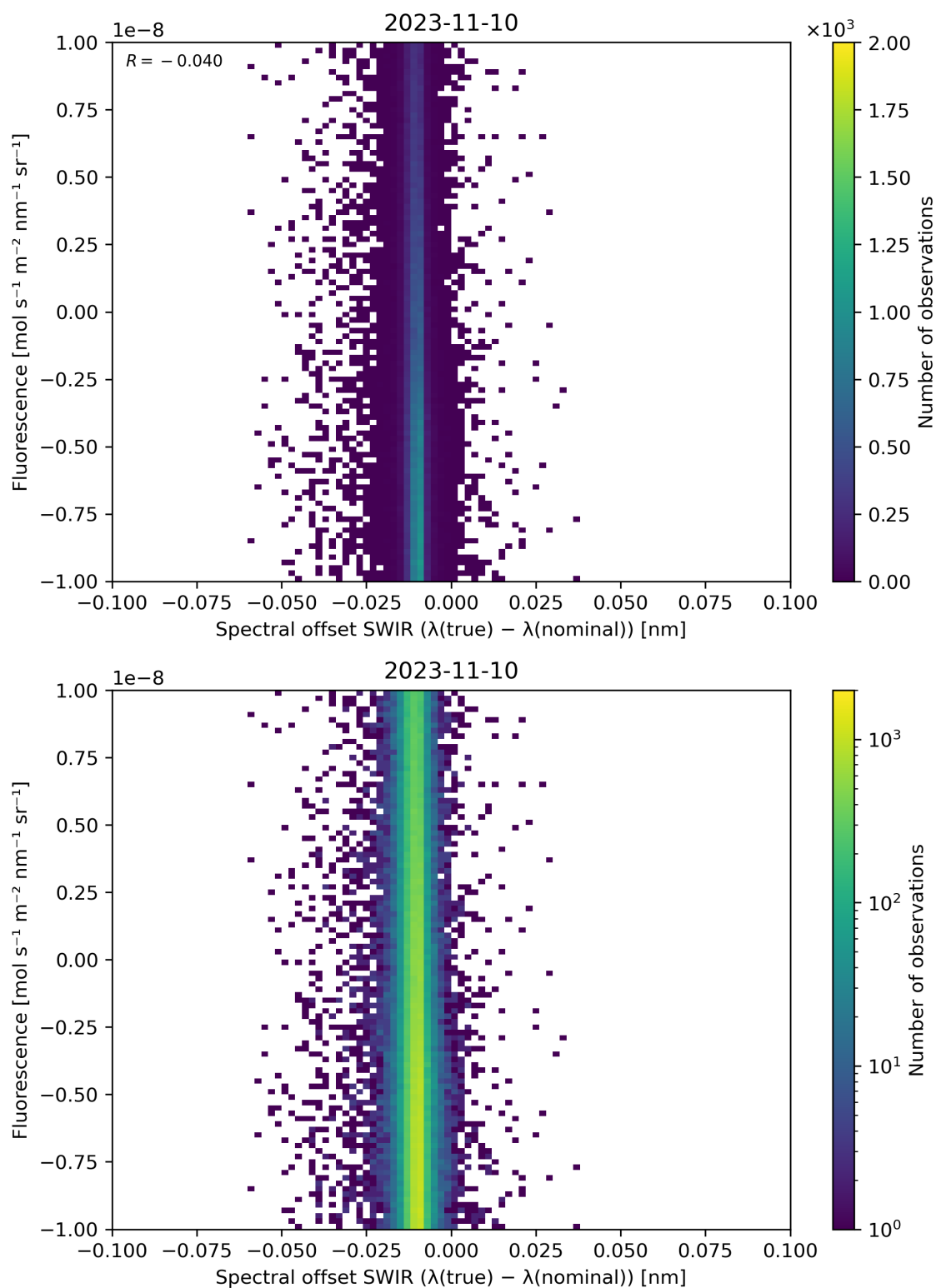
Figure 120: Scatter density plot of “Spectral offset SWIR ( \lambda(\text{true}) - \lambda(\text{nominal}) )” against “Fluorescence” for 2023-11-09 to 2023-11-11.
