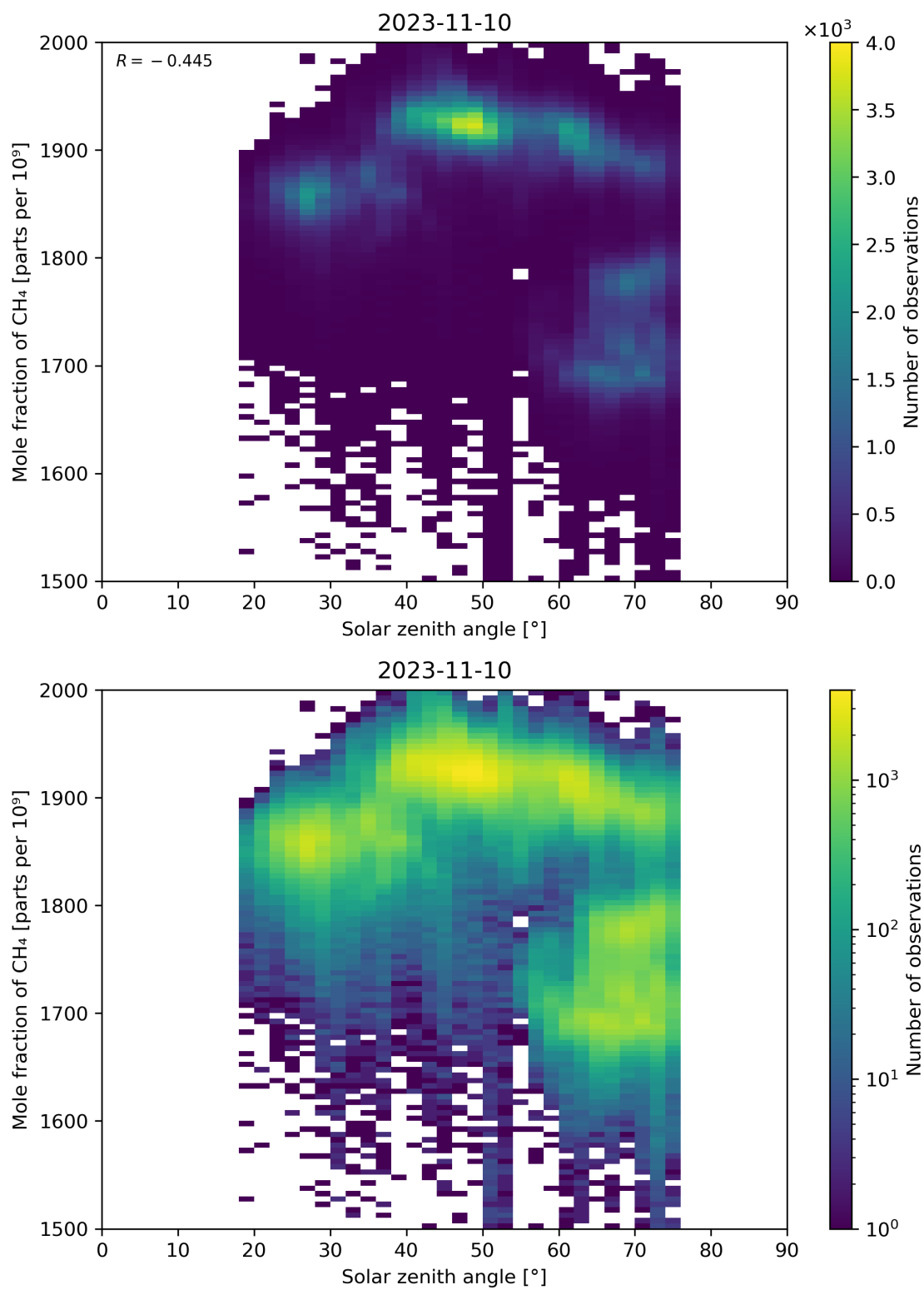
Figure 99: Scatter density plot of “Solar zenith angle” against “Mole fraction of \text{CH}_4 ” for 2023-11-09 to 2023-11-11.
