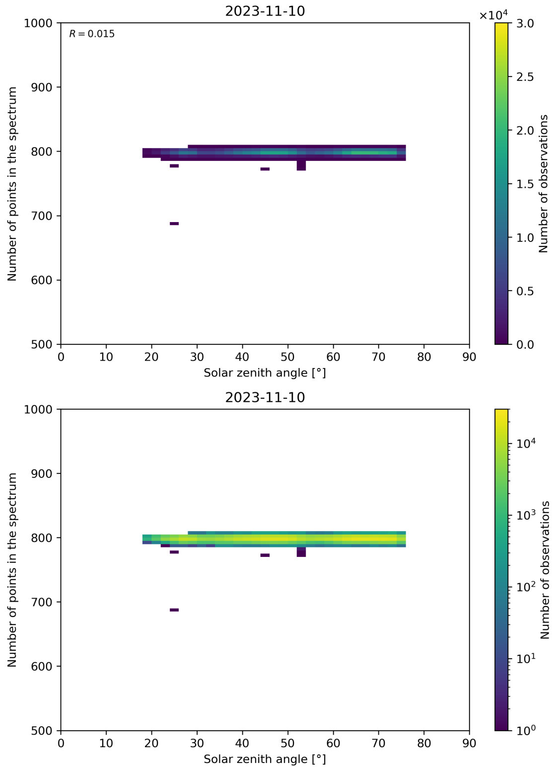
Figure 103: Scatter density plot of “Solar zenith angle” against “Number of points in the spectrum” for 2023-11-09 to 2023-11-11.
