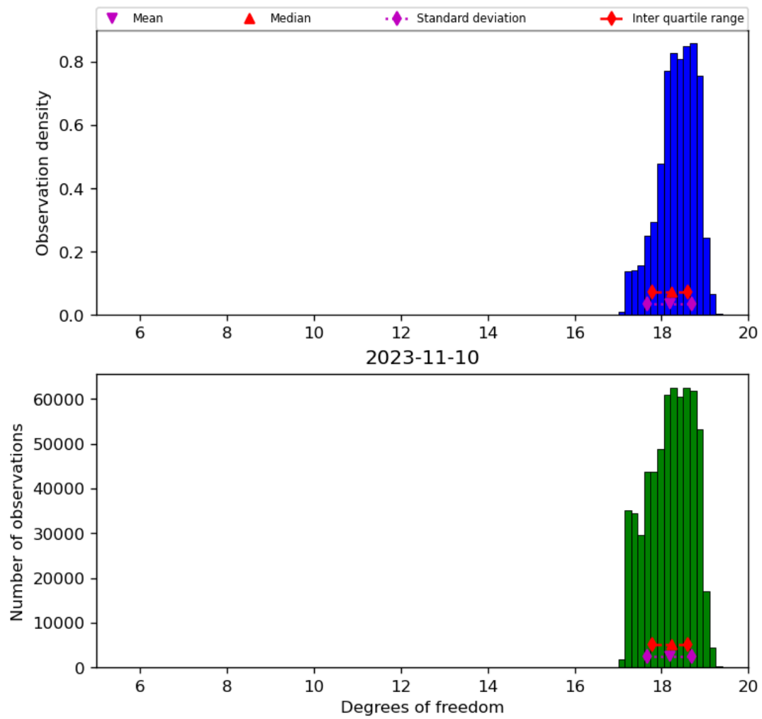
Figure 30: Histogram of “Degrees of freedom” for 2023-11-09 to 2023-11-11
