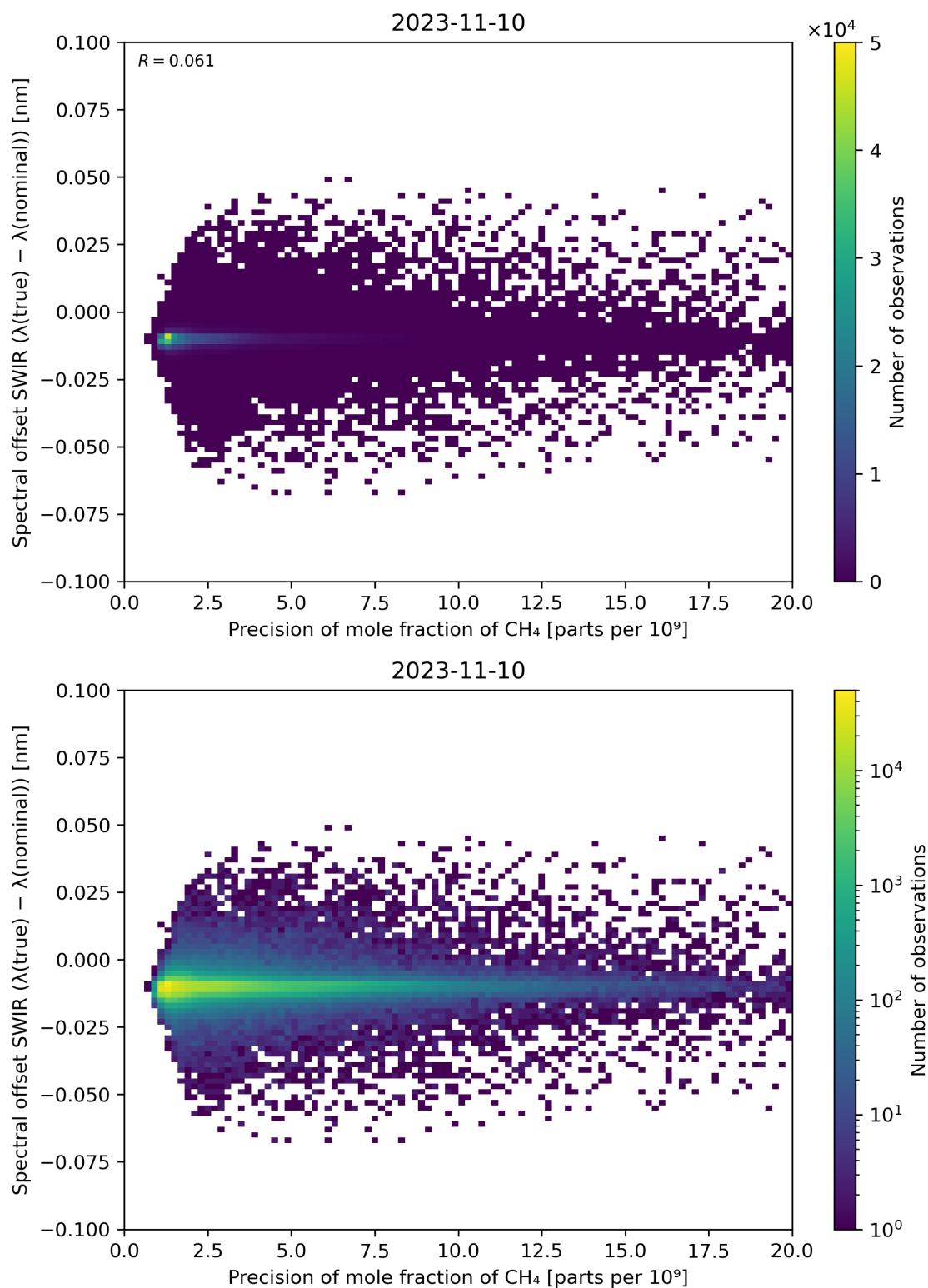
Figure 85: Scatter density plot of “Precision of mole fraction of CH 4 ” against “Spectral offset SWIR ( \lambda(\text{true}) - \lambda(\text{nominal}) )” for 2023-11-09 to 2023-11-11.
