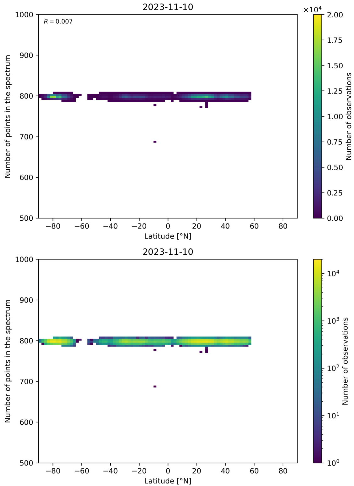
Figure 61: Scatter density plot of “Latitude” against “Number of points in the spectrum” for 2023-11-09 to 2023-11-11.
