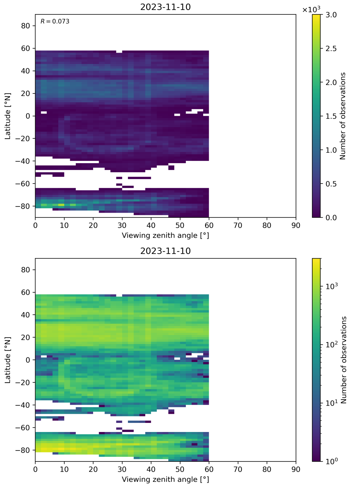
Figure 109: Scatter density plot of “Viewing zenith angle” against “Latitude” for 2023-11-09 to 2023-11-11.
