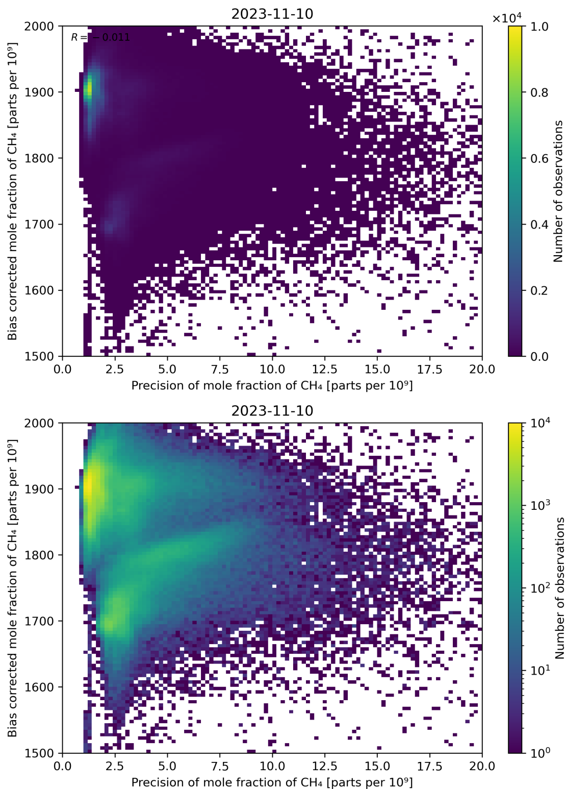
Figure 82: Scatter density plot of “Precision of mole fraction of CH 4 ” against “Bias corrected mole fraction of CH 4 ” for 2023-11-09 to 2023-11-11.
