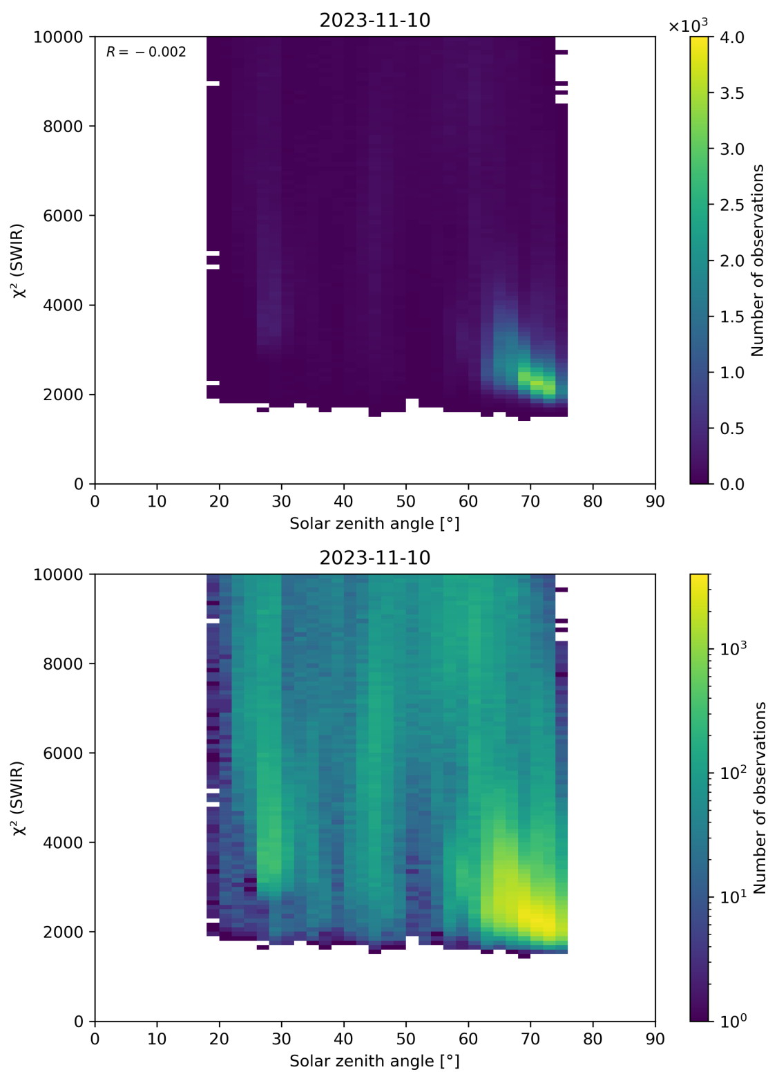
Figure 95: Scatter density plot of “Solar zenith angle” against “ \chi^2 (SWIR)” for 2023-11-09 to 2023-11-11.
