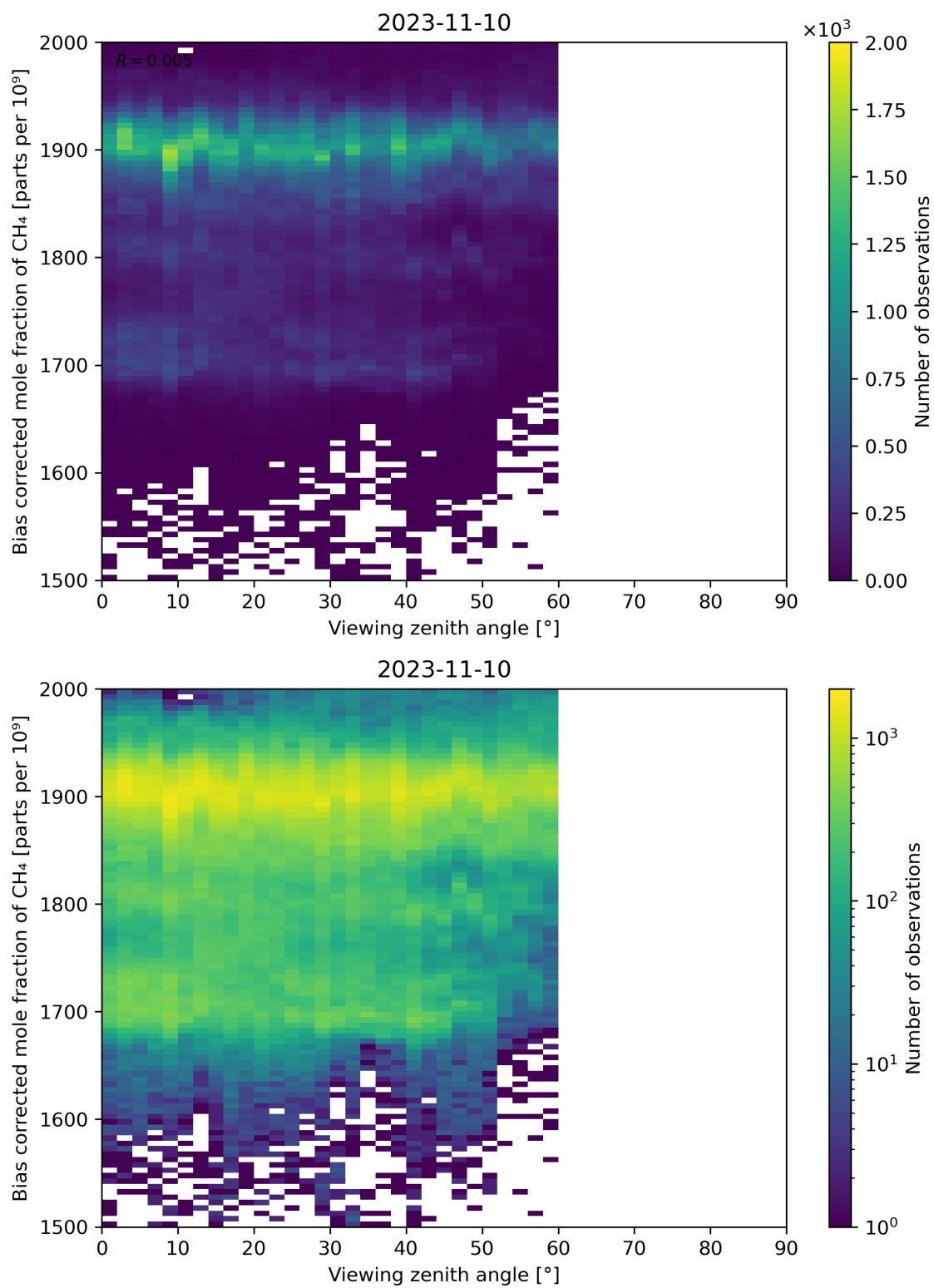
Figure 111: Scatter density plot of “Viewing zenith angle” against “Bias corrected mole fraction of CH 4 ” for 2023-11-09 to 2023-11-11.
