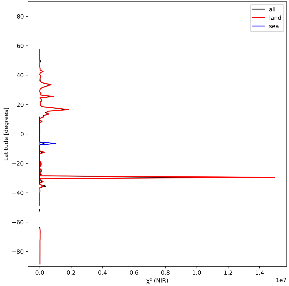
Figure 18: Zonal average of “ \chi^2 (NIR)” for 2023-11-09 to 2023-11-11.
