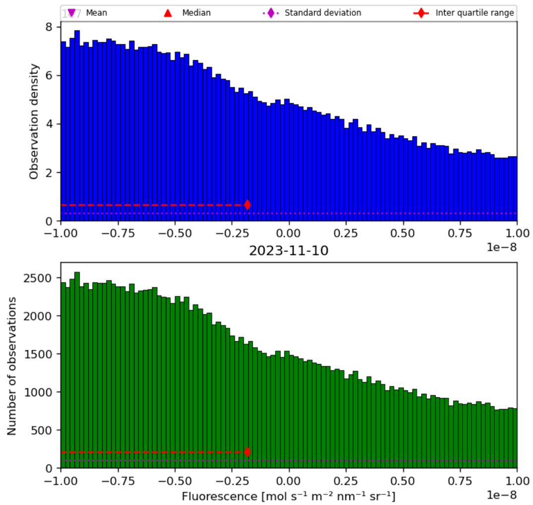
Figure 32: Histogram of “Fluorescence” for 2023-11-09 to 2023-11-11
