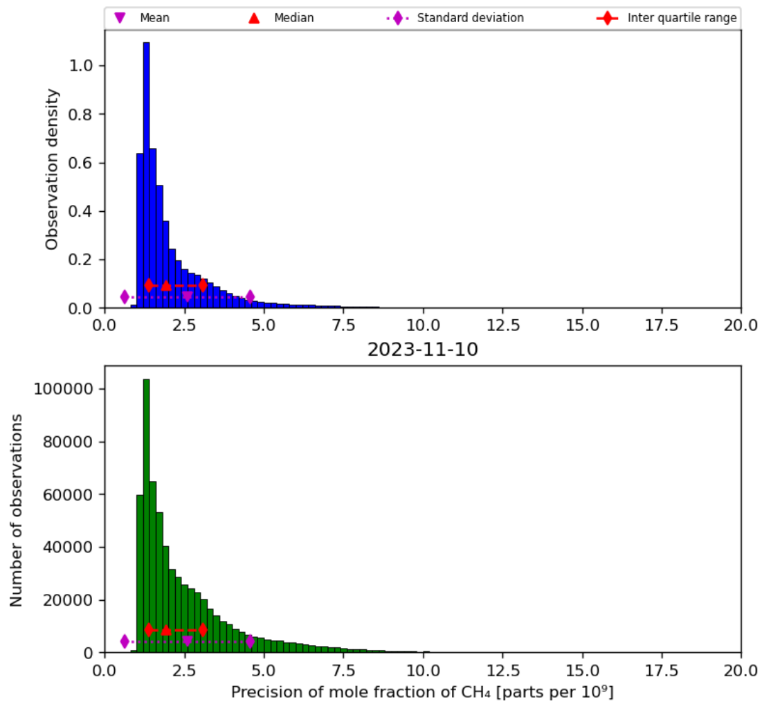
Figure 24: Histogram of “Precision of mole fraction of CH 4 ” for 2023-11-09 to 2023-11-11
