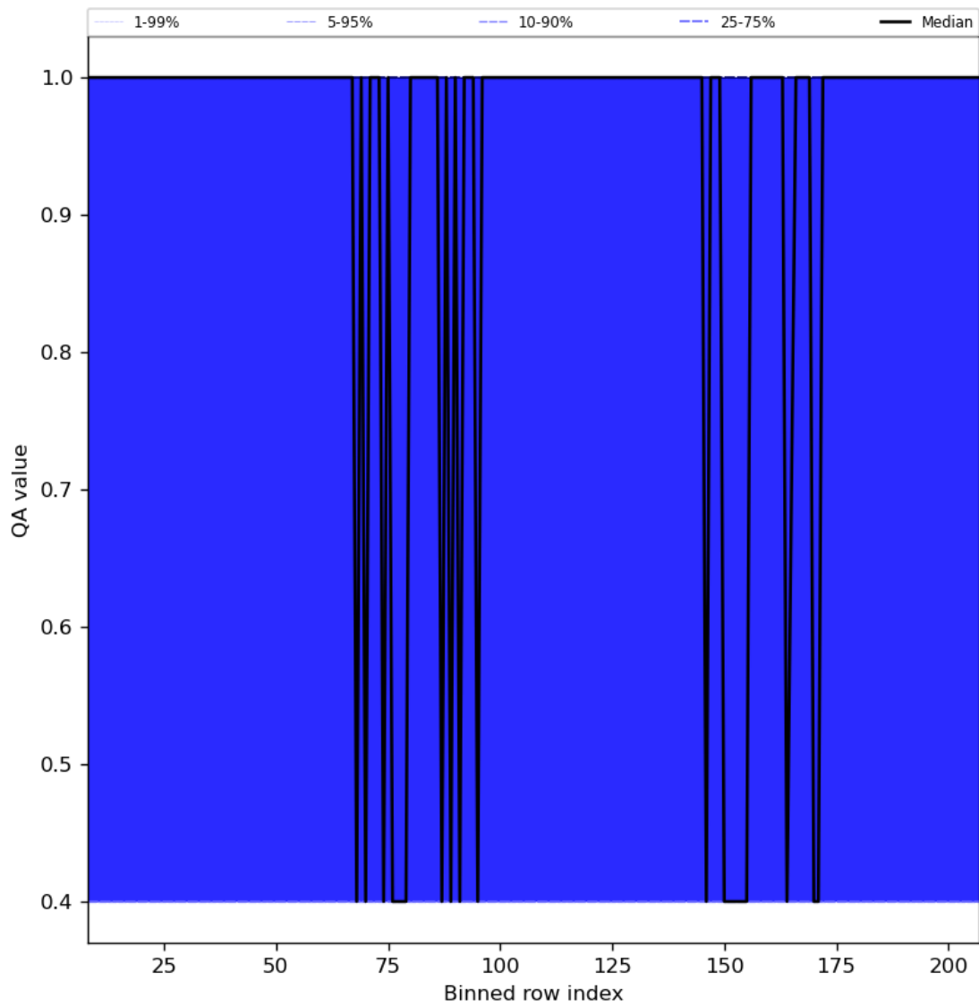
Figure 33: Along track statistics of “QA value” for 2023-11-09 to 2023-11-11
