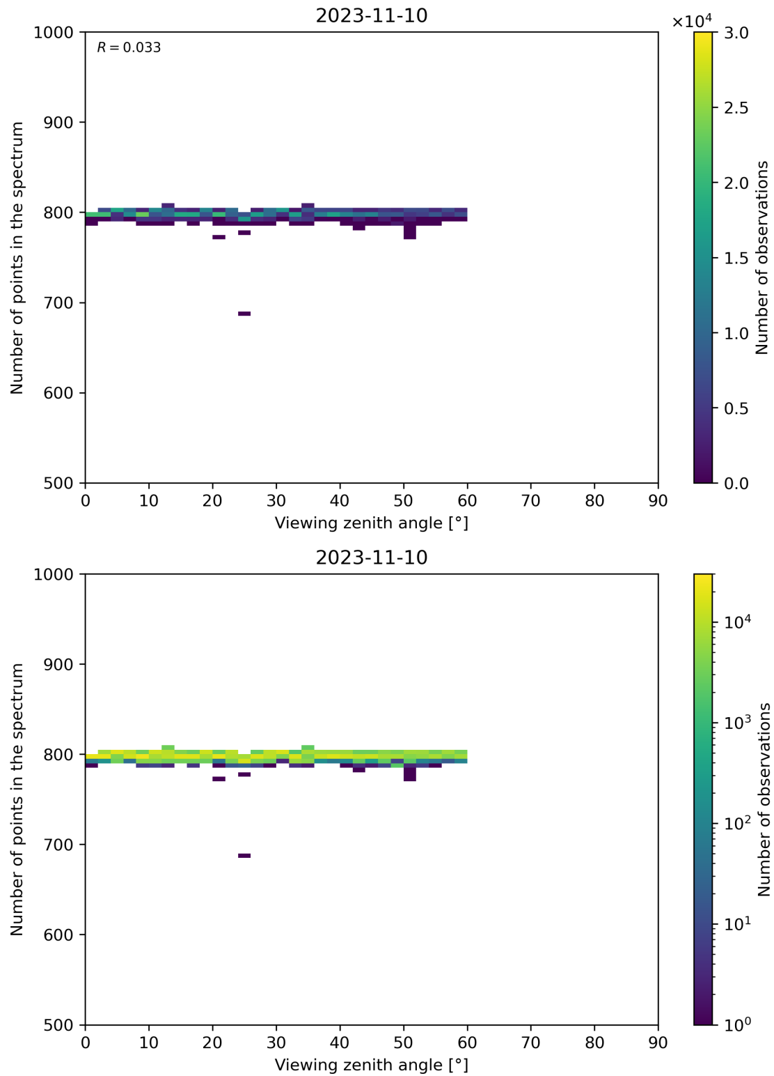
Figure 114: Scatter density plot of “Viewing zenith angle” against “Number of points in the spectrum” for 2023-11-09 to 2023-11-11.
