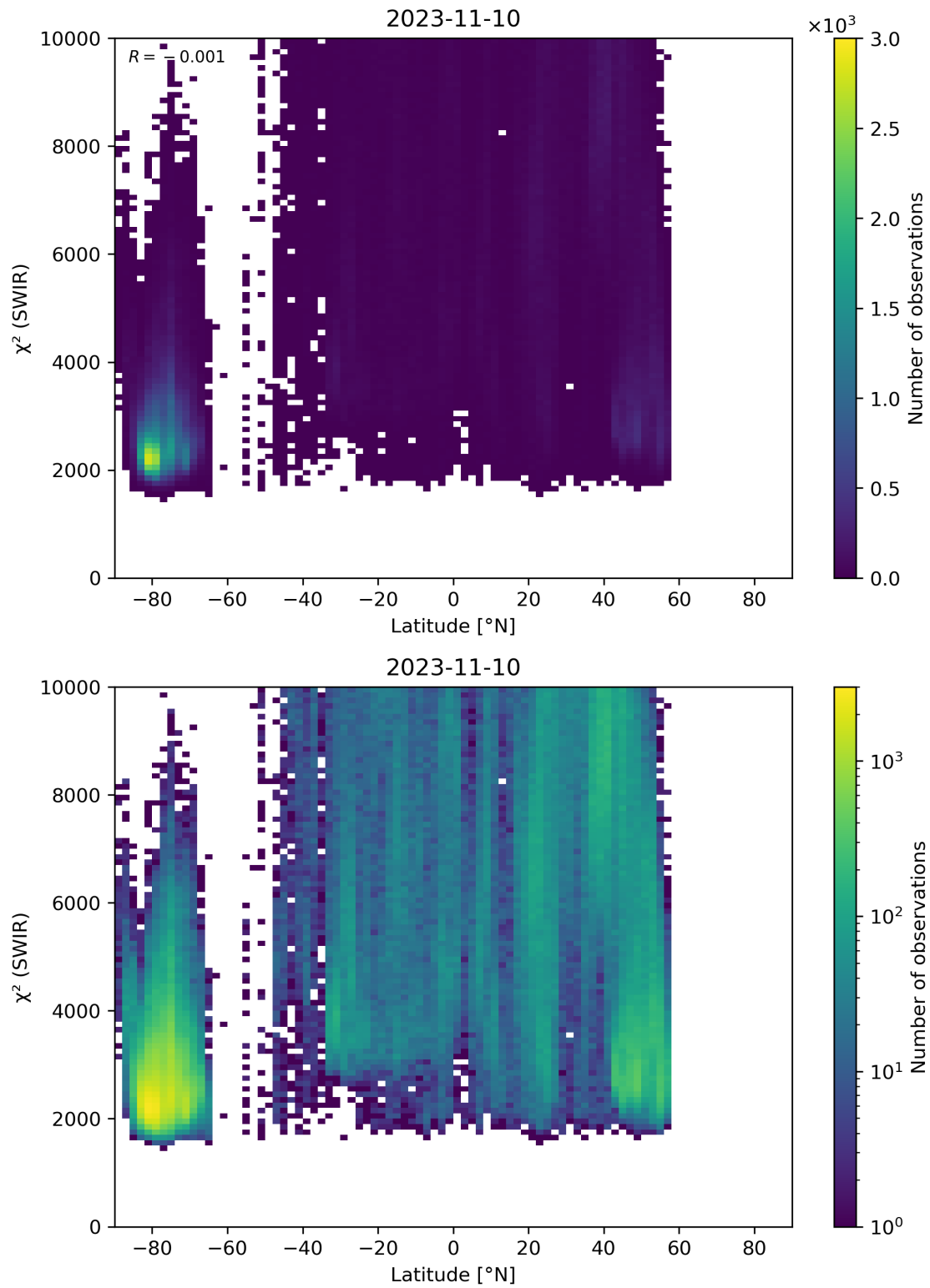
Figure 54: Scatter density plot of “Latitude” against “ \chi^2 (SWIR)” for 2023-11-09 to 2023-11-11.
