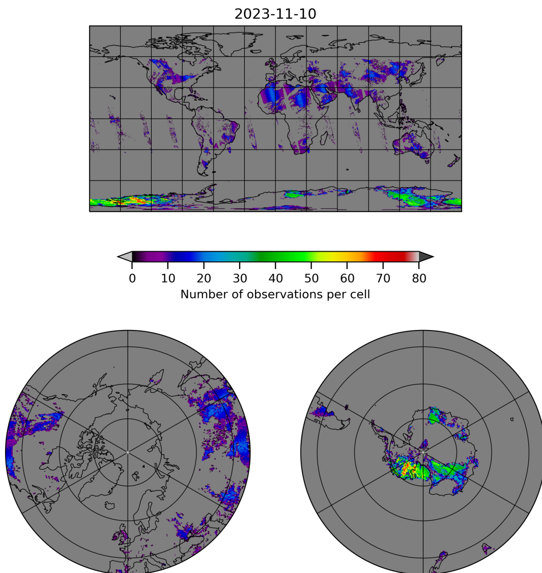
Figure 10: Map of the number of observations for 2023-11-09 to 2023-11-11
