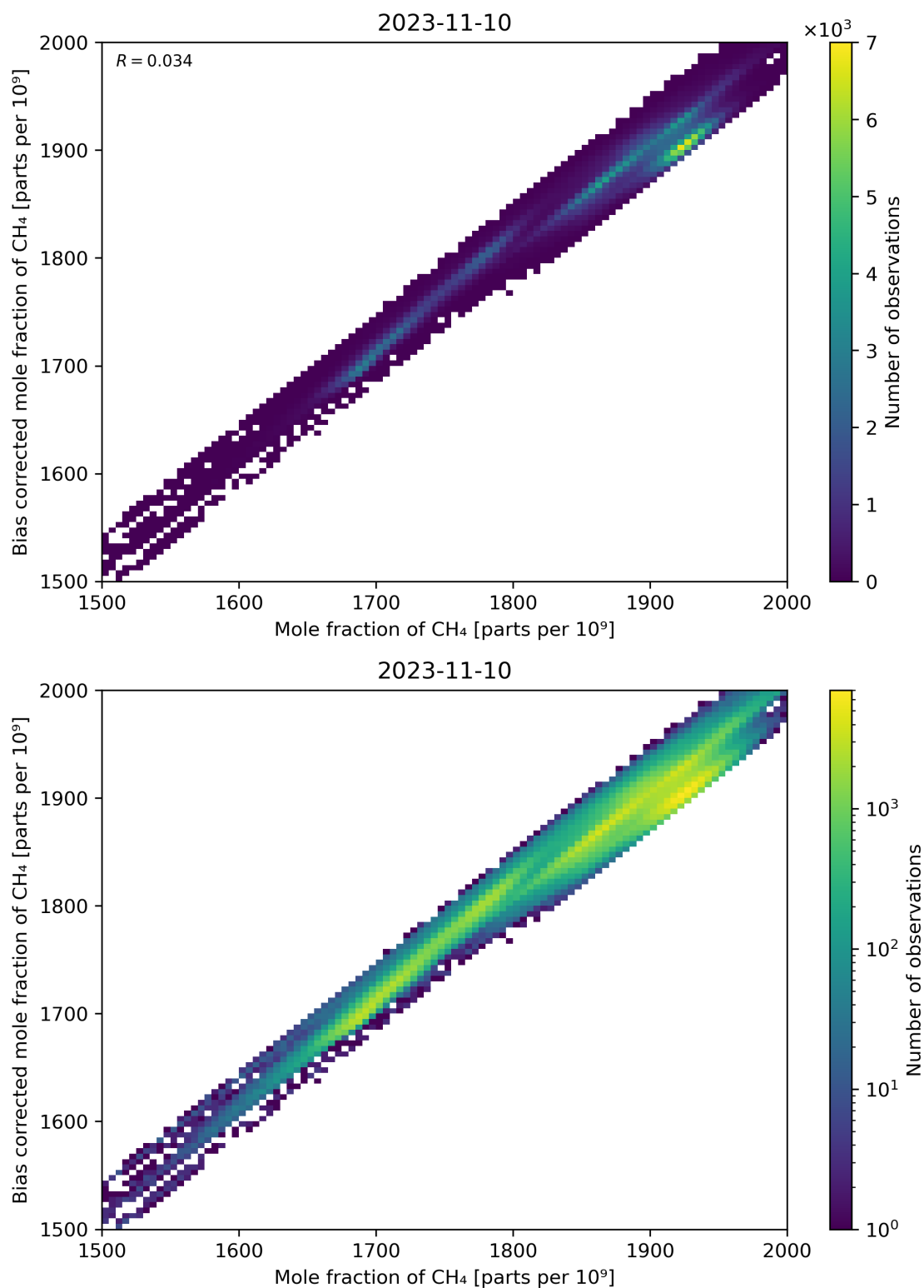
Figure 74: Scatter density plot of “Mole fraction of CH 4 ” against “Bias corrected mole fraction of CH 4 ” for 2023-11-09 to 2023-11-11.
