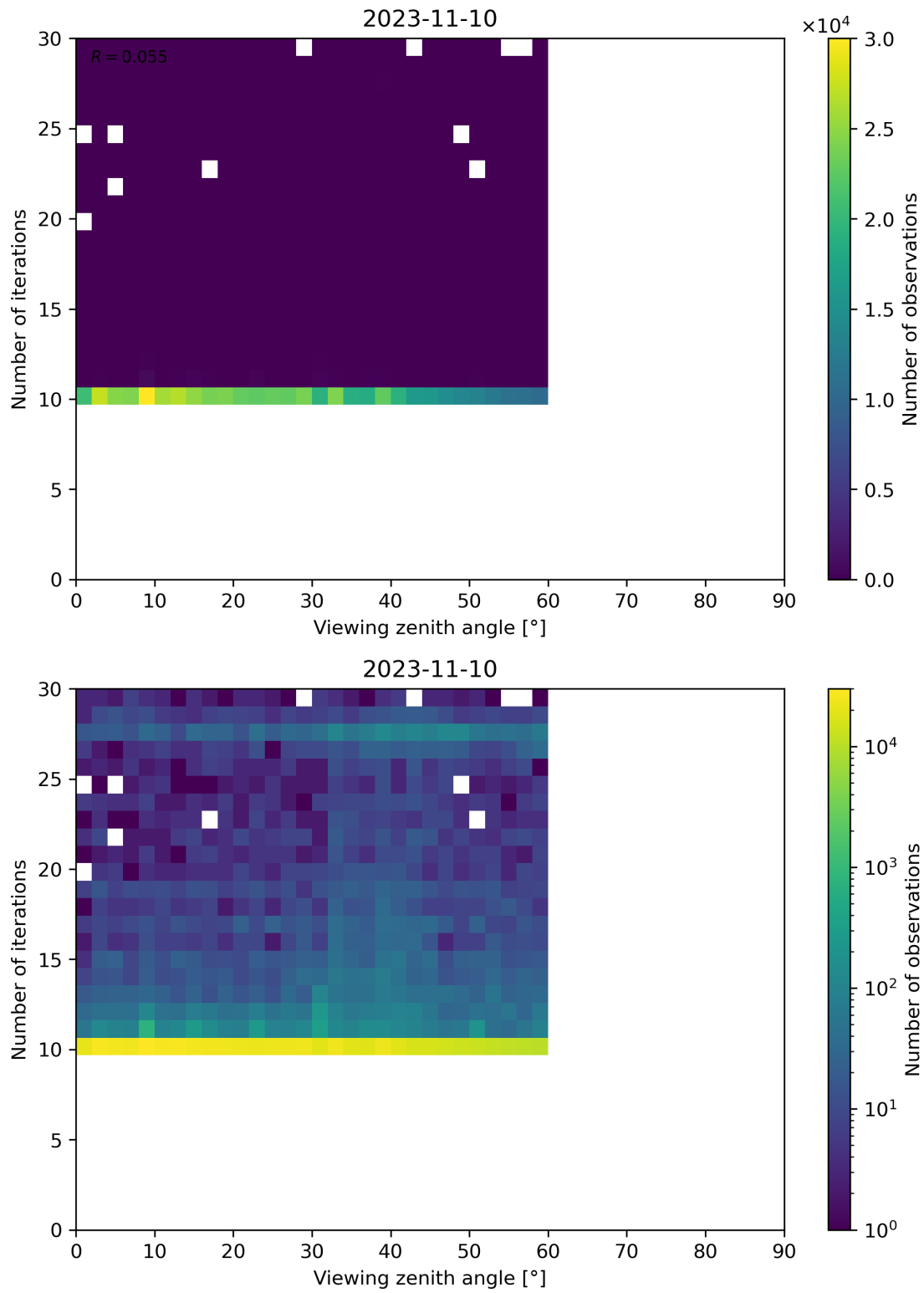
Figure 113: Scatter density plot of “Viewing zenith angle” against “Number of iterations” for 2023-11-09 to 2023-11-11.
