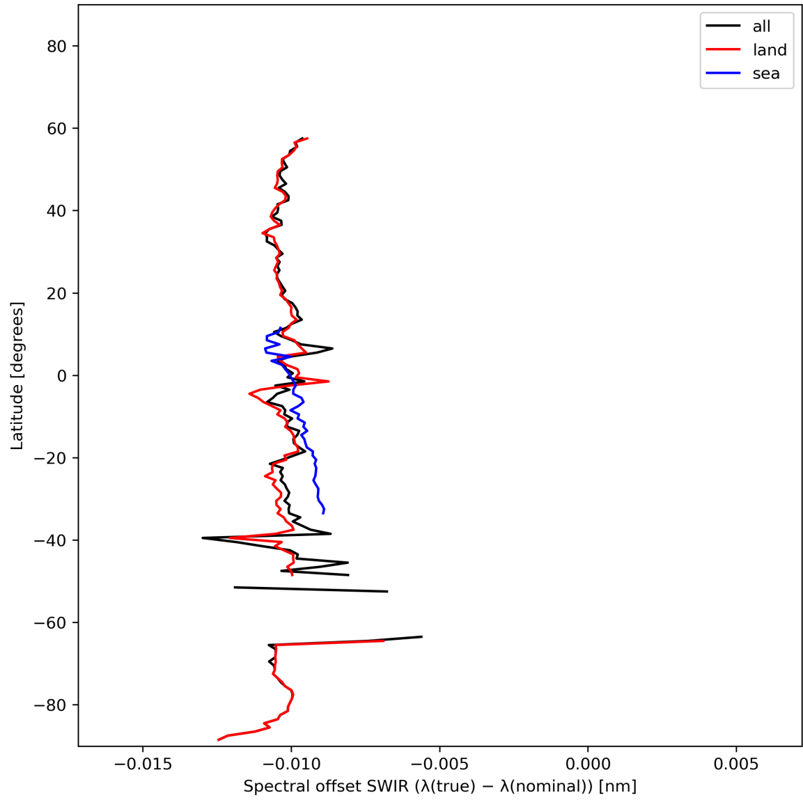
Figure 16: Zonal average of “Spectral offset SWIR ( \lambda(\text{true}) - \lambda(\text{nominal}) )” for 2023-11-09 to 2023-11-11.
