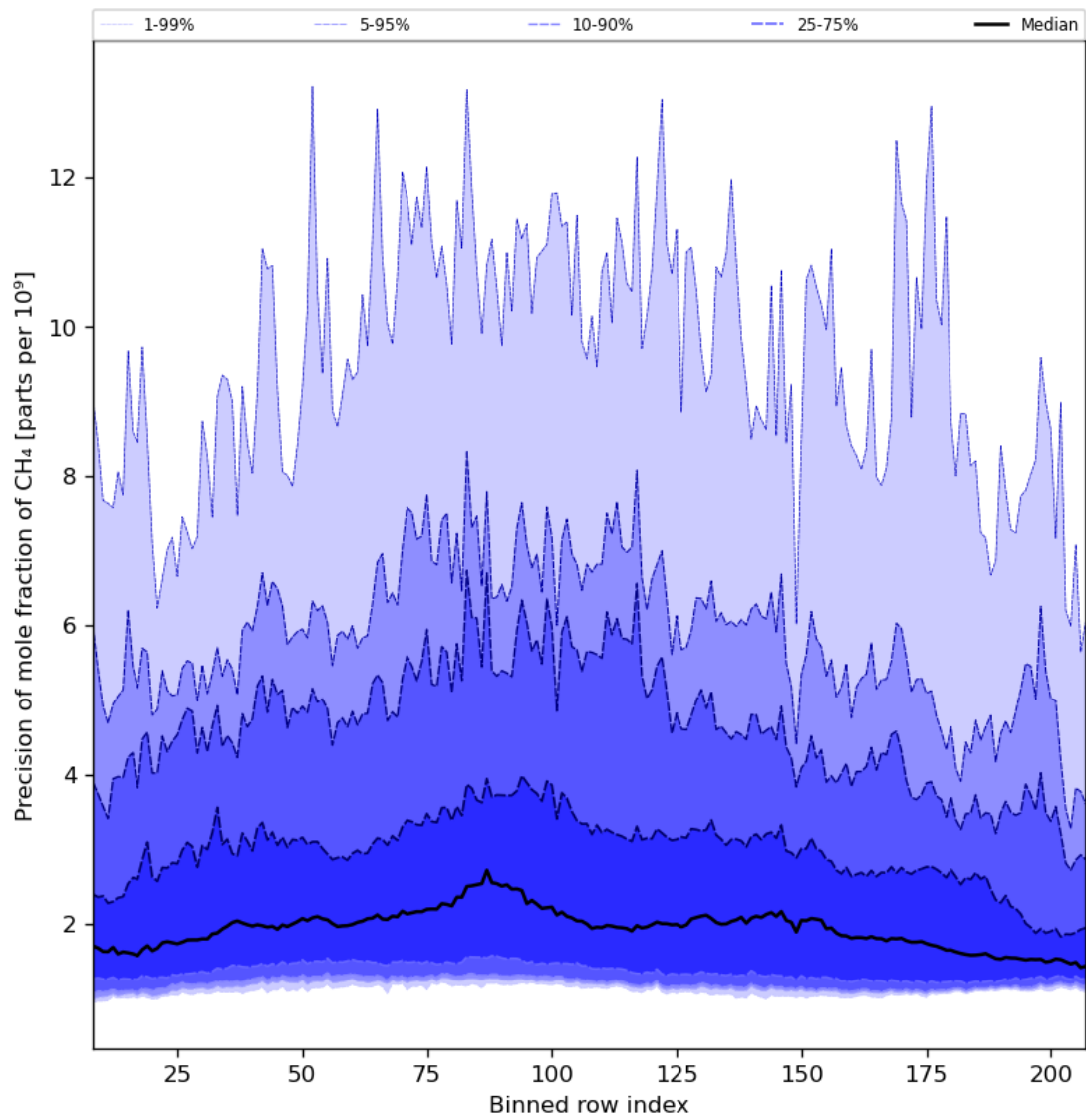
Figure 35: Along track statistics of “Precision of mole fraction of CH 4 ” for 2023-11-09 to 2023-11-11
