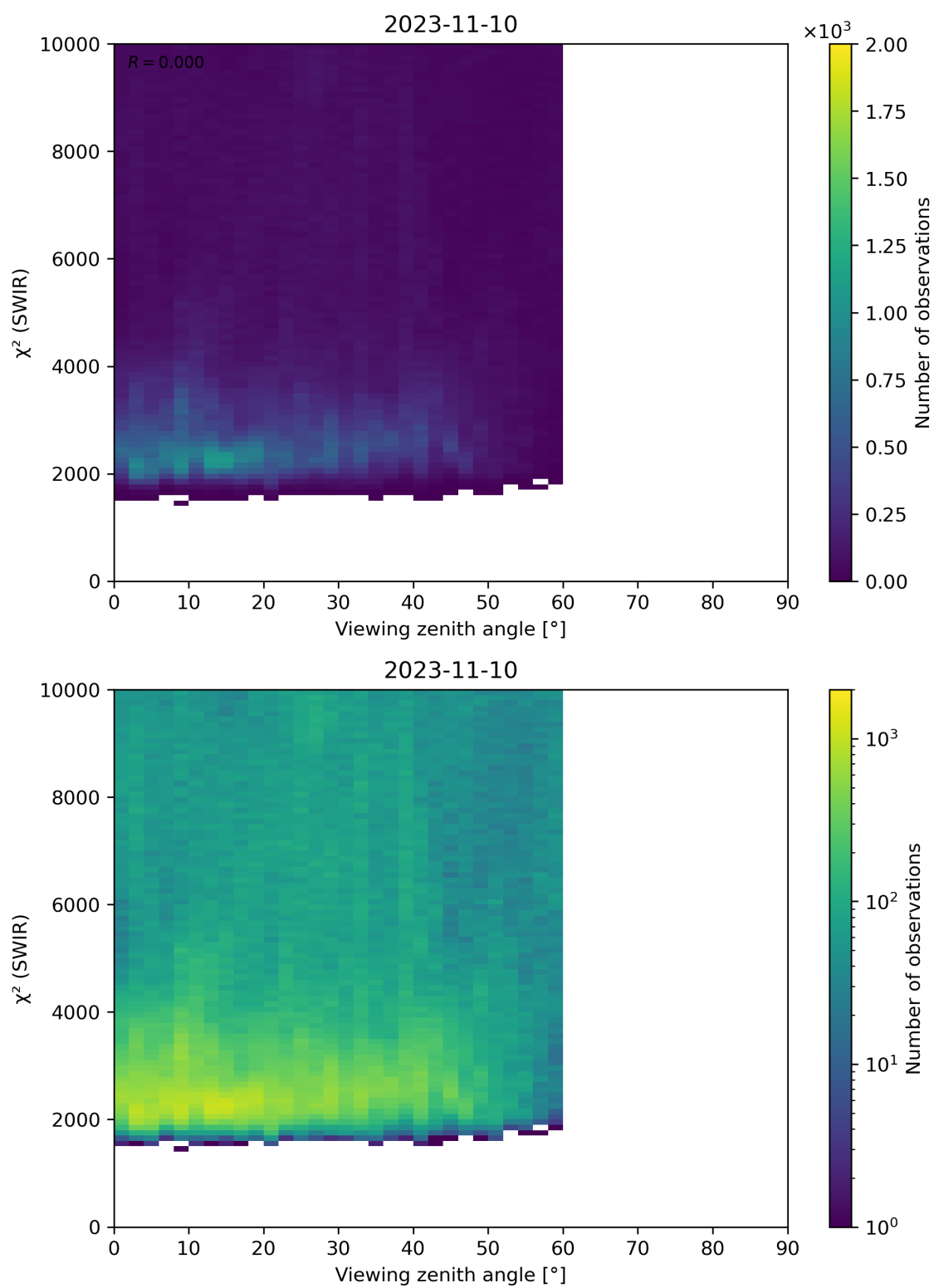
Figure 106: Scatter density plot of “Viewing zenith angle” against “ \chi^2 (SWIR)” for 2023-11-09 to 2023-11-11.
