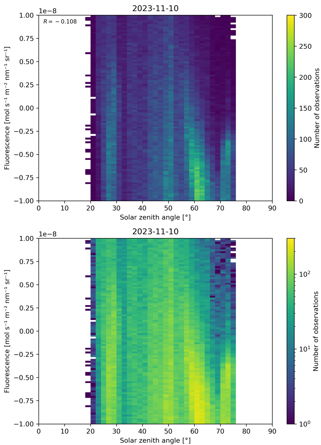
Figure 97: Scatter density plot of “Solar zenith angle” against “Fluorescence” for 2023-11-09 to 2023-11-11.
