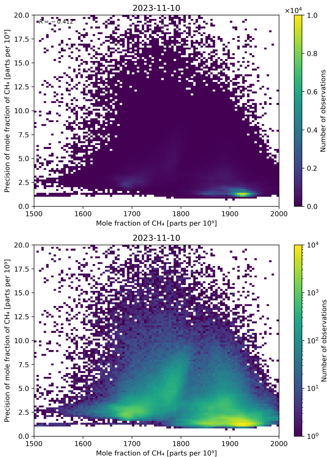
Figure 75: Scatter density plot of “Mole fraction of CH 4 ” against “Precision of mole fraction of CH 4 ” for 2023-11-09 to 2023-11-11.
