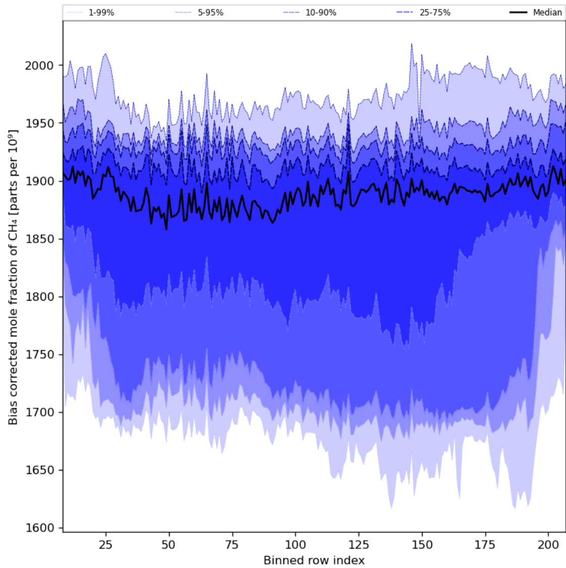
Figure 36: Along track statistics of “Bias corrected mole fraction of CH 4 ” for 2023-11-09 to 2023-11-11
