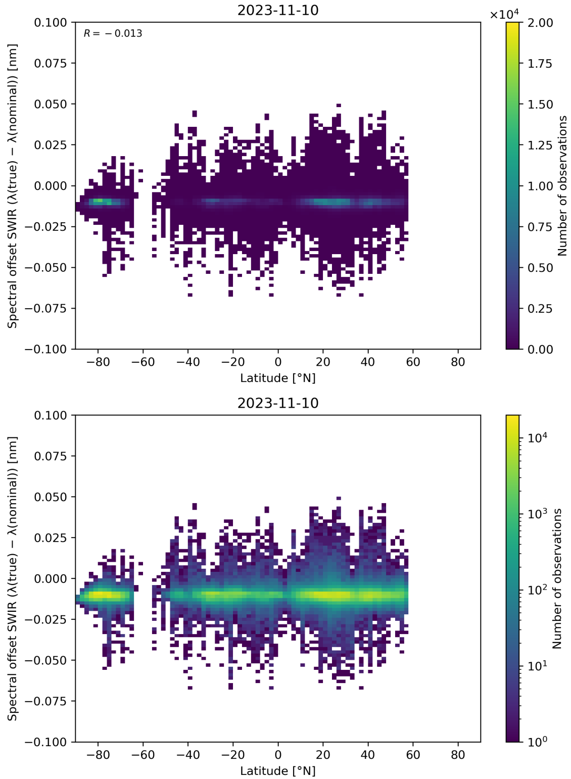
Figure 62: Scatter density plot of “Latitude” against “Spectral offset SWIR ( \lambda(\text{true}) - \lambda(\text{nominal}) )” for 2023-11-09 to 2023-11-11.
