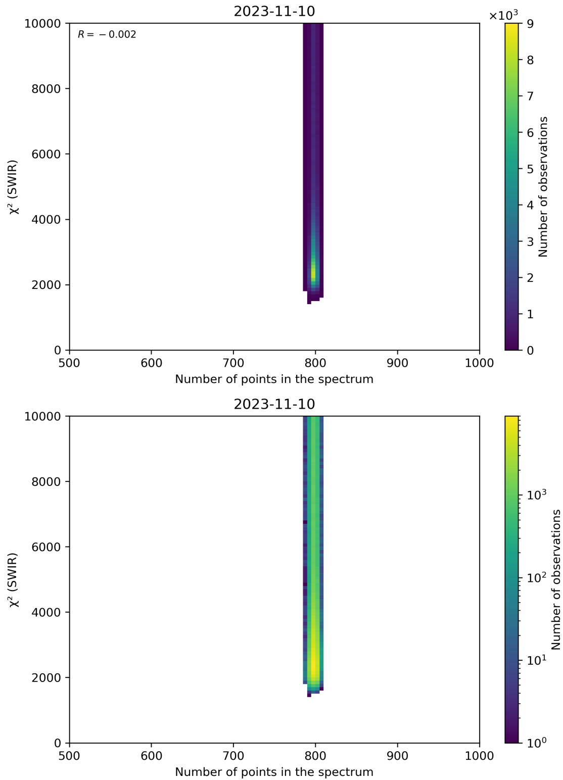
Figure 89: Scatter density plot of “Number of points in the spectrum” against “ \chi^2 (SWIR)” for 2023-11-09 to 2023-11-11.
