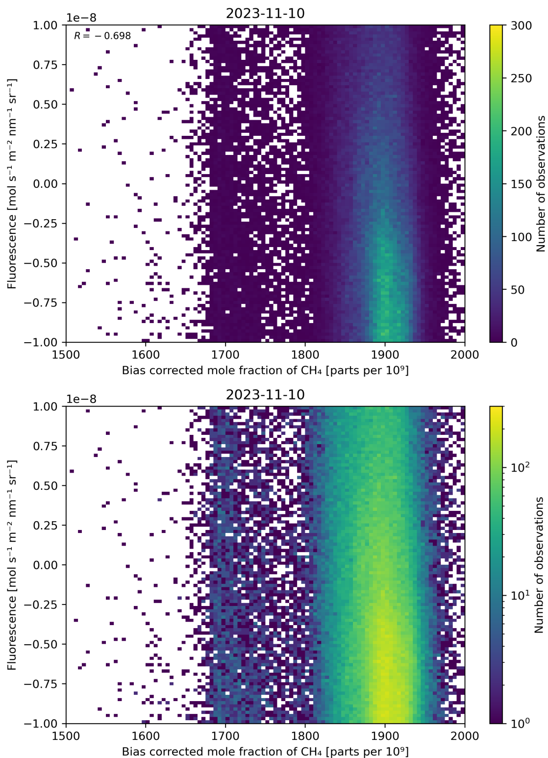
Figure 66: Scatter density plot of “Bias corrected mole fraction of \text{CH}_4 ” against “Fluorescence” for 2023-11-09 to 2023-11-11.
