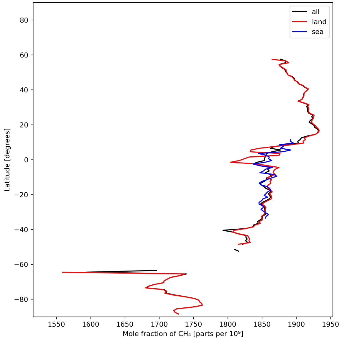
Figure 12: Zonal average of “Mole fraction of CH 4 ” for 2023-11-09 to 2023-11-11.
