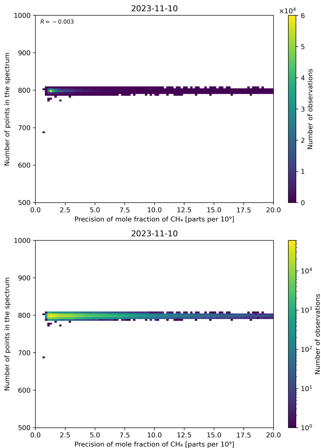
Figure 84: Scatter density plot of “Precision of mole fraction of CH 4 ” against “Number of points in the spectrum” for 2023-11-09 to 2023-11-11.
