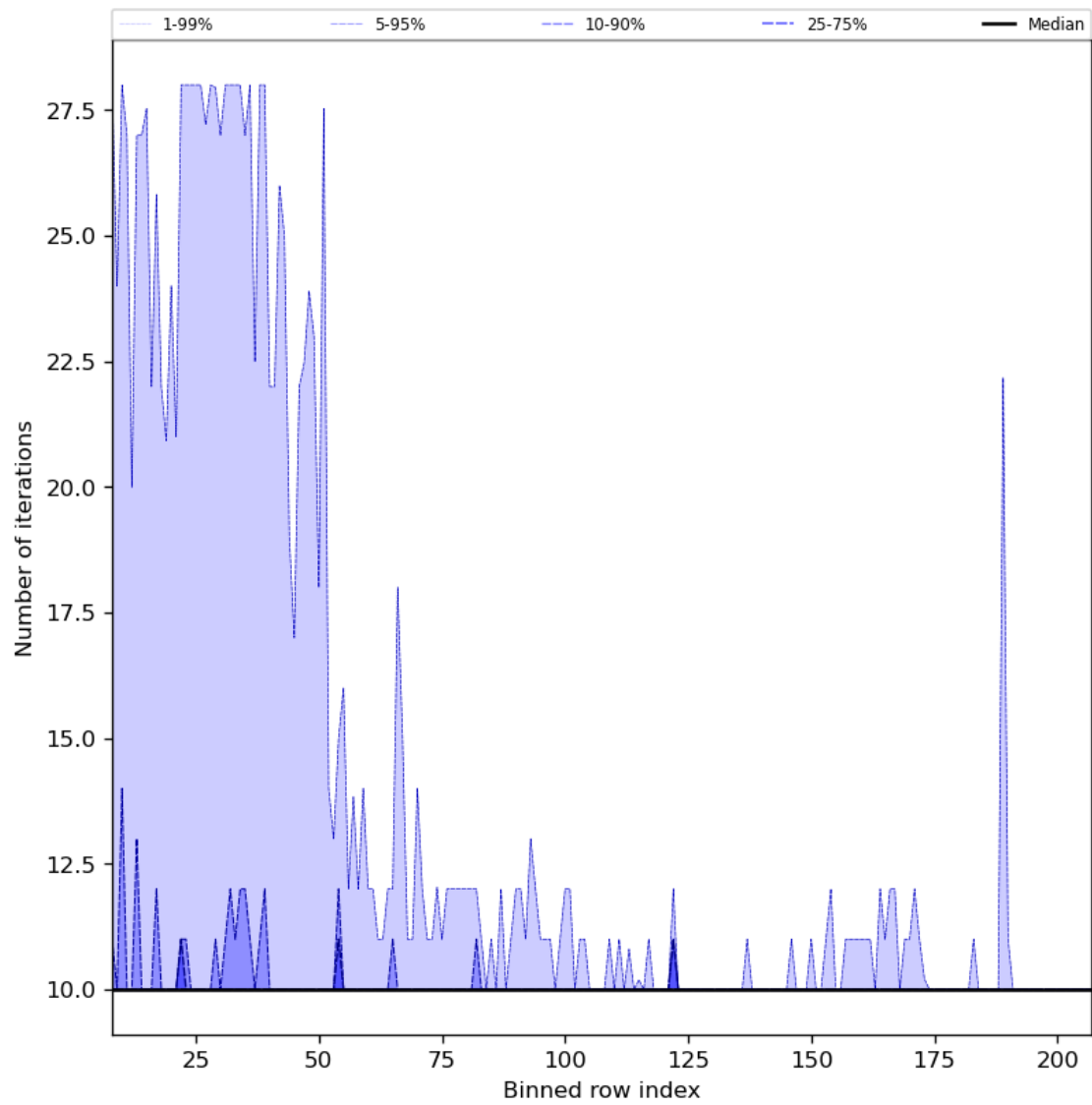
Figure 42: Along track statistics of “Number of iterations” for 2023-11-09 to 2023-11-11
