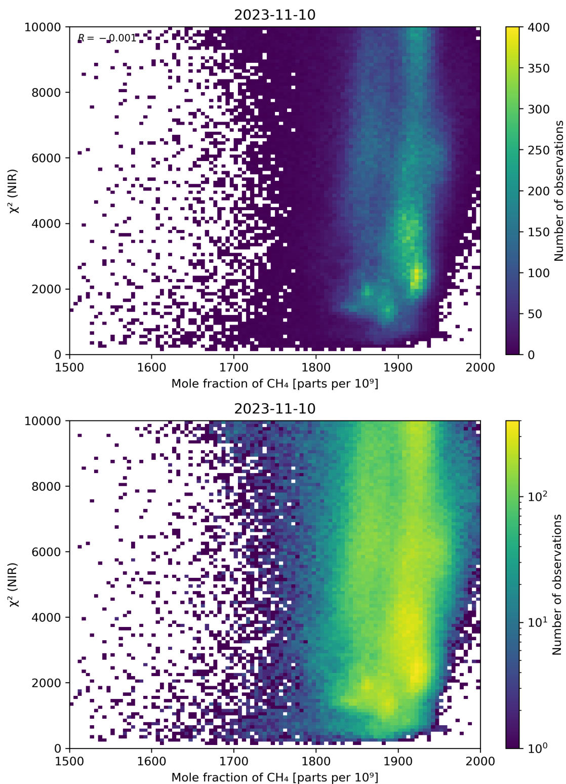
Figure 70: Scatter density plot of “Mole fraction of CH 4 ” against “ \chi^2 (NIR)” for 2023-11-09 to 2023-11-11.
