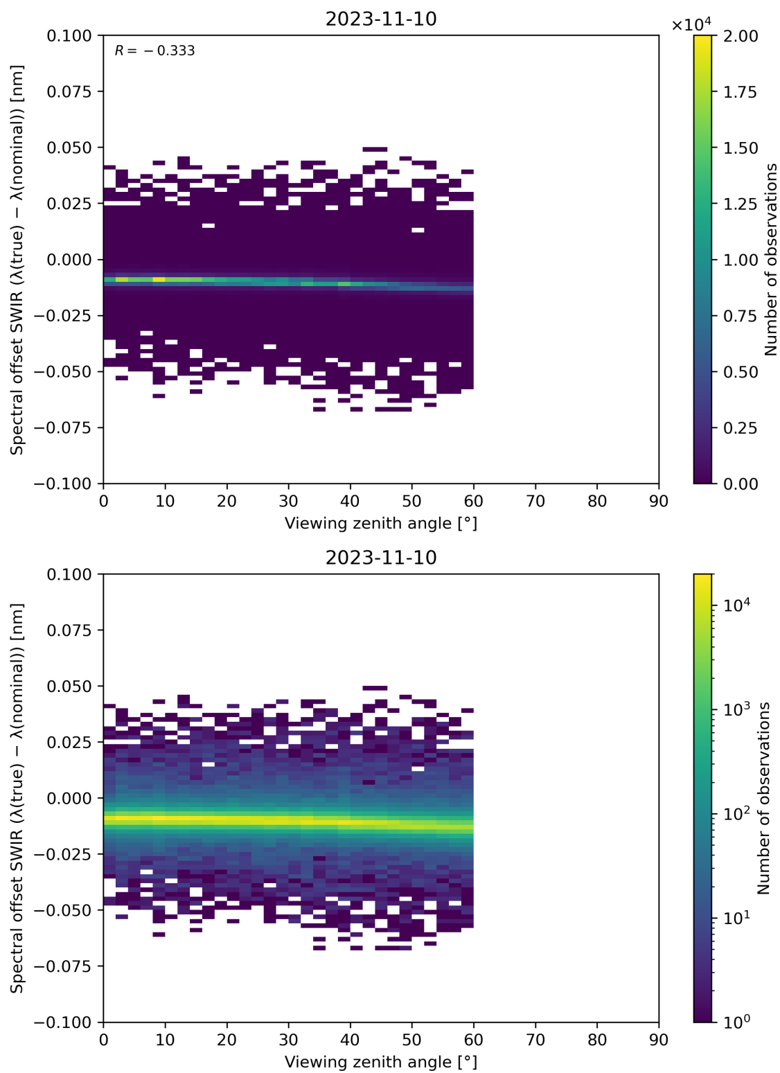
Figure 116: Scatter density plot of “Viewing zenith angle” against “Spectral offset SWIR ( \lambda(\text{true}) - \lambda(\text{nominal}) )” for 2023-11-09 to 2023-11-11.
