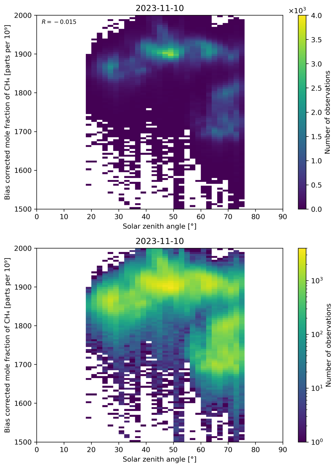
Figure 100: Scatter density plot of “Solar zenith angle” against “Bias corrected mole fraction of \text{CH}_4 ” for 2023-11-09 to 2023-11-11.
