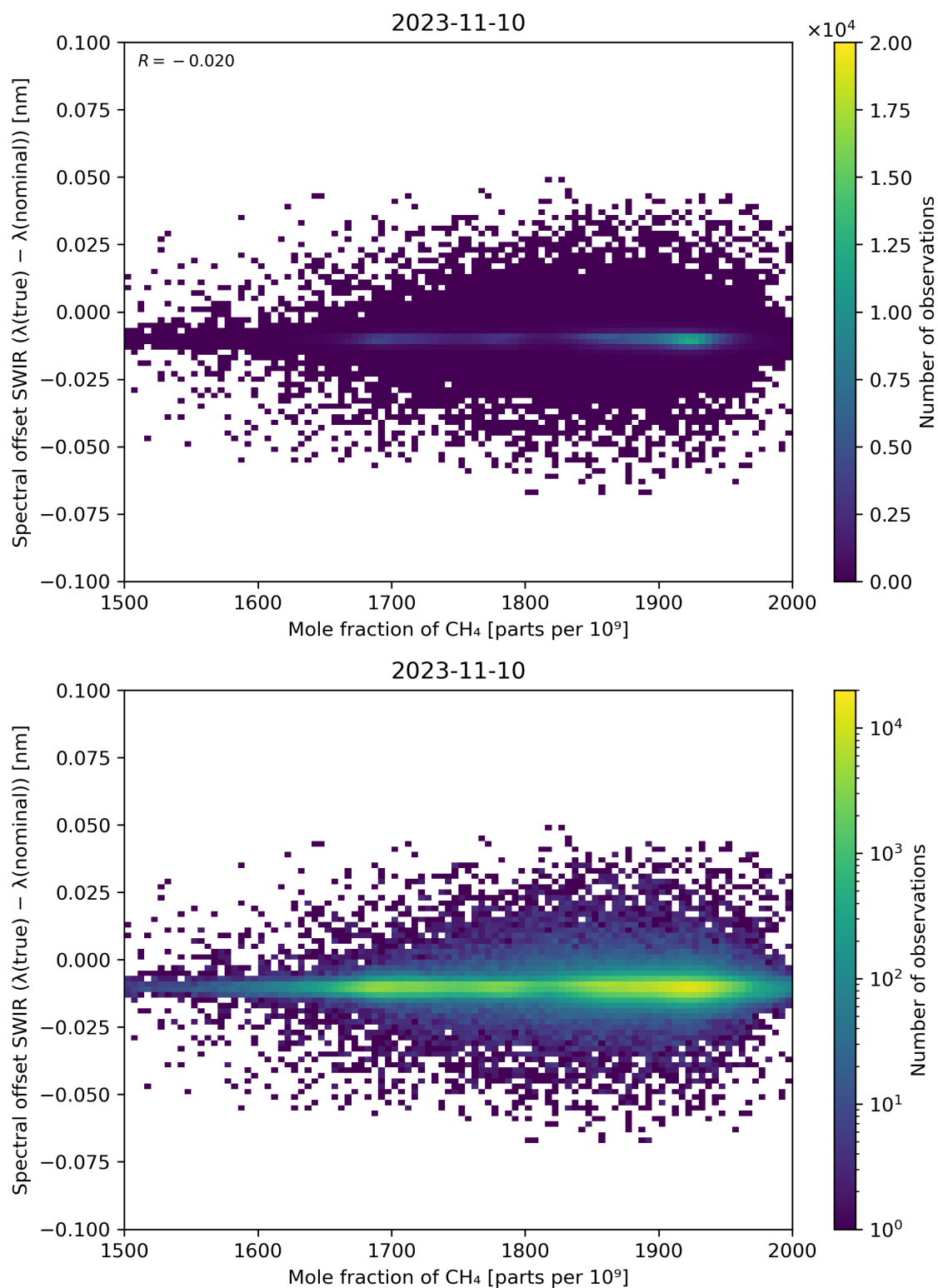
Figure 86: Scatter density plot of “Mole fraction of CH 4 ” against “Spectral offset SWIR ( \lambda(\text{true}) - \lambda(\text{nominal}) )” for 2023-11-09 to 2023-11-11.
