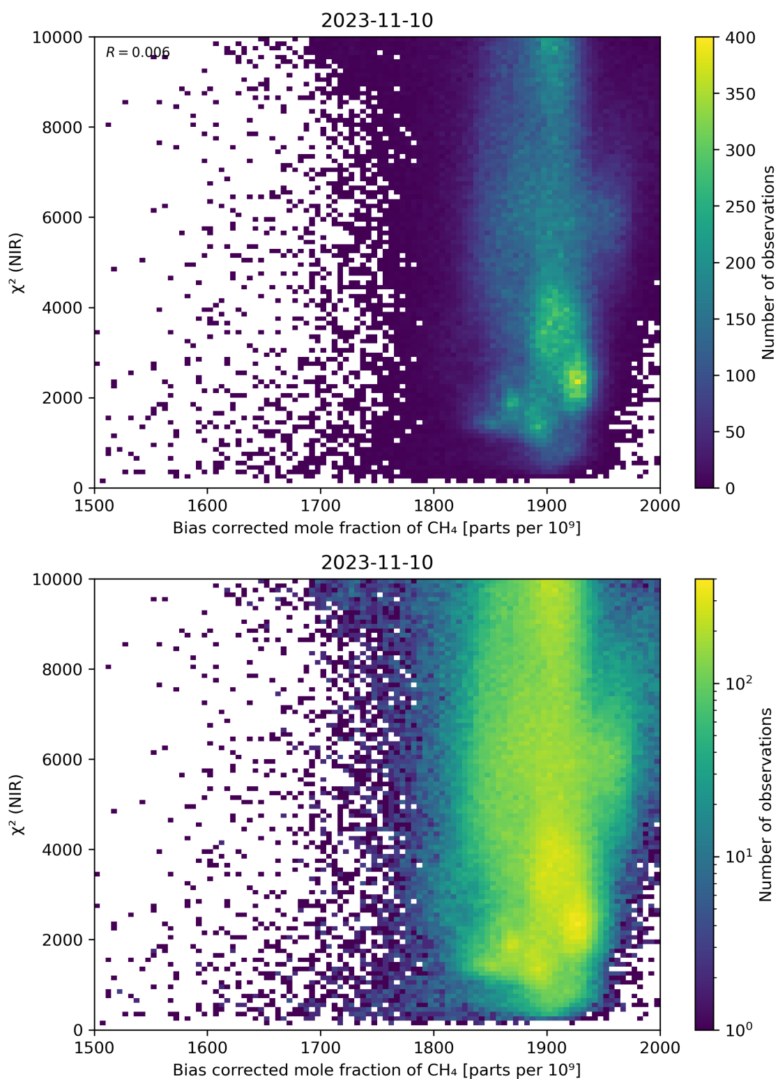
Figure 63: Scatter density plot of “Bias corrected mole fraction of CH 4 ” against “ \chi^2 (NIR)” for 2023-11-09 to 2023-11-11.
