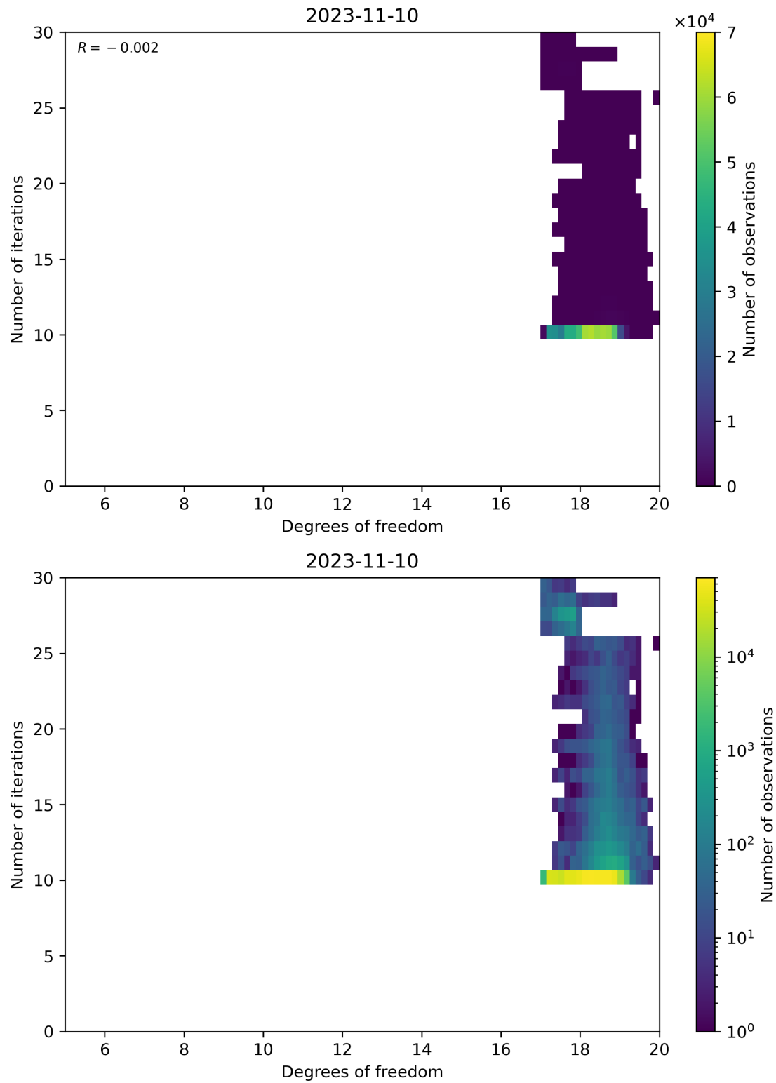
Figure 52: Scatter density plot of “Degrees of freedom” against “Number of iterations” for 2023-11-09 to 2023-11-11.
