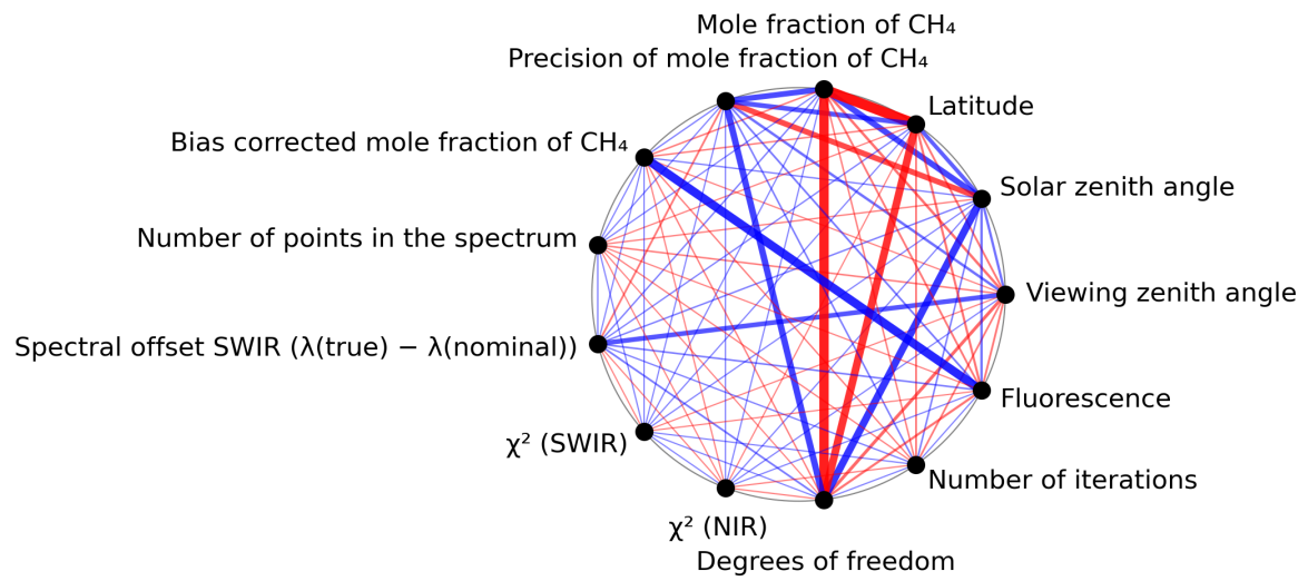
Figure 1: Map of correlation graph for 2023-11-09 to 2023-11-11.
