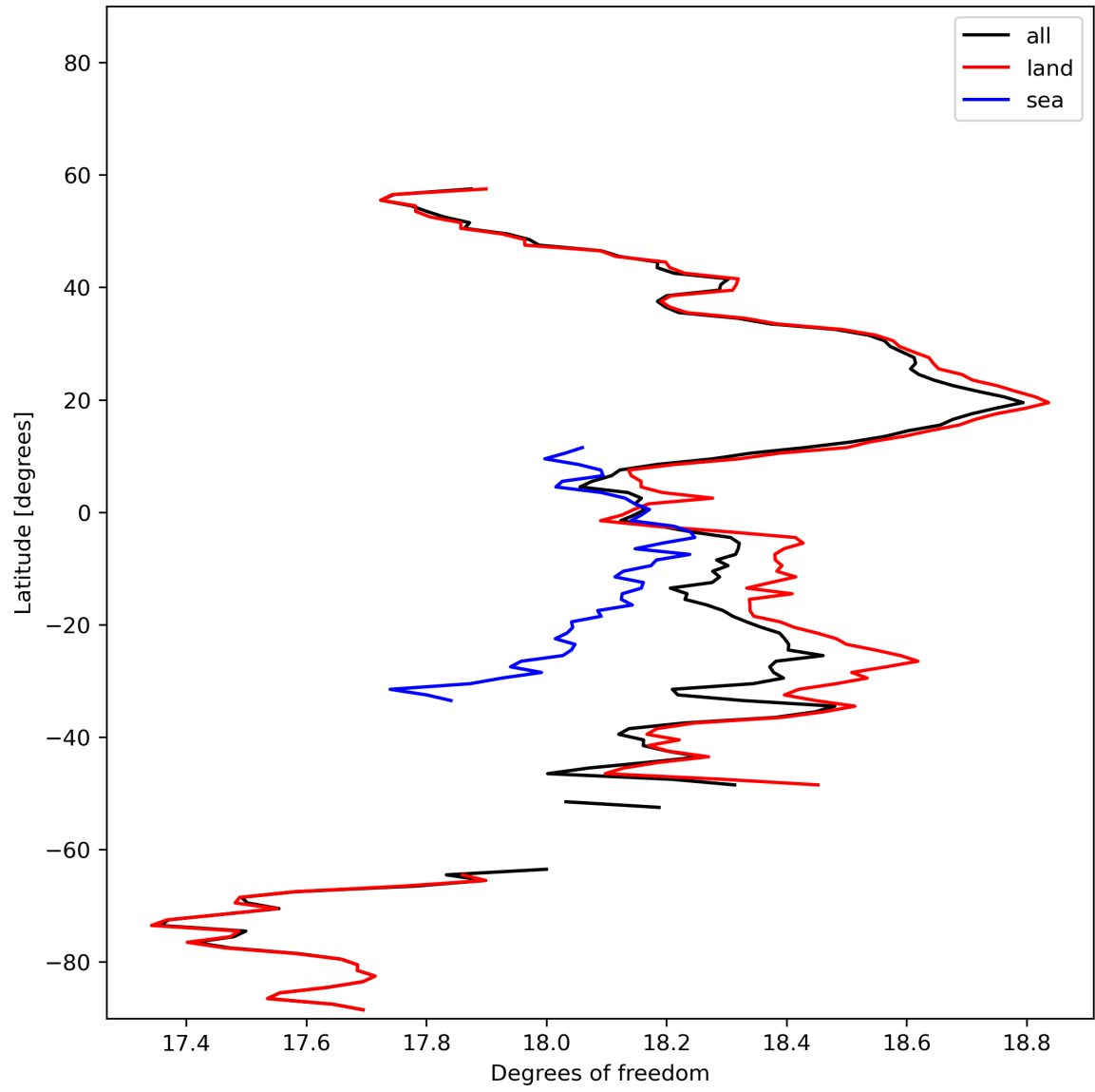
Figure 19: Zonal average of “Degrees of freedom” for 2023-11-09 to 2023-11-11.
