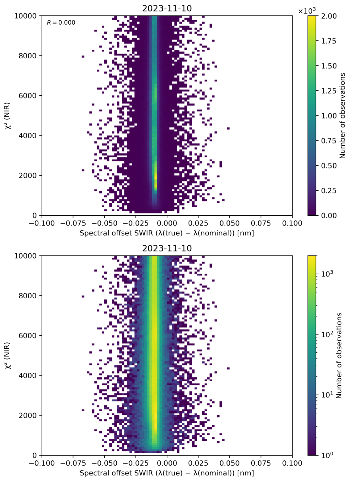
Figure 117: Scatter density plot of “Spectral offset SWIR ( \lambda(\text{true}) - \lambda(\text{nominal}) )” against “ \chi^2 (NIR)” for 2023-11-09 to 2023-11-11.
