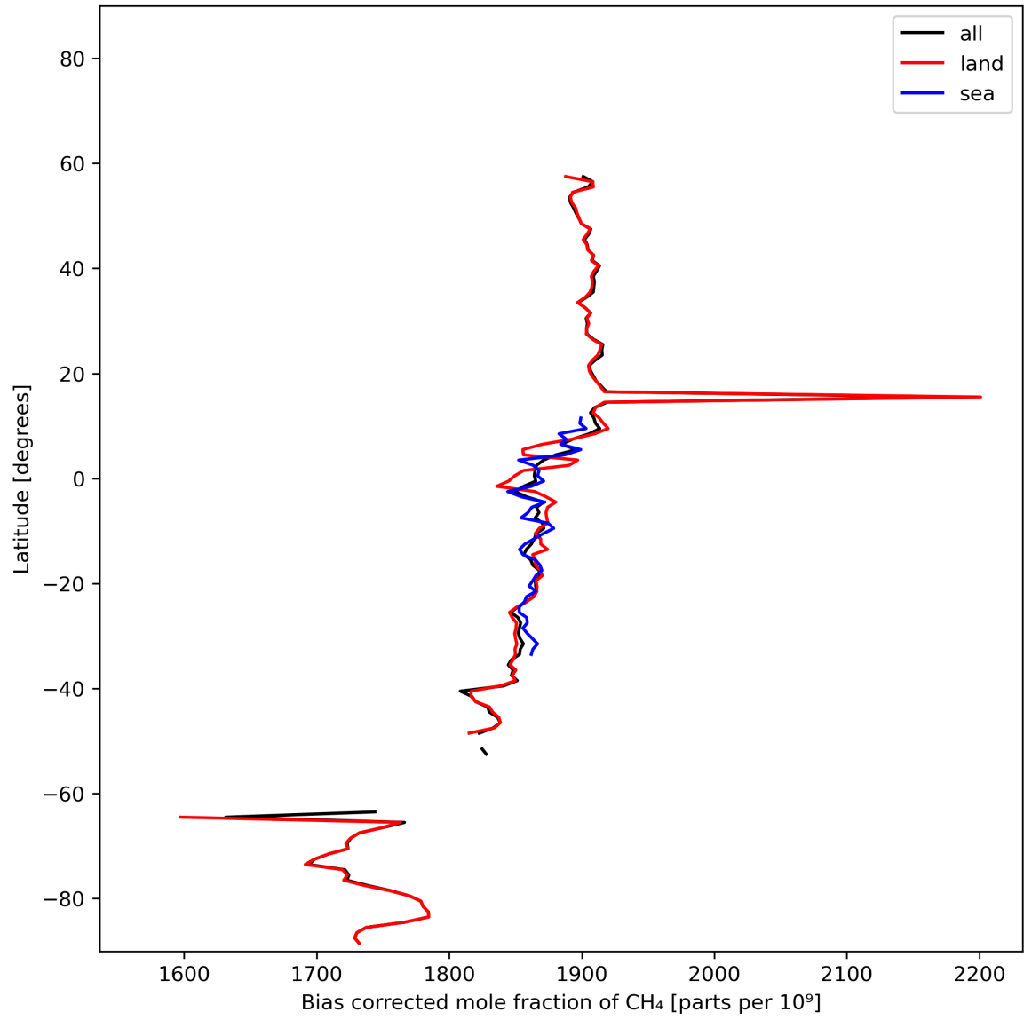
Figure 14: Zonal average of “Bias corrected mole fraction of CH 4 ” for 2023-11-09 to 2023-11-11.
