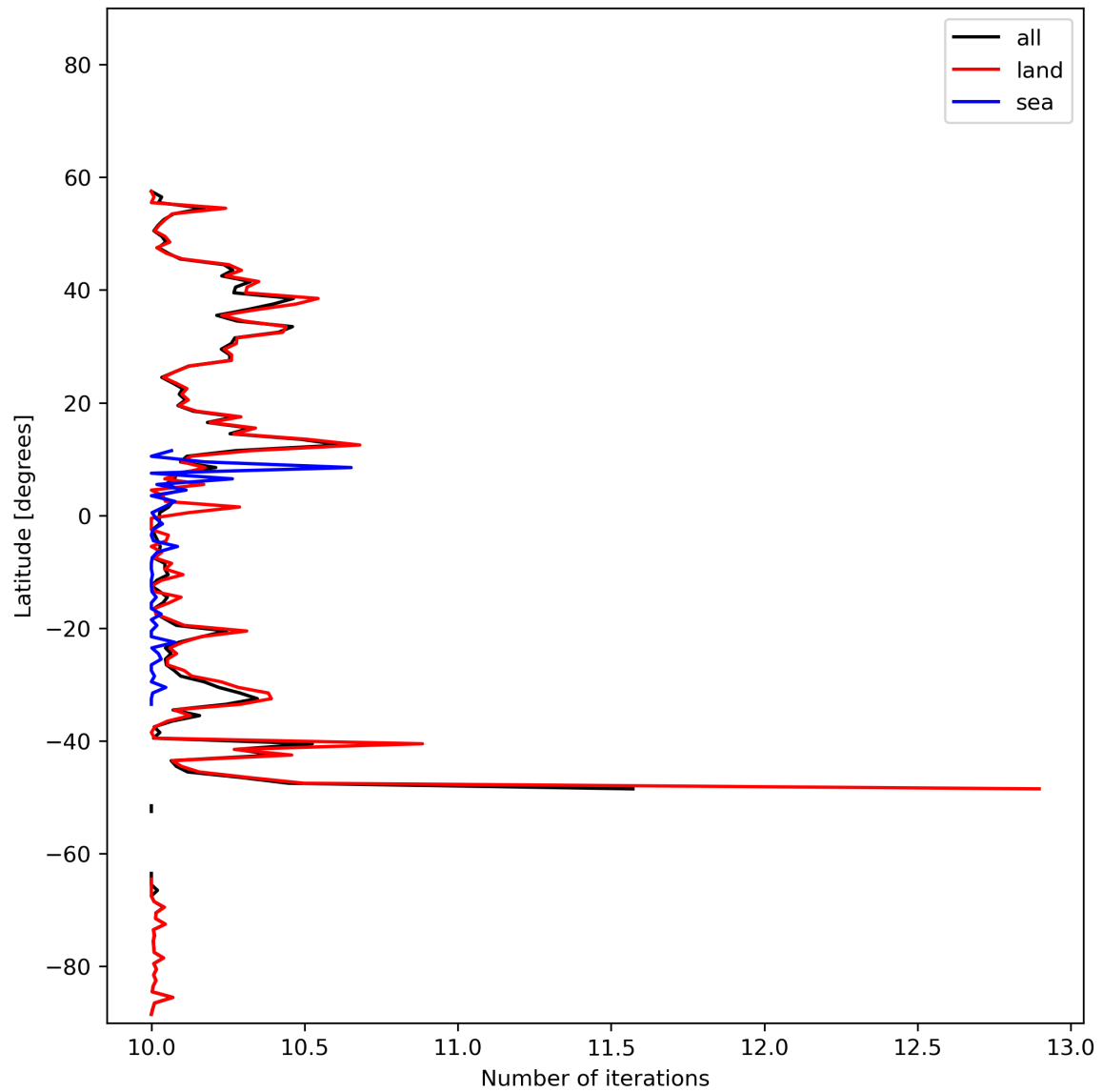
Figure 20: Zonal average of “Number of iterations” for 2023-11-09 to 2023-11-11.
