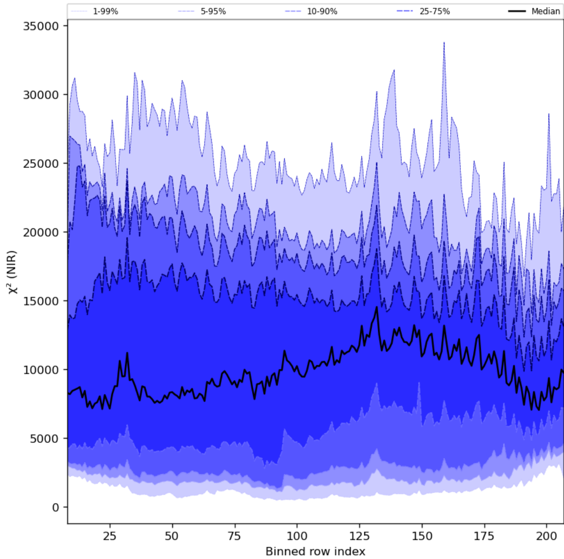
Figure 40: Along track statistics of “ \chi^2 (NIR)” for 2023-11-09 to 2023-11-11
