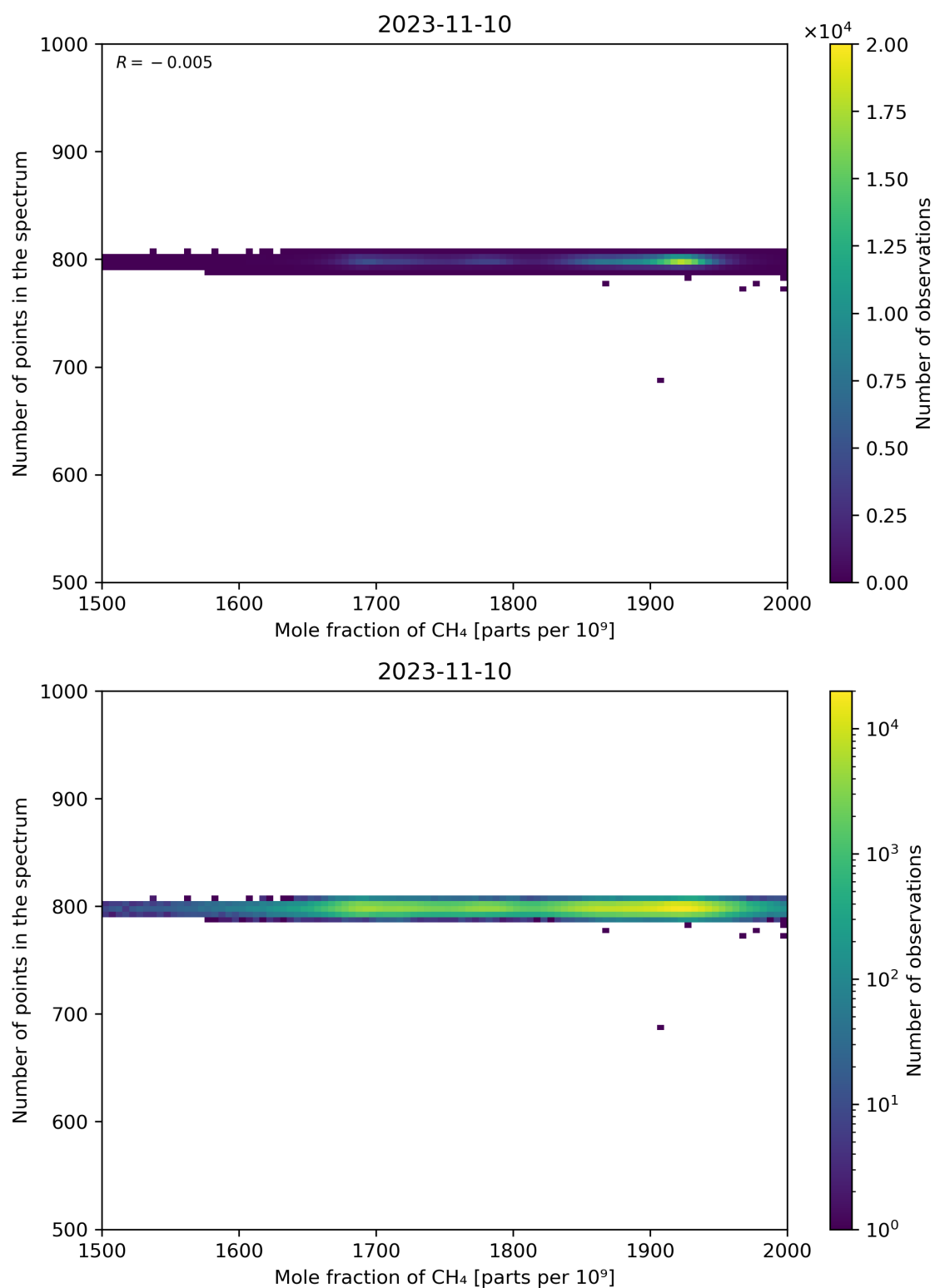
Figure 77: Scatter density plot of “Mole fraction of CH 4 ” against “Number of points in the spectrum” for 2023-11-09 to 2023-11-11.
