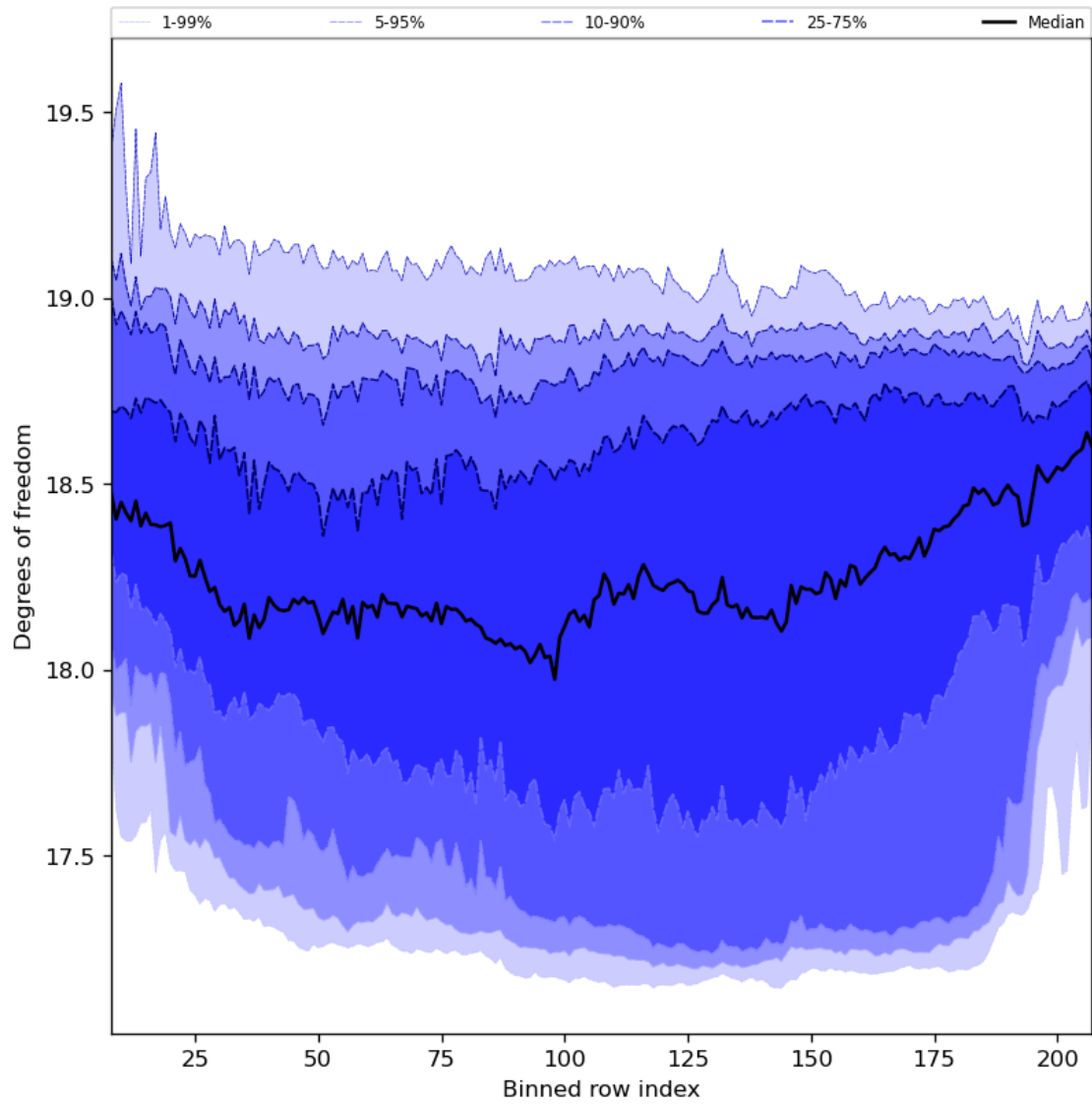
Figure 41: Along track statistics of “Degrees of freedom” for 2023-11-09 to 2023-11-11
