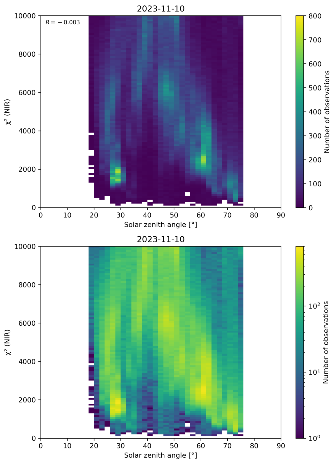
Figure 94: Scatter density plot of “Solar zenith angle” against “ \chi^2 (NIR)” for 2023-11-09 to 2023-11-11.
