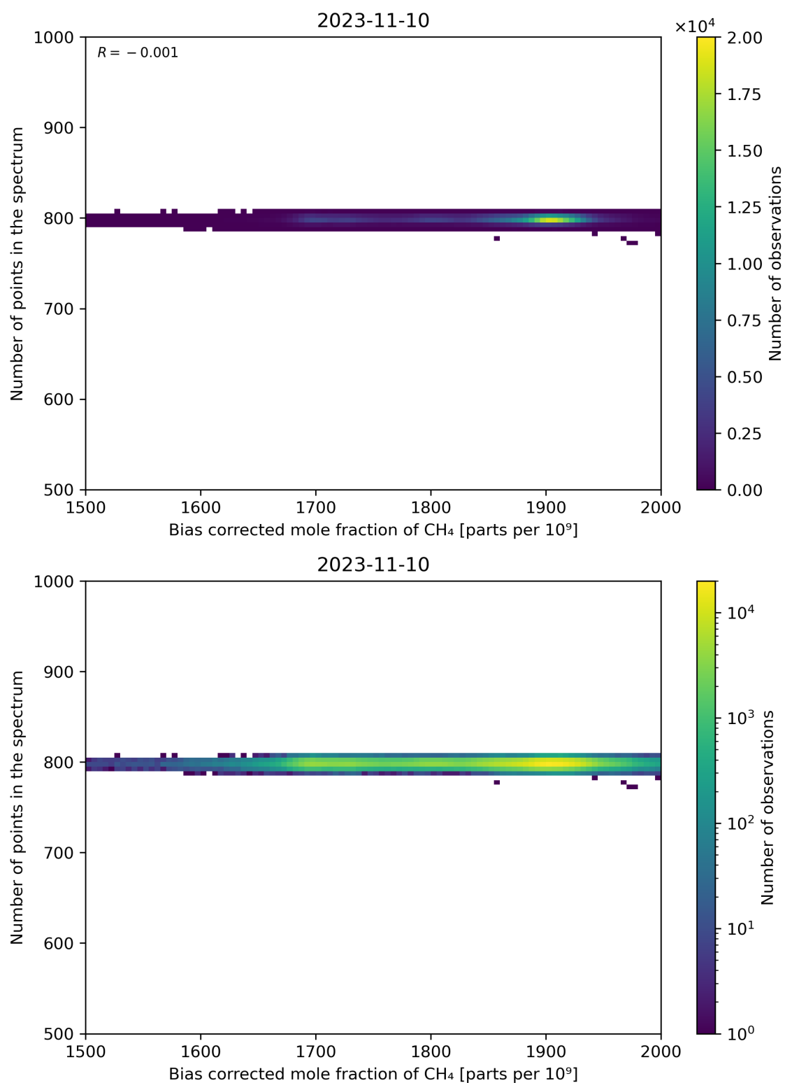
Figure 68: Scatter density plot of “Bias corrected mole fraction of CH 4 ” against “Number of points in the spectrum” for 2023-11-09 to 2023-11-11.
