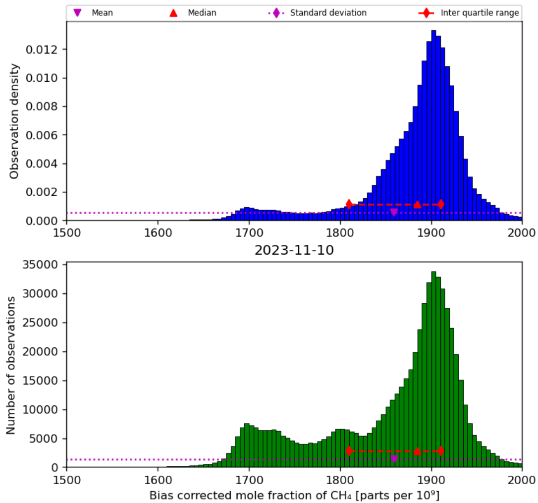
Figure 25: Histogram of “Bias corrected mole fraction of CH 4 ” for 2023-11-09 to 2023-11-11
