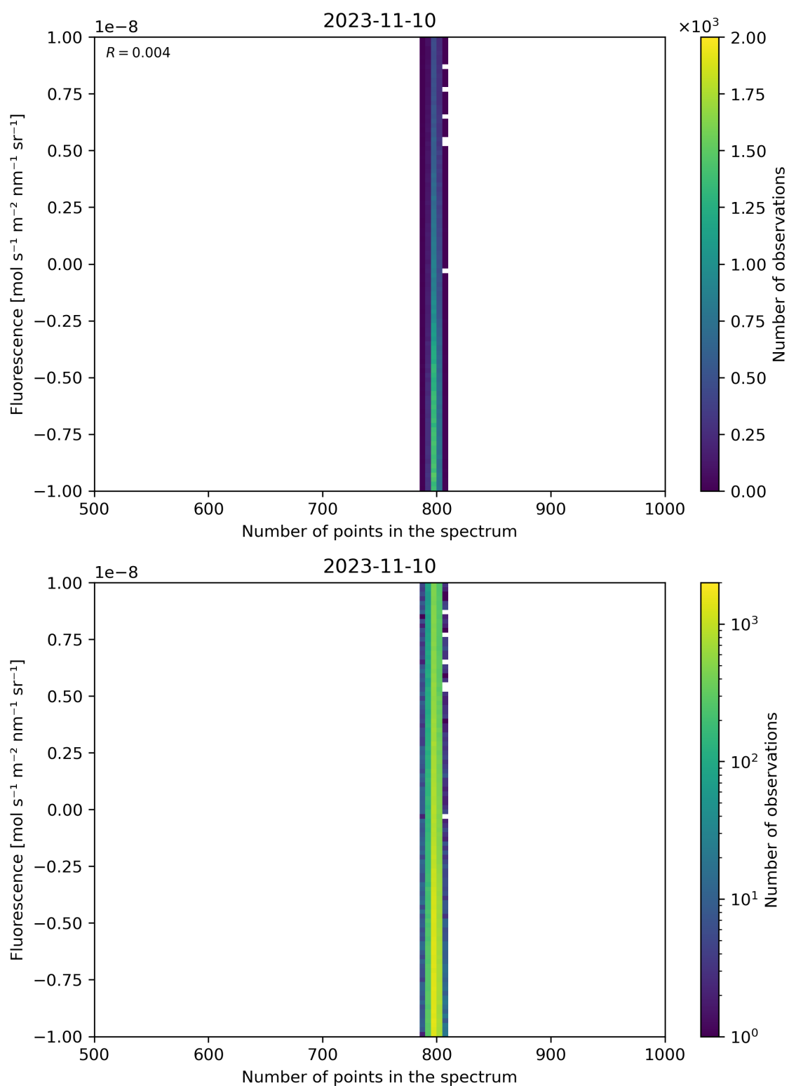
Figure 91: Scatter density plot of “Number of points in the spectrum” against “Fluorescence” for 2023-11-09 to 2023-11-11.
