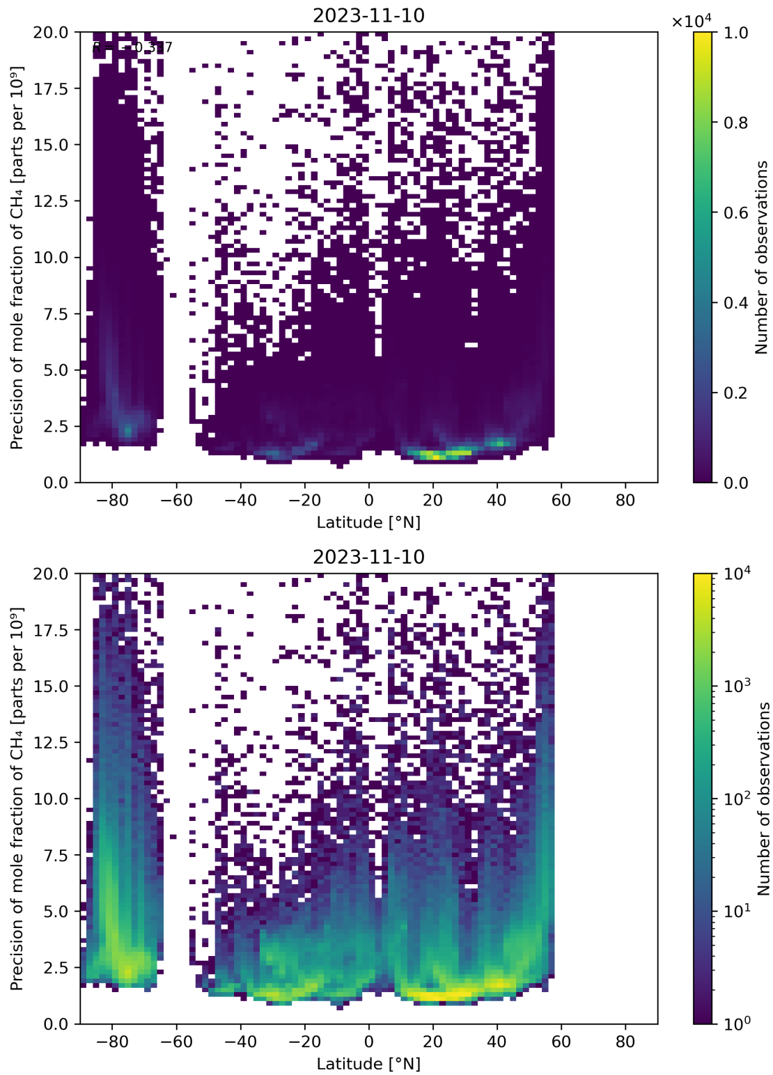
Figure 59: Scatter density plot of “Latitude” against “Precision of mole fraction of CH 4 ” for 2023-11-09 to 2023-11-11.
