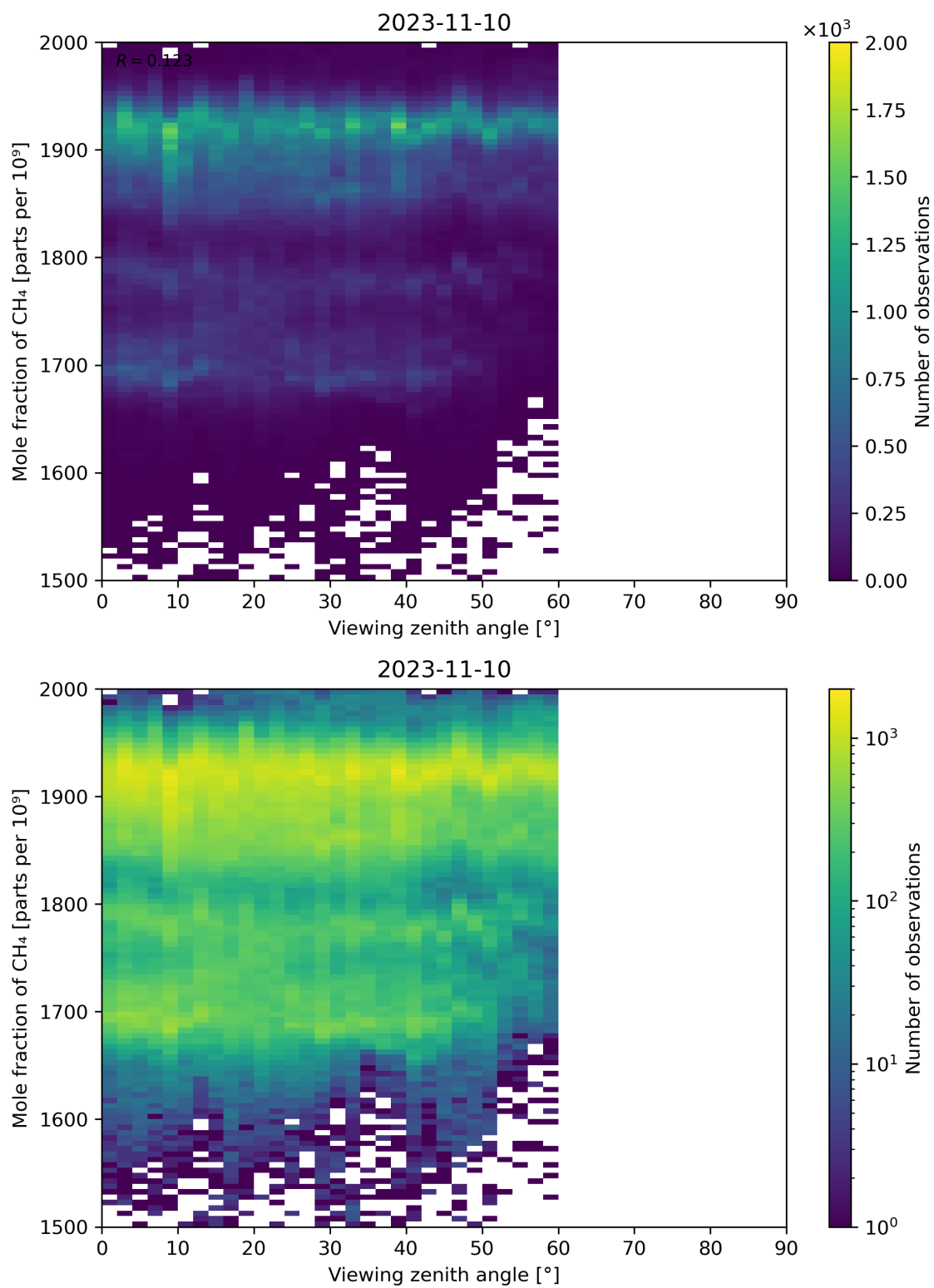
Figure 110: Scatter density plot of “Viewing zenith angle” against “Mole fraction of CH 4 ” for 2023-11-09 to 2023-11-11.
