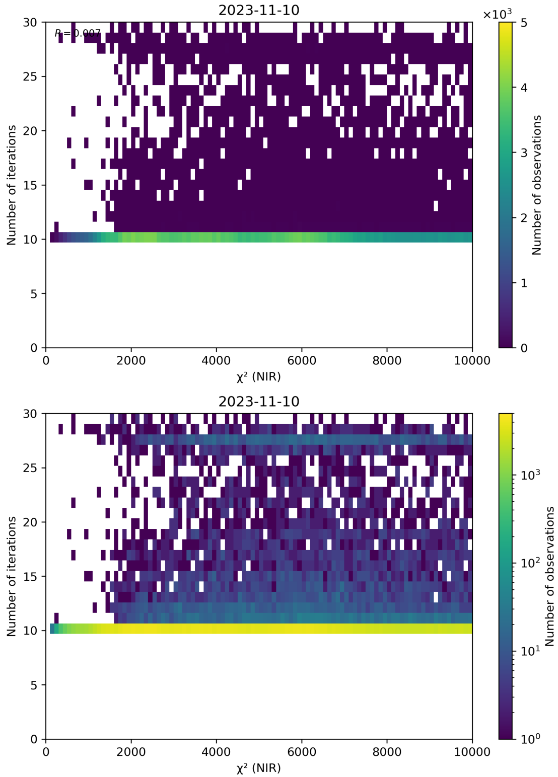
Figure 46: Scatter density plot of “ \chi^2 (NIR)” against “Number of iterations” for 2023-11-09 to 2023-11-11.
