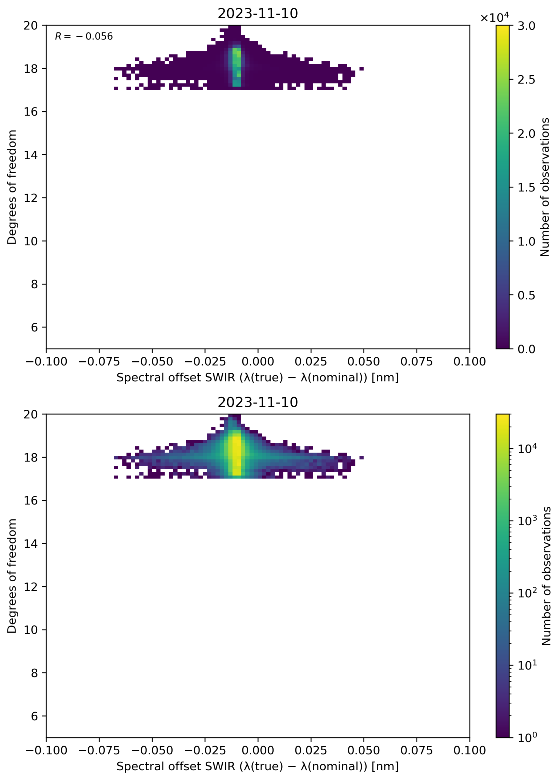
Figure 119: Scatter density plot of “Spectral offset SWIR ( \lambda(\text{true}) - \lambda(\text{nominal}) )” against “Degrees of freedom” for 2023-11-09 to 2023-11-11.
