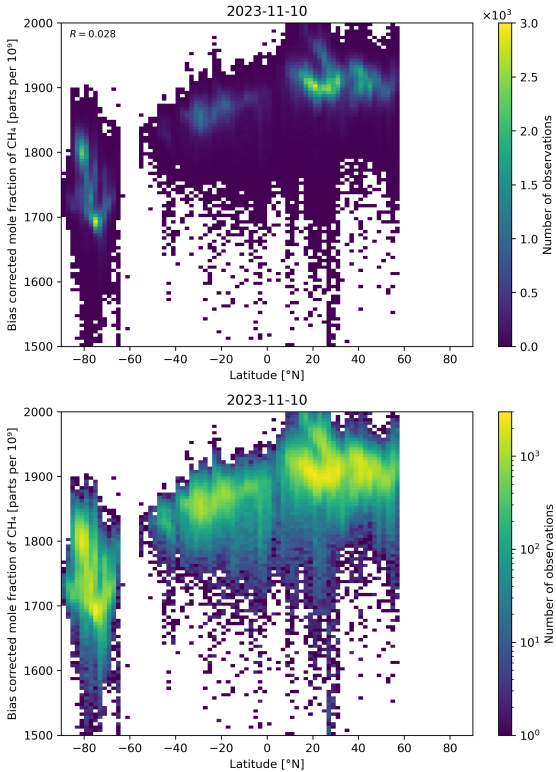
Figure 58: Scatter density plot of “Latitude” against “Bias corrected mole fraction of \text{CH}_4 ” for 2023-11-09 to 2023-11-11.
