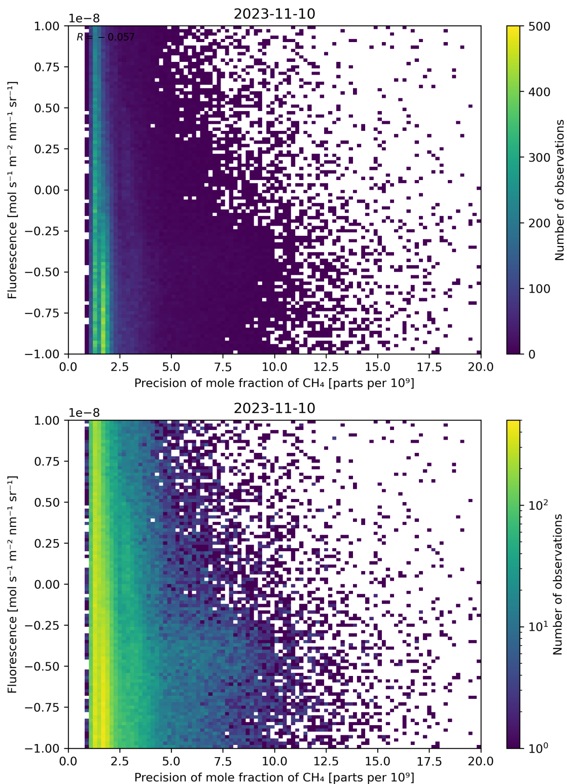
Figure 81: Scatter density plot of “Precision of mole fraction of \text{CH}_4 ” against “Fluorescence” for 2023-11-09 to 2023-11-11.
