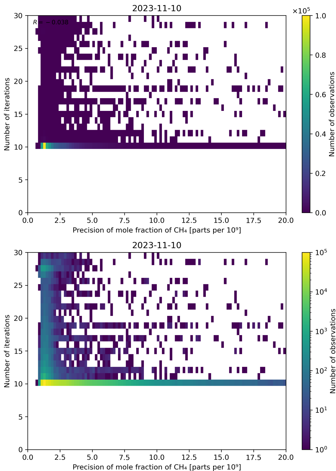
Figure 83: Scatter density plot of “Precision of mole fraction of CH 4 ” against “Number of iterations” for 2023-11-09 to 2023-11-11.
