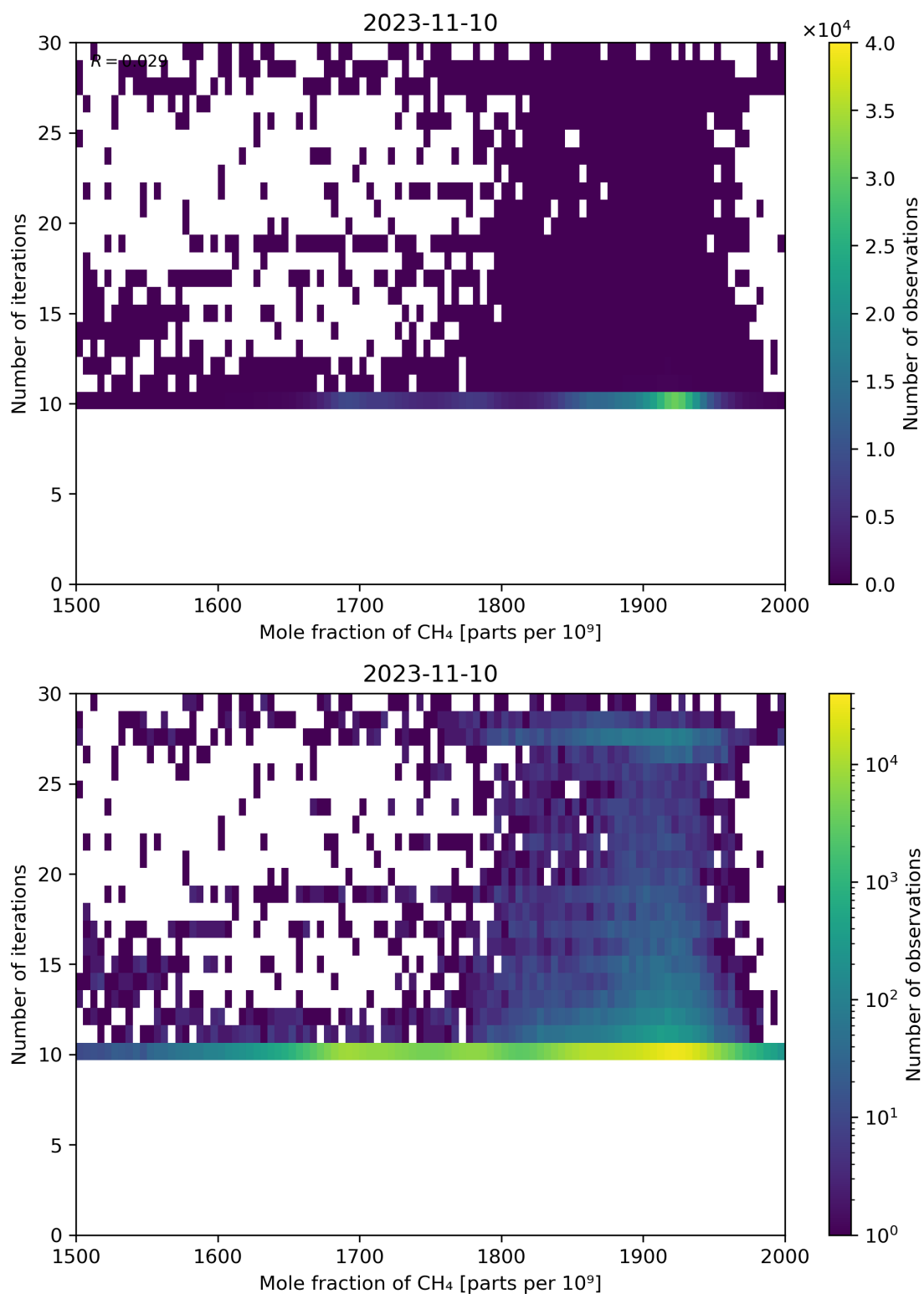
Figure 76: Scatter density plot of “Mole fraction of CH 4 ” against “Number of iterations” for 2023-11-09 to 2023-11-11.
