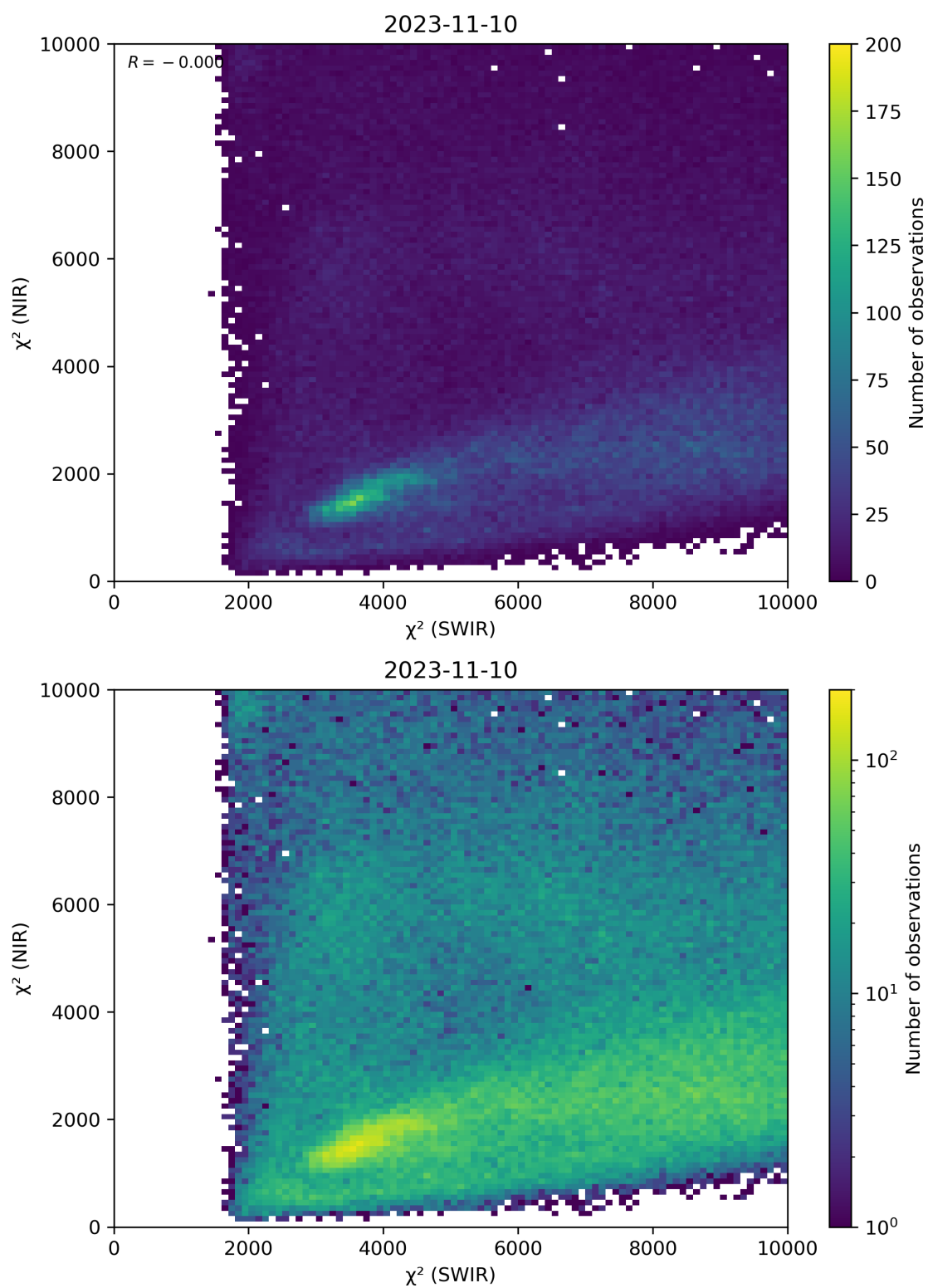
Figure 47: Scatter density plot of “ \chi^2 (SWIR)” against “ \chi^2 (NIR)” for 2023-11-09 to 2023-11-11.
