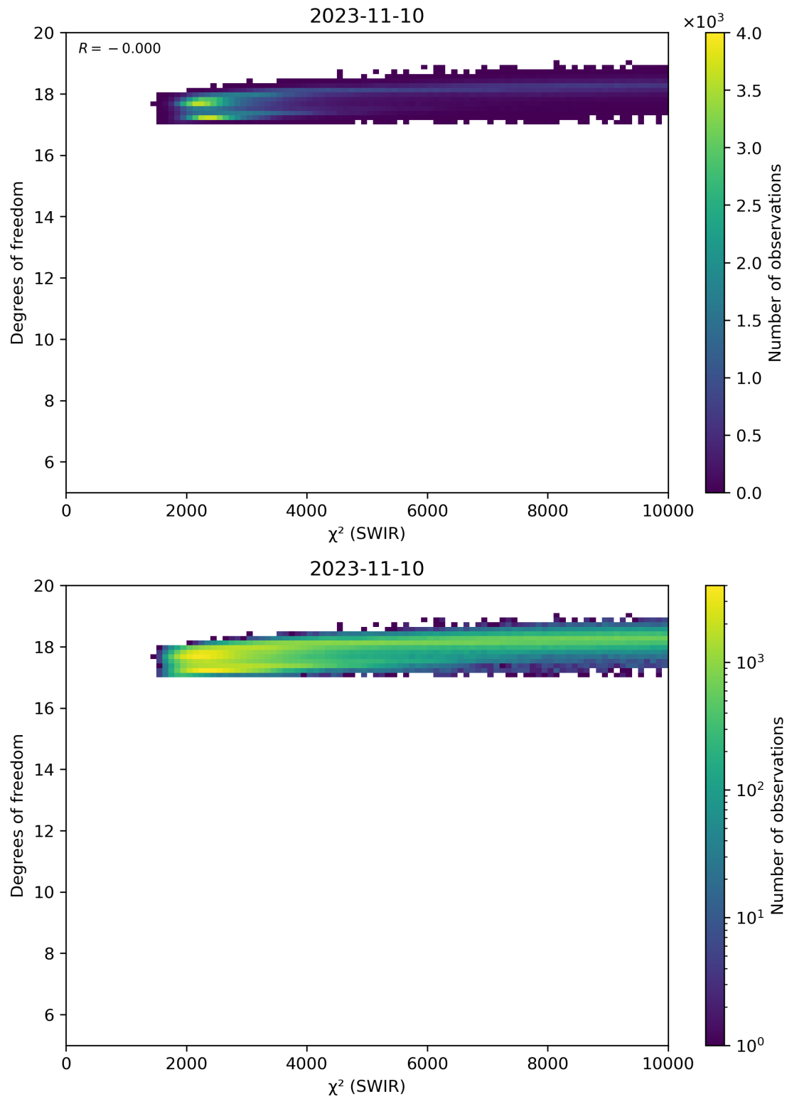
Figure 48: Scatter density plot of “ \chi^2 (SWIR)” against “Degrees of freedom” for 2023-11-09 to 2023-11-11.
