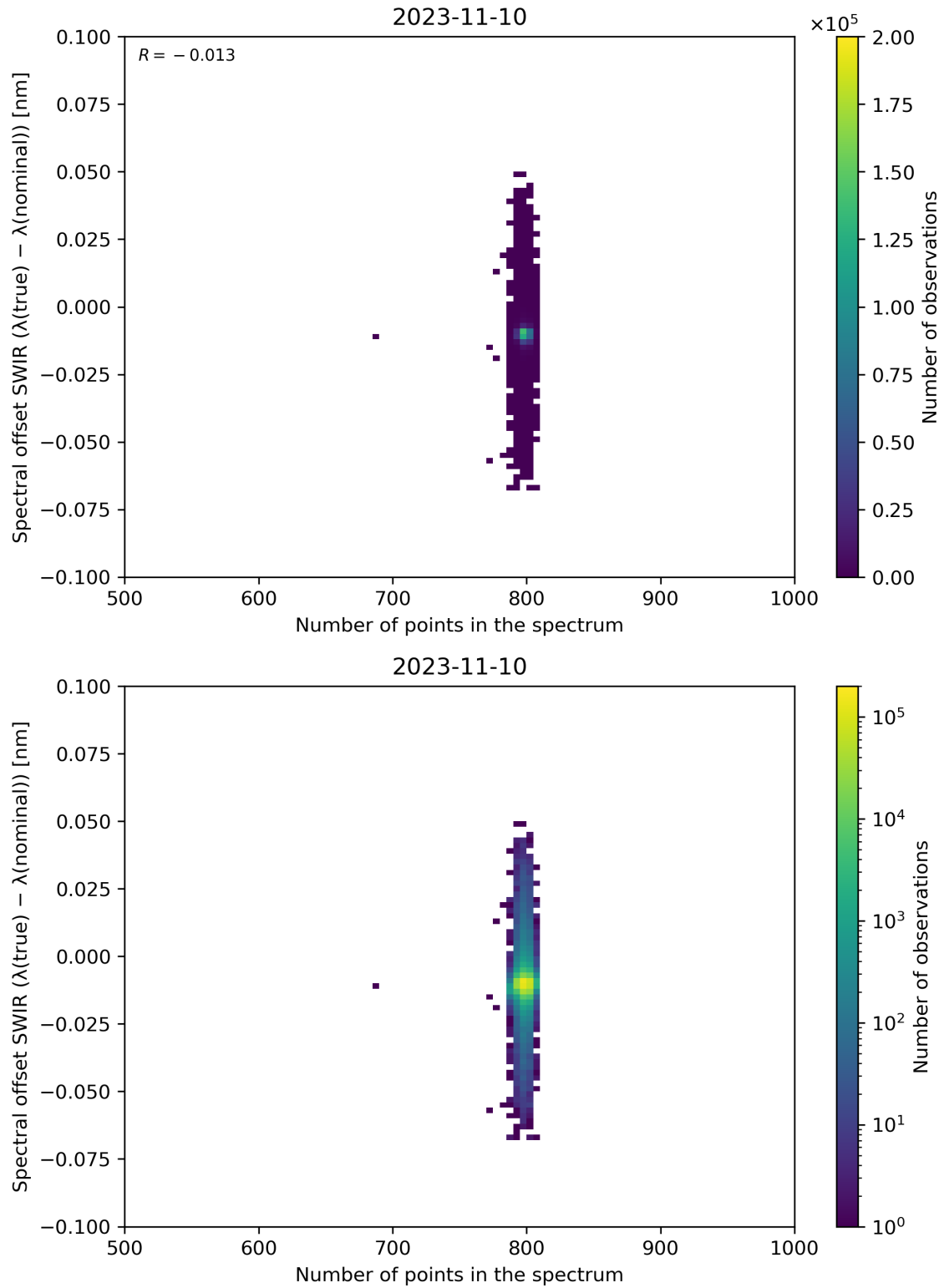
Figure 93: Scatter density plot of “Number of points in the spectrum” against “Spectral offset SWIR ( \lambda(\text{true}) - \lambda(\text{nominal}) )” for 2023-11-09 to 2023-11-11.
