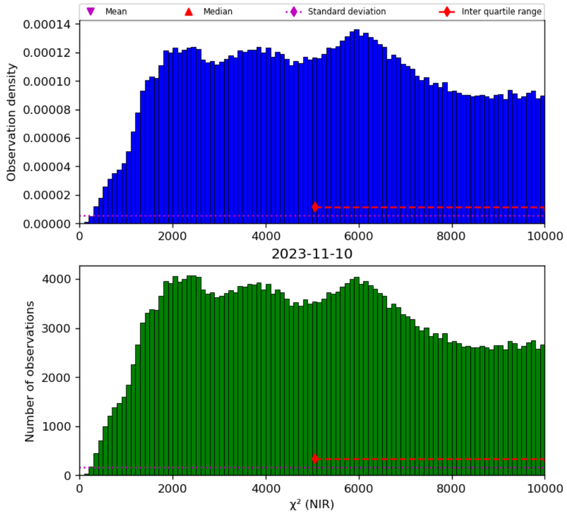
Figure 29: Histogram of “ \chi^2 (NIR)” for 2023-11-09 to 2023-11-11
