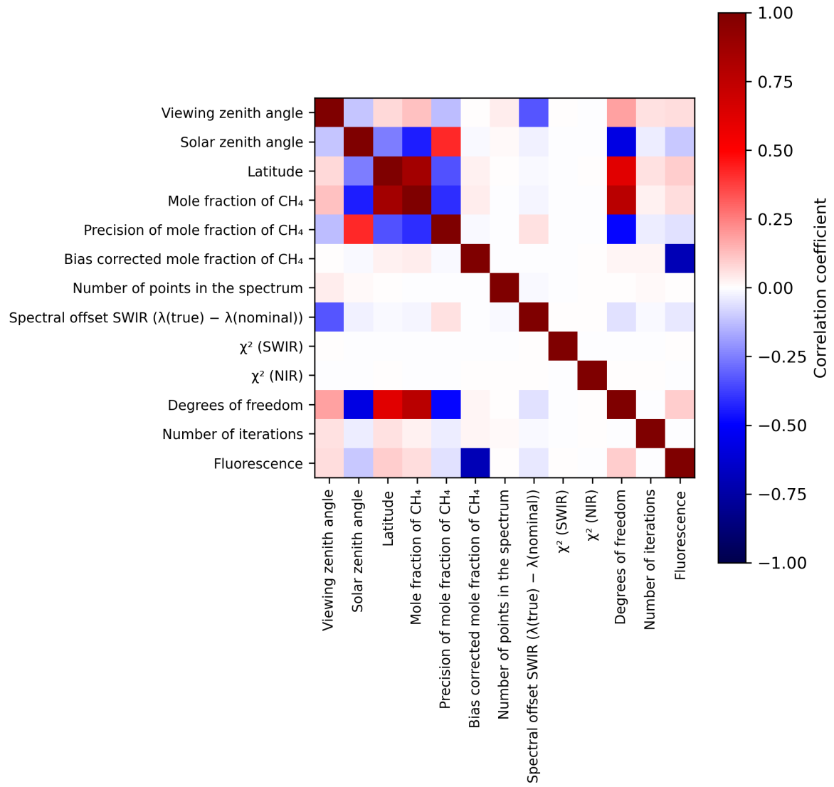
Figure 2: Map of correlation matrix for 2023-11-09 to 2023-11-11.
