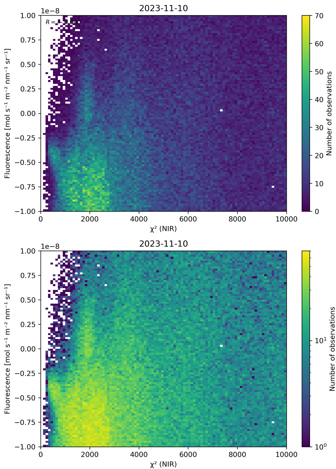
Figure 45: Scatter density plot of “ \chi^2 (NIR)” against “Fluorescence” for 2023-11-09 to 2023-11-11.
