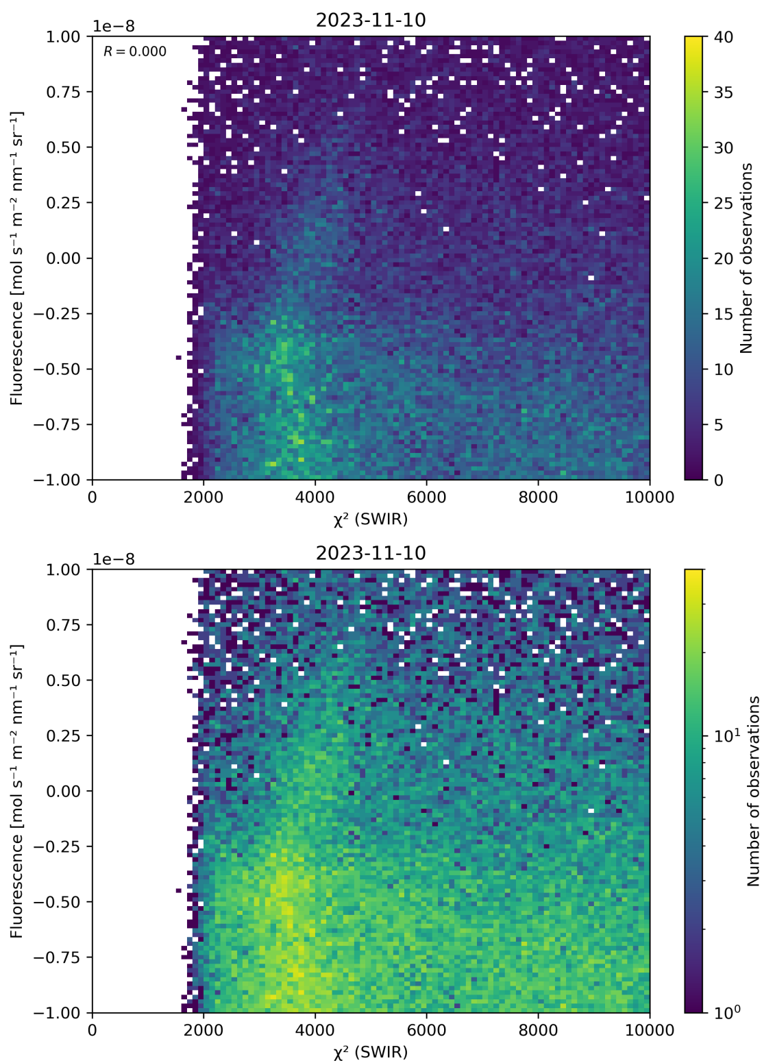
Figure 49: Scatter density plot of “ \chi^2 (SWIR)” against “Fluorescence” for 2023-11-09 to 2023-11-11.
