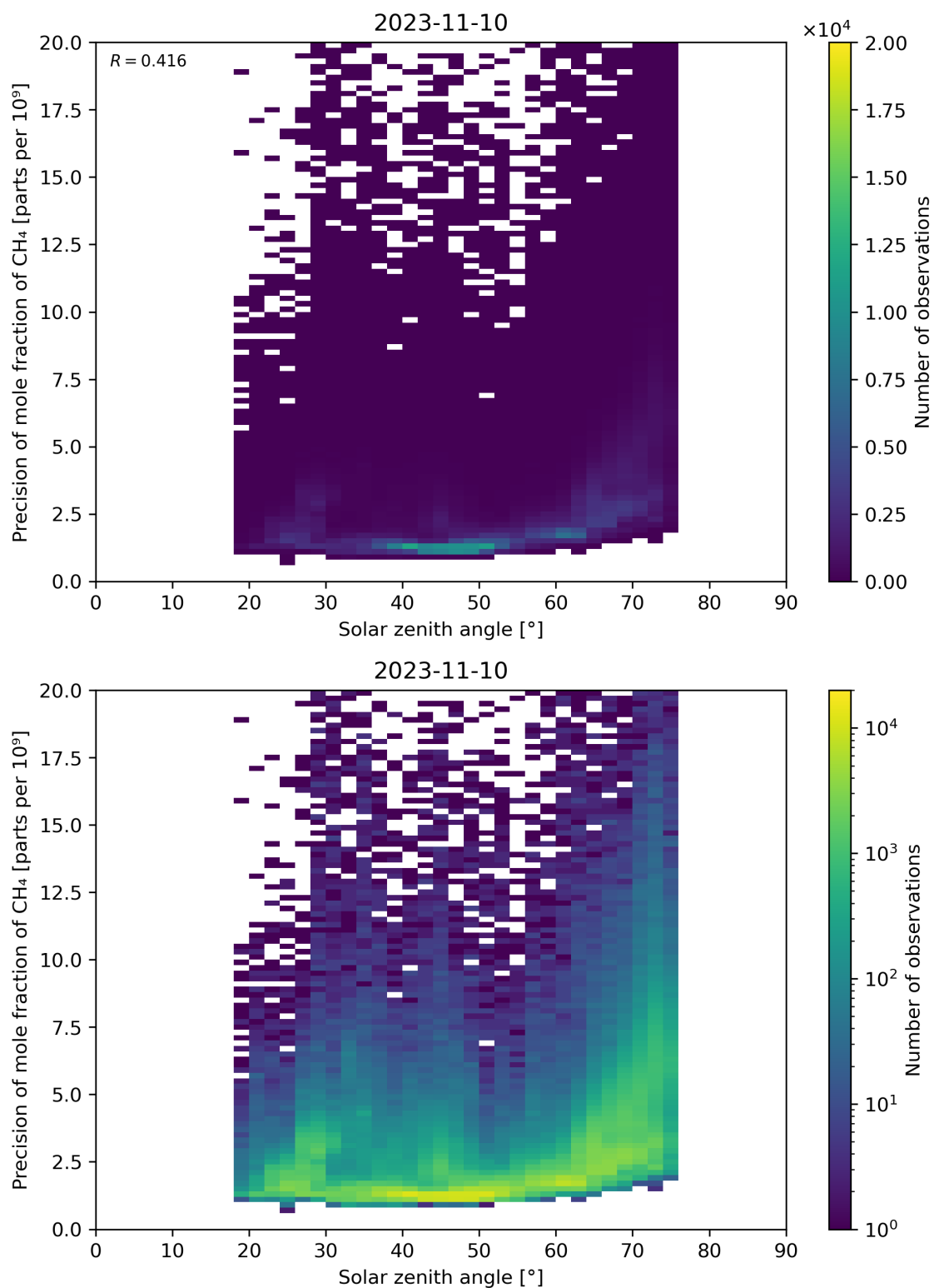
Figure 101: Scatter density plot of “Solar zenith angle” against “Precision of mole fraction of CH 4 ” for 2023-11-09 to 2023-11-11.
