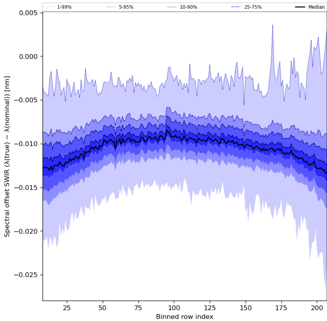
Figure 38: Along track statistics of “Spectral offset SWIR ( \lambda(\text{true}) - \lambda(\text{nominal}) )” for 2023-11-09 to 2023-11-11
