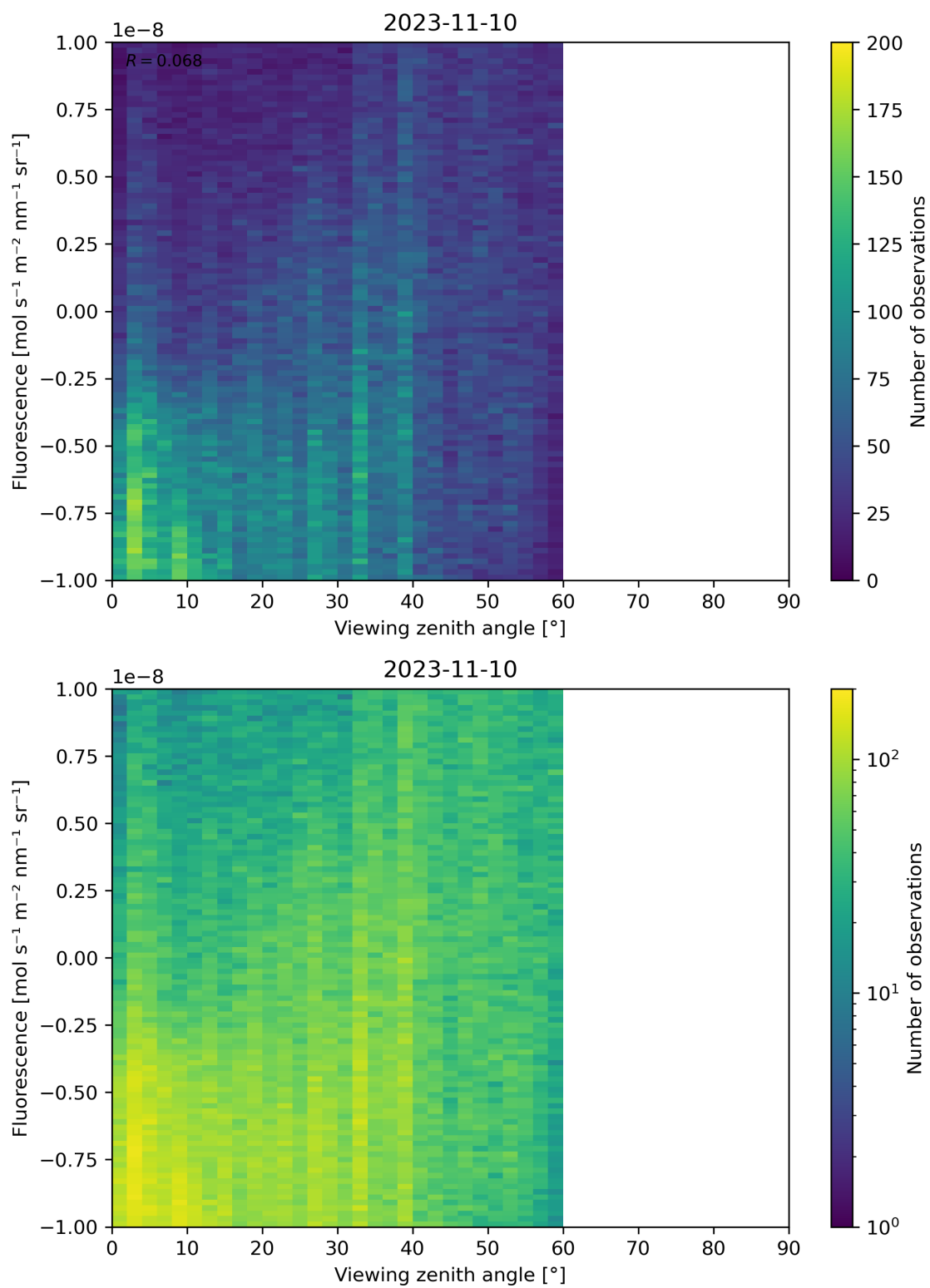
Figure 108: Scatter density plot of “Viewing zenith angle” against “Fluorescence” for 2023-11-09 to 2023-11-11.
