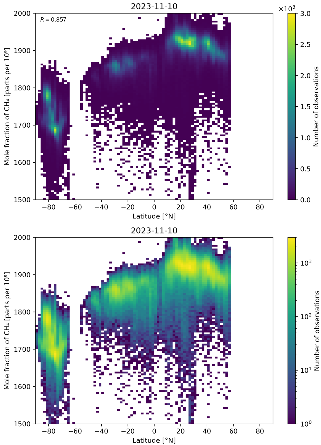
Figure 57: Scatter density plot of “Latitude” against “Mole fraction of \text{CH}_4 ” for 2023-11-09 to 2023-11-11.
