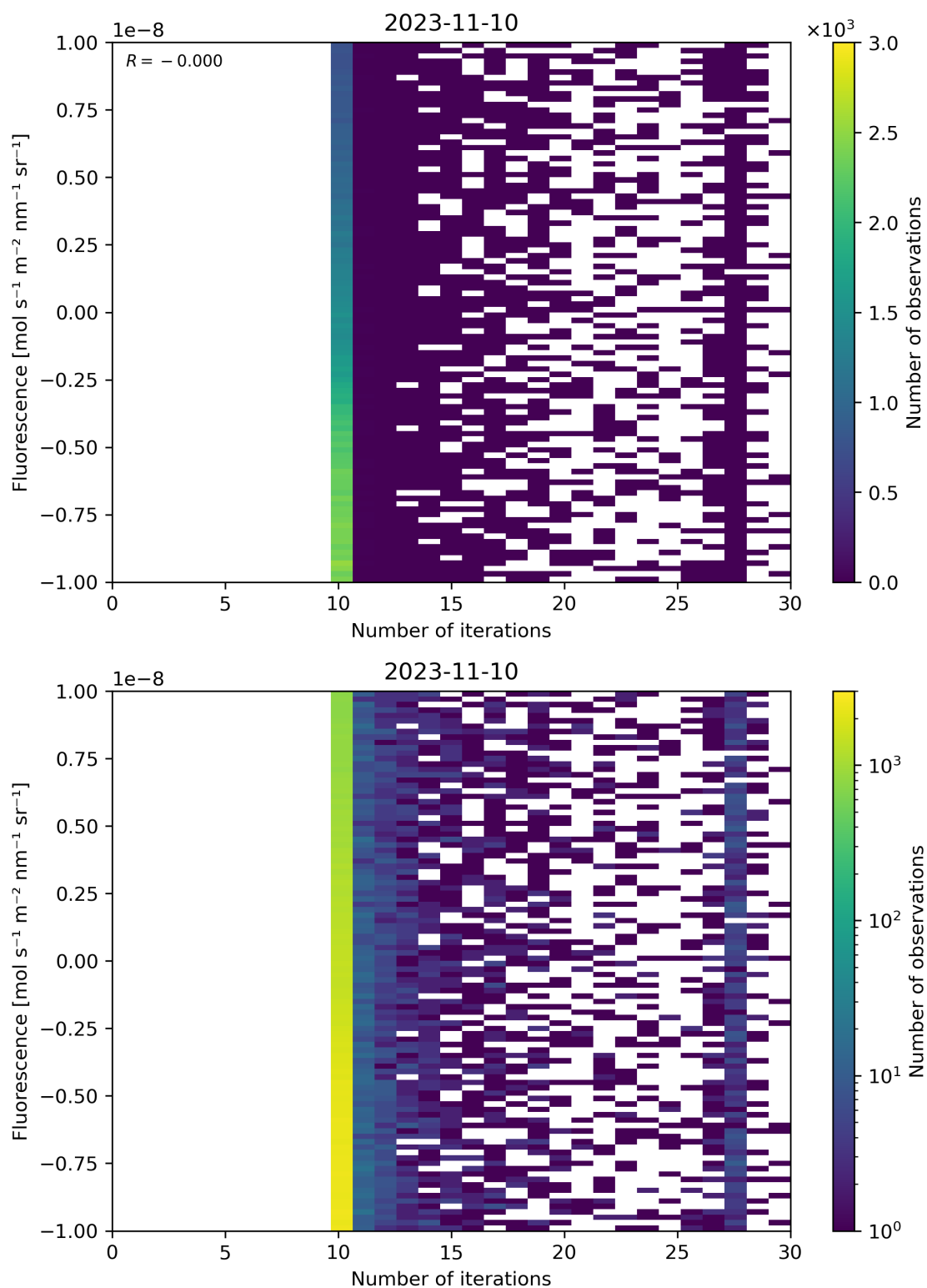
Figure 87: Scatter density plot of “Number of iterations” against “Fluorescence” for 2023-11-09 to 2023-11-11.
