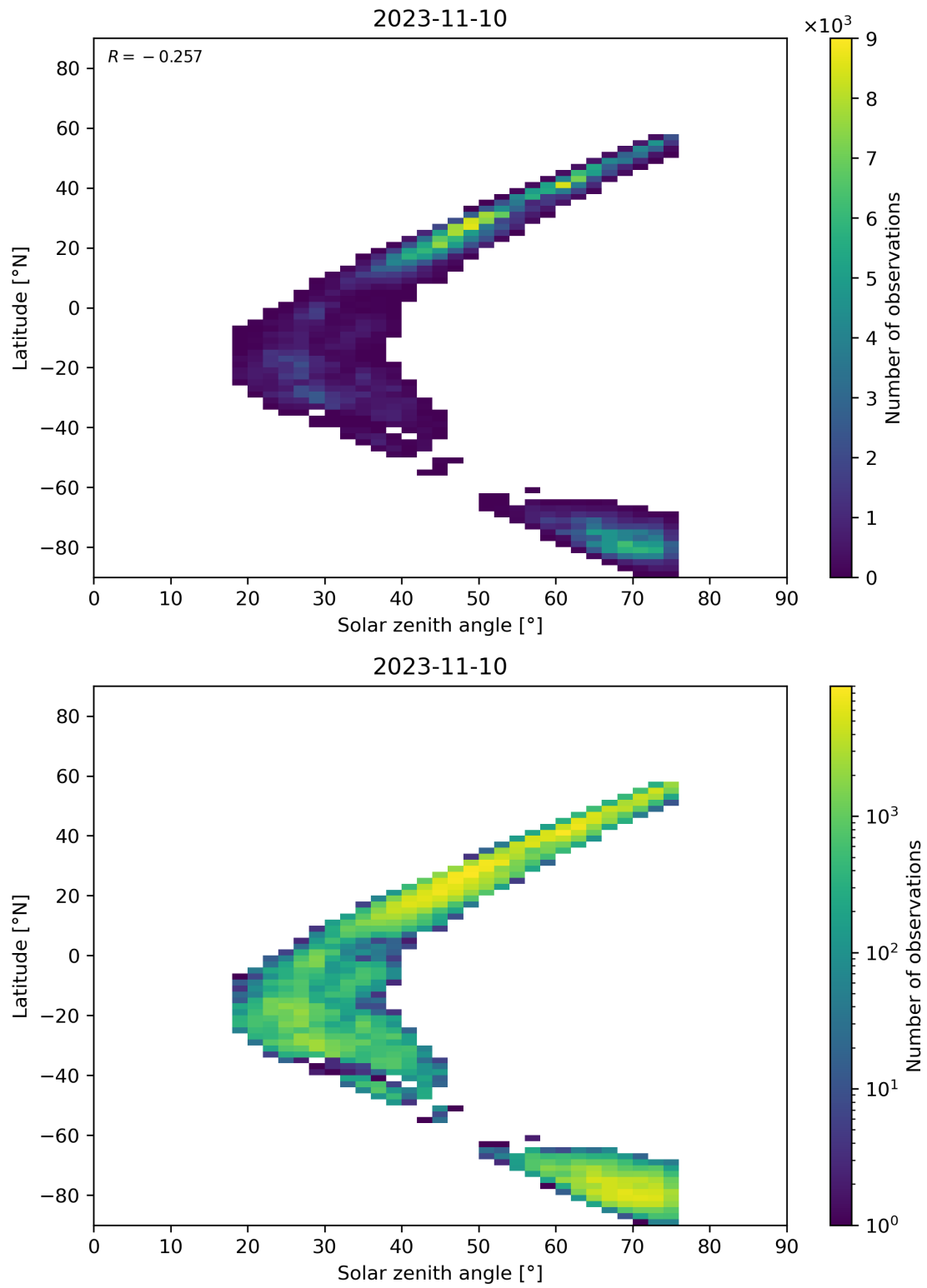
Figure 98: Scatter density plot of “Solar zenith angle” against “Latitude” for 2023-11-09 to 2023-11-11.
