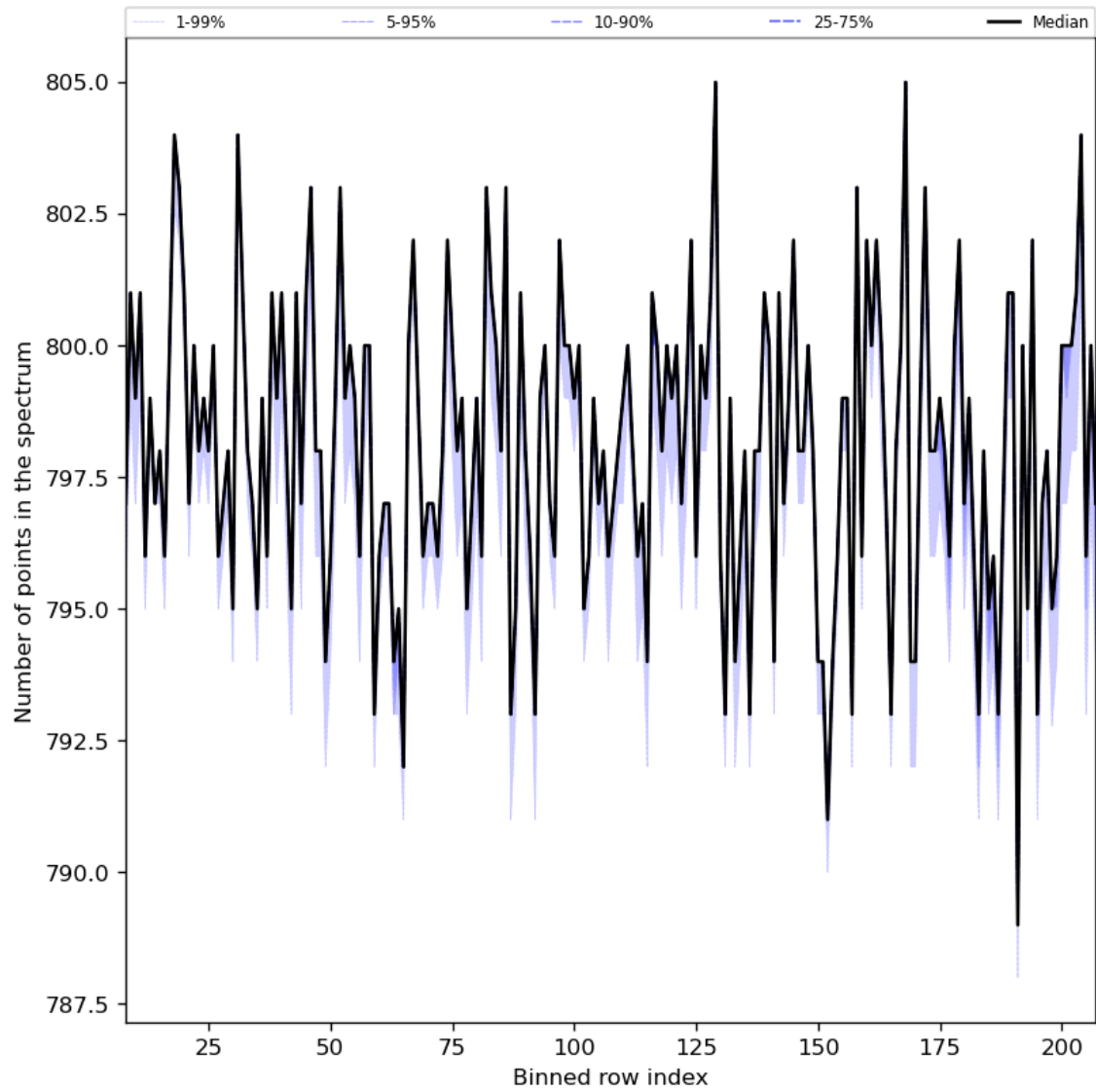
Figure 37: Along track statistics of “Number of points in the spectrum” for 2023-11-09 to 2023-11-11
