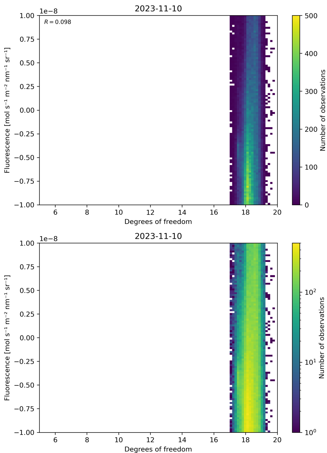
Figure 51: Scatter density plot of “Degrees of freedom” against “Fluorescence” for 2023-11-09 to 2023-11-11.
