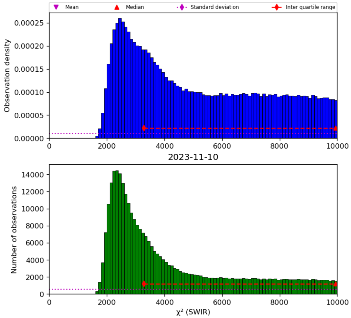
Figure 28: Histogram of “ \chi^2 (SWIR)” for 2023-11-09 to 2023-11-11
