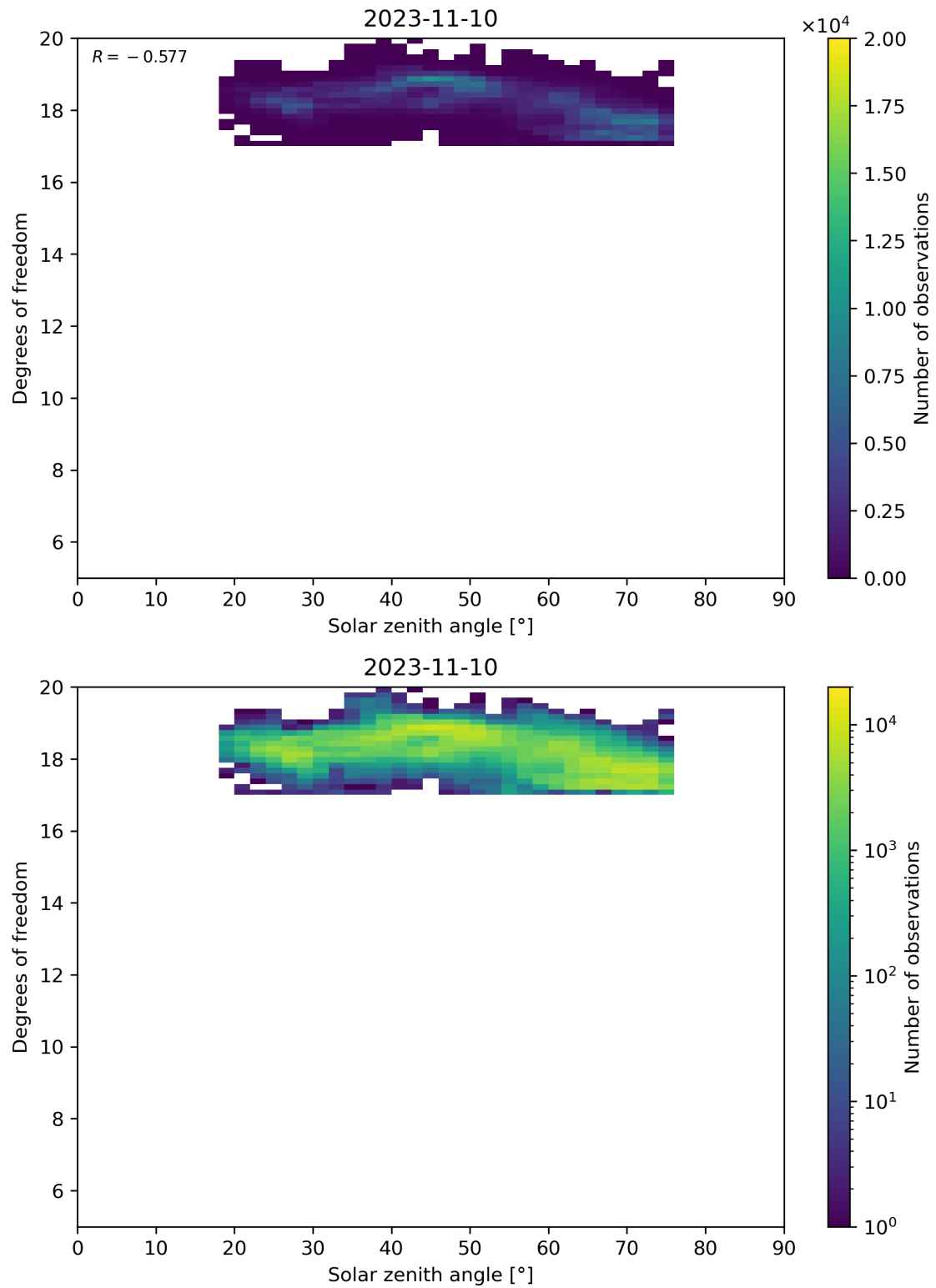
Figure 96: Scatter density plot of “Solar zenith angle” against “Degrees of freedom” for 2023-11-09 to 2023-11-11.
