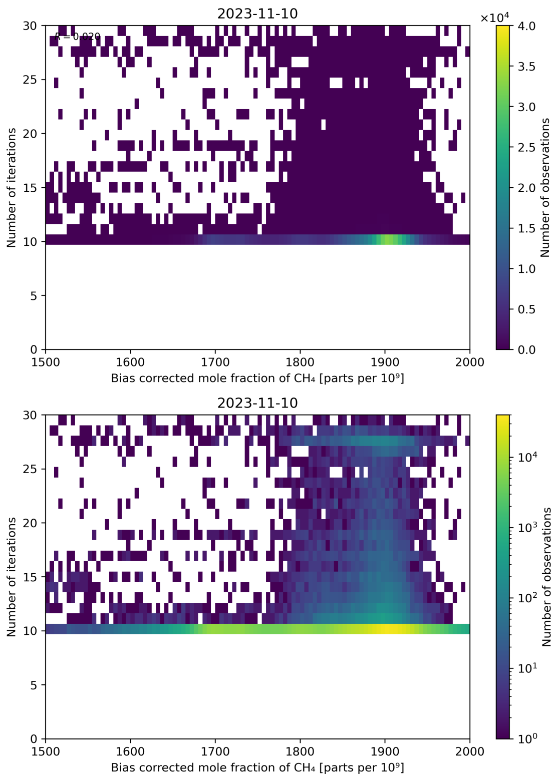
Figure 67: Scatter density plot of “Bias corrected mole fraction of \text{CH}_4 ” against “Number of iterations” for 2023-11-09 to 2023-11-11.
