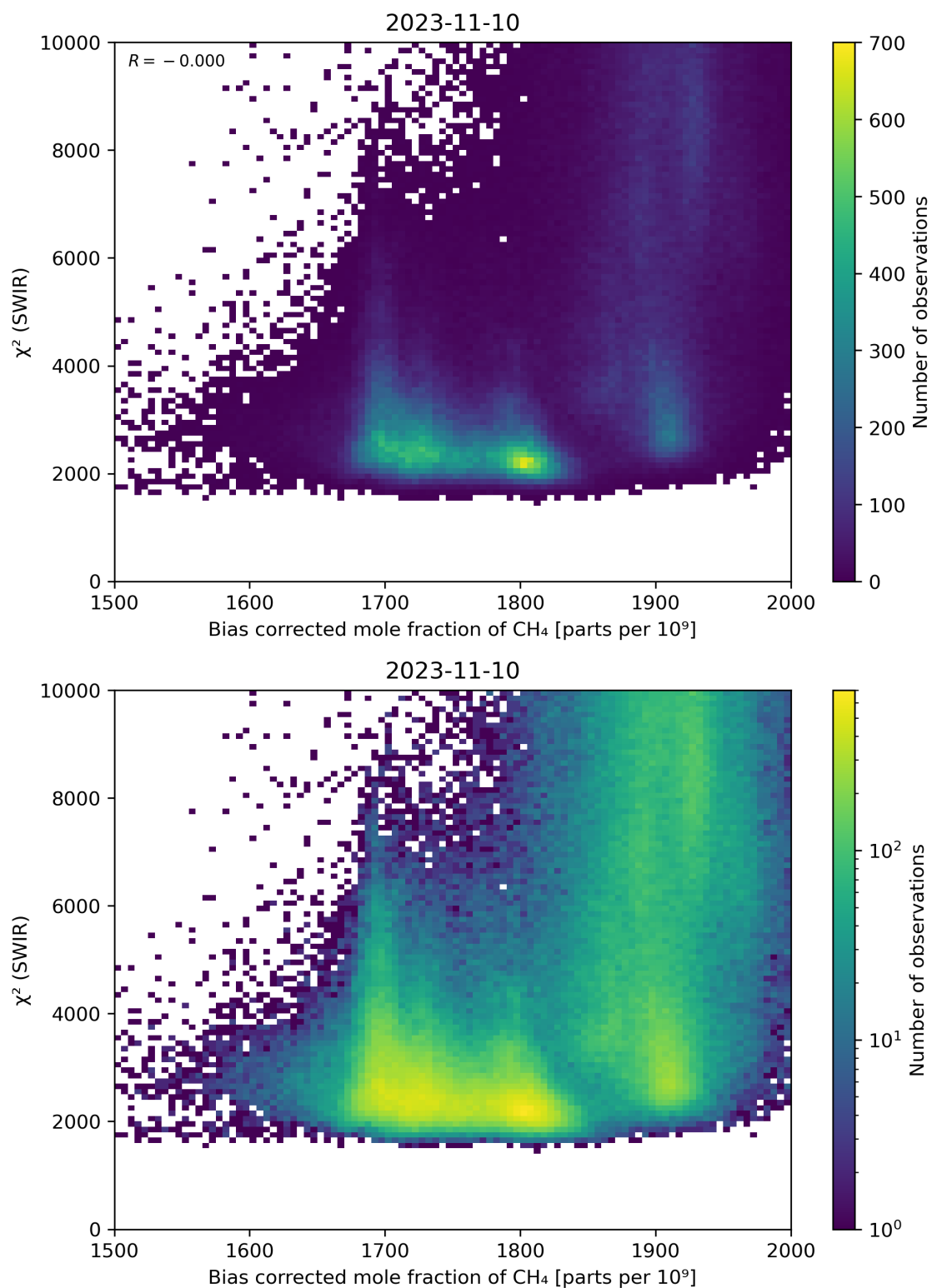
Figure 64: Scatter density plot of “Bias corrected mole fraction of \text{CH}_4 ” against “ \chi^2 (SWIR)” for 2023-11-09 to 2023-11-11.
