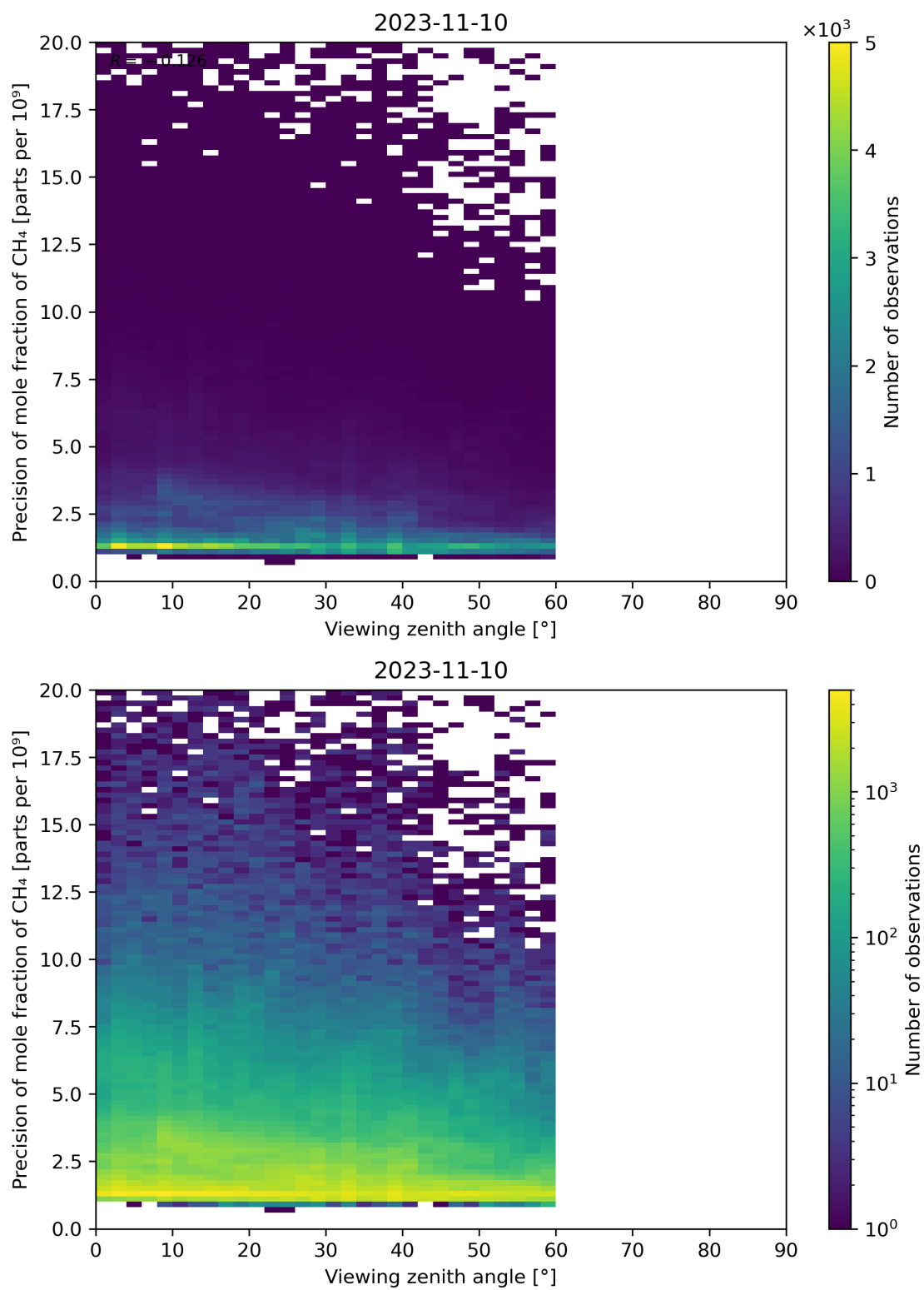
Figure 112: Scatter density plot of “Viewing zenith angle” against “Precision of mole fraction of CH 4 ” for 2023-11-09 to 2023-11-11.
