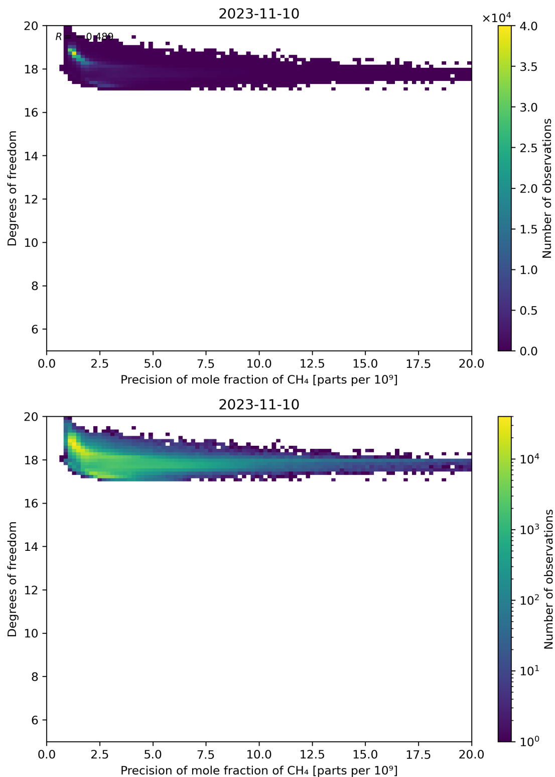
Figure 80: Scatter density plot of “Precision of mole fraction of CH 4 ” against “Degrees of freedom” for 2023-11-09 to 2023-11-11.
