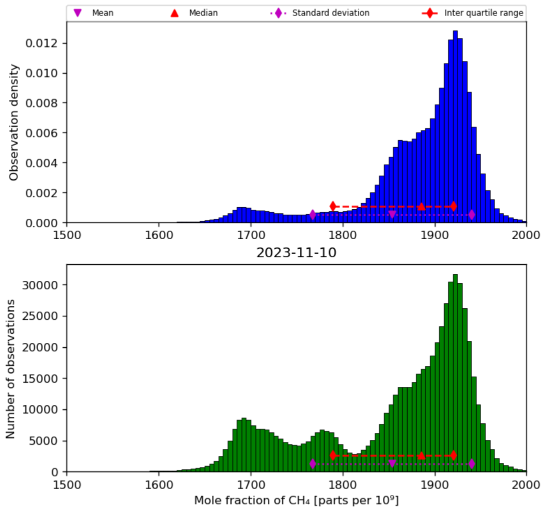
Figure 23: Histogram of “Mole fraction of CH 4 ” for 2023-11-09 to 2023-11-11
