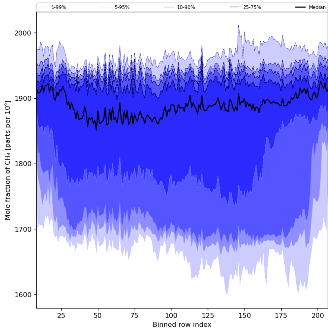
Figure 34: Along track statistics of “Mole fraction of CH 4 ” for 2023-11-09 to 2023-11-11
