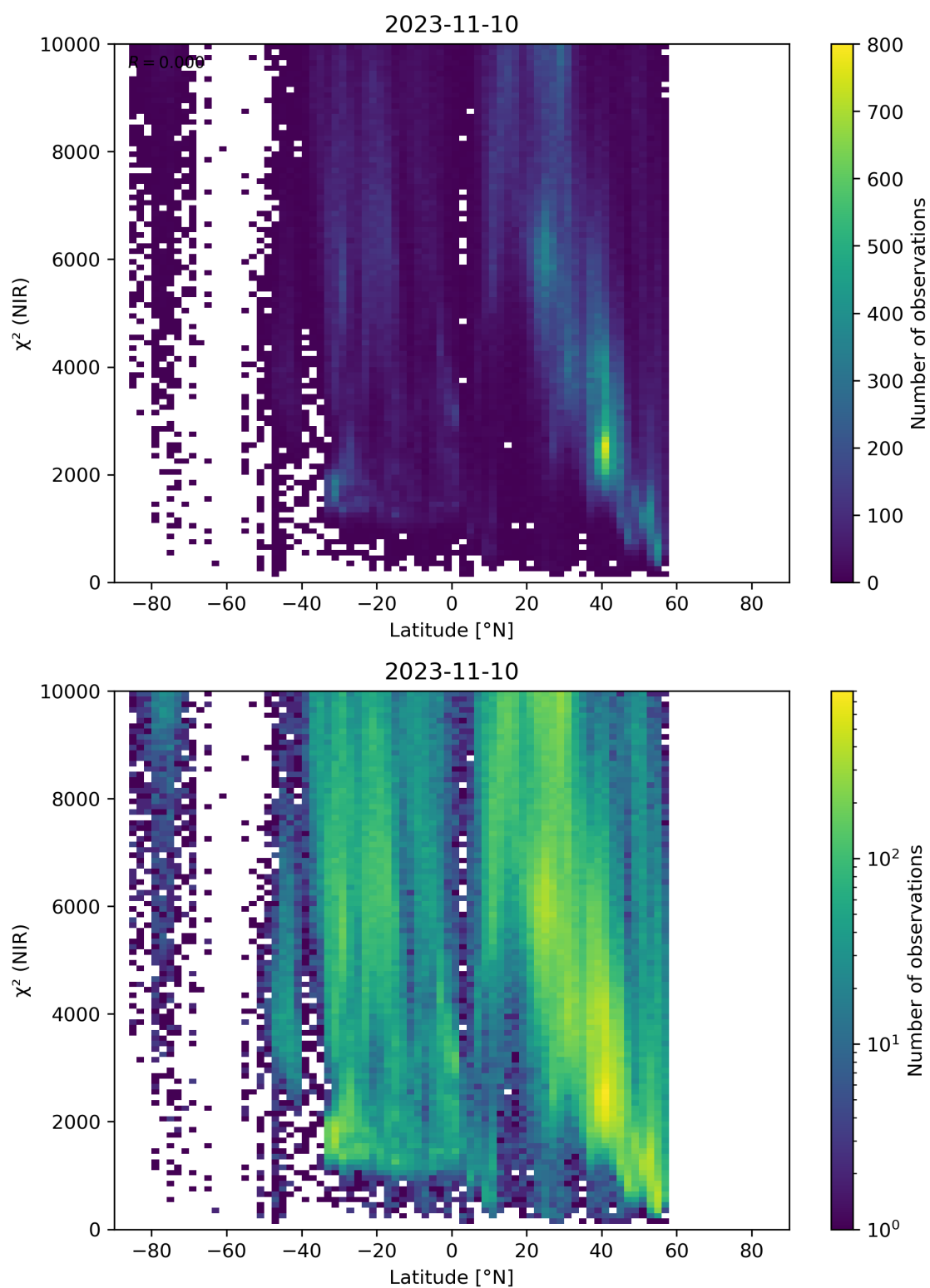
Figure 53: Scatter density plot of “Latitude” against “ \chi^2 (NIR)” for 2023-11-09 to 2023-11-11.
