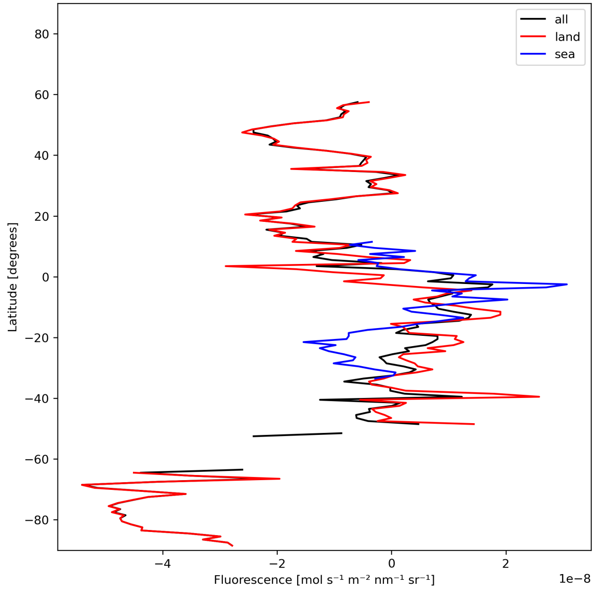
Figure 21: Zonal average of “Fluorescence” for 2023-11-09 to 2023-11-11.
