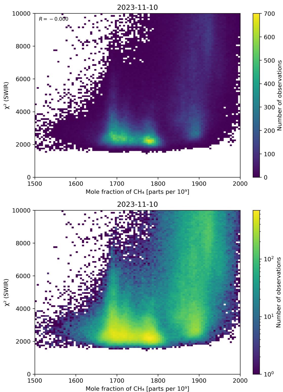
Figure 71: Scatter density plot of “Mole fraction of \text{CH}_4 ” against “ \chi^2 (SWIR)” for 2023-11-09 to 2023-11-11.
