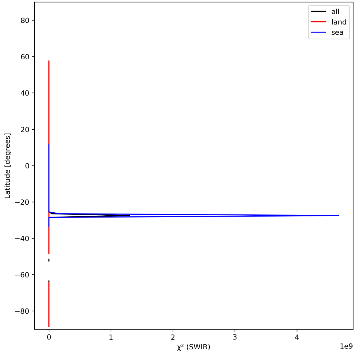
Figure 17: Zonal average of “ \chi^2 (SWIR)” for 2023-11-09 to 2023-11-11.
