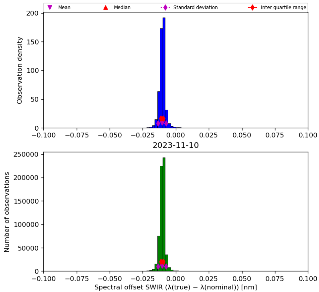
Figure 27: Histogram of “Spectral offset SWIR ( \lambda(\text{true}) - \lambda(\text{nominal}) )” for 2023-11-09 to 2023-11-11
