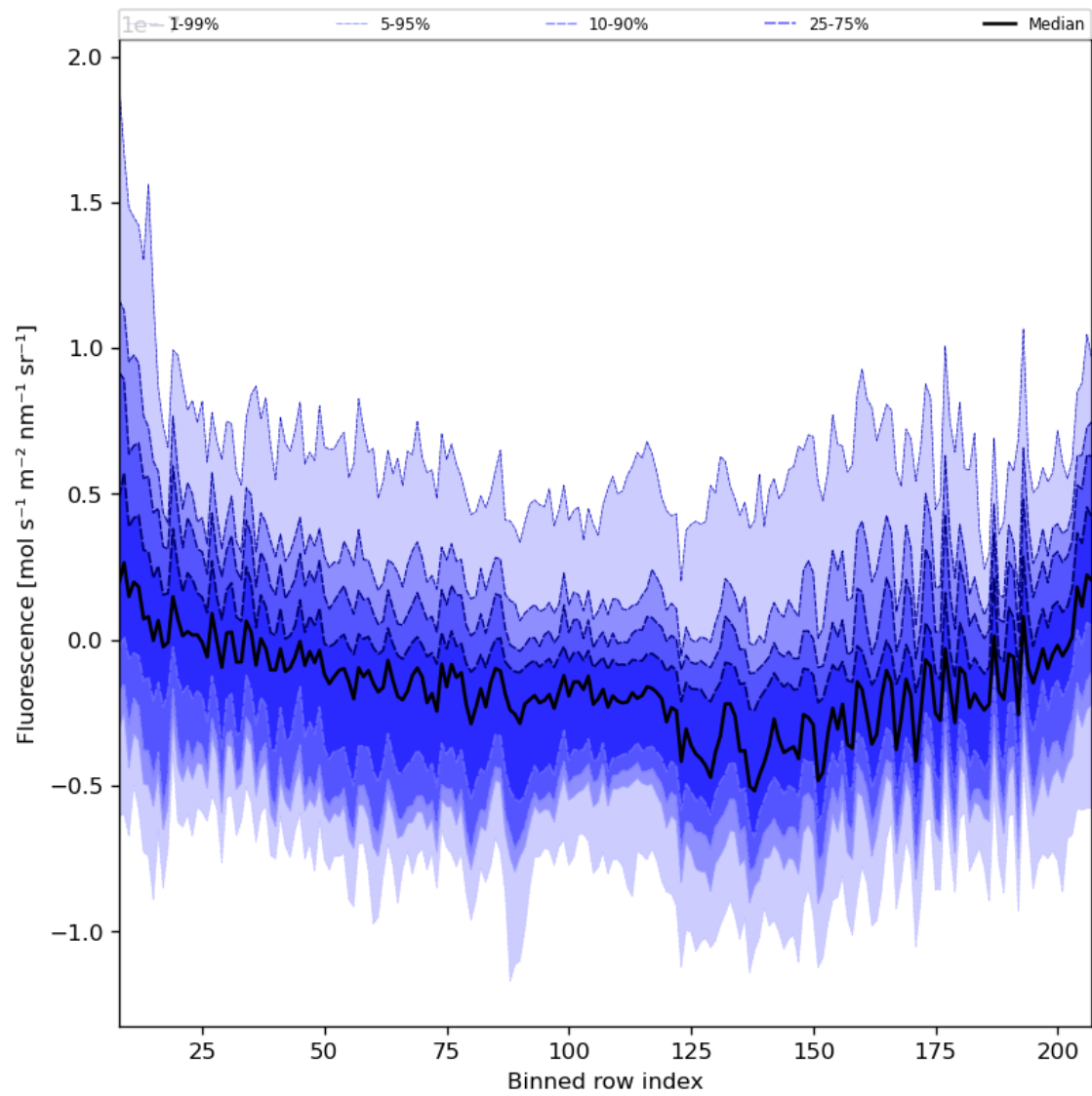
Figure 43: Along track statistics of “Fluorescence” for 2023-11-09 to 2023-11-11
