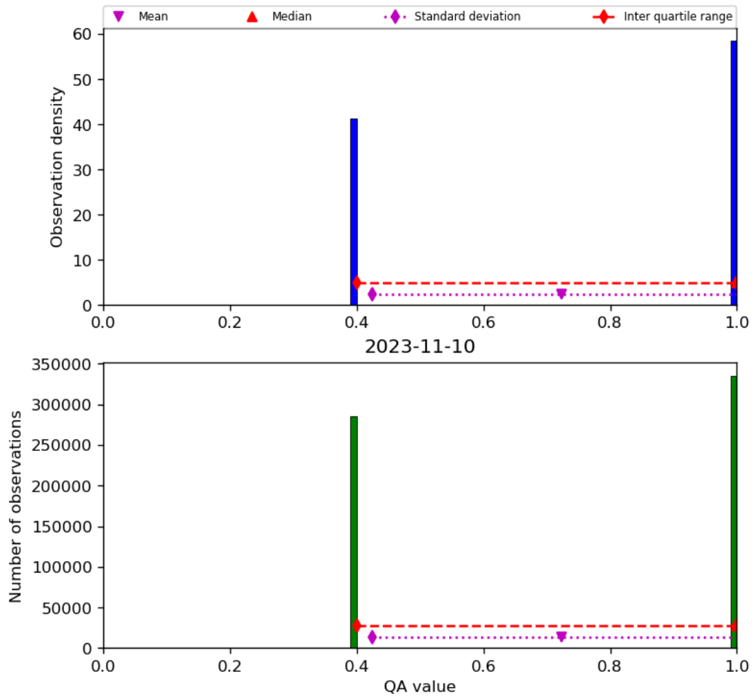
Figure 22: Histogram of “QA value” for 2023-11-09 to 2023-11-11
