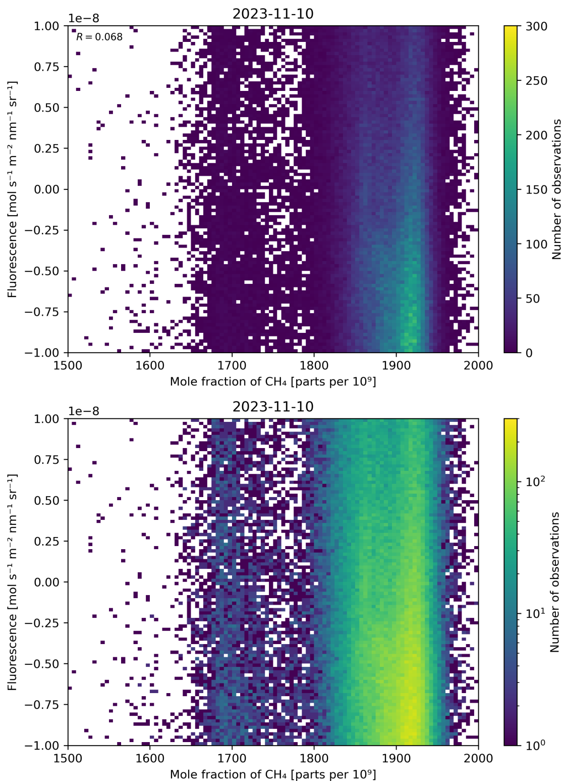
Figure 73: Scatter density plot of “Mole fraction of \text{CH}_4 ” against “Fluorescence” for 2023-11-09 to 2023-11-11.
