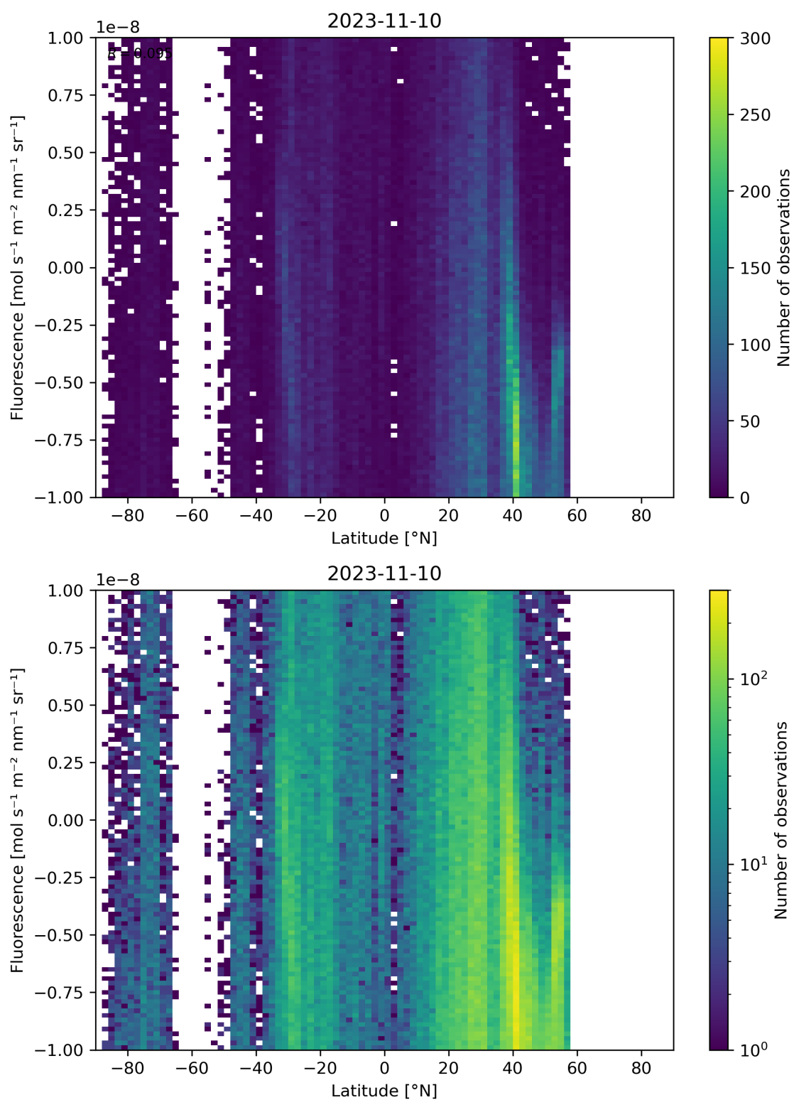
Figure 56: Scatter density plot of “Latitude” against “Fluorescence” for 2023-11-09 to 2023-11-11.
