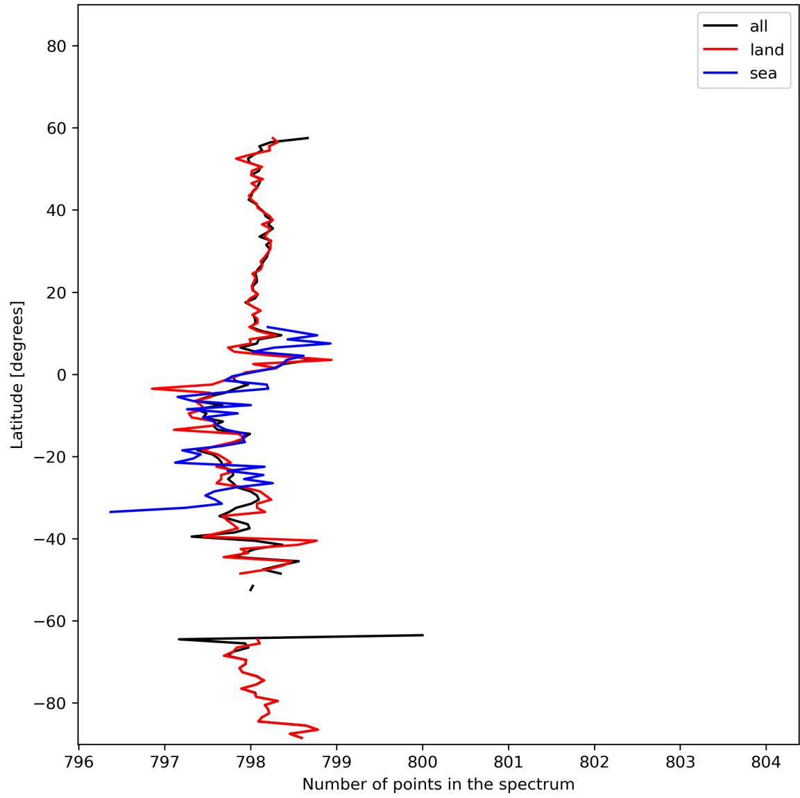
Figure 15: Zonal average of “Number of points in the spectrum” for 2023-11-09 to 2023-11-11.
