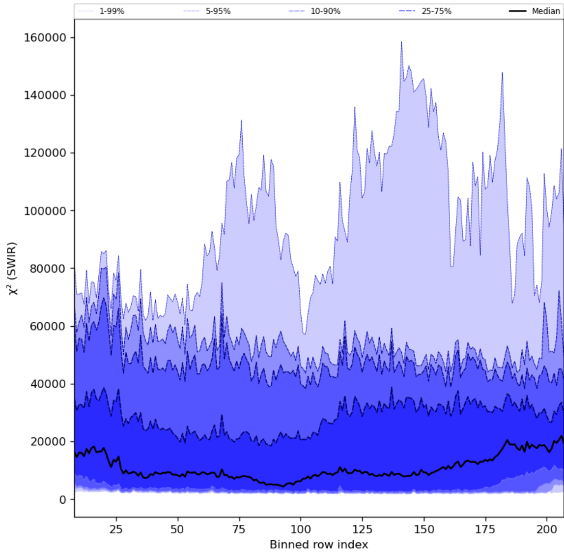
Figure 39: Along track statistics of " \chi^2 (SWIR)" for 2023-11-09 to 2023-11-11
