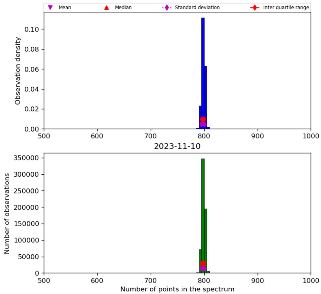
Figure 26: Histogram of “Number of points in the spectrum” for 2023-11-09 to 2023-11-11
