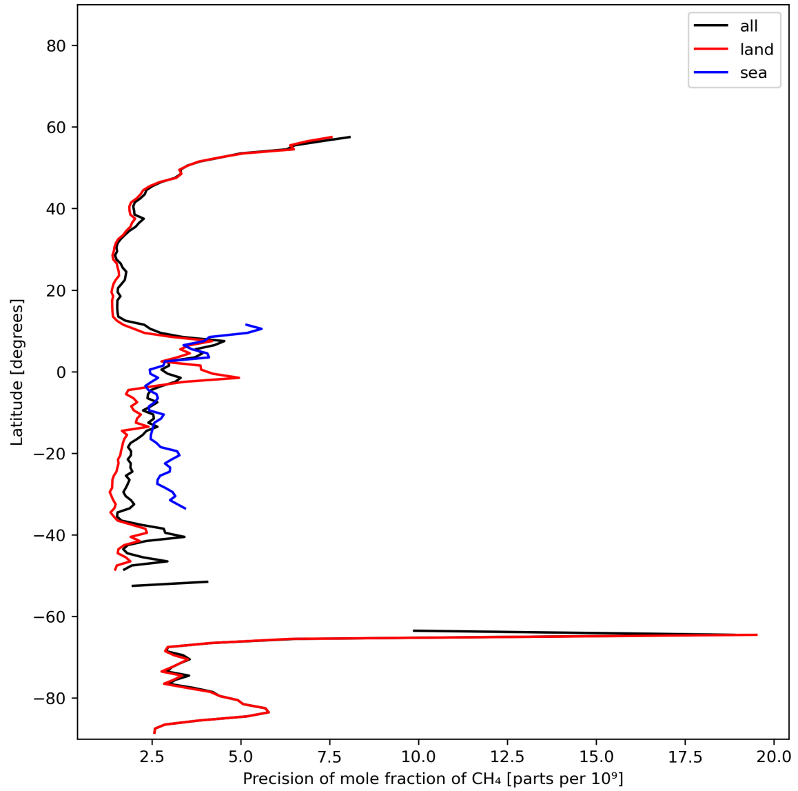
Figure 13: Zonal average of “Precision of mole fraction of CH 4 ” for 2023-11-09 to 2023-11-11.
