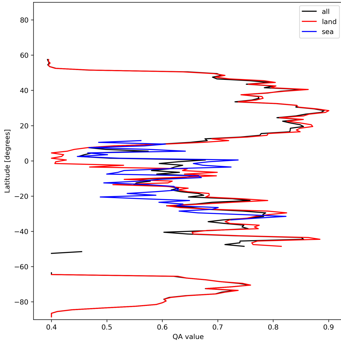
Figure 11: Zonal average of “QA value” for 2023-11-09 to 2023-11-11.
