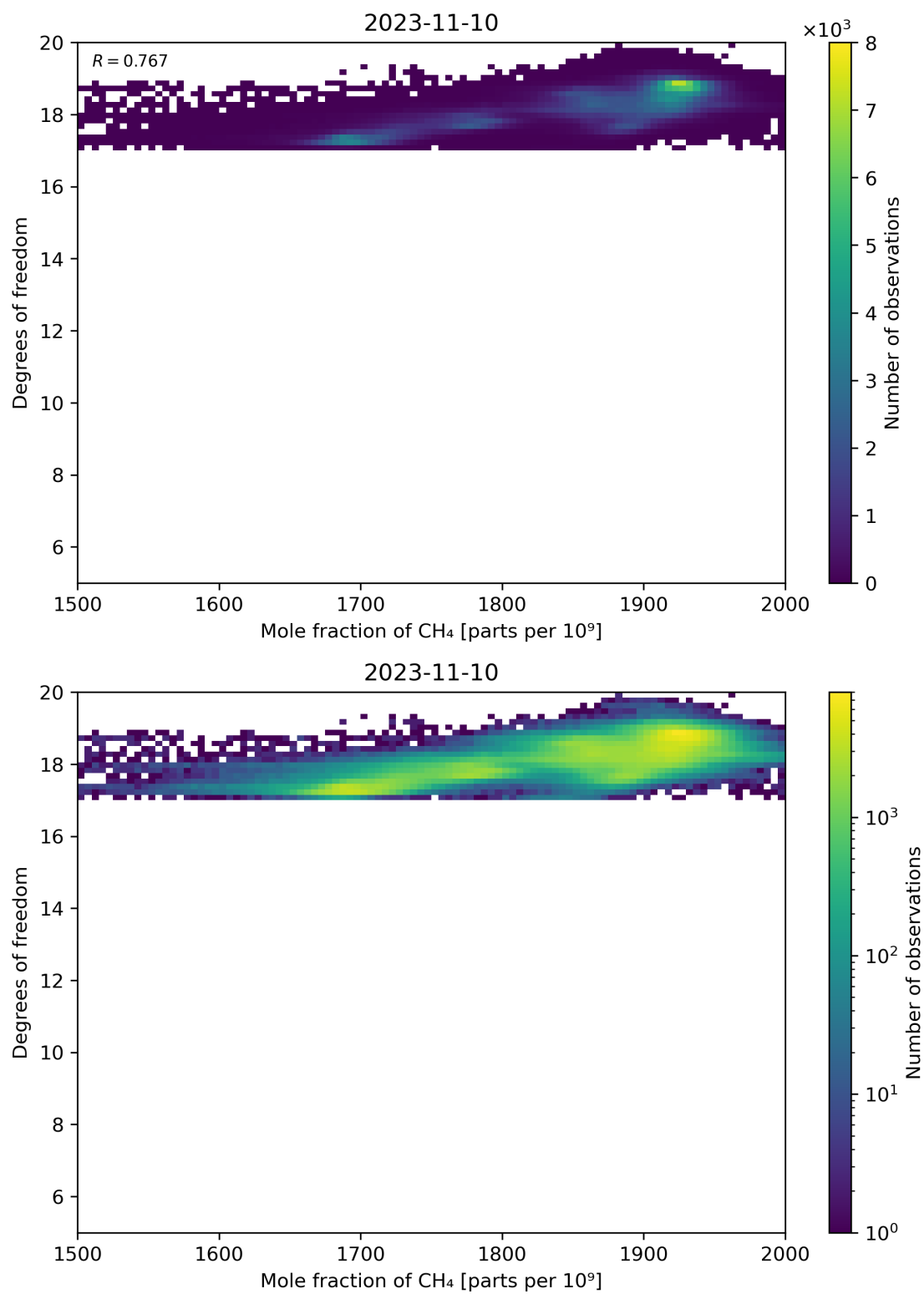
Figure 72: Scatter density plot of “Mole fraction of CH 4 ” against “Degrees of freedom” for 2023-11-09 to 2023-11-11.
