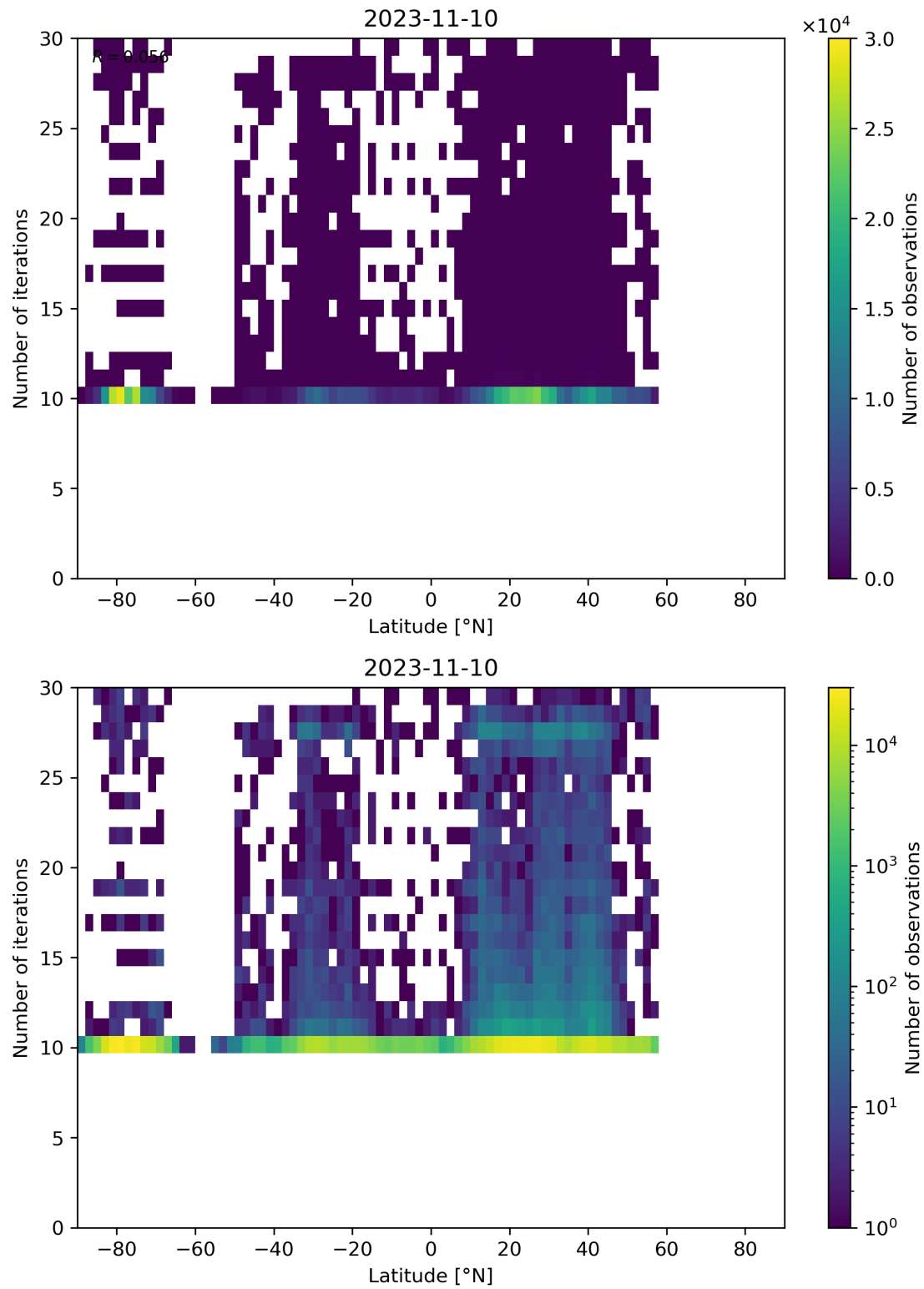
Figure 60: Scatter density plot of “Latitude” against “Number of iterations” for 2023-11-09 to 2023-11-11.
