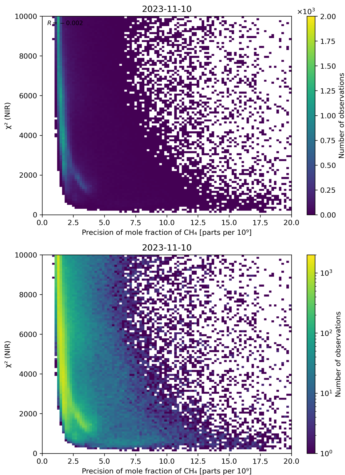
Figure 78: Scatter density plot of “Precision of mole fraction of CH 4 ” against “ \chi^2 (NIR)” for 2023-11-09 to 2023-11-11.
