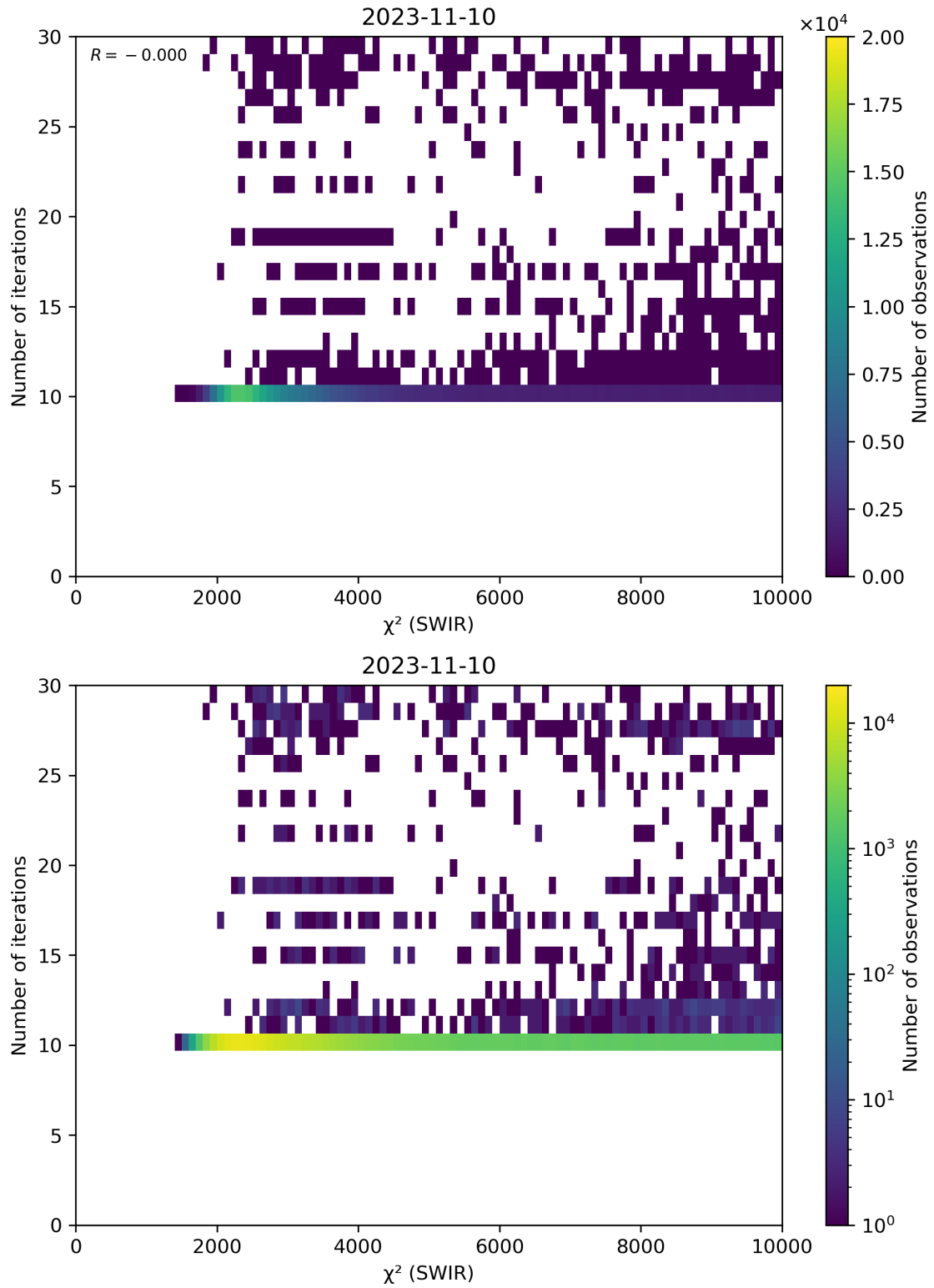
Figure 50: Scatter density plot of “ \chi^2 (SWIR)” against “Number of iterations” for 2023-11-09 to 2023-11-11.
