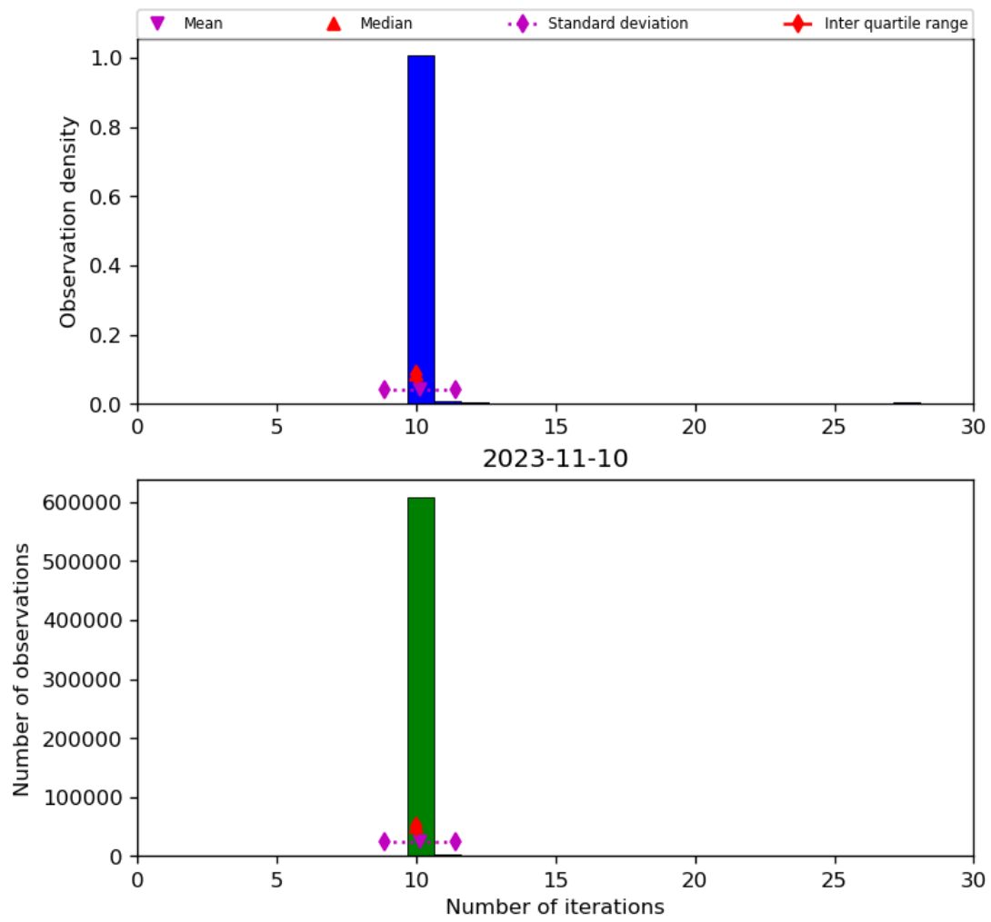
Figure 31: Histogram of “Number of iterations” for 2023-11-09 to 2023-11-11
