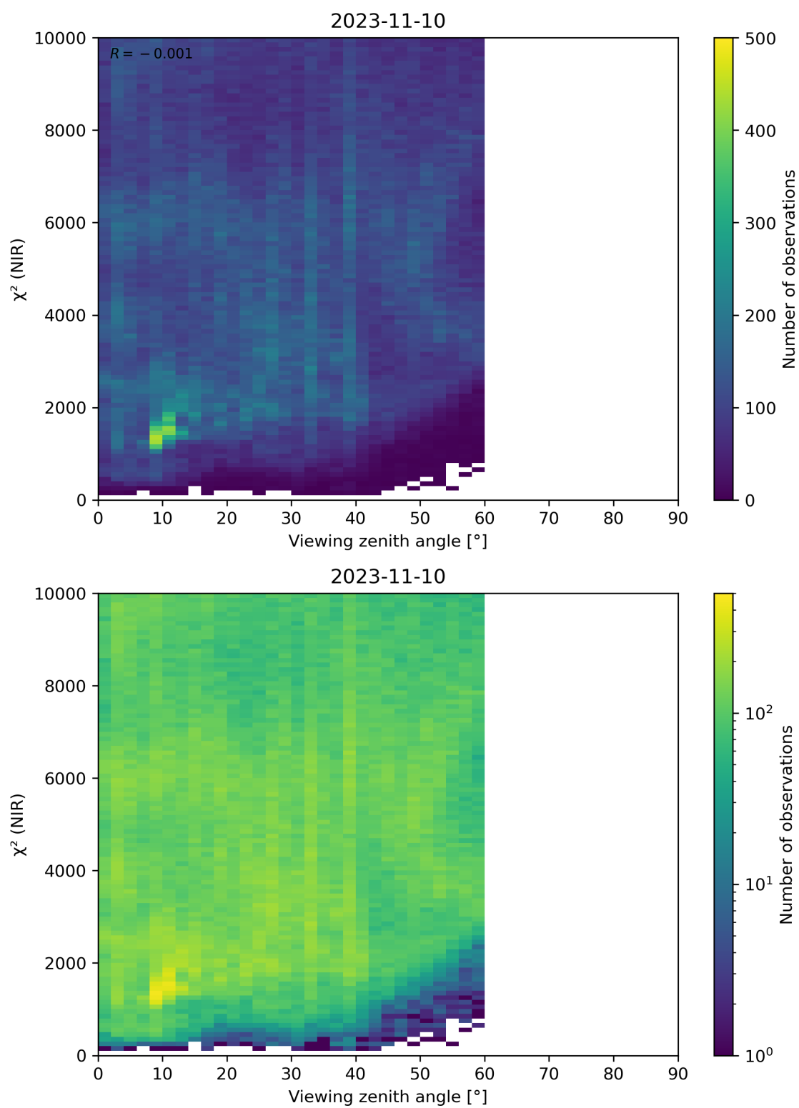
Figure 105: Scatter density plot of “Viewing zenith angle” against “ \chi^2 (NIR)” for 2023-11-09 to 2023-11-11.
