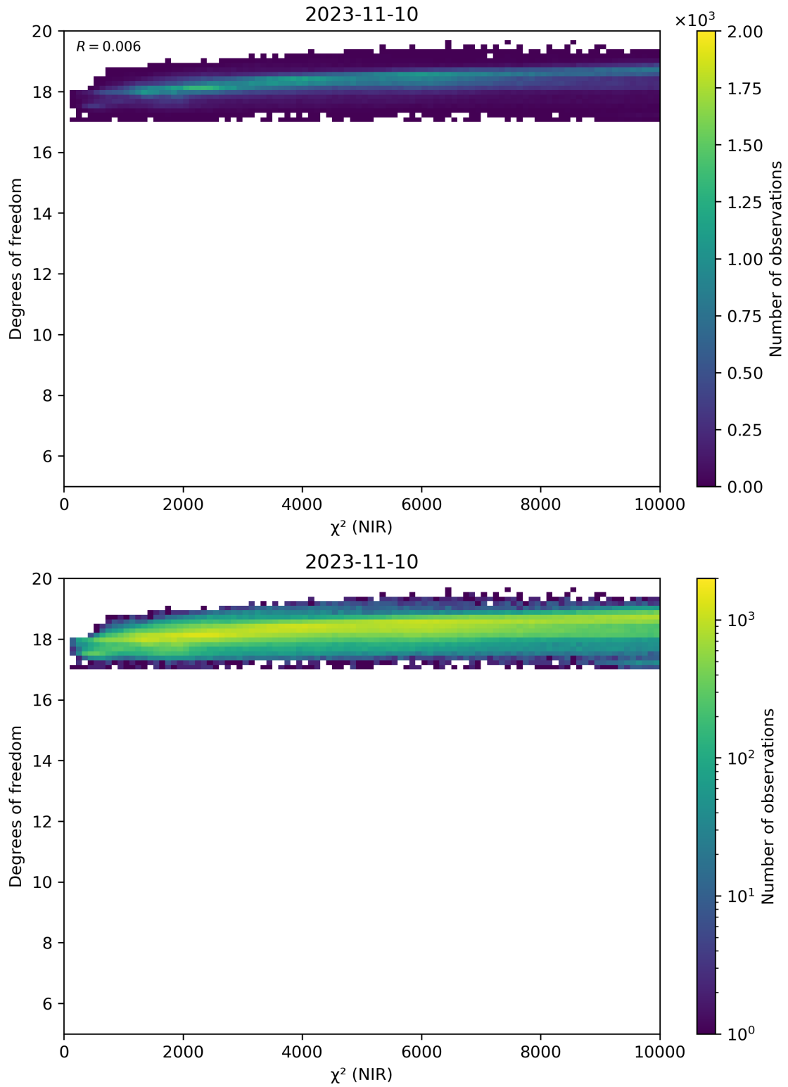
Figure 44: Scatter density plot of “ \chi^2 (NIR)” against “Degrees of freedom” for 2023-11-09 to 2023-11-11.
