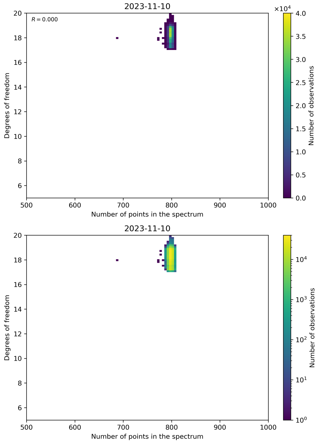
Figure 90: Scatter density plot of “Number of points in the spectrum” against “Degrees of freedom” for 2023-11-09 to 2023-11-11.
