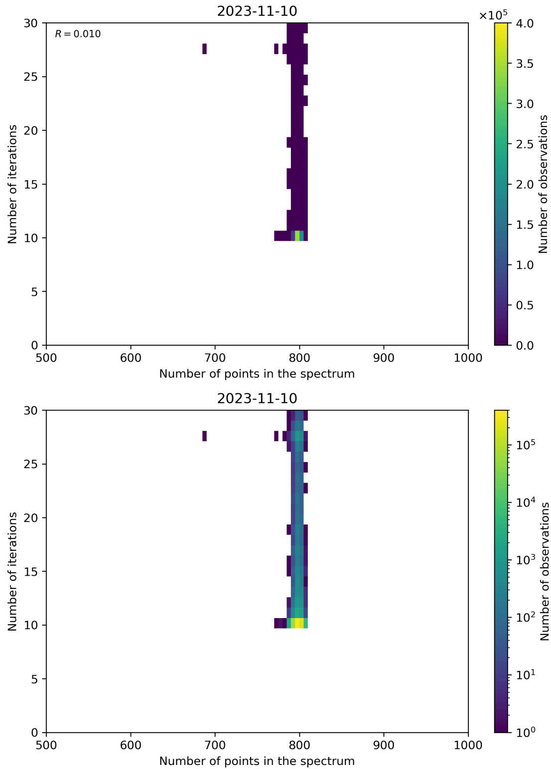
Figure 92: Scatter density plot of “Number of points in the spectrum” against “Number of iterations” for 2023-11-09 to 2023-11-11.
