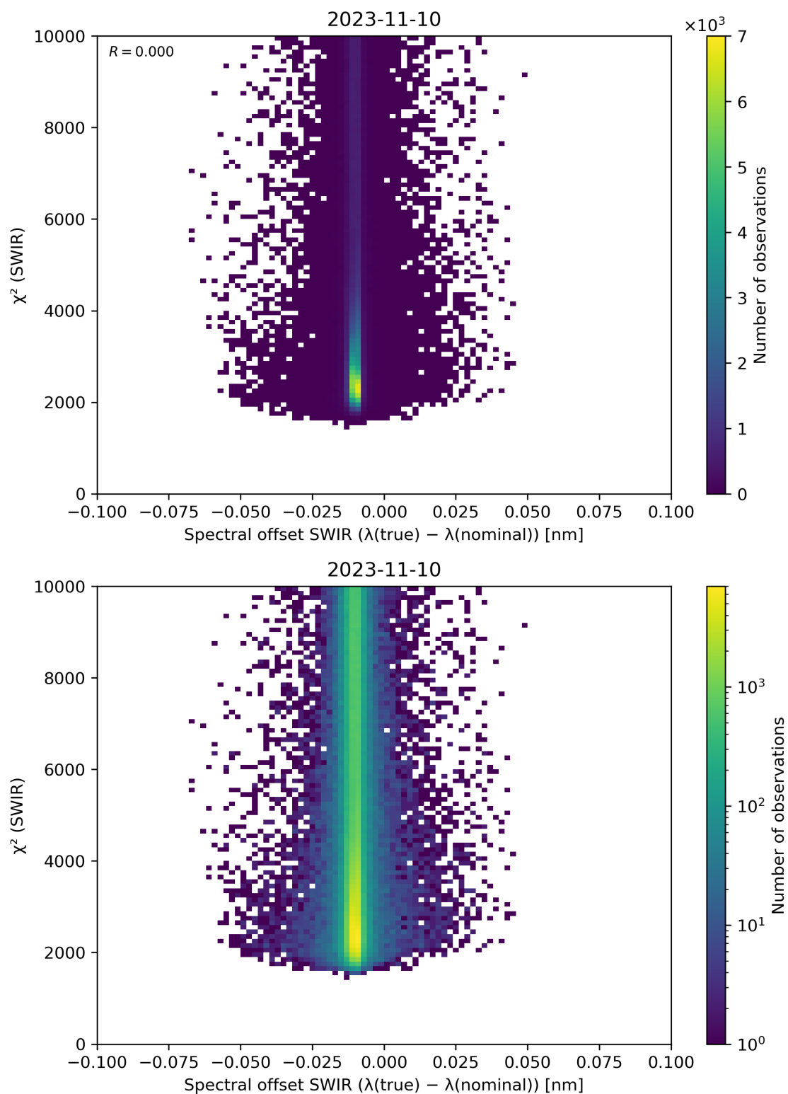
Figure 118: Scatter density plot of “Spectral offset SWIR ( \lambda(\text{true}) - \lambda(\text{nominal}) )” against “ \chi^2 (SWIR)” for 2023-11-09 to 2023-11-11.
