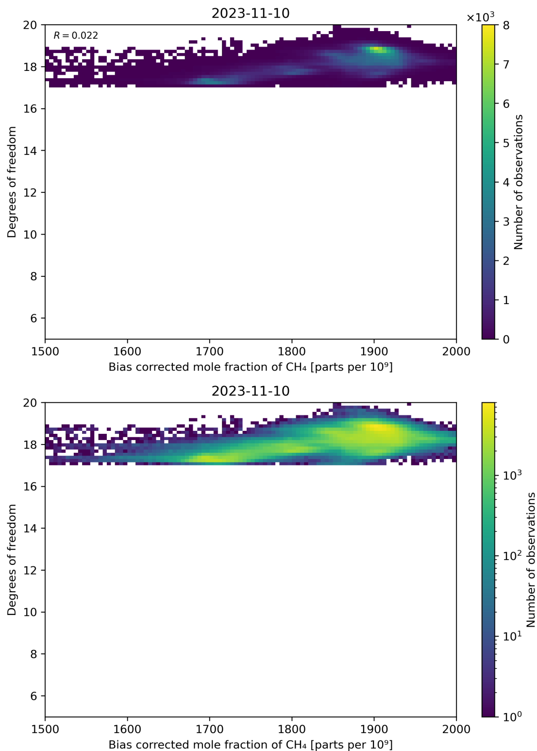
Figure 65: Scatter density plot of “Bias corrected mole fraction of CH 4 ” against “Degrees of freedom” for 2023-11-09 to 2023-11-11.
