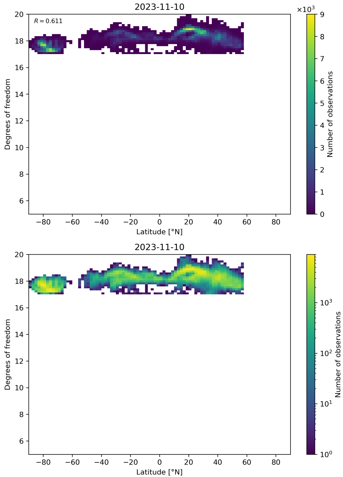
Figure 55: Scatter density plot of “Latitude” against “Degrees of freedom” for 2023-11-09 to 2023-11-11.
