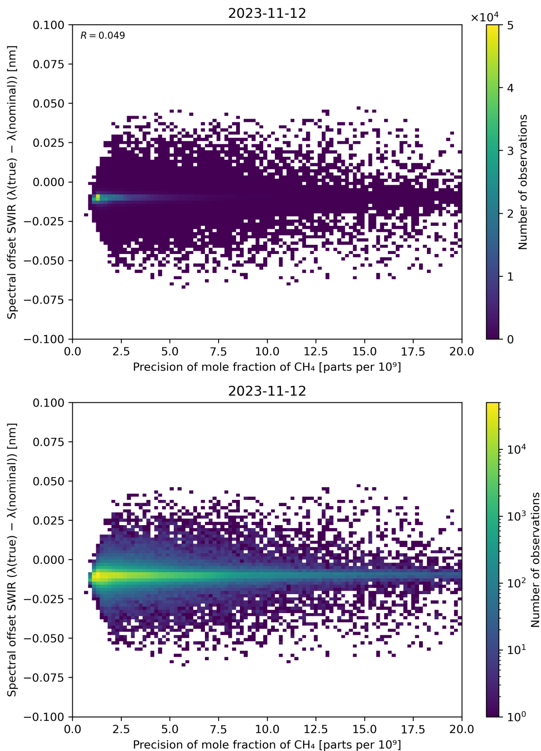
Figure 85: Scatter density plot of “Precision of mole fraction of CH 4 ” against “Spectral offset SWIR ( \lambda(\text{true}) - \lambda(\text{nominal}) )” for 2023-11-12 to 2023-11-13.
