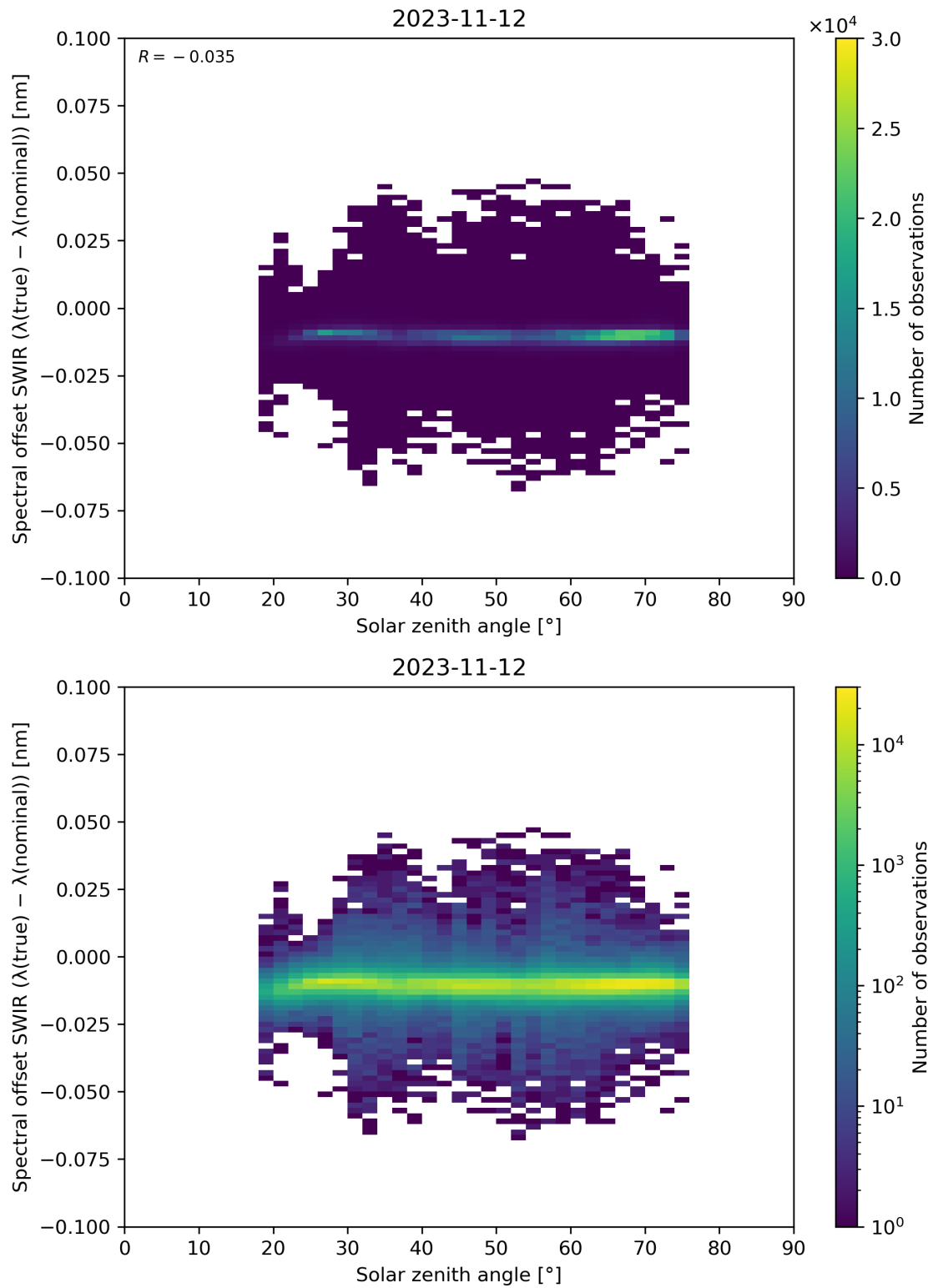
Figure 104: Scatter density plot of “Solar zenith angle” against “Spectral offset SWIR ( \lambda(\text{true}) - \lambda(\text{nominal}) )” for 2023-11-12 to 2023-11-13.
