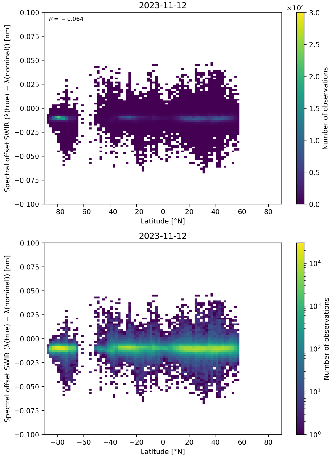
Figure 62: Scatter density plot of “Latitude” against “Spectral offset SWIR ( \lambda(\text{true}) - \lambda(\text{nominal}) )” for 2023-11-12 to 2023-11-13.
