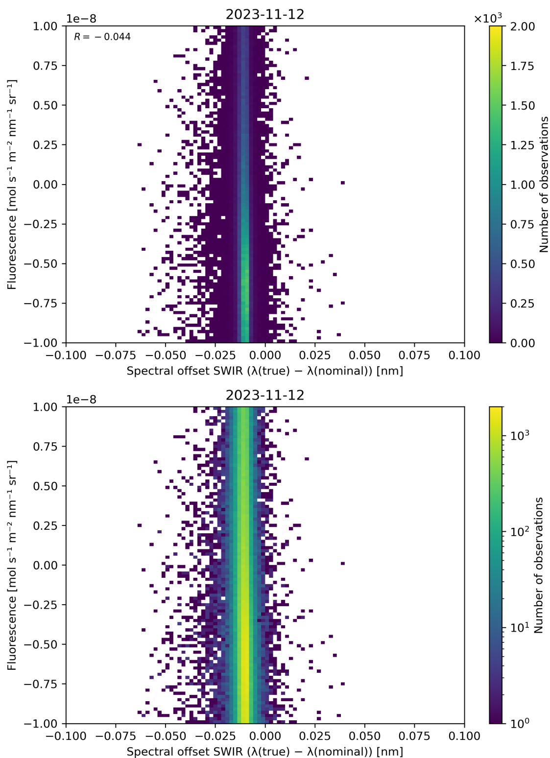
Figure 120: Scatter density plot of “Spectral offset SWIR ( \lambda(\text{true}) - \lambda(\text{nominal}) )” against “Fluorescence” for 2023-11-12 to 2023-11-13.
