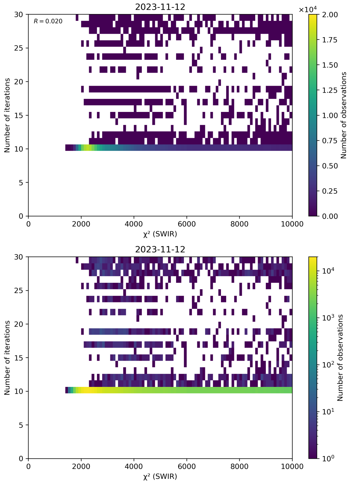
Figure 50: Scatter density plot of “ \chi^2 (SWIR)” against “Number of iterations” for 2023-11-12 to 2023-11-13.
