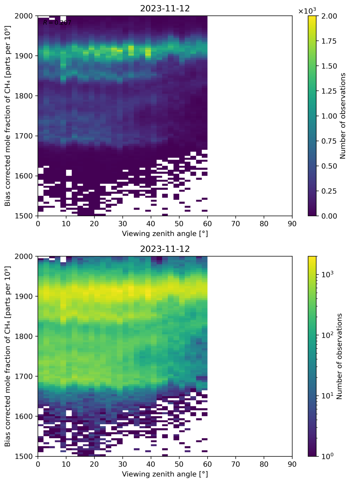
Figure 111: Scatter density plot of “Viewing zenith angle” against “Bias corrected mole fraction of CH 4 ” for 2023-11-12 to 2023-11-13.
