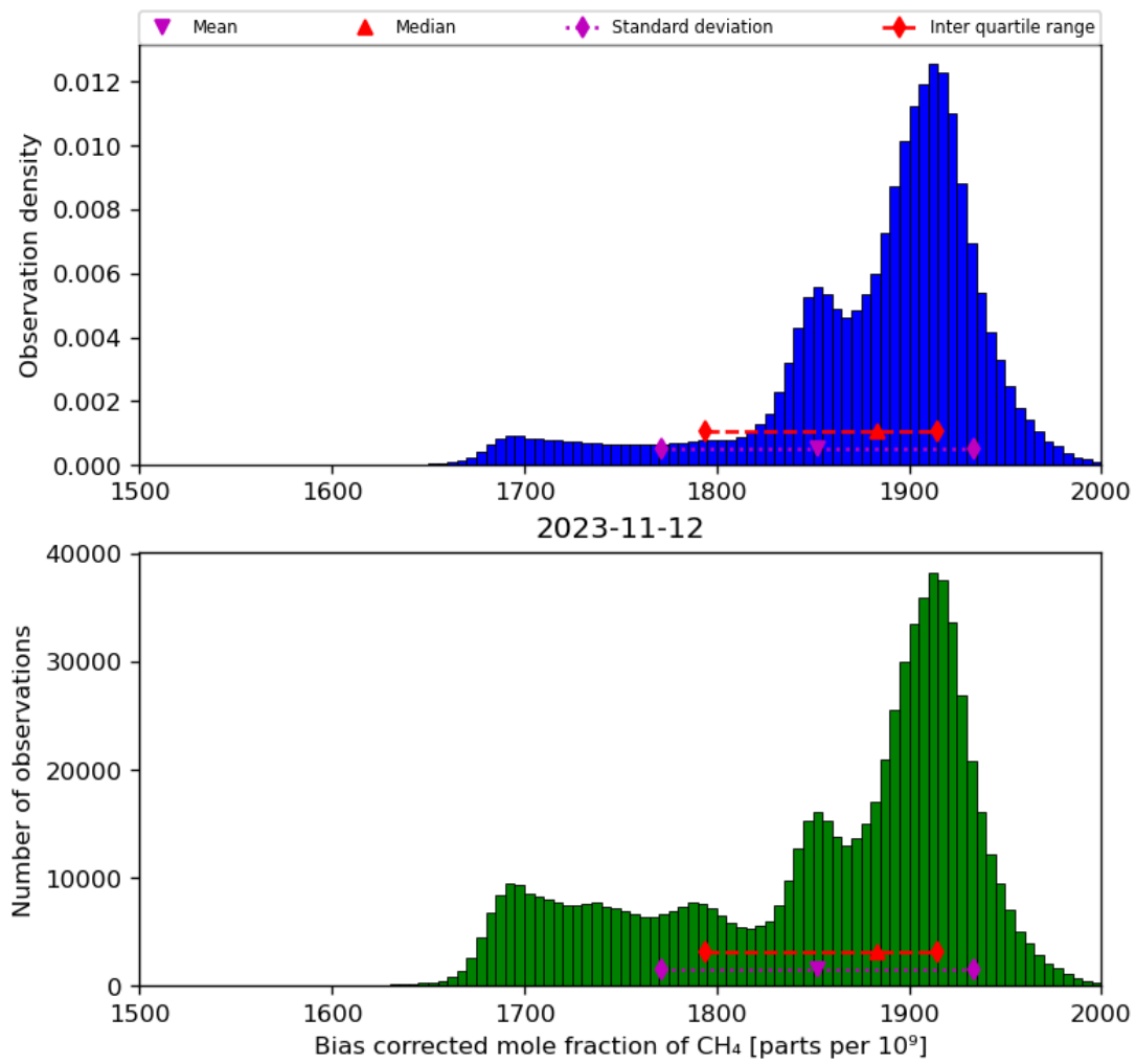
Figure 25: Histogram of “Bias corrected mole fraction of CH 4 ” for 2023-11-12 to 2023-11-13
