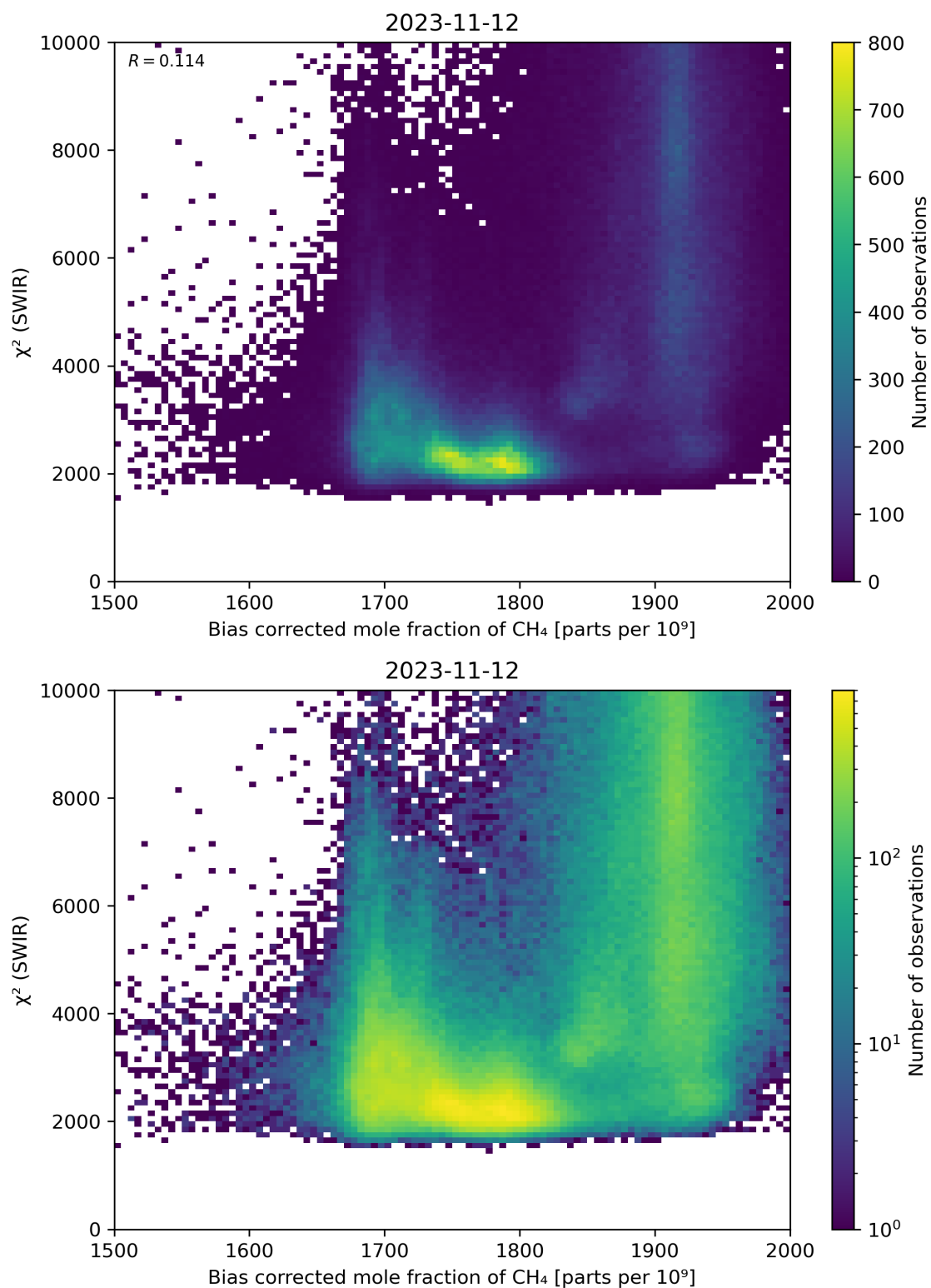
Figure 64: Scatter density plot of “Bias corrected mole fraction of CH 4 ” against “ \chi^2 (SWIR)” for 2023-11-12 to 2023-11-13.
