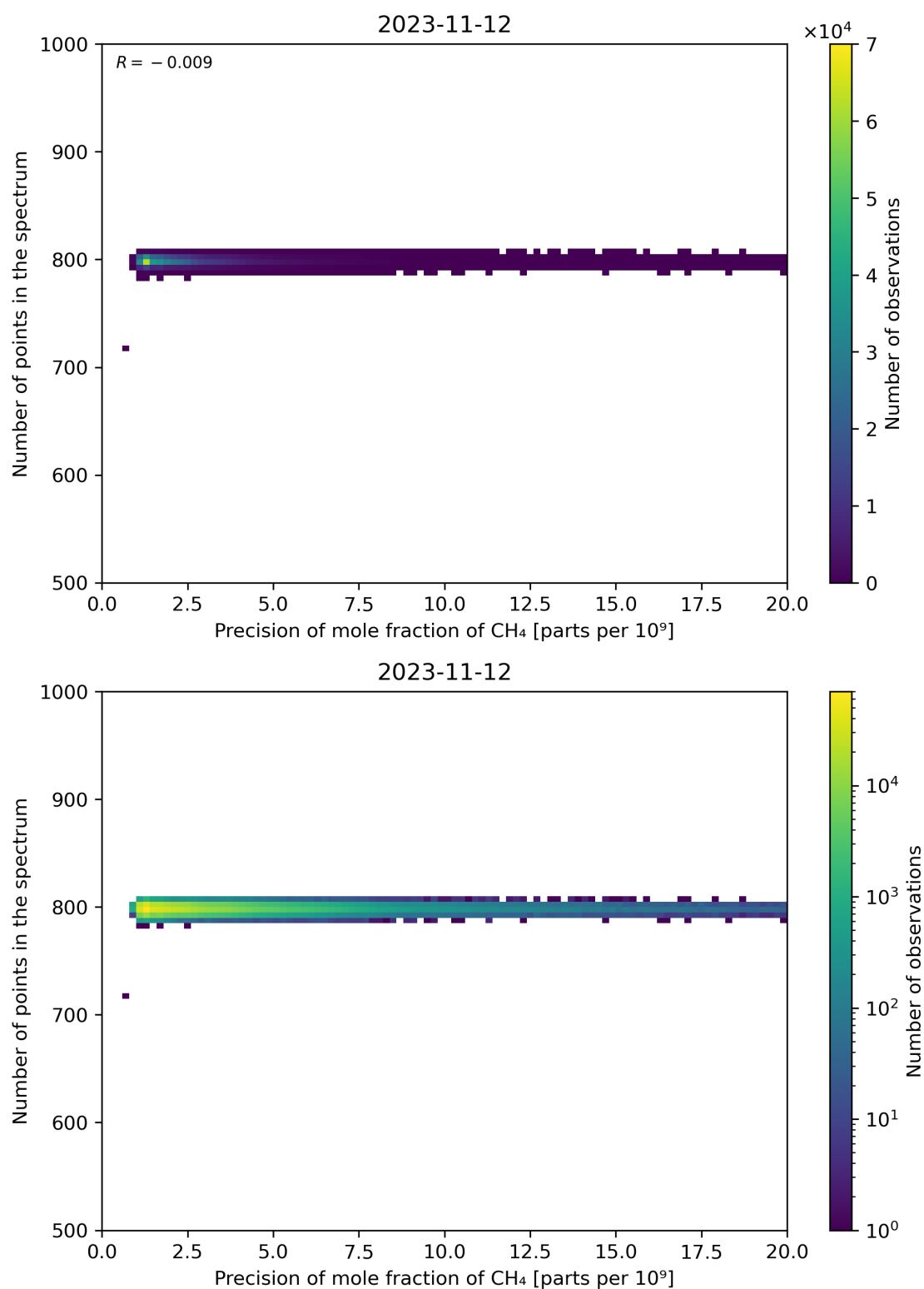
Figure 84: Scatter density plot of “Precision of mole fraction of CH 4 ” against “Number of points in the spectrum” for 2023-11-12 to 2023-11-13.
