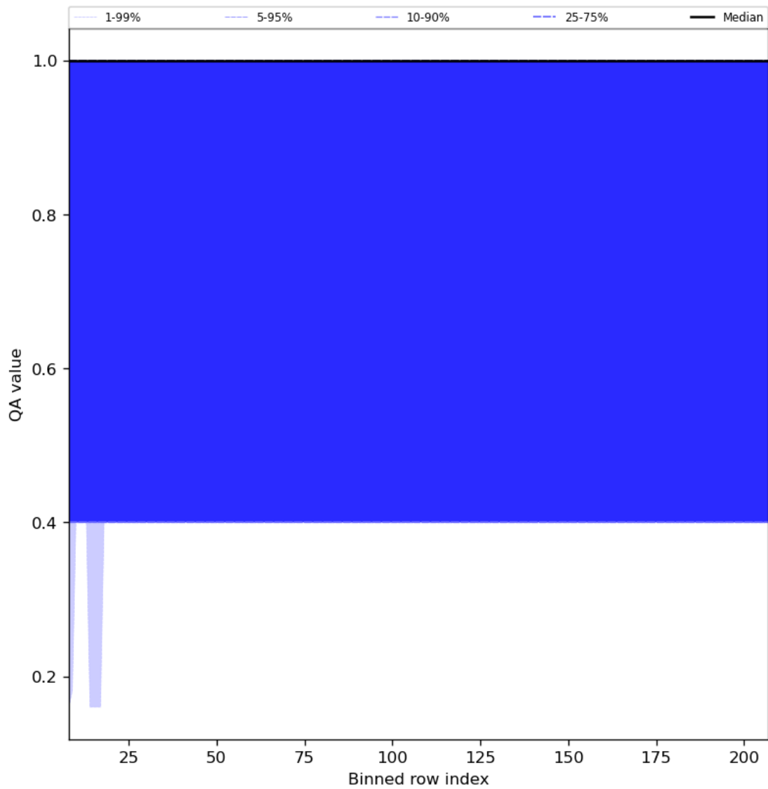
Figure 33: Along track statistics of “QA value” for 2023-11-12 to 2023-11-13
