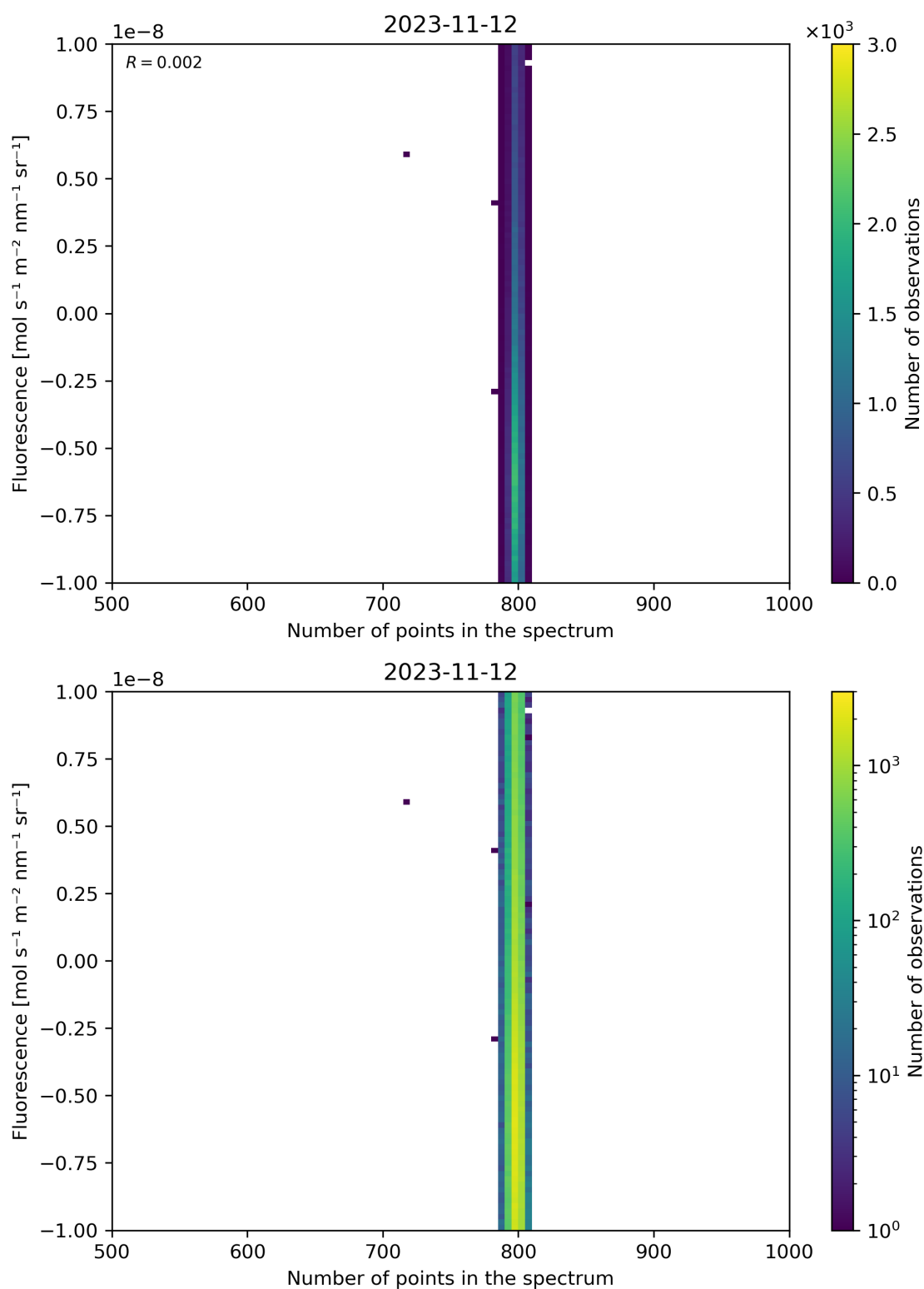
Figure 91: Scatter density plot of “Number of points in the spectrum” against “Fluorescence” for 2023-11-12 to 2023-11-13.
