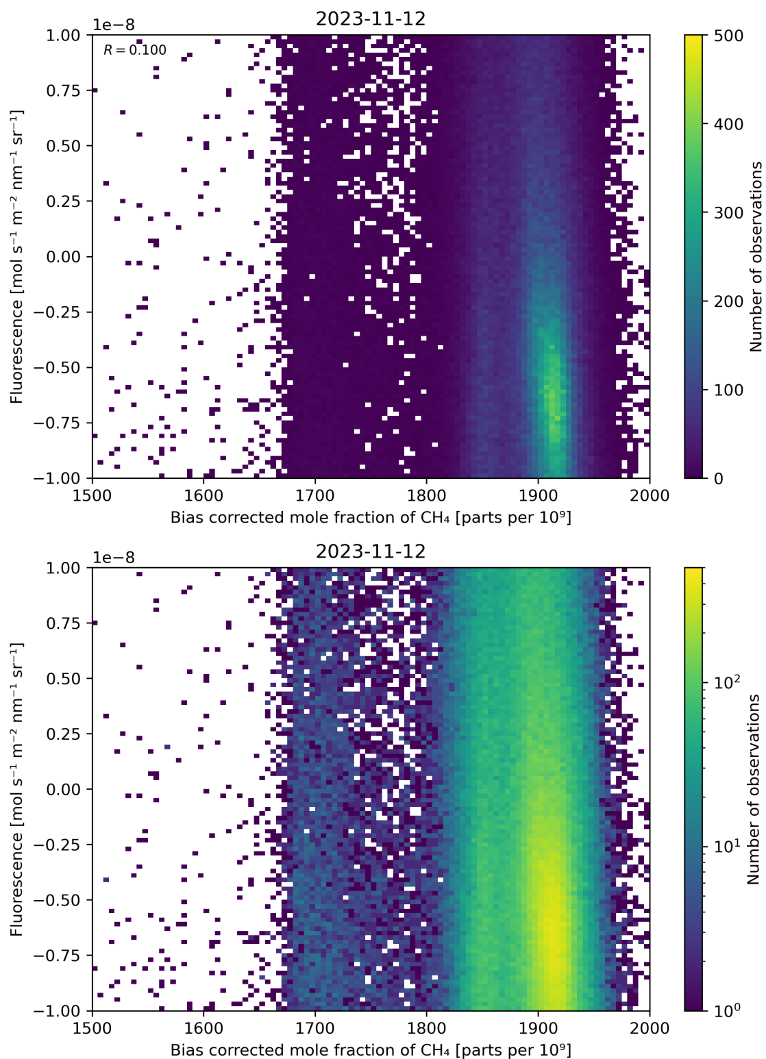
Figure 66: Scatter density plot of “Bias corrected mole fraction of CH 4 ” against “Fluorescence” for 2023-11-12 to 2023-11-13.
