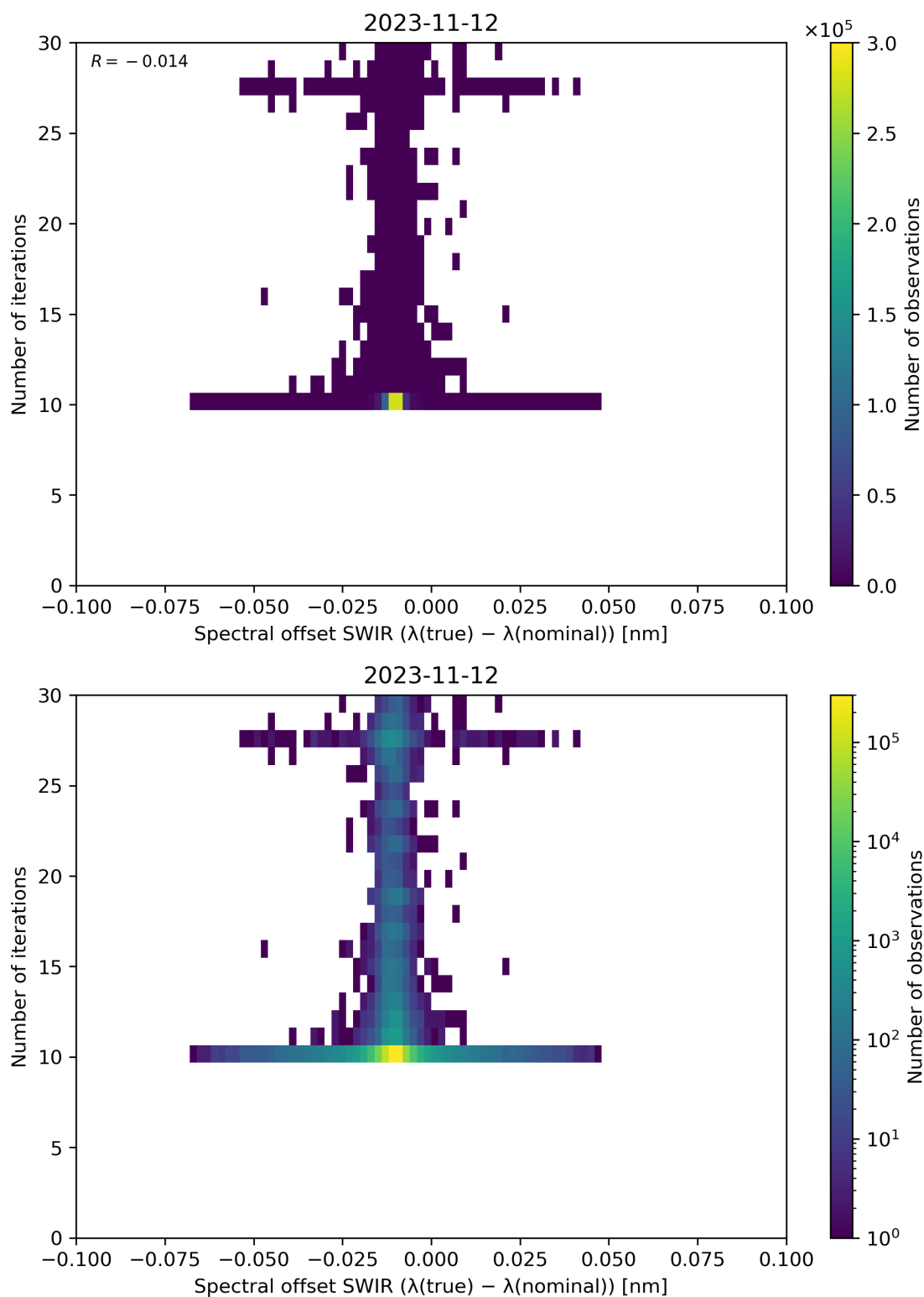
Figure 121: Scatter density plot of “Spectral offset SWIR ( \lambda(\text{true}) - \lambda(\text{nominal}) )” against “Number of iterations” for 2023-11-12 to 2023-11-13.
