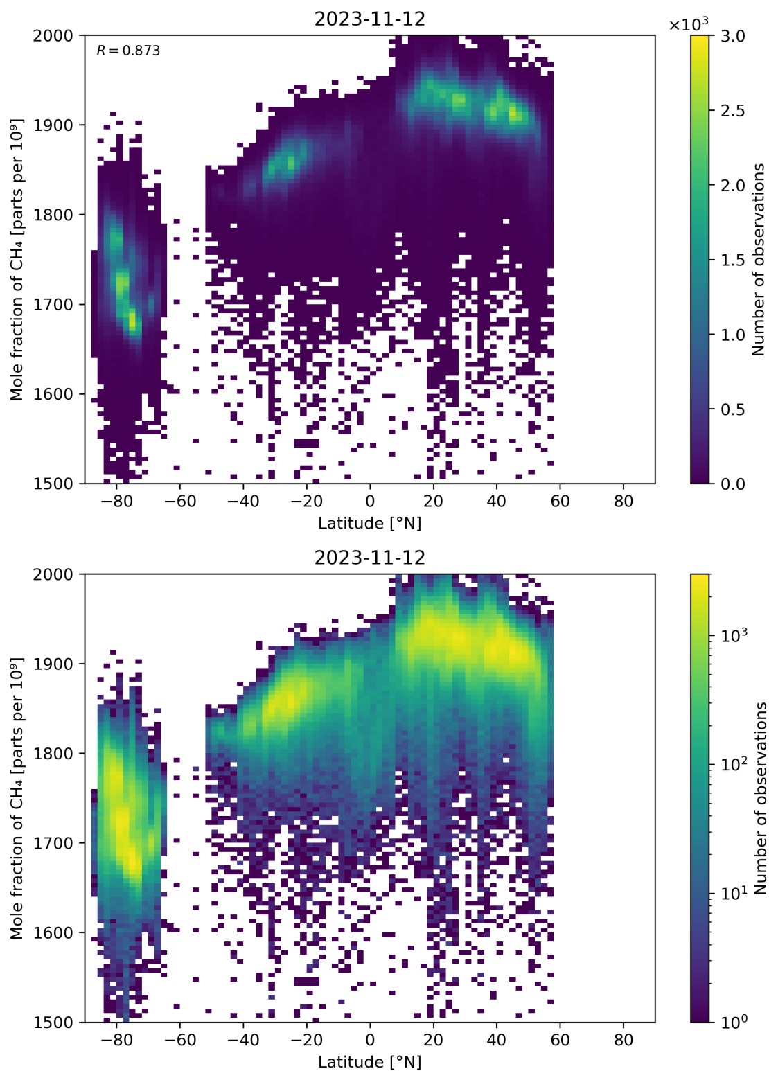
Figure 57: Scatter density plot of “Latitude” against “Mole fraction of CH 4 ” for 2023-11-12 to 2023-11-13.
