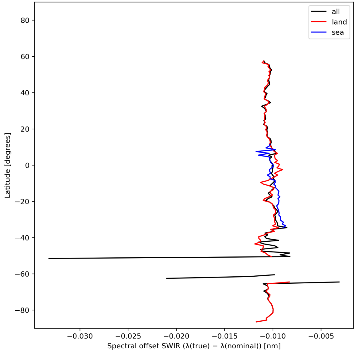
Figure 16: Zonal average of “Spectral offset SWIR ( \lambda(\text{true}) - \lambda(\text{nominal}) )” for 2023-11-12 to 2023-11-13.
