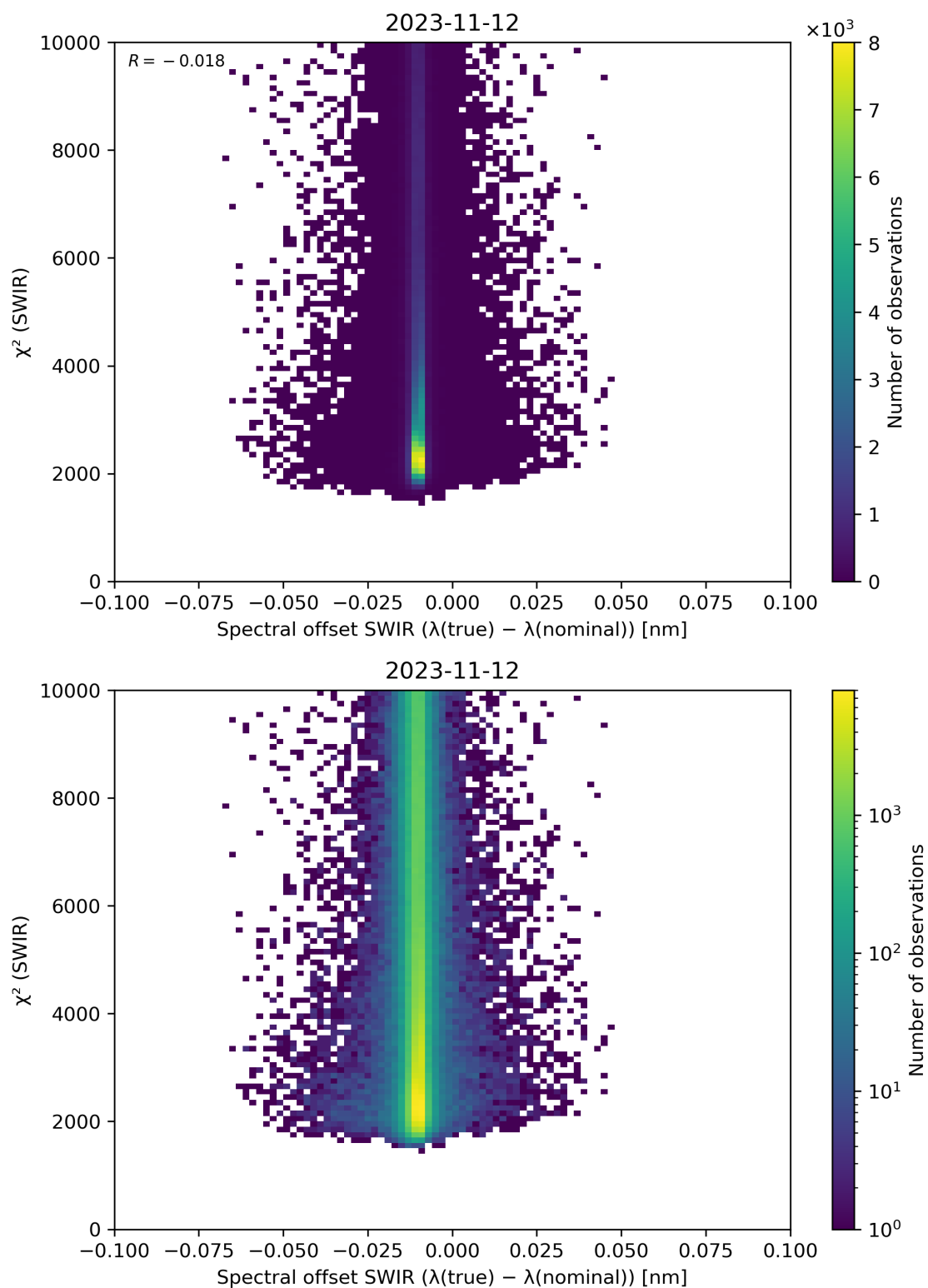
Figure 118: Scatter density plot of “Spectral offset SWIR ( \lambda(\text{true}) - \lambda(\text{nominal}) )” against “ \chi^2 (SWIR)” for 2023-11-12 to 2023-11-13.
