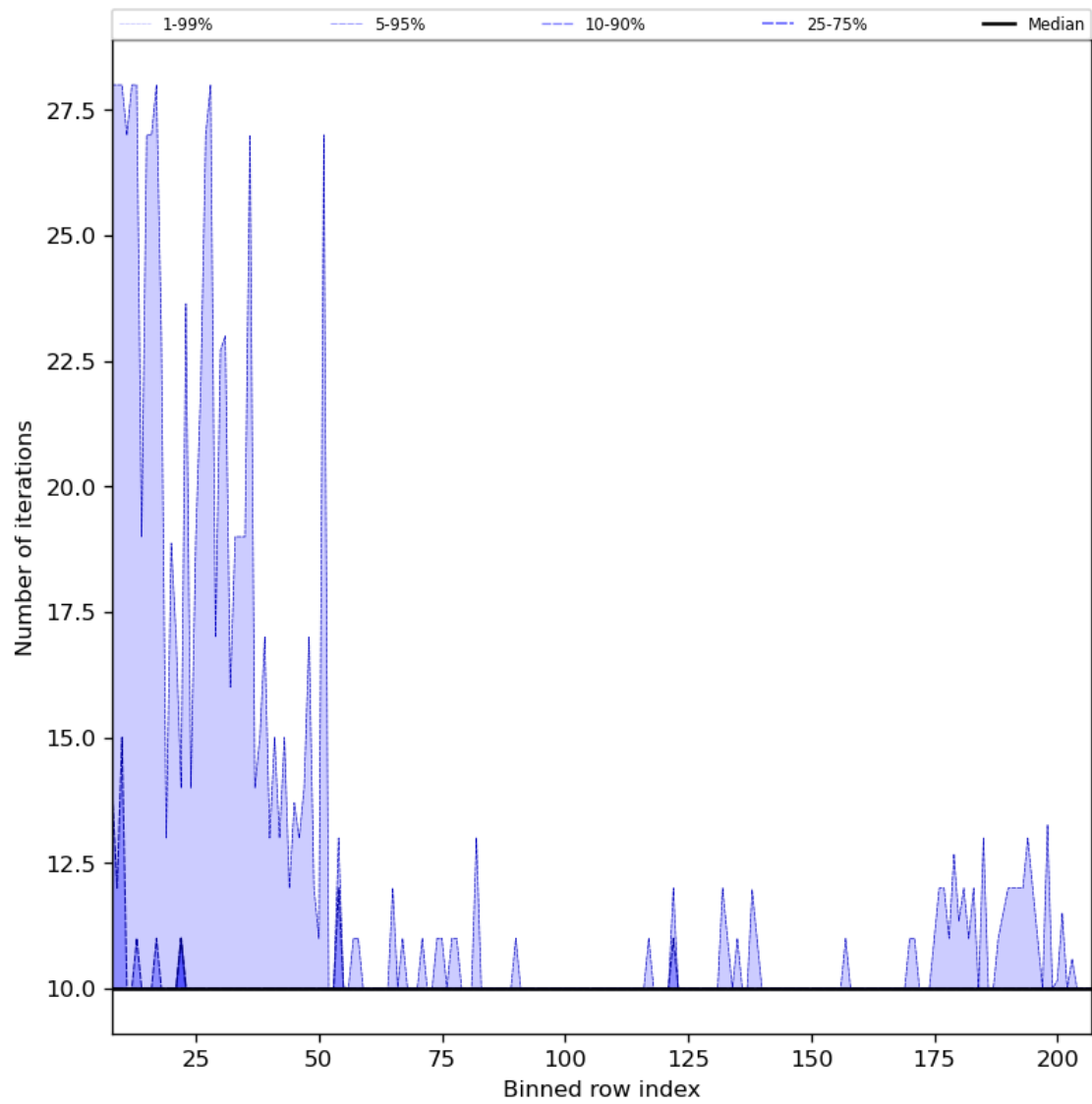
Figure 42: Along track statistics of “Number of iterations” for 2023-11-12 to 2023-11-13
