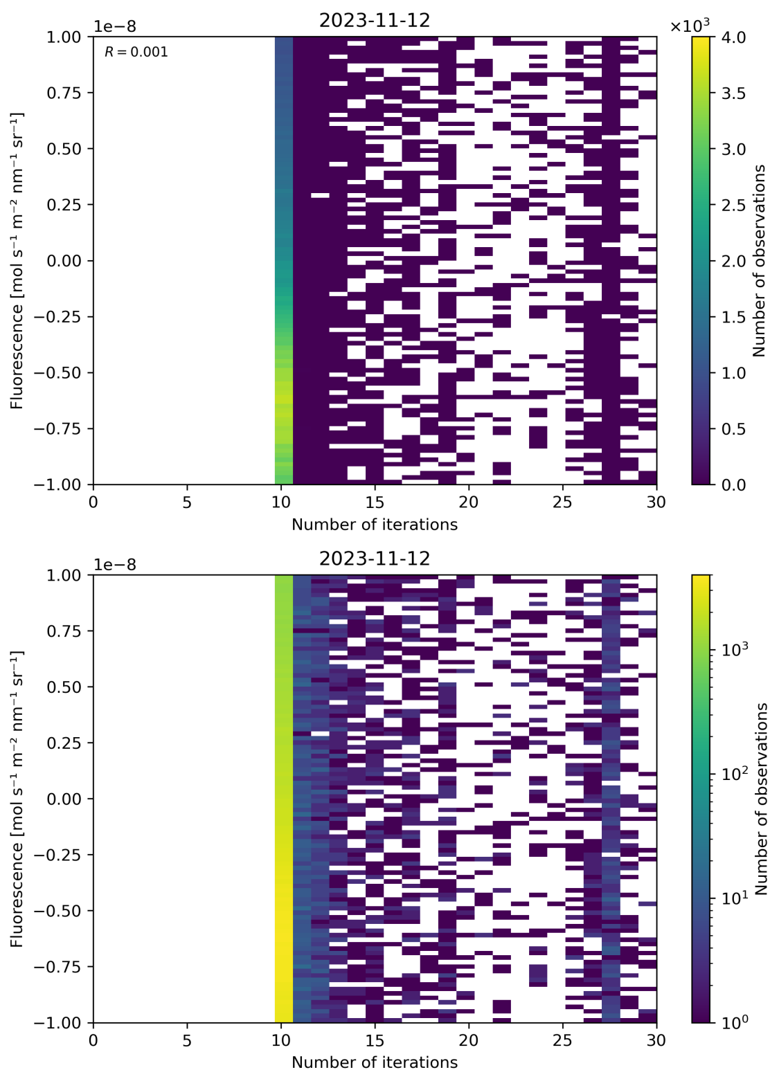
Figure 87: Scatter density plot of “Number of iterations” against “Fluorescence” for 2023-11-12 to 2023-11-13.
