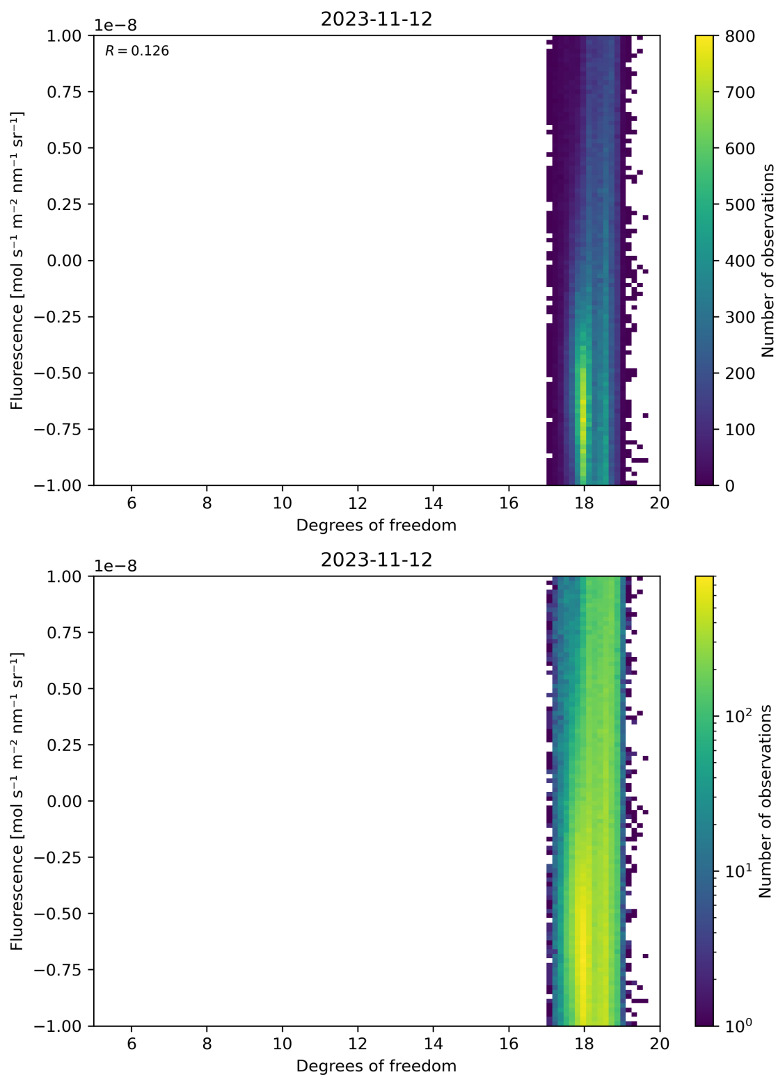
Figure 51: Scatter density plot of “Degrees of freedom” against “Fluorescence” for 2023-11-12 to 2023-11-13.
