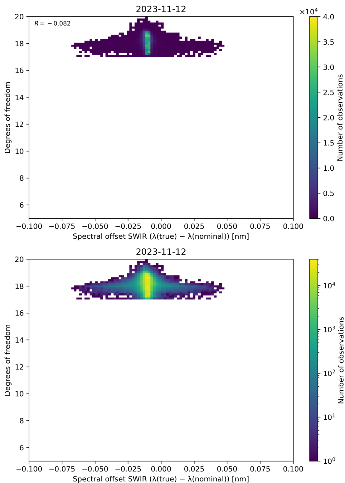
Figure 119: Scatter density plot of “Spectral offset SWIR ( \lambda(\text{true}) - \lambda(\text{nominal}) )” against “Degrees of freedom” for 2023-11-12 to 2023-11-13.
