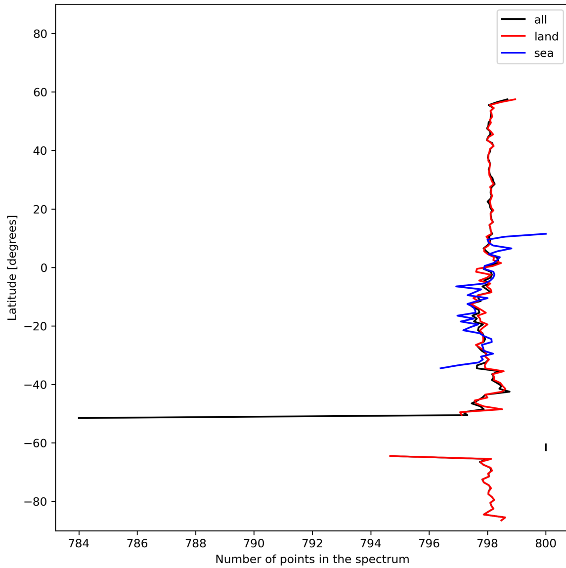
Figure 15: Zonal average of “Number of points in the spectrum” for 2023-11-12 to 2023-11-13.
