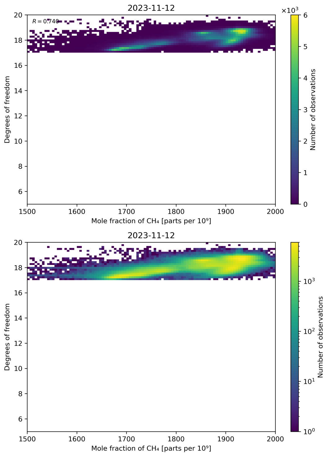
Figure 72: Scatter density plot of “Mole fraction of CH 4 ” against “Degrees of freedom” for 2023-11-12 to 2023-11-13.
