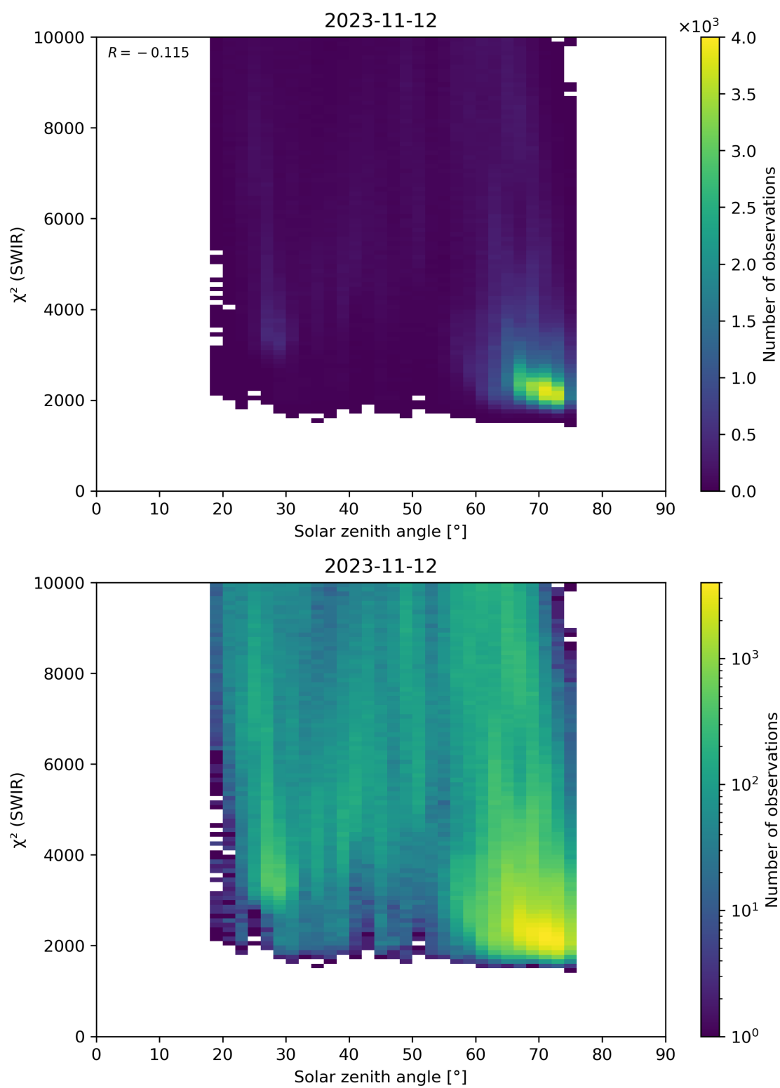
Figure 95: Scatter density plot of “Solar zenith angle” against “ \chi^2 (SWIR)” for 2023-11-12 to 2023-11-13.
