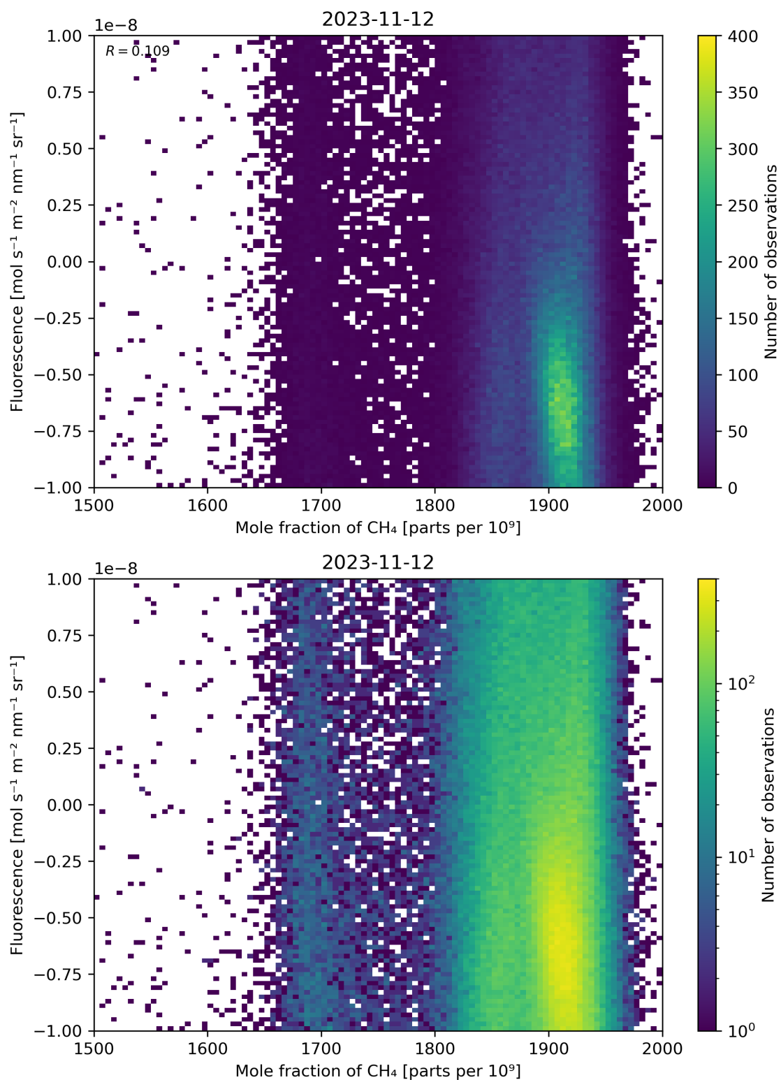
Figure 73: Scatter density plot of “Mole fraction of \text{CH}_4 ” against “Fluorescence” for 2023-11-12 to 2023-11-13.
