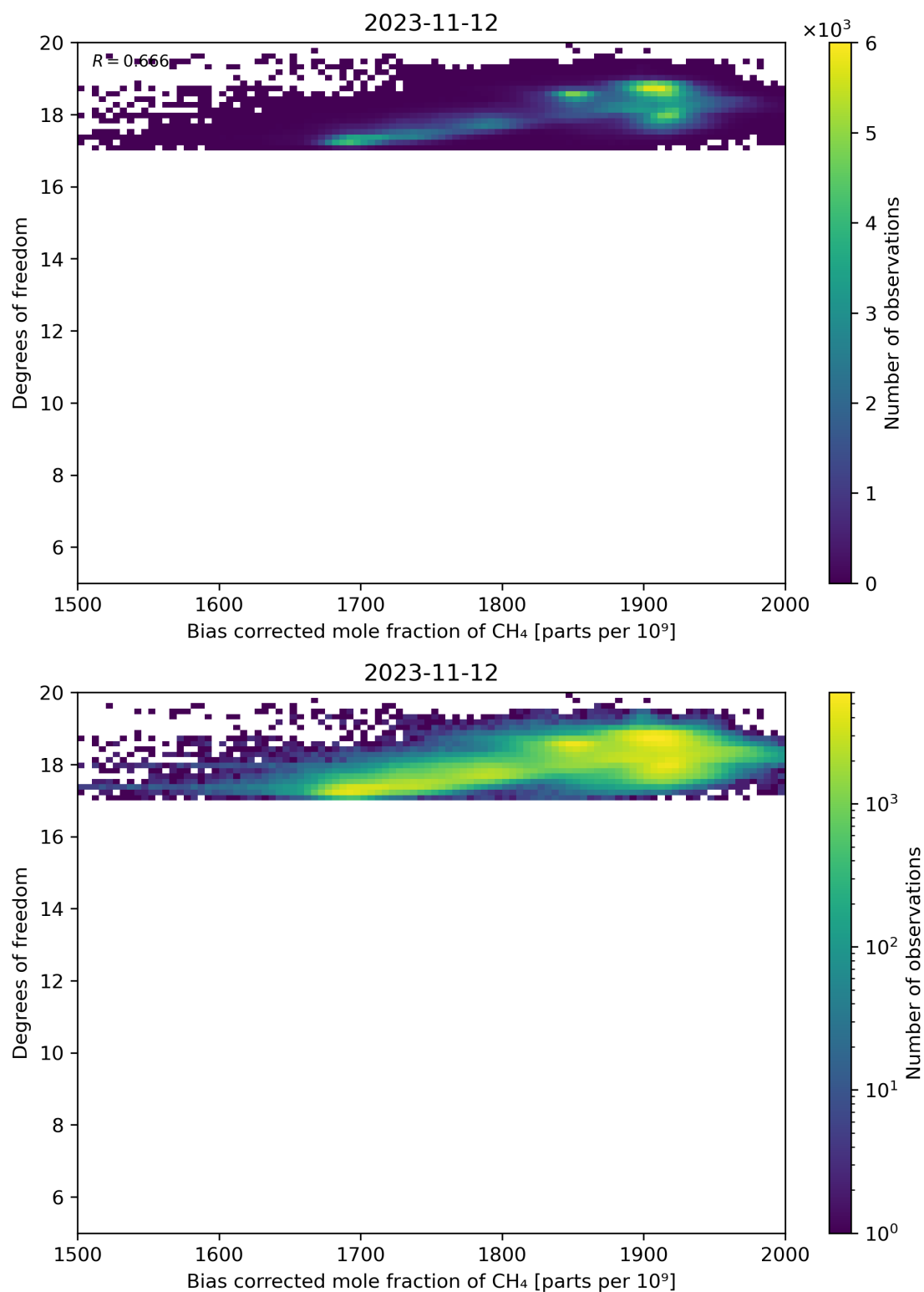
Figure 65: Scatter density plot of “Bias corrected mole fraction of CH 4 ” against “Degrees of freedom” for 2023-11-12 to 2023-11-13.
