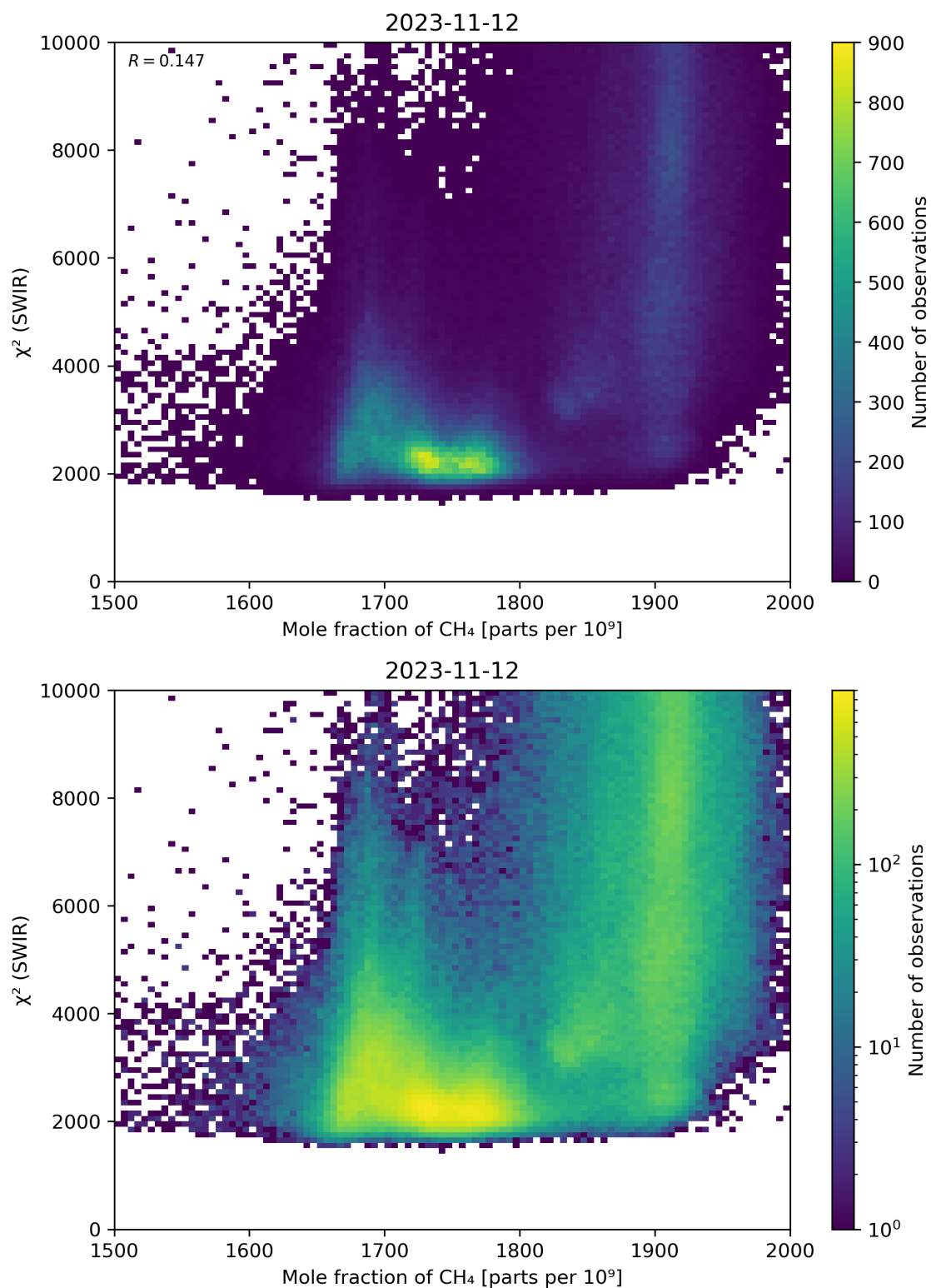
Figure 71: Scatter density plot of “Mole fraction of \text{CH}_4 ” against “ \chi^2 (SWIR)” for 2023-11-12 to 2023-11-13.
