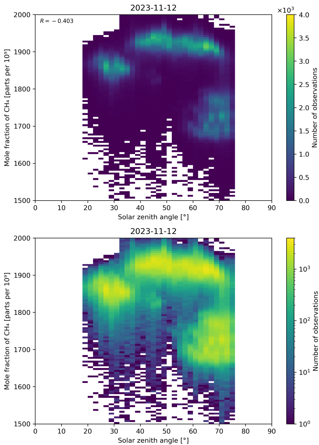
Figure 99: Scatter density plot of “Solar zenith angle” against “Mole fraction of CH 4 ” for 2023-11-12 to 2023-11-13.
