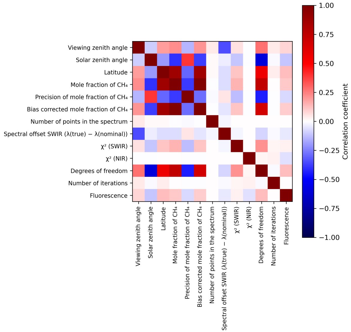
Figure 2: Map of correlation matrix for 2023-11-12 to 2023-11-13.
