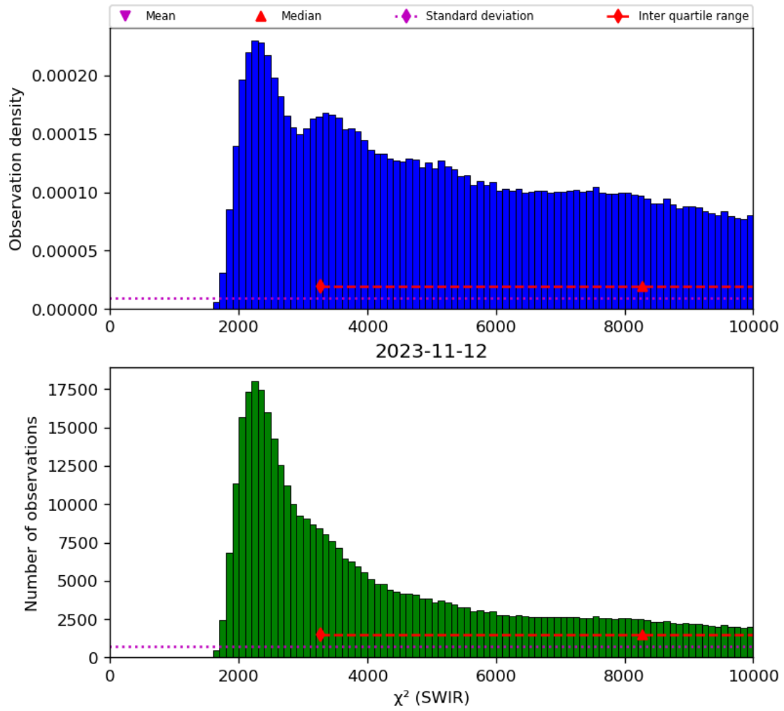
Figure 28: Histogram of “ \chi^2 (SWIR)” for 2023-11-12 to 2023-11-13
