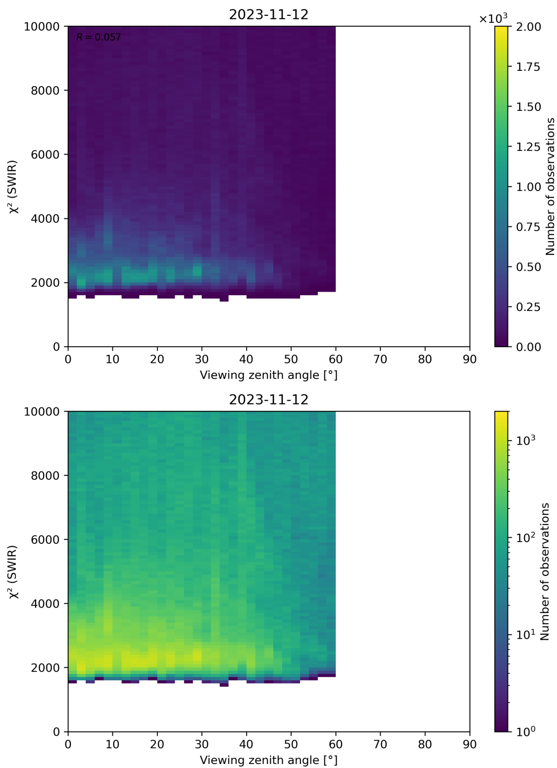
Figure 106: Scatter density plot of “Viewing zenith angle” against “ \chi^2 (SWIR)” for 2023-11-12 to 2023-11-13.
