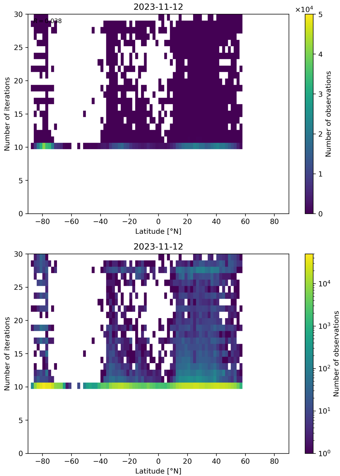
Figure 60: Scatter density plot of “Latitude” against “Number of iterations” for 2023-11-12 to 2023-11-13.
