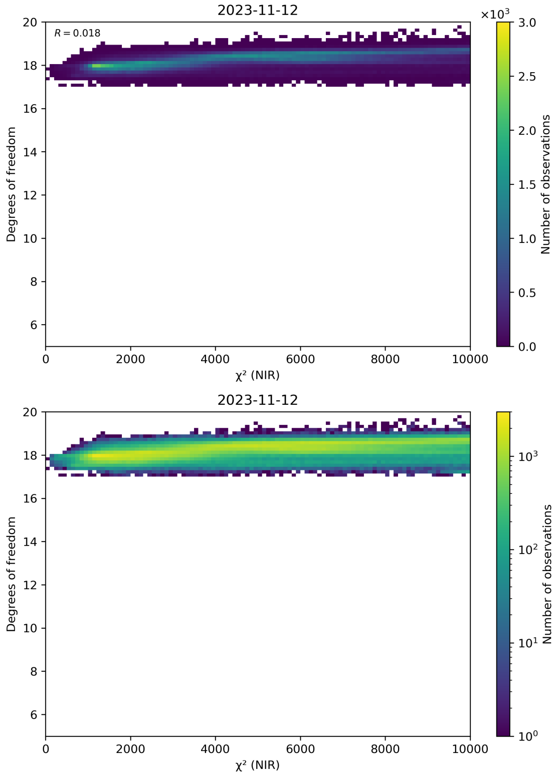
Figure 44: Scatter density plot of “ \chi^2 (NIR)” against “Degrees of freedom” for 2023-11-12 to 2023-11-13.
