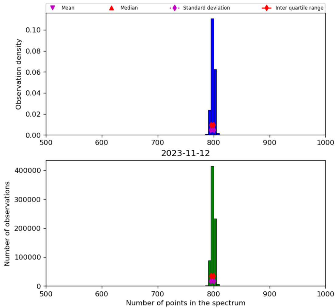
Figure 26: Histogram of “Number of points in the spectrum” for 2023-11-12 to 2023-11-13
