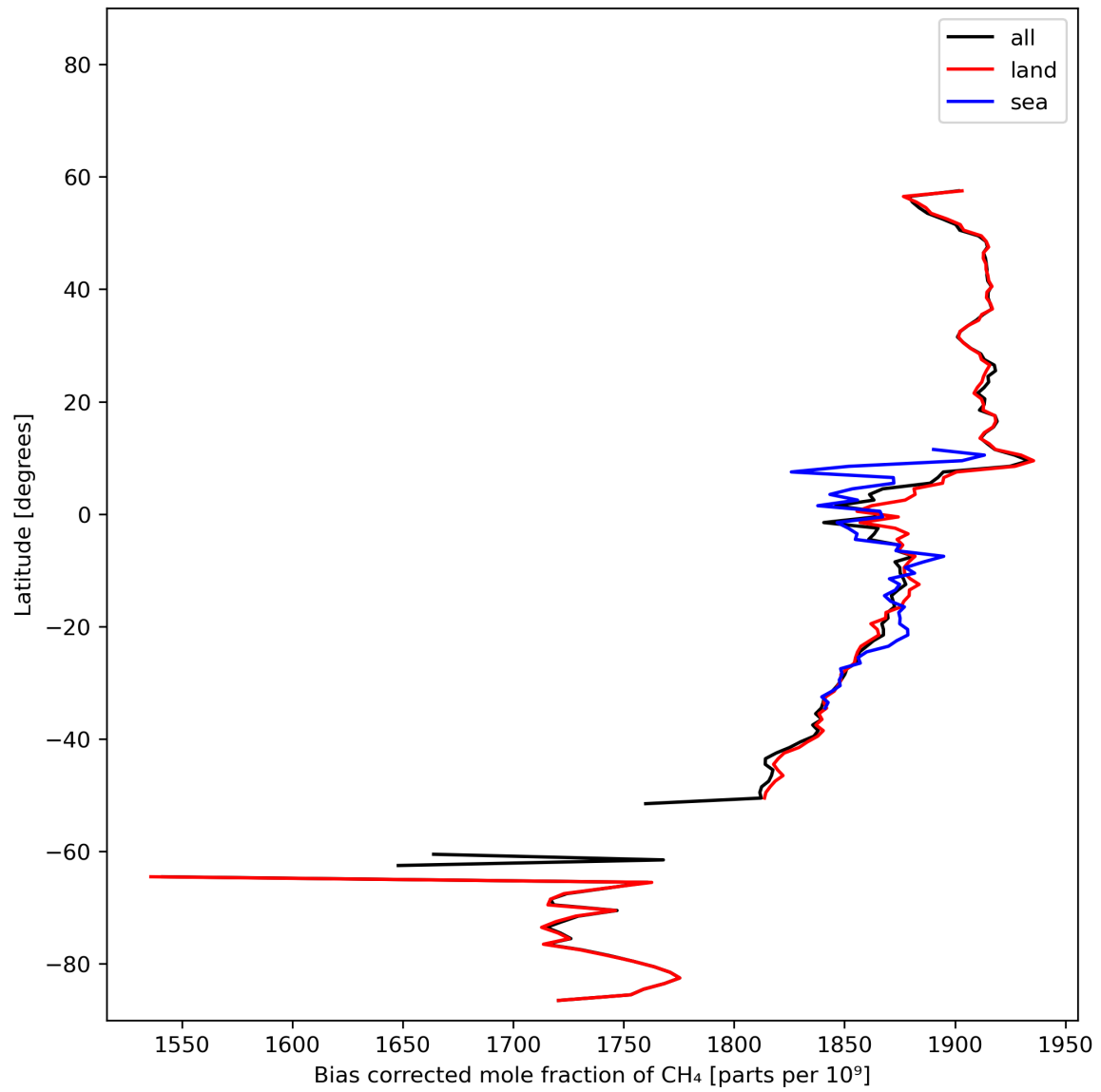
Figure 14: Zonal average of “Bias corrected mole fraction of CH 4 ” for 2023-11-12 to 2023-11-13.
