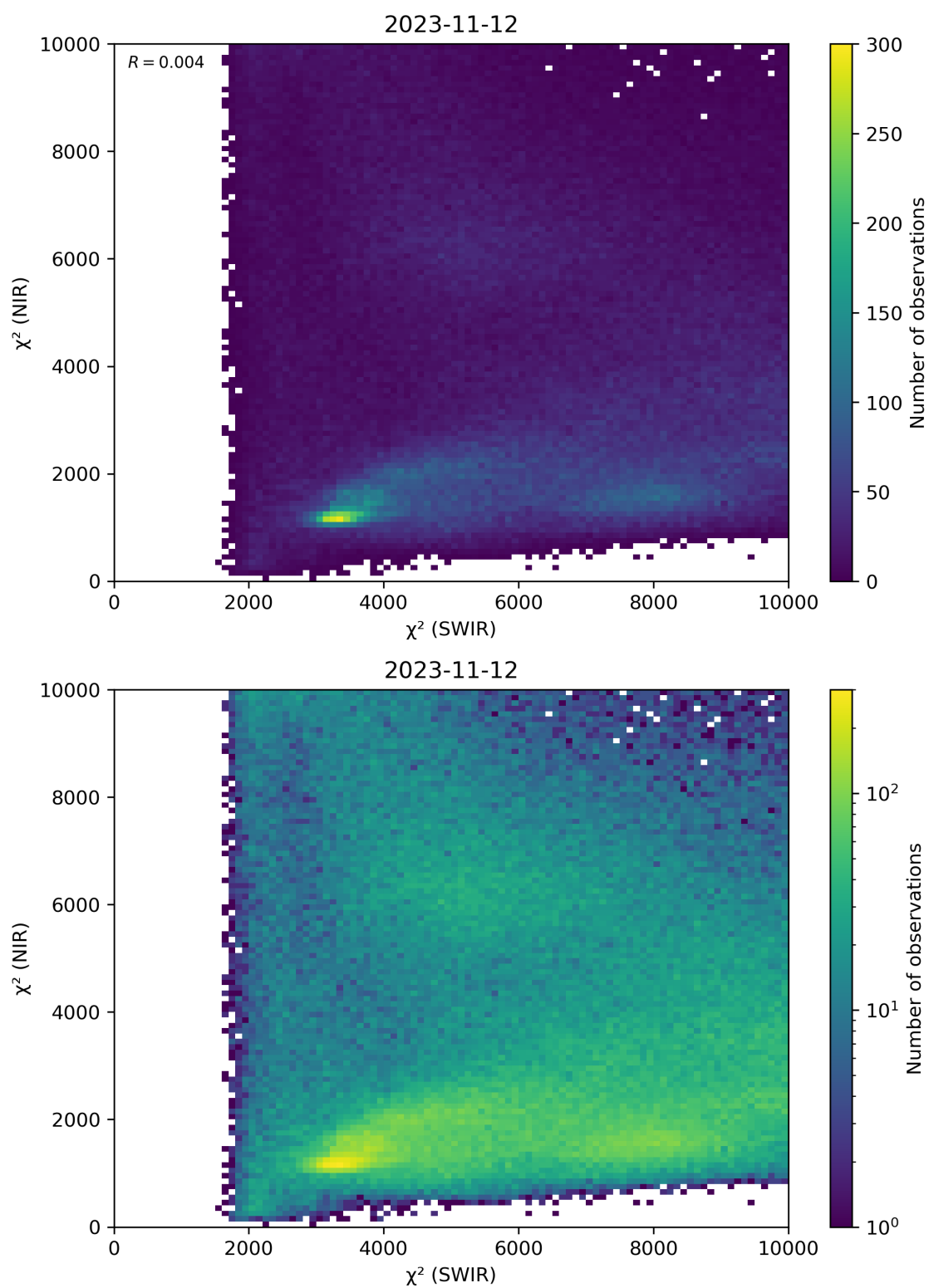
Figure 47: Scatter density plot of “ \chi^2 (SWIR)” against “ \chi^2 (NIR)” for 2023-11-12 to 2023-11-13.
