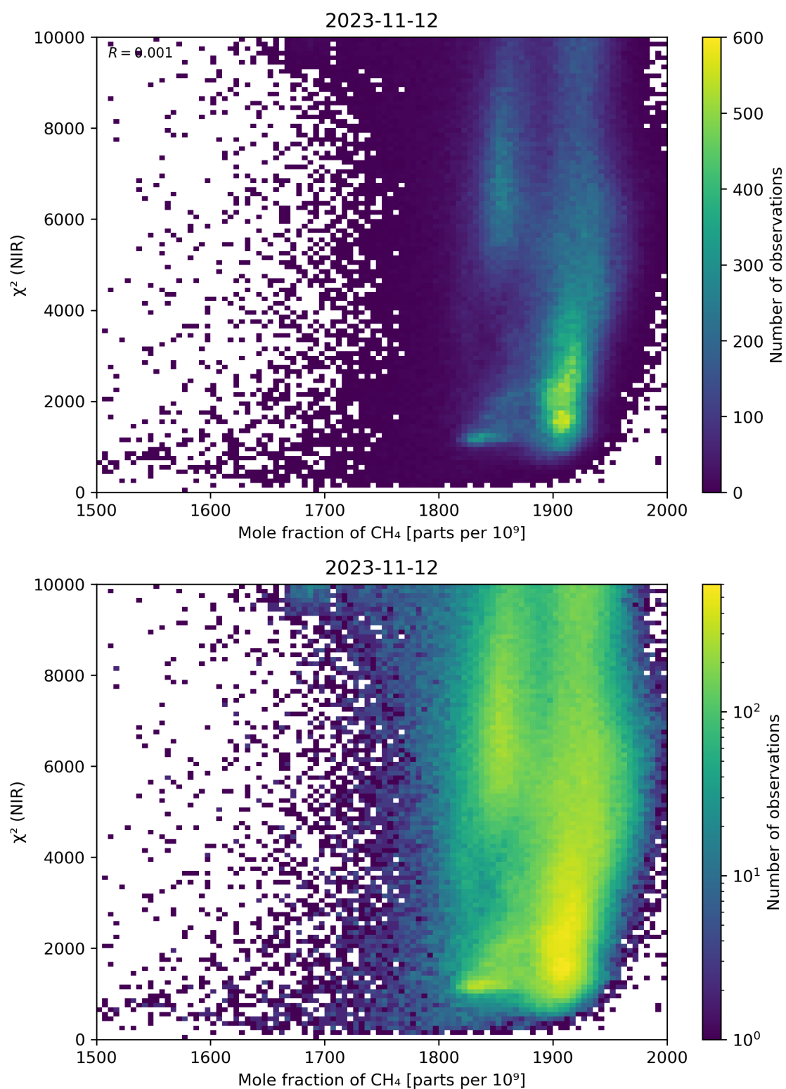
Figure 70: Scatter density plot of “Mole fraction of CH 4 ” against “ \chi^2 (NIR)” for 2023-11-12 to 2023-11-13.
