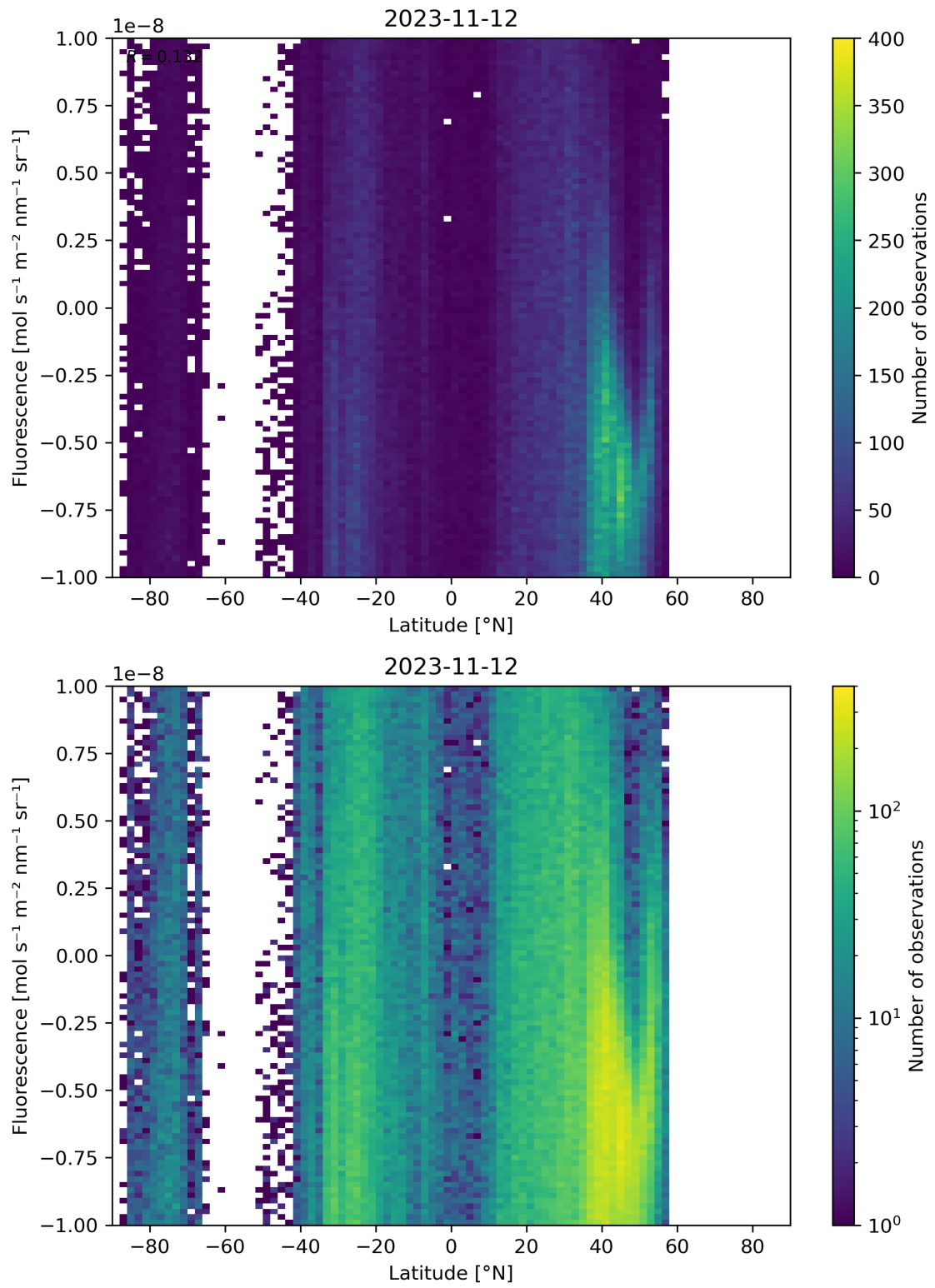
Figure 56: Scatter density plot of “Latitude” against “Fluorescence” for 2023-11-12 to 2023-11-13.
