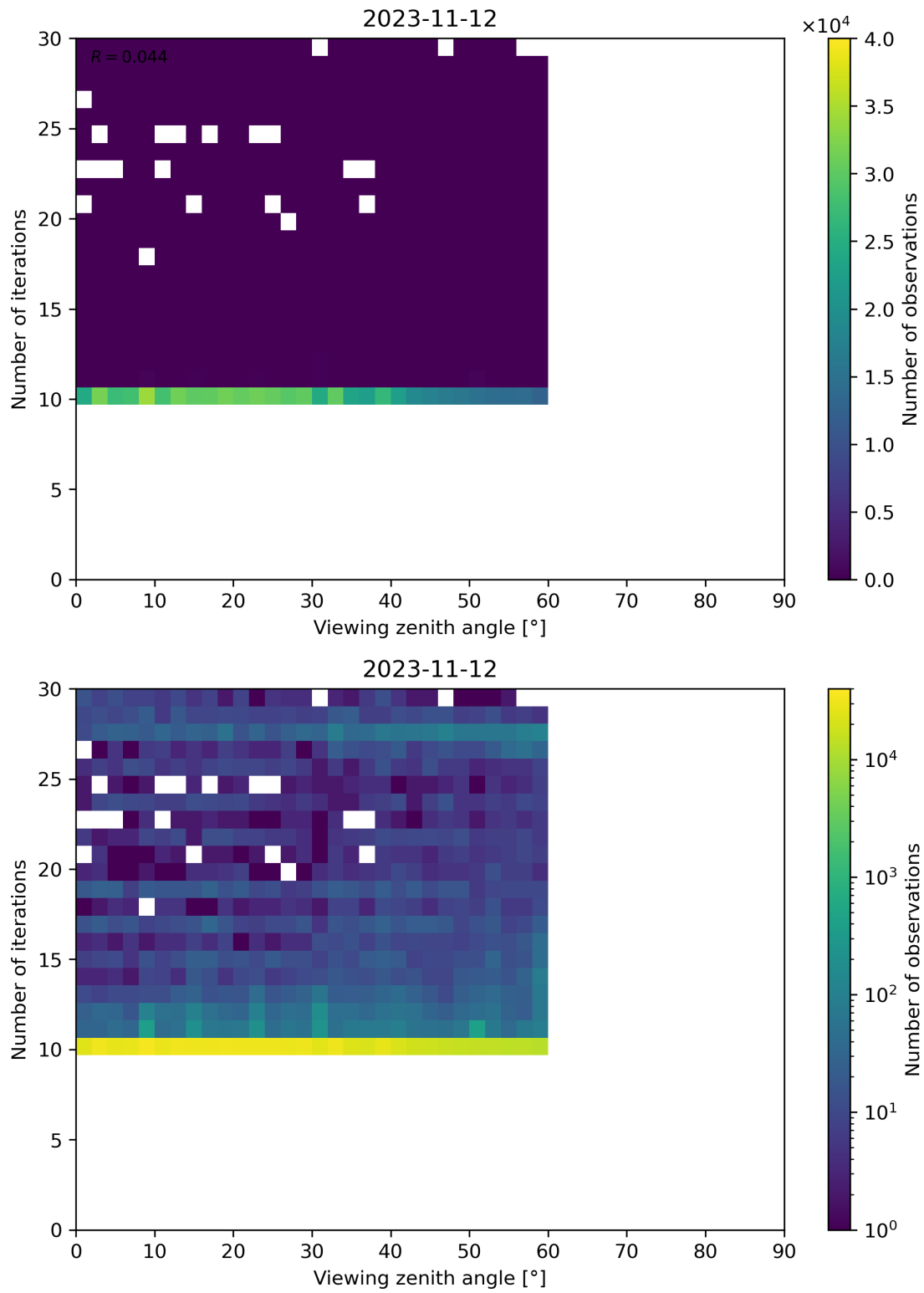
Figure 113: Scatter density plot of “Viewing zenith angle” against “Number of iterations” for 2023-11-12 to 2023-11-13.
