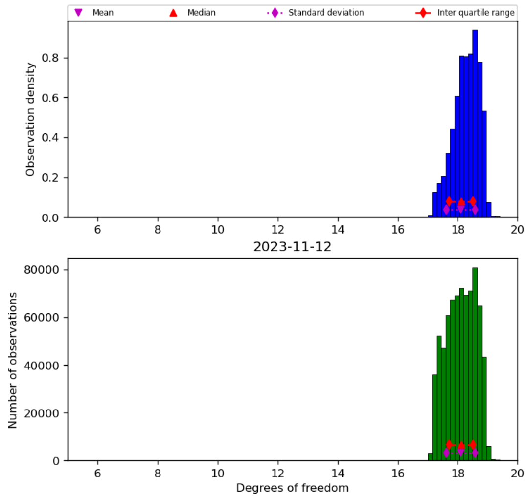
Figure 30: Histogram of “Degrees of freedom” for 2023-11-12 to 2023-11-13
