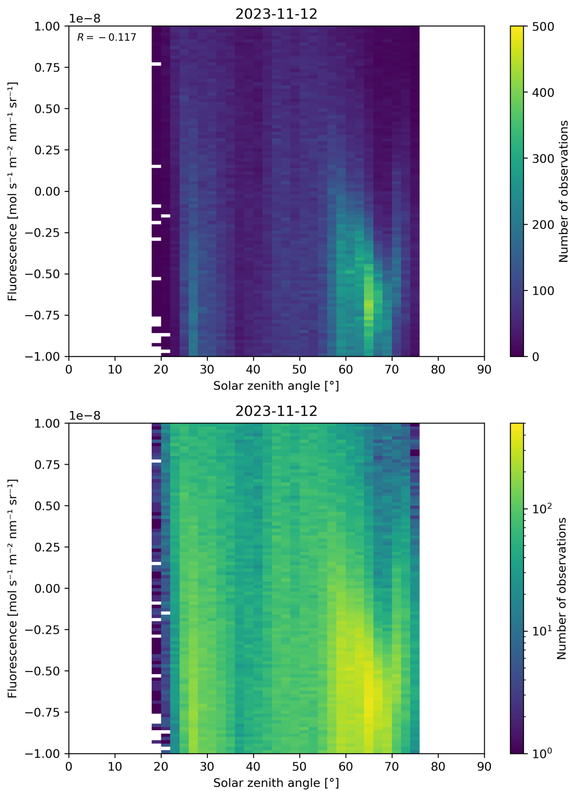
Figure 97: Scatter density plot of “Solar zenith angle” against “Fluorescence” for 2023-11-12 to 2023-11-13.
