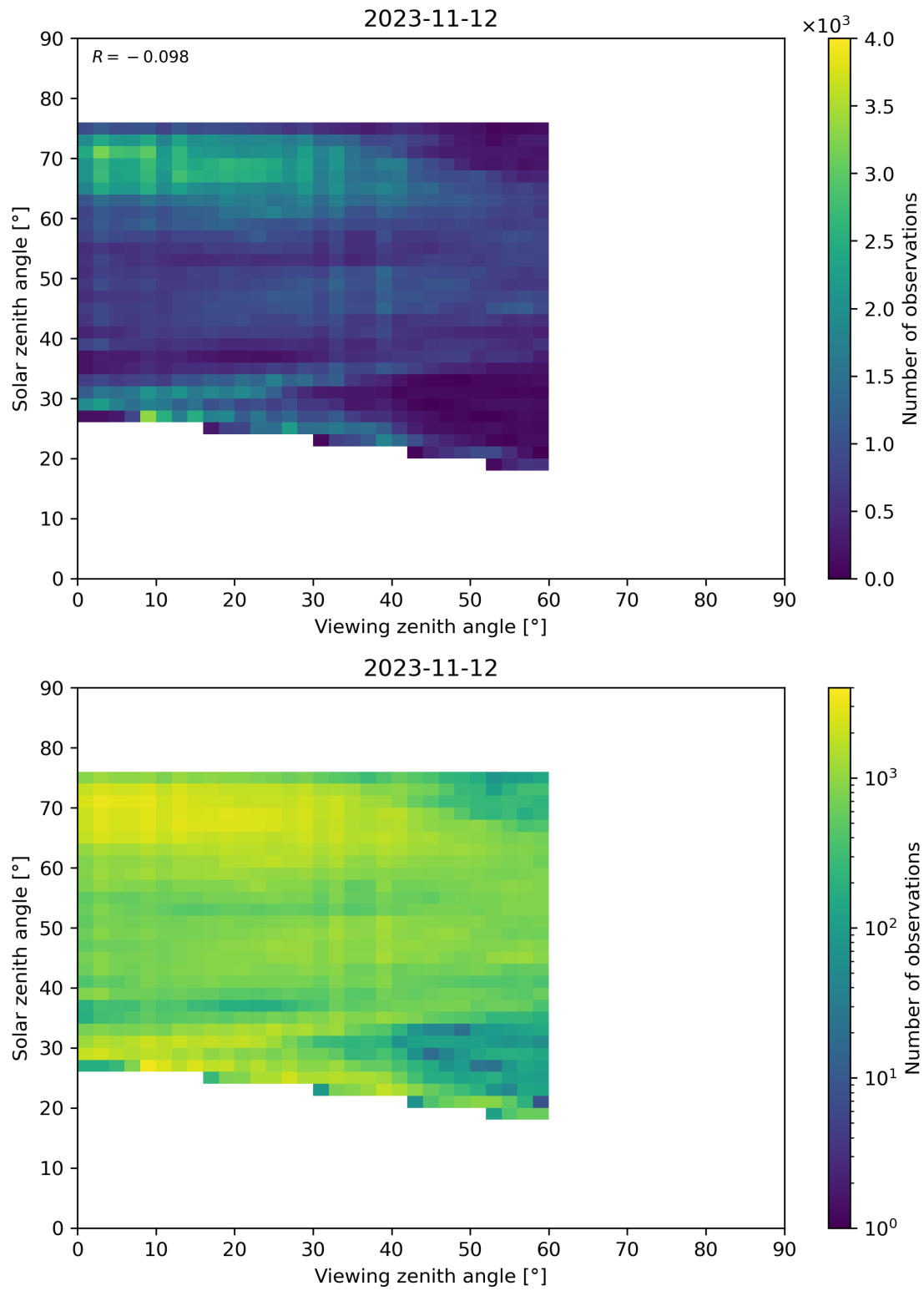
Figure 115: Scatter density plot of “Viewing zenith angle” against “Solar zenith angle” for 2023-11-12 to 2023-11-13.
