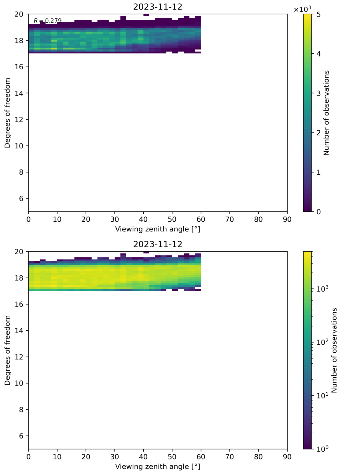
Figure 107: Scatter density plot of “Viewing zenith angle” against “Degrees of freedom” for 2023-11-12 to 2023-11-13.
