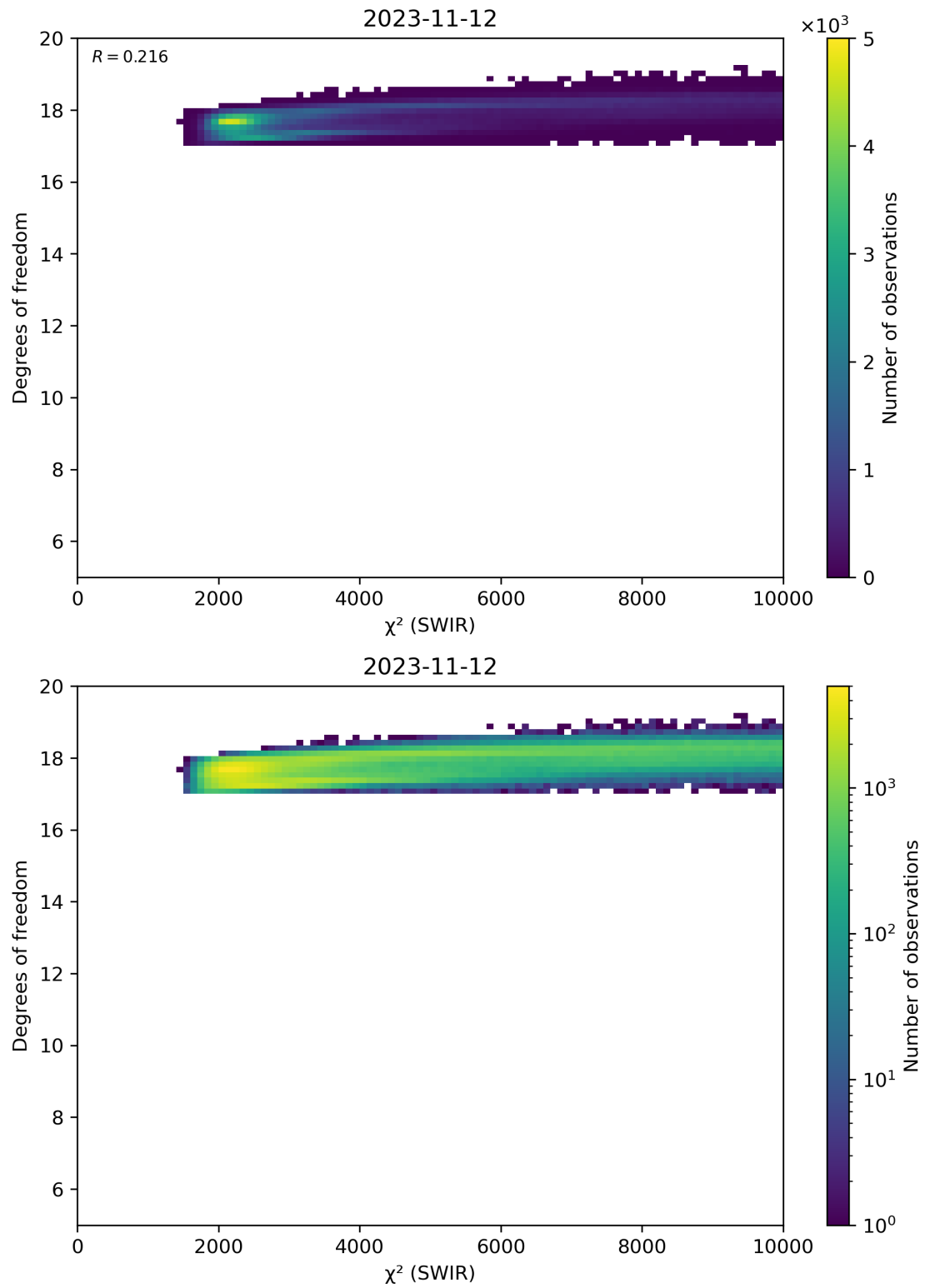
Figure 48: Scatter density plot of “ \chi^2 (SWIR)” against “Degrees of freedom” for 2023-11-12 to 2023-11-13.
