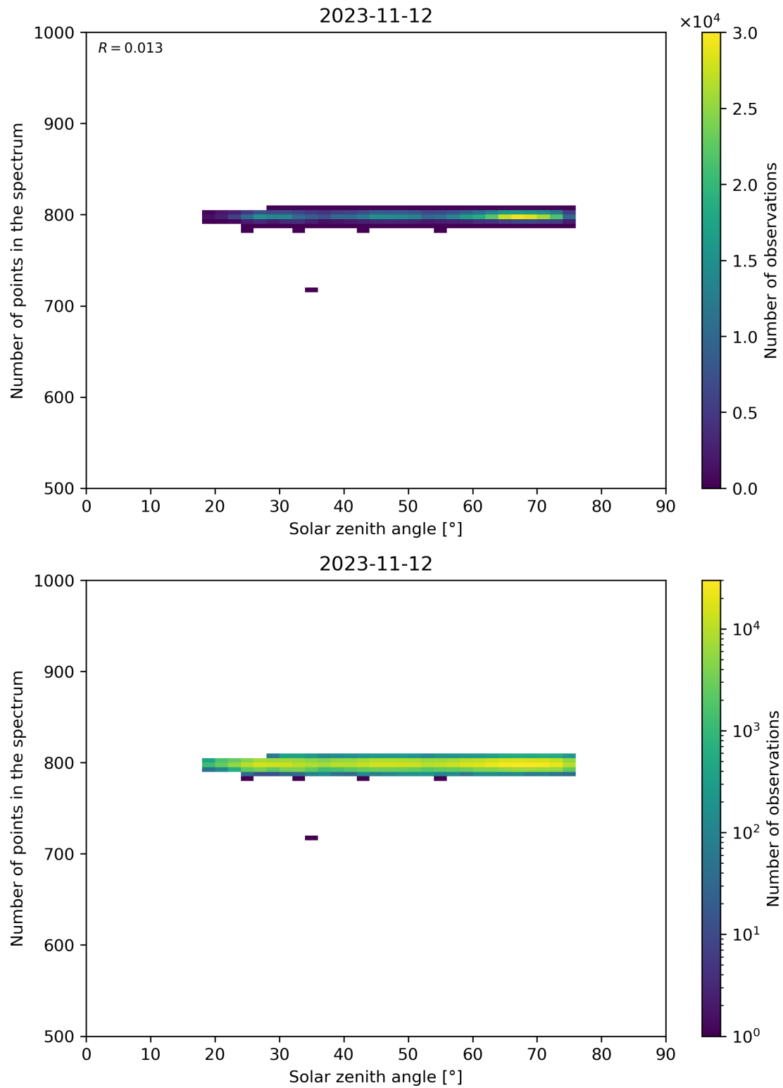
Figure 103: Scatter density plot of “Solar zenith angle” against “Number of points in the spectrum” for 2023-11-12 to 2023-11-13.
