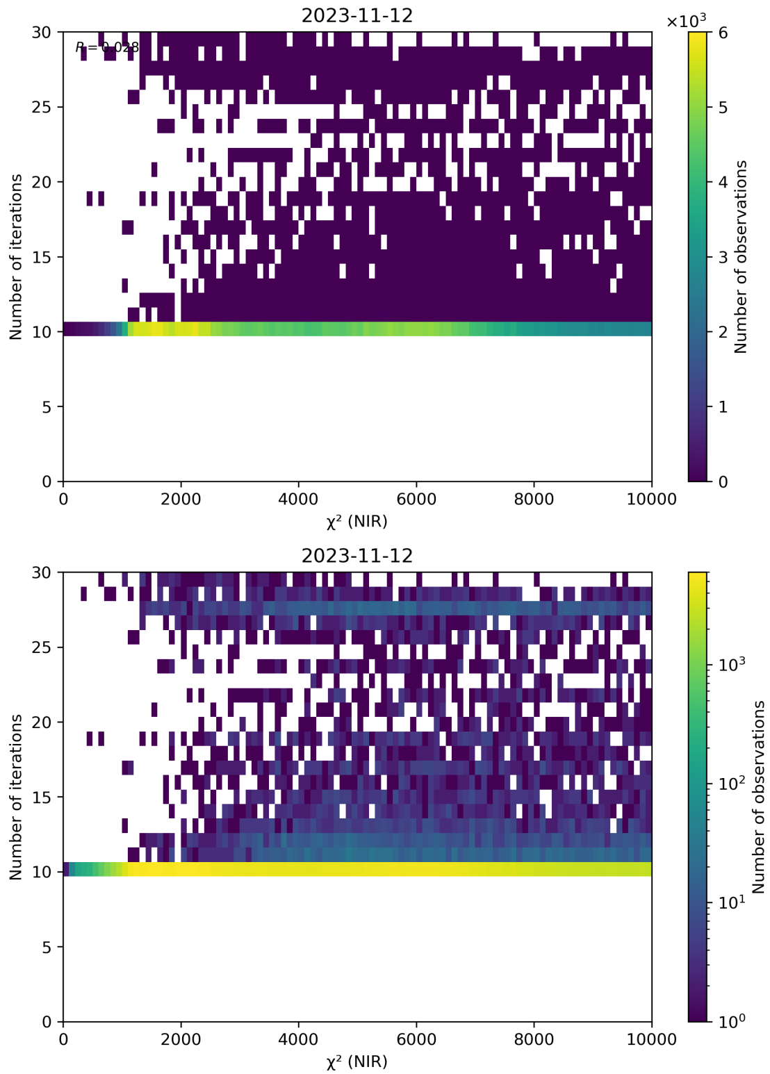
Figure 46: Scatter density plot of “ \chi^2 (NIR)” against “Number of iterations” for 2023-11-12 to 2023-11-13.
