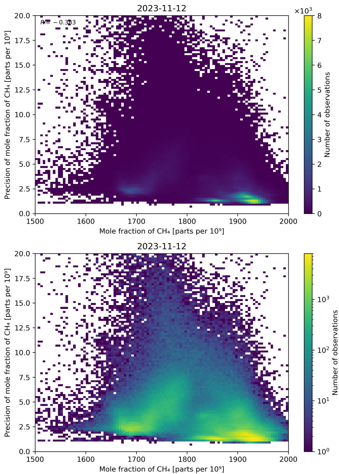
Figure 75: Scatter density plot of “Mole fraction of CH 4 ” against “Precision of mole fraction of CH 4 ” for 2023-11-12 to 2023-11-13.
