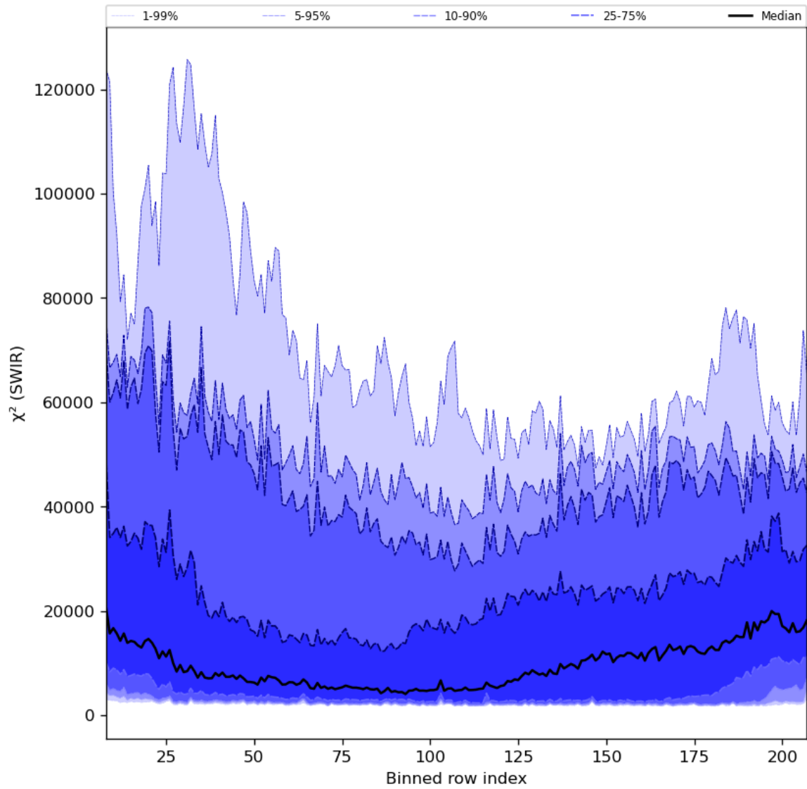
Figure 39: Along track statistics of “ \chi^2 (SWIR)” for 2023-11-12 to 2023-11-13
