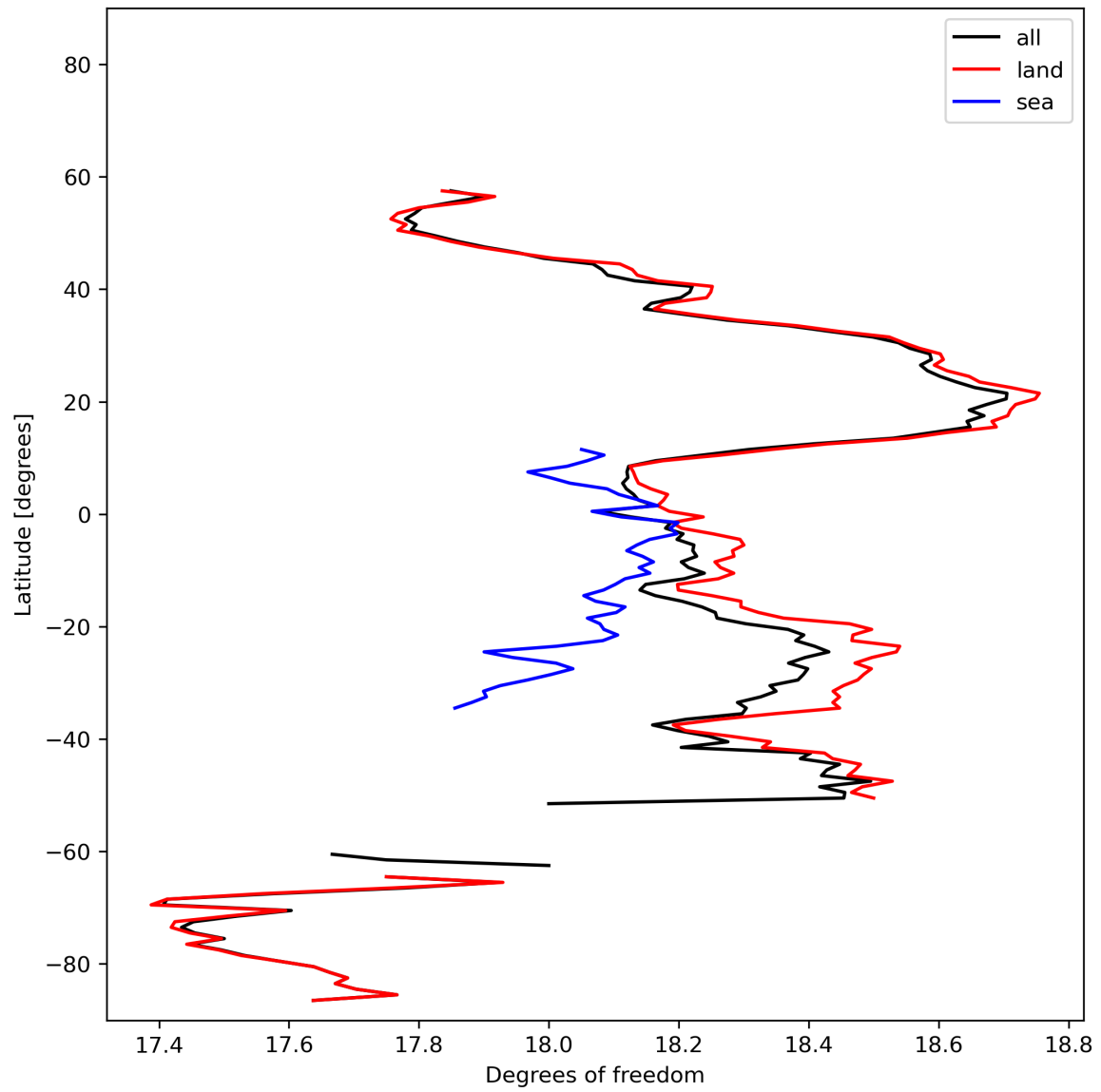
Figure 19: Zonal average of “Degrees of freedom” for 2023-11-12 to 2023-11-13.
