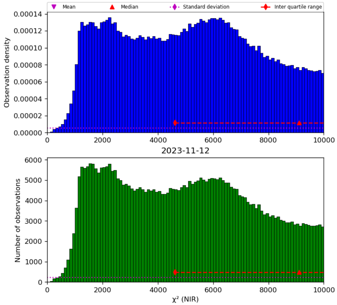
Figure 29: Histogram of “ \chi^2 (NIR)” for 2023-11-12 to 2023-11-13
