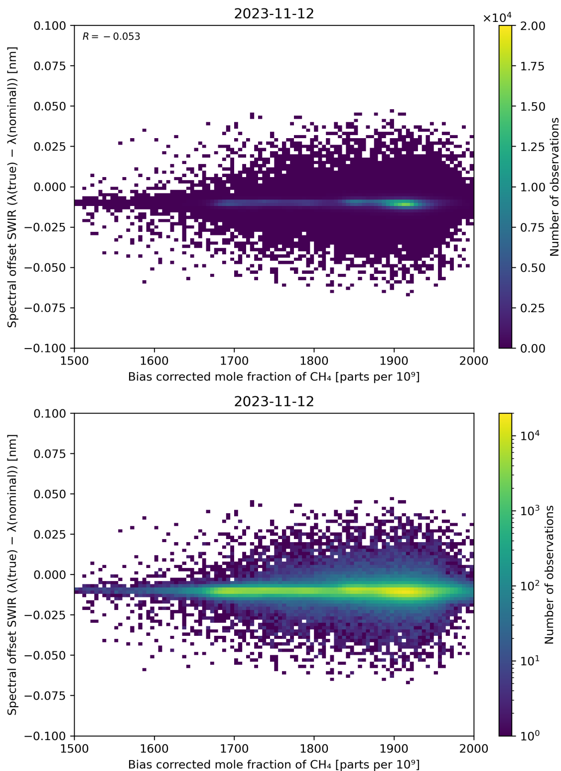
Figure 69: Scatter density plot of “Bias corrected mole fraction of \text{CH}_4 ” against “Spectral offset SWIR ( \lambda(\text{true}) - \lambda(\text{nominal}) )” for 2023-11-12 to 2023-11-13.
