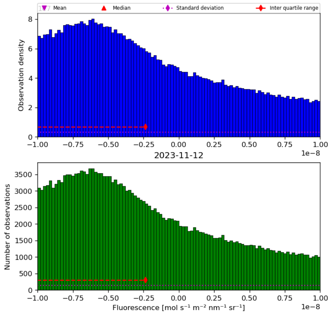
Figure 32: Histogram of “Fluorescence” for 2023-11-12 to 2023-11-13
