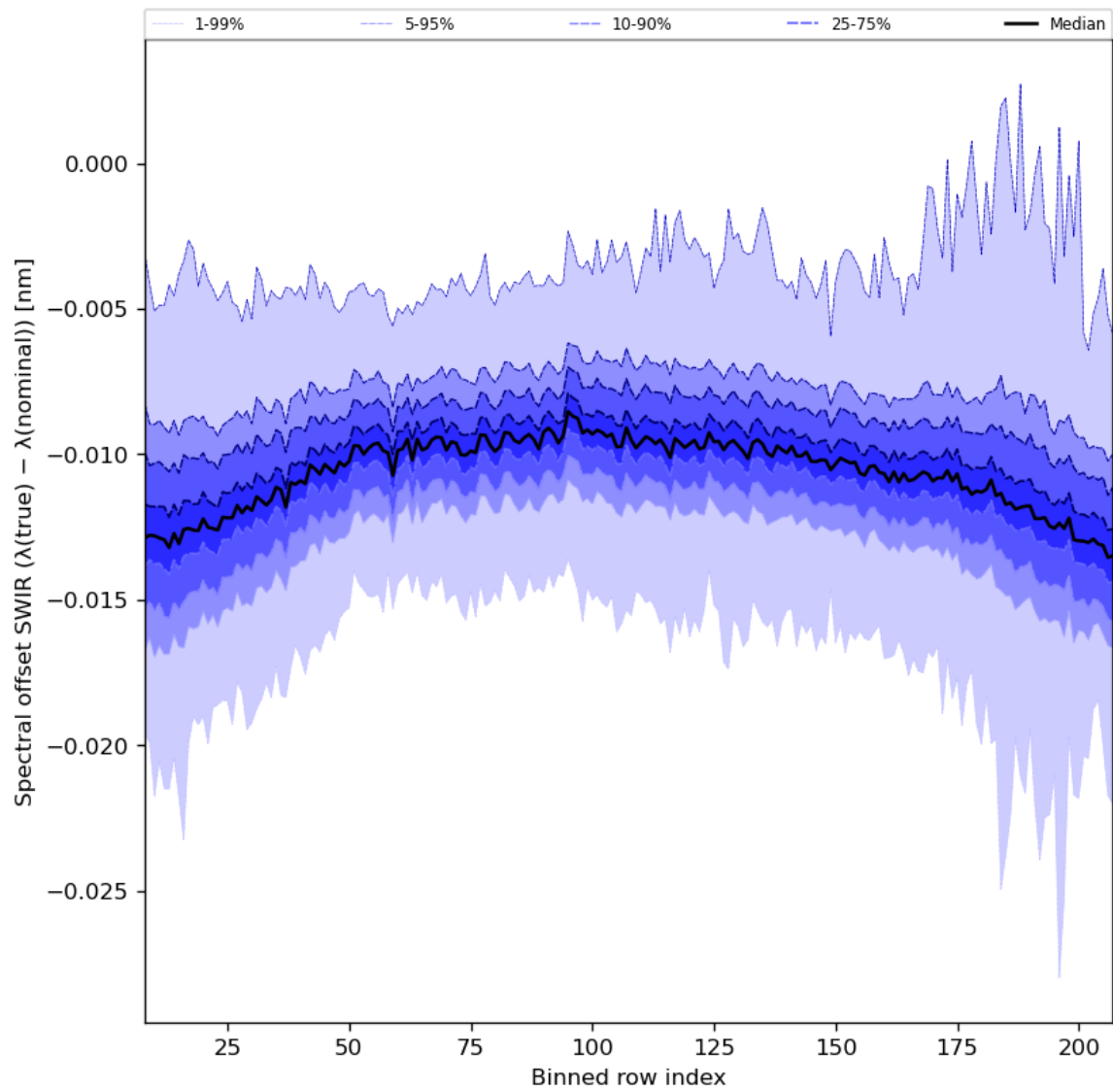
Figure 38: Along track statistics of “Spectral offset SWIR ( \lambda(\text{true}) - \lambda(\text{nominal}) )” for 2023-11-12 to 2023-11-13
