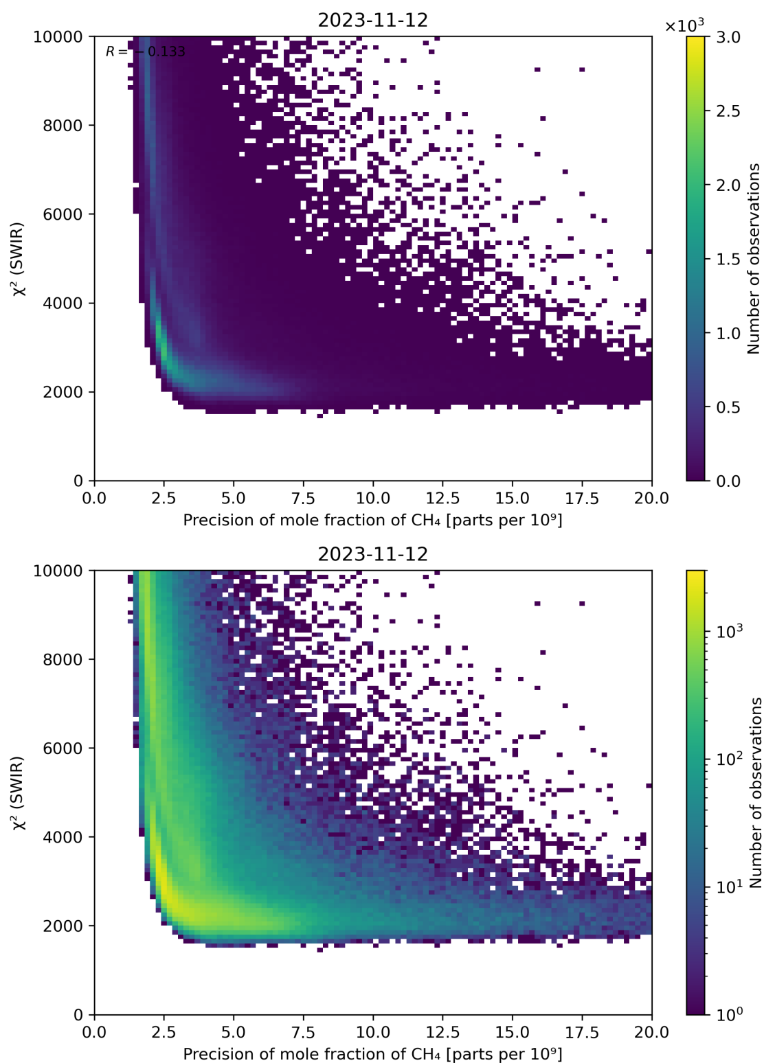
Figure 79: Scatter density plot of “Precision of mole fraction of \text{CH}_4 ” against “ \chi^2 (SWIR)” for 2023-11-12 to 2023-11-13.
