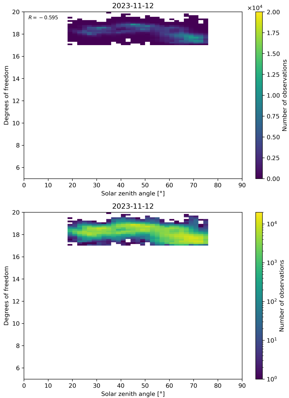
Figure 96: Scatter density plot of “Solar zenith angle” against “Degrees of freedom” for 2023-11-12 to 2023-11-13.
