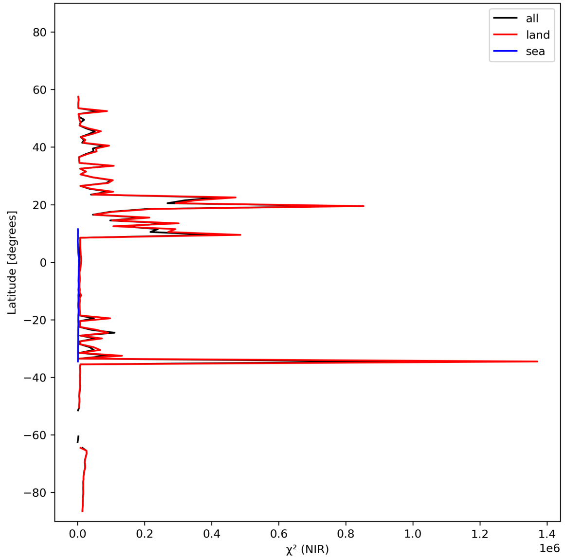
Figure 18: Zonal average of “ \chi^2 (NIR)” for 2023-11-12 to 2023-11-13.
