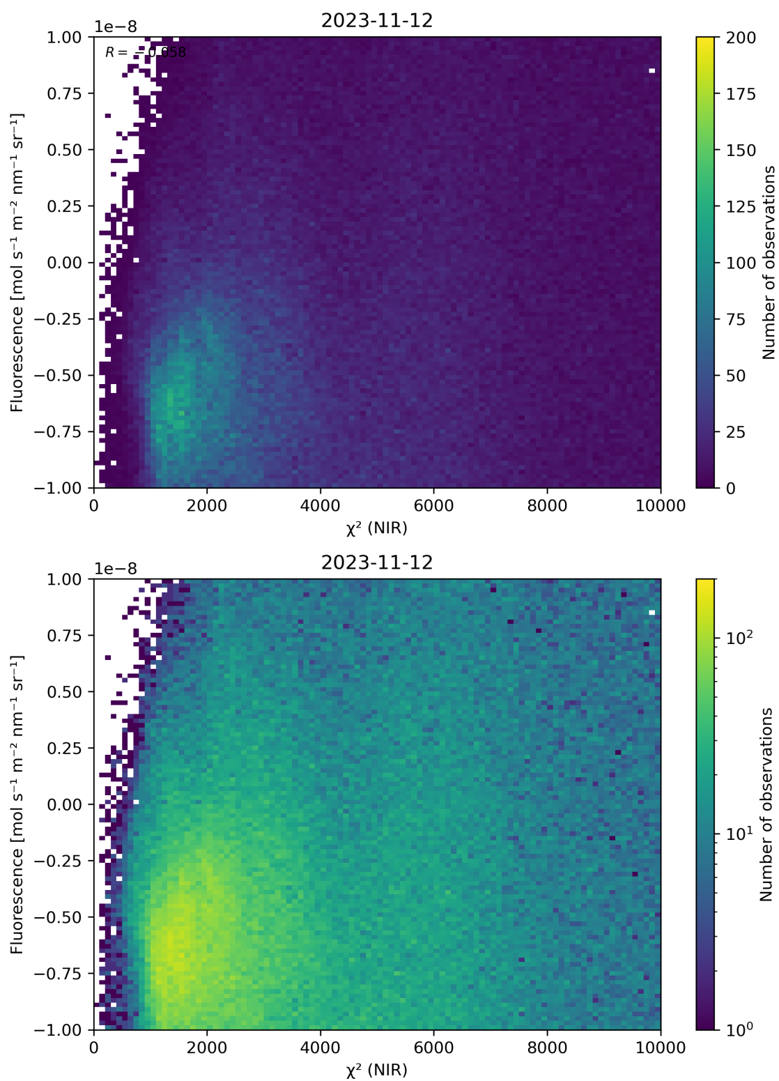
Figure 45: Scatter density plot of “ \chi^2 (NIR)” against “Fluorescence” for 2023-11-12 to 2023-11-13.
