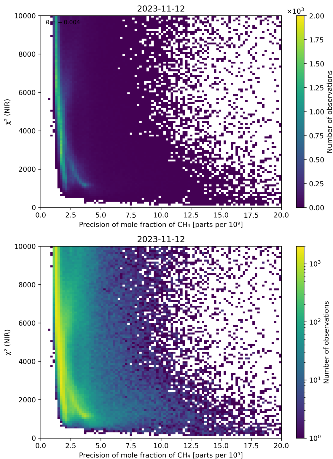
Figure 78: Scatter density plot of “Precision of mole fraction of \text{CH}_4 ” against “ \chi^2 (NIR)” for 2023-11-12 to 2023-11-13.
