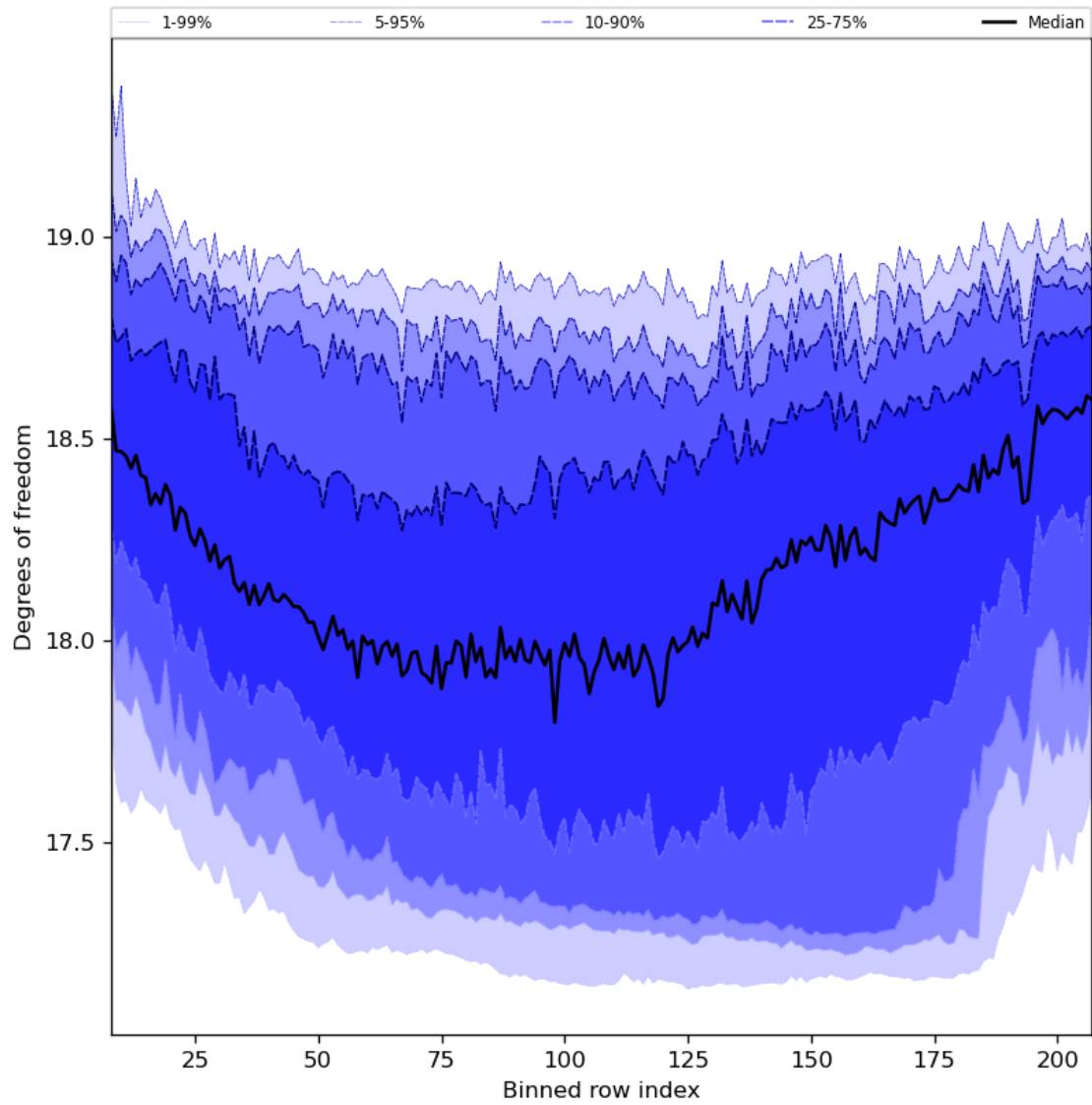
Figure 41: Along track statistics of “Degrees of freedom” for 2023-11-12 to 2023-11-13
