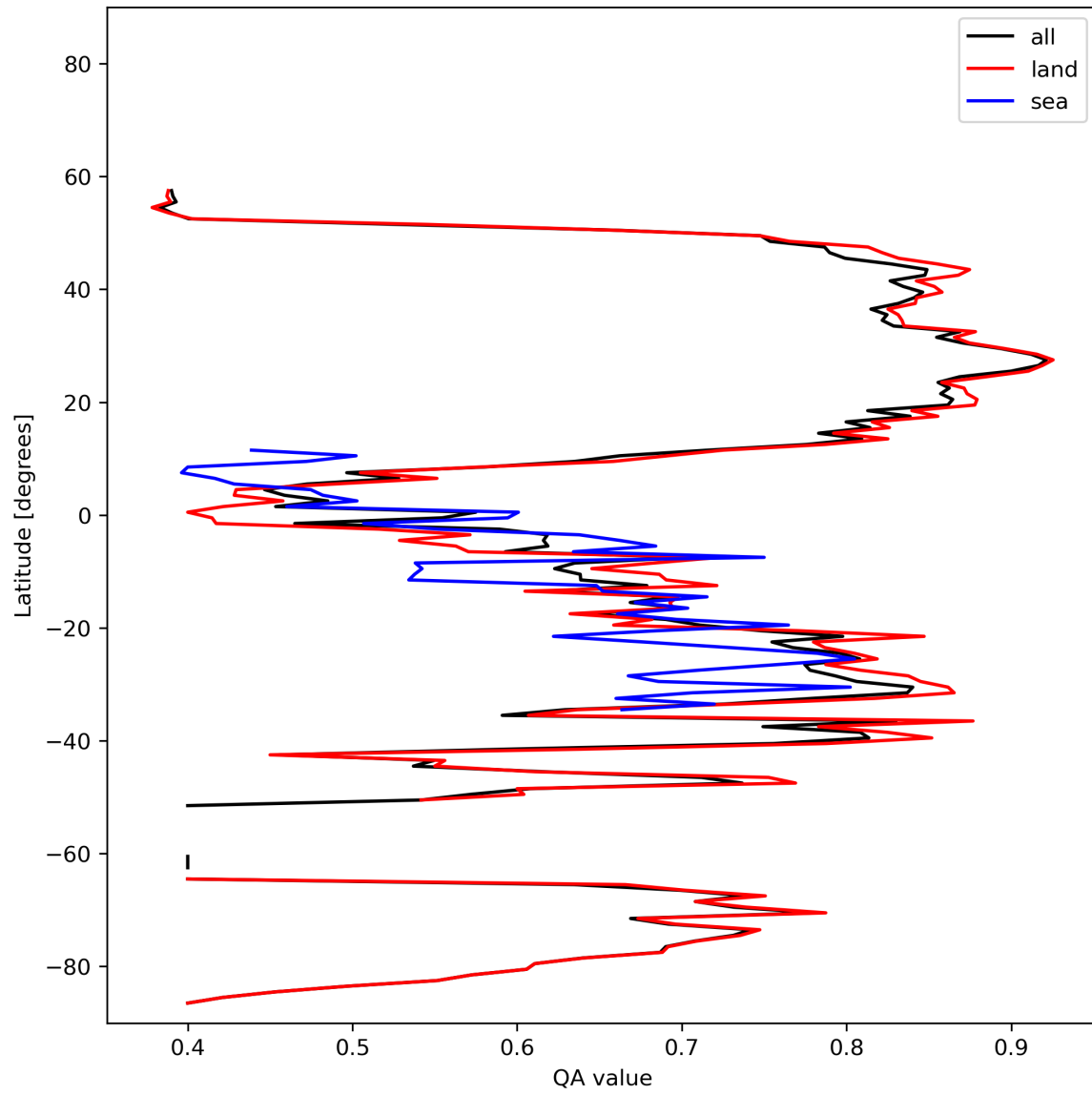
Figure 11: Zonal average of “QA value” for 2023-11-12 to 2023-11-13.
