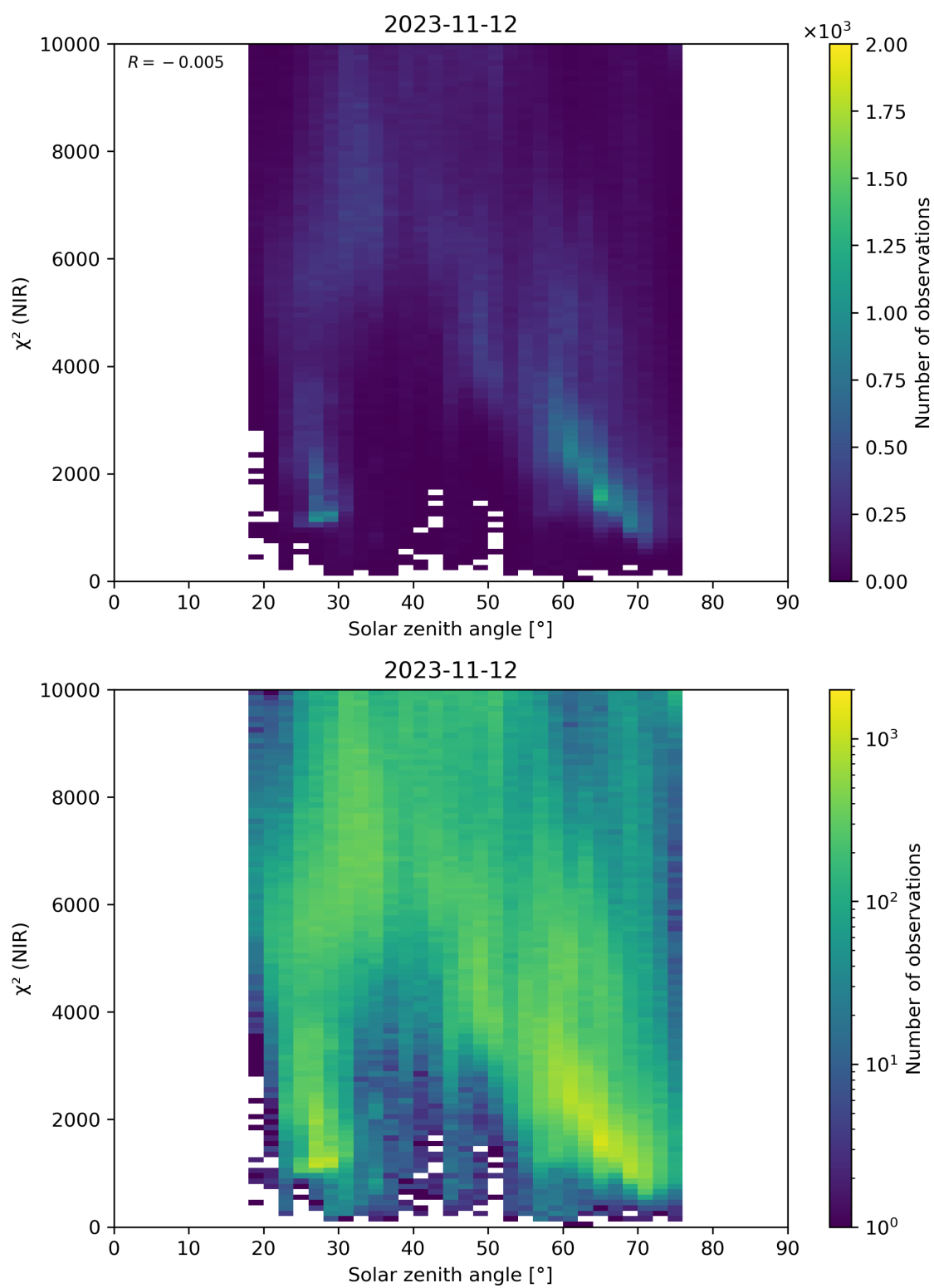
Figure 94: Scatter density plot of “Solar zenith angle” against “ \chi^2 (NIR)” for 2023-11-12 to 2023-11-13.
