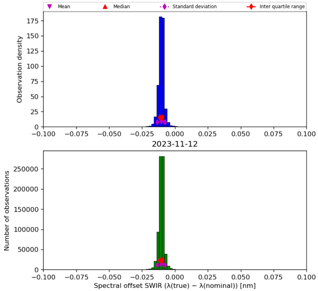
Figure 27: Histogram of “Spectral offset SWIR ( \lambda(\text{true}) - \lambda(\text{nominal}) )” for 2023-11-12 to 2023-11-13
