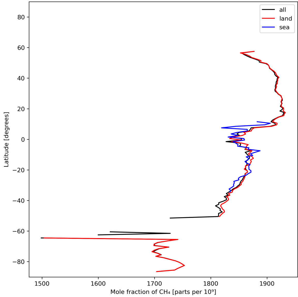
Figure 12: Zonal average of “Mole fraction of \text{CH}_4 ” for 2023-11-12 to 2023-11-13.
