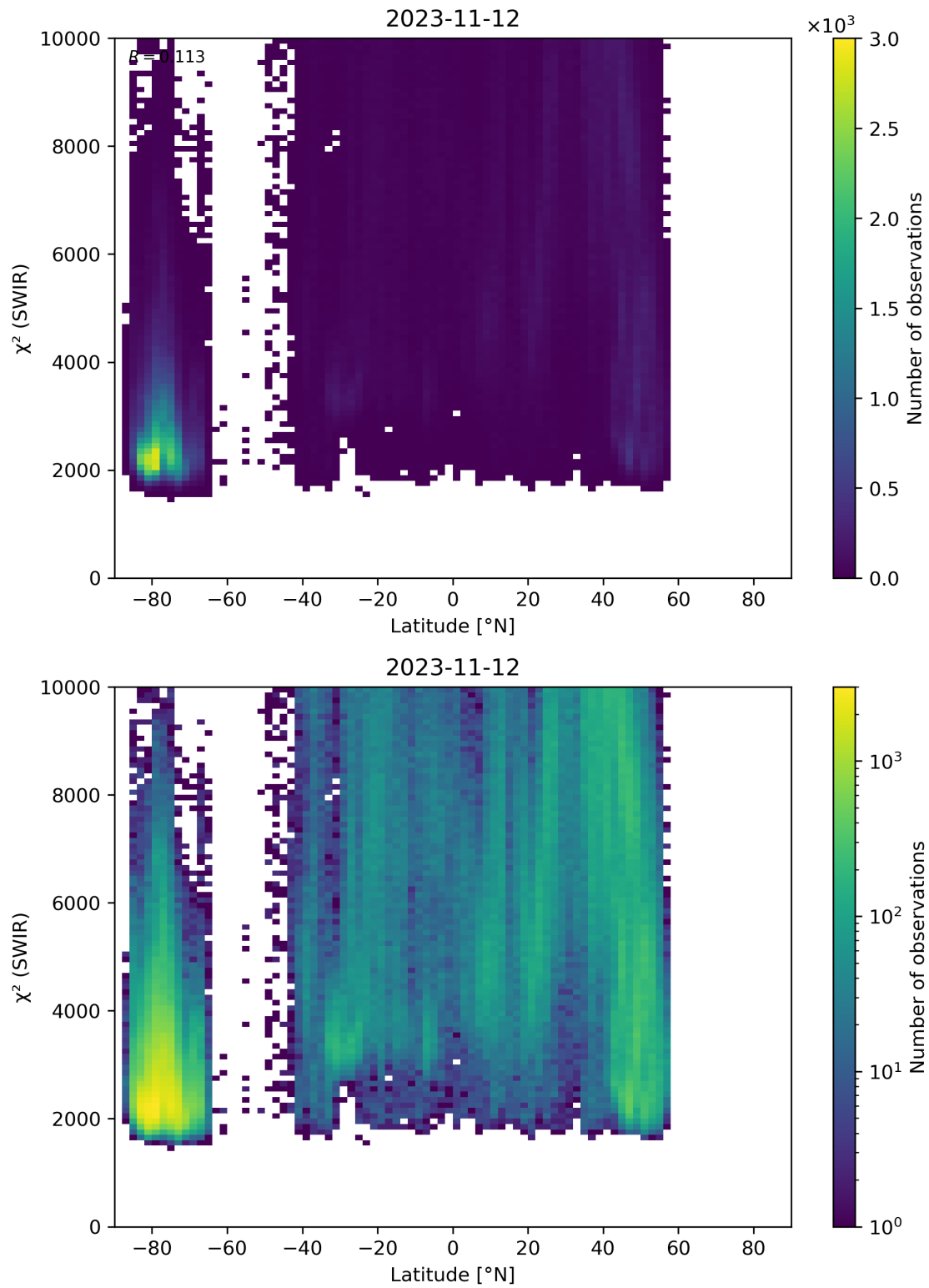
Figure 54: Scatter density plot of “Latitude” against “ \chi^2 (SWIR)” for 2023-11-12 to 2023-11-13.
