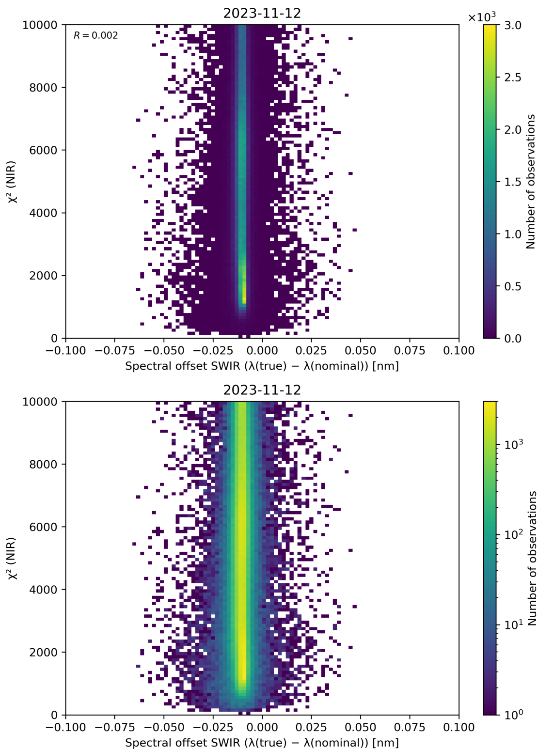
Figure 117: Scatter density plot of “Spectral offset SWIR ( \lambda(\text{true}) - \lambda(\text{nominal}) )” against “ \chi^2 (NIR)” for 2023-11-12 to 2023-11-13.
