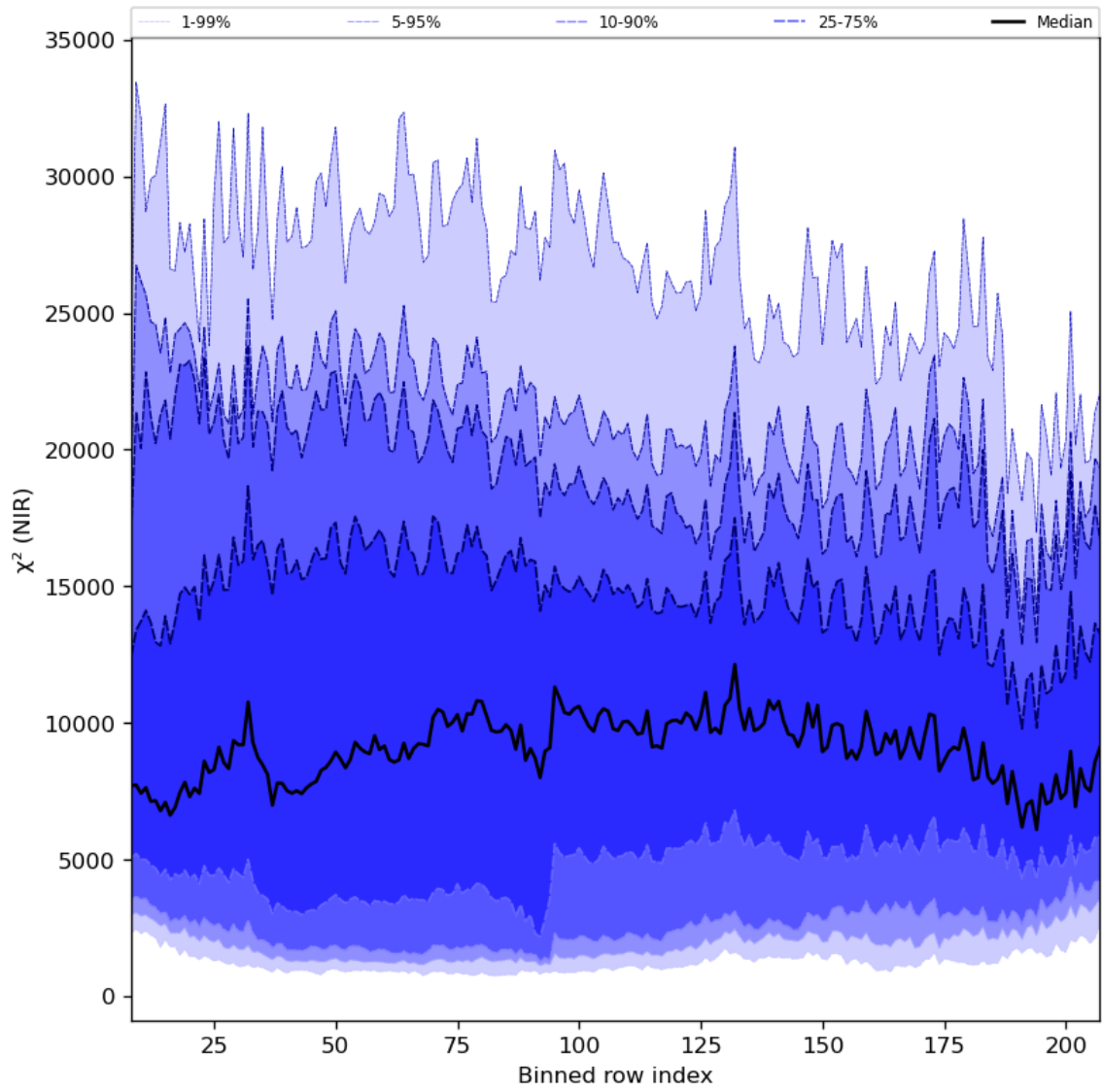
Figure 40: Along track statistics of “ \chi^2 (NIR)” for 2023-11-12 to 2023-11-13
