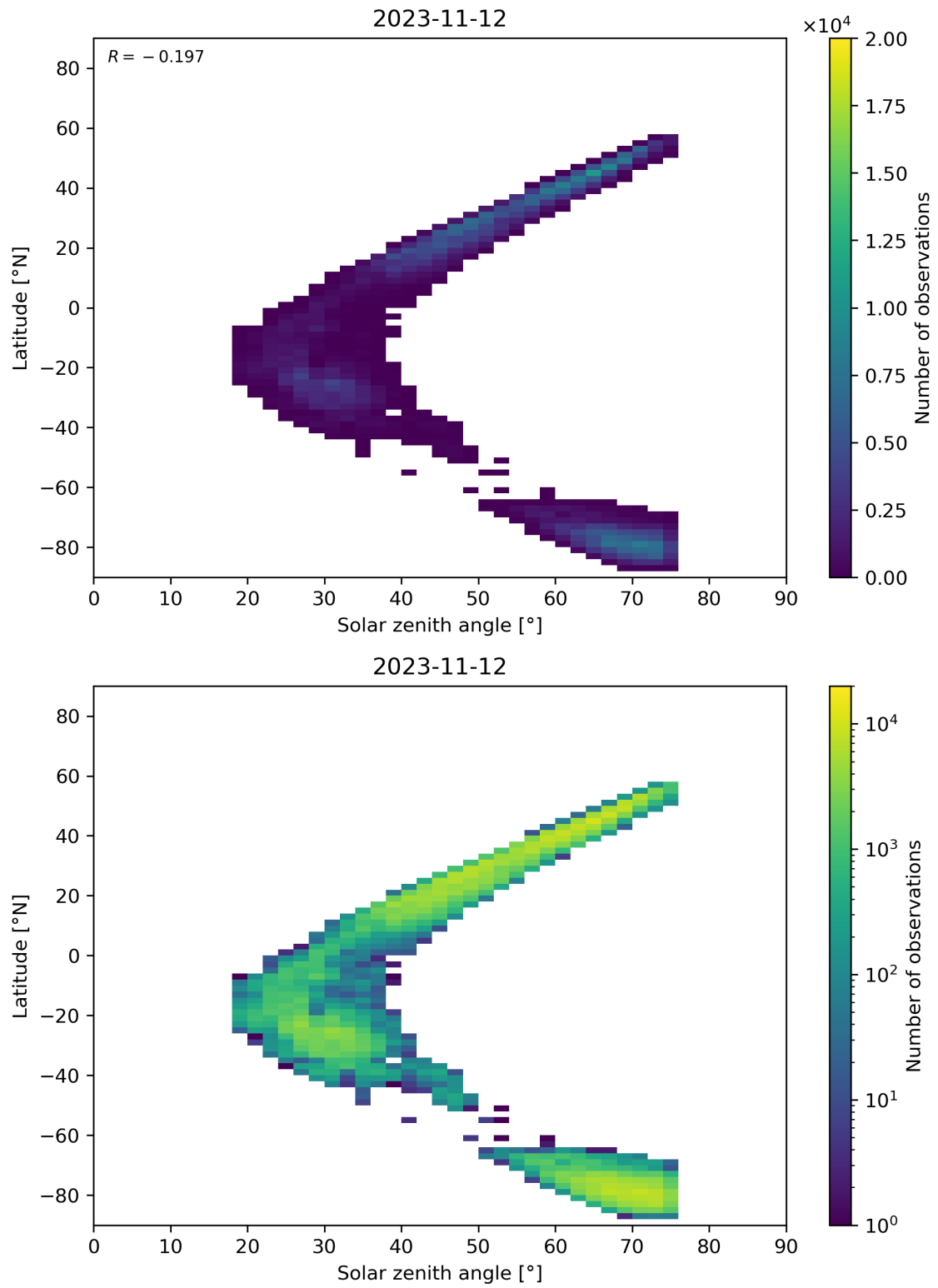
Figure 98: Scatter density plot of “Solar zenith angle” against “Latitude” for 2023-11-12 to 2023-11-13.
