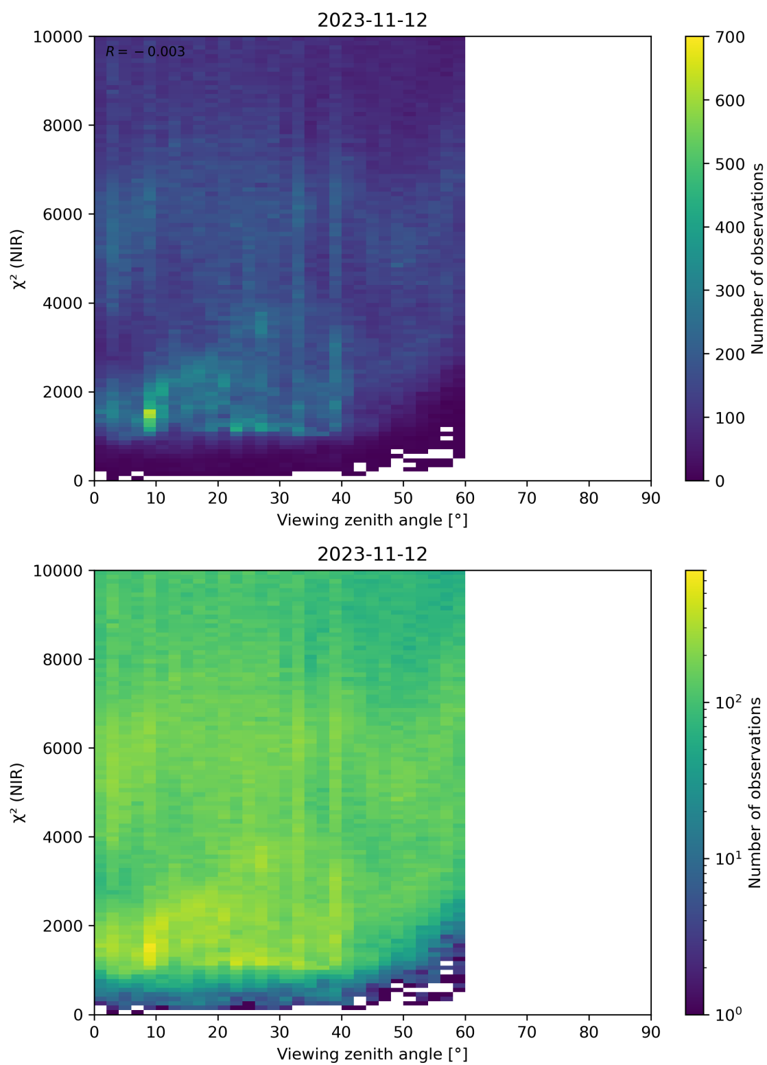
Figure 105: Scatter density plot of “Viewing zenith angle” against “ \chi^2 (NIR)” for 2023-11-12 to 2023-11-13.
