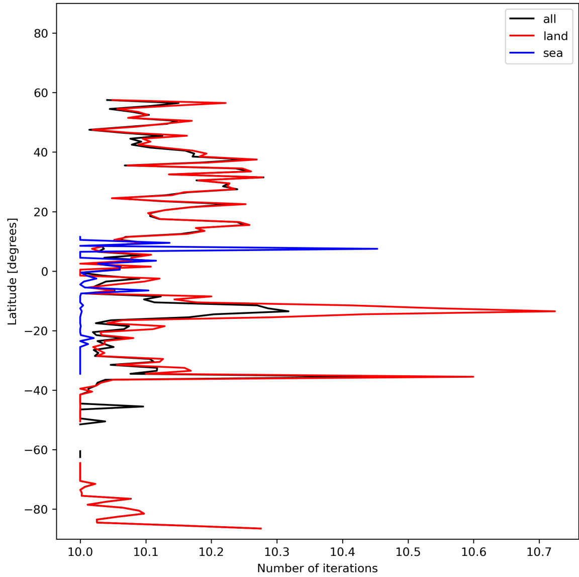
Figure 20: Zonal average of “Number of iterations” for 2023-11-12 to 2023-11-13.
