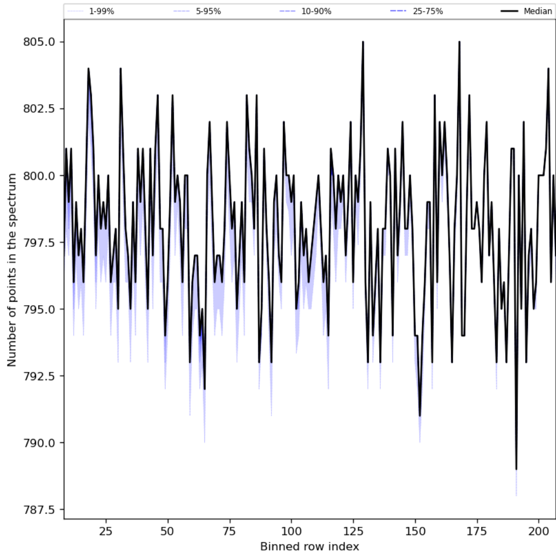
Figure 37: Along track statistics of “Number of points in the spectrum” for 2023-11-12 to 2023-11-13
