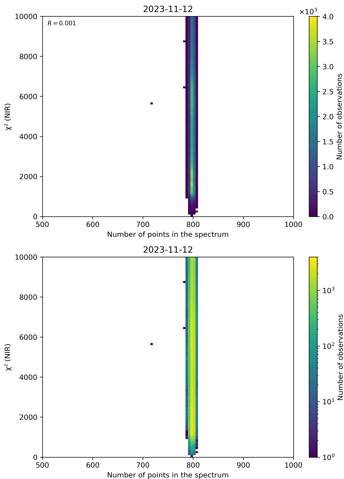
Figure 88: Scatter density plot of “Number of points in the spectrum” against “ \chi^2 (NIR)” for 2023-11-12 to 2023-11-13.
