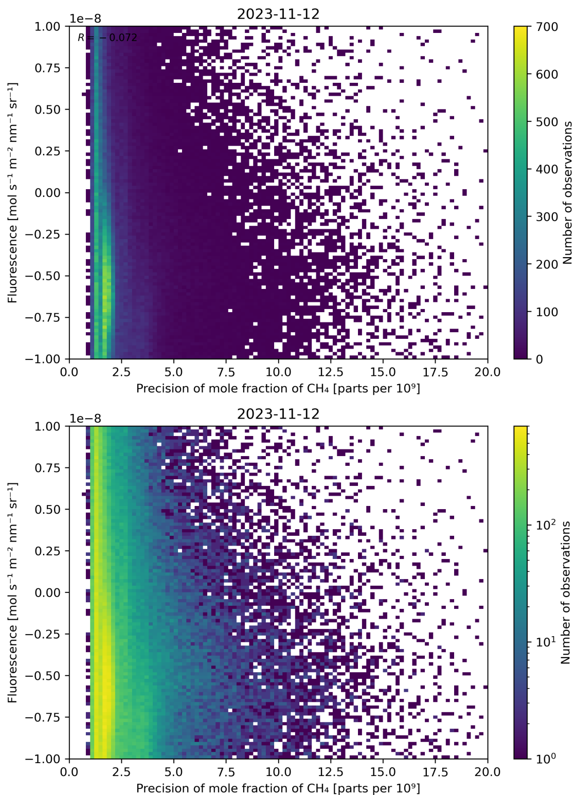
Figure 81: Scatter density plot of “Precision of mole fraction of \text{CH}_4 ” against “Fluorescence” for 2023-11-12 to 2023-11-13.
