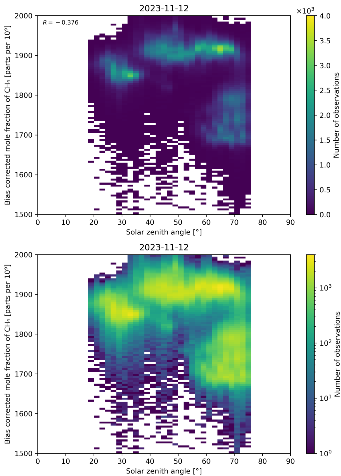
Figure 100: Scatter density plot of “Solar zenith angle” against “Bias corrected mole fraction of CH 4 ” for 2023-11-12 to 2023-11-13.
