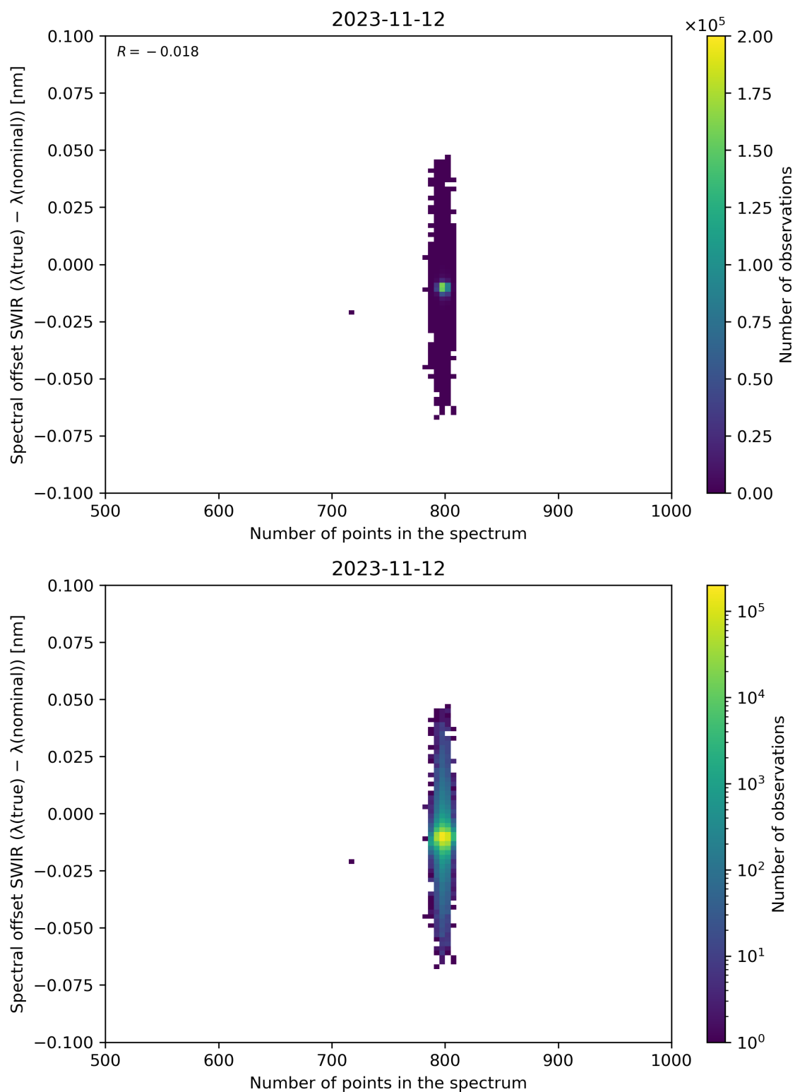
Figure 93: Scatter density plot of “Number of points in the spectrum” against “Spectral offset SWIR ( \lambda(\text{true}) - \lambda(\text{nominal}) )” for 2023-11-12 to 2023-11-13.
