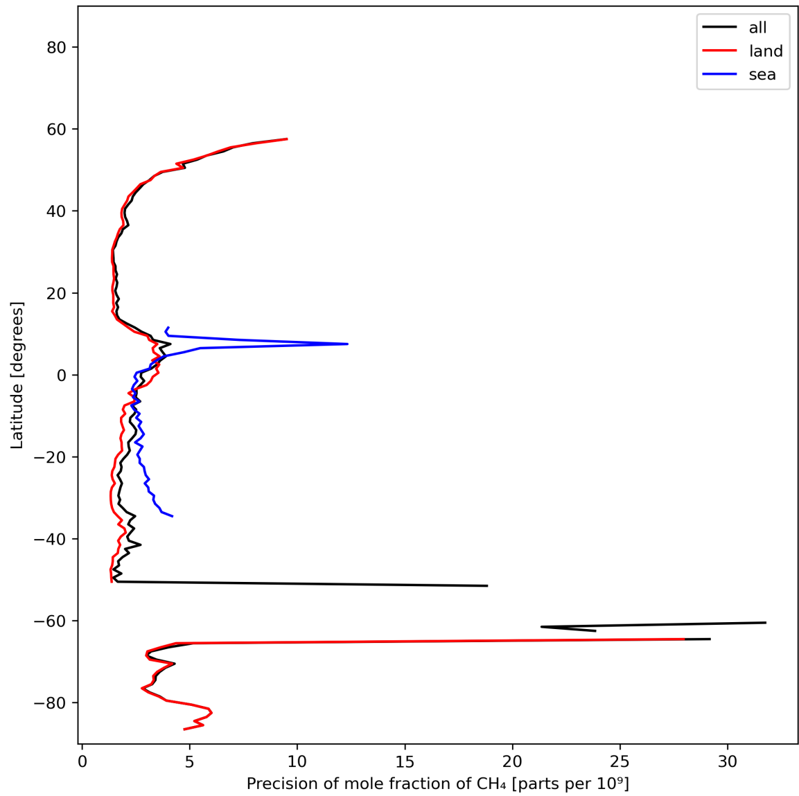
Figure 13: Zonal average of “Precision of mole fraction of CH 4 ” for 2023-11-12 to 2023-11-13.
