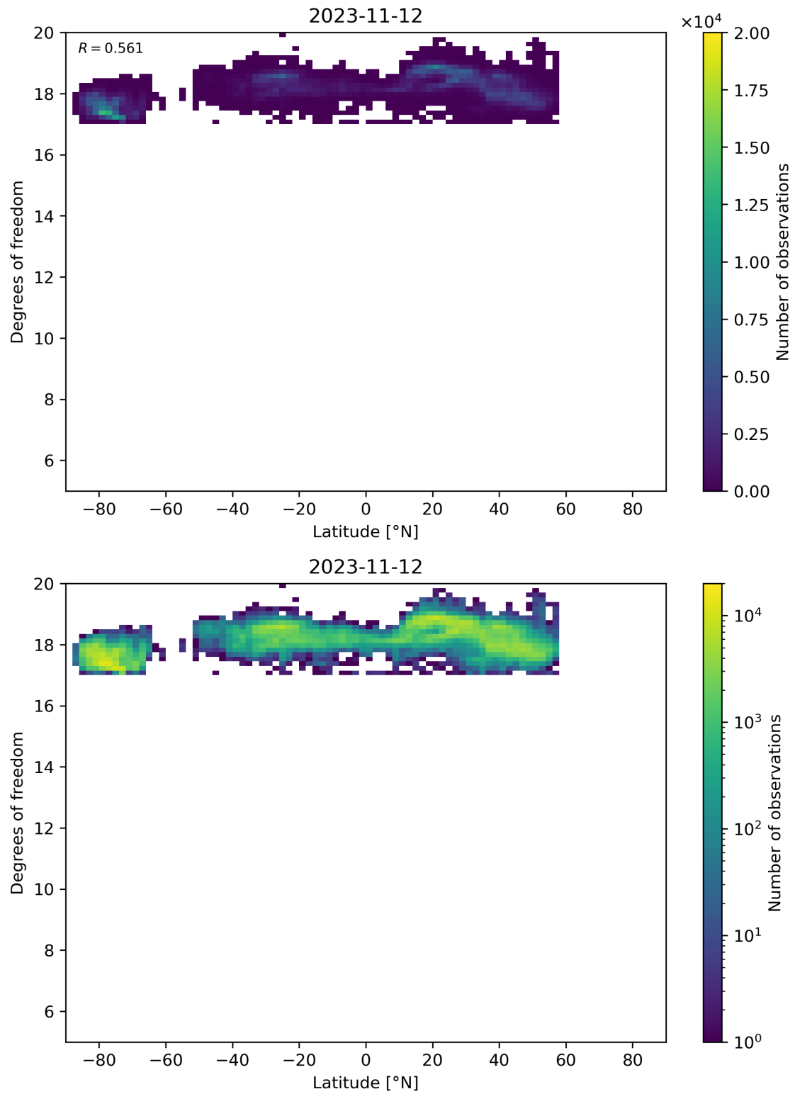
Figure 55: Scatter density plot of “Latitude” against “Degrees of freedom” for 2023-11-12 to 2023-11-13.
