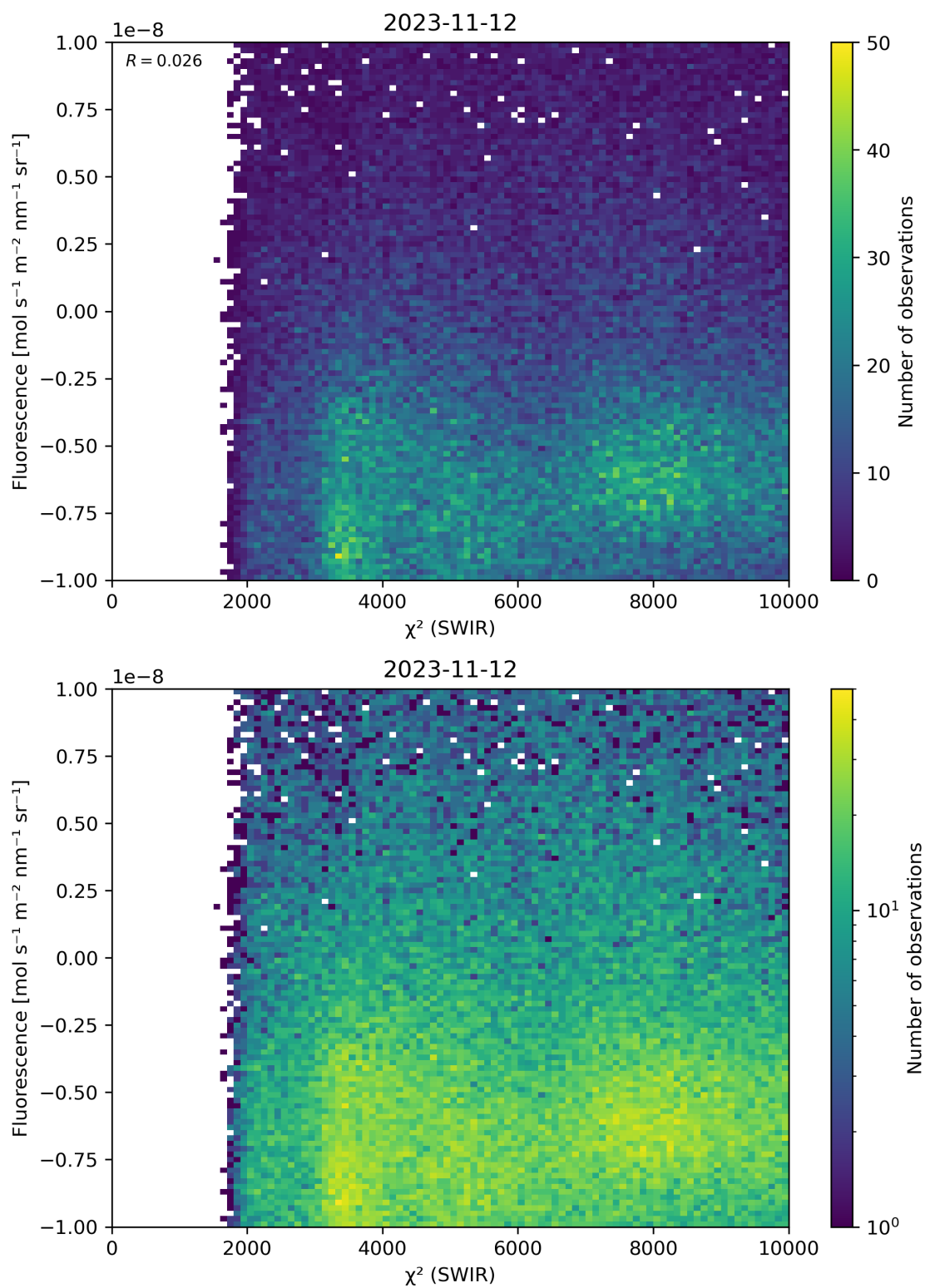
Figure 49: Scatter density plot of “ \chi^2 (SWIR)” against “Fluorescence” for 2023-11-12 to 2023-11-13.
