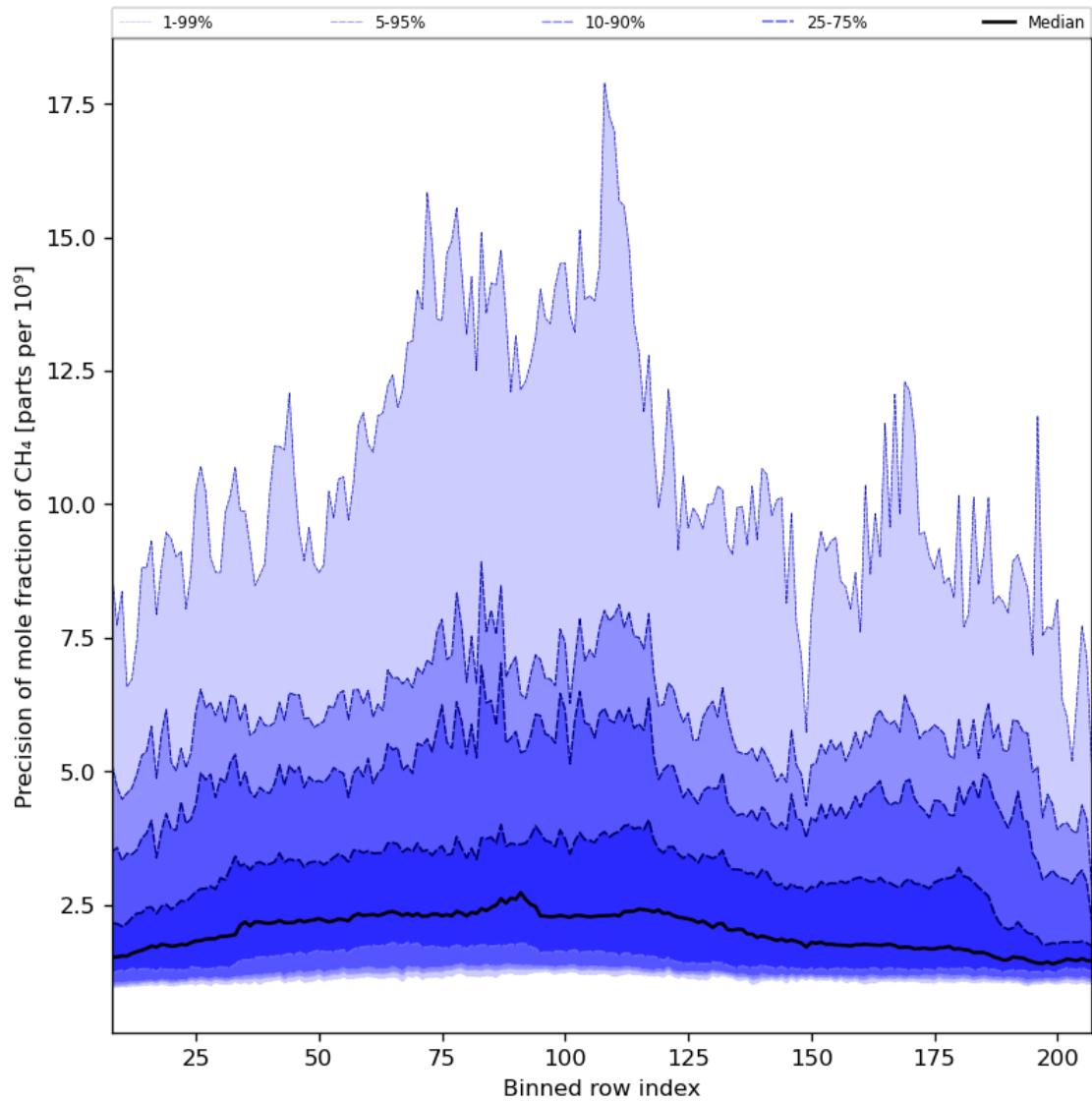
Figure 35: Along track statistics of “Precision of mole fraction of CH 4 ” for 2023-11-12 to 2023-11-13
