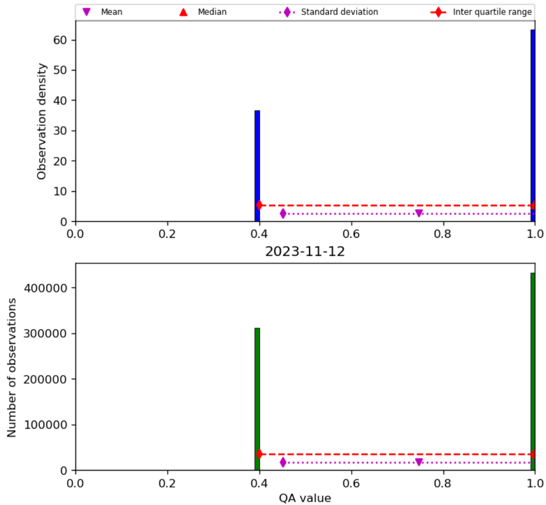
Figure 22: Histogram of “QA value” for 2023-11-12 to 2023-11-13
