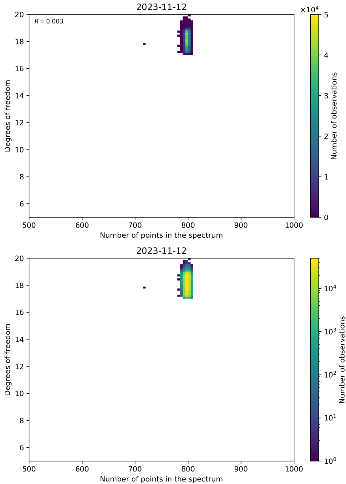
Figure 90: Scatter density plot of “Number of points in the spectrum” against “Degrees of freedom” for 2023-11-12 to 2023-11-13.
