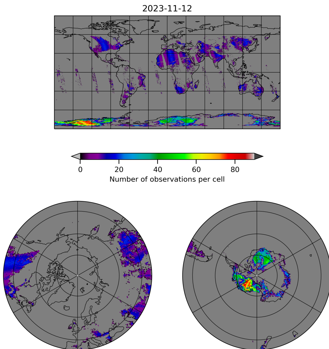
Figure 10: Map of the number of observations for 2023-11-12 to 2023-11-13
