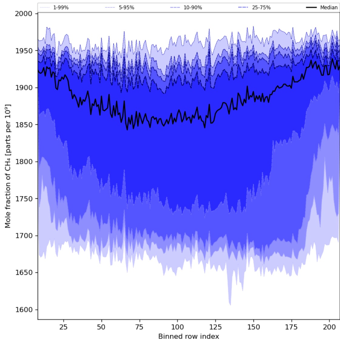
Figure 34: Along track statistics of “Mole fraction of CH 4 ” for 2023-11-12 to 2023-11-13
