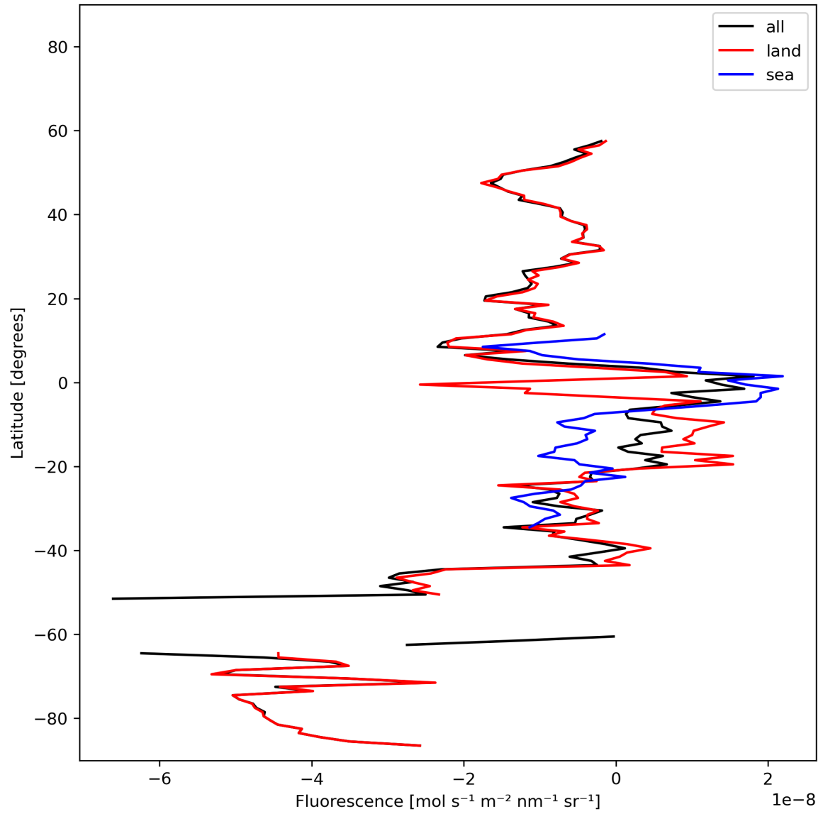
Figure 21: Zonal average of “Fluorescence” for 2023-11-12 to 2023-11-13.
