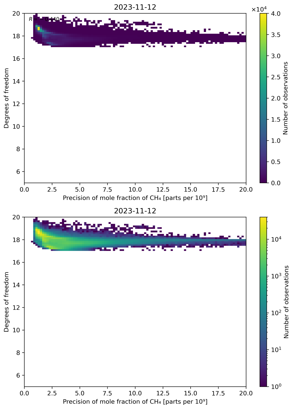
Figure 80: Scatter density plot of “Precision of mole fraction of CH 4 ” against “Degrees of freedom” for 2023-11-12 to 2023-11-13.
