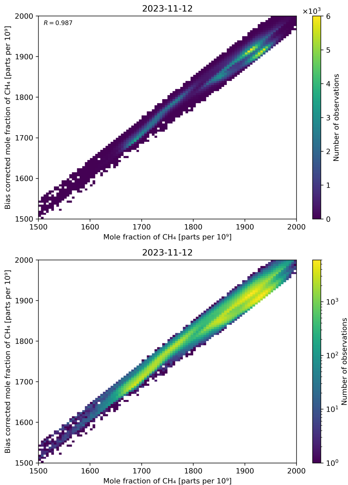
Figure 74: Scatter density plot of “Mole fraction of CH 4 ” against “Bias corrected mole fraction of CH 4 ” for 2023-11-12 to 2023-11-13.
