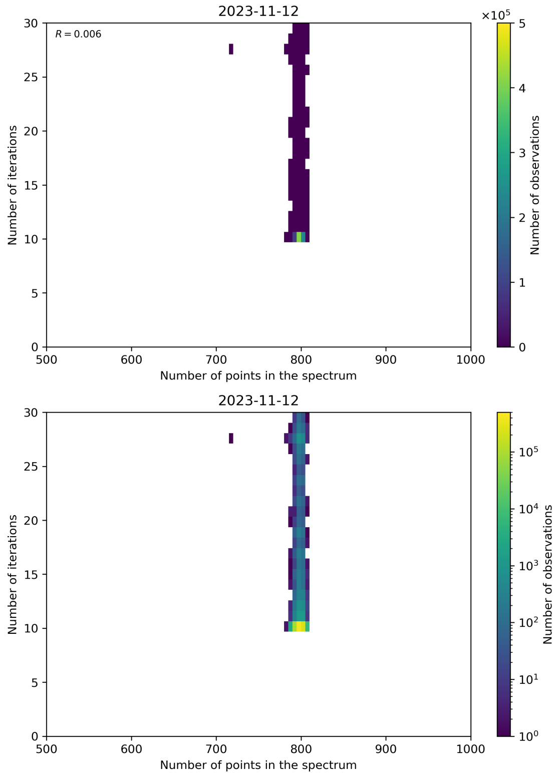
Figure 92: Scatter density plot of “Number of points in the spectrum” against “Number of iterations” for 2023-11-12 to 2023-11-13.
