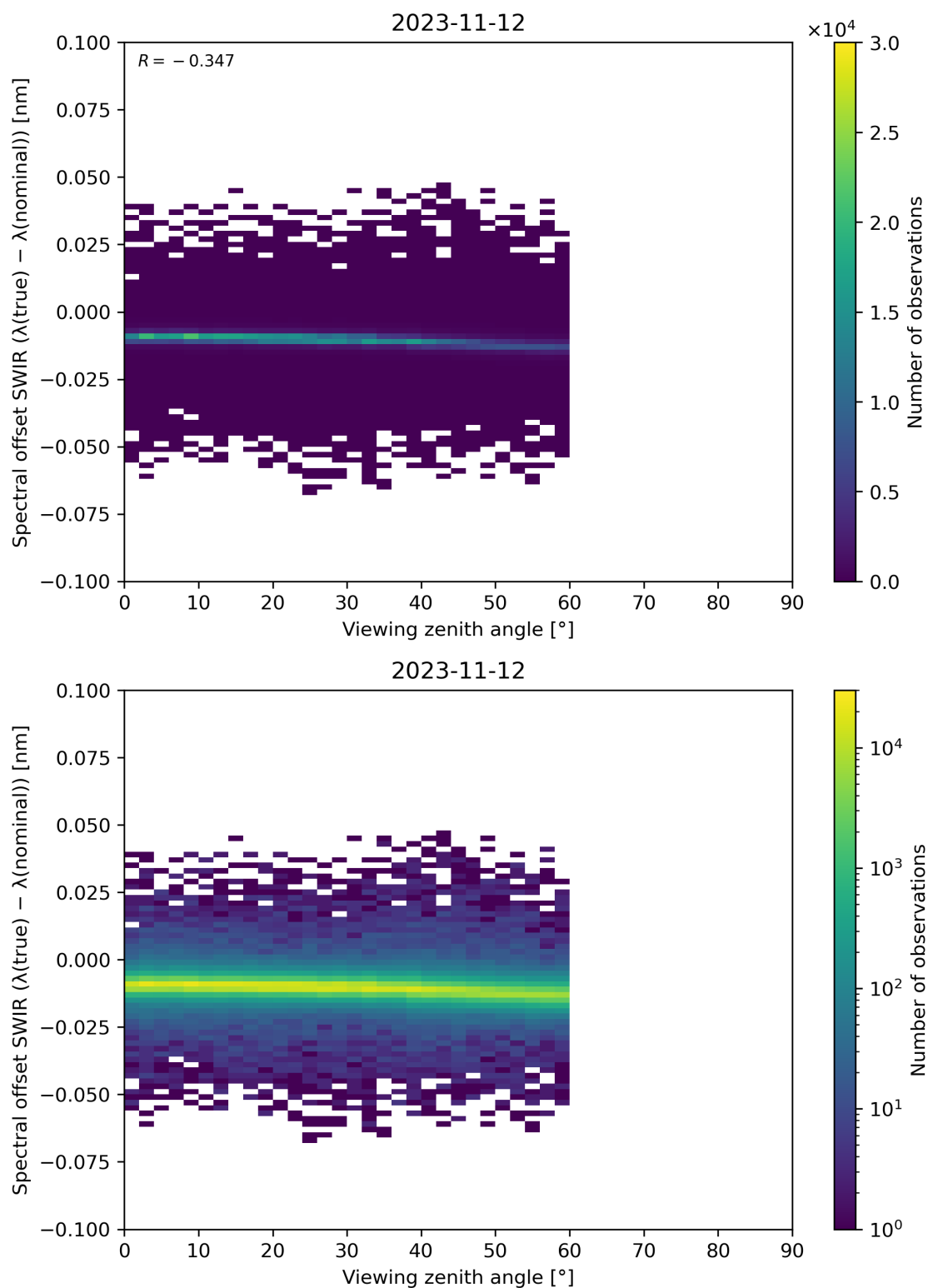
Figure 116: Scatter density plot of “Viewing zenith angle” against “Spectral offset SWIR ( \lambda(\text{true}) - \lambda(\text{nominal}) )” for 2023-11-12 to 2023-11-13.
