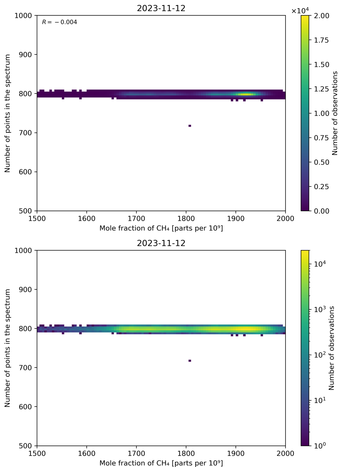
Figure 77: Scatter density plot of “Mole fraction of CH 4 ” against “Number of points in the spectrum” for 2023-11-12 to 2023-11-13.
