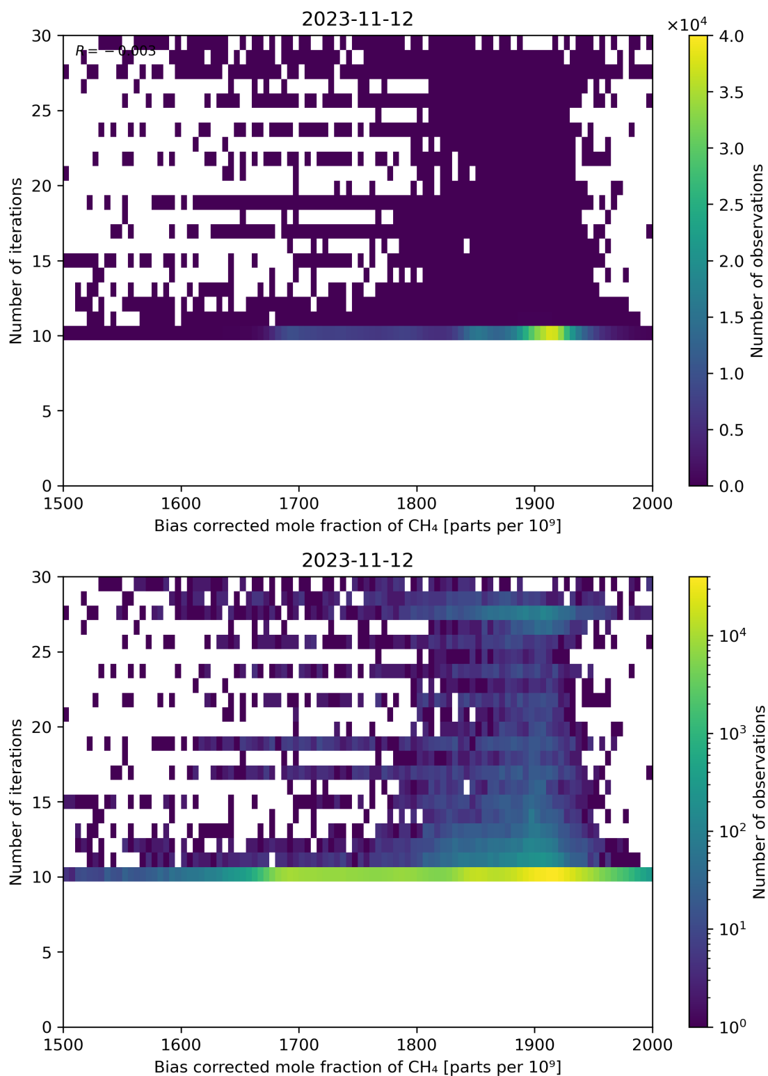
Figure 67: Scatter density plot of “Bias corrected mole fraction of CH 4 ” against “Number of iterations” for 2023-11-12 to 2023-11-13.
