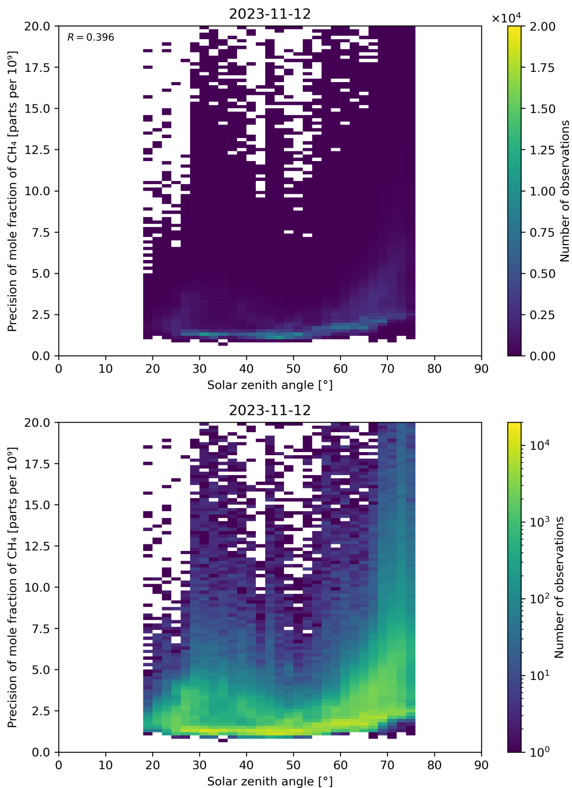
Figure 101: Scatter density plot of “Solar zenith angle” against “Precision of mole fraction of CH 4 ” for 2023-11-12 to 2023-11-13.
