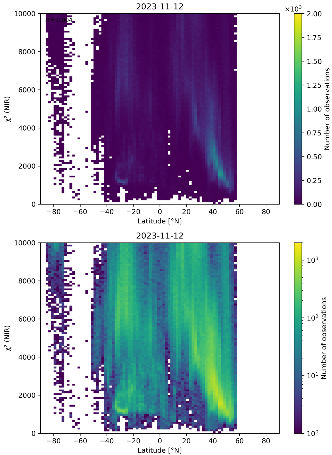
Figure 53: Scatter density plot of “Latitude” against “ \chi^2 (NIR)” for 2023-11-12 to 2023-11-13.
