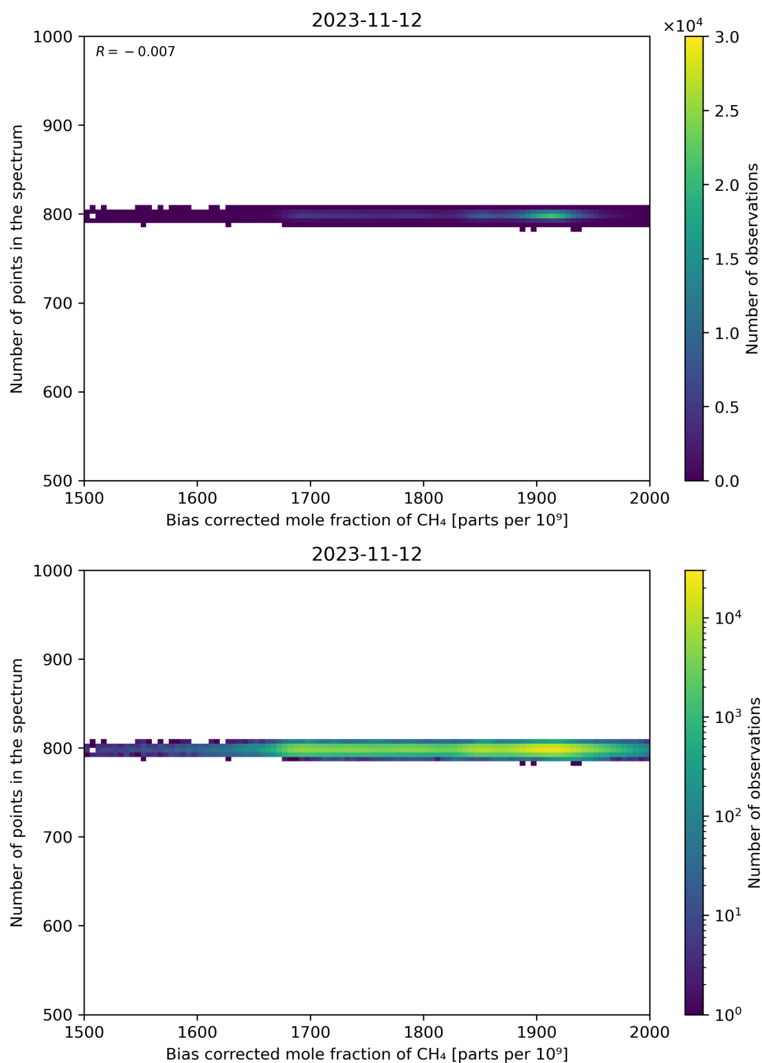
Figure 68: Scatter density plot of “Bias corrected mole fraction of CH 4 ” against “Number of points in the spectrum” for 2023-11-12 to 2023-11-13.
