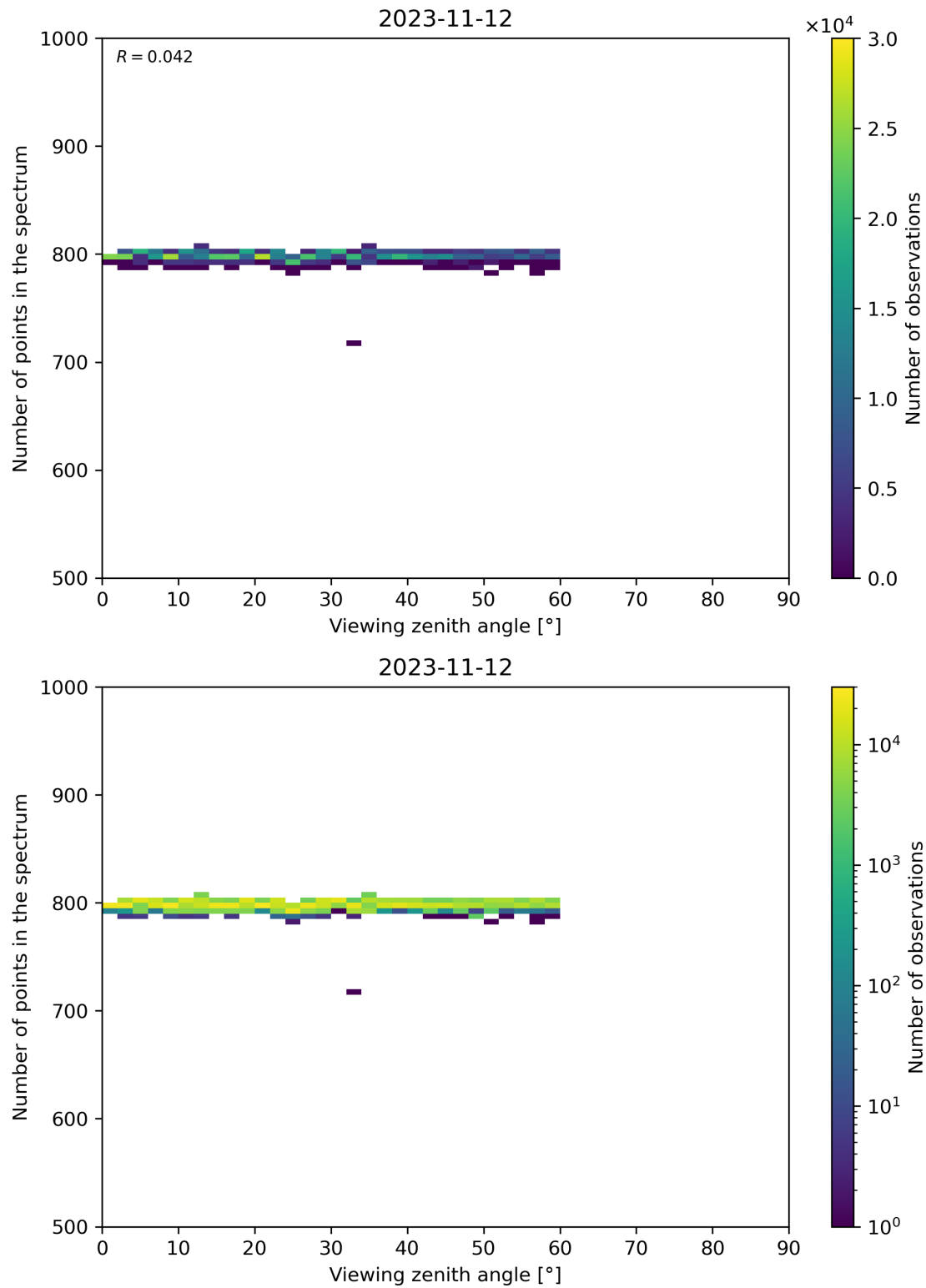
Figure 114: Scatter density plot of “Viewing zenith angle” against “Number of points in the spectrum” for 2023-11-12 to 2023-11-13.
