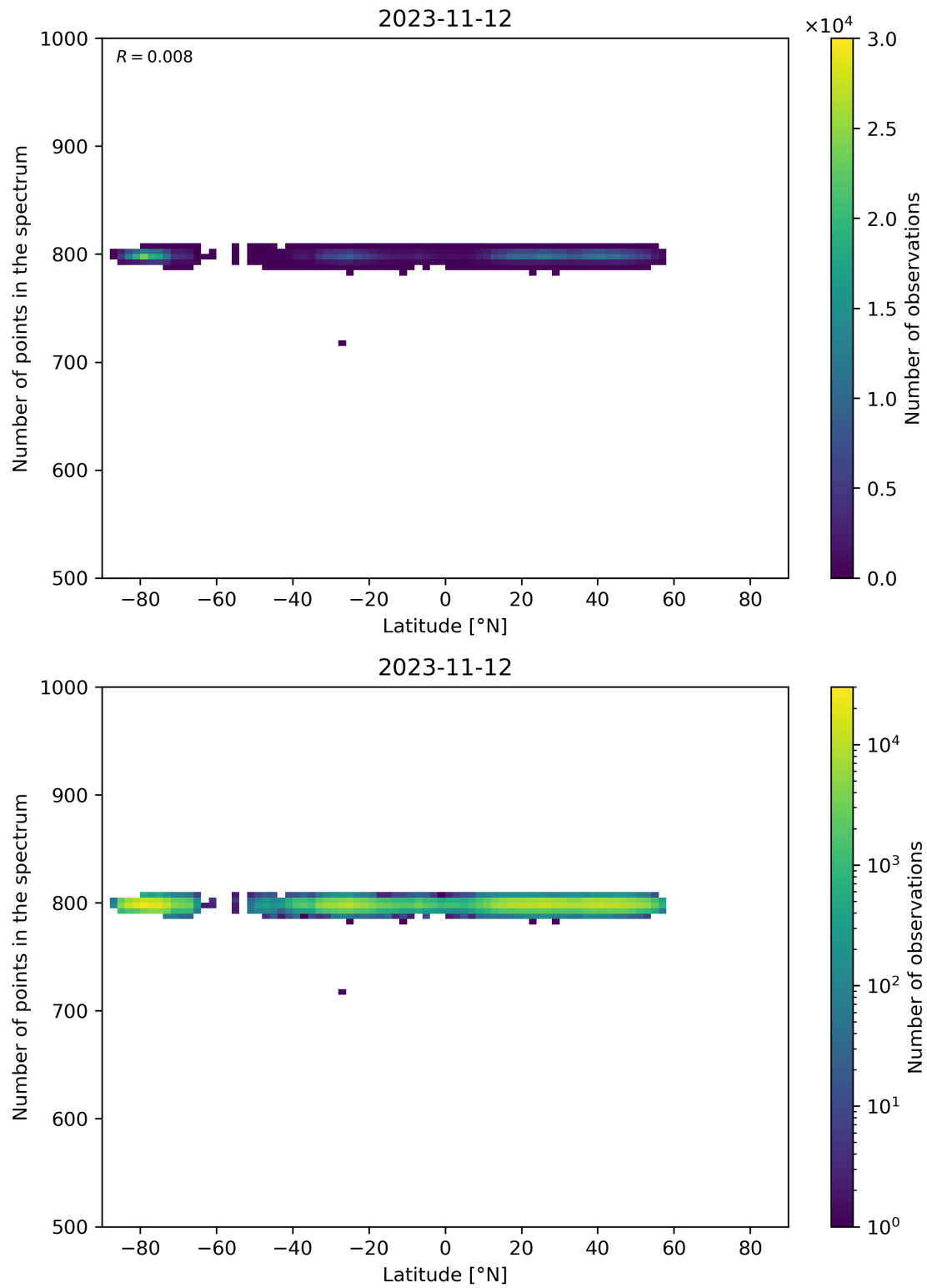
Figure 61: Scatter density plot of “Latitude” against “Number of points in the spectrum” for 2023-11-12 to 2023-11-13.
