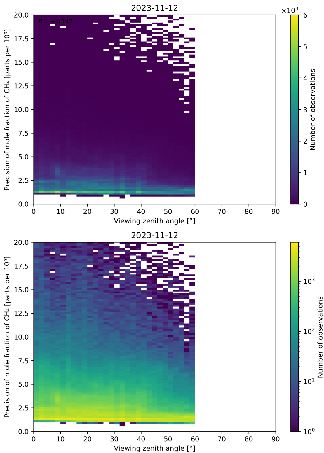
Figure 112: Scatter density plot of “Viewing zenith angle” against “Precision of mole fraction of CH 4 ” for 2023-11-12 to 2023-11-13.
