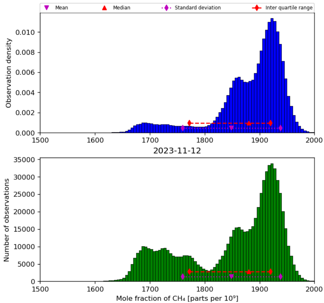
Figure 23: Histogram of “Mole fraction of CH 4 ” for 2023-11-12 to 2023-11-13
