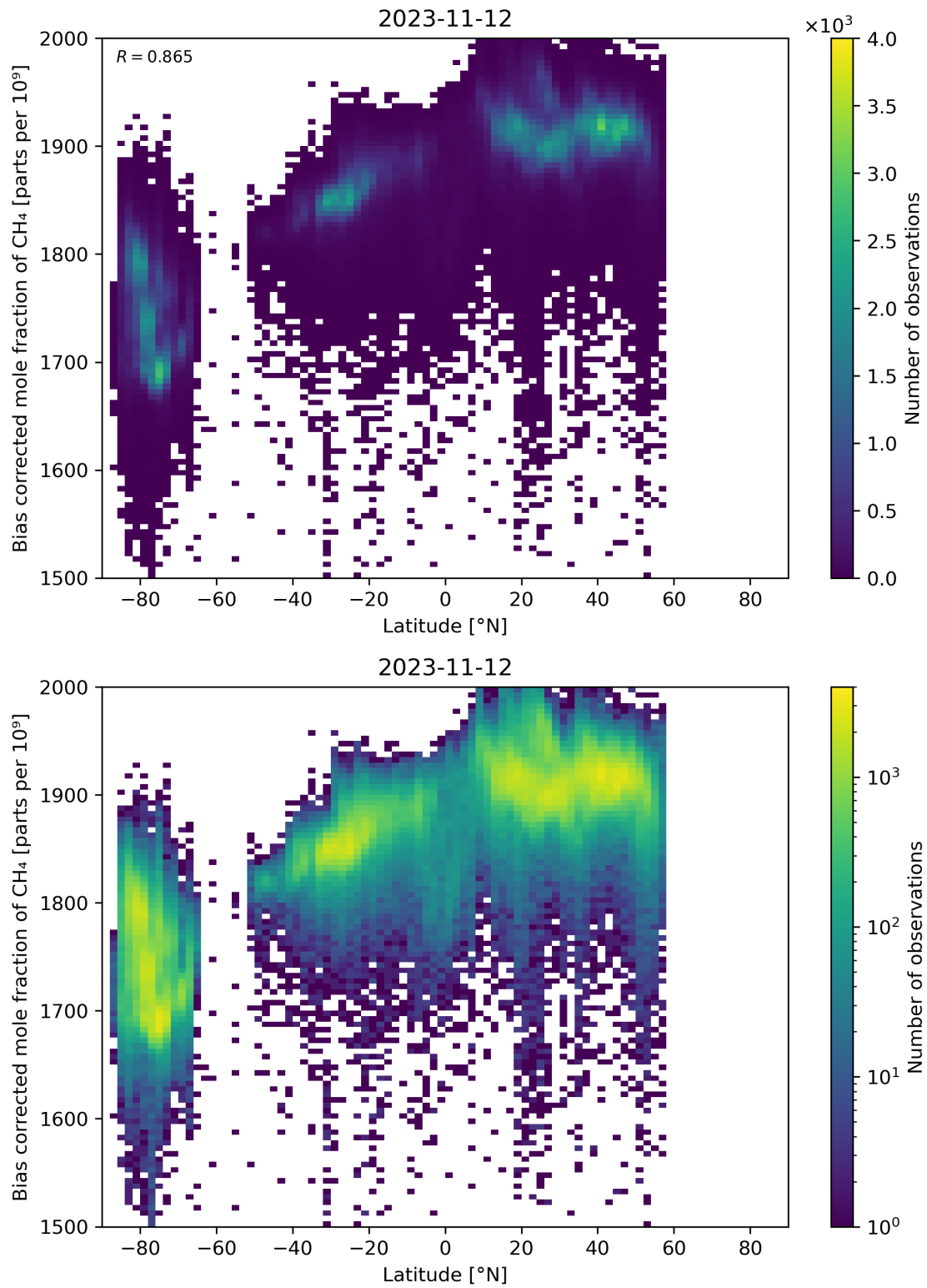
Figure 58: Scatter density plot of “Latitude” against “Bias corrected mole fraction of CH 4 ” for 2023-11-12 to 2023-11-13.
