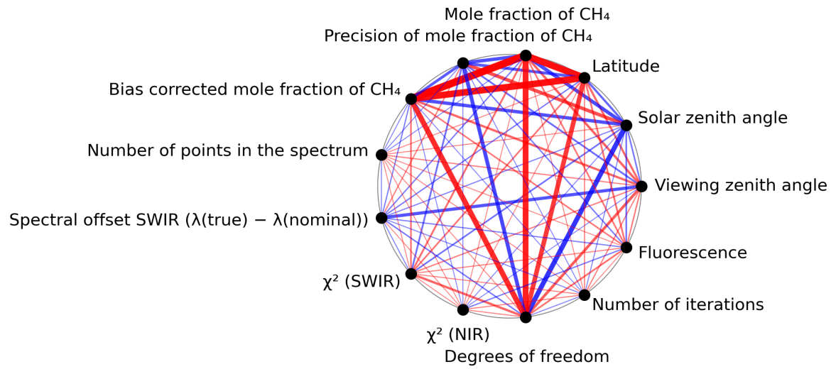
Figure 1: Map of correlation graph for 2023-11-12 to 2023-11-13.
