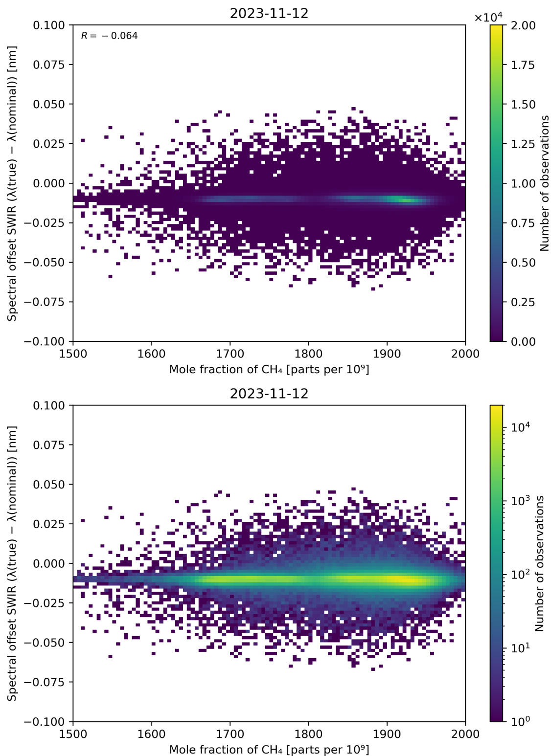
Figure 86: Scatter density plot of “Mole fraction of CH 4 ” against “Spectral offset SWIR ( \lambda(\text{true}) - \lambda(\text{nominal}) )” for 2023-11-12 to 2023-11-13.
