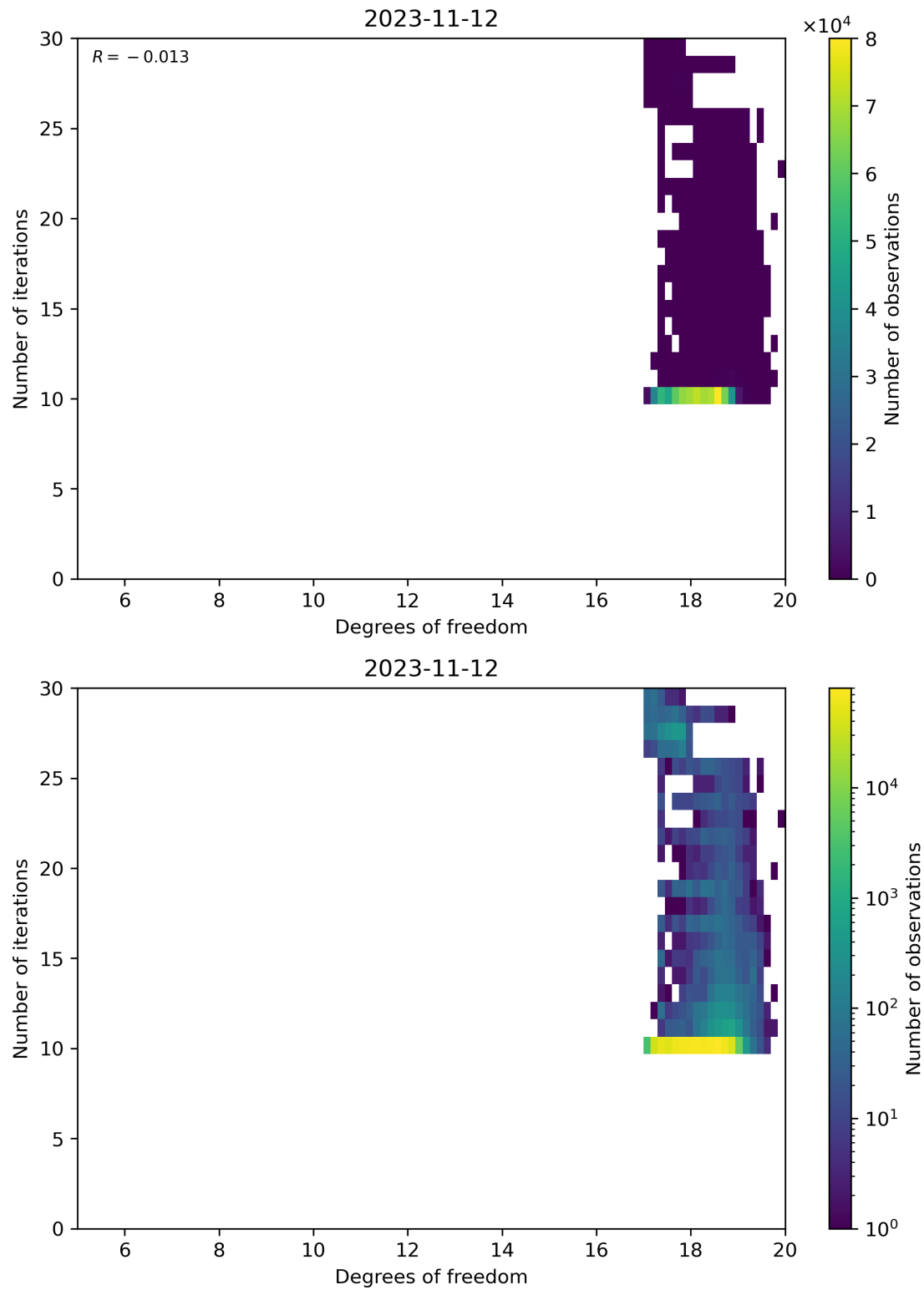
Figure 52: Scatter density plot of “Degrees of freedom” against “Number of iterations” for 2023-11-12 to 2023-11-13.
