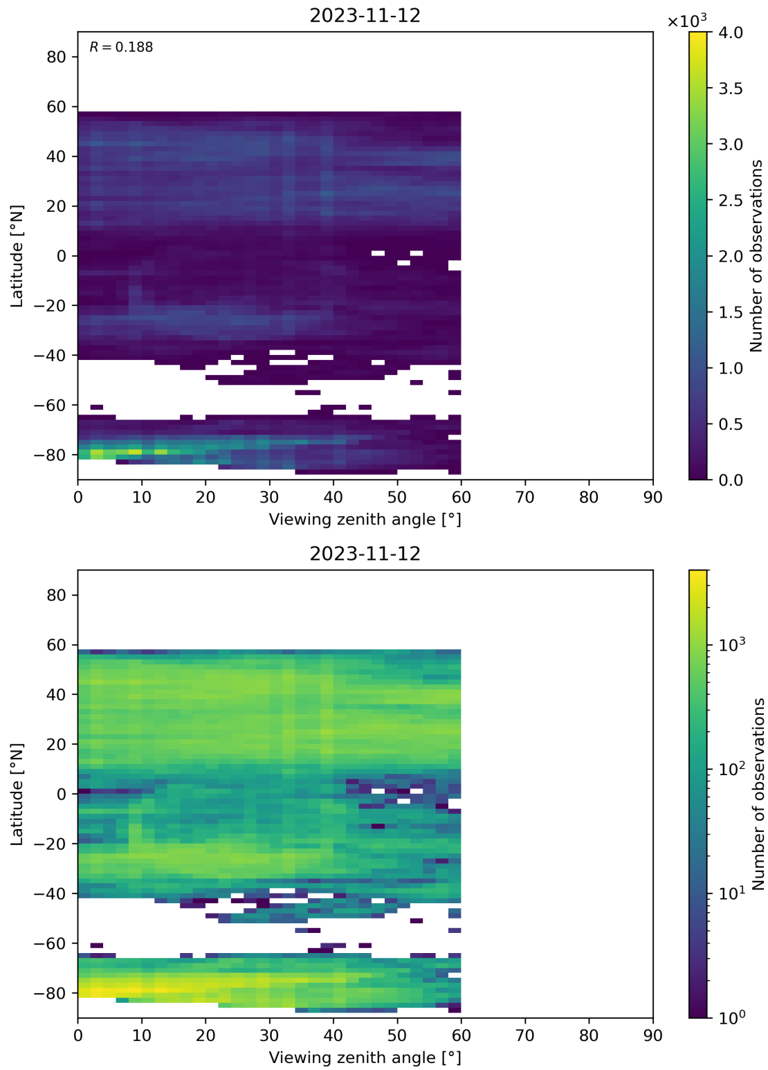
Figure 109: Scatter density plot of “Viewing zenith angle” against “Latitude” for 2023-11-12 to 2023-11-13.
