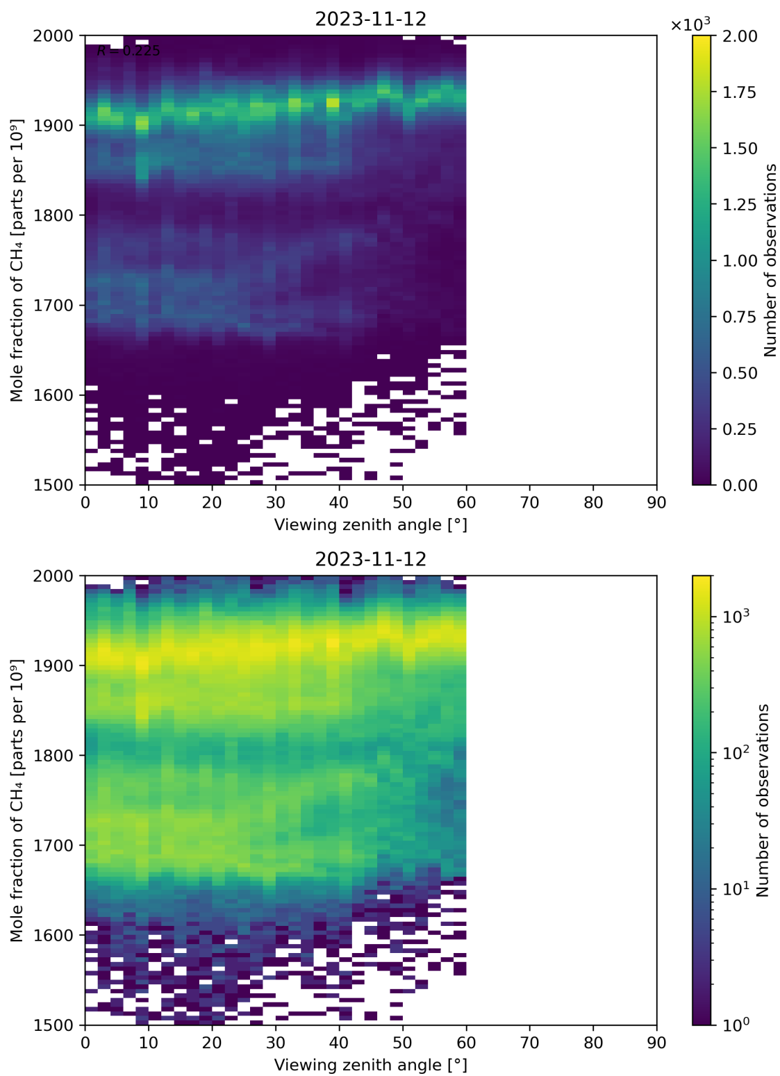
Figure 110: Scatter density plot of “Viewing zenith angle” against “Mole fraction of CH 4 ” for 2023-11-12 to 2023-11-13.
