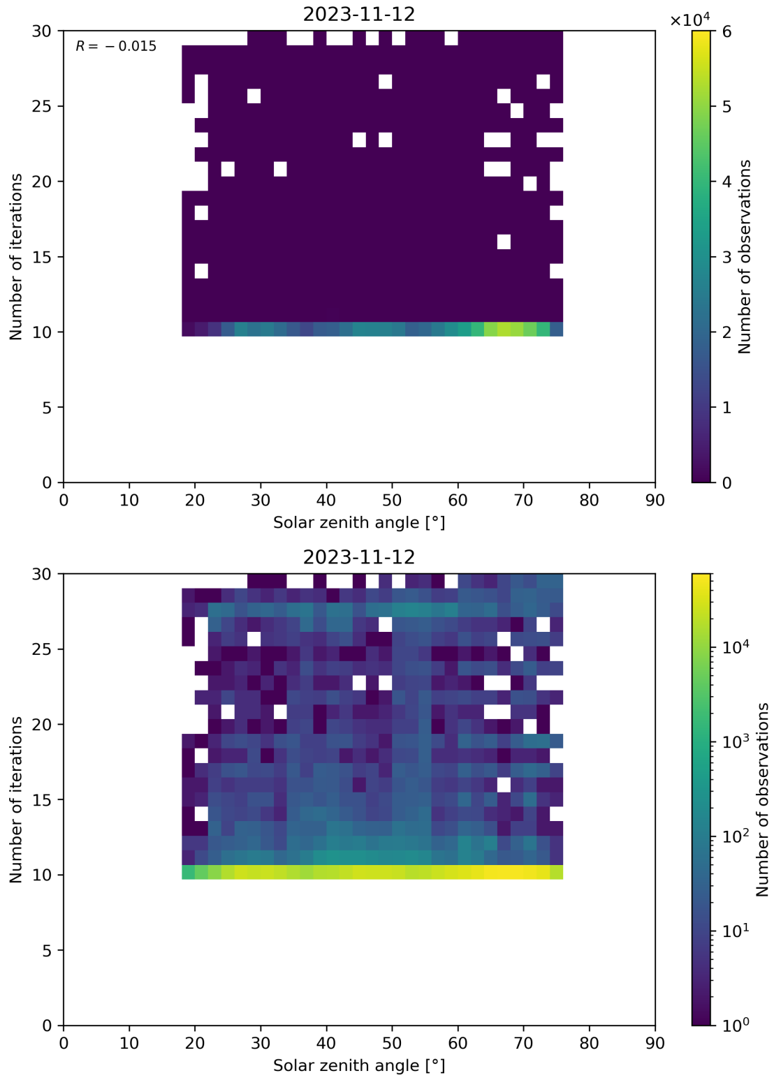
Figure 102: Scatter density plot of “Solar zenith angle” against “Number of iterations” for 2023-11-12 to 2023-11-13.
