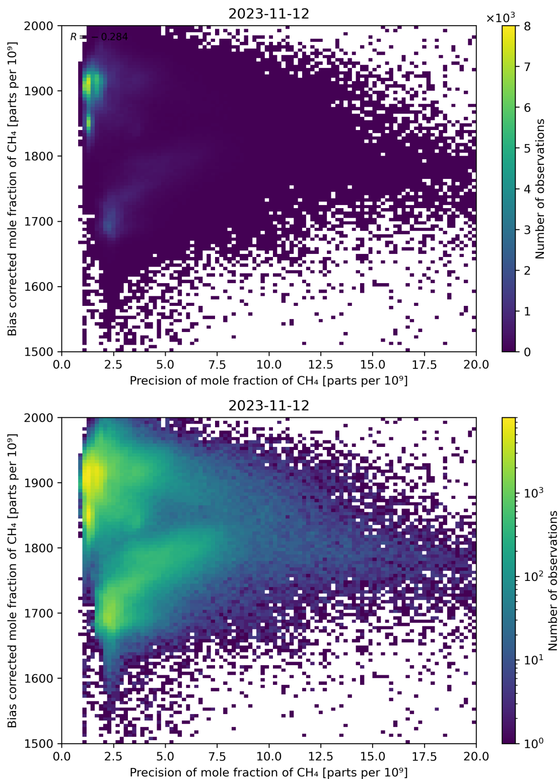
Figure 82: Scatter density plot of “Precision of mole fraction of CH 4 ” against “Bias corrected mole fraction of CH 4 ” for 2023-11-12 to 2023-11-13.
