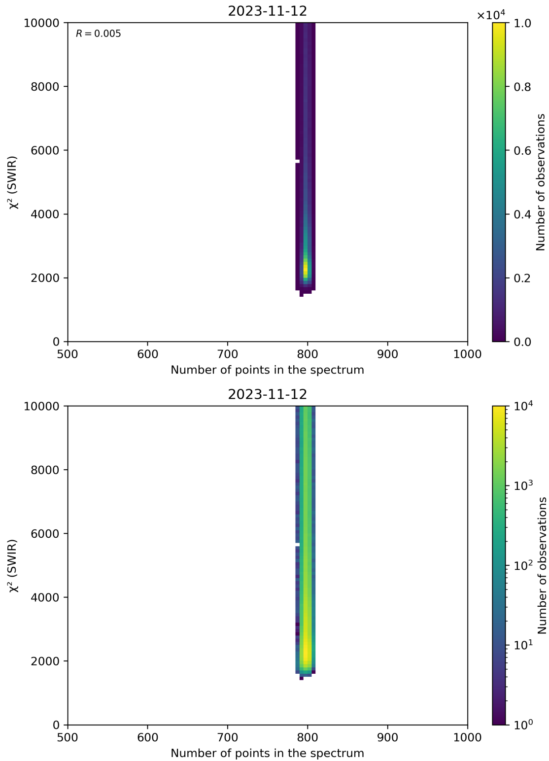
Figure 89: Scatter density plot of “Number of points in the spectrum” against “ \chi^2 (SWIR)” for 2023-11-12 to 2023-11-13.
