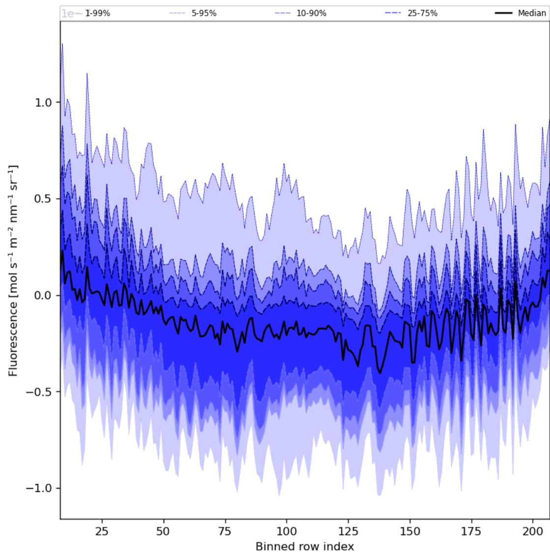
Figure 43: Along track statistics of “Fluorescence” for 2023-11-12 to 2023-11-13
