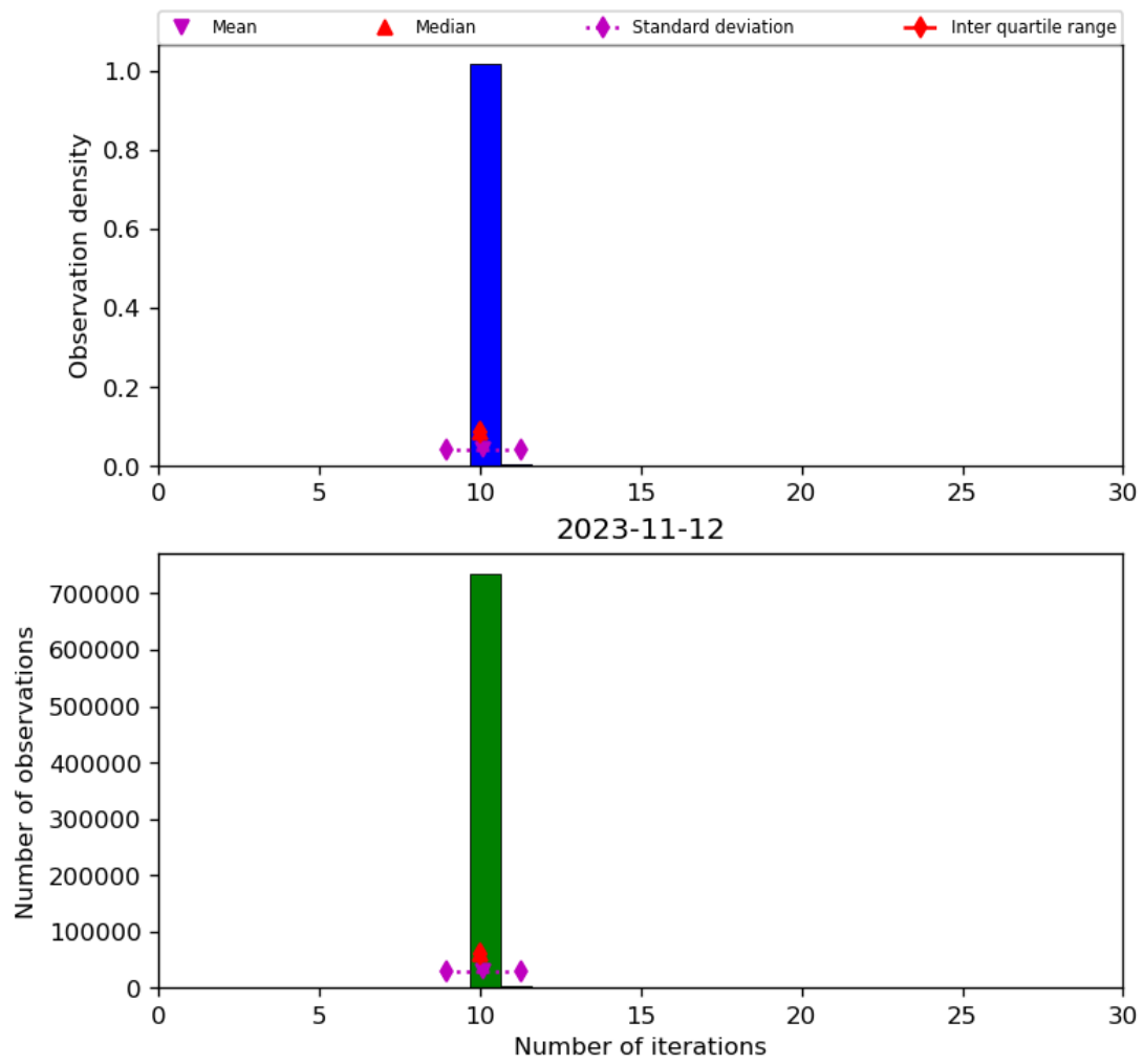
Figure 31: Histogram of “Number of iterations” for 2023-11-12 to 2023-11-13
