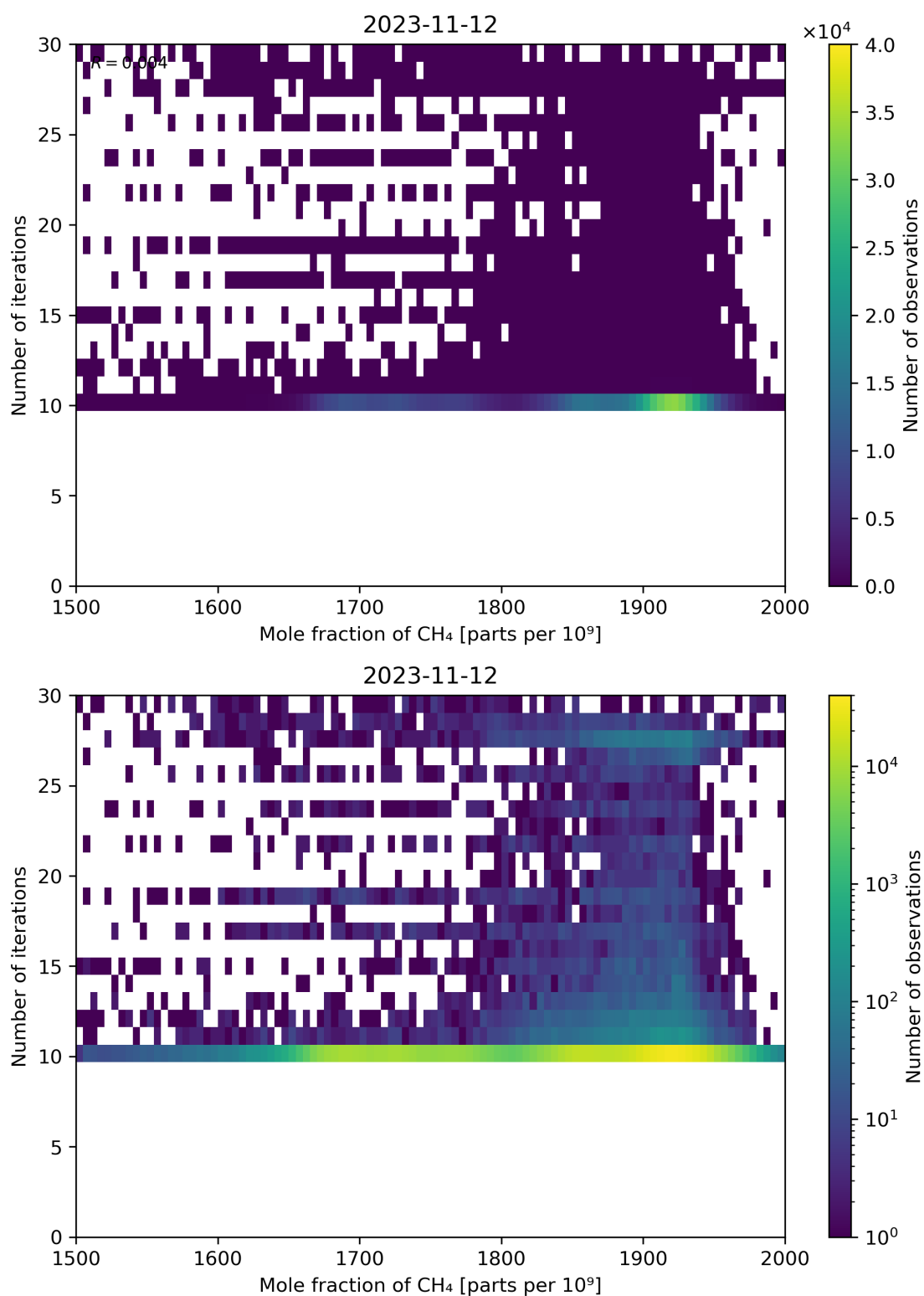
Figure 76: Scatter density plot of “Mole fraction of CH 4 ” against “Number of iterations” for 2023-11-12 to 2023-11-13.
