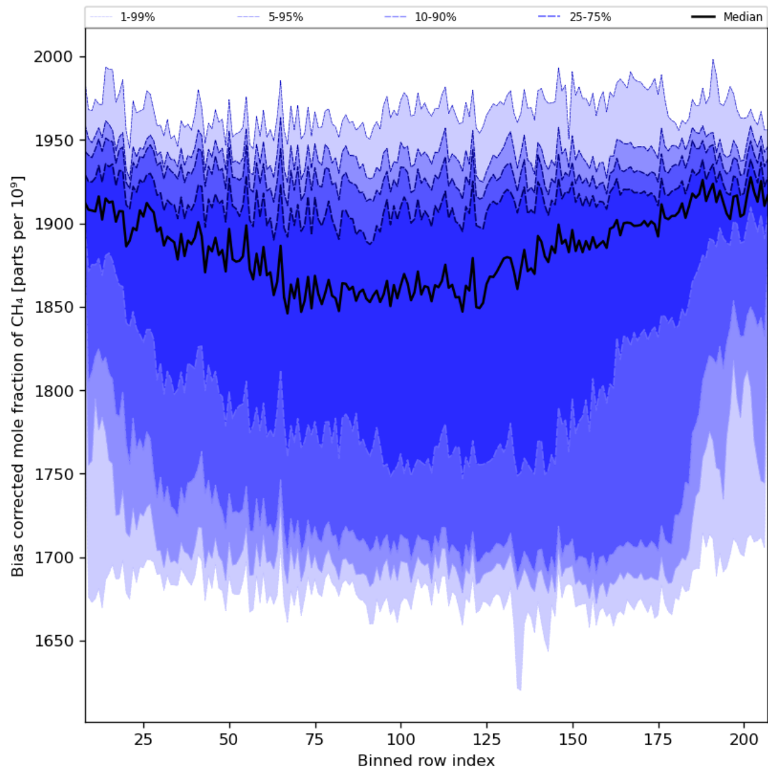
Figure 36: Along track statistics of “Bias corrected mole fraction of CH 4 ” for 2023-11-12 to 2023-11-13
