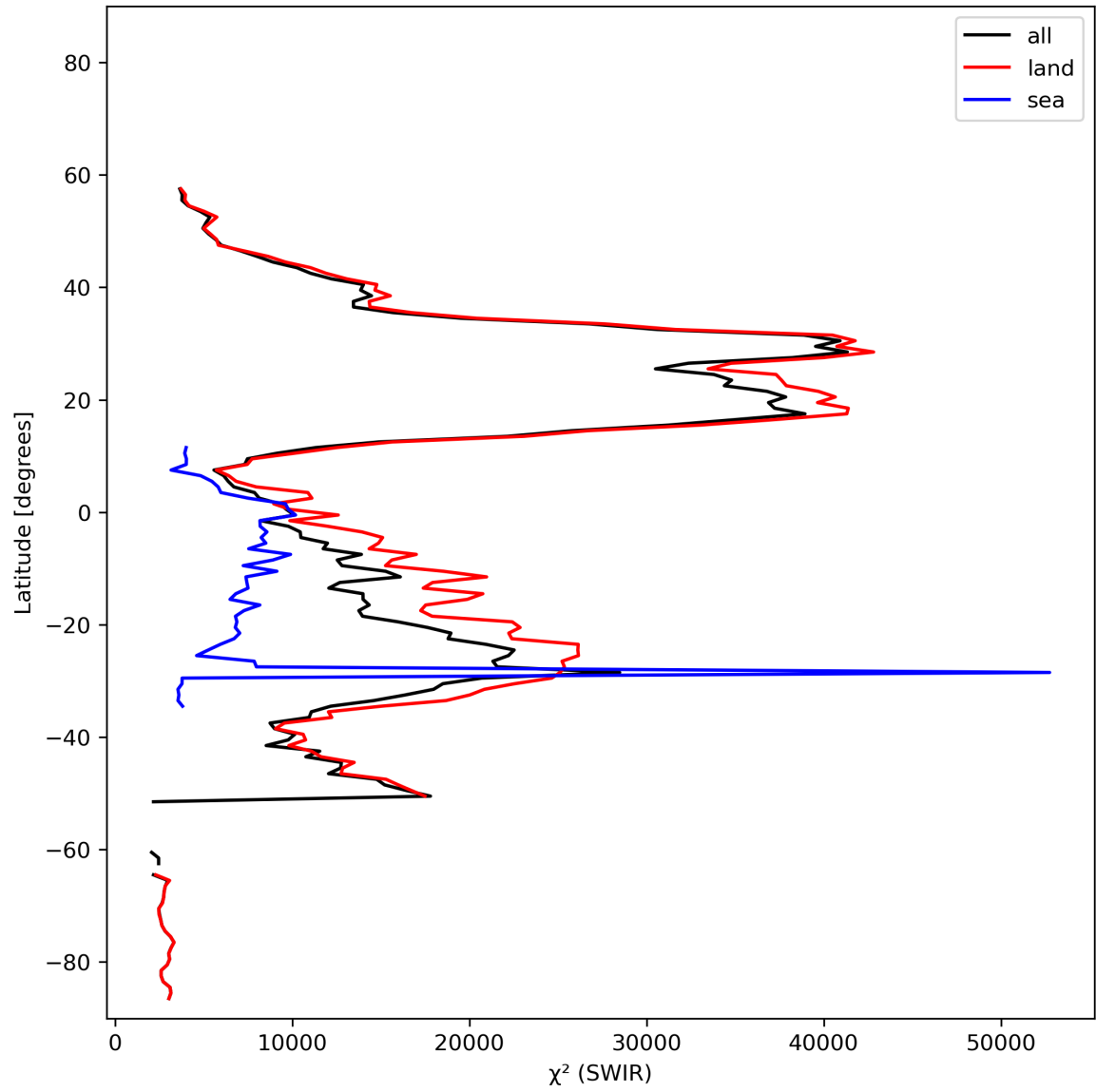
Figure 17: Zonal average of “ \chi^2 (SWIR)” for 2023-11-12 to 2023-11-13.
