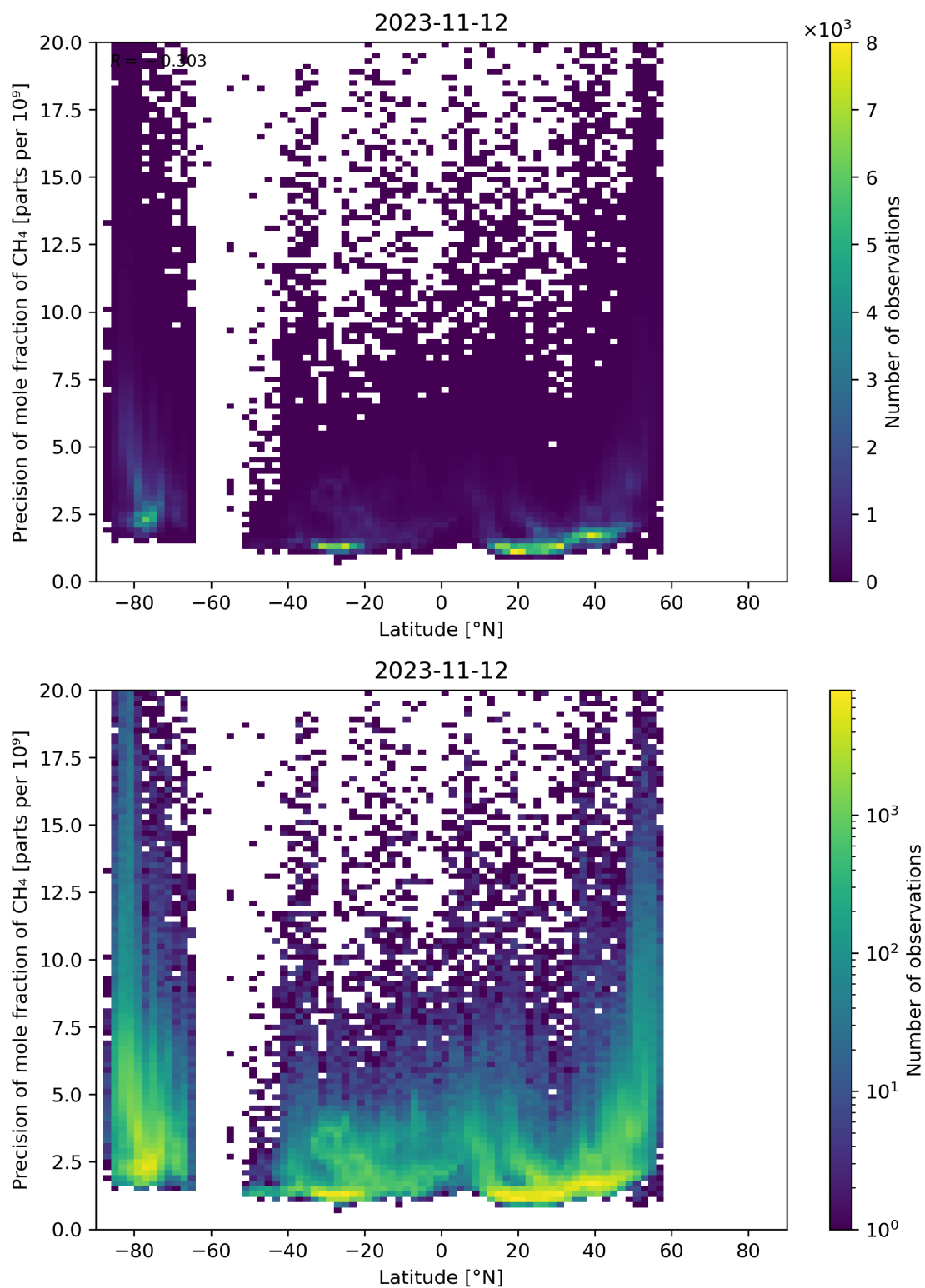
Figure 59: Scatter density plot of “Latitude” against “Precision of mole fraction of CH 4 ” for 2023-11-12 to 2023-11-13.
