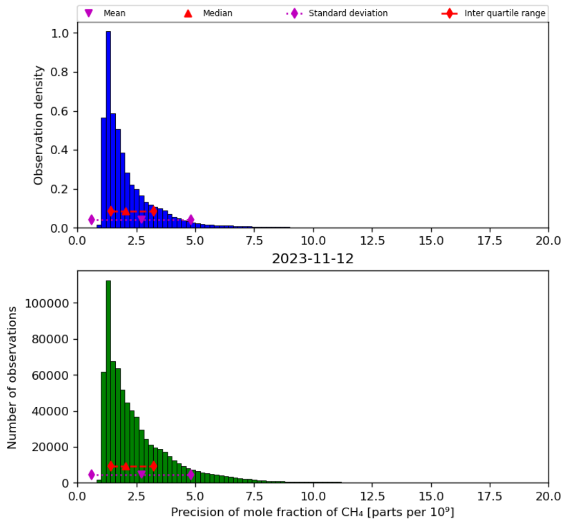
Figure 24: Histogram of “Precision of mole fraction of CH 4 ” for 2023-11-12 to 2023-11-13
