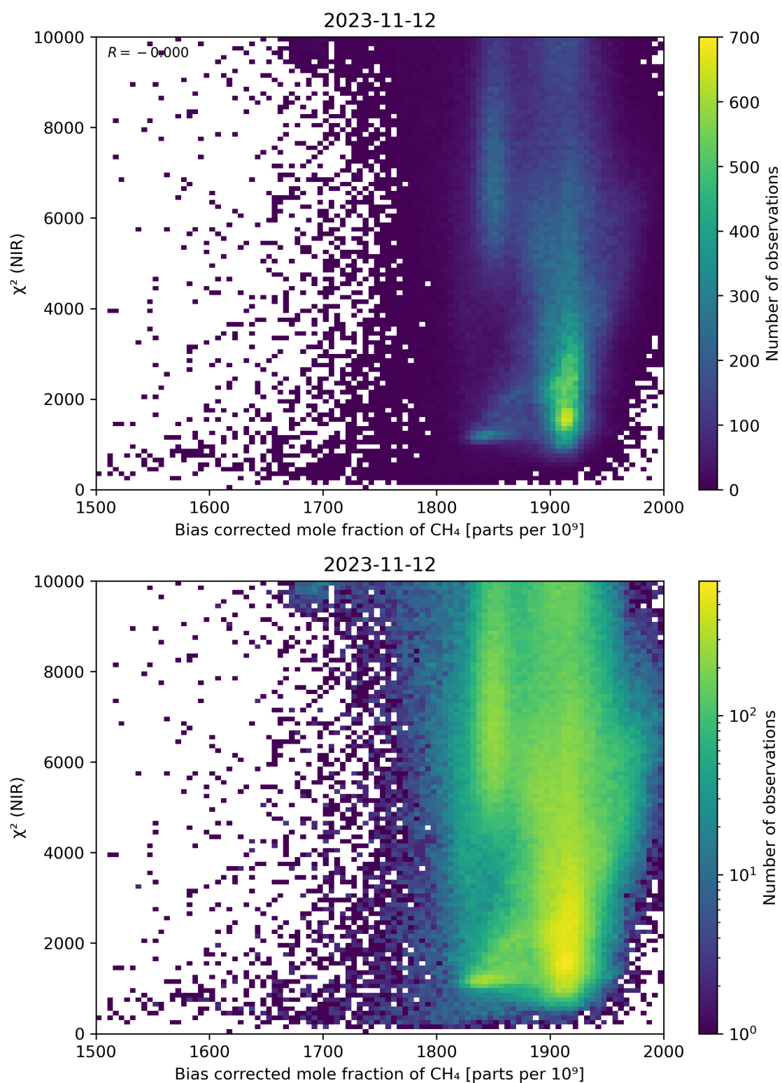
Figure 63: Scatter density plot of “Bias corrected mole fraction of CH 4 ” against “ \chi^2 (NIR)” for 2023-11-12 to 2023-11-13.
