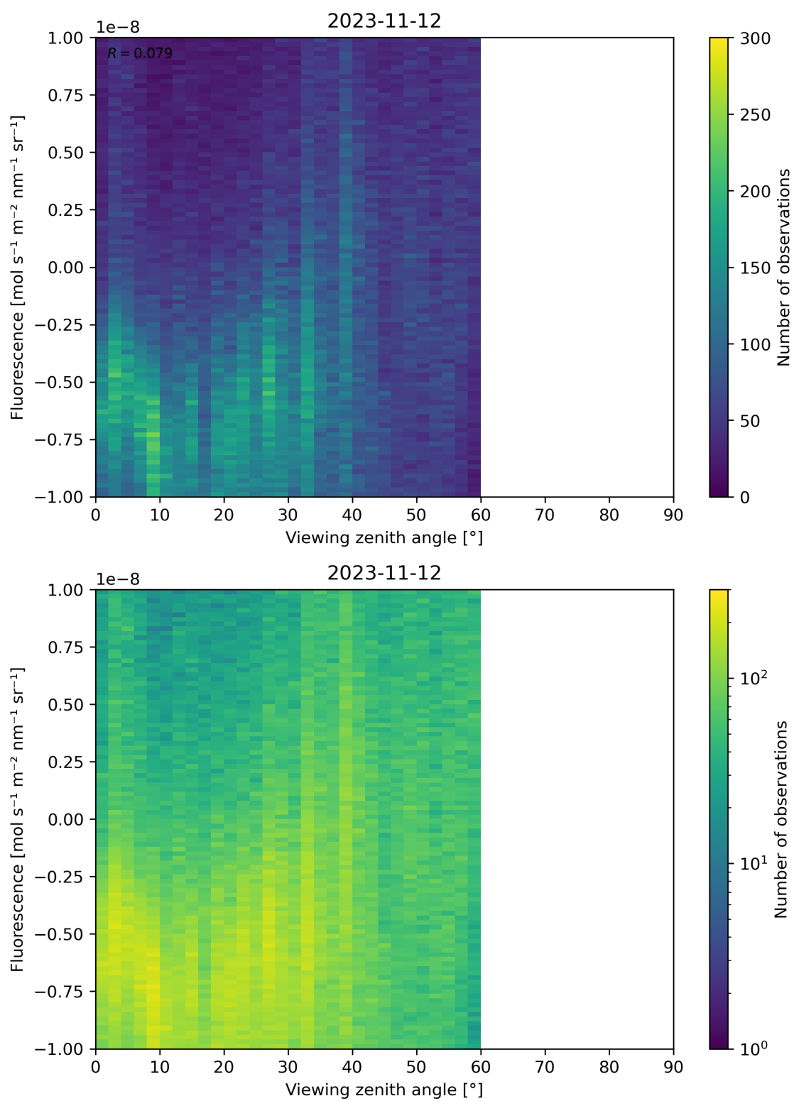
Figure 108: Scatter density plot of “Viewing zenith angle” against “Fluorescence” for 2023-11-12 to 2023-11-13.
