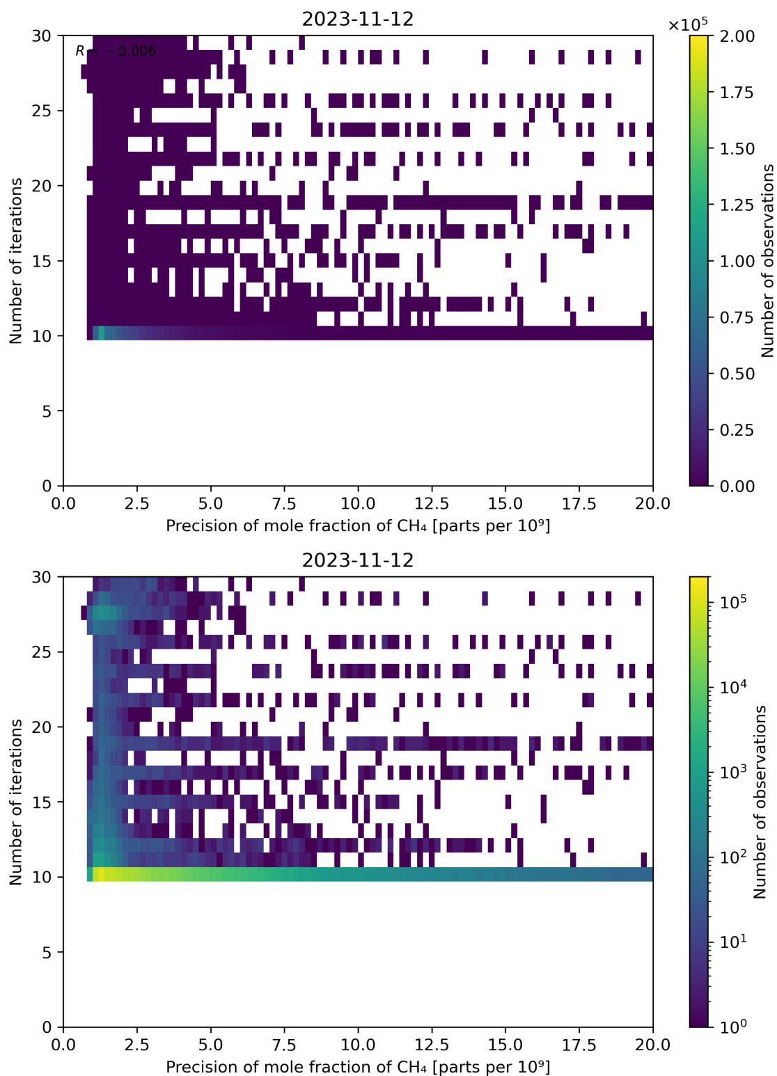
Figure 83: Scatter density plot of “Precision of mole fraction of CH 4 ” against “Number of iterations” for 2023-11-12 to 2023-11-13.
