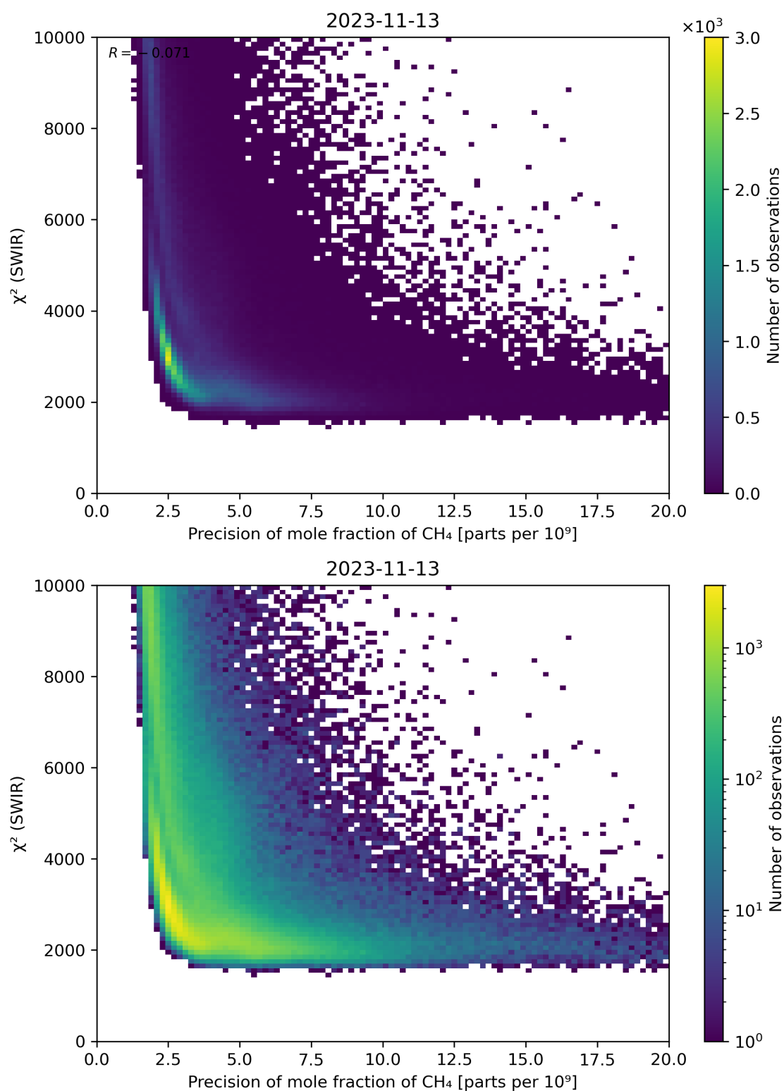
Figure 79: Scatter density plot of “Precision of mole fraction of \text{CH}_4 ” against “ \chi^2 (SWIR)” for 2023-11-13 to 2023-11-14.
