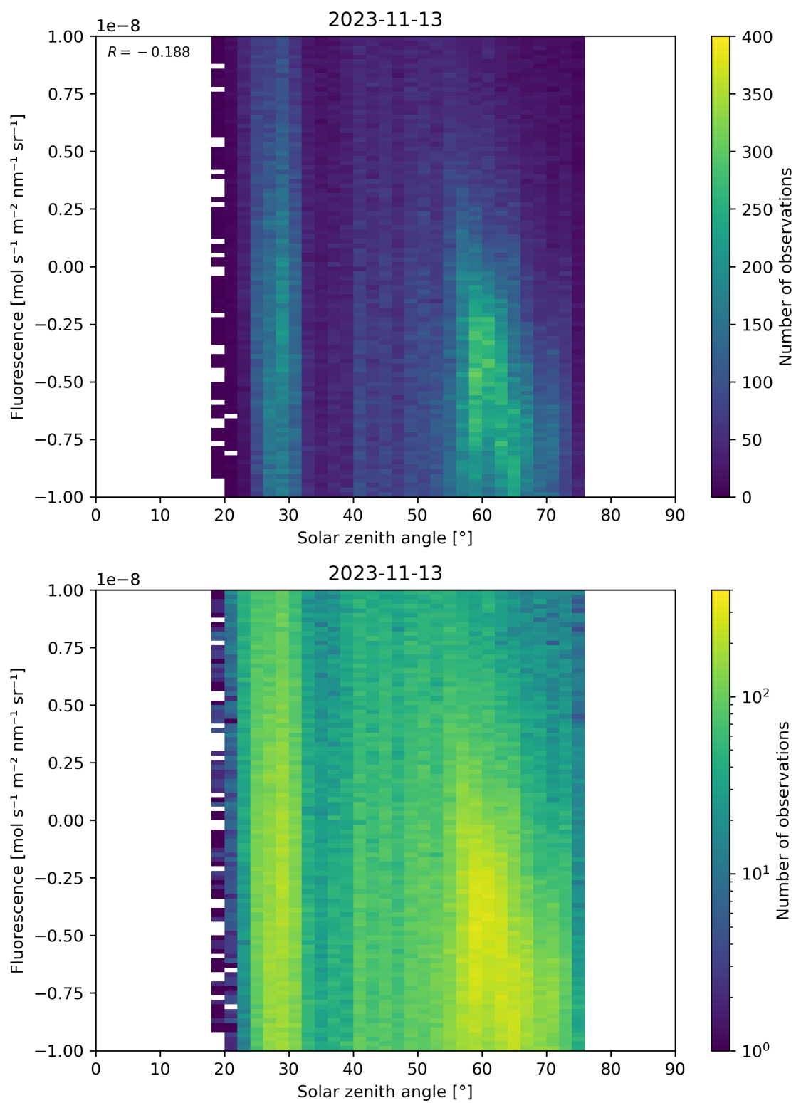
Figure 97: Scatter density plot of “Solar zenith angle” against “Fluorescence” for 2023-11-13 to 2023-11-14.
