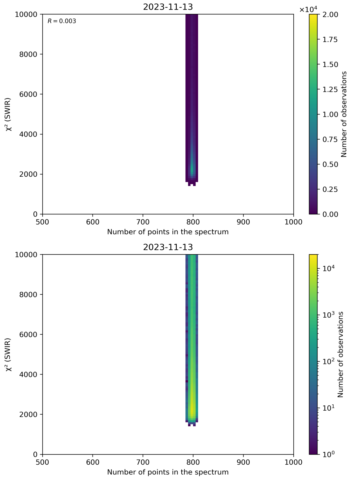
Figure 89: Scatter density plot of “Number of points in the spectrum” against “ \chi^2 (SWIR)” for 2023-11-13 to 2023-11-14.
