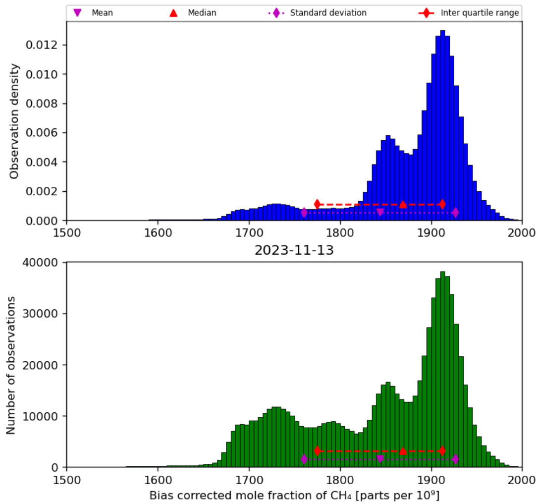
Figure 25: Histogram of “Bias corrected mole fraction of CH 4 ” for 2023-11-13 to 2023-11-14
