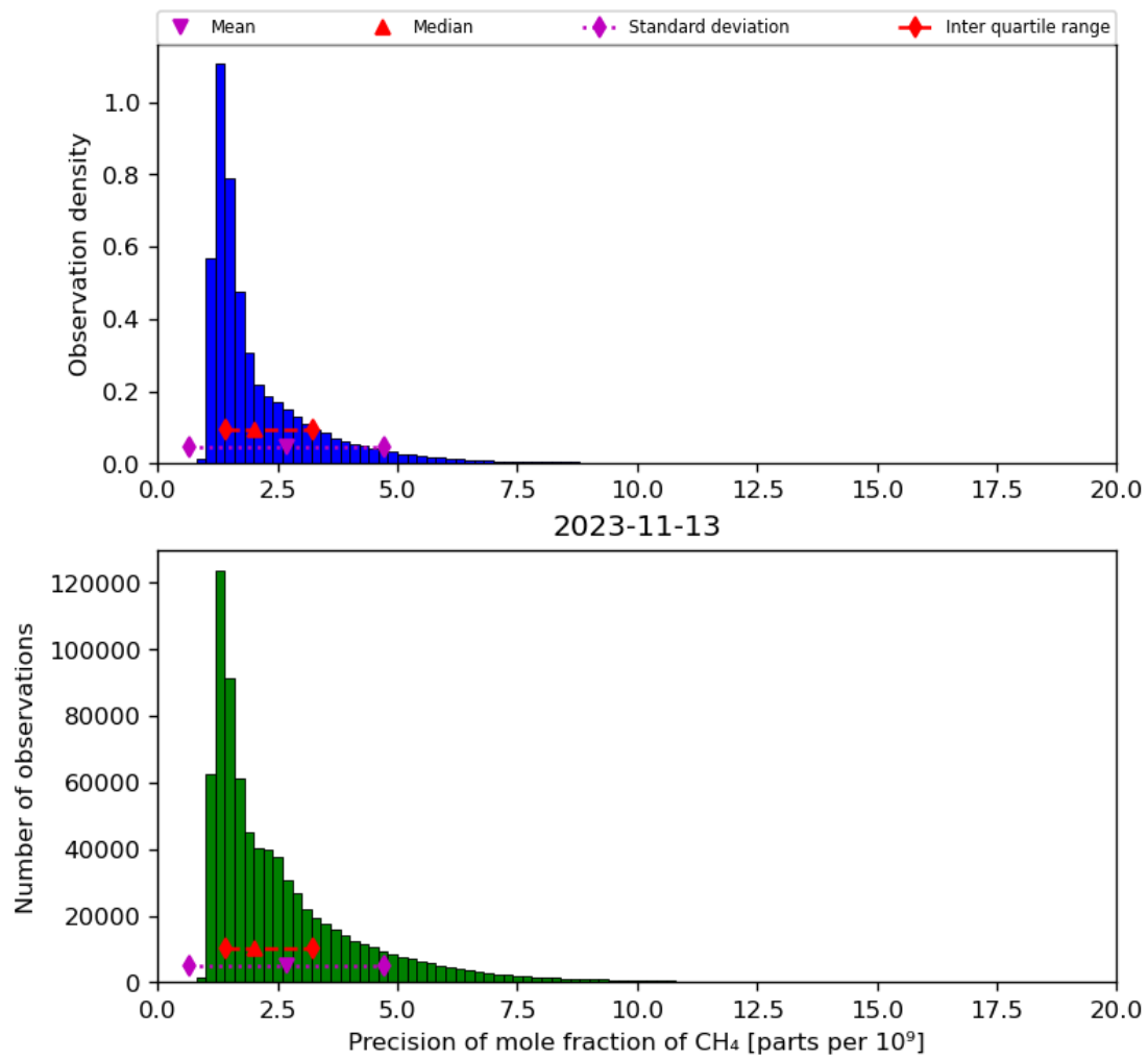
Figure 24: Histogram of “Precision of mole fraction of CH 4 ” for 2023-11-13 to 2023-11-14
