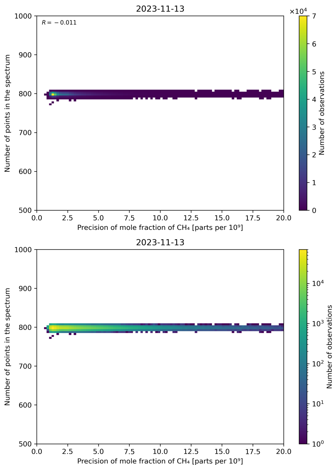
Figure 84: Scatter density plot of “Precision of mole fraction of CH 4 ” against “Number of points in the spectrum” for 2023-11-13 to 2023-11-14.
