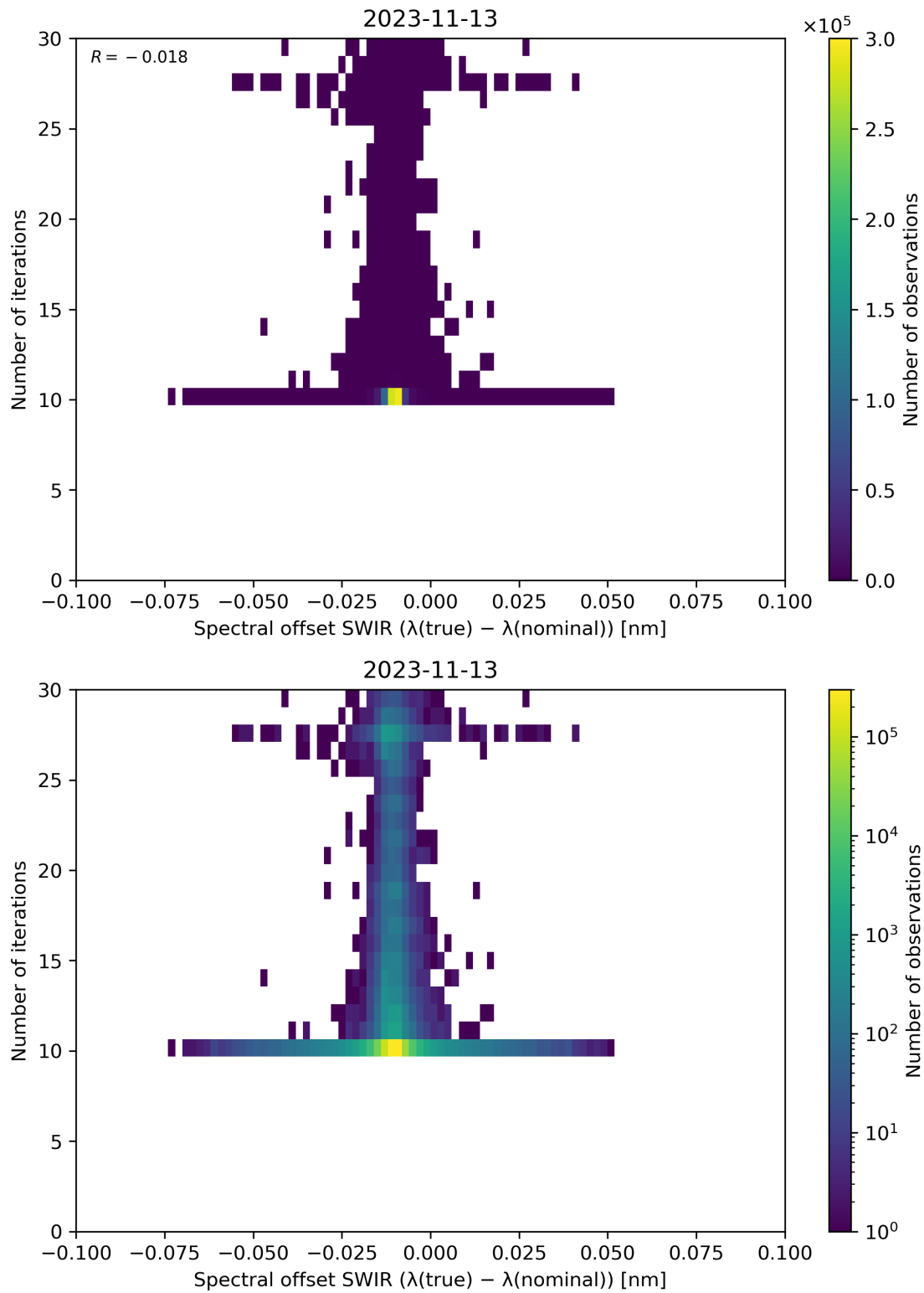
Figure 121: Scatter density plot of “Spectral offset SWIR ( \lambda(\text{true}) - \lambda(\text{nominal}) )” against “Number of iterations” for 2023-11-13 to 2023-11-14.
