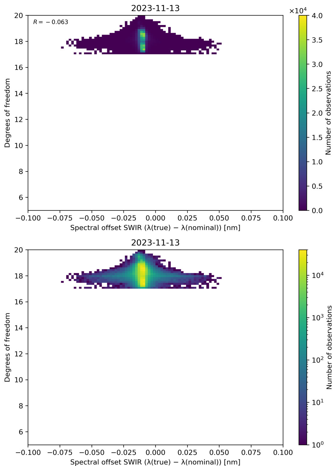
Figure 119: Scatter density plot of “Spectral offset SWIR ( \lambda(\text{true}) - \lambda(\text{nominal}) )” against “Degrees of freedom” for 2023-11-13 to 2023-11-14.
