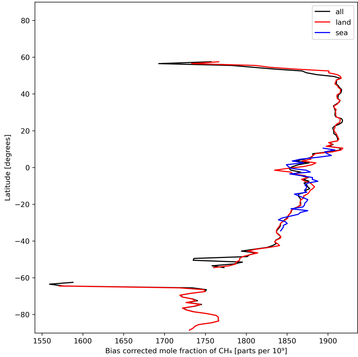
Figure 14: Zonal average of “Bias corrected mole fraction of \text{CH}_4 ” for 2023-11-13 to 2023-11-14.
