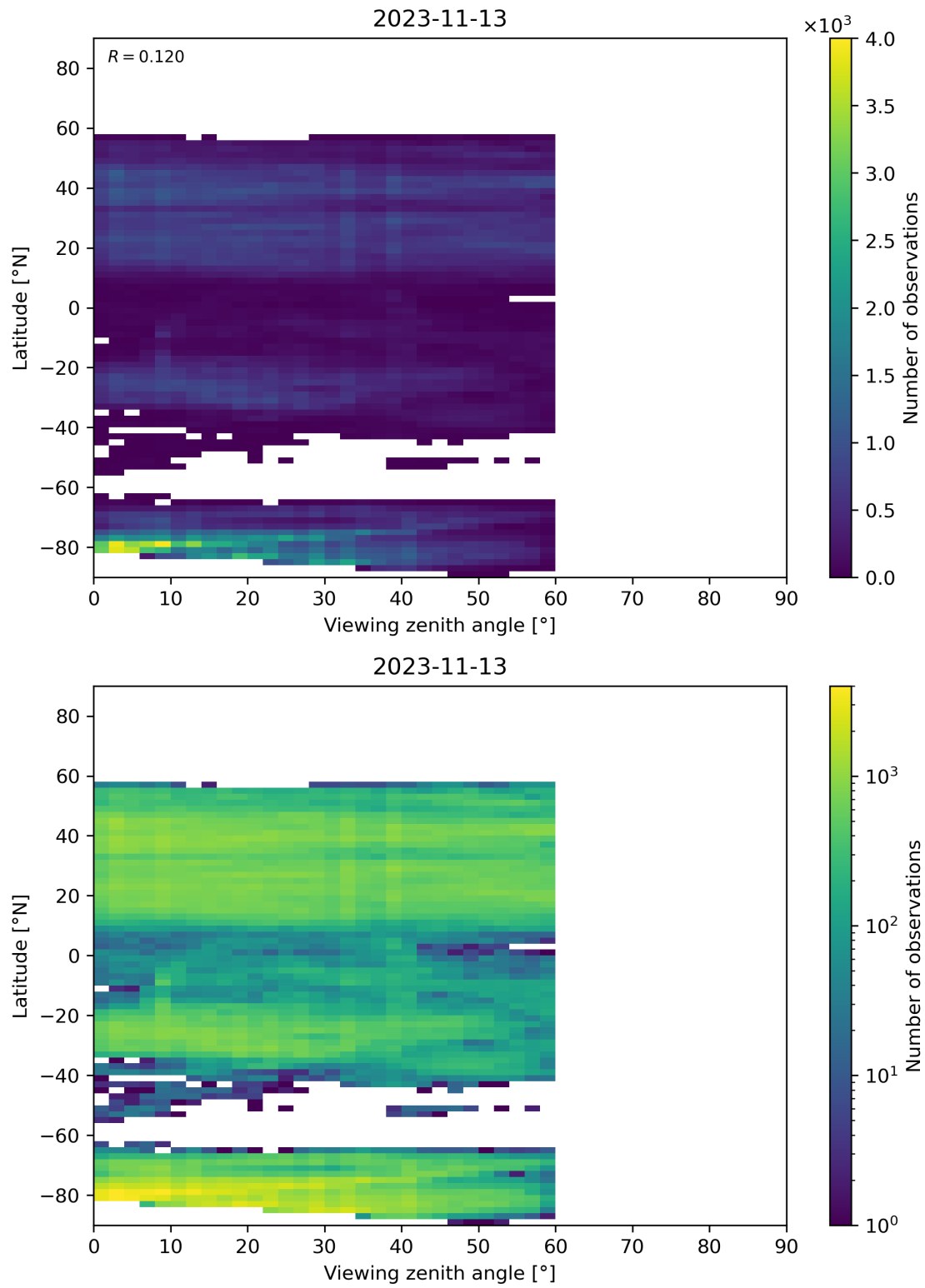
Figure 109: Scatter density plot of “Viewing zenith angle” against “Latitude” for 2023-11-13 to 2023-11-14.
