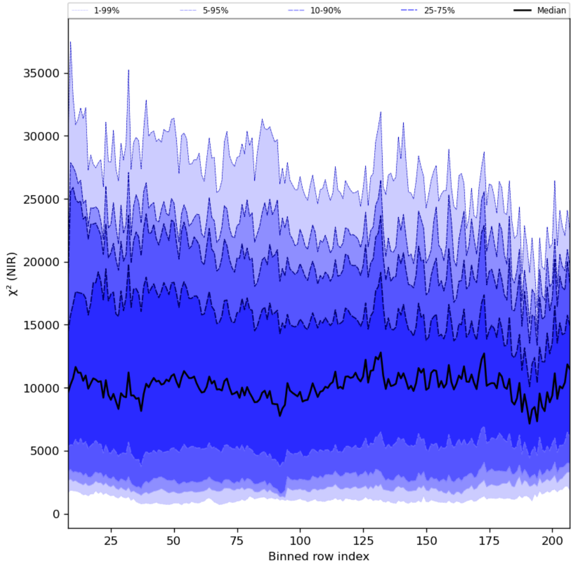
Figure 40: Along track statistics of “ \chi^2 (NIR)” for 2023-11-13 to 2023-11-14
