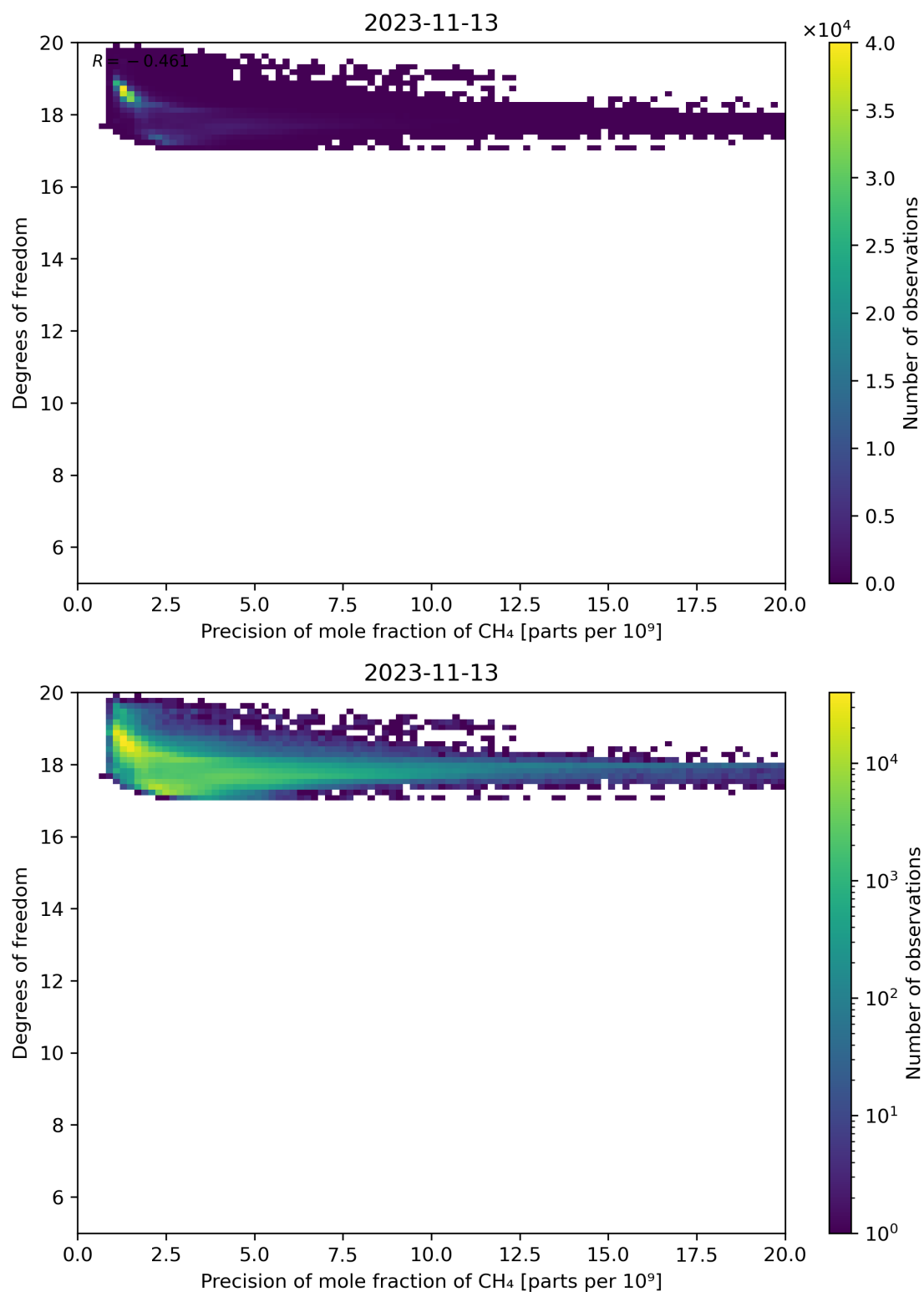
Figure 80: Scatter density plot of “Precision of mole fraction of CH 4 ” against “Degrees of freedom” for 2023-11-13 to 2023-11-14.
