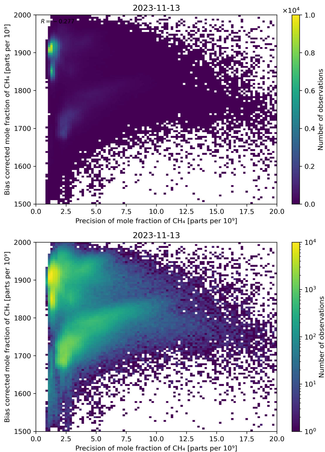
Figure 82: Scatter density plot of “Precision of mole fraction of CH 4 ” against “Bias corrected mole fraction of CH 4 ” for 2023-11-13 to 2023-11-14.
