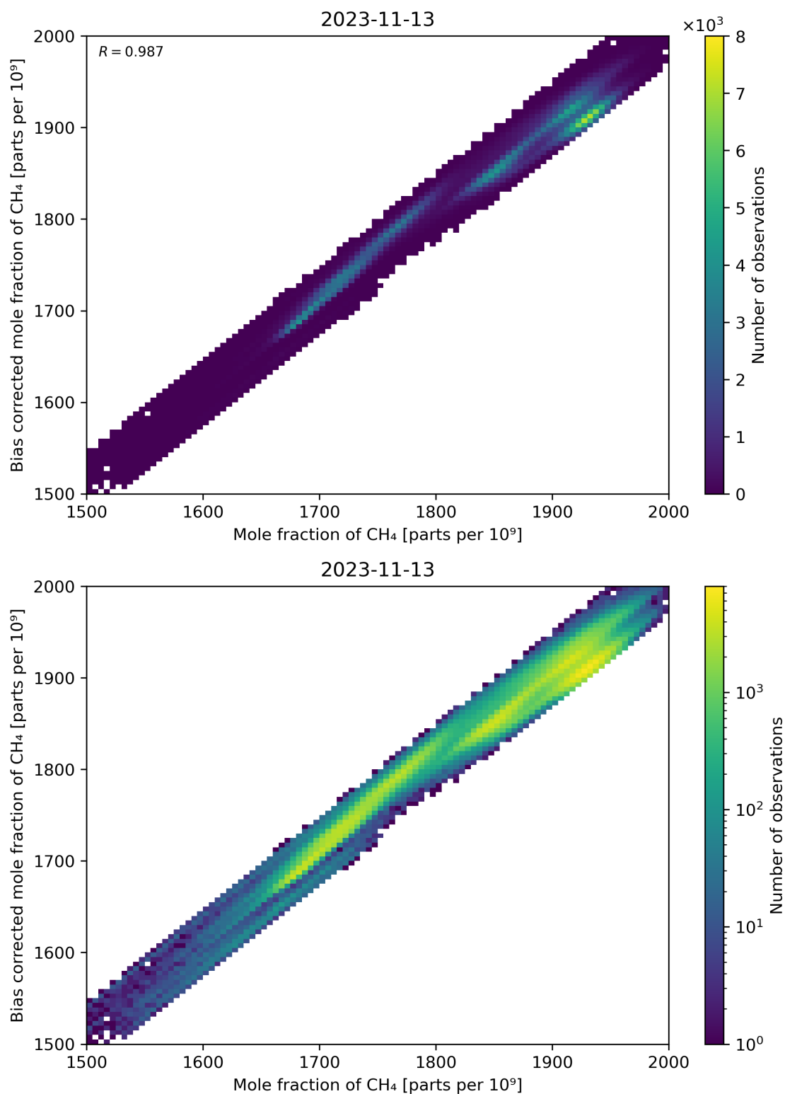
Figure 74: Scatter density plot of “Mole fraction of CH 4 ” against “Bias corrected mole fraction of CH 4 ” for 2023-11-13 to 2023-11-14.
