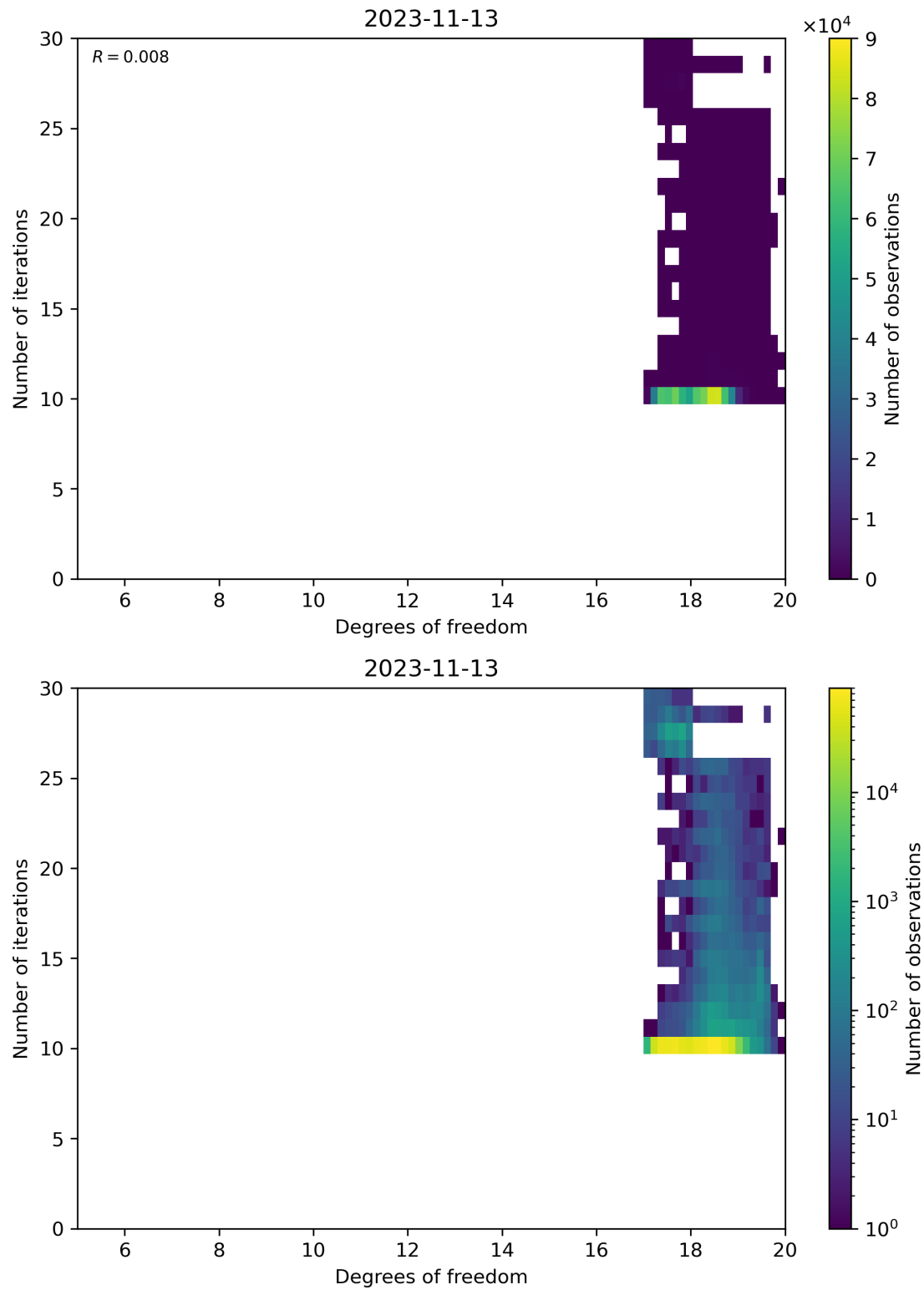
Figure 52: Scatter density plot of “Degrees of freedom” against “Number of iterations” for 2023-11-13 to 2023-11-14.
