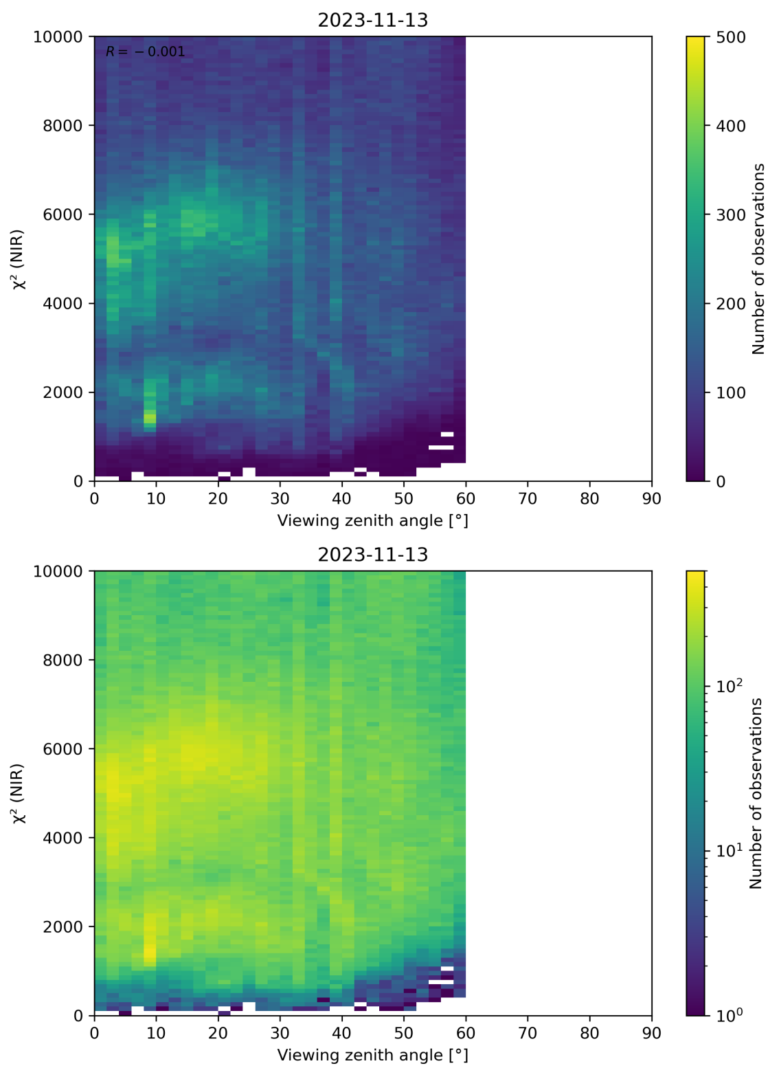
Figure 105: Scatter density plot of “Viewing zenith angle” against “ \chi^2 (NIR)” for 2023-11-13 to 2023-11-14.
