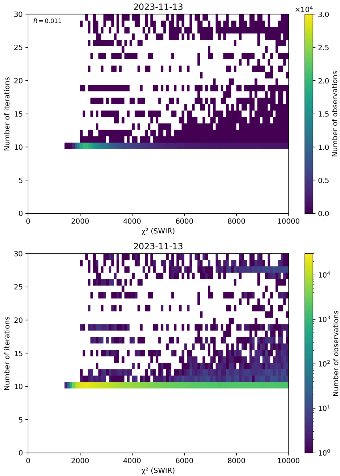
Figure 50: Scatter density plot of “ \chi^2 (SWIR)” against “Number of iterations” for 2023-11-13 to 2023-11-14.
