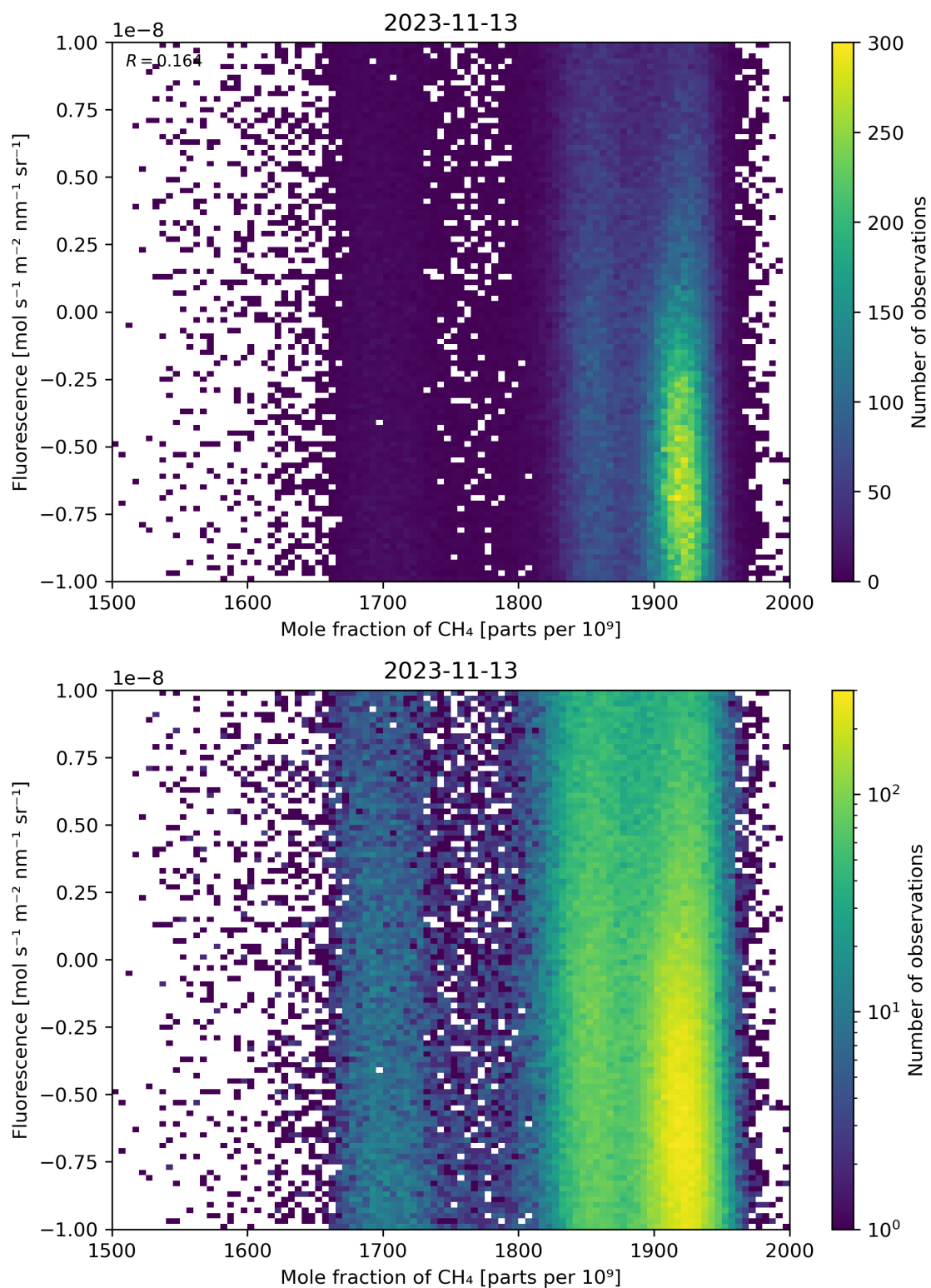
Figure 73: Scatter density plot of “Mole fraction of \text{CH}_4 ” against “Fluorescence” for 2023-11-13 to 2023-11-14.
