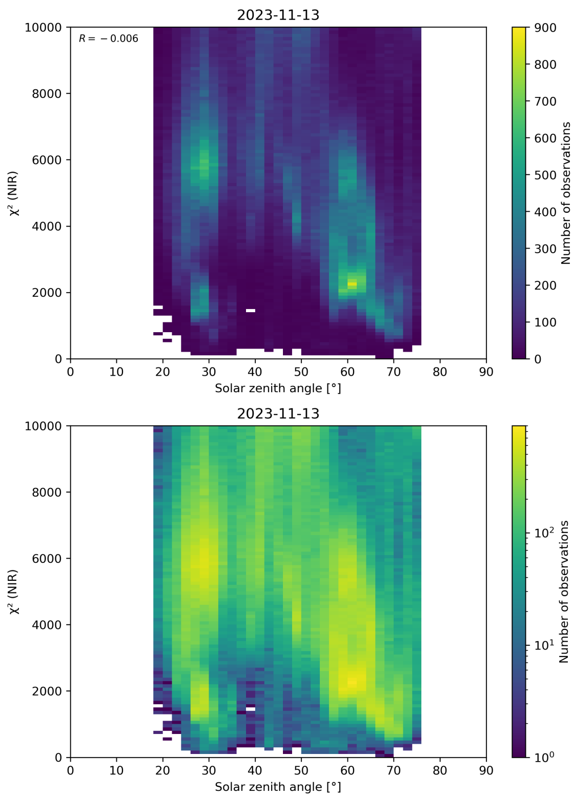
Figure 94: Scatter density plot of “Solar zenith angle” against “ \chi^2 (NIR)” for 2023-11-13 to 2023-11-14.
