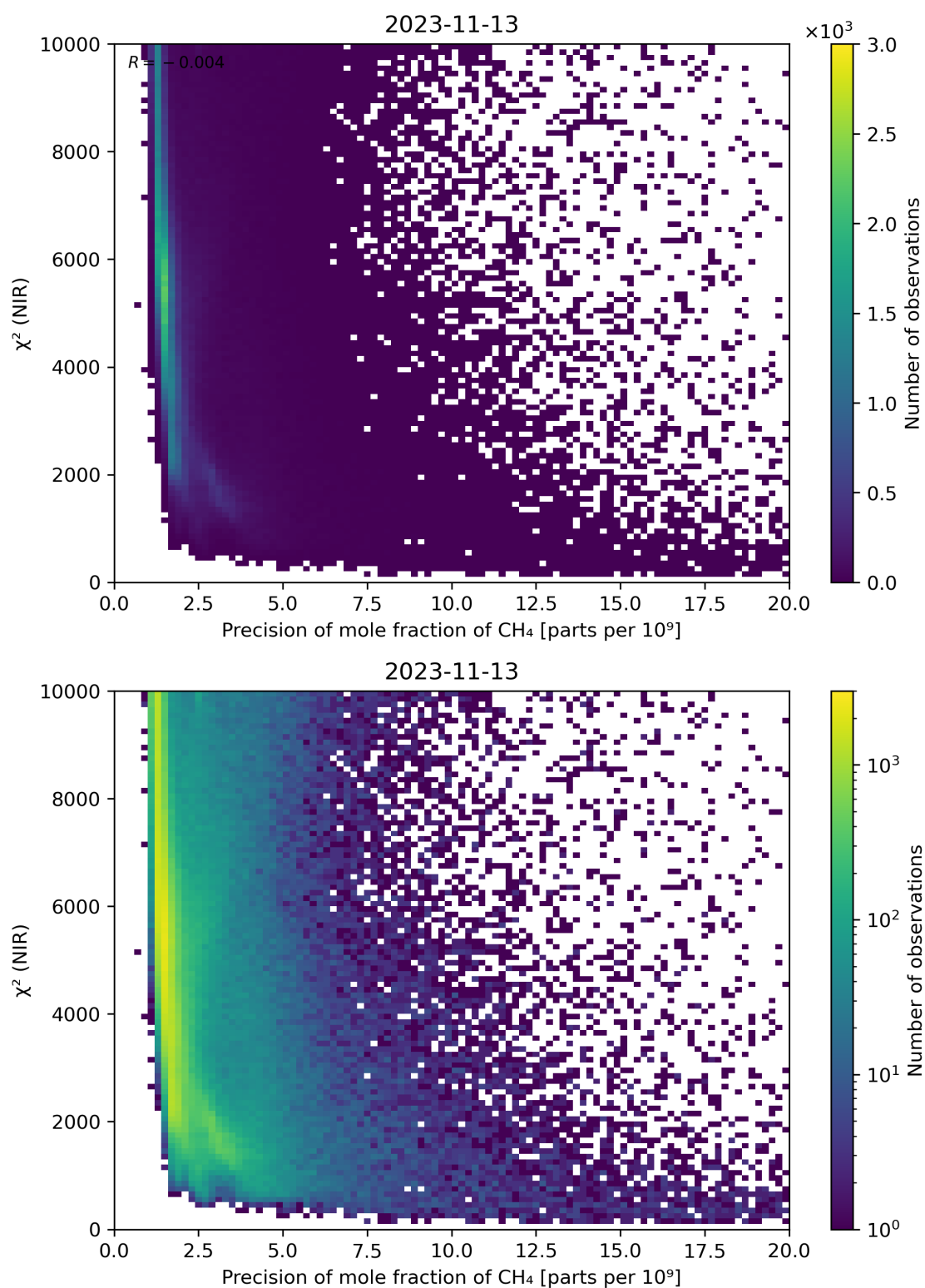
Figure 78: Scatter density plot of “Precision of mole fraction of \text{CH}_4 ” against “ \chi^2 (NIR)” for 2023-11-13 to 2023-11-14.
