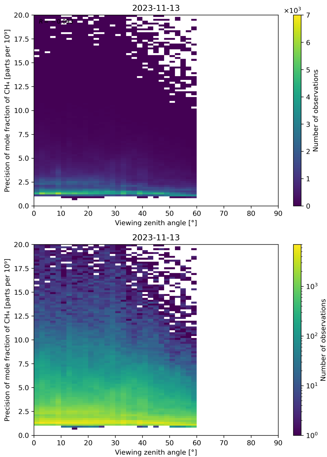
Figure 112: Scatter density plot of “Viewing zenith angle” against “Precision of mole fraction of CH 4 ” for 2023-11-13 to 2023-11-14.
