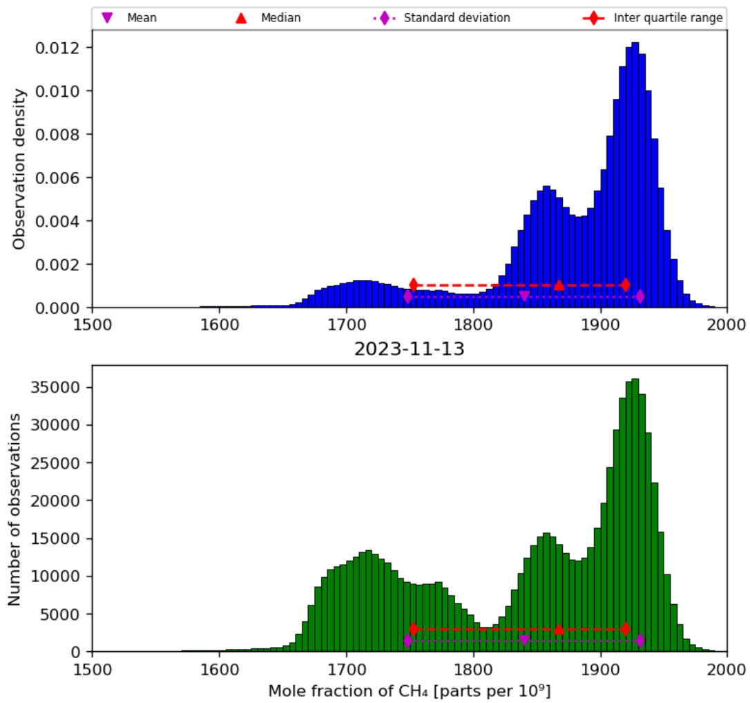
Figure 23: Histogram of “Mole fraction of CH 4 ” for 2023-11-13 to 2023-11-14
