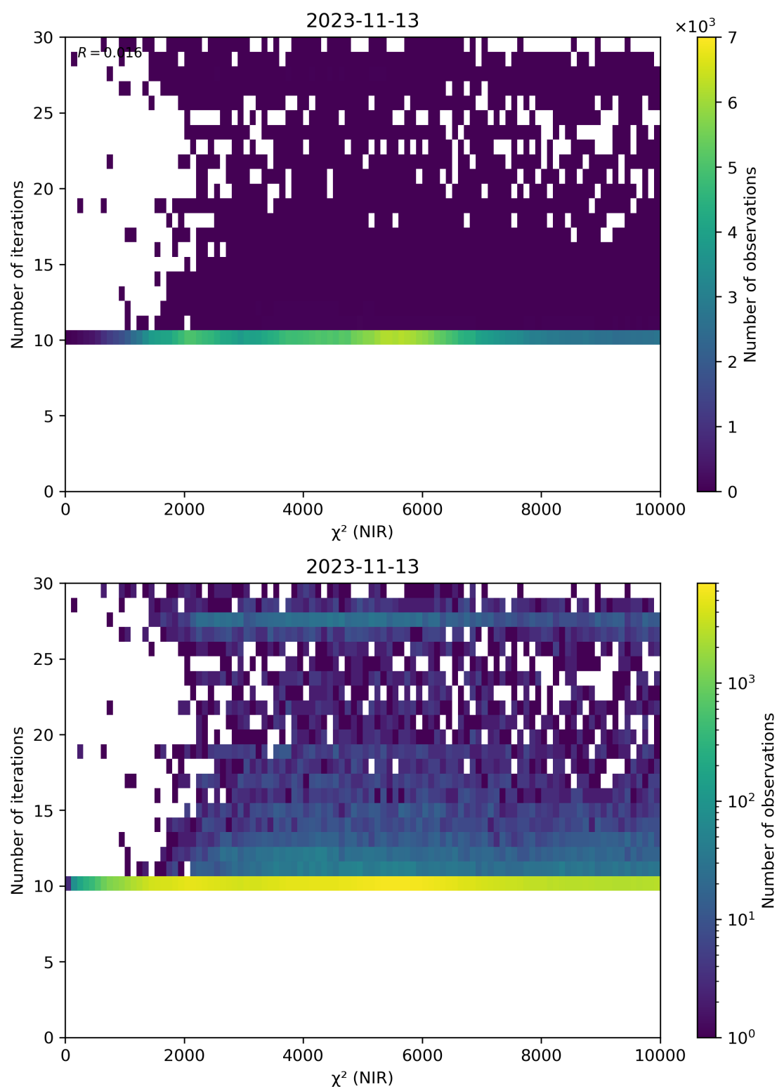
Figure 46: Scatter density plot of “ \chi^2 (NIR)” against “Number of iterations” for 2023-11-13 to 2023-11-14.
