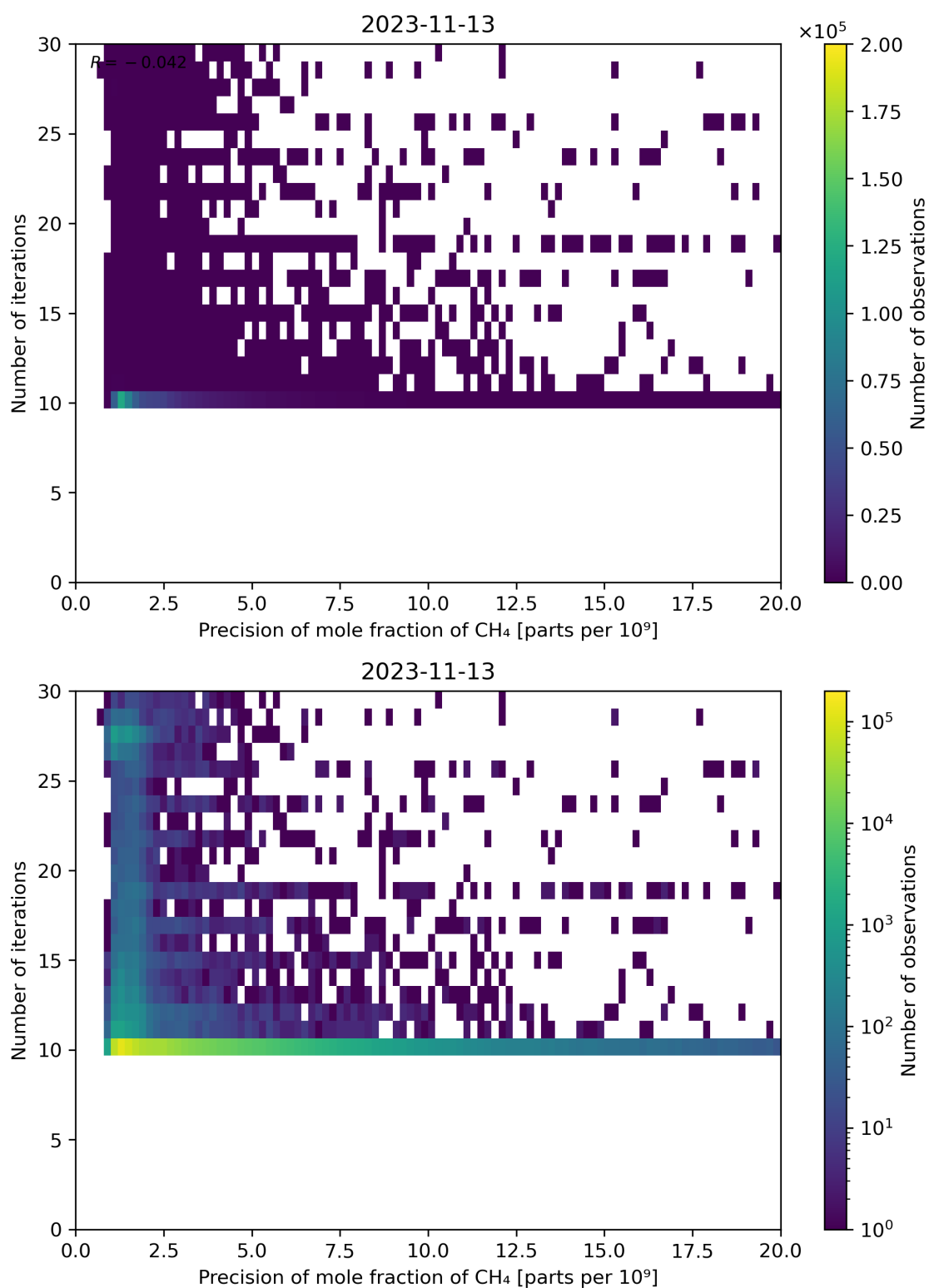
Figure 83: Scatter density plot of “Precision of mole fraction of CH 4 ” against “Number of iterations” for 2023-11-13 to 2023-11-14.
