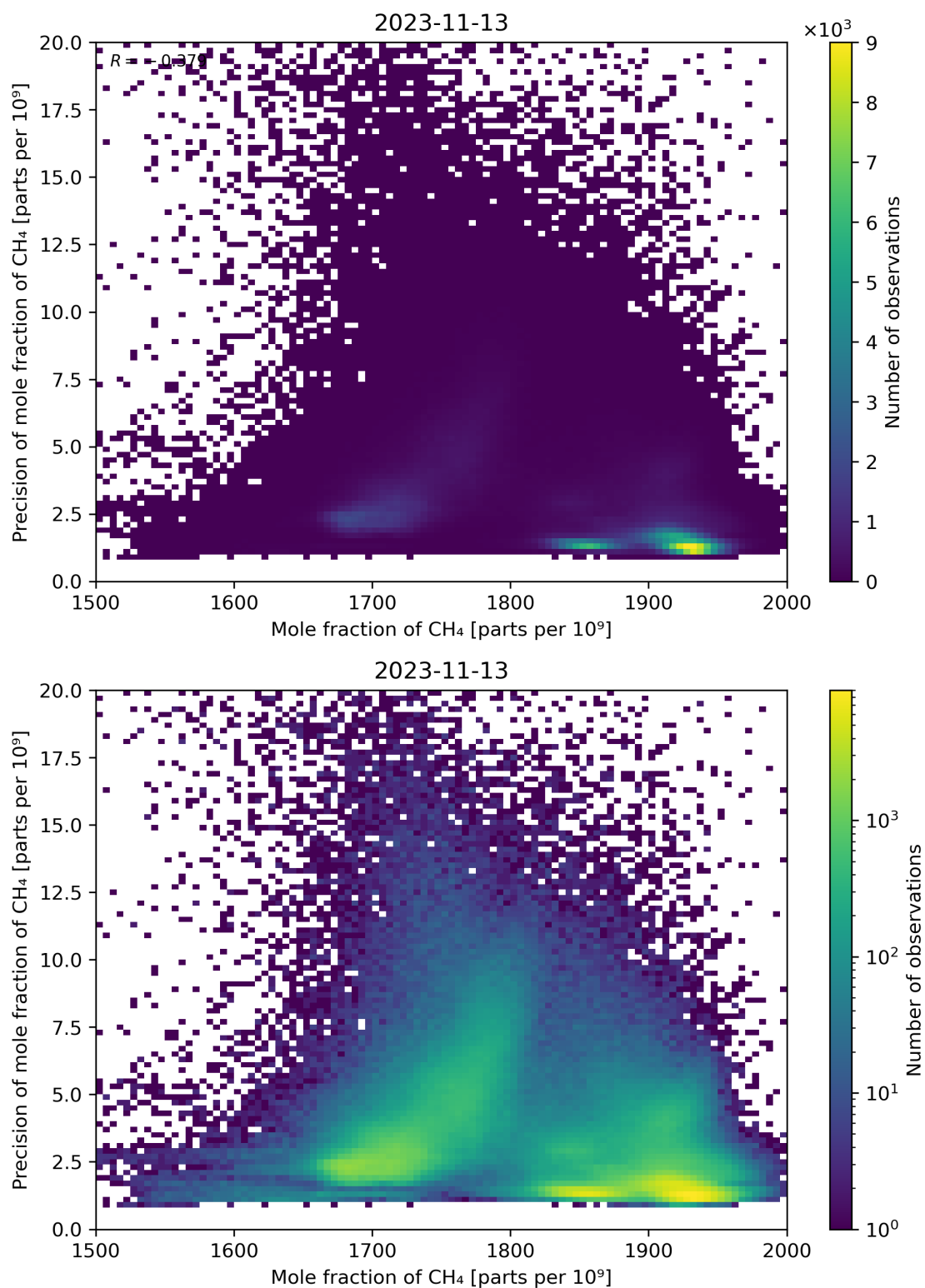
Figure 75: Scatter density plot of “Mole fraction of CH 4 ” against “Precision of mole fraction of CH 4 ” for 2023-11-13 to 2023-11-14.
