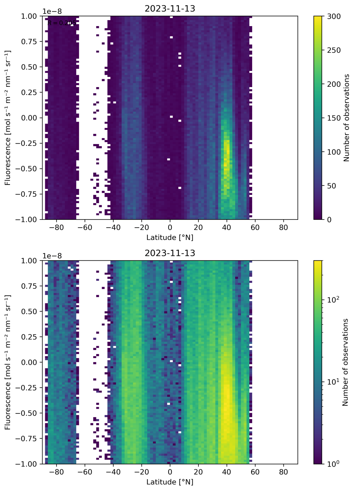
Figure 56: Scatter density plot of “Latitude” against “Fluorescence” for 2023-11-13 to 2023-11-14.
