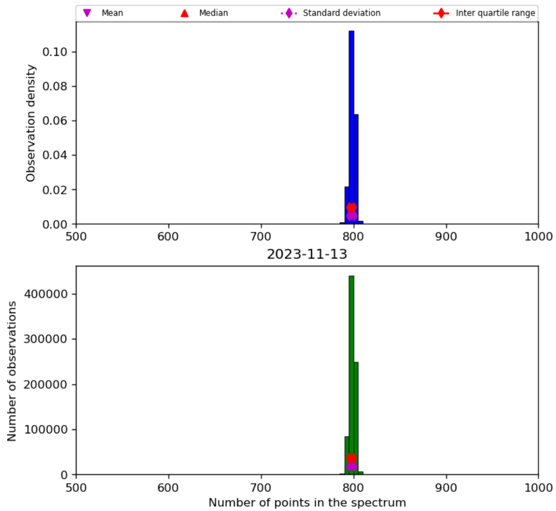
Figure 26: Histogram of “Number of points in the spectrum” for 2023-11-13 to 2023-11-14
