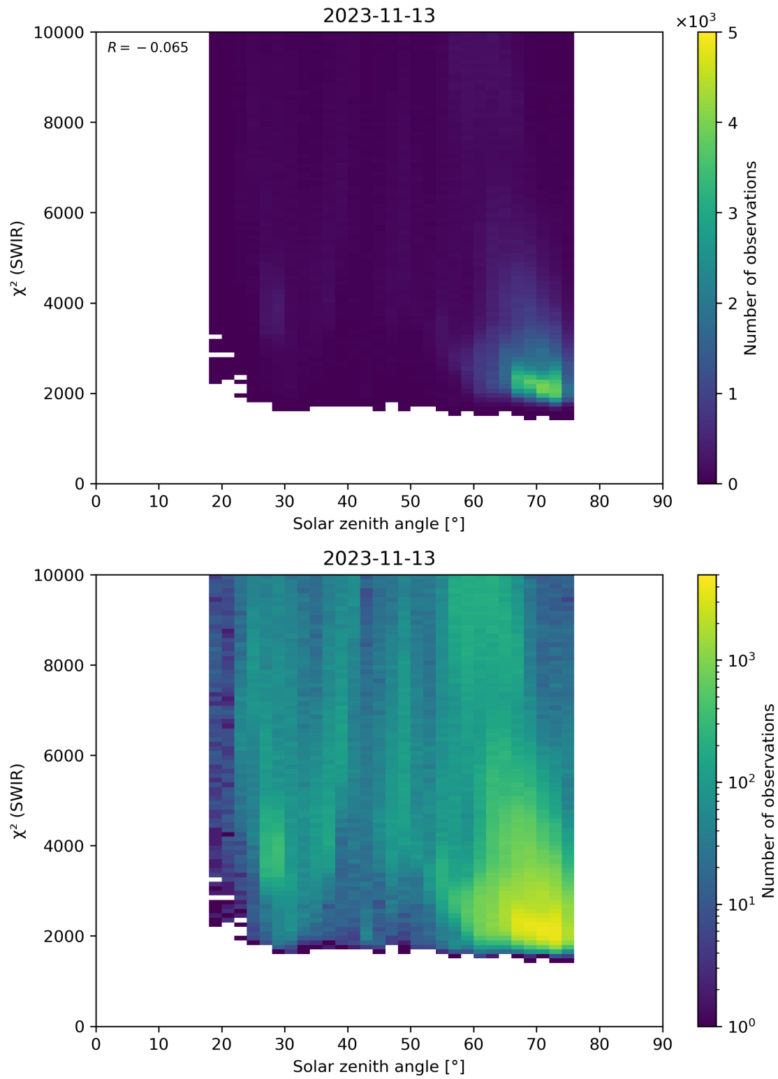
Figure 95: Scatter density plot of “Solar zenith angle” against “ \chi^2 (SWIR)” for 2023-11-13 to 2023-11-14.
