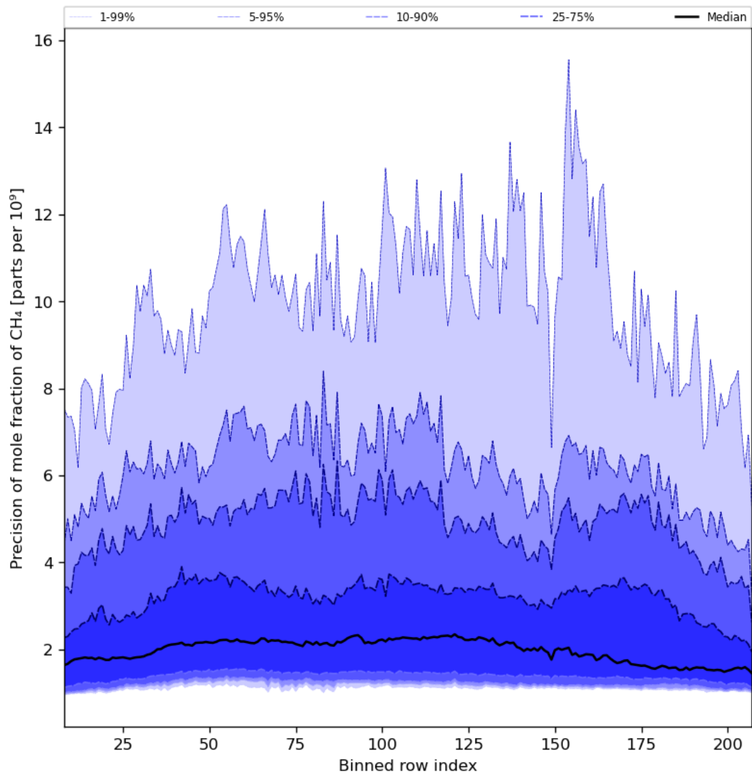
Figure 35: Along track statistics of “Precision of mole fraction of CH 4 ” for 2023-11-13 to 2023-11-14
