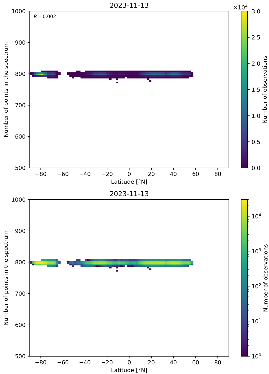
Figure 61: Scatter density plot of “Latitude” against “Number of points in the spectrum” for 2023-11-13 to 2023-11-14.
