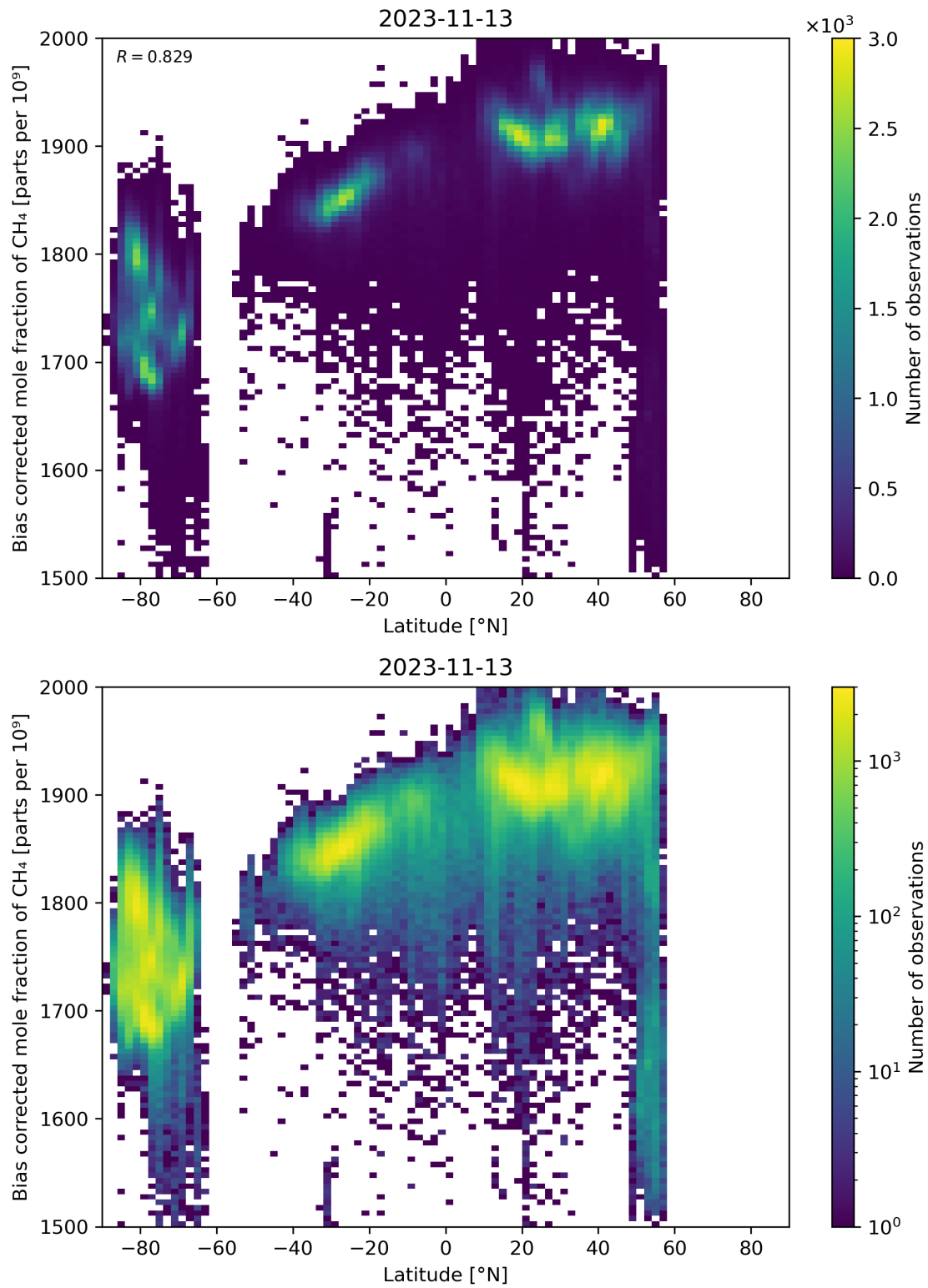
Figure 58: Scatter density plot of “Latitude” against “Bias corrected mole fraction of CH 4 ” for 2023-11-13 to 2023-11-14.
