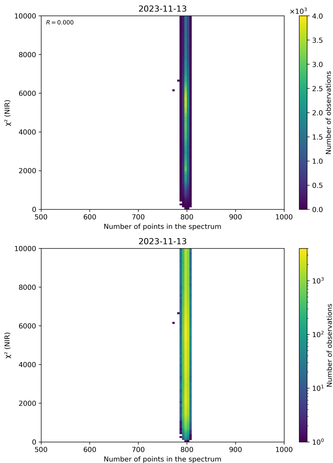
Figure 88: Scatter density plot of “Number of points in the spectrum” against “ \chi^2 (NIR)” for 2023-11-13 to 2023-11-14.
