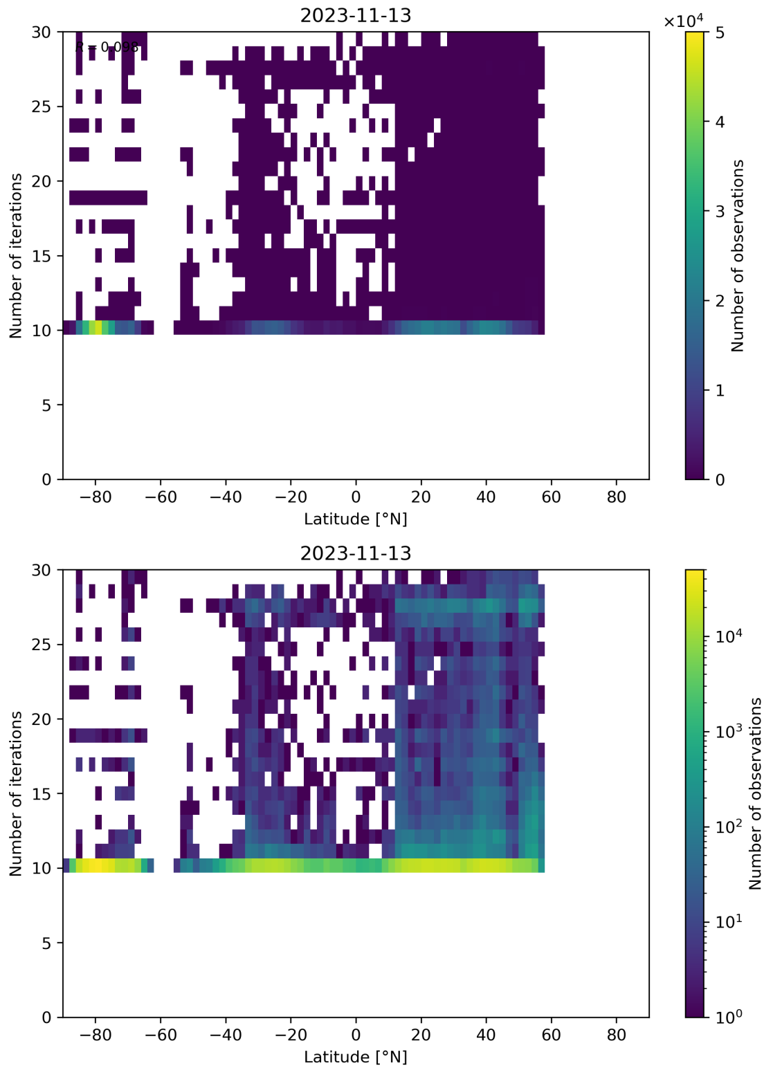
Figure 60: Scatter density plot of “Latitude” against “Number of iterations” for 2023-11-13 to 2023-11-14.
