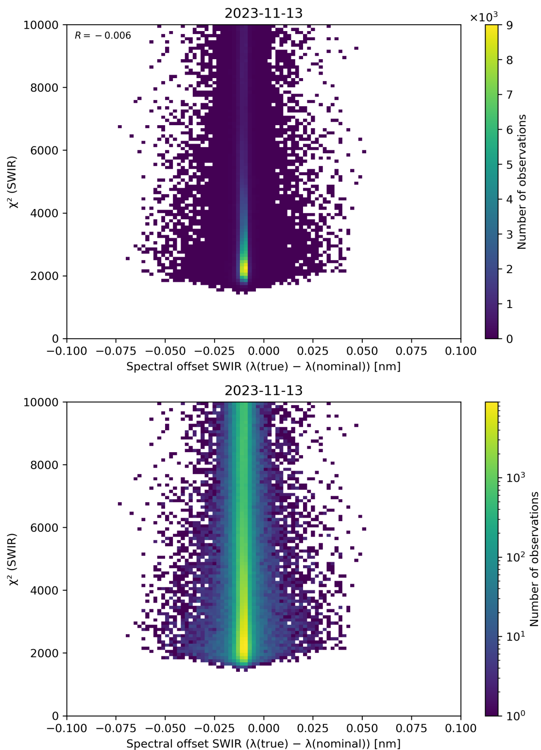
Figure 118: Scatter density plot of “Spectral offset SWIR ( \lambda(\text{true}) - \lambda(\text{nominal}) )” against “ \chi^2 (SWIR)” for 2023-11-13 to 2023-11-14.
