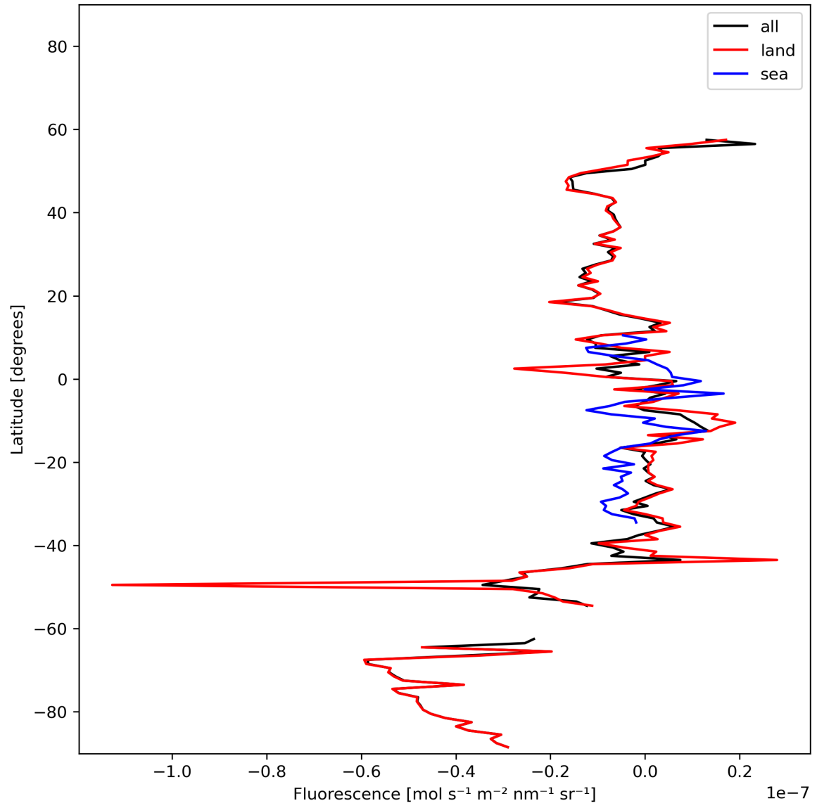
Figure 21: Zonal average of “Fluorescence” for 2023-11-13 to 2023-11-14.
