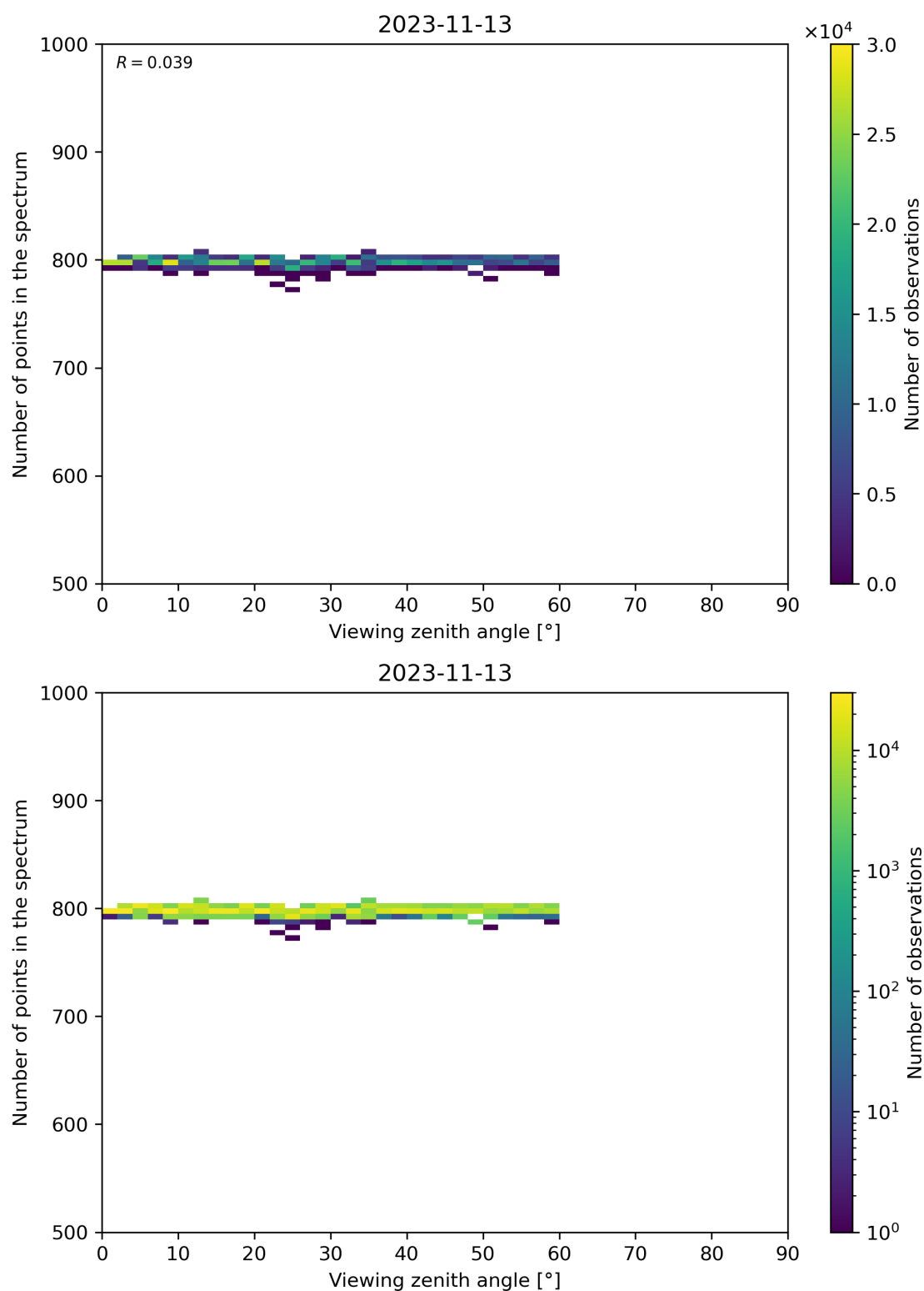
Figure 114: Scatter density plot of “Viewing zenith angle” against “Number of points in the spectrum” for 2023-11-13 to 2023-11-14.
