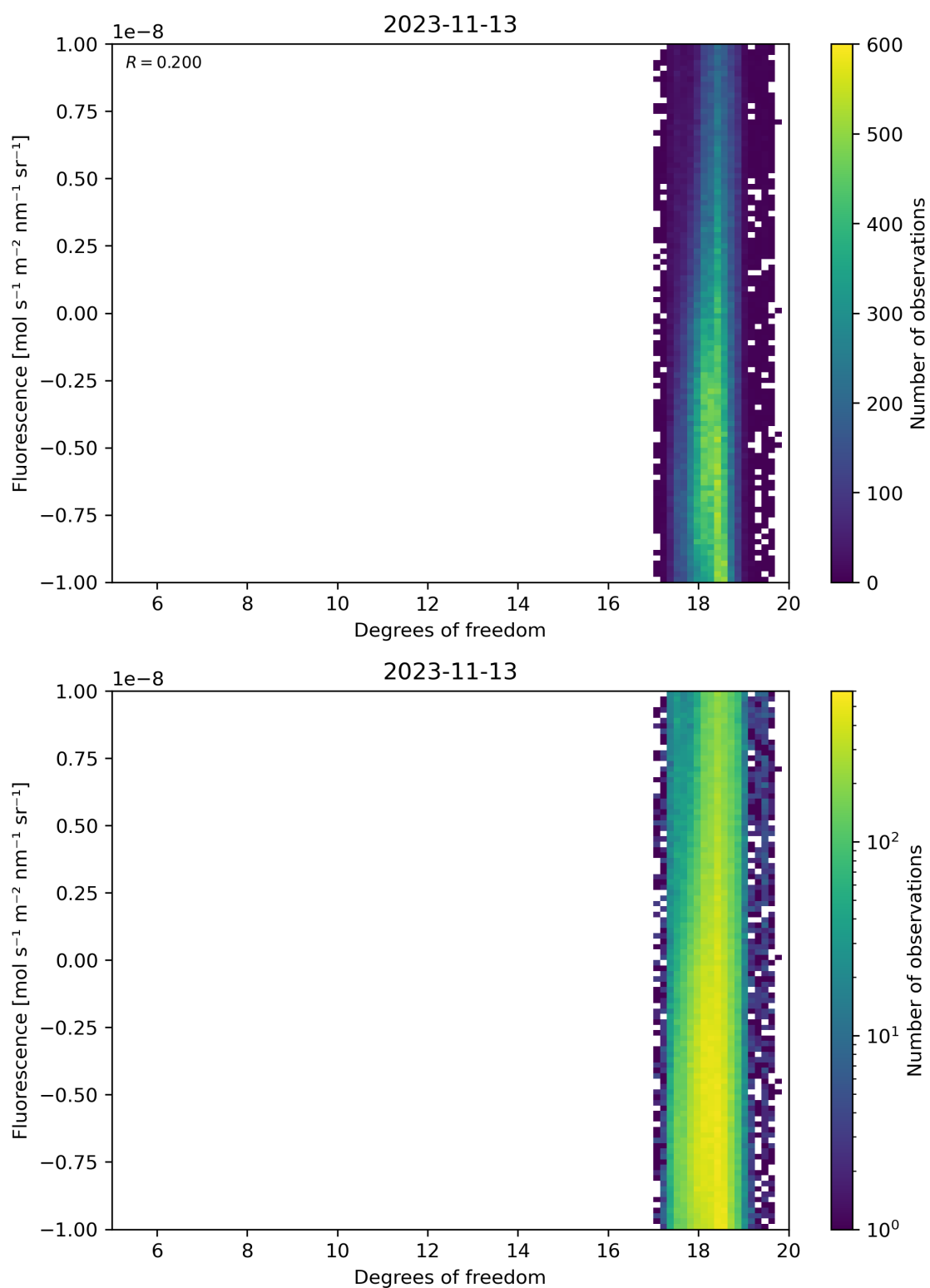
Figure 51: Scatter density plot of “Degrees of freedom” against “Fluorescence” for 2023-11-13 to 2023-11-14.
