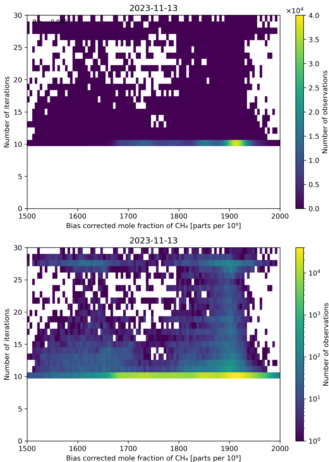
Figure 67: Scatter density plot of “Bias corrected mole fraction of CH 4 ” against “Number of iterations” for 2023-11-13 to 2023-11-14.
