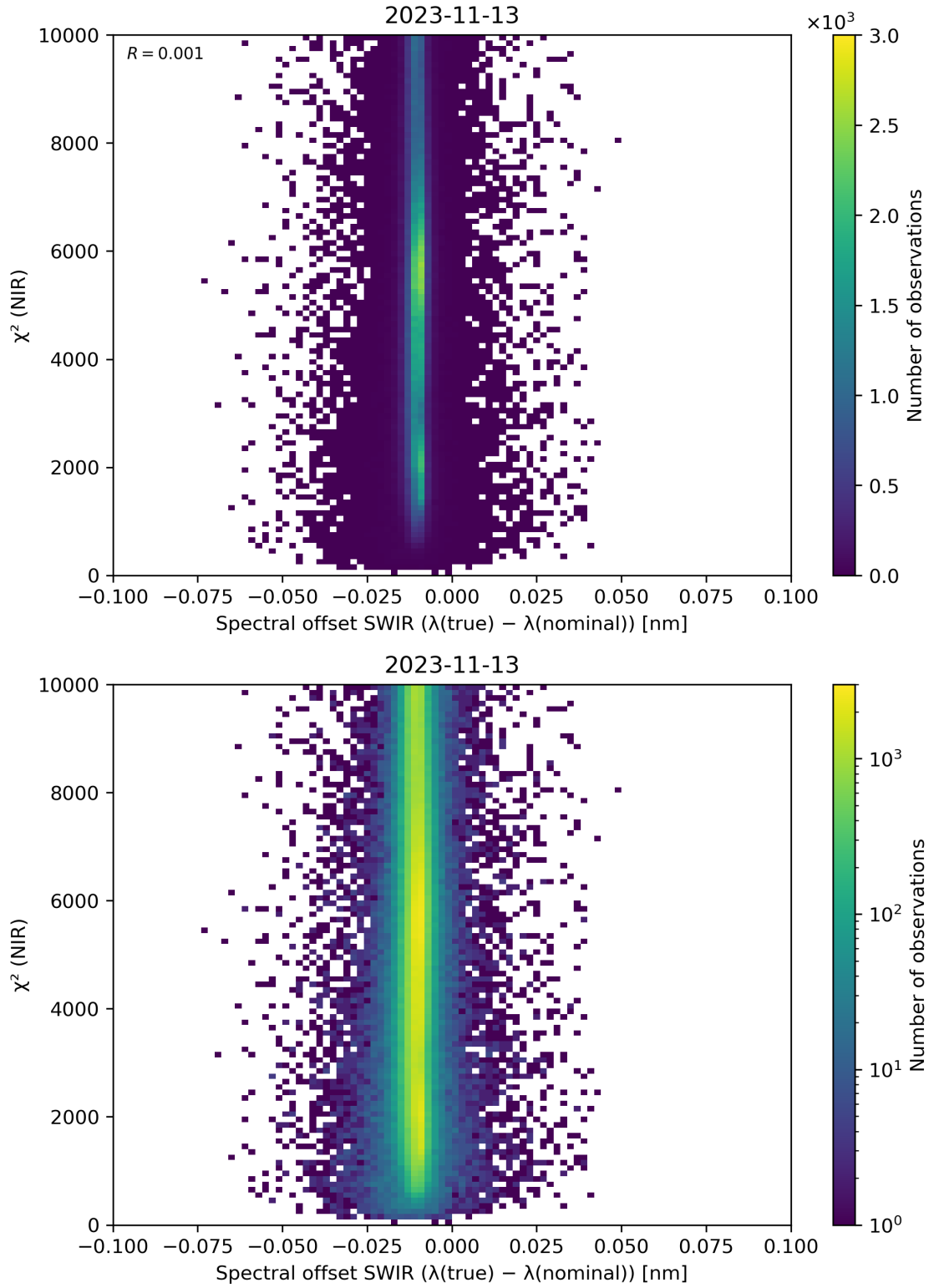
Figure 117: Scatter density plot of “Spectral offset SWIR ( \lambda(\text{true}) - \lambda(\text{nominal}) )” against “ \chi^2 (NIR)” for 2023-11-13 to 2023-11-14.
