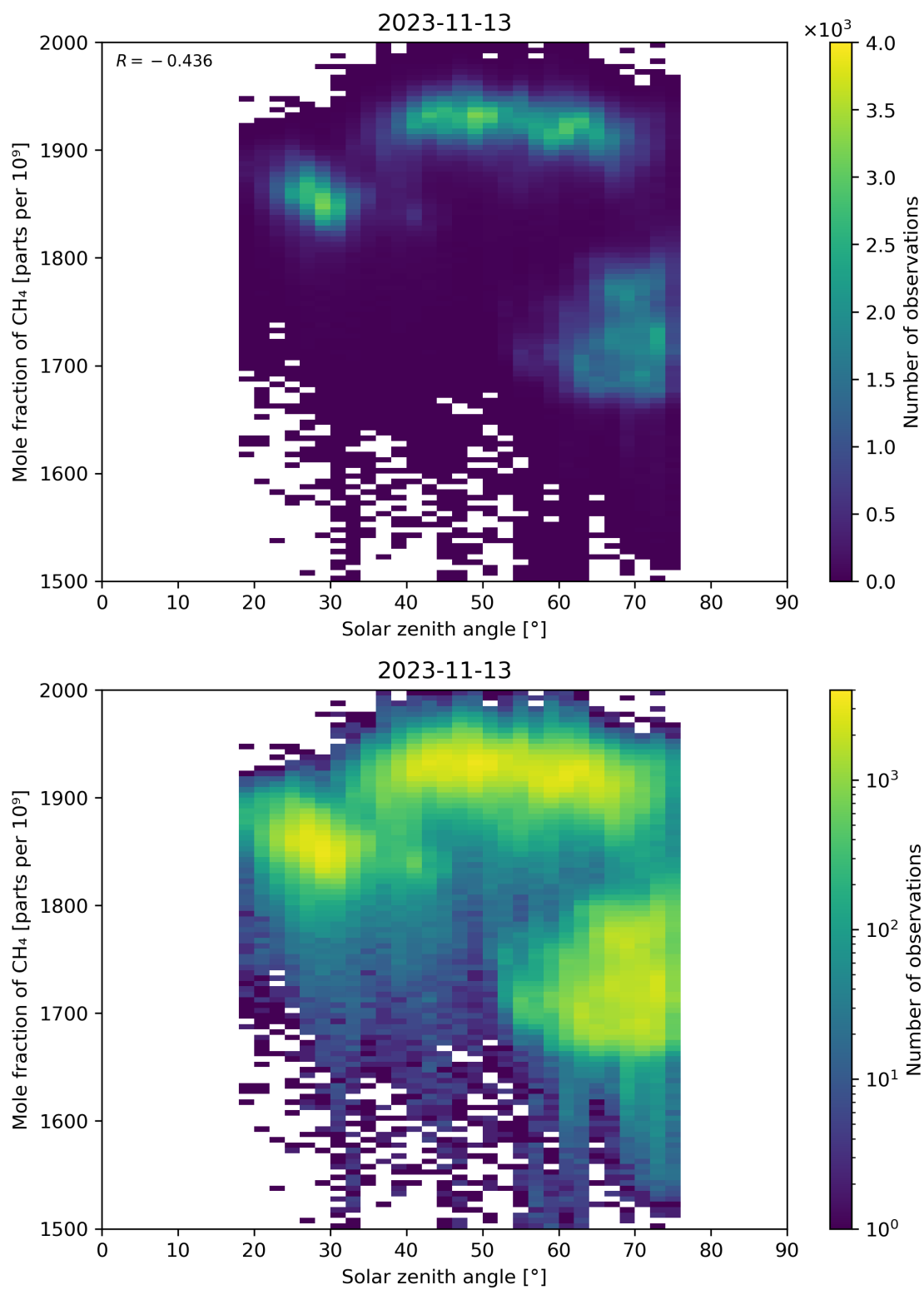
Figure 99: Scatter density plot of “Solar zenith angle” against “Mole fraction of CH 4 ” for 2023-11-13 to 2023-11-14.
