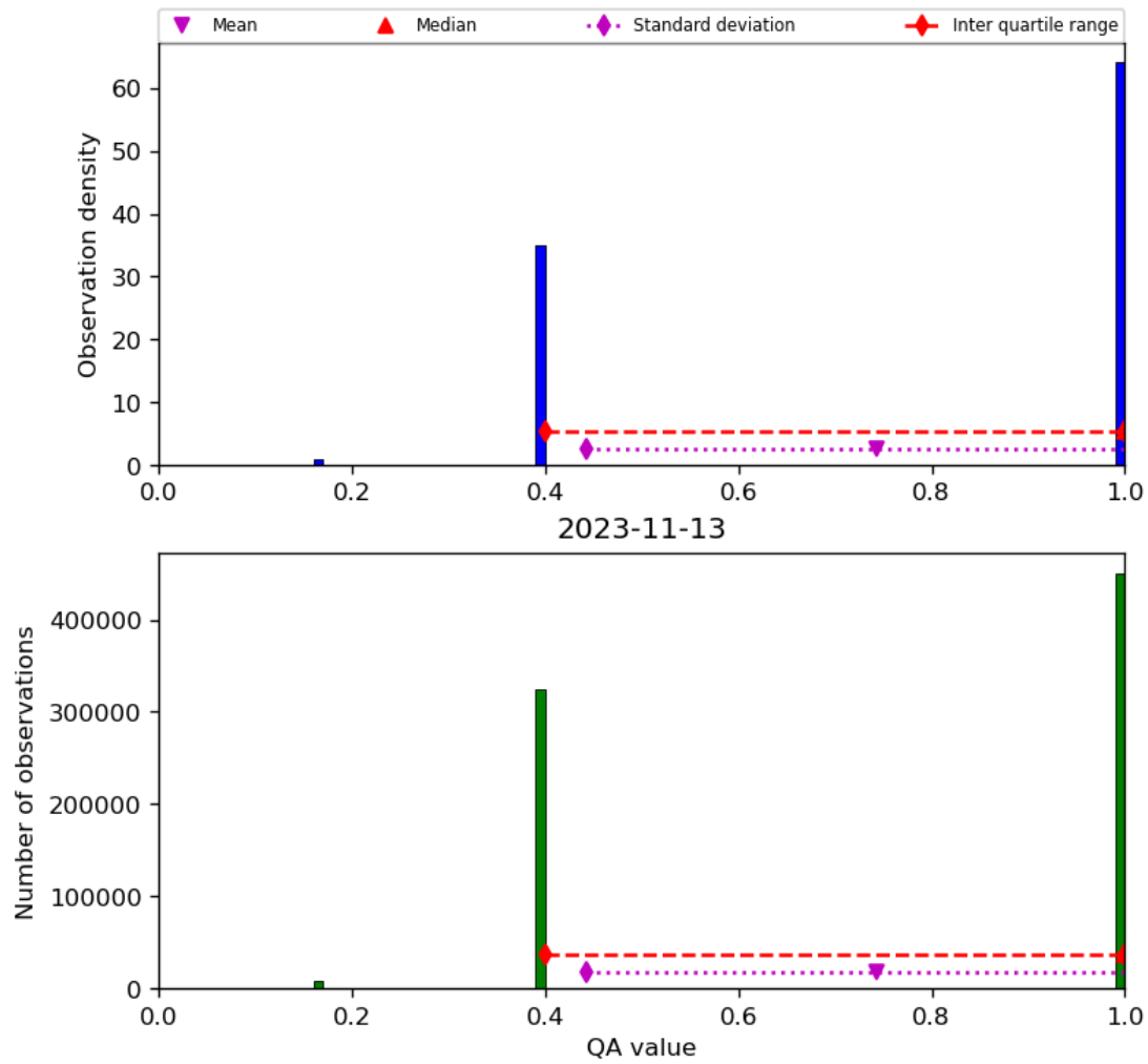
Figure 22: Histogram of “QA value” for 2023-11-13 to 2023-11-14
