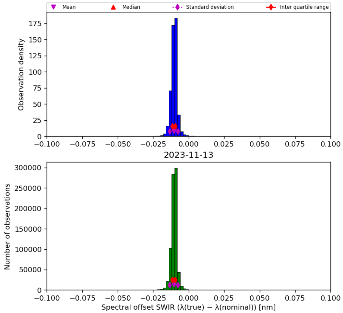
Figure 27: Histogram of “Spectral offset SWIR ( \lambda(\text{true}) - \lambda(\text{nominal}) )” for 2023-11-13 to 2023-11-14
