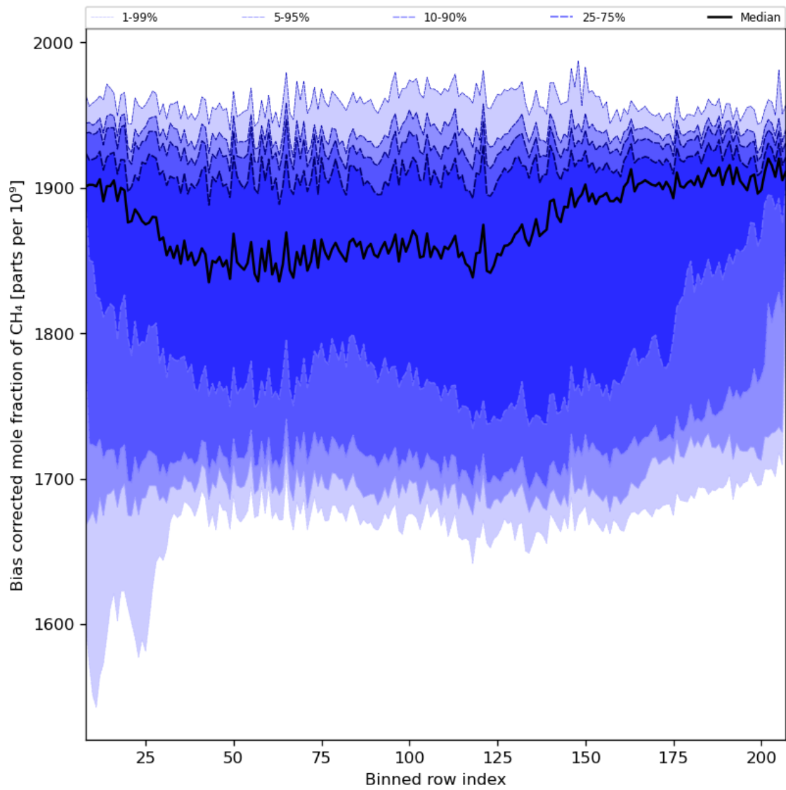
Figure 36: Along track statistics of “Bias corrected mole fraction of CH 4 ” for 2023-11-13 to 2023-11-14
