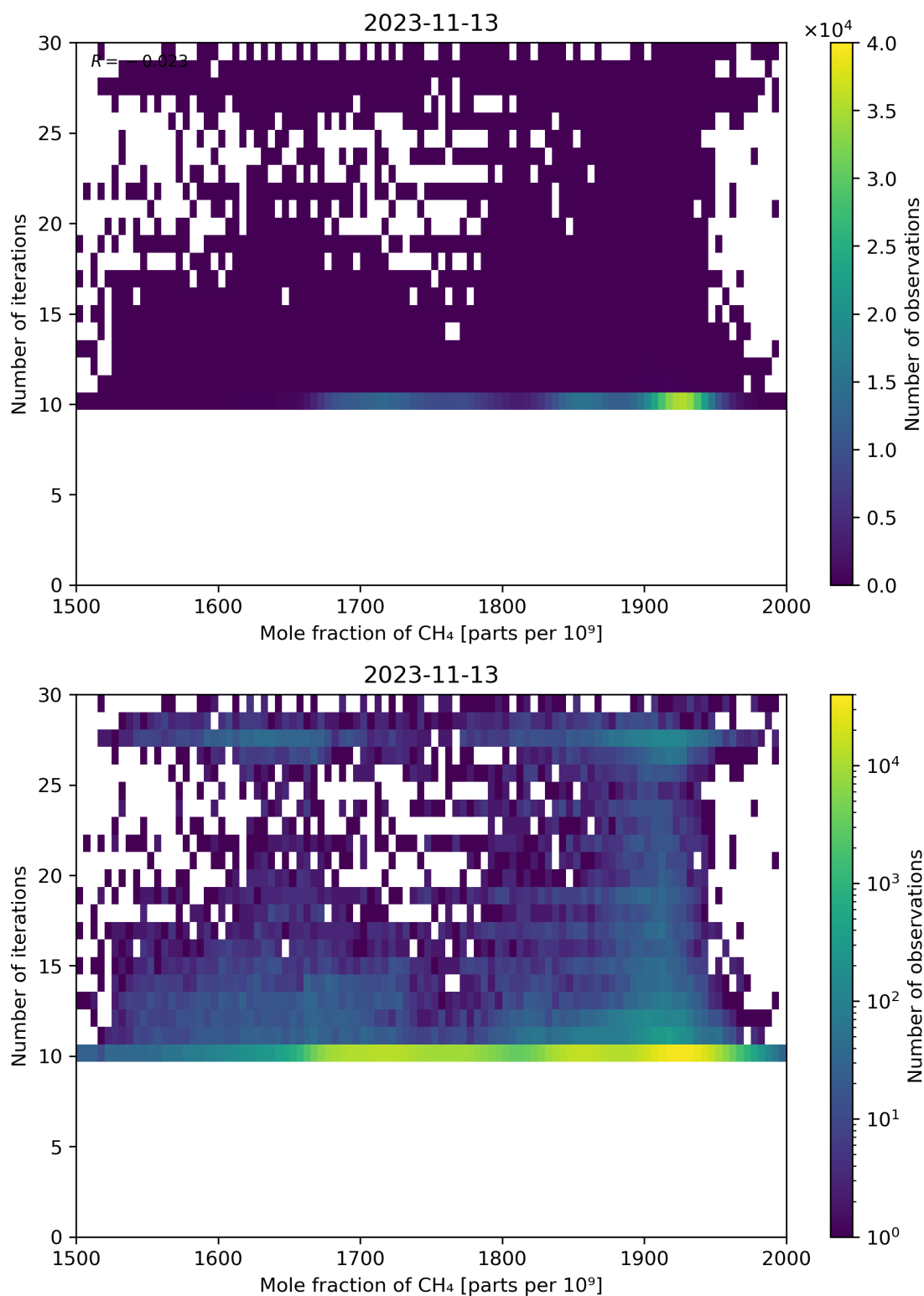
Figure 76: Scatter density plot of “Mole fraction of CH 4 ” against “Number of iterations” for 2023-11-13 to 2023-11-14.
