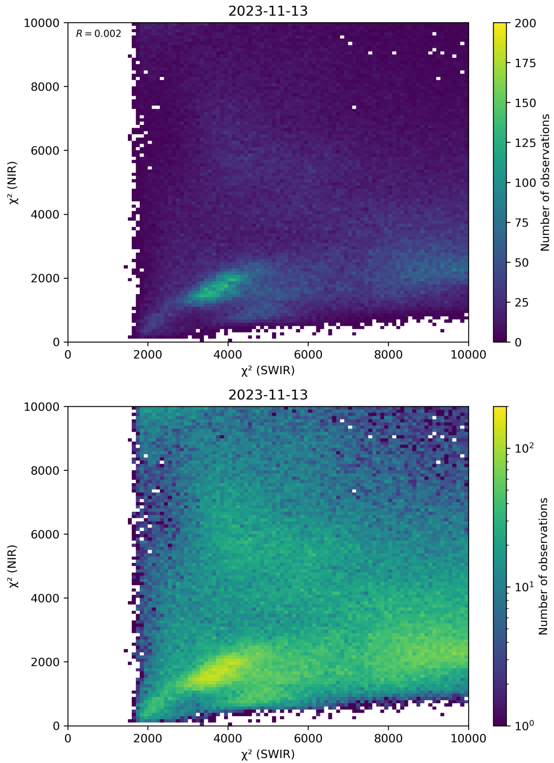
Figure 47: Scatter density plot of “ \chi^2 (SWIR)” against “ \chi^2 (NIR)” for 2023-11-13 to 2023-11-14.
