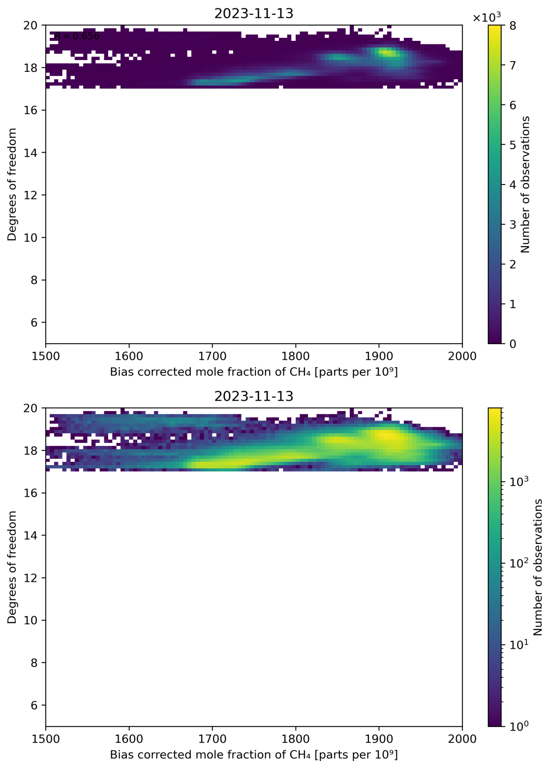
Figure 65: Scatter density plot of “Bias corrected mole fraction of CH 4 ” against “Degrees of freedom” for 2023-11-13 to 2023-11-14.
