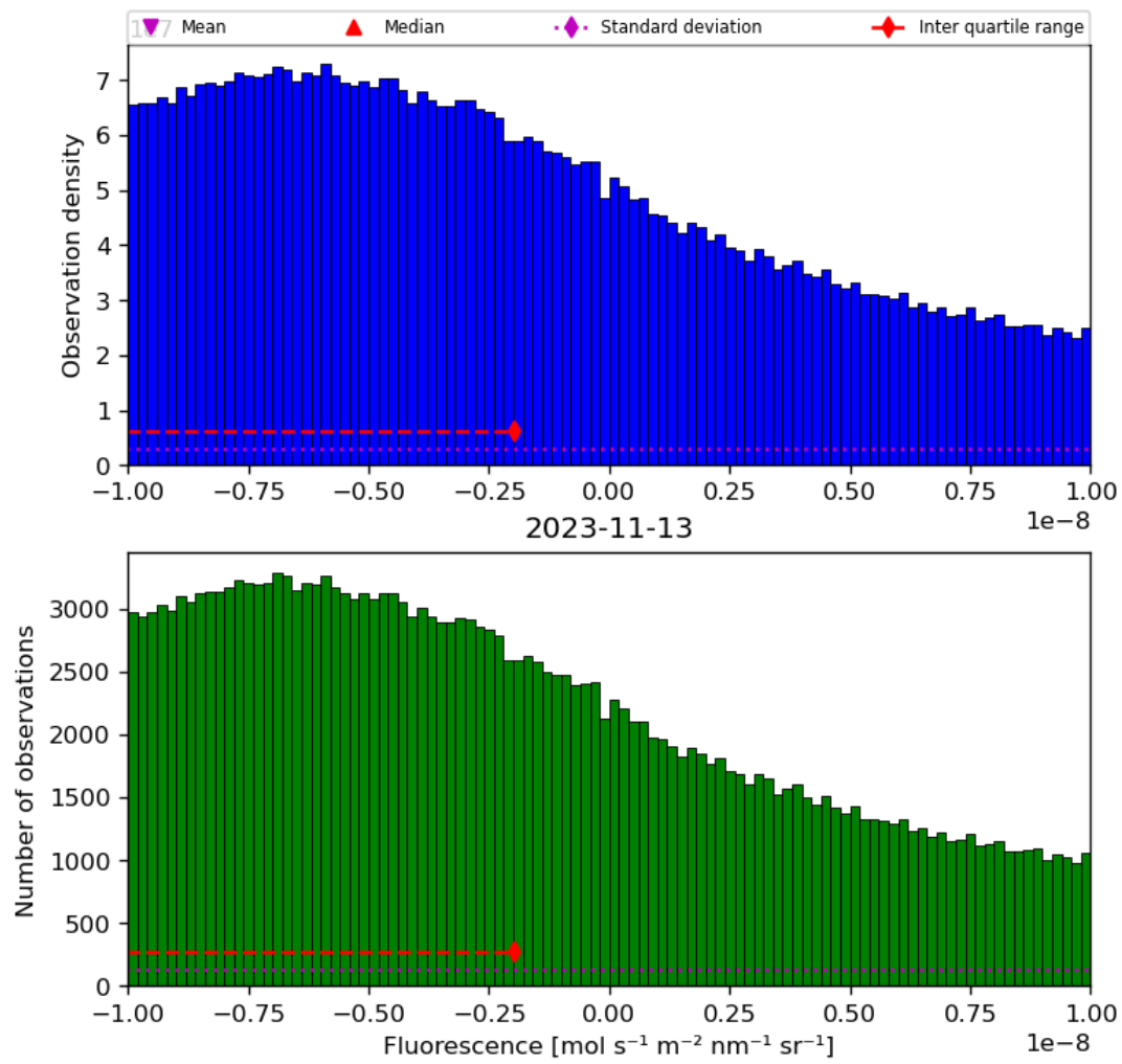
Figure 32: Histogram of “Fluorescence” for 2023-11-13 to 2023-11-14
