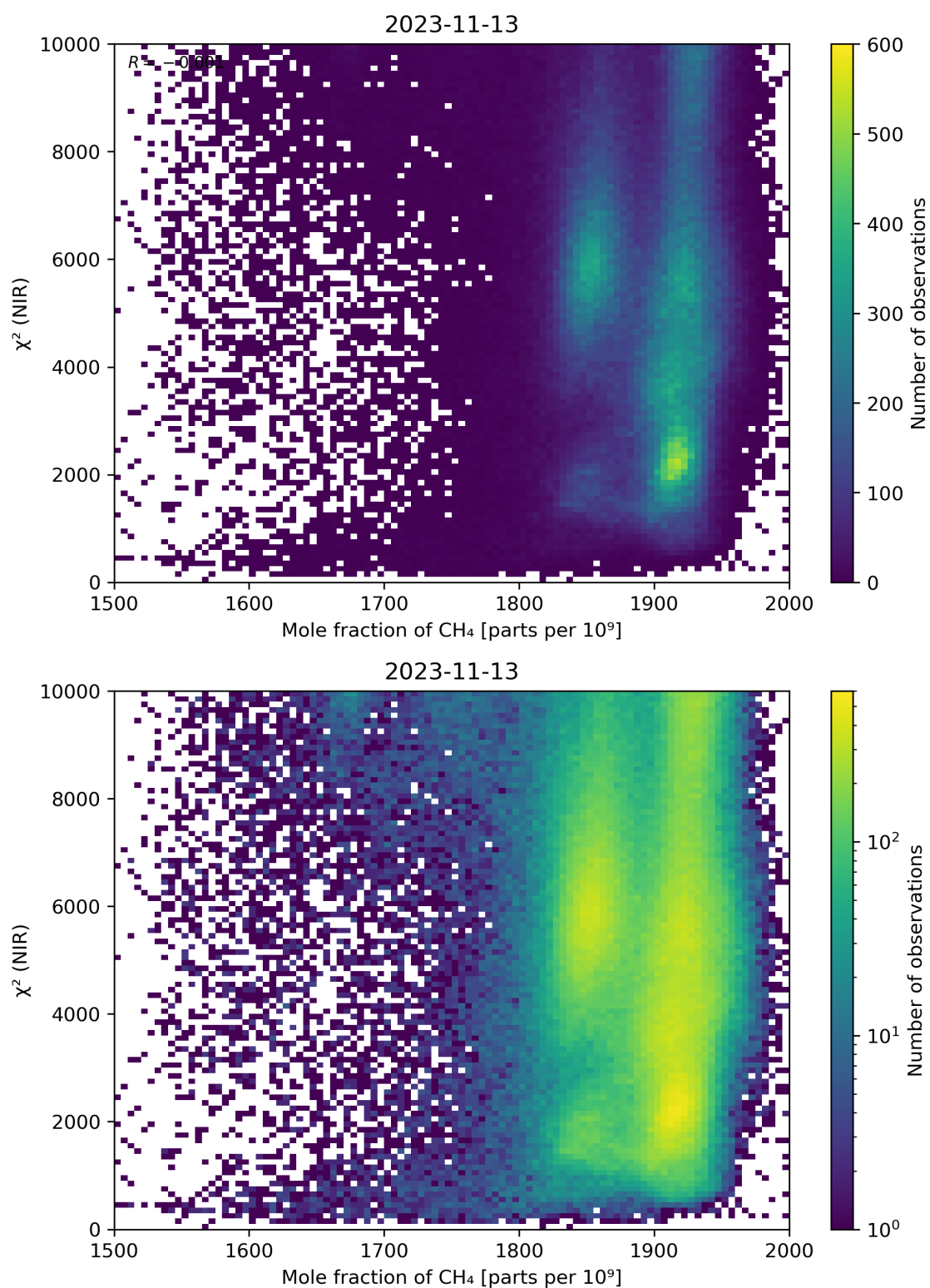
Figure 70: Scatter density plot of “Mole fraction of \text{CH}_4 ” against “ \chi^2 (NIR)” for 2023-11-13 to 2023-11-14.
