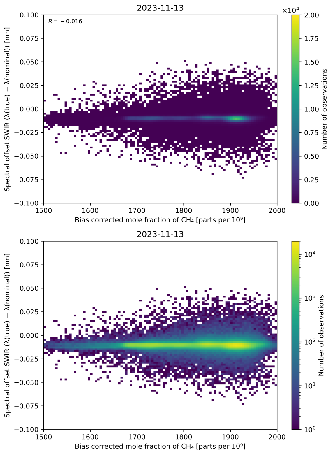
Figure 69: Scatter density plot of “Bias corrected mole fraction of \text{CH}_4 ” against “Spectral offset SWIR ( \lambda(\text{true}) - \lambda(\text{nominal}) )” for 2023-11-13 to 2023-11-14.
