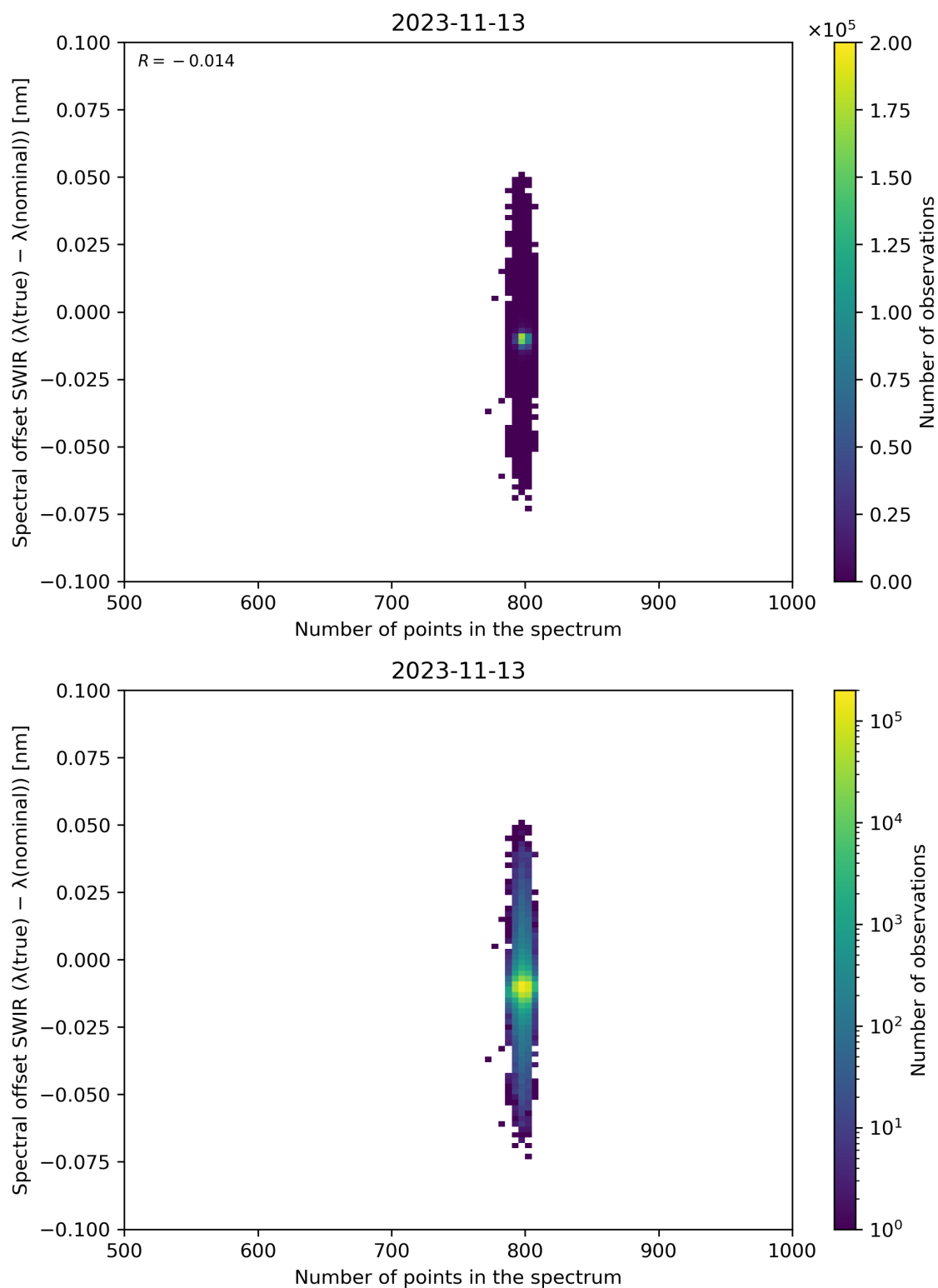
Figure 93: Scatter density plot of “Number of points in the spectrum” against “Spectral offset SWIR ( \lambda(\text{true}) - \lambda(\text{nominal}) )” for 2023-11-13 to 2023-11-14.
