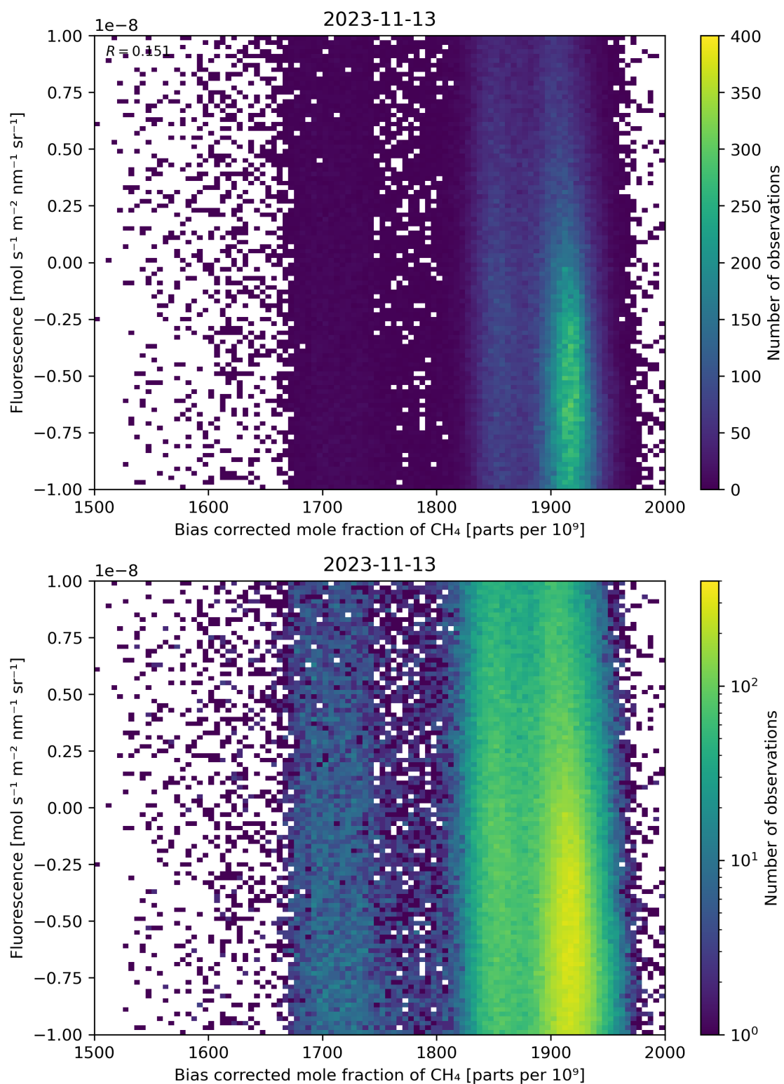
Figure 66: Scatter density plot of “Bias corrected mole fraction of CH 4 ” against “Fluorescence” for 2023-11-13 to 2023-11-14.
