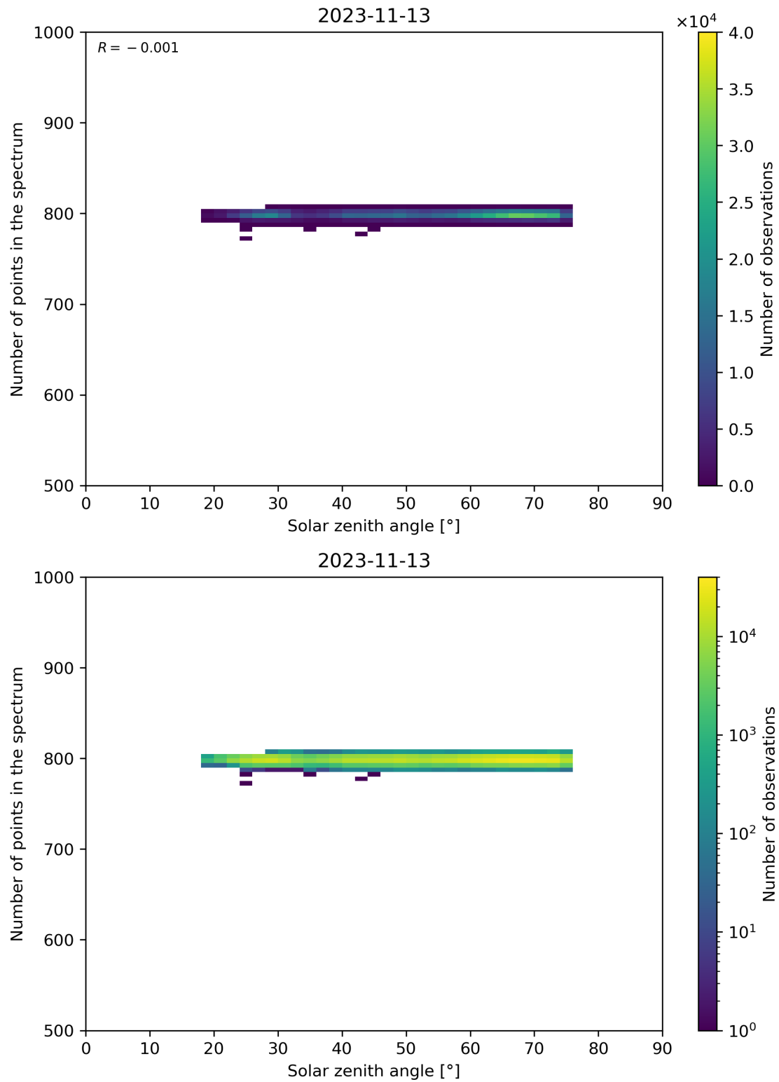
Figure 103: Scatter density plot of “Solar zenith angle” against “Number of points in the spectrum” for 2023-11-13 to 2023-11-14.
