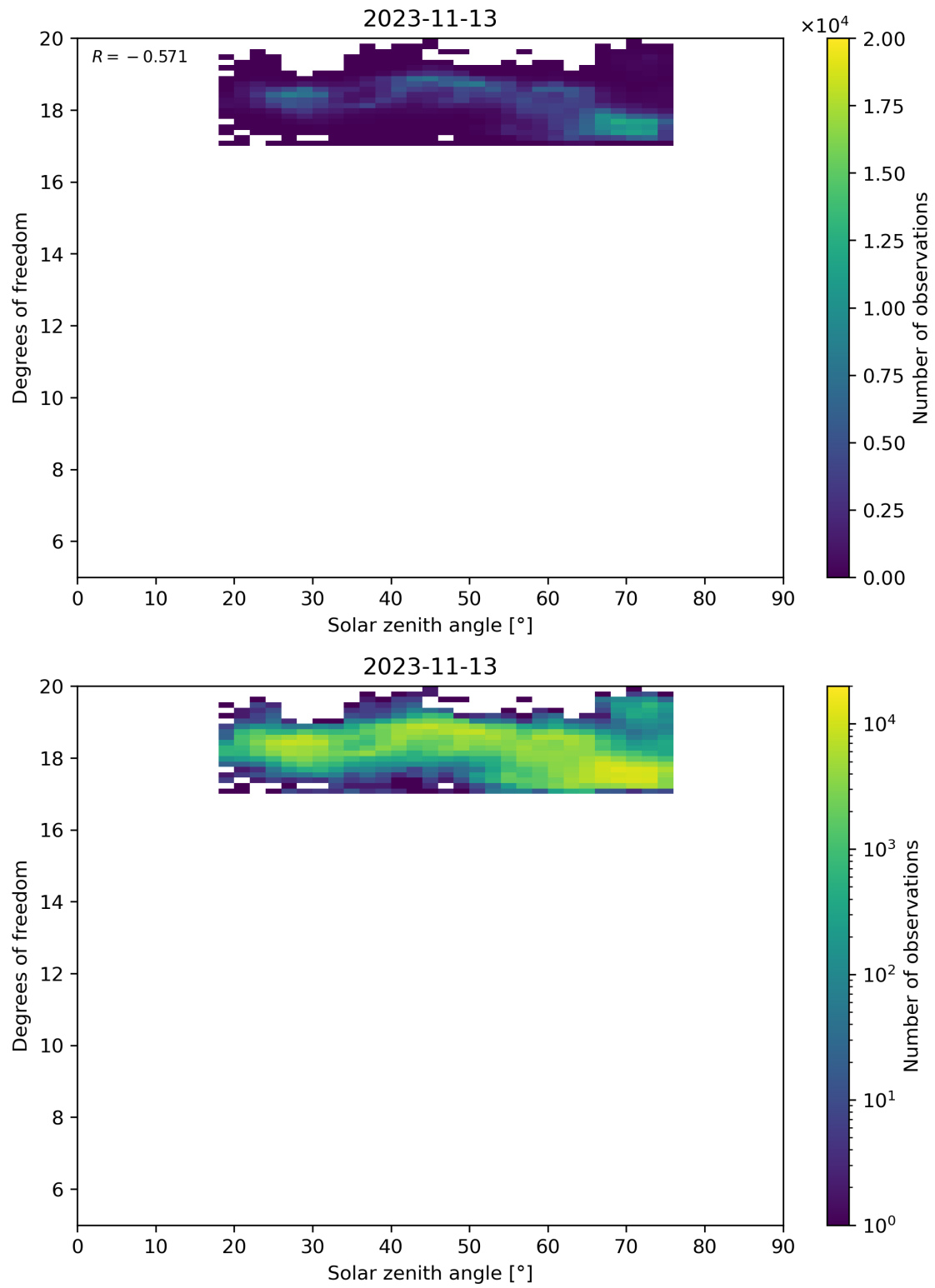
Figure 96: Scatter density plot of “Solar zenith angle” against “Degrees of freedom” for 2023-11-13 to 2023-11-14.
