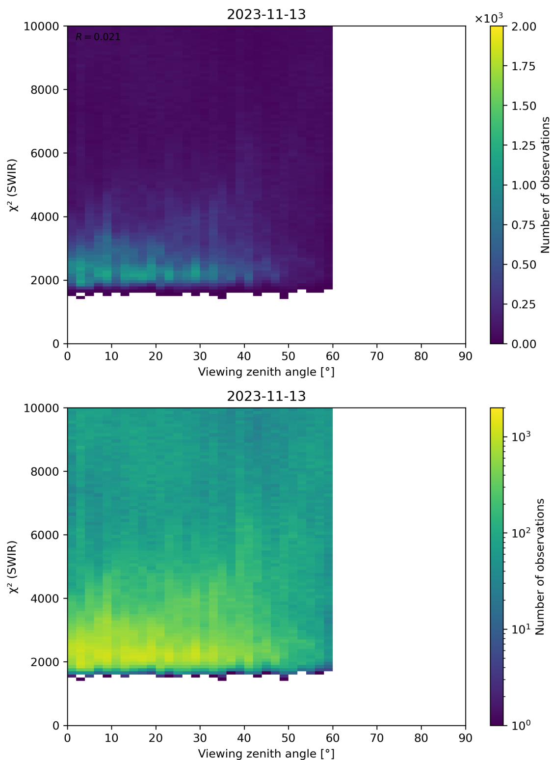
Figure 106: Scatter density plot of “Viewing zenith angle” against “ \chi^2 (SWIR)” for 2023-11-13 to 2023-11-14.
