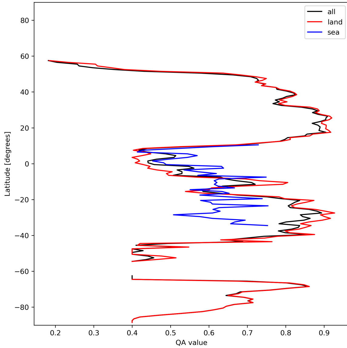
Figure 11: Zonal average of “QA value” for 2023-11-13 to 2023-11-14.
