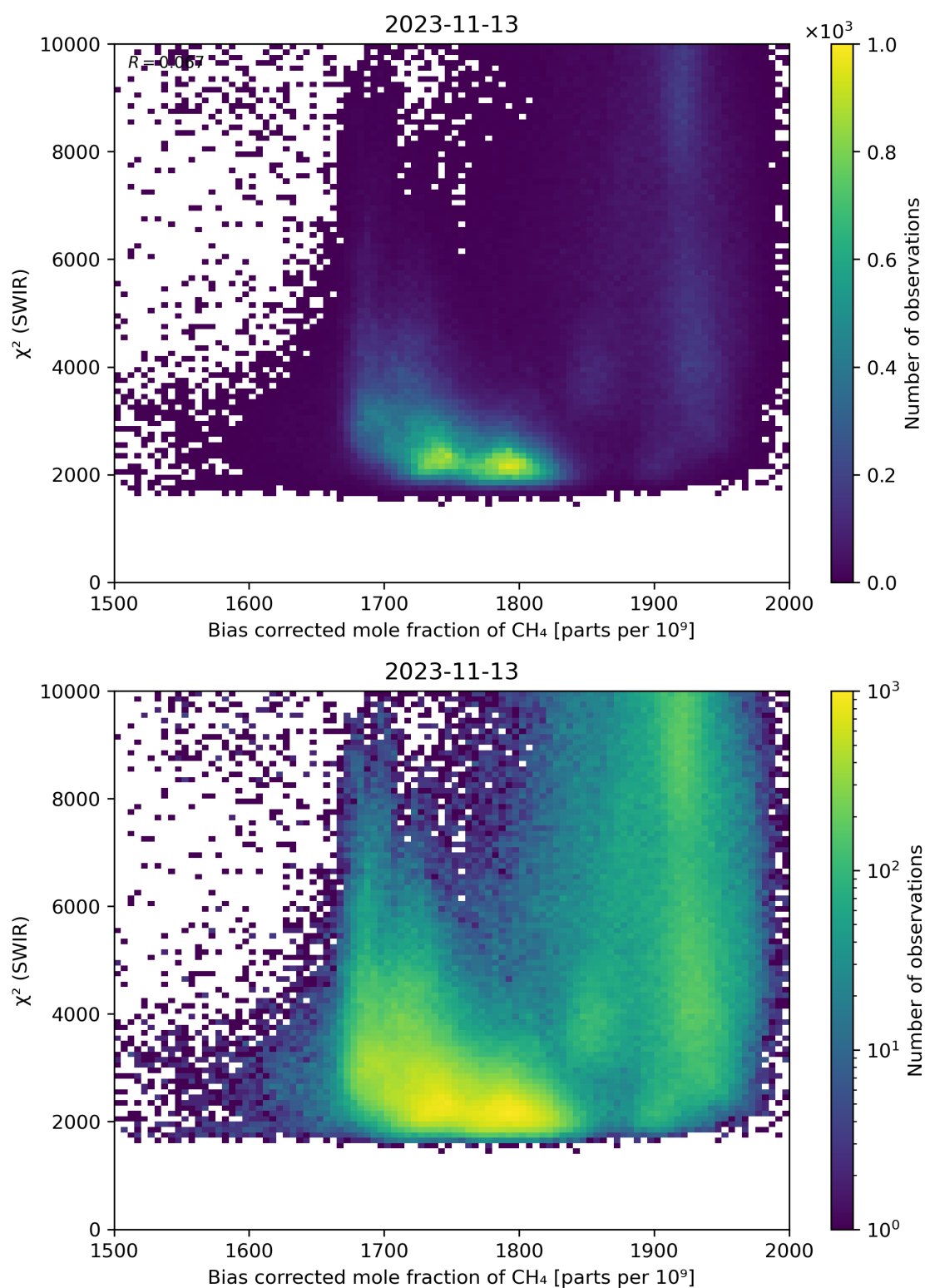
Figure 64: Scatter density plot of “Bias corrected mole fraction of CH 4 ” against “ \chi^2 (SWIR)” for 2023-11-13 to 2023-11-14.
