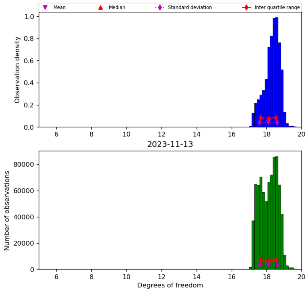
Figure 30: Histogram of “Degrees of freedom” for 2023-11-13 to 2023-11-14
