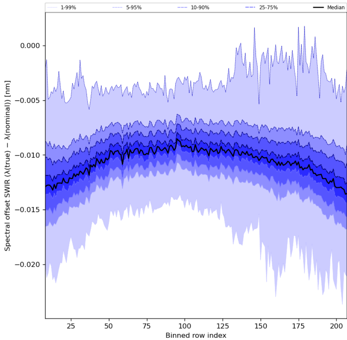
Figure 38: Along track statistics of “Spectral offset SWIR ( \lambda(\text{true}) - \lambda(\text{nominal}) )” for 2023-11-13 to 2023-11-14
