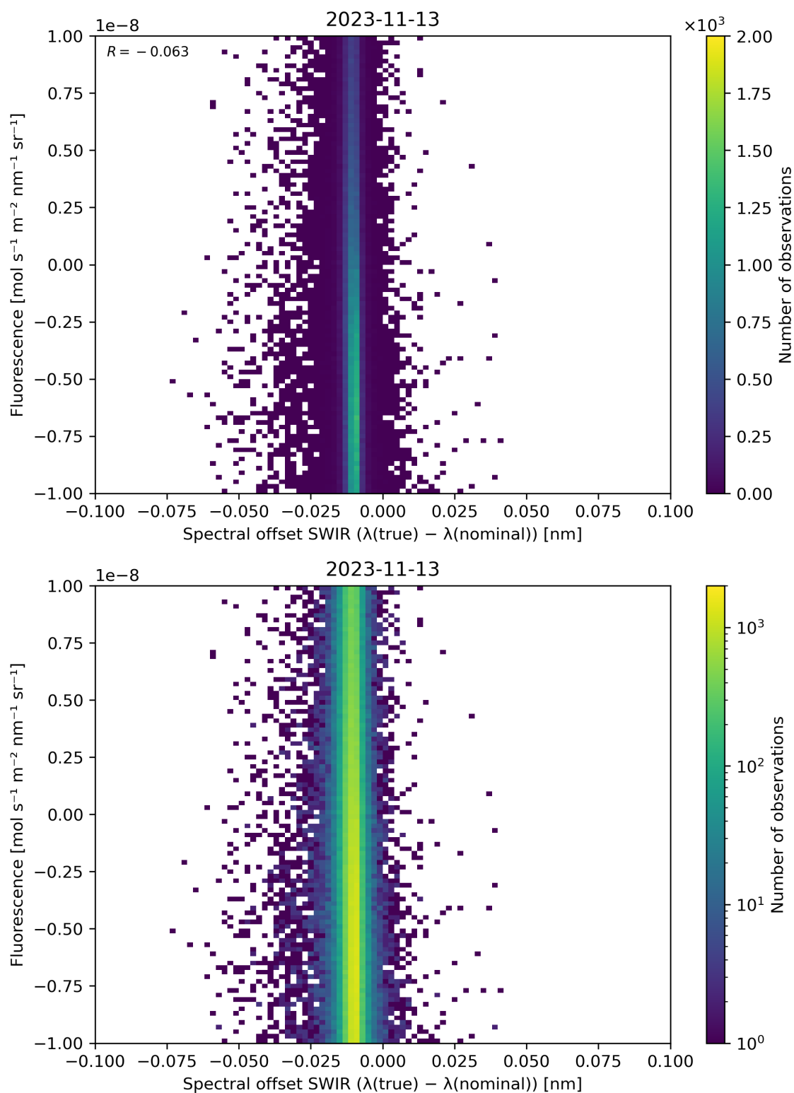
Figure 120: Scatter density plot of “Spectral offset SWIR ( \lambda(\text{true}) - \lambda(\text{nominal}) )” against “Fluorescence” for 2023-11-13 to 2023-11-14.
