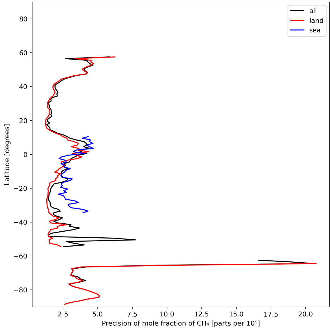
Figure 13: Zonal average of “Precision of mole fraction of CH 4 ” for 2023-11-13 to 2023-11-14.
