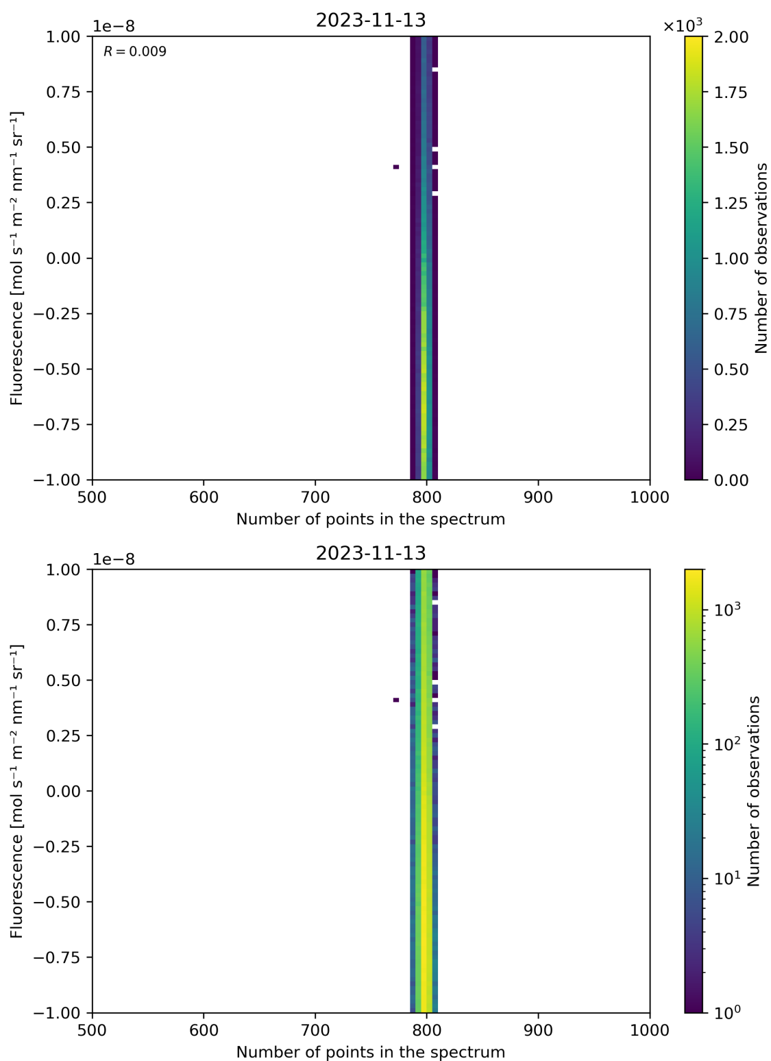
Figure 91: Scatter density plot of “Number of points in the spectrum” against “Fluorescence” for 2023-11-13 to 2023-11-14.
