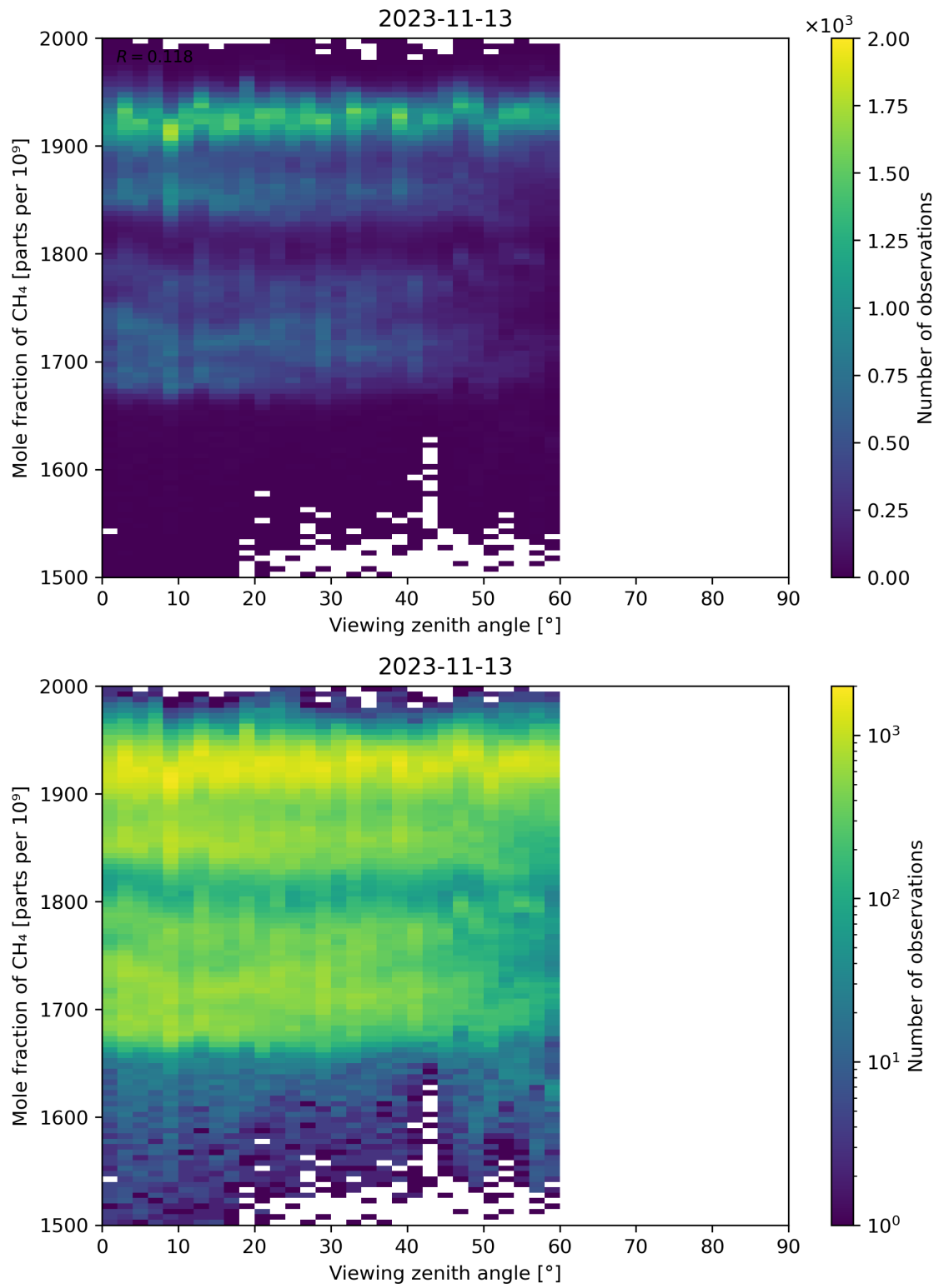
Figure 110: Scatter density plot of “Viewing zenith angle” against “Mole fraction of CH 4 ” for 2023-11-13 to 2023-11-14.
