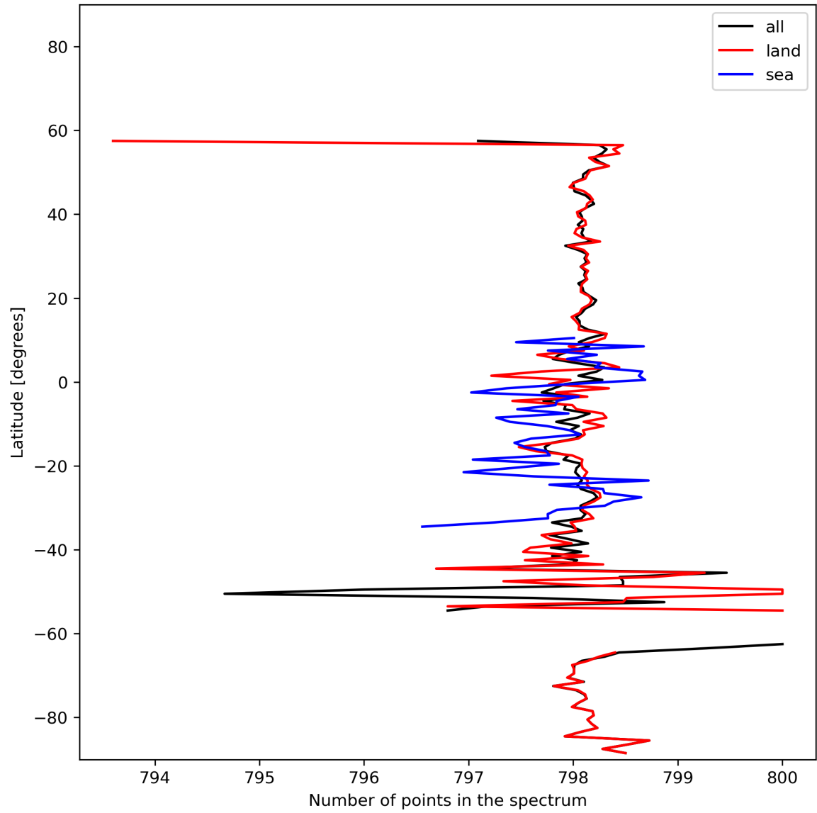
Figure 15: Zonal average of “Number of points in the spectrum” for 2023-11-13 to 2023-11-14.
