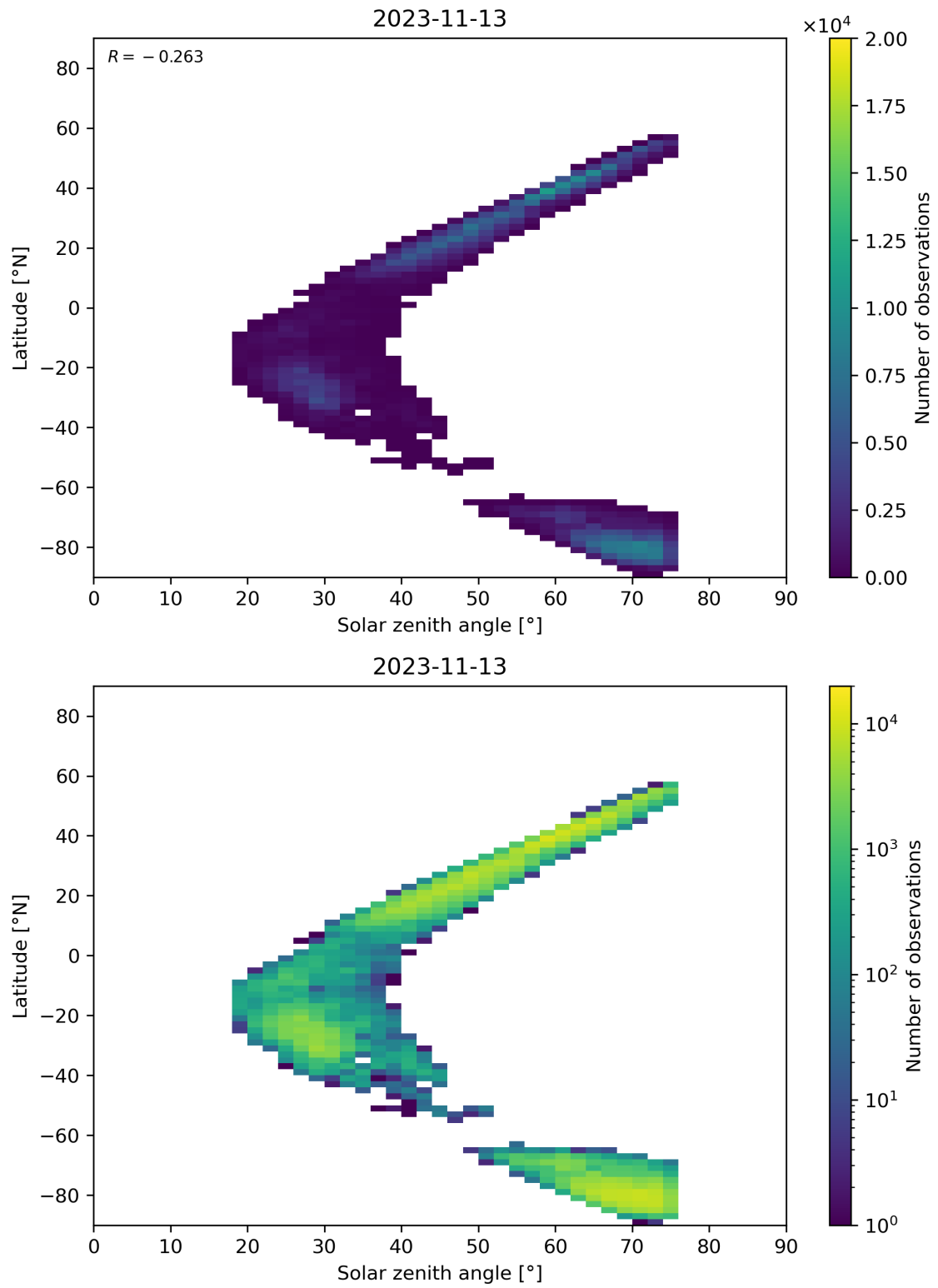
Figure 98: Scatter density plot of “Solar zenith angle” against “Latitude” for 2023-11-13 to 2023-11-14.
