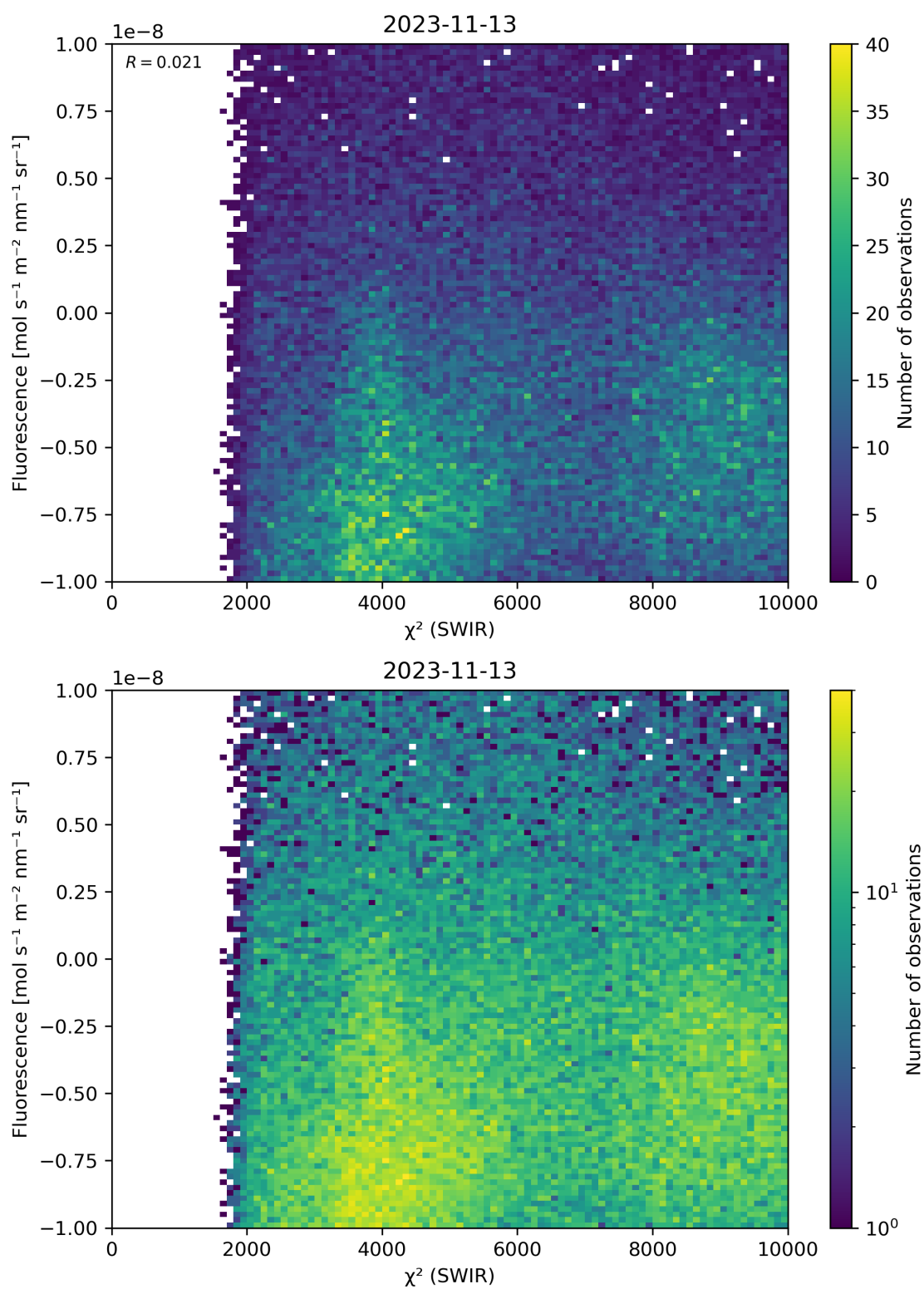
Figure 49: Scatter density plot of “ \chi^2 (SWIR)” against “Fluorescence” for 2023-11-13 to 2023-11-14.
