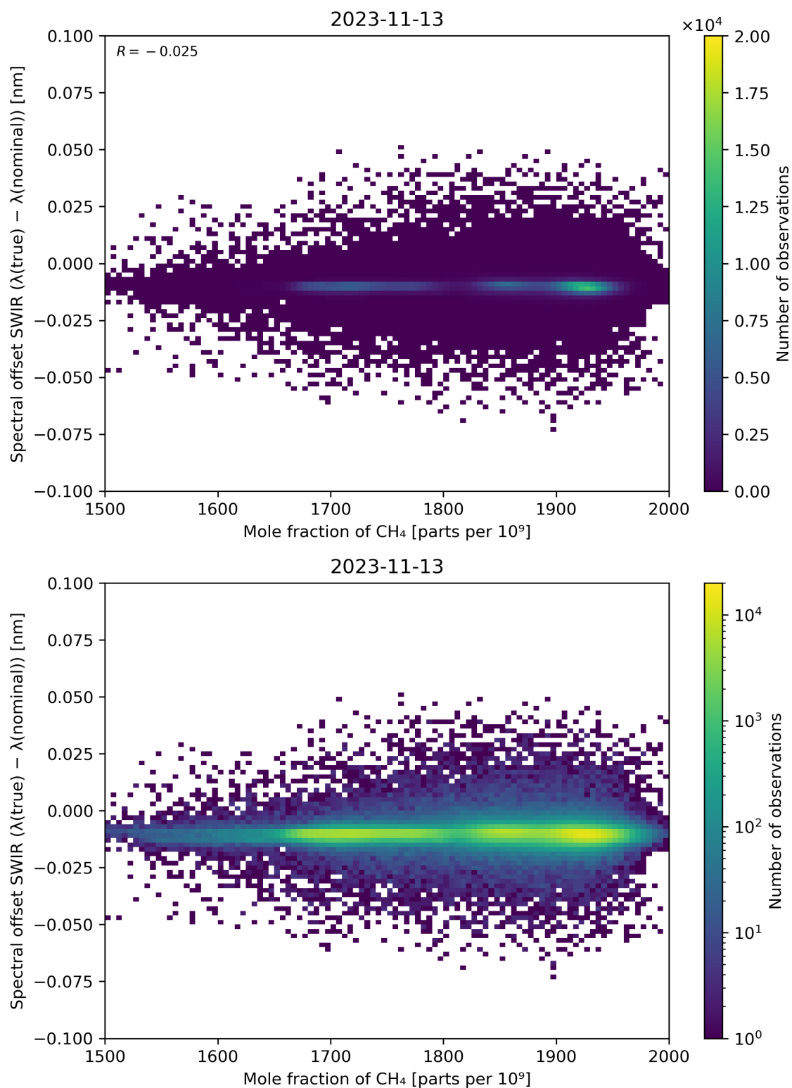
Figure 86: Scatter density plot of “Mole fraction of CH 4 ” against “Spectral offset SWIR ( \lambda(\text{true}) - \lambda(\text{nominal}) )” for 2023-11-13 to 2023-11-14.
