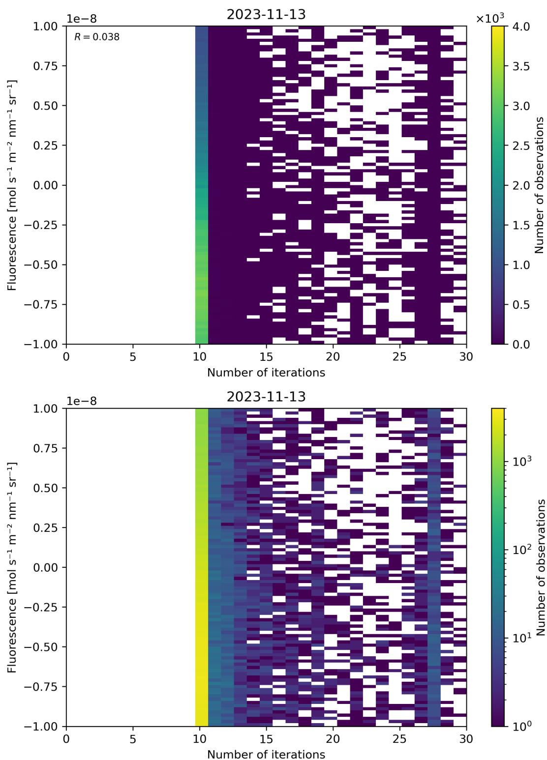
Figure 87: Scatter density plot of “Number of iterations” against “Fluorescence” for 2023-11-13 to 2023-11-14.
