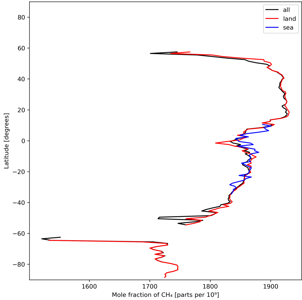
Figure 12: Zonal average of “Mole fraction of \text{CH}_4 ” for 2023-11-13 to 2023-11-14.
