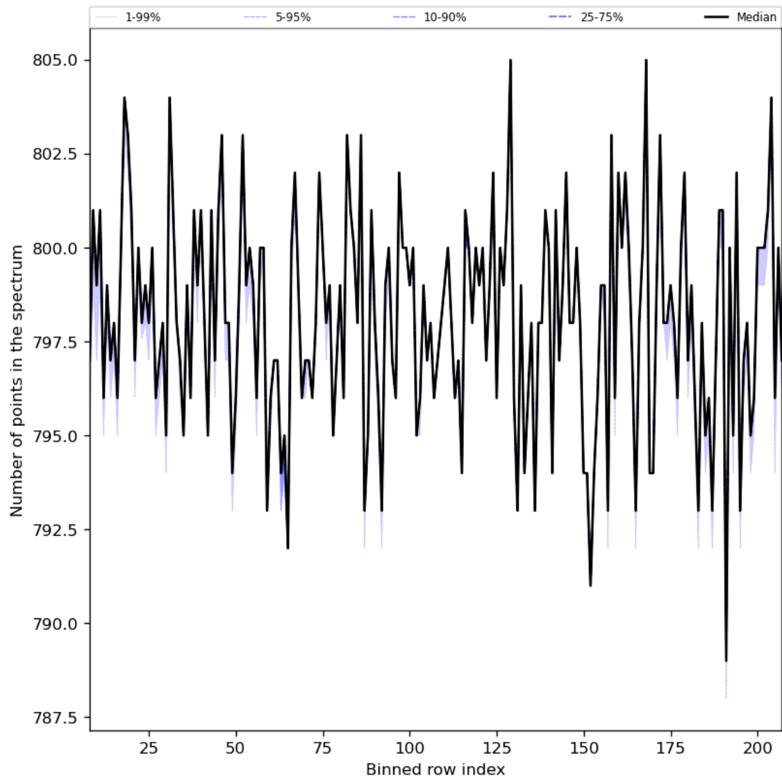
Figure 37: Along track statistics of “Number of points in the spectrum” for 2023-11-13 to 2023-11-14
