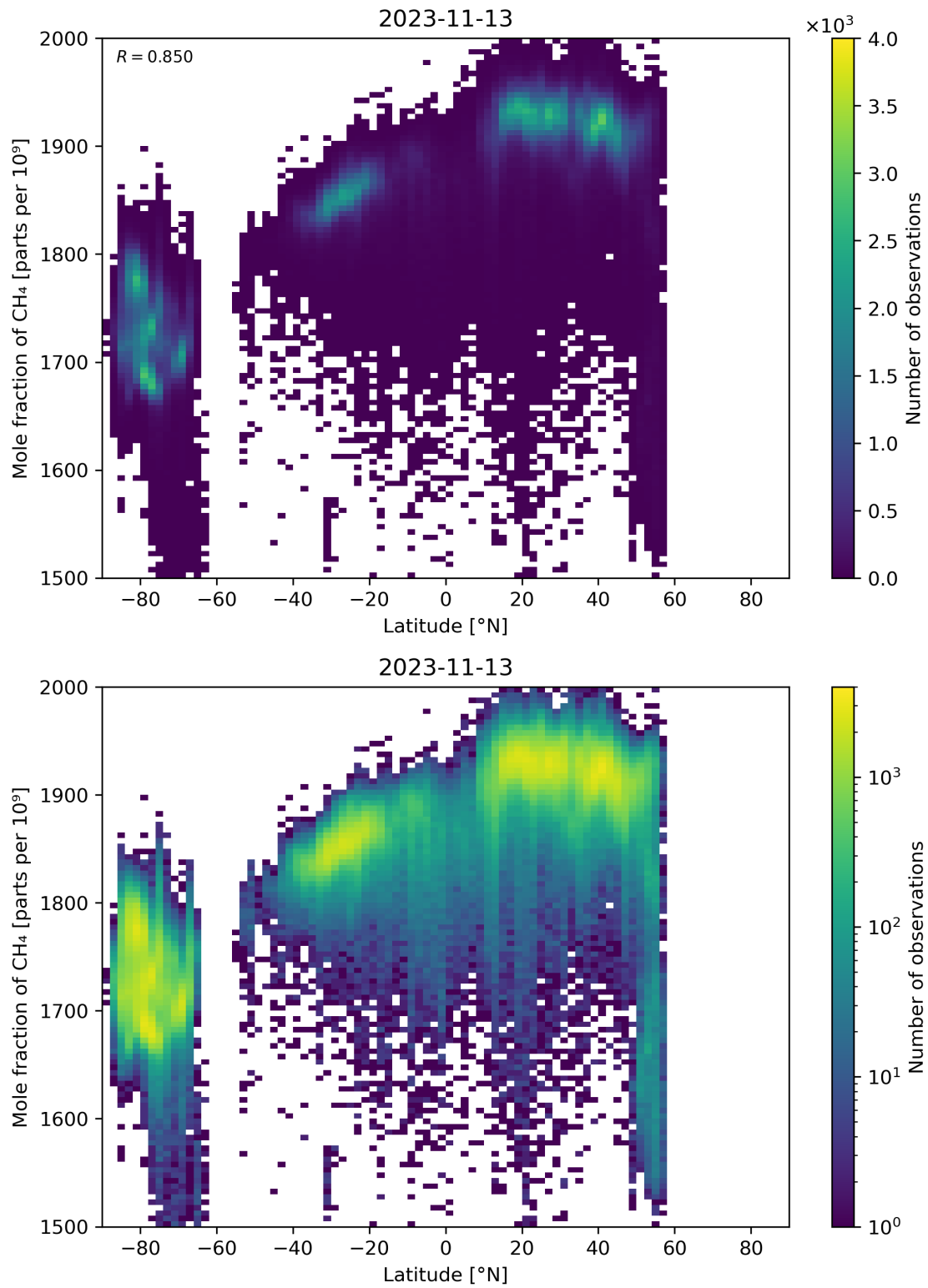
Figure 57: Scatter density plot of “Latitude” against “Mole fraction of CH 4 ” for 2023-11-13 to 2023-11-14.
