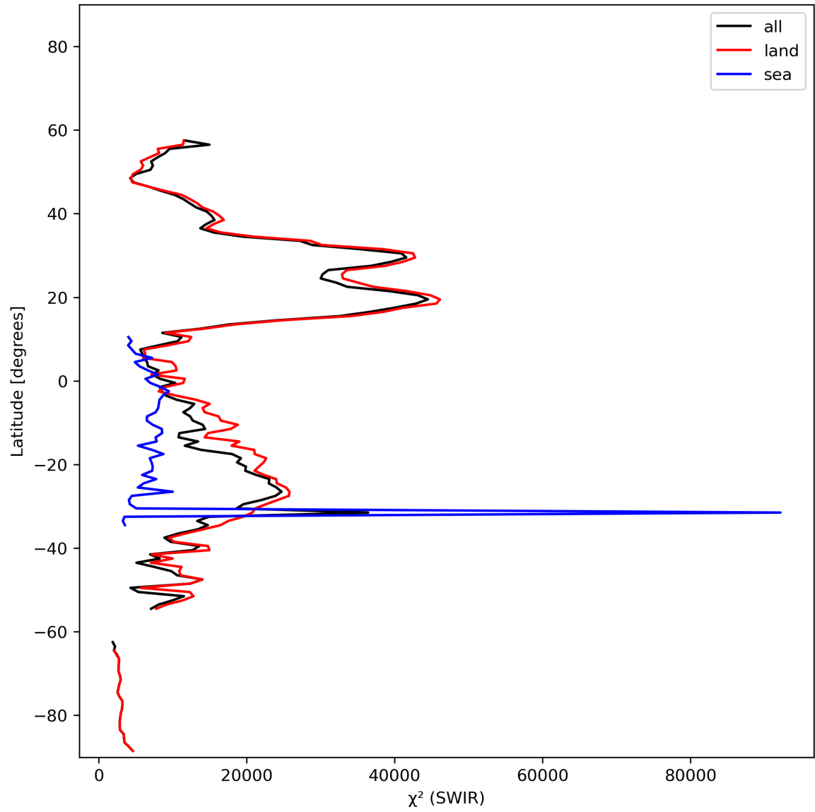
Figure 17: Zonal average of “ \chi^2 (SWIR)” for 2023-11-13 to 2023-11-14.
