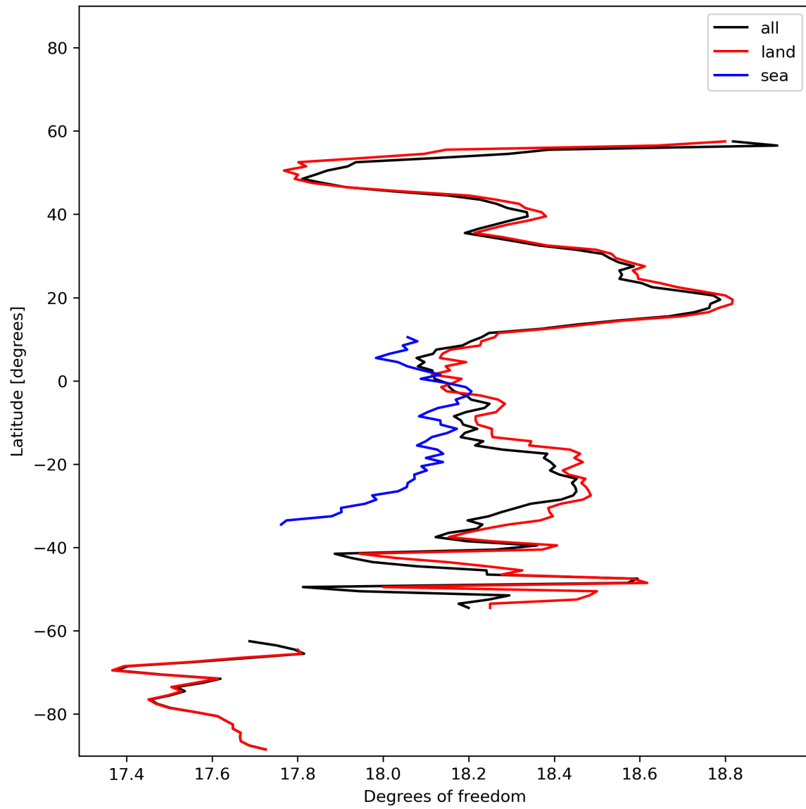
Figure 19: Zonal average of “Degrees of freedom” for 2023-11-13 to 2023-11-14.
