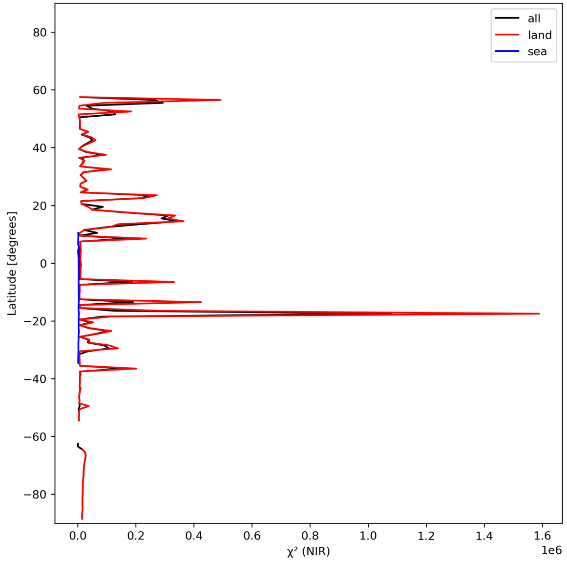
Figure 18: Zonal average of “ \chi^2 (NIR)” for 2023-11-13 to 2023-11-14.
