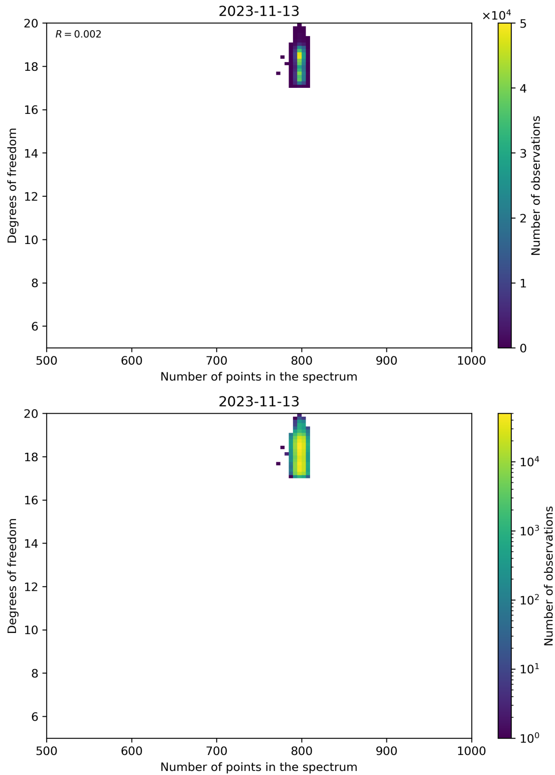
Figure 90: Scatter density plot of “Number of points in the spectrum” against “Degrees of freedom” for 2023-11-13 to 2023-11-14.
