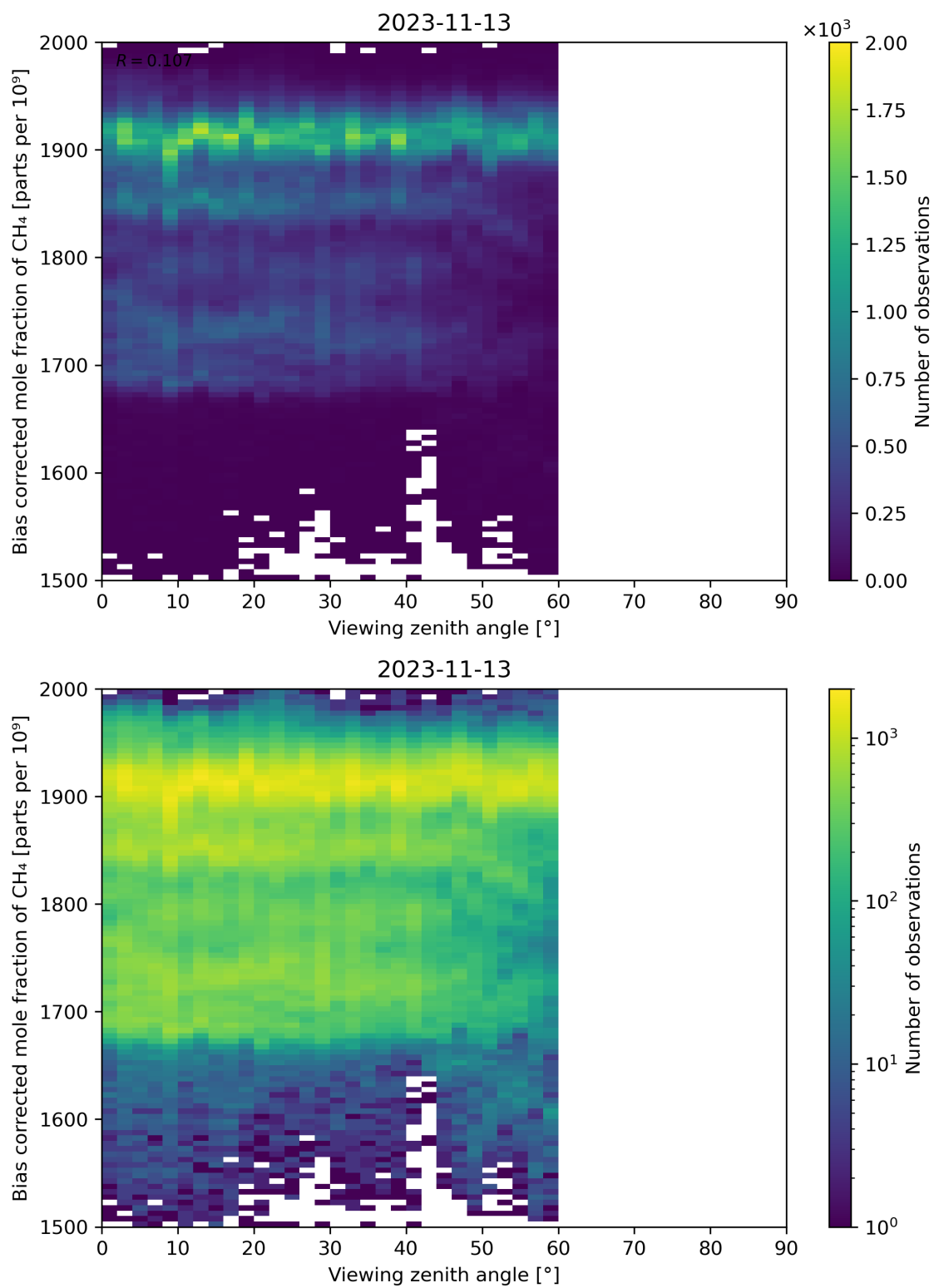
Figure 111: Scatter density plot of “Viewing zenith angle” against “Bias corrected mole fraction of CH 4 ” for 2023-11-13 to 2023-11-14.
