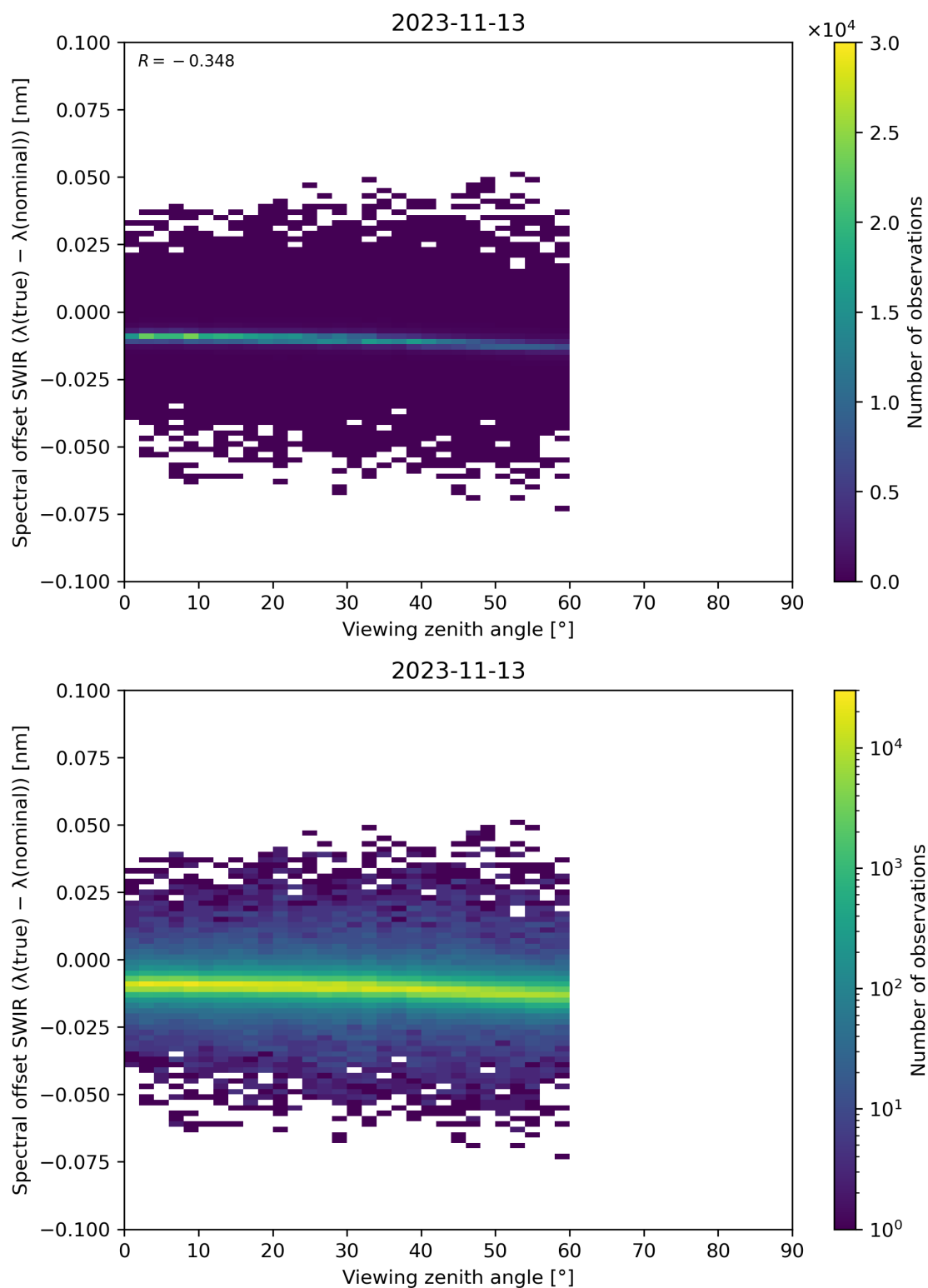
Figure 116: Scatter density plot of “Viewing zenith angle” against “Spectral offset SWIR ( \lambda(\text{true}) - \lambda(\text{nominal}) )” for 2023-11-13 to 2023-11-14.
