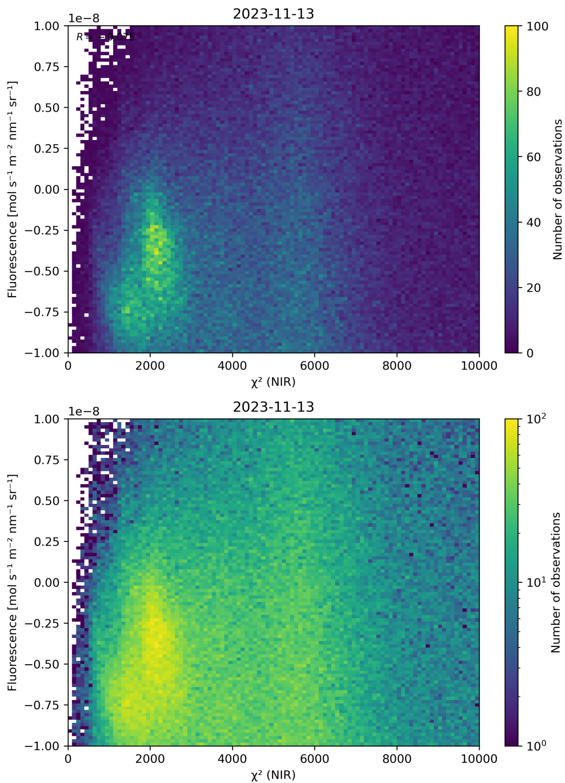
Figure 45: Scatter density plot of “ \chi^2 (NIR)” against “Fluorescence” for 2023-11-13 to 2023-11-14.
