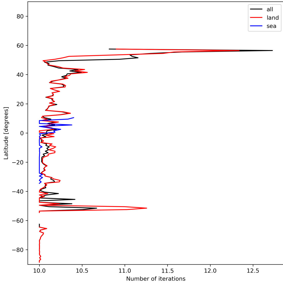
Figure 20: Zonal average of “Number of iterations” for 2023-11-13 to 2023-11-14.
