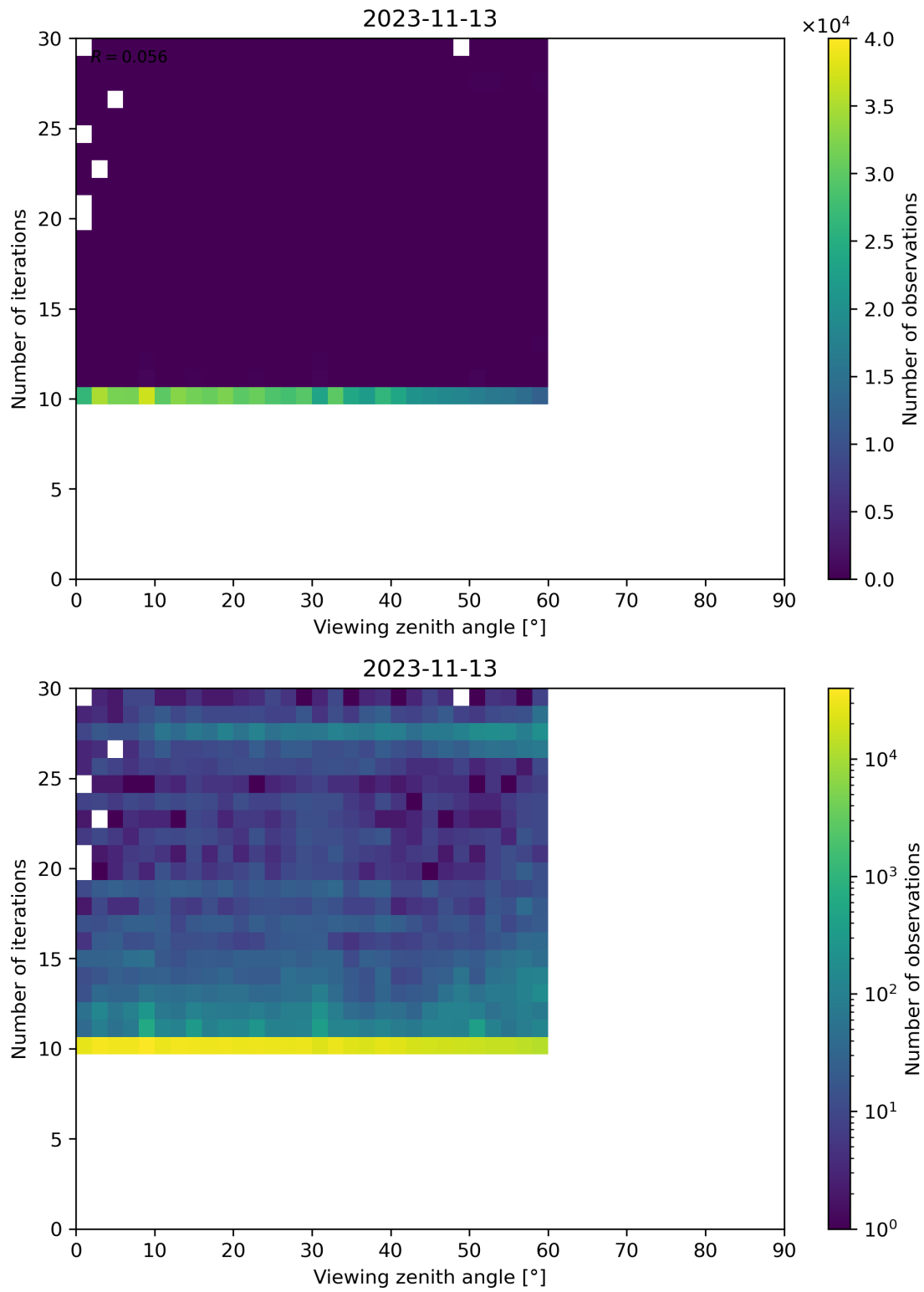
Figure 113: Scatter density plot of “Viewing zenith angle” against “Number of iterations” for 2023-11-13 to 2023-11-14.
