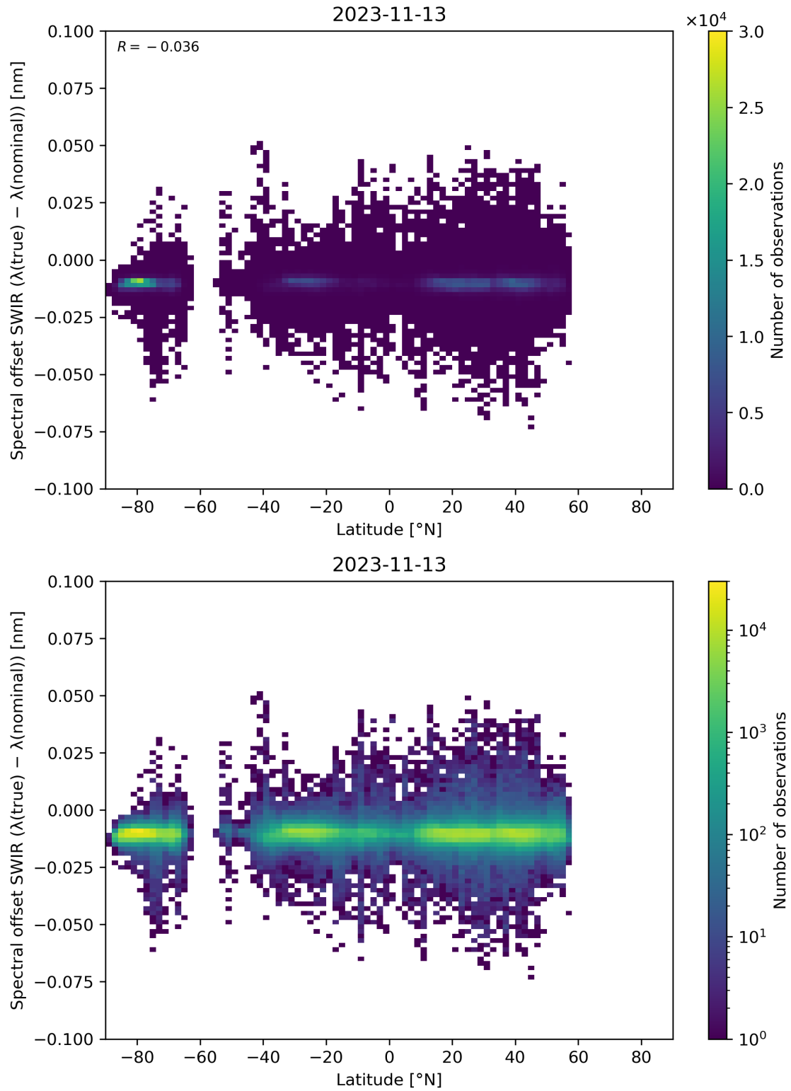
Figure 62: Scatter density plot of “Latitude” against “Spectral offset SWIR ( \lambda(\text{true}) - \lambda(\text{nominal}) )” for 2023-11-13 to 2023-11-14.
