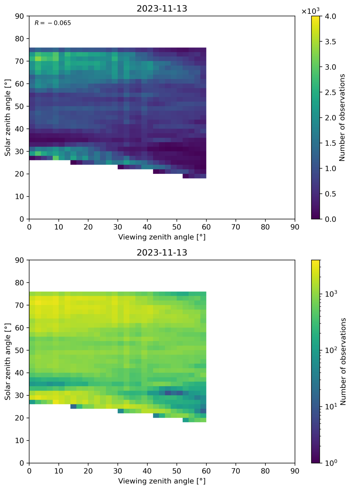
Figure 115: Scatter density plot of “Viewing zenith angle” against “Solar zenith angle” for 2023-11-13 to 2023-11-14.
