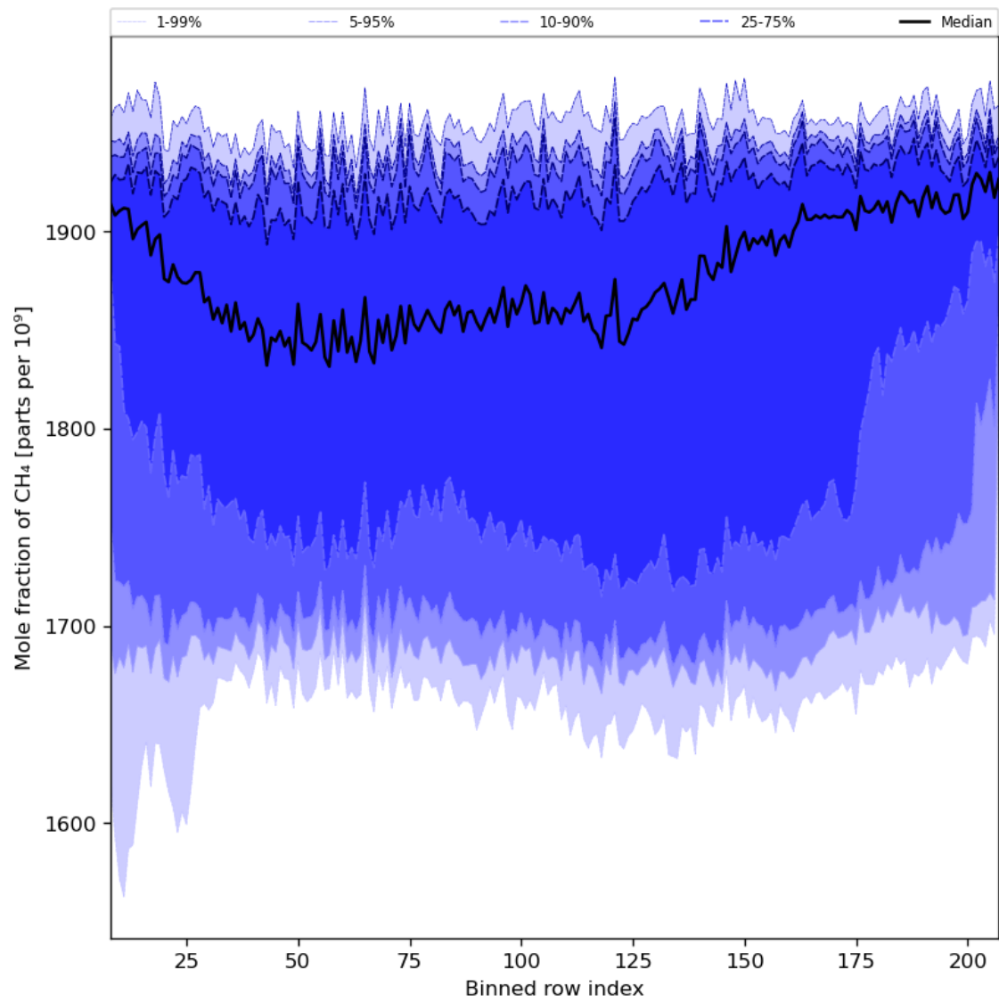
Figure 34: Along track statistics of “Mole fraction of CH 4 ” for 2023-11-13 to 2023-11-14
