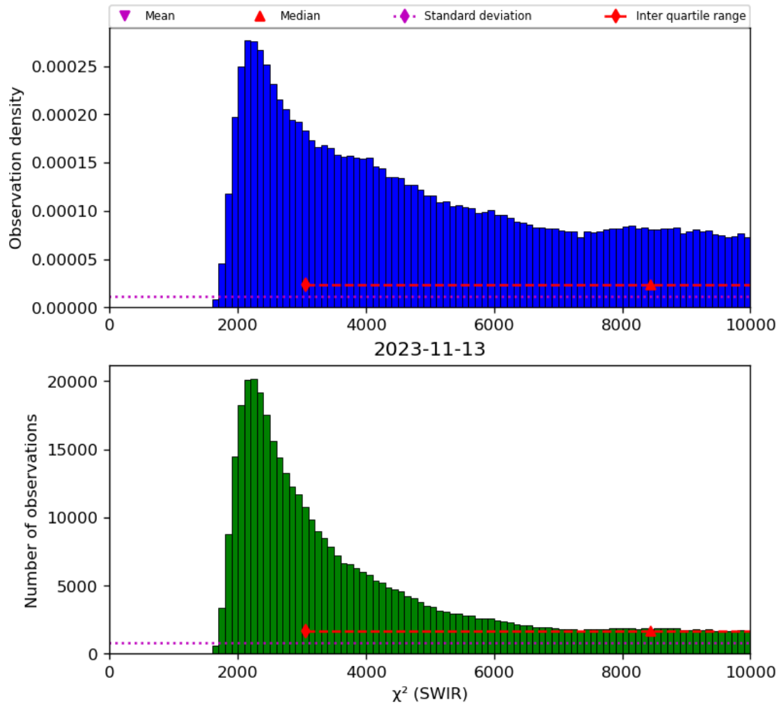
Figure 28: Histogram of “ \chi^2 (SWIR)” for 2023-11-13 to 2023-11-14
