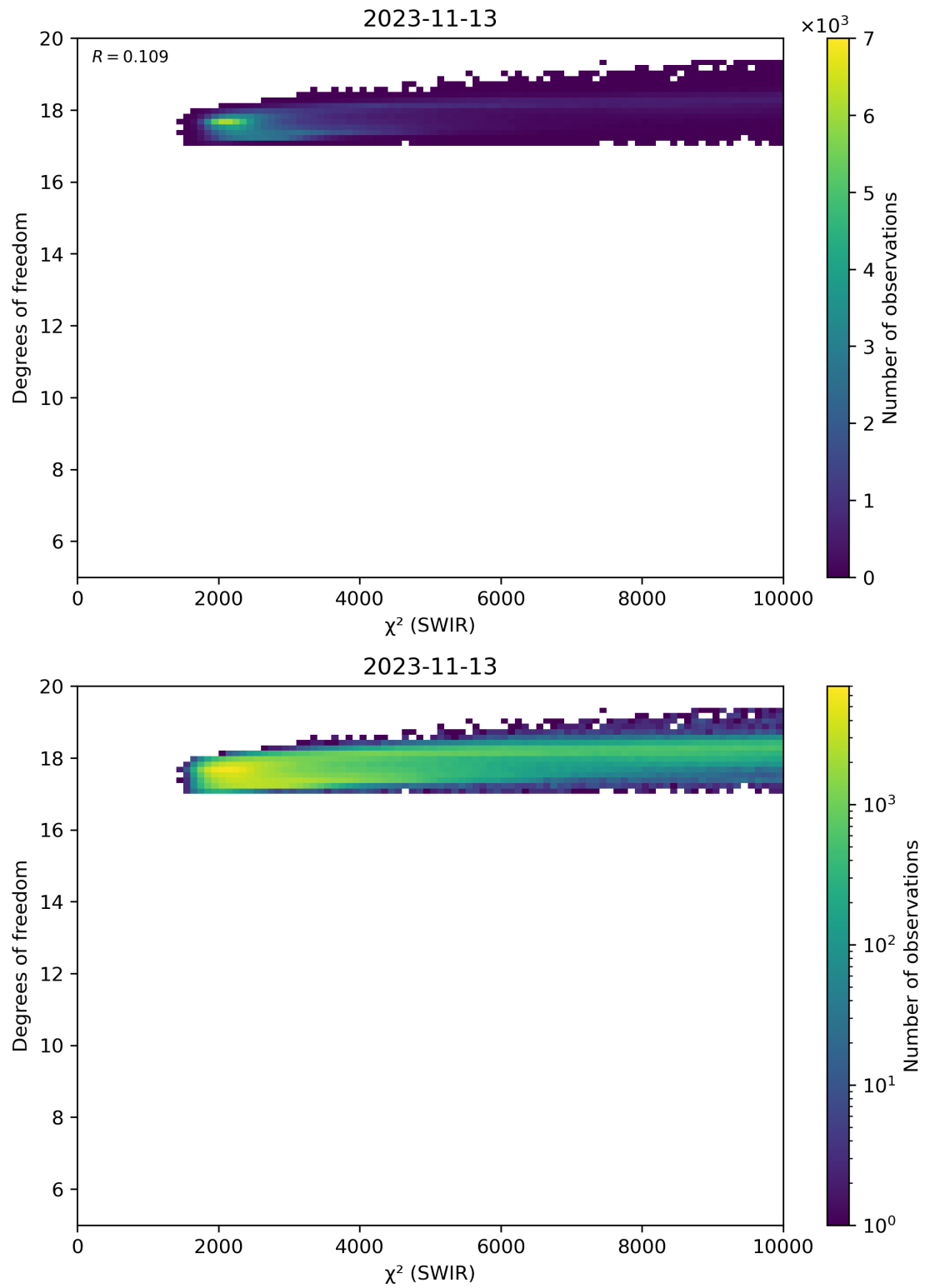
Figure 48: Scatter density plot of “ \chi^2 (SWIR)” against “Degrees of freedom” for 2023-11-13 to 2023-11-14.
