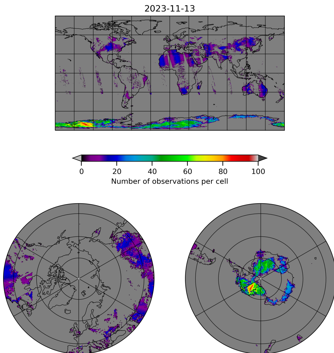
Figure 10: Map of the number of observations for 2023-11-13 to 2023-11-14
