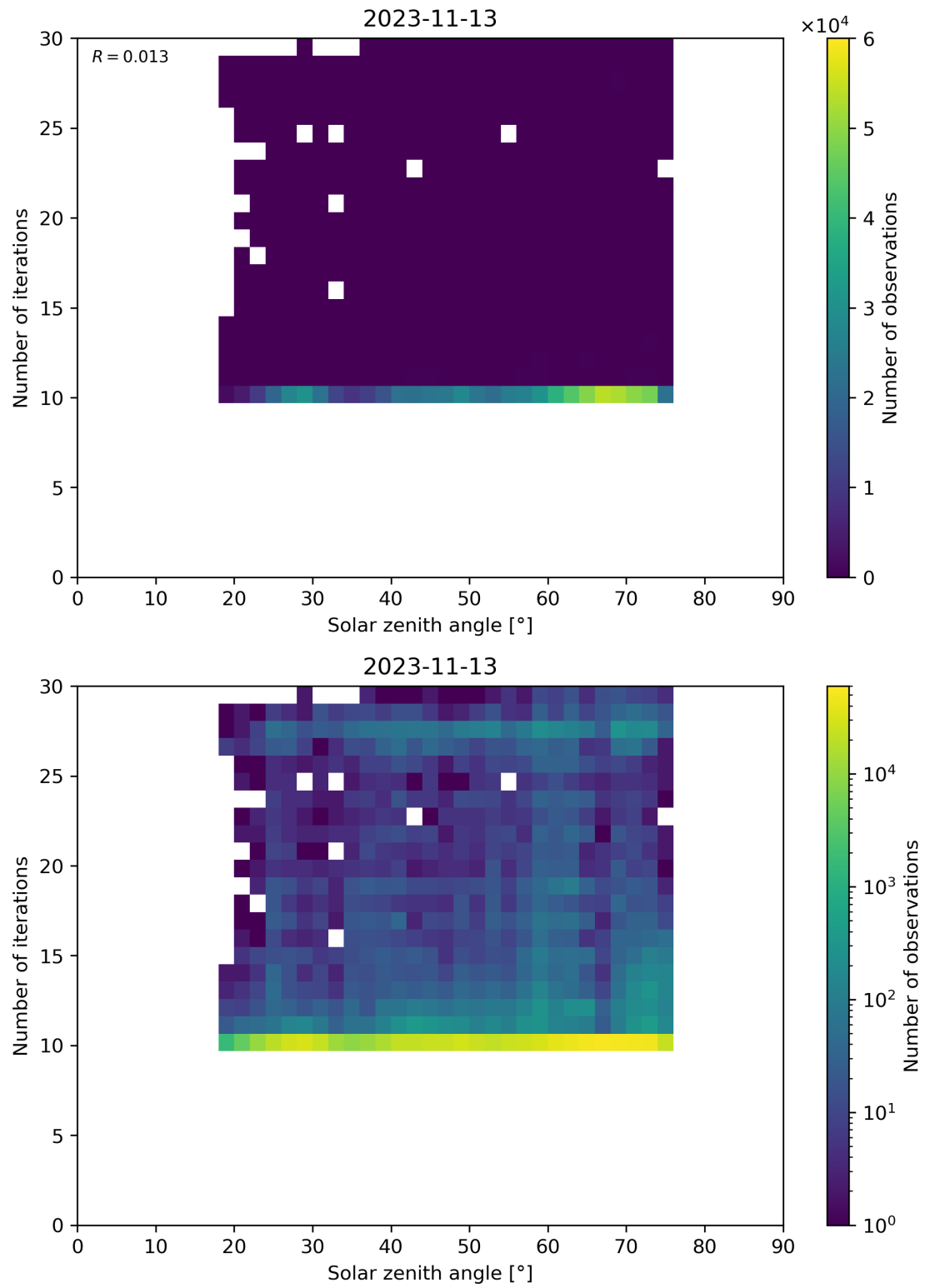
Figure 102: Scatter density plot of “Solar zenith angle” against “Number of iterations” for 2023-11-13 to 2023-11-14.
