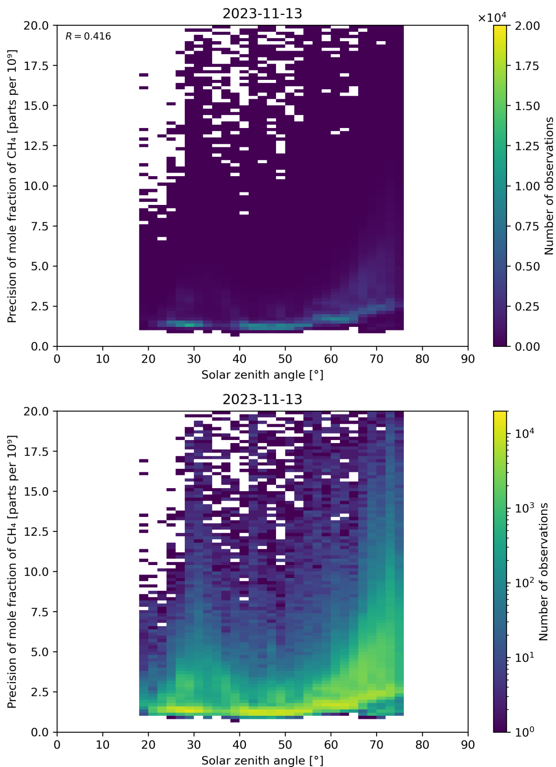
Figure 101: Scatter density plot of “Solar zenith angle” against “Precision of mole fraction of \text{CH}_4 ” for 2023-11-13 to 2023-11-14.
