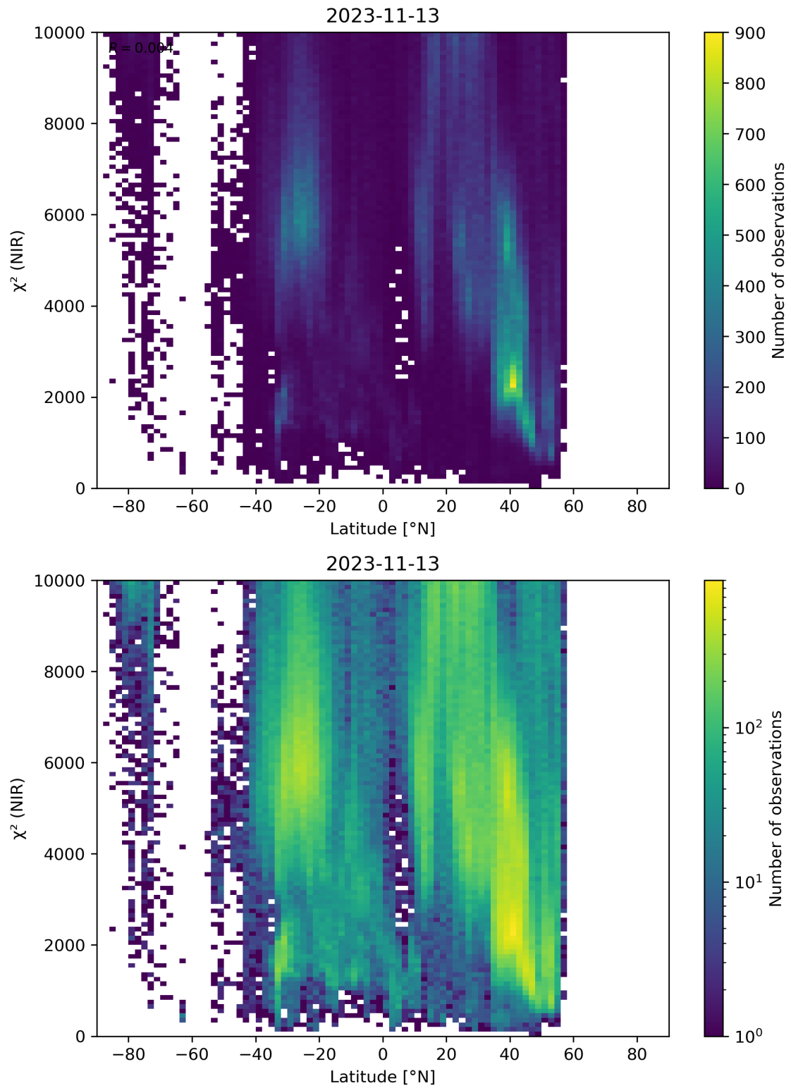
Figure 53: Scatter density plot of “Latitude” against “ \chi^2 (NIR)” for 2023-11-13 to 2023-11-14.
