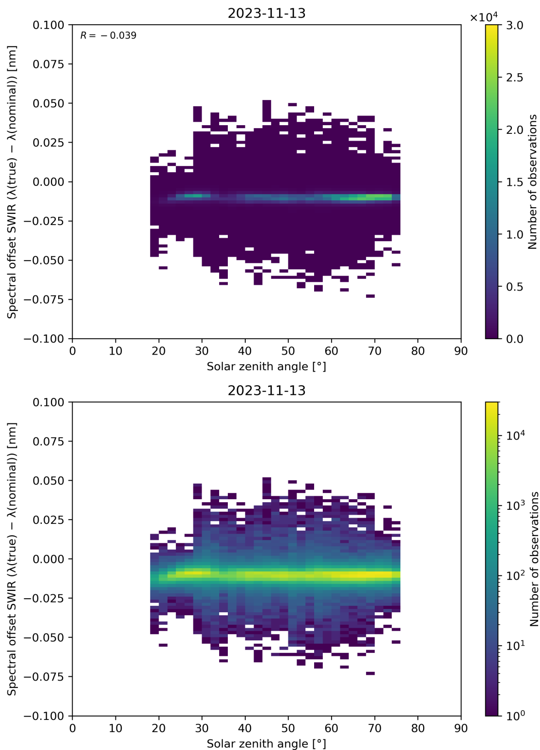
Figure 104: Scatter density plot of “Solar zenith angle” against “Spectral offset SWIR ( \lambda(\text{true}) - \lambda(\text{nominal}) )” for 2023-11-13 to 2023-11-14.
