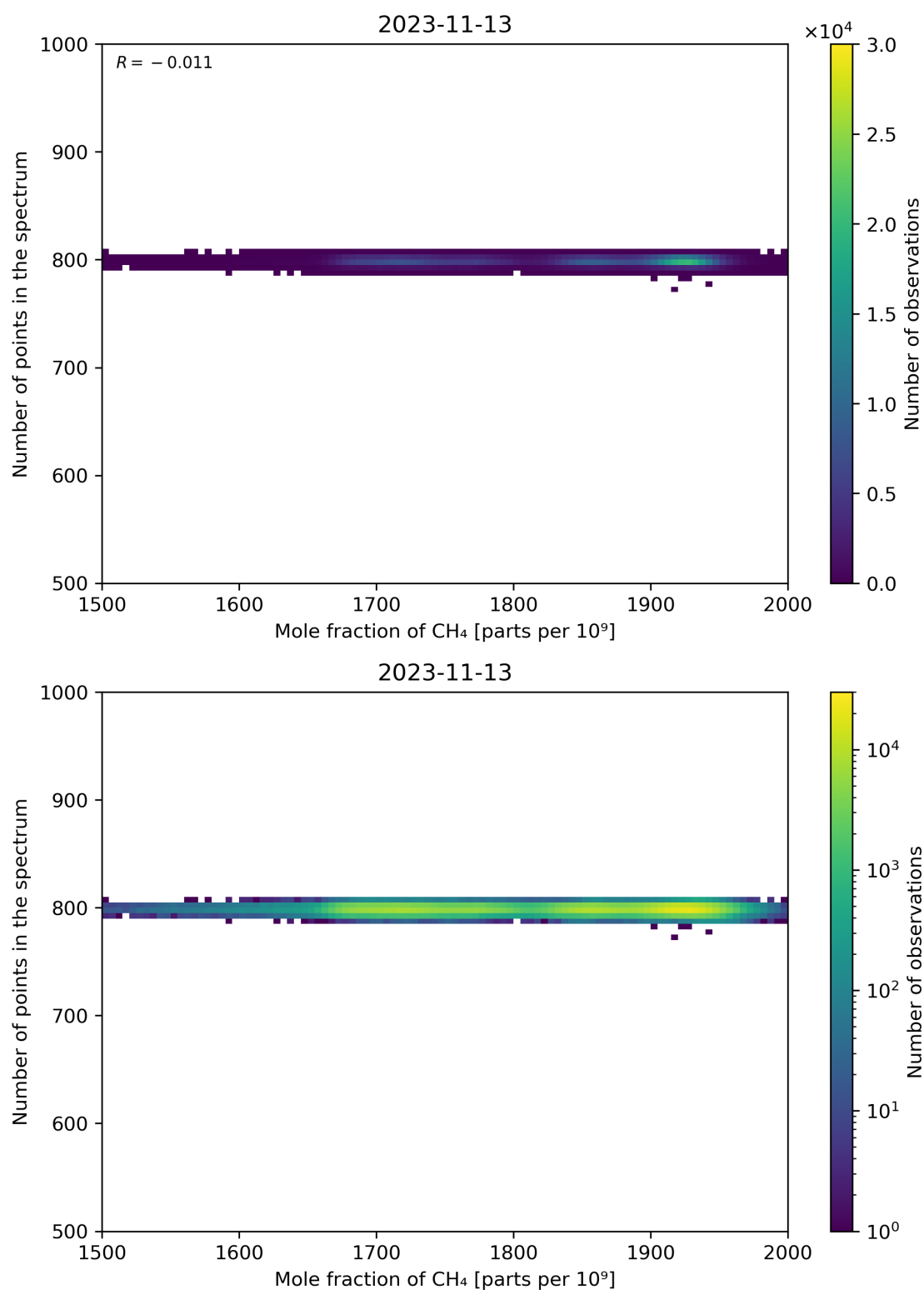
Figure 77: Scatter density plot of “Mole fraction of CH 4 ” against “Number of points in the spectrum” for 2023-11-13 to 2023-11-14.
