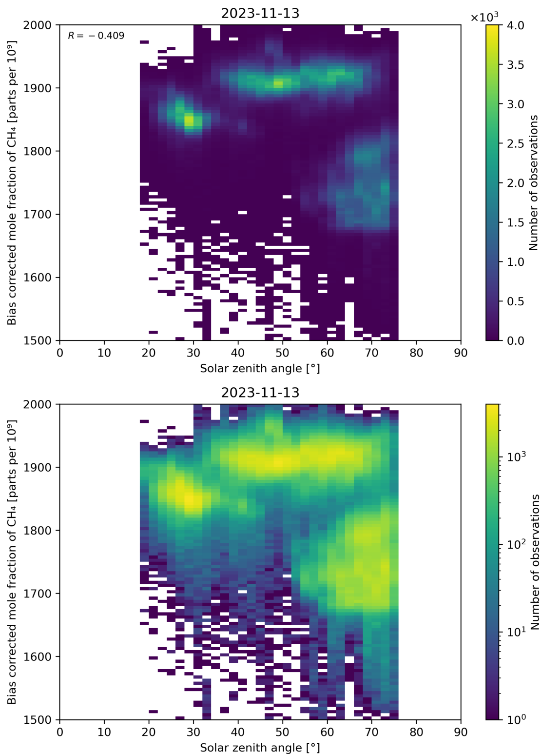
Figure 100: Scatter density plot of “Solar zenith angle” against “Bias corrected mole fraction of CH 4 ” for 2023-11-13 to 2023-11-14.
