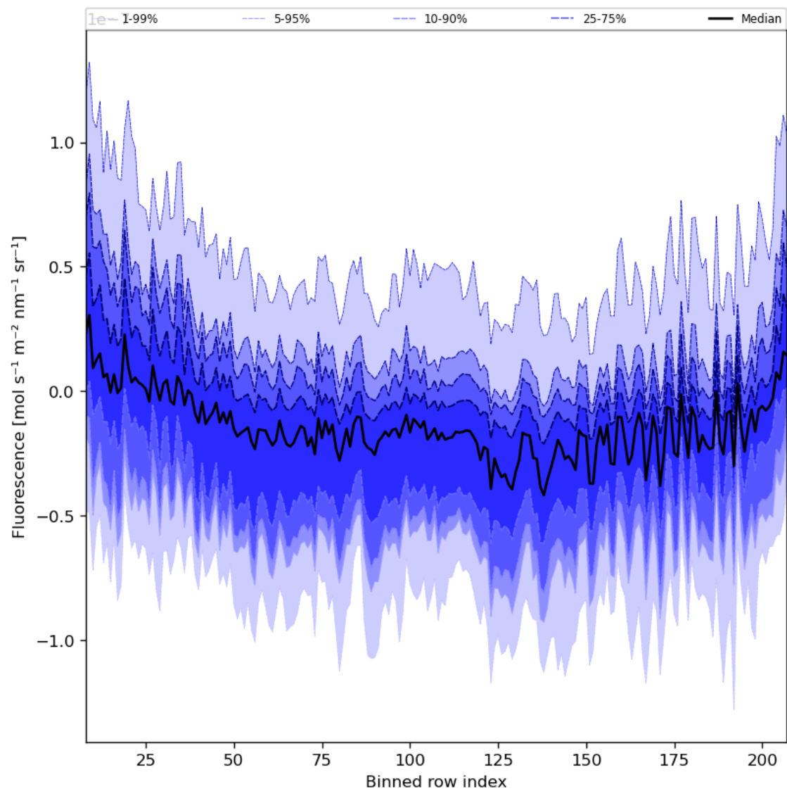
Figure 43: Along track statistics of “Fluorescence” for 2023-11-13 to 2023-11-14
