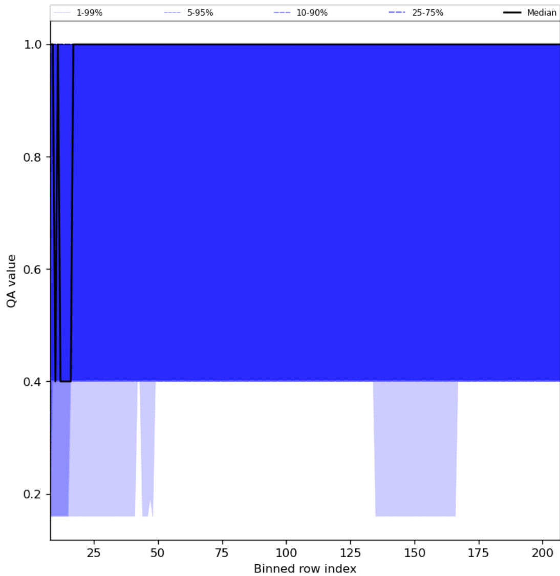
Figure 33: Along track statistics of “QA value” for 2023-11-13 to 2023-11-14
