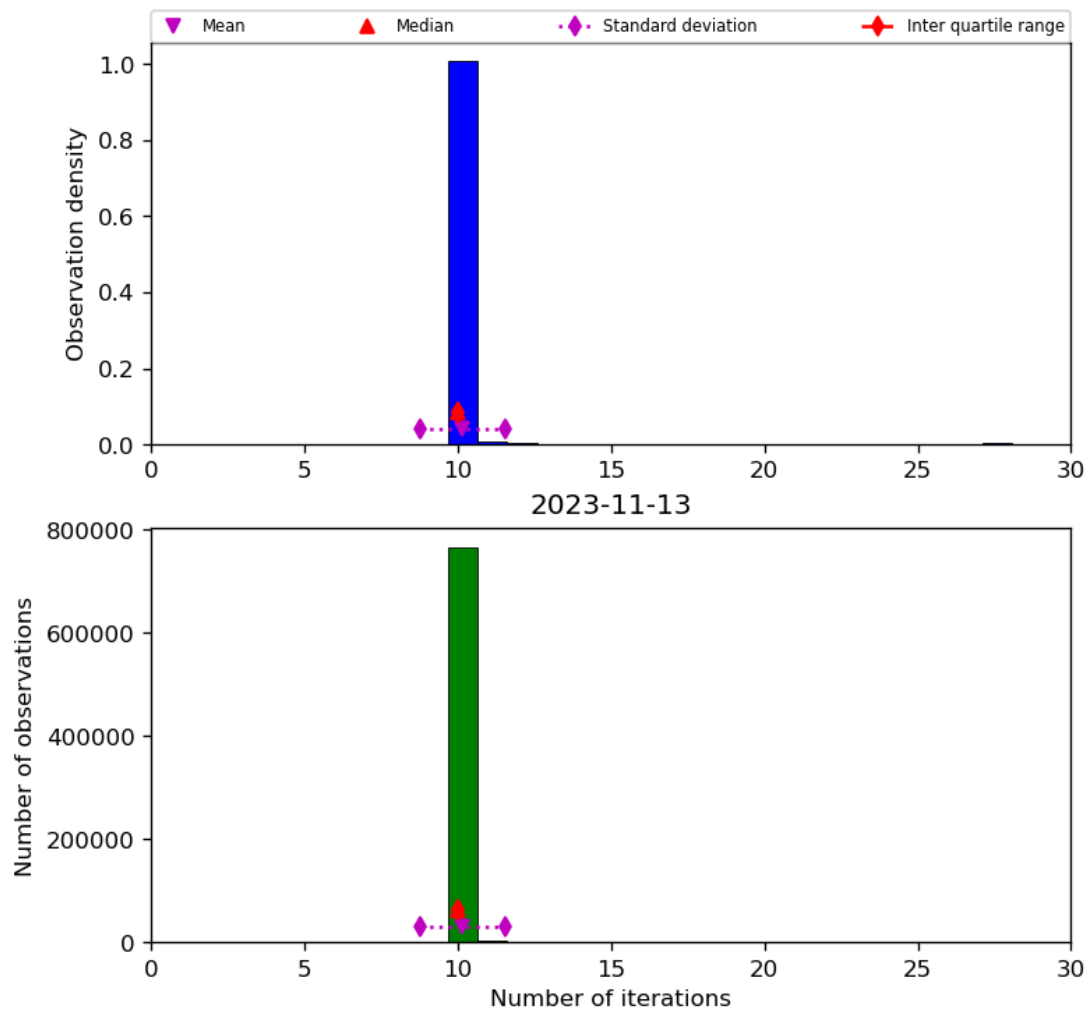
Figure 31: Histogram of “Number of iterations” for 2023-11-13 to 2023-11-14
