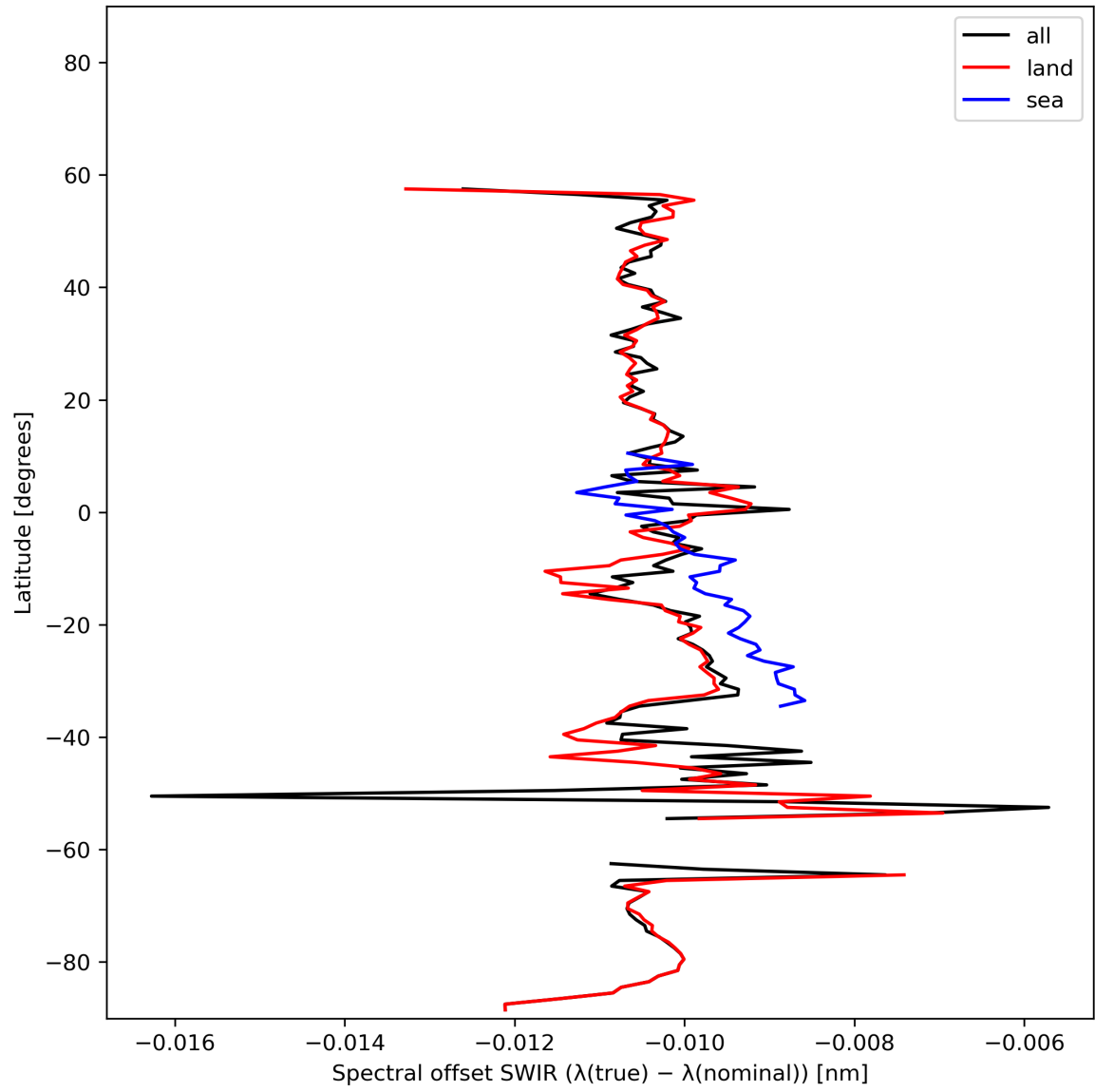
Figure 16: Zonal average of “Spectral offset SWIR ( \lambda(\text{true}) - \lambda(\text{nominal}) )” for 2023-11-13 to 2023-11-14.
