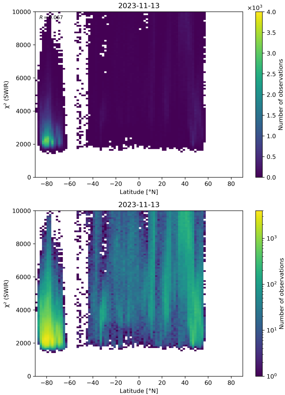
Figure 54: Scatter density plot of “Latitude” against “ \chi^2 (SWIR)” for 2023-11-13 to 2023-11-14.
