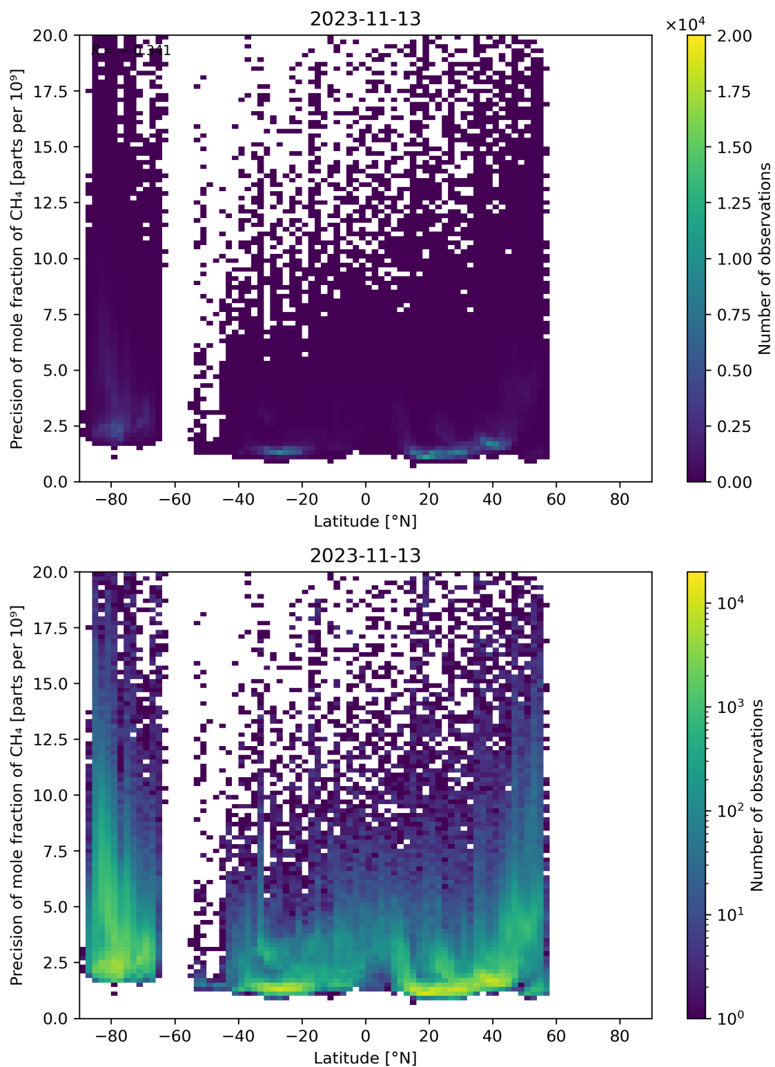
Figure 59: Scatter density plot of “Latitude” against “Precision of mole fraction of CH 4 ” for 2023-11-13 to 2023-11-14.
