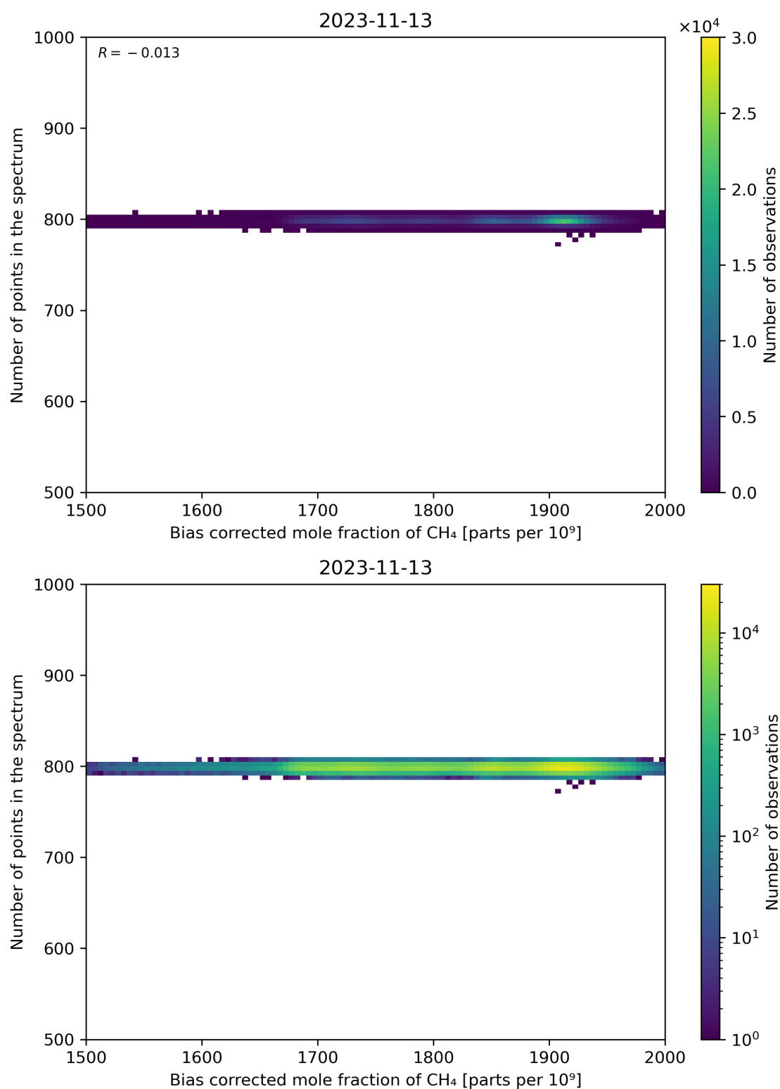
Figure 68: Scatter density plot of “Bias corrected mole fraction of CH 4 ” against “Number of points in the spectrum” for 2023-11-13 to 2023-11-14.
