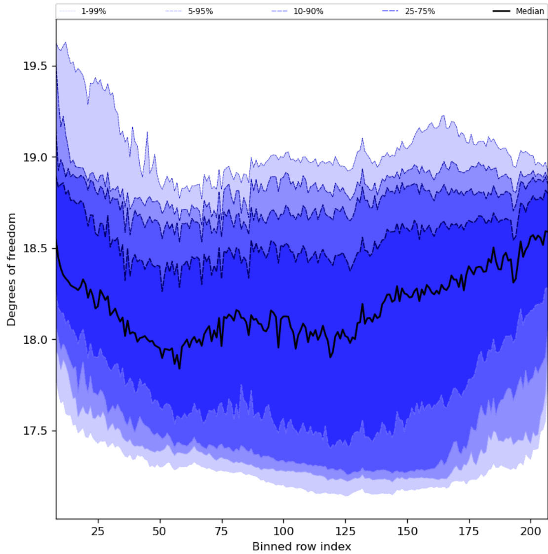
Figure 41: Along track statistics of “Degrees of freedom” for 2023-11-13 to 2023-11-14
