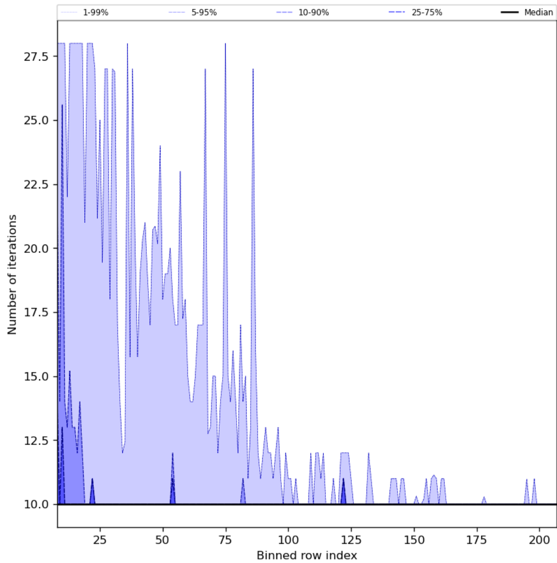
Figure 42: Along track statistics of “Number of iterations” for 2023-11-13 to 2023-11-14
