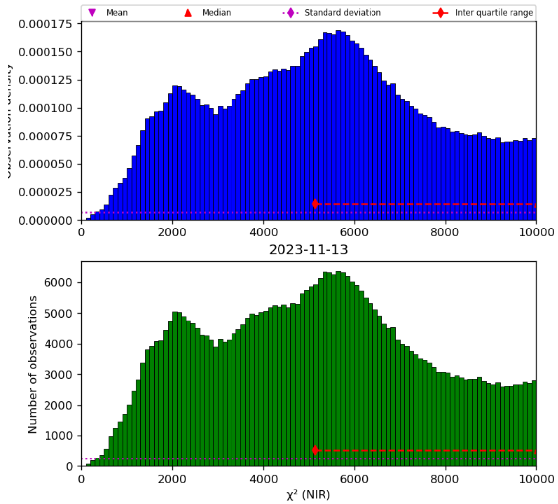
Figure 29: Histogram of “ \chi^2 (NIR)” for 2023-11-13 to 2023-11-14
