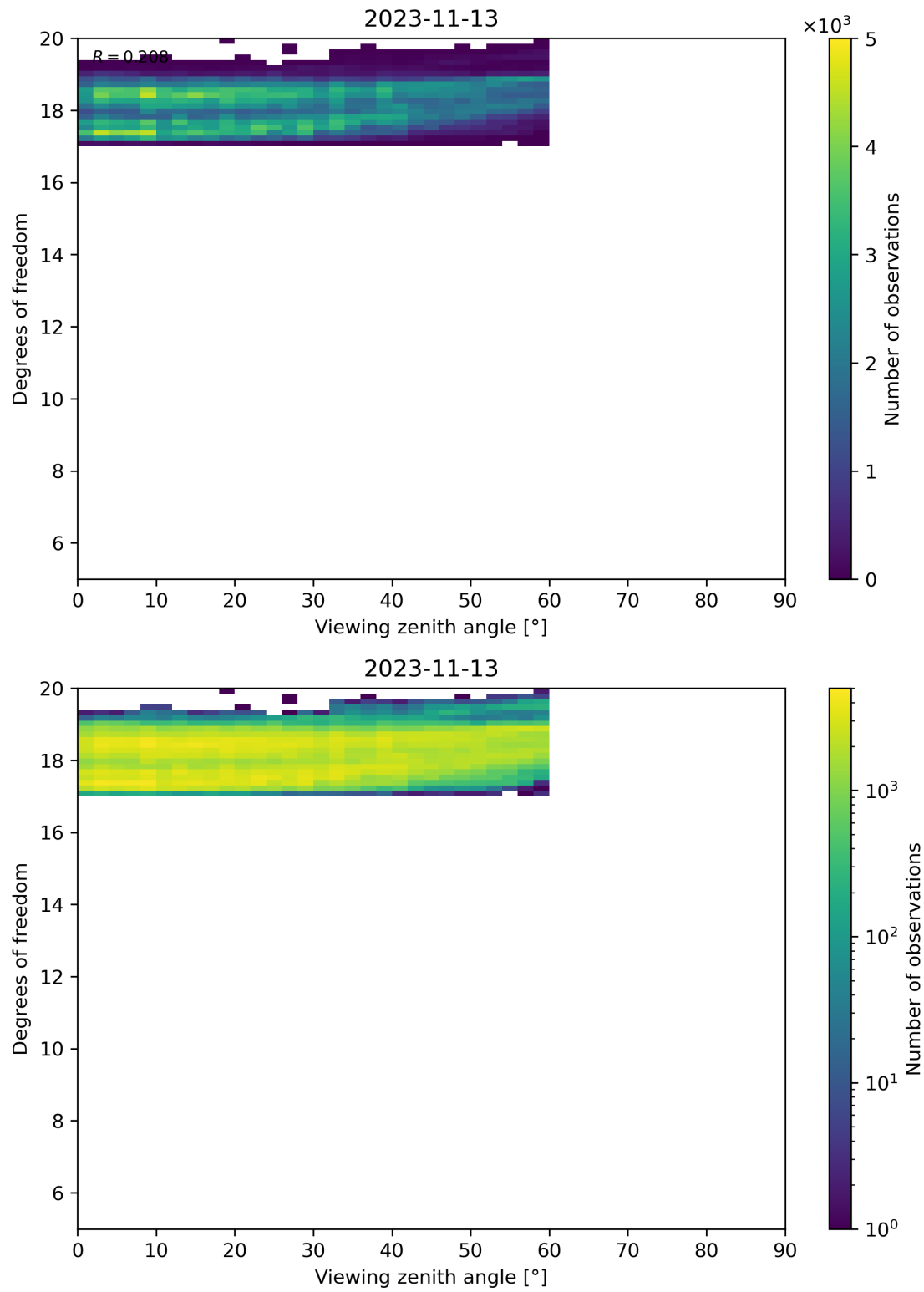
Figure 107: Scatter density plot of “Viewing zenith angle” against “Degrees of freedom” for 2023-11-13 to 2023-11-14.
