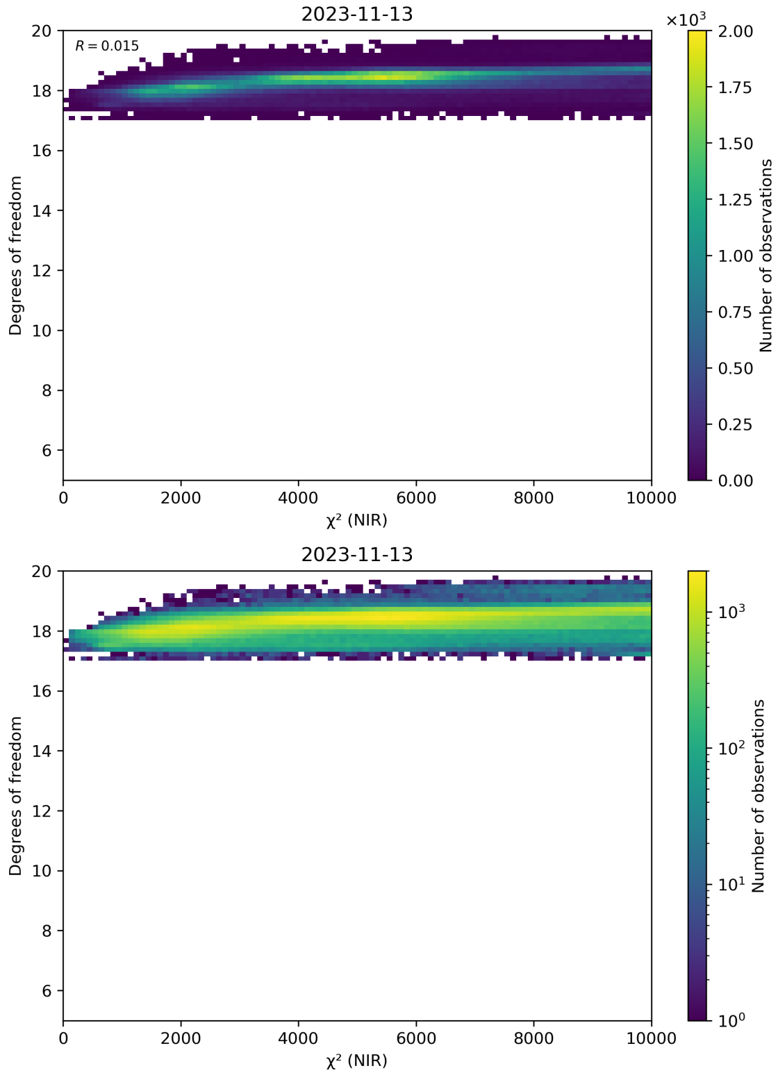
Figure 44: Scatter density plot of “ \chi^2 (NIR)” against “Degrees of freedom” for 2023-11-13 to 2023-11-14.
