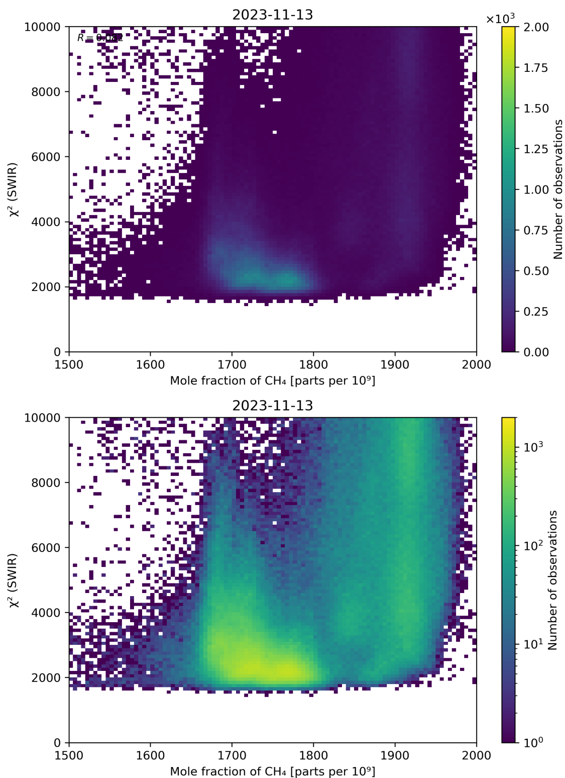
Figure 71: Scatter density plot of “Mole fraction of CH 4 ” against “ \chi^2 (SWIR)” for 2023-11-13 to 2023-11-14.
