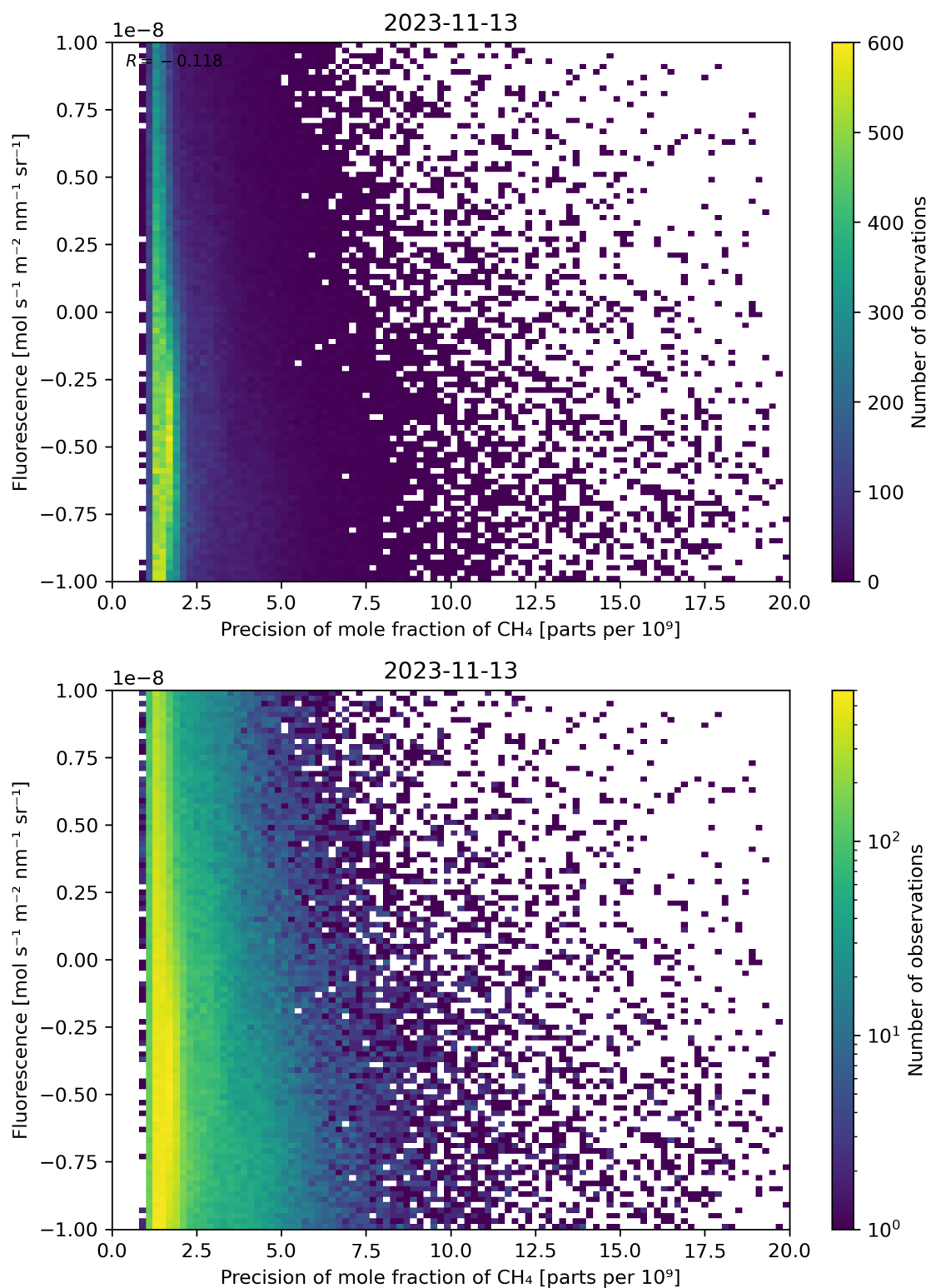
Figure 81: Scatter density plot of “Precision of mole fraction of CH 4 ” against “Fluorescence” for 2023-11-13 to 2023-11-14.
