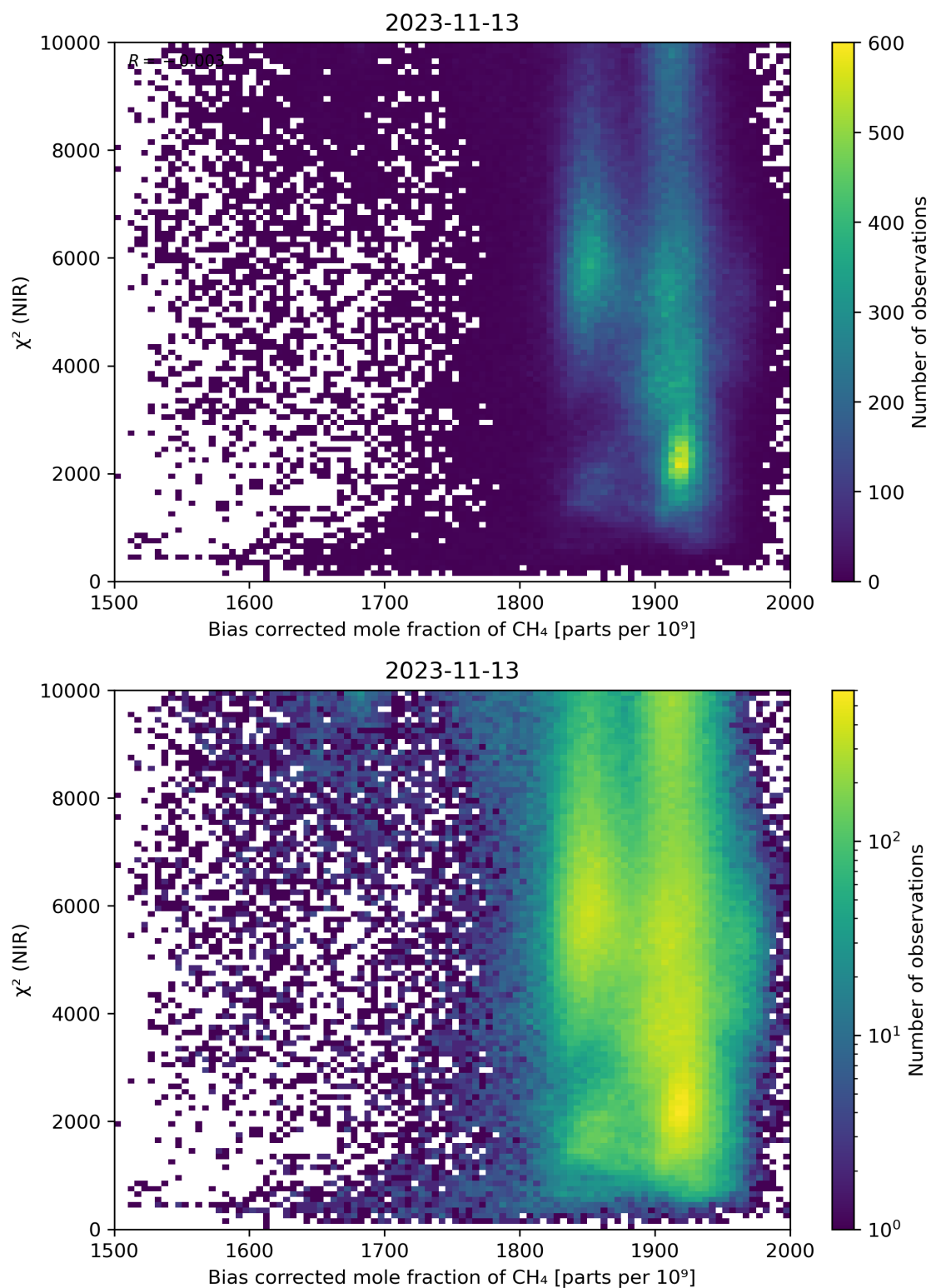
Figure 63: Scatter density plot of “Bias corrected mole fraction of CH 4 ” against “ \chi^2 (NIR)” for 2023-11-13 to 2023-11-14.
