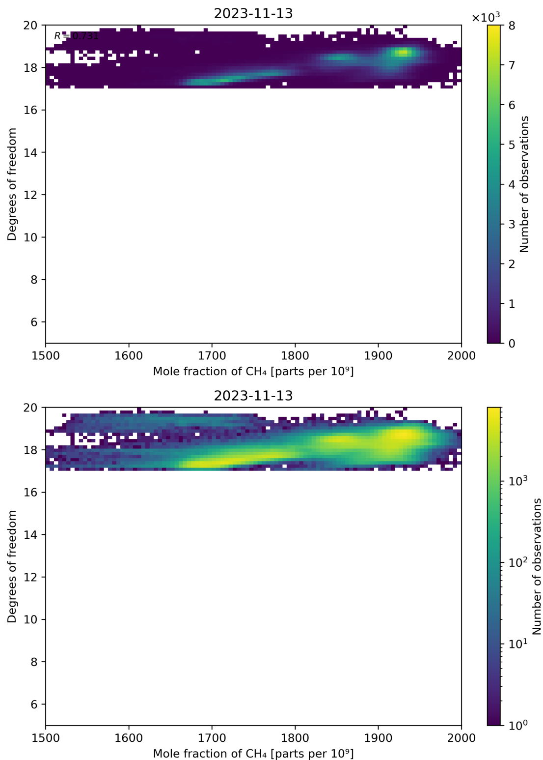
Figure 72: Scatter density plot of “Mole fraction of CH 4 ” against “Degrees of freedom” for 2023-11-13 to 2023-11-14.
