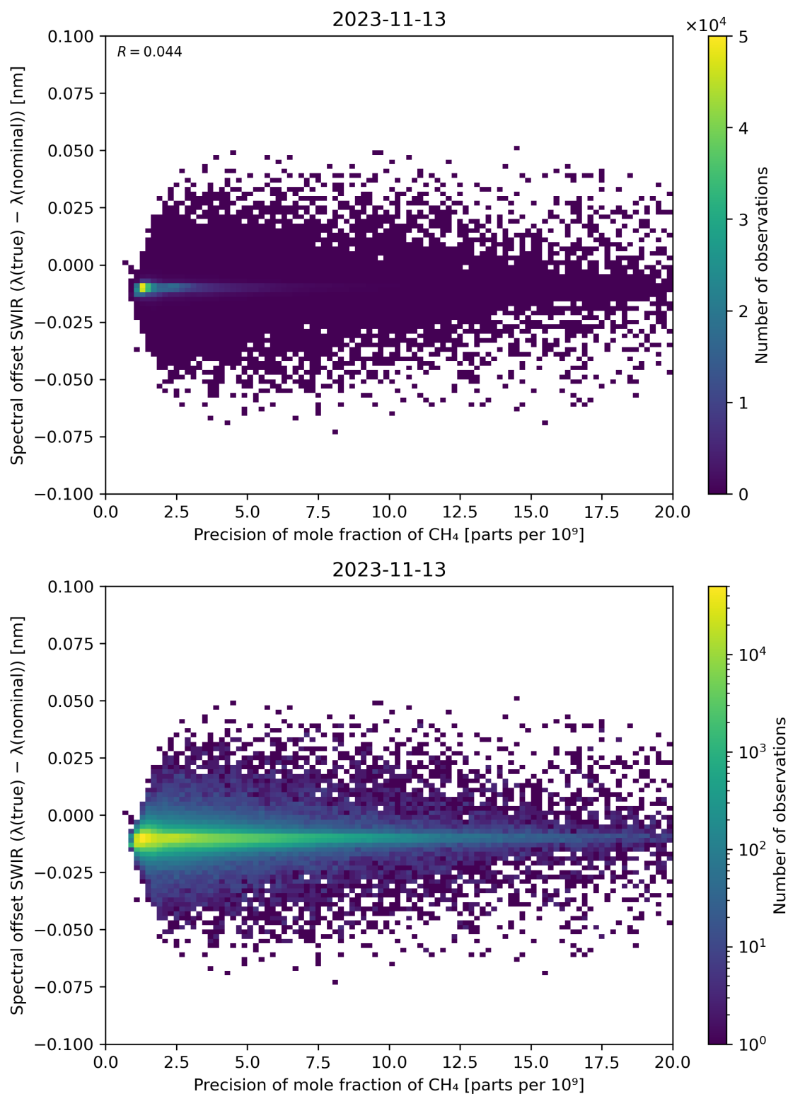
Figure 85: Scatter density plot of “Precision of mole fraction of CH 4 ” against “Spectral offset SWIR ( \lambda(\text{true}) - \lambda(\text{nominal}) )” for 2023-11-13 to 2023-11-14.
