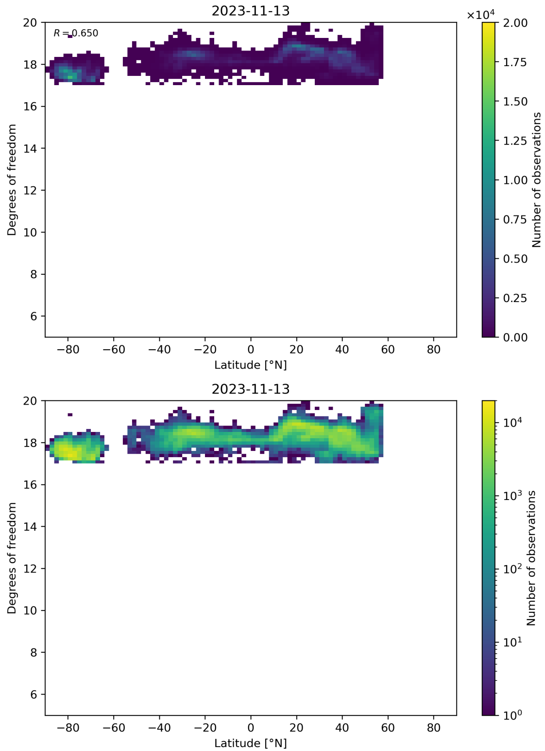
Figure 55: Scatter density plot of “Latitude” against “Degrees of freedom” for 2023-11-13 to 2023-11-14.
