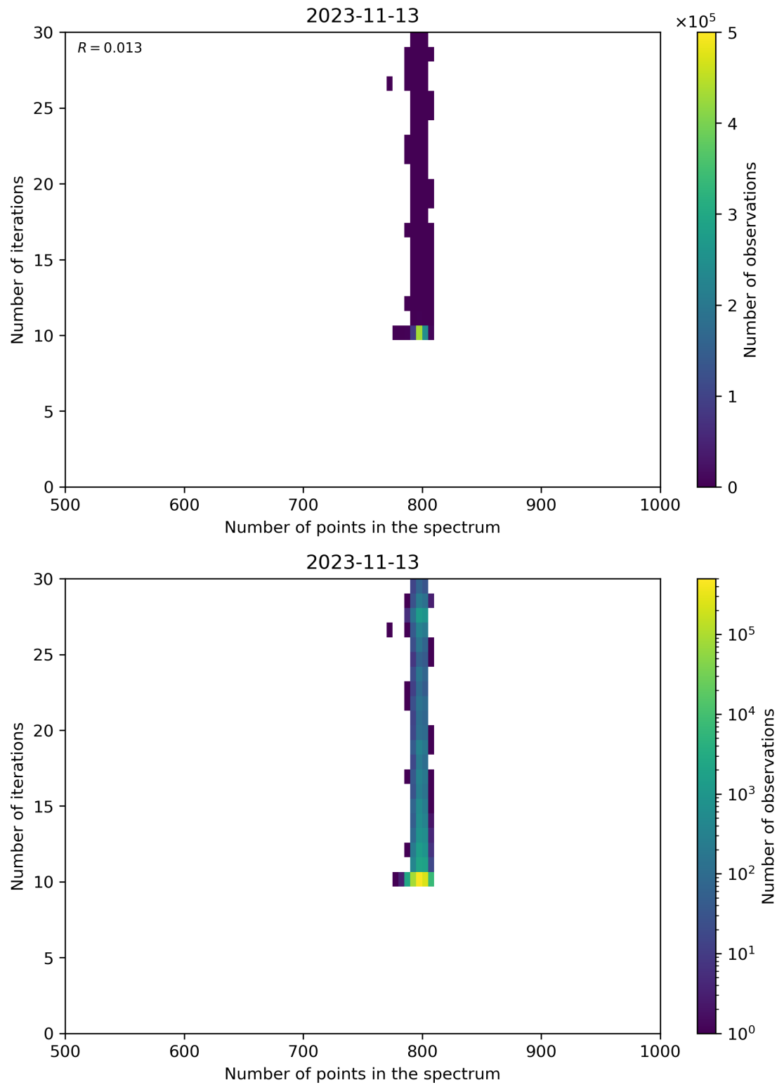
Figure 92: Scatter density plot of “Number of points in the spectrum” against “Number of iterations” for 2023-11-13 to 2023-11-14.
