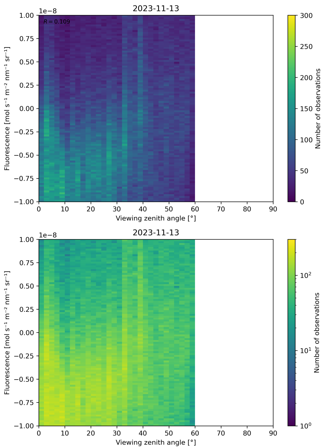
Figure 108: Scatter density plot of “Viewing zenith angle” against “Fluorescence” for 2023-11-13 to 2023-11-14.
