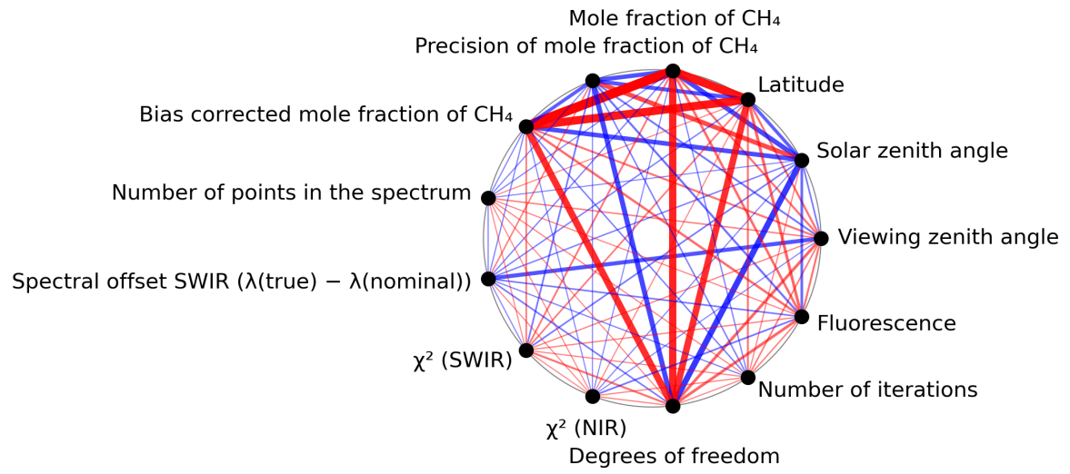
Figure 1: Map of correlation graph for 2023-11-13 to 2023-11-14.
