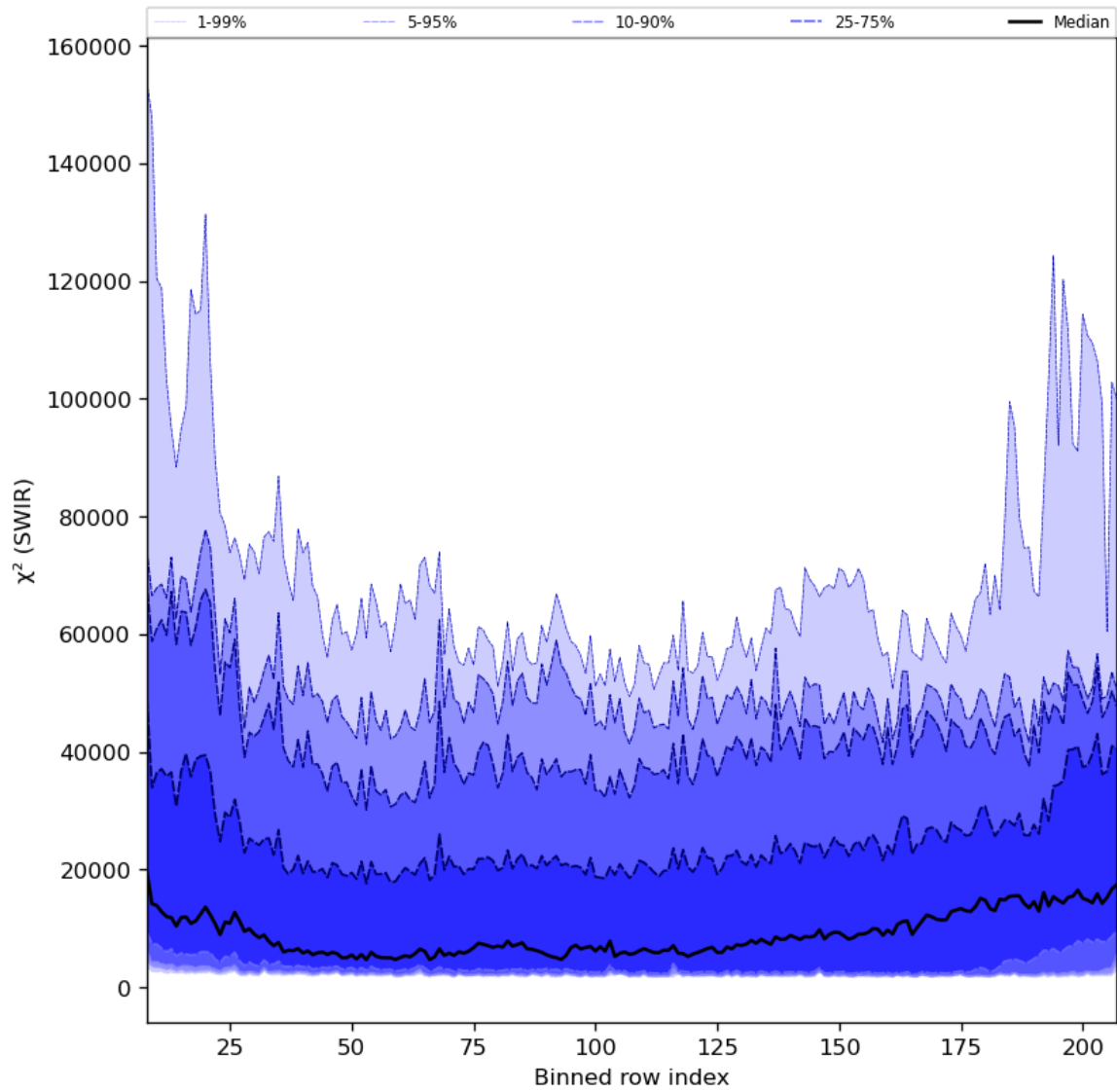
Figure 39: Along track statistics of “ \chi^2 (SWIR)” for 2023-11-13 to 2023-11-14
