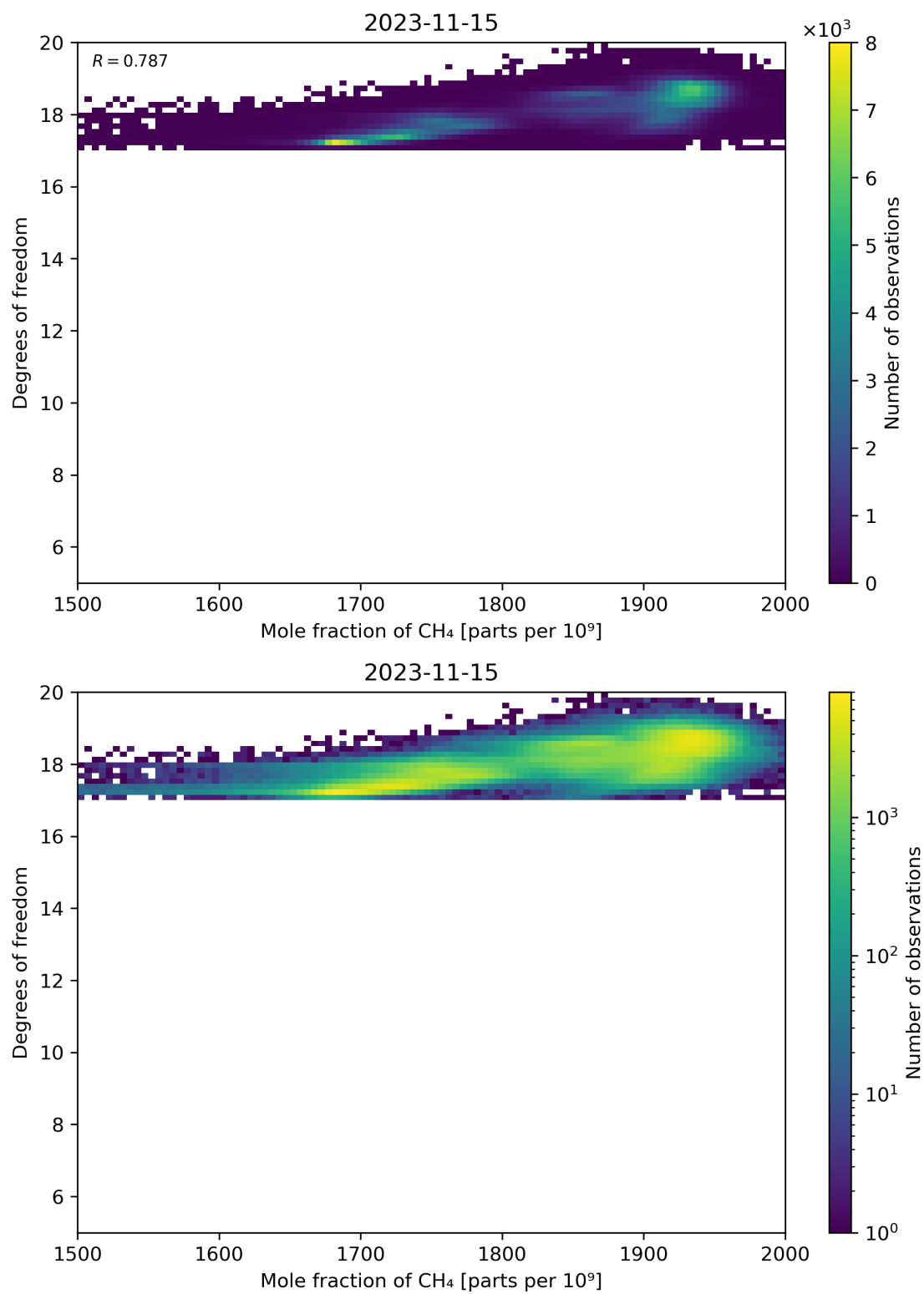
Figure 72: Scatter density plot of “Mole fraction of CH 4 ” against “Degrees of freedom” for 2023-11-14 to 2023-11-16.
