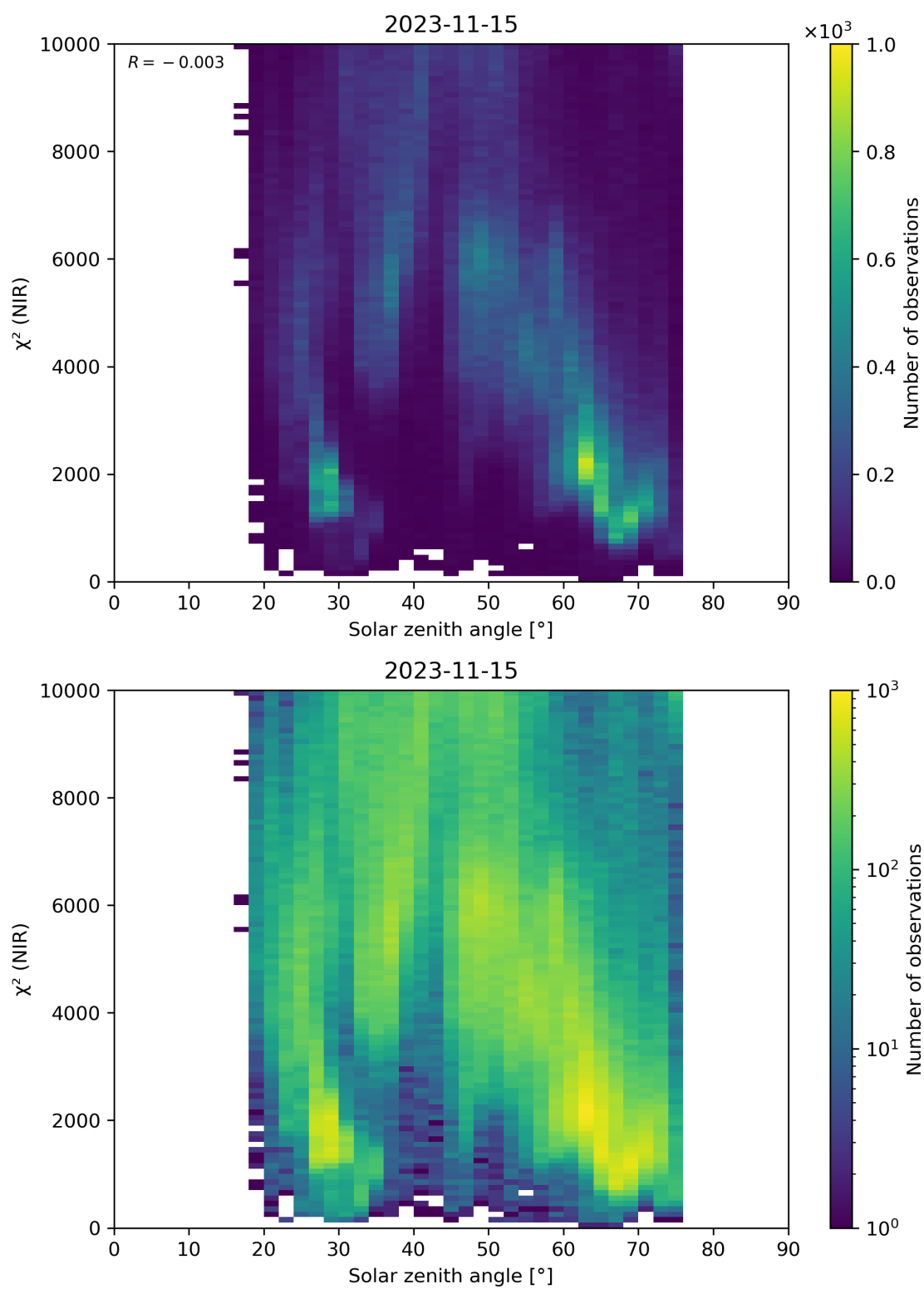
Figure 94: Scatter density plot of “Solar zenith angle” against “ \chi^2 (NIR)” for 2023-11-14 to 2023-11-16.
