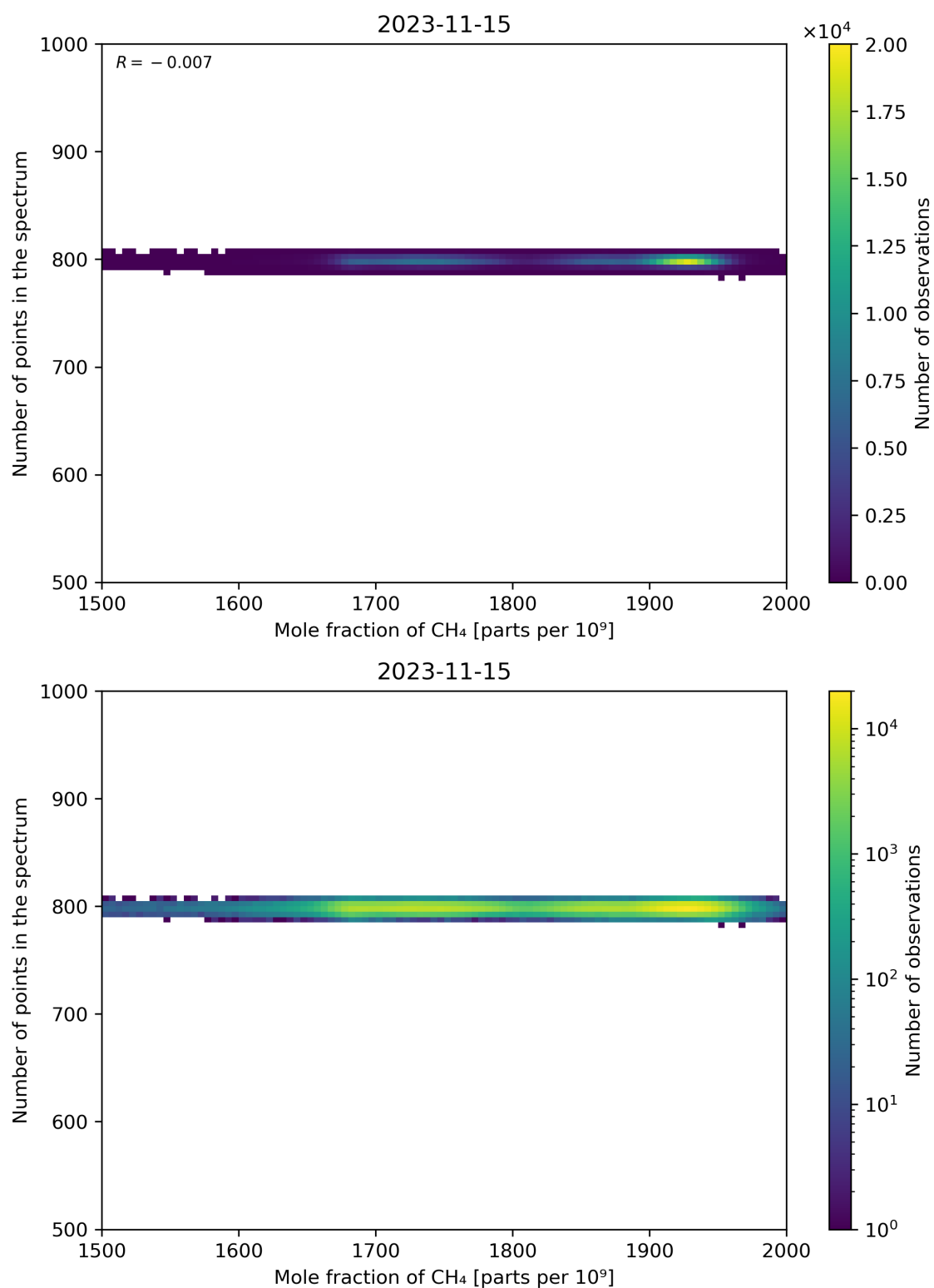
Figure 77: Scatter density plot of “Mole fraction of CH 4 ” against “Number of points in the spectrum” for 2023-11-14 to 2023-11-16.
