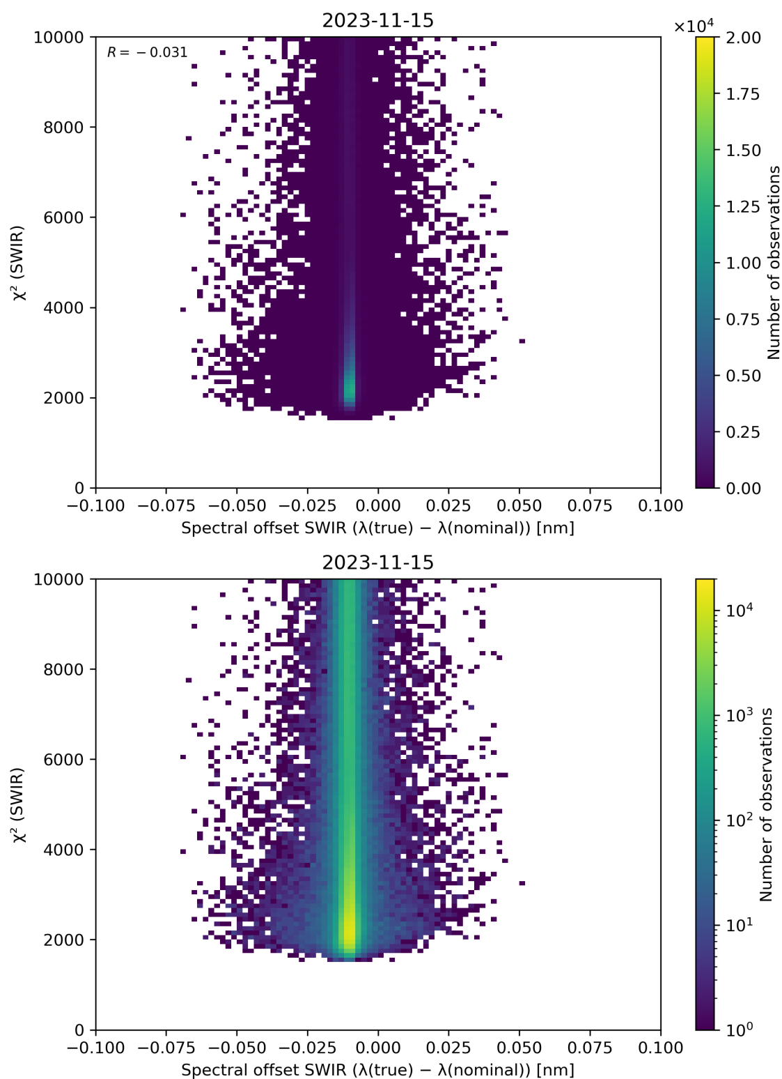
Figure 118: Scatter density plot of “Spectral offset SWIR ( \lambda(\text{true}) - \lambda(\text{nominal}) )” against “ \chi^2 (SWIR)” for 2023-11-14 to 2023-11-16.
