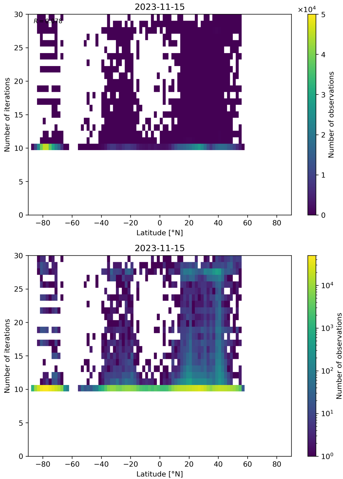
Figure 60: Scatter density plot of “Latitude” against “Number of iterations” for 2023-11-14 to 2023-11-16.
