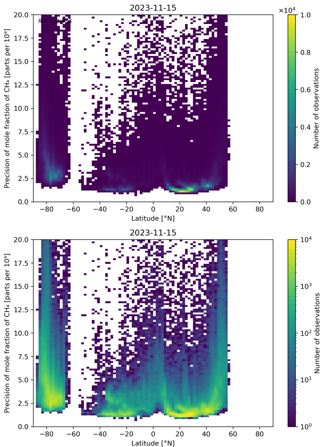
Figure 59: Scatter density plot of “Latitude” against “Precision of mole fraction of CH 4 ” for 2023-11-14 to 2023-11-16.
