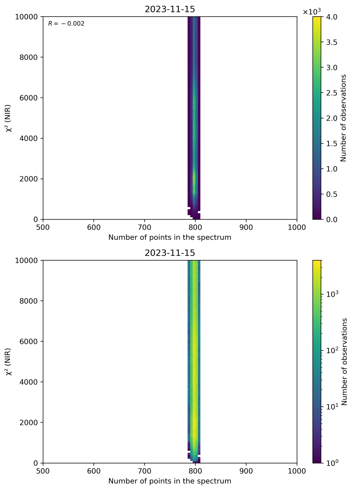
Figure 88: Scatter density plot of “Number of points in the spectrum” against “ \chi^2 (NIR)” for 2023-11-14 to 2023-11-16.
