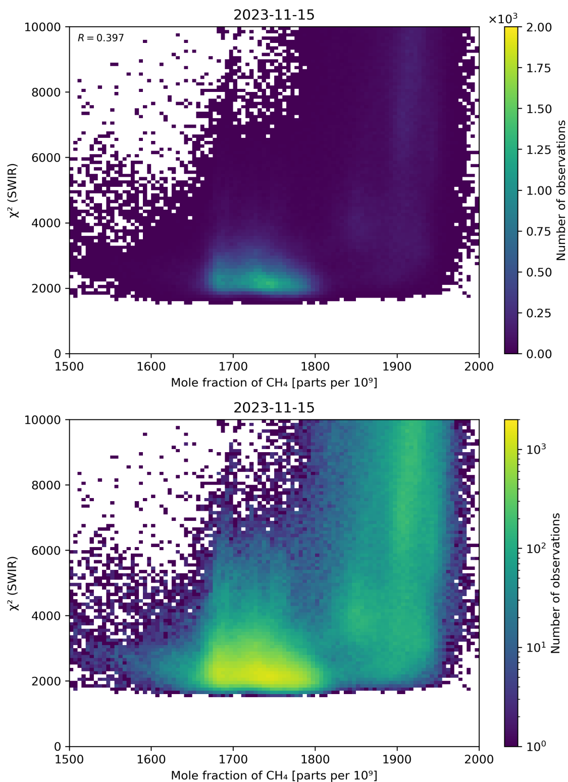
Figure 71: Scatter density plot of “Mole fraction of \text{CH}_4 ” against “ \chi^2 (SWIR)” for 2023-11-14 to 2023-11-16.
