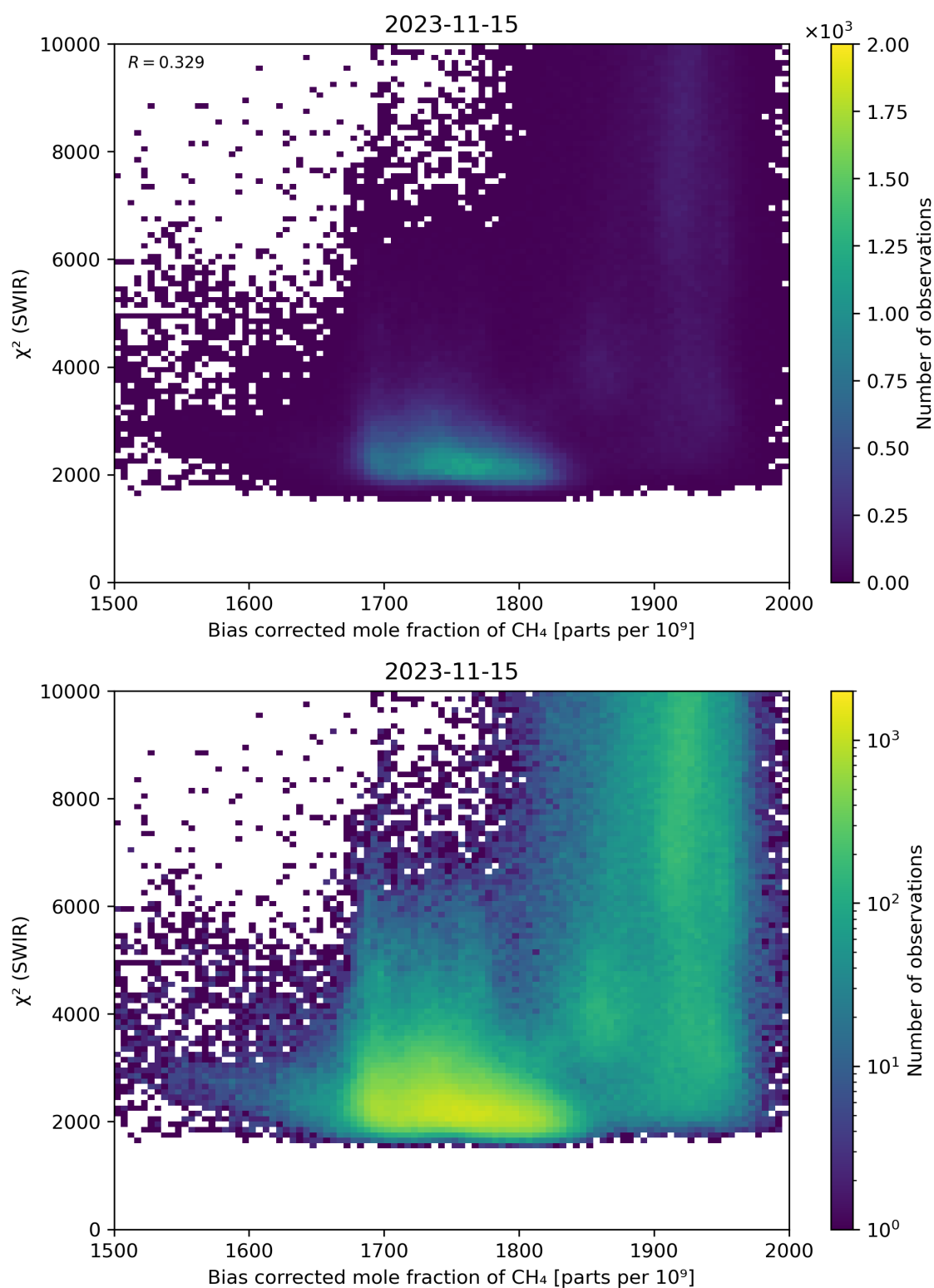
Figure 64: Scatter density plot of “Bias corrected mole fraction of CH 4 ” against “ \chi^2 (SWIR)” for 2023-11-14 to 2023-11-16.
