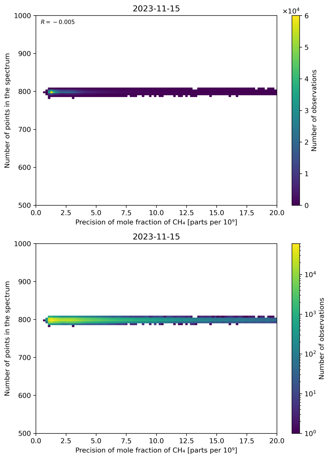
Figure 84: Scatter density plot of “Precision of mole fraction of CH 4 ” against “Number of points in the spectrum” for 2023-11-14 to 2023-11-16.
