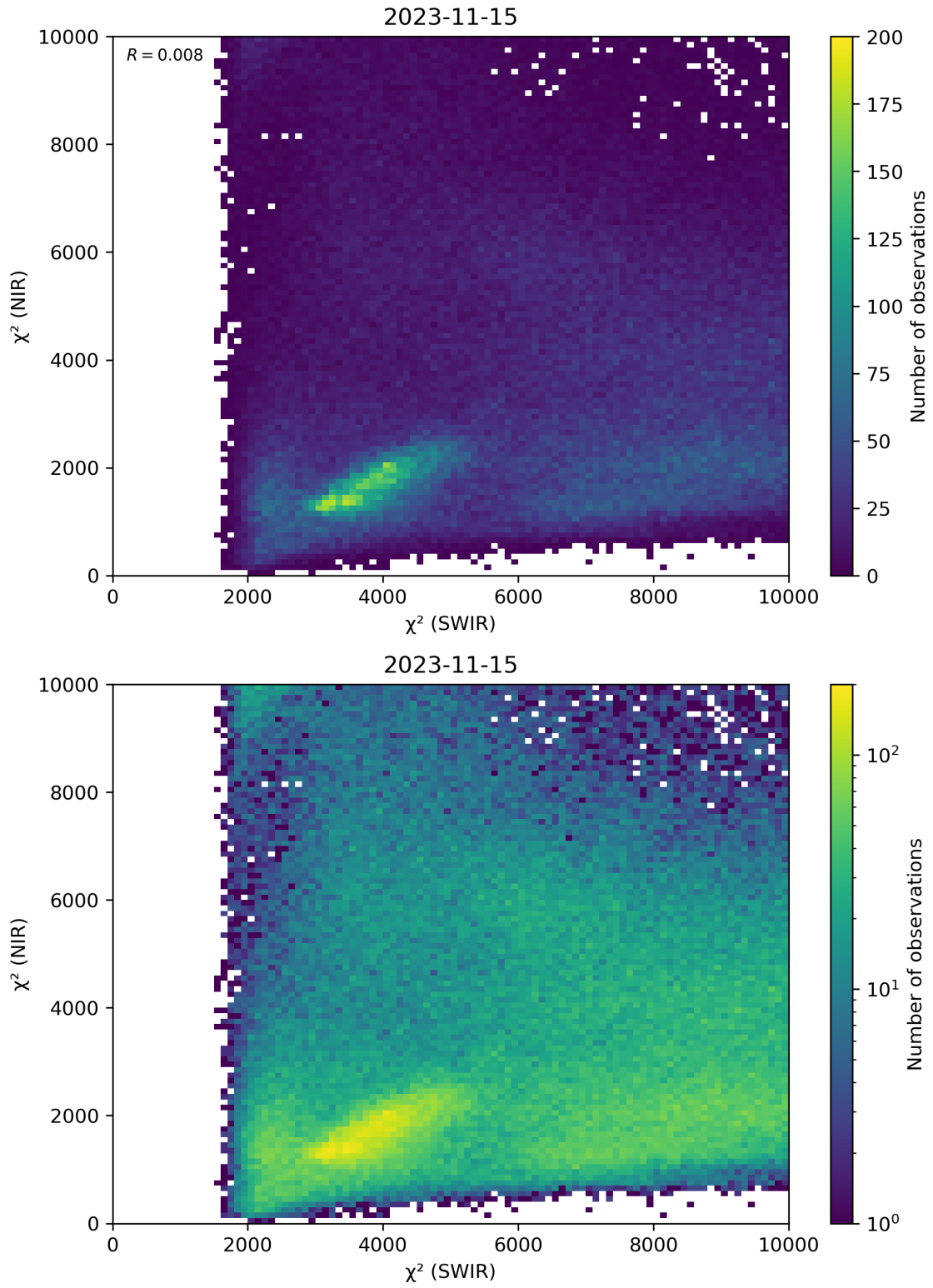
Figure 47: Scatter density plot of “ \chi^2 (SWIR)” against “ \chi^2 (NIR)” for 2023-11-14 to 2023-11-16.
