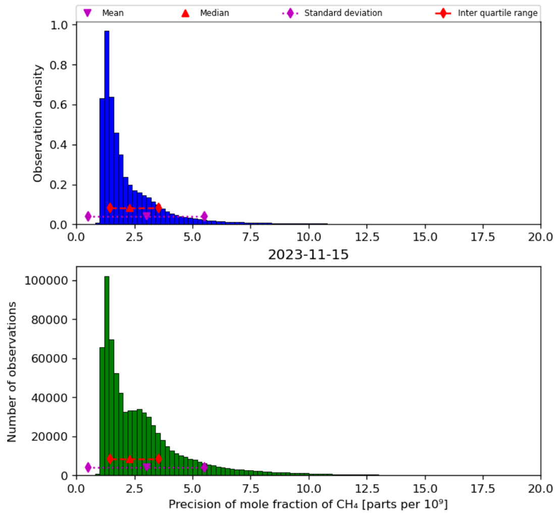
Figure 24: Histogram of “Precision of mole fraction of CH 4 ” for 2023-11-14 to 2023-11-16
