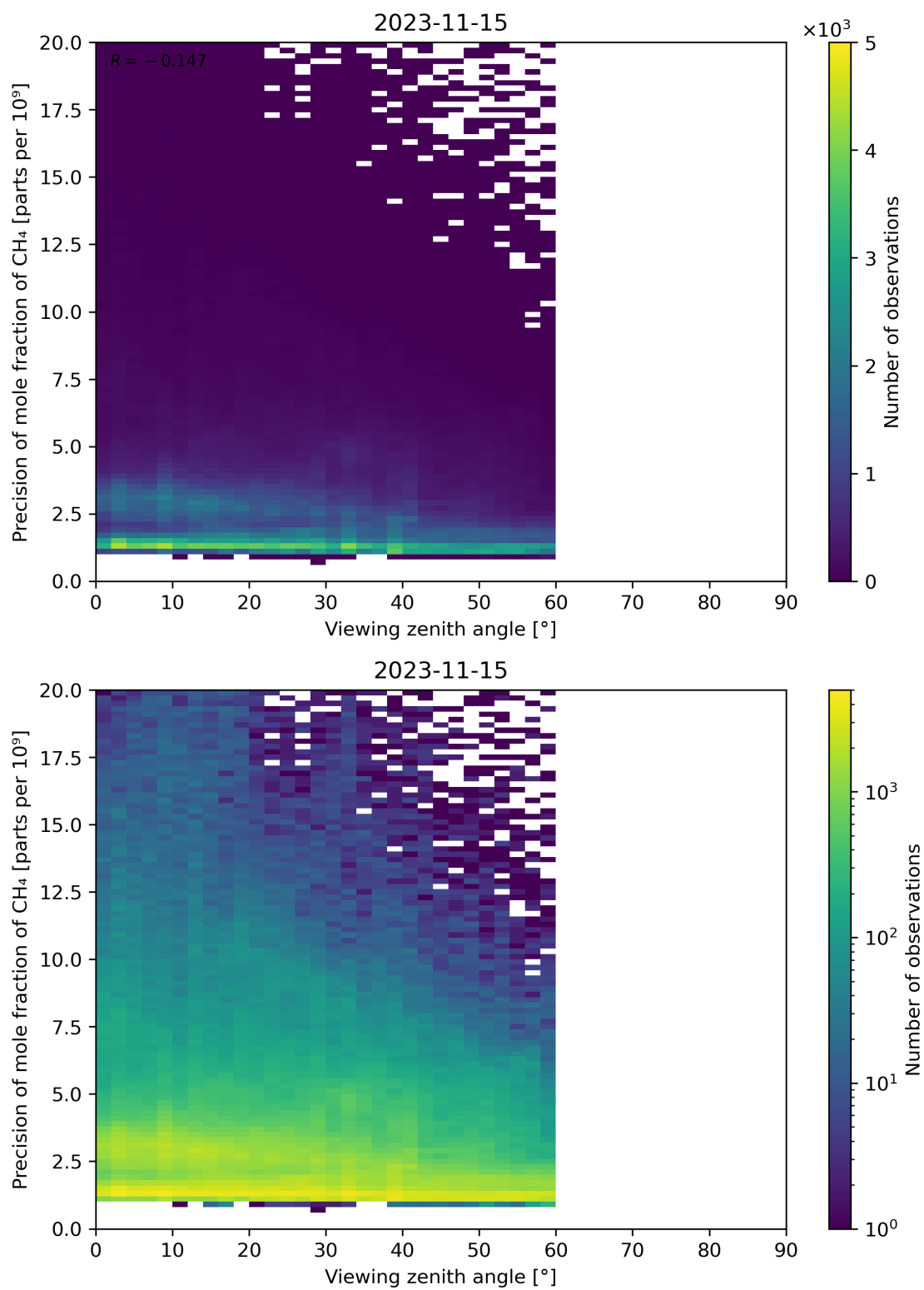
Figure 112: Scatter density plot of “Viewing zenith angle” against “Precision of mole fraction of CH 4 ” for 2023-11-14 to 2023-11-16.
