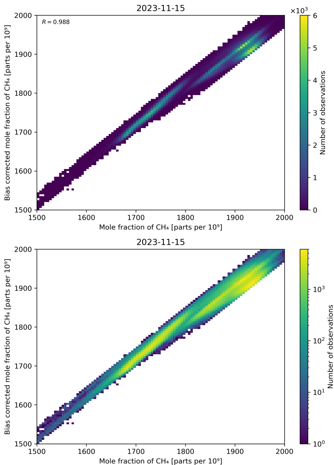
Figure 74: Scatter density plot of “Mole fraction of CH 4 ” against “Bias corrected mole fraction of CH 4 ” for 2023-11-14 to 2023-11-16.
