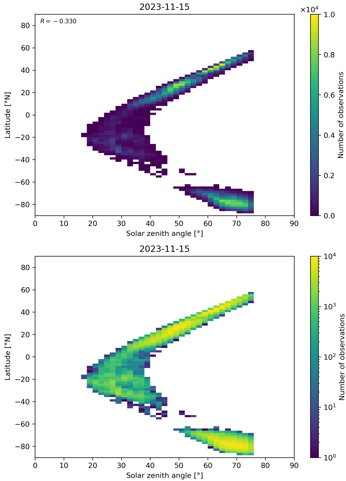
Figure 98: Scatter density plot of “Solar zenith angle” against “Latitude” for 2023-11-14 to 2023-11-16.
