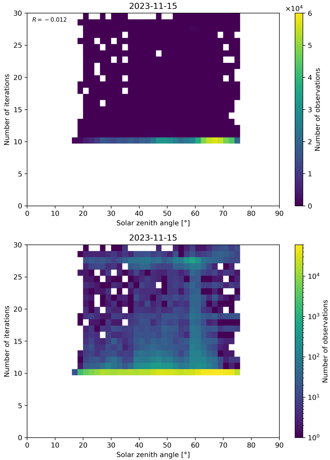
Figure 102: Scatter density plot of “Solar zenith angle” against “Number of iterations” for 2023-11-14 to 2023-11-16.
