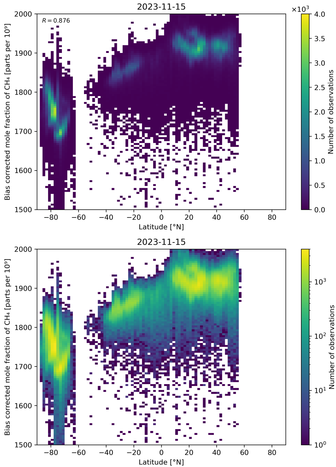
Figure 58: Scatter density plot of “Latitude” against “Bias corrected mole fraction of CH 4 ” for 2023-11-14 to 2023-11-16.
