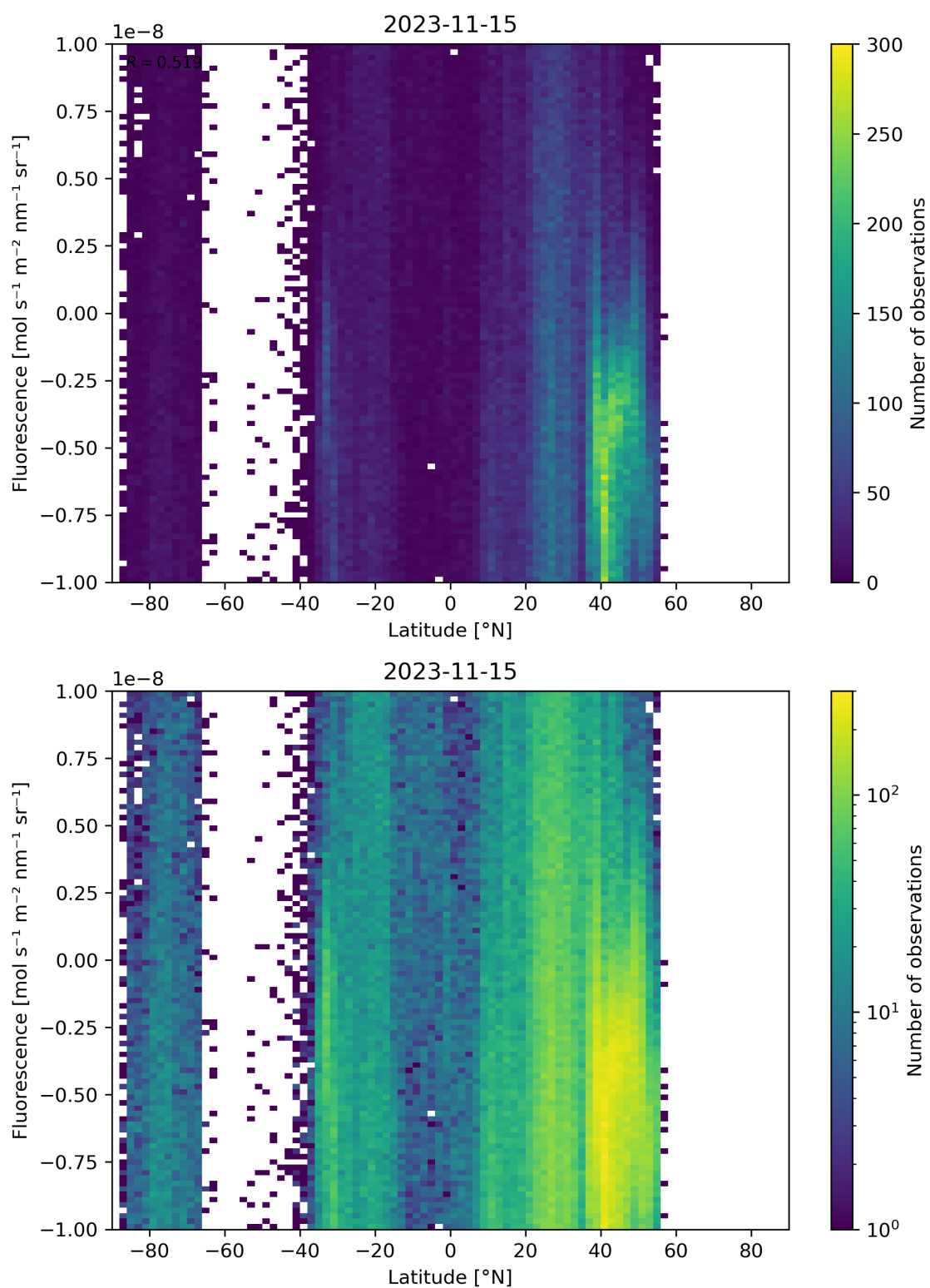
Figure 56: Scatter density plot of “Latitude” against “Fluorescence” for 2023-11-14 to 2023-11-16.
