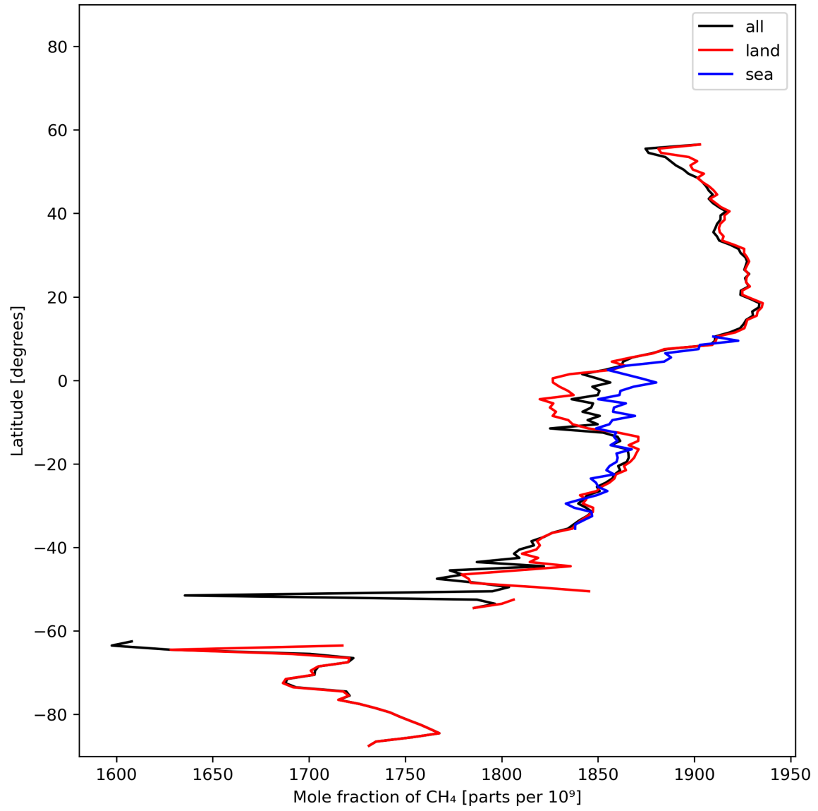
Figure 12: Zonal average of “Mole fraction of \text{CH}_4 ” for 2023-11-14 to 2023-11-16.
