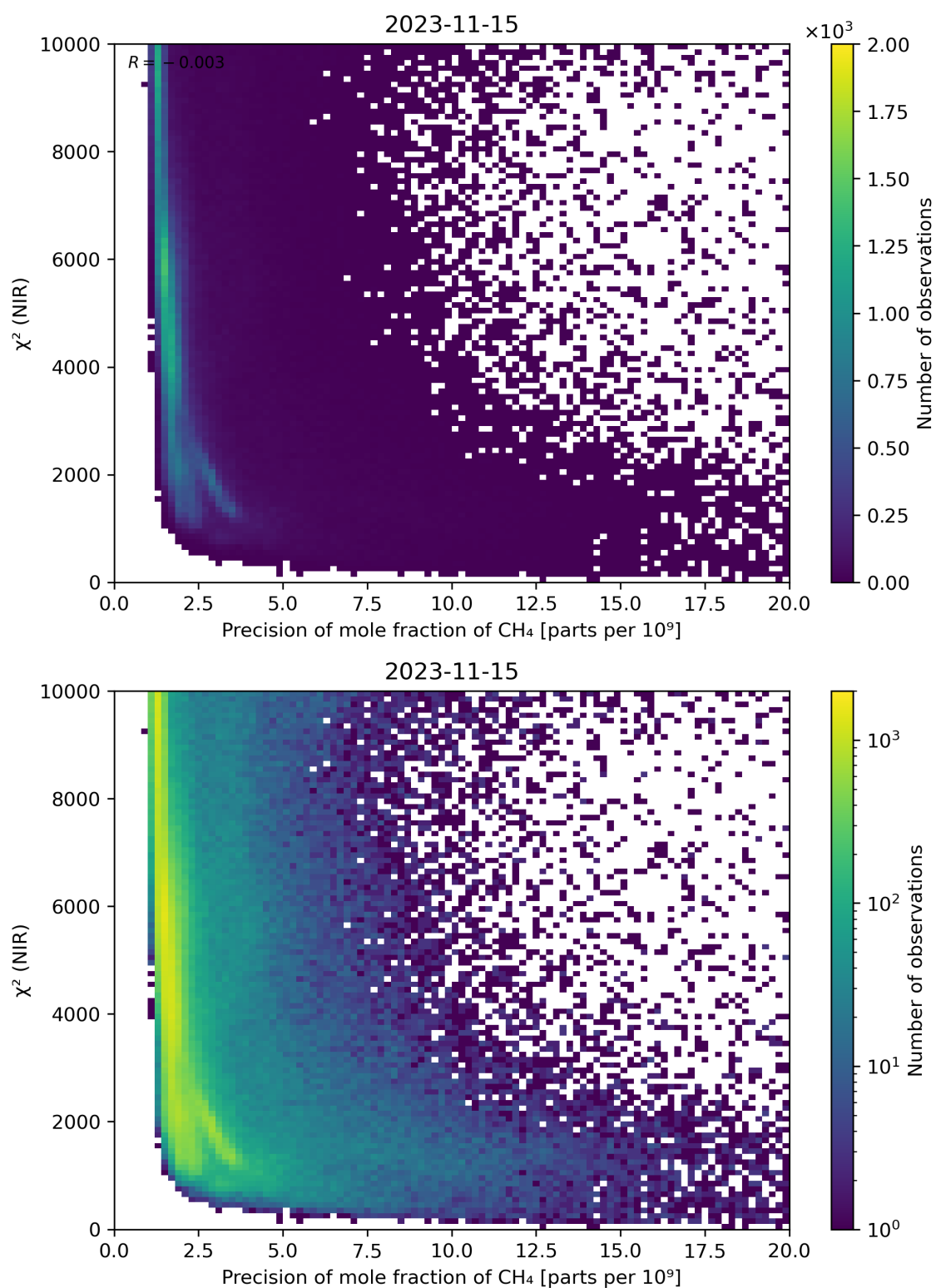
Figure 78: Scatter density plot of “Precision of mole fraction of CH 4 ” against “ \chi^2 (NIR)” for 2023-11-14 to 2023-11-16.
