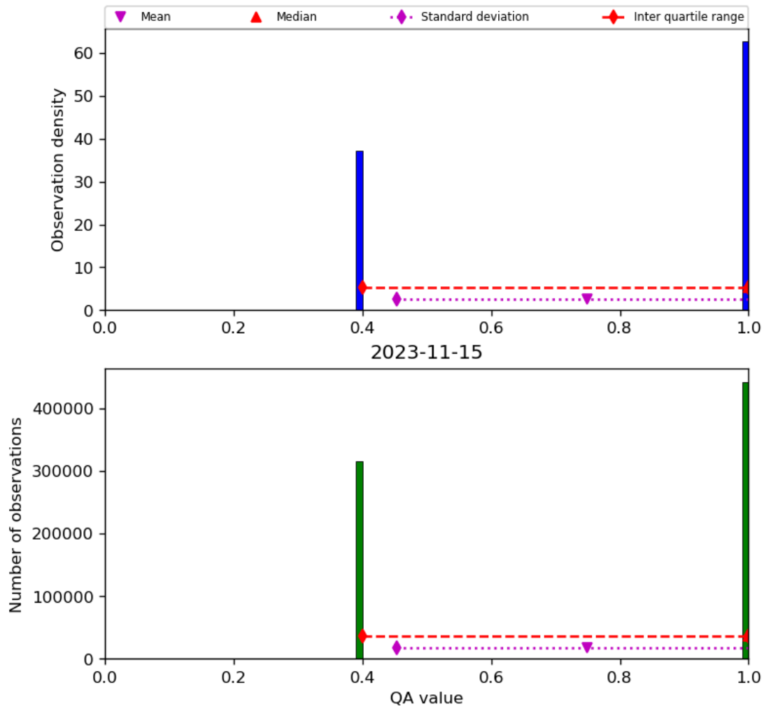
Figure 22: Histogram of “QA value” for 2023-11-14 to 2023-11-16
