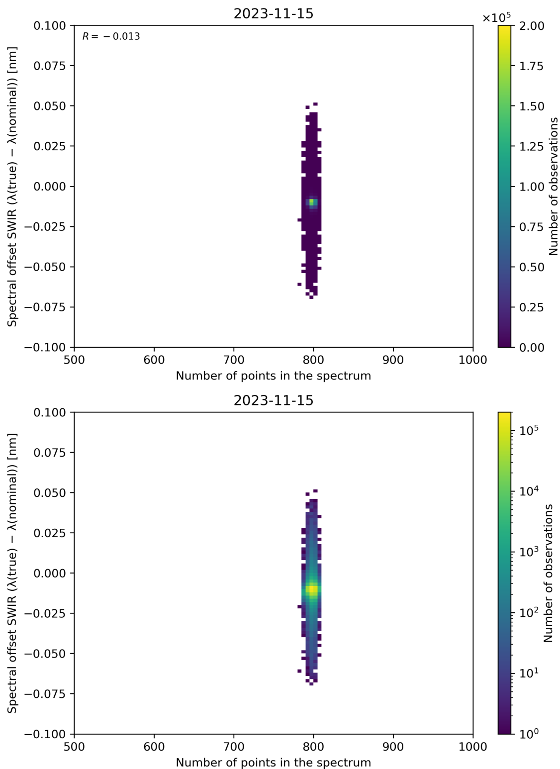
Figure 93: Scatter density plot of “Number of points in the spectrum” against “Spectral offset SWIR ( \lambda(\text{true}) - \lambda(\text{nominal}) )” for 2023-11-14 to 2023-11-16.
