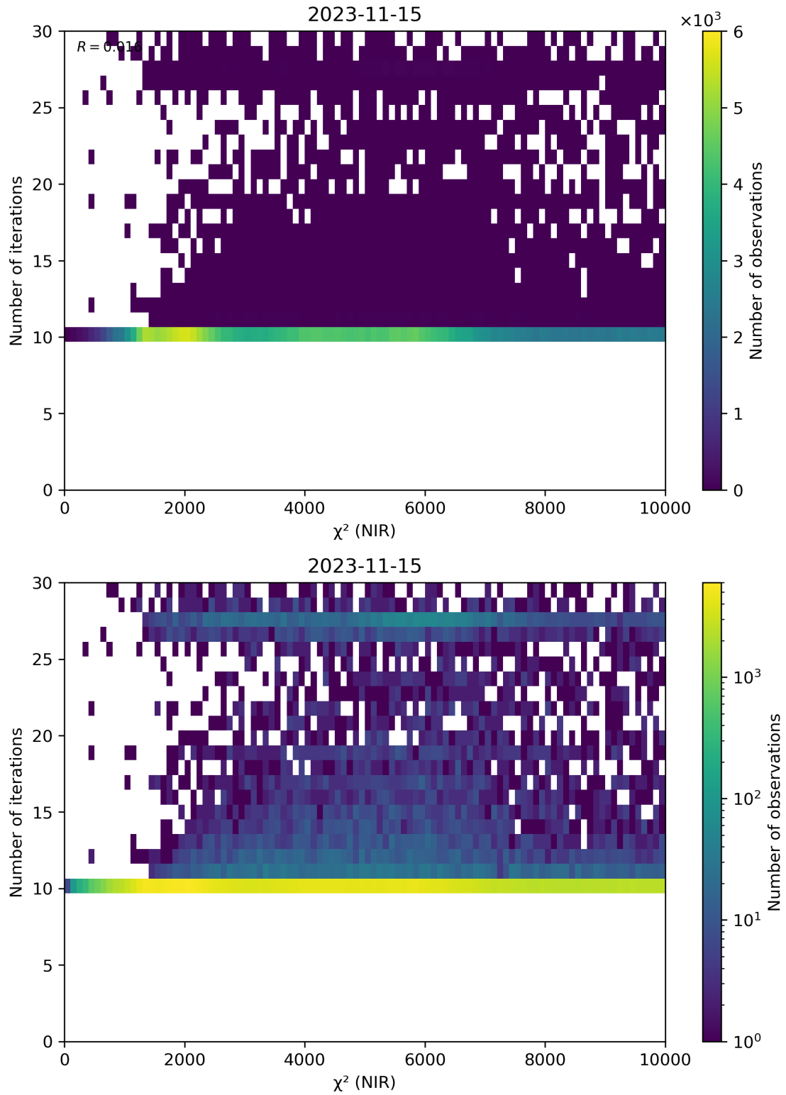
Figure 46: Scatter density plot of “ \chi^2 (NIR)” against “Number of iterations” for 2023-11-14 to 2023-11-16.
