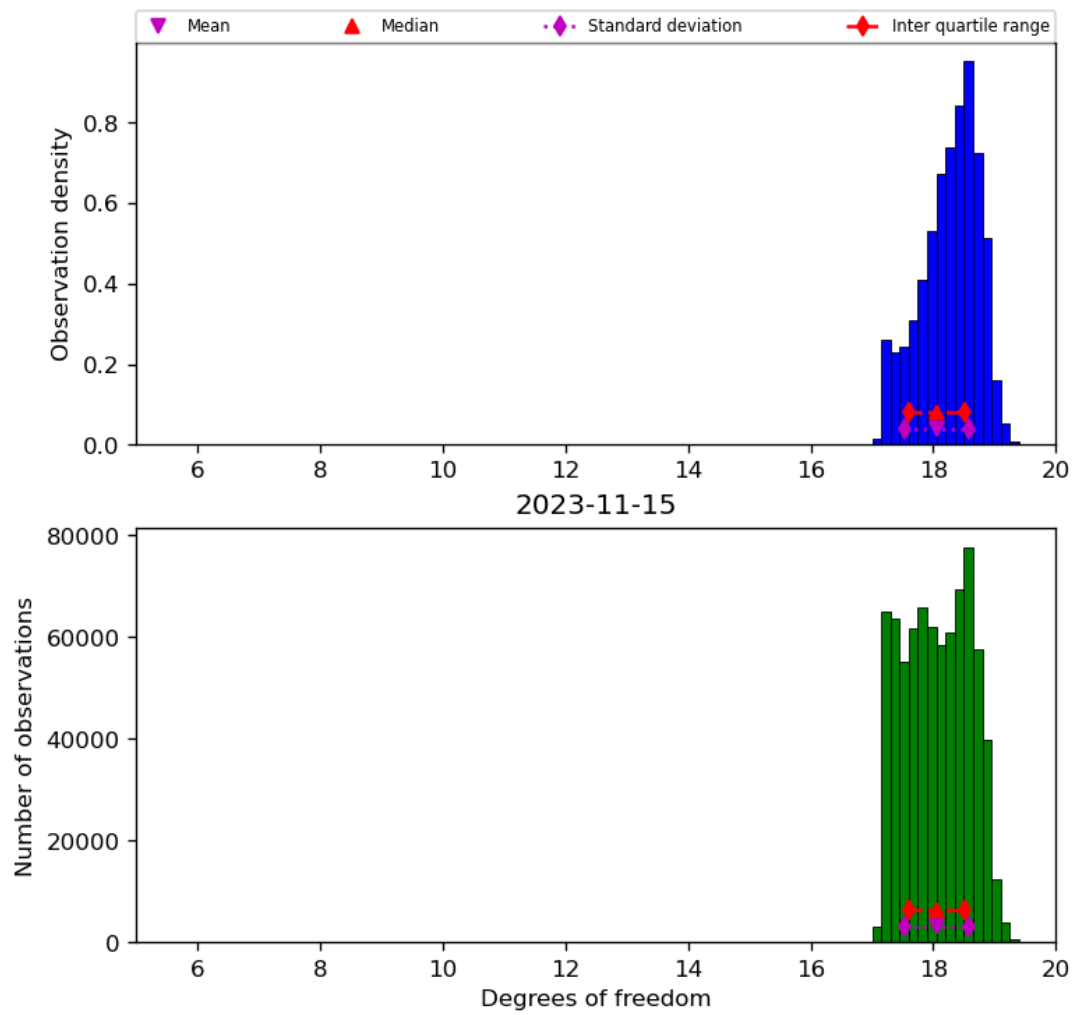
Figure 30: Histogram of "Degrees of freedom" for 2023-11-14 to 2023-11-16
