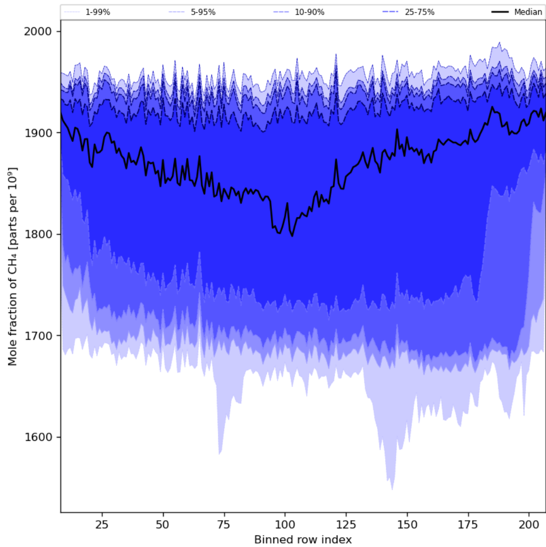
Figure 34: Along track statistics of “Mole fraction of CH 4 ” for 2023-11-14 to 2023-11-16
