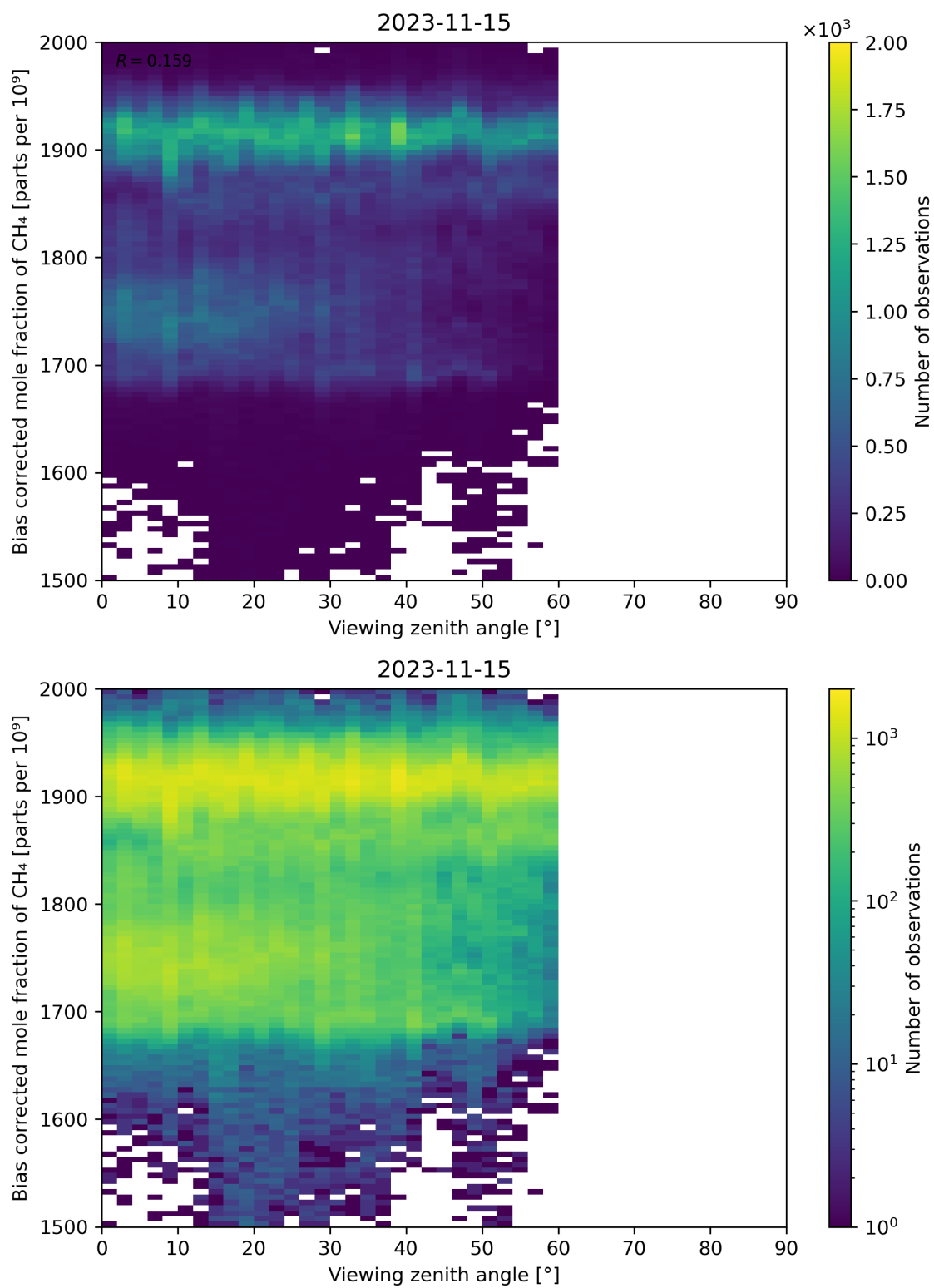
Figure 111: Scatter density plot of “Viewing zenith angle” against “Bias corrected mole fraction of CH 4 ” for 2023-11-14 to 2023-11-16.
