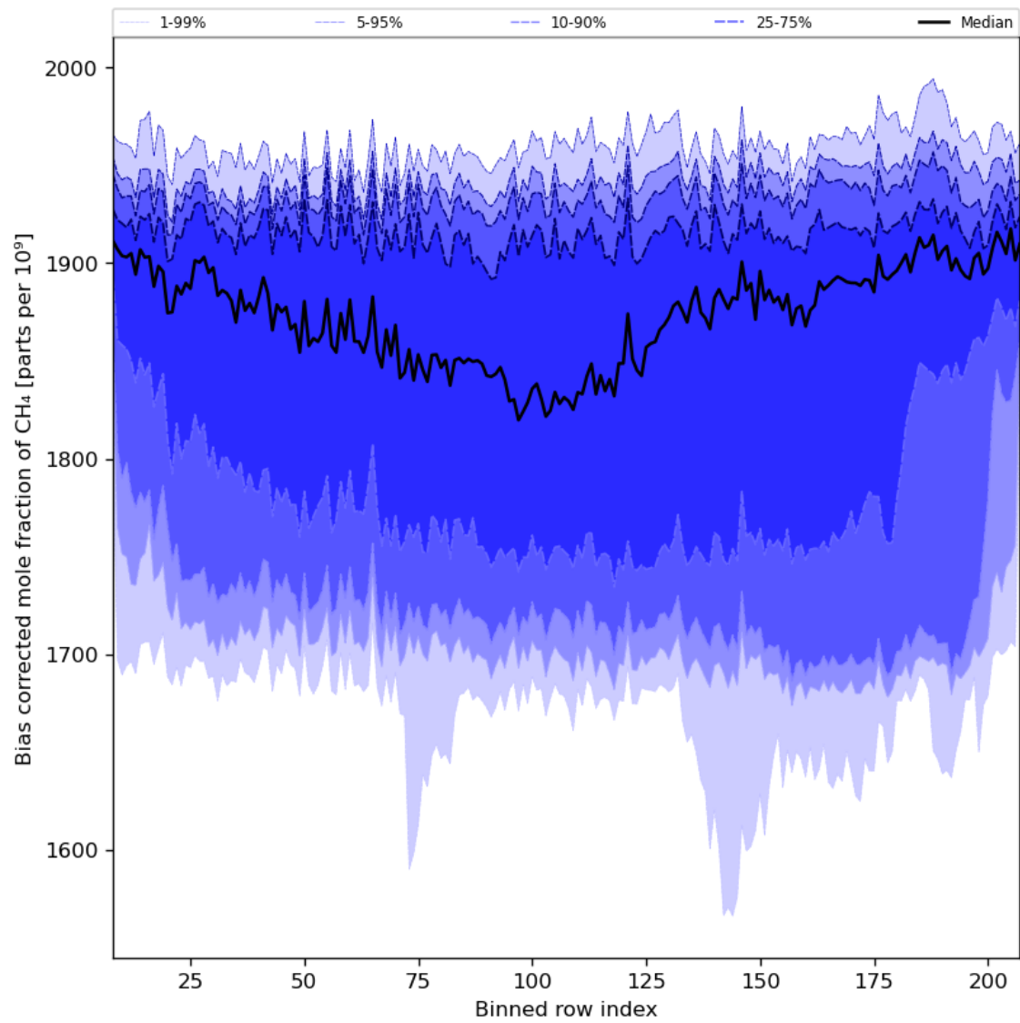
Figure 36: Along track statistics of “Bias corrected mole fraction of CH 4 ” for 2023-11-14 to 2023-11-16
