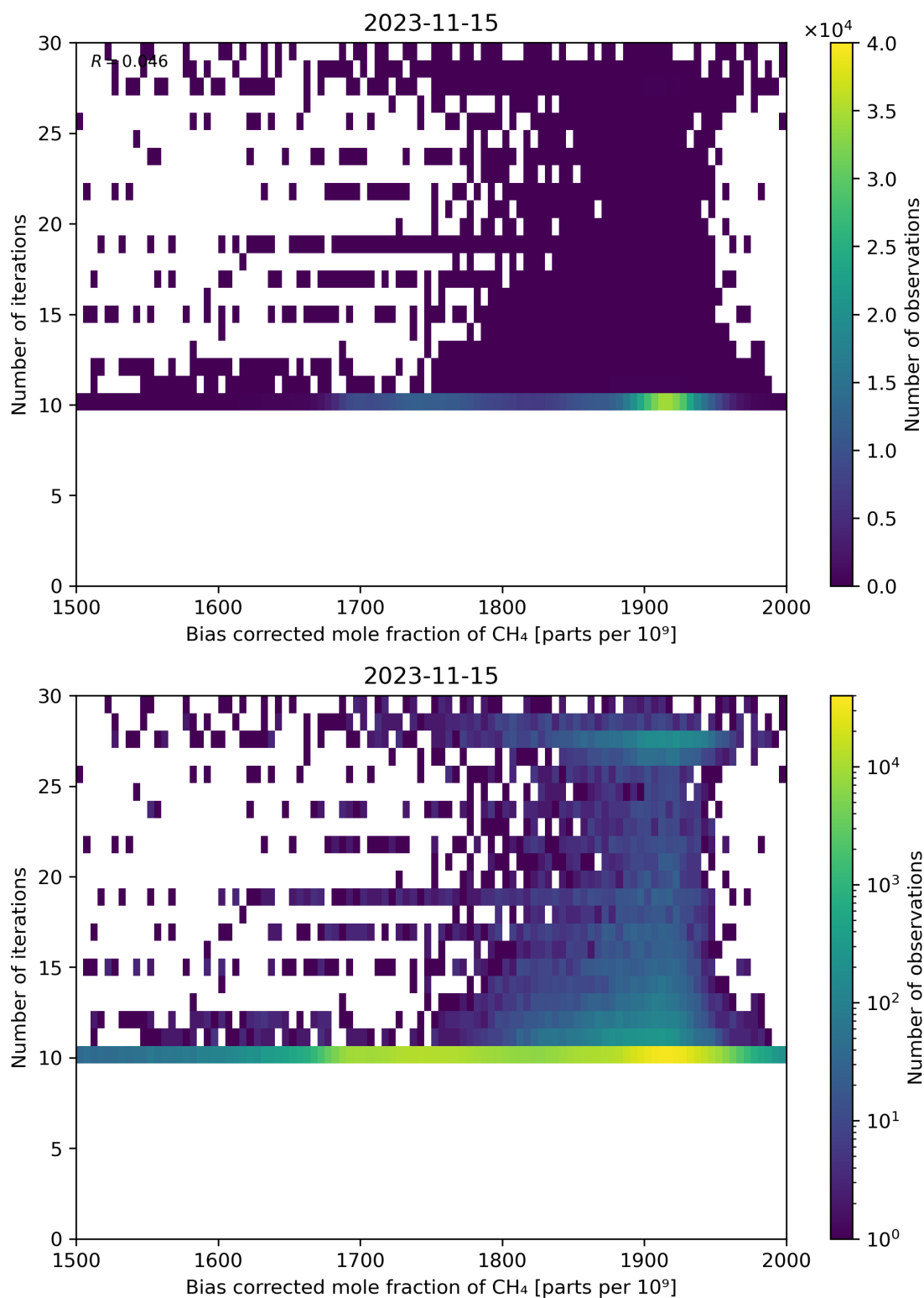
Figure 67: Scatter density plot of “Bias corrected mole fraction of \text{CH}_4 ” against “Number of iterations” for 2023-11-14 to 2023-11-16.
