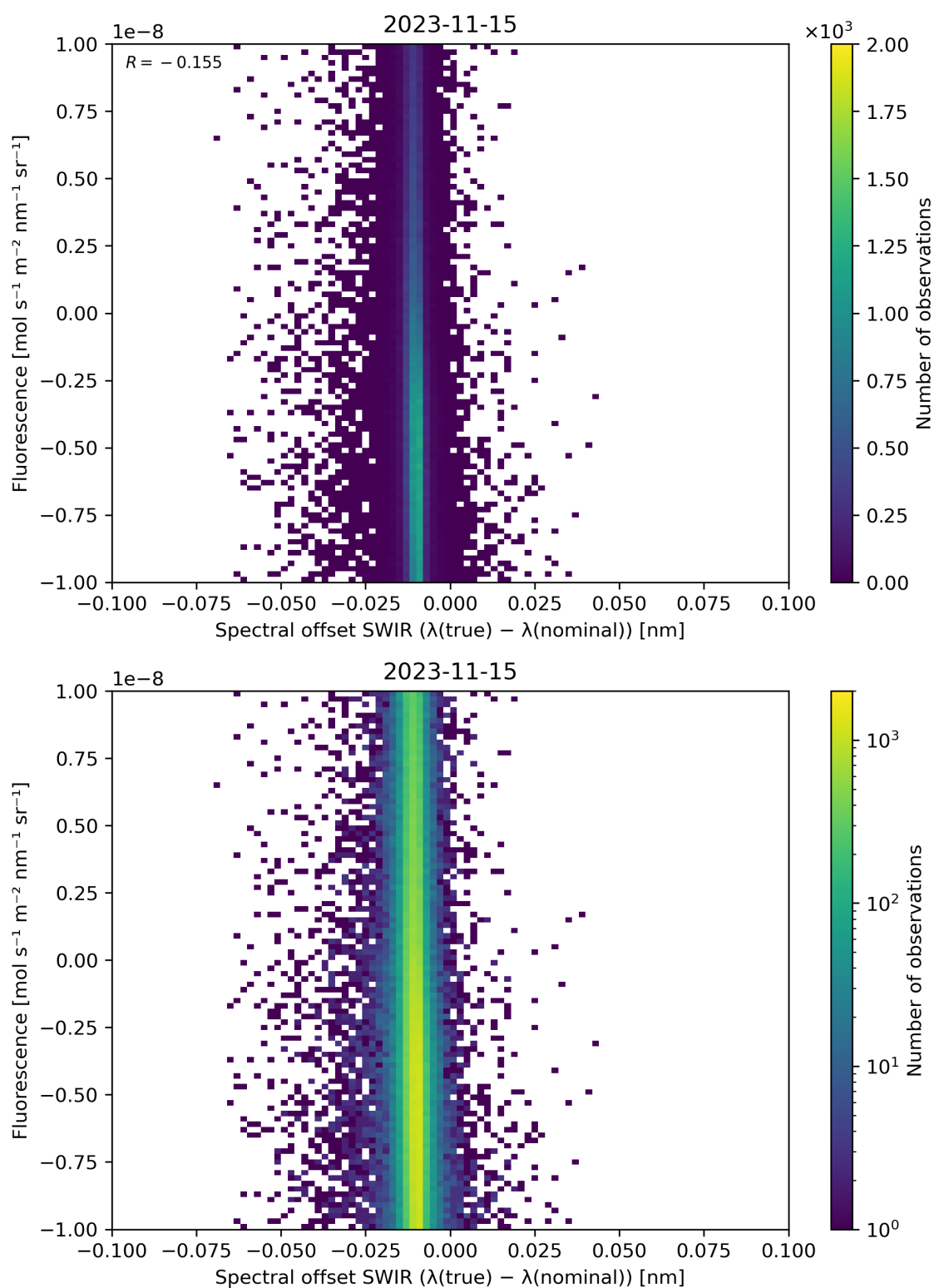
Figure 120: Scatter density plot of “Spectral offset SWIR ( \lambda(\text{true}) - \lambda(\text{nominal}) )” against “Fluorescence” for 2023-11-14 to 2023-11-16.
