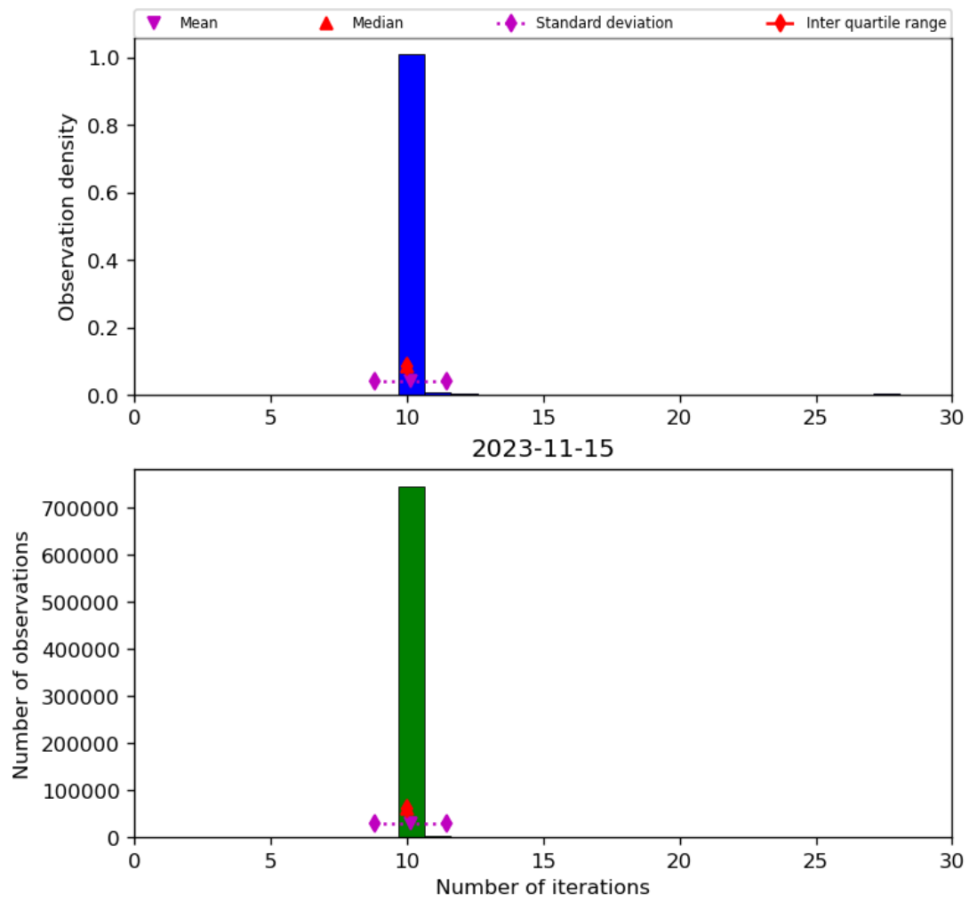
Figure 31: Histogram of “Number of iterations” for 2023-11-14 to 2023-11-16
