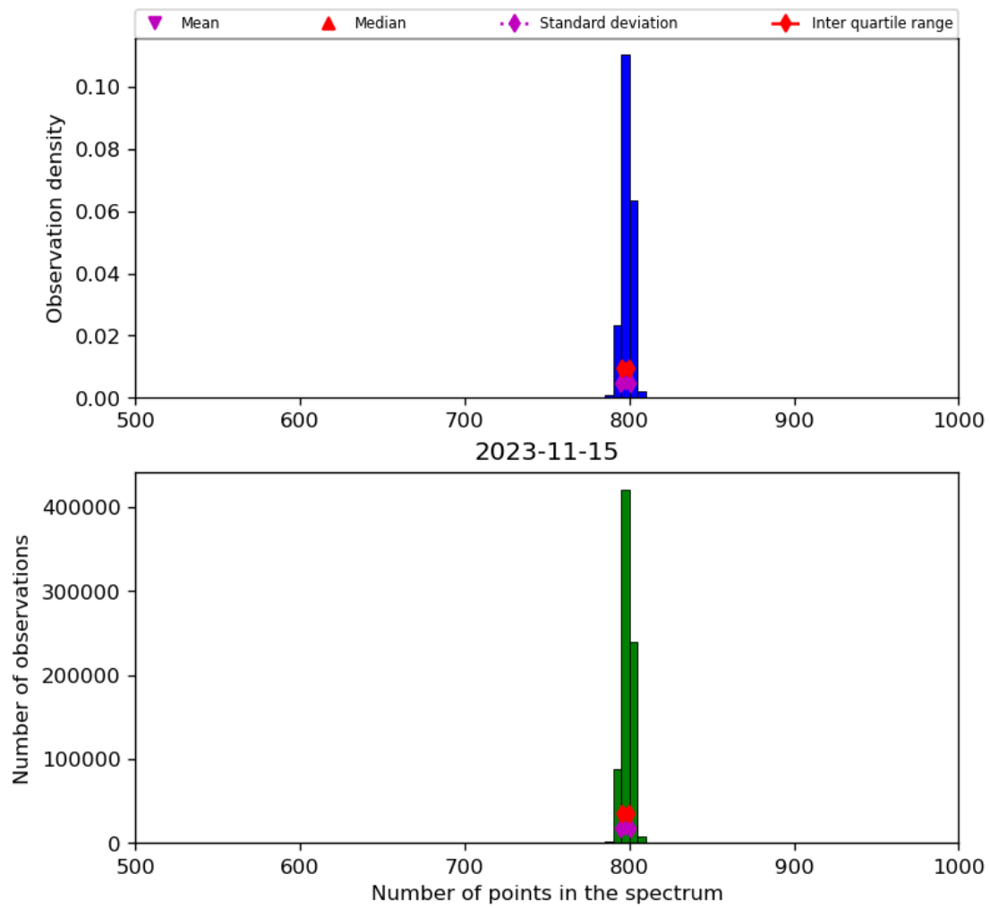
Figure 26: Histogram of “Number of points in the spectrum” for 2023-11-14 to 2023-11-16
