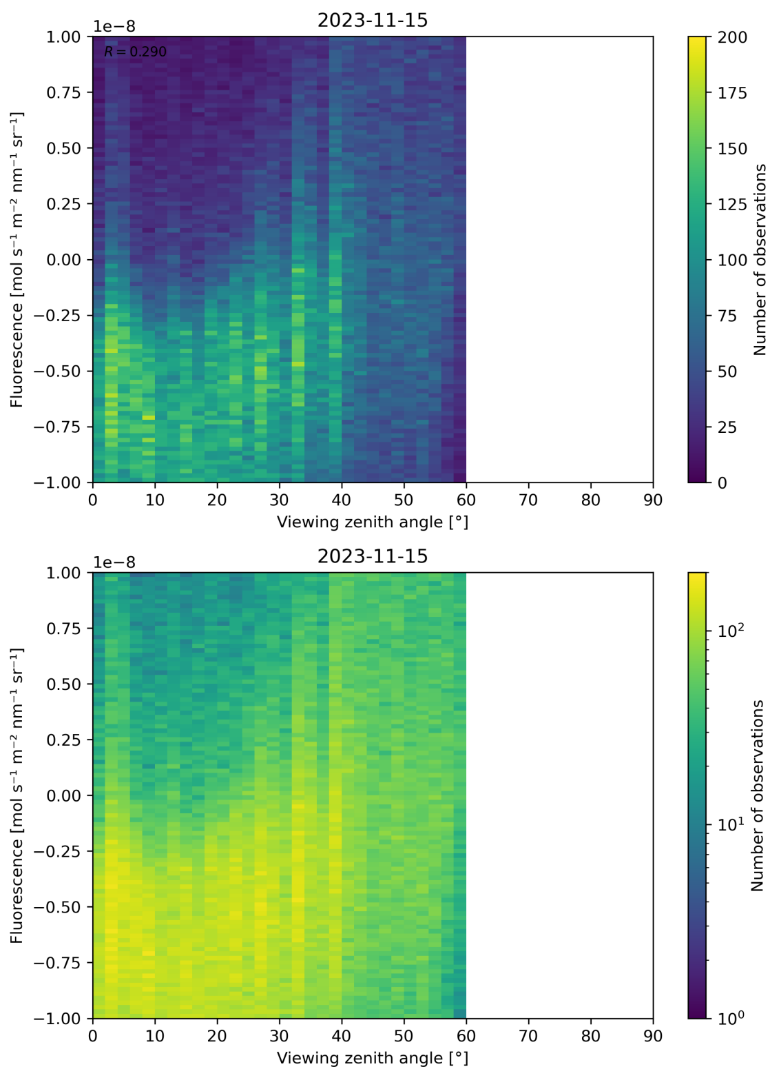
Figure 108: Scatter density plot of “Viewing zenith angle” against “Fluorescence” for 2023-11-14 to 2023-11-16.
