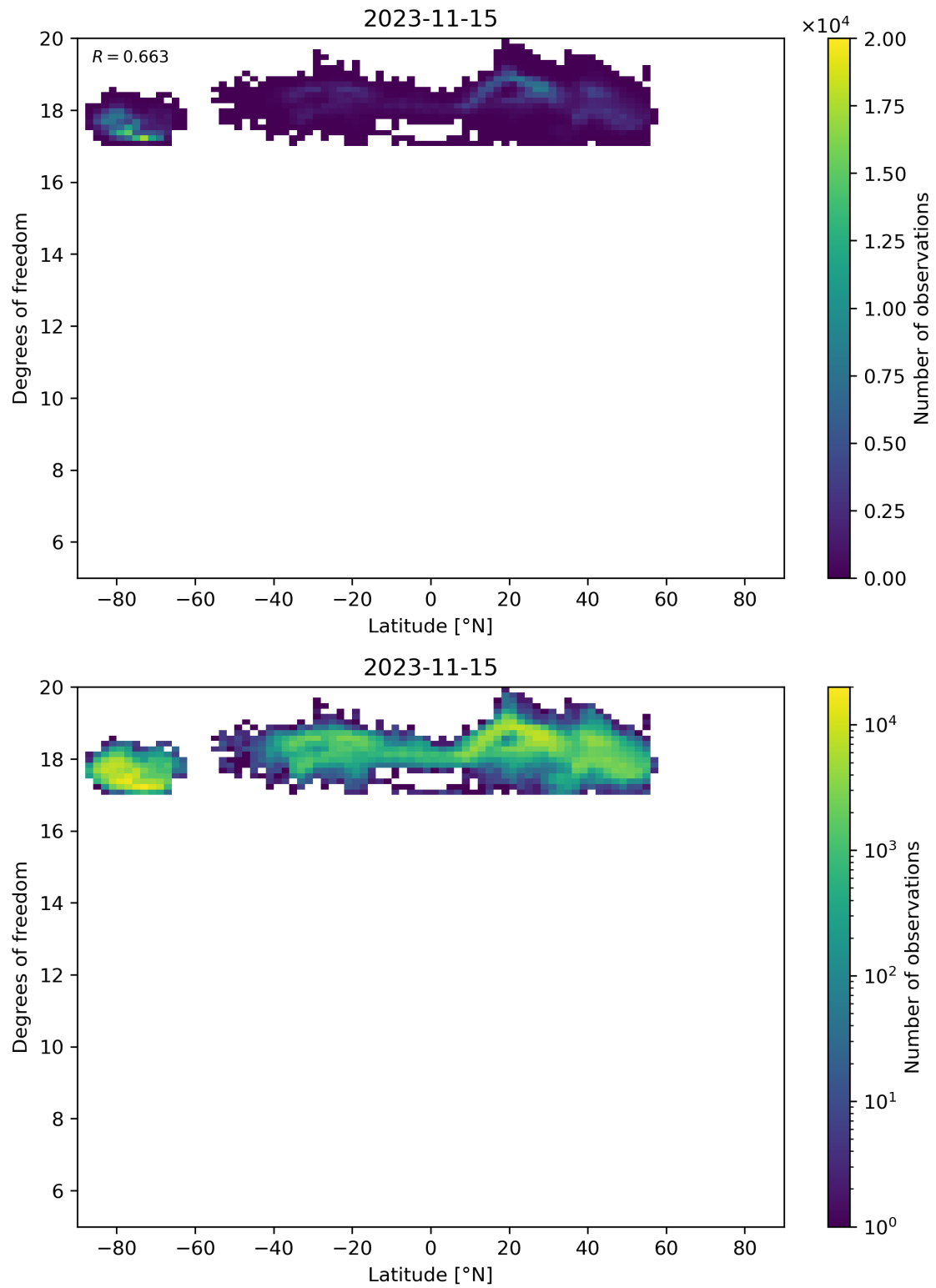
Figure 55: Scatter density plot of “Latitude” against “Degrees of freedom” for 2023-11-14 to 2023-11-16.
