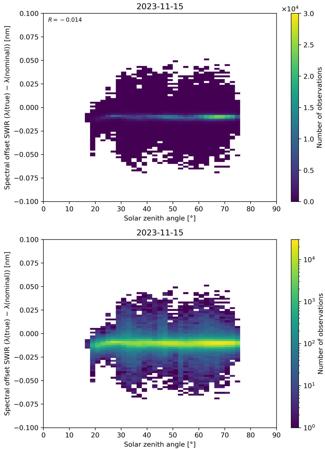
Figure 104: Scatter density plot of “Solar zenith angle” against “Spectral offset SWIR ( \lambda(\text{true}) - \lambda(\text{nominal}) )” for 2023-11-14 to 2023-11-16.
