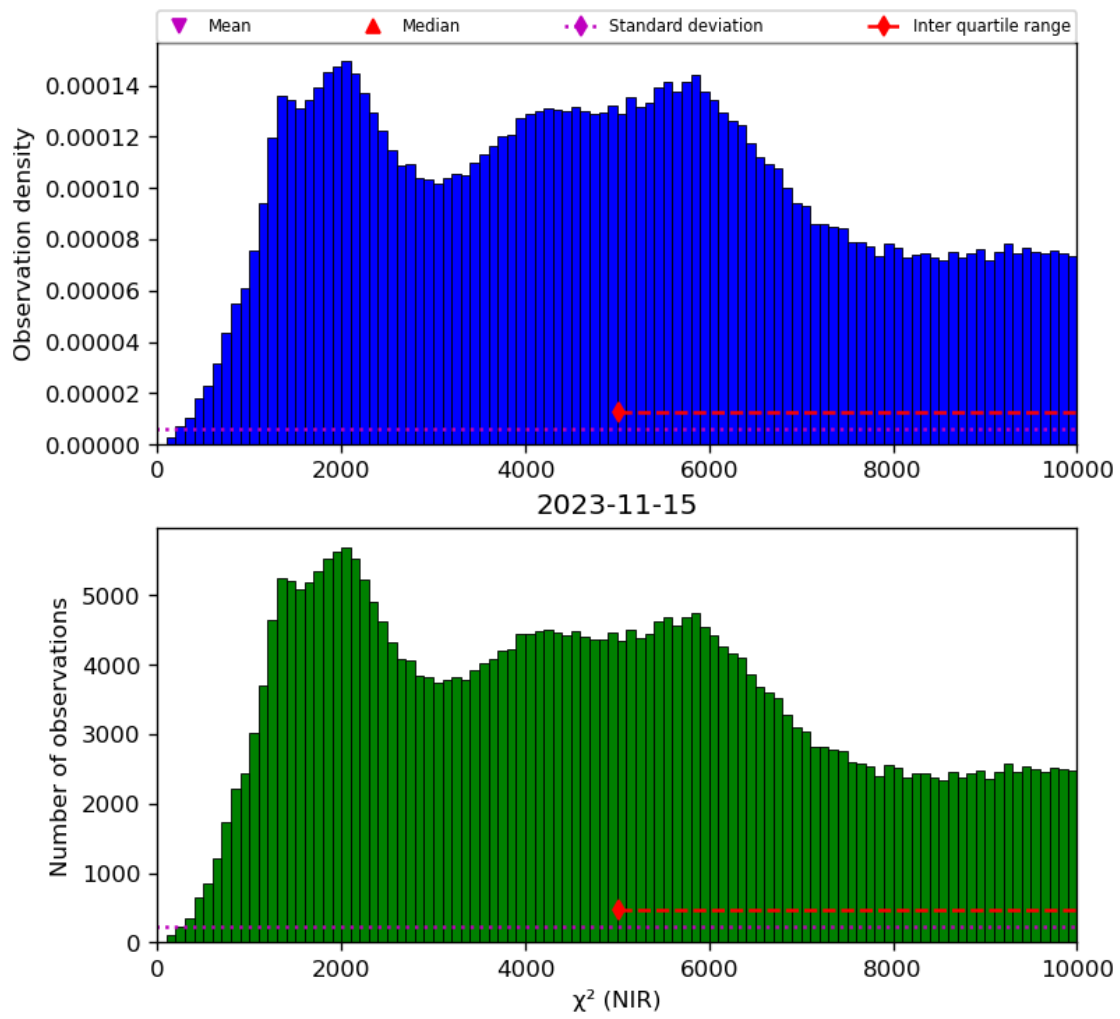
Figure 29: Histogram of “ \chi^2 (NIR)” for 2023-11-14 to 2023-11-16
