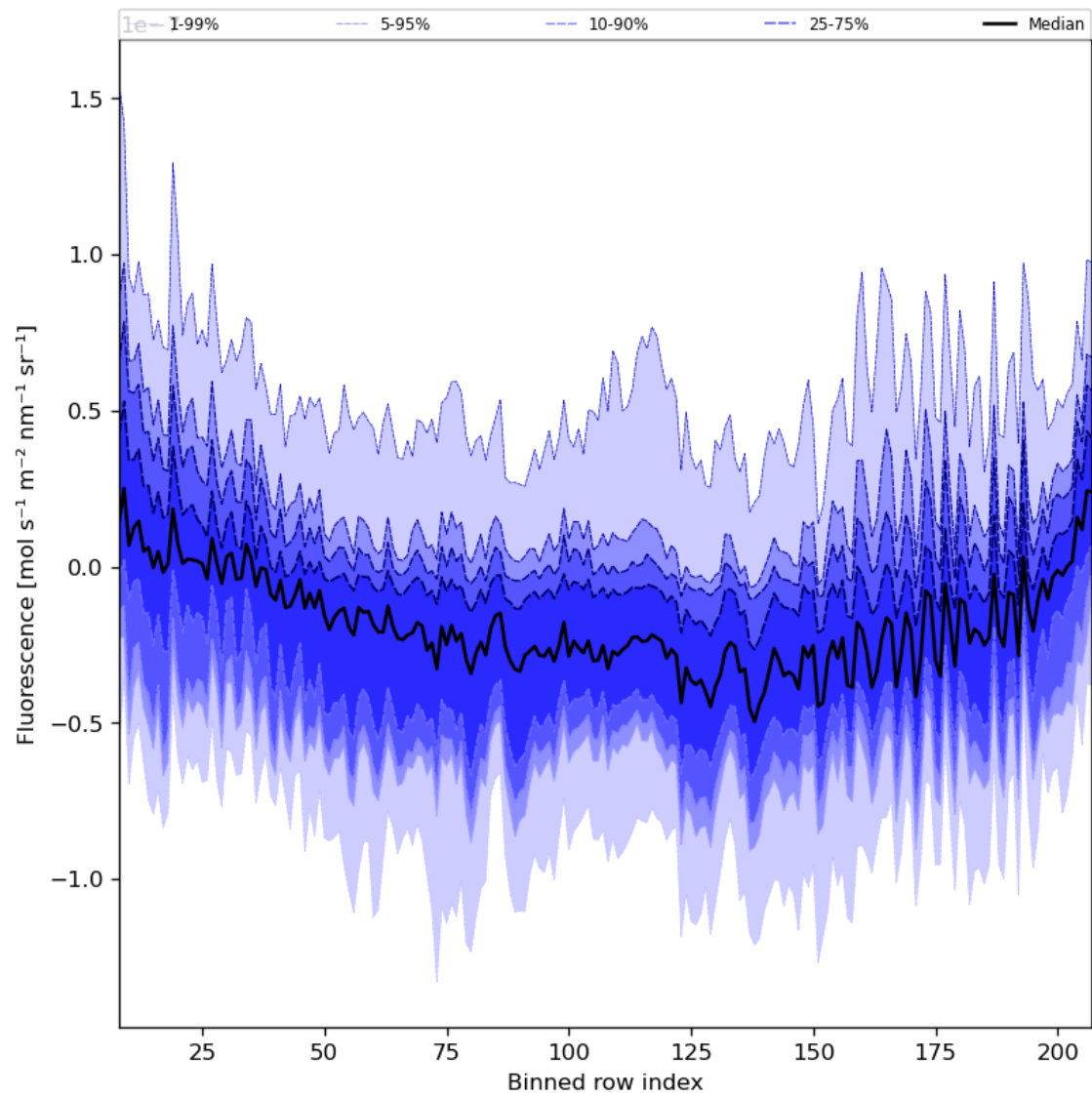
Figure 43: Along track statistics of “Fluorescence” for 2023-11-14 to 2023-11-16
