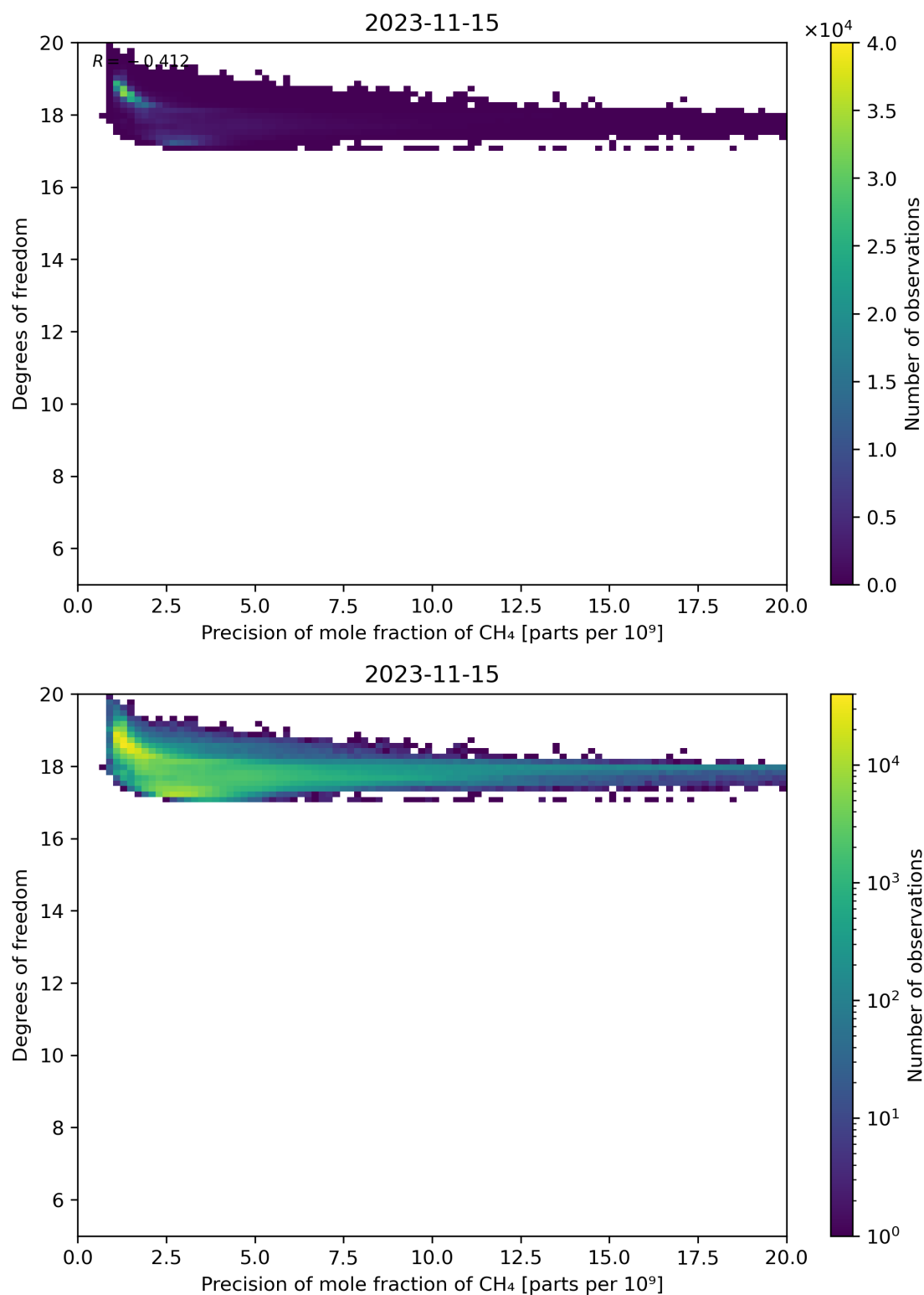
Figure 80: Scatter density plot of “Precision of mole fraction of CH 4 ” against “Degrees of freedom” for 2023-11-14 to 2023-11-16.
