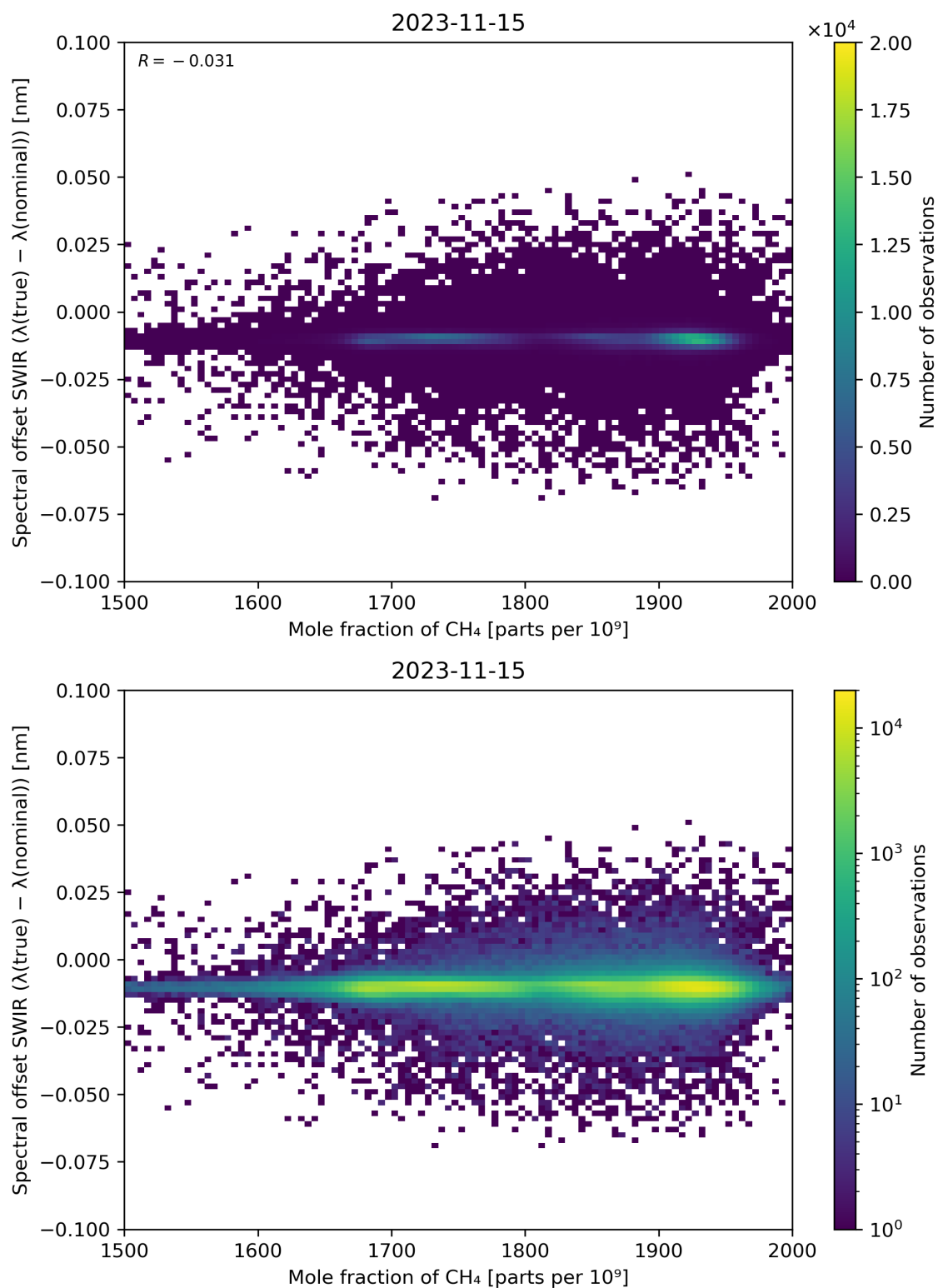
Figure 86: Scatter density plot of “Mole fraction of CH 4 ” against “Spectral offset SWIR ( \lambda(\text{true}) - \lambda(\text{nominal}) )” for 2023-11-14 to 2023-11-16.
