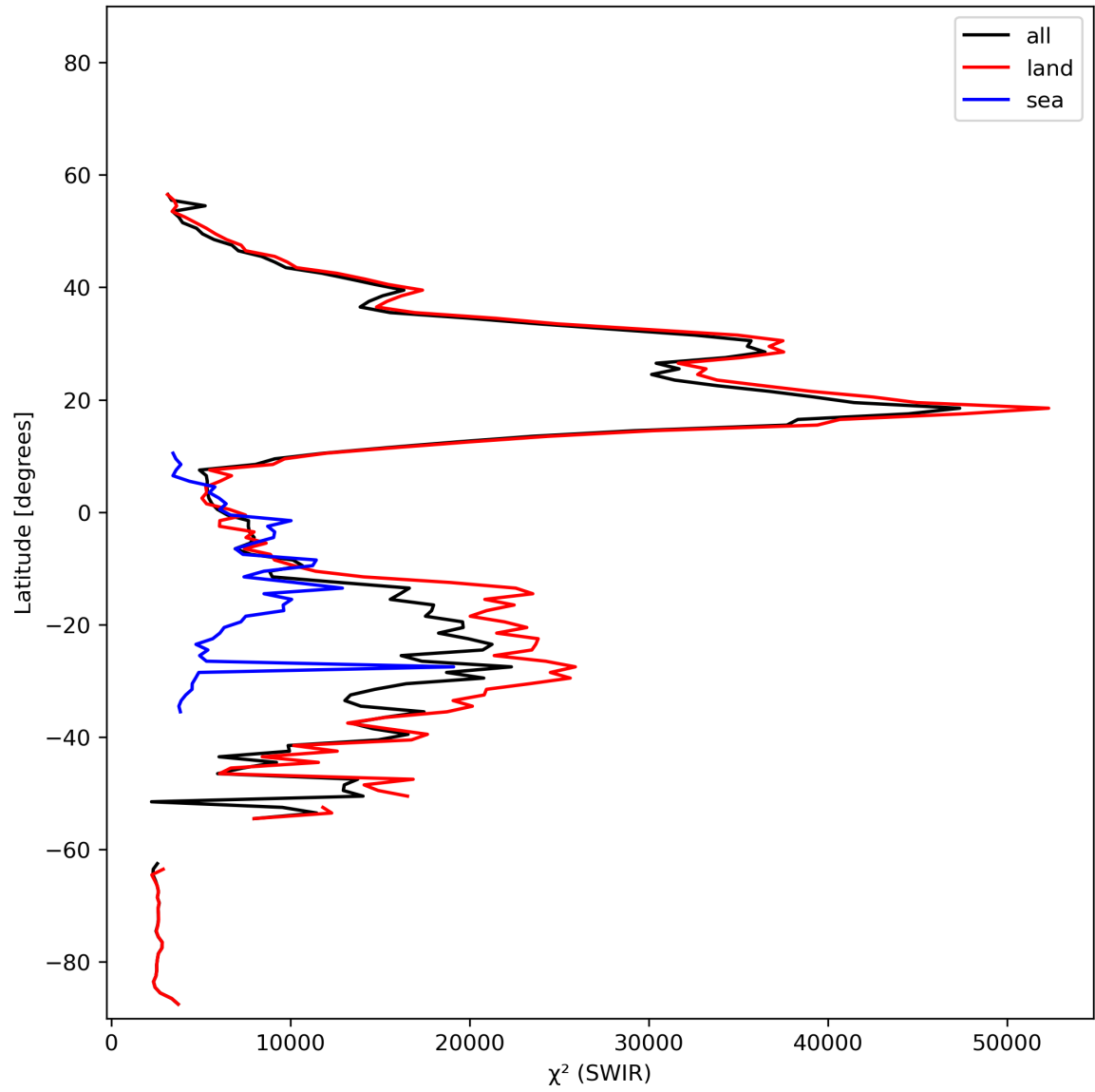
Figure 17: Zonal average of “ \chi^2 (SWIR)” for 2023-11-14 to 2023-11-16.
