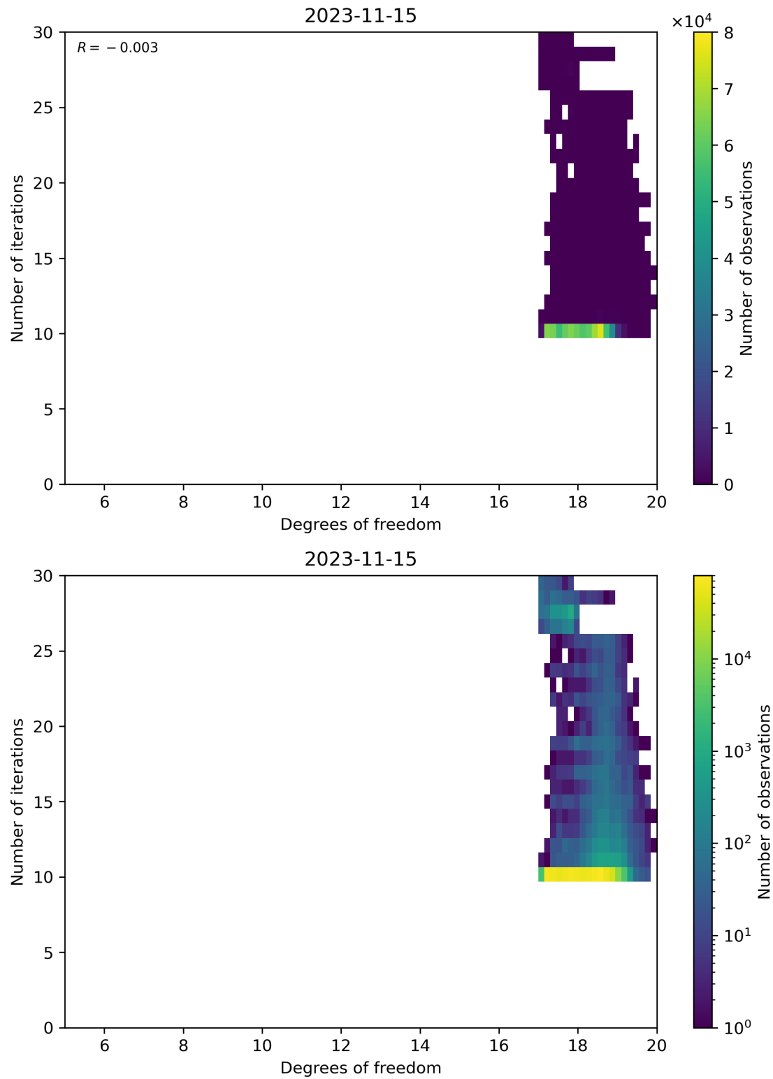
Figure 52: Scatter density plot of “Degrees of freedom” against “Number of iterations” for 2023-11-14 to 2023-11-16.
