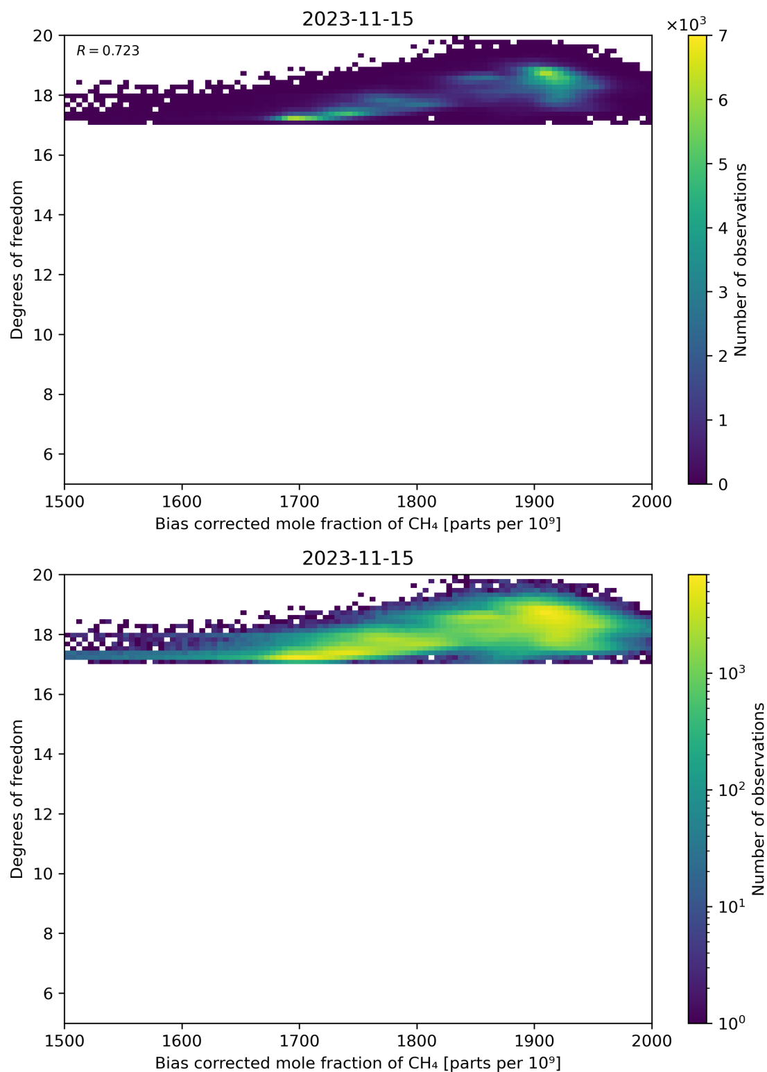
Figure 65: Scatter density plot of “Bias corrected mole fraction of CH 4 ” against “Degrees of freedom” for 2023-11-14 to 2023-11-16.
