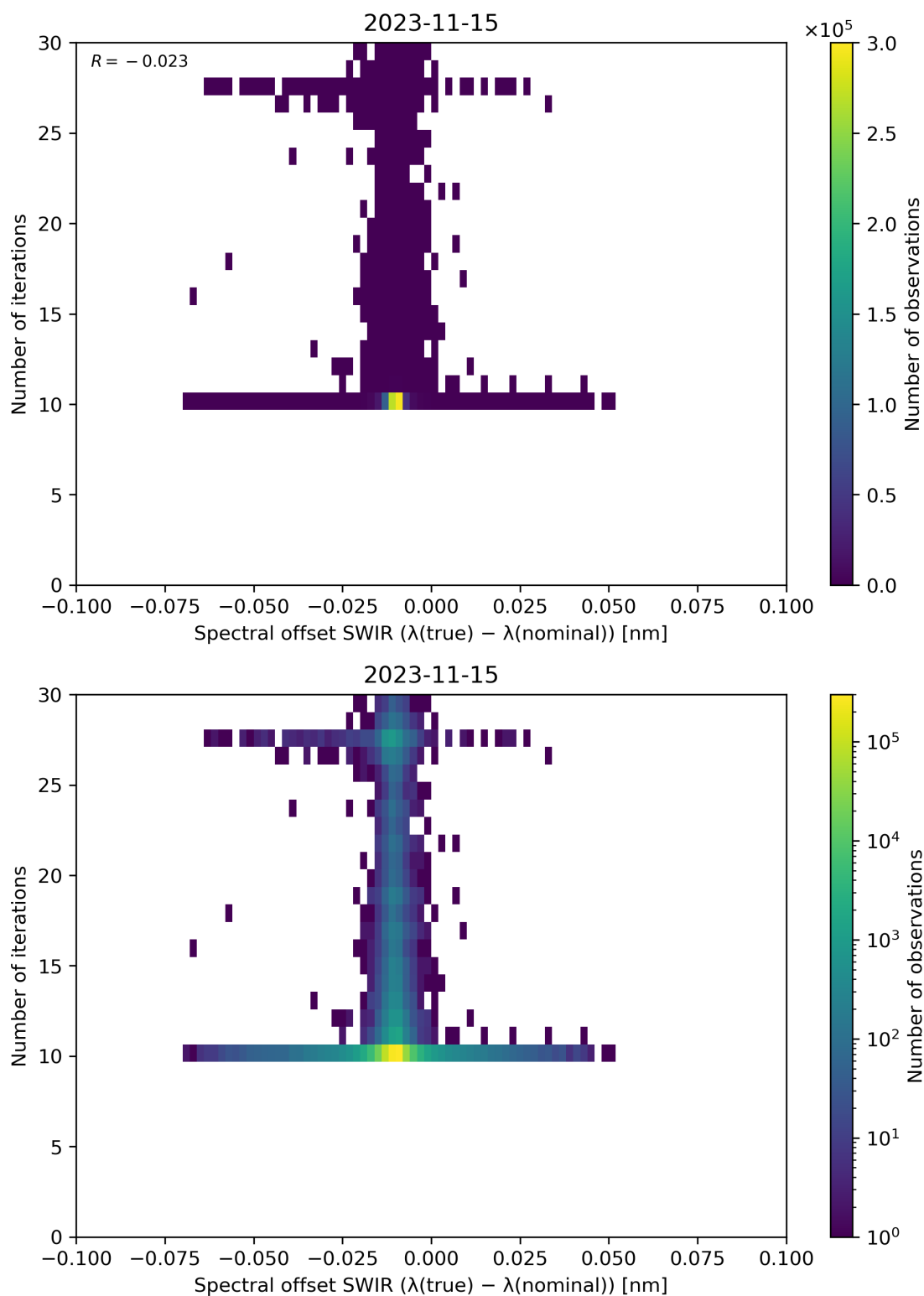
Figure 121: Scatter density plot of “Spectral offset SWIR ( \lambda(\text{true}) - \lambda(\text{nominal}) )” against “Number of iterations” for 2023-11-14 to 2023-11-16.
