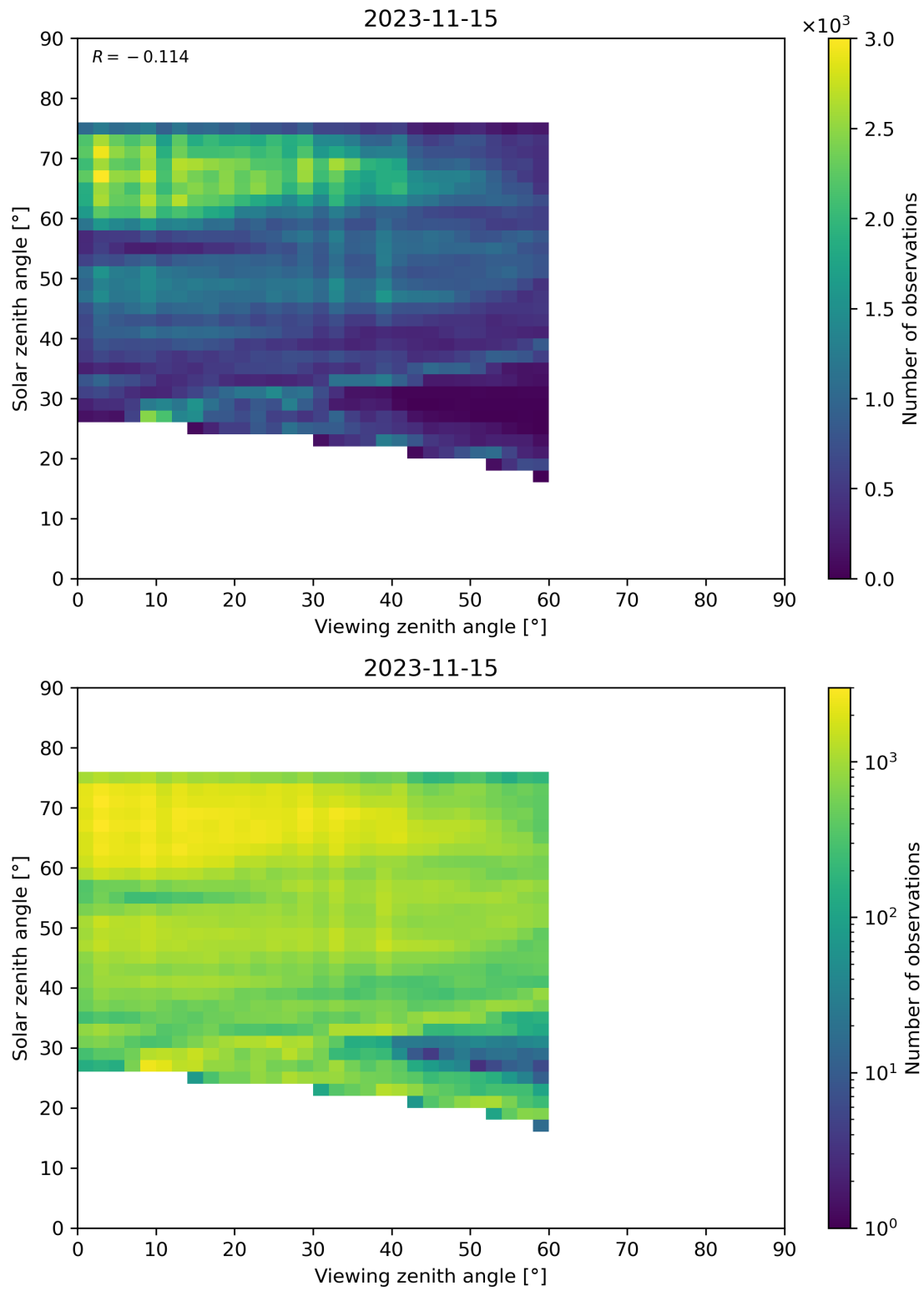
Figure 115: Scatter density plot of “Viewing zenith angle” against “Solar zenith angle” for 2023-11-14 to 2023-11-16.
