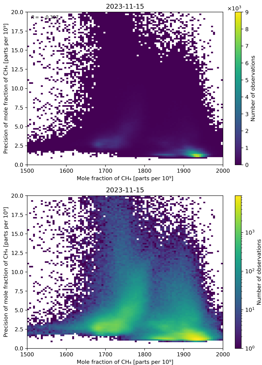
Figure 75: Scatter density plot of “Mole fraction of CH 4 ” against “Precision of mole fraction of CH 4 ” for 2023-11-14 to 2023-11-16.
