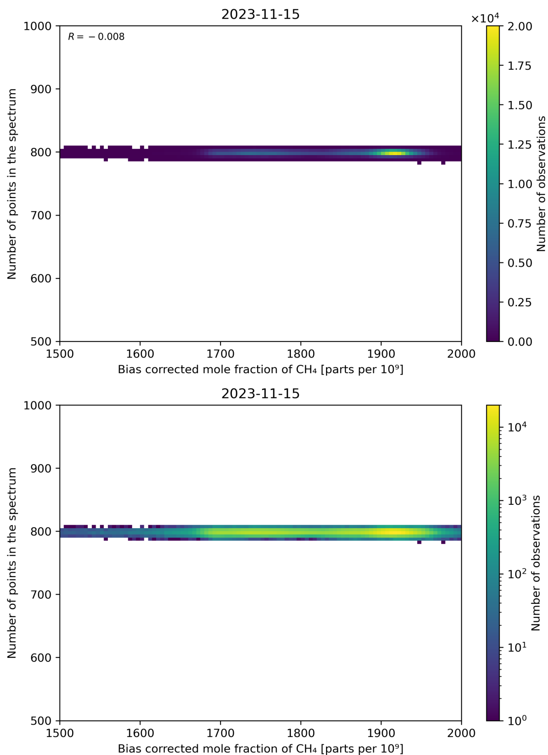
Figure 68: Scatter density plot of “Bias corrected mole fraction of CH 4 ” against “Number of points in the spectrum” for 2023-11-14 to 2023-11-16.
