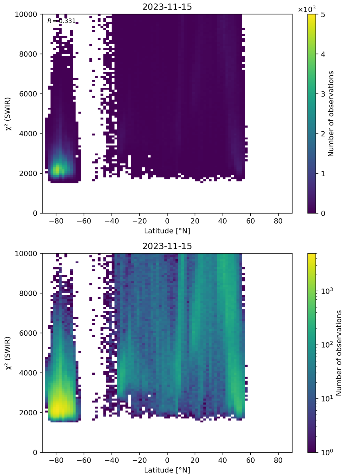
Figure 54: Scatter density plot of “Latitude” against “ \chi^2 (SWIR)” for 2023-11-14 to 2023-11-16.
