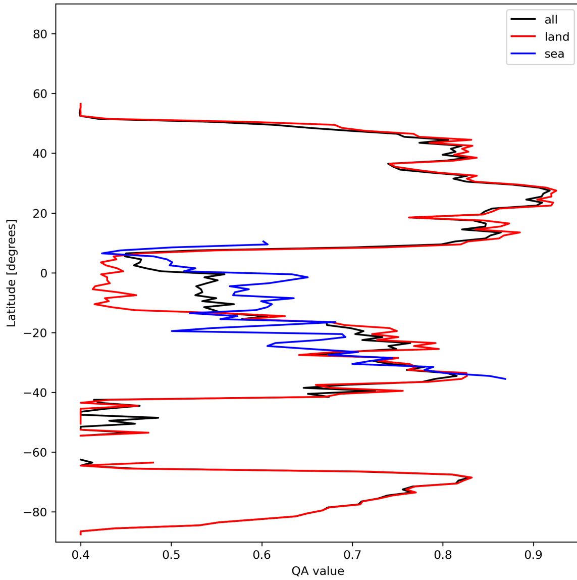
Figure 11: Zonal average of “QA value” for 2023-11-14 to 2023-11-16.
