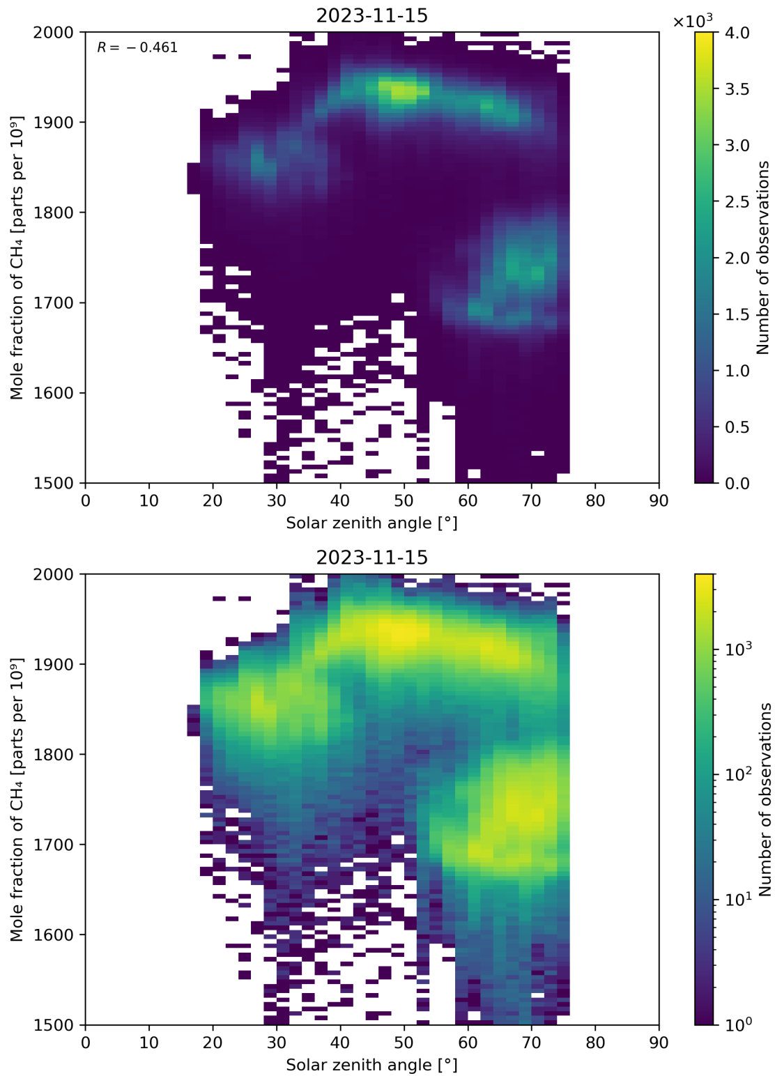
Figure 99: Scatter density plot of “Solar zenith angle” against “Mole fraction of CH 4 ” for 2023-11-14 to 2023-11-16.
