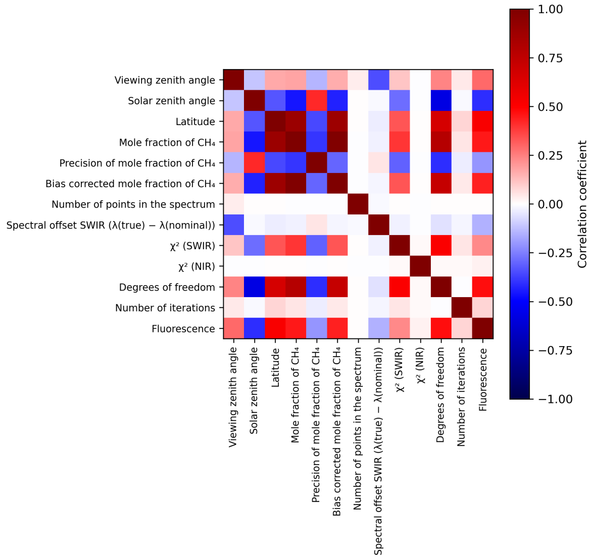
Figure 2: Map of correlation matrix for 2023-11-14 to 2023-11-16.
