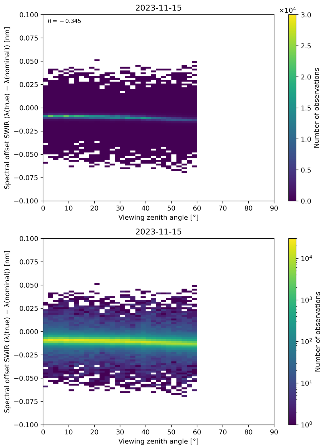
Figure 116: Scatter density plot of “Viewing zenith angle” against “Spectral offset SWIR ( \lambda(\text{true}) - \lambda(\text{nominal}) )” for 2023-11-14 to 2023-11-16.
