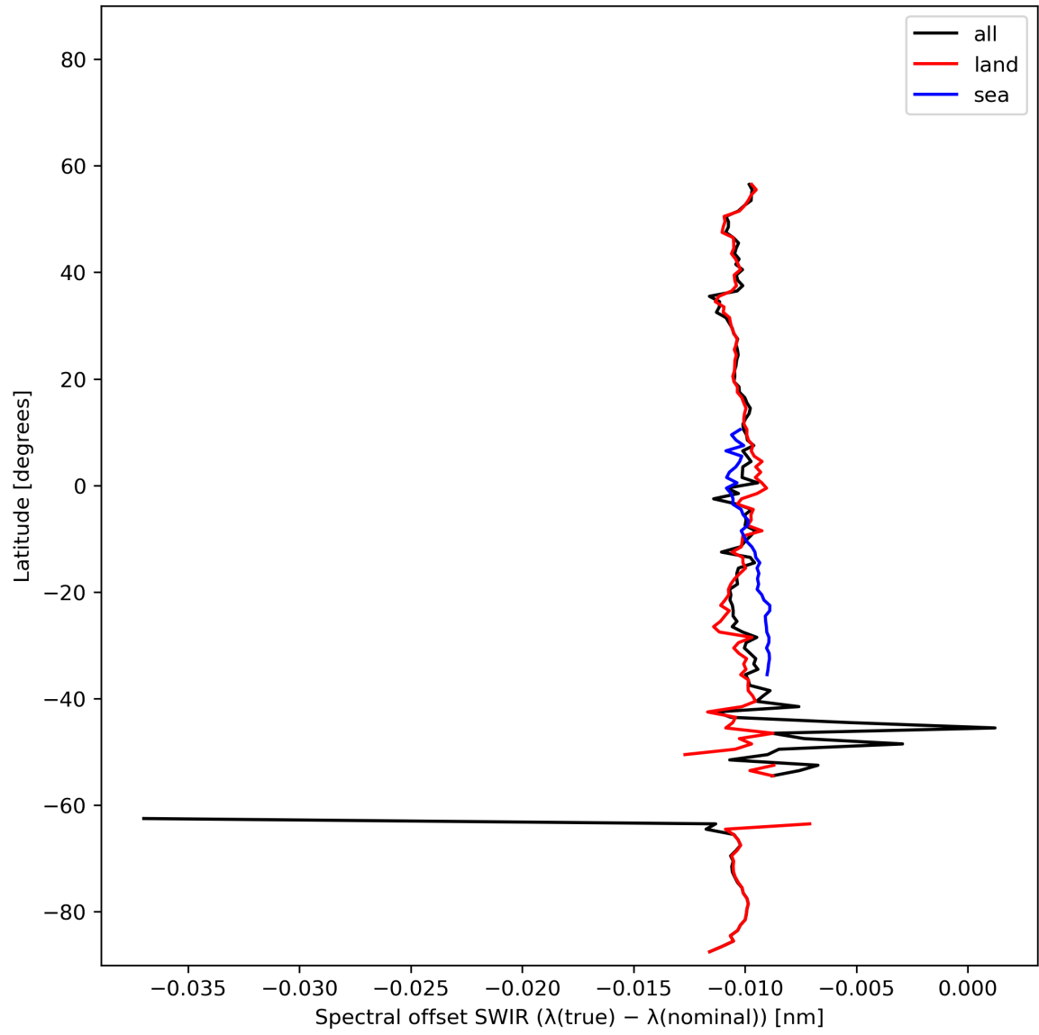
Figure 16: Zonal average of “Spectral offset SWIR ( \lambda(\text{true}) - \lambda(\text{nominal}) )” for 2023-11-14 to 2023-11-16.
