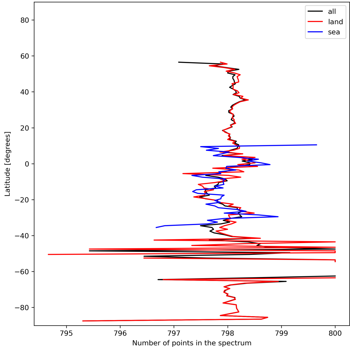
Figure 15: Zonal average of “Number of points in the spectrum” for 2023-11-14 to 2023-11-16.
