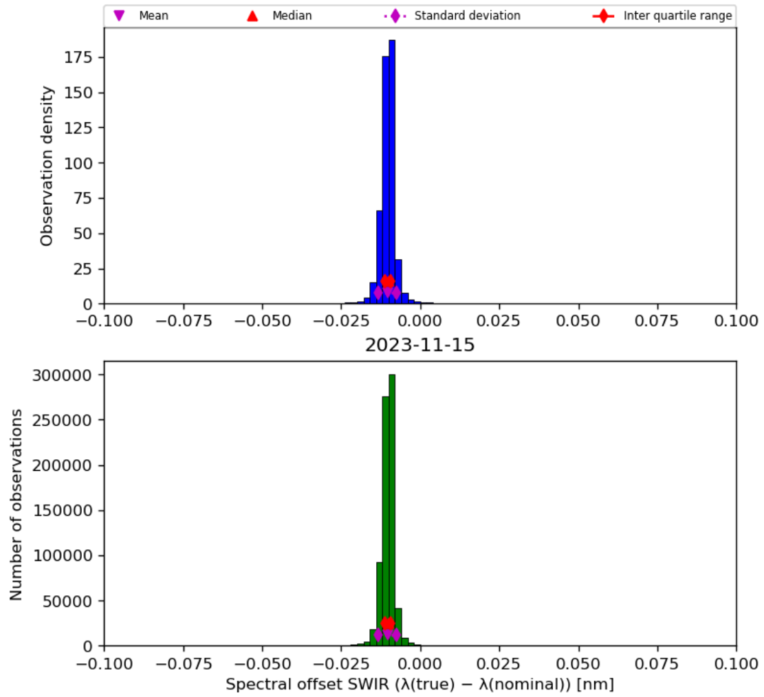
Figure 27: Histogram of “Spectral offset SWIR ( \lambda(\text{true}) - \lambda(\text{nominal}) )” for 2023-11-14 to 2023-11-16
