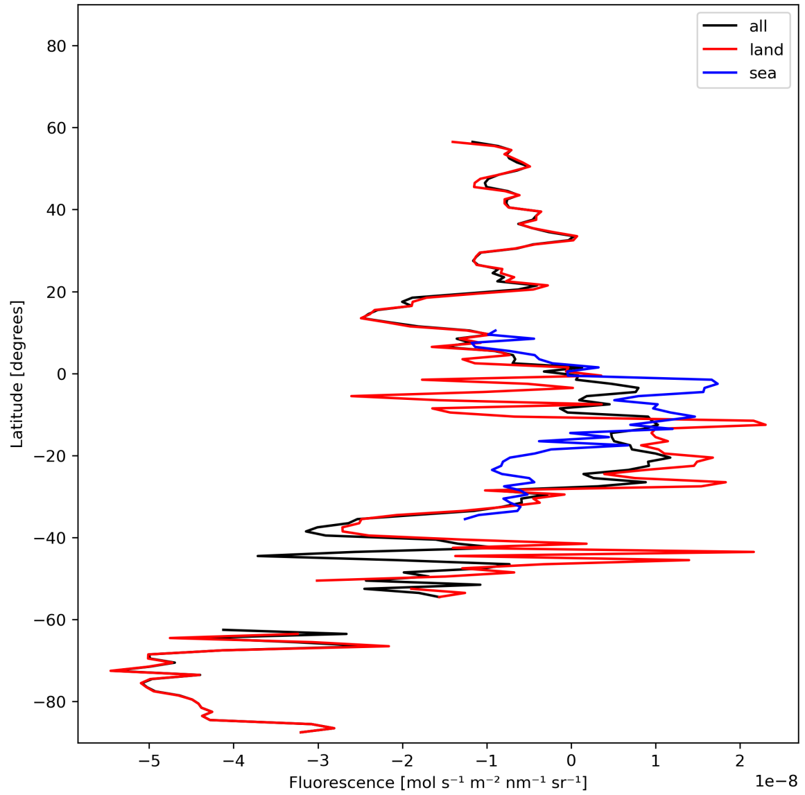
Figure 21: Zonal average of “Fluorescence” for 2023-11-14 to 2023-11-16.
