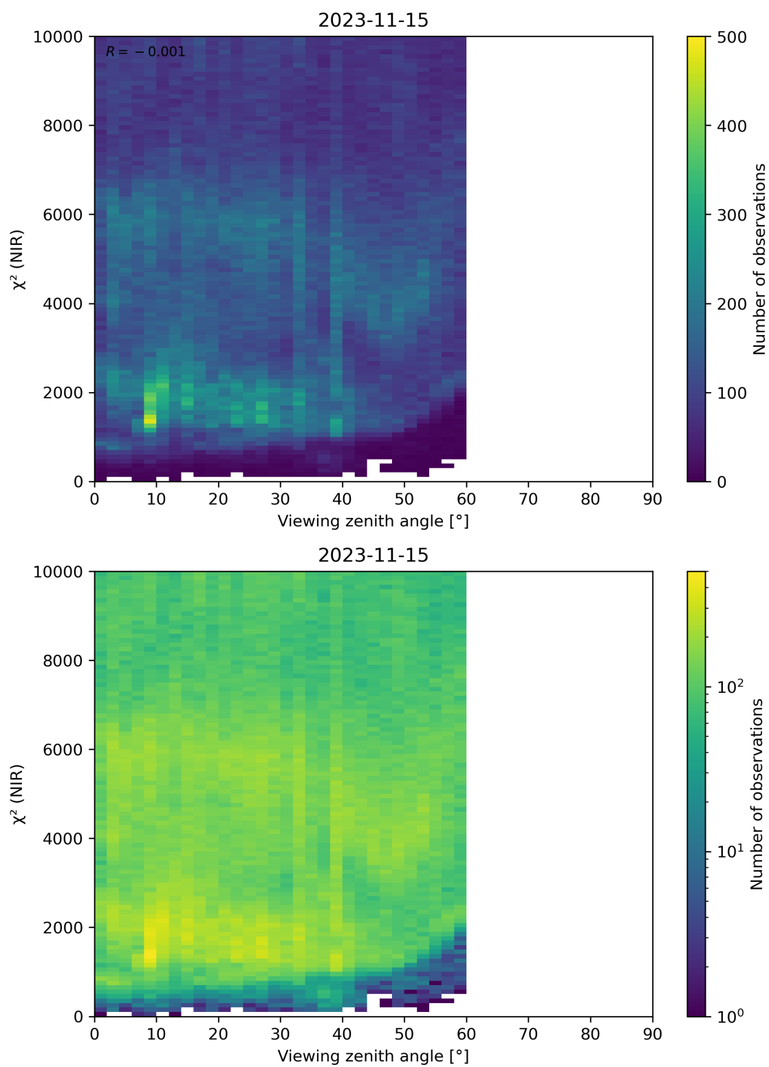
Figure 105: Scatter density plot of “Viewing zenith angle” against “ \chi^2 (NIR)” for 2023-11-14 to 2023-11-16.
