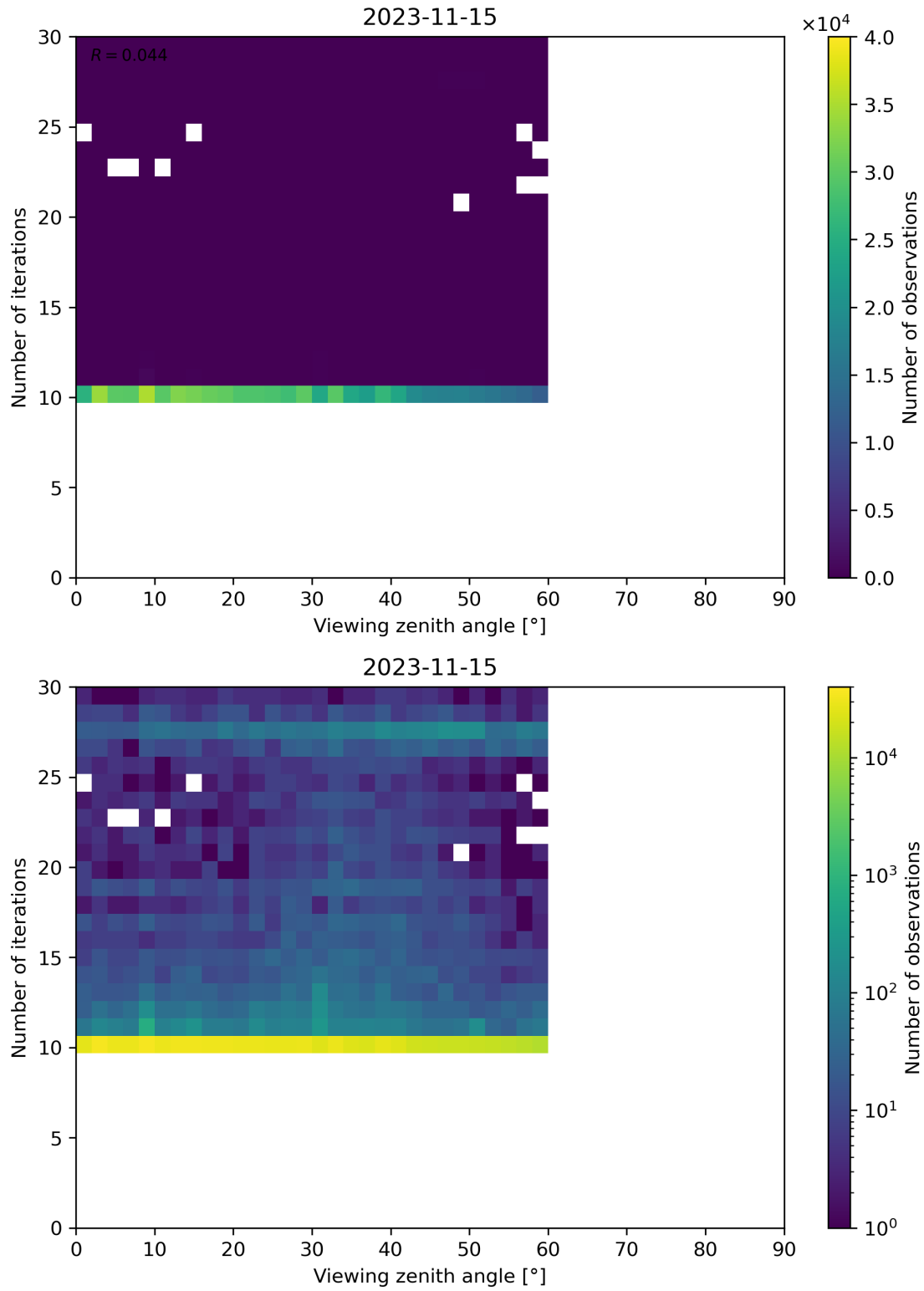
Figure 113: Scatter density plot of “Viewing zenith angle” against “Number of iterations” for 2023-11-14 to 2023-11-16.
