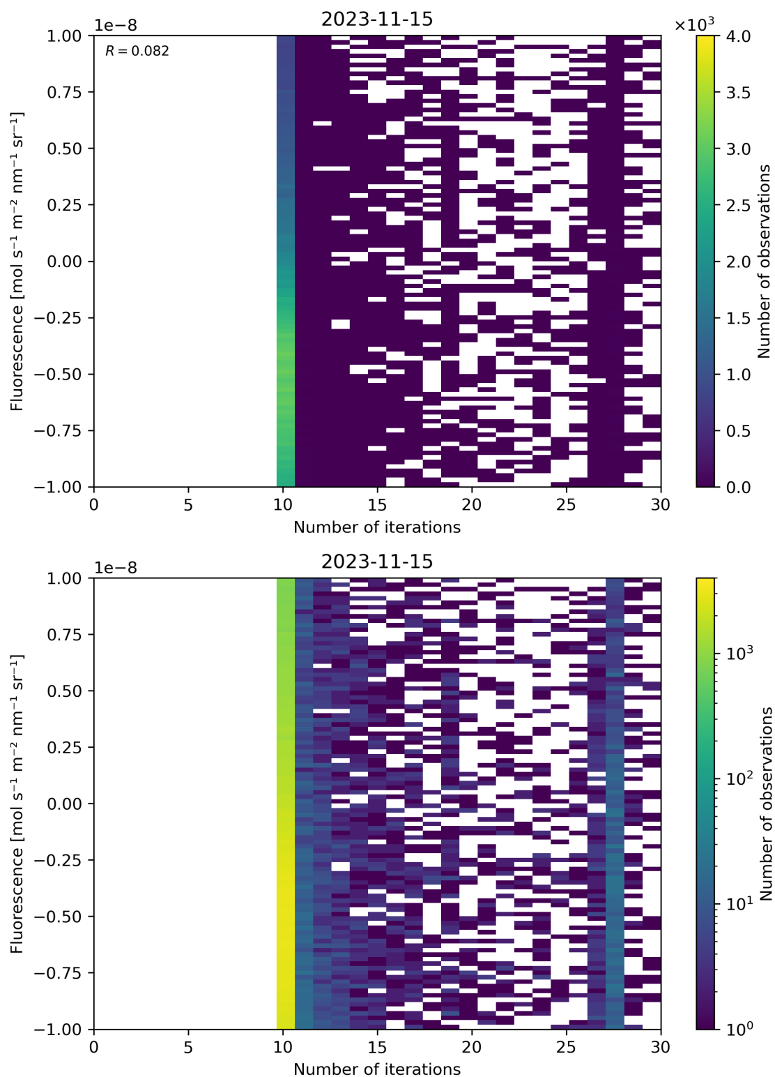
Figure 87: Scatter density plot of “Number of iterations” against “Fluorescence” for 2023-11-14 to 2023-11-16.
