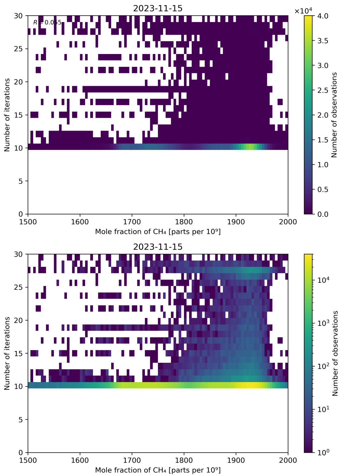
Figure 76: Scatter density plot of “Mole fraction of CH 4 ” against “Number of iterations” for 2023-11-14 to 2023-11-16.
