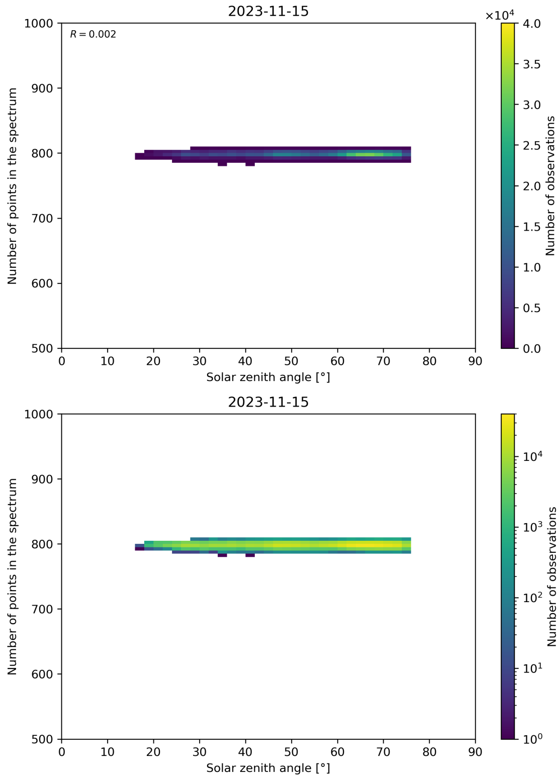
Figure 103: Scatter density plot of “Solar zenith angle” against “Number of points in the spectrum” for 2023-11-14 to 2023-11-16.
