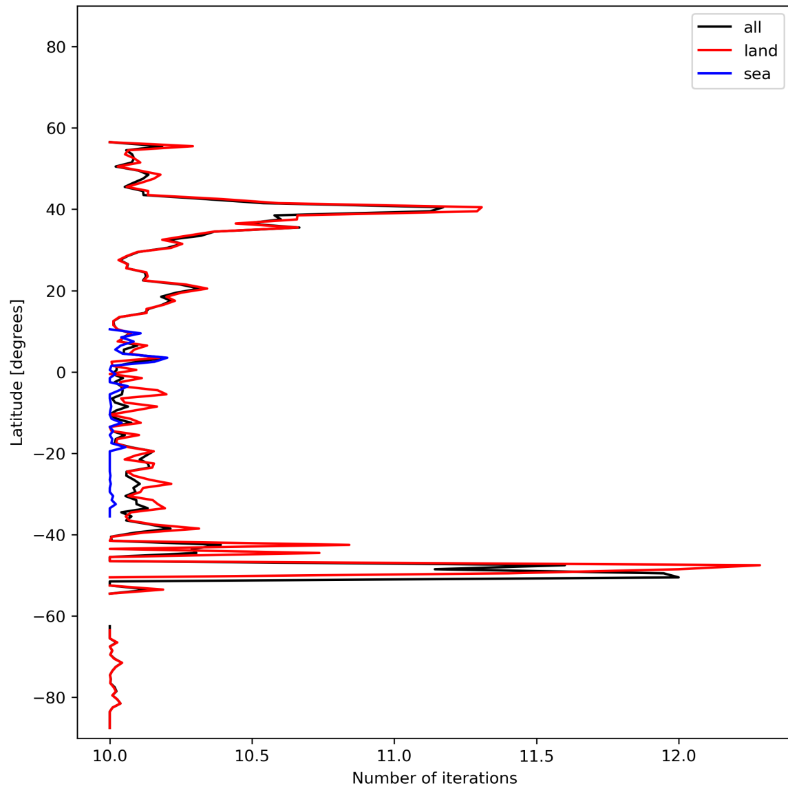
Figure 20: Zonal average of “Number of iterations” for 2023-11-14 to 2023-11-16.
