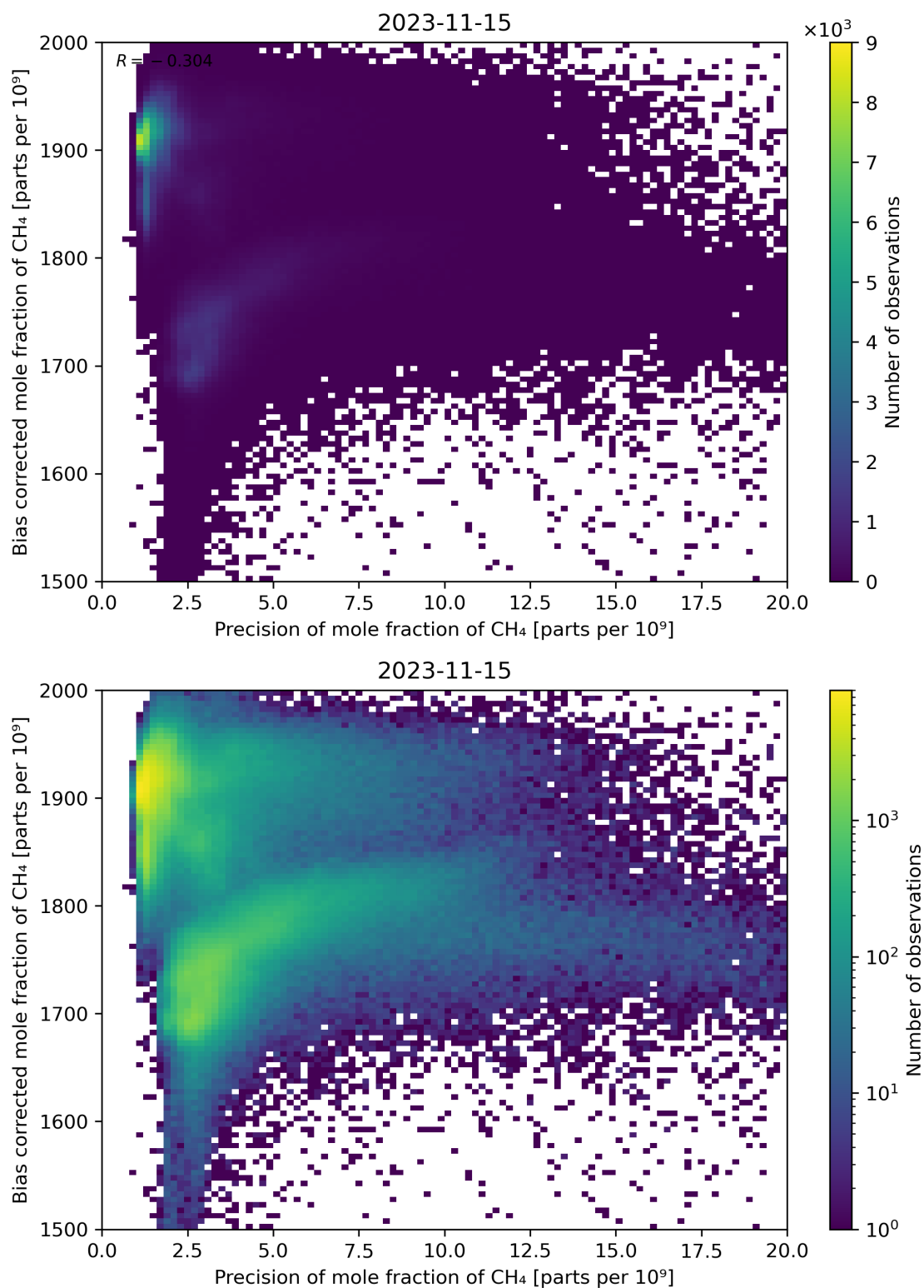
Figure 82: Scatter density plot of “Precision of mole fraction of \text{CH}_4 ” against “Bias corrected mole fraction of \text{CH}_4 ” for 2023-11-14 to 2023-11-16.
