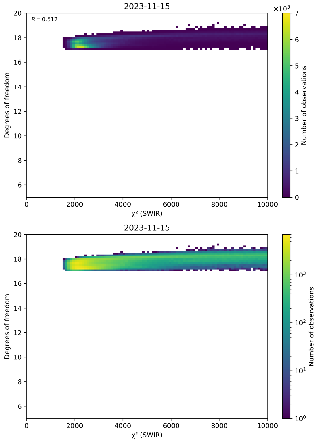
Figure 48: Scatter density plot of “ \chi^2 (SWIR)” against “Degrees of freedom” for 2023-11-14 to 2023-11-16.
