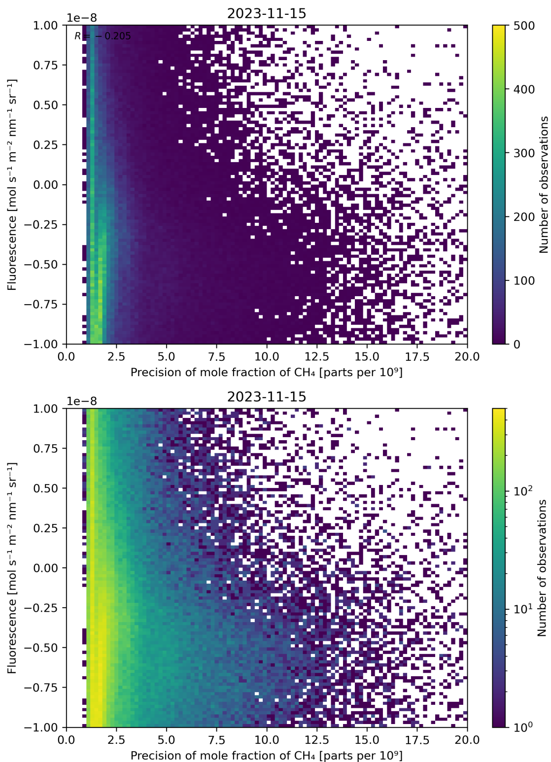
Figure 81: Scatter density plot of “Precision of mole fraction of CH 4 ” against “Fluorescence” for 2023-11-14 to 2023-11-16.
