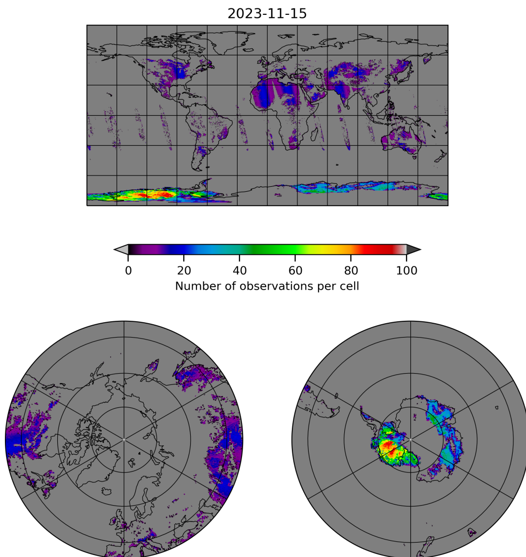
Figure 10: Map of the number of observations for 2023-11-14 to 2023-11-16
