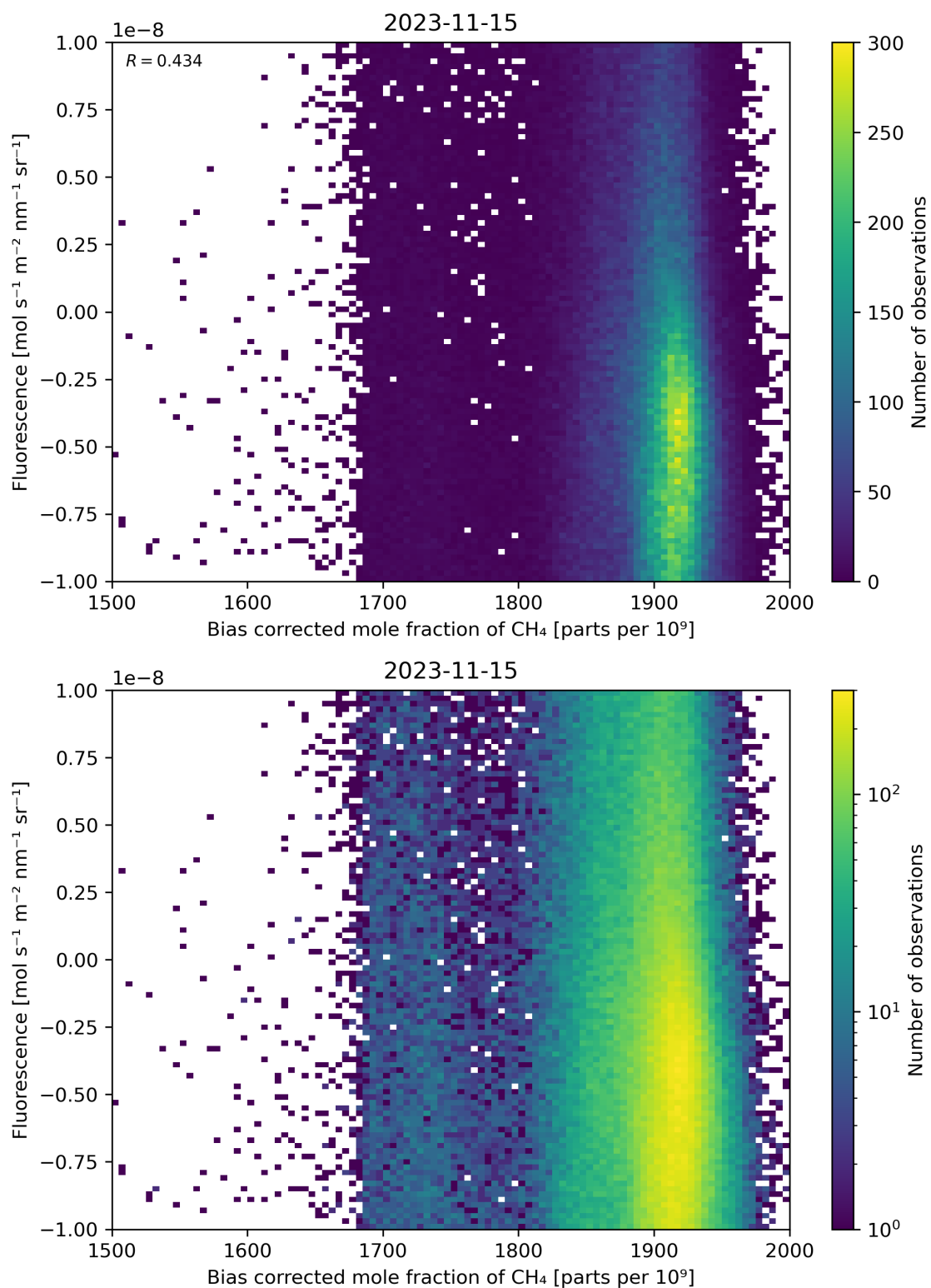
Figure 66: Scatter density plot of “Bias corrected mole fraction of CH 4 ” against “Fluorescence” for 2023-11-14 to 2023-11-16.
