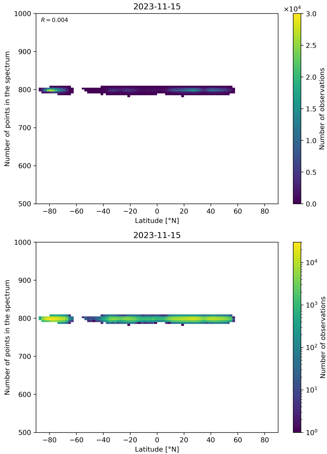
Figure 61: Scatter density plot of “Latitude” against “Number of points in the spectrum” for 2023-11-14 to 2023-11-16.
