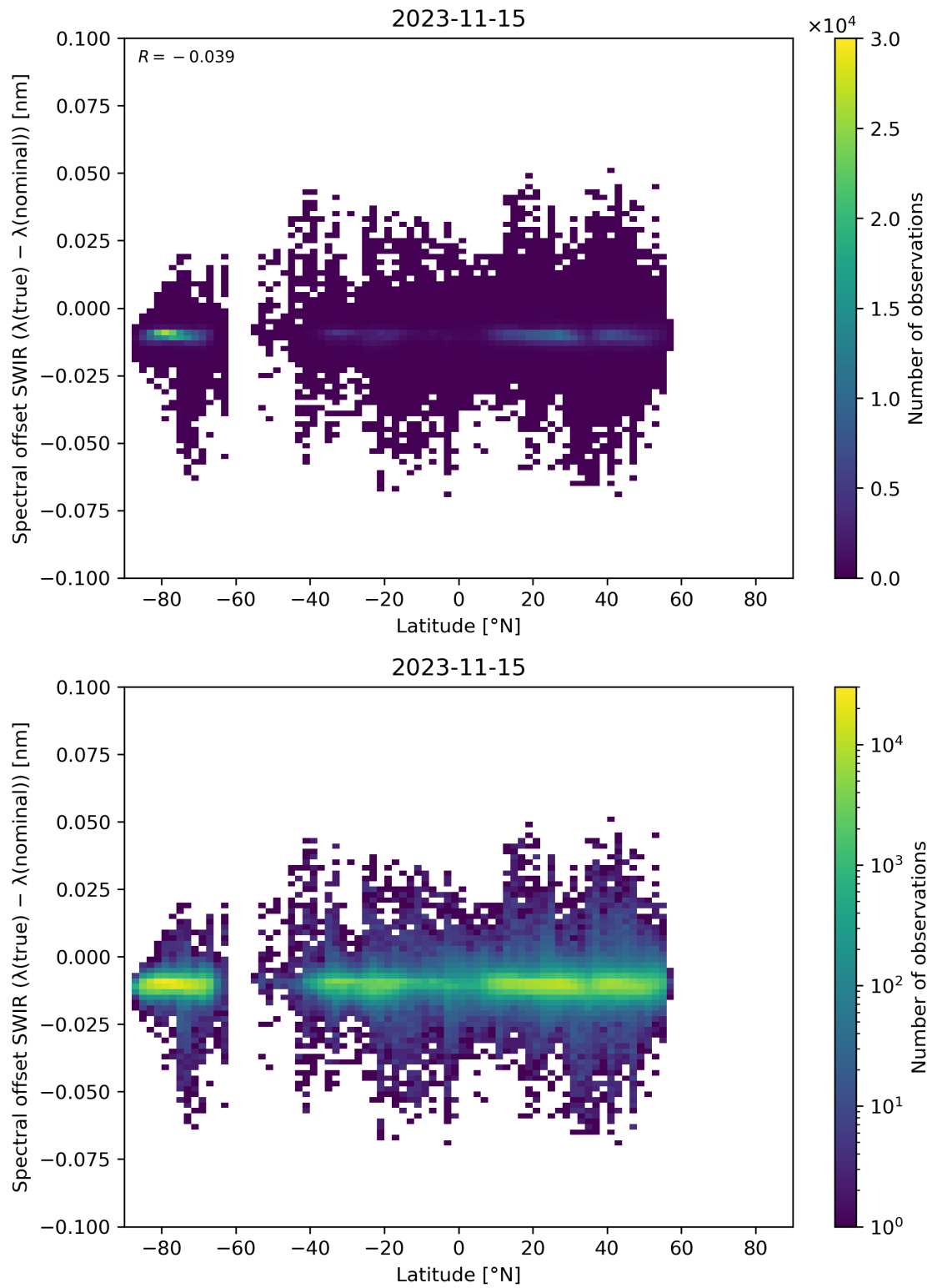
Figure 62: Scatter density plot of “Latitude” against “Spectral offset SWIR ( \lambda(\text{true}) - \lambda(\text{nominal}) )” for 2023-11-14 to 2023-11-16.
