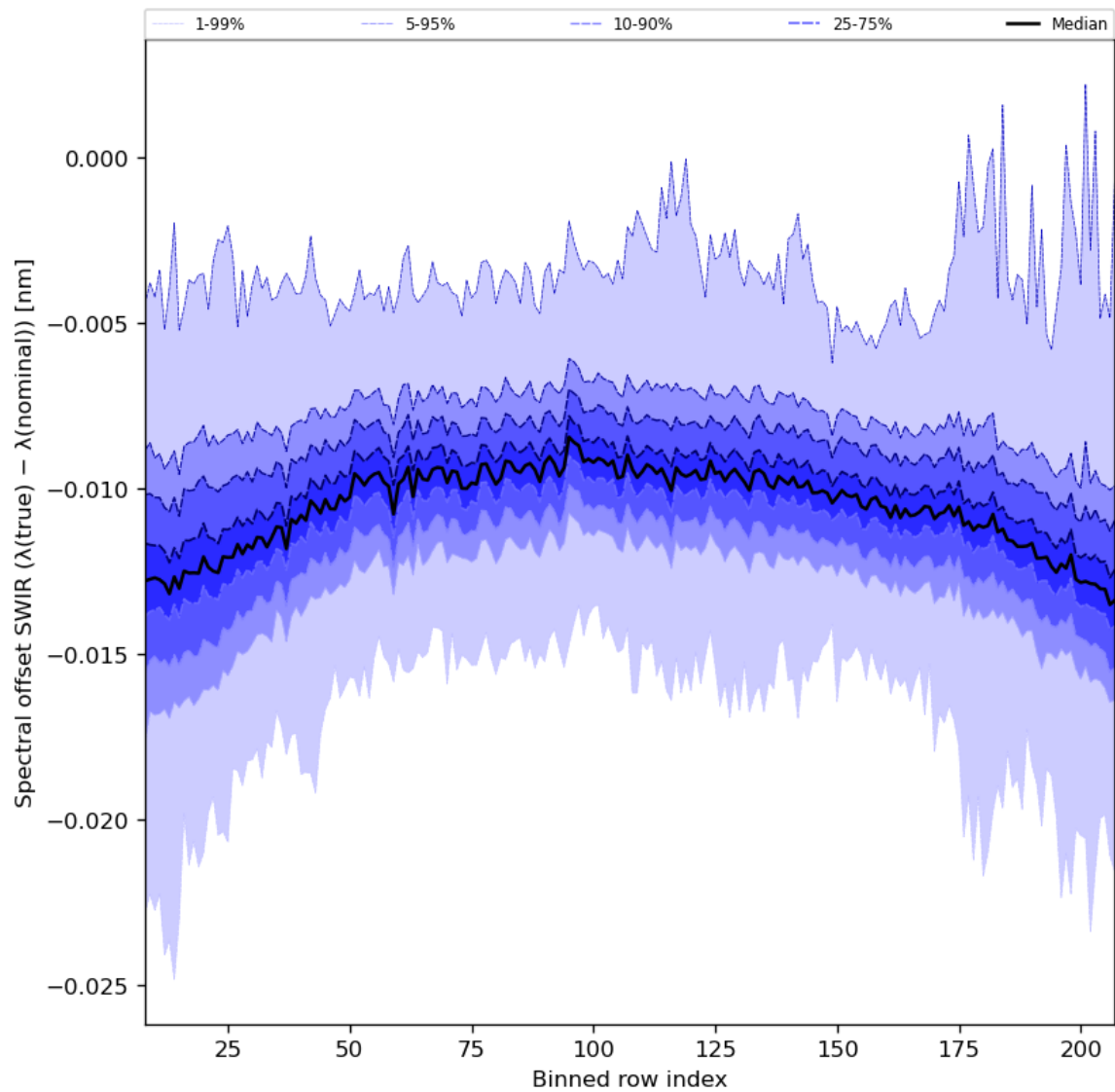
Figure 38: Along track statistics of “Spectral offset SWIR ( \lambda(\text{true}) - \lambda(\text{nominal}) )” for 2023-11-14 to 2023-11-16
