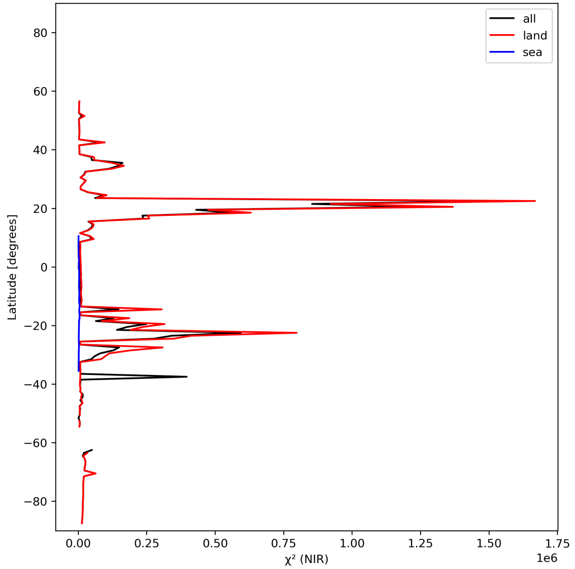
Figure 18: Zonal average of “ \chi^2 (NIR)” for 2023-11-14 to 2023-11-16.
