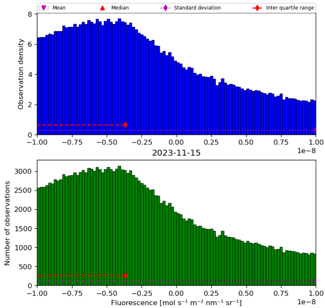
Figure 32: Histogram of “Fluorescence” for 2023-11-14 to 2023-11-16
