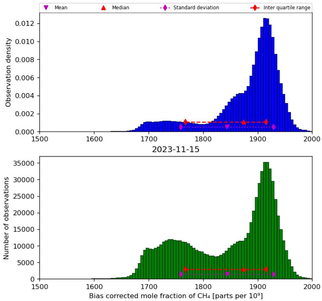
Figure 25: Histogram of “Bias corrected mole fraction of CH 4 ” for 2023-11-14 to 2023-11-16
