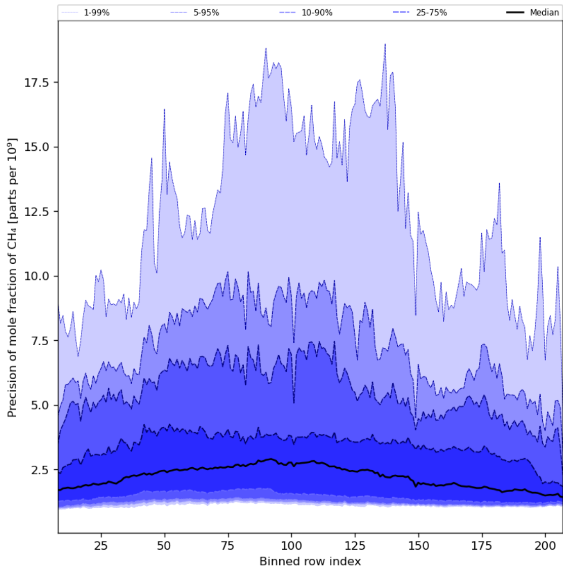
Figure 35: Along track statistics of “Precision of mole fraction of CH 4 ” for 2023-11-14 to 2023-11-16
