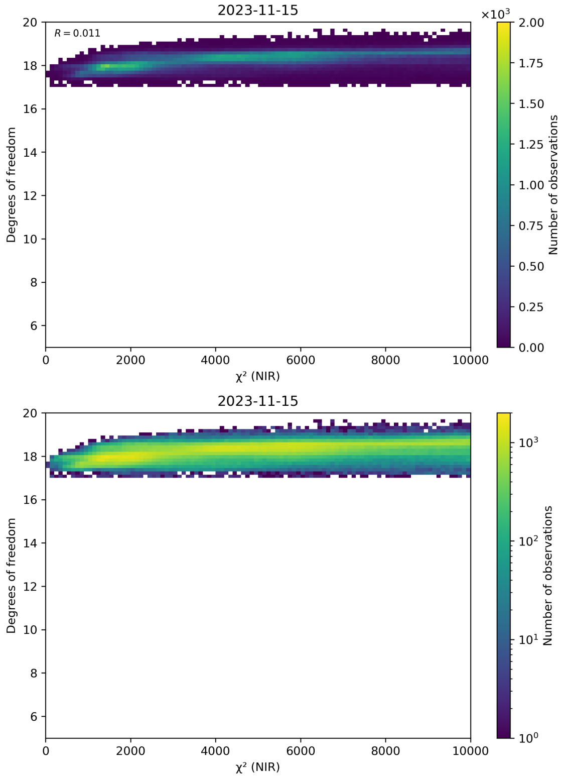
Figure 44: Scatter density plot of “ \chi^2 (NIR)” against “Degrees of freedom” for 2023-11-14 to 2023-11-16.
