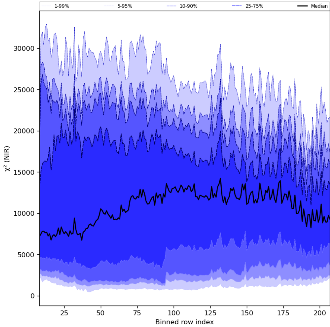
Figure 40: Along track statistics of “ \chi^2 (NIR)” for 2023-11-14 to 2023-11-16
