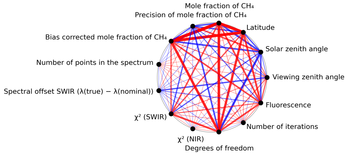
Figure 1: Map of correlation graph for 2023-11-14 to 2023-11-16.
