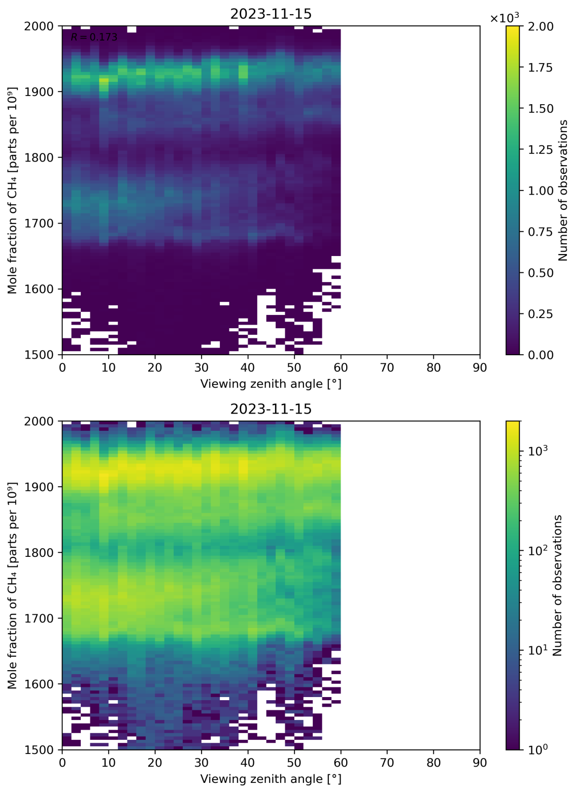
Figure 110: Scatter density plot of “Viewing zenith angle” against “Mole fraction of CH 4 ” for 2023-11-14 to 2023-11-16.
