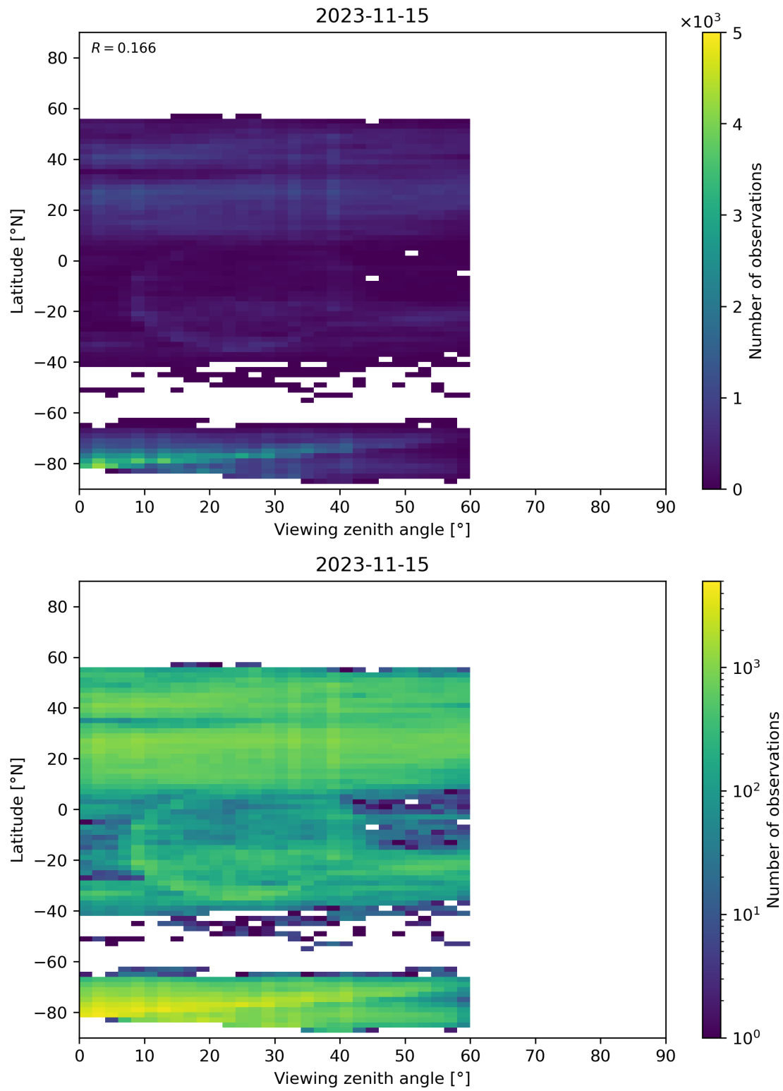
Figure 109: Scatter density plot of “Viewing zenith angle” against “Latitude” for 2023-11-14 to 2023-11-16.
