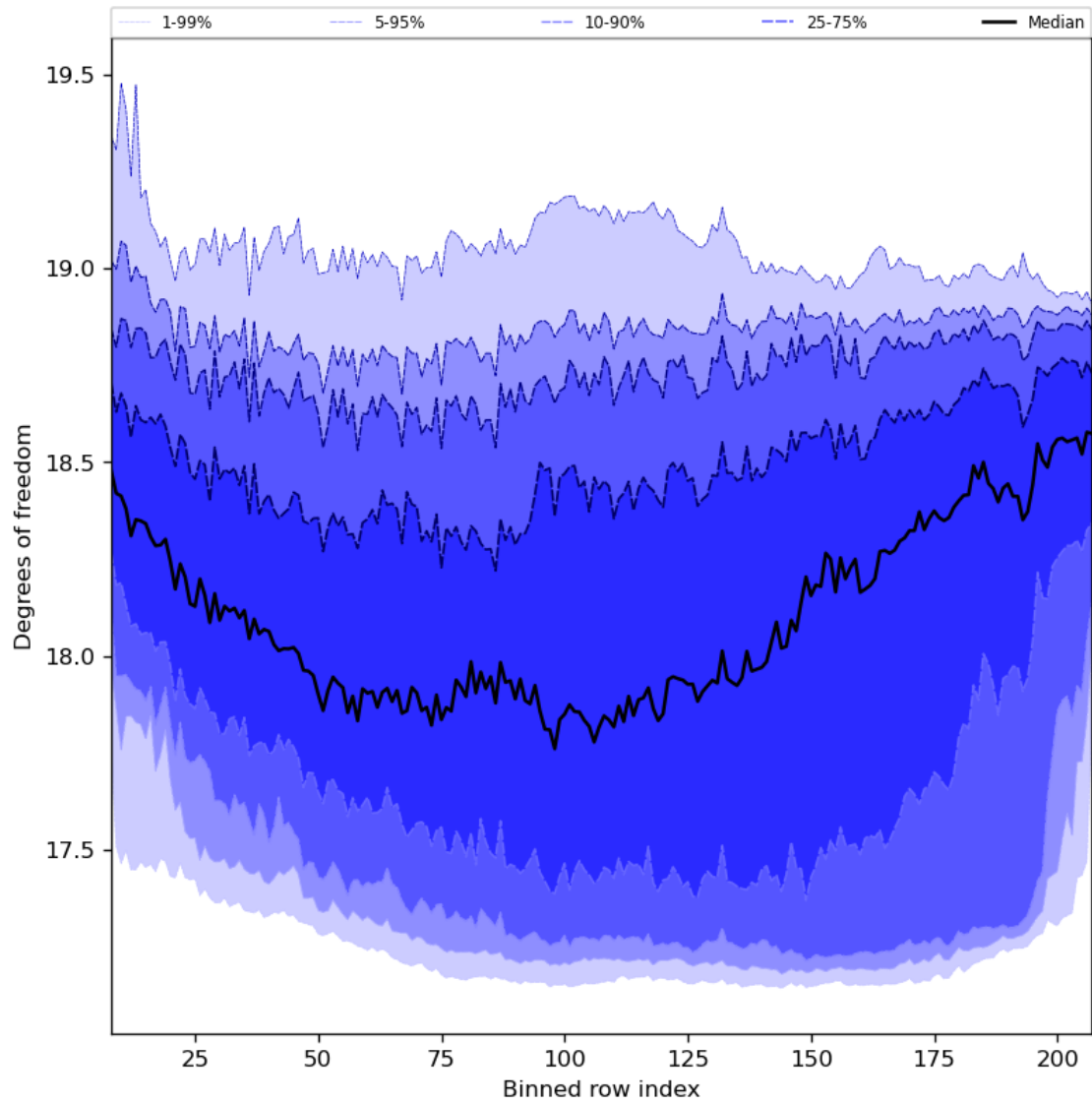
Figure 41: Along track statistics of “Degrees of freedom” for 2023-11-14 to 2023-11-16
