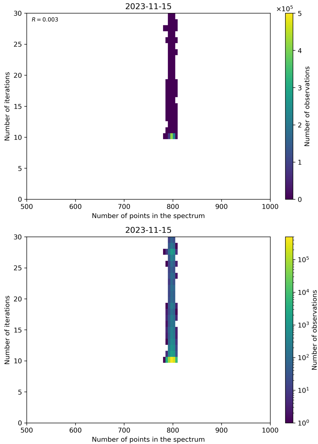
Figure 92: Scatter density plot of “Number of points in the spectrum” against “Number of iterations” for 2023-11-14 to 2023-11-16.
