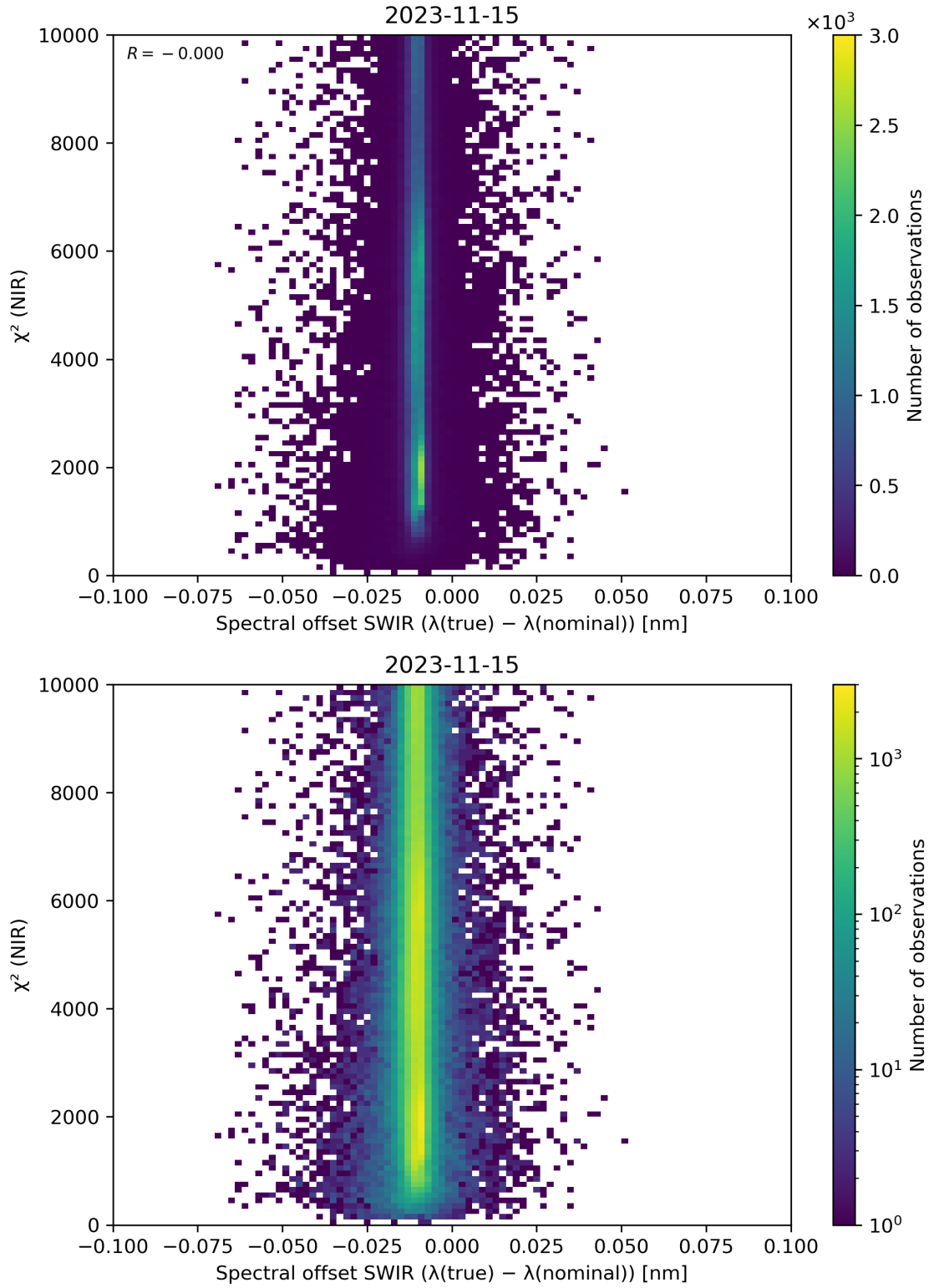
Figure 117: Scatter density plot of “Spectral offset SWIR ( \lambda(\text{true}) - \lambda(\text{nominal}) )” against “ \chi^2 (NIR)” for 2023-11-14 to 2023-11-16.
