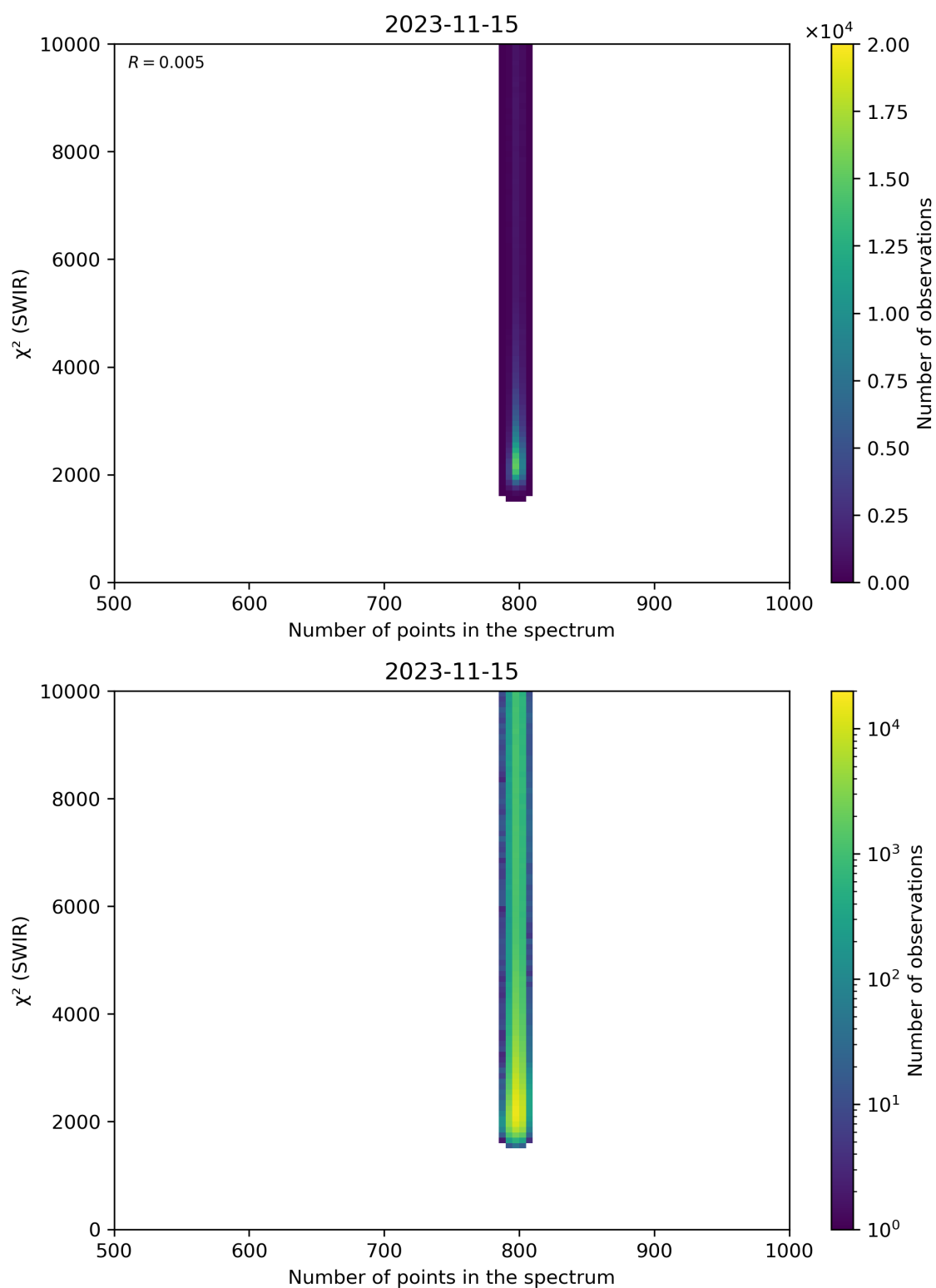
Figure 89: Scatter density plot of “Number of points in the spectrum” against “ \chi^2 (SWIR)” for 2023-11-14 to 2023-11-16.
