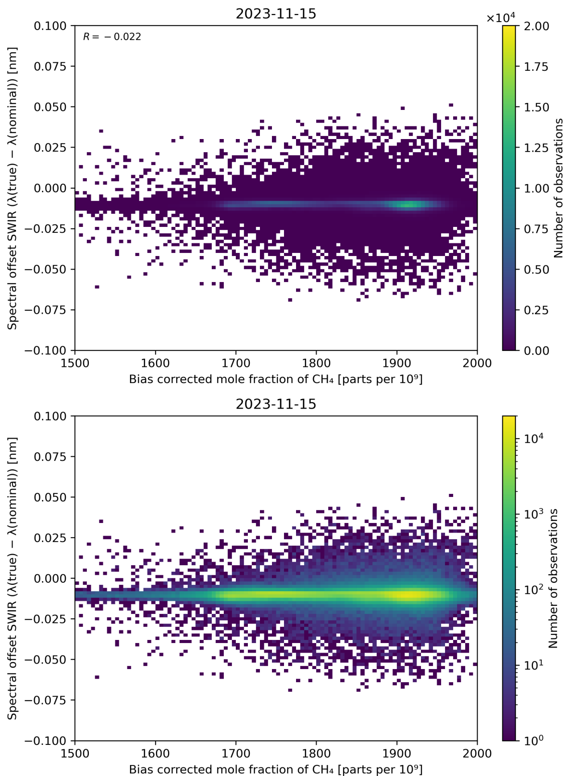
Figure 69: Scatter density plot of “Bias corrected mole fraction of \text{CH}_4 ” against “Spectral offset SWIR ( \lambda(\text{true}) - \lambda(\text{nominal}) )” for 2023-11-14 to 2023-11-16.
