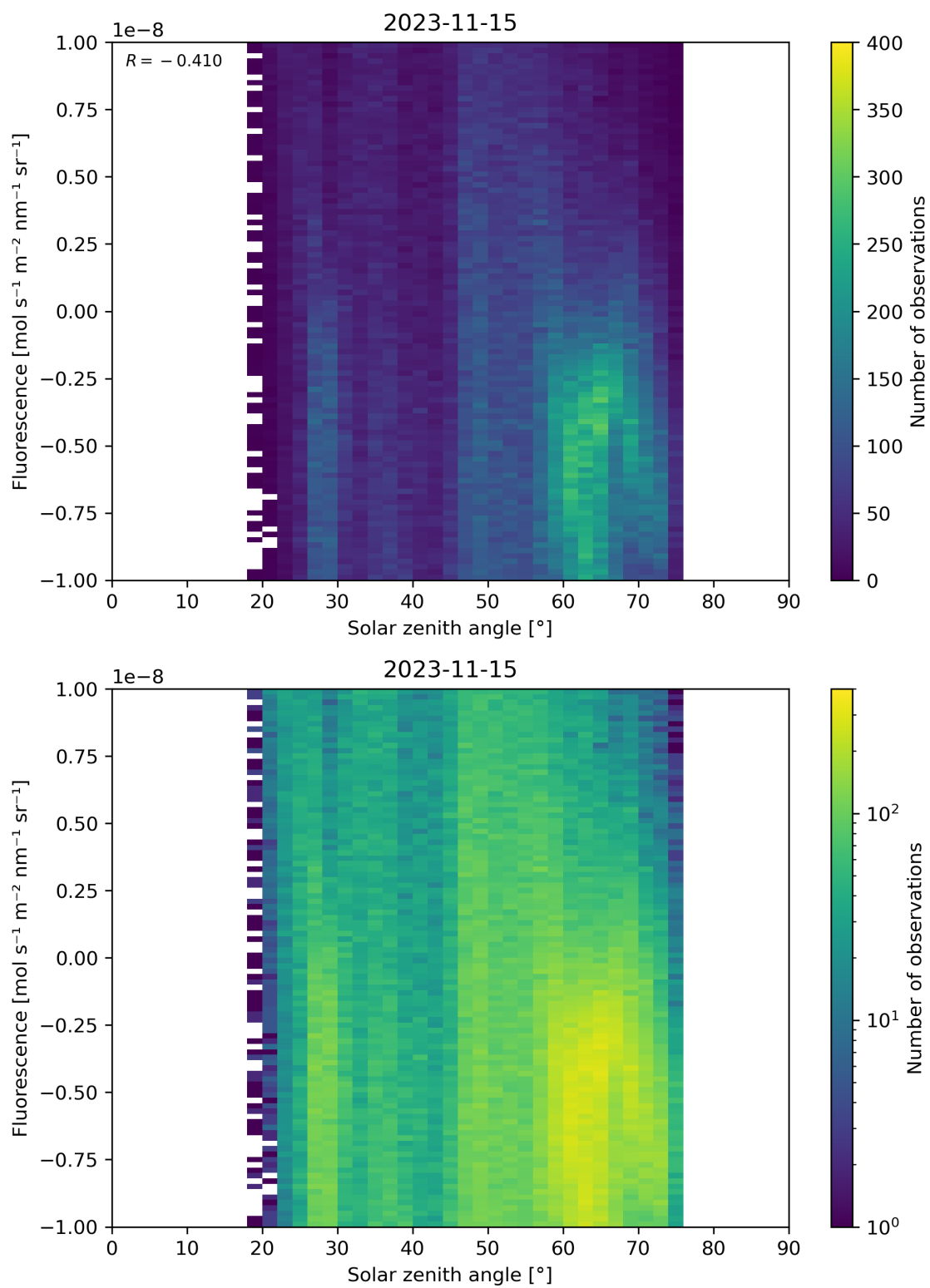
Figure 97: Scatter density plot of “Solar zenith angle” against “Fluorescence” for 2023-11-14 to 2023-11-16.
