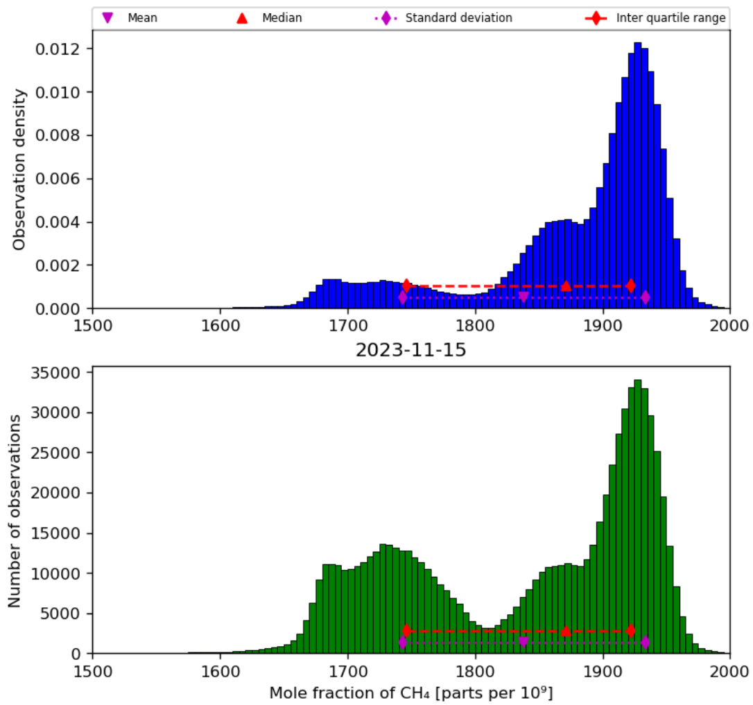
Figure 23: Histogram of “Mole fraction of CH 4 ” for 2023-11-14 to 2023-11-16
