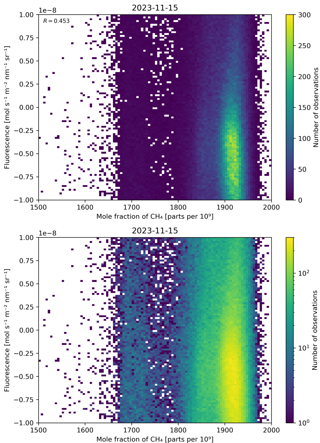
Figure 73: Scatter density plot of “Mole fraction of \text{CH}_4 ” against “Fluorescence” for 2023-11-14 to 2023-11-16.
