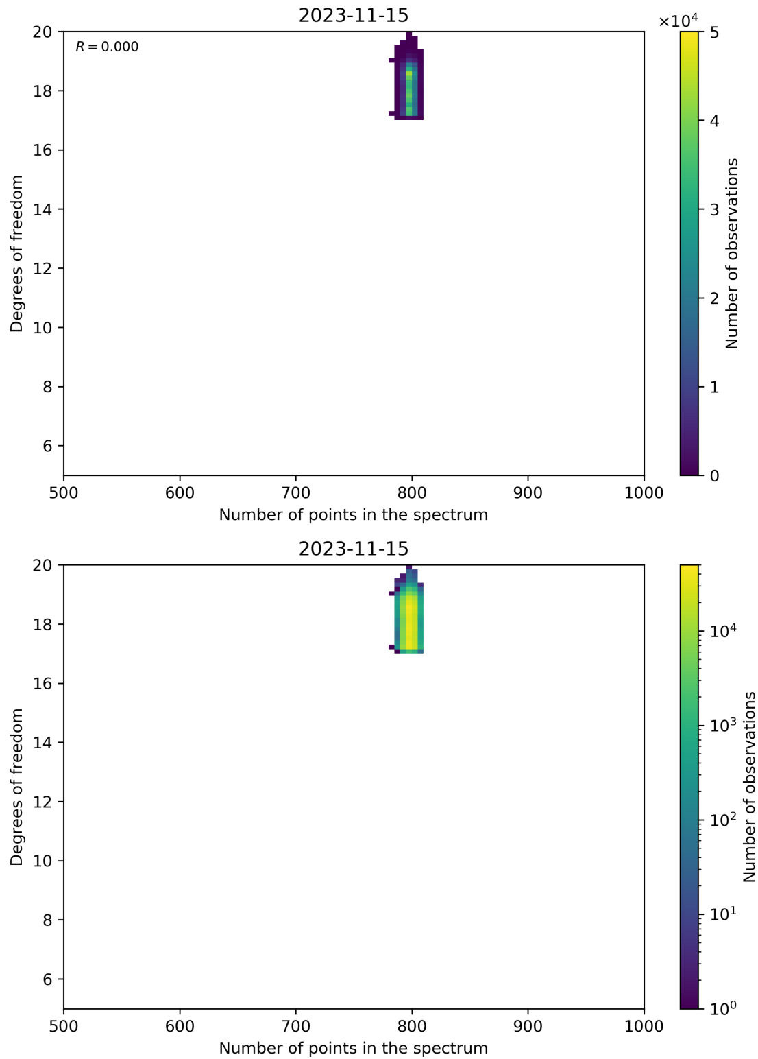
Figure 90: Scatter density plot of “Number of points in the spectrum” against “Degrees of freedom” for 2023-11-14 to 2023-11-16.
