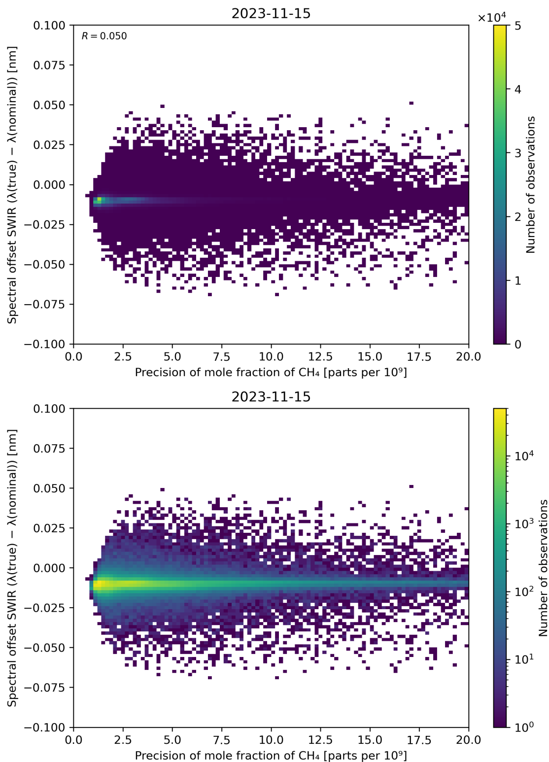
Figure 85: Scatter density plot of “Precision of mole fraction of \text{CH}_4 ” against “Spectral offset SWIR ( \lambda(\text{true}) - \lambda(\text{nominal}) )” for 2023-11-14 to 2023-11-16.
