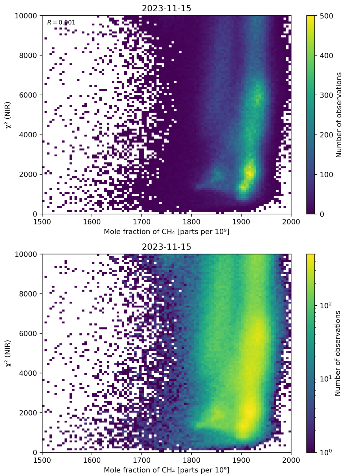
Figure 70: Scatter density plot of “Mole fraction of CH 4 ” against “ \chi^2 (NIR)” for 2023-11-14 to 2023-11-16.
