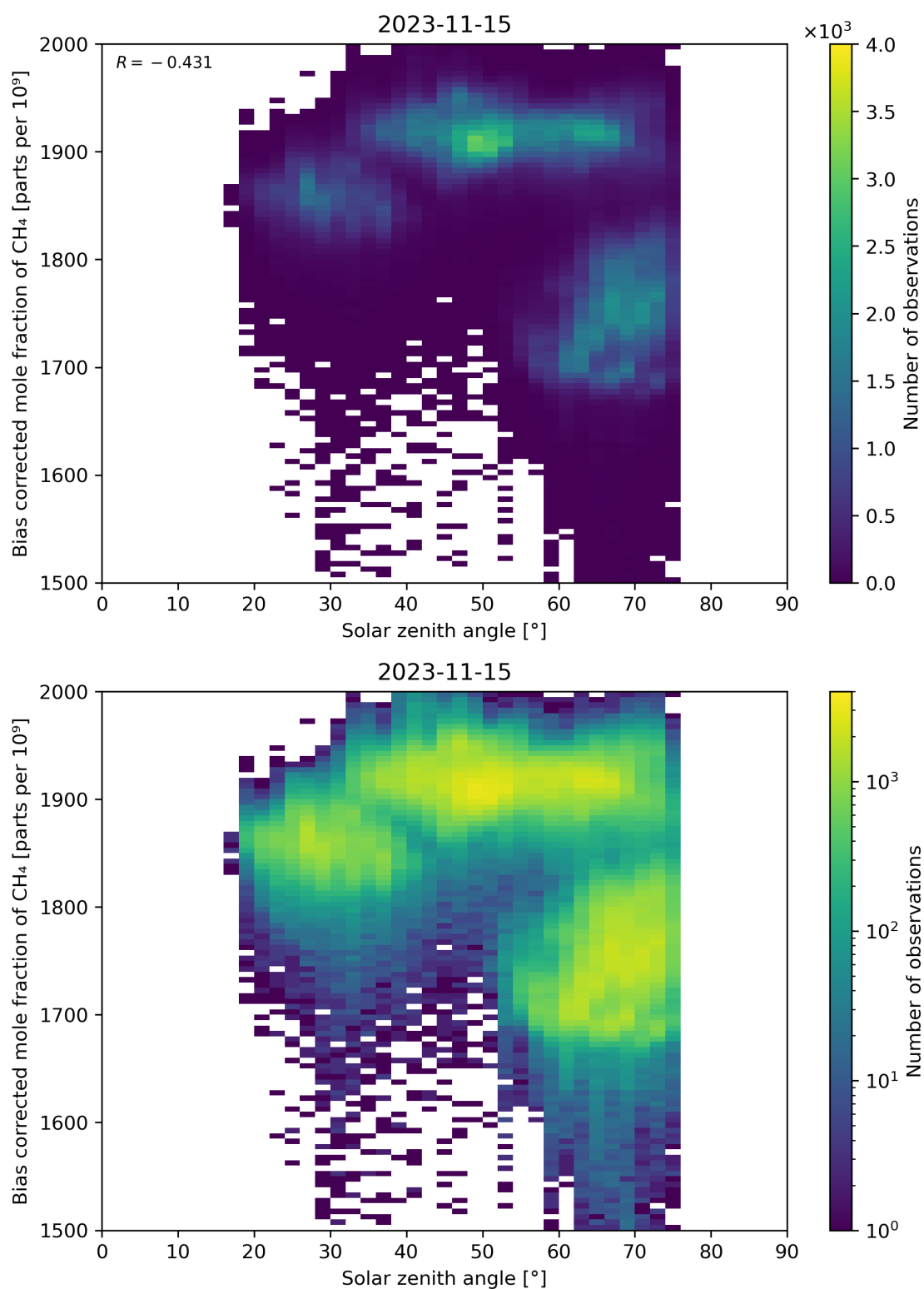
Figure 100: Scatter density plot of “Solar zenith angle” against “Bias corrected mole fraction of \text{CH}_4 ” for 2023-11-14 to 2023-11-16.
