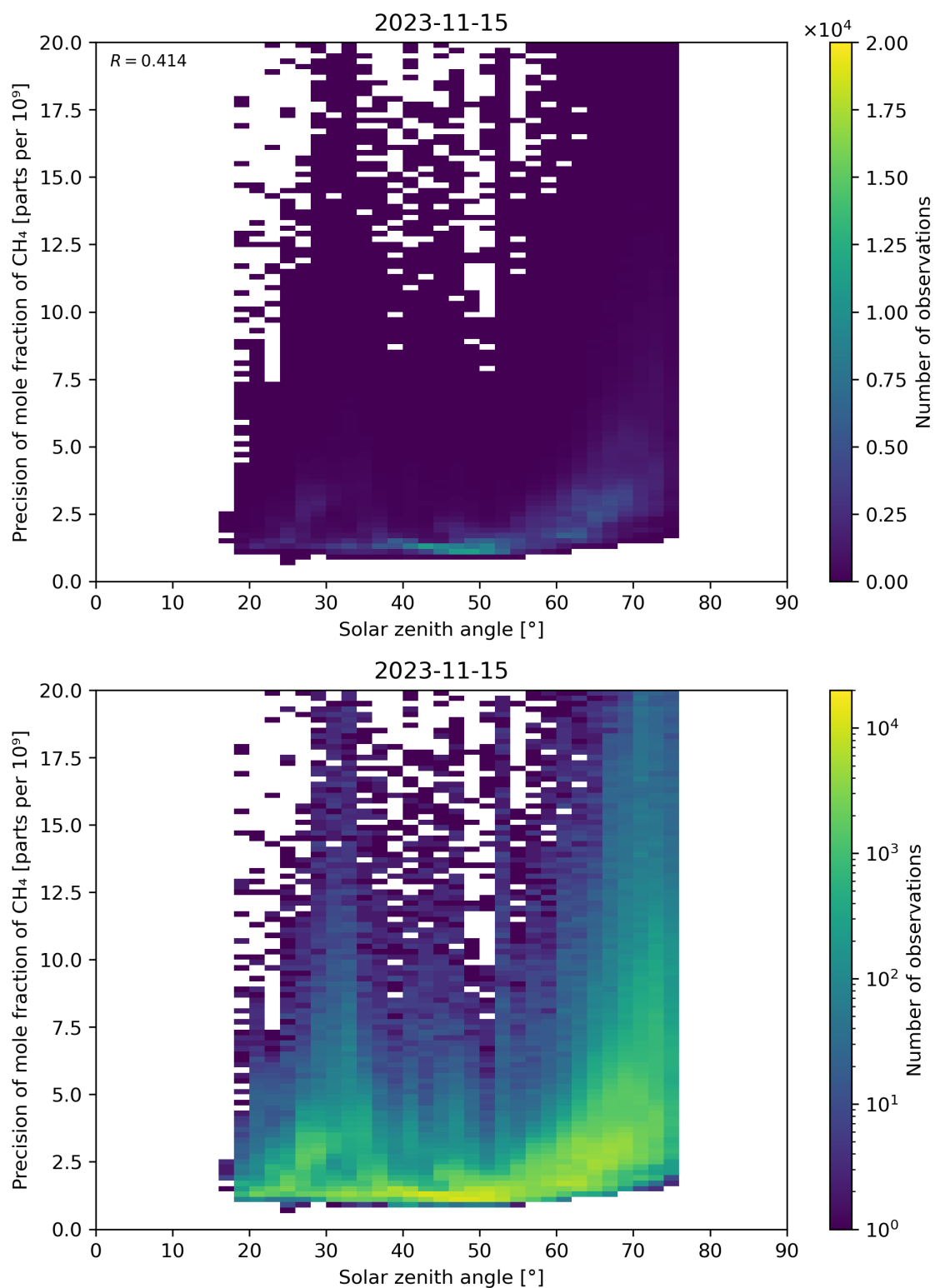
Figure 101: Scatter density plot of “Solar zenith angle” against “Precision of mole fraction of \text{CH}_4 ” for 2023-11-14 to 2023-11-16.
