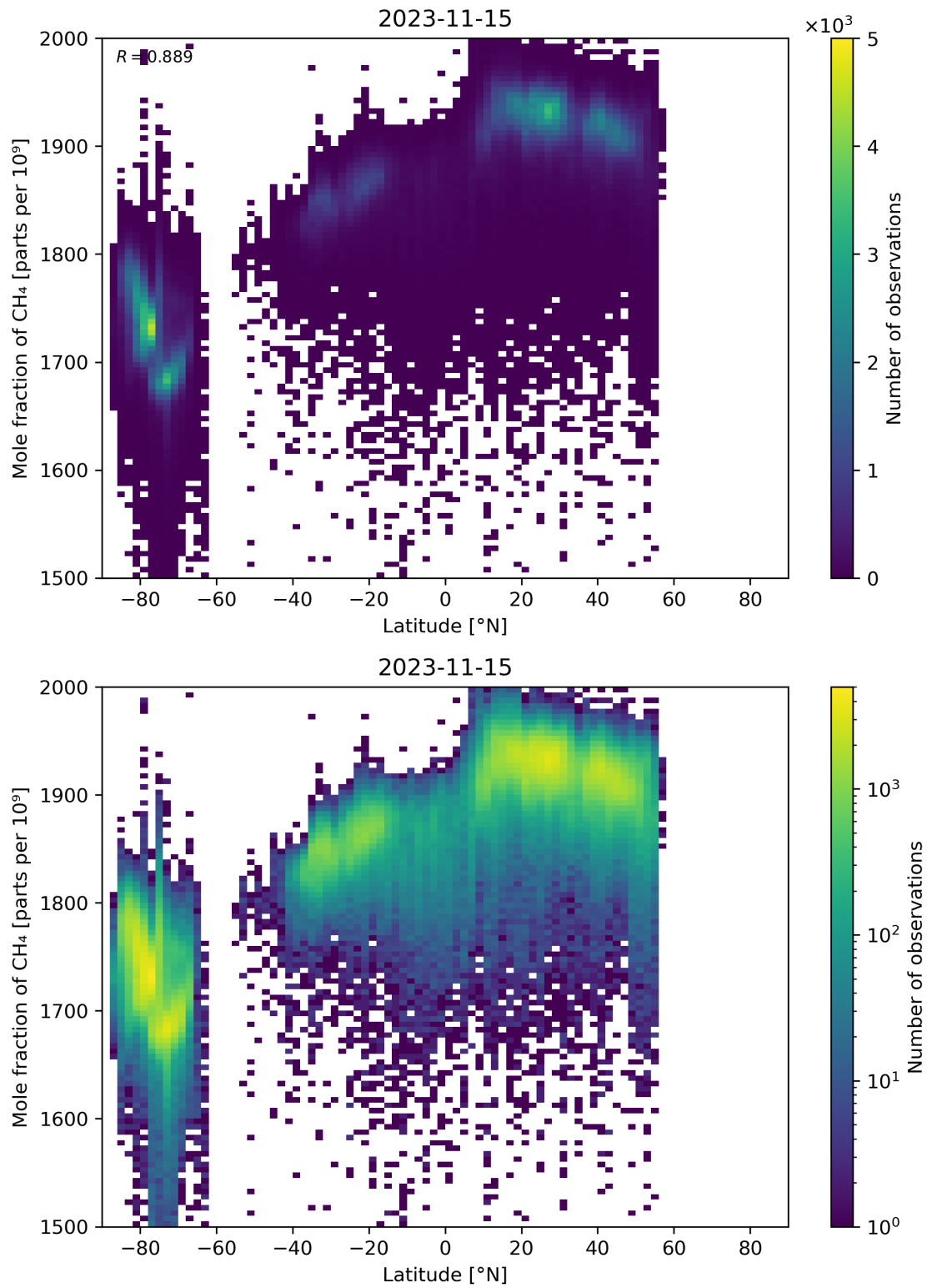
Figure 57: Scatter density plot of “Latitude” against “Mole fraction of CH 4 ” for 2023-11-14 to 2023-11-16.
