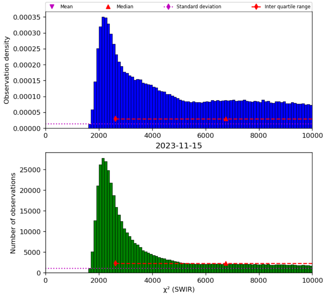
Figure 28: Histogram of “ \chi^2 (SWIR)” for 2023-11-14 to 2023-11-16
