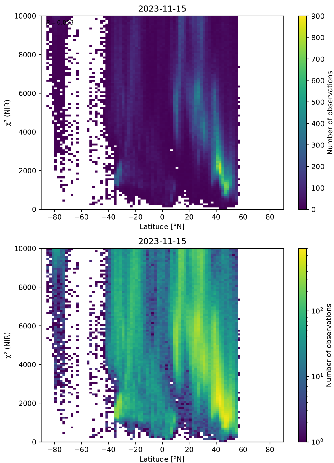
Figure 53: Scatter density plot of “Latitude” against “ \chi^2 (NIR)” for 2023-11-14 to 2023-11-16.
