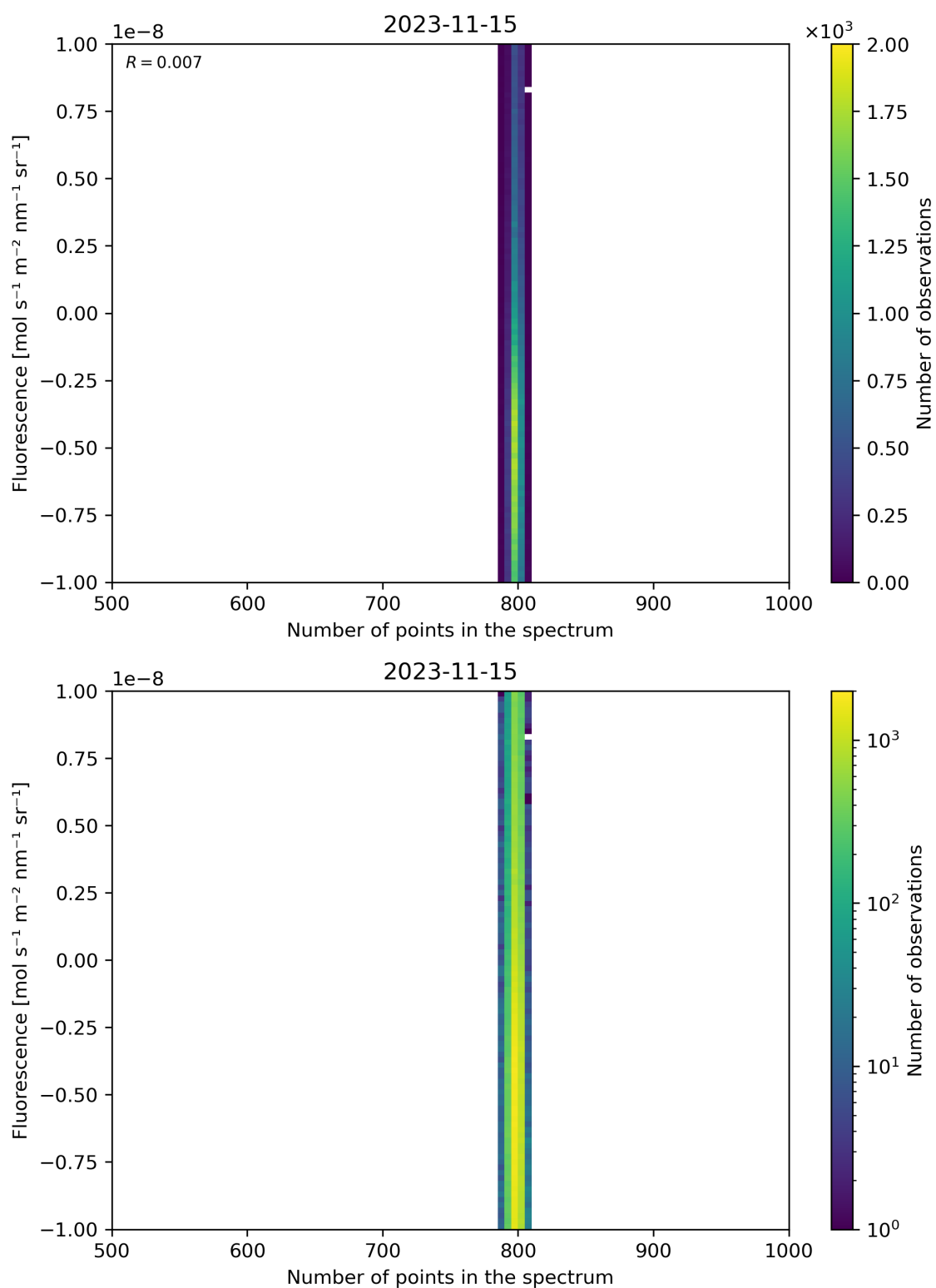
Figure 91: Scatter density plot of “Number of points in the spectrum” against “Fluorescence” for 2023-11-14 to 2023-11-16.
