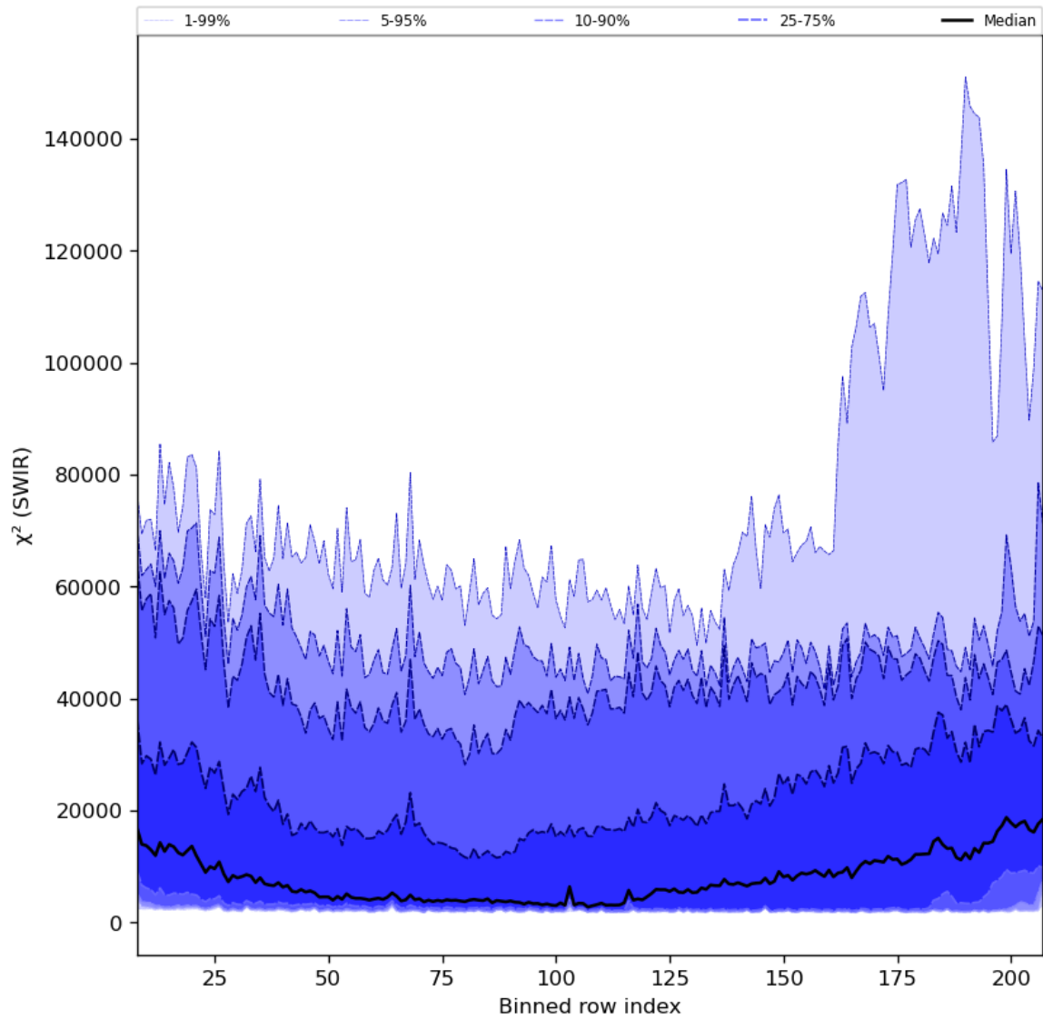
Figure 39: Along track statistics of “ \chi^2 (SWIR)” for 2023-11-14 to 2023-11-16
