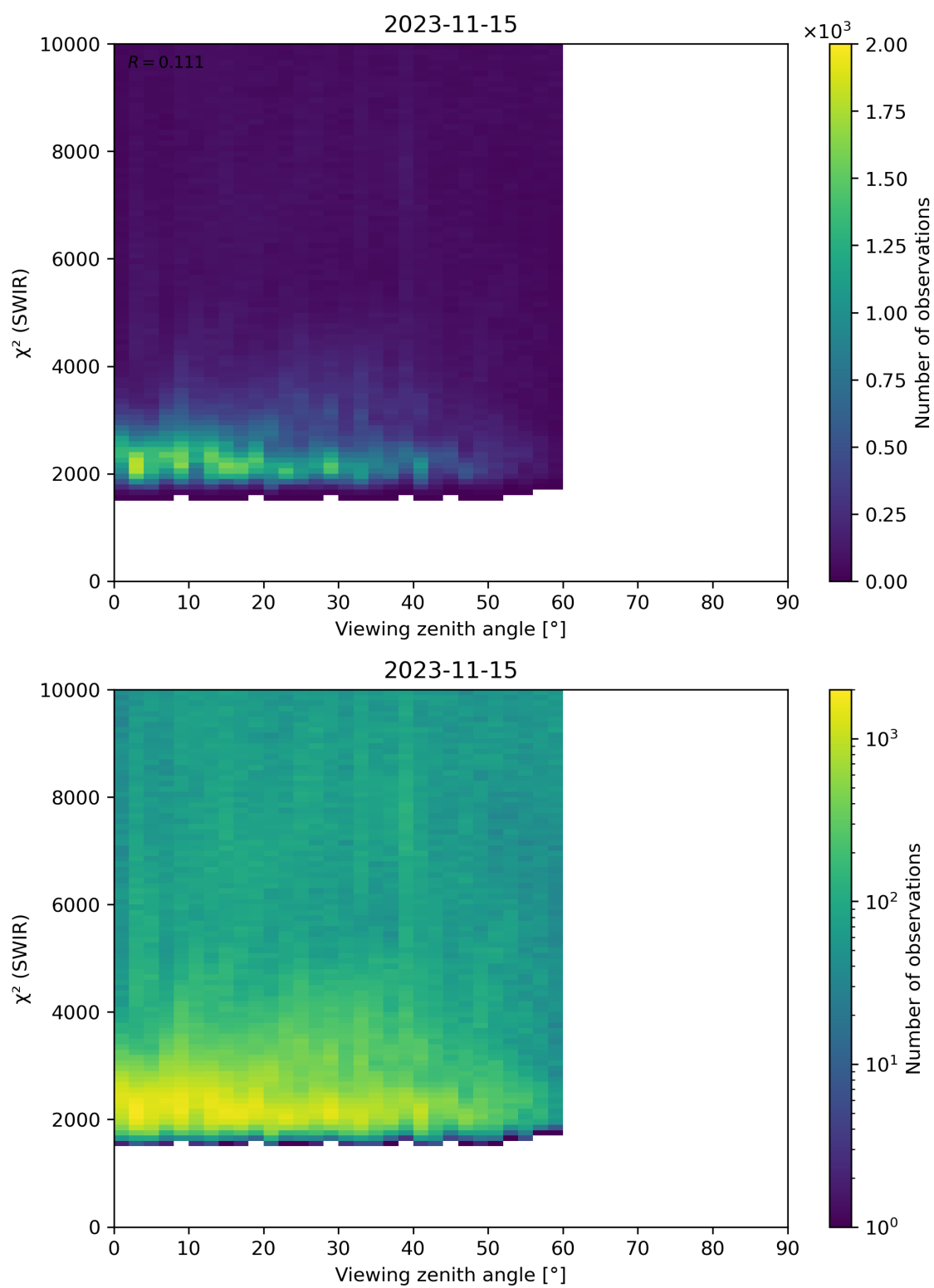
Figure 106: Scatter density plot of “Viewing zenith angle” against “ \chi^2 (SWIR)” for 2023-11-14 to 2023-11-16.
