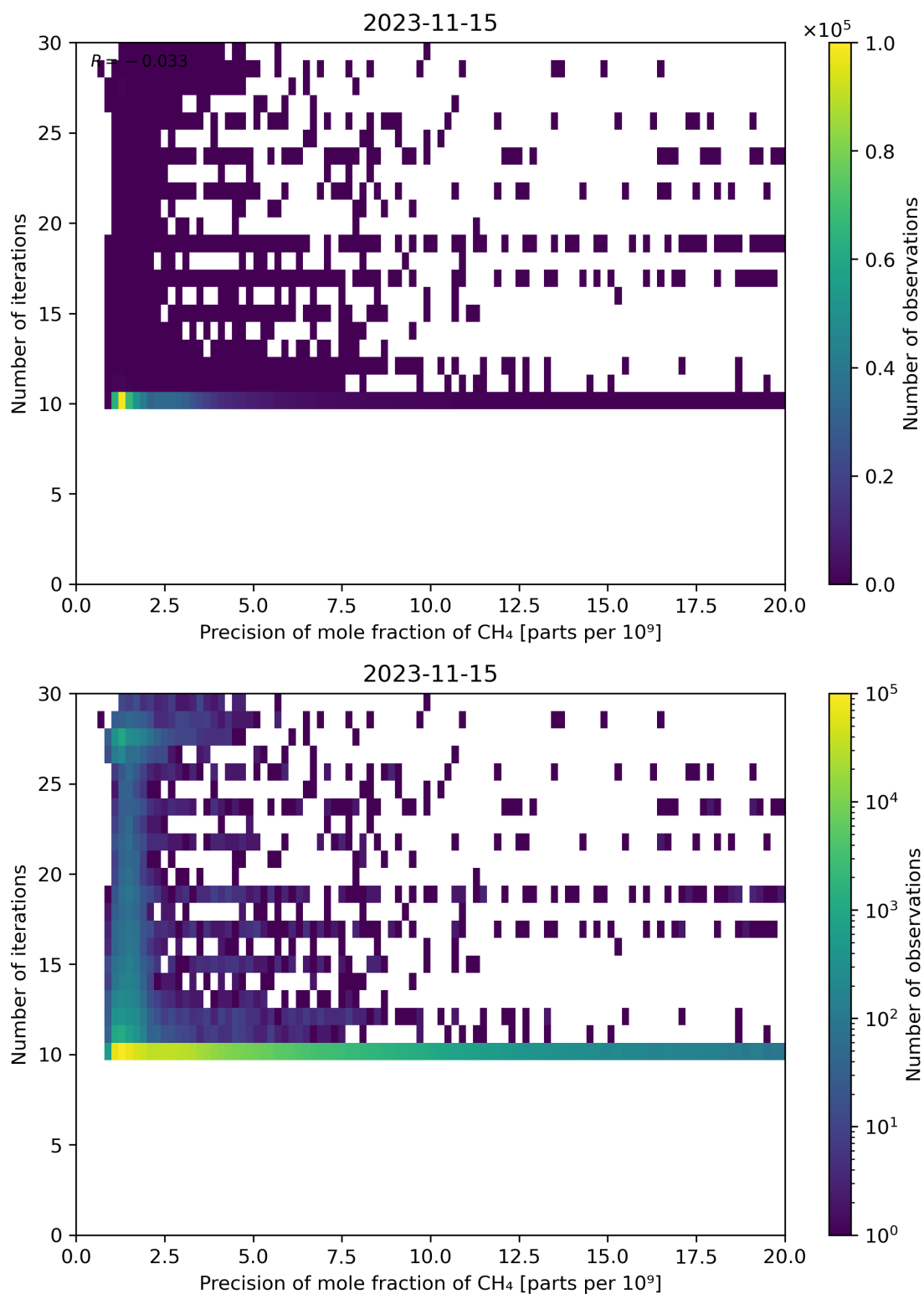
Figure 83: Scatter density plot of “Precision of mole fraction of CH 4 ” against “Number of iterations” for 2023-11-14 to 2023-11-16.
