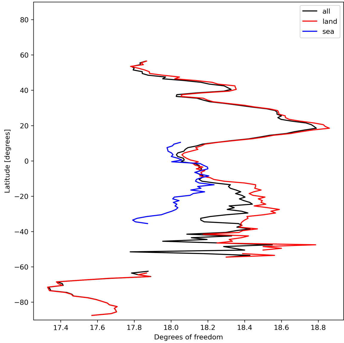
Figure 19: Zonal average of “Degrees of freedom” for 2023-11-14 to 2023-11-16.
