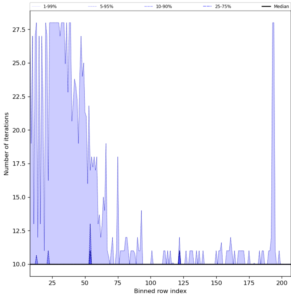
Figure 42: Along track statistics of “Number of iterations” for 2023-11-14 to 2023-11-16
