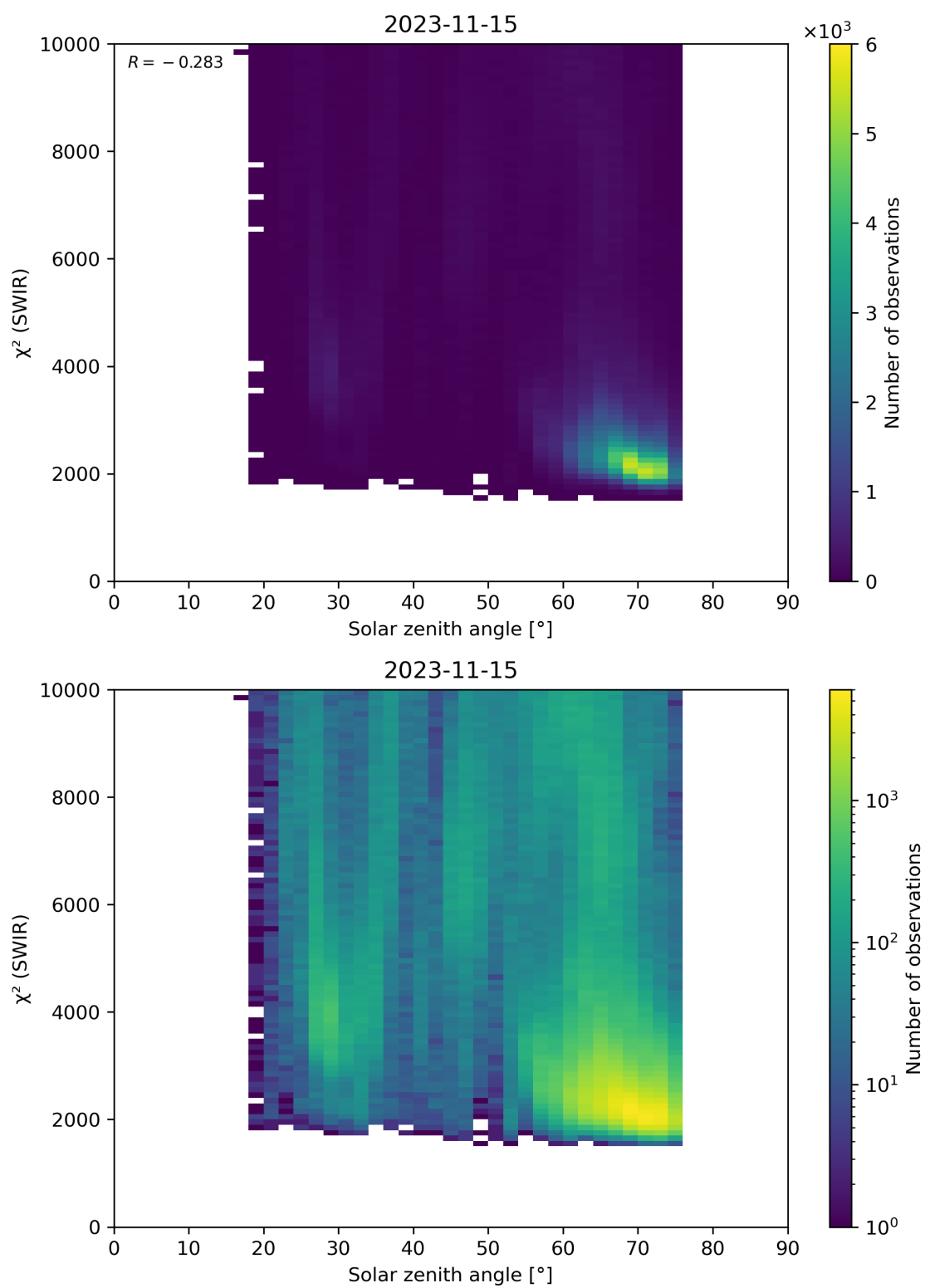
Figure 95: Scatter density plot of “Solar zenith angle” against “ \chi^2 (SWIR)” for 2023-11-14 to 2023-11-16.
