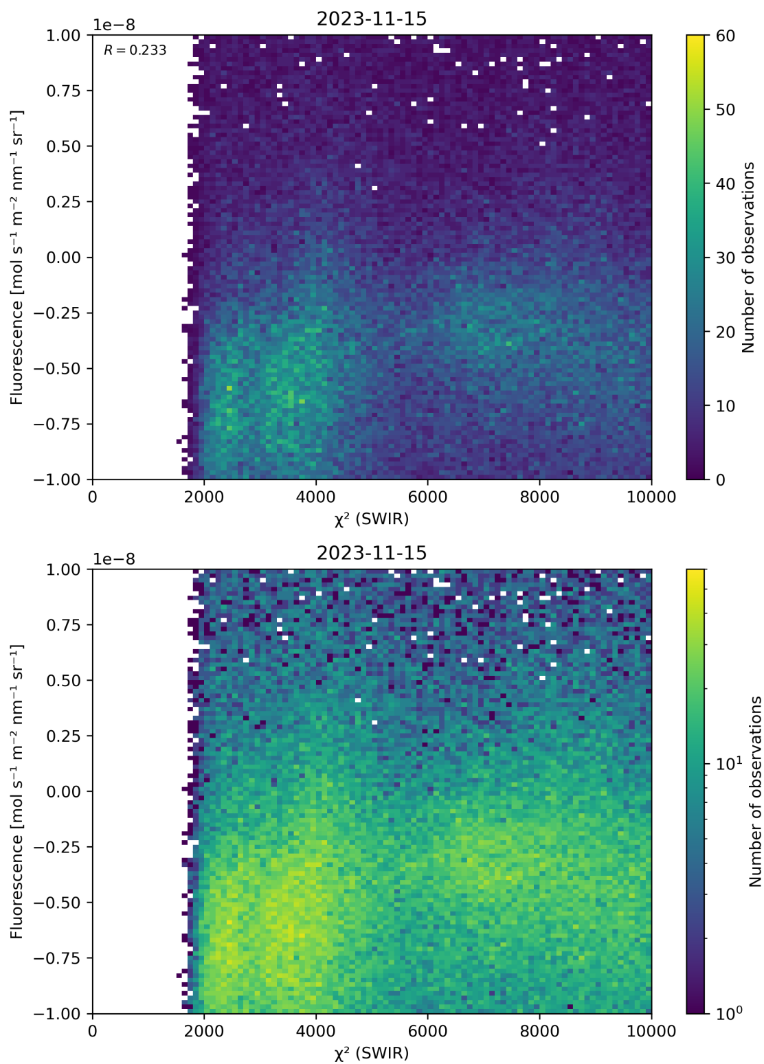
Figure 49: Scatter density plot of “ \chi^2 (SWIR)” against “Fluorescence” for 2023-11-14 to 2023-11-16.
