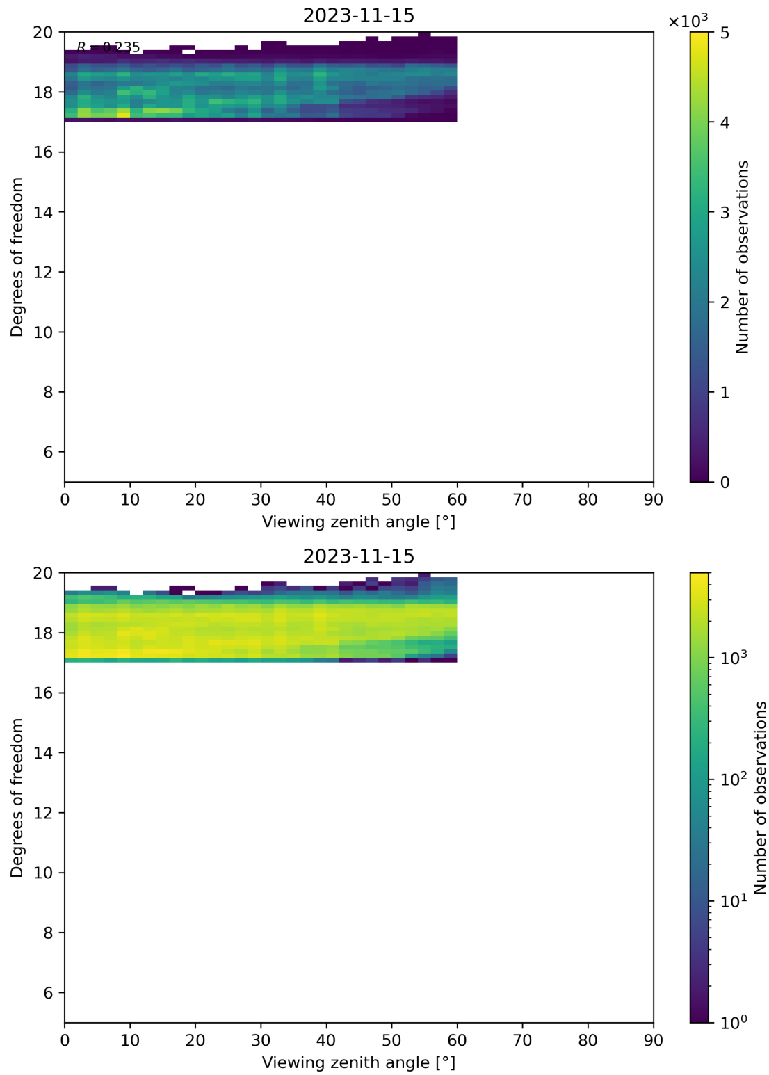
Figure 107: Scatter density plot of “Viewing zenith angle” against “Degrees of freedom” for 2023-11-14 to 2023-11-16.
