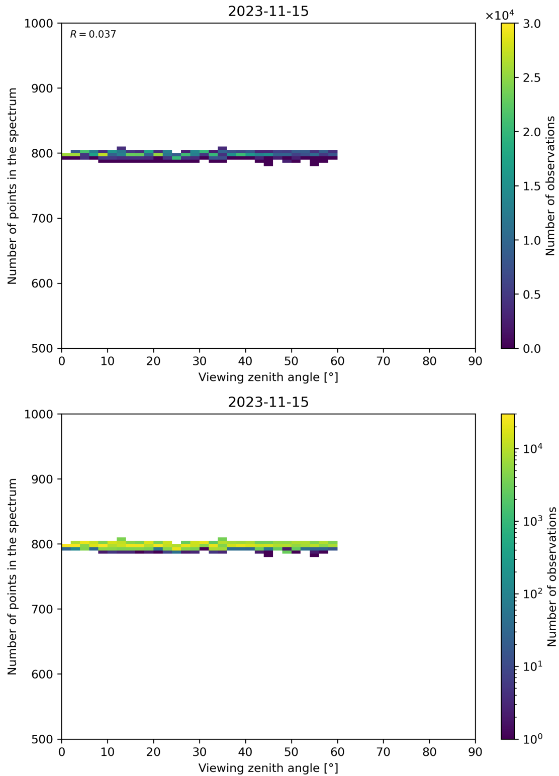
Figure 114: Scatter density plot of “Viewing zenith angle” against “Number of points in the spectrum” for 2023-11-14 to 2023-11-16.
