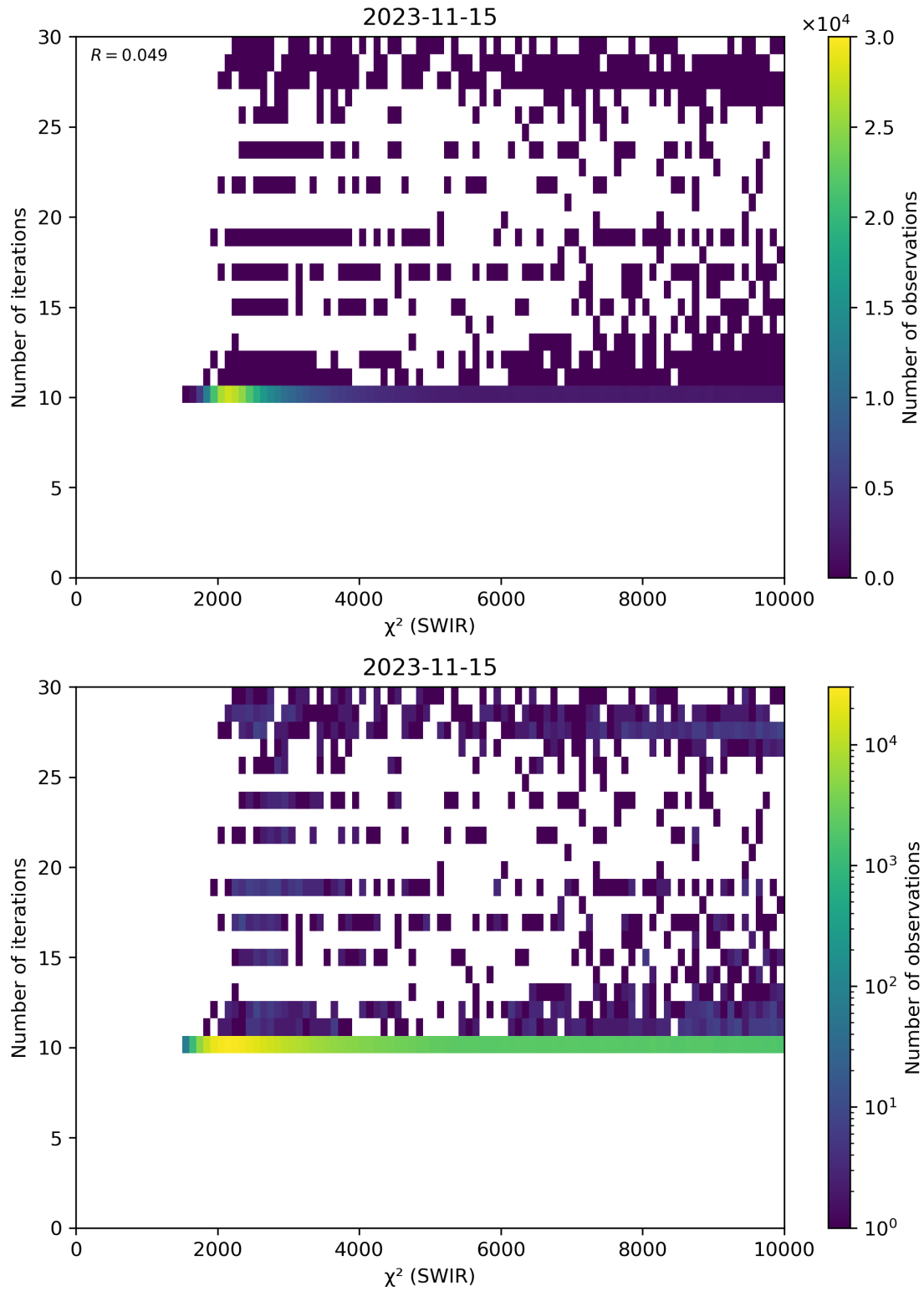
Figure 50: Scatter density plot of “ \chi^2 (SWIR)” against “Number of iterations” for 2023-11-14 to 2023-11-16.
