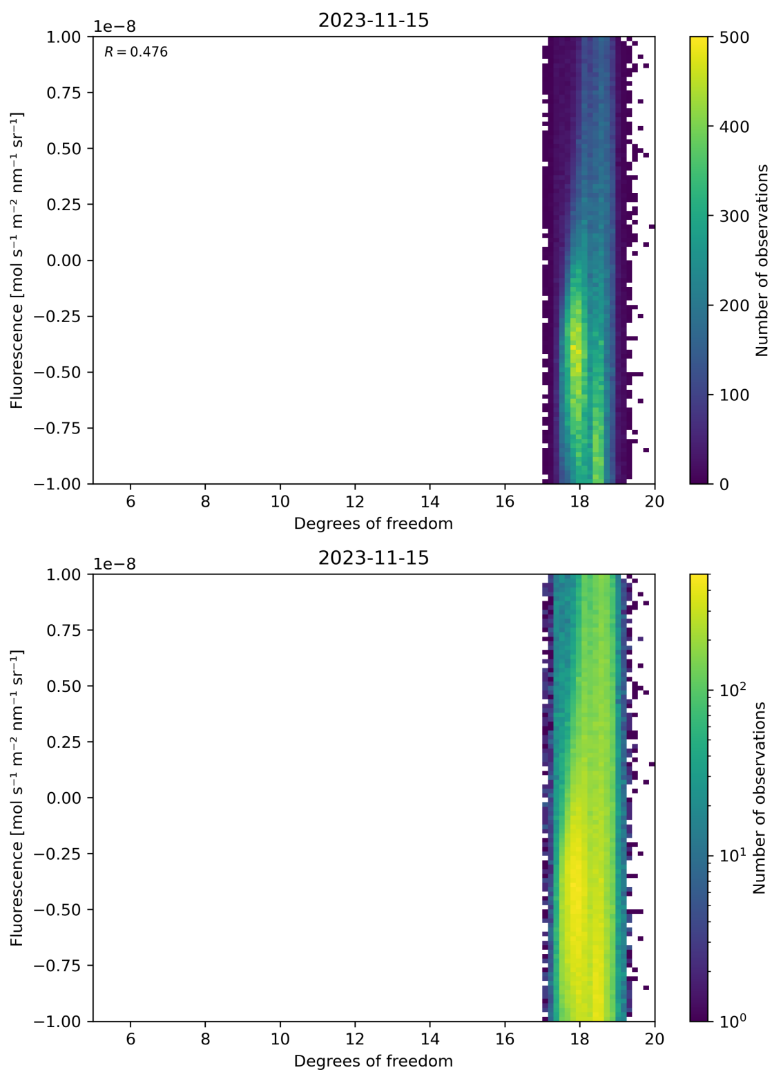
Figure 51: Scatter density plot of “Degrees of freedom” against “Fluorescence” for 2023-11-14 to 2023-11-16.
