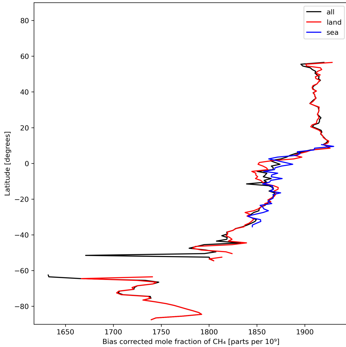
Figure 14: Zonal average of “Bias corrected mole fraction of CH 4 ” for 2023-11-14 to 2023-11-16.
