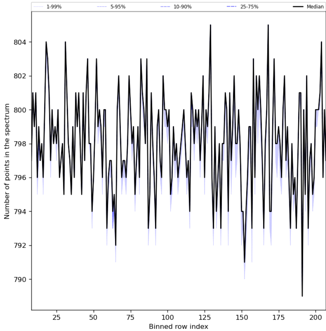
Figure 37: Along track statistics of “Number of points in the spectrum” for 2023-11-14 to 2023-11-16
