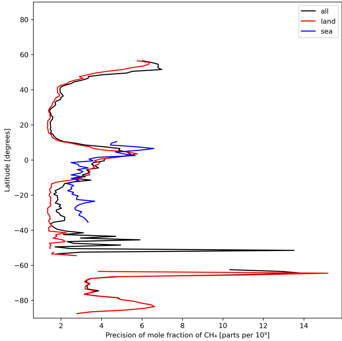
Figure 13: Zonal average of “Precision of mole fraction of CH 4 ” for 2023-11-14 to 2023-11-16.
