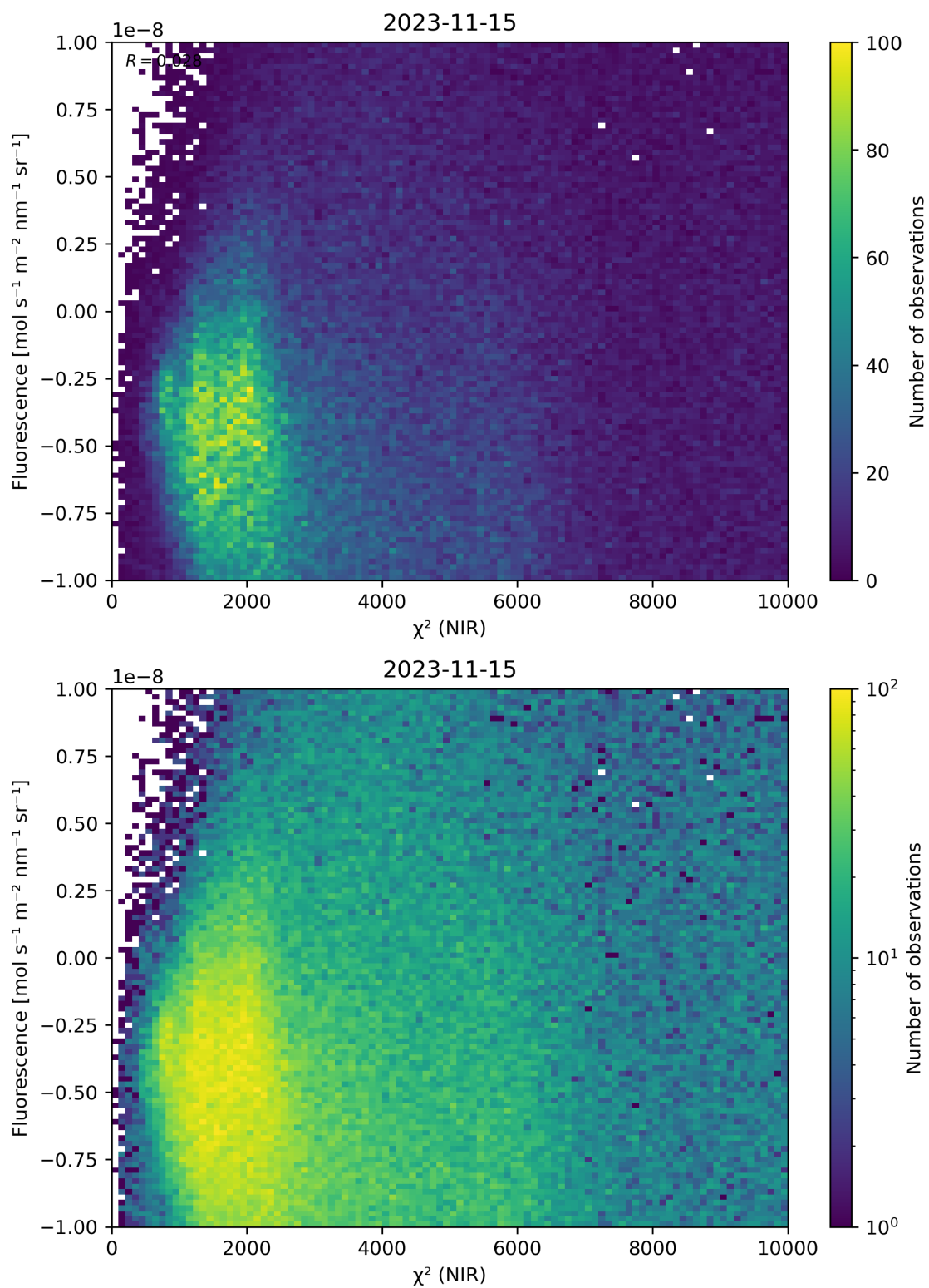
Figure 45: Scatter density plot of “ \chi^2 (NIR)” against “Fluorescence” for 2023-11-14 to 2023-11-16.
