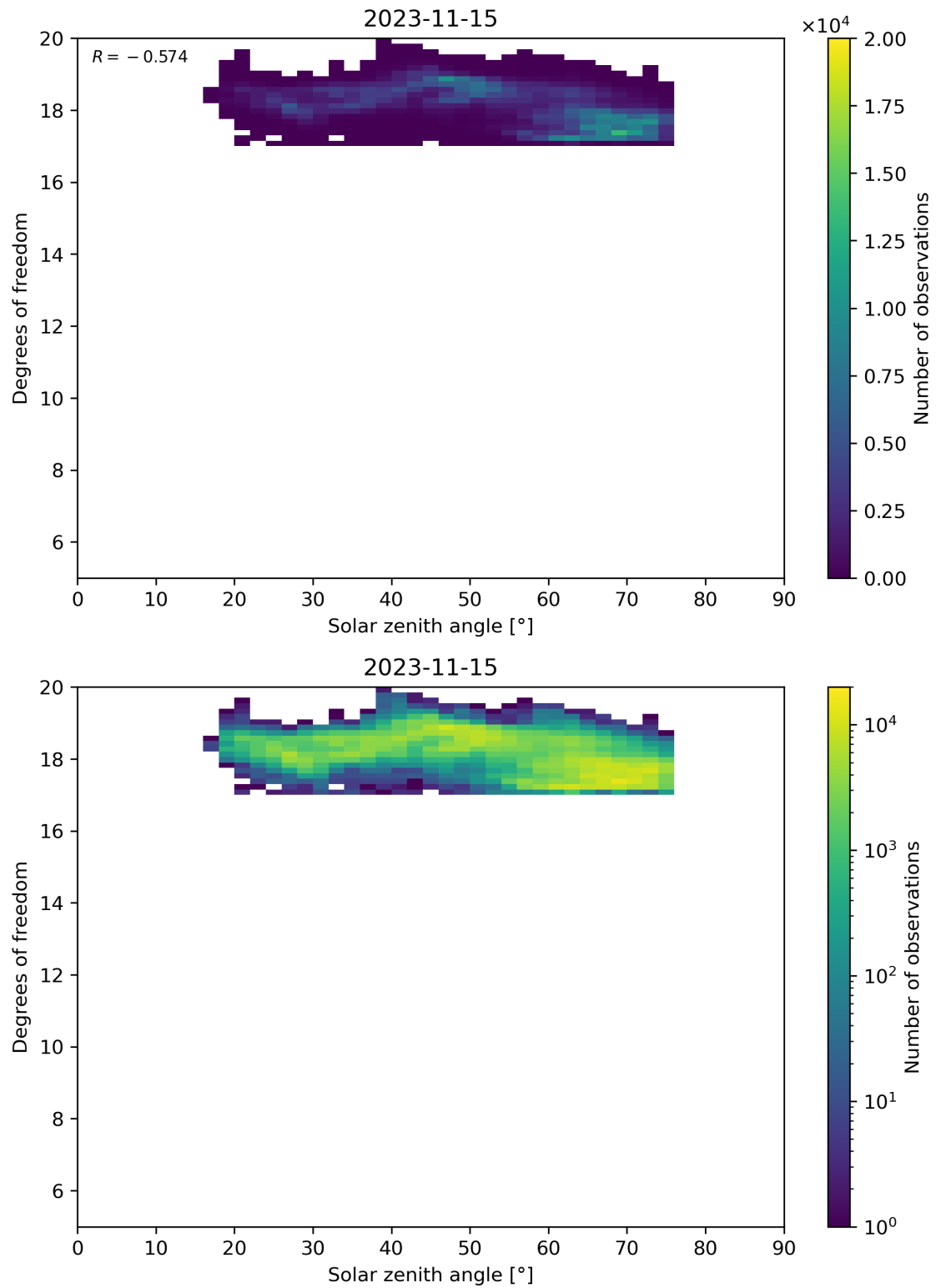
Figure 96: Scatter density plot of “Solar zenith angle” against “Degrees of freedom” for 2023-11-14 to 2023-11-16.
