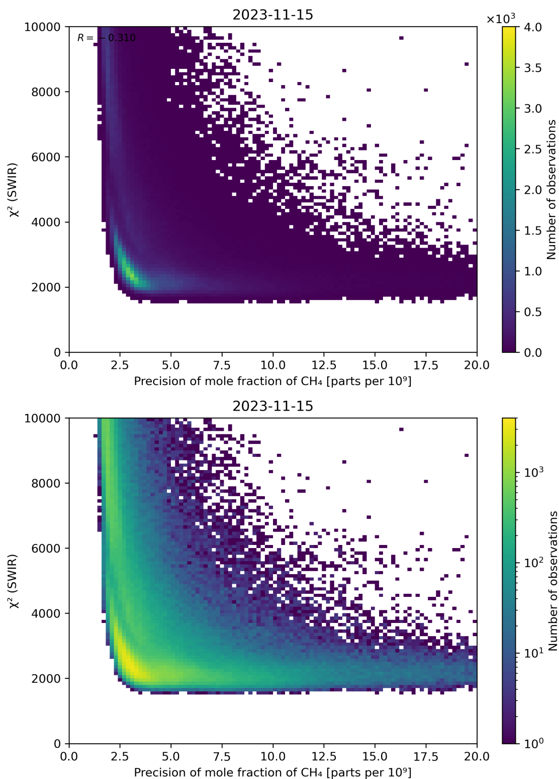
Figure 79: Scatter density plot of “Precision of mole fraction of CH 4 ” against “ \chi^2 (SWIR)” for 2023-11-14 to 2023-11-16.
