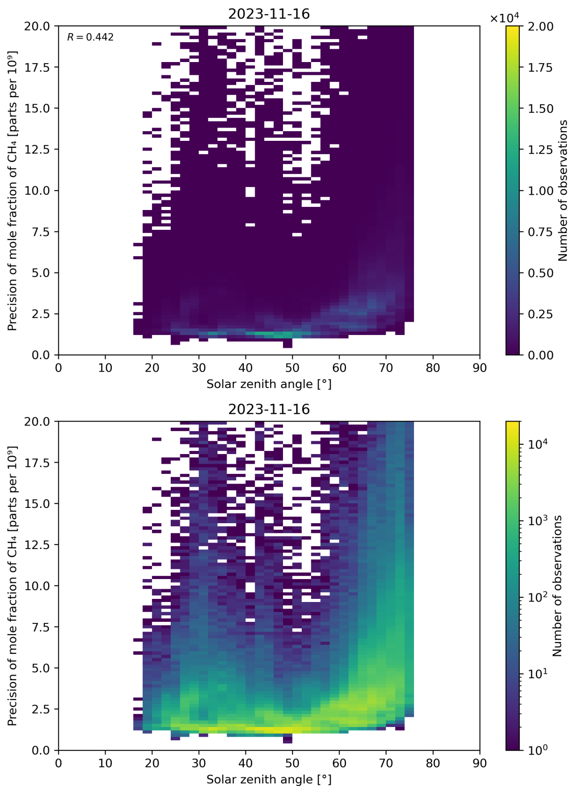
Figure 101: Scatter density plot of “Solar zenith angle” against “Precision of mole fraction of \text{CH}_4 ” for 2023-11-15 to 2023-11-17.
