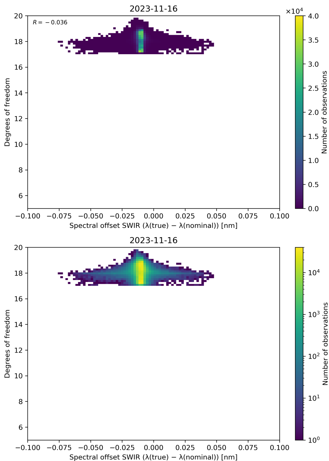
Figure 119: Scatter density plot of “Spectral offset SWIR ( \lambda(\text{true}) - \lambda(\text{nominal}) )” against “Degrees of freedom” for 2023-11-15 to 2023-11-17.
