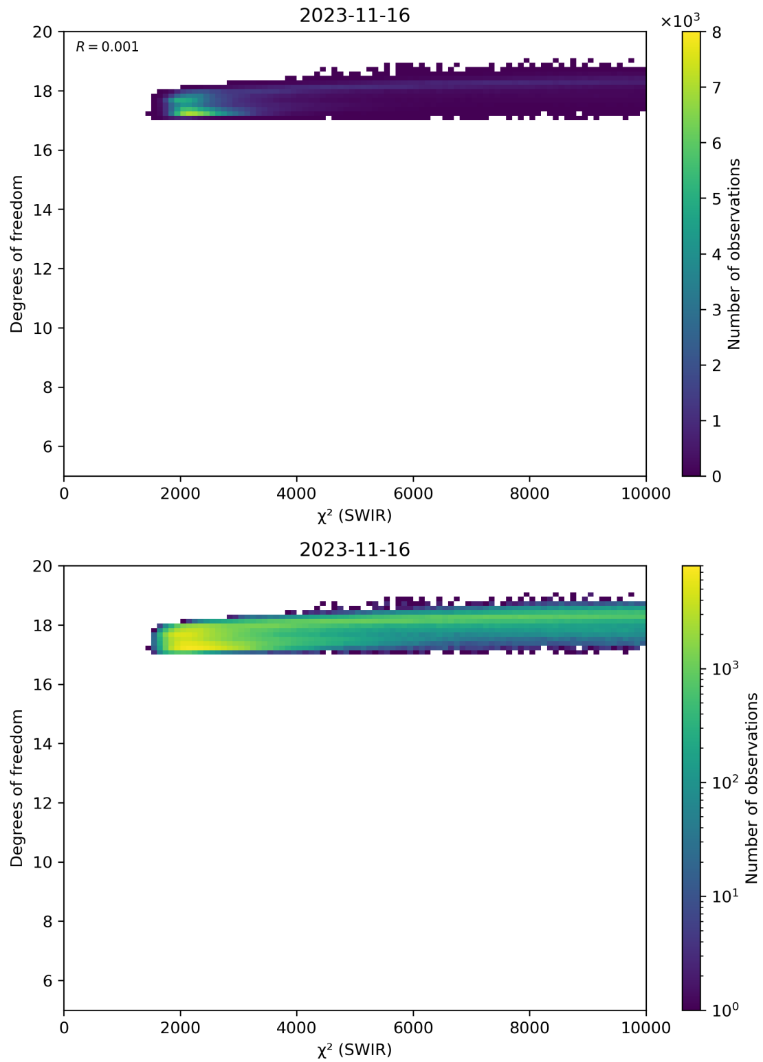
Figure 48: Scatter density plot of “ \chi^2 (SWIR)” against “Degrees of freedom” for 2023-11-15 to 2023-11-17.
