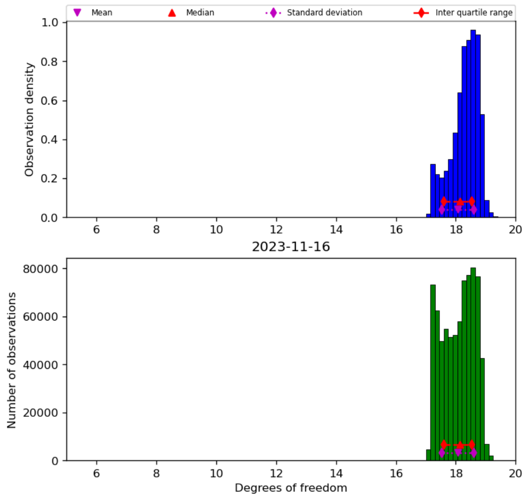
Figure 30: Histogram of “Degrees of freedom” for 2023-11-15 to 2023-11-17
