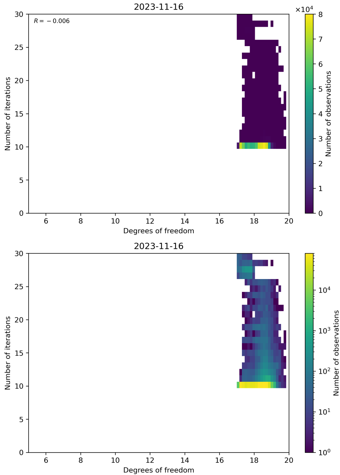
Figure 52: Scatter density plot of “Degrees of freedom” against “Number of iterations” for 2023-11-15 to 2023-11-17.
