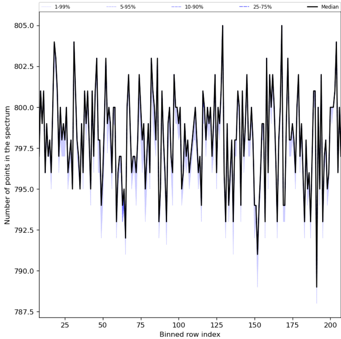
Figure 37: Along track statistics of “Number of points in the spectrum” for 2023-11-15 to 2023-11-17
