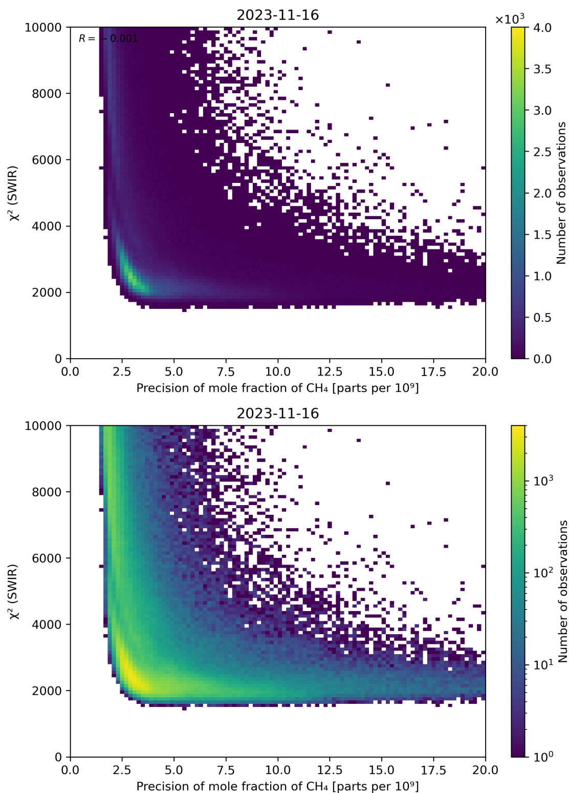
Figure 79: Scatter density plot of “Precision of mole fraction of \text{CH}_4 ” against “ \chi^2 (SWIR)” for 2023-11-15 to 2023-11-17.
