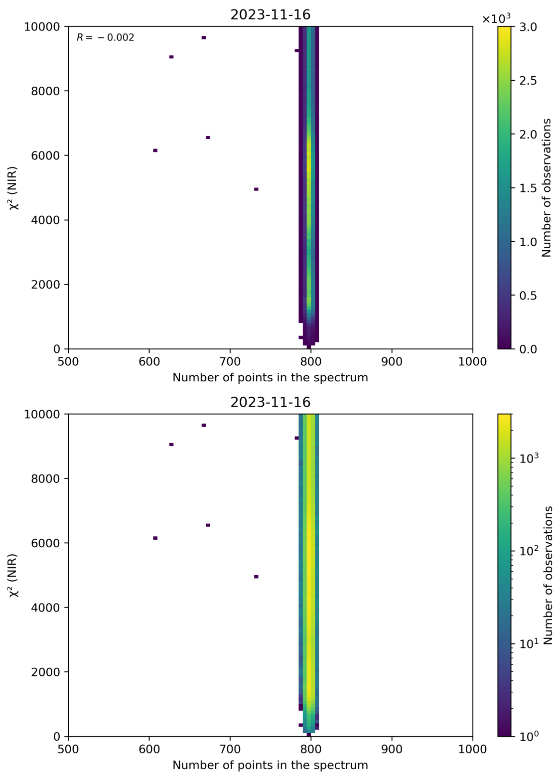
Figure 88: Scatter density plot of “Number of points in the spectrum” against “ \chi^2 (NIR)” for 2023-11-15 to 2023-11-17.
