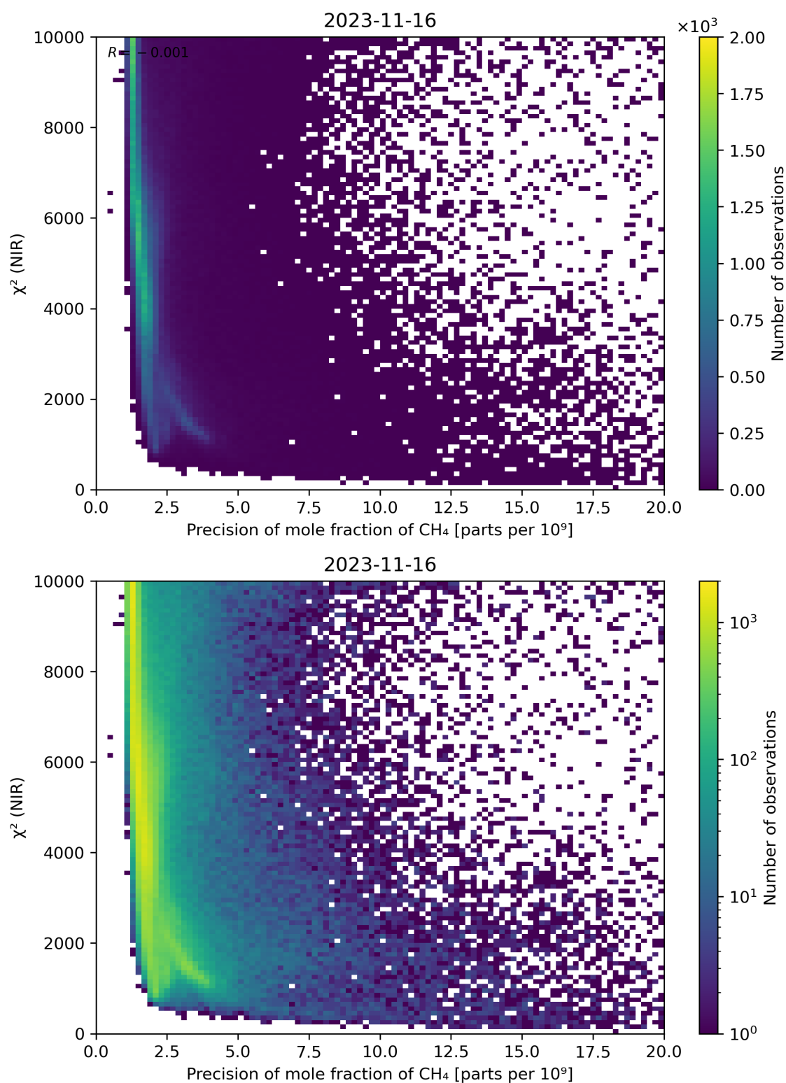
Figure 78: Scatter density plot of “Precision of mole fraction of \text{CH}_4 ” against “ \chi^2 (NIR)” for 2023-11-15 to 2023-11-17.
