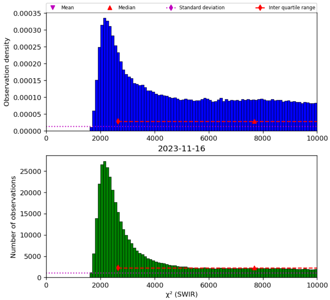
Figure 28: Histogram of “ \chi^2 (SWIR)” for 2023-11-15 to 2023-11-17
