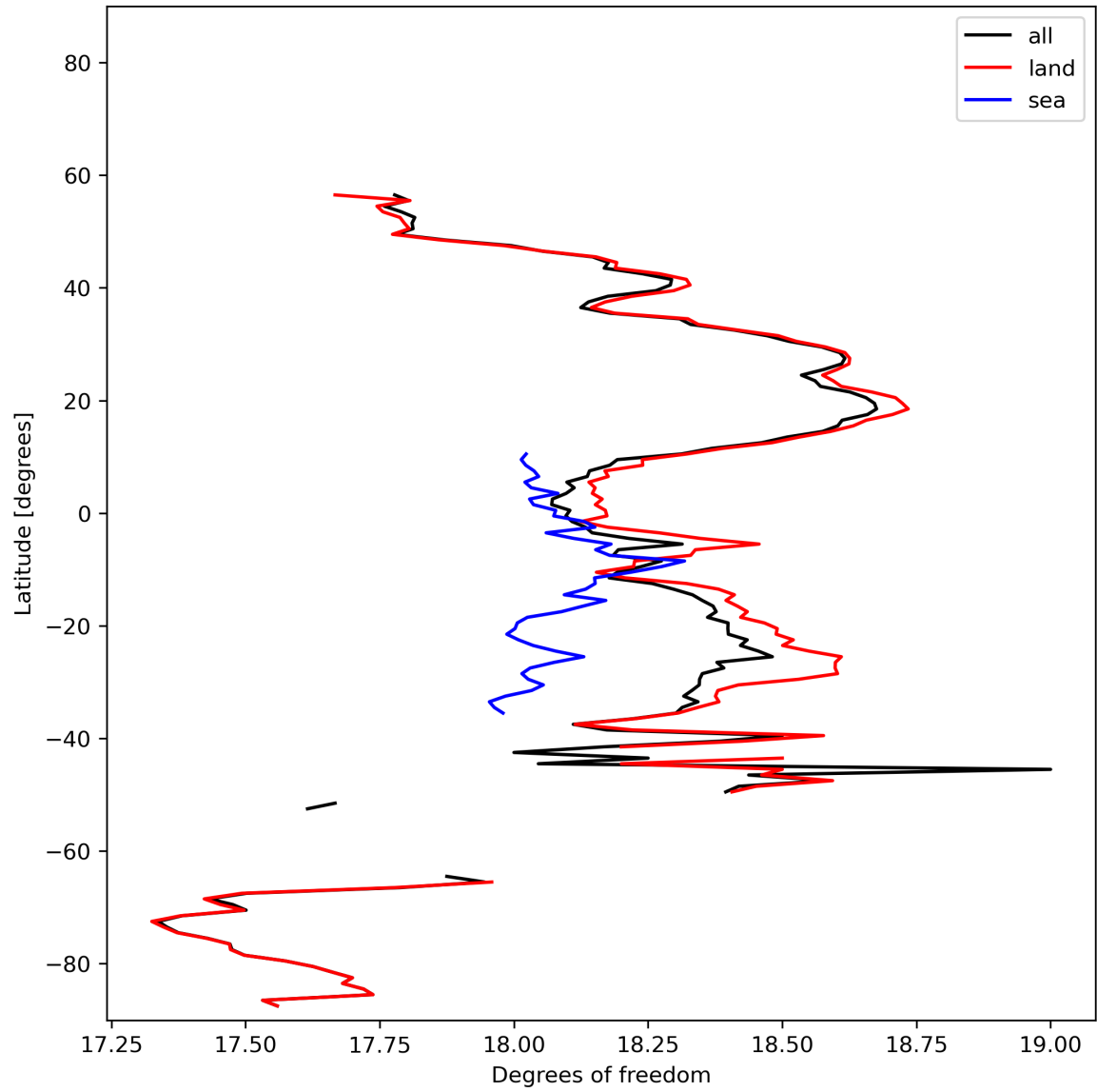
Figure 19: Zonal average of “Degrees of freedom” for 2023-11-15 to 2023-11-17.
