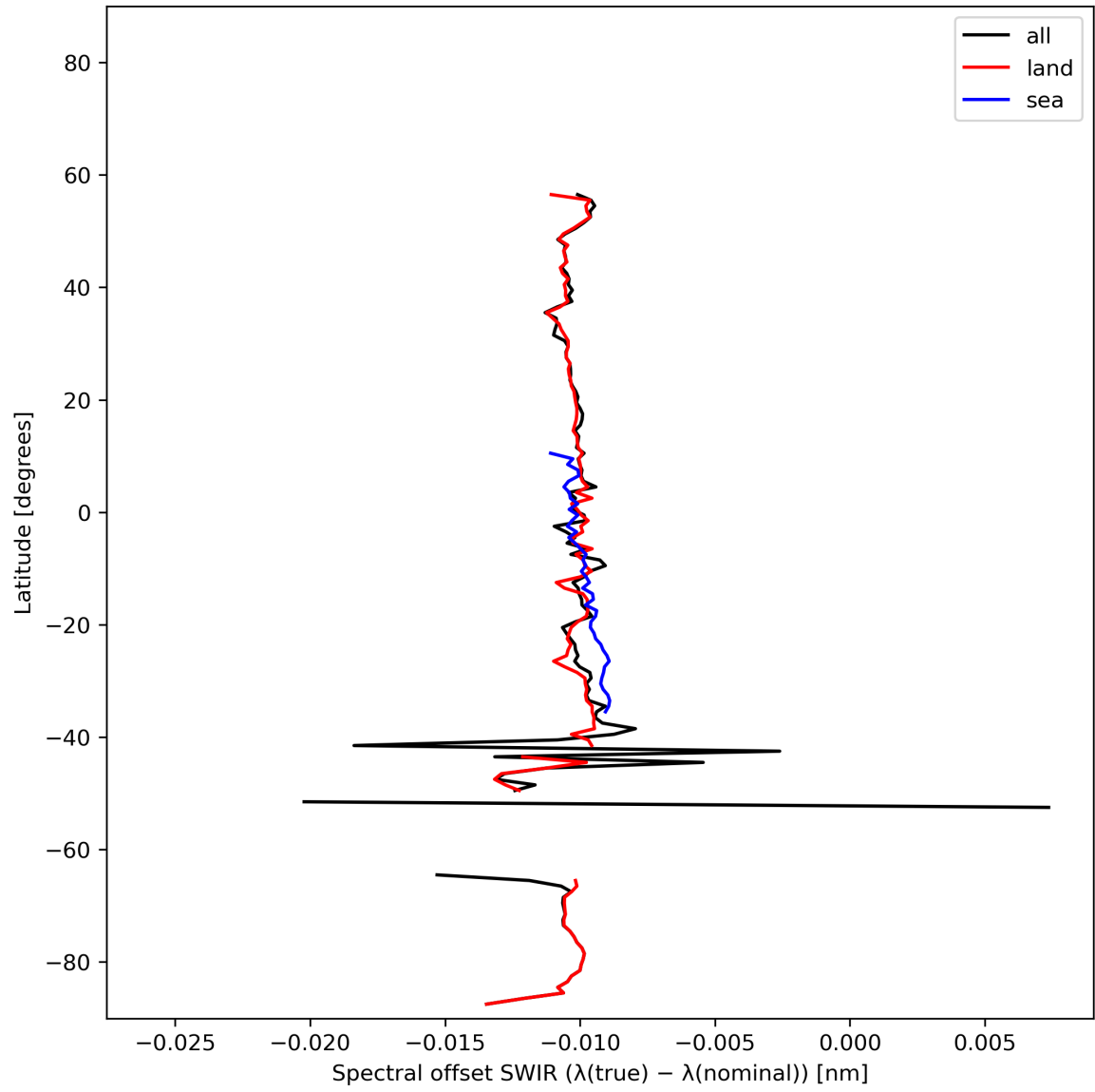
Figure 16: Zonal average of “Spectral offset SWIR ( \lambda(\text{true}) - \lambda(\text{nominal}) )” for 2023-11-15 to 2023-11-17.
