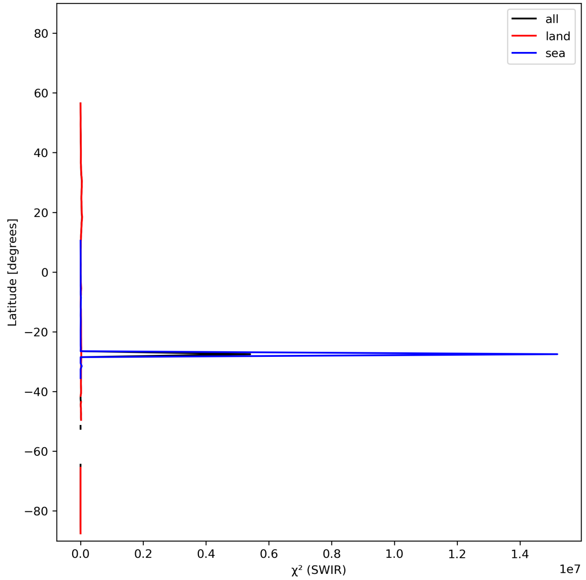
Figure 17: Zonal average of “ \chi^2 (SWIR)” for 2023-11-15 to 2023-11-17.
