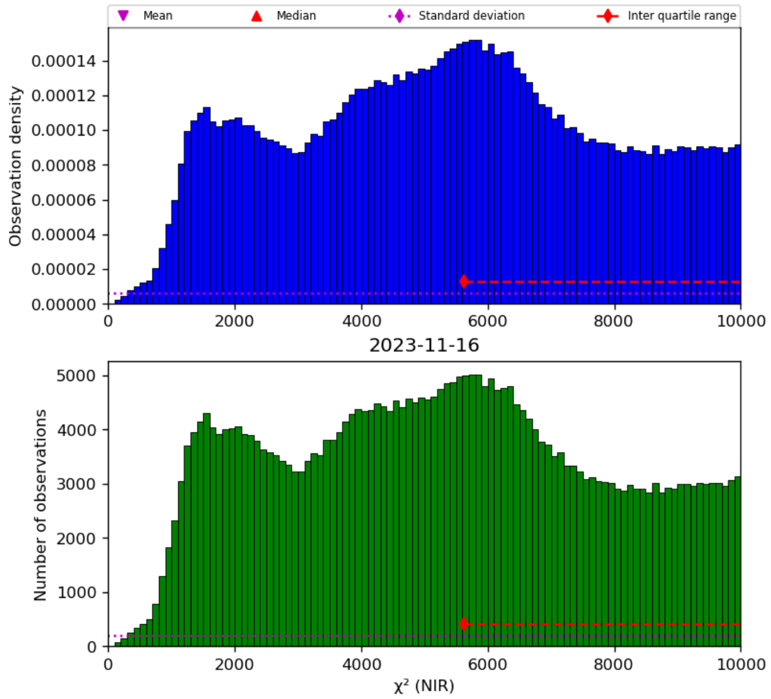
Figure 29: Histogram of “ \chi^2 (NIR)” for 2023-11-15 to 2023-11-17
