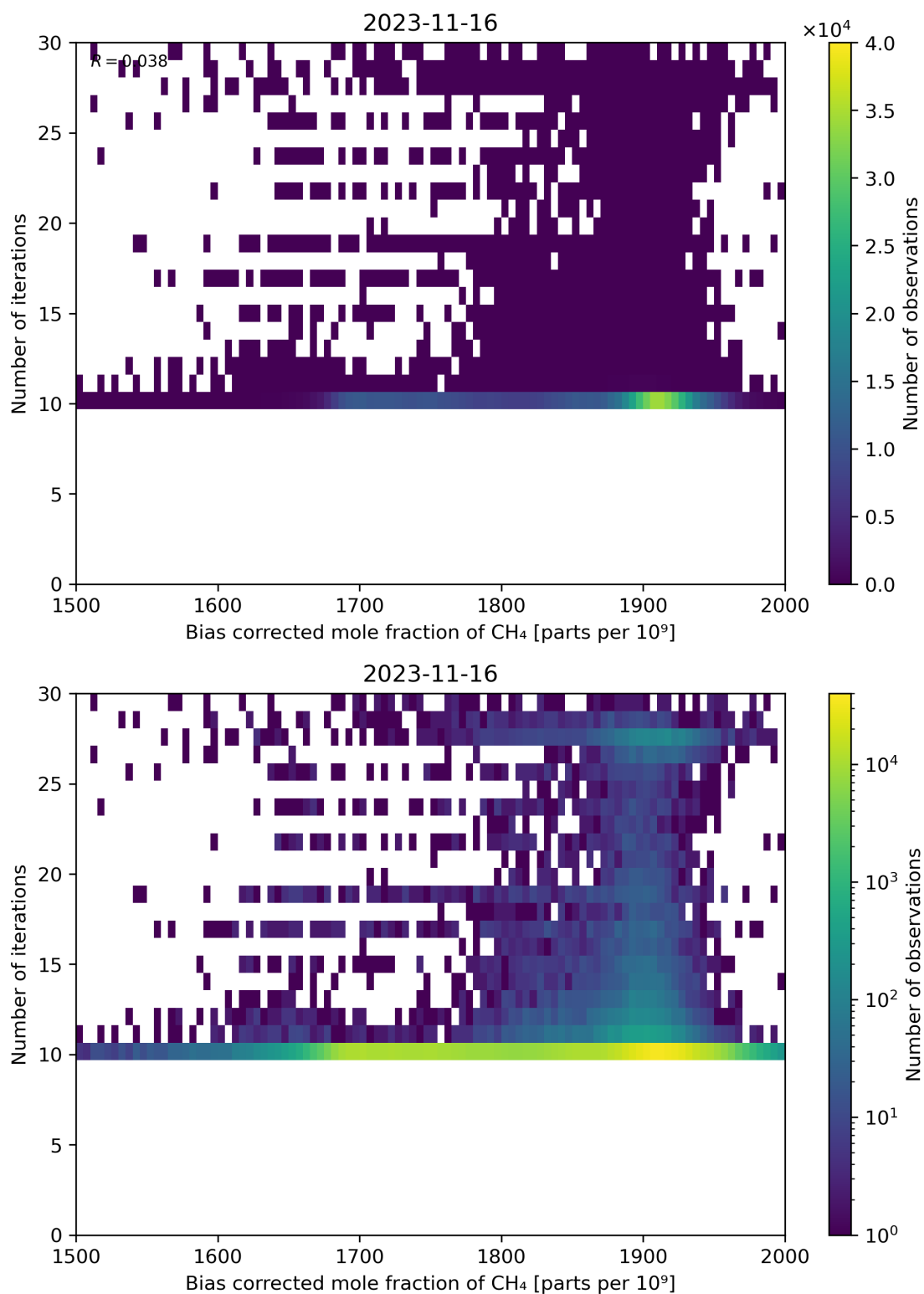
Figure 67: Scatter density plot of “Bias corrected mole fraction of CH 4 ” against “Number of iterations” for 2023-11-15 to 2023-11-17.
