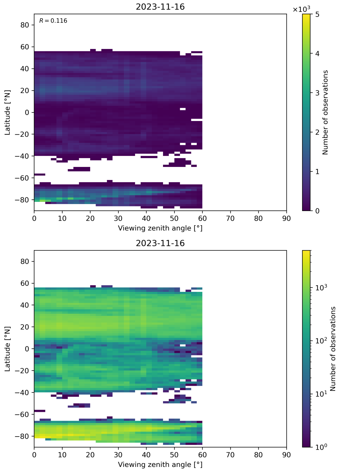
Figure 109: Scatter density plot of “Viewing zenith angle” against “Latitude” for 2023-11-15 to 2023-11-17.
