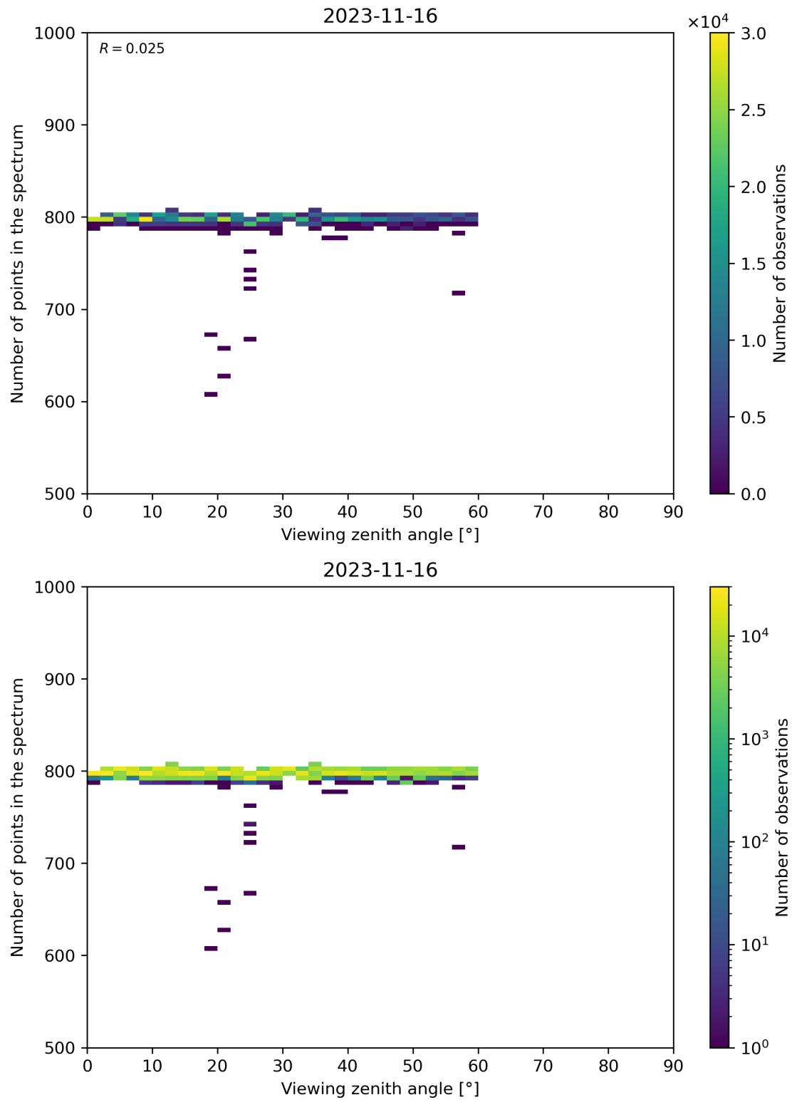
Figure 114: Scatter density plot of “Viewing zenith angle” against “Number of points in the spectrum” for 2023-11-15 to 2023-11-17.
