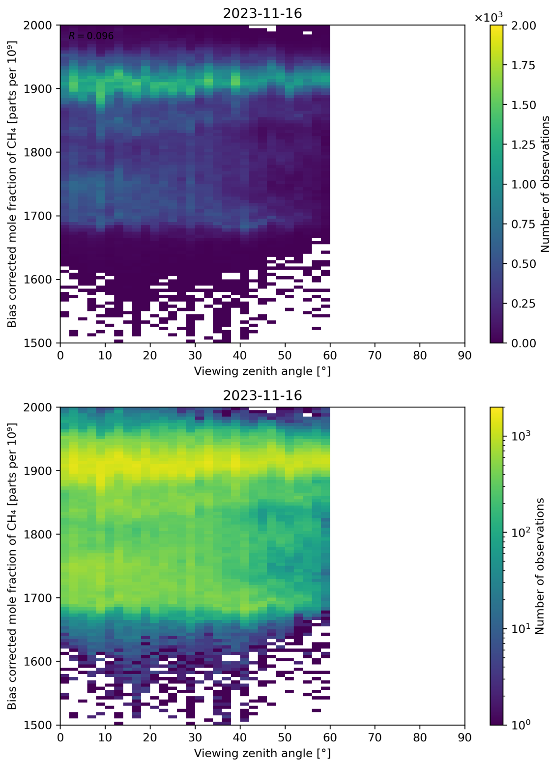
Figure 111: Scatter density plot of “Viewing zenith angle” against “Bias corrected mole fraction of CH 4 ” for 2023-11-15 to 2023-11-17.
