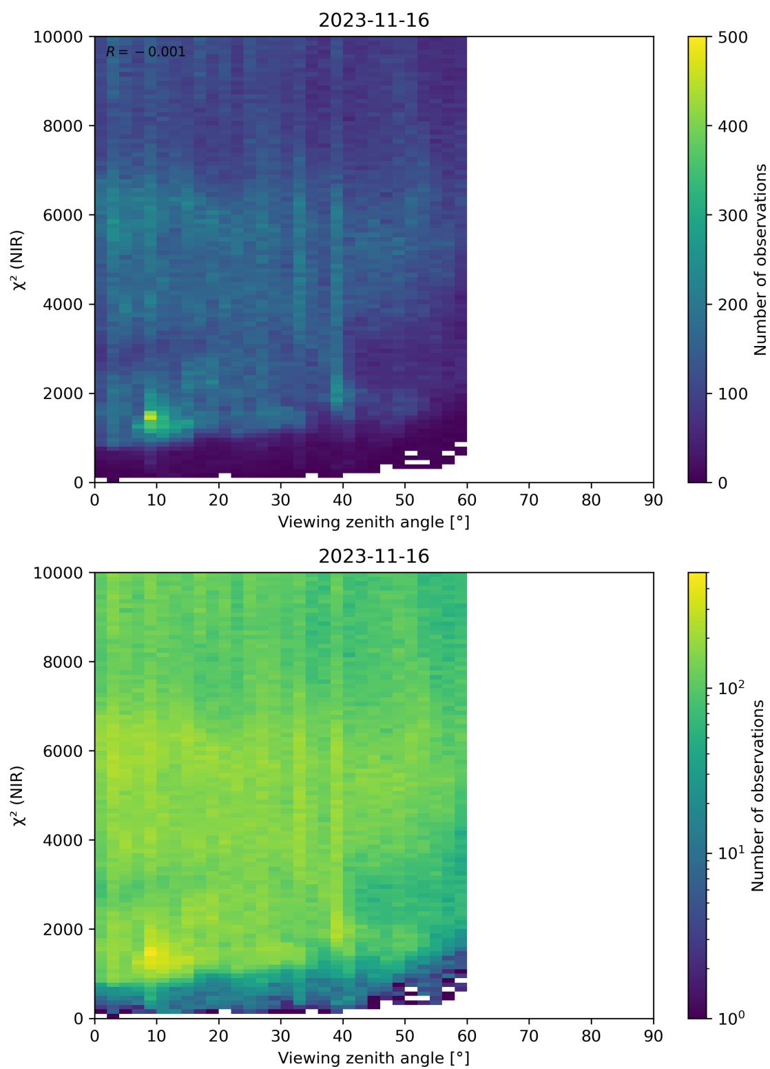
Figure 105: Scatter density plot of “Viewing zenith angle” against “ \chi^2 (NIR)” for 2023-11-15 to 2023-11-17.
