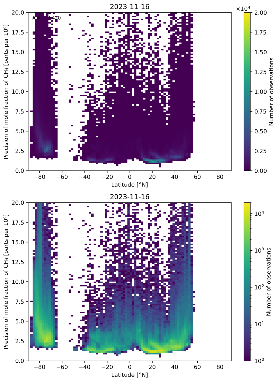
Figure 59: Scatter density plot of “Latitude” against “Precision of mole fraction of CH 4 ” for 2023-11-15 to 2023-11-17.
