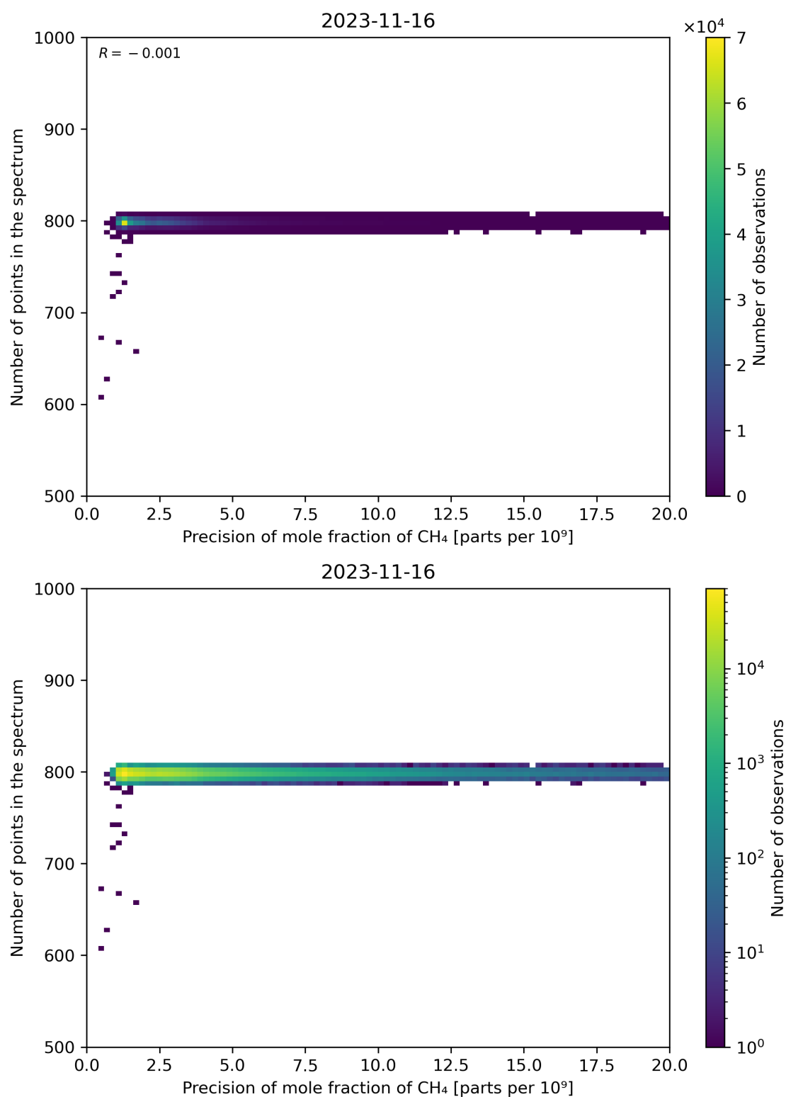
Figure 84: Scatter density plot of “Precision of mole fraction of CH 4 ” against “Number of points in the spectrum” for 2023-11-15 to 2023-11-17.
