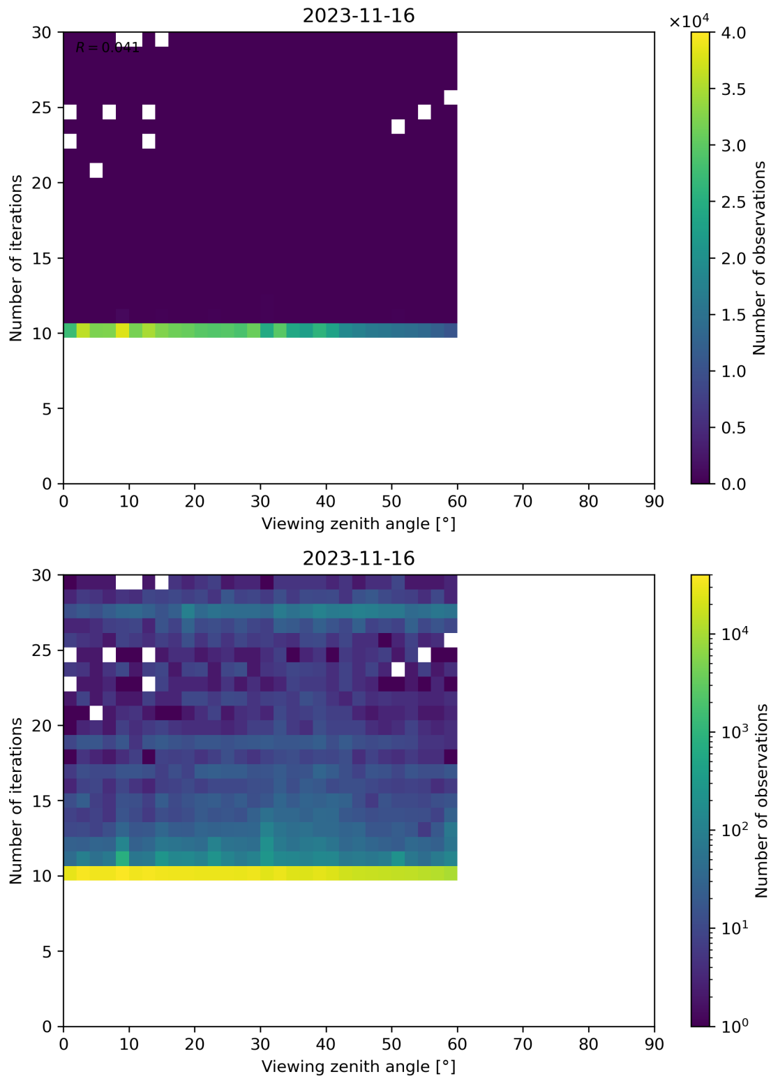
Figure 113: Scatter density plot of “Viewing zenith angle” against “Number of iterations” for 2023-11-15 to 2023-11-17.
