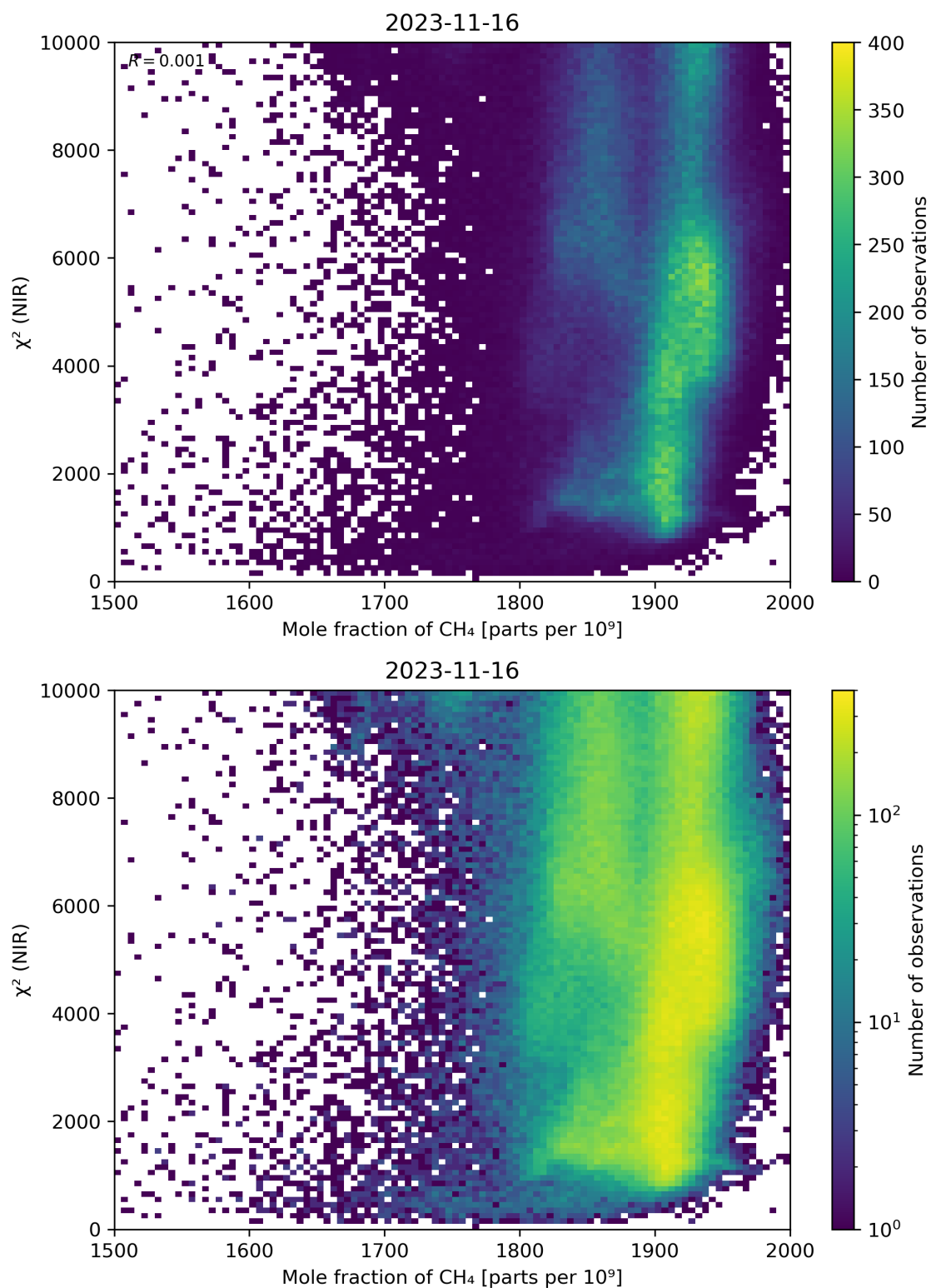
Figure 70: Scatter density plot of “Mole fraction of CH 4 ” against “ \chi^2 (NIR)” for 2023-11-15 to 2023-11-17.
