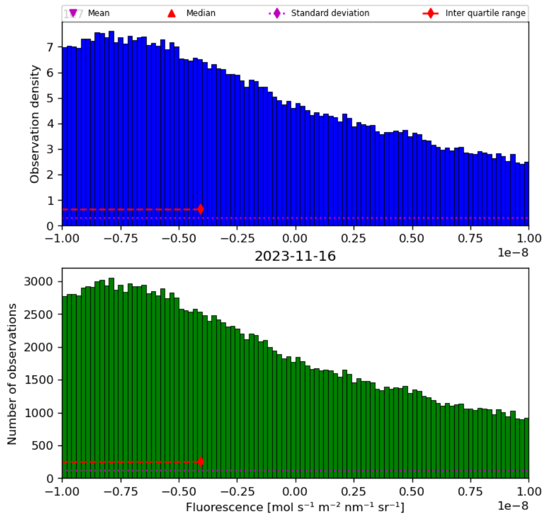
Figure 32: Histogram of “Fluorescence” for 2023-11-15 to 2023-11-17
