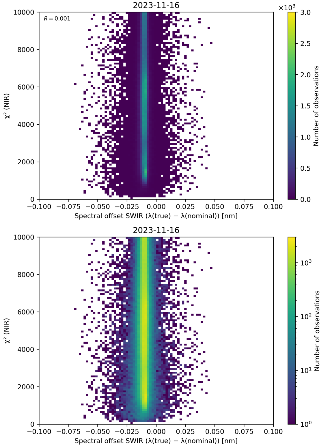
Figure 117: Scatter density plot of “Spectral offset SWIR ( \lambda(\text{true}) - \lambda(\text{nominal}) )” against “ \chi^2 (NIR)” for 2023-11-15 to 2023-11-17.
