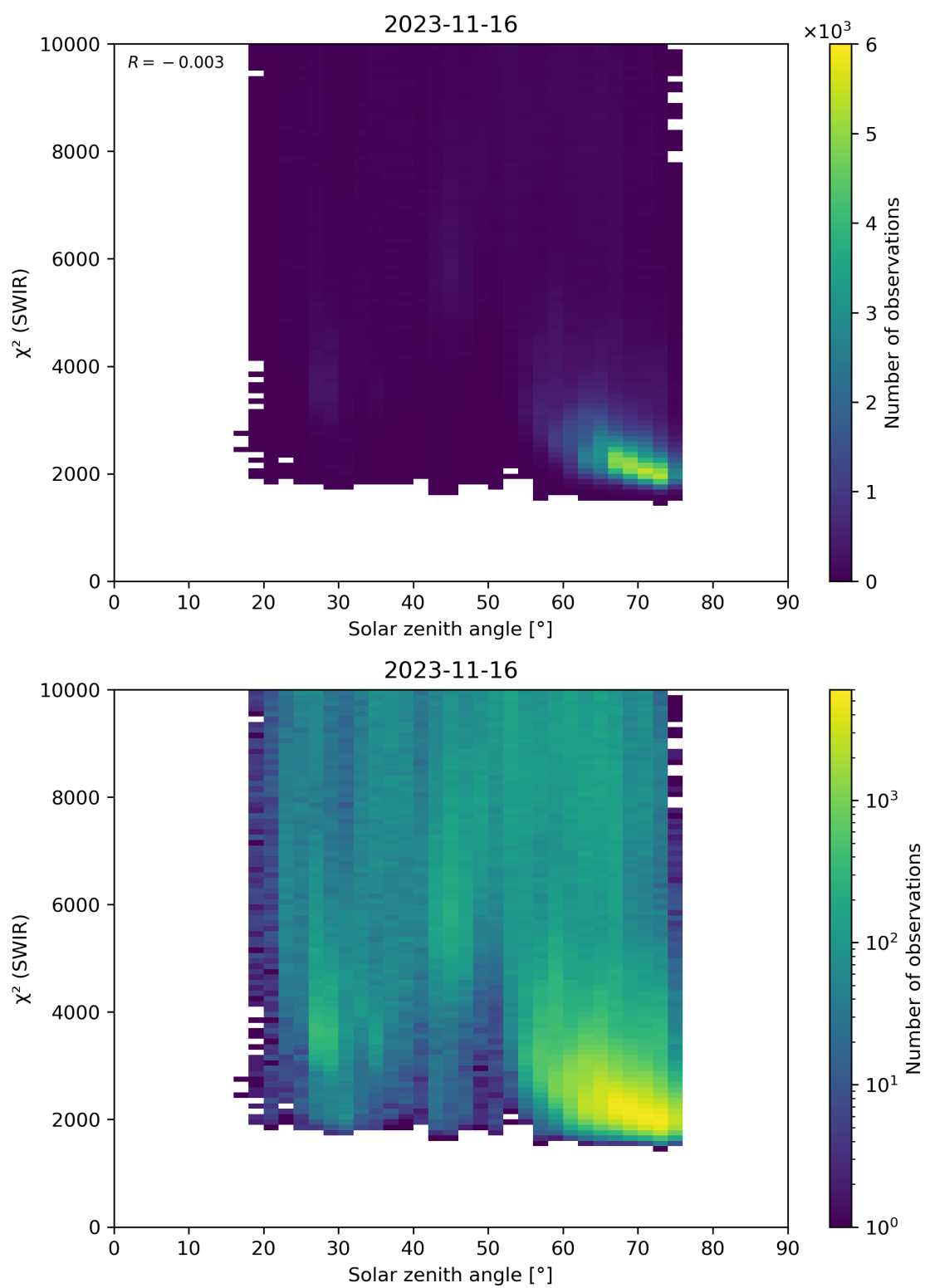
Figure 95: Scatter density plot of “Solar zenith angle” against “ \chi^2 (SWIR)” for 2023-11-15 to 2023-11-17.
