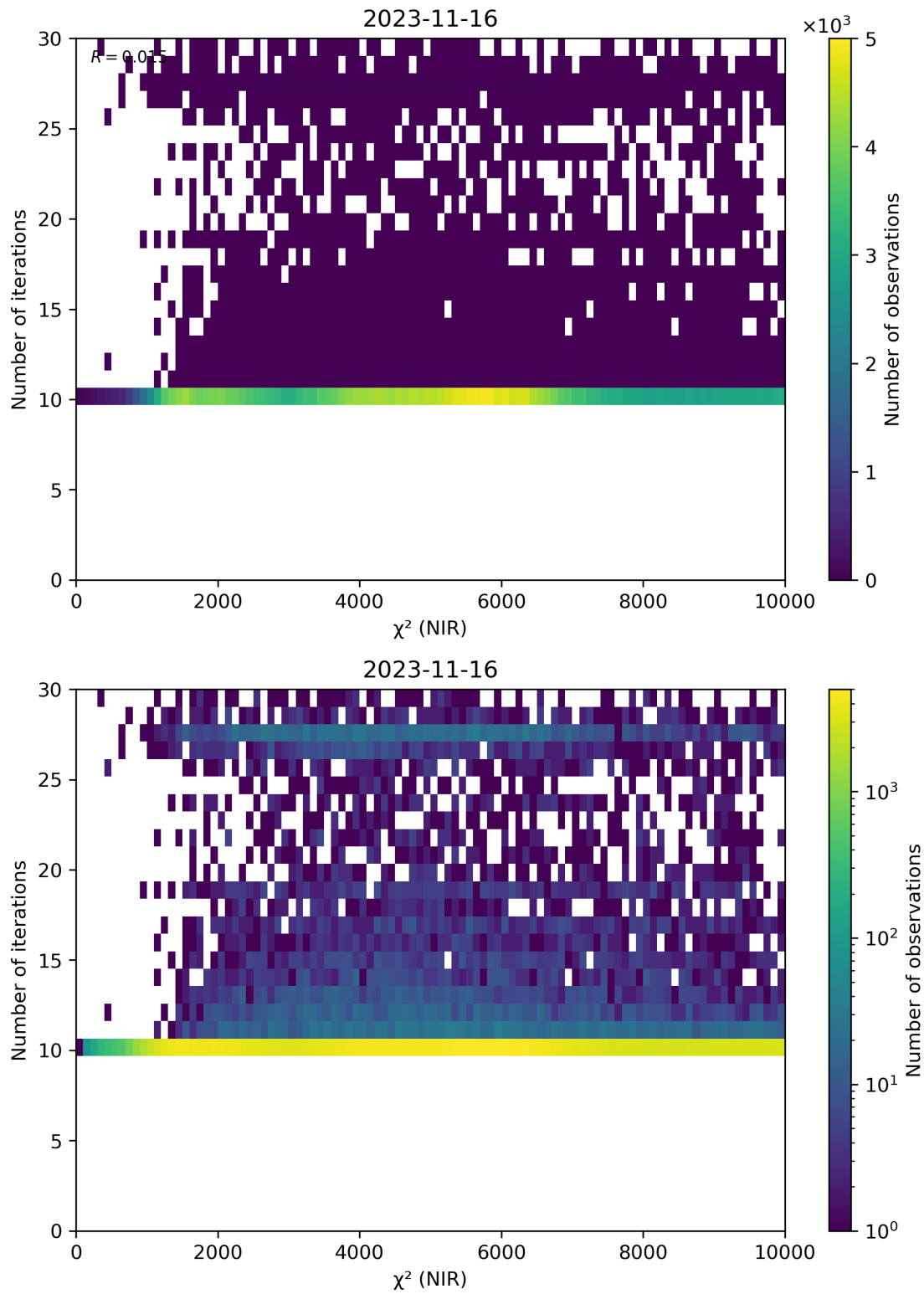
Figure 46: Scatter density plot of “ \chi^2 (NIR)” against “Number of iterations” for 2023-11-15 to 2023-11-17.
