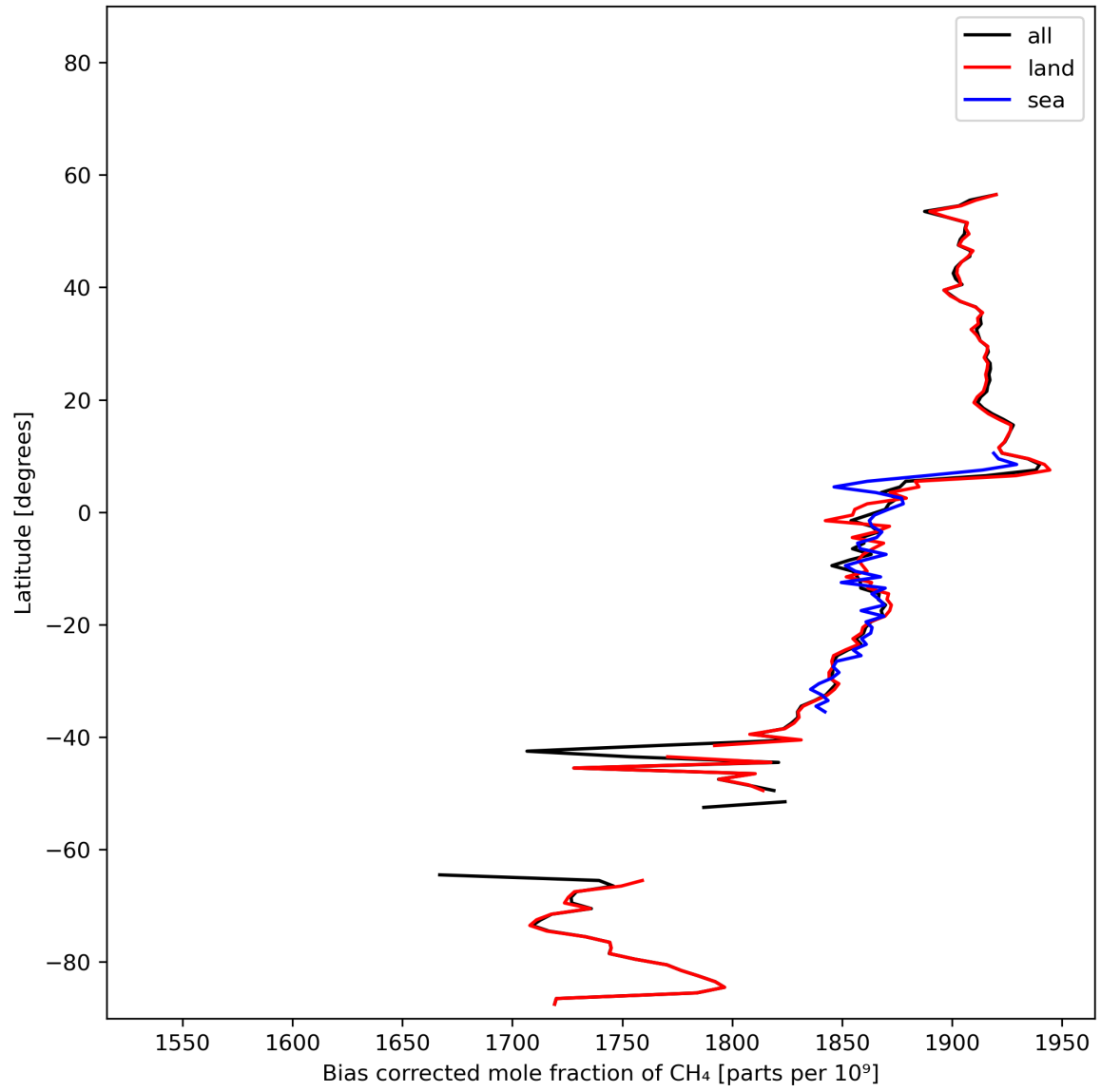
Figure 14: Zonal average of “Bias corrected mole fraction of CH 4 ” for 2023-11-15 to 2023-11-17.
