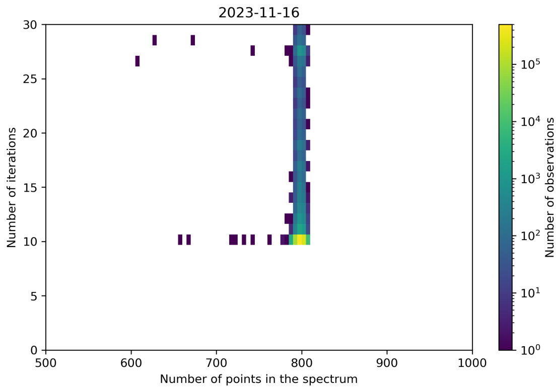
Figure 92: Scatter density plot of “Number of points in the spectrum” against “Number of iterations” for 2023-11-15 to 2023-11-17.
