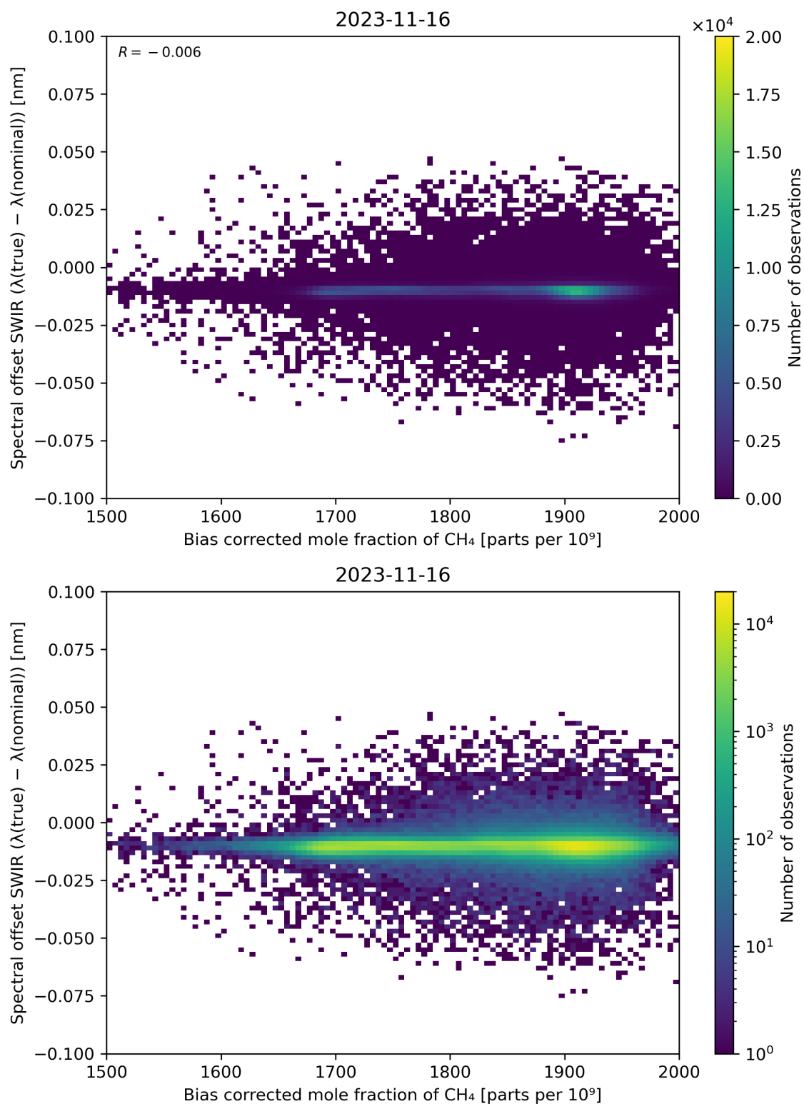
Figure 69: Scatter density plot of “Bias corrected mole fraction of \text{CH}_4 ” against “Spectral offset SWIR ( \lambda(\text{true}) - \lambda(\text{nominal}) )” for 2023-11-15 to 2023-11-17.
