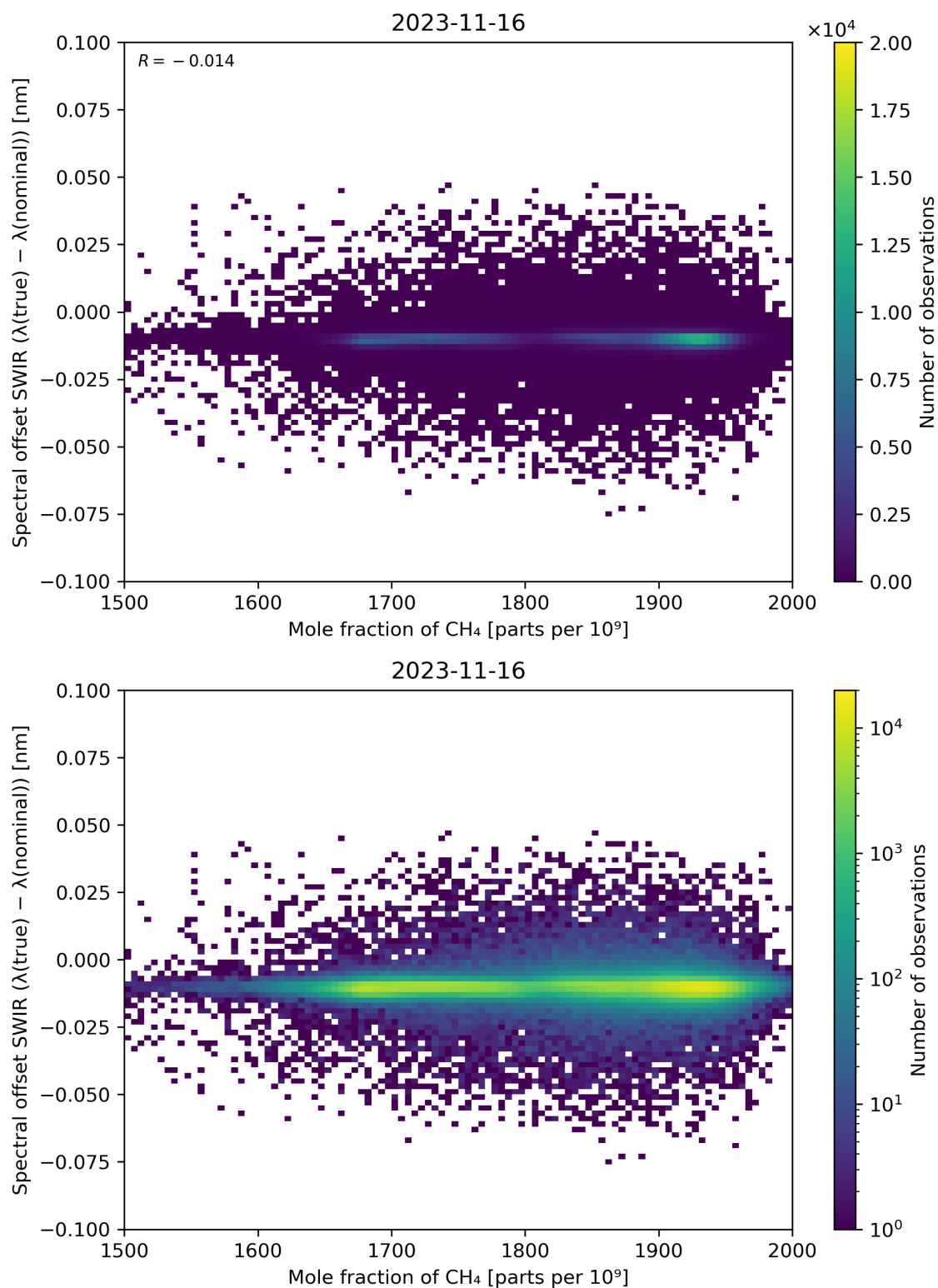
Figure 86: Scatter density plot of “Mole fraction of CH 4 ” against “Spectral offset SWIR ( \lambda(\text{true}) - \lambda(\text{nominal}) )” for 2023-11-15 to 2023-11-17.
