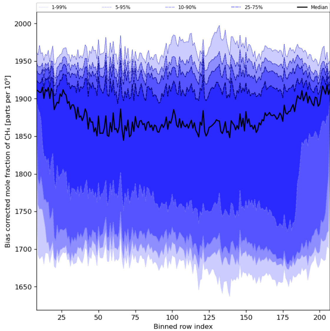
Figure 36: Along track statistics of “Bias corrected mole fraction of CH 4 ” for 2023-11-15 to 2023-11-17
