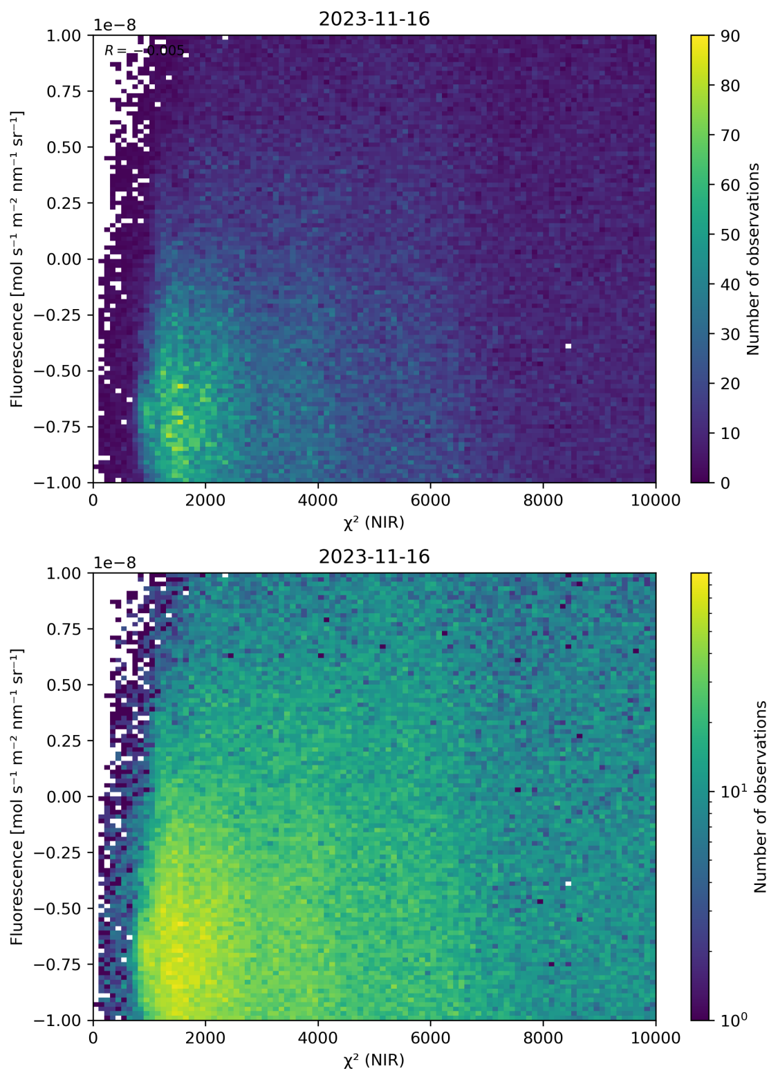
Figure 45: Scatter density plot of “ \chi^2 (NIR)” against “Fluorescence” for 2023-11-15 to 2023-11-17.
