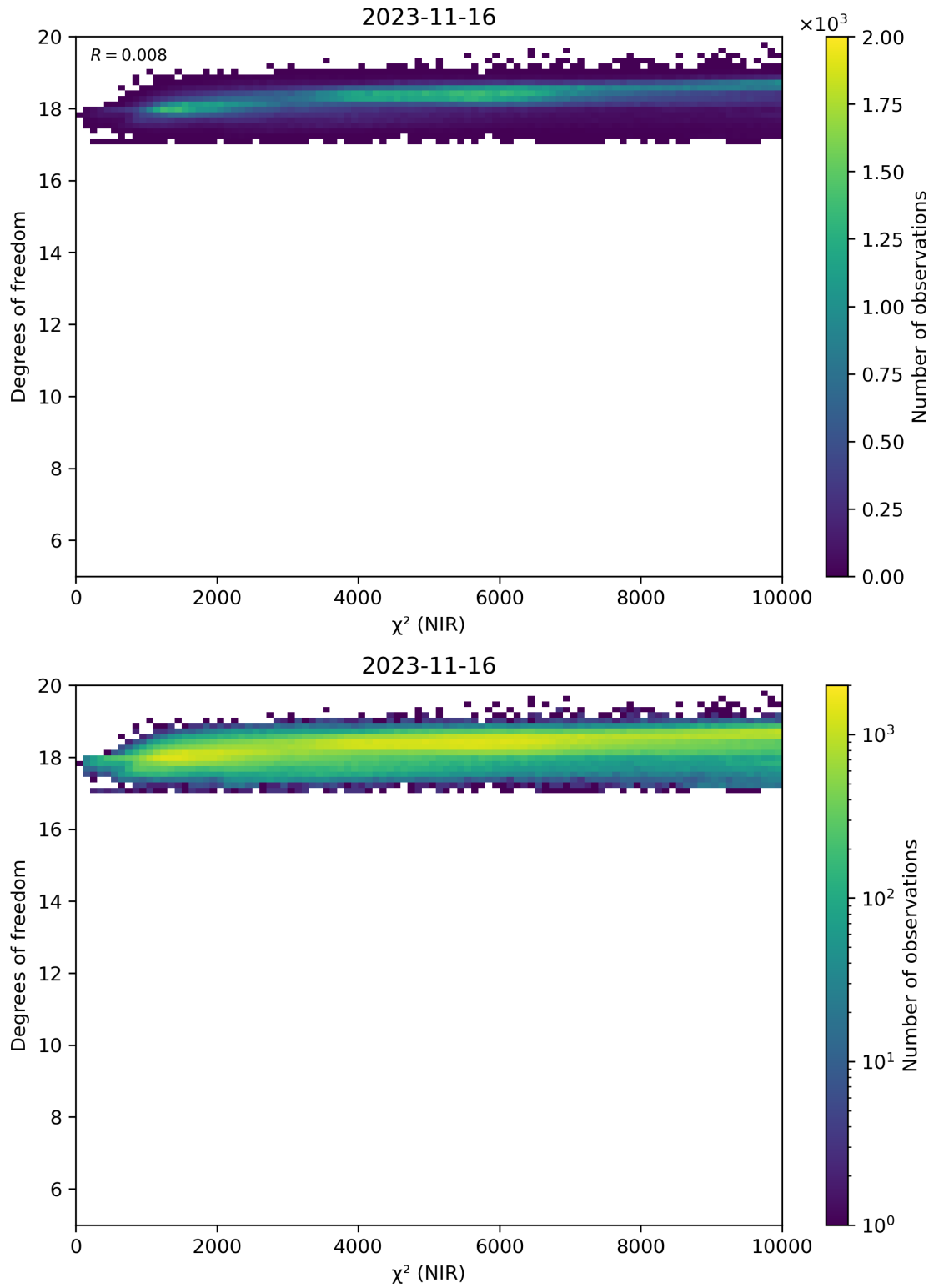
Figure 44: Scatter density plot of “ \chi^2 (NIR)” against “Degrees of freedom” for 2023-11-15 to 2023-11-17.
