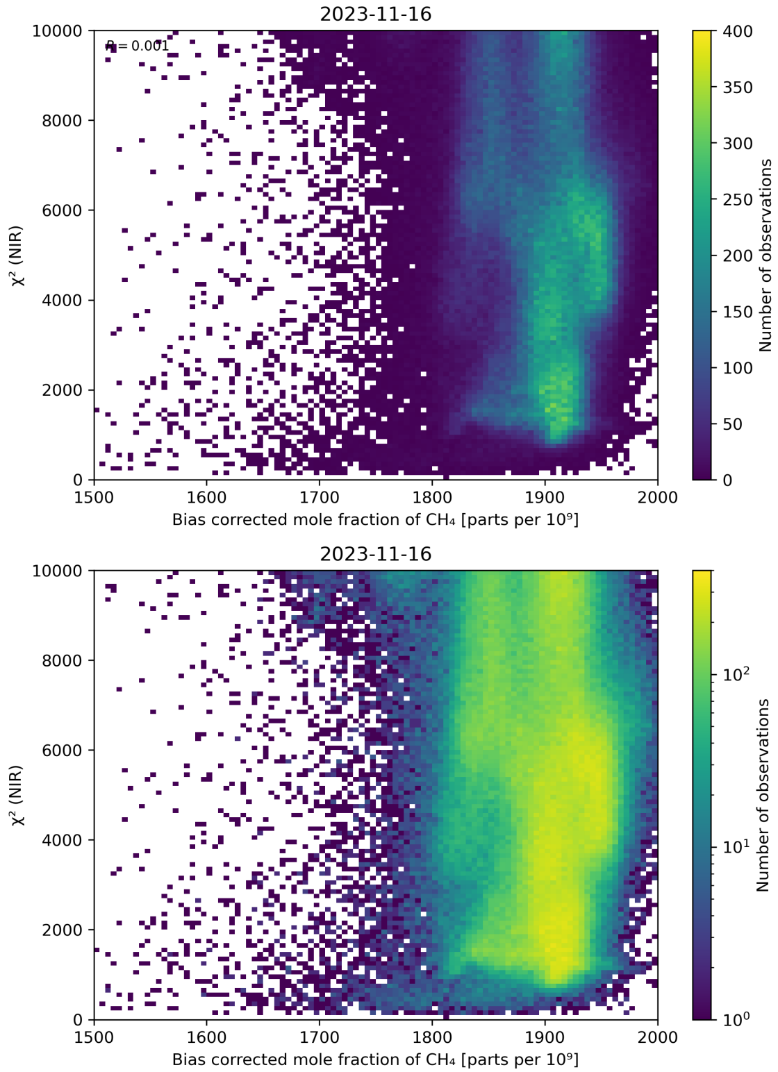
Figure 63: Scatter density plot of “Bias corrected mole fraction of \text{CH}_4 ” against “ \chi^2 (NIR)” for 2023-11-15 to 2023-11-17.
