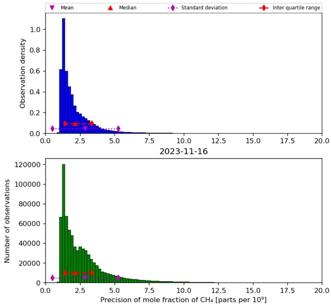
Figure 24: Histogram of “Precision of mole fraction of CH 4 ” for 2023-11-15 to 2023-11-17
