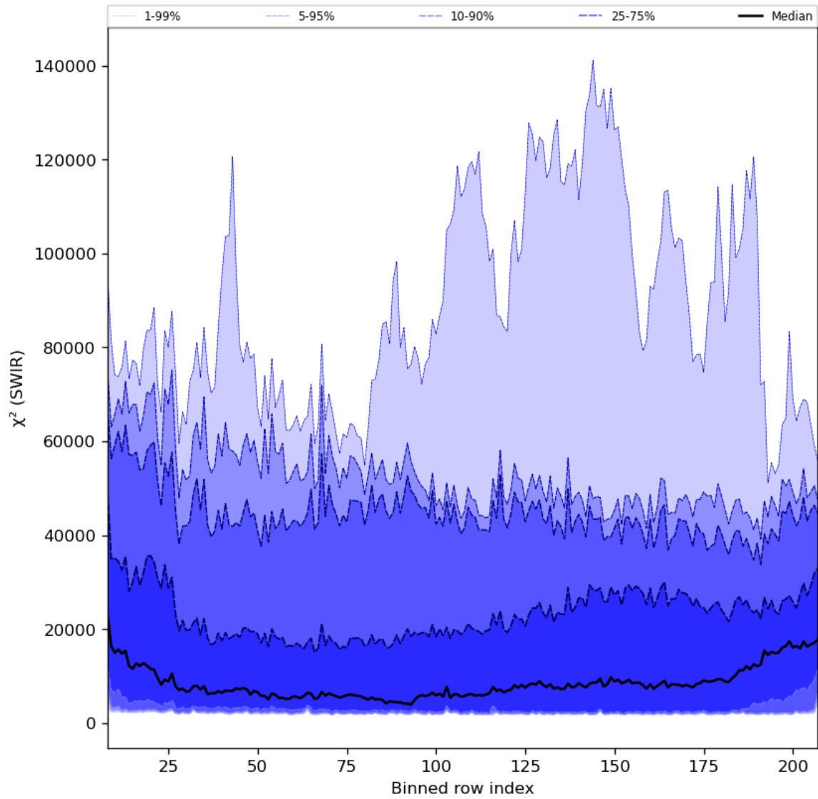
Figure 39: Along track statistics of “ \chi^2 (SWIR)” for 2023-11-15 to 2023-11-17
