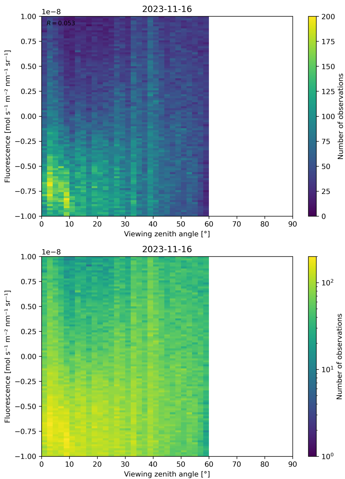
Figure 108: Scatter density plot of “Viewing zenith angle” against “Fluorescence” for 2023-11-15 to 2023-11-17.
