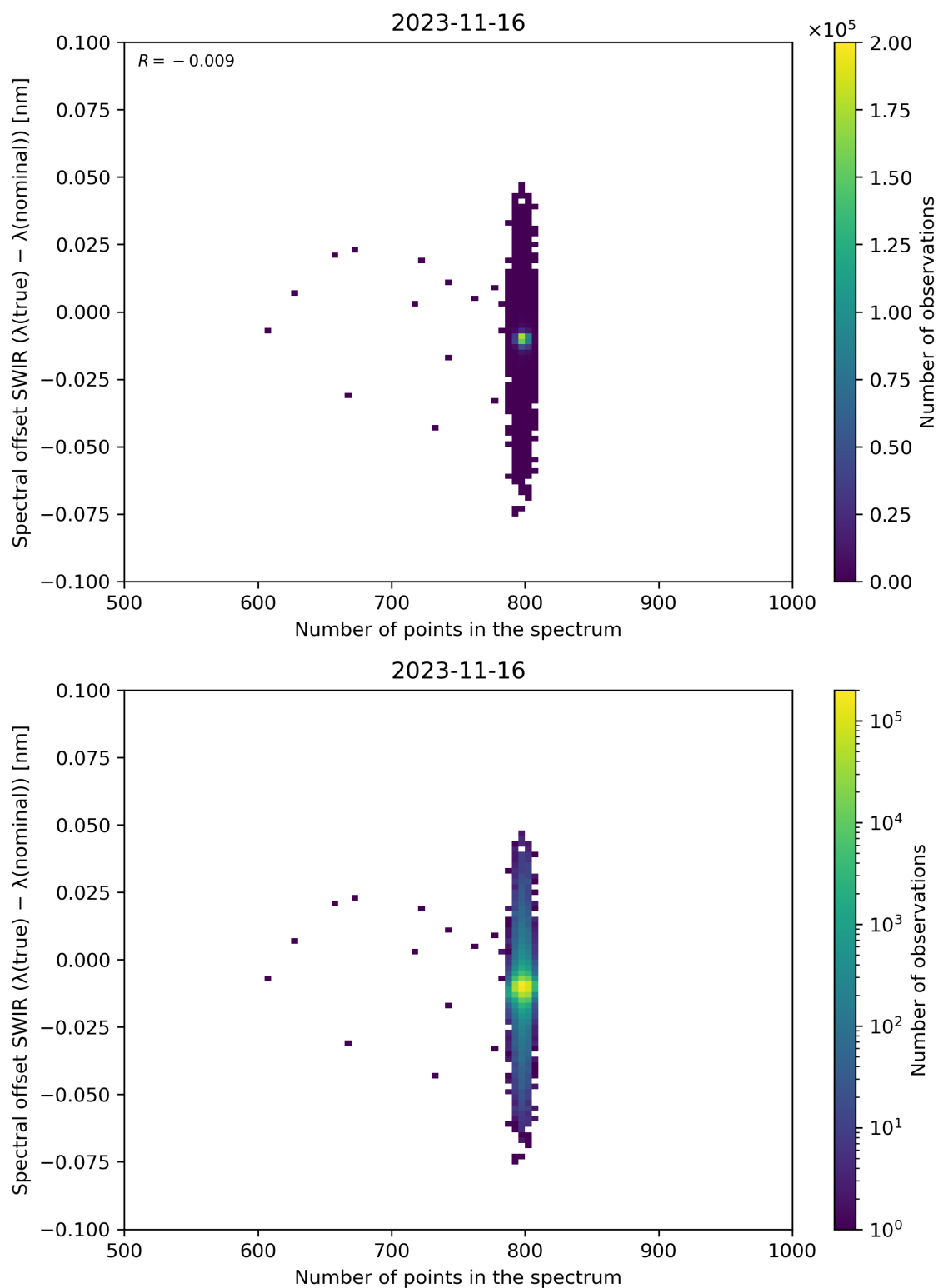
Figure 93: Scatter density plot of “Number of points in the spectrum” against “Spectral offset SWIR ( \lambda(\text{true}) - \lambda(\text{nominal}) )” for 2023-11-15 to 2023-11-17.
