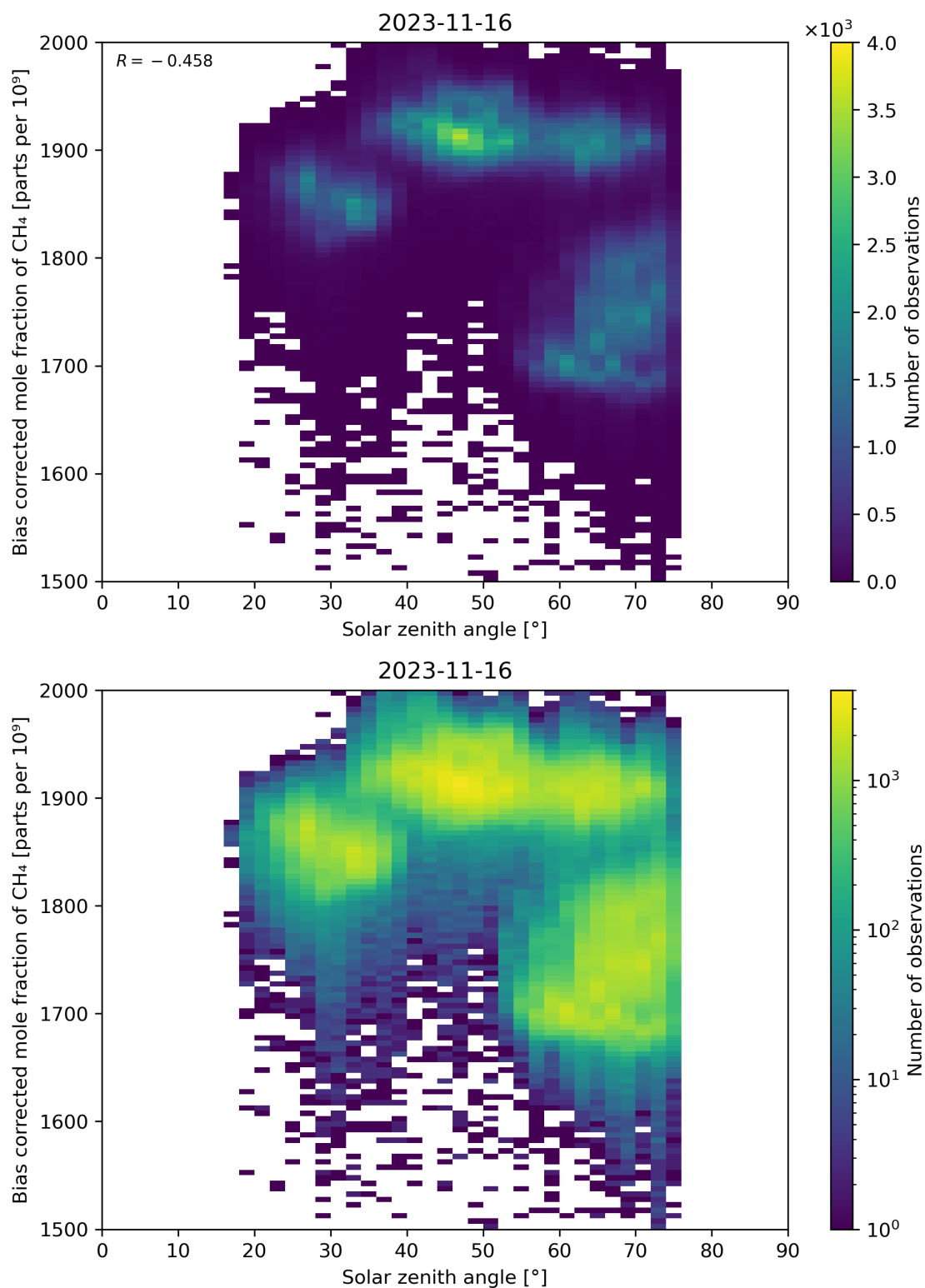
Figure 100: Scatter density plot of “Solar zenith angle” against “Bias corrected mole fraction of \text{CH}_4 ” for 2023-11-15 to 2023-11-17.
