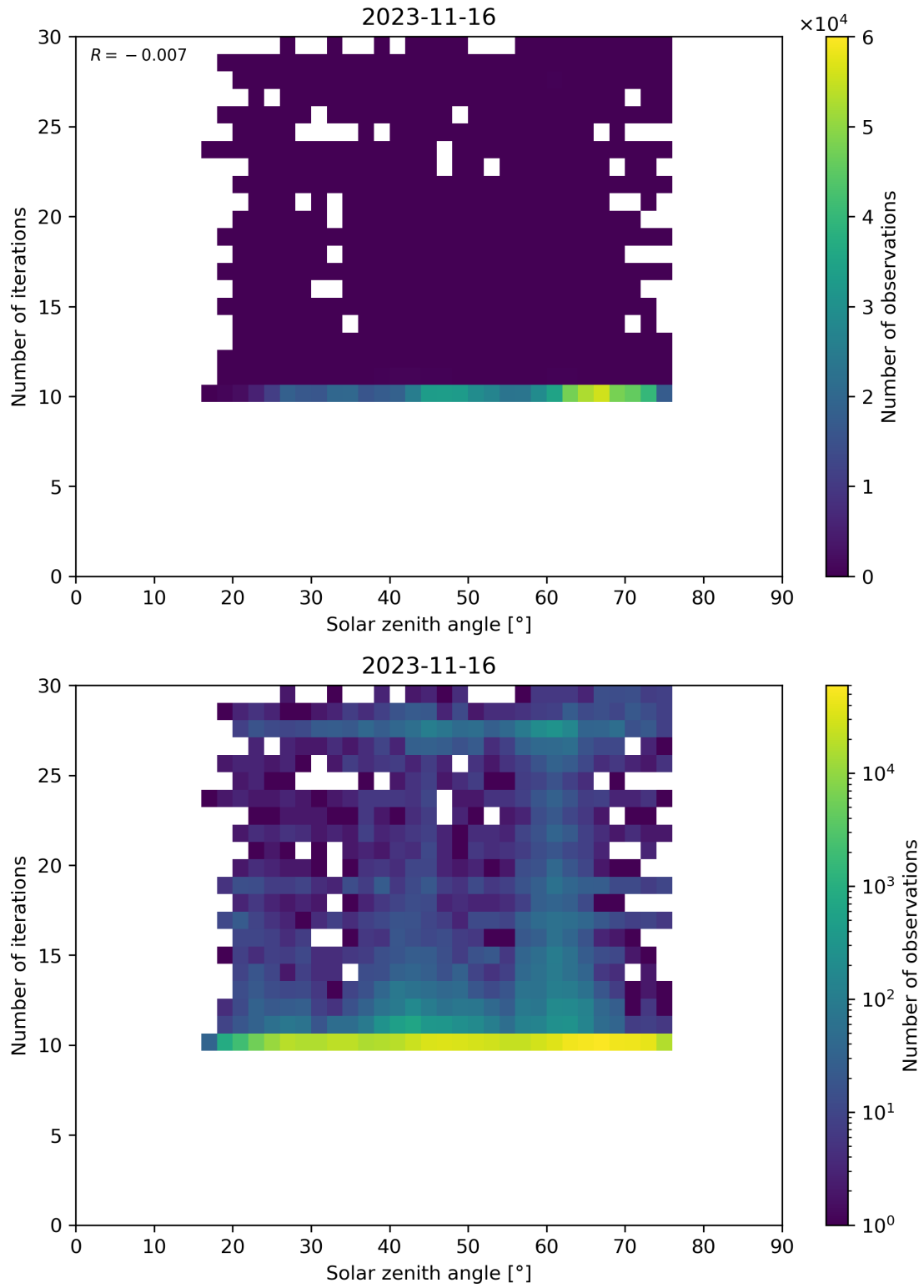
Figure 102: Scatter density plot of “Solar zenith angle” against “Number of iterations” for 2023-11-15 to 2023-11-17.
