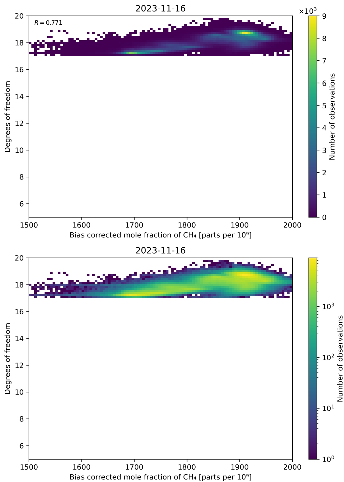
Figure 65: Scatter density plot of “Bias corrected mole fraction of CH 4 ” against “Degrees of freedom” for 2023-11-15 to 2023-11-17.
