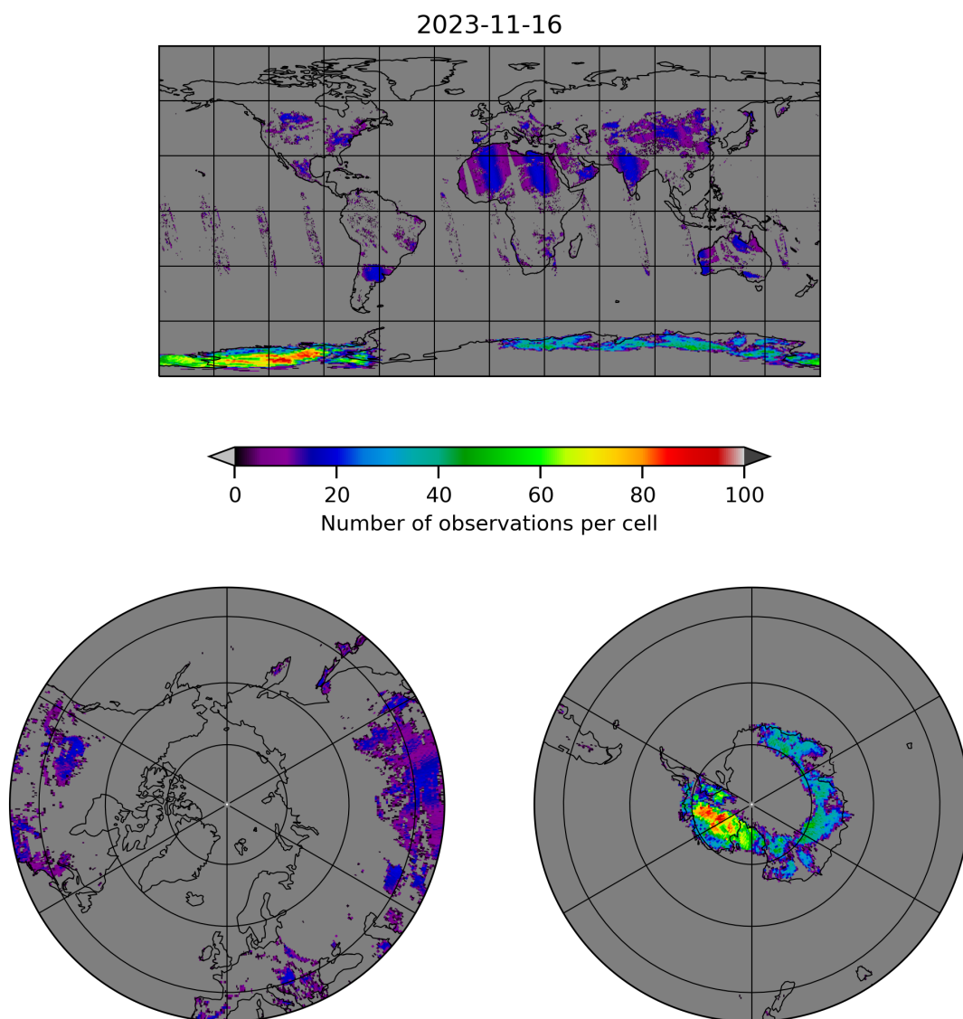
Figure 10: Map of the number of observations for 2023-11-15 to 2023-11-17
