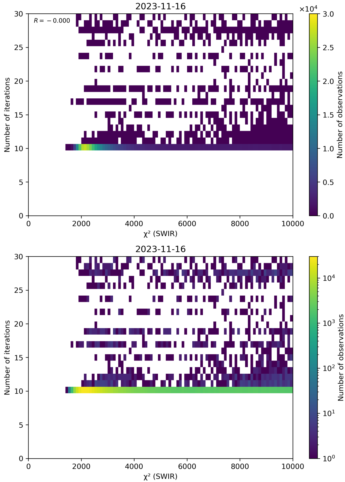
Figure 50: Scatter density plot of “ \chi^2 (SWIR)” against “Number of iterations” for 2023-11-15 to 2023-11-17.
