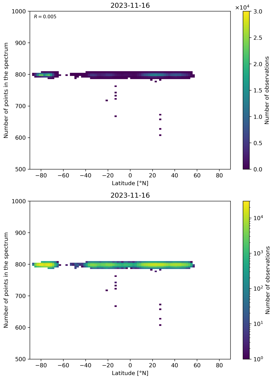
Figure 61: Scatter density plot of “Latitude” against “Number of points in the spectrum” for 2023-11-15 to 2023-11-17.
