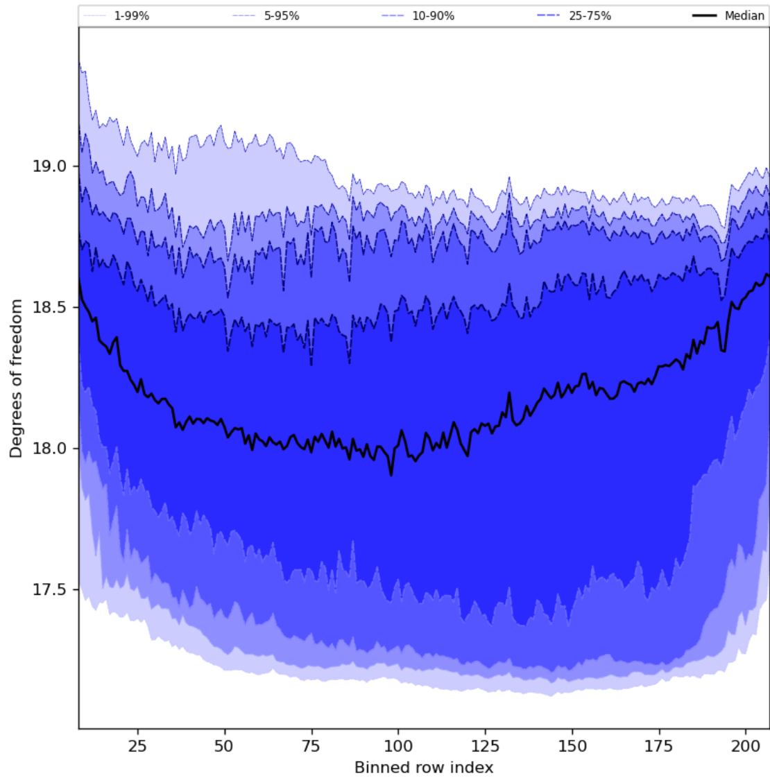
Figure 41: Along track statistics of “Degrees of freedom” for 2023-11-15 to 2023-11-17
