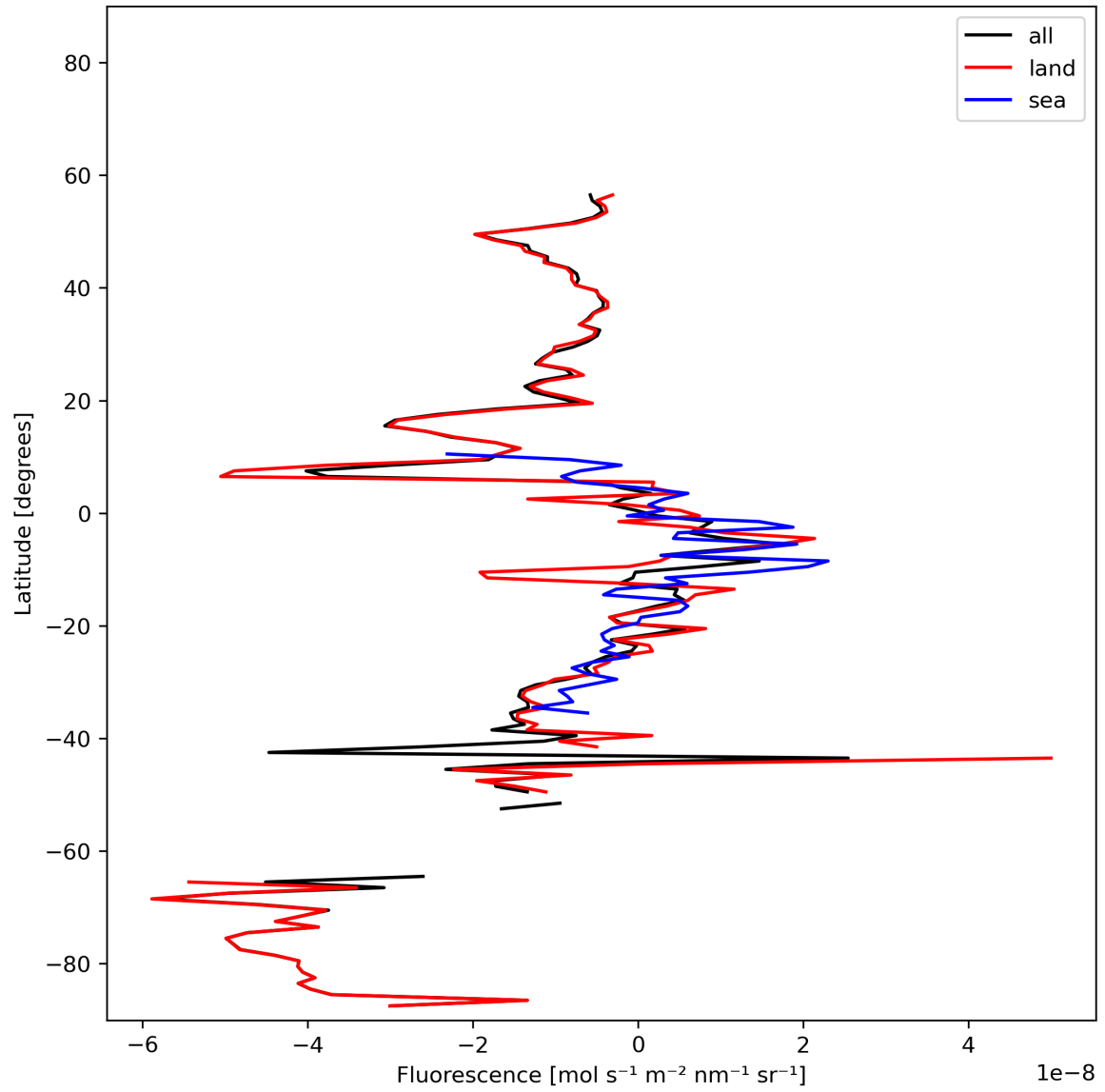
Figure 21: Zonal average of “Fluorescence” for 2023-11-15 to 2023-11-17.
