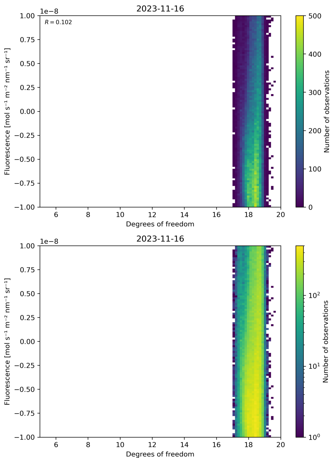
Figure 51: Scatter density plot of “Degrees of freedom” against “Fluorescence” for 2023-11-15 to 2023-11-17.
