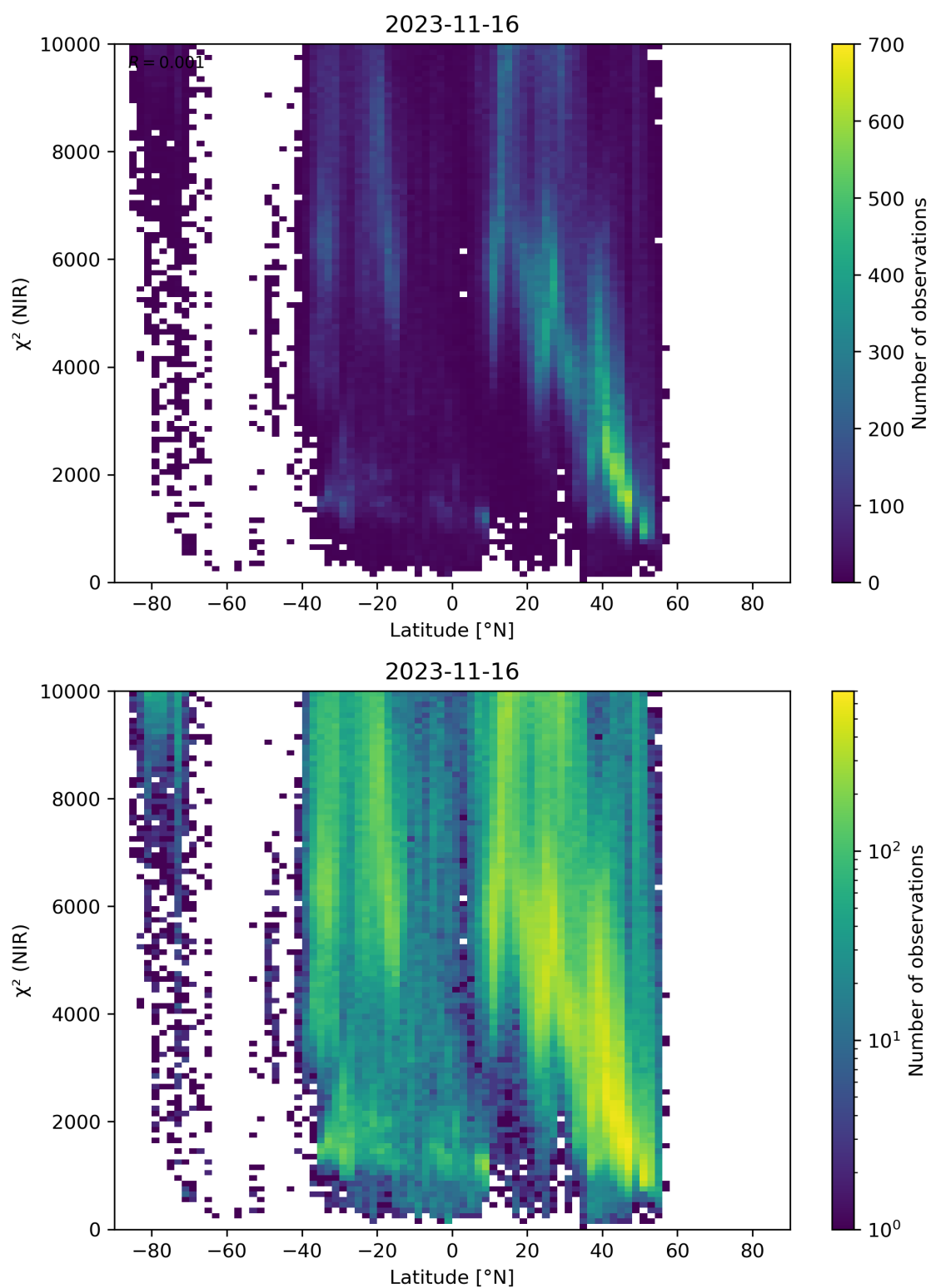
Figure 53: Scatter density plot of “Latitude” against “ \chi^2 (NIR)” for 2023-11-15 to 2023-11-17.
