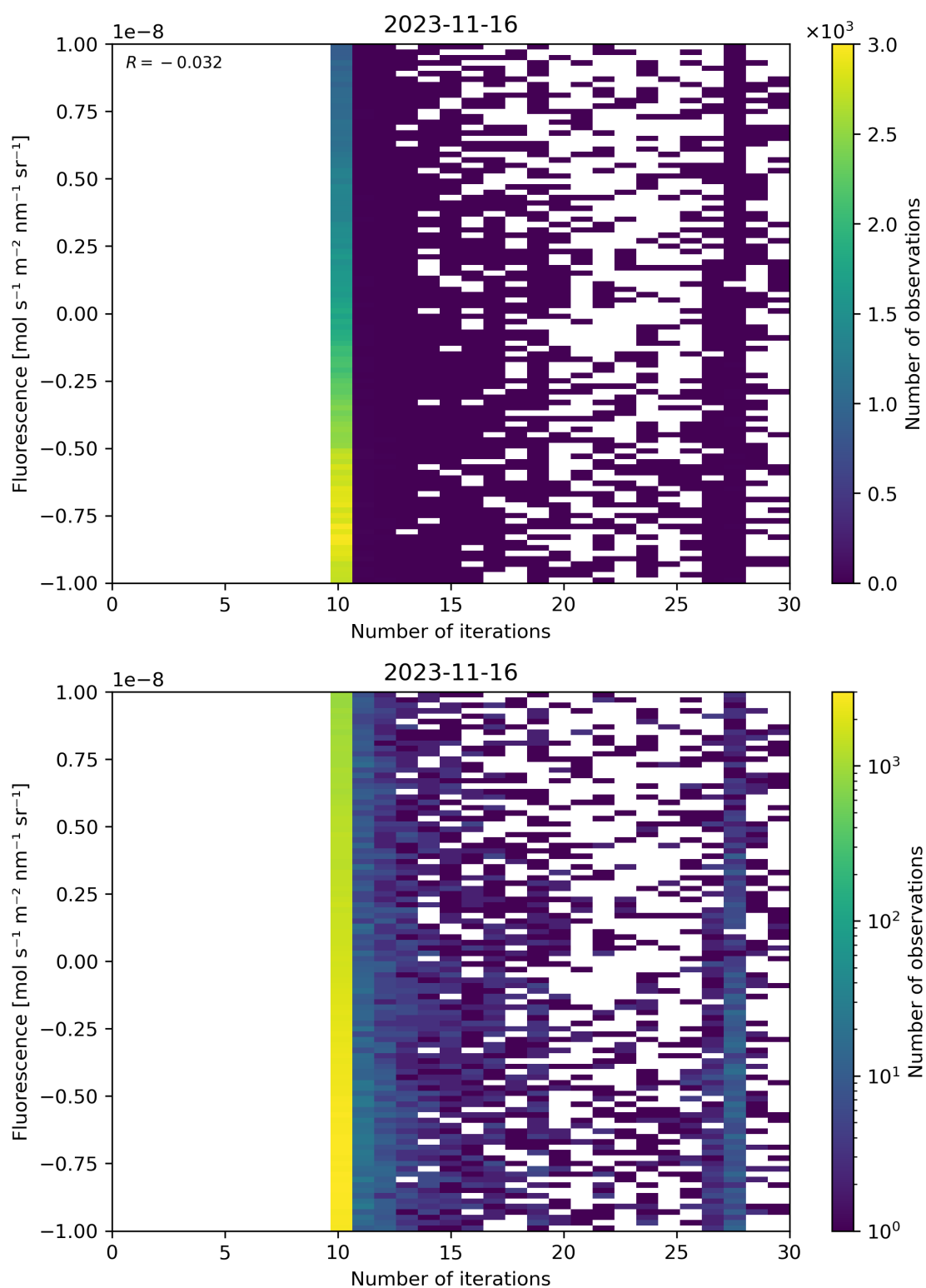
Figure 87: Scatter density plot of “Number of iterations” against “Fluorescence” for 2023-11-15 to 2023-11-17.
