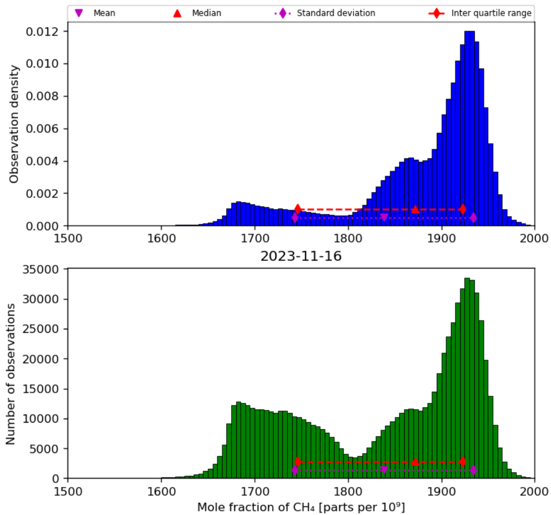
Figure 23: Histogram of “Mole fraction of CH 4 ” for 2023-11-15 to 2023-11-17
