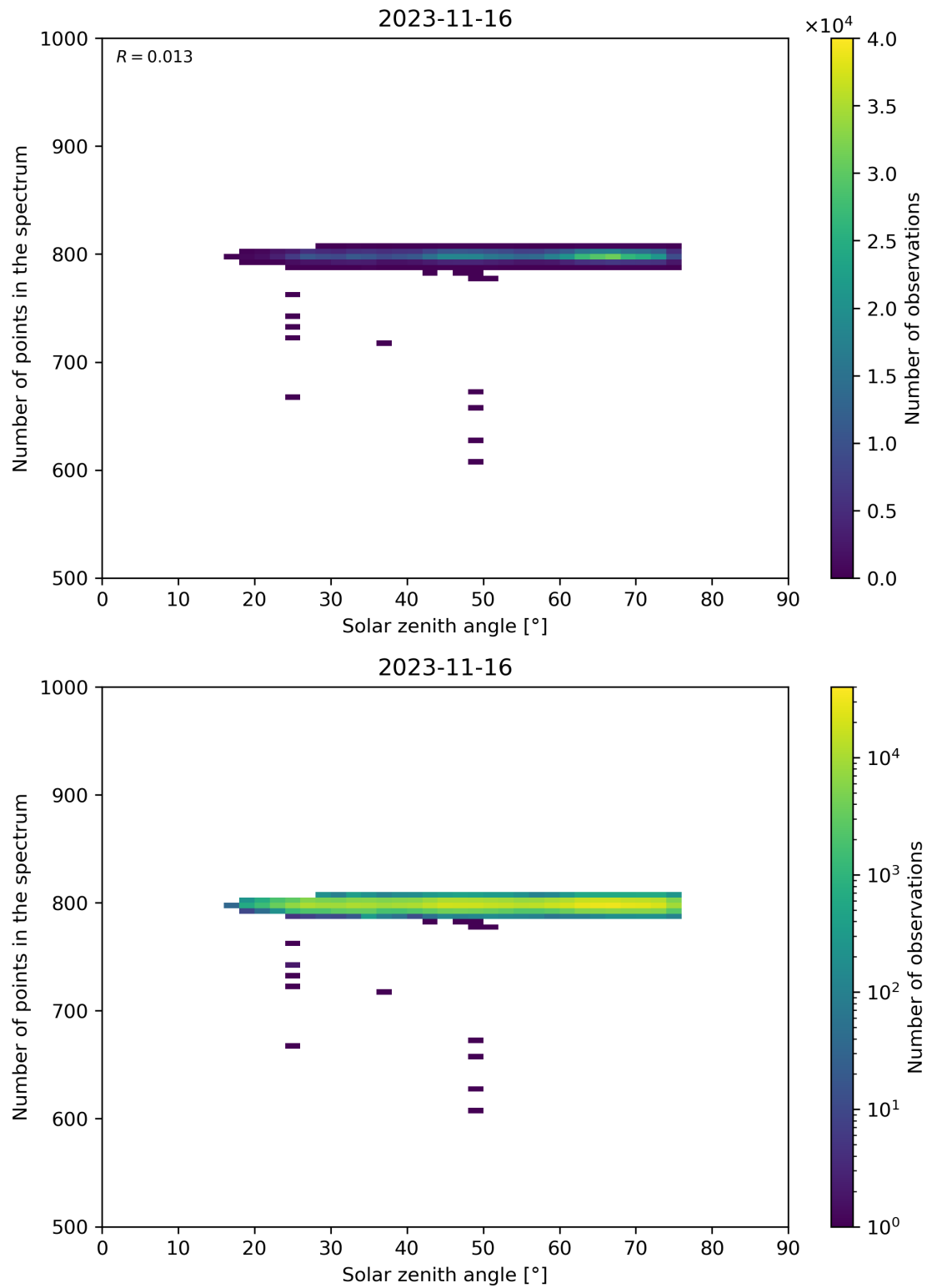
Figure 103: Scatter density plot of “Solar zenith angle” against “Number of points in the spectrum” for 2023-11-15 to 2023-11-17.
