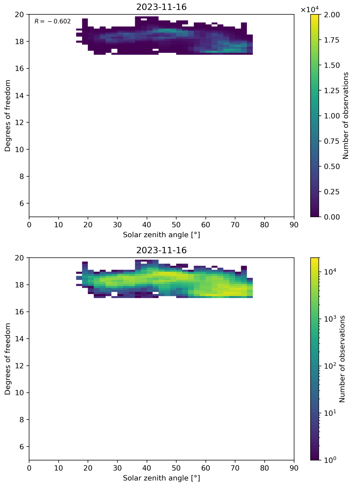
Figure 96: Scatter density plot of “Solar zenith angle” against “Degrees of freedom” for 2023-11-15 to 2023-11-17.
