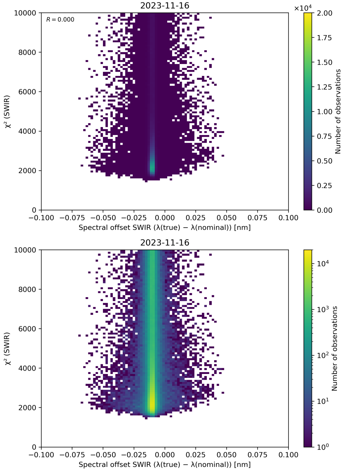
Figure 118: Scatter density plot of “Spectral offset SWIR ( \lambda(\text{true}) - \lambda(\text{nominal}) )” against “ \chi^2 (SWIR)” for 2023-11-15 to 2023-11-17.
