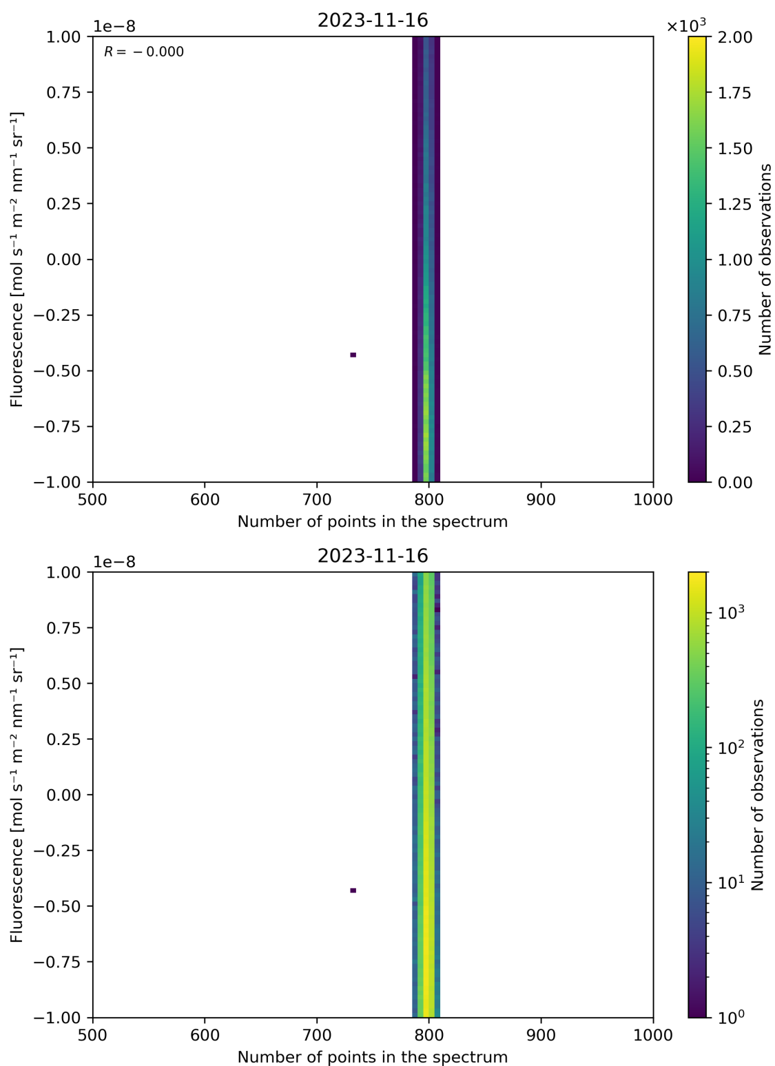
Figure 91: Scatter density plot of “Number of points in the spectrum” against “Fluorescence” for 2023-11-15 to 2023-11-17.
