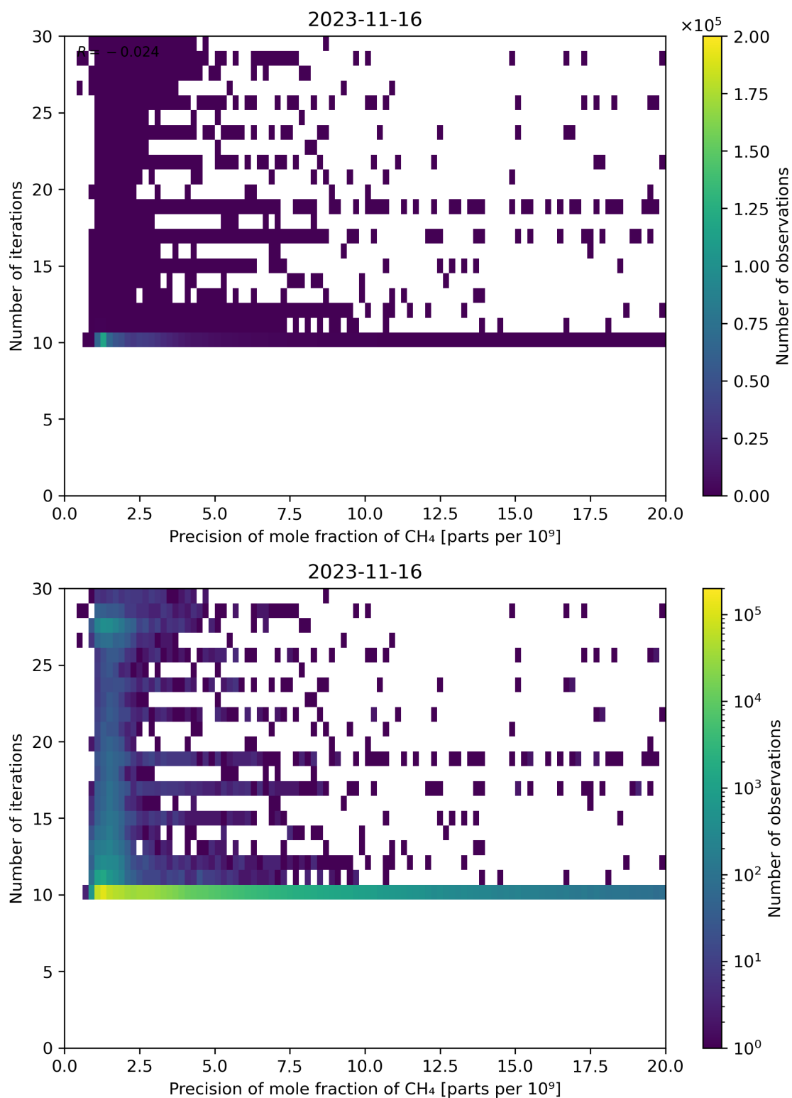
Figure 83: Scatter density plot of “Precision of mole fraction of CH 4 ” against “Number of iterations” for 2023-11-15 to 2023-11-17.
