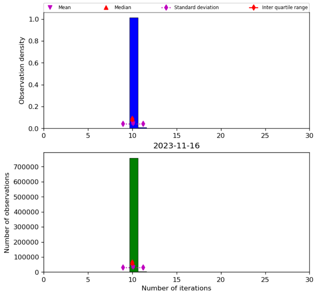
Figure 31: Histogram of “Number of iterations” for 2023-11-15 to 2023-11-17
