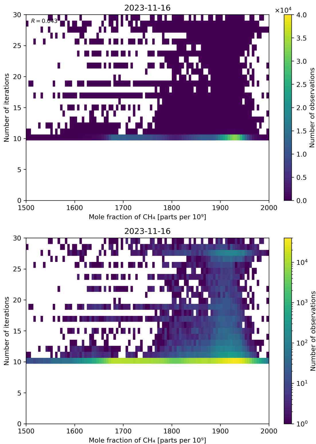
Figure 76: Scatter density plot of “Mole fraction of CH 4 ” against “Number of iterations” for 2023-11-15 to 2023-11-17.
