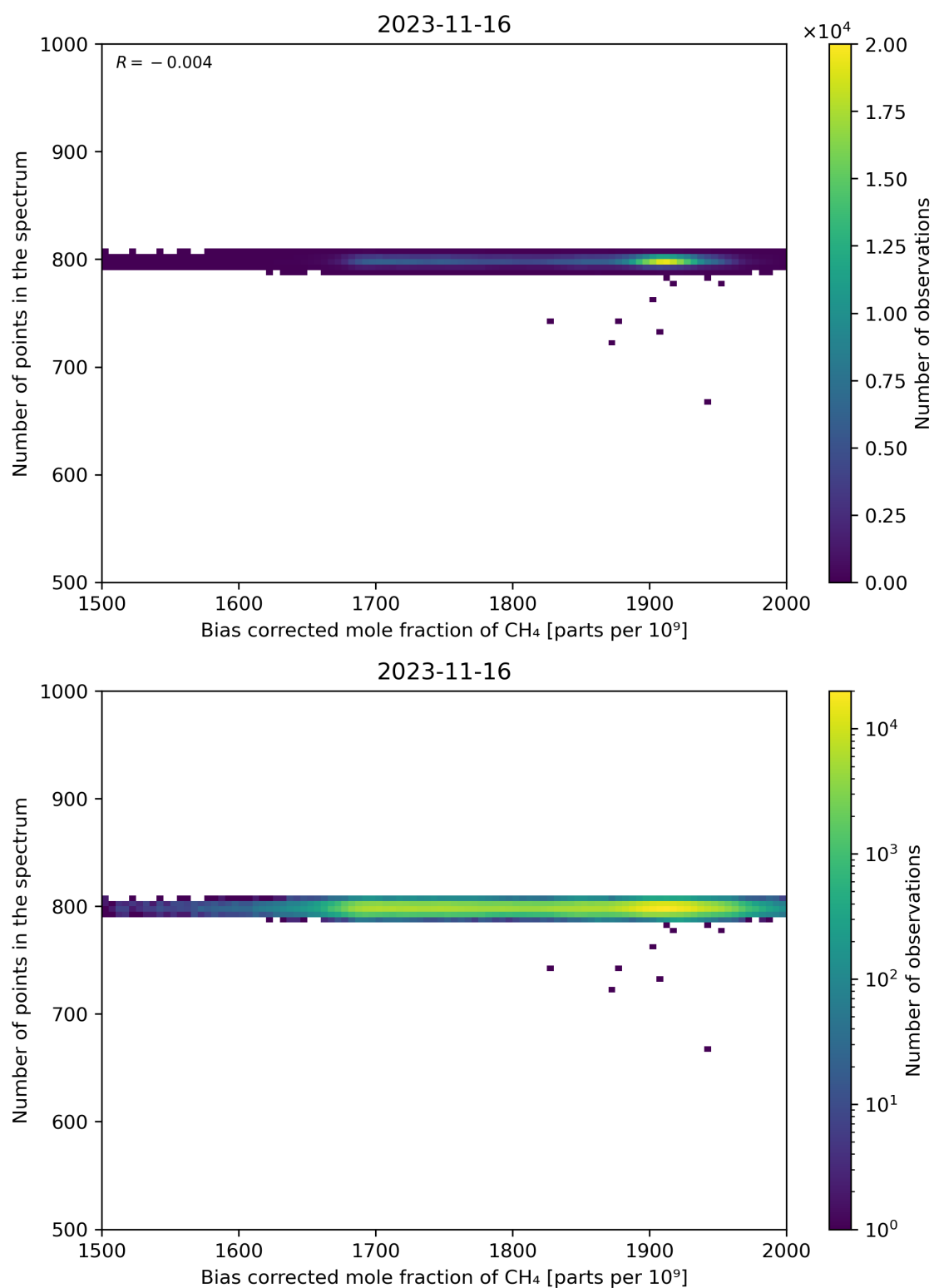
Figure 68: Scatter density plot of “Bias corrected mole fraction of CH 4 ” against “Number of points in the spectrum” for 2023-11-15 to 2023-11-17.
