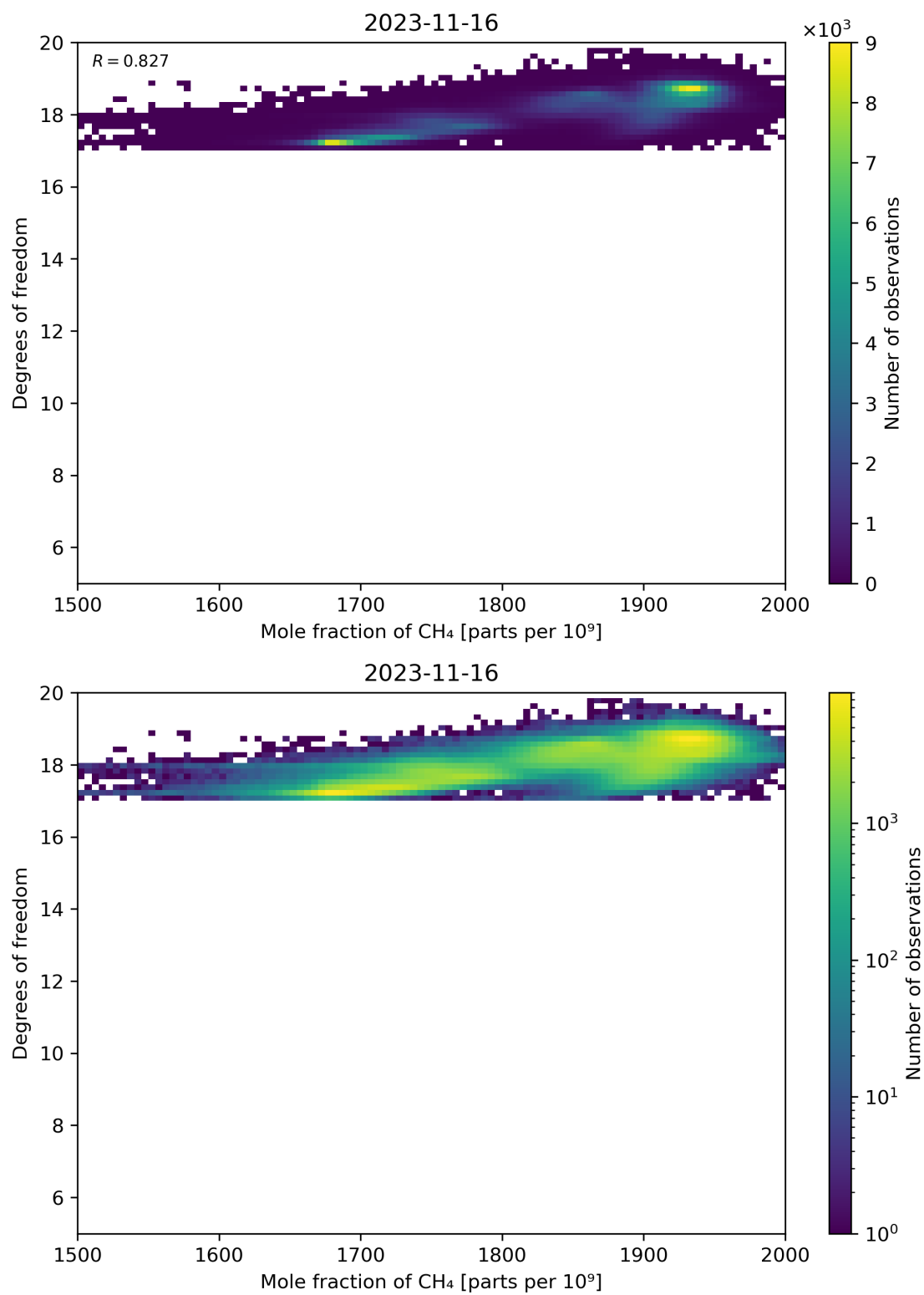
Figure 72: Scatter density plot of “Mole fraction of CH 4 ” against “Degrees of freedom” for 2023-11-15 to 2023-11-17.
