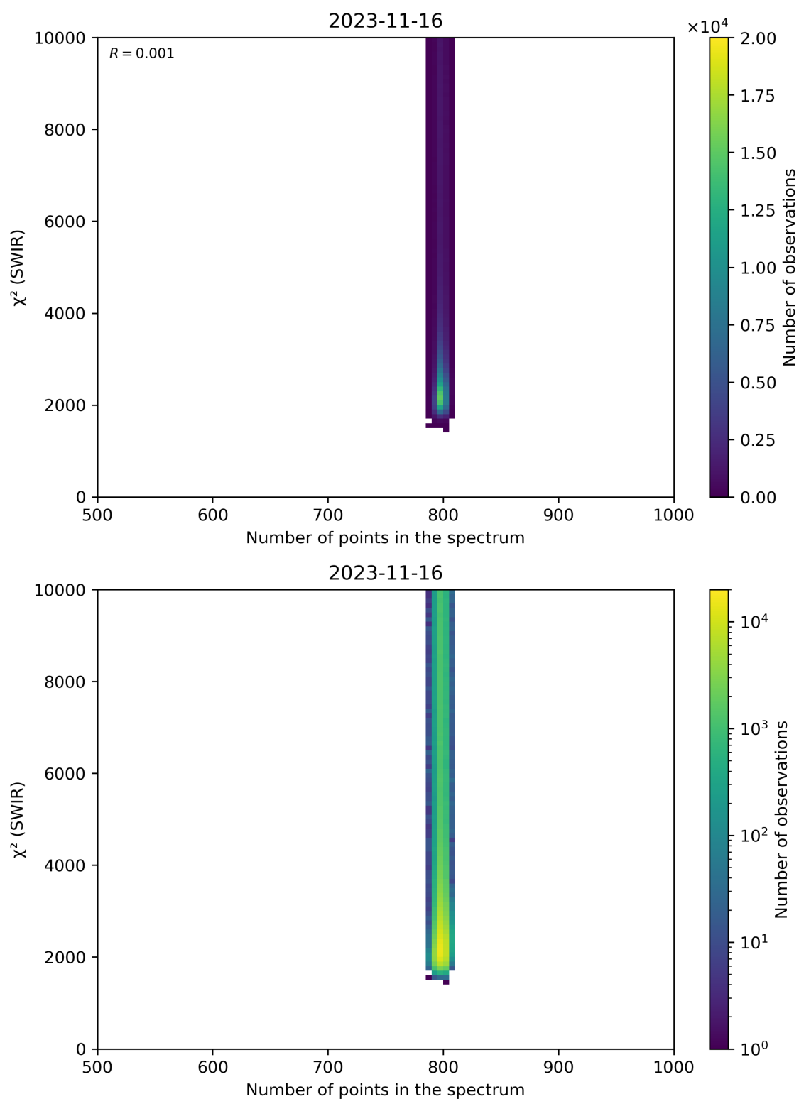
Figure 89: Scatter density plot of “Number of points in the spectrum” against “ \chi^2 (SWIR)” for 2023-11-15 to 2023-11-17.
