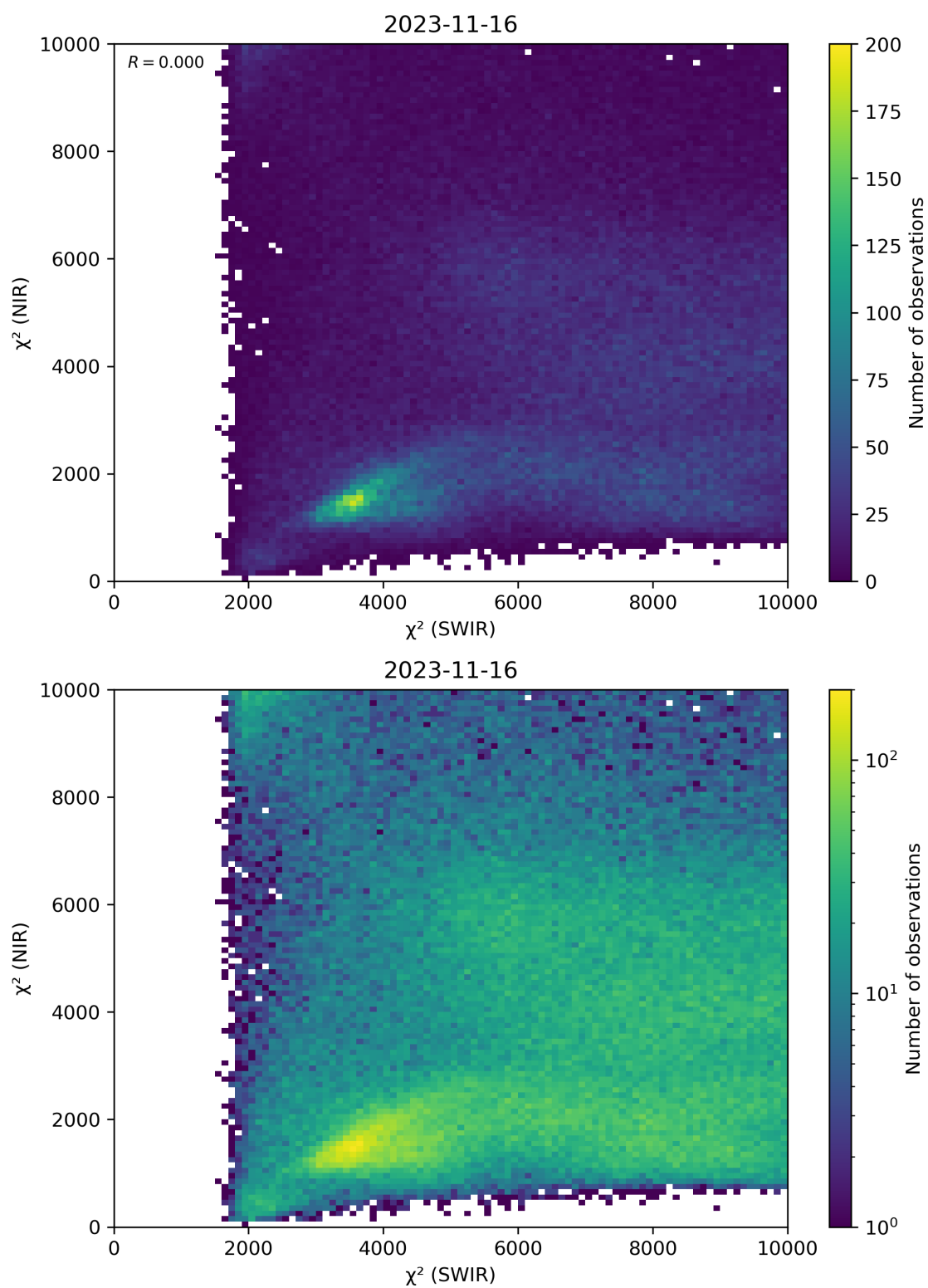
Figure 47: Scatter density plot of “ \chi^2 (SWIR)” against “ \chi^2 (NIR)” for 2023-11-15 to 2023-11-17.
