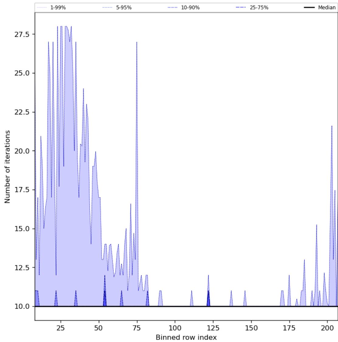
Figure 42: Along track statistics of “Number of iterations” for 2023-11-15 to 2023-11-17
