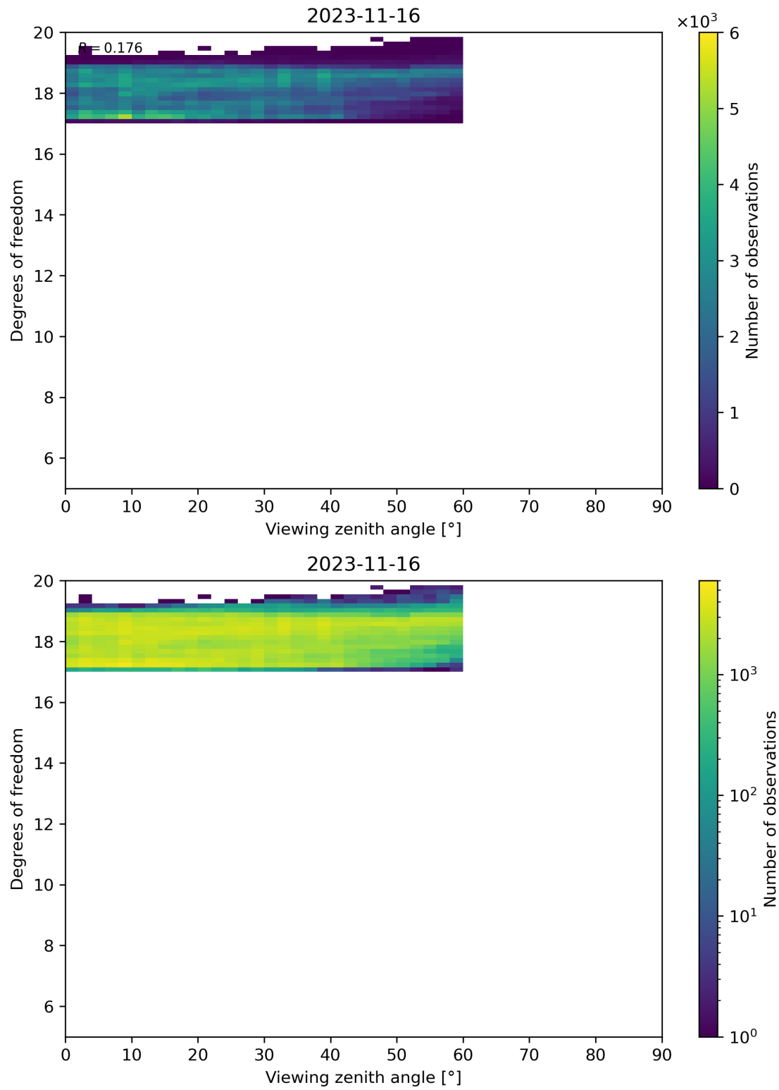
Figure 107: Scatter density plot of “Viewing zenith angle” against “Degrees of freedom” for 2023-11-15 to 2023-11-17.
