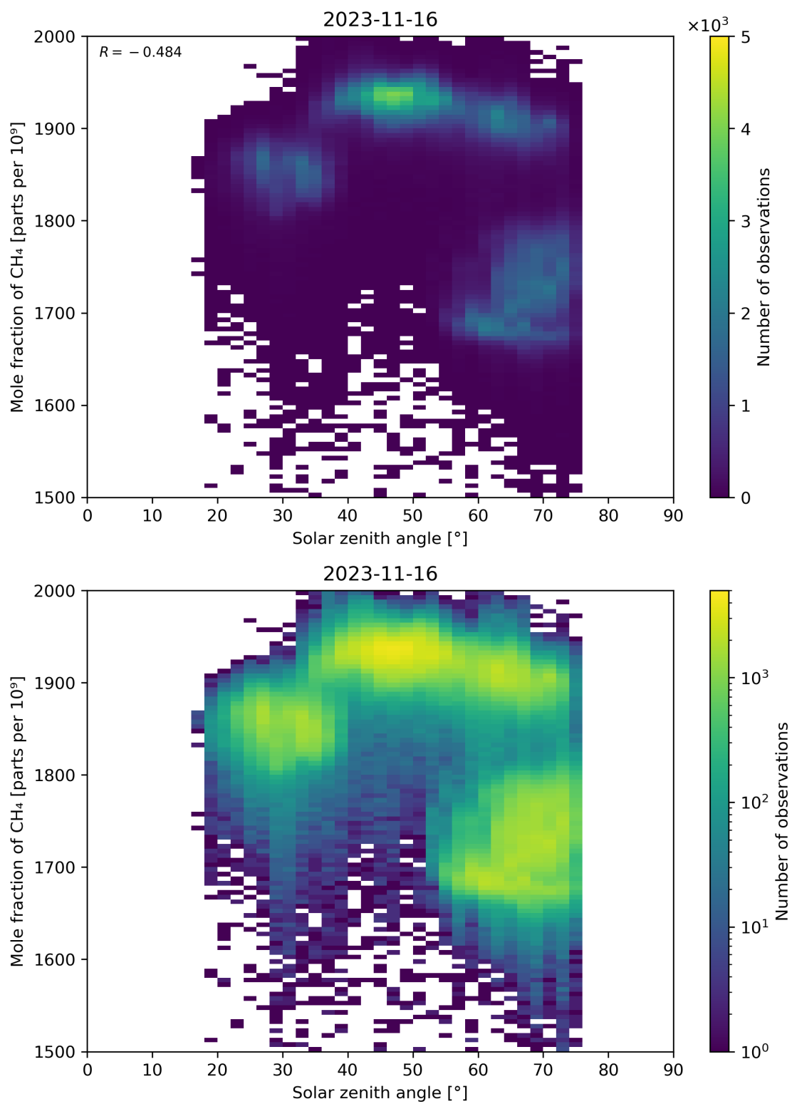
Figure 99: Scatter density plot of “Solar zenith angle” against “Mole fraction of CH 4 ” for 2023-11-15 to 2023-11-17.
