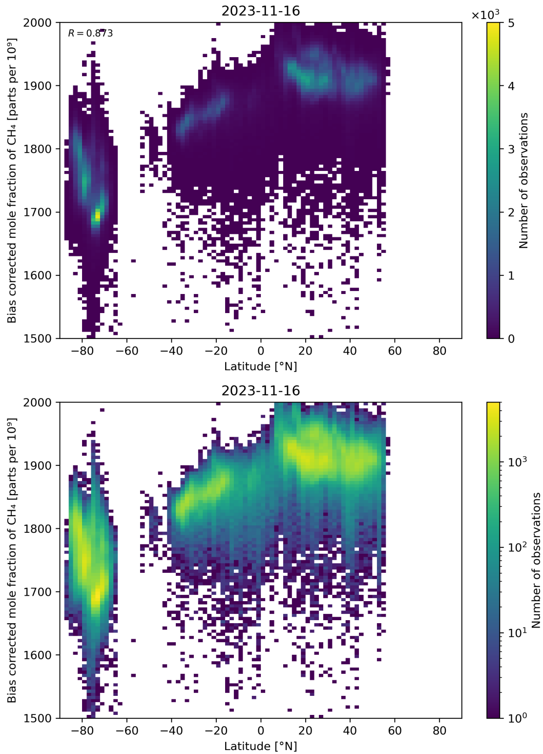
Figure 58: Scatter density plot of “Latitude” against “Bias corrected mole fraction of CH 4 ” for 2023-11-15 to 2023-11-17.
