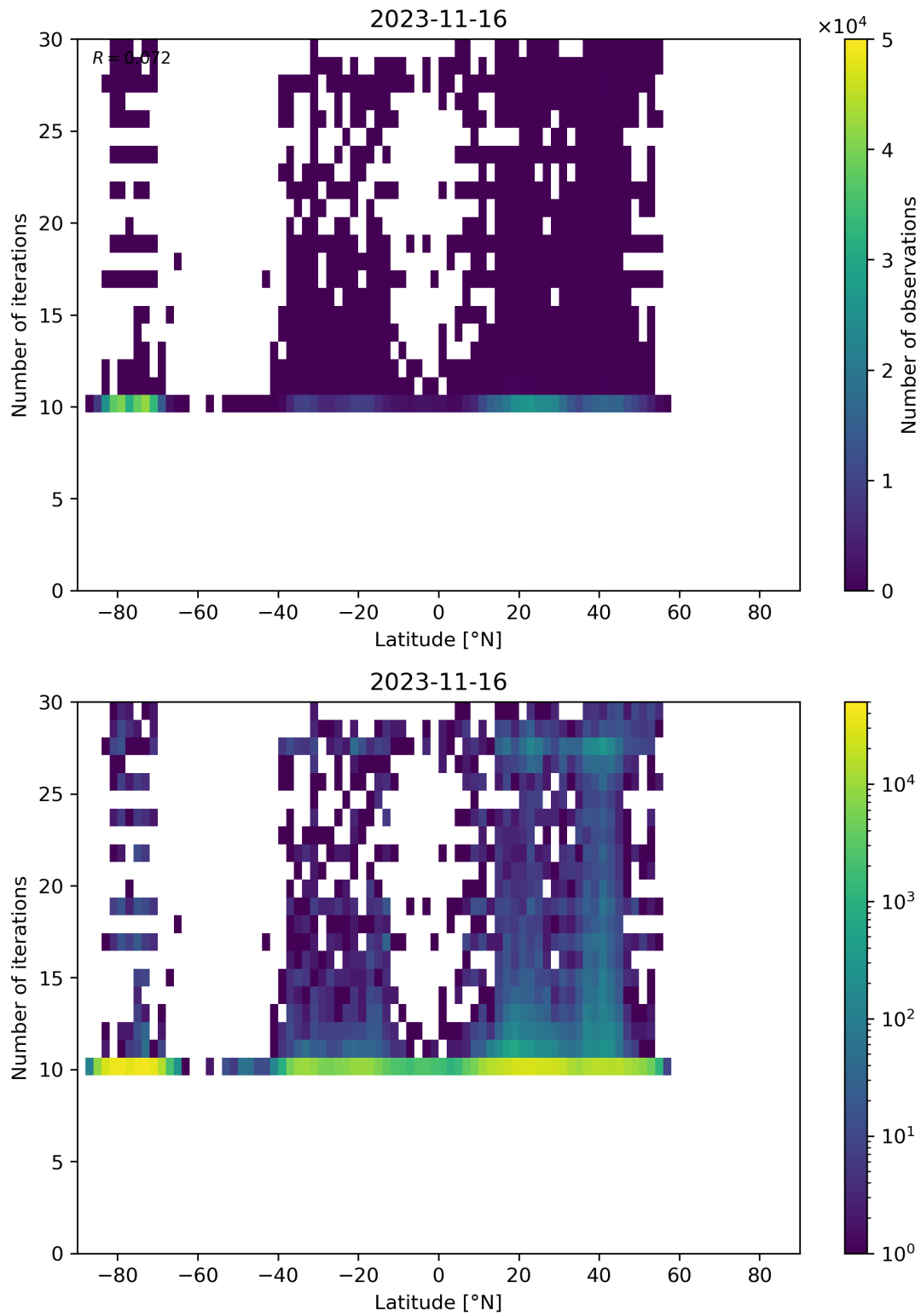
Figure 60: Scatter density plot of “Latitude” against “Number of iterations” for 2023-11-15 to 2023-11-17.
