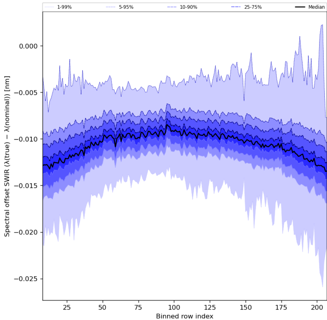
Figure 38: Along track statistics of “Spectral offset SWIR ( \lambda(\text{true}) - \lambda(\text{nominal}) )” for 2023-11-15 to 2023-11-17
