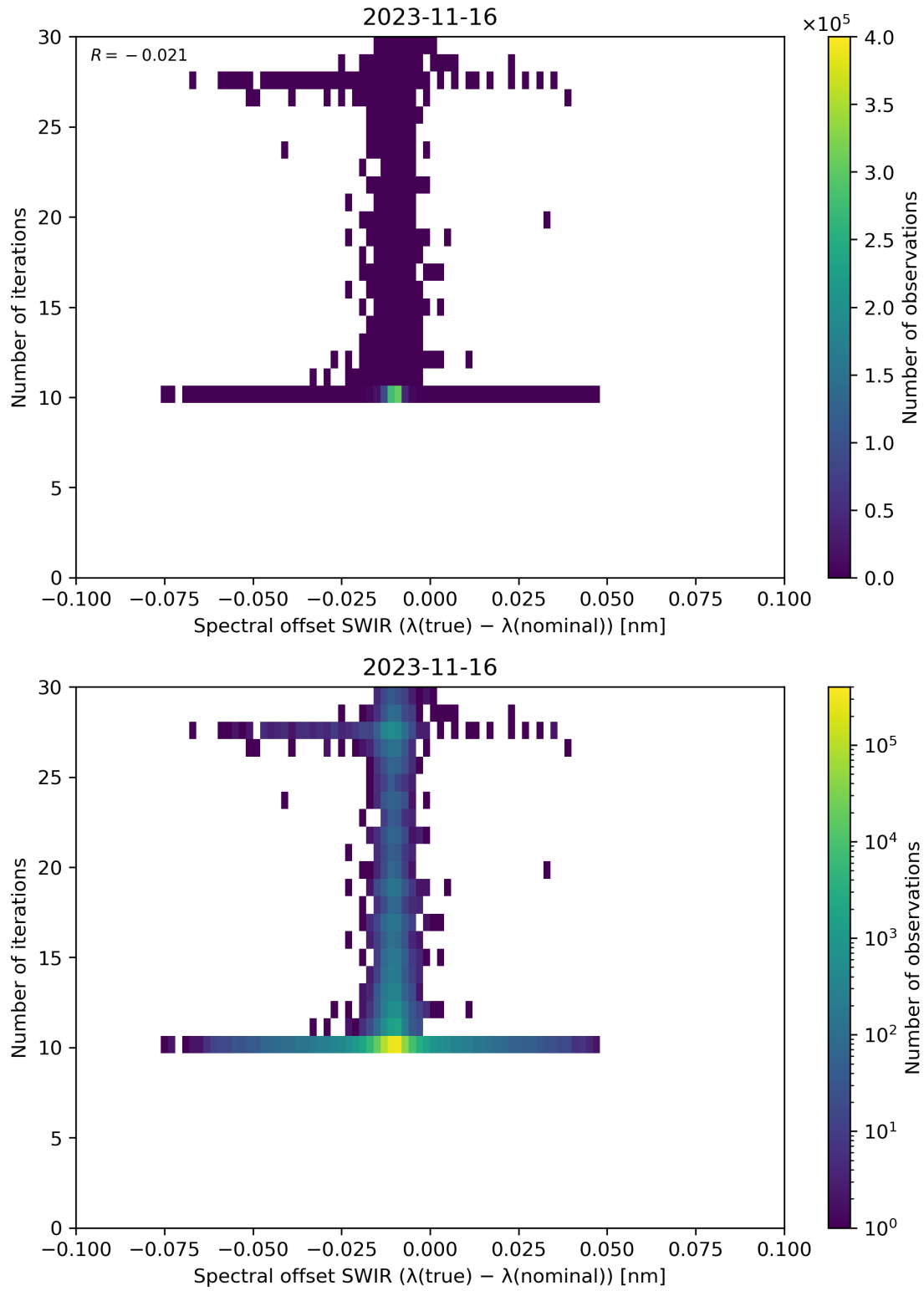
Figure 121: Scatter density plot of “Spectral offset SWIR ( \lambda(\text{true}) - \lambda(\text{nominal}) )” against “Number of iterations” for 2023-11-15 to 2023-11-17.
