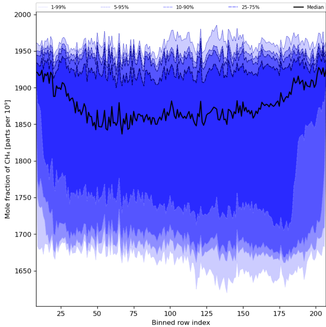
Figure 34: Along track statistics of “Mole fraction of CH 4 ” for 2023-11-15 to 2023-11-17
