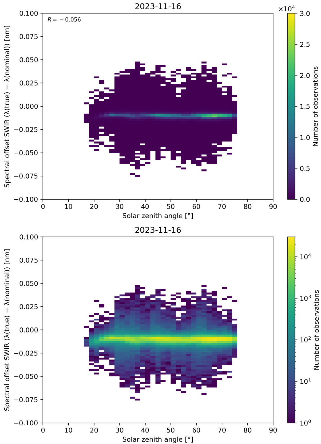
Figure 104: Scatter density plot of “Solar zenith angle” against “Spectral offset SWIR ( \lambda(\text{true}) - \lambda(\text{nominal}) )” for 2023-11-15 to 2023-11-17.
