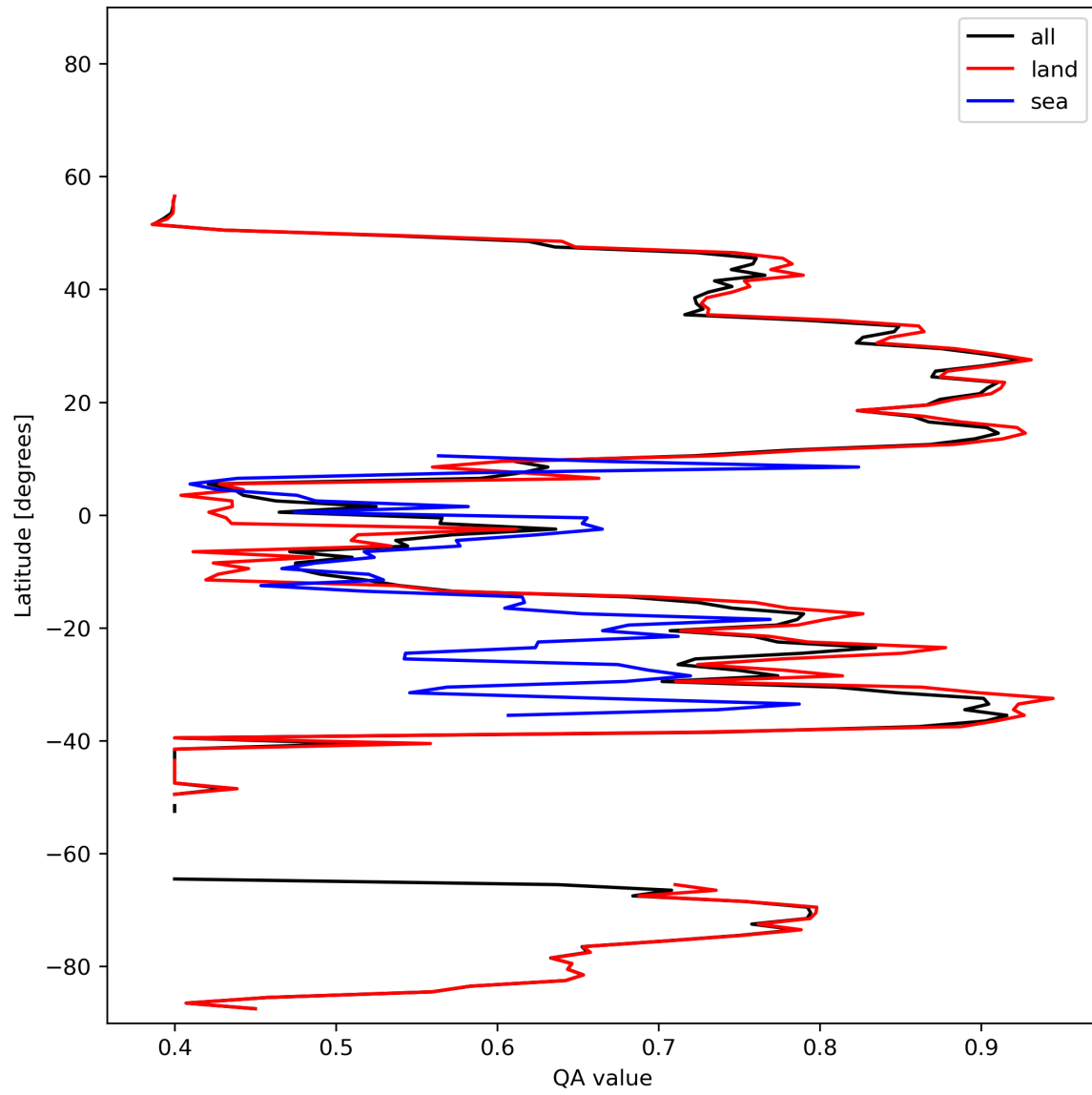
Figure 11: Zonal average of “QA value” for 2023-11-15 to 2023-11-17.
