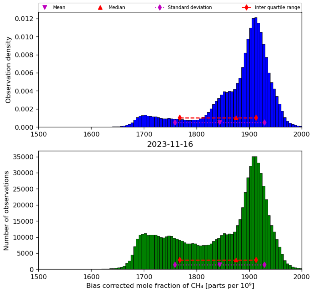
Figure 25: Histogram of “Bias corrected mole fraction of CH 4 ” for 2023-11-15 to 2023-11-17
