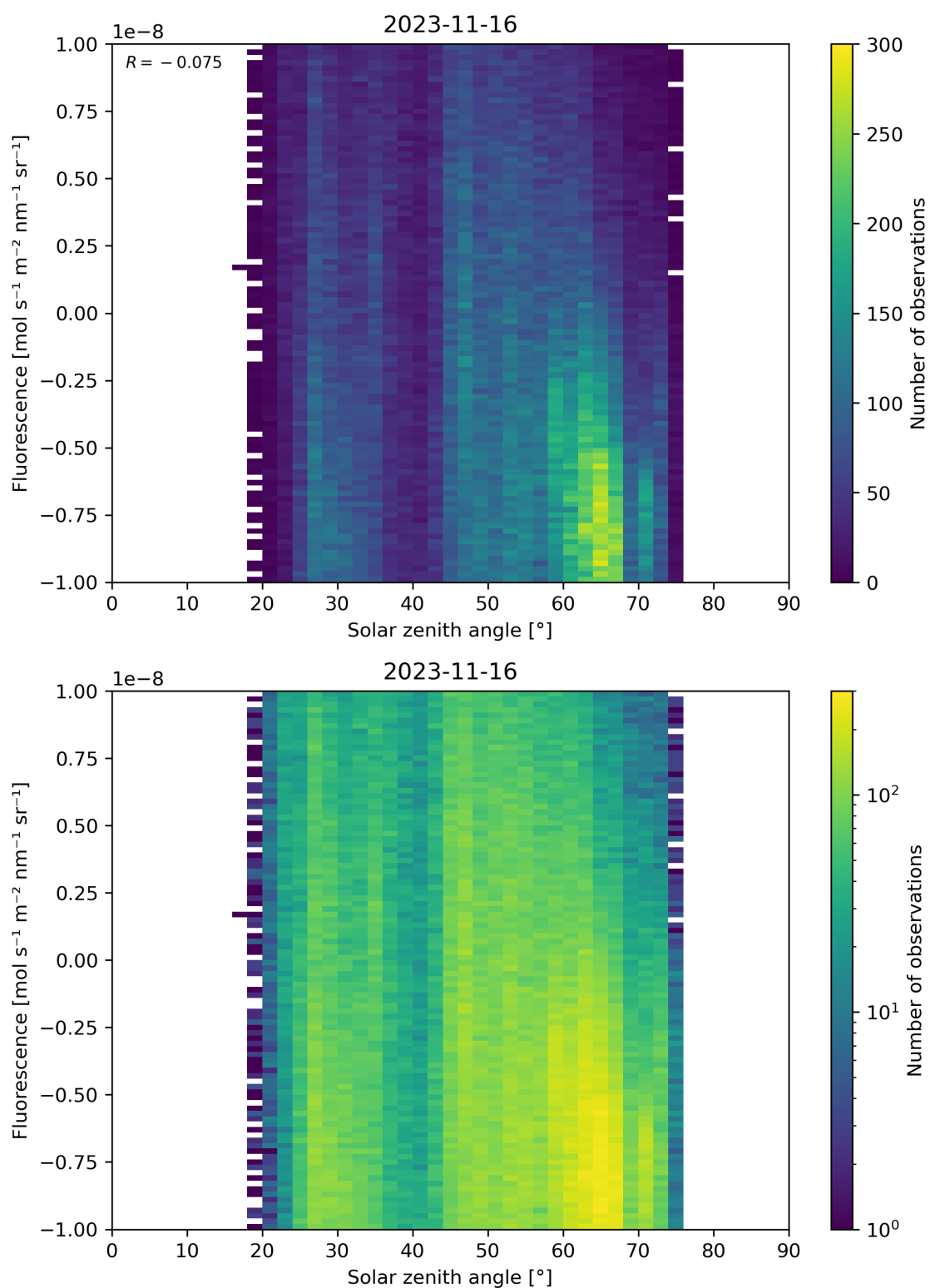
Figure 97: Scatter density plot of “Solar zenith angle” against “Fluorescence” for 2023-11-15 to 2023-11-17.
