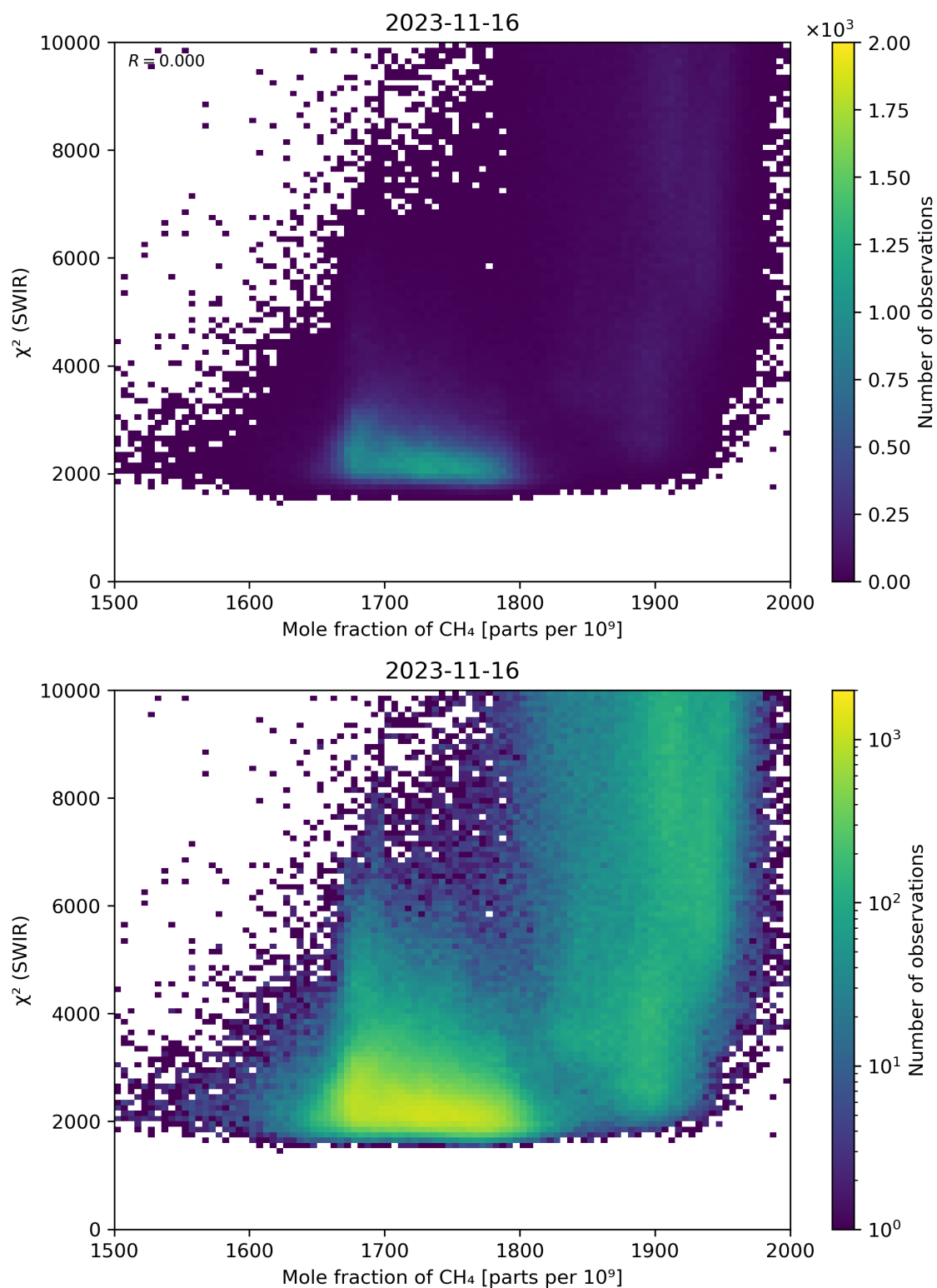
Figure 71: Scatter density plot of “Mole fraction of \text{CH}_4 ” against “ \chi^2 (SWIR)” for 2023-11-15 to 2023-11-17.
