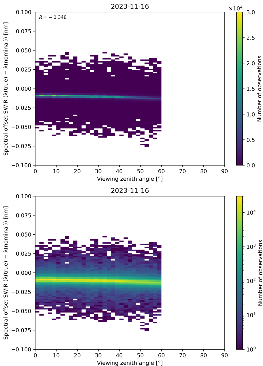
Figure 116: Scatter density plot of “Viewing zenith angle” against “Spectral offset SWIR ( \lambda(\text{true}) - \lambda(\text{nominal}) )” for 2023-11-15 to 2023-11-17.
