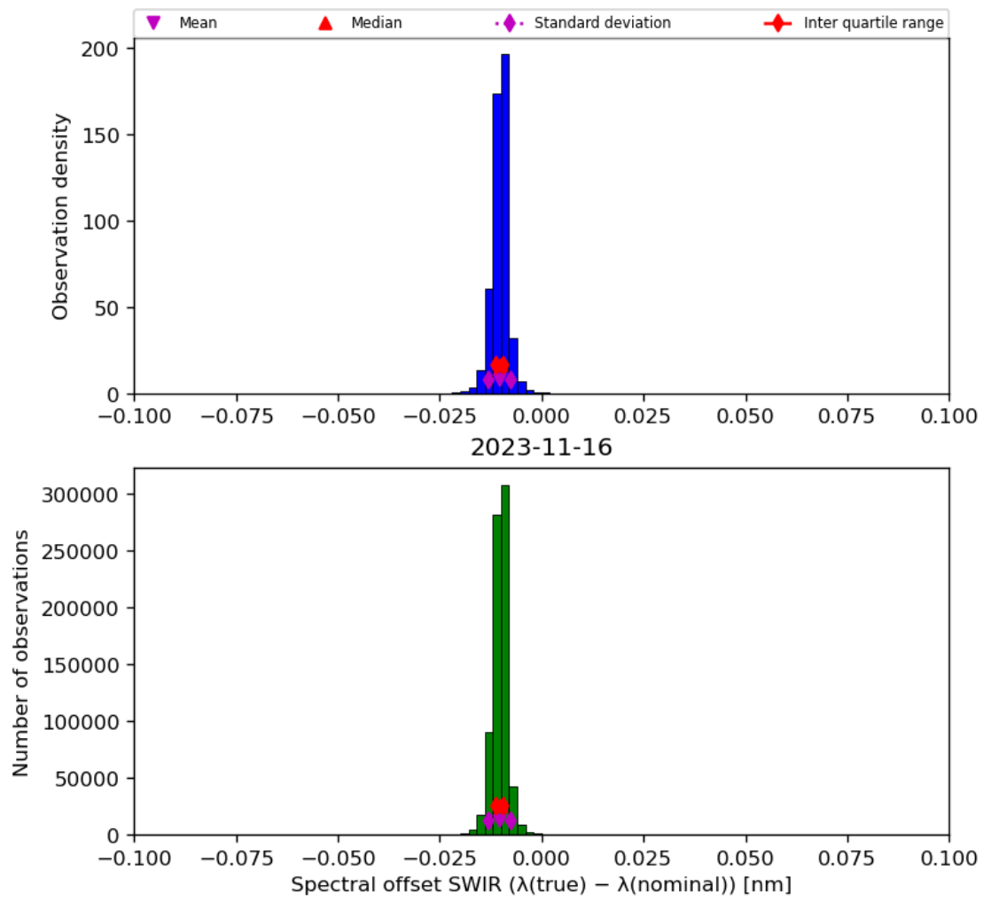
Figure 27: Histogram of “Spectral offset SWIR ( \lambda(\text{true}) - \lambda(\text{nominal}) )” for 2023-11-15 to 2023-11-17
