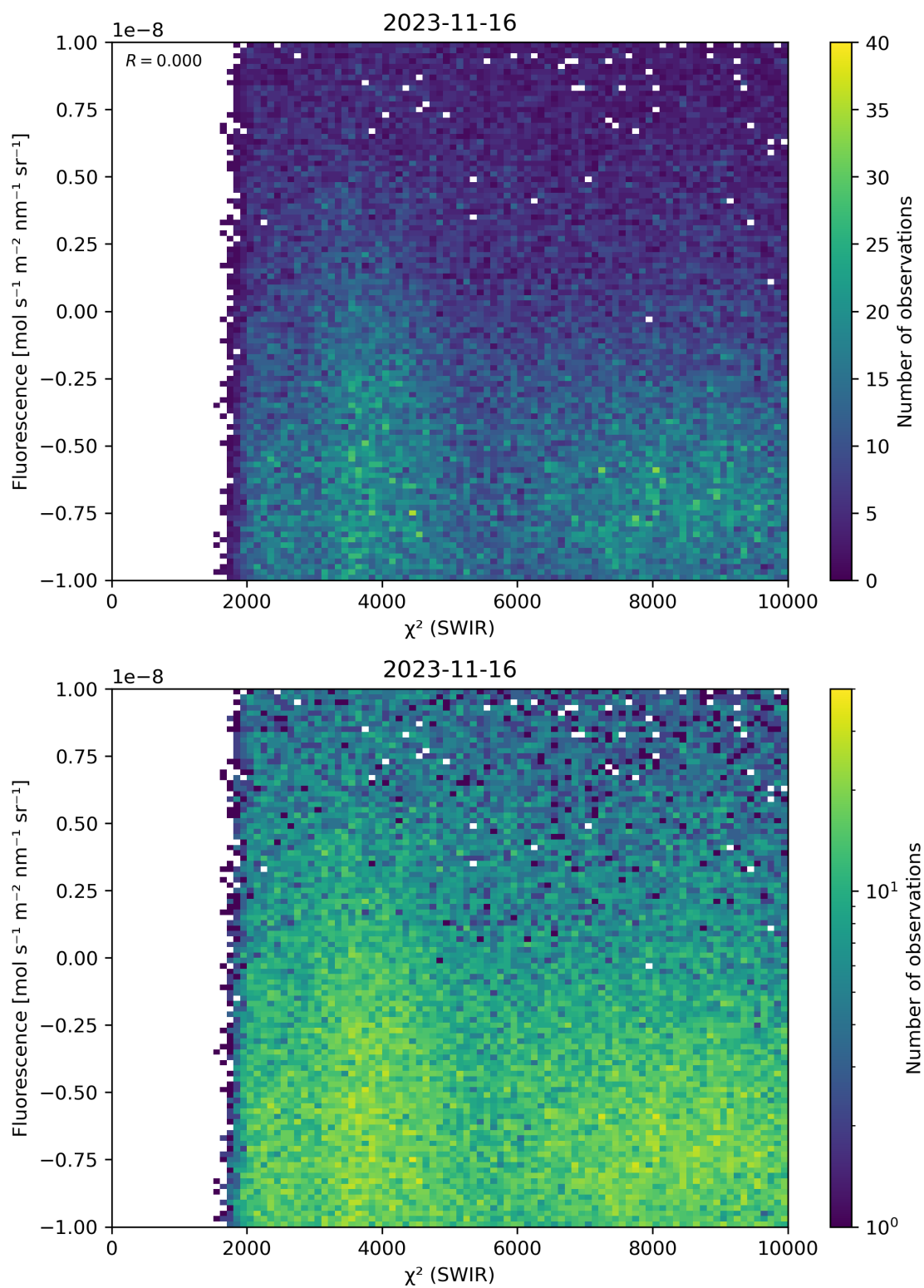
Figure 49: Scatter density plot of “ \chi^2 (SWIR)” against “Fluorescence” for 2023-11-15 to 2023-11-17.
