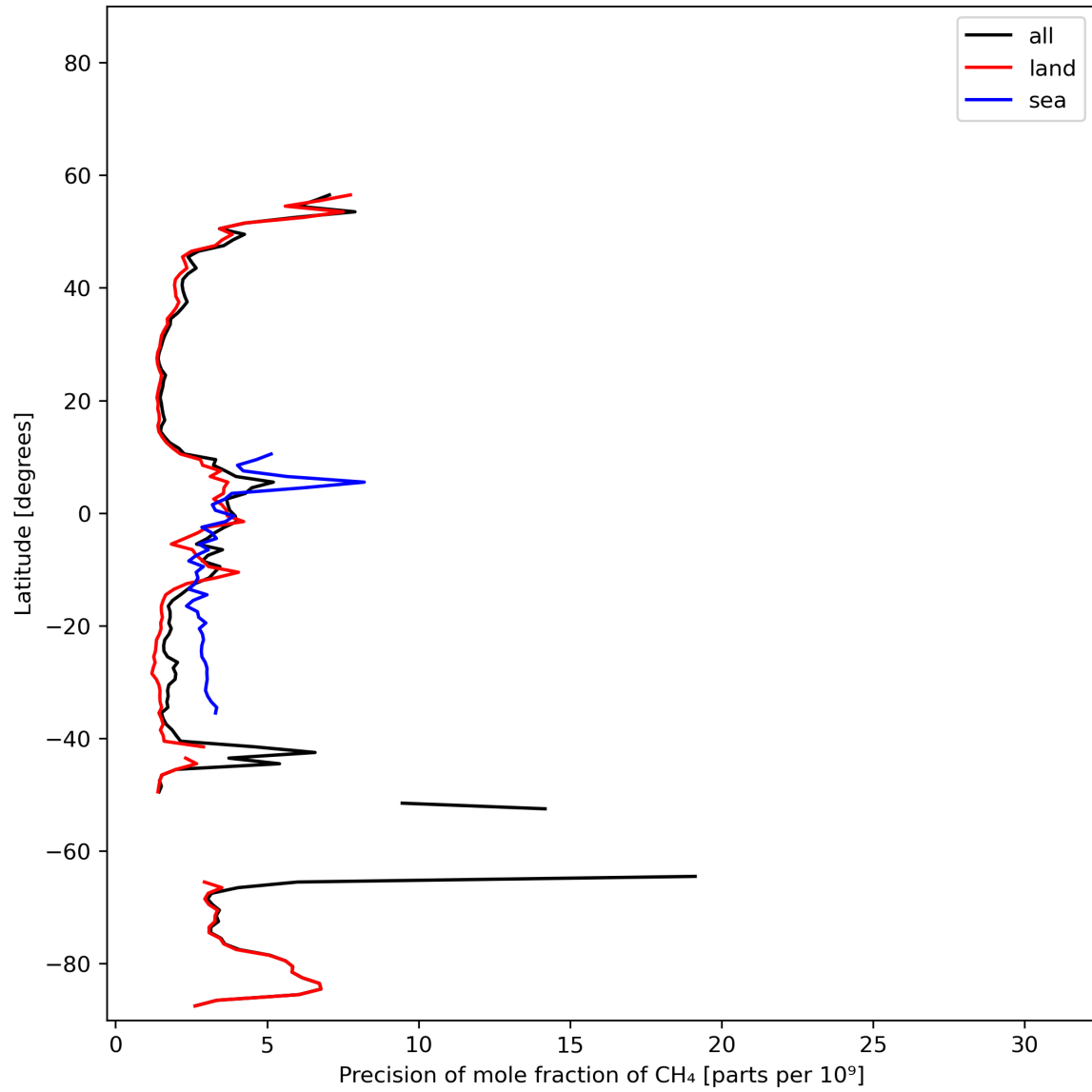
Figure 13: Zonal average of “Precision of mole fraction of CH 4 ” for 2023-11-15 to 2023-11-17.
