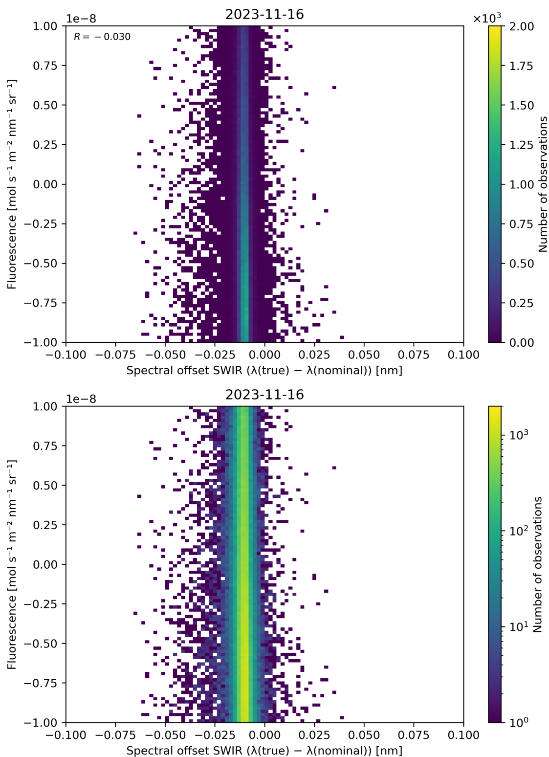
Figure 120: Scatter density plot of “Spectral offset SWIR ( \lambda(\text{true}) - \lambda(\text{nominal}) )” against “Fluorescence” for 2023-11-15 to 2023-11-17.
