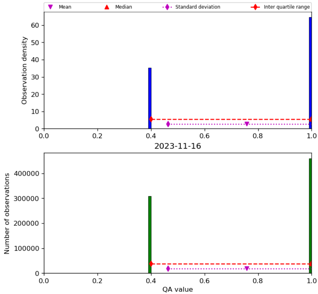
Figure 22: Histogram of “QA value” for 2023-11-15 to 2023-11-17
