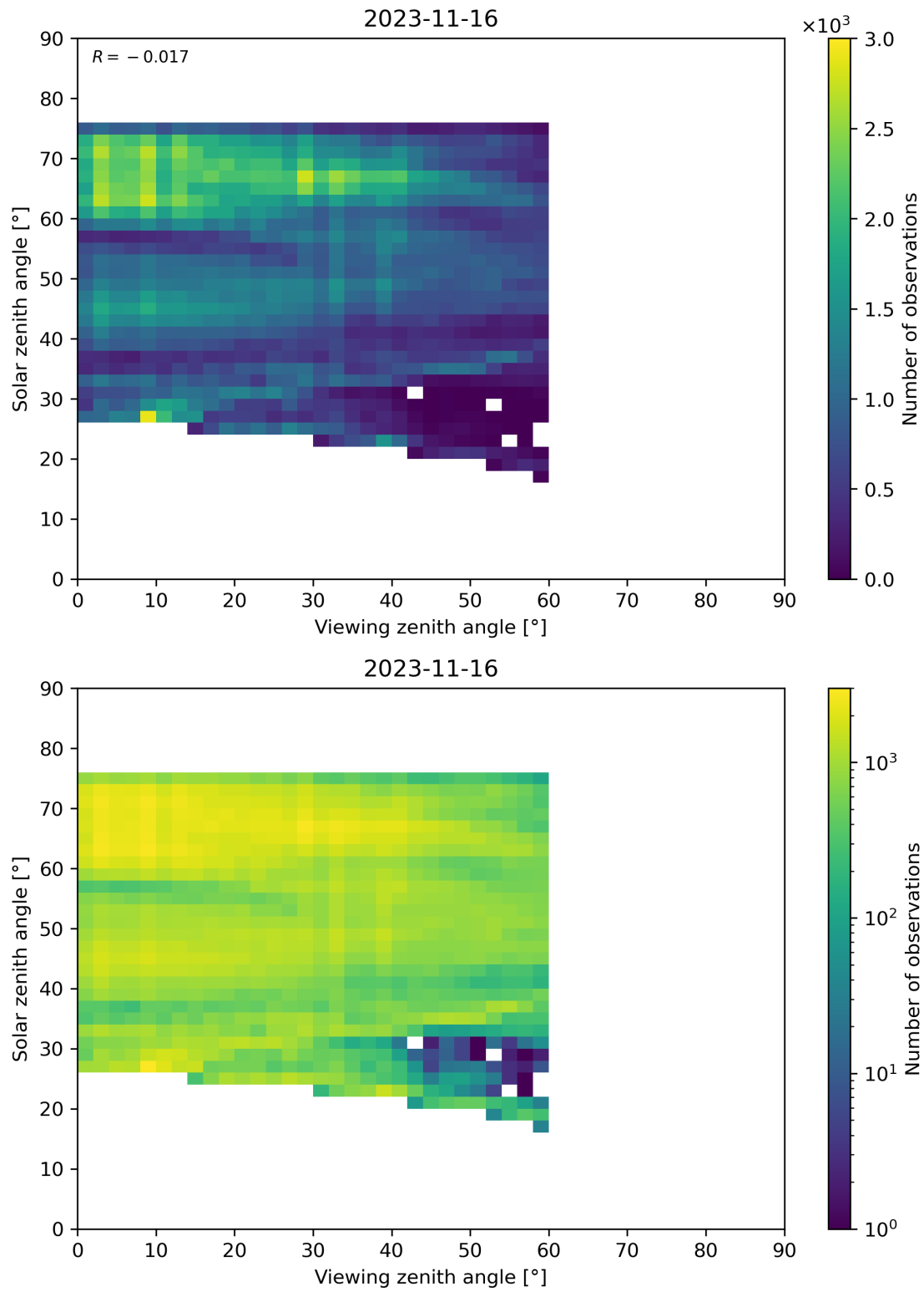
Figure 115: Scatter density plot of “Viewing zenith angle” against “Solar zenith angle” for 2023-11-15 to 2023-11-17.
