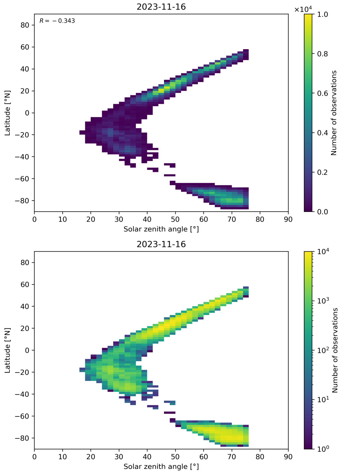
Figure 98: Scatter density plot of “Solar zenith angle” against “Latitude” for 2023-11-15 to 2023-11-17.
