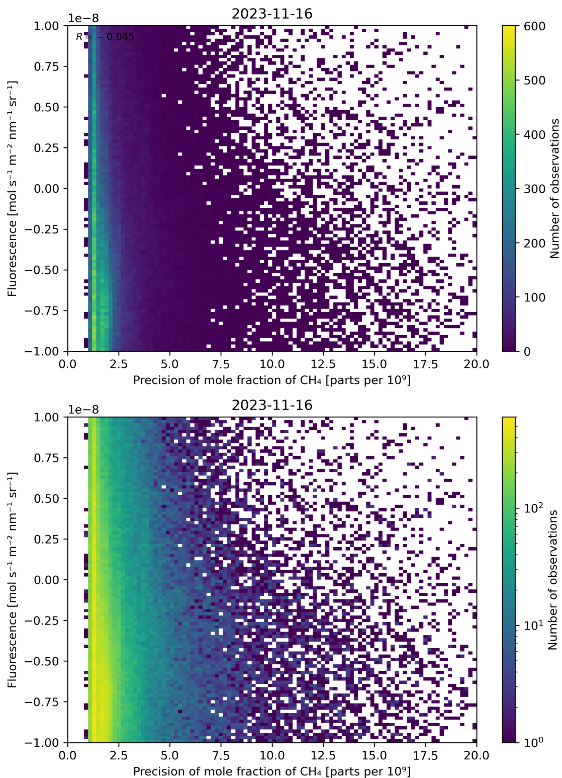
Figure 81: Scatter density plot of “Precision of mole fraction of \text{CH}_4 ” against “Fluorescence” for 2023-11-15 to 2023-11-17.
