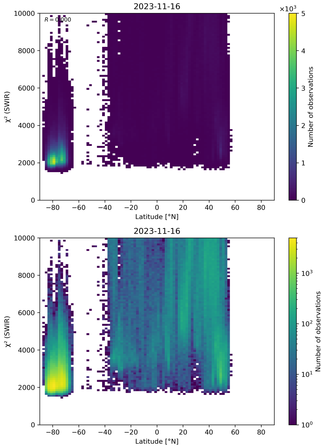
Figure 54: Scatter density plot of “Latitude” against “ \chi^2 (SWIR)” for 2023-11-15 to 2023-11-17.
