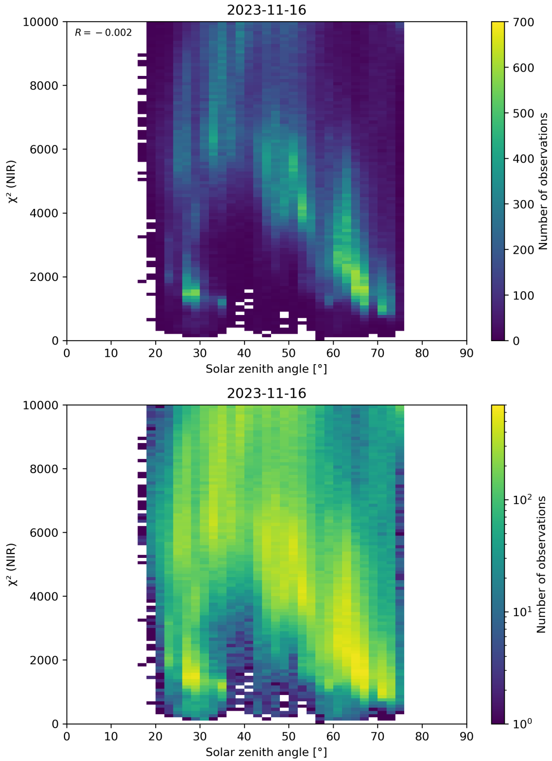
Figure 94: Scatter density plot of “Solar zenith angle” against “ \chi^2 (NIR)” for 2023-11-15 to 2023-11-17.
