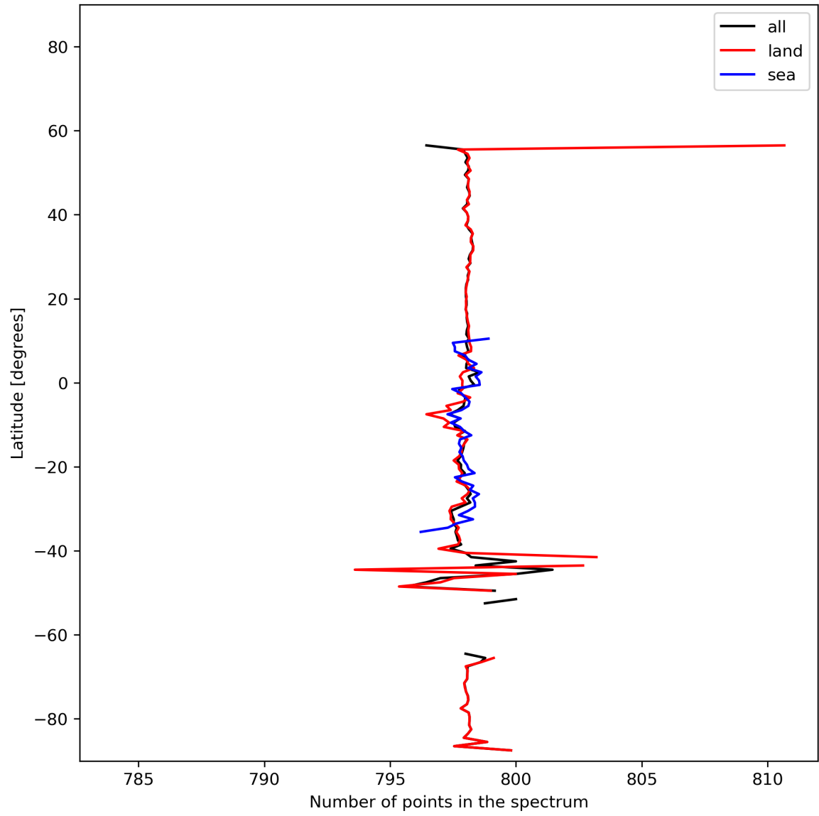
Figure 15: Zonal average of “Number of points in the spectrum” for 2023-11-15 to 2023-11-17.
