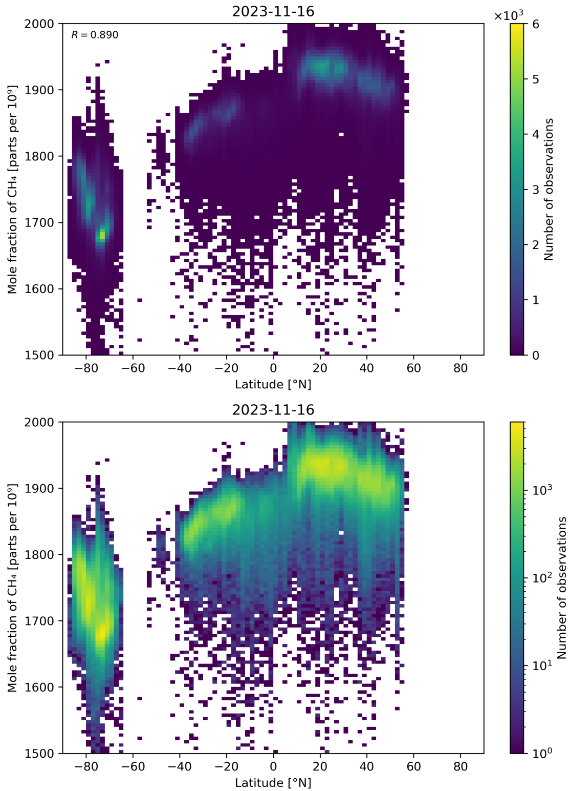
Figure 57: Scatter density plot of “Latitude” against “Mole fraction of CH 4 ” for 2023-11-15 to 2023-11-17.
