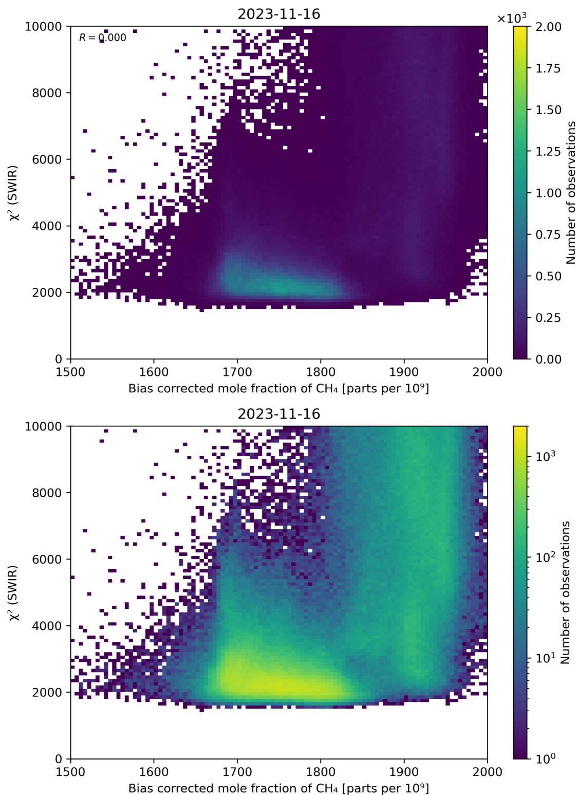
Figure 64: Scatter density plot of “Bias corrected mole fraction of CH 4 ” against “ \chi^2 (SWIR)” for 2023-11-15 to 2023-11-17.
