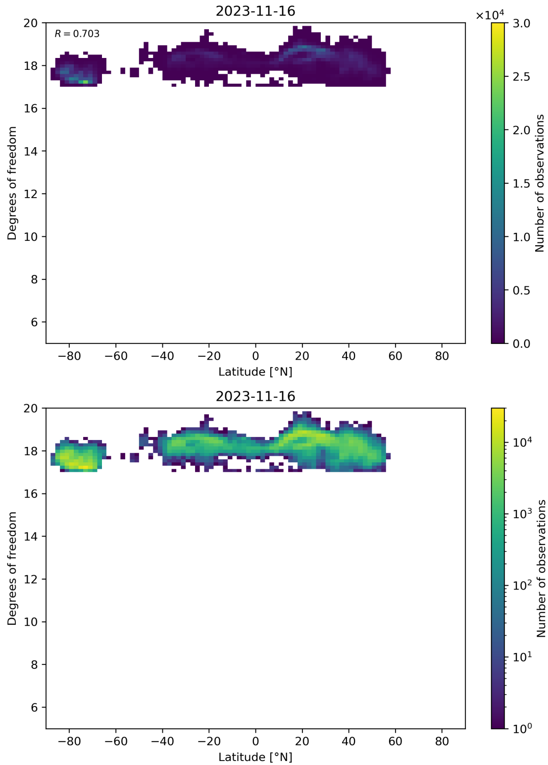
Figure 55: Scatter density plot of “Latitude” against “Degrees of freedom” for 2023-11-15 to 2023-11-17.
