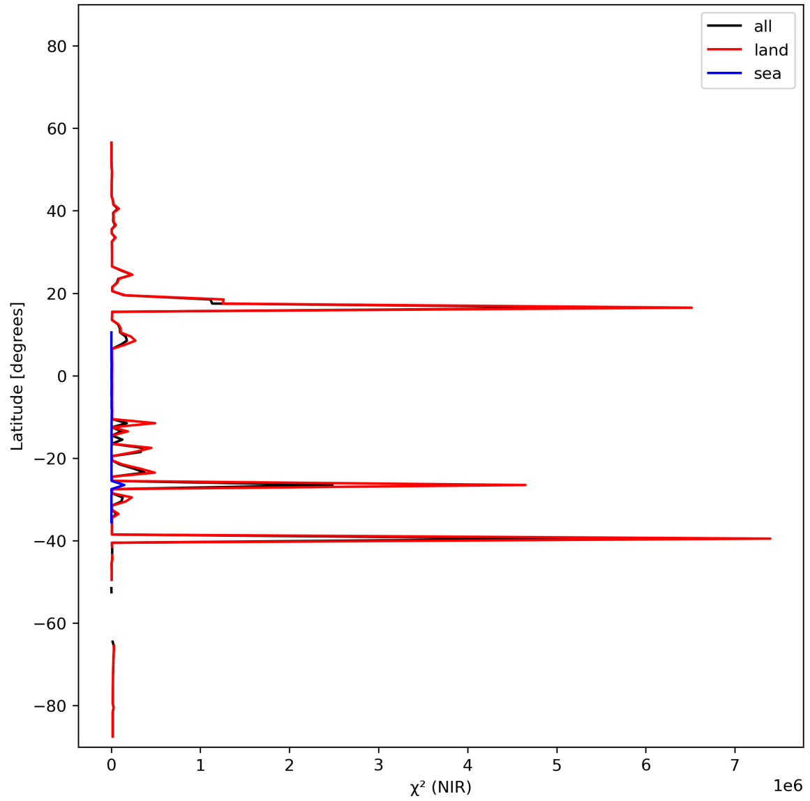
Figure 18: Zonal average of “ \chi^2 (NIR)” for 2023-11-15 to 2023-11-17.
