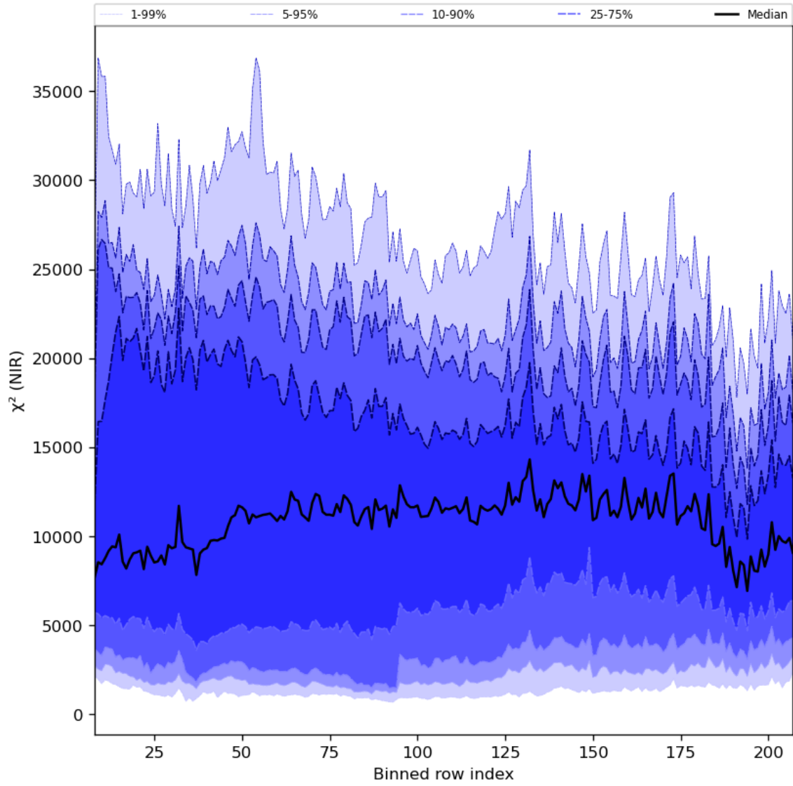
Figure 40: Along track statistics of “ \chi^2 (NIR)” for 2023-11-15 to 2023-11-17
