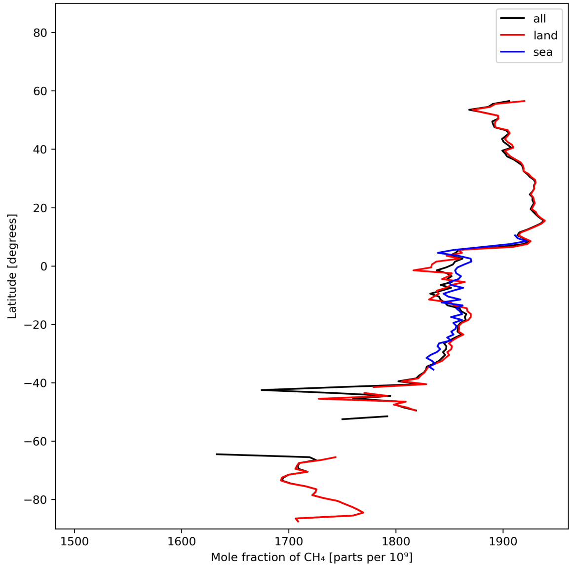
Figure 12: Zonal average of “Mole fraction of \text{CH}_4 ” for 2023-11-15 to 2023-11-17.
