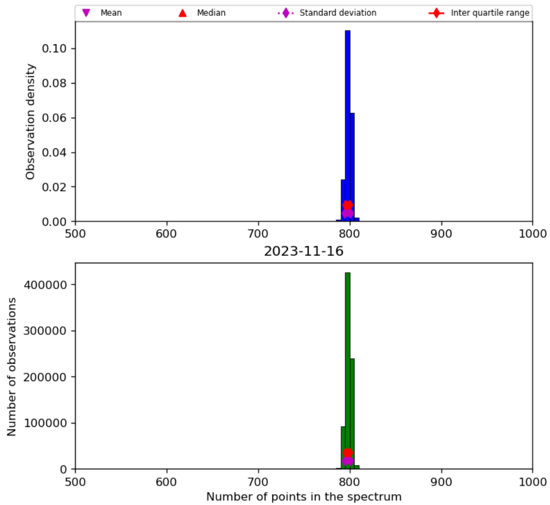
Figure 26: Histogram of “Number of points in the spectrum” for 2023-11-15 to 2023-11-17
