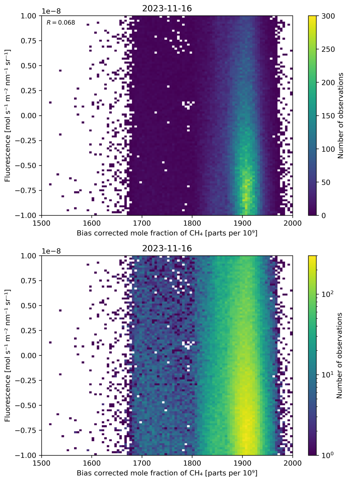
Figure 66: Scatter density plot of “Bias corrected mole fraction of \text{CH}_4 ” against “Fluorescence” for 2023-11-15 to 2023-11-17.
