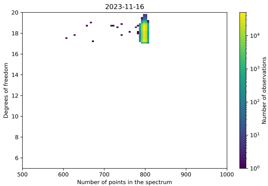
Figure 90: Scatter density plot of “Number of points in the spectrum” against “Degrees of freedom” for 2023-11-15 to 2023-11-17.
