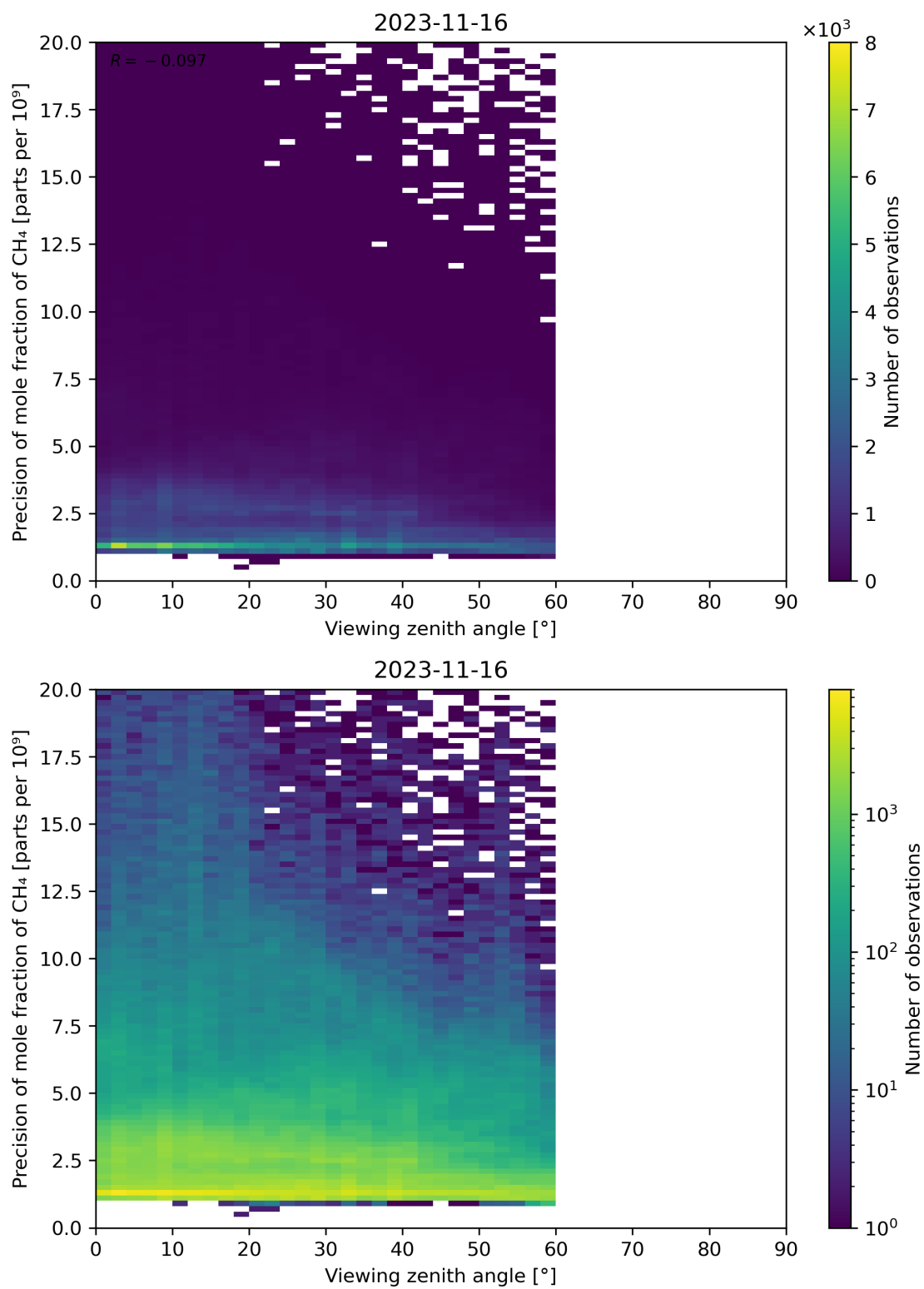
Figure 112: Scatter density plot of “Viewing zenith angle” against “Precision of mole fraction of CH 4 ” for 2023-11-15 to 2023-11-17.
