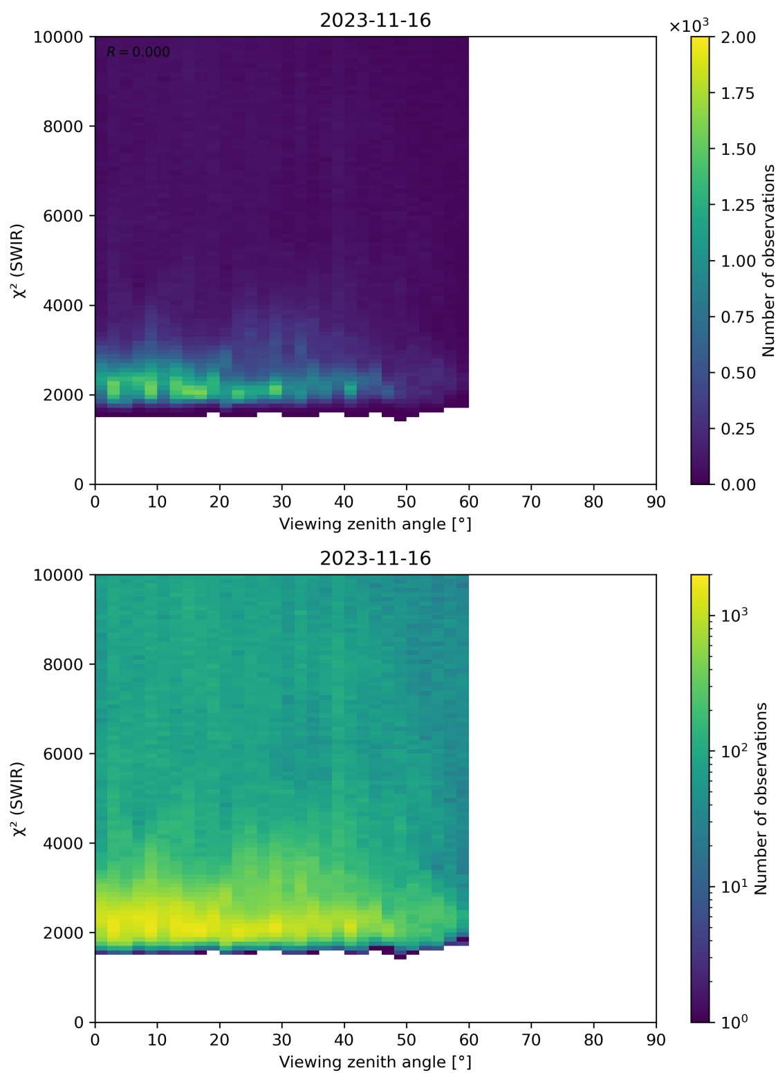
Figure 106: Scatter density plot of “Viewing zenith angle” against “ \chi^2 (SWIR)” for 2023-11-15 to 2023-11-17.
