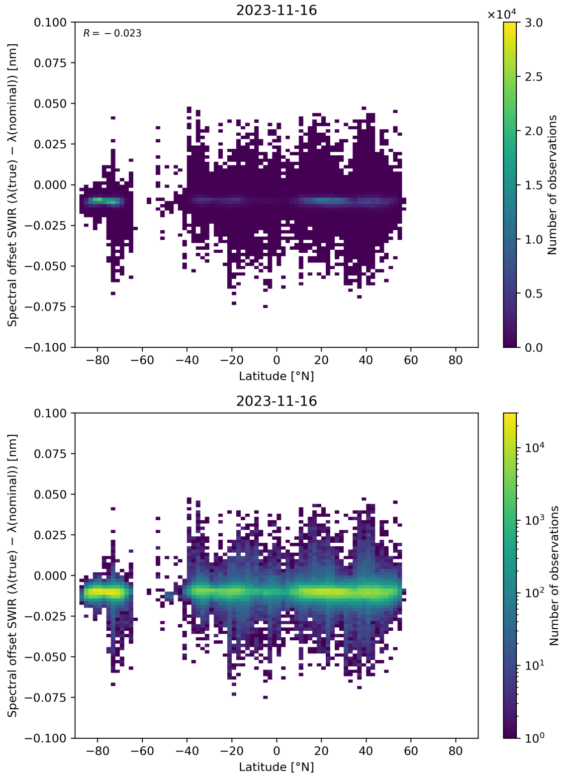
Figure 62: Scatter density plot of “Latitude” against “Spectral offset SWIR ( \lambda(\text{true}) - \lambda(\text{nominal}) )” for 2023-11-15 to 2023-11-17.
