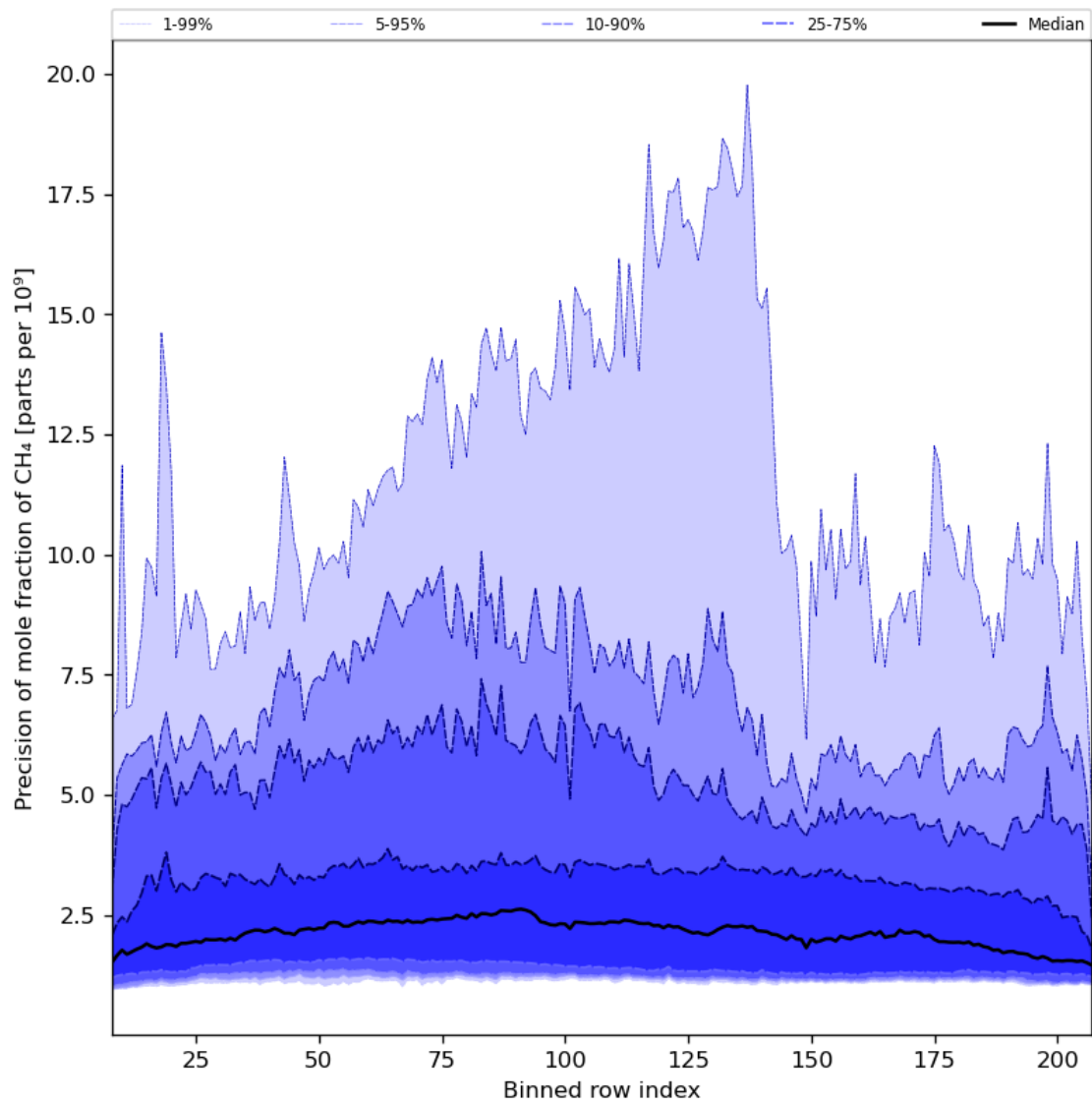
Figure 35: Along track statistics of “Precision of mole fraction of CH 4 ” for 2023-11-15 to 2023-11-17
