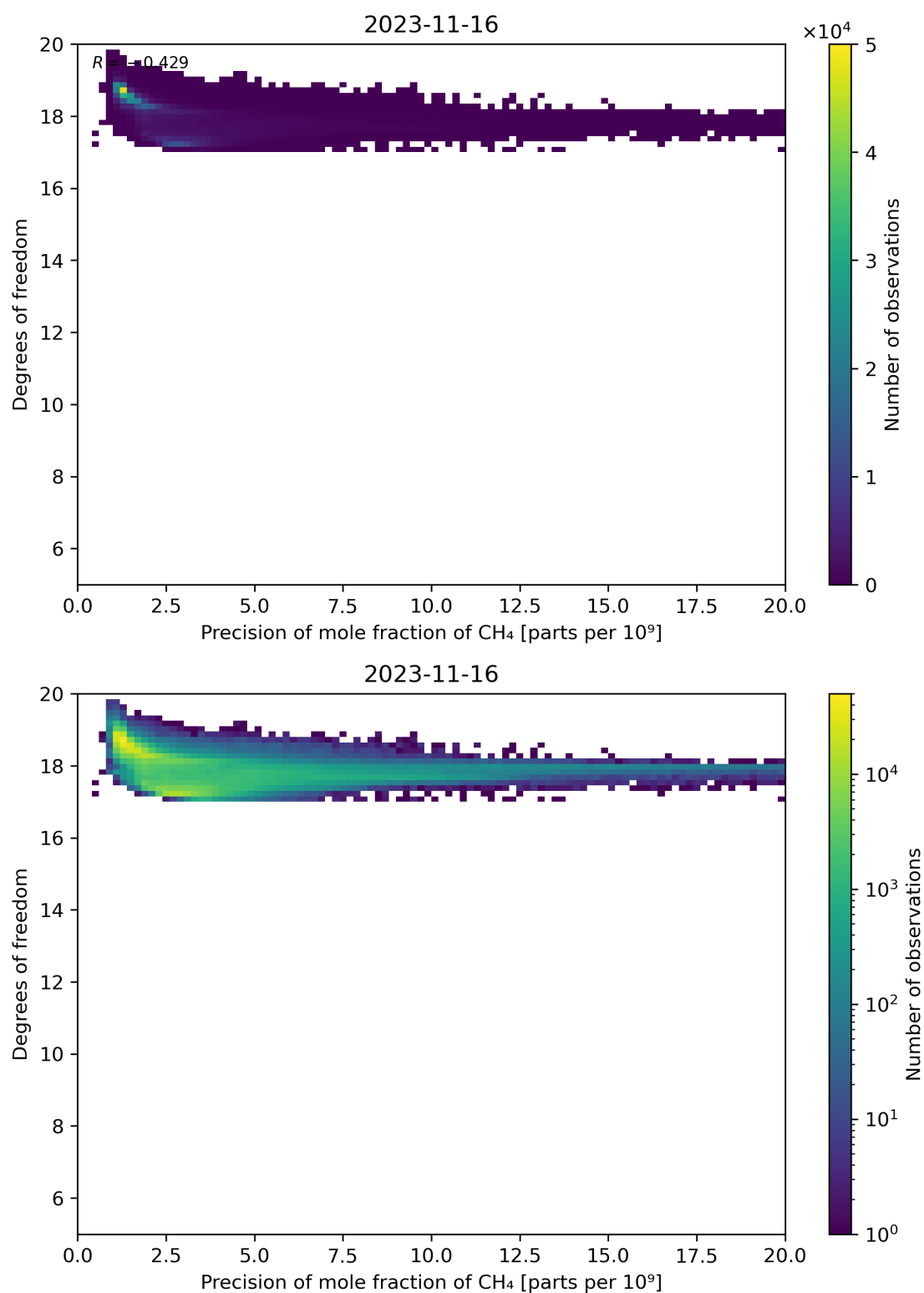
Figure 80: Scatter density plot of “Precision of mole fraction of CH 4 ” against “Degrees of freedom” for 2023-11-15 to 2023-11-17.
