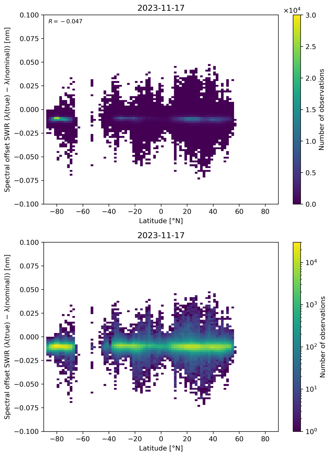
Figure 62: Scatter density plot of “Latitude” against “Spectral offset SWIR ( \lambda(\text{true}) - \lambda(\text{nominal}) )” for 2023-11-16 to 2023-11-18.
