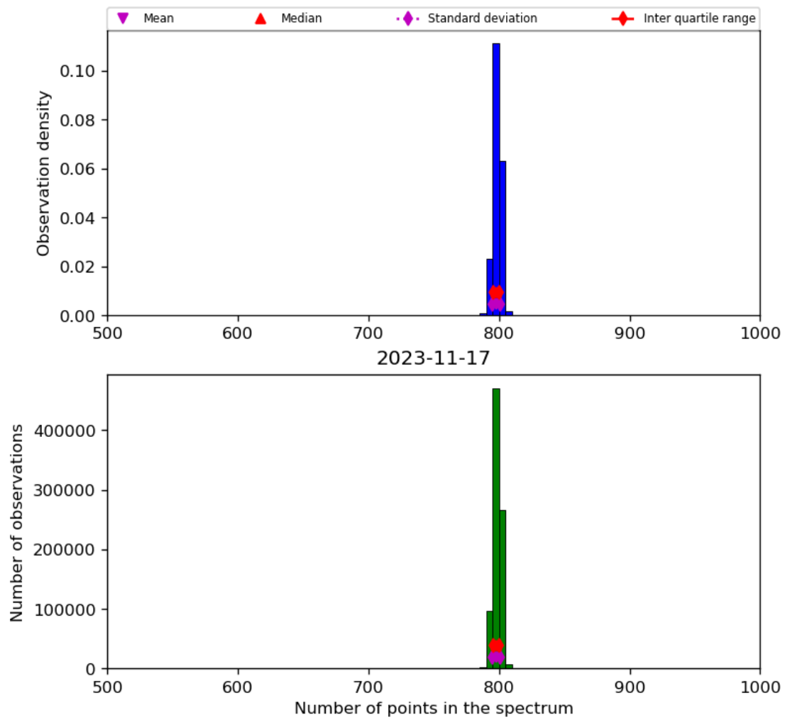
Figure 26: Histogram of “Number of points in the spectrum” for 2023-11-16 to 2023-11-18
