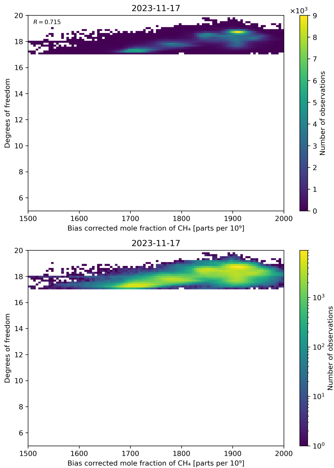
Figure 65: Scatter density plot of “Bias corrected mole fraction of CH 4 ” against “Degrees of freedom” for 2023-11-16 to 2023-11-18.
