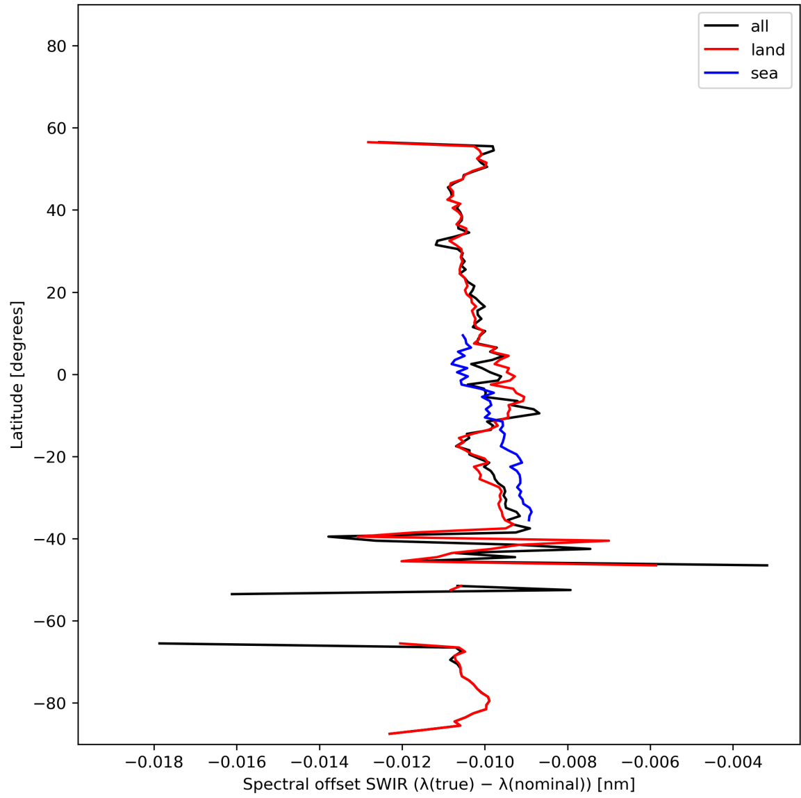
Figure 16: Zonal average of “Spectral offset SWIR ( \lambda(\text{true}) - \lambda(\text{nominal}) )” for 2023-11-16 to 2023-11-18.
