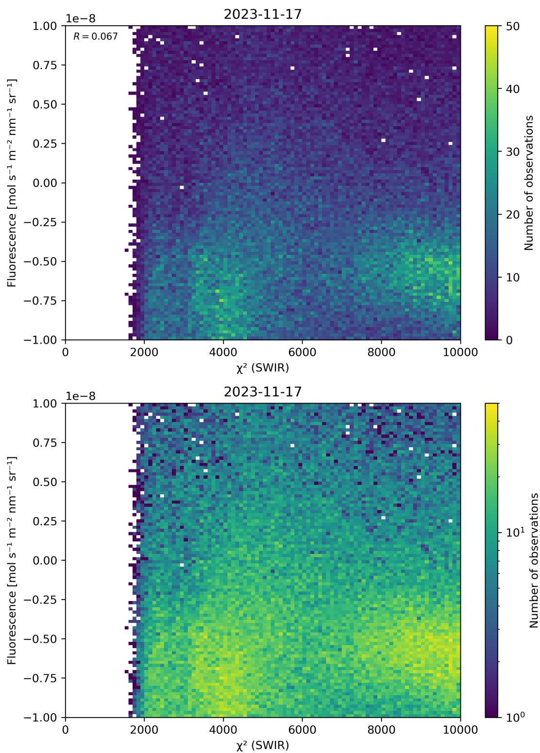
Figure 49: Scatter density plot of “ \chi^2 (SWIR)” against “Fluorescence” for 2023-11-16 to 2023-11-18.
