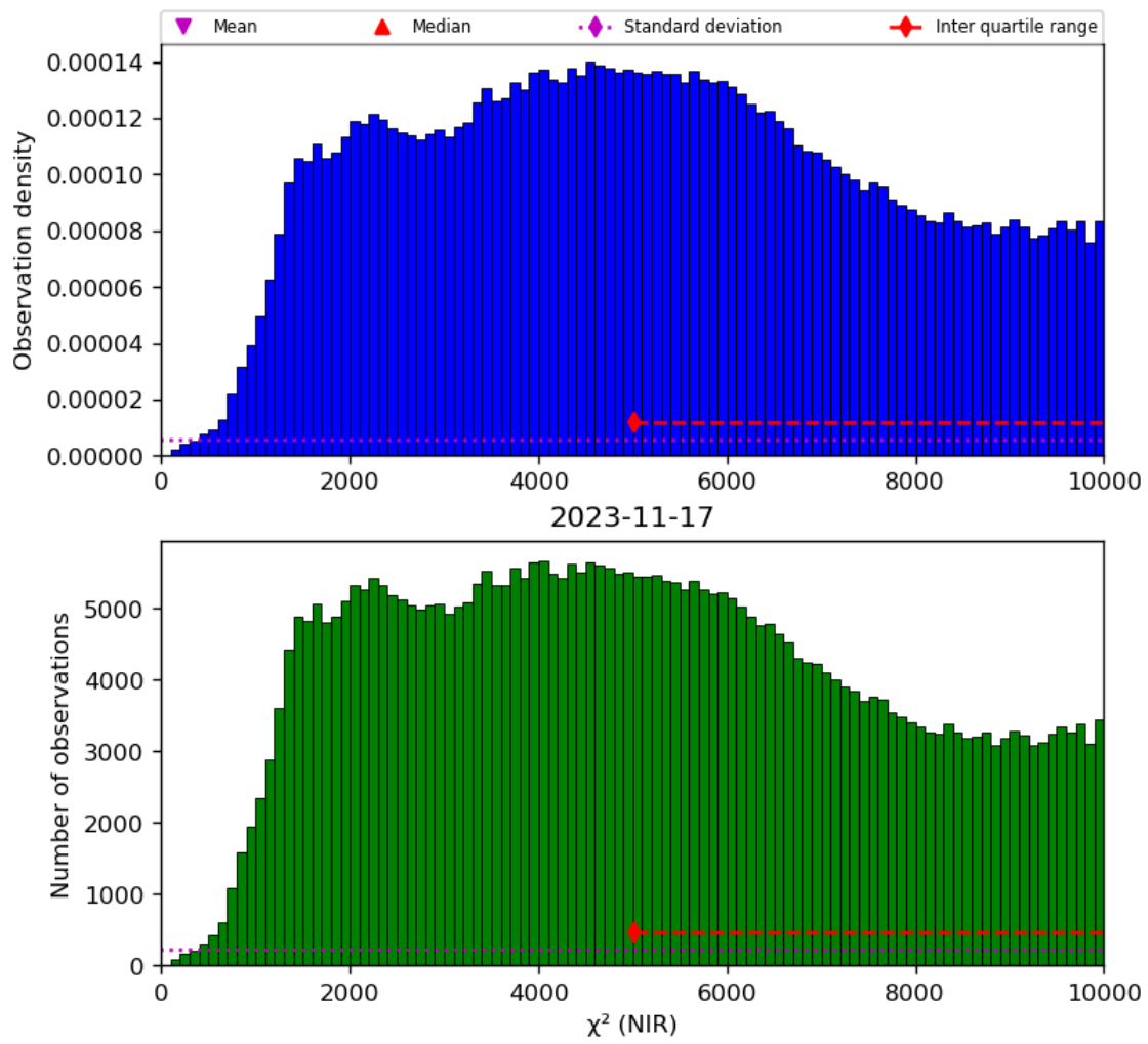
Figure 29: Histogram of “ \chi^2 (NIR)” for 2023-11-16 to 2023-11-18
