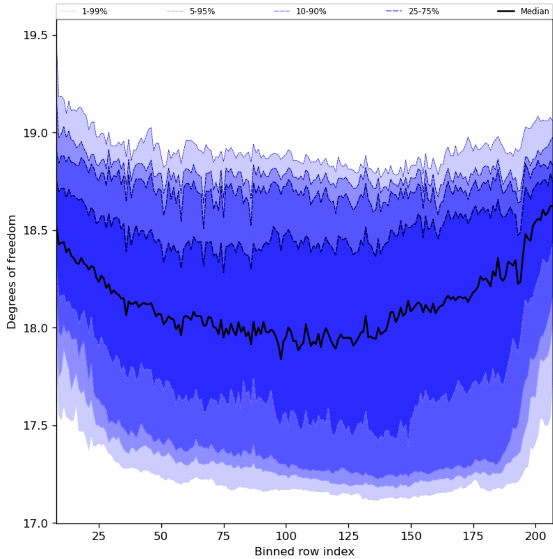
Figure 41: Along track statistics of “Degrees of freedom” for 2023-11-16 to 2023-11-18
