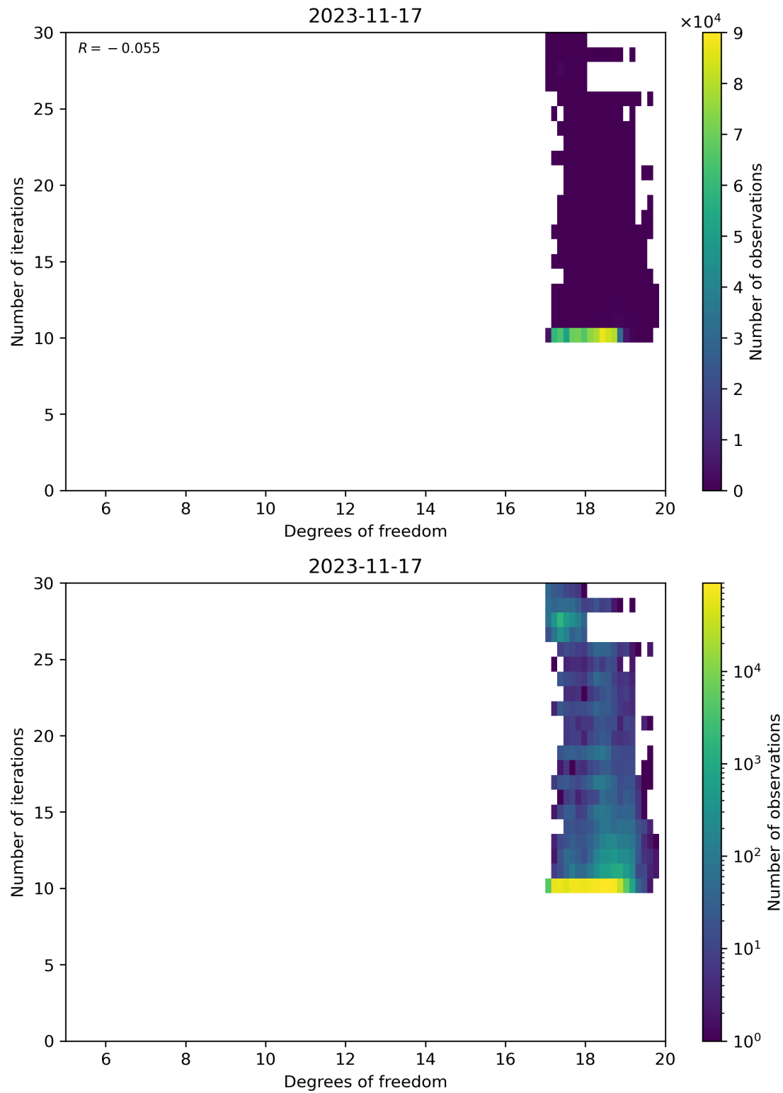
Figure 52: Scatter density plot of “Degrees of freedom” against “Number of iterations” for 2023-11-16 to 2023-11-18.
