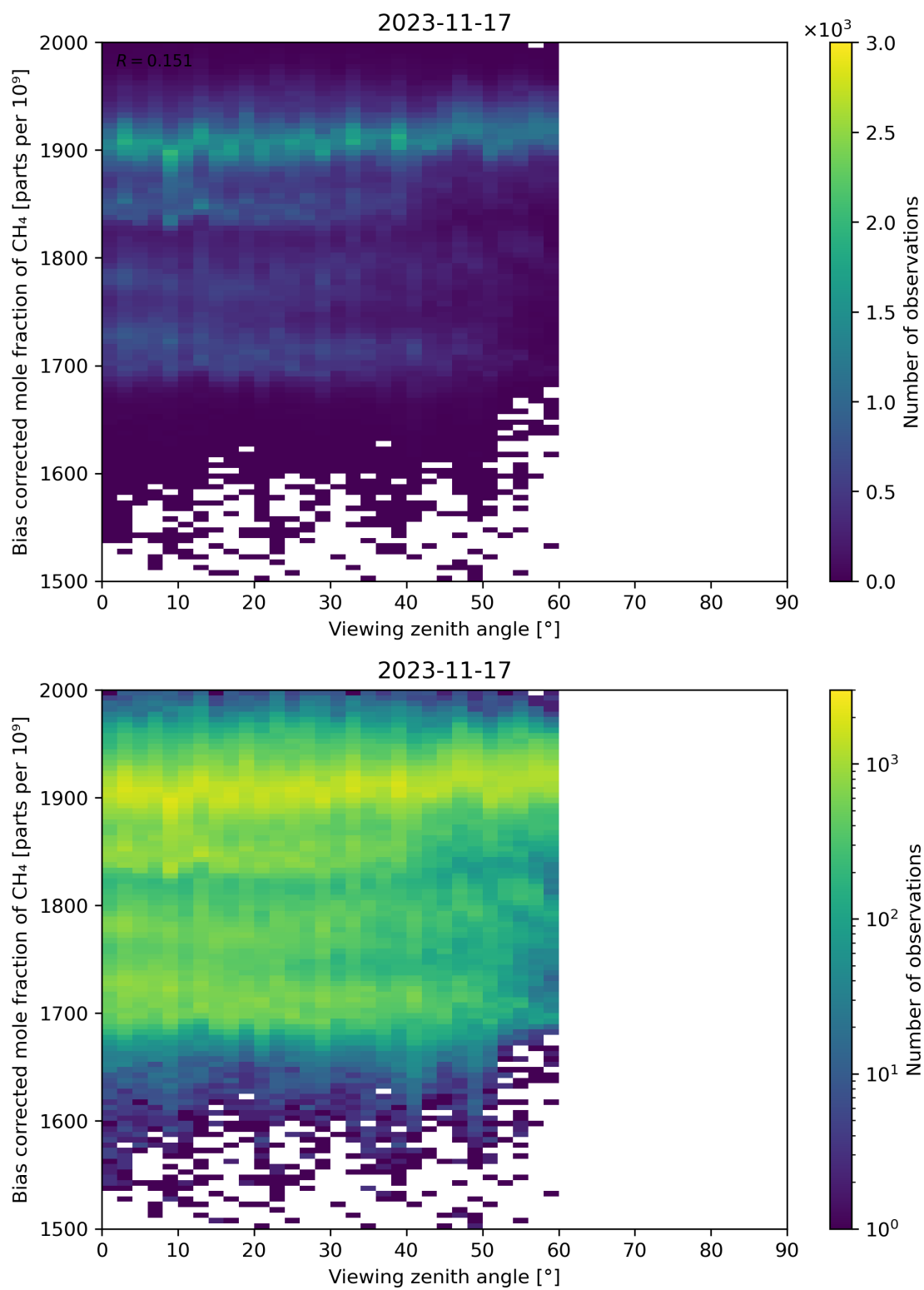
Figure 111: Scatter density plot of “Viewing zenith angle” against “Bias corrected mole fraction of CH 4 ” for 2023-11-16 to 2023-11-18.
