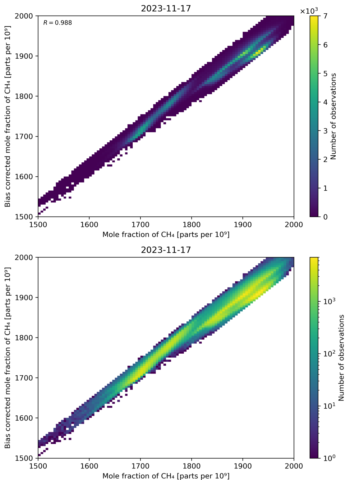
Figure 74: Scatter density plot of “Mole fraction of CH 4 ” against “Bias corrected mole fraction of CH 4 ” for 2023-11-16 to 2023-11-18.
