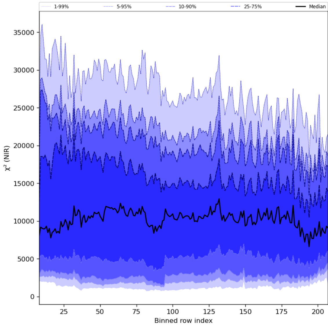
Figure 40: Along track statistics of " \chi^2 (NIR)" for 2023-11-16 to 2023-11-18
