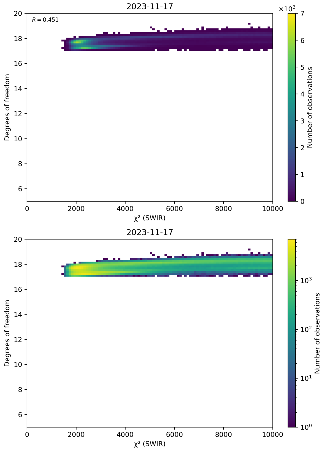
Figure 48: Scatter density plot of “ \chi^2 (SWIR)” against “Degrees of freedom” for 2023-11-16 to 2023-11-18.
