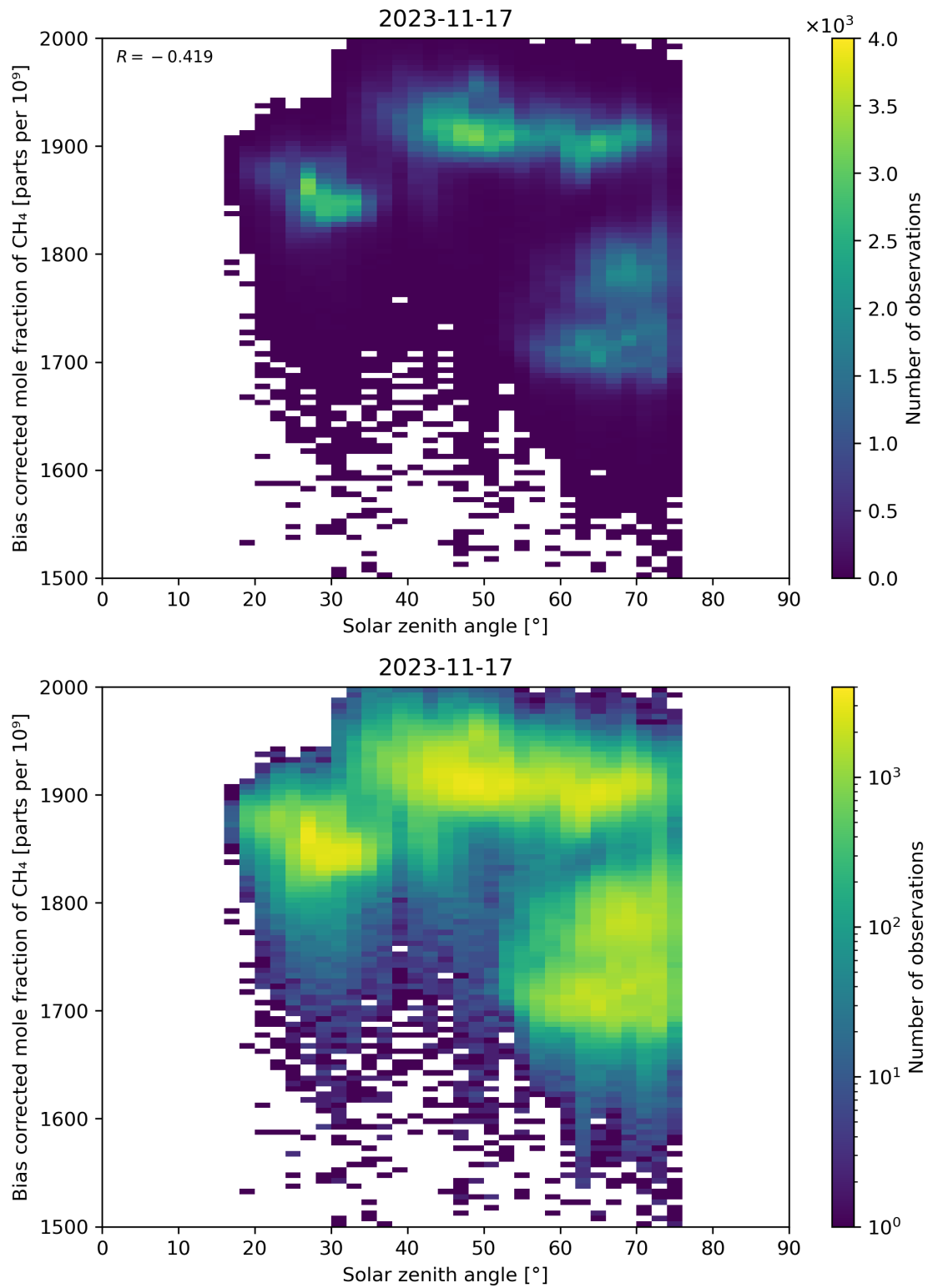
Figure 100: Scatter density plot of “Solar zenith angle” against “Bias corrected mole fraction of \text{CH}_4 ” for 2023-11-16 to 2023-11-18.
