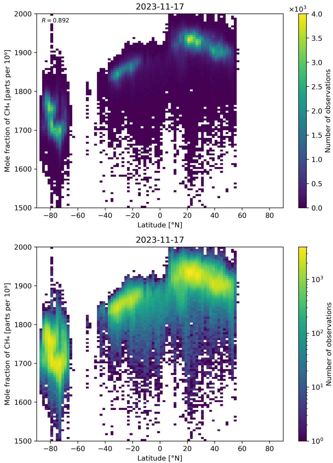
Figure 57: Scatter density plot of “Latitude” against “Mole fraction of CH 4 ” for 2023-11-16 to 2023-11-18.
