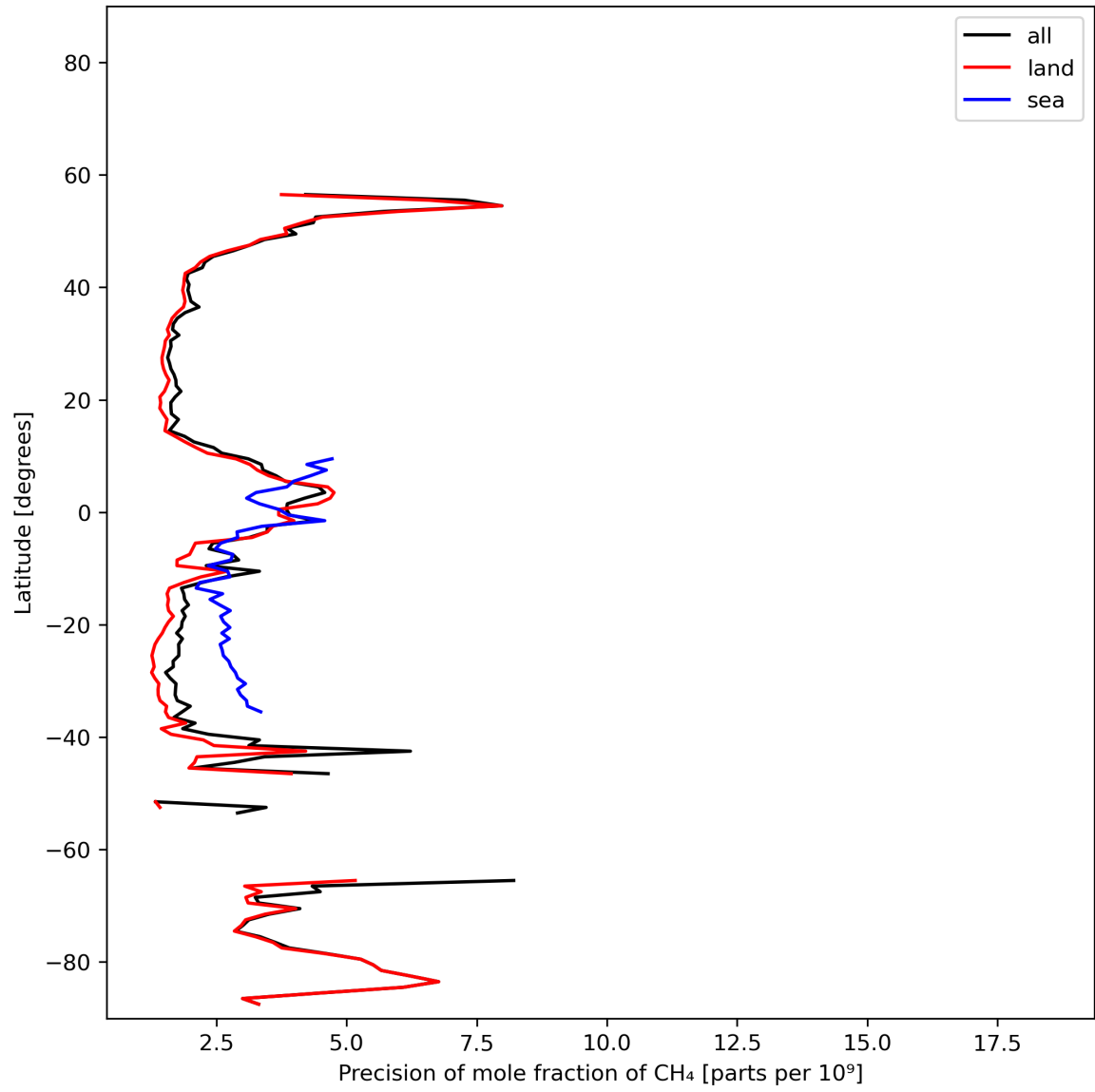
Figure 13: Zonal average of “Precision of mole fraction of CH 4 ” for 2023-11-16 to 2023-11-18.
