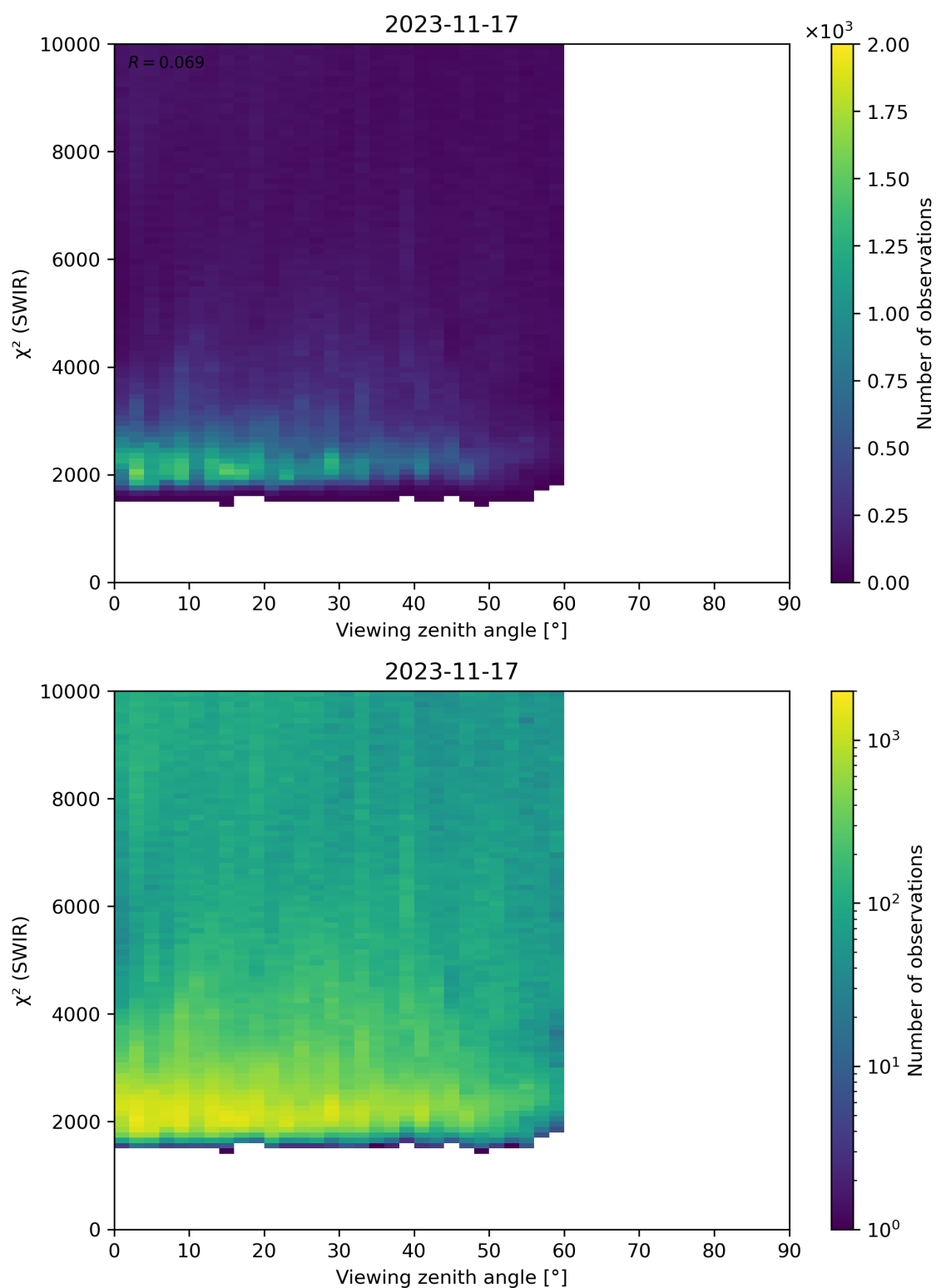
Figure 106: Scatter density plot of “Viewing zenith angle” against “ \chi^2 (SWIR)” for 2023-11-16 to 2023-11-18.
