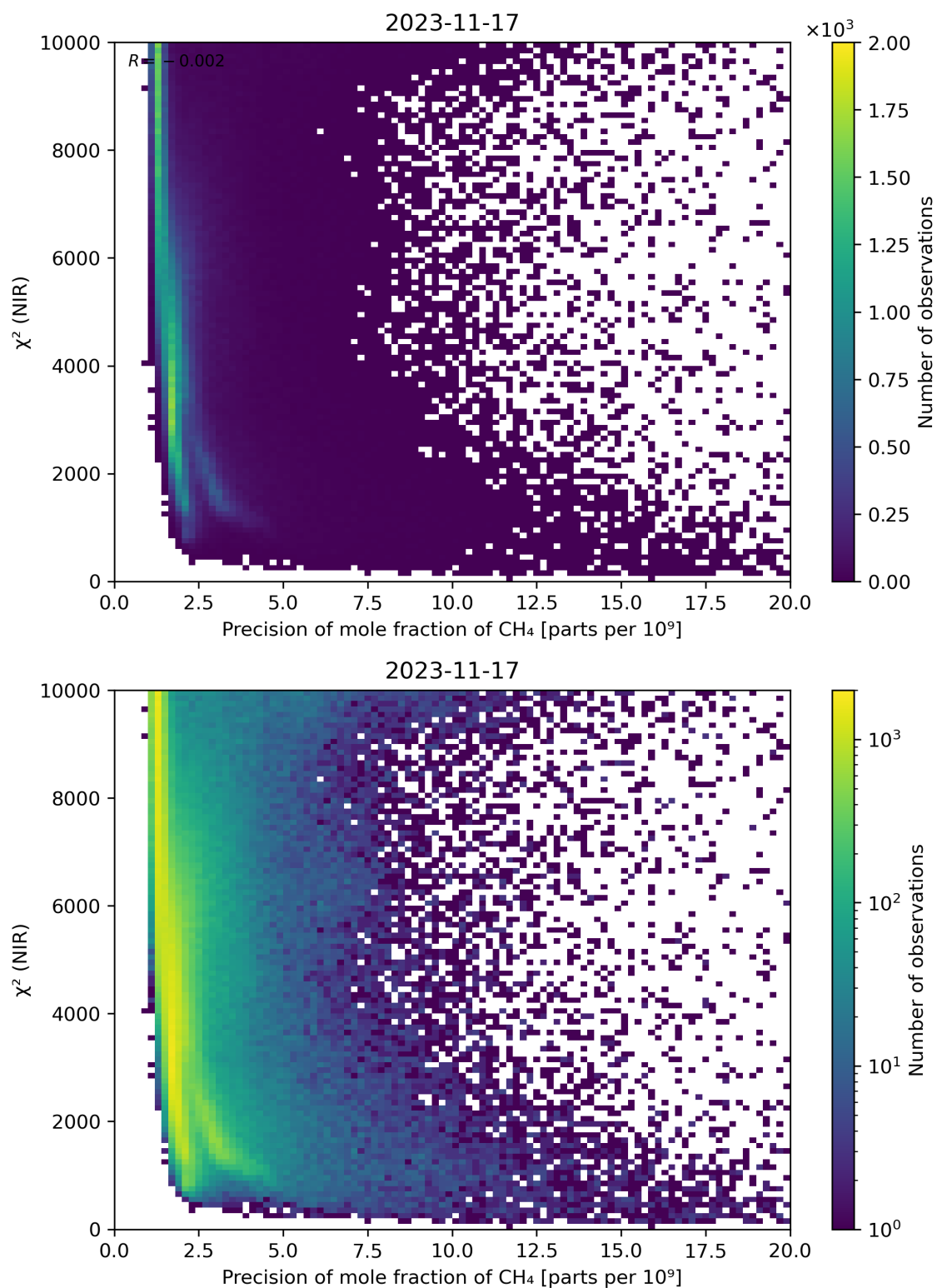
Figure 78: Scatter density plot of “Precision of mole fraction of CH 4 ” against “ \chi^2 (NIR)” for 2023-11-16 to 2023-11-18.
