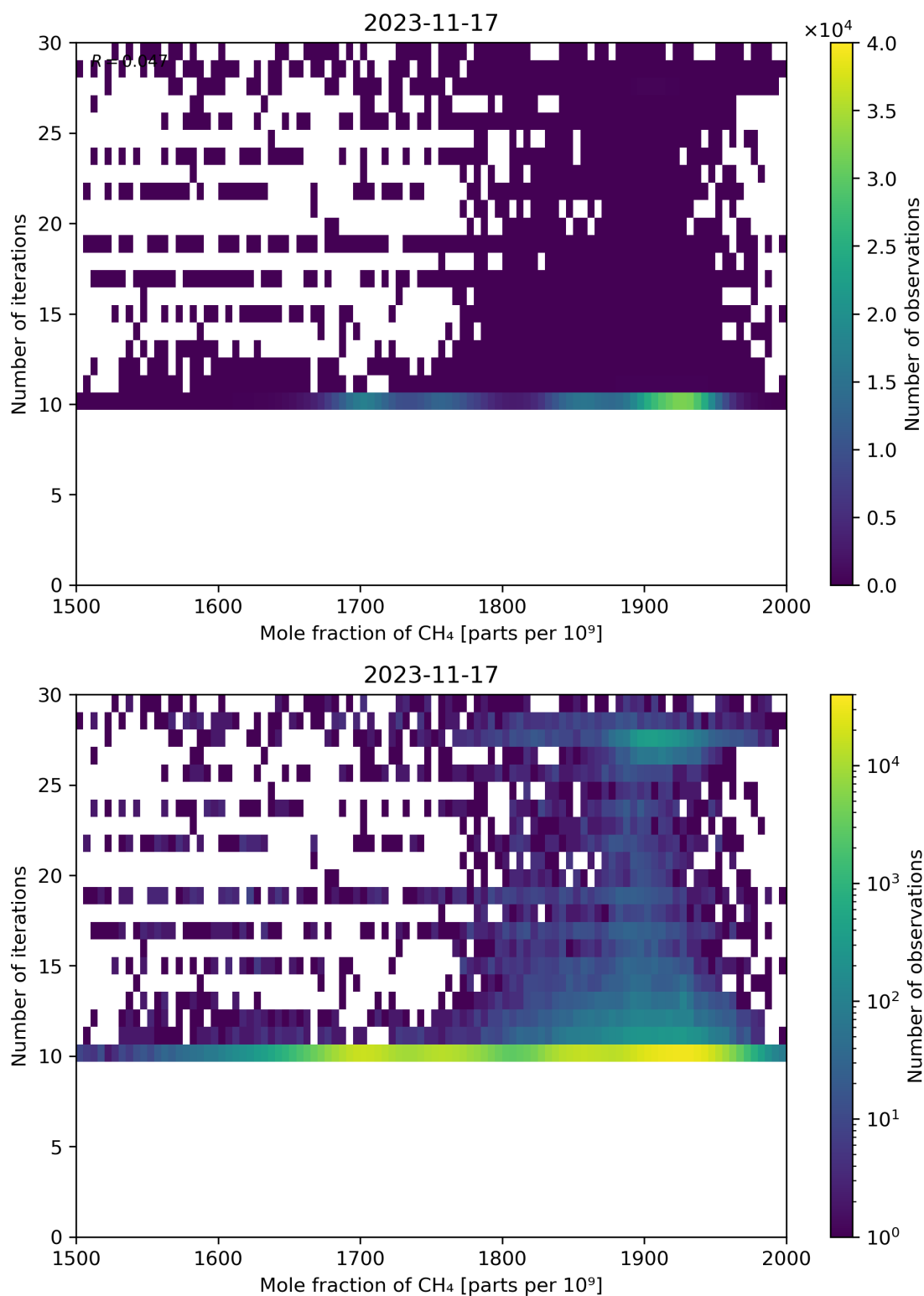
Figure 76: Scatter density plot of “Mole fraction of CH 4 ” against “Number of iterations” for 2023-11-16 to 2023-11-18.
