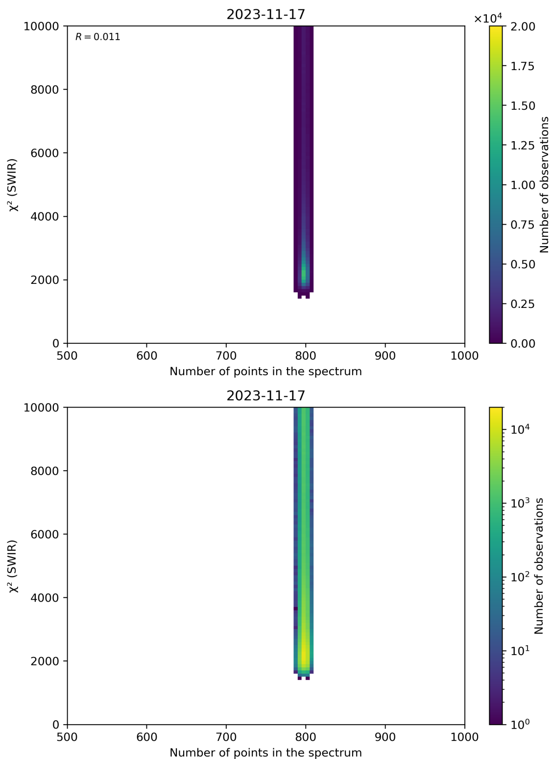
Figure 89: Scatter density plot of “Number of points in the spectrum” against “ \chi^2 (SWIR)” for 2023-11-16 to 2023-11-18.
