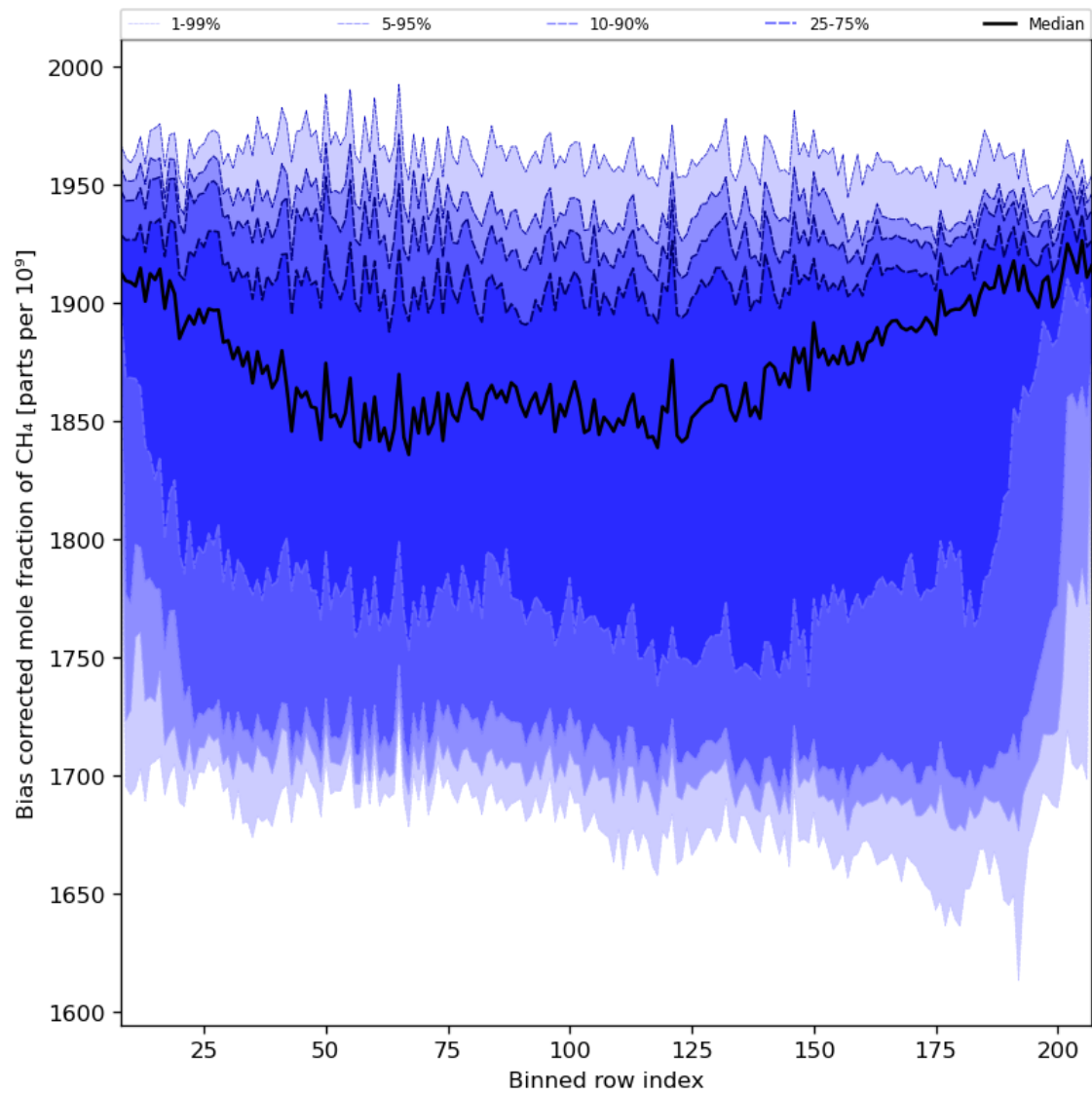
Figure 36: Along track statistics of “Bias corrected mole fraction of CH 4 ” for 2023-11-16 to 2023-11-18
