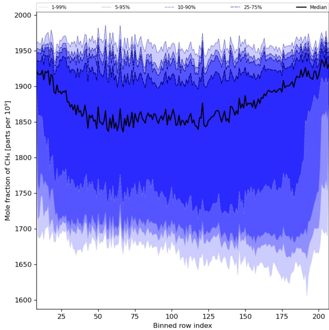
Figure 34: Along track statistics of “Mole fraction of CH 4 ” for 2023-11-16 to 2023-11-18
