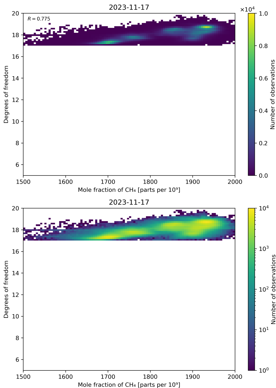
Figure 72: Scatter density plot of “Mole fraction of CH 4 ” against “Degrees of freedom” for 2023-11-16 to 2023-11-18.
