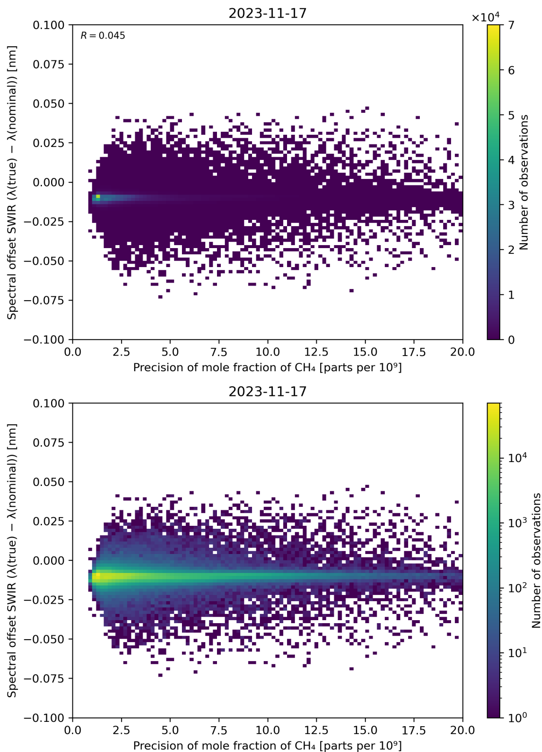
Figure 85: Scatter density plot of “Precision of mole fraction of CH 4 ” against “Spectral offset SWIR ( \lambda(\text{true}) - \lambda(\text{nominal}) )” for 2023-11-16 to 2023-11-18.
