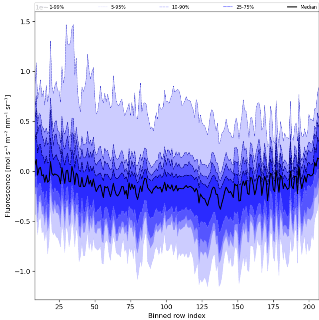
Figure 43: Along track statistics of “Fluorescence” for 2023-11-16 to 2023-11-18
