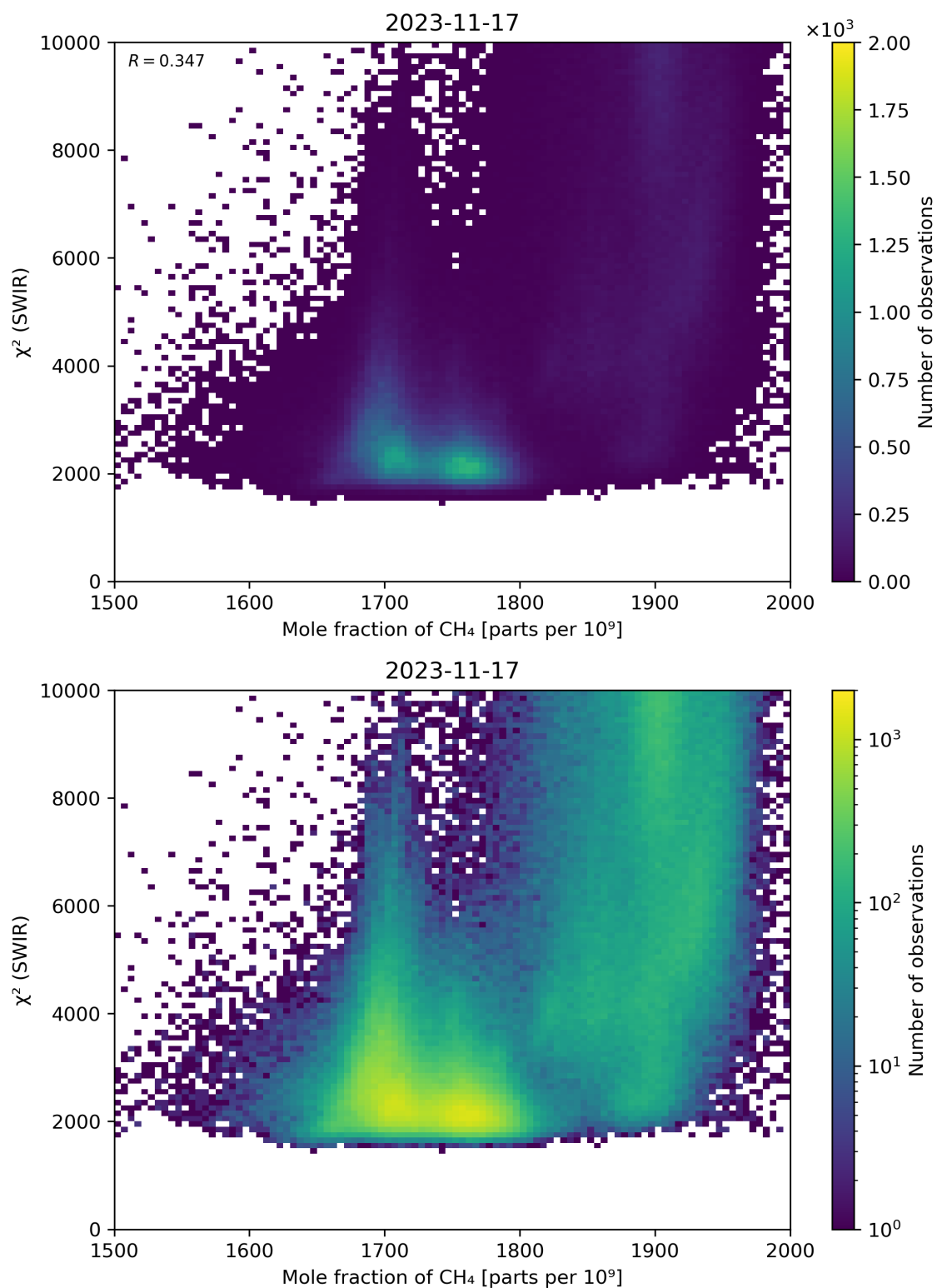
Figure 71: Scatter density plot of “Mole fraction of \text{CH}_4 ” against “ \chi^2 (SWIR)” for 2023-11-16 to 2023-11-18.
