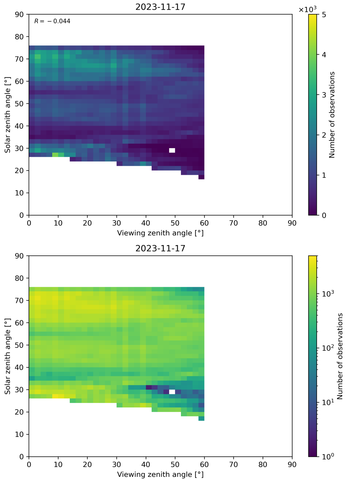
Figure 115: Scatter density plot of “Viewing zenith angle” against “Solar zenith angle” for 2023-11-16 to 2023-11-18.
