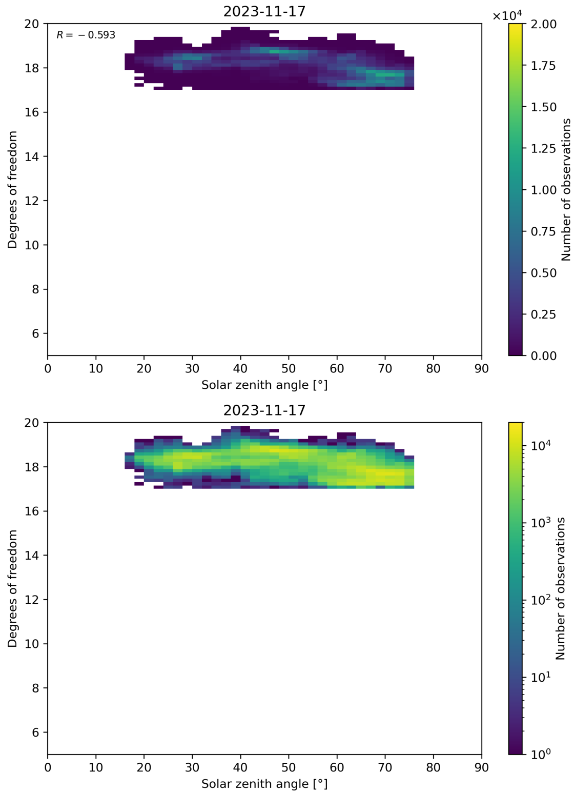
Figure 96: Scatter density plot of “Solar zenith angle” against “Degrees of freedom” for 2023-11-16 to 2023-11-18.
