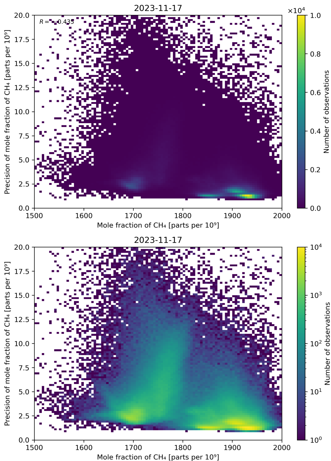
Figure 75: Scatter density plot of “Mole fraction of CH 4 ” against “Precision of mole fraction of CH 4 ” for 2023-11-16 to 2023-11-18.
