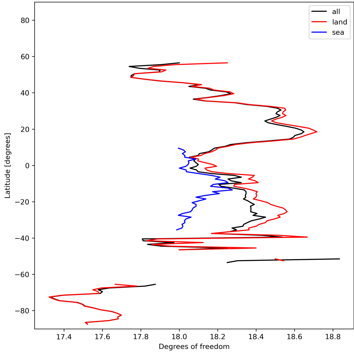
Figure 19: Zonal average of “Degrees of freedom” for 2023-11-16 to 2023-11-18.
