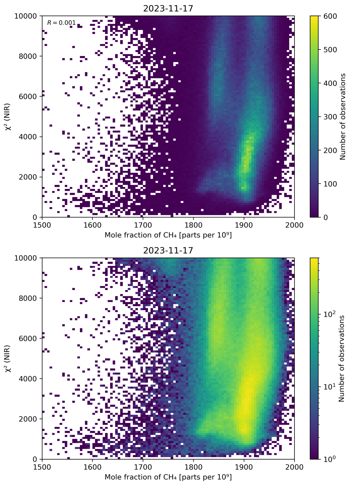
Figure 70: Scatter density plot of “Mole fraction of CH 4 ” against “ \chi^2 (NIR)” for 2023-11-16 to 2023-11-18.
