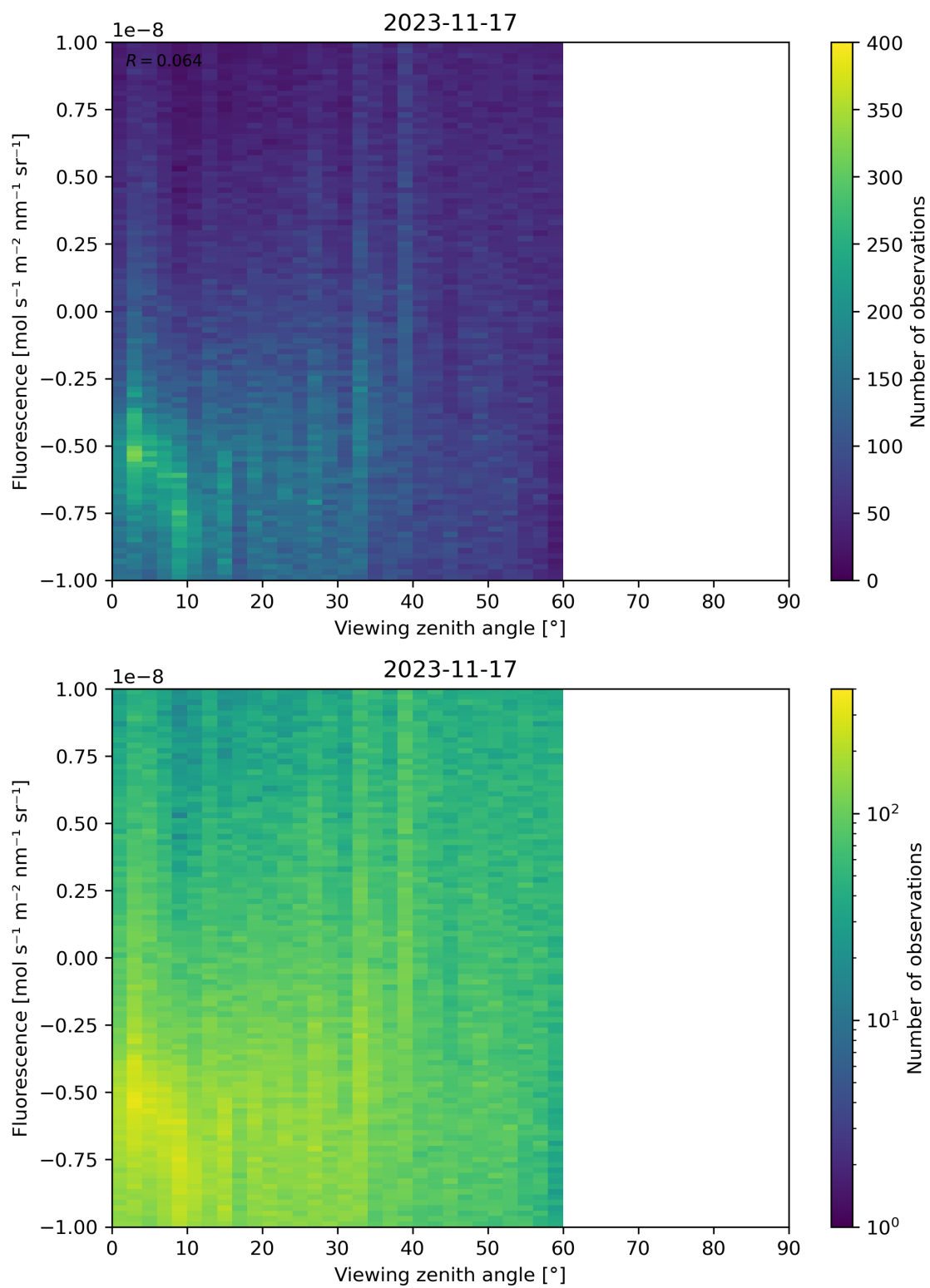
Figure 108: Scatter density plot of “Viewing zenith angle” against “Fluorescence” for 2023-11-16 to 2023-11-18.
