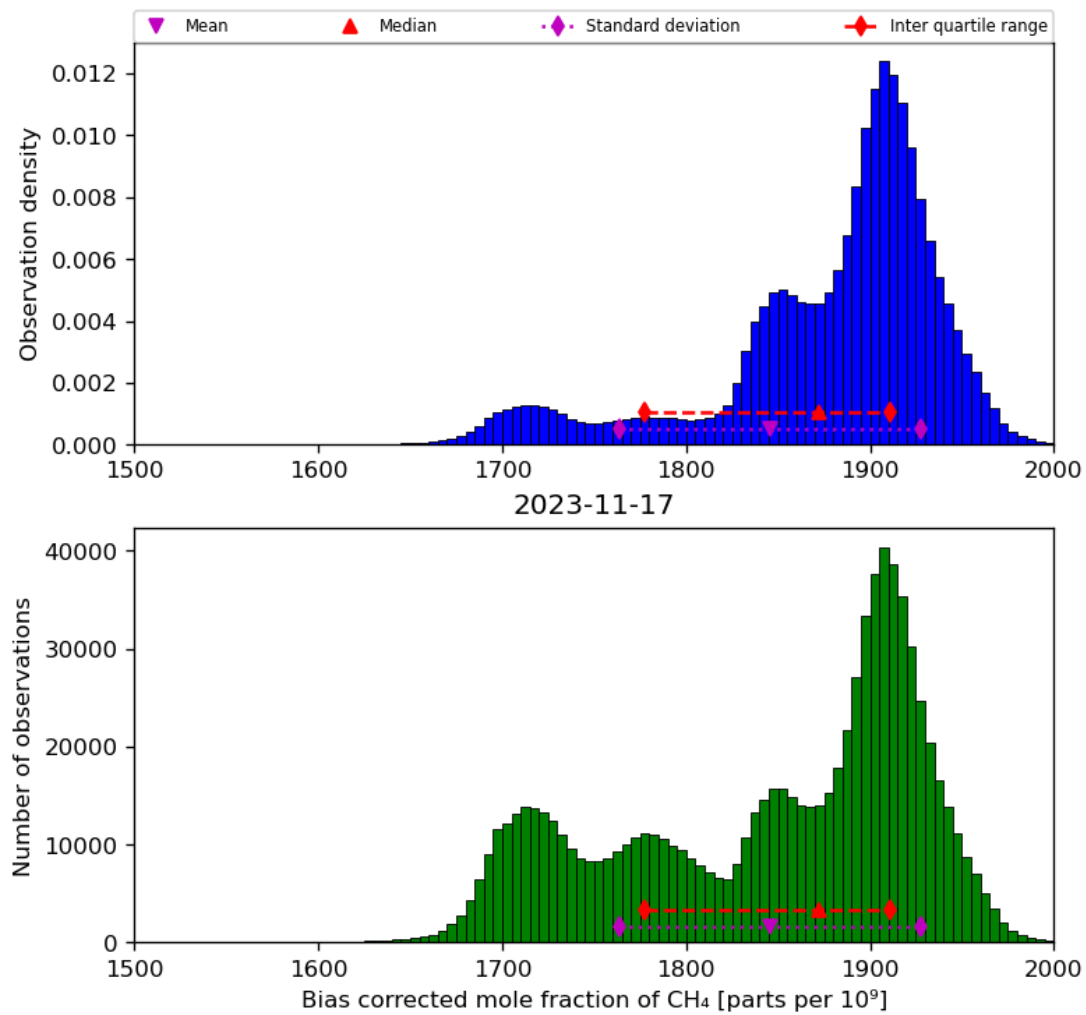
Figure 25: Histogram of “Bias corrected mole fraction of CH 4 ” for 2023-11-16 to 2023-11-18
