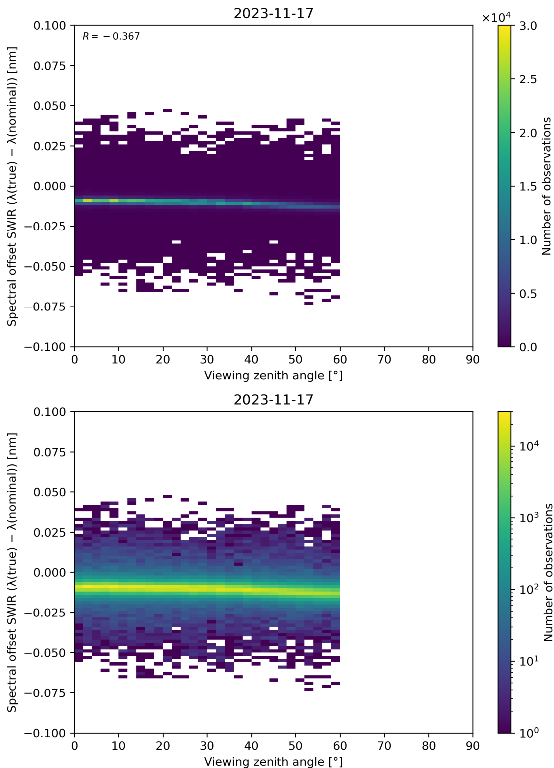
Figure 116: Scatter density plot of “Viewing zenith angle” against “Spectral offset SWIR ( \lambda(\text{true}) - \lambda(\text{nominal}) )” for 2023-11-16 to 2023-11-18.
