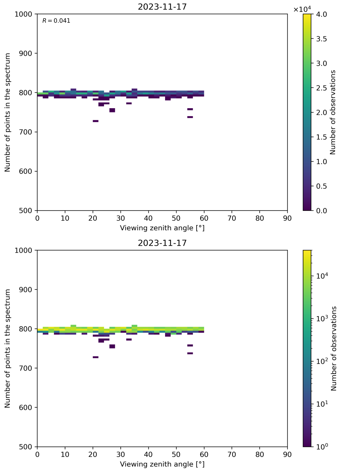
Figure 114: Scatter density plot of “Viewing zenith angle” against “Number of points in the spectrum” for 2023-11-16 to 2023-11-18.
