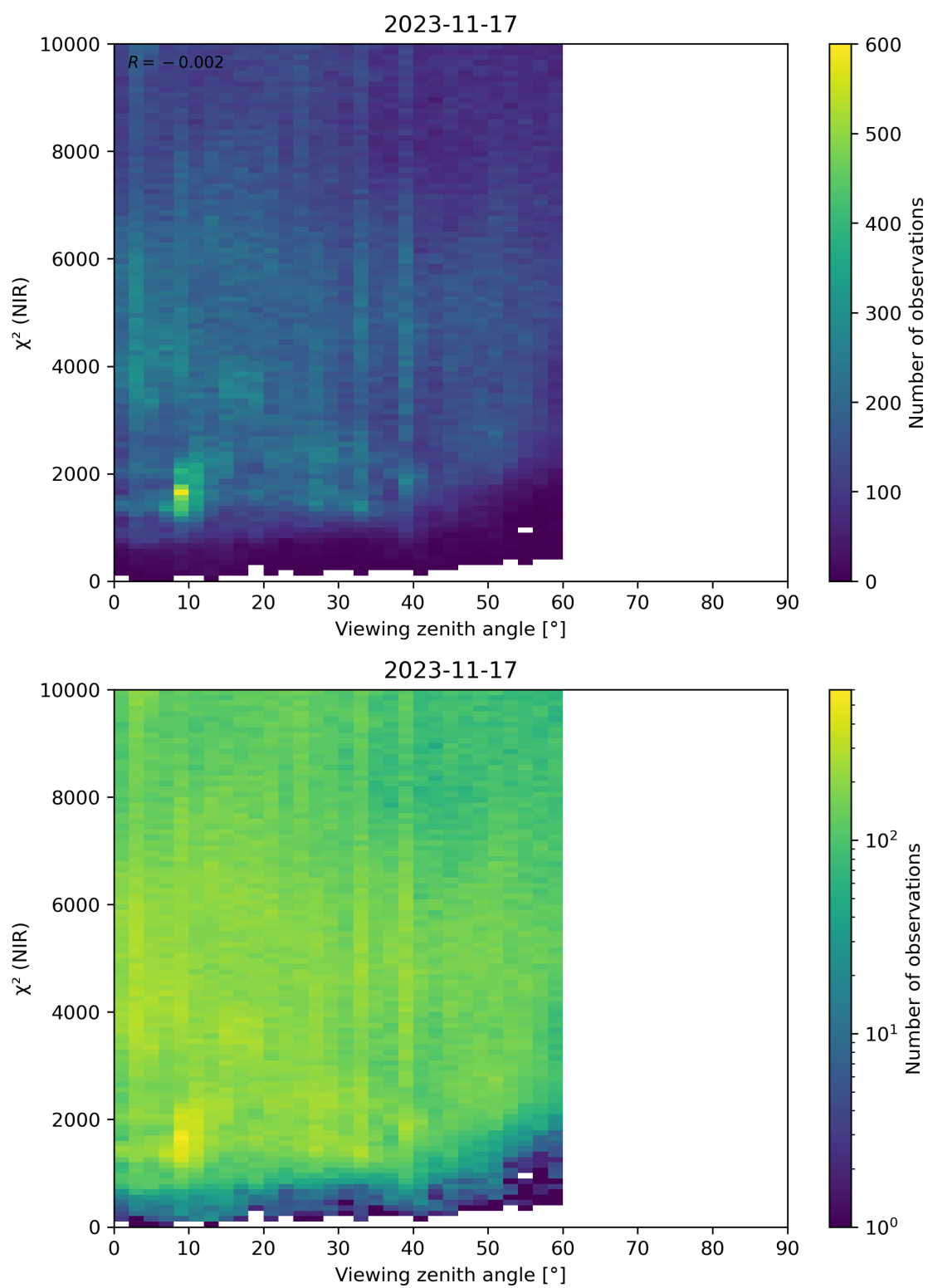
Figure 105: Scatter density plot of “Viewing zenith angle” against “ \chi^2 (NIR)” for 2023-11-16 to 2023-11-18.
