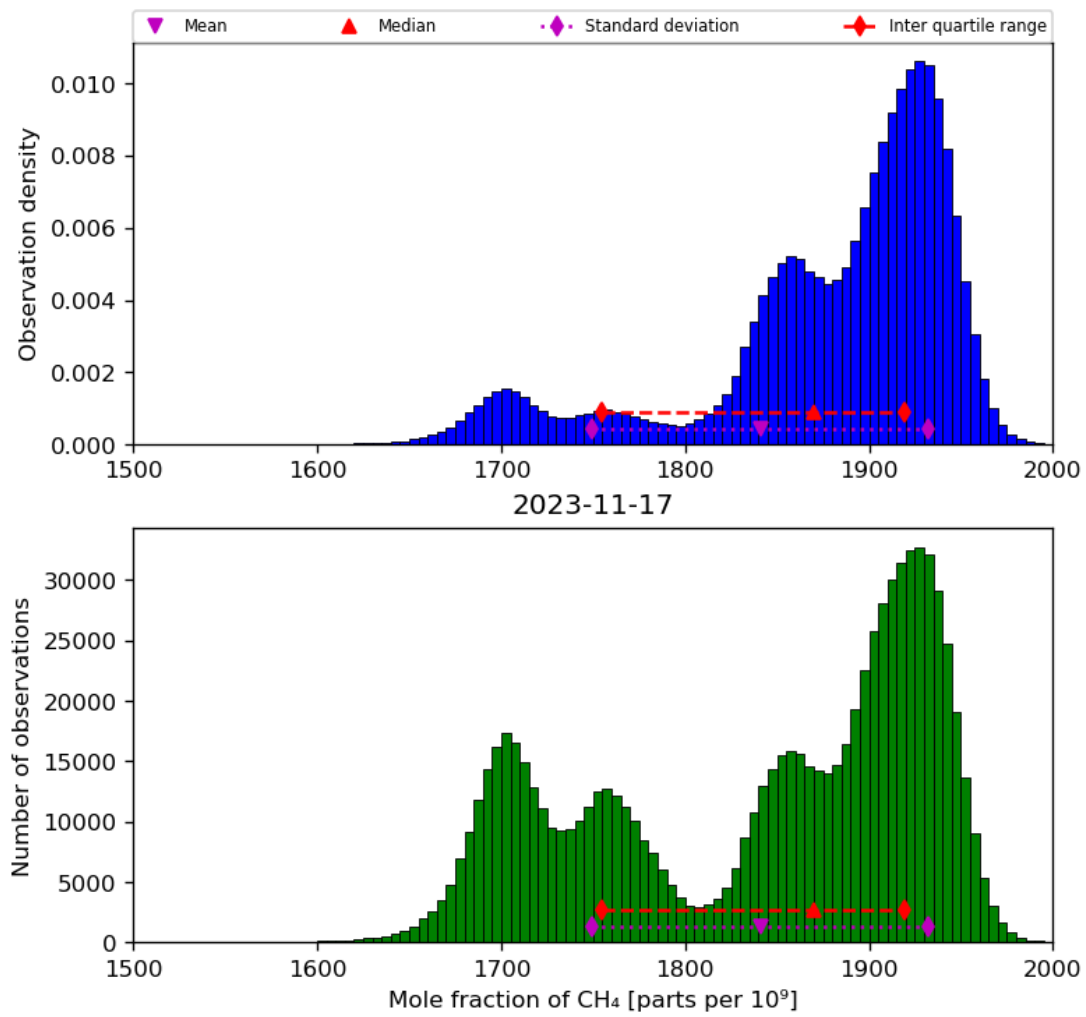
Figure 23: Histogram of “Mole fraction of CH 4 ” for 2023-11-16 to 2023-11-18
