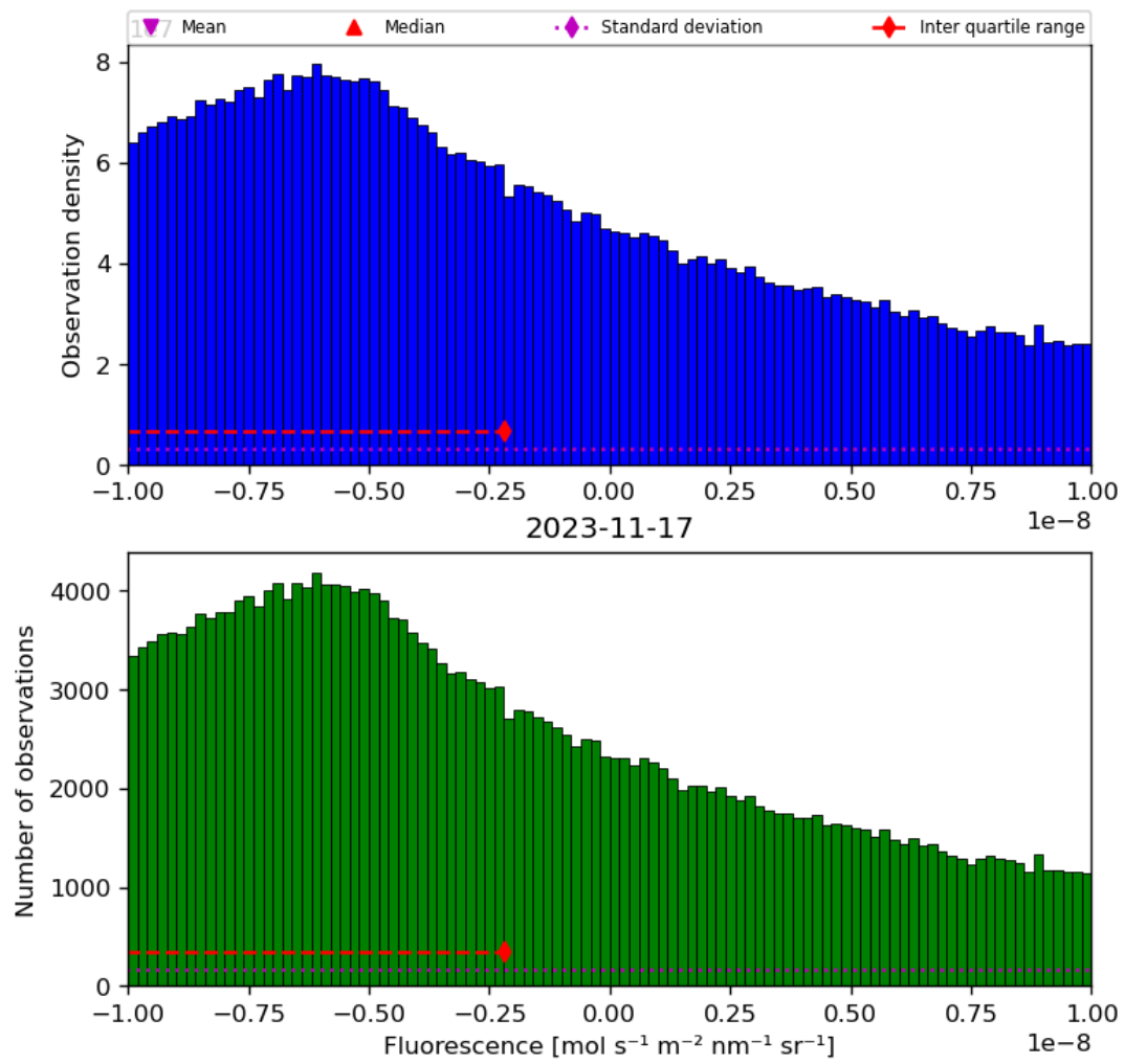
Figure 32: Histogram of “Fluorescence” for 2023-11-16 to 2023-11-18
