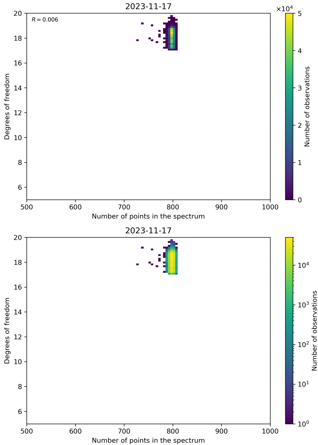
Figure 90: Scatter density plot of “Number of points in the spectrum” against “Degrees of freedom” for 2023-11-16 to 2023-11-18.
