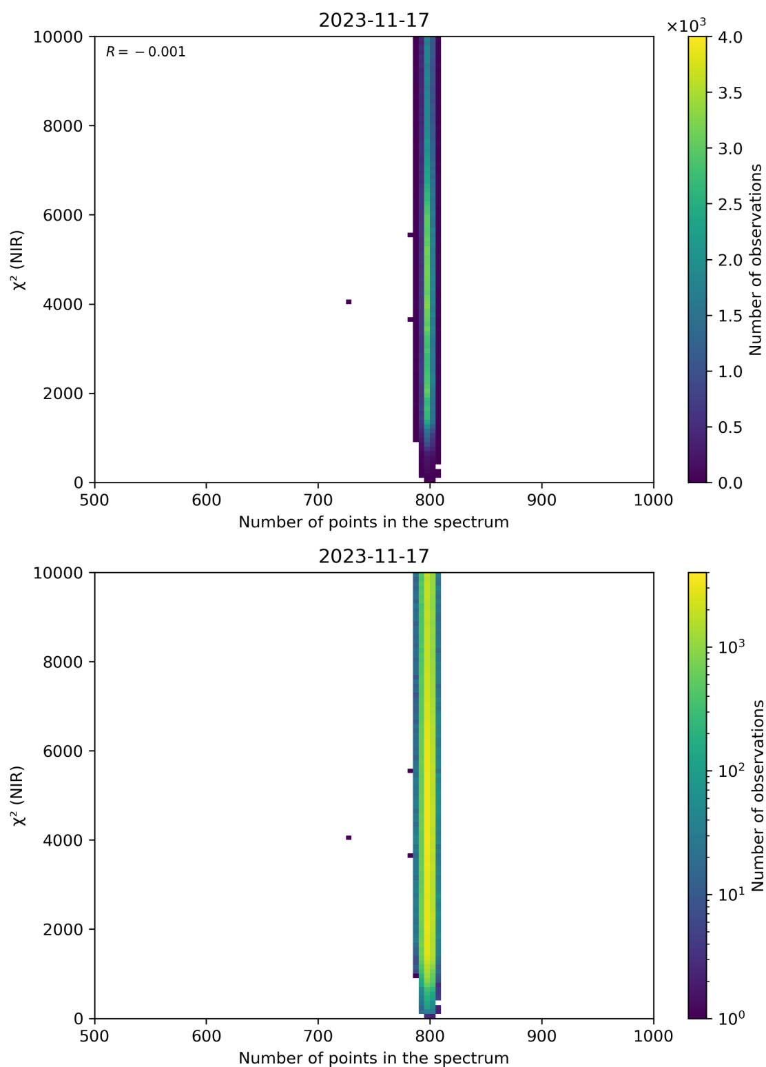
Figure 88: Scatter density plot of “Number of points in the spectrum” against “ \chi^2 (NIR)” for 2023-11-16 to 2023-11-18.
