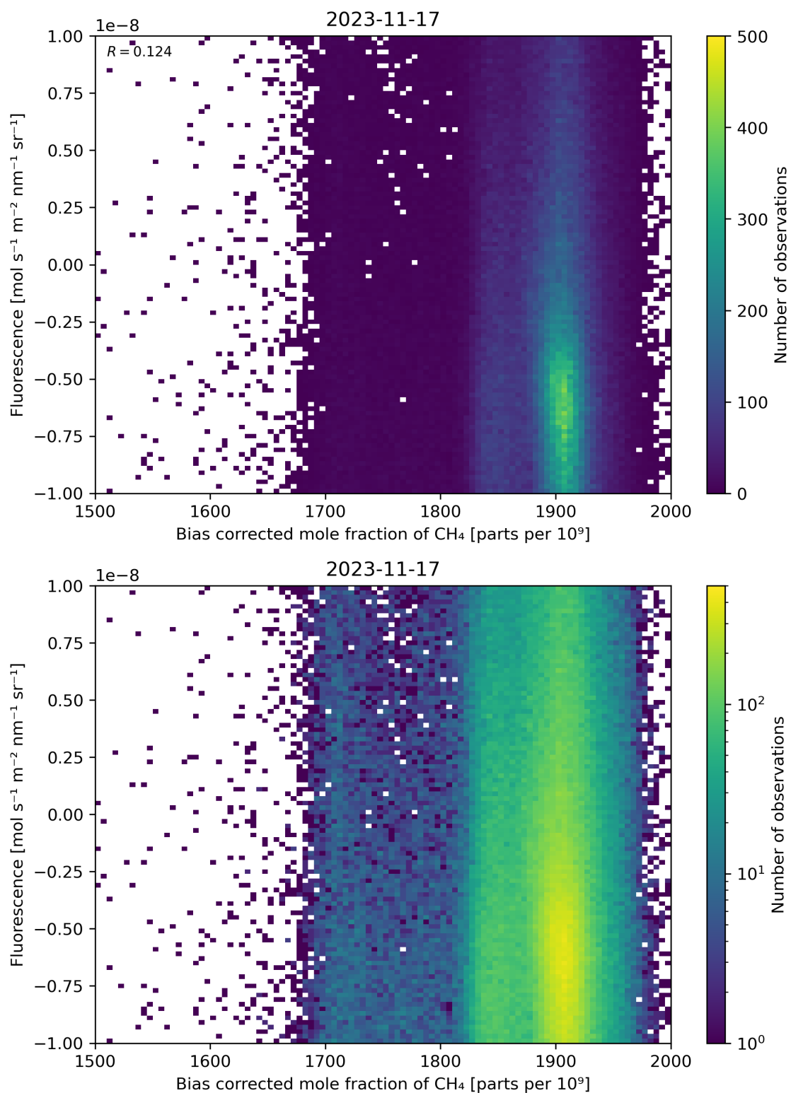
Figure 66: Scatter density plot of “Bias corrected mole fraction of \text{CH}_4 ” against “Fluorescence” for 2023-11-16 to 2023-11-18.
