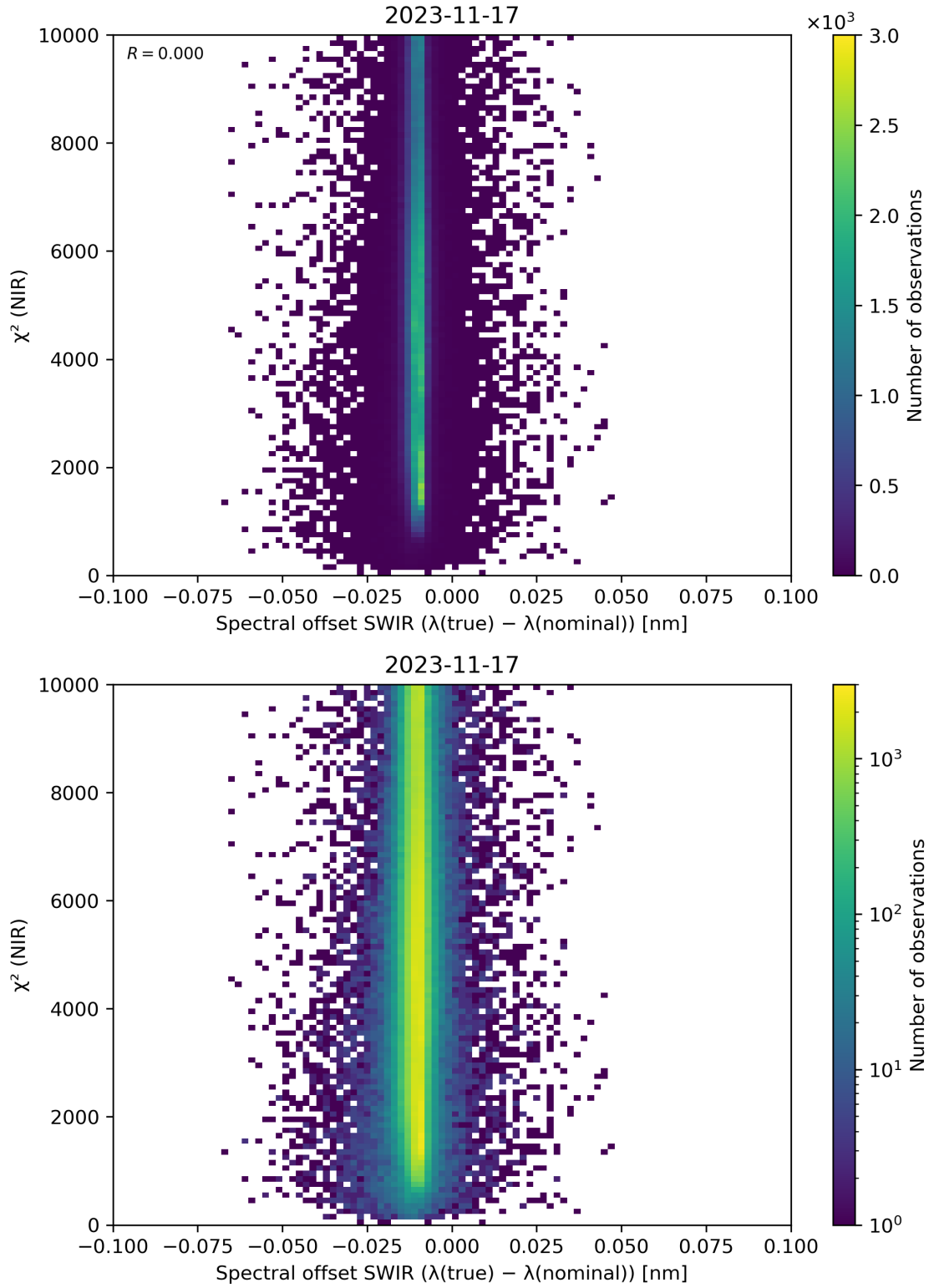
Figure 117: Scatter density plot of “Spectral offset SWIR ( \lambda(\text{true}) - \lambda(\text{nominal}) )” against “ \chi^2 (NIR)” for 2023-11-16 to 2023-11-18.
