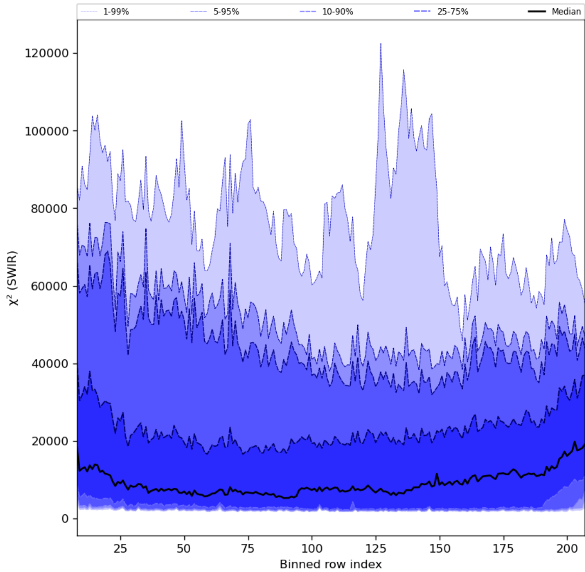
Figure 39: Along track statistics of " \chi^2 (SWIR)" for 2023-11-16 to 2023-11-18
