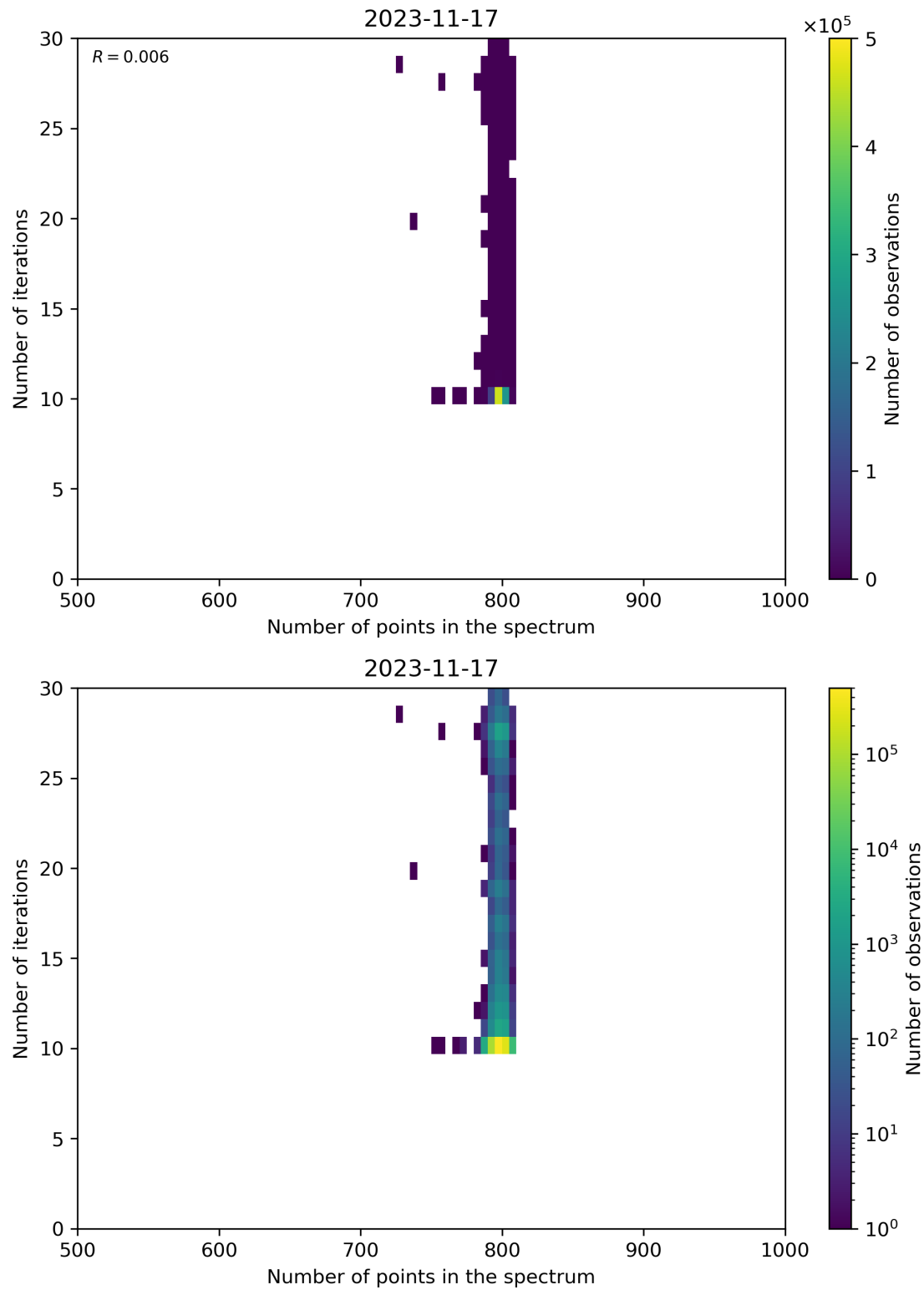
Figure 92: Scatter density plot of “Number of points in the spectrum” against “Number of iterations” for 2023-11-16 to 2023-11-18.
