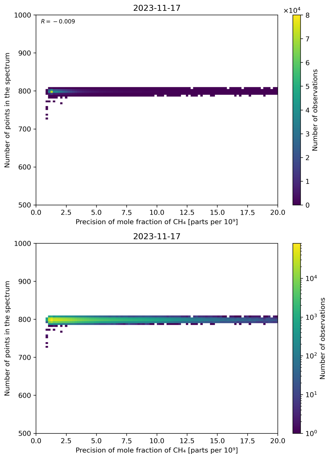
Figure 84: Scatter density plot of “Precision of mole fraction of CH 4 ” against “Number of points in the spectrum” for 2023-11-16 to 2023-11-18.
