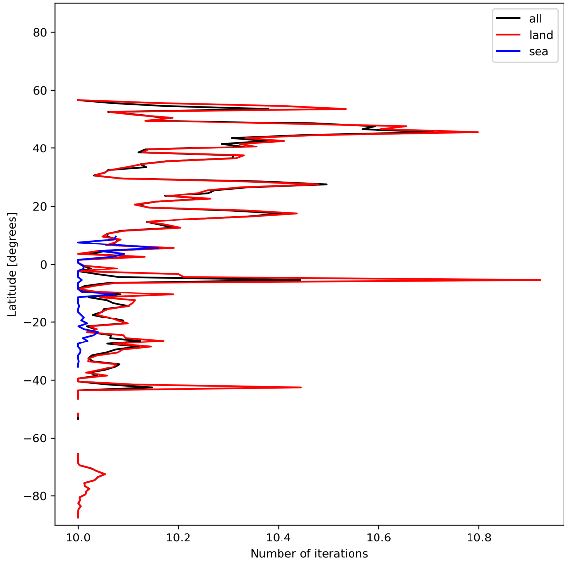
Figure 20: Zonal average of “Number of iterations” for 2023-11-16 to 2023-11-18.
