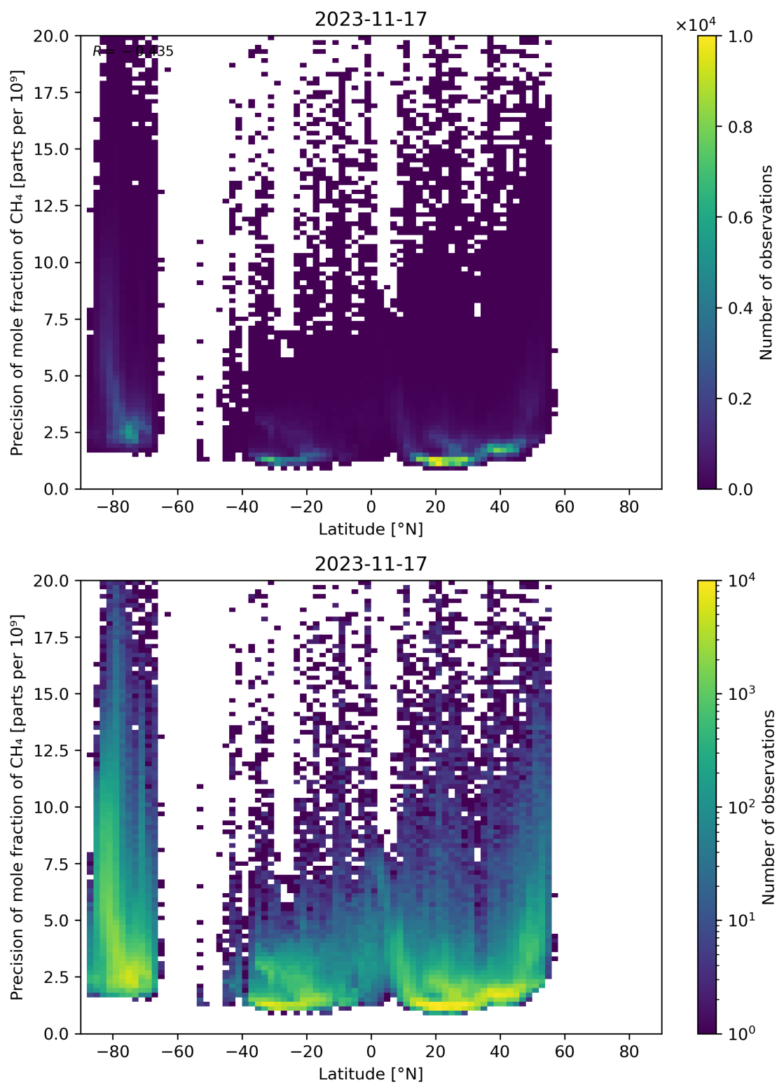
Figure 59: Scatter density plot of “Latitude” against “Precision of mole fraction of CH 4 ” for 2023-11-16 to 2023-11-18.
