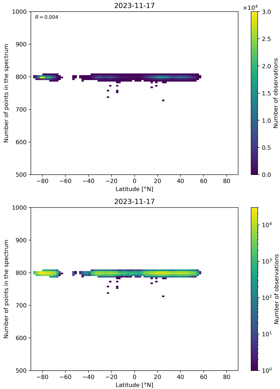
Figure 61: Scatter density plot of “Latitude” against “Number of points in the spectrum” for 2023-11-16 to 2023-11-18.
