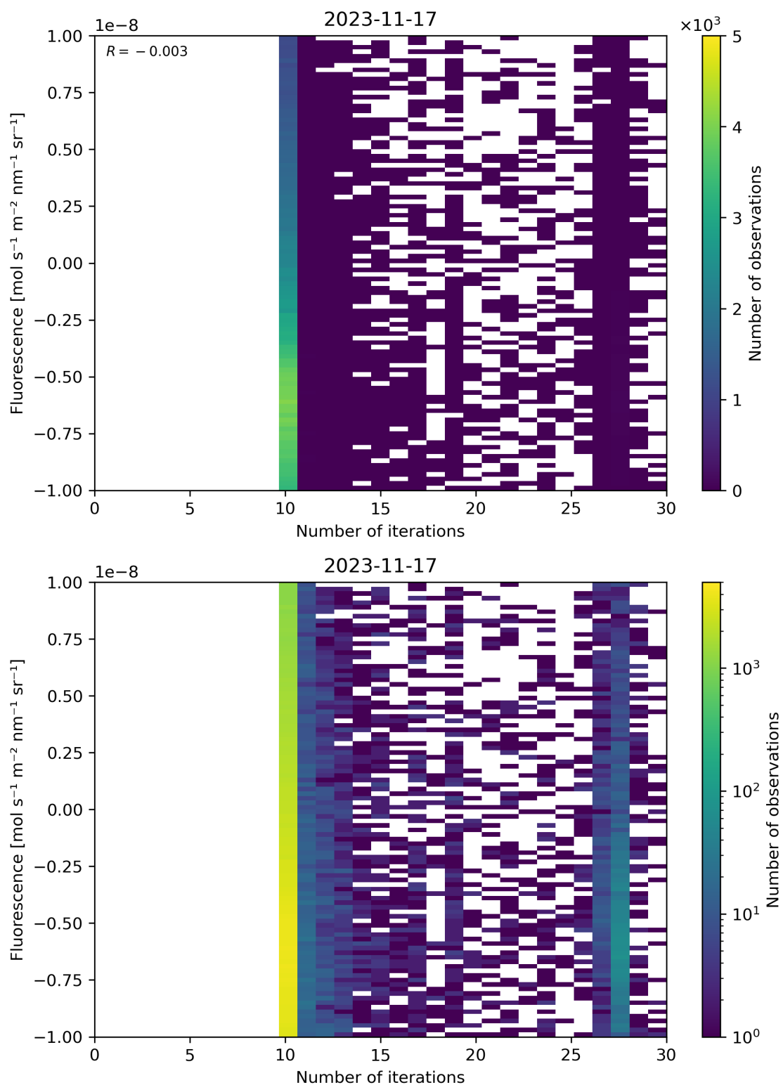
Figure 87: Scatter density plot of “Number of iterations” against “Fluorescence” for 2023-11-16 to 2023-11-18.
