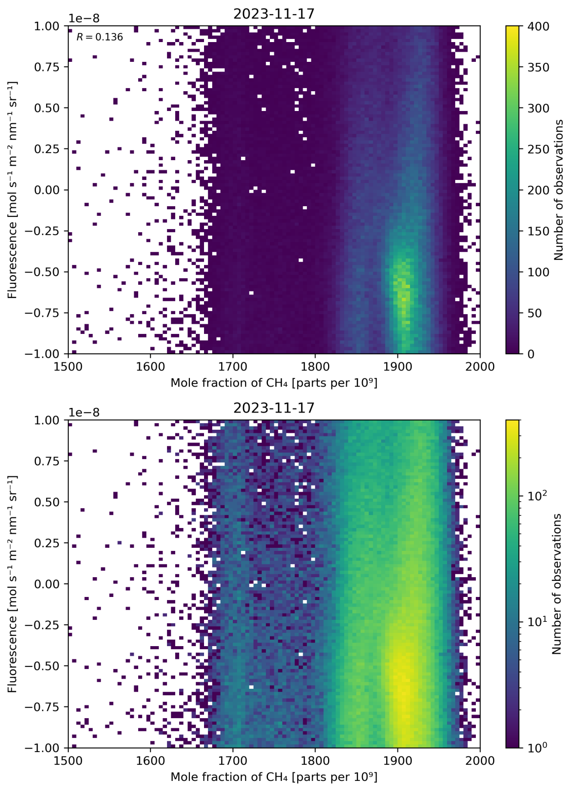
Figure 73: Scatter density plot of “Mole fraction of \text{CH}_4 ” against “Fluorescence” for 2023-11-16 to 2023-11-18.
