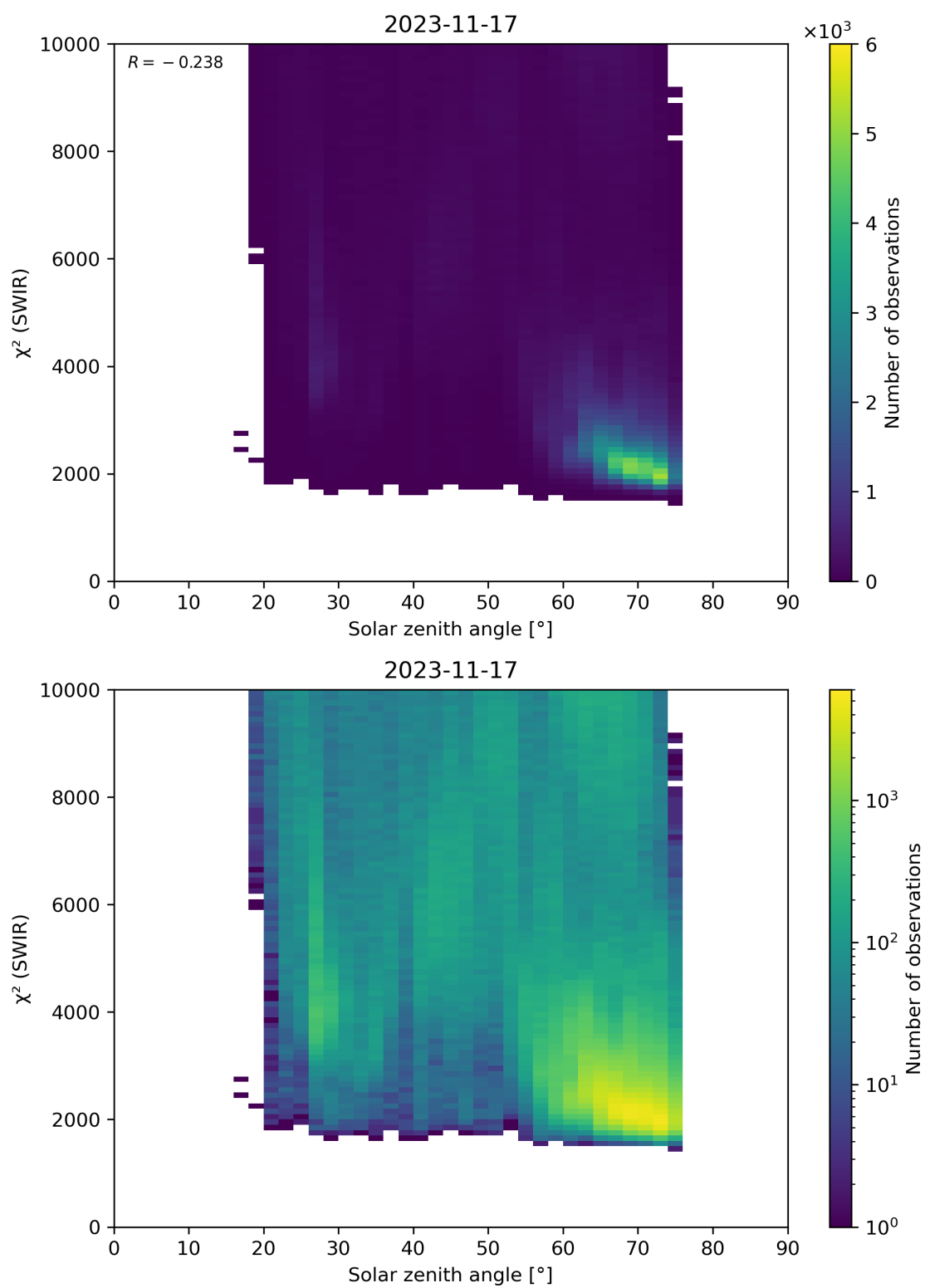
Figure 95: Scatter density plot of “Solar zenith angle” against “ \chi^2 (SWIR)” for 2023-11-16 to 2023-11-18.
