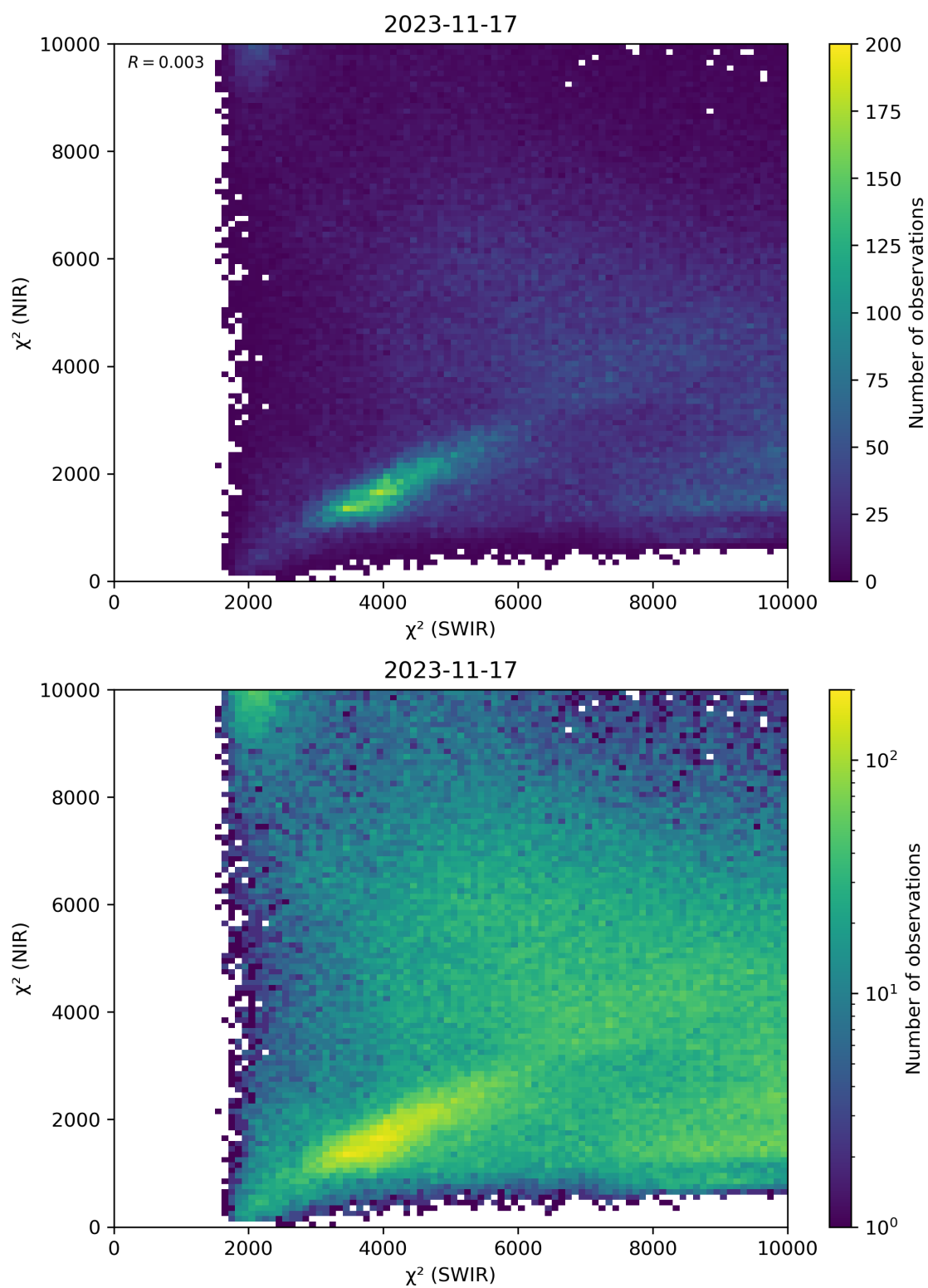
Figure 47: Scatter density plot of “ \chi^2 (SWIR)” against “ \chi^2 (NIR)” for 2023-11-16 to 2023-11-18.
