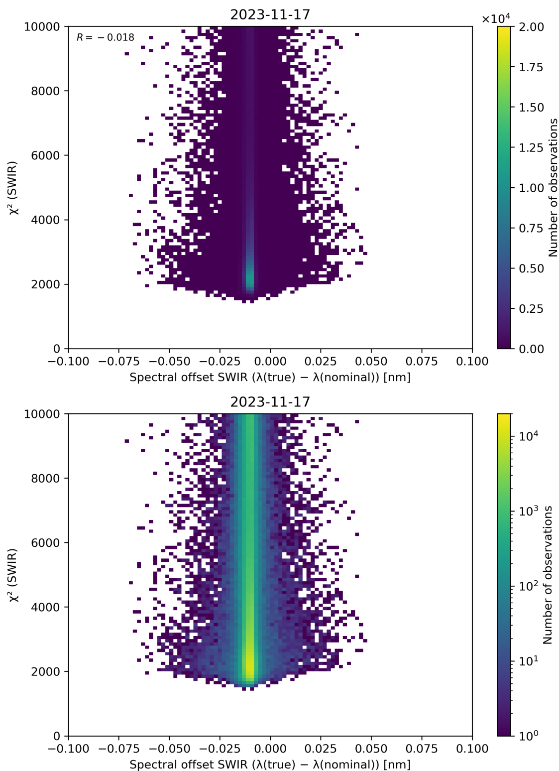
Figure 118: Scatter density plot of “Spectral offset SWIR ( \lambda(\text{true}) - \lambda(\text{nominal}) )” against “ \chi^2 (SWIR)” for 2023-11-16 to 2023-11-18.
