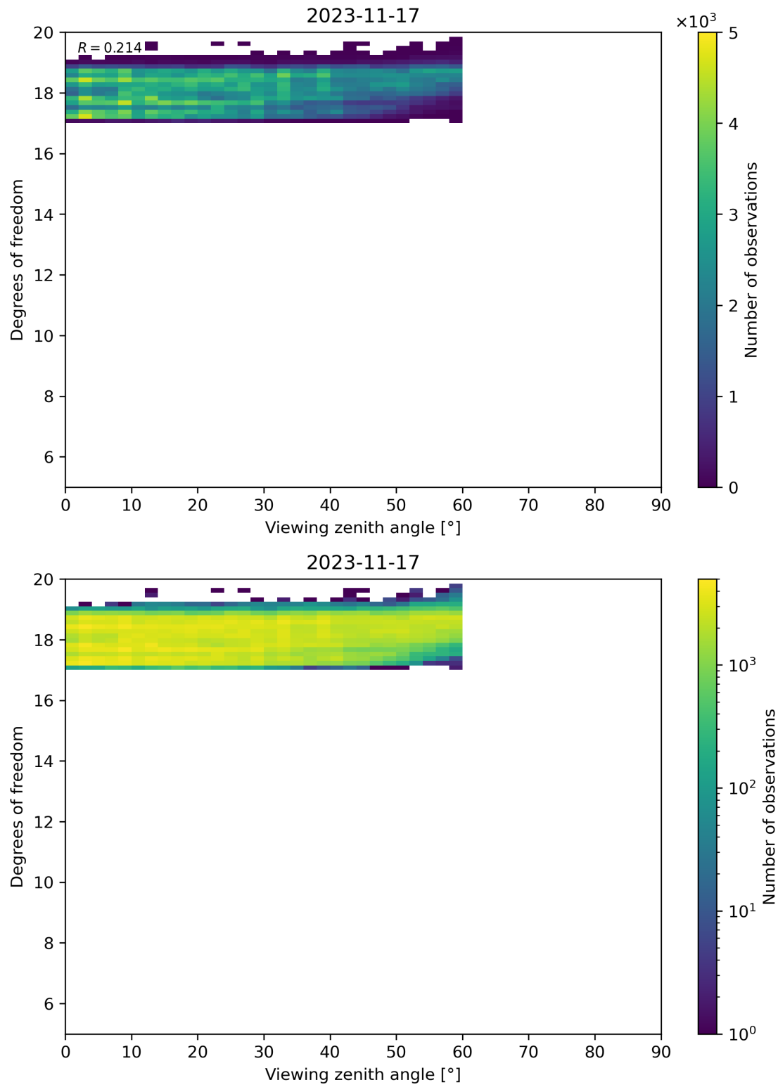
Figure 107: Scatter density plot of “Viewing zenith angle” against “Degrees of freedom” for 2023-11-16 to 2023-11-18.
