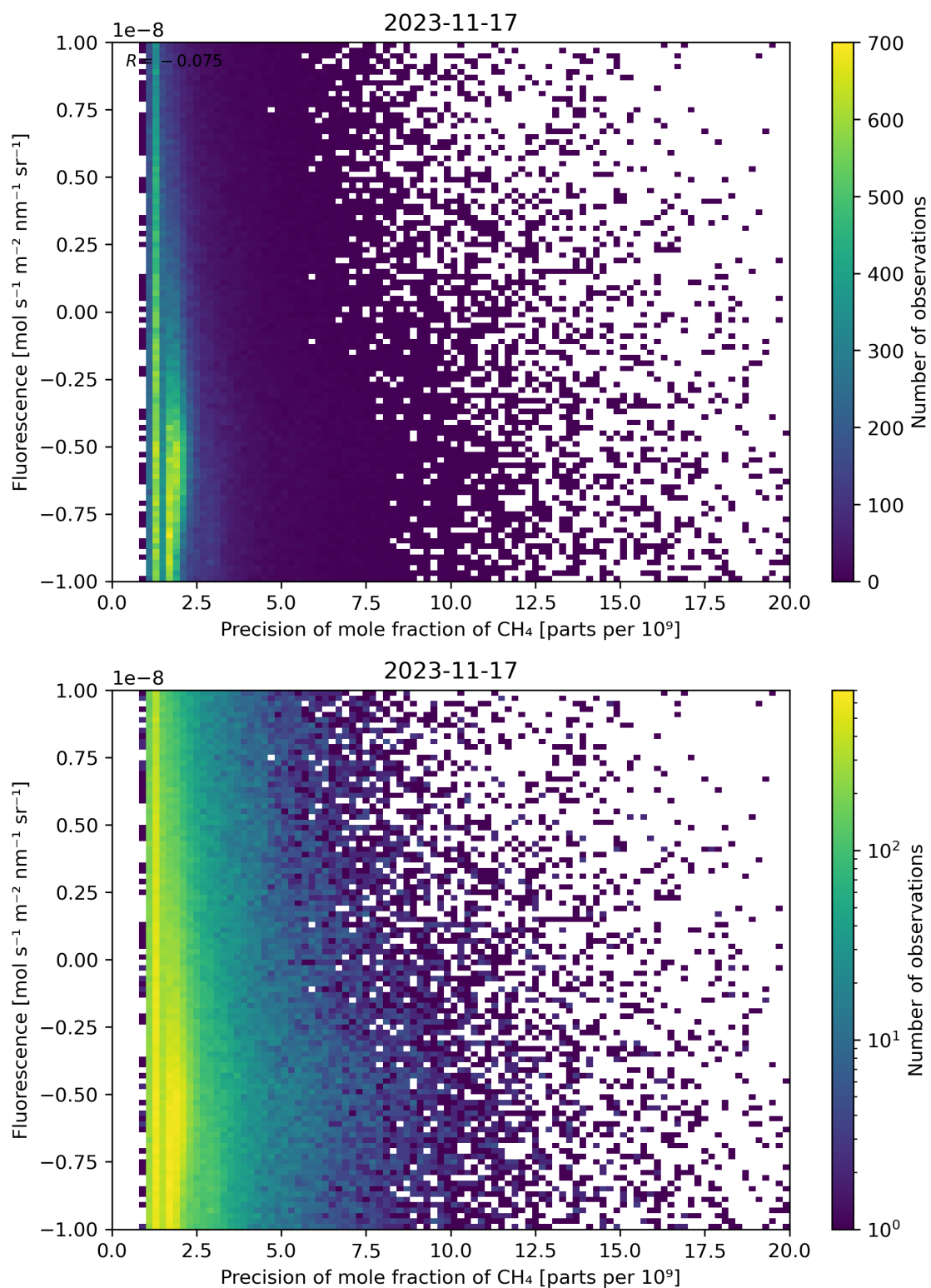
Figure 81: Scatter density plot of “Precision of mole fraction of \text{CH}_4 ” against “Fluorescence” for 2023-11-16 to 2023-11-18.
