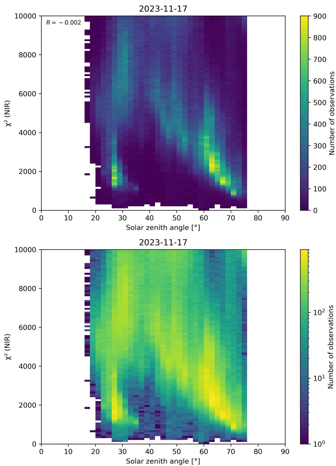
Figure 94: Scatter density plot of “Solar zenith angle” against “ \chi^2 (NIR)” for 2023-11-16 to 2023-11-18.
