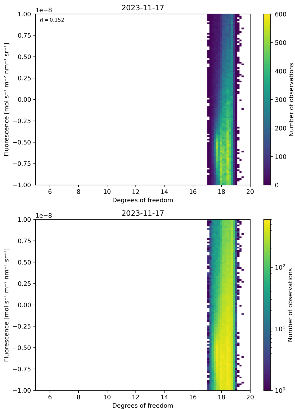
Figure 51: Scatter density plot of “Degrees of freedom” against “Fluorescence” for 2023-11-16 to 2023-11-18.
