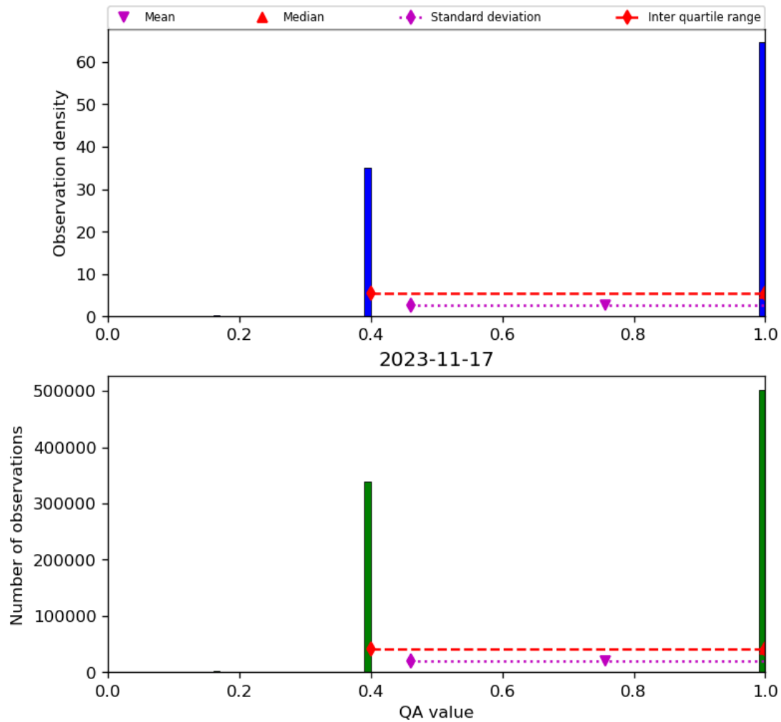
Figure 22: Histogram of “QA value” for 2023-11-16 to 2023-11-18
