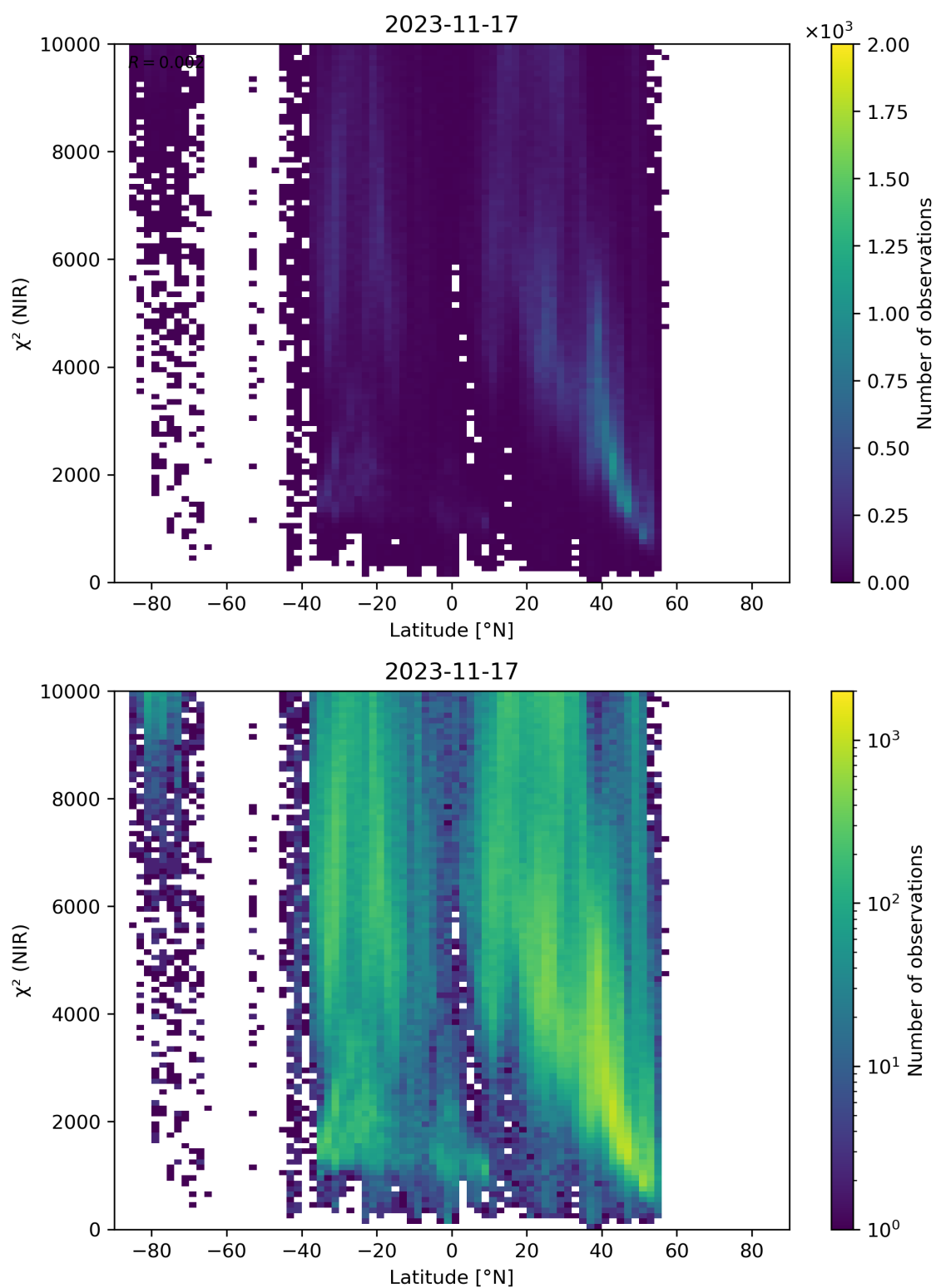
Figure 53: Scatter density plot of “Latitude” against “ \chi^2 (NIR)” for 2023-11-16 to 2023-11-18.
