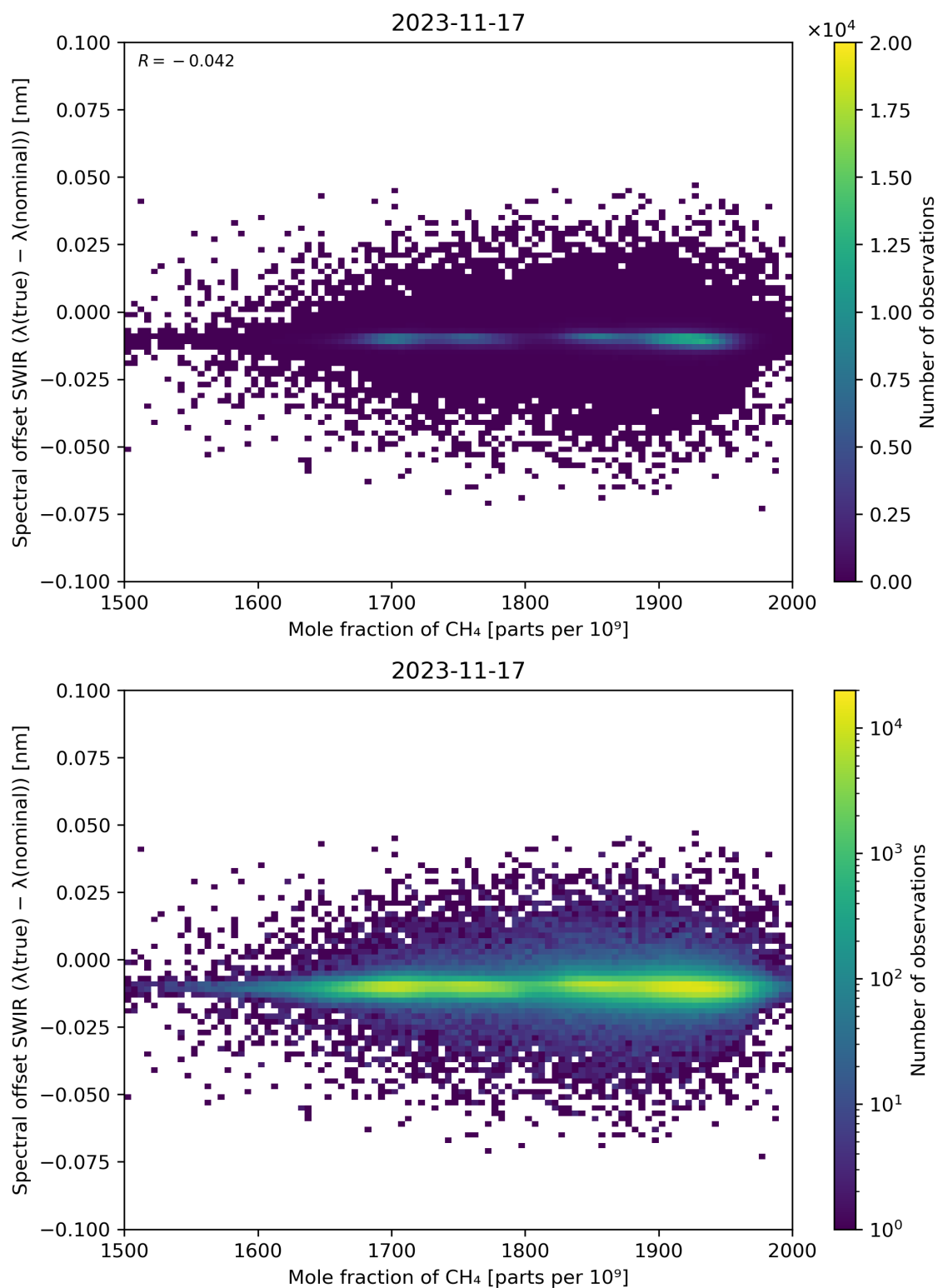
Figure 86: Scatter density plot of “Mole fraction of CH 4 ” against “Spectral offset SWIR ( \lambda(\text{true}) - \lambda(\text{nominal}) )” for 2023-11-16 to 2023-11-18.
