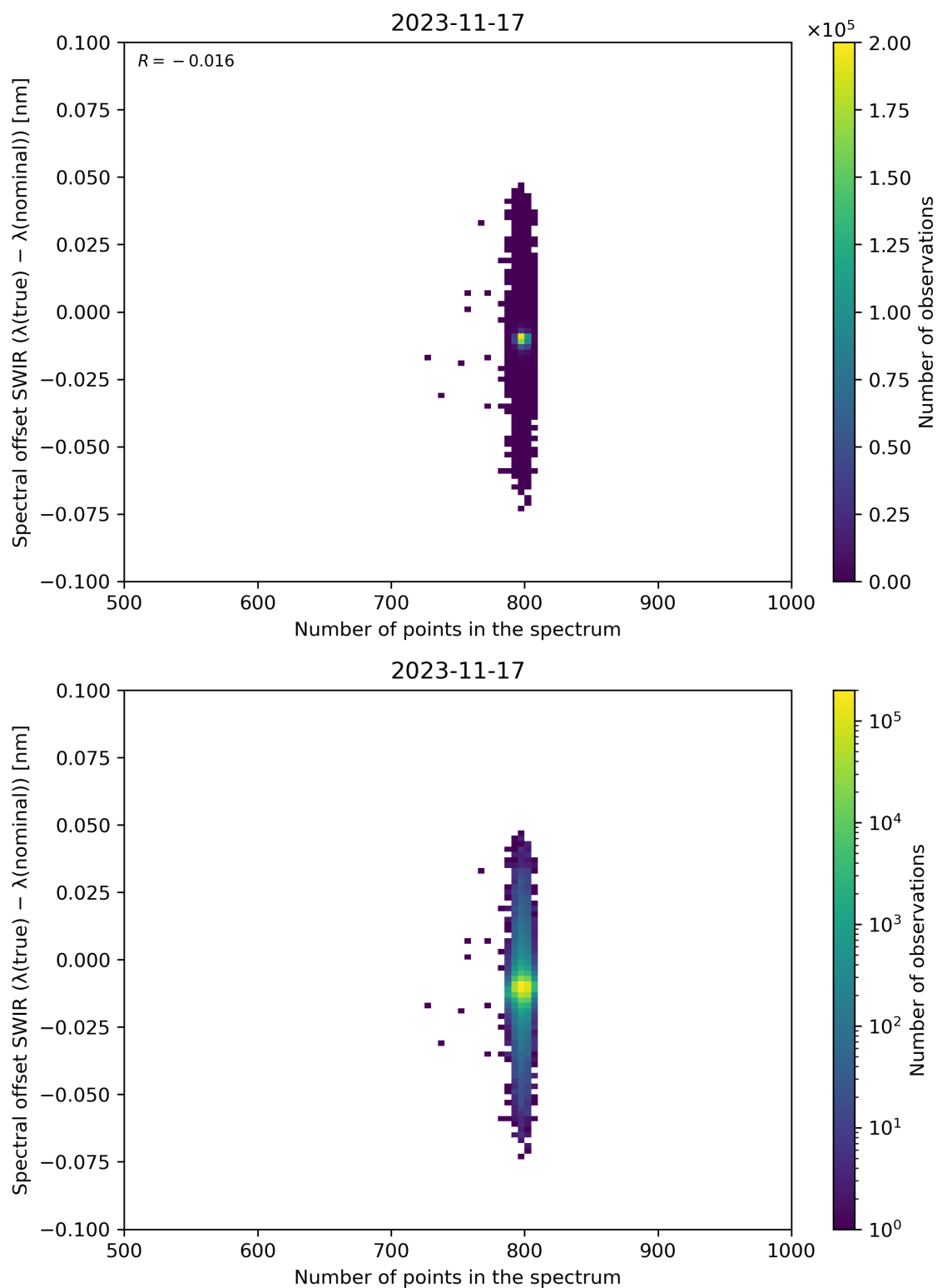
Figure 93: Scatter density plot of “Number of points in the spectrum” against “Spectral offset SWIR ( \lambda(\text{true}) - \lambda(\text{nominal}) )” for 2023-11-16 to 2023-11-18.
