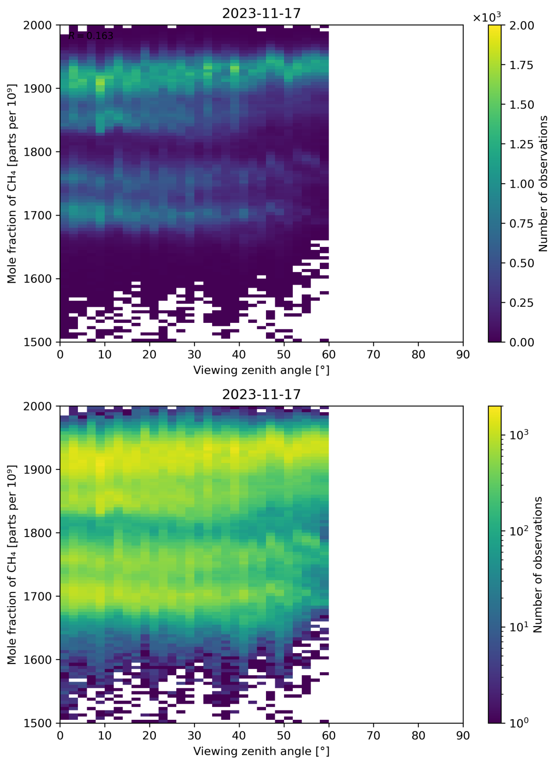
Figure 110: Scatter density plot of “Viewing zenith angle” against “Mole fraction of CH 4 ” for 2023-11-16 to 2023-11-18.
