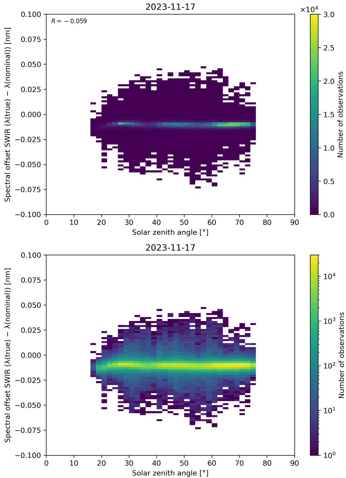
Figure 104: Scatter density plot of “Solar zenith angle” against “Spectral offset SWIR ( \lambda(\text{true}) - \lambda(\text{nominal}) )” for 2023-11-16 to 2023-11-18.
