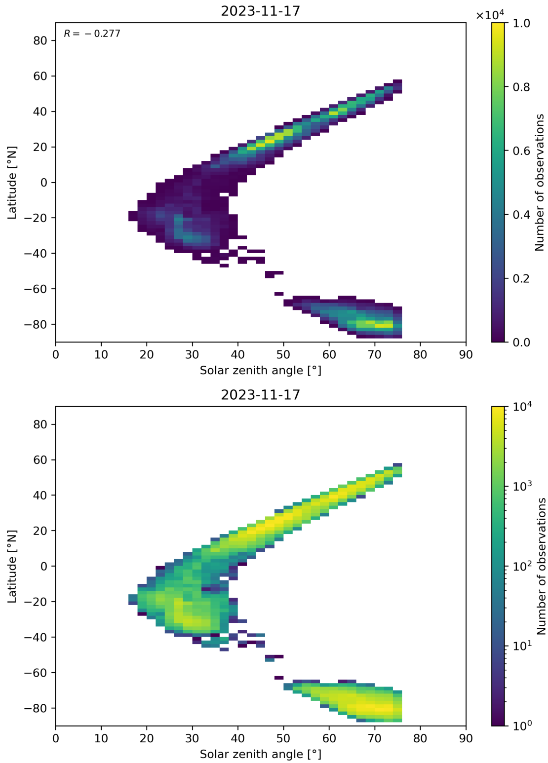
Figure 98: Scatter density plot of “Solar zenith angle” against “Latitude” for 2023-11-16 to 2023-11-18.
