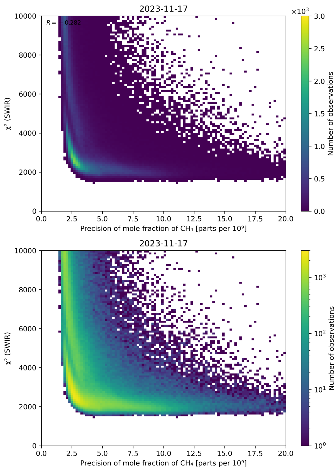
Figure 79: Scatter density plot of “Precision of mole fraction of \text{CH}_4 ” against “ \chi^2 (SWIR)” for 2023-11-16 to 2023-11-18.
