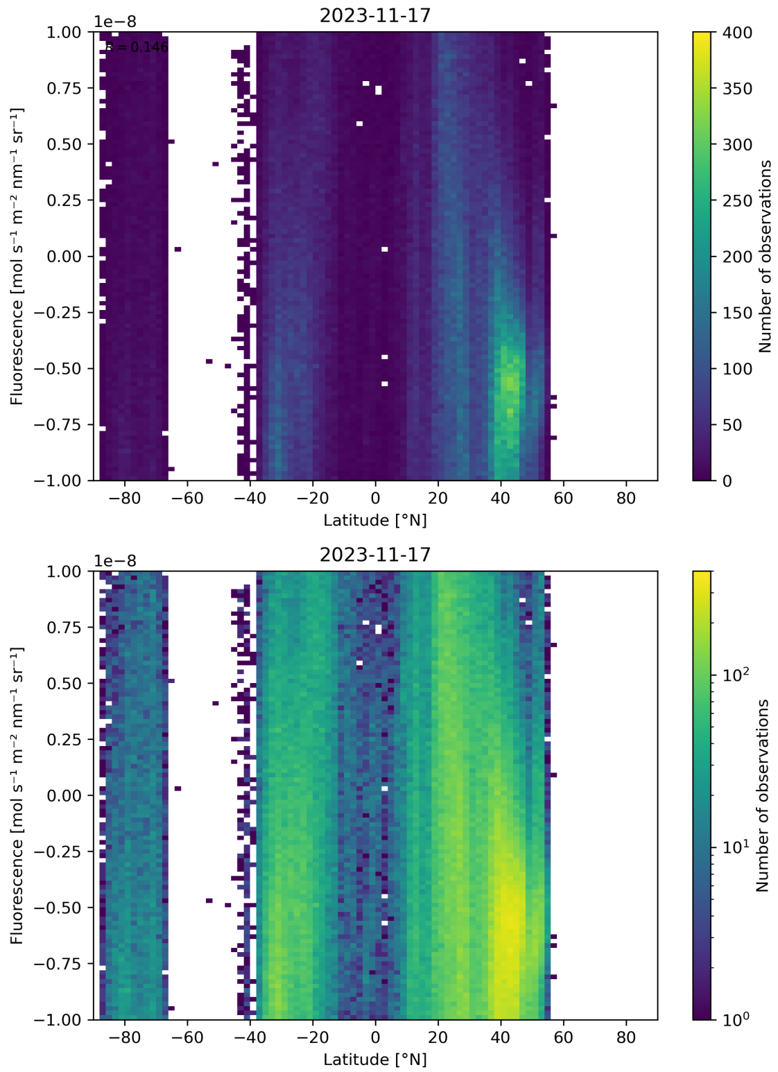
Figure 56: Scatter density plot of “Latitude” against “Fluorescence” for 2023-11-16 to 2023-11-18.
