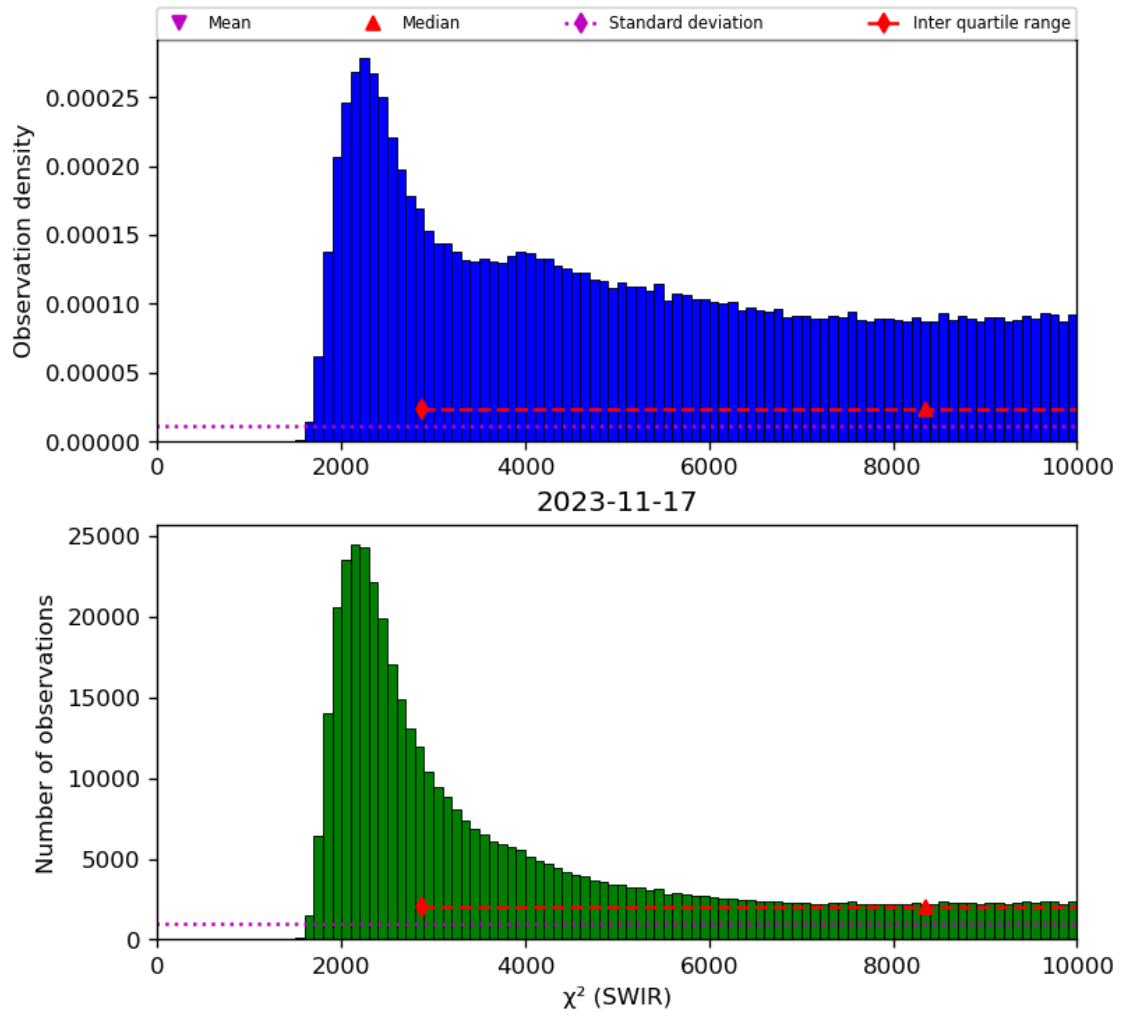
Figure 28: Histogram of “ \chi^2 (SWIR)” for 2023-11-16 to 2023-11-18
