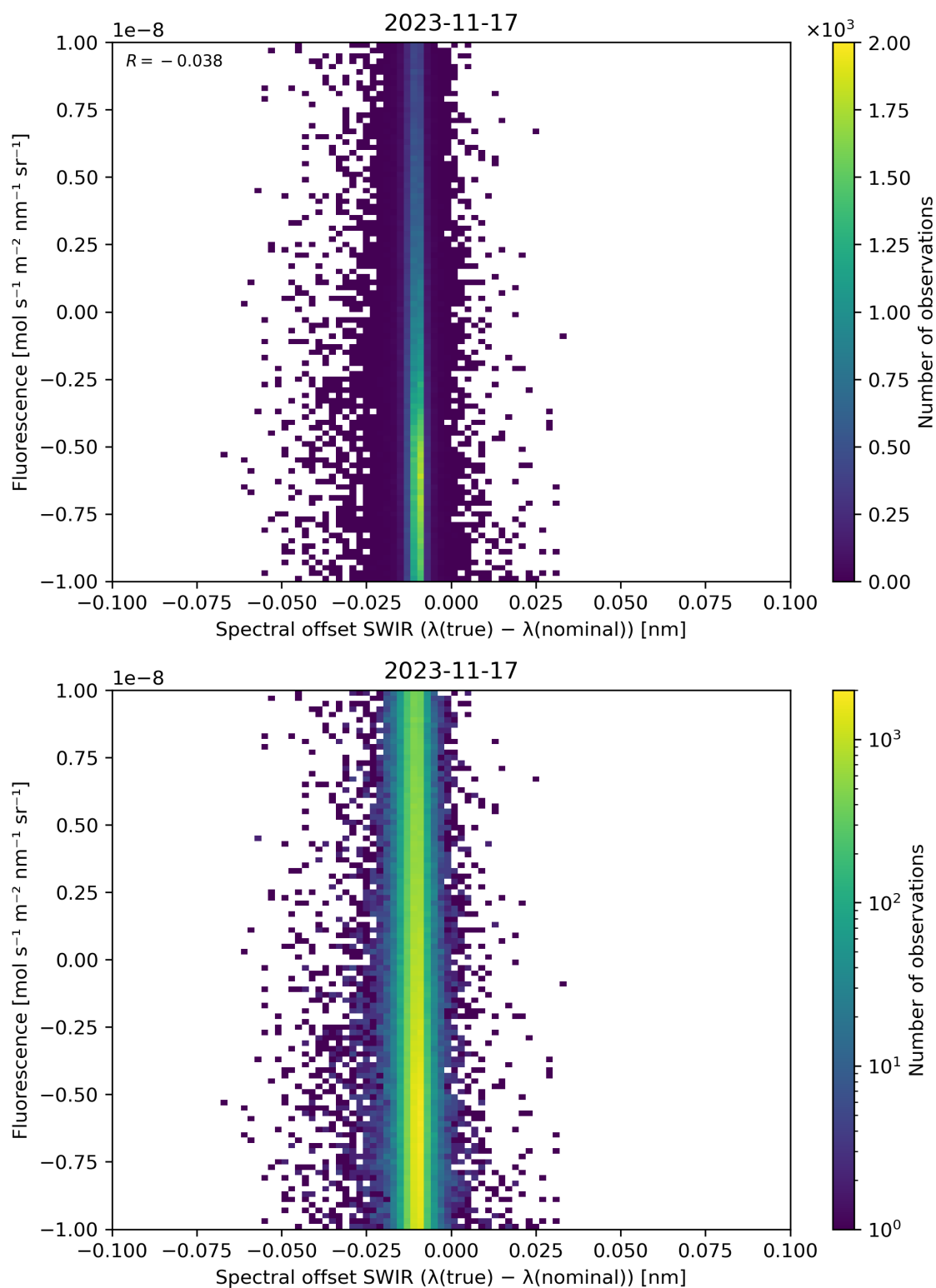
Figure 120: Scatter density plot of “Spectral offset SWIR ( \lambda(\text{true}) - \lambda(\text{nominal}) )” against “Fluorescence” for 2023-11-16 to 2023-11-18.
