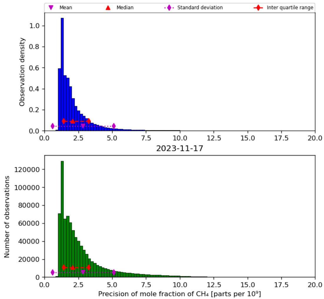
Figure 24: Histogram of “Precision of mole fraction of CH 4 ” for 2023-11-16 to 2023-11-18
