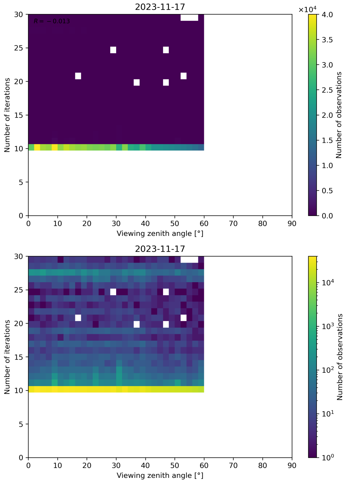
Figure 113: Scatter density plot of “Viewing zenith angle” against “Number of iterations” for 2023-11-16 to 2023-11-18.
