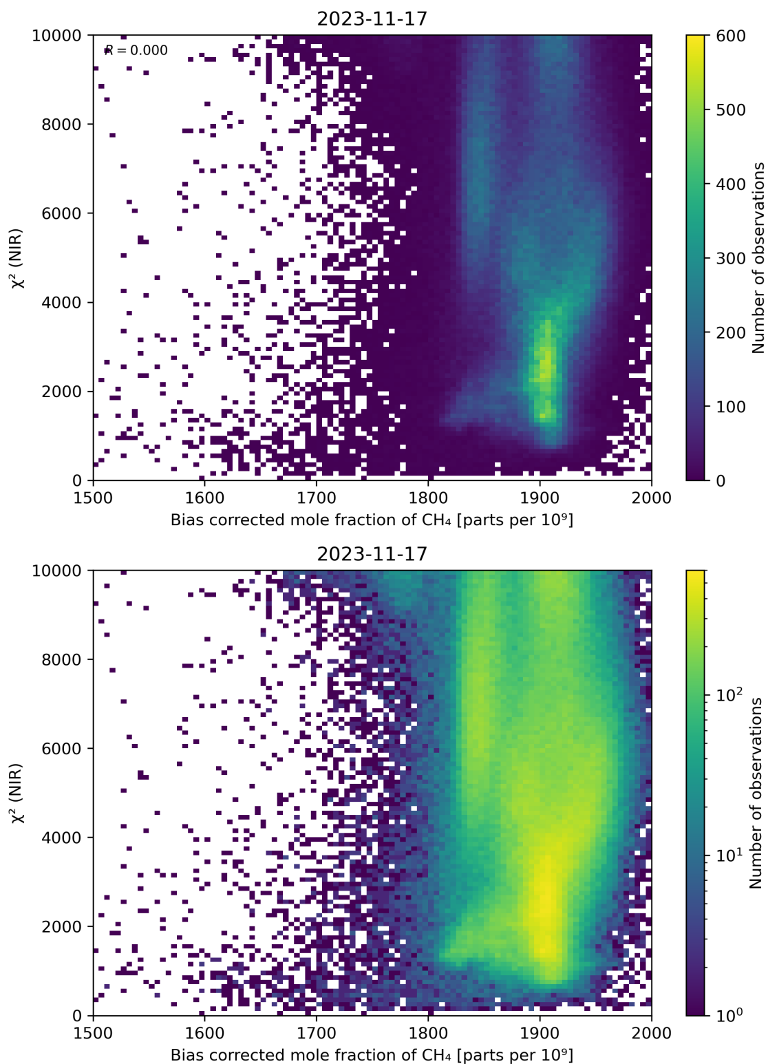
Figure 63: Scatter density plot of “Bias corrected mole fraction of \text{CH}_4 ” against “ \chi^2 (NIR)” for 2023-11-16 to 2023-11-18.
