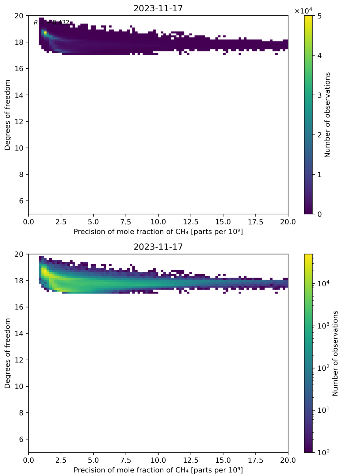
Figure 80: Scatter density plot of “Precision of mole fraction of CH 4 ” against “Degrees of freedom” for 2023-11-16 to 2023-11-18.
