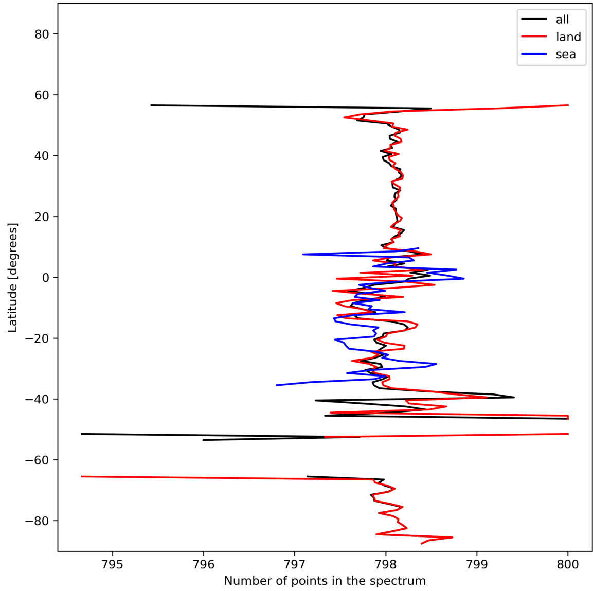
Figure 15: Zonal average of “Number of points in the spectrum” for 2023-11-16 to 2023-11-18.
