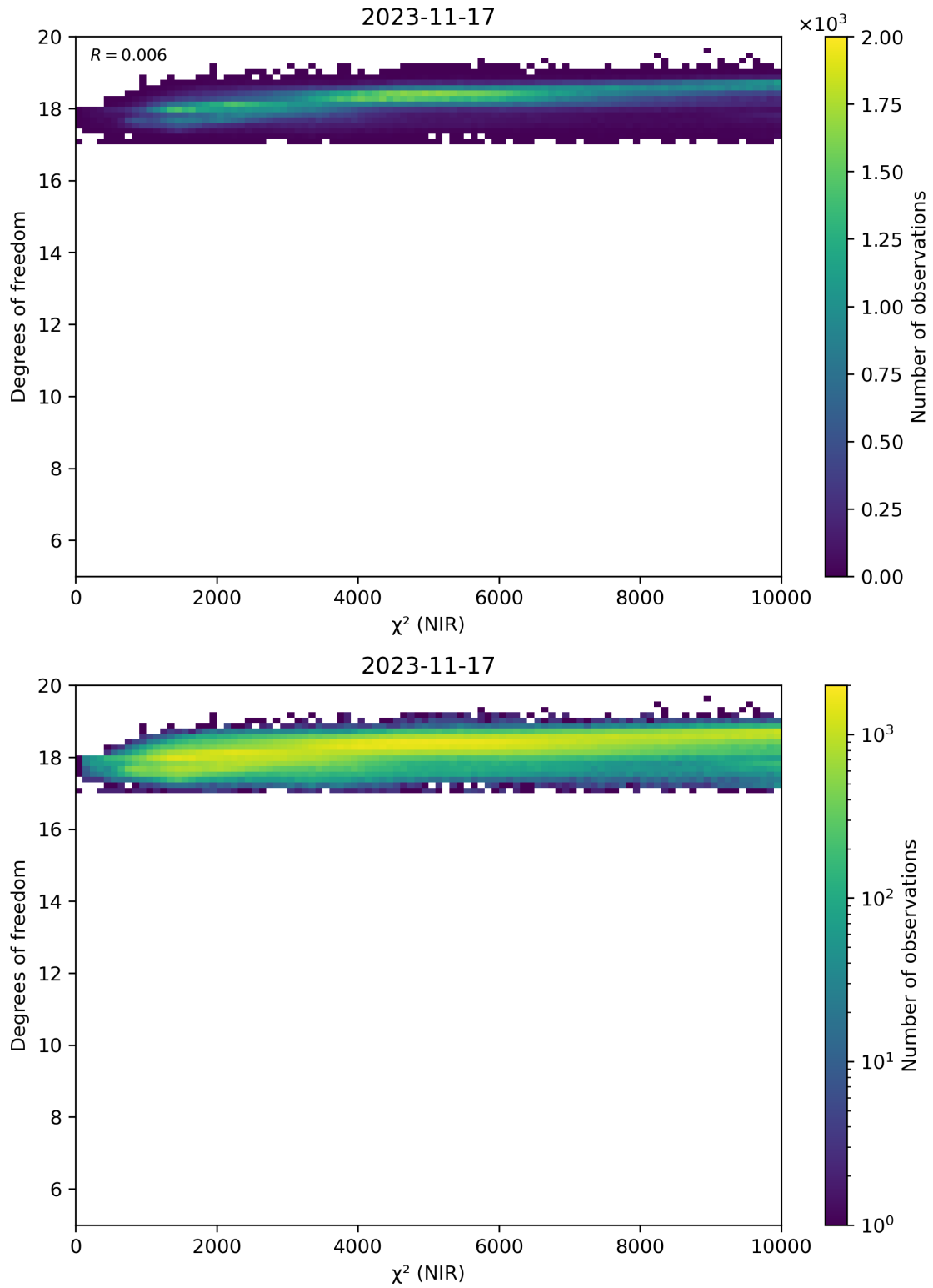
Figure 44: Scatter density plot of “ \chi^2 (NIR)” against “Degrees of freedom” for 2023-11-16 to 2023-11-18.
