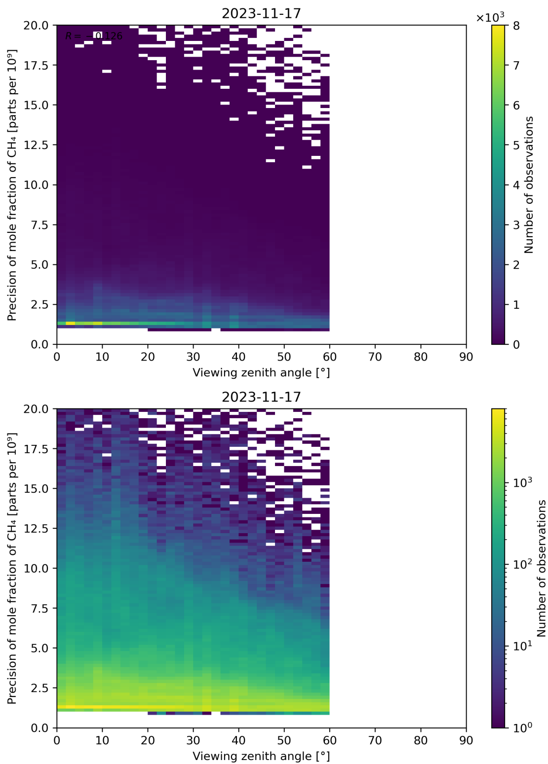
Figure 112: Scatter density plot of “Viewing zenith angle” against “Precision of mole fraction of CH 4 ” for 2023-11-16 to 2023-11-18.
