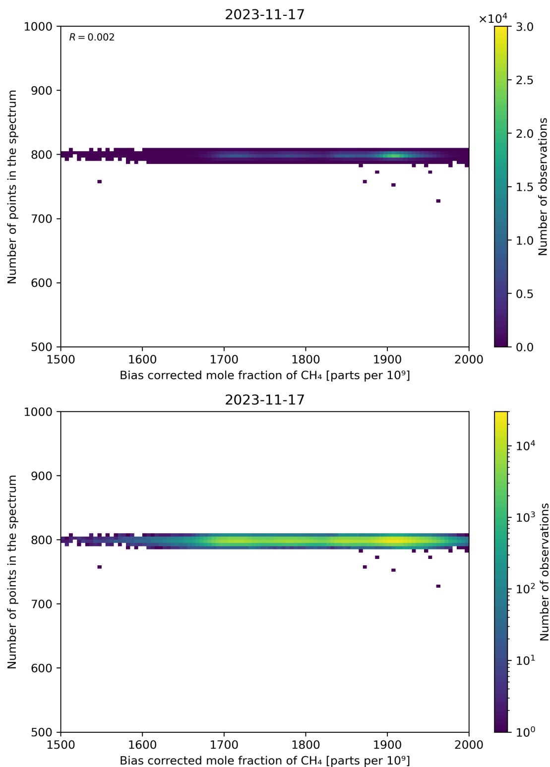
Figure 68: Scatter density plot of “Bias corrected mole fraction of CH 4 ” against “Number of points in the spectrum” for 2023-11-16 to 2023-11-18.
