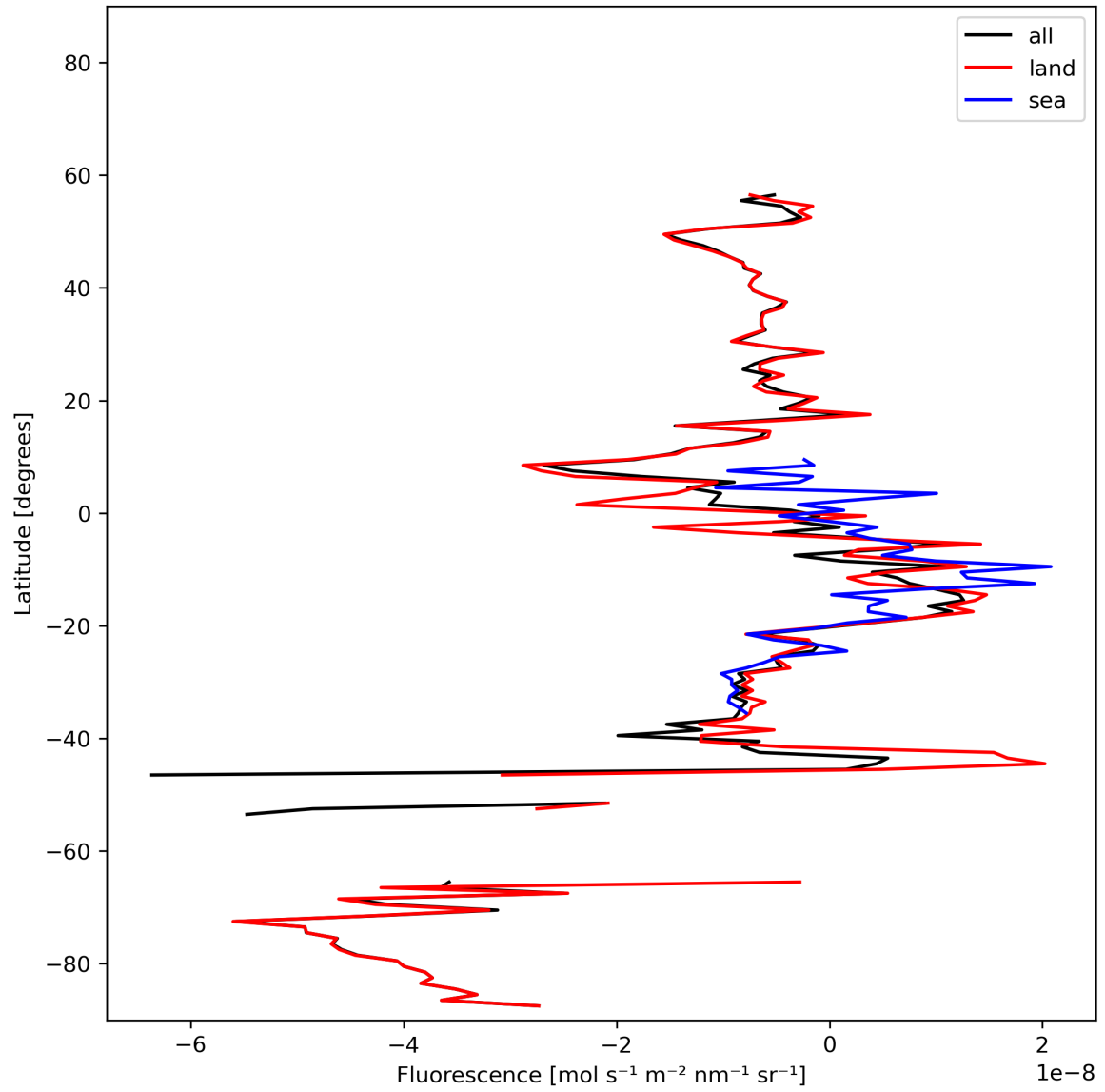
Figure 21: Zonal average of “Fluorescence” for 2023-11-16 to 2023-11-18.
