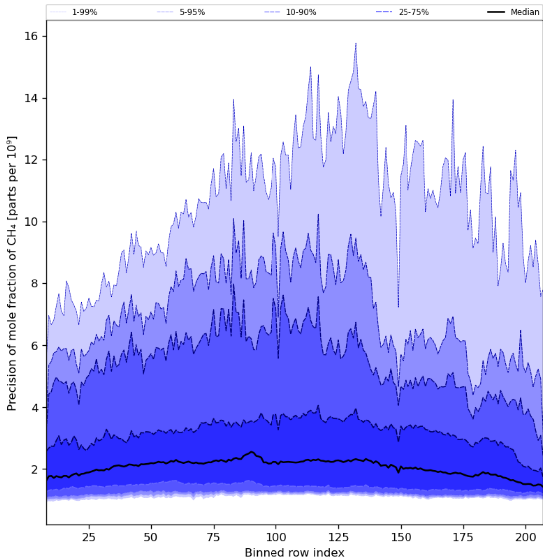
Figure 35: Along track statistics of “Precision of mole fraction of CH 4 ” for 2023-11-16 to 2023-11-18
