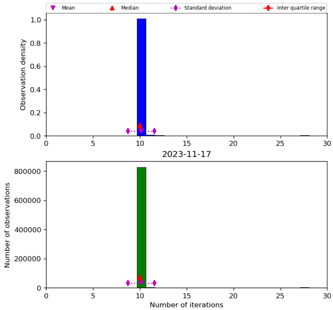
Figure 31: Histogram of “Number of iterations” for 2023-11-16 to 2023-11-18
