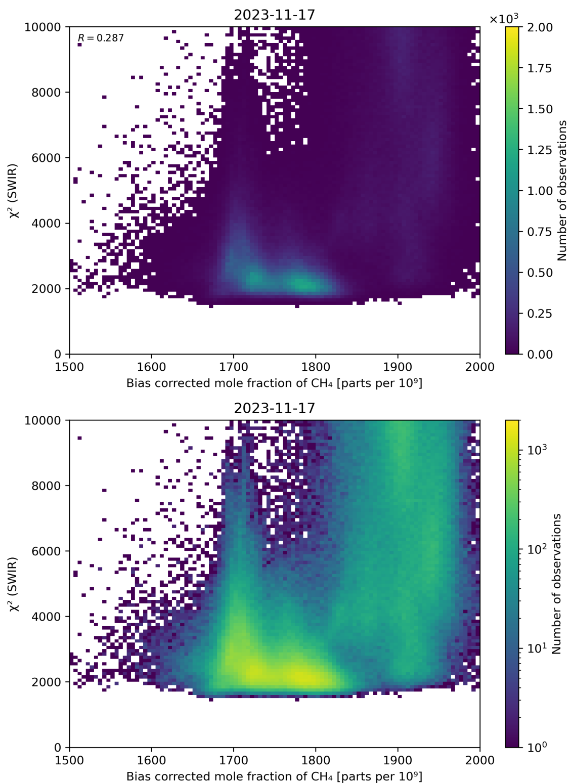
Figure 64: Scatter density plot of “Bias corrected mole fraction of \text{CH}_4 ” against “ \chi^2 (SWIR)” for 2023-11-16 to 2023-11-18.
