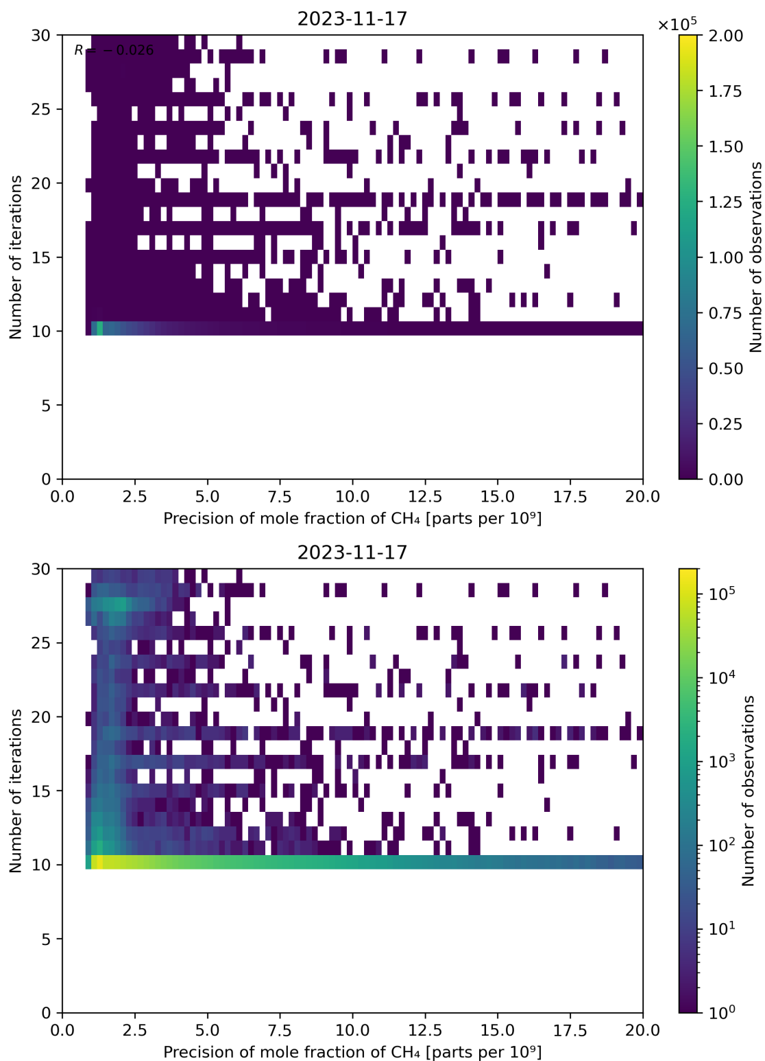
Figure 83: Scatter density plot of “Precision of mole fraction of CH 4 ” against “Number of iterations” for 2023-11-16 to 2023-11-18.
