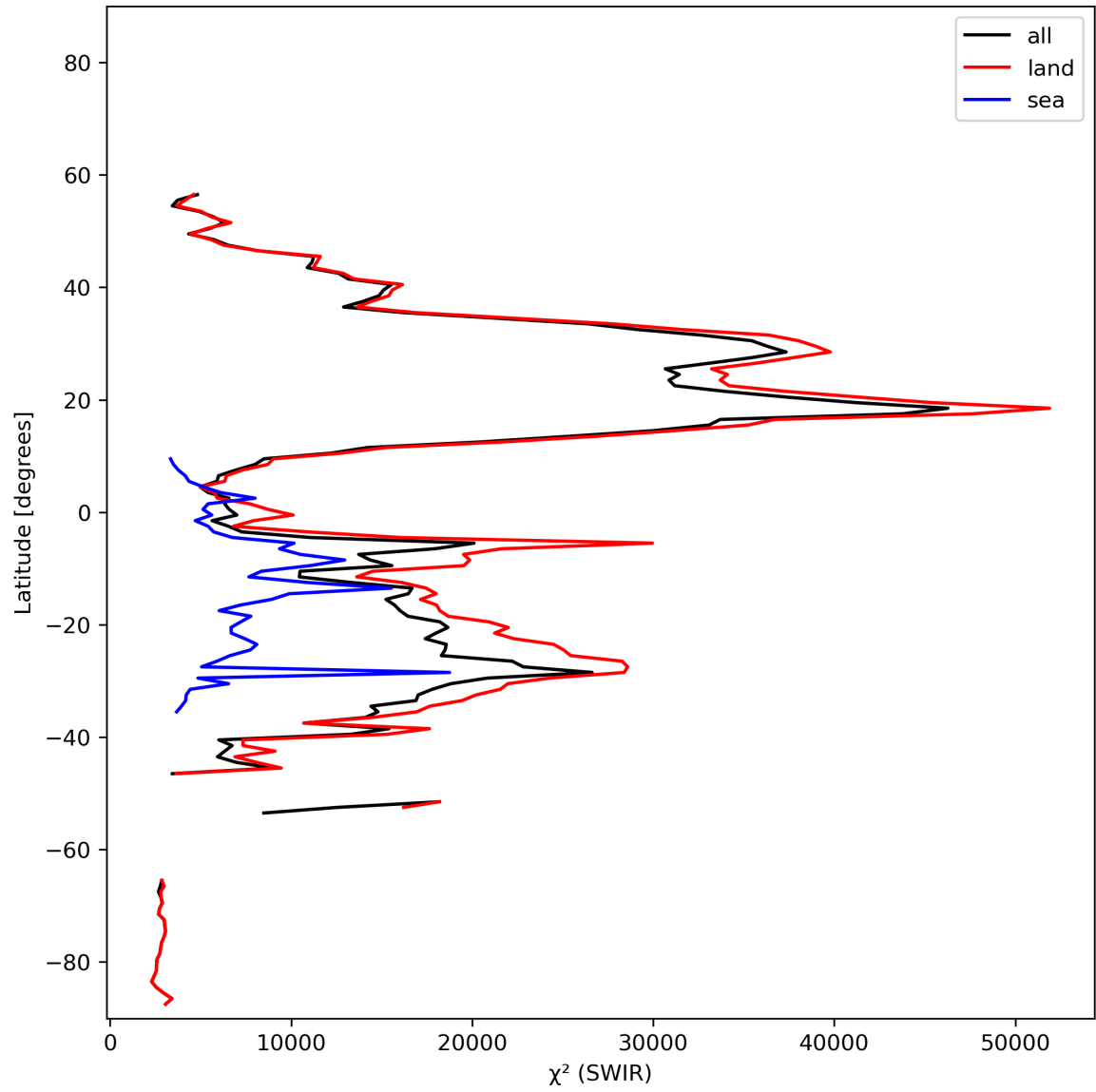
Figure 17: Zonal average of “ \chi^2 (SWIR)” for 2023-11-16 to 2023-11-18.
