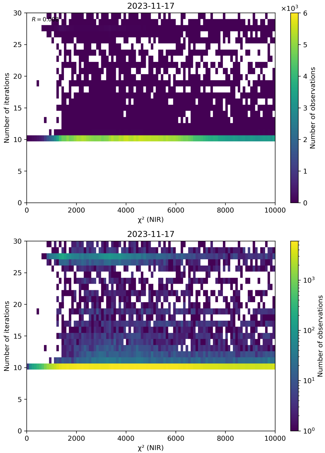
Figure 46: Scatter density plot of “ \chi^2 (NIR)” against “Number of iterations” for 2023-11-16 to 2023-11-18.
