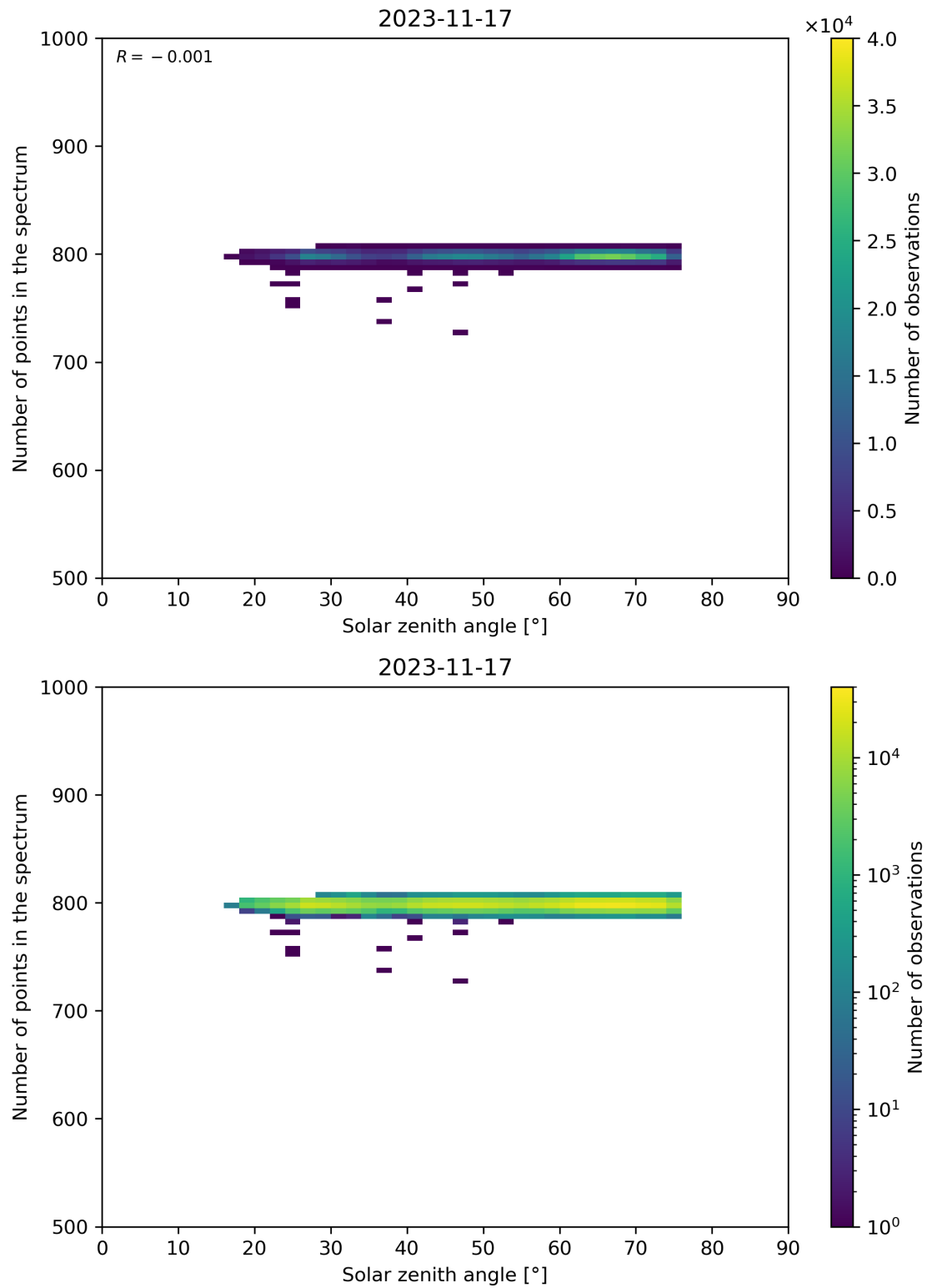
Figure 103: Scatter density plot of “Solar zenith angle” against “Number of points in the spectrum” for 2023-11-16 to 2023-11-18.
