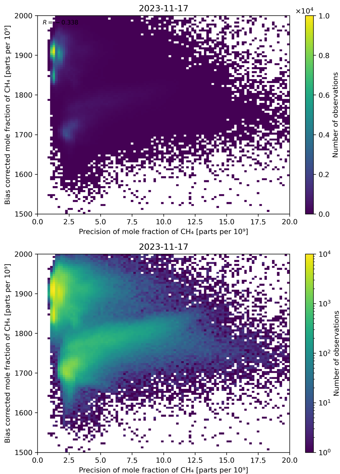
Figure 82: Scatter density plot of “Precision of mole fraction of CH 4 ” against “Bias corrected mole fraction of CH 4 ” for 2023-11-16 to 2023-11-18.
