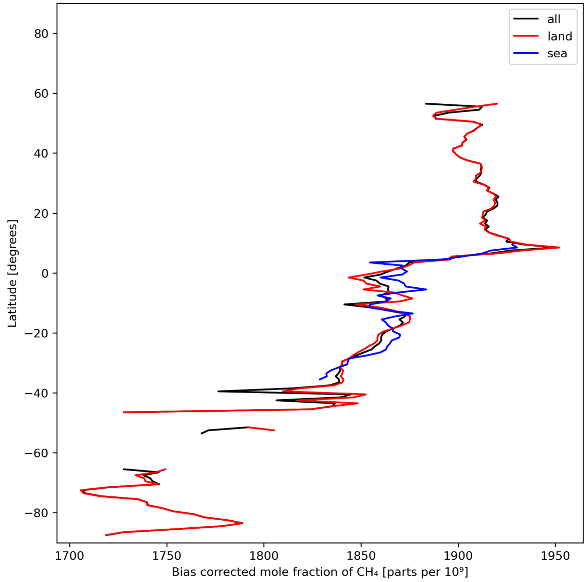
Figure 14: Zonal average of “Bias corrected mole fraction of CH 4 ” for 2023-11-16 to 2023-11-18.
