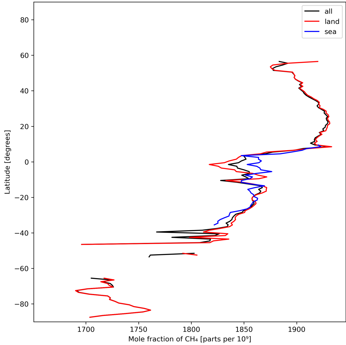
Figure 12: Zonal average of “Mole fraction of \text{CH}_4 ” for 2023-11-16 to 2023-11-18.
