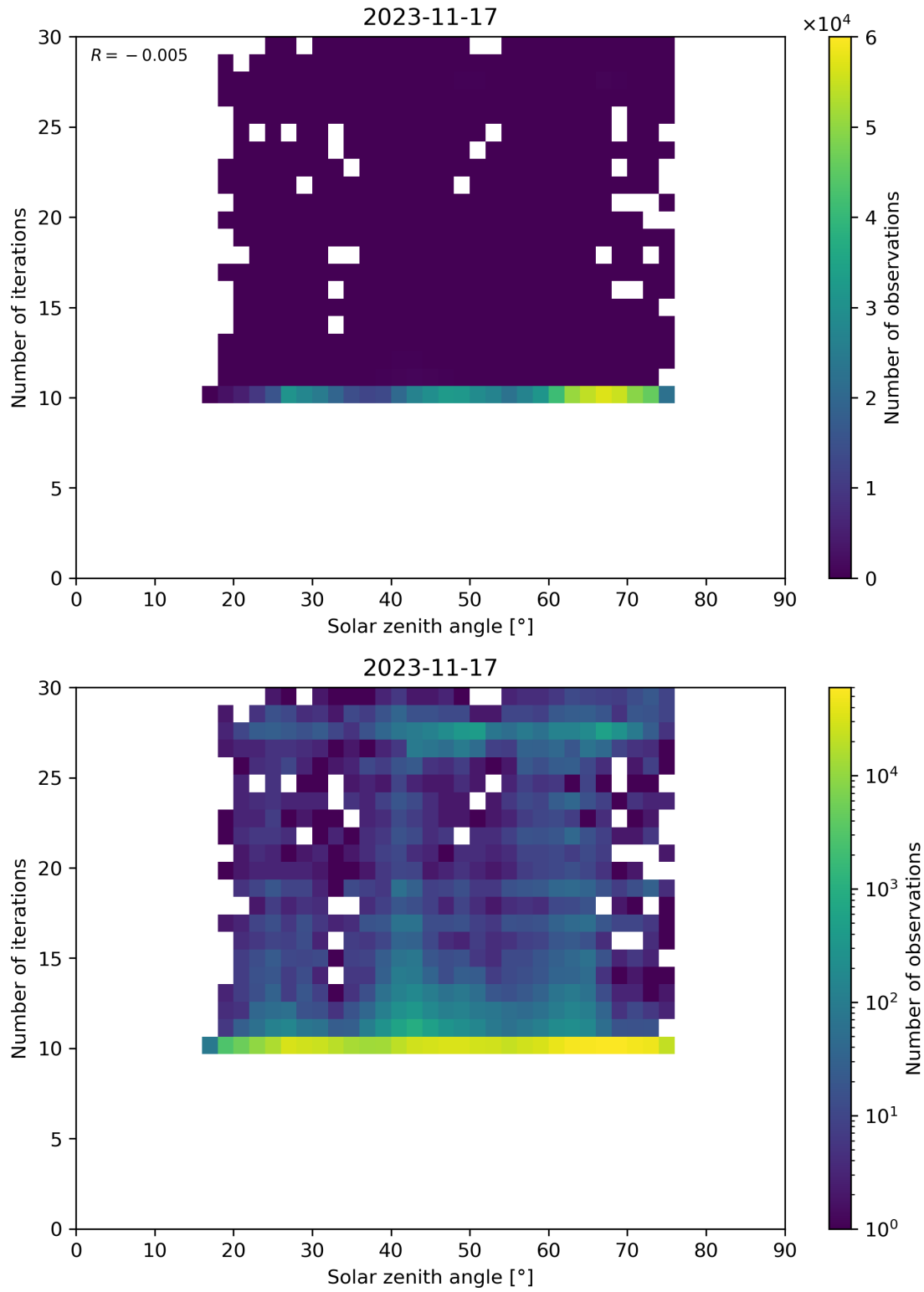
Figure 102: Scatter density plot of “Solar zenith angle” against “Number of iterations” for 2023-11-16 to 2023-11-18.
