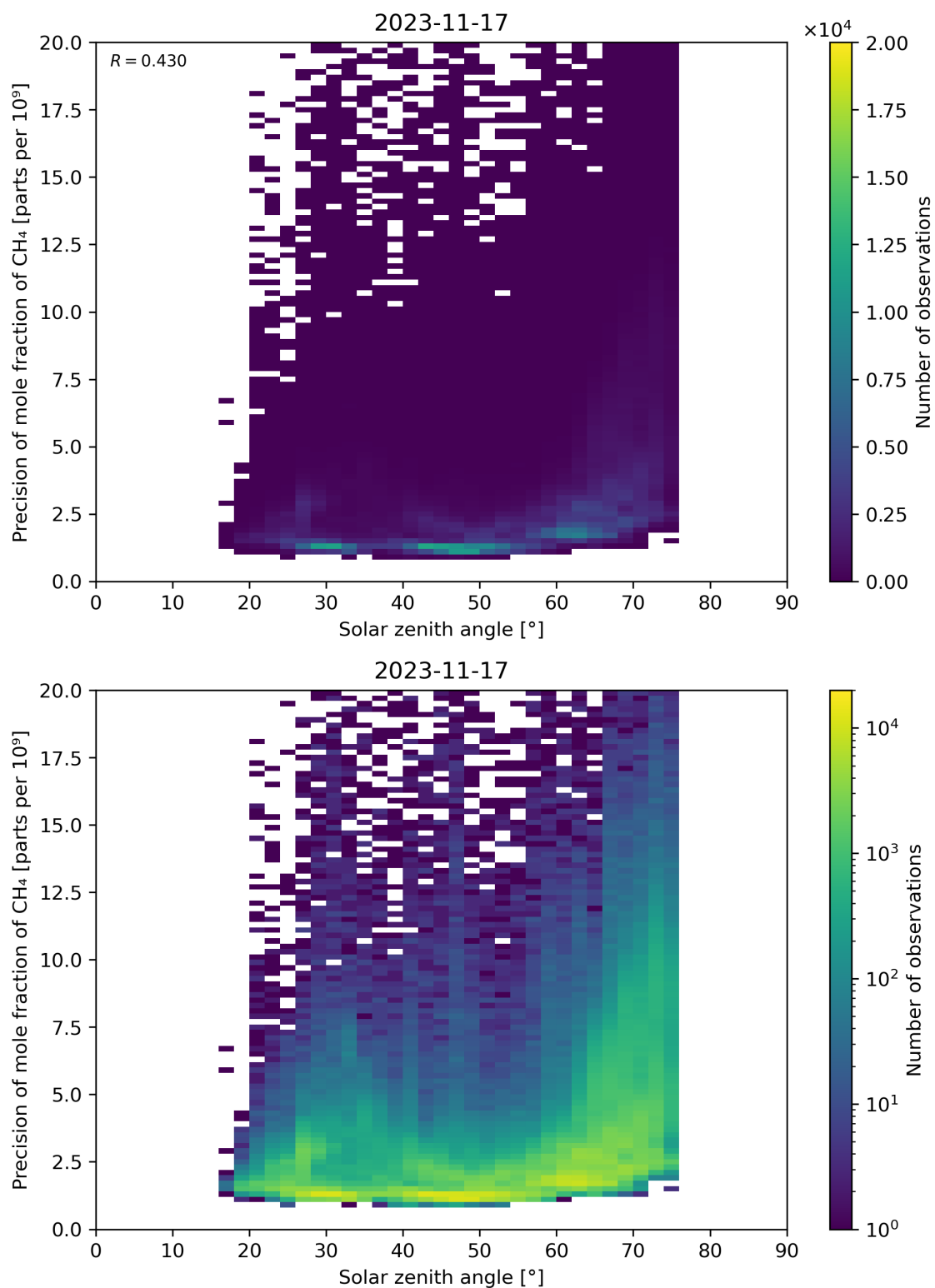
Figure 101: Scatter density plot of “Solar zenith angle” against “Precision of mole fraction of \text{CH}_4 ” for 2023-11-16 to 2023-11-18.
