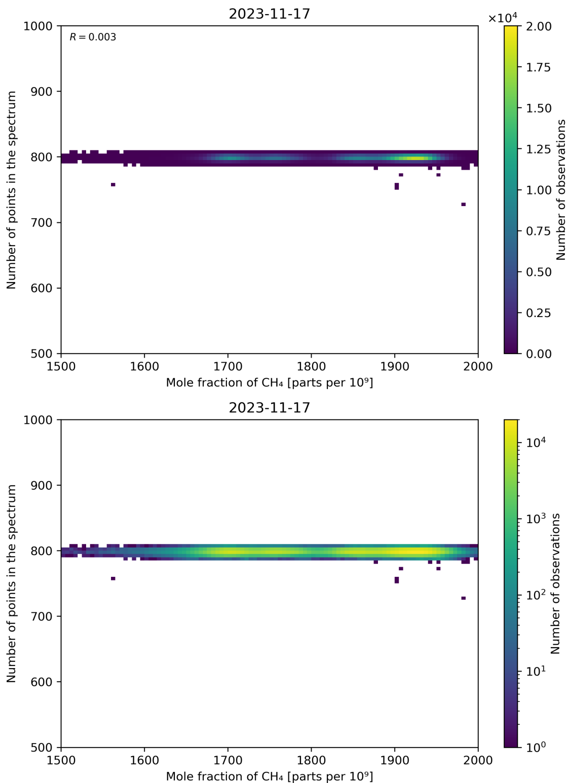
Figure 77: Scatter density plot of “Mole fraction of CH 4 ” against “Number of points in the spectrum” for 2023-11-16 to 2023-11-18.
