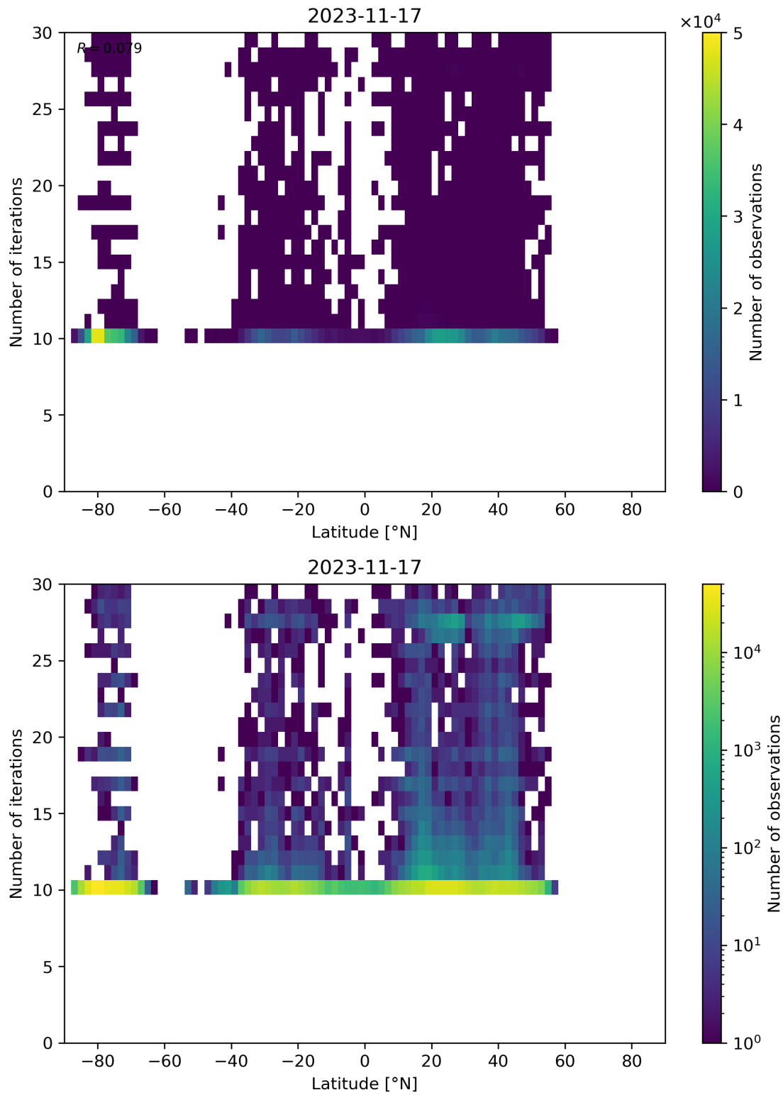
Figure 60: Scatter density plot of “Latitude” against “Number of iterations” for 2023-11-16 to 2023-11-18.
