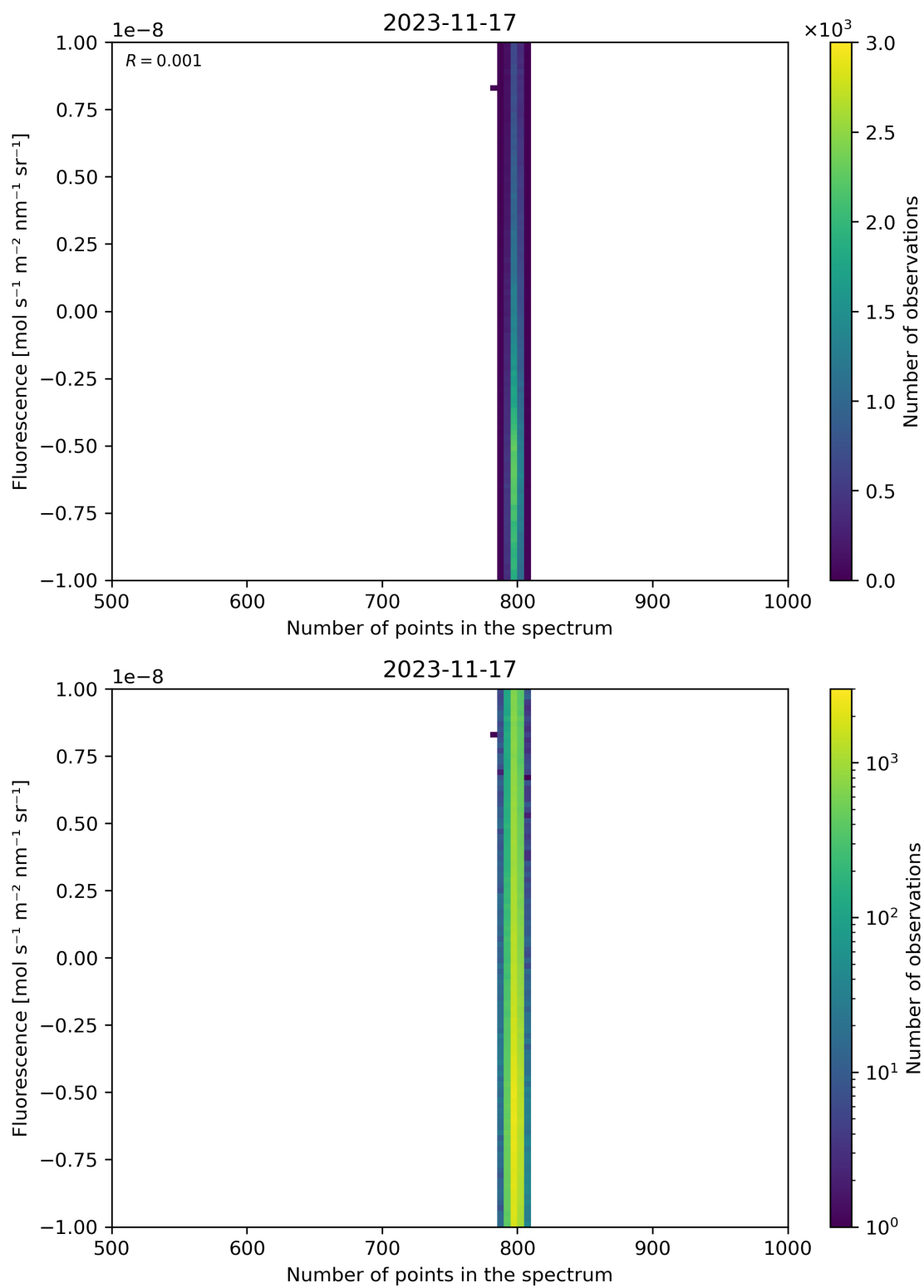
Figure 91: Scatter density plot of “Number of points in the spectrum” against “Fluorescence” for 2023-11-16 to 2023-11-18.
