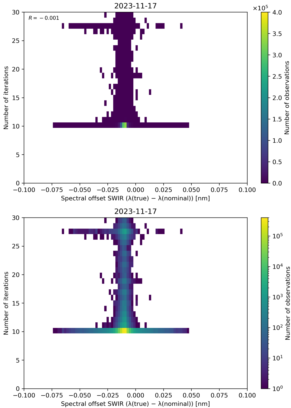
Figure 121: Scatter density plot of “Spectral offset SWIR ( \lambda(\text{true}) - \lambda(\text{nominal}) )” against “Number of iterations” for 2023-11-16 to 2023-11-18.
