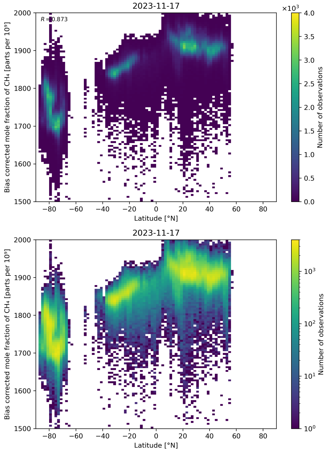
Figure 58: Scatter density plot of “Latitude” against “Bias corrected mole fraction of CH 4 ” for 2023-11-16 to 2023-11-18.
