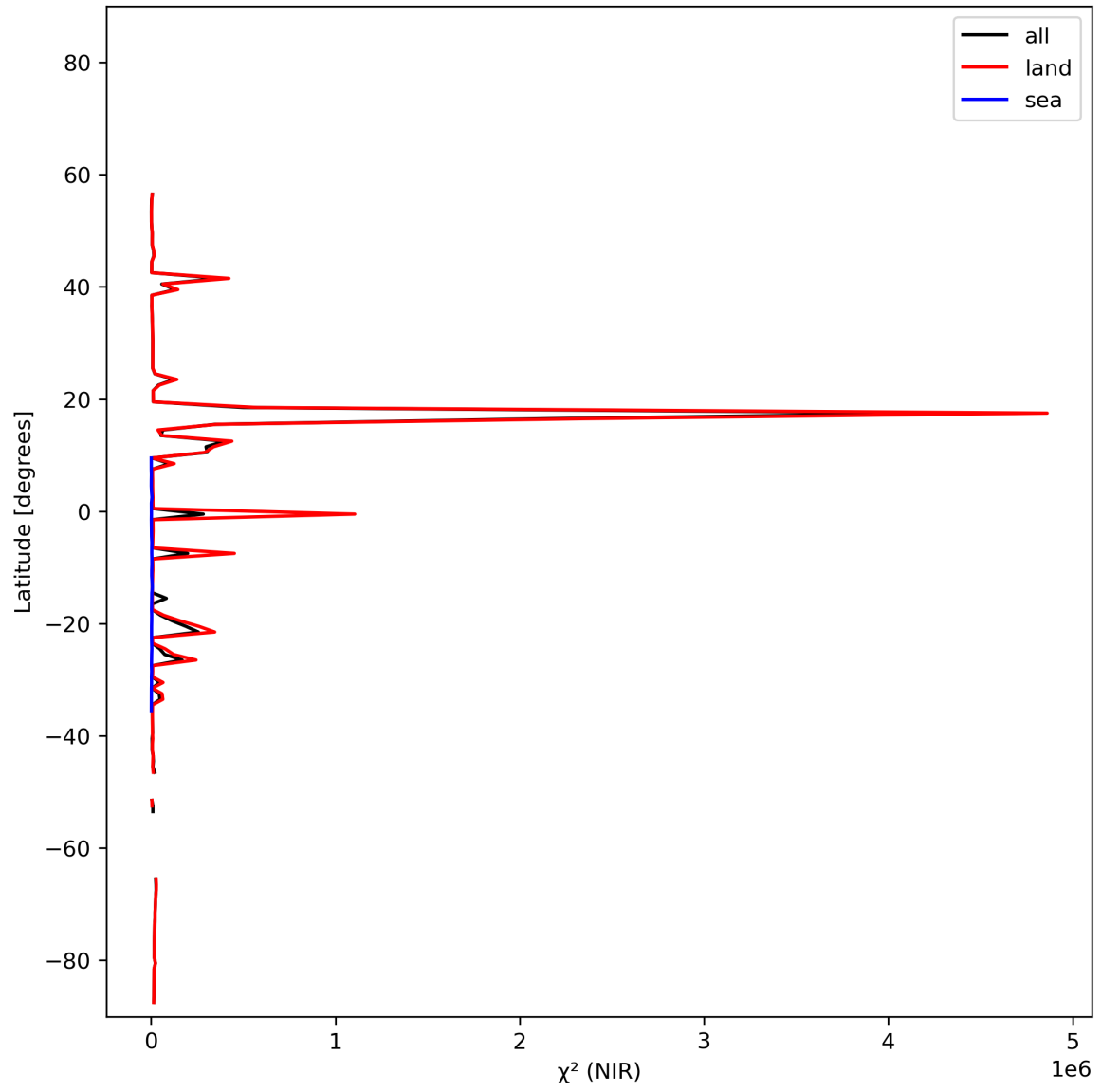
Figure 18: Zonal average of “ \chi^2 (NIR)” for 2023-11-16 to 2023-11-18.
