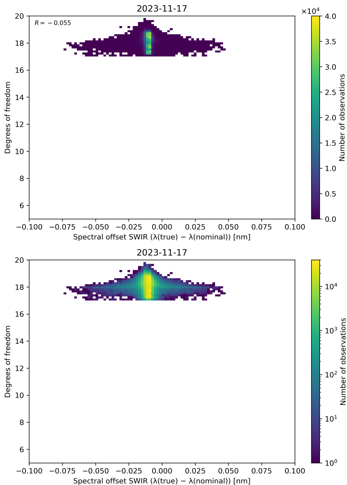
Figure 119: Scatter density plot of “Spectral offset SWIR ( \lambda(\text{true}) - \lambda(\text{nominal}) )” against “Degrees of freedom” for 2023-11-16 to 2023-11-18.
