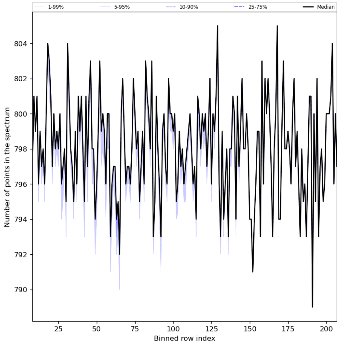
Figure 37: Along track statistics of “Number of points in the spectrum” for 2023-11-16 to 2023-11-18
