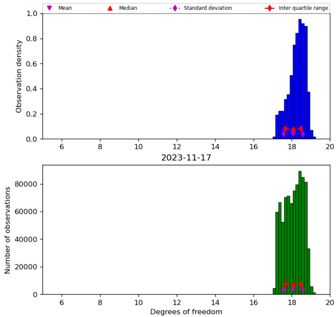
Figure 30: Histogram of “Degrees of freedom” for 2023-11-16 to 2023-11-18
