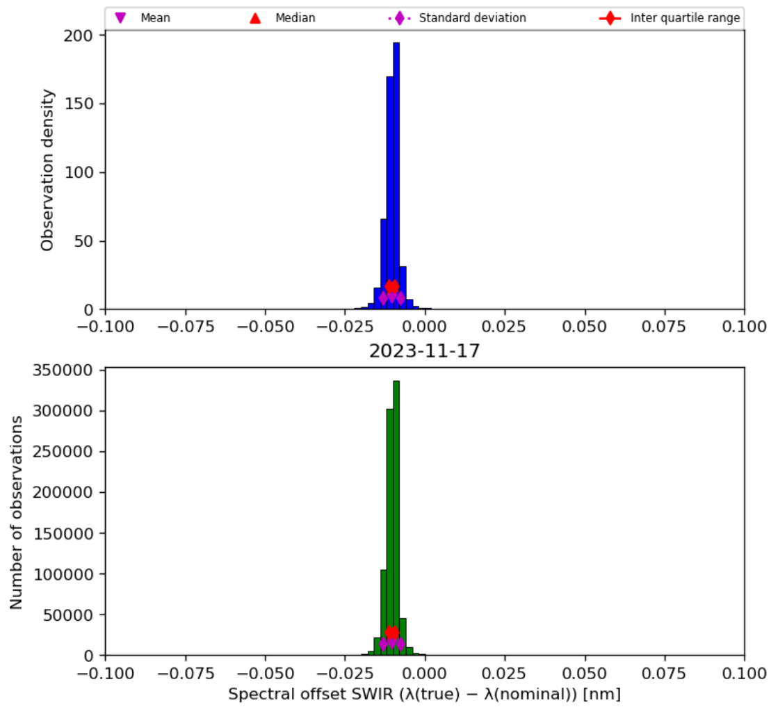
Figure 27: Histogram of “Spectral offset SWIR ( \lambda(\text{true}) - \lambda(\text{nominal}) )” for 2023-11-16 to 2023-11-18
