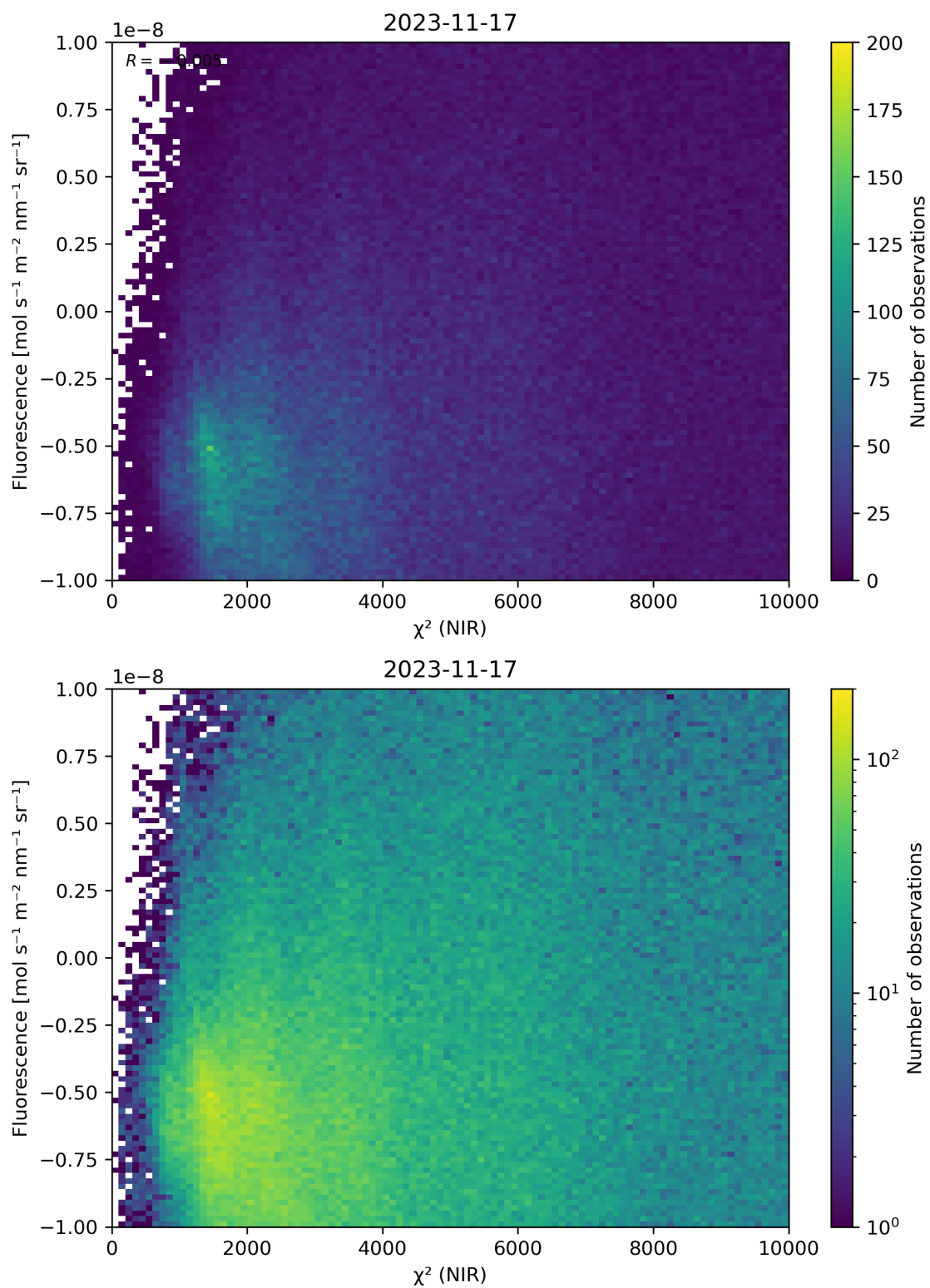
Figure 45: Scatter density plot of “ \chi^2 (NIR)” against “Fluorescence” for 2023-11-16 to 2023-11-18.
