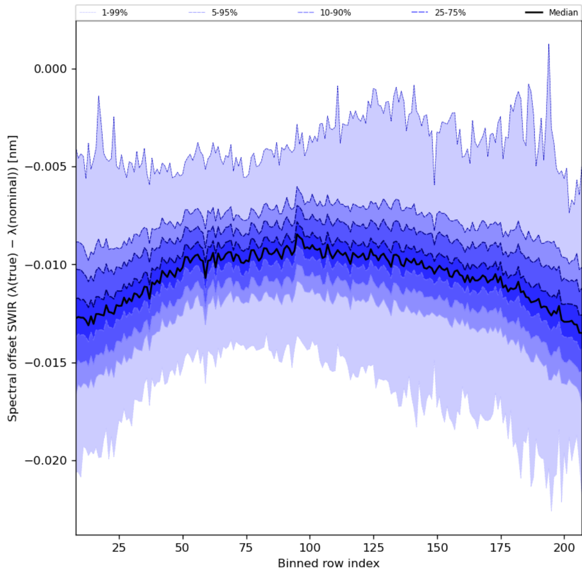
Figure 38: Along track statistics of “Spectral offset SWIR ( \lambda(\text{true}) - \lambda(\text{nominal}) )” for 2023-11-16 to 2023-11-18
