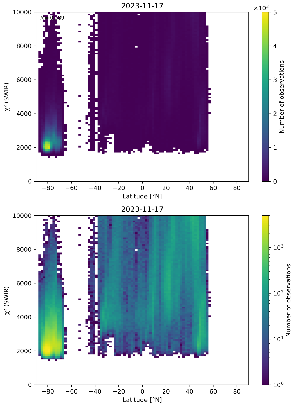
Figure 54: Scatter density plot of “Latitude” against “ \chi^2 (SWIR)” for 2023-11-16 to 2023-11-18.
