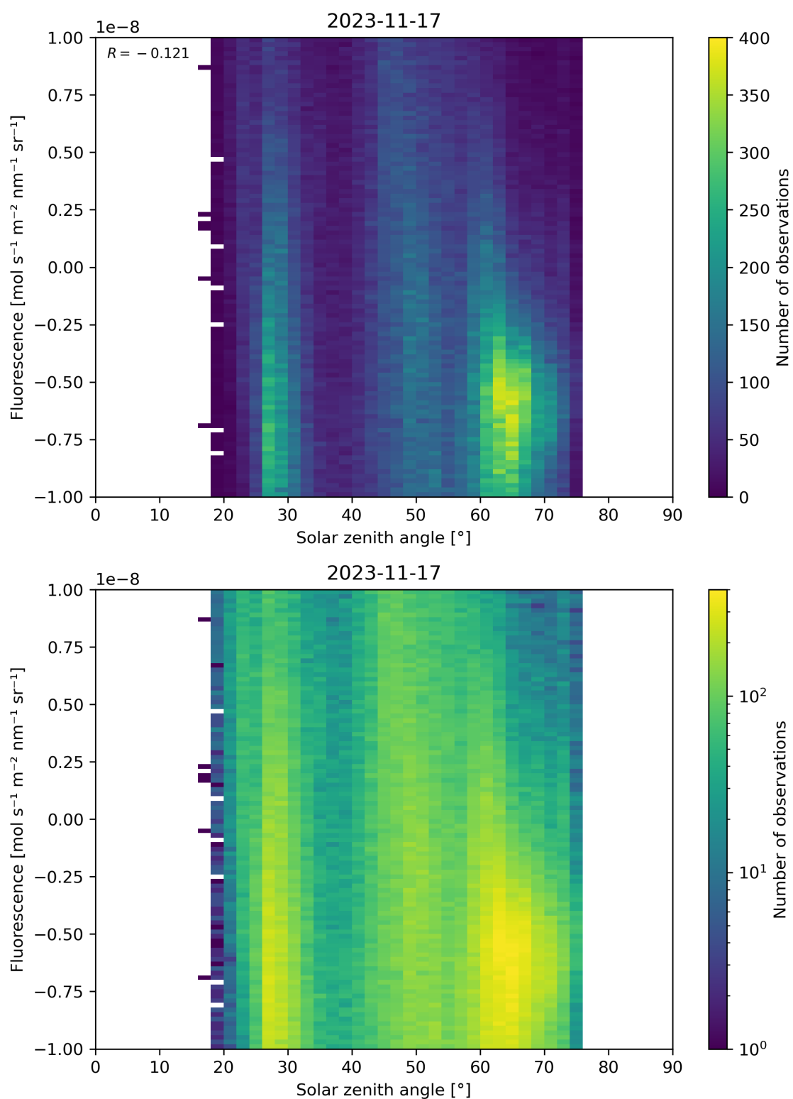
Figure 97: Scatter density plot of “Solar zenith angle” against “Fluorescence” for 2023-11-16 to 2023-11-18.
