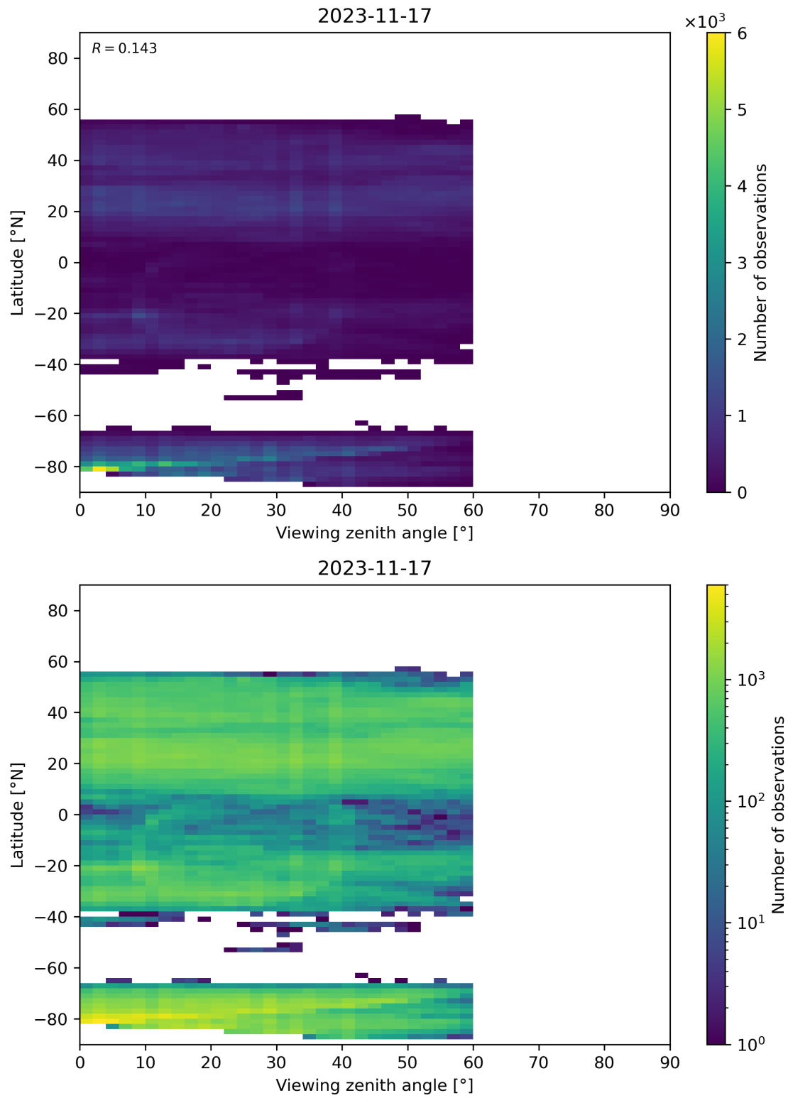
Figure 109: Scatter density plot of “Viewing zenith angle” against “Latitude” for 2023-11-16 to 2023-11-18.
