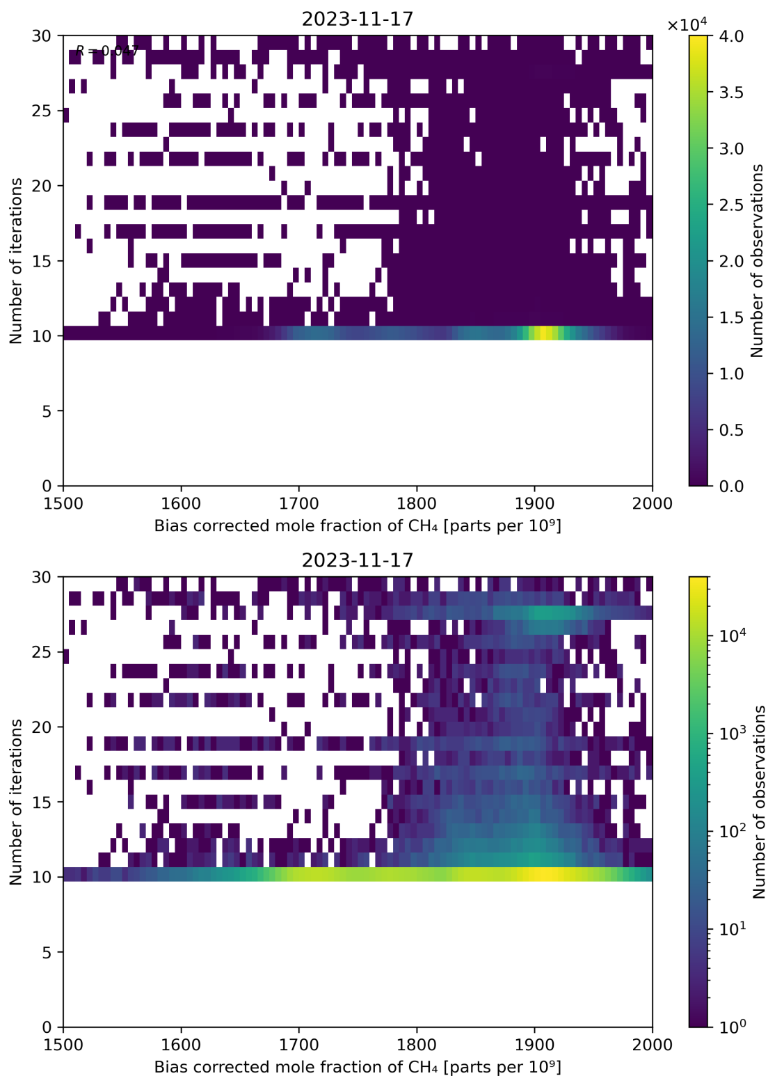
Figure 67: Scatter density plot of “Bias corrected mole fraction of \text{CH}_4 ” against “Number of iterations” for 2023-11-16 to 2023-11-18.
