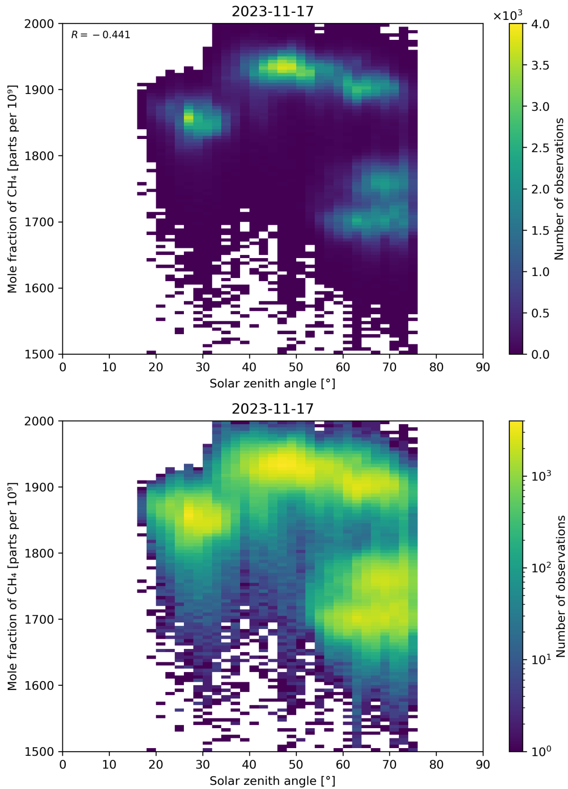
Figure 99: Scatter density plot of “Solar zenith angle” against “Mole fraction of CH 4 ” for 2023-11-16 to 2023-11-18.
