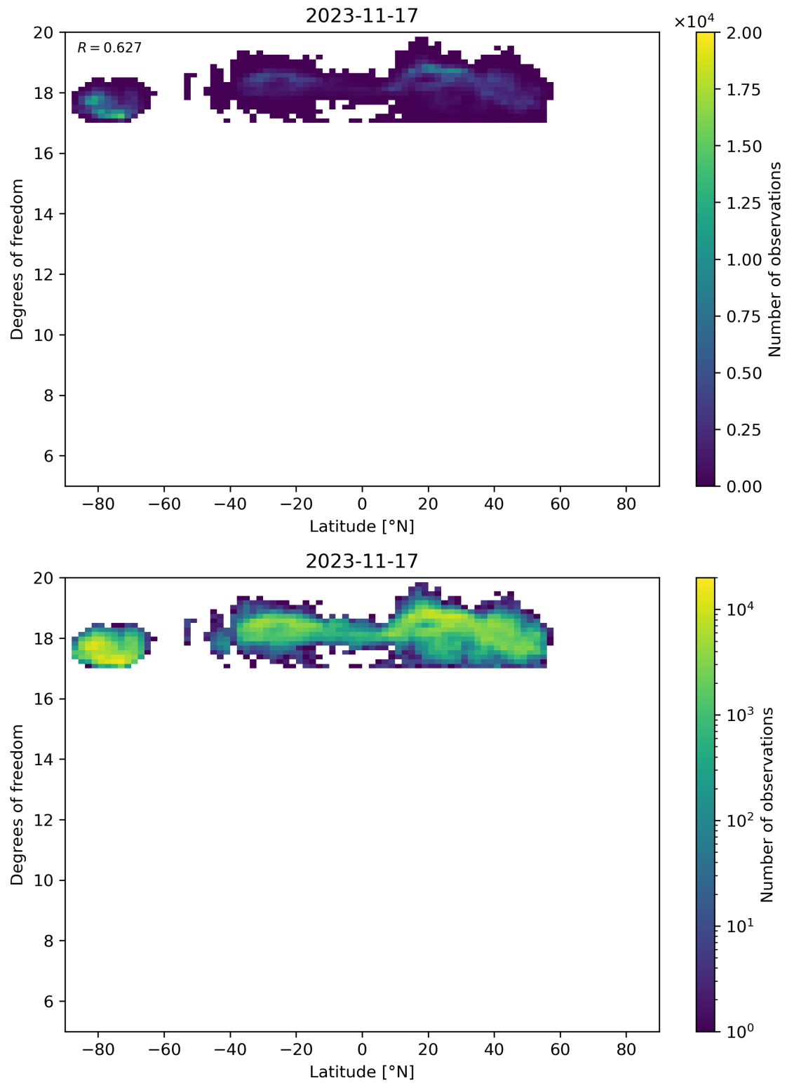
Figure 55: Scatter density plot of “Latitude” against “Degrees of freedom” for 2023-11-16 to 2023-11-18.
