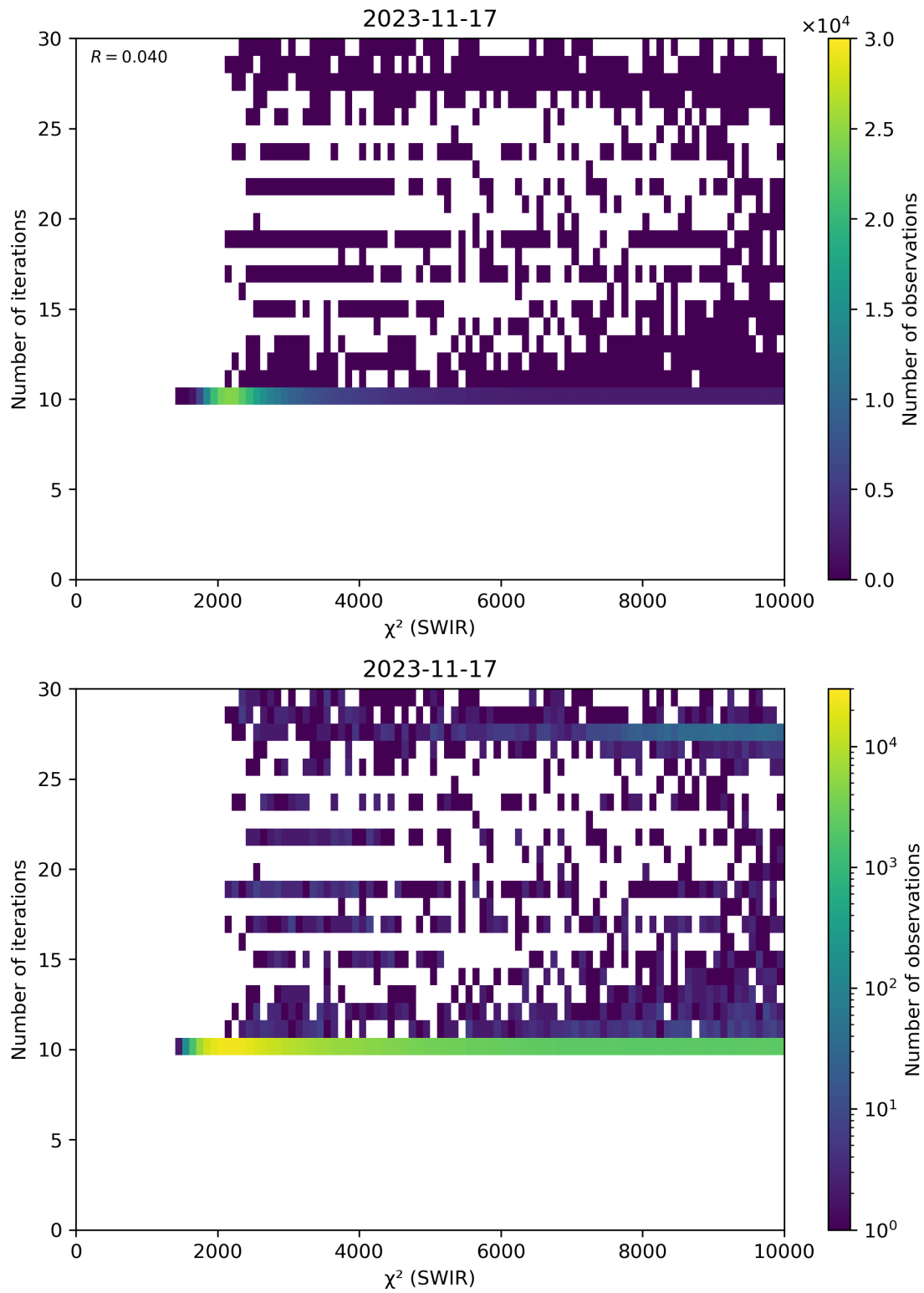
Figure 50: Scatter density plot of “ \chi^2 (SWIR)” against “Number of iterations” for 2023-11-16 to 2023-11-18.
