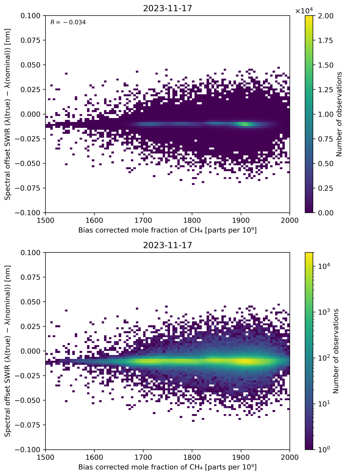
Figure 69: Scatter density plot of “Bias corrected mole fraction of \text{CH}_4 ” against “Spectral offset SWIR ( \lambda(\text{true}) - \lambda(\text{nominal}) )” for 2023-11-16 to 2023-11-18.
