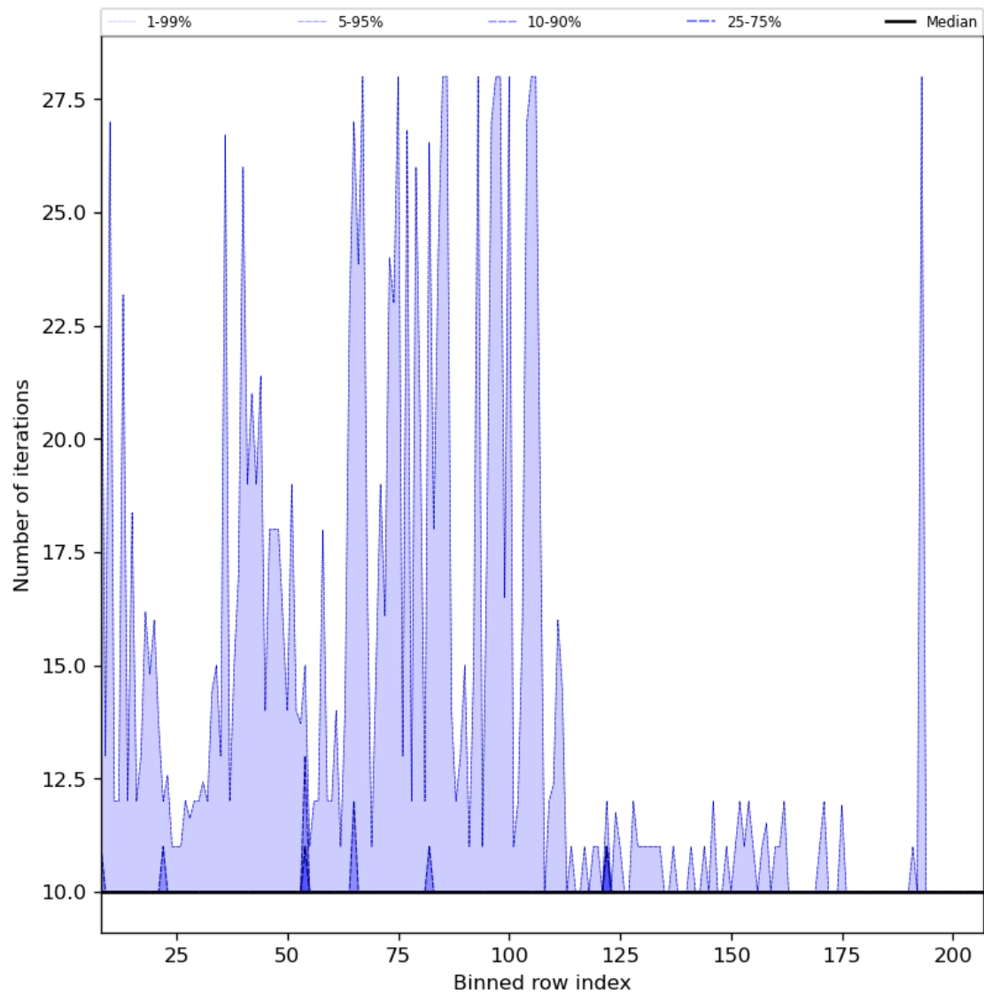
Figure 42: Along track statistics of “Number of iterations” for 2023-11-16 to 2023-11-18
