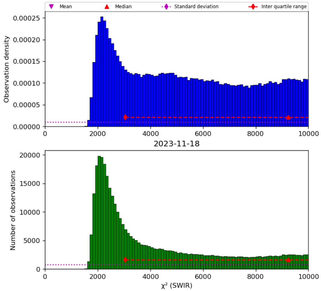
Figure 28: Histogram of “ \chi^2 (SWIR)” for 2023-11-18 to 2023-11-19
