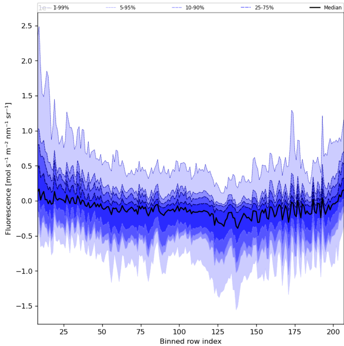
Figure 43: Along track statistics of “Fluorescence” for 2023-11-18 to 2023-11-19
