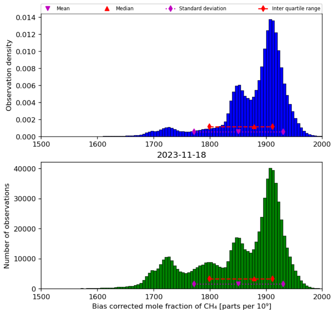
Figure 25: Histogram of “Bias corrected mole fraction of CH 4 ” for 2023-11-18 to 2023-11-19
