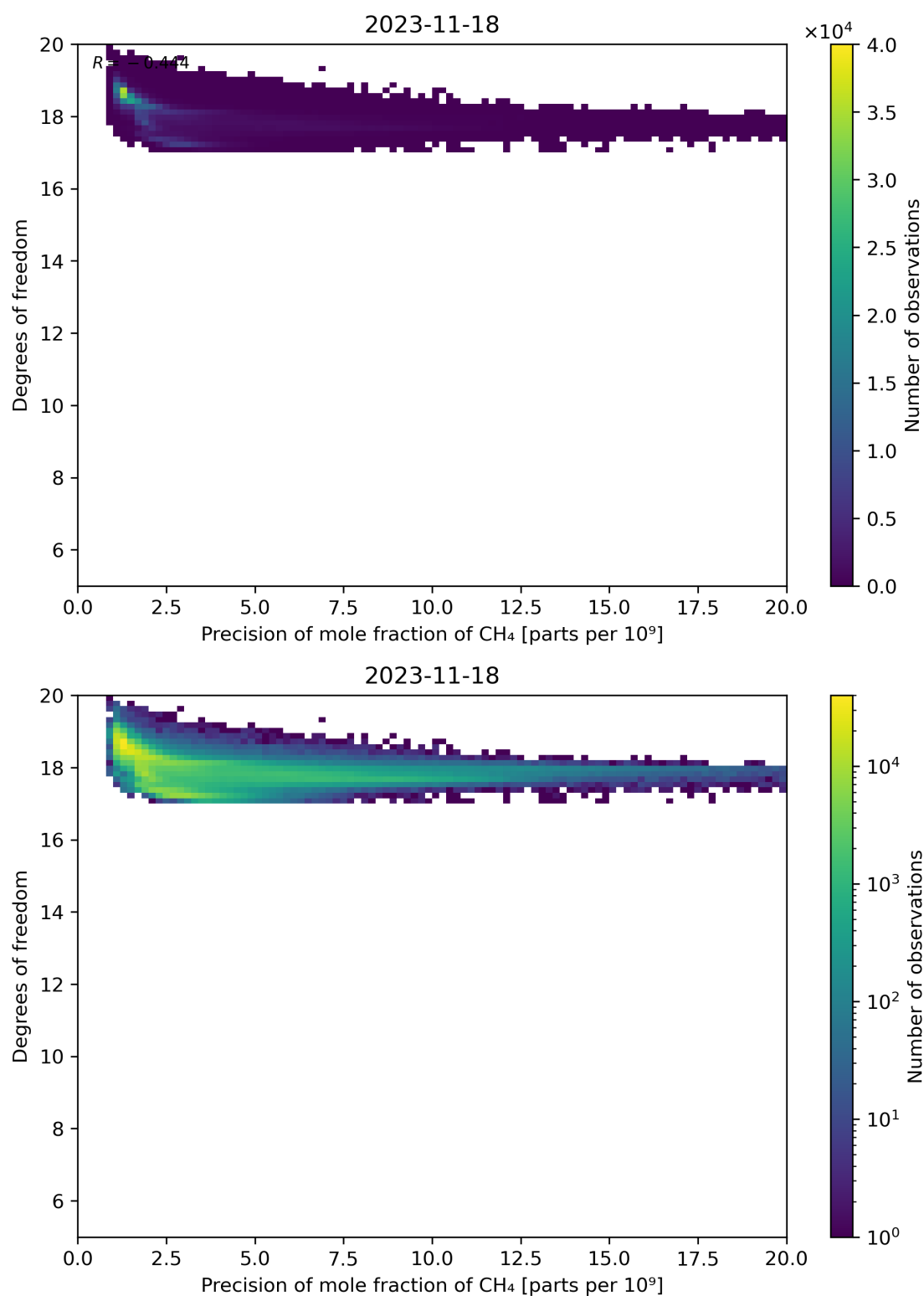
Figure 80: Scatter density plot of “Precision of mole fraction of CH 4 ” against “Degrees of freedom” for 2023-11-18 to 2023-11-19.
