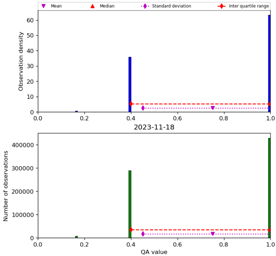
Figure 22: Histogram of “QA value” for 2023-11-18 to 2023-11-19
