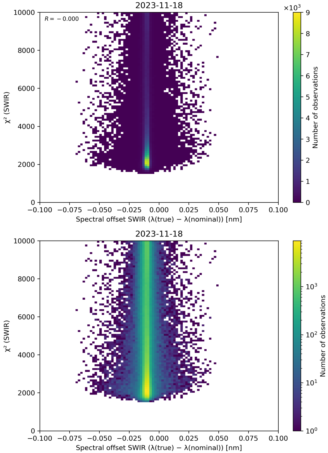
Figure 118: Scatter density plot of “Spectral offset SWIR ( \lambda(\text{true}) - \lambda(\text{nominal}) )” against “ \chi^2 (SWIR)” for 2023-11-18 to 2023-11-19.
