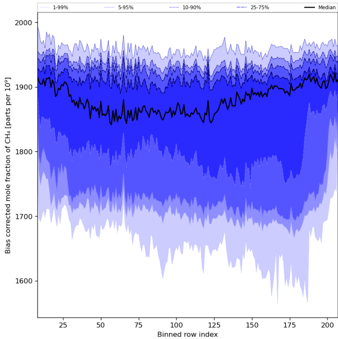
Figure 36: Along track statistics of “Bias corrected mole fraction of CH 4 ” for 2023-11-18 to 2023-11-19
