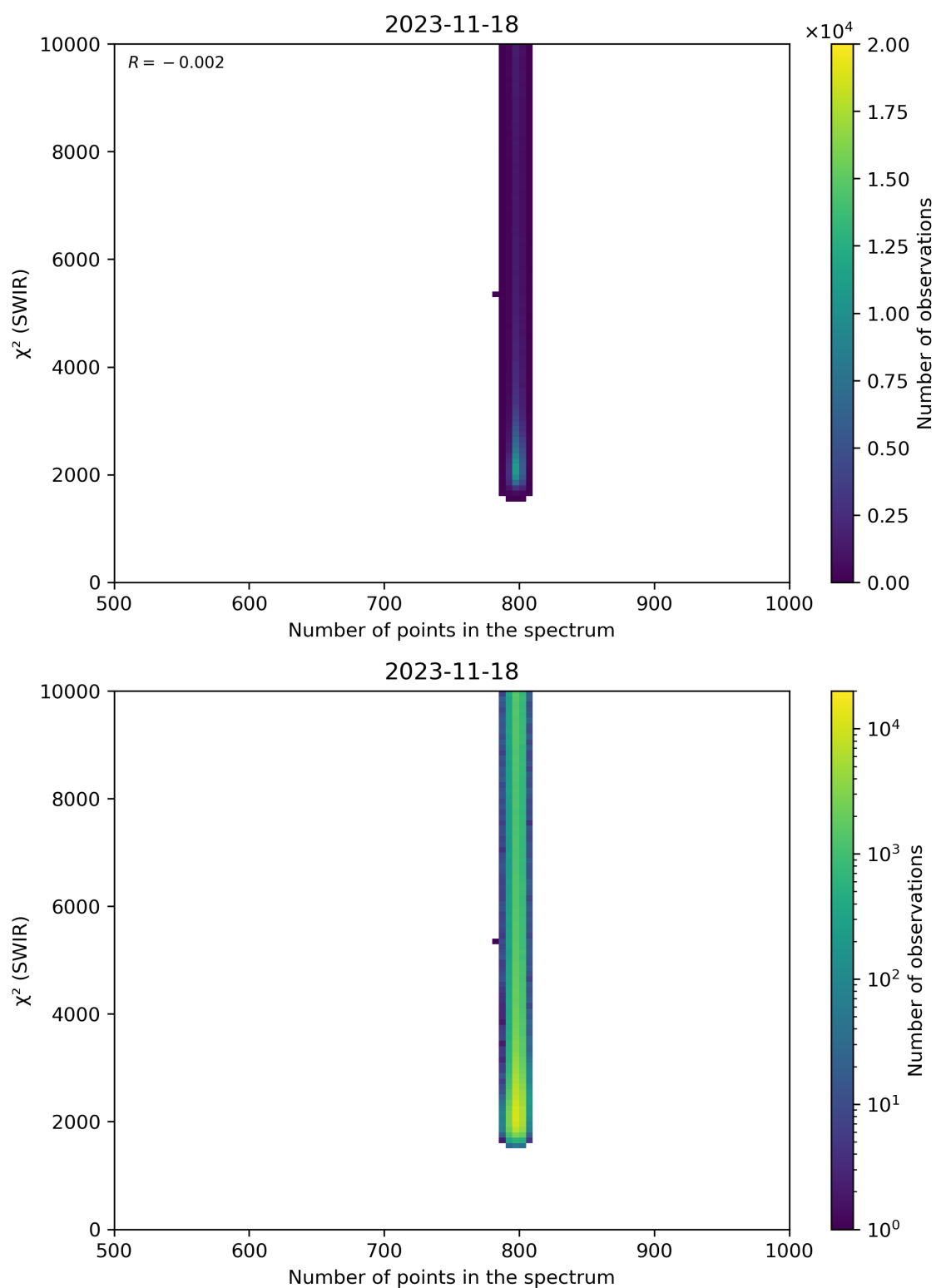
Figure 89: Scatter density plot of “Number of points in the spectrum” against “ \chi^2 (SWIR)” for 2023-11-18 to 2023-11-19.
