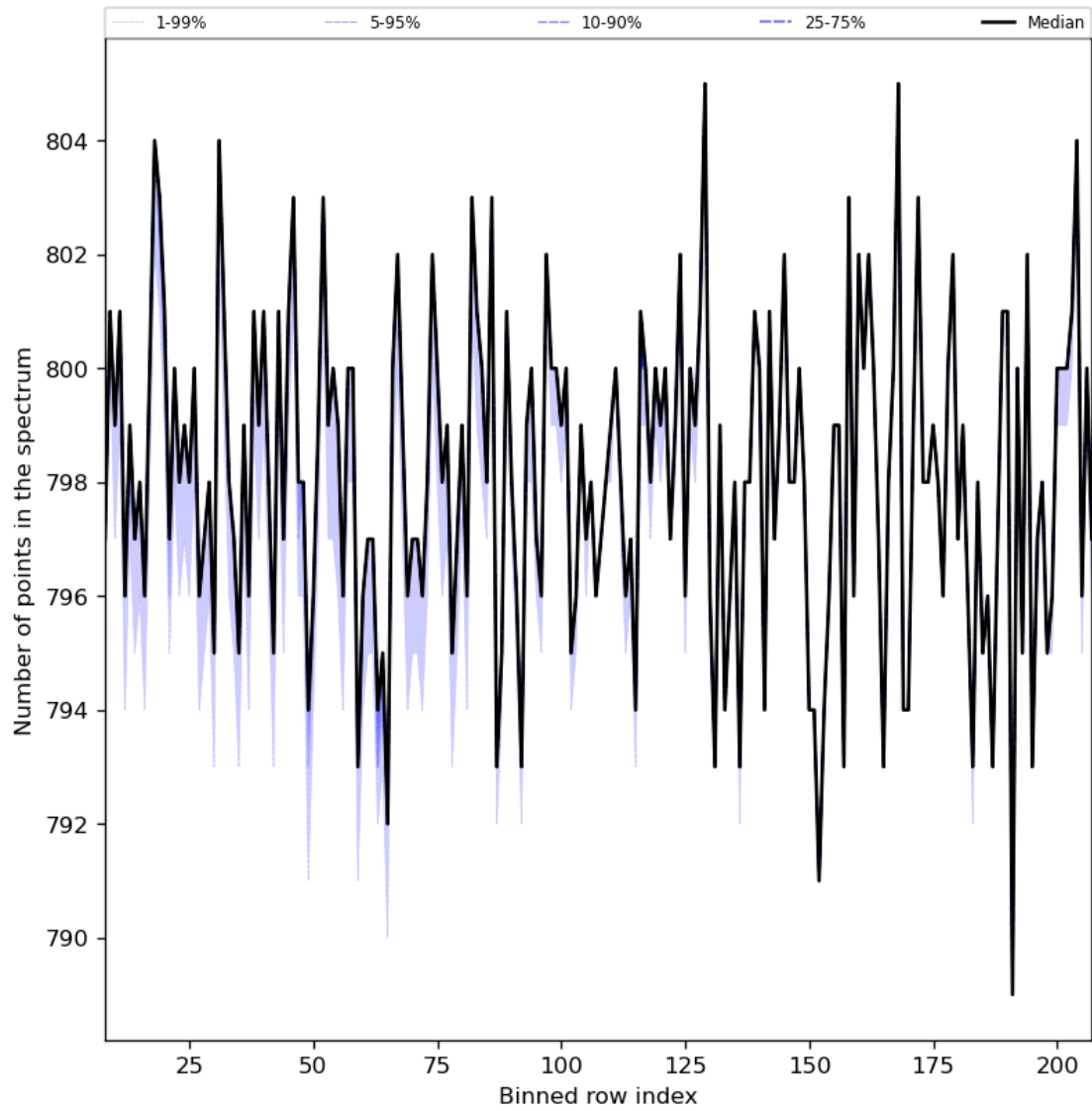
Figure 37: Along track statistics of “Number of points in the spectrum” for 2023-11-18 to 2023-11-19
