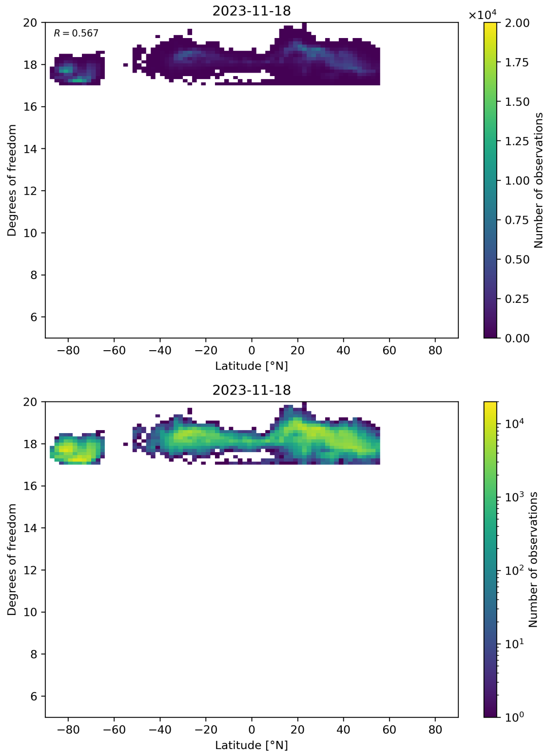
Figure 55: Scatter density plot of “Latitude” against “Degrees of freedom” for 2023-11-18 to 2023-11-19.
