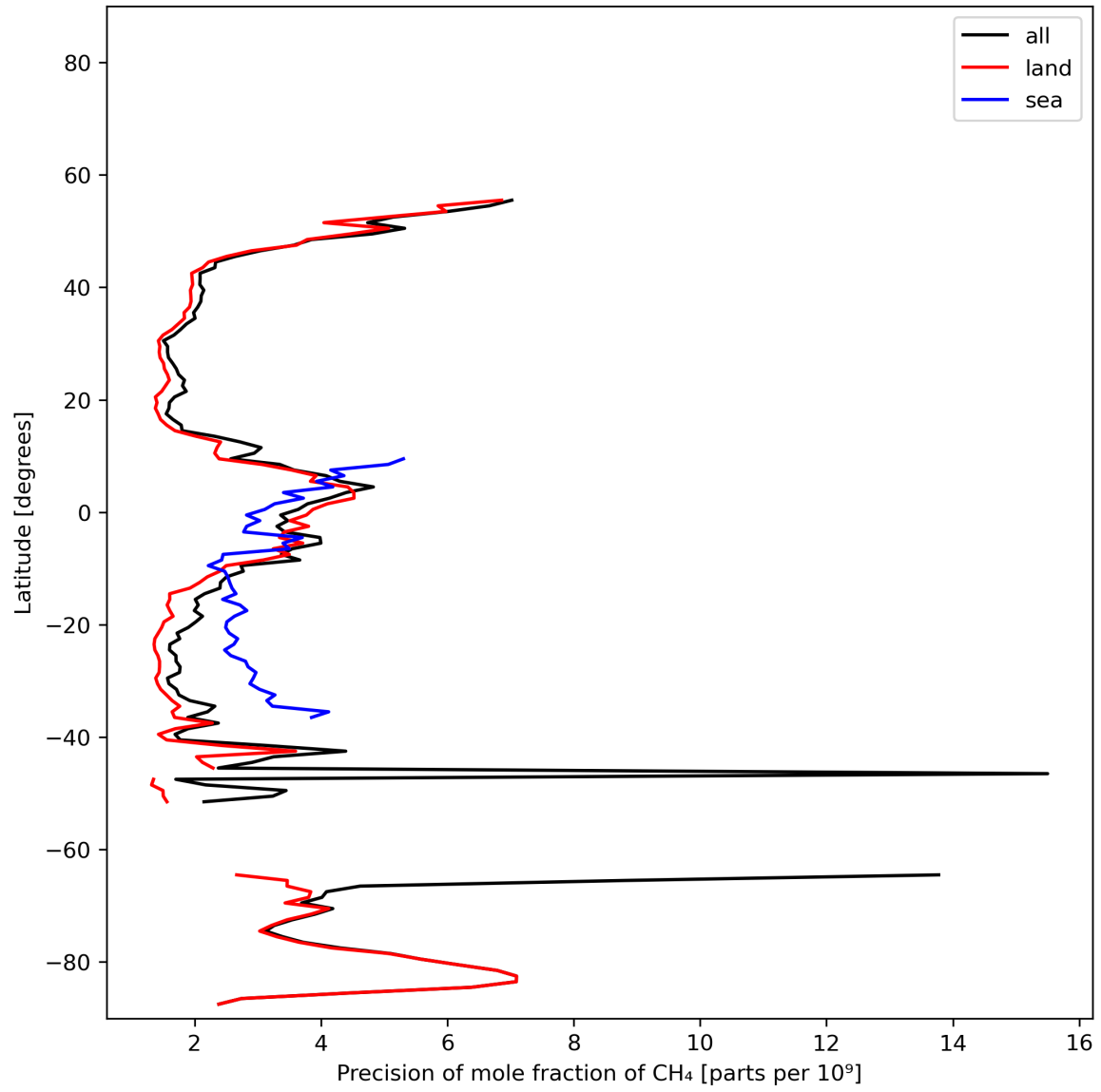
Figure 13: Zonal average of “Precision of mole fraction of \text{CH}_4 ” for 2023-11-18 to 2023-11-19.
