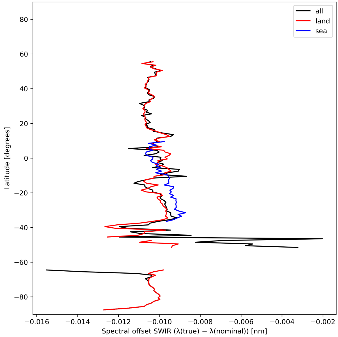
Figure 16: Zonal average of “Spectral offset SWIR ( \lambda(\text{true}) - \lambda(\text{nominal}) )” for 2023-11-18 to 2023-11-19.
