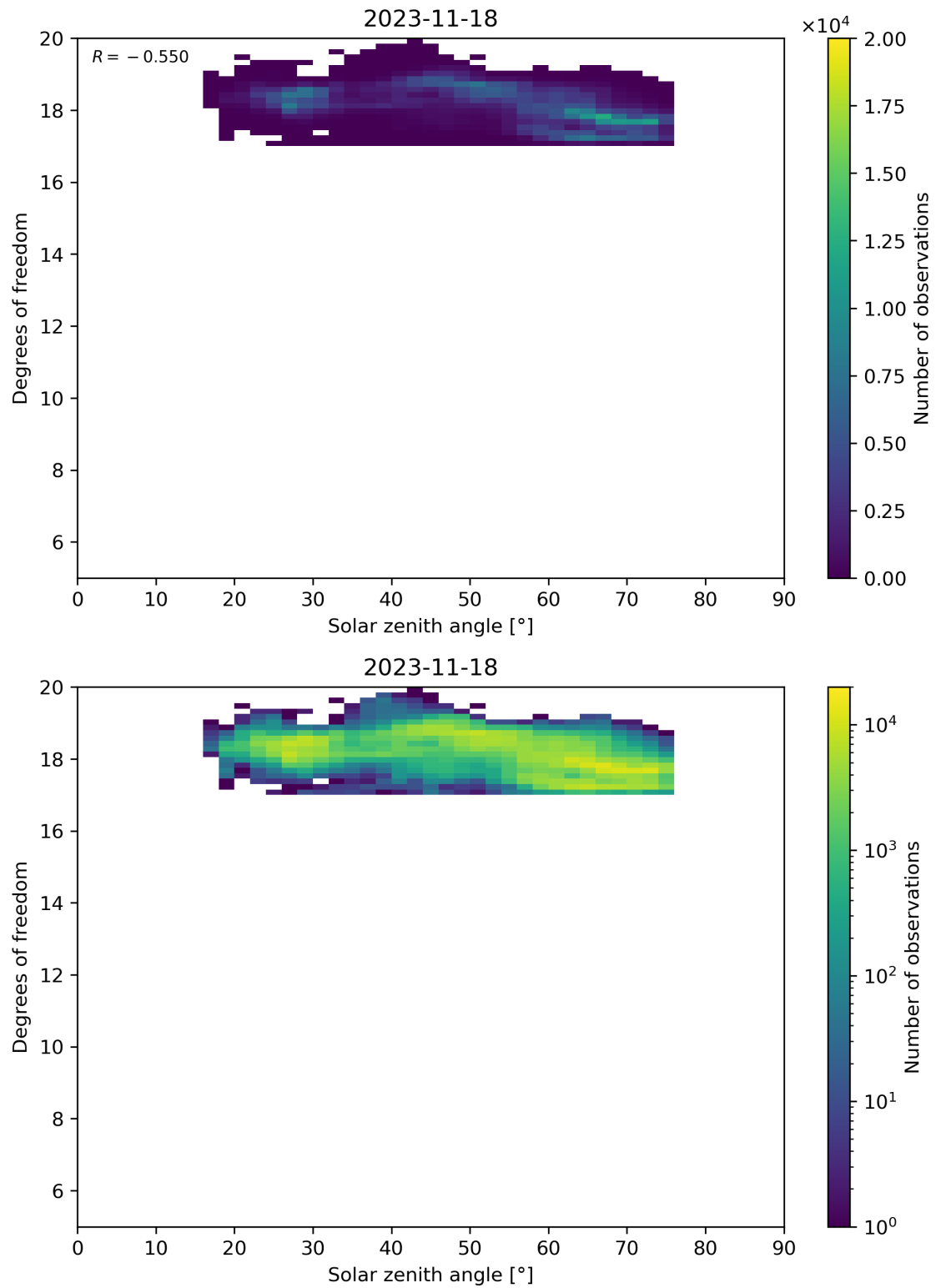
Figure 96: Scatter density plot of “Solar zenith angle” against “Degrees of freedom” for 2023-11-18 to 2023-11-19.
