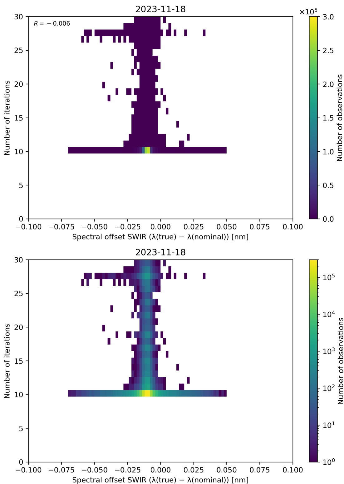
Figure 121: Scatter density plot of “Spectral offset SWIR ( \lambda(\text{true}) - \lambda(\text{nominal}) )” against “Number of iterations” for 2023-11-18 to 2023-11-19.
