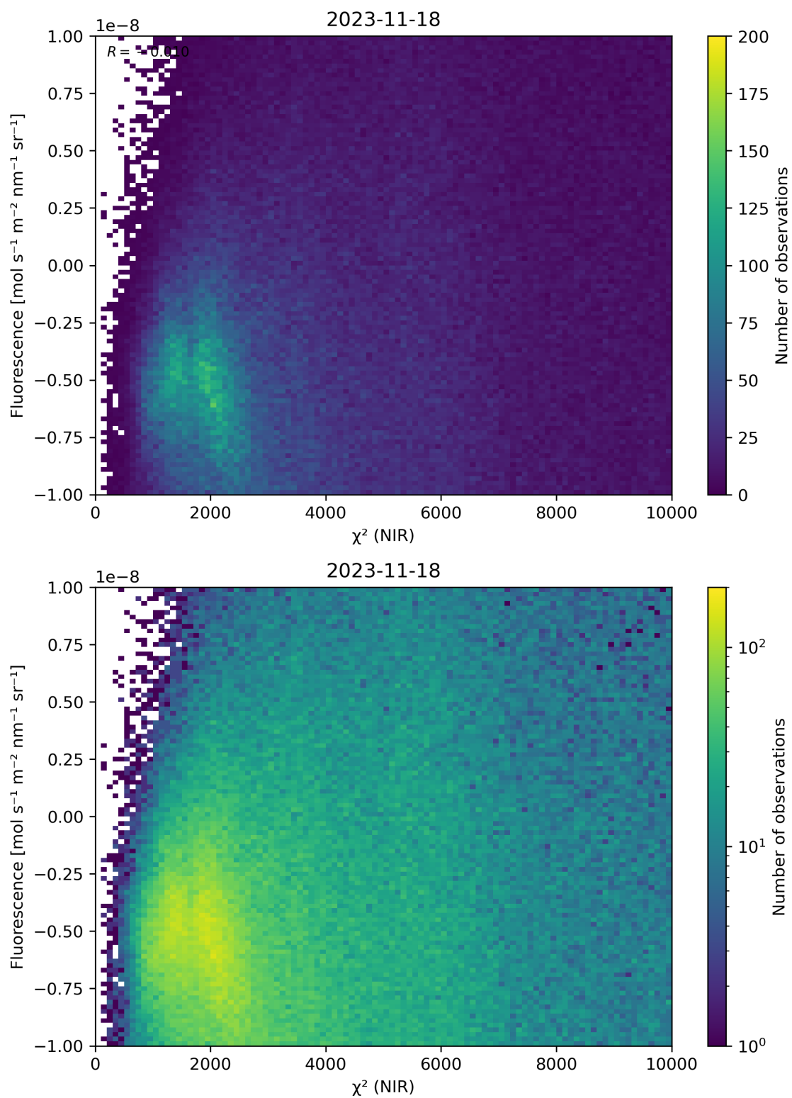
Figure 45: Scatter density plot of “ \chi^2 (NIR)” against “Fluorescence” for 2023-11-18 to 2023-11-19.
