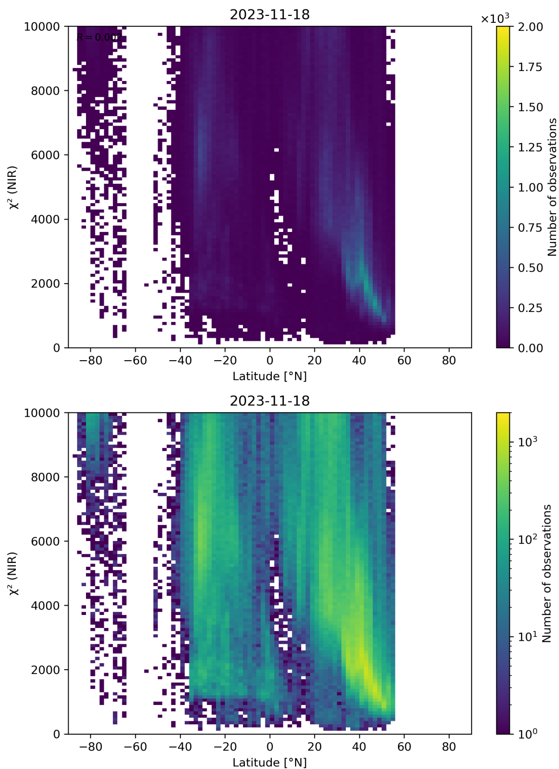
Figure 53: Scatter density plot of “Latitude” against “ \chi^2 (NIR)” for 2023-11-18 to 2023-11-19.
