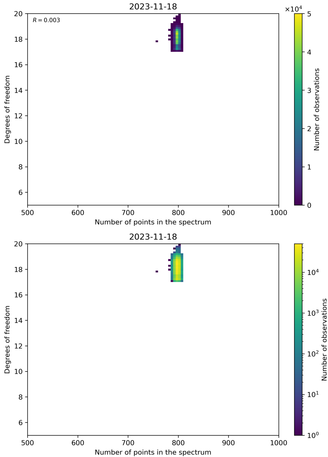
Figure 90: Scatter density plot of “Number of points in the spectrum” against “Degrees of freedom” for 2023-11-18 to 2023-11-19.
