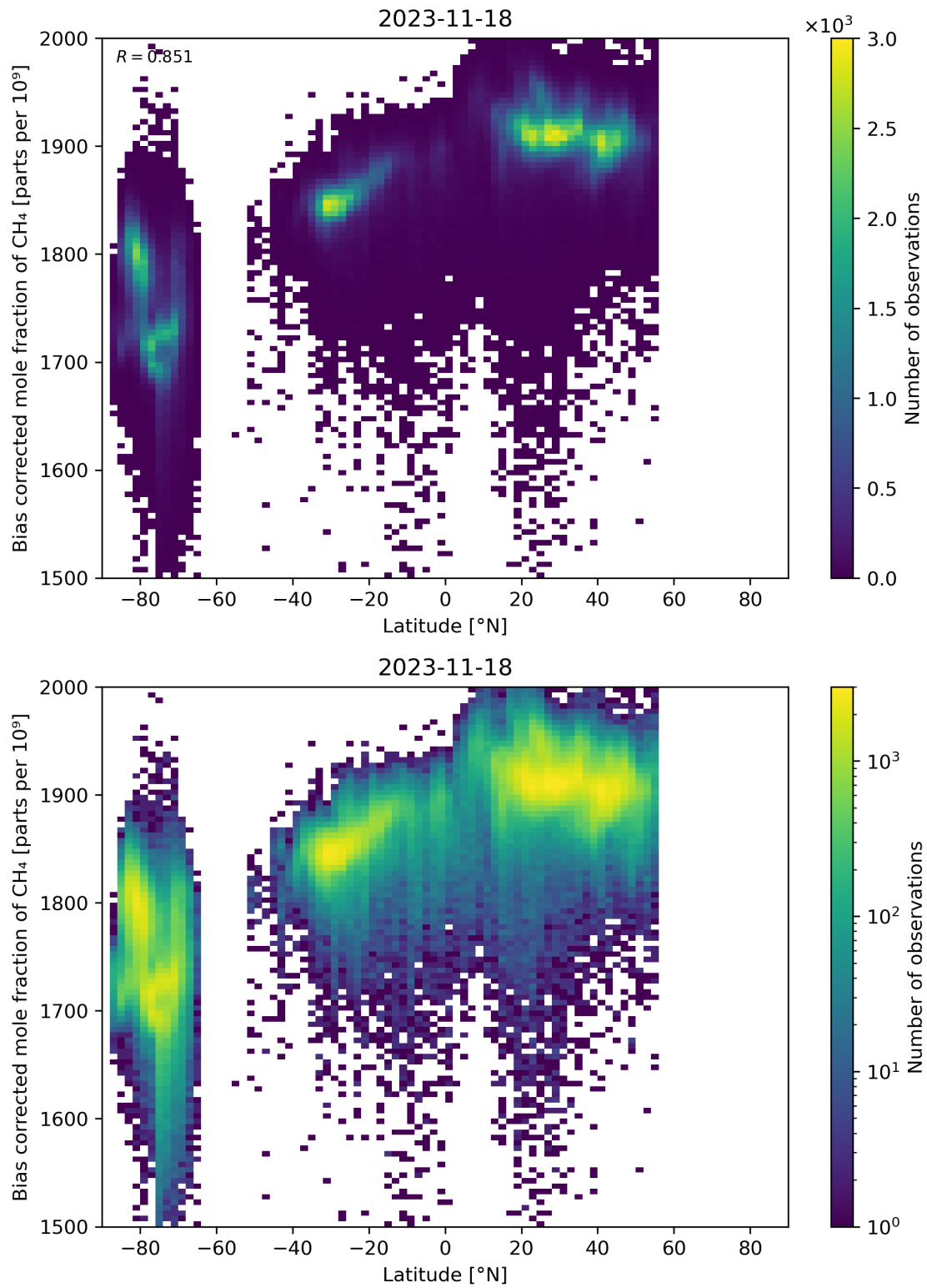
Figure 58: Scatter density plot of “Latitude” against “Bias corrected mole fraction of CH 4 ” for 2023-11-18 to 2023-11-19.
