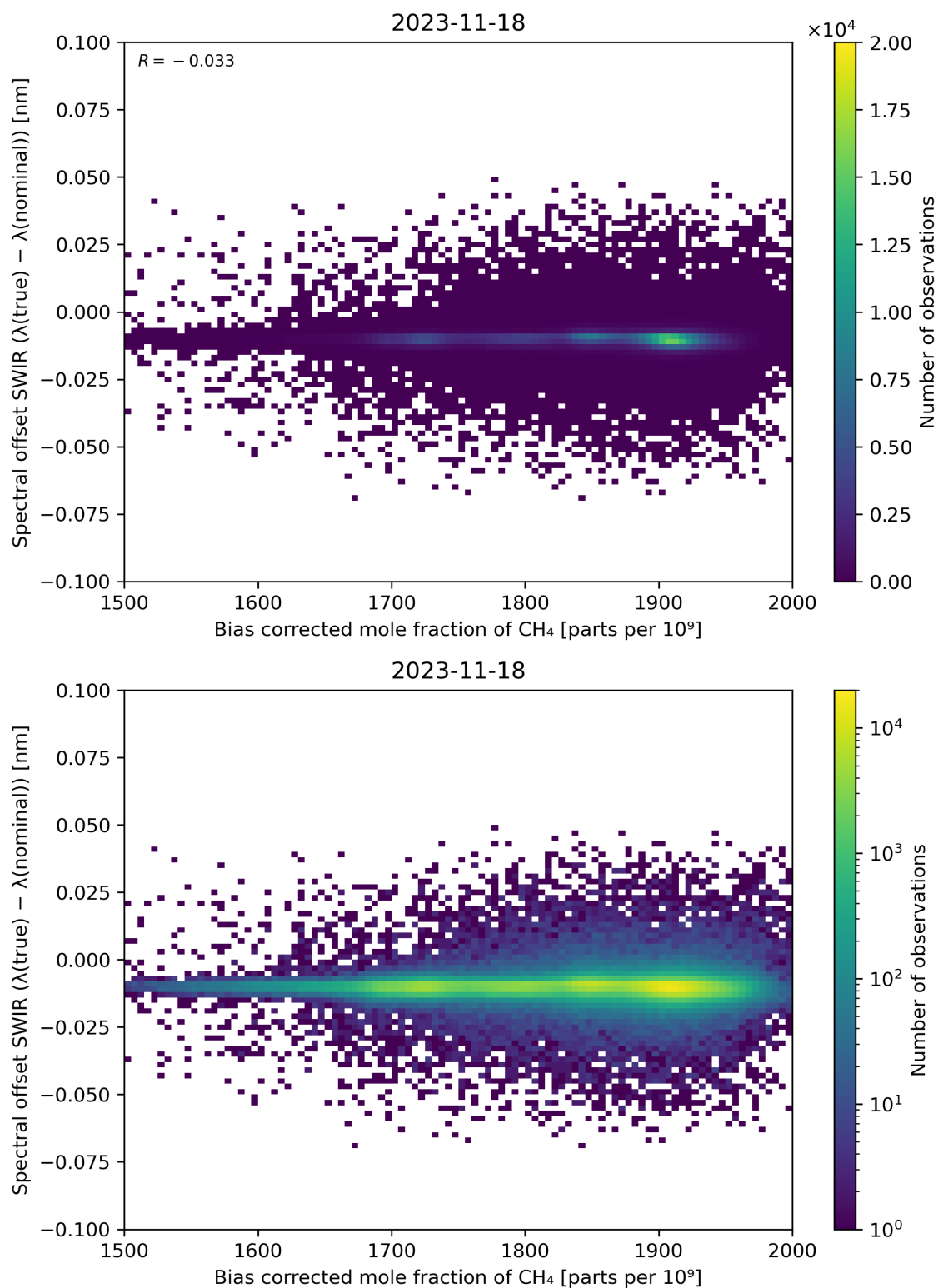
Figure 69: Scatter density plot of “Bias corrected mole fraction of \text{CH}_4 ” against “Spectral offset SWIR ( \lambda(\text{true}) - \lambda(\text{nominal}) )” for 2023-11-18 to 2023-11-19.
