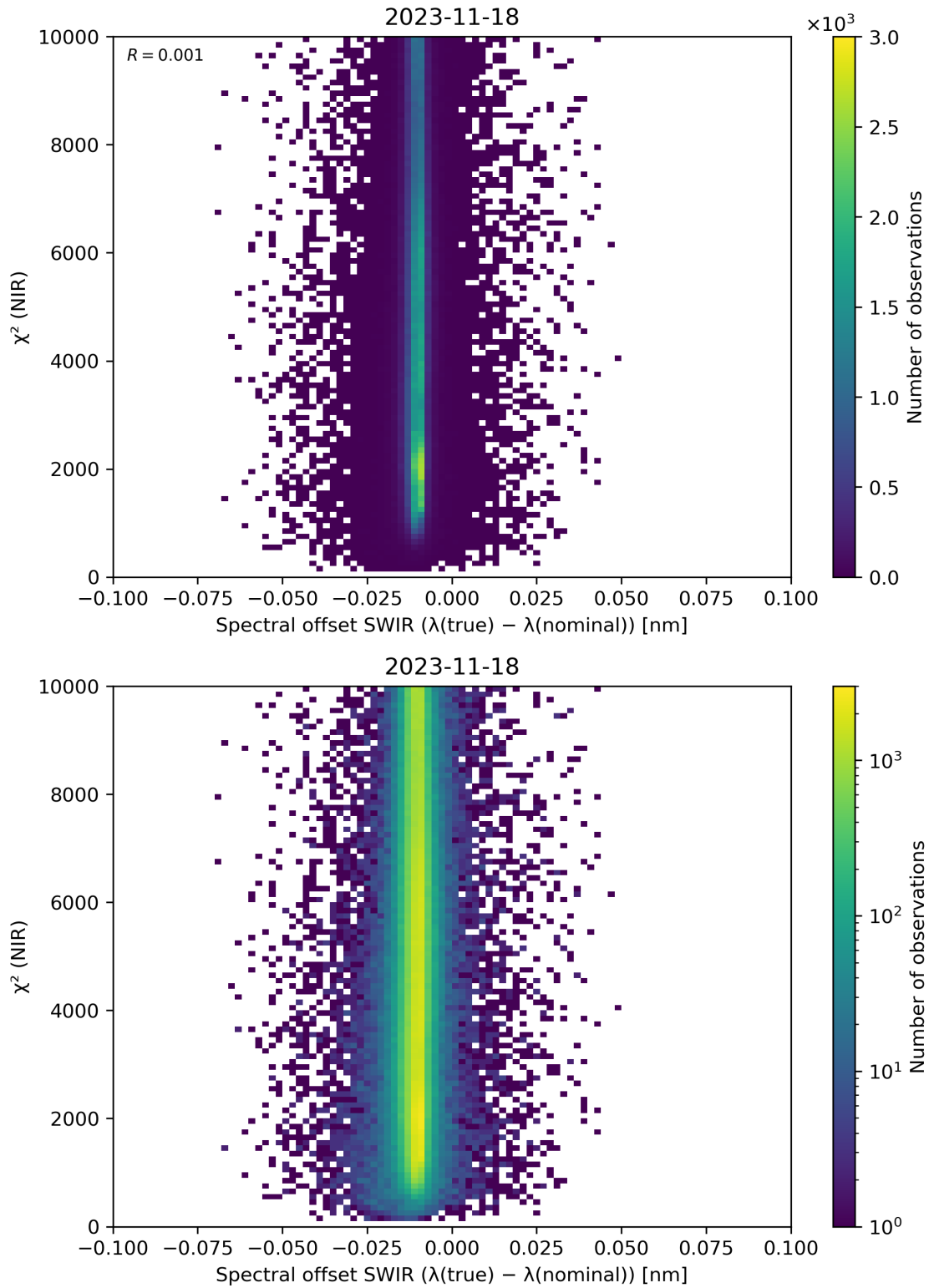
Figure 117: Scatter density plot of “Spectral offset SWIR ( \lambda(\text{true}) - \lambda(\text{nominal}) )” against “ \chi^2 (NIR)” for 2023-11-18 to 2023-11-19.
