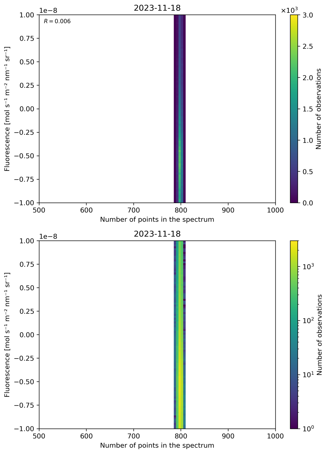
Figure 91: Scatter density plot of “Number of points in the spectrum” against “Fluorescence” for 2023-11-18 to 2023-11-19.
