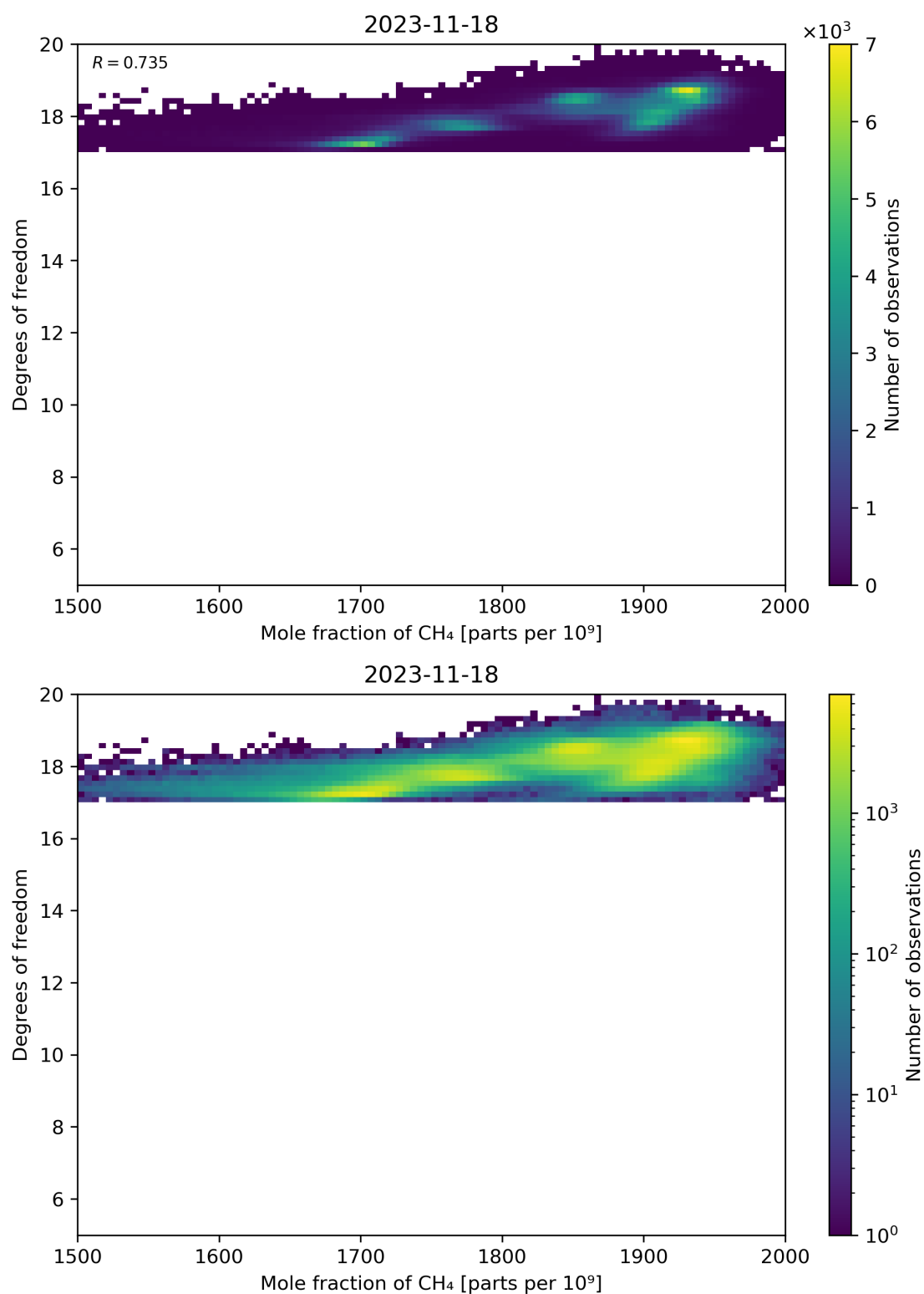
Figure 72: Scatter density plot of “Mole fraction of CH 4 ” against “Degrees of freedom” for 2023-11-18 to 2023-11-19.
