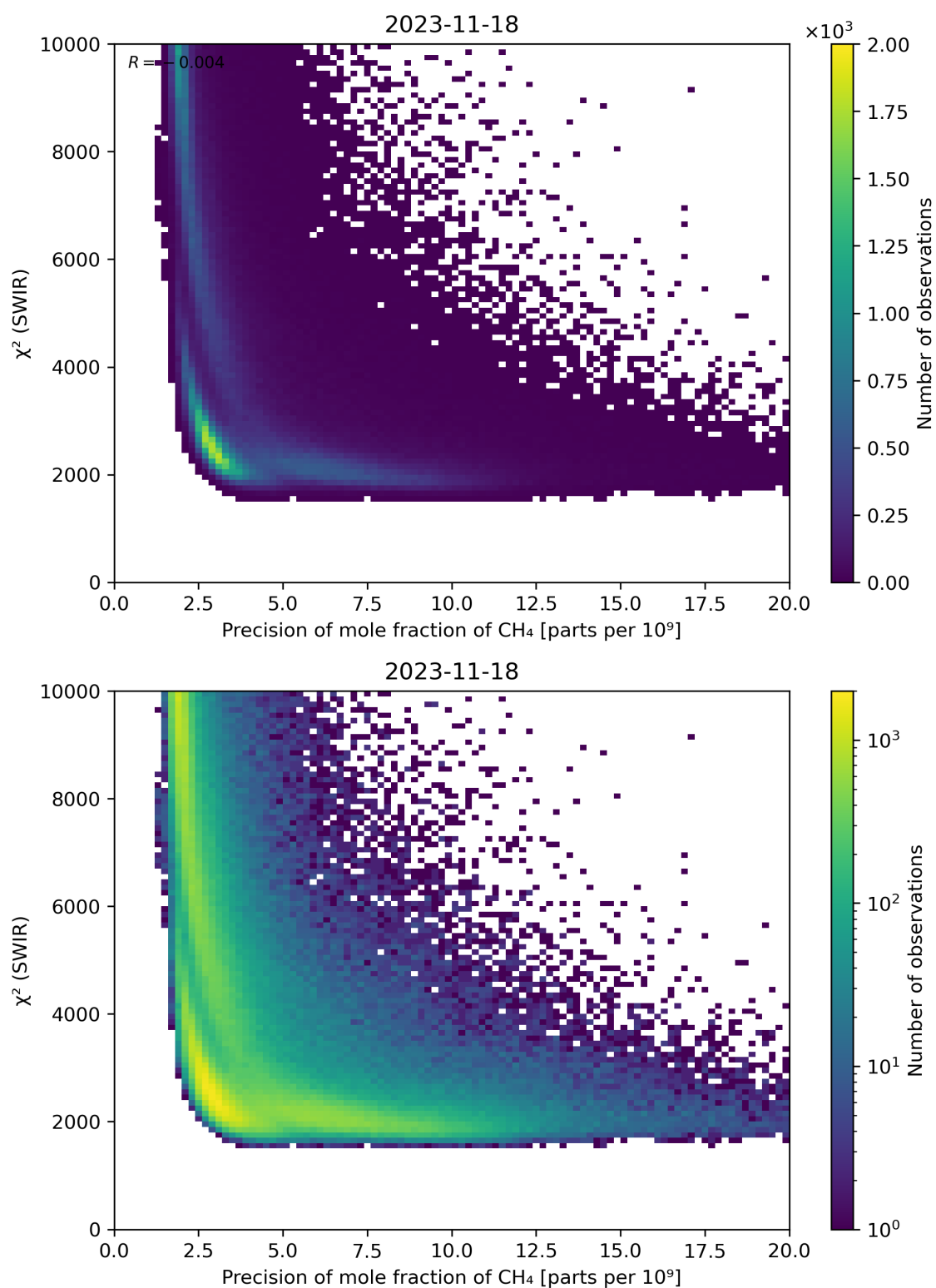
Figure 79: Scatter density plot of “Precision of mole fraction of \text{CH}_4 ” against “ \chi^2 (SWIR)” for 2023-11-18 to 2023-11-19.
