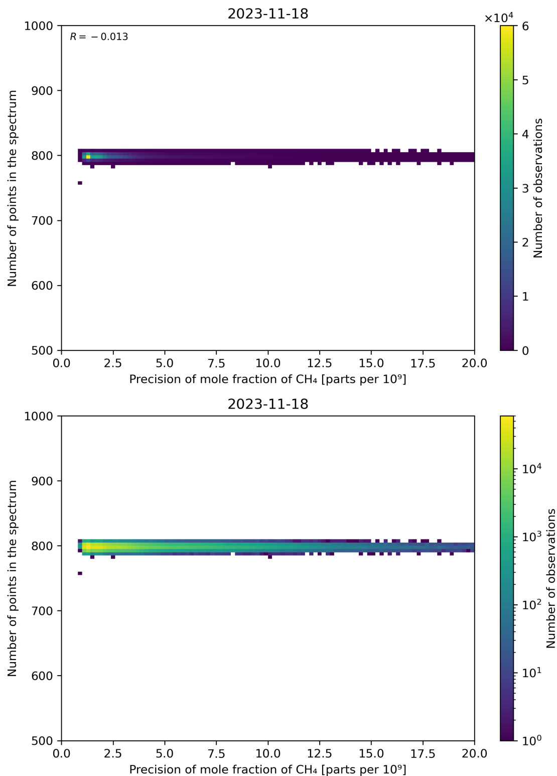
Figure 84: Scatter density plot of “Precision of mole fraction of CH 4 ” against “Number of points in the spectrum” for 2023-11-18 to 2023-11-19.
