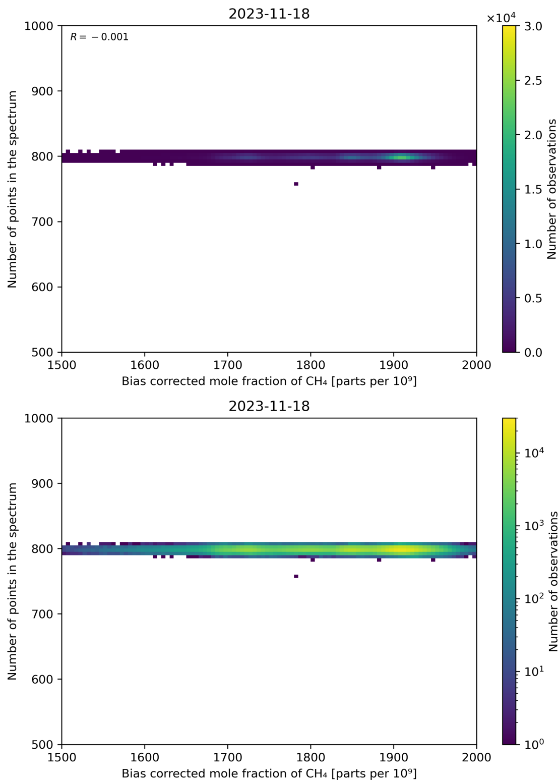
Figure 68: Scatter density plot of “Bias corrected mole fraction of CH 4 ” against “Number of points in the spectrum” for 2023-11-18 to 2023-11-19.
