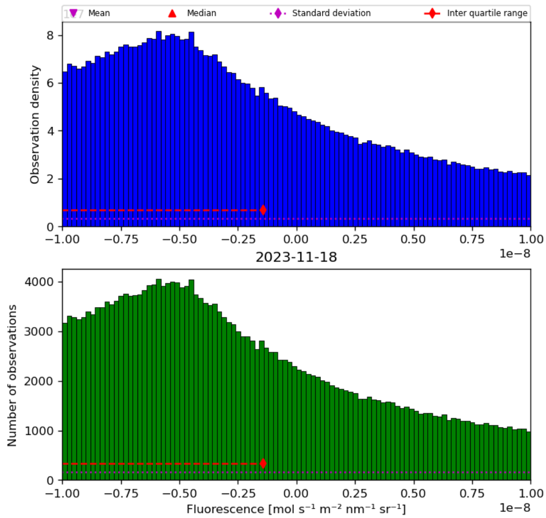
Figure 32: Histogram of “Fluorescence” for 2023-11-18 to 2023-11-19
