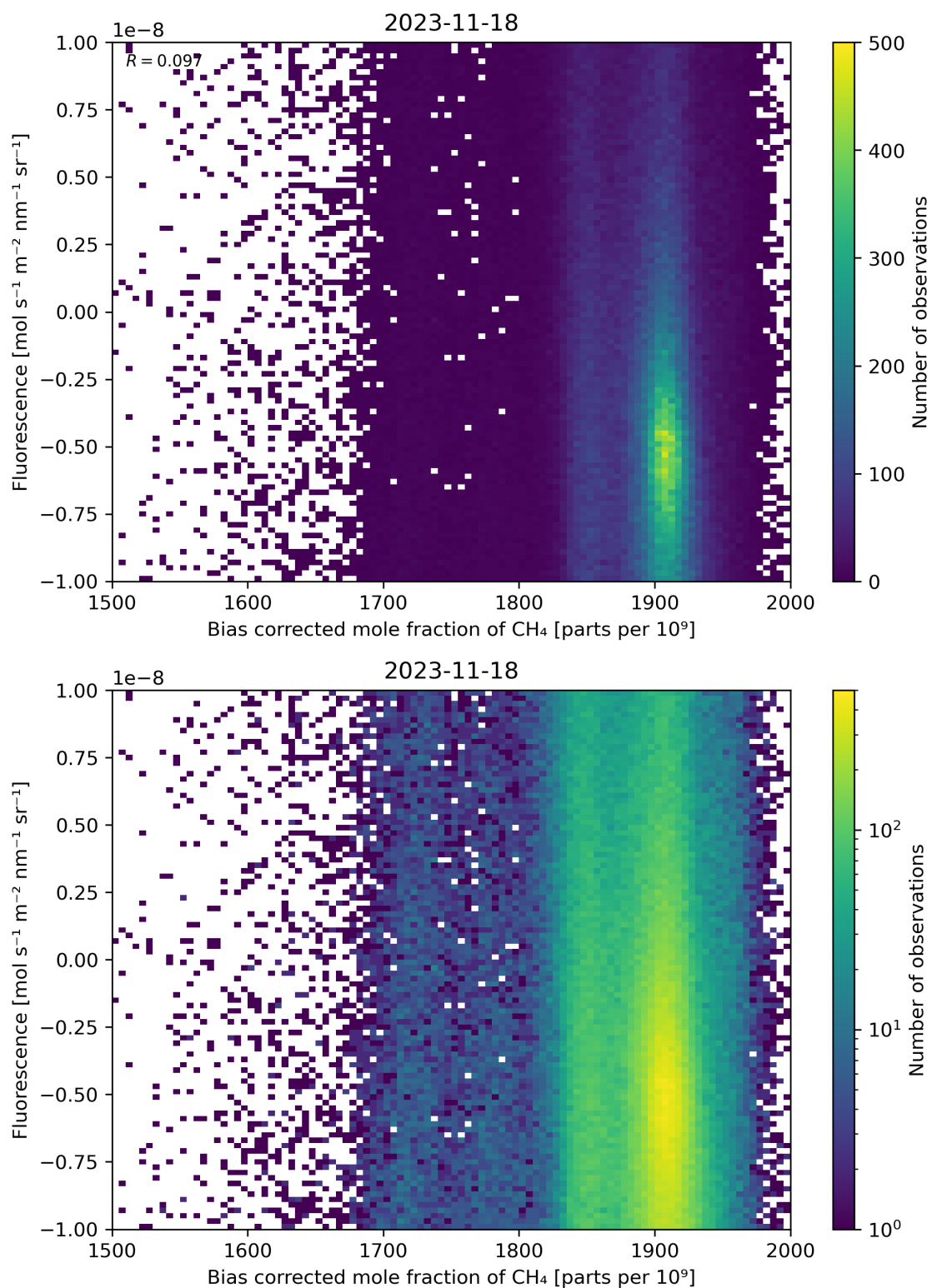
Figure 66: Scatter density plot of “Bias corrected mole fraction of CH 4 ” against “Fluorescence” for 2023-11-18 to 2023-11-19.
