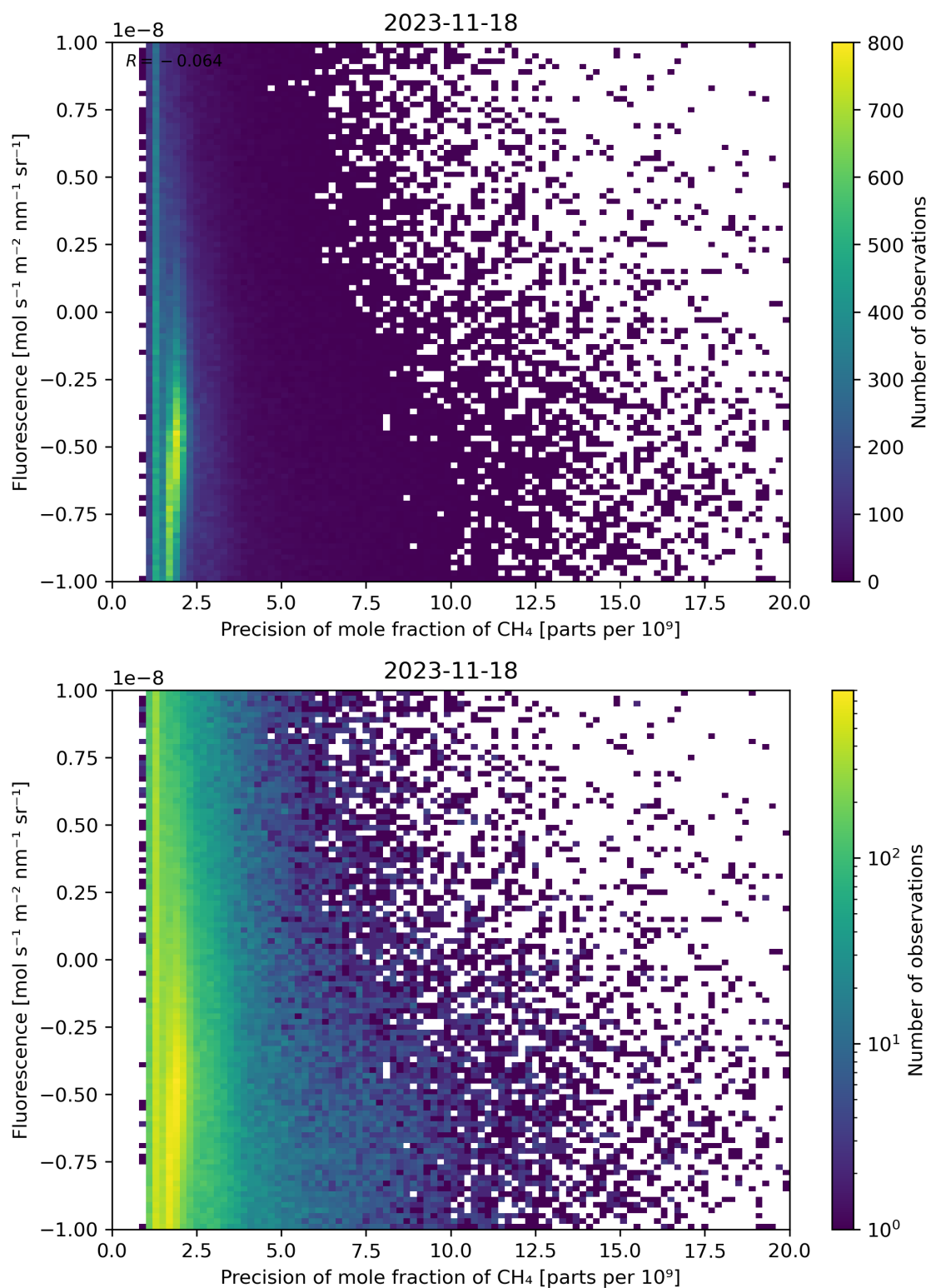
Figure 81: Scatter density plot of “Precision of mole fraction of CH 4 ” against “Fluorescence” for 2023-11-18 to 2023-11-19.
