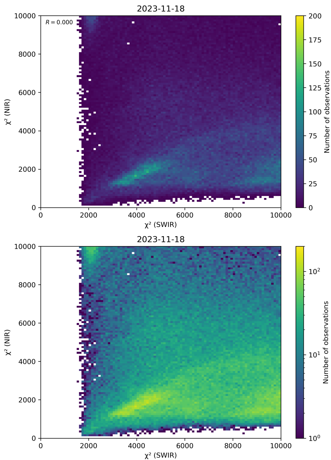
Figure 47: Scatter density plot of “ \chi^2 (SWIR)” against “ \chi^2 (NIR)” for 2023-11-18 to 2023-11-19.
