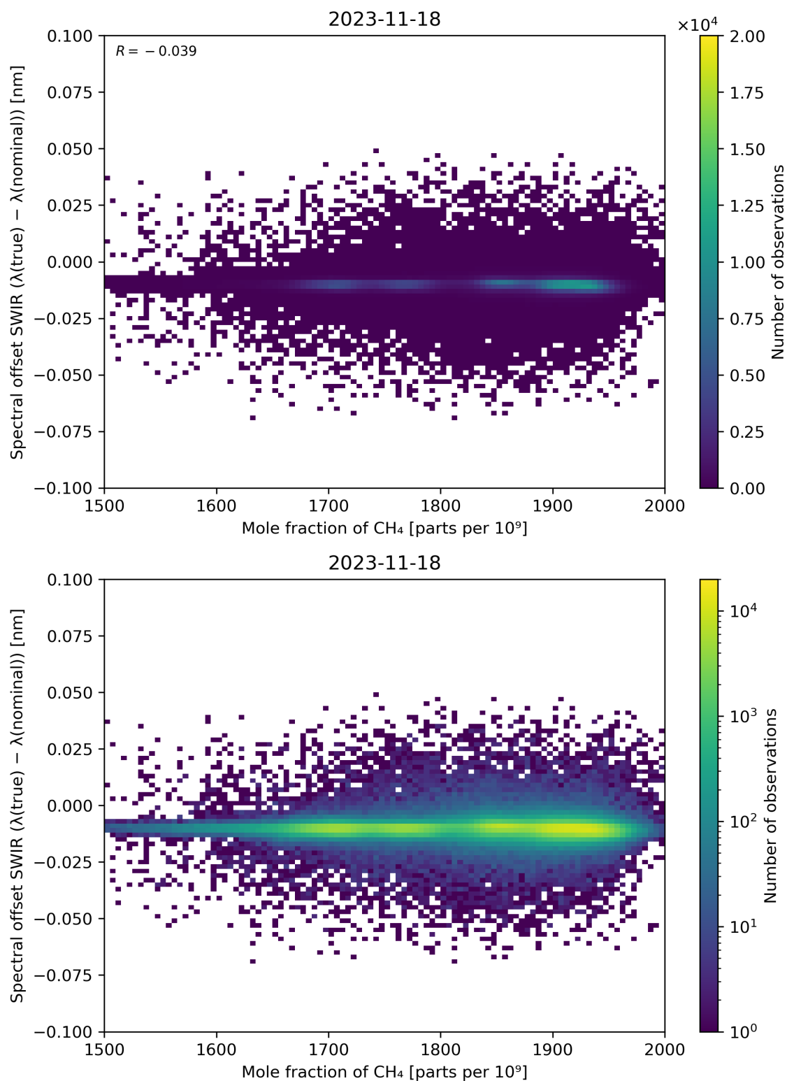
Figure 86: Scatter density plot of “Mole fraction of CH 4 ” against “Spectral offset SWIR ( \lambda(\text{true}) - \lambda(\text{nominal}) )” for 2023-11-18 to 2023-11-19.
