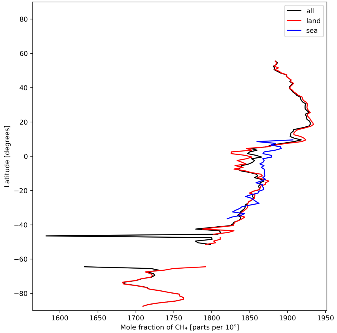
Figure 12: Zonal average of “Mole fraction of \text{CH}_4 ” for 2023-11-18 to 2023-11-19.
