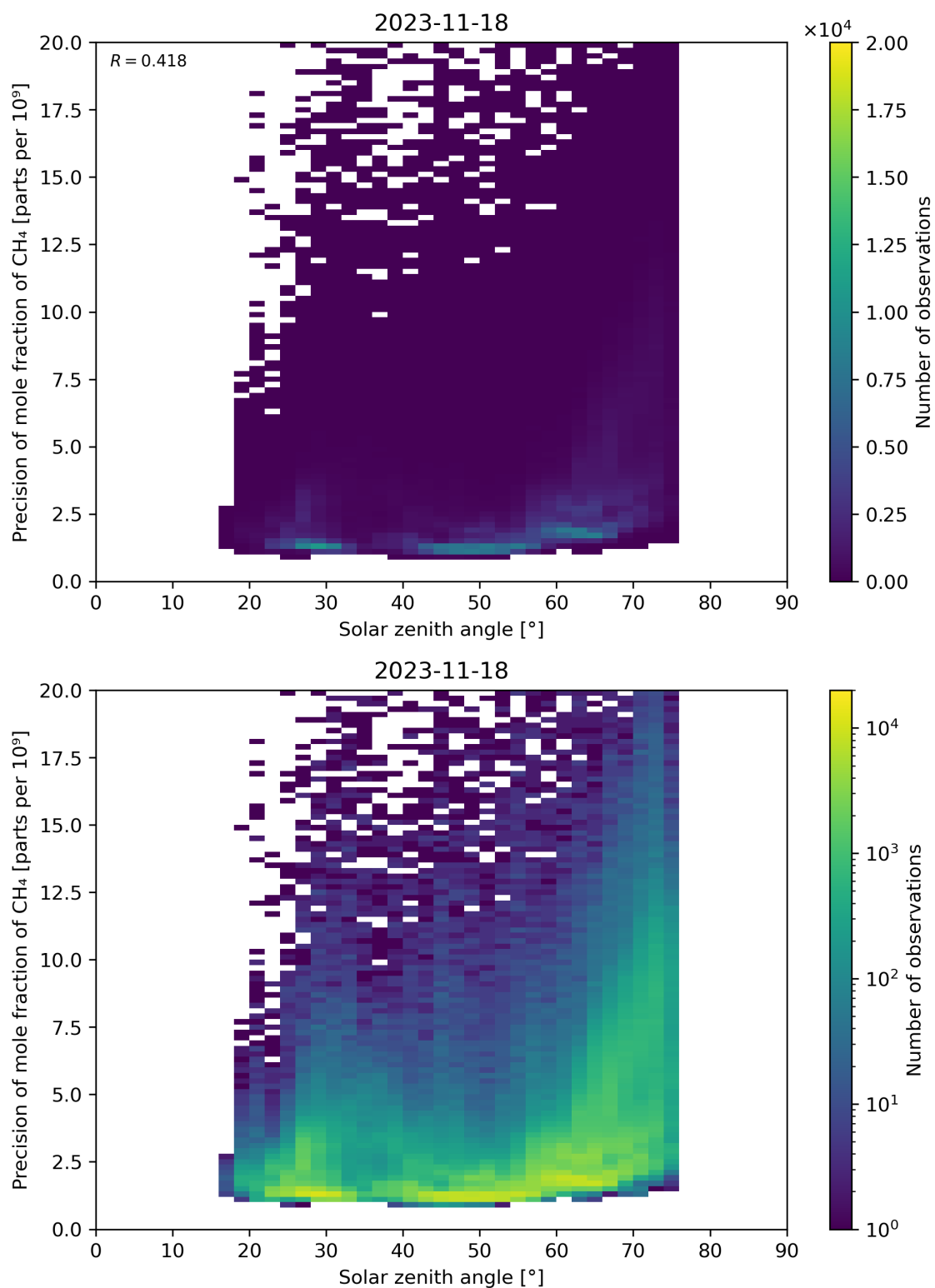
Figure 101: Scatter density plot of “Solar zenith angle” against “Precision of mole fraction of CH 4 ” for 2023-11-18 to 2023-11-19.
