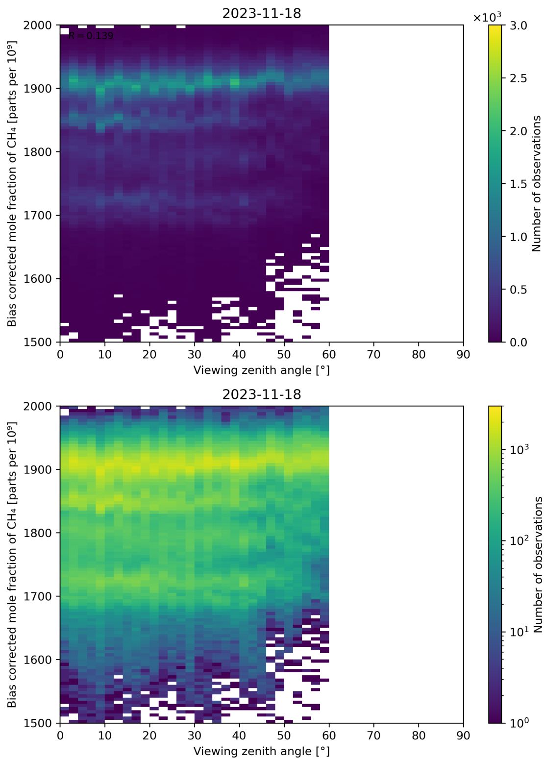
Figure 111: Scatter density plot of “Viewing zenith angle” against “Bias corrected mole fraction of CH 4 ” for 2023-11-18 to 2023-11-19.
