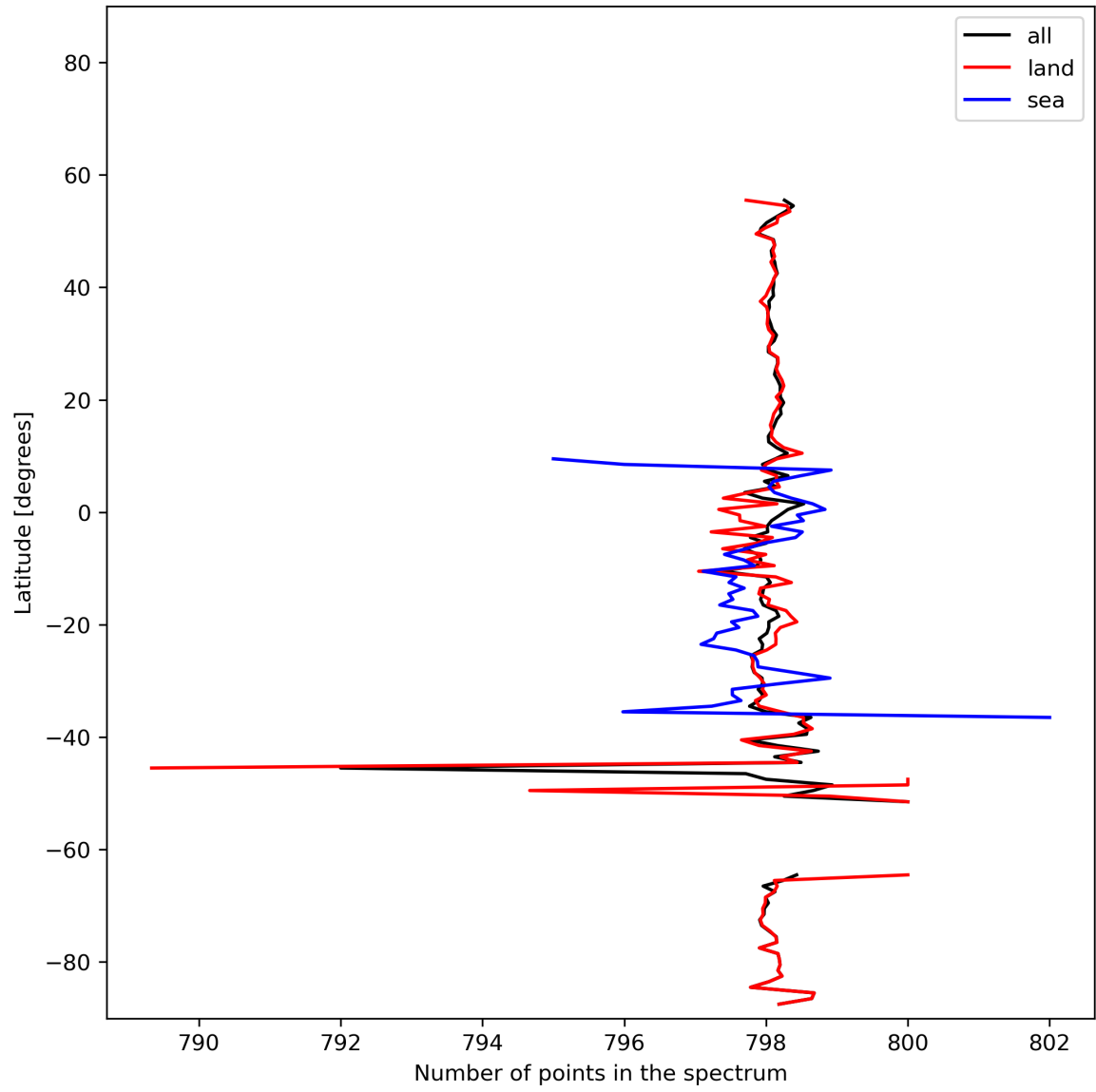
Figure 15: Zonal average of “Number of points in the spectrum” for 2023-11-18 to 2023-11-19.
