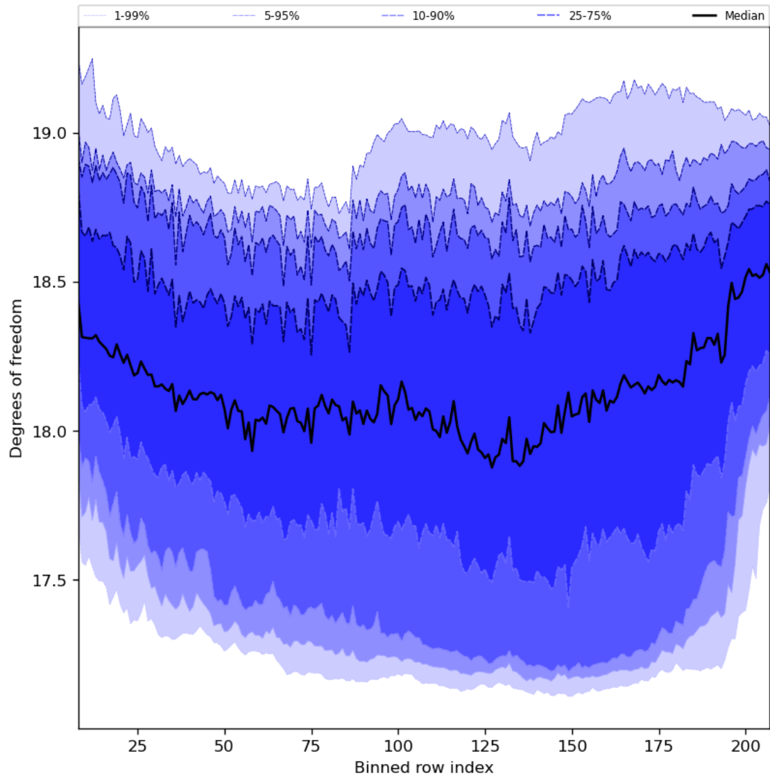
Figure 41: Along track statistics of “Degrees of freedom” for 2023-11-18 to 2023-11-19
