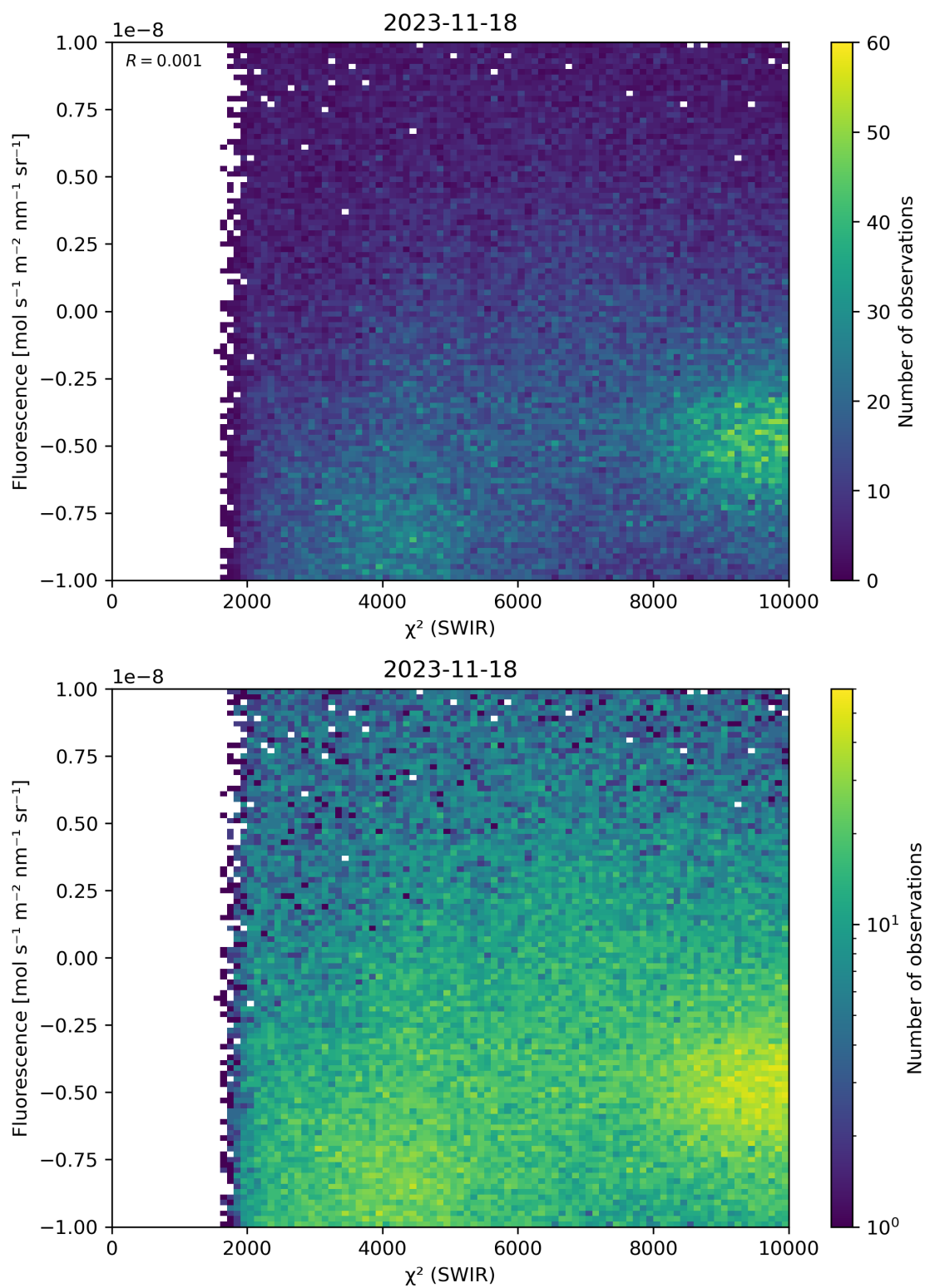
Figure 49: Scatter density plot of “ \chi^2 (SWIR)” against “Fluorescence” for 2023-11-18 to 2023-11-19.
