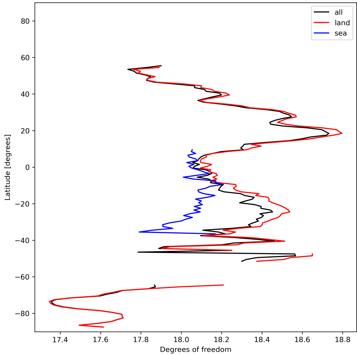
Figure 19: Zonal average of “Degrees of freedom” for 2023-11-18 to 2023-11-19.
