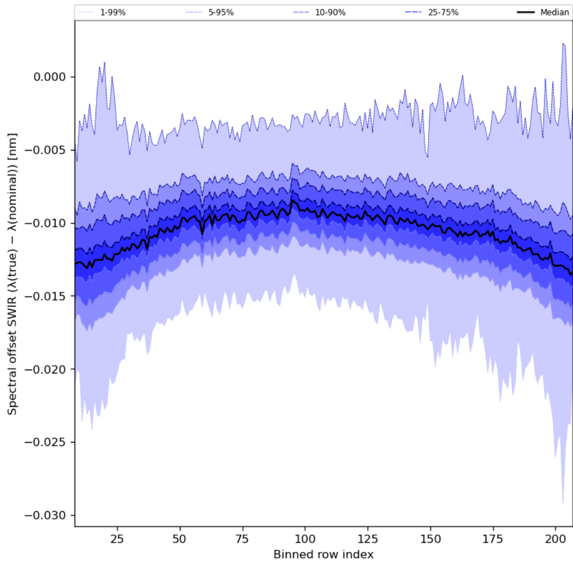
Figure 38: Along track statistics of “Spectral offset SWIR ( \lambda(\text{true}) - \lambda(\text{nominal}) )” for 2023-11-18 to 2023-11-19
