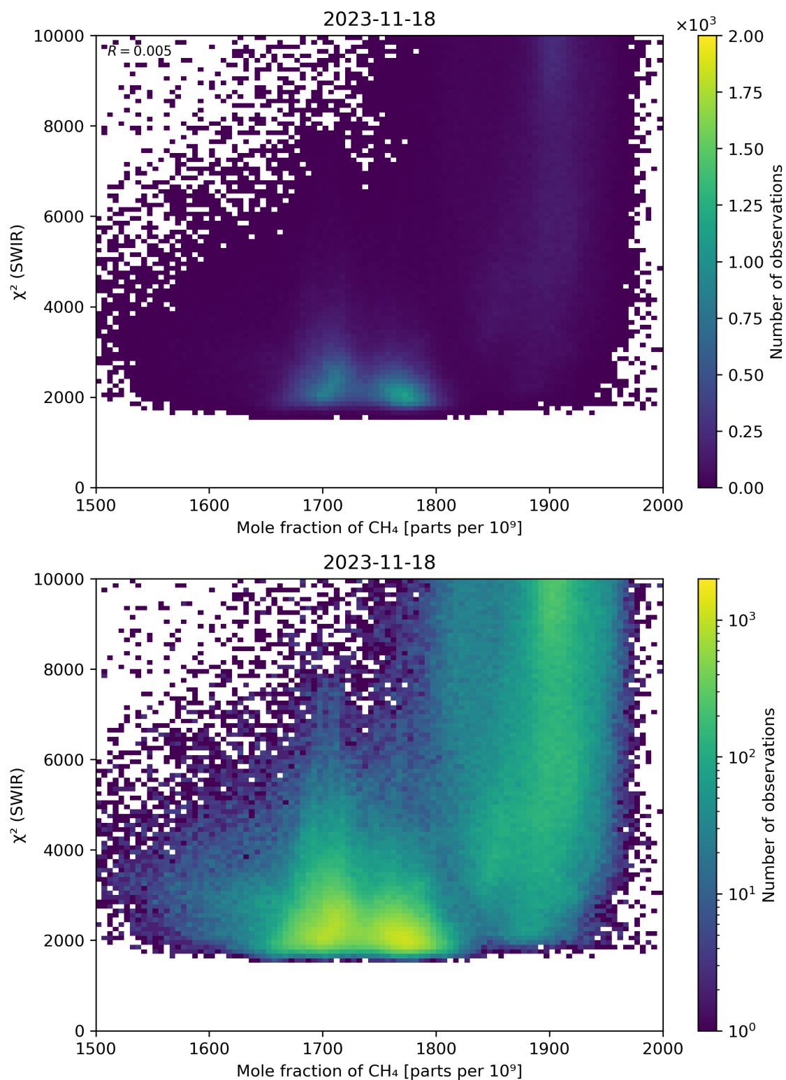
Figure 71: Scatter density plot of “Mole fraction of \text{CH}_4 ” against “ \chi^2 (SWIR)” for 2023-11-18 to 2023-11-19.
