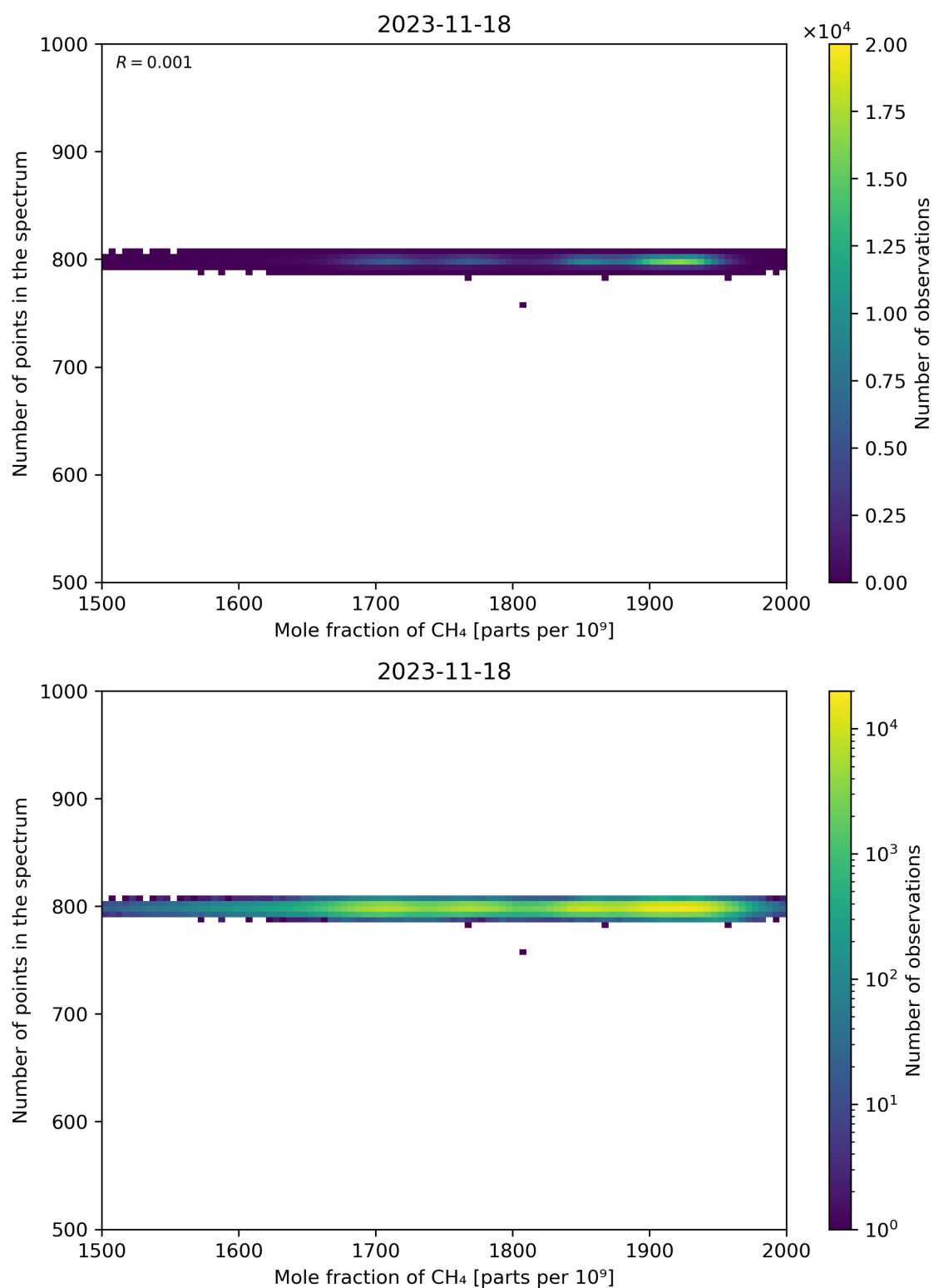
Figure 77: Scatter density plot of “Mole fraction of CH 4 ” against “Number of points in the spectrum” for 2023-11-18 to 2023-11-19.
