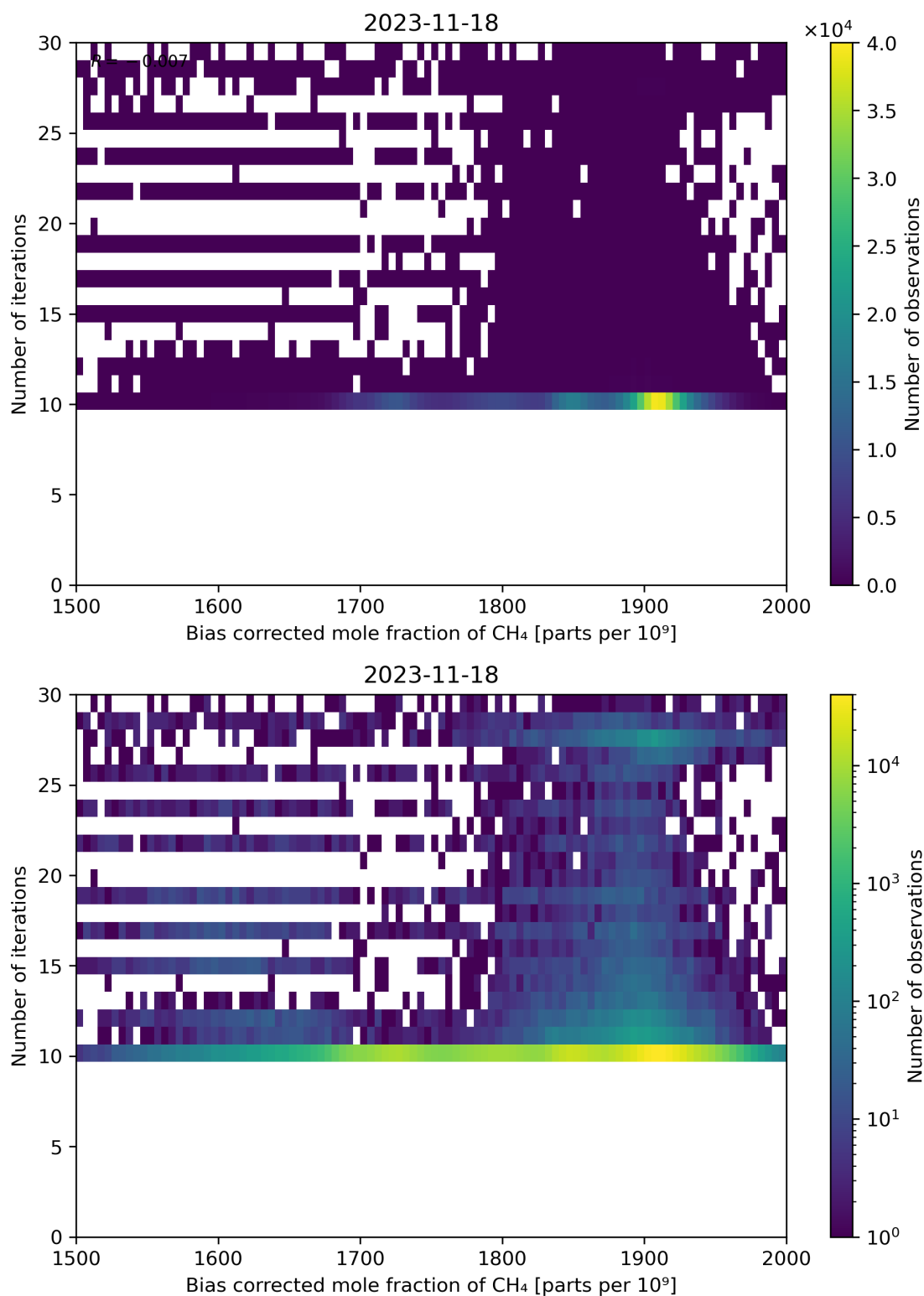
Figure 67: Scatter density plot of “Bias corrected mole fraction of CH 4 ” against “Number of iterations” for 2023-11-18 to 2023-11-19.
