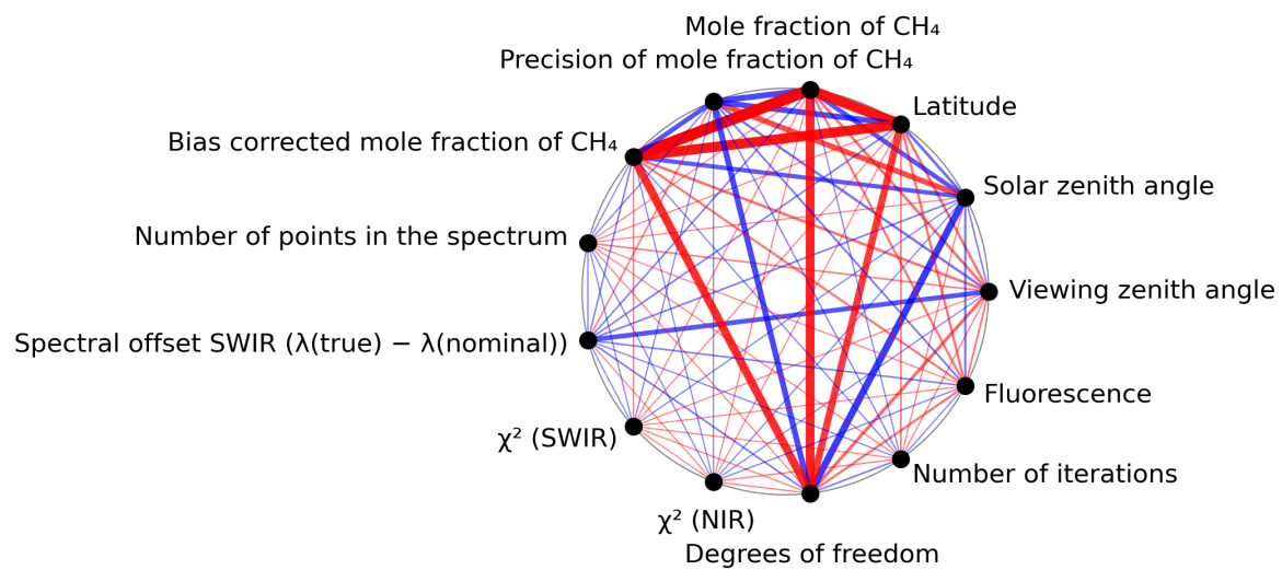
Figure 1: Map of correlation graph for 2023-11-18 to 2023-11-19.
