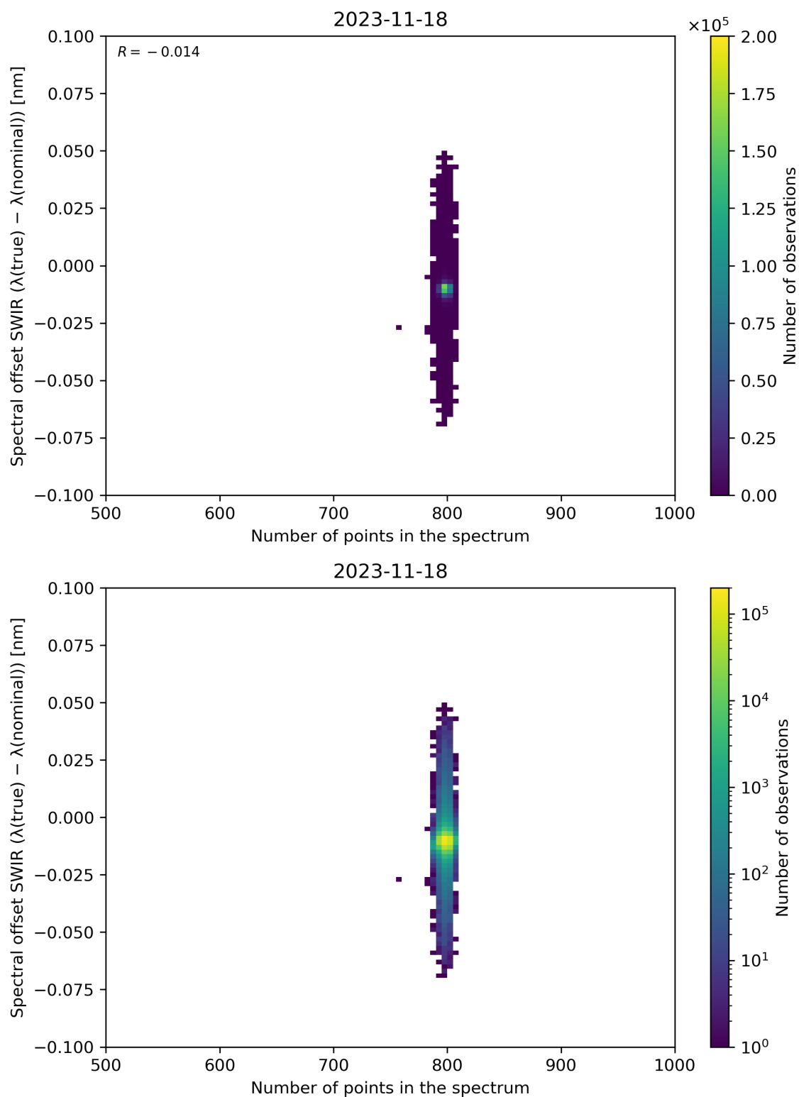
Figure 93: Scatter density plot of “Number of points in the spectrum” against “Spectral offset SWIR ( \lambda(\text{true}) - \lambda(\text{nominal}) )” for 2023-11-18 to 2023-11-19.
