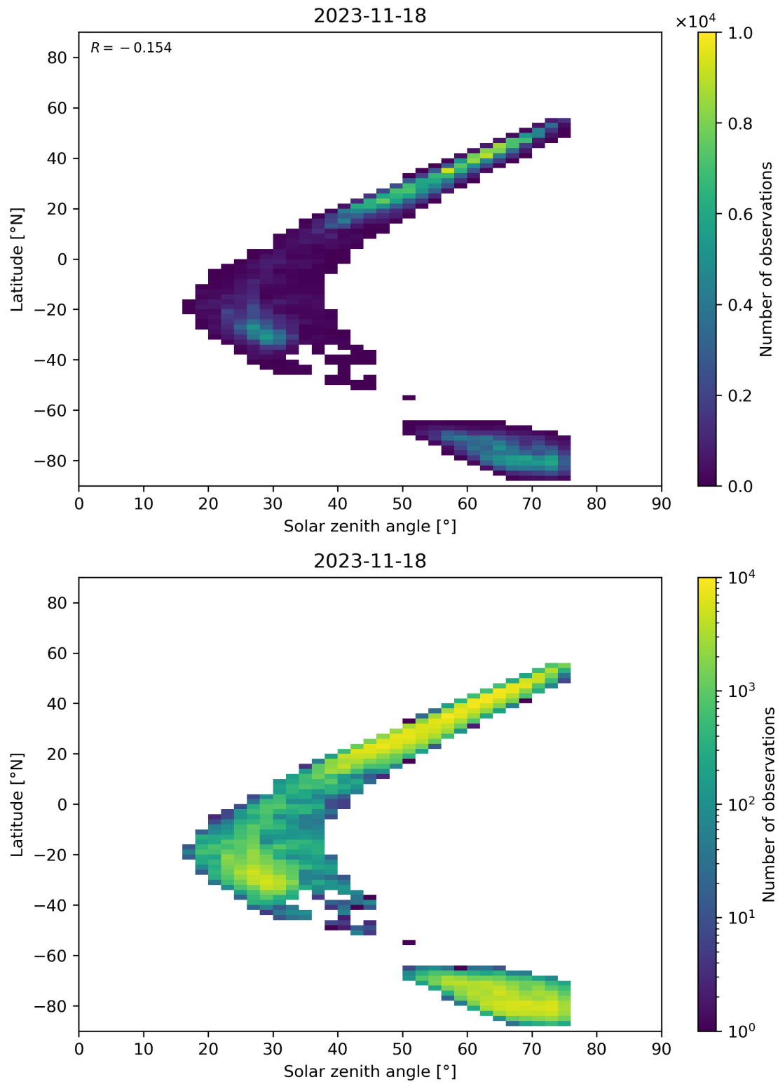
Figure 98: Scatter density plot of “Solar zenith angle” against “Latitude” for 2023-11-18 to 2023-11-19.
