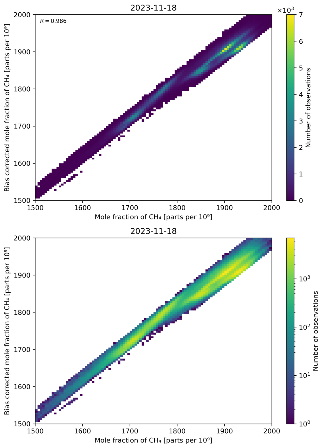
Figure 74: Scatter density plot of “Mole fraction of CH 4 ” against “Bias corrected mole fraction of CH 4 ” for 2023-11-18 to 2023-11-19.
