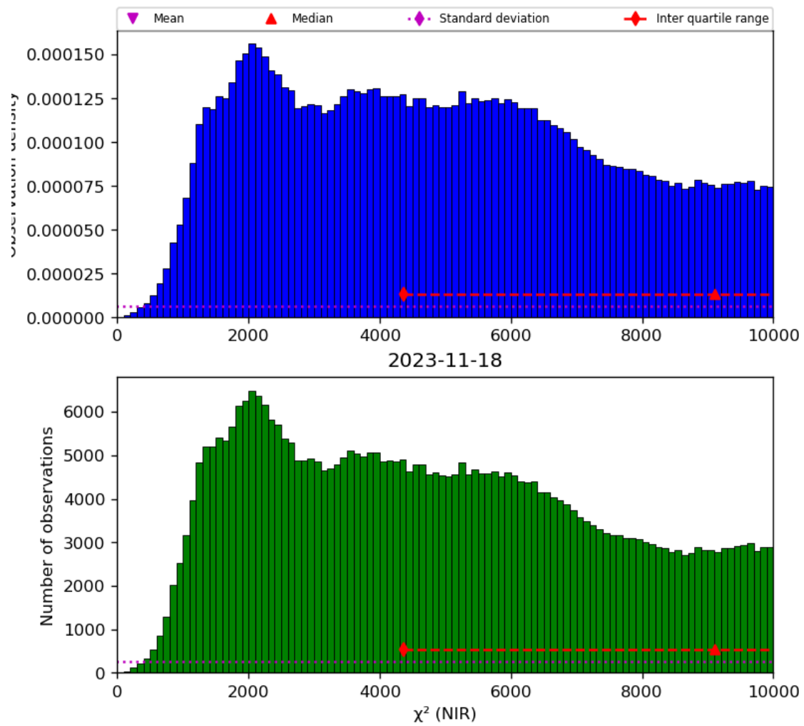
Figure 29: Histogram of “ \chi^2 (NIR)” for 2023-11-18 to 2023-11-19
