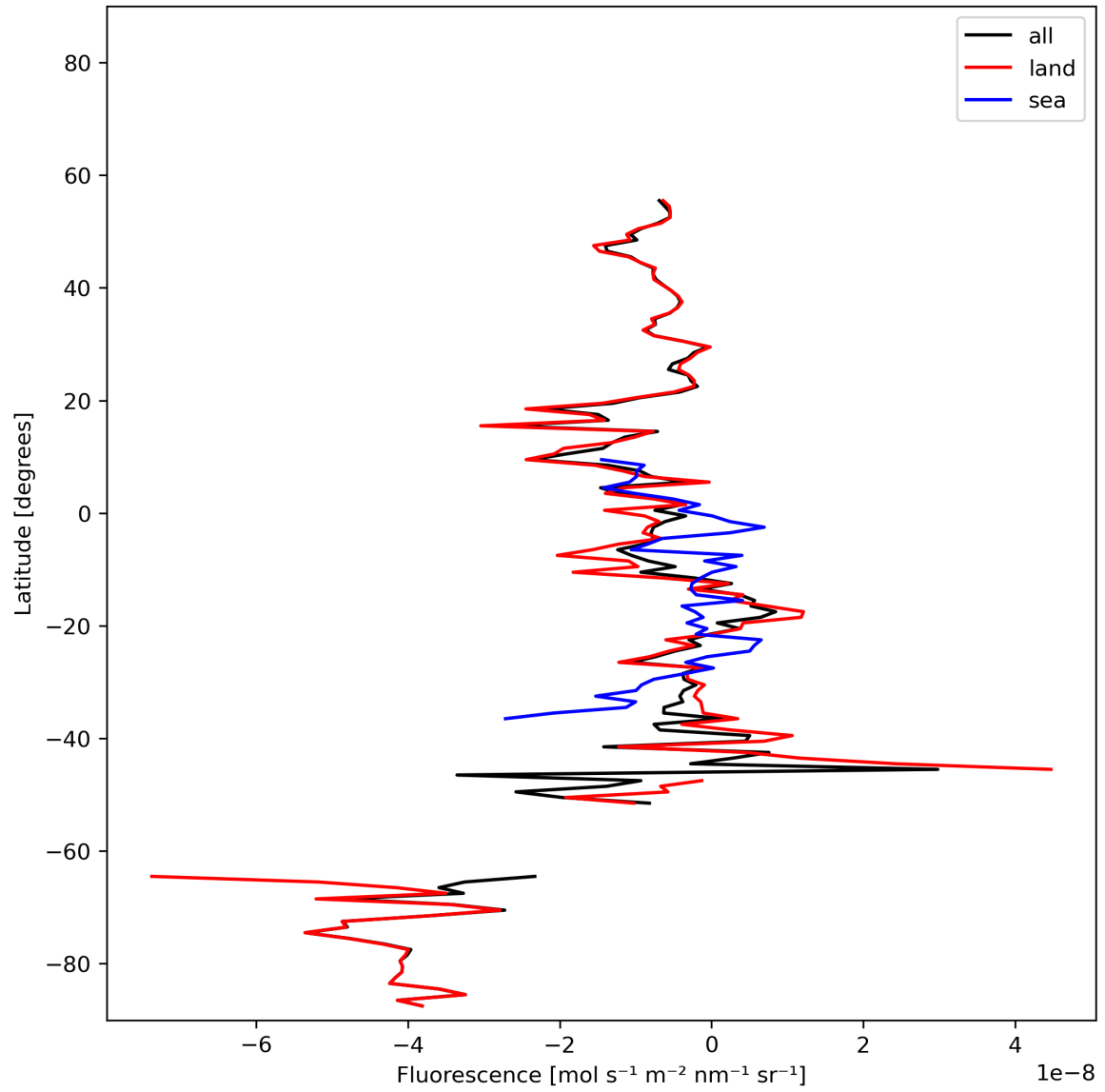
Figure 21: Zonal average of “Fluorescence” for 2023-11-18 to 2023-11-19.
