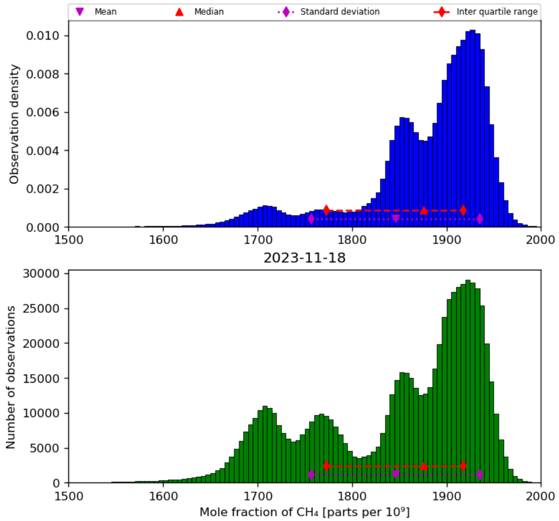
Figure 23: Histogram of “Mole fraction of CH 4 ” for 2023-11-18 to 2023-11-19
