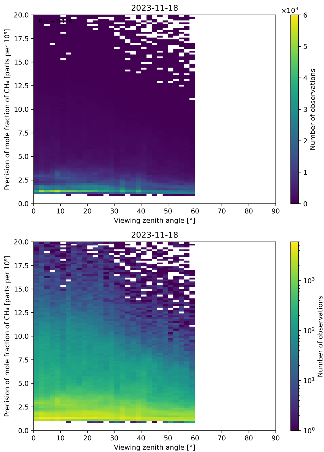
Figure 112: Scatter density plot of “Viewing zenith angle” against “Precision of mole fraction of CH 4 ” for 2023-11-18 to 2023-11-19.
