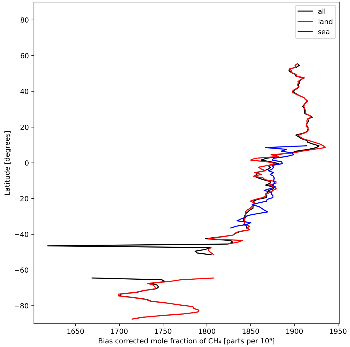
Figure 14: Zonal average of “Bias corrected mole fraction of CH 4 ” for 2023-11-18 to 2023-11-19.
