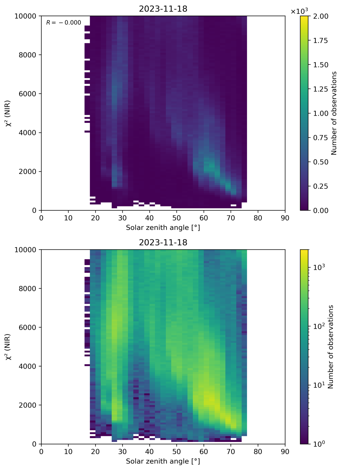
Figure 94: Scatter density plot of “Solar zenith angle” against “ \chi^2 (NIR)” for 2023-11-18 to 2023-11-19.
