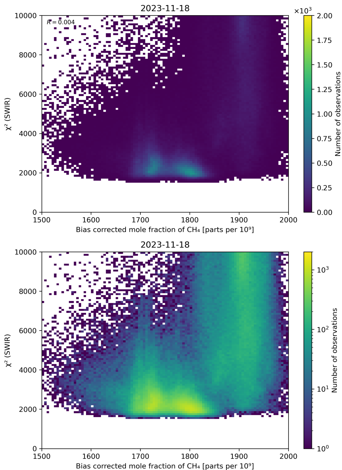
Figure 64: Scatter density plot of “Bias corrected mole fraction of \text{CH}_4 ” against “ \chi^2 (SWIR)” for 2023-11-18 to 2023-11-19.
