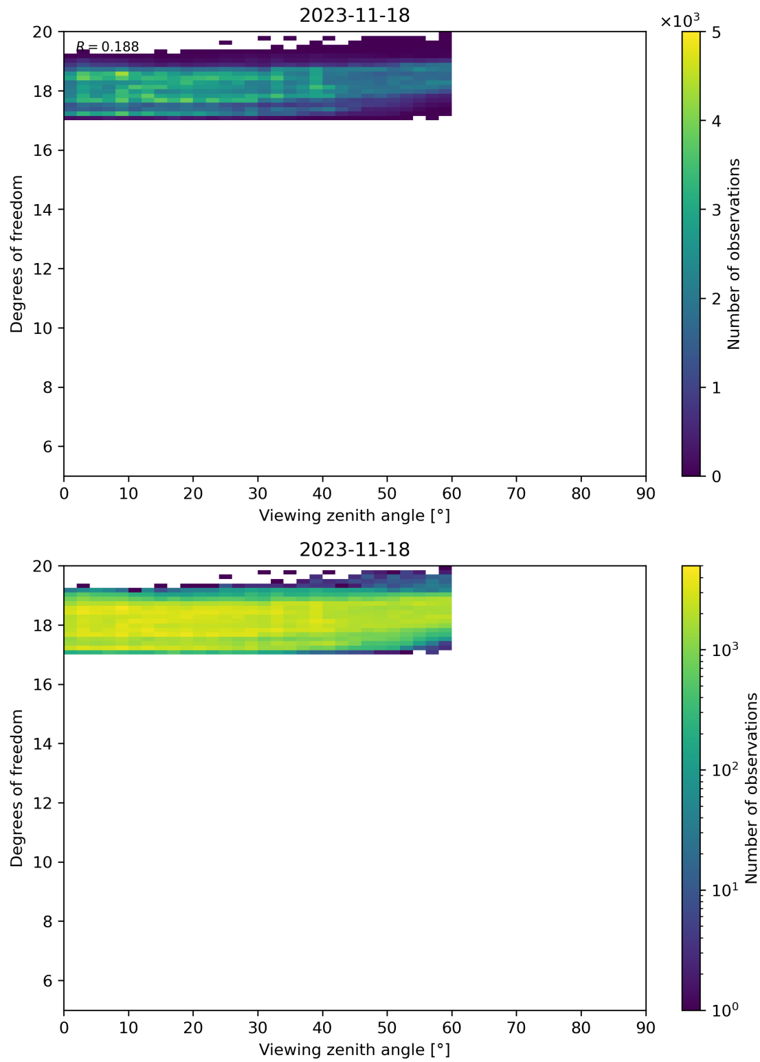
Figure 107: Scatter density plot of “Viewing zenith angle” against “Degrees of freedom” for 2023-11-18 to 2023-11-19.
