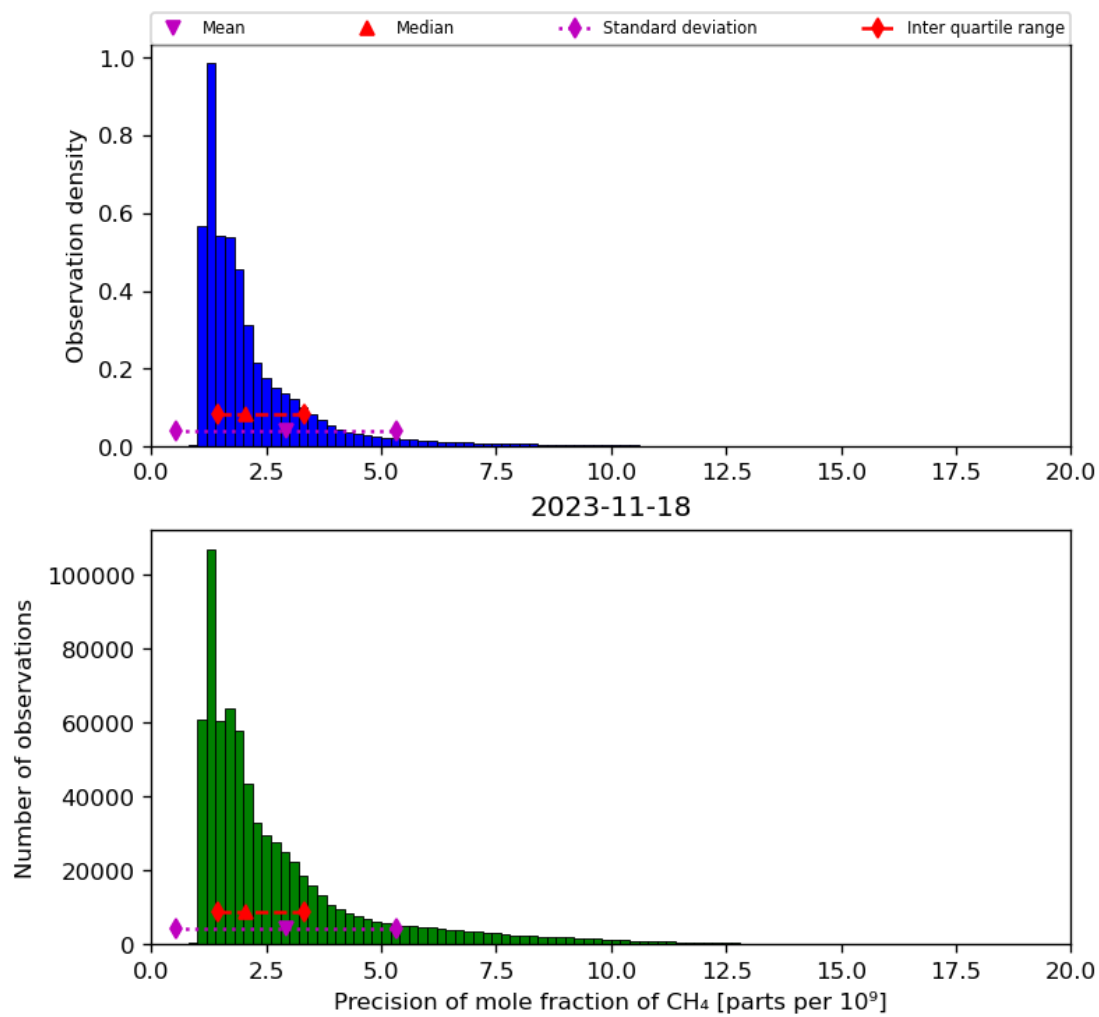
Figure 24: Histogram of “Precision of mole fraction of CH 4 ” for 2023-11-18 to 2023-11-19
