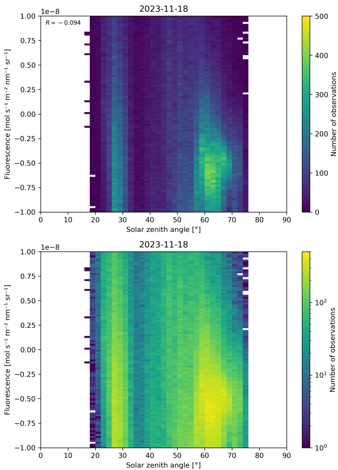
Figure 97: Scatter density plot of “Solar zenith angle” against “Fluorescence” for 2023-11-18 to 2023-11-19.
