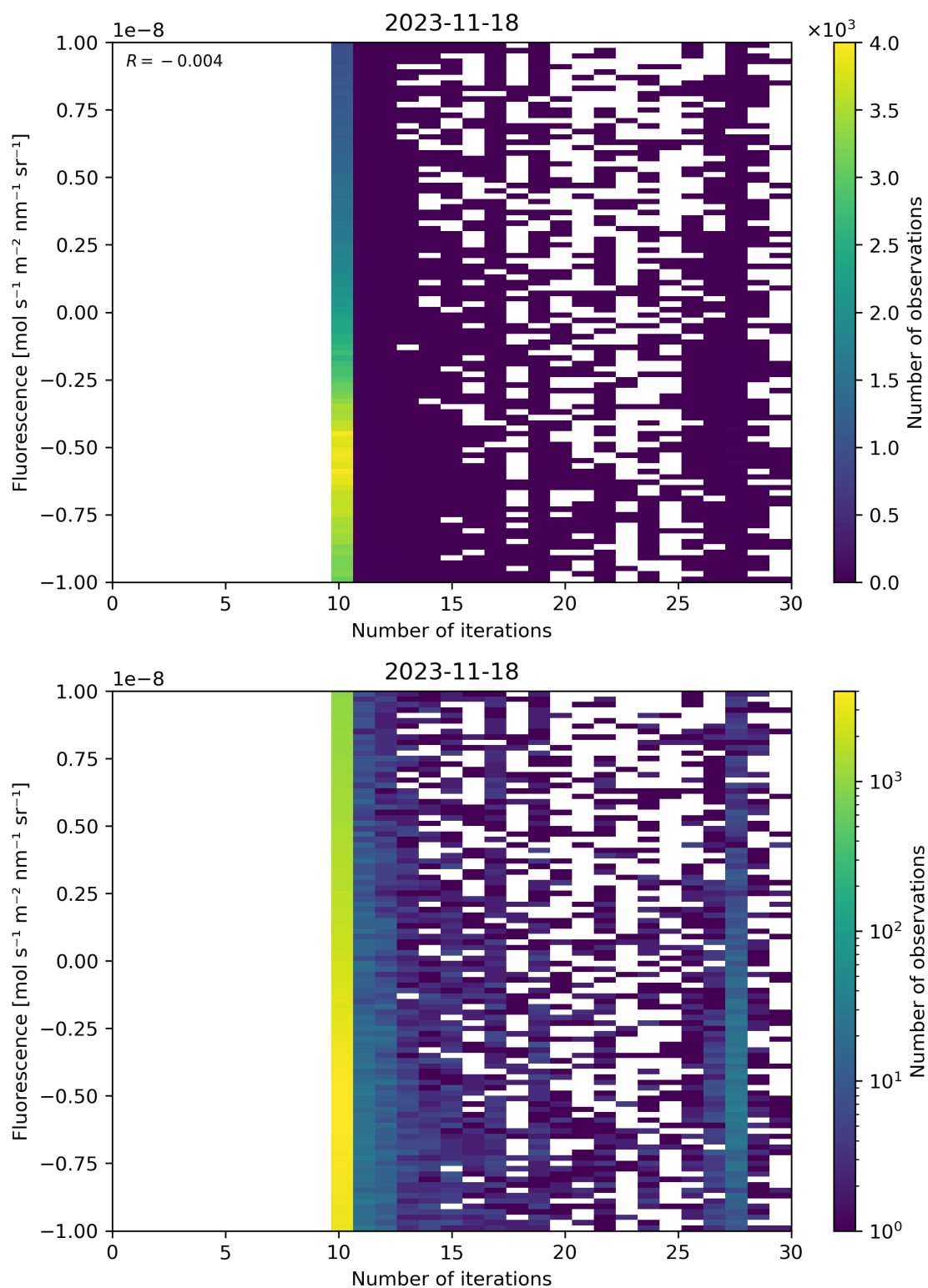
Figure 87: Scatter density plot of “Number of iterations” against “Fluorescence” for 2023-11-18 to 2023-11-19.
