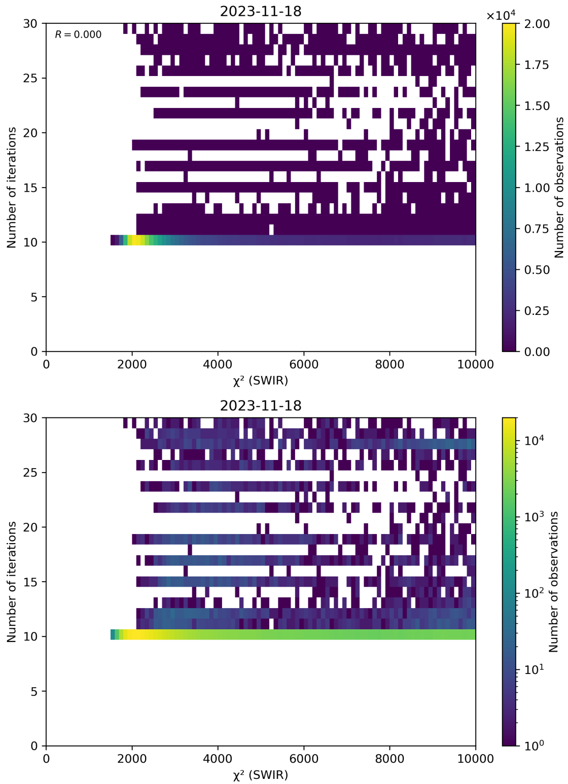
Figure 50: Scatter density plot of “ \chi^2 (SWIR)” against “Number of iterations” for 2023-11-18 to 2023-11-19.
