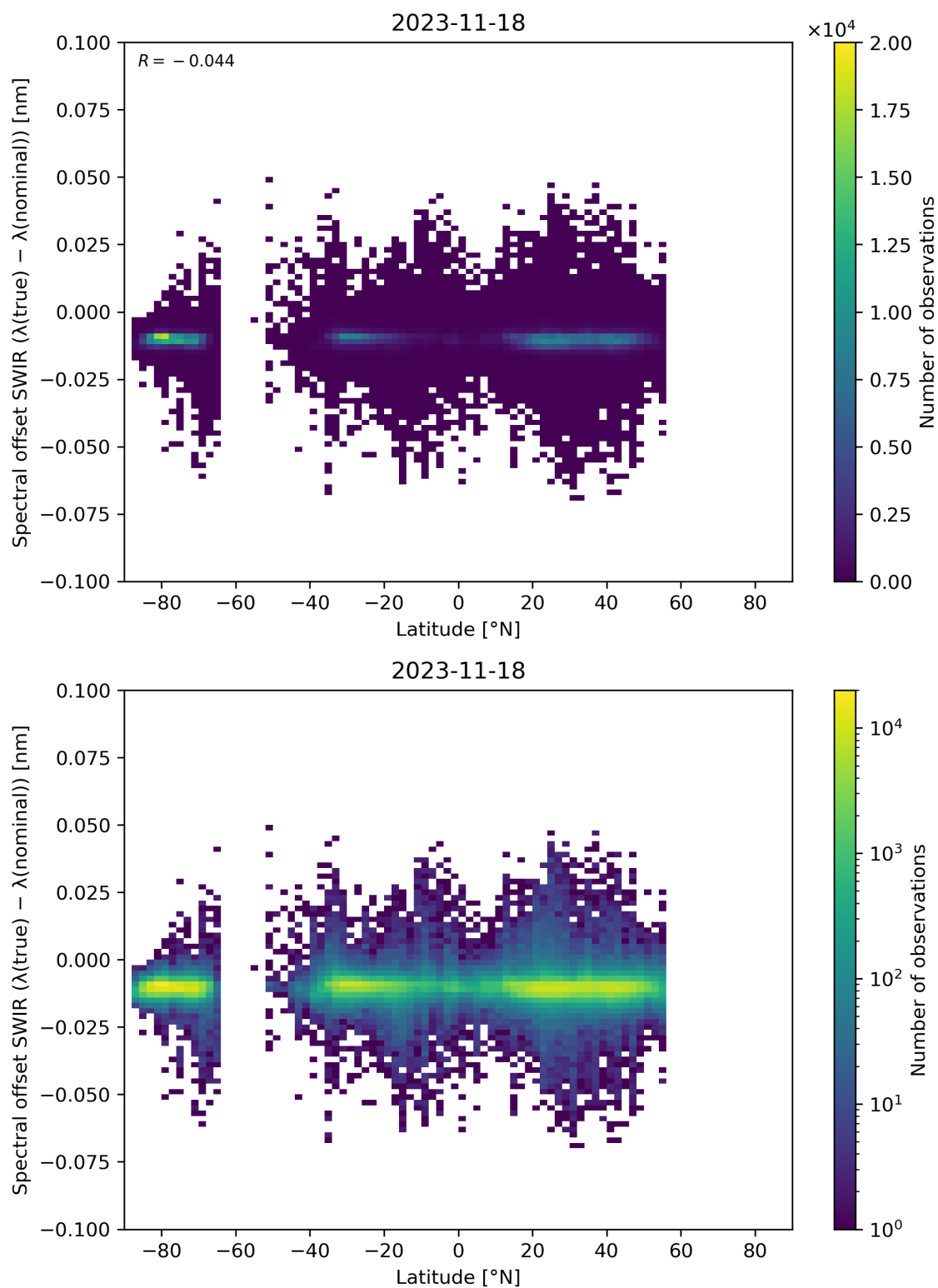
Figure 62: Scatter density plot of “Latitude” against “Spectral offset SWIR ( \lambda(\text{true}) - \lambda(\text{nominal}) )” for 2023-11-18 to 2023-11-19.
