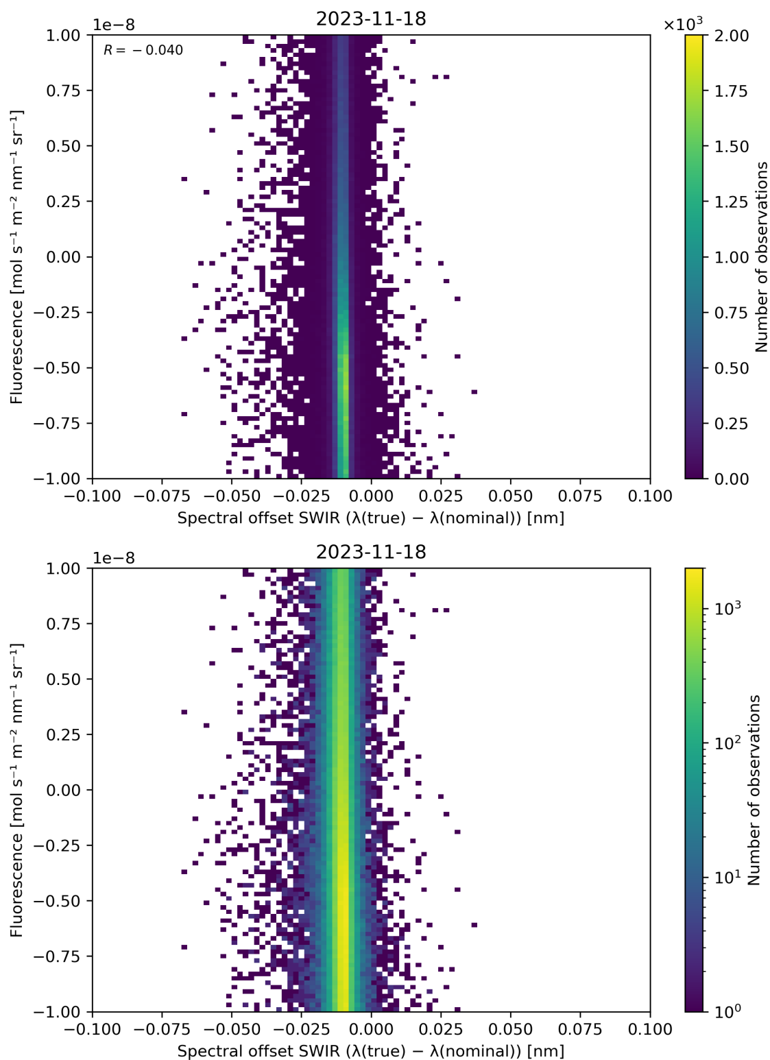
Figure 120: Scatter density plot of “Spectral offset SWIR ( \lambda(\text{true}) - \lambda(\text{nominal}) )” against “Fluorescence” for 2023-11-18 to 2023-11-19.
