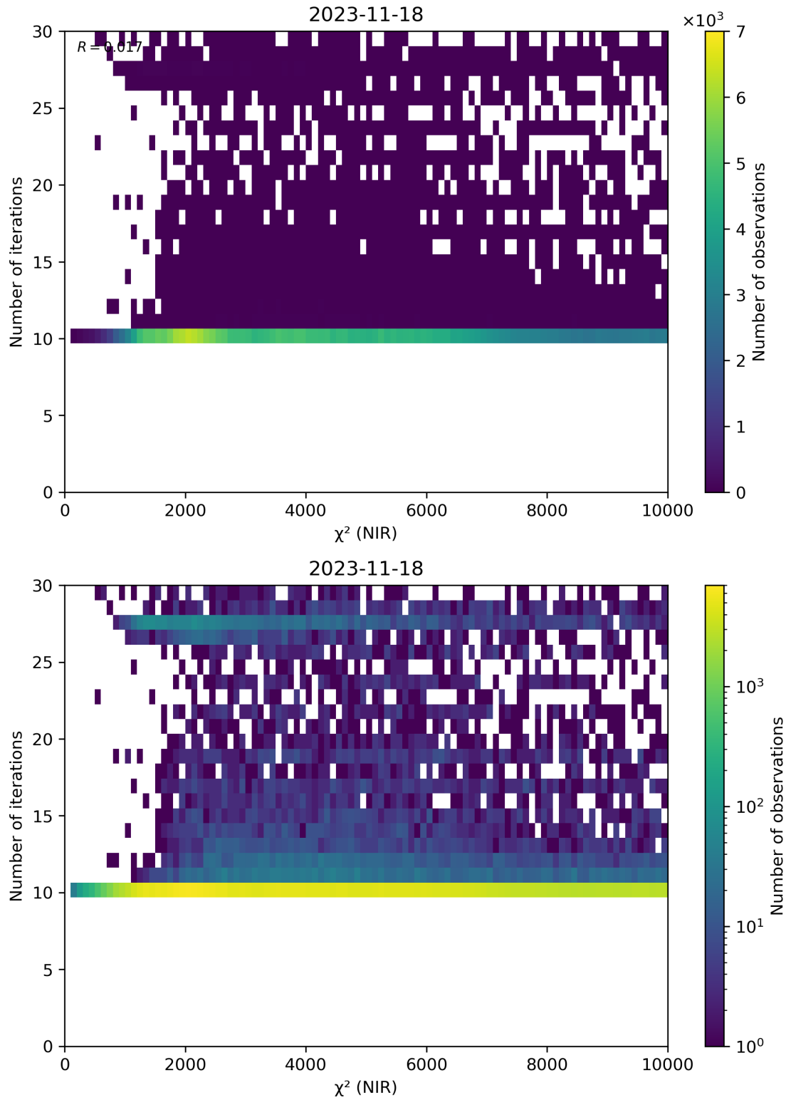
Figure 46: Scatter density plot of “ \chi^2 (NIR)” against “Number of iterations” for 2023-11-18 to 2023-11-19.
