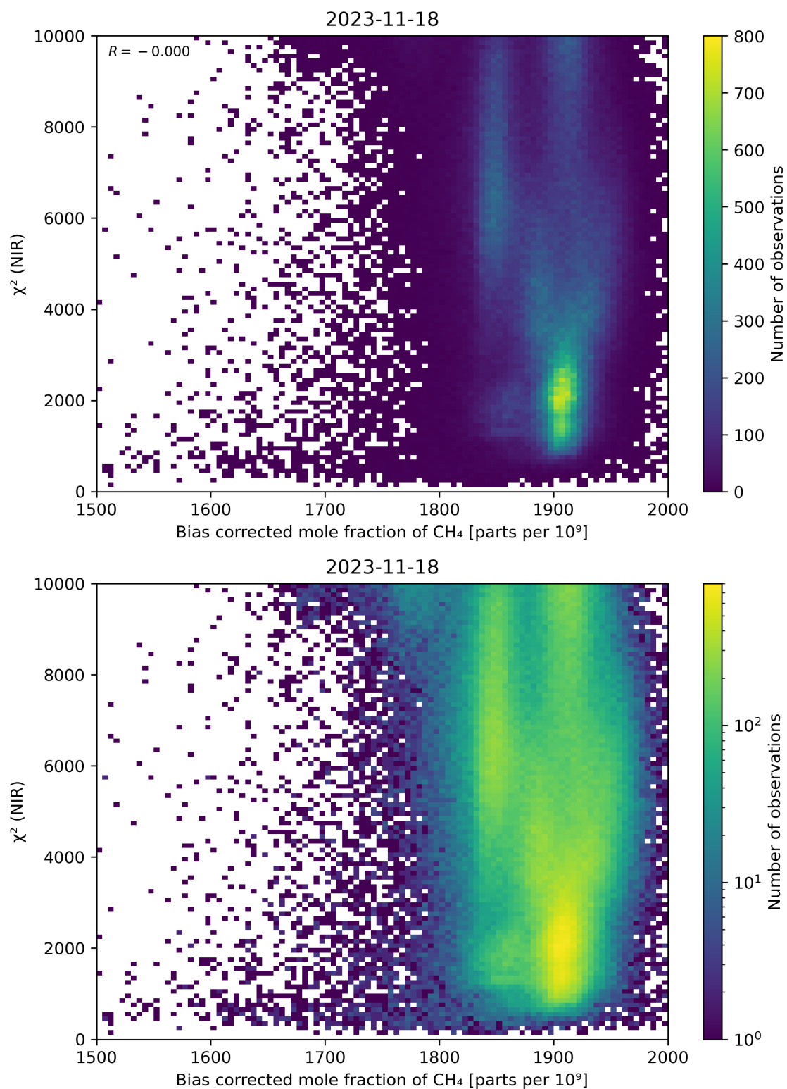
Figure 63: Scatter density plot of “Bias corrected mole fraction of CH 4 ” against “ \chi^2 (NIR)” for 2023-11-18 to 2023-11-19.
