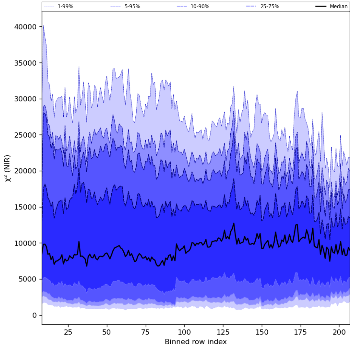
Figure 40: Along track statistics of “ \chi^2 (NIR)” for 2023-11-18 to 2023-11-19
