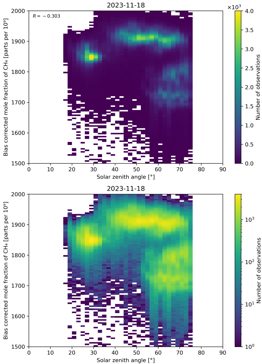
Figure 100: Scatter density plot of “Solar zenith angle” against “Bias corrected mole fraction of \text{CH}_4 ” for 2023-11-18 to 2023-11-19.
