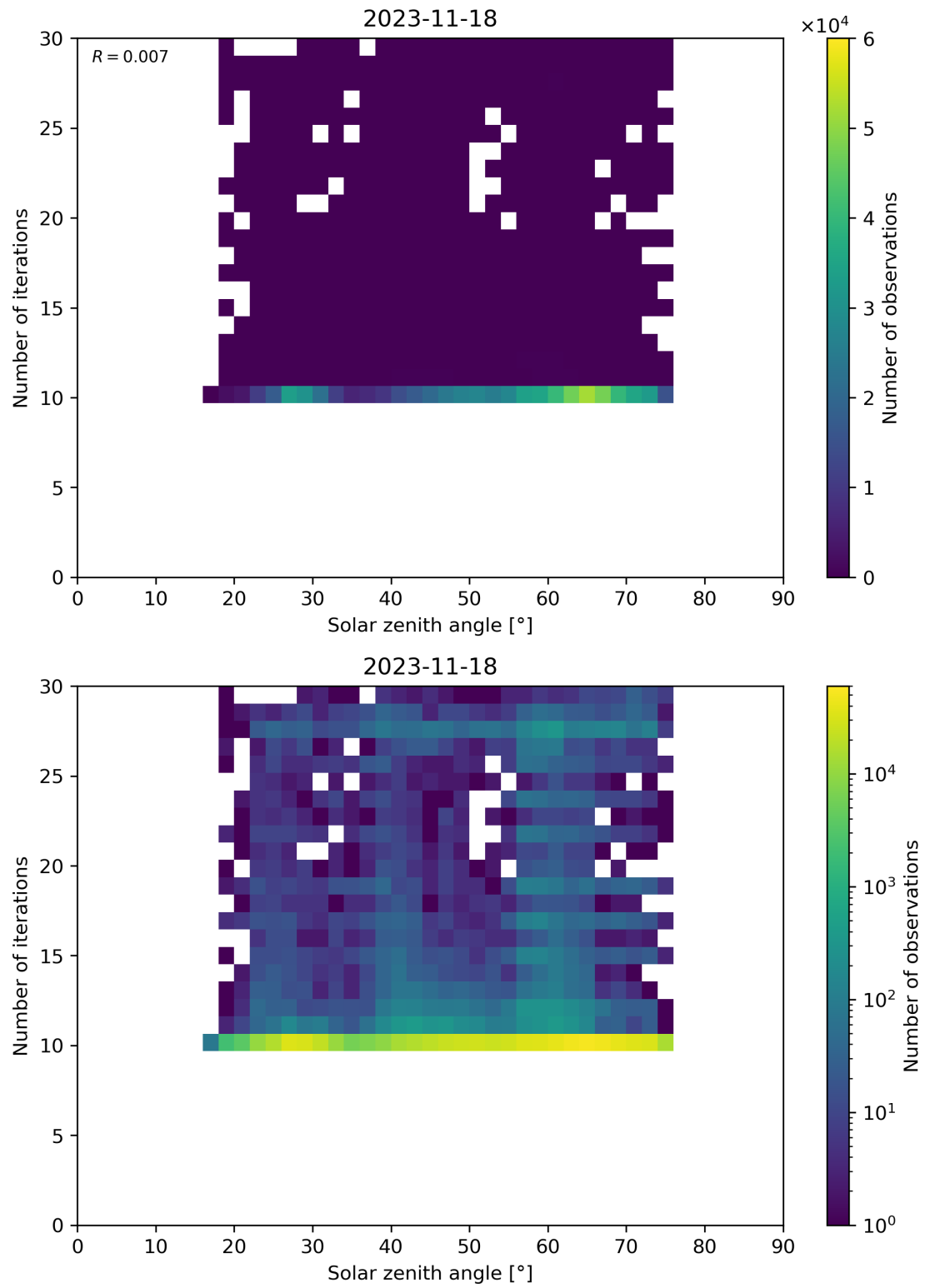
Figure 102: Scatter density plot of “Solar zenith angle” against “Number of iterations” for 2023-11-18 to 2023-11-19.
