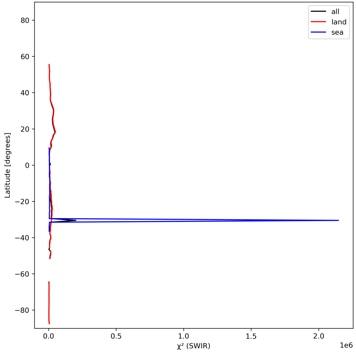
Figure 17: Zonal average of “ \chi^2 (SWIR)” for 2023-11-18 to 2023-11-19.
