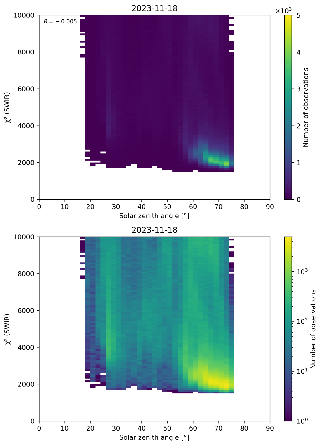
Figure 95: Scatter density plot of “Solar zenith angle” against “ \chi^2 (SWIR)” for 2023-11-18 to 2023-11-19.
