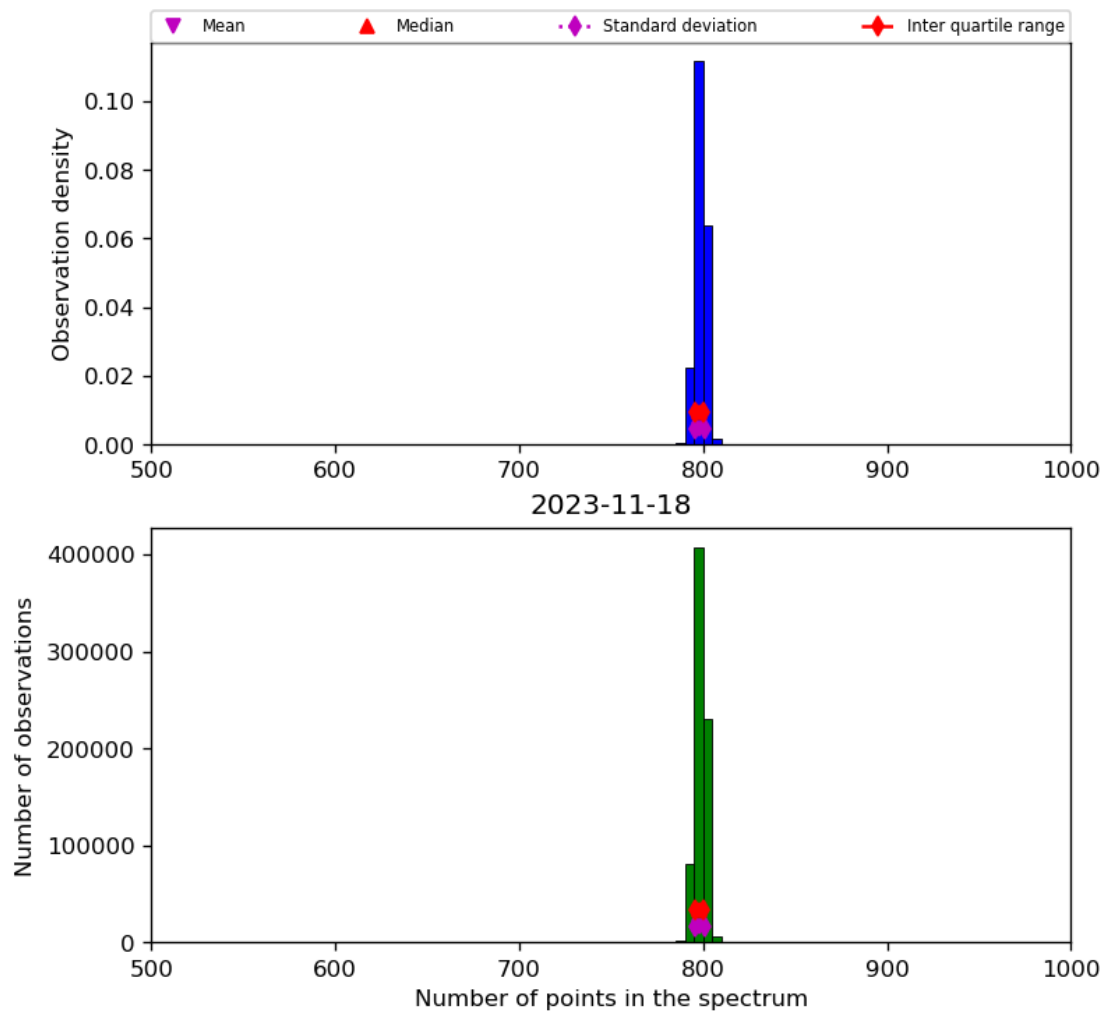
Figure 26: Histogram of “Number of points in the spectrum” for 2023-11-18 to 2023-11-19
