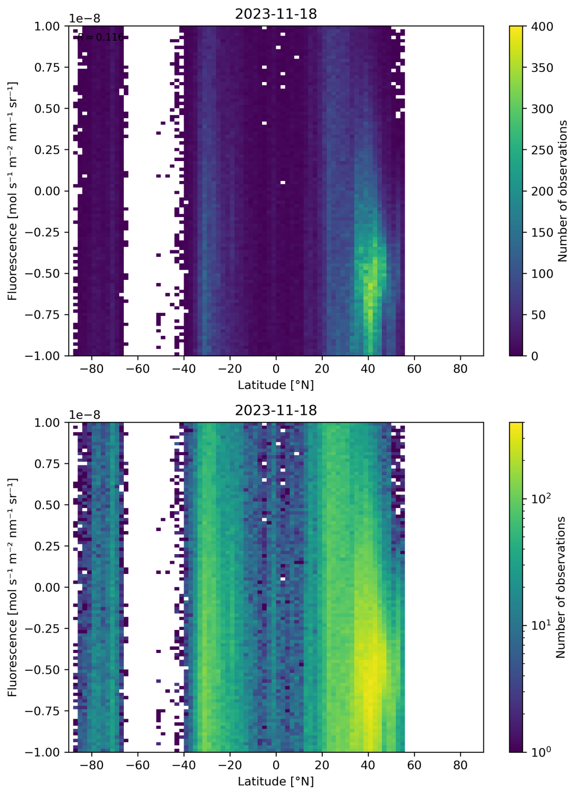
Figure 56: Scatter density plot of “Latitude” against “Fluorescence” for 2023-11-18 to 2023-11-19.
