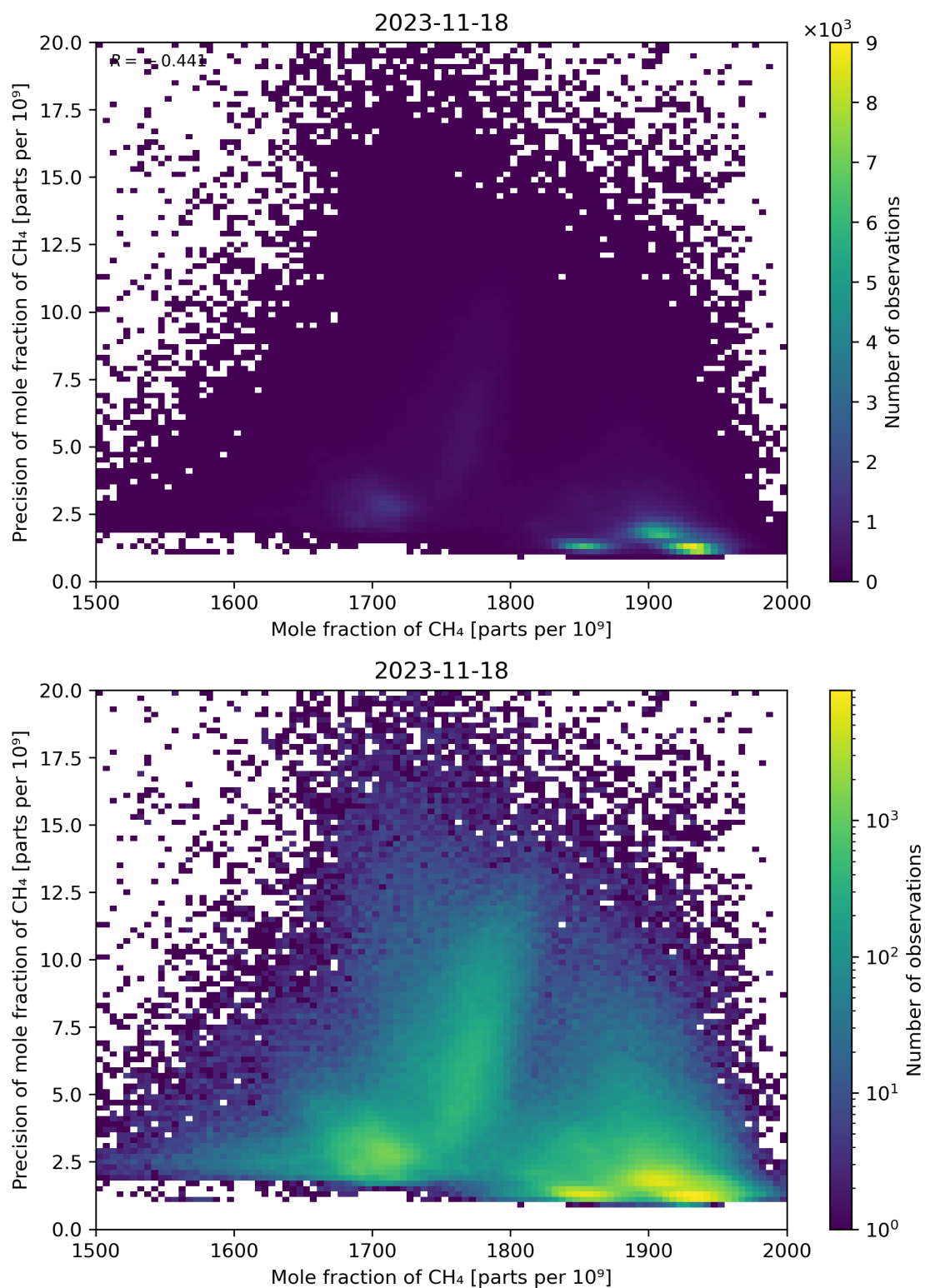
Figure 75: Scatter density plot of “Mole fraction of CH 4 ” against “Precision of mole fraction of CH 4 ” for 2023-11-18 to 2023-11-19.
