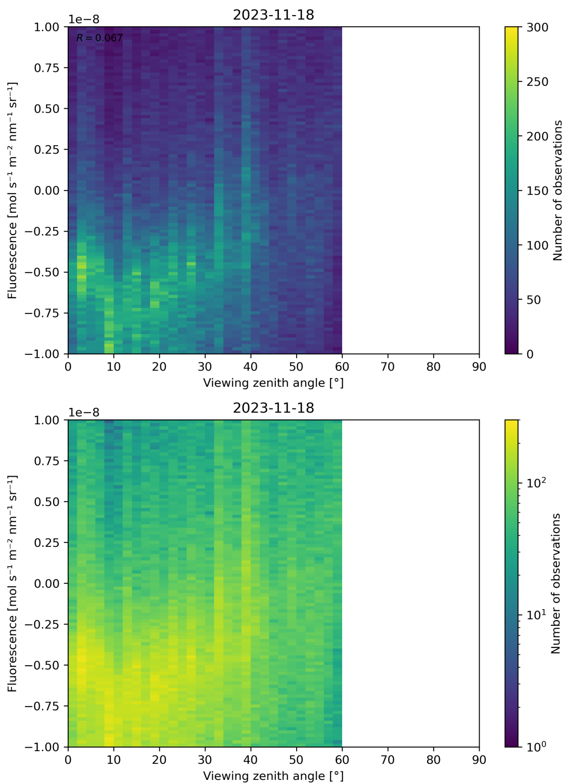
Figure 108: Scatter density plot of “Viewing zenith angle” against “Fluorescence” for 2023-11-18 to 2023-11-19.
