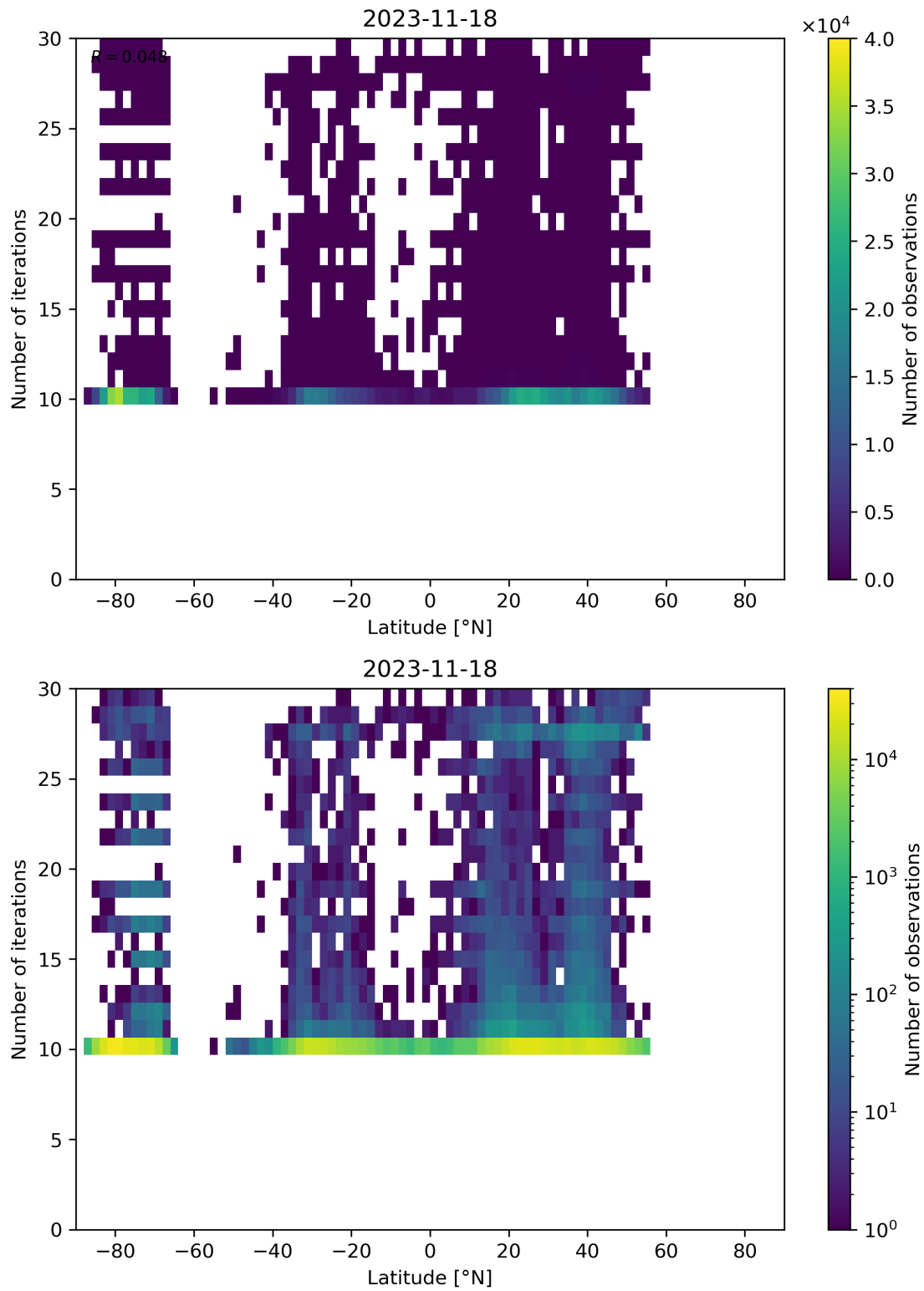
Figure 60: Scatter density plot of “Latitude” against “Number of iterations” for 2023-11-18 to 2023-11-19.
