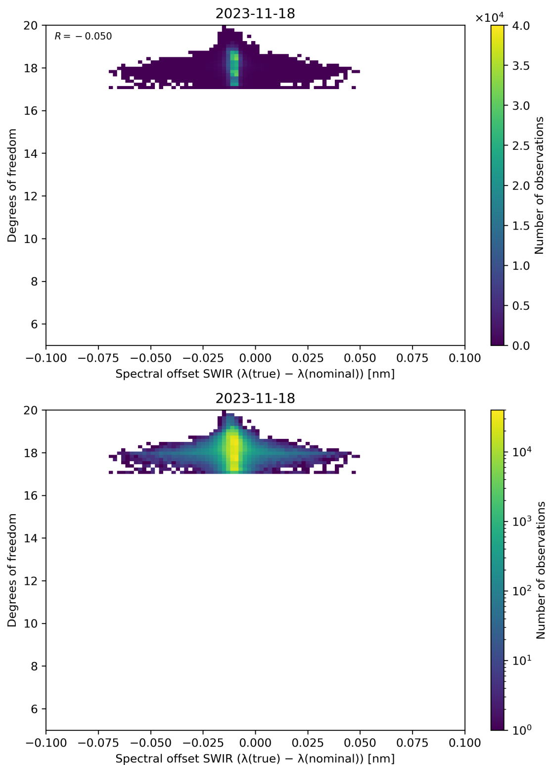
Figure 119: Scatter density plot of “Spectral offset SWIR ( \lambda(\text{true}) - \lambda(\text{nominal}) )” against “Degrees of freedom” for 2023-11-18 to 2023-11-19.
