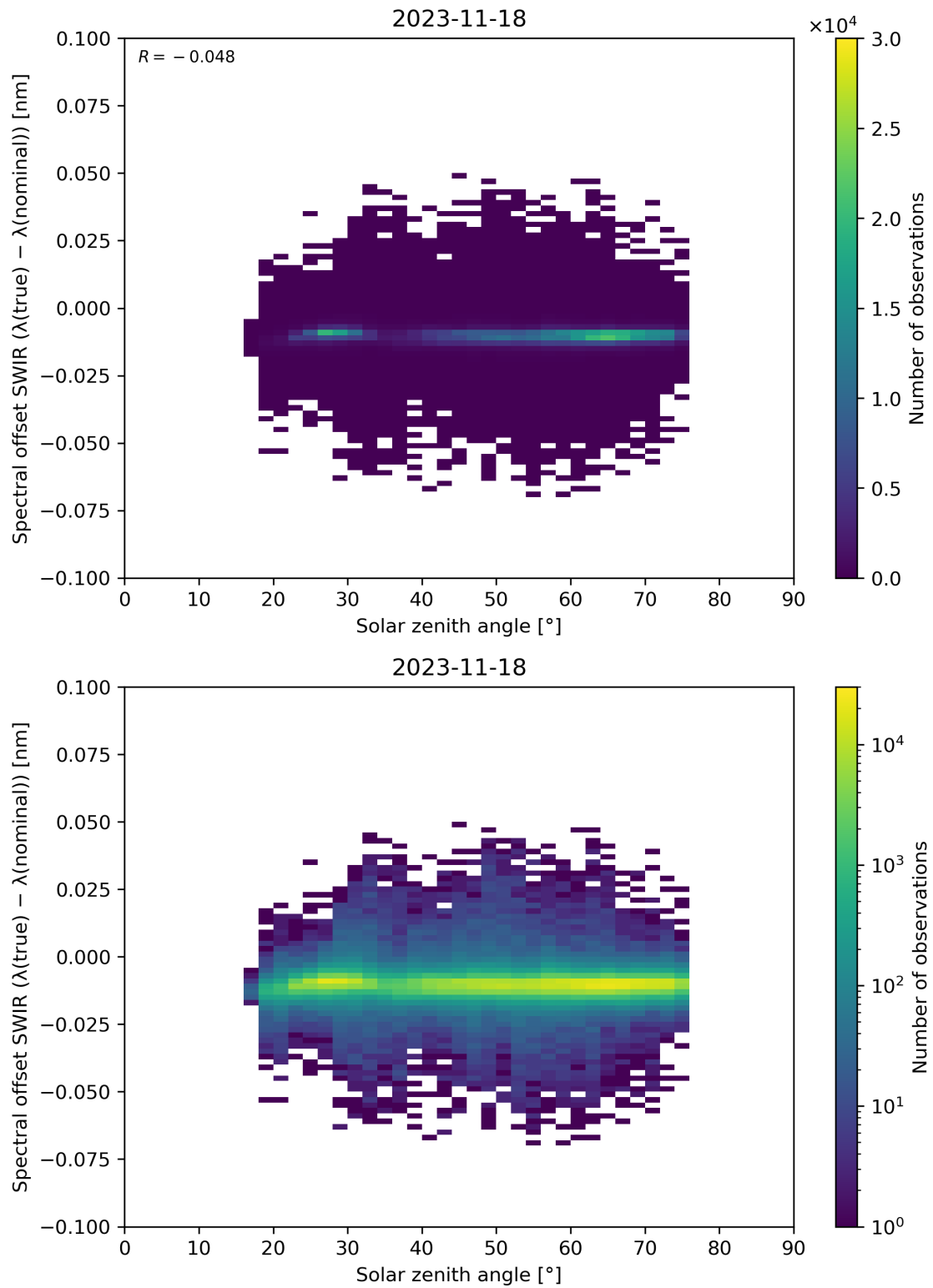
Figure 104: Scatter density plot of “Solar zenith angle” against “Spectral offset SWIR ( \lambda(\text{true}) - \lambda(\text{nominal}) )” for 2023-11-18 to 2023-11-19.
