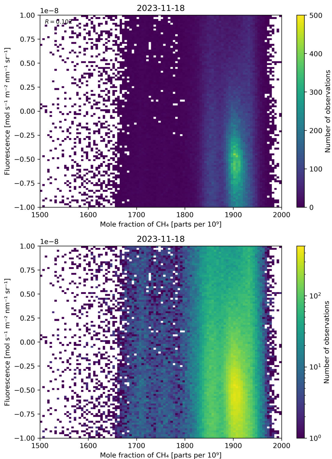
Figure 73: Scatter density plot of “Mole fraction of \text{CH}_4 ” against “Fluorescence” for 2023-11-18 to 2023-11-19.
