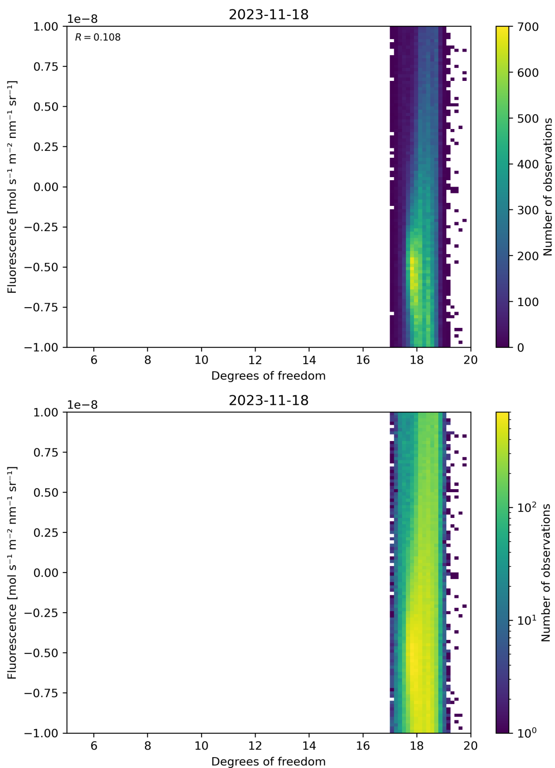
Figure 51: Scatter density plot of “Degrees of freedom” against “Fluorescence” for 2023-11-18 to 2023-11-19.
