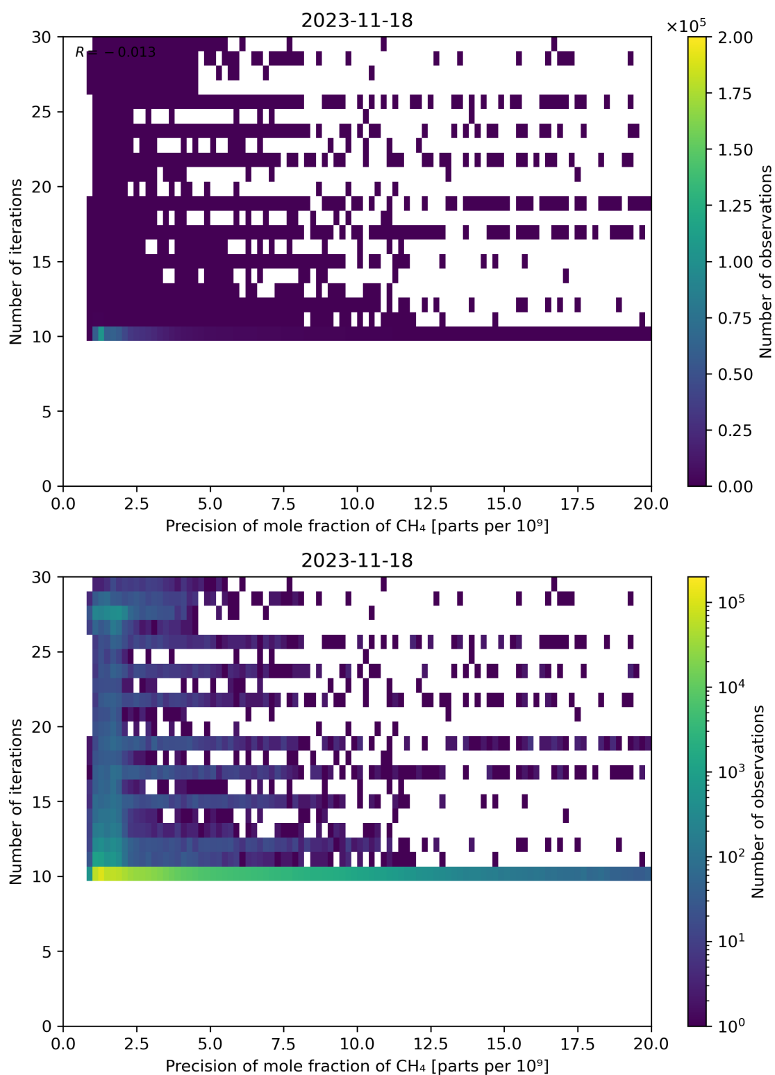
Figure 83: Scatter density plot of “Precision of mole fraction of CH 4 ” against “Number of iterations” for 2023-11-18 to 2023-11-19.
