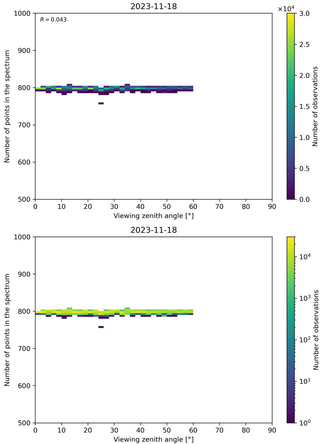
Figure 114: Scatter density plot of “Viewing zenith angle” against “Number of points in the spectrum” for 2023-11-18 to 2023-11-19.
