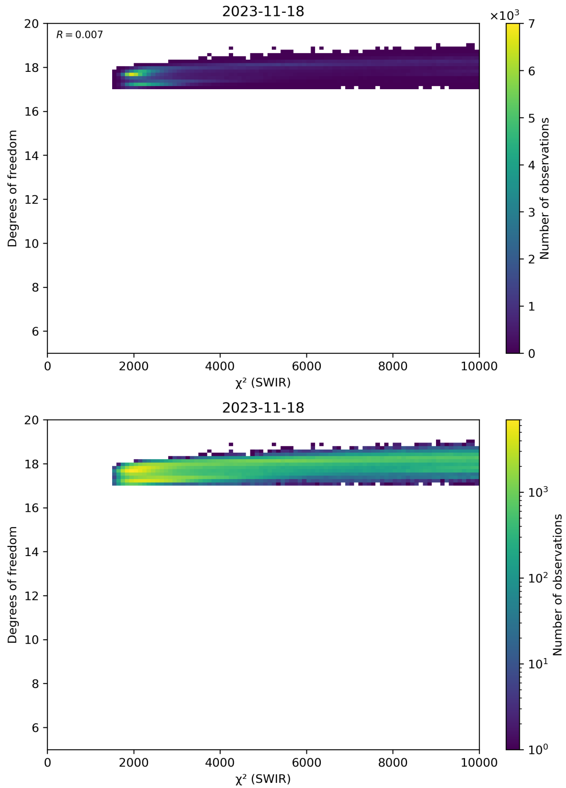
Figure 48: Scatter density plot of “ \chi^2 (SWIR)” against “Degrees of freedom” for 2023-11-18 to 2023-11-19.
