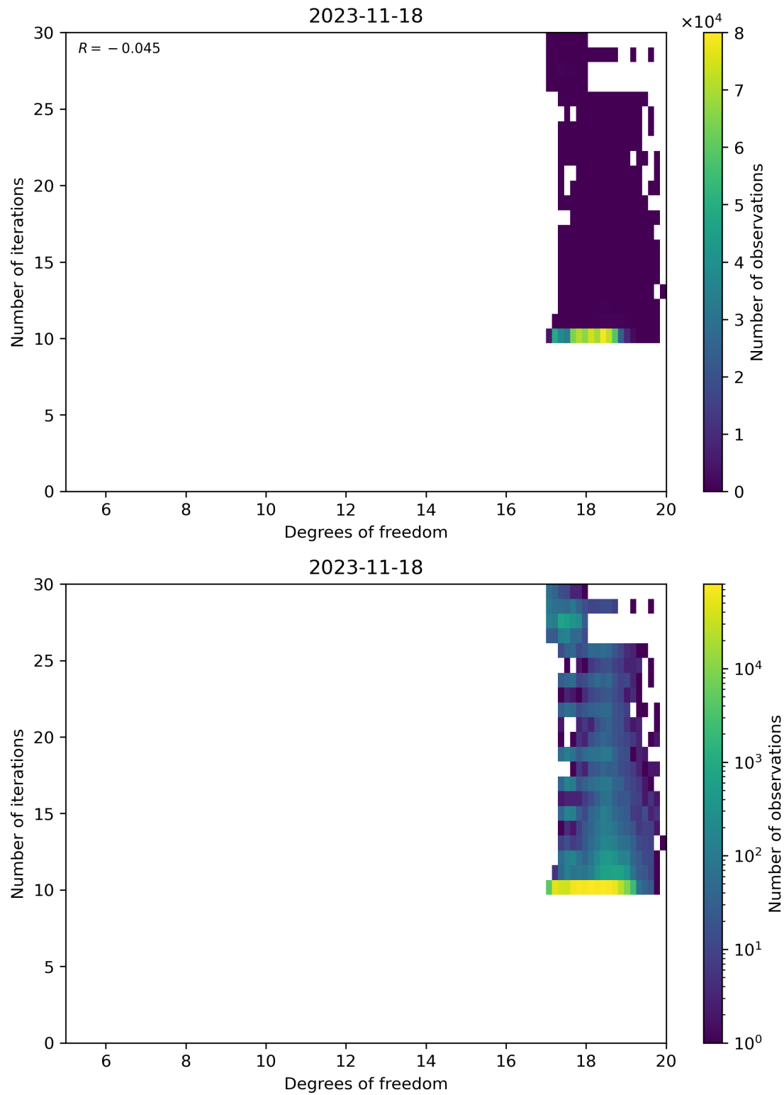
Figure 52: Scatter density plot of “Degrees of freedom” against “Number of iterations” for 2023-11-18 to 2023-11-19.
