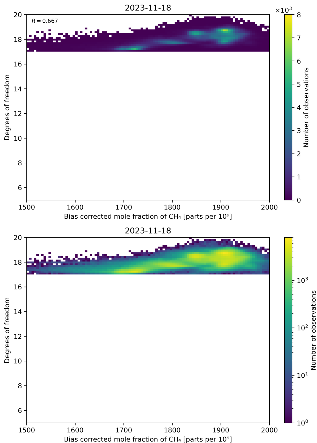
Figure 65: Scatter density plot of “Bias corrected mole fraction of CH 4 ” against “Degrees of freedom” for 2023-11-18 to 2023-11-19.
