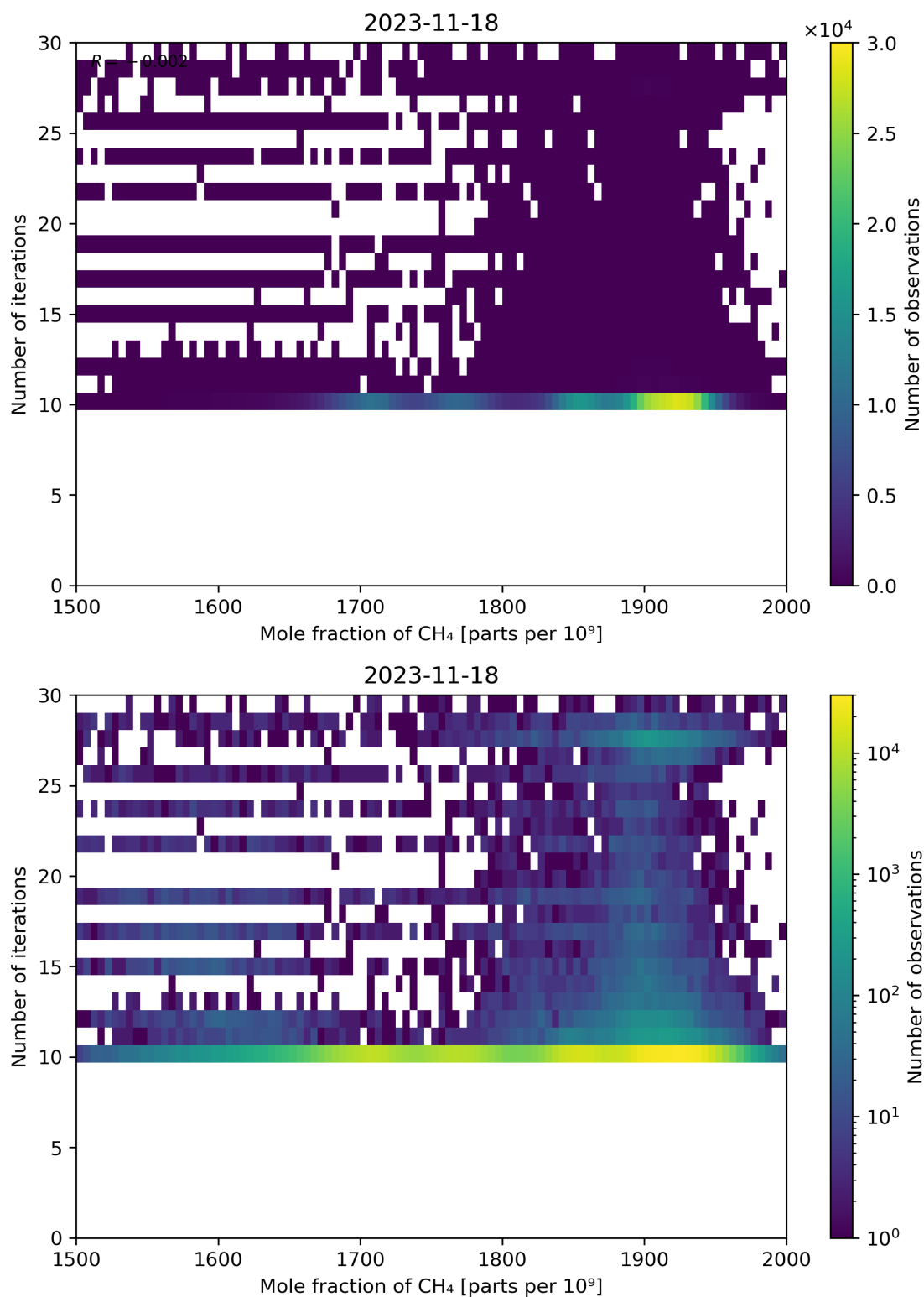
Figure 76: Scatter density plot of “Mole fraction of CH 4 ” against “Number of iterations” for 2023-11-18 to 2023-11-19.
