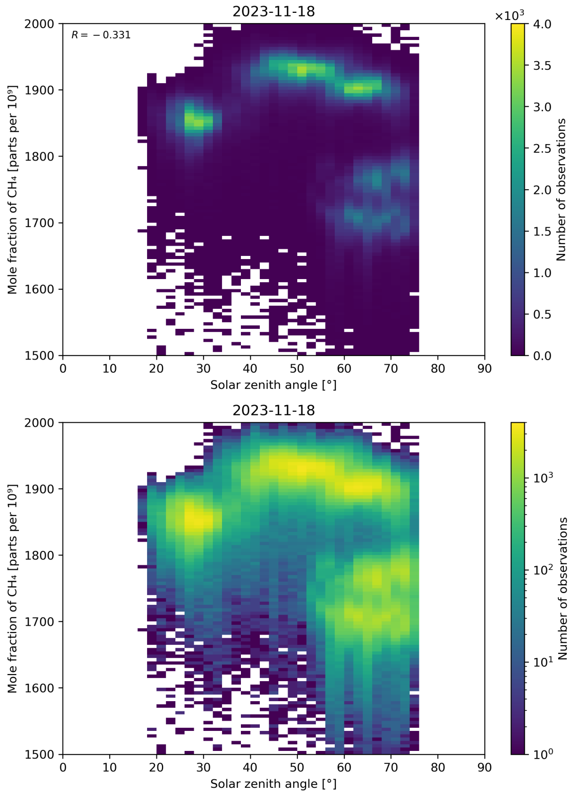
Figure 99: Scatter density plot of “Solar zenith angle” against “Mole fraction of \text{CH}_4 ” for 2023-11-18 to 2023-11-19.
