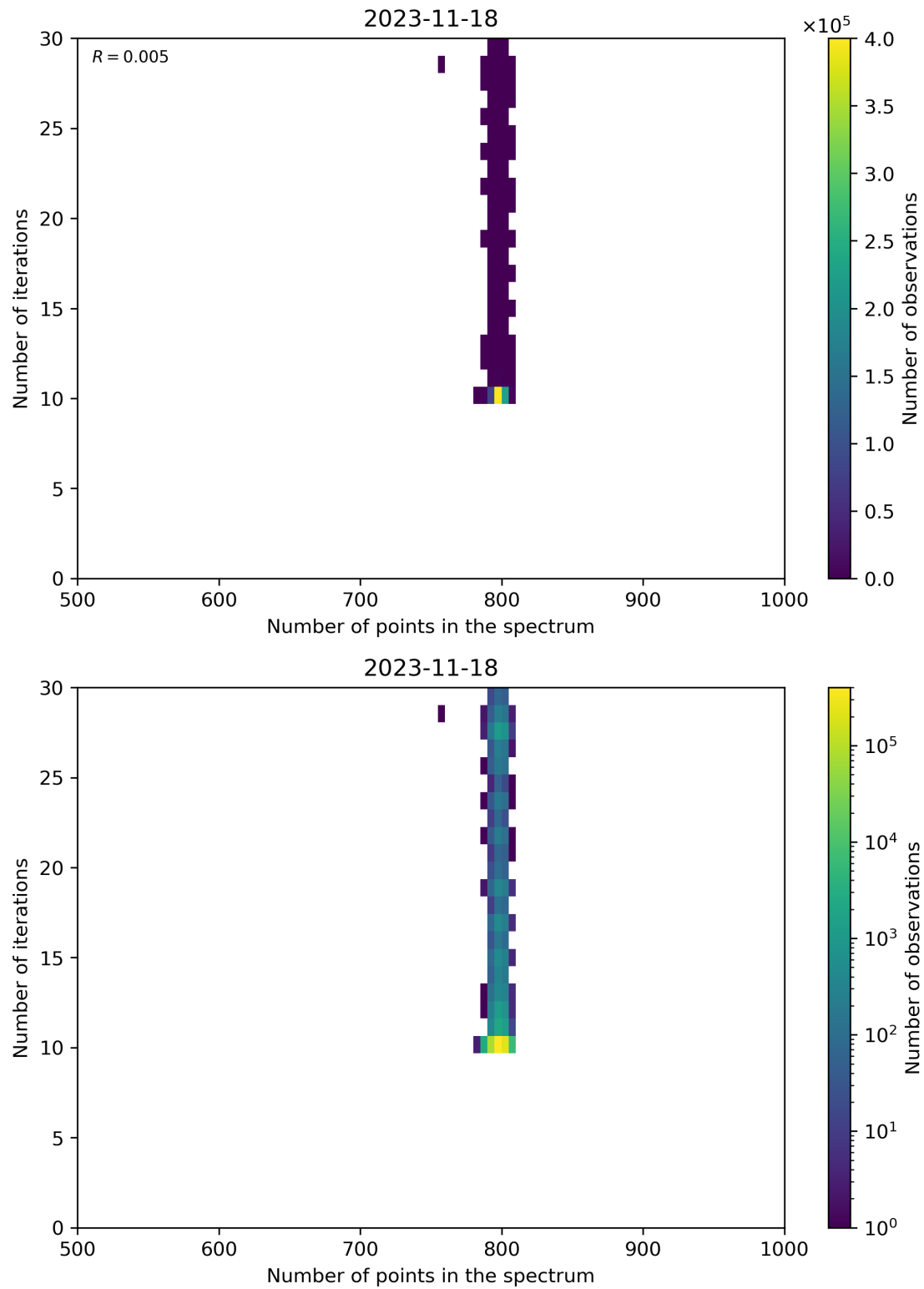
Figure 92: Scatter density plot of “Number of points in the spectrum” against “Number of iterations” for 2023-11-18 to 2023-11-19.
