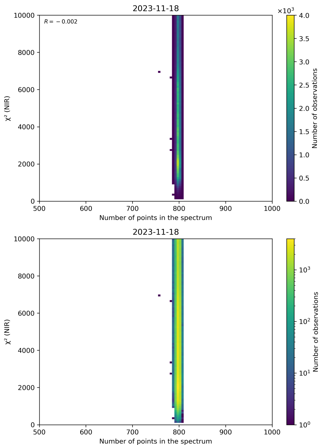
Figure 88: Scatter density plot of “Number of points in the spectrum” against “ \chi^2 (NIR)” for 2023-11-18 to 2023-11-19.
