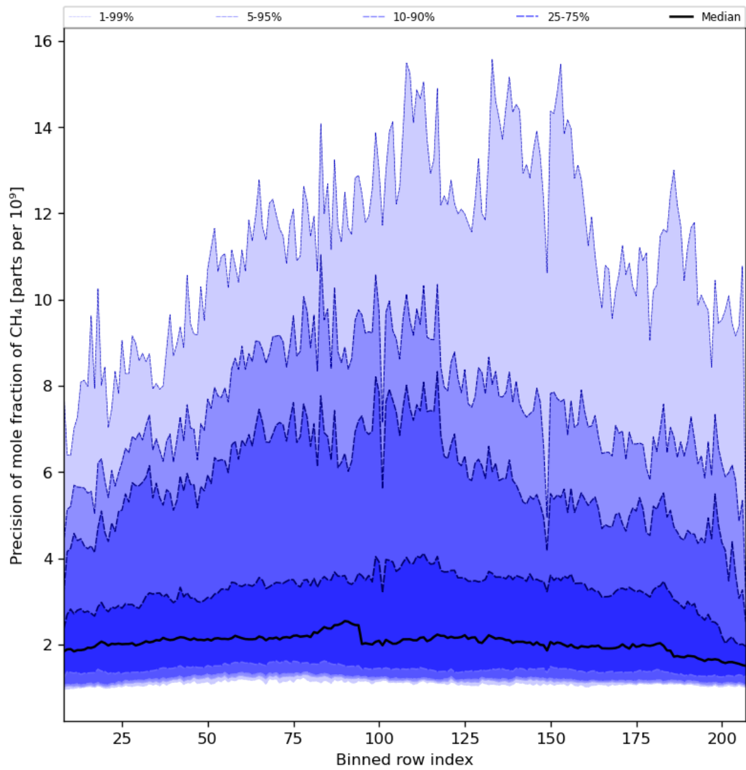
Figure 35: Along track statistics of “Precision of mole fraction of CH 4 ” for 2023-11-18 to 2023-11-19
