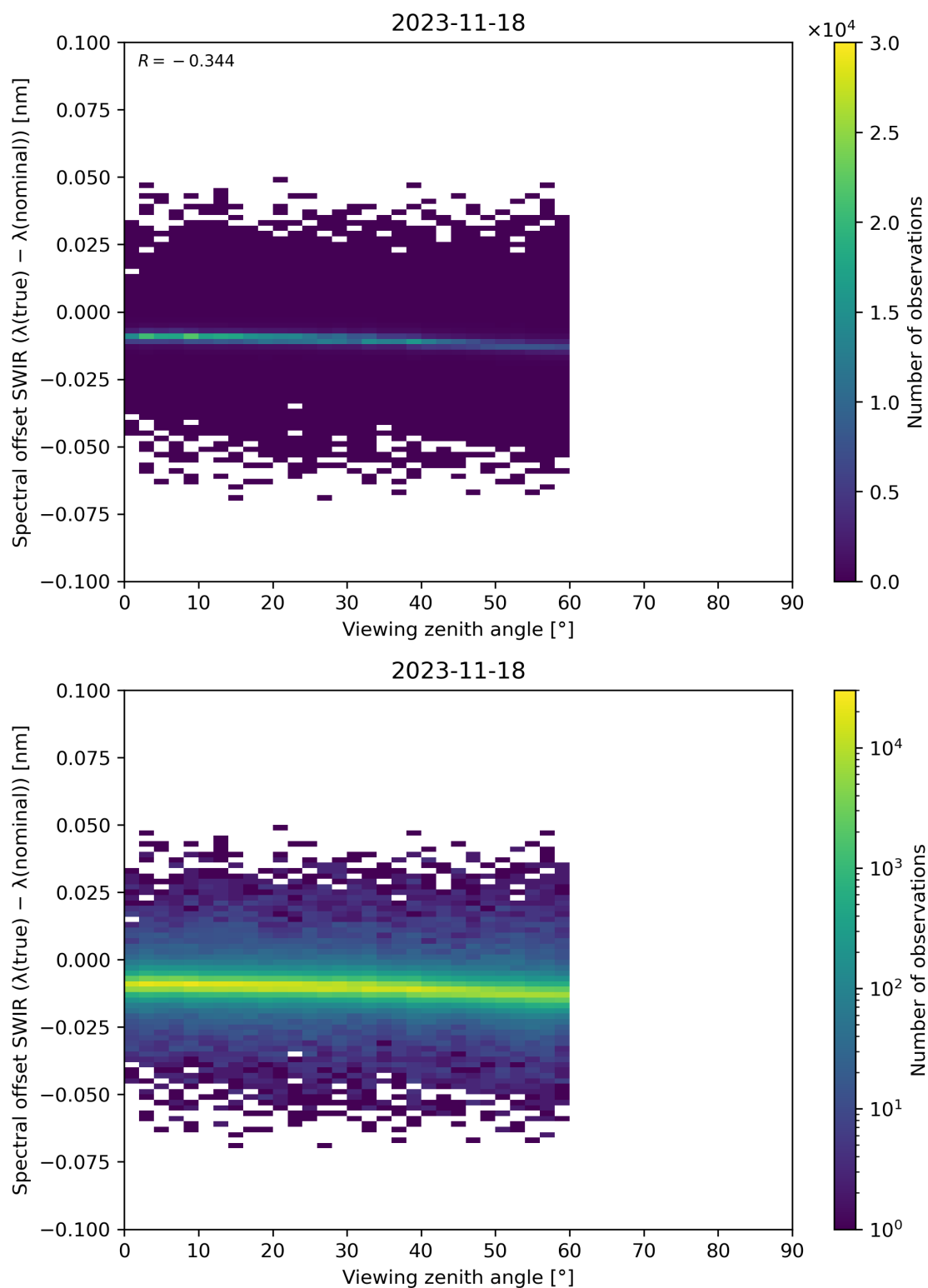
Figure 116: Scatter density plot of “Viewing zenith angle” against “Spectral offset SWIR ( \lambda(\text{true}) - \lambda(\text{nominal}) )” for 2023-11-18 to 2023-11-19.
