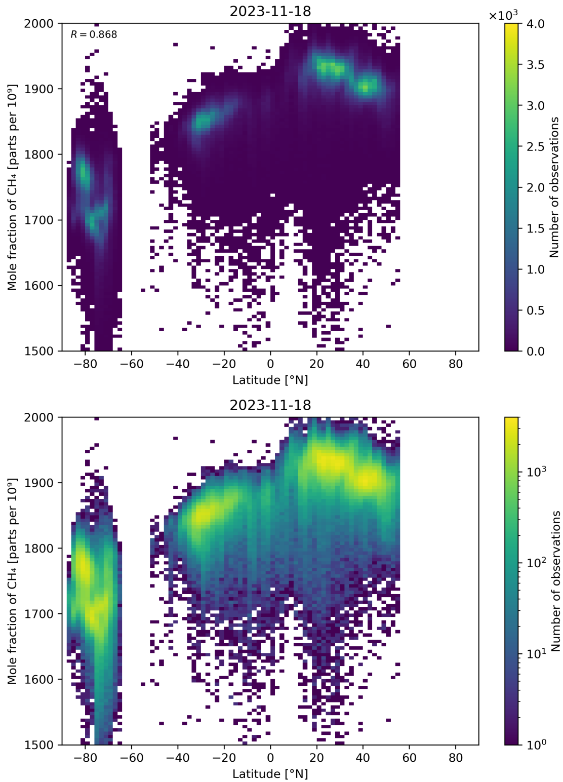
Figure 57: Scatter density plot of “Latitude” against “Mole fraction of CH 4 ” for 2023-11-18 to 2023-11-19.
