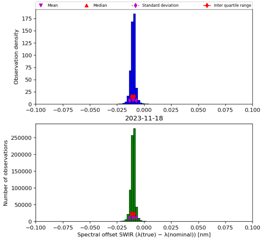
Figure 27: Histogram of “Spectral offset SWIR ( \lambda(\text{true}) - \lambda(\text{nominal}) )” for 2023-11-18 to 2023-11-19
