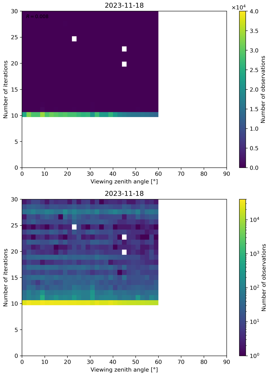
Figure 113: Scatter density plot of “Viewing zenith angle” against “Number of iterations” for 2023-11-18 to 2023-11-19.
