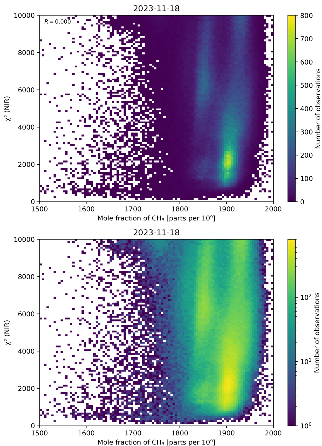
Figure 70: Scatter density plot of “Mole fraction of \text{CH}_4 ” against “ \chi^2 (NIR)” for 2023-11-18 to 2023-11-19.
