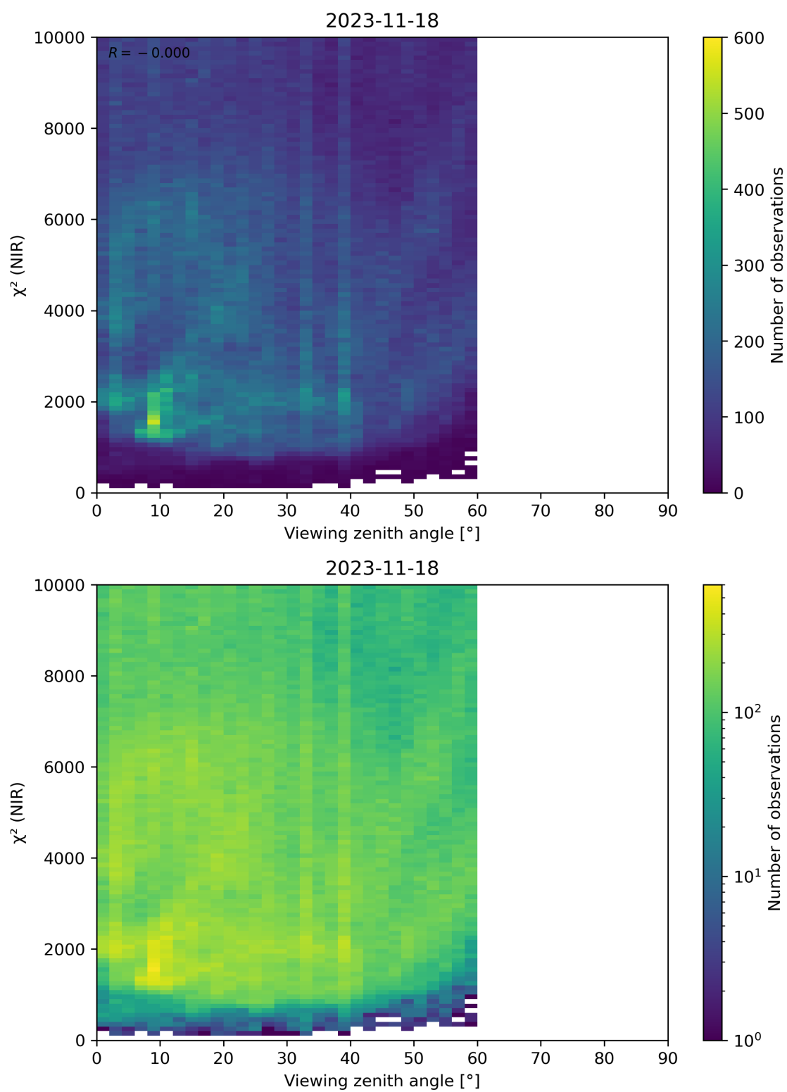
Figure 105: Scatter density plot of “Viewing zenith angle” against “ \chi^2 (NIR)” for 2023-11-18 to 2023-11-19.
