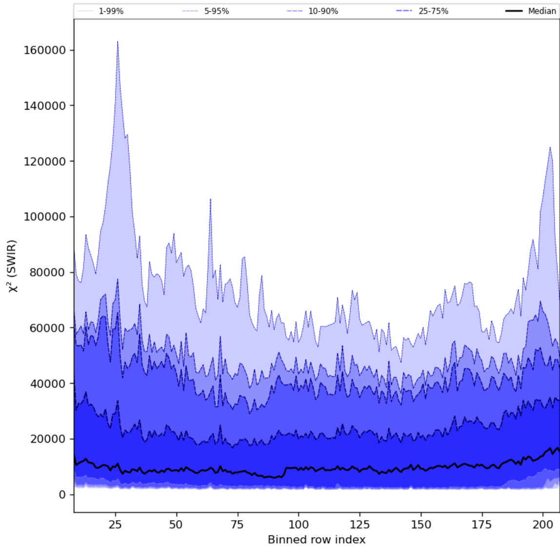
Figure 39: Along track statistics of “ \chi^2 (SWIR)” for 2023-11-18 to 2023-11-19
