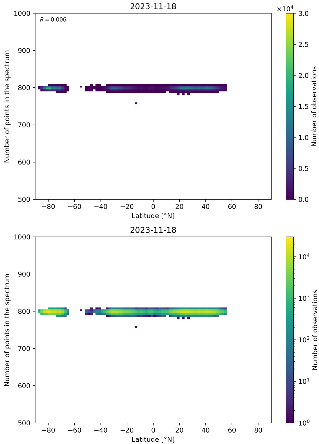
Figure 61: Scatter density plot of “Latitude” against “Number of points in the spectrum” for 2023-11-18 to 2023-11-19.
