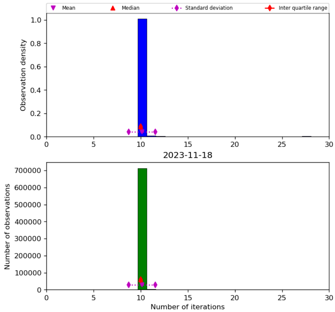
Figure 31: Histogram of “Number of iterations” for 2023-11-18 to 2023-11-19
