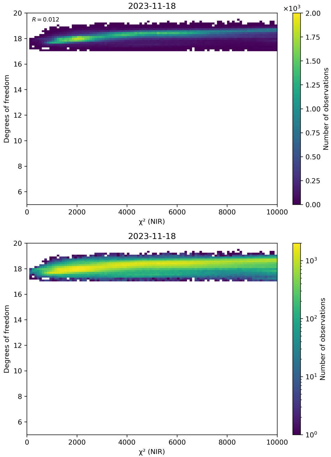
Figure 44: Scatter density plot of “ \chi^2 (NIR)” against “Degrees of freedom” for 2023-11-18 to 2023-11-19.
