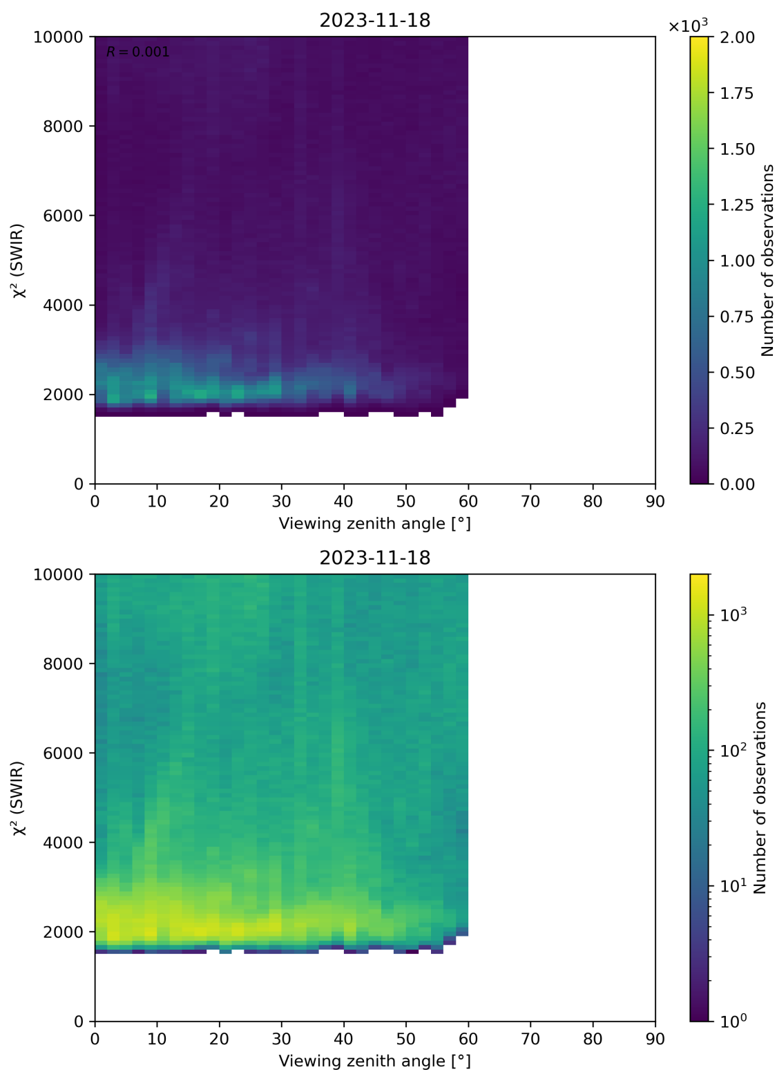
Figure 106: Scatter density plot of “Viewing zenith angle” against “ \chi^2 (SWIR)” for 2023-11-18 to 2023-11-19.
