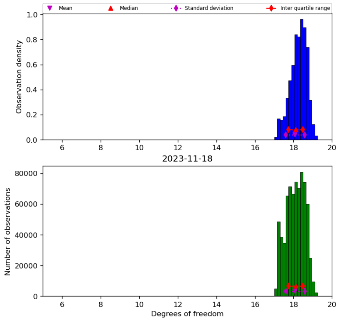
Figure 30: Histogram of “Degrees of freedom” for 2023-11-18 to 2023-11-19
