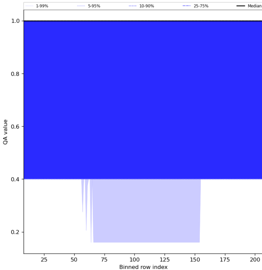
Figure 33: Along track statistics of “QA value” for 2023-11-18 to 2023-11-19
