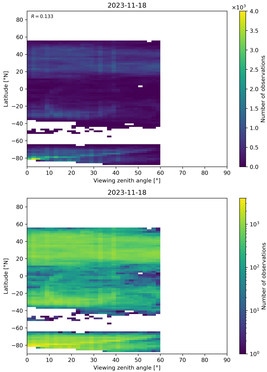
Figure 109: Scatter density plot of “Viewing zenith angle” against “Latitude” for 2023-11-18 to 2023-11-19.
