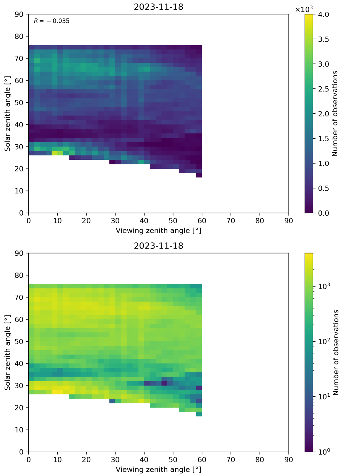
Figure 115: Scatter density plot of “Viewing zenith angle” against “Solar zenith angle” for 2023-11-18 to 2023-11-19.
