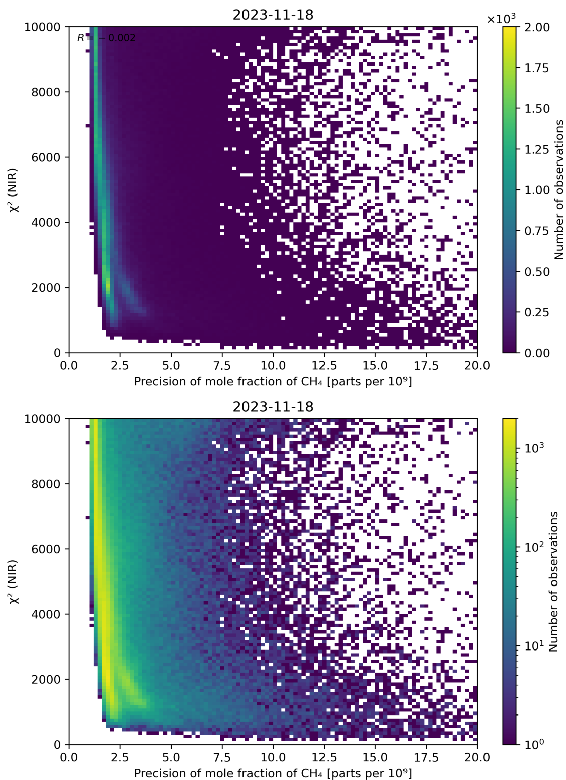
Figure 78: Scatter density plot of “Precision of mole fraction of \text{CH}_4 ” against “ \chi^2 (NIR)” for 2023-11-18 to 2023-11-19.
