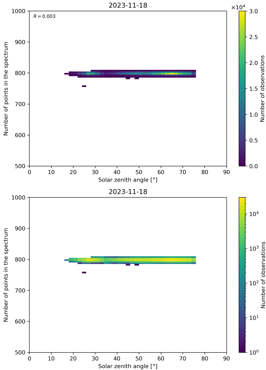
Figure 103: Scatter density plot of “Solar zenith angle” against “Number of points in the spectrum” for 2023-11-18 to 2023-11-19.
