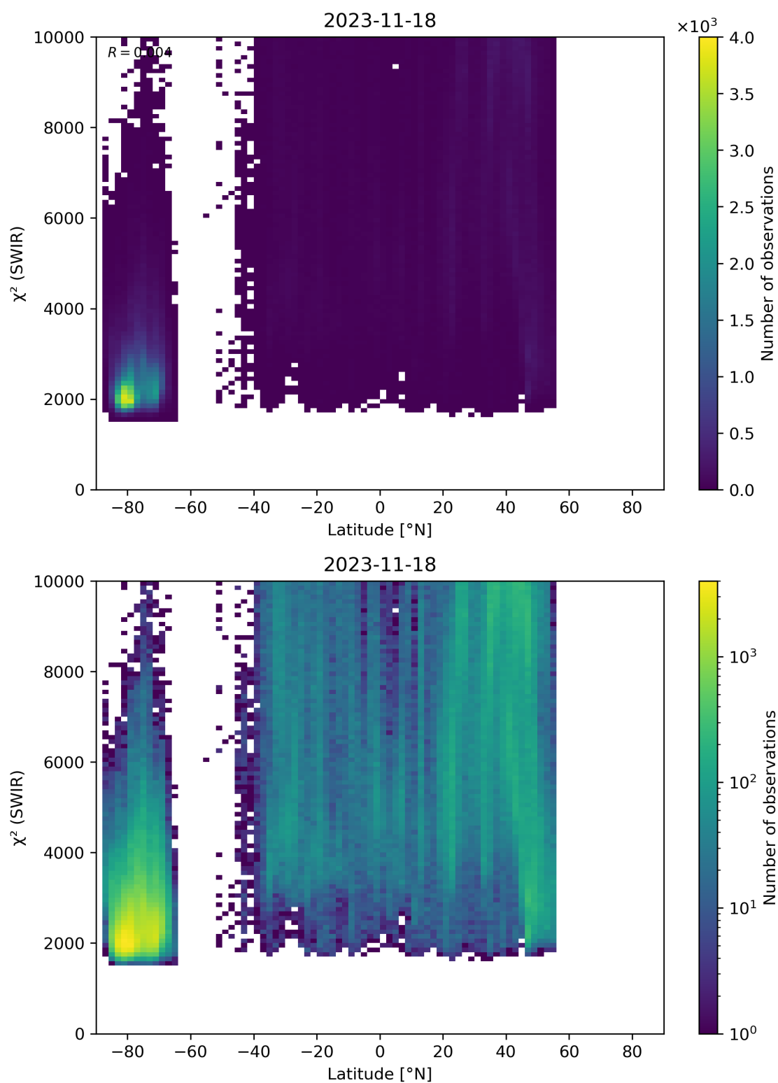
Figure 54: Scatter density plot of “Latitude” against “ \chi^2 (SWIR)” for 2023-11-18 to 2023-11-19.
