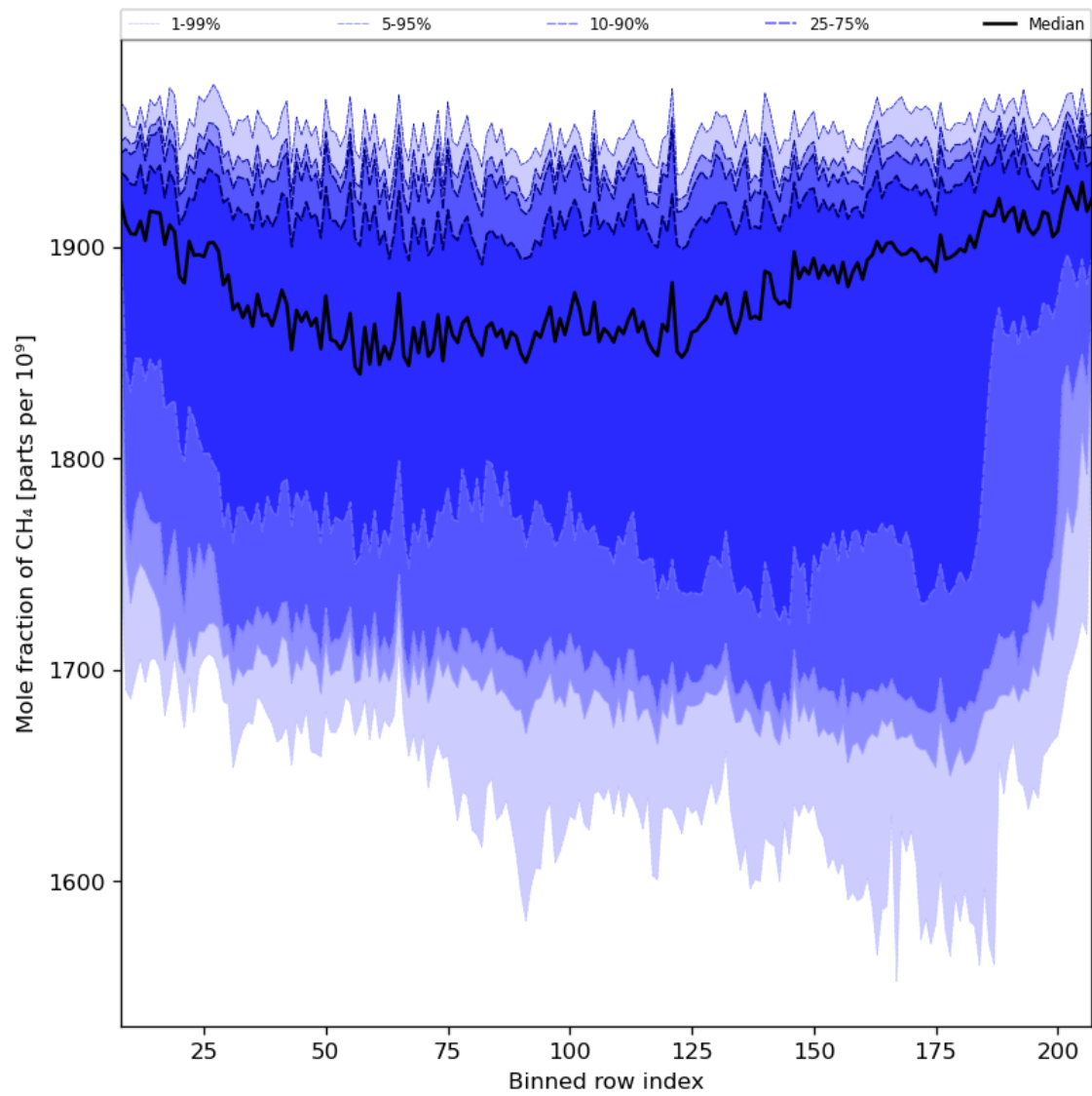
Figure 34: Along track statistics of “Mole fraction of CH 4 ” for 2023-11-18 to 2023-11-19
