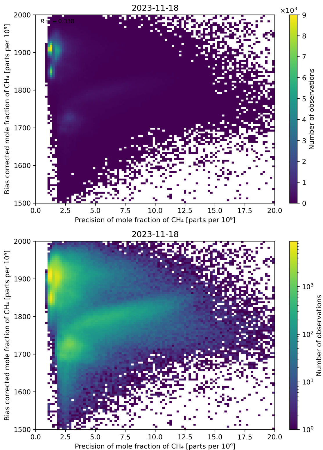
Figure 82: Scatter density plot of “Precision of mole fraction of CH 4 ” against “Bias corrected mole fraction of CH 4 ” for 2023-11-18 to 2023-11-19.
