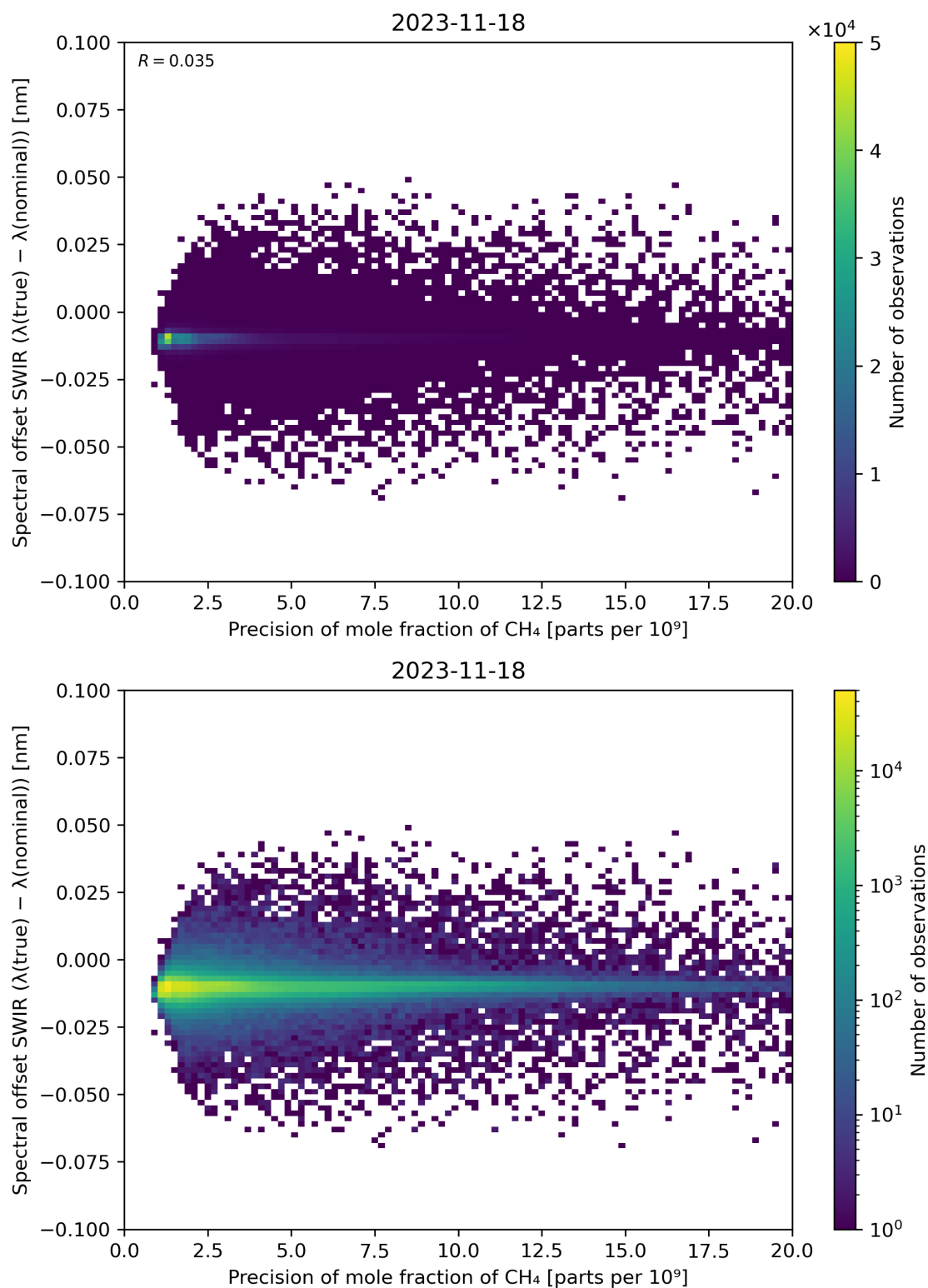
Figure 85: Scatter density plot of “Precision of mole fraction of CH 4 ” against “Spectral offset SWIR ( \lambda(\text{true}) - \lambda(\text{nominal}) )” for 2023-11-18 to 2023-11-19.
