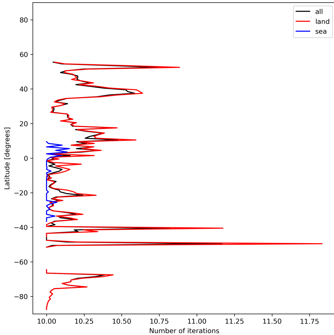
Figure 20: Zonal average of “Number of iterations” for 2023-11-18 to 2023-11-19.
