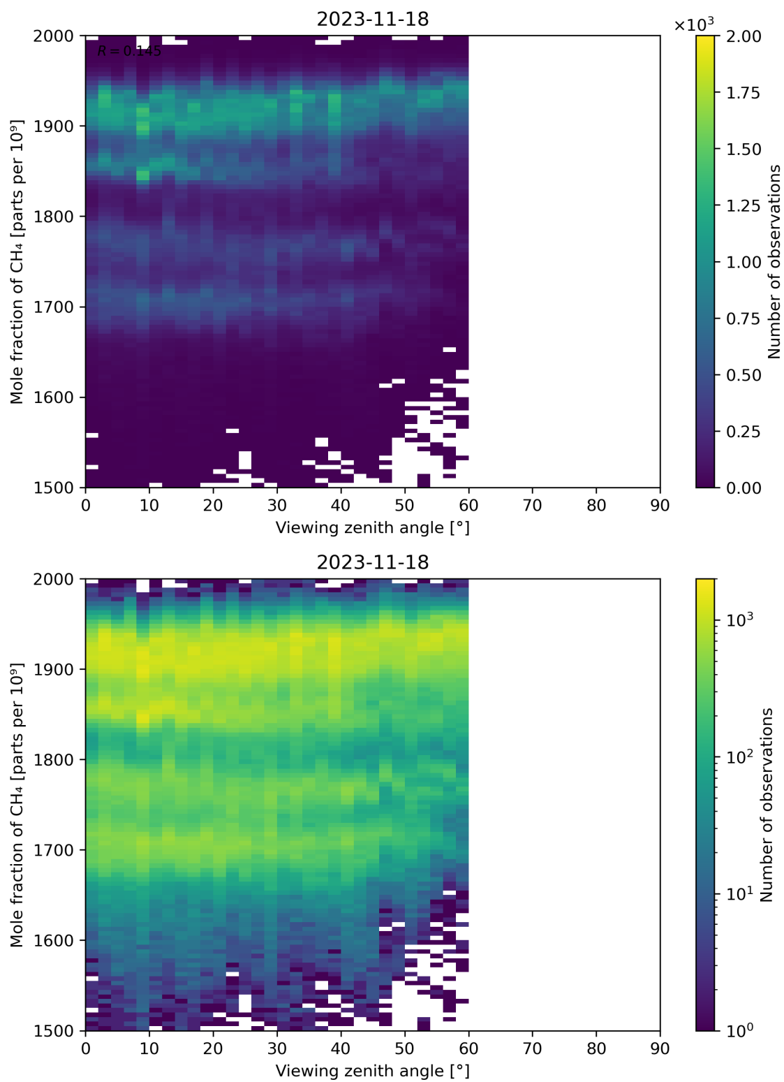
Figure 110: Scatter density plot of “Viewing zenith angle” against “Mole fraction of CH 4 ” for 2023-11-18 to 2023-11-19.
