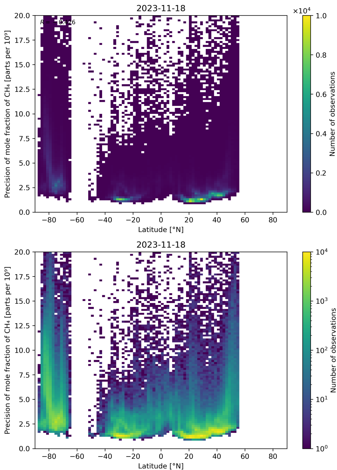
Figure 59: Scatter density plot of “Latitude” against “Precision of mole fraction of CH 4 ” for 2023-11-18 to 2023-11-19.
