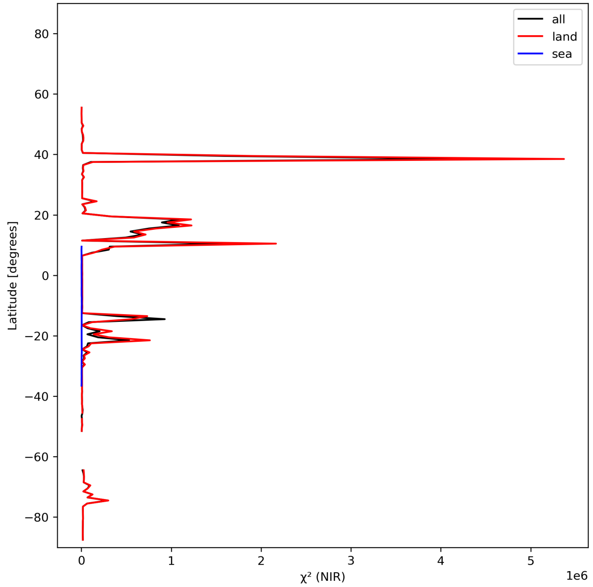
Figure 18: Zonal average of “ \chi^2 (NIR)” for 2023-11-18 to 2023-11-19.
