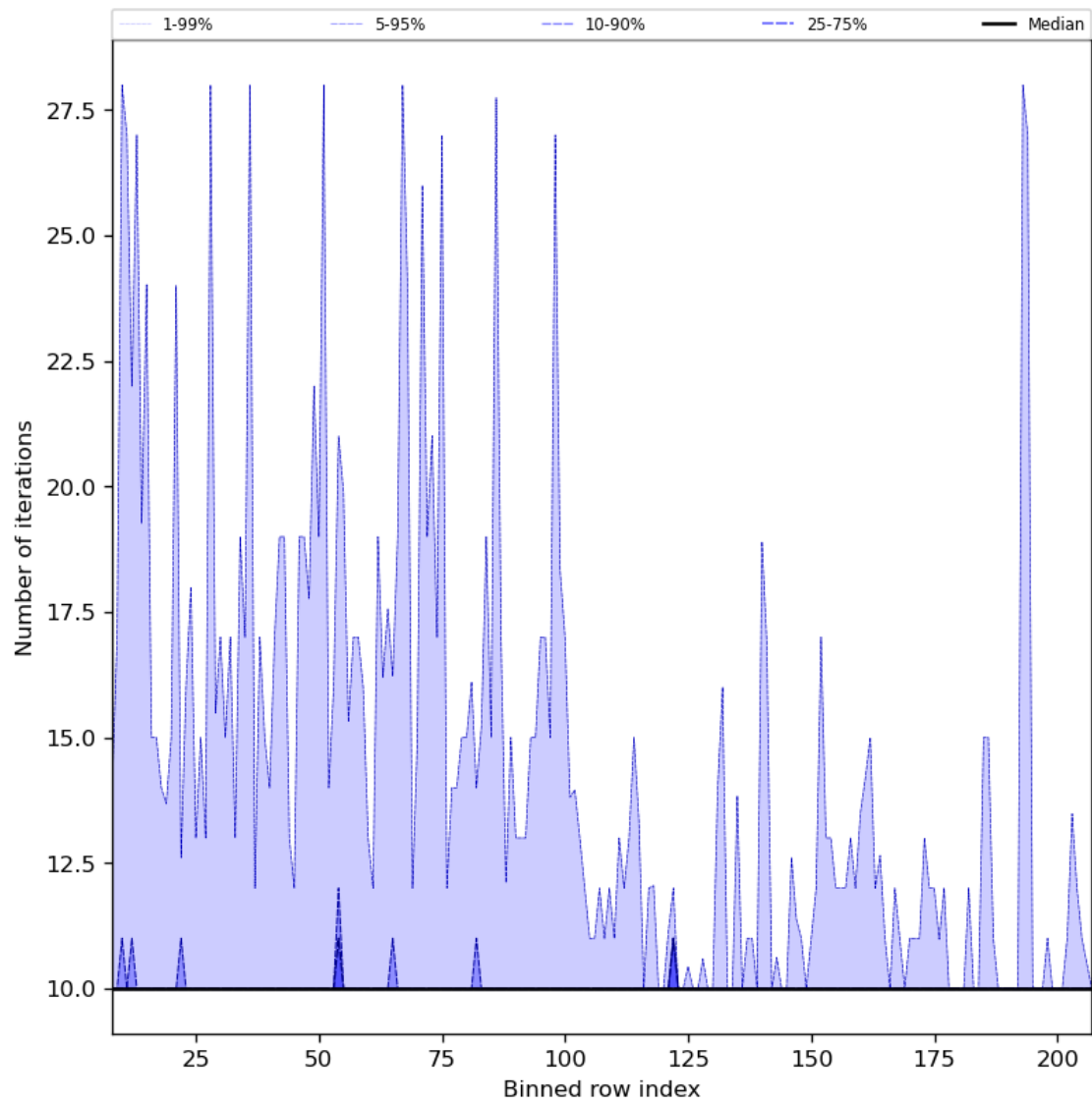
Figure 42: Along track statistics of “Number of iterations” for 2023-11-18 to 2023-11-19
