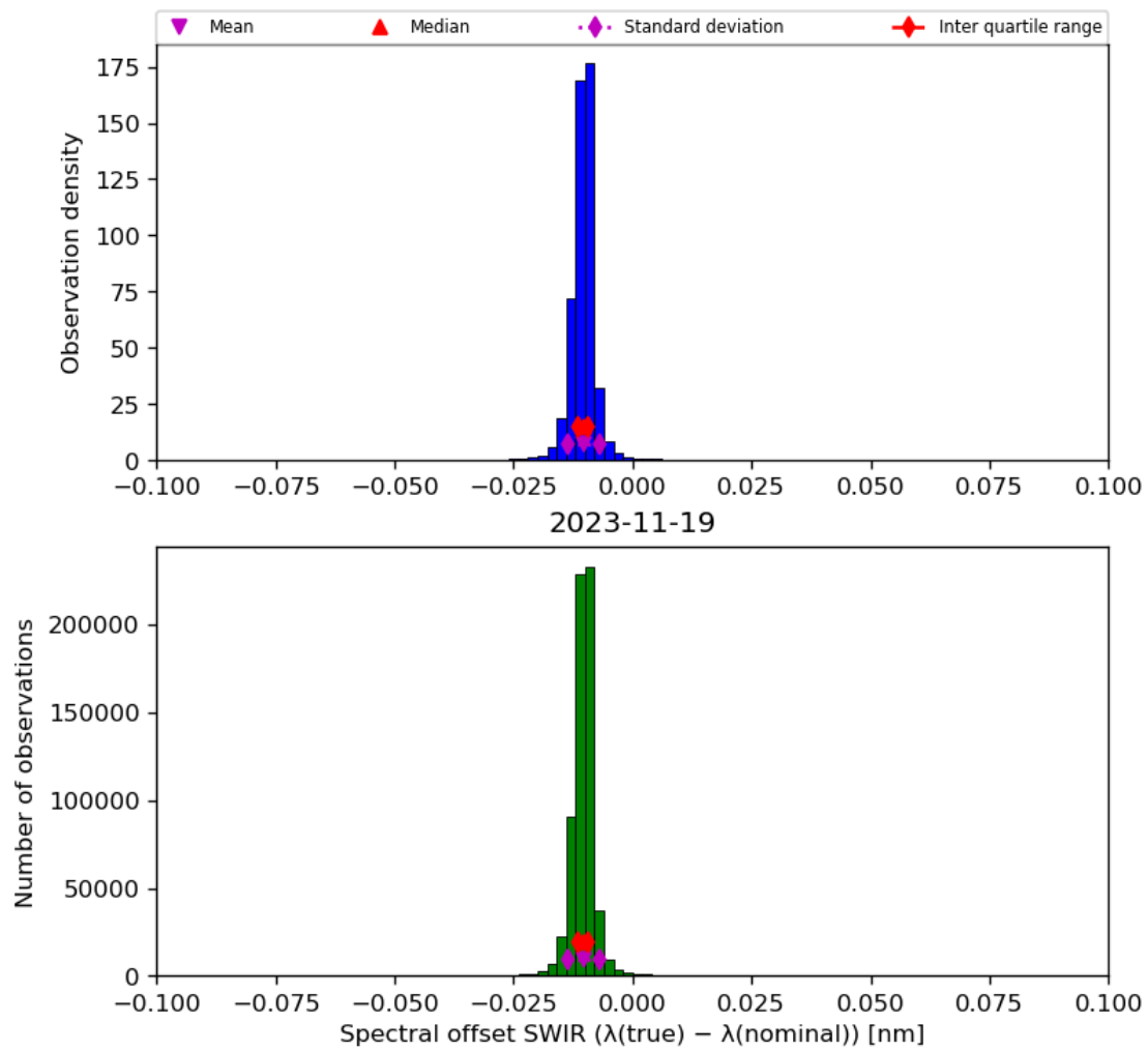
Figure 27: Histogram of “Spectral offset SWIR ( \lambda(\text{true}) - \lambda(\text{nominal}) )” for 2023-11-18 to 2023-11-20
