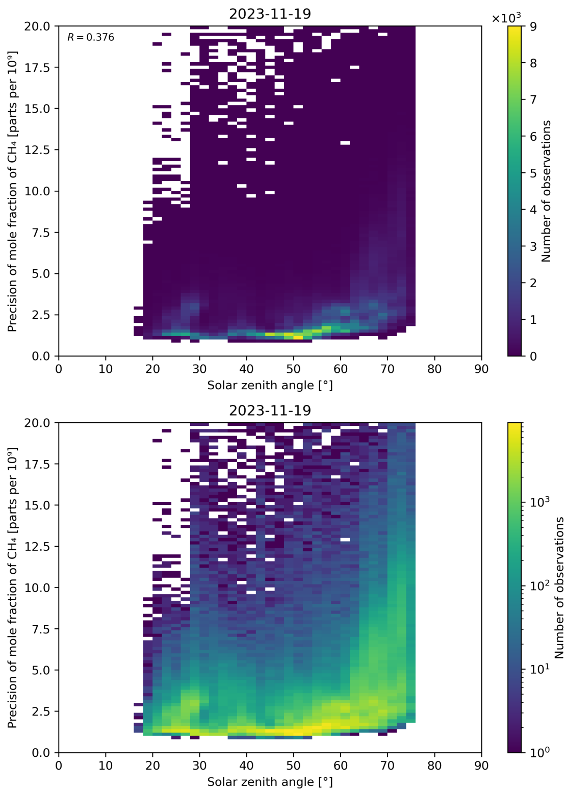
Figure 101: Scatter density plot of “Solar zenith angle” against “Precision of mole fraction of \text{CH}_4 ” for 2023-11-18 to 2023-11-20.
