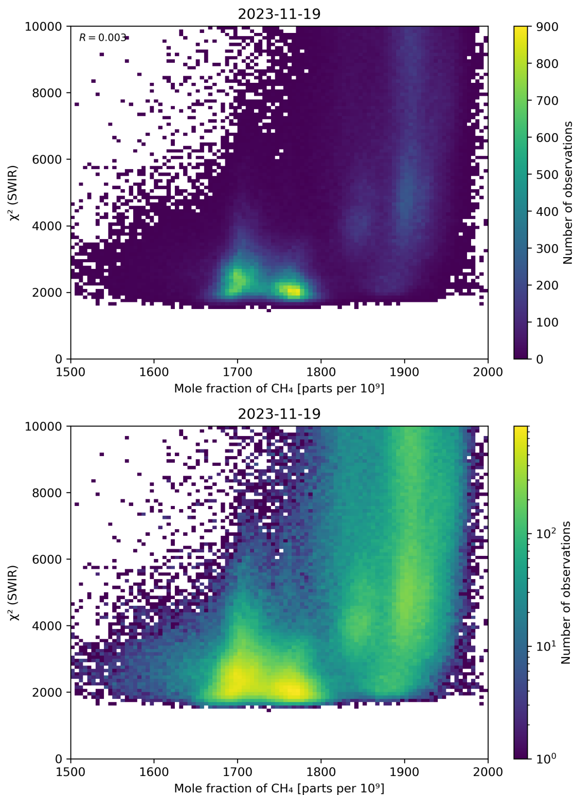
Figure 71: Scatter density plot of “Mole fraction of \text{CH}_4 ” against “ \chi^2 (SWIR)” for 2023-11-18 to 2023-11-20.
