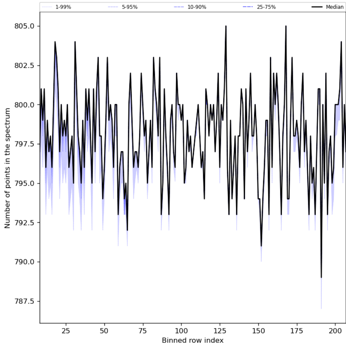
Figure 37: Along track statistics of “Number of points in the spectrum” for 2023-11-18 to 2023-11-20
