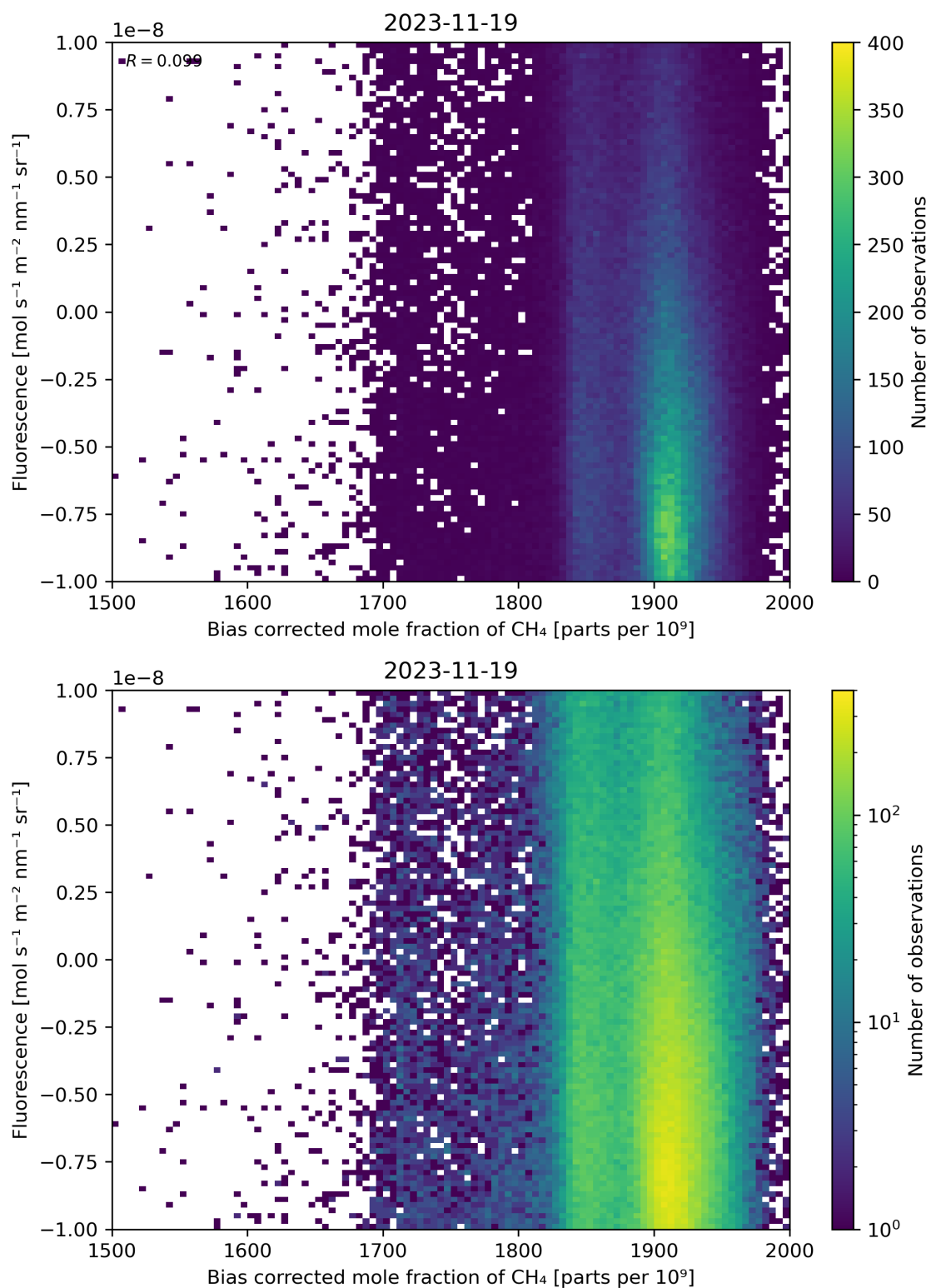
Figure 66: Scatter density plot of “Bias corrected mole fraction of \text{CH}_4 ” against “Fluorescence” for 2023-11-18 to 2023-11-20.
