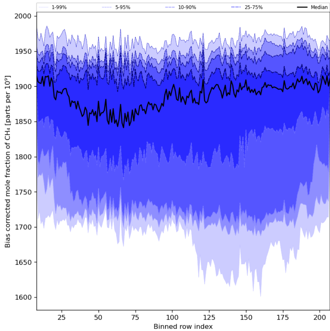
Figure 36: Along track statistics of “Bias corrected mole fraction of CH 4 ” for 2023-11-18 to 2023-11-20
