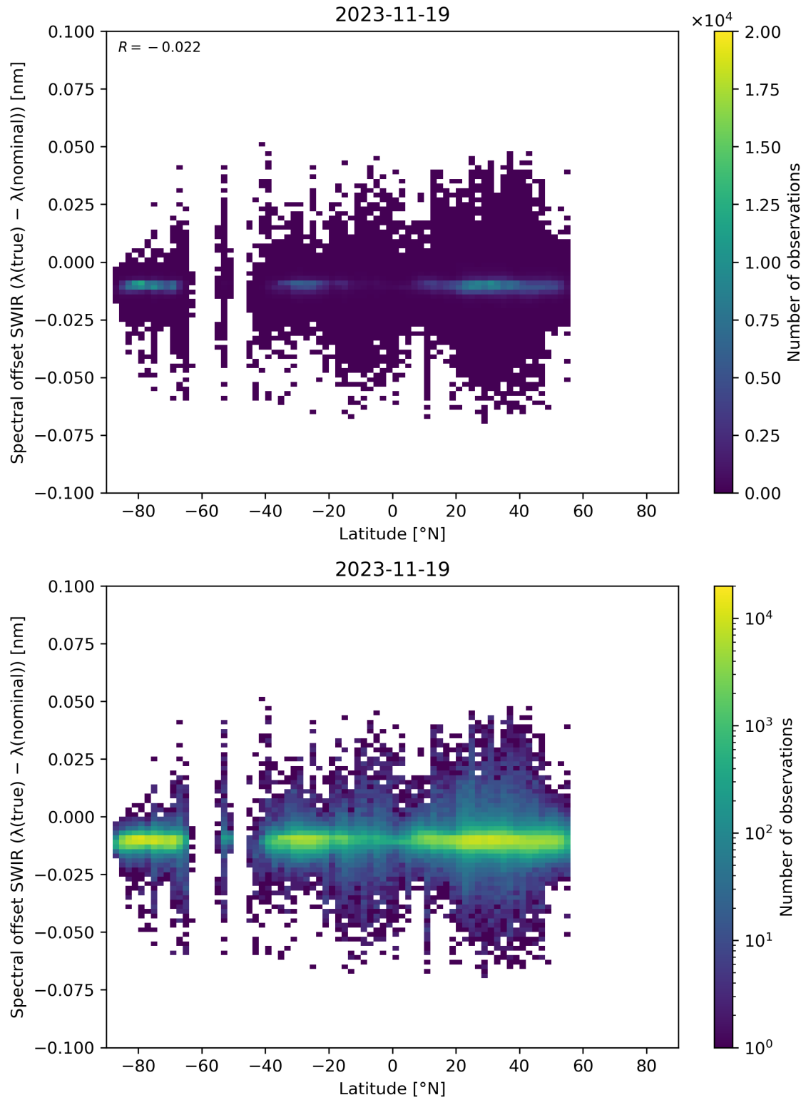
Figure 62: Scatter density plot of “Latitude” against “Spectral offset SWIR ( \lambda(\text{true}) - \lambda(\text{nominal}) )” for 2023-11-18 to 2023-11-20.
