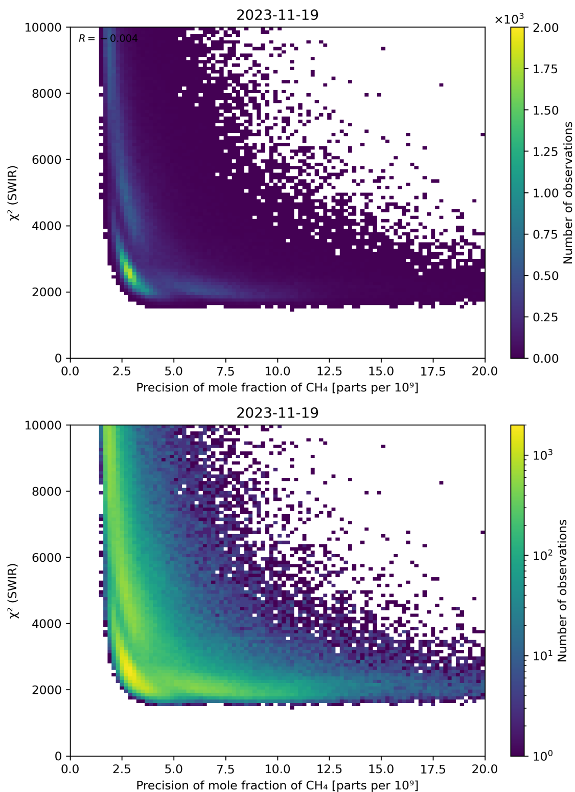
Figure 79: Scatter density plot of “Precision of mole fraction of \text{CH}_4 ” against “ \chi^2 (SWIR)” for 2023-11-18 to 2023-11-20.
