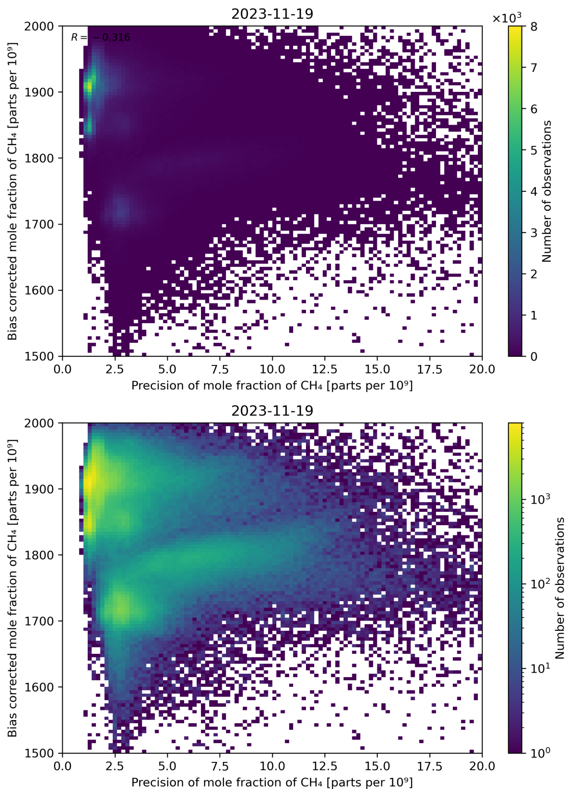
Figure 82: Scatter density plot of “Precision of mole fraction of CH 4 ” against “Bias corrected mole fraction of CH 4 ” for 2023-11-18 to 2023-11-20.
