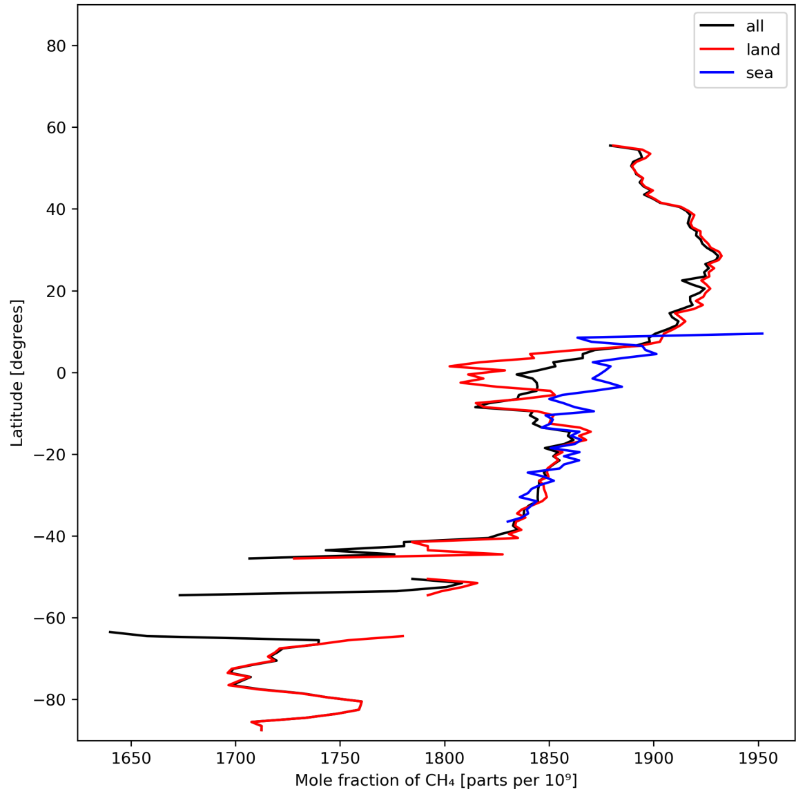
Figure 12: Zonal average of “Mole fraction of CH 4 ” for 2023-11-18 to 2023-11-20.
