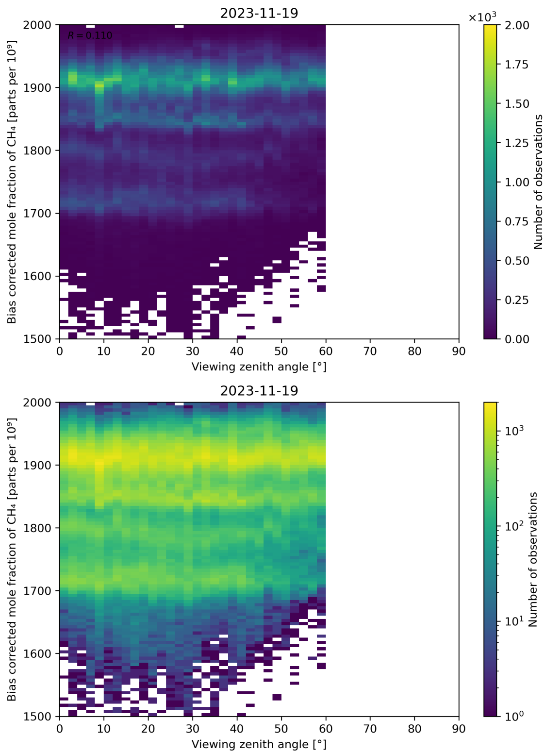
Figure 111: Scatter density plot of “Viewing zenith angle” against “Bias corrected mole fraction of \text{CH}_4 ” for 2023-11-18 to 2023-11-20.
