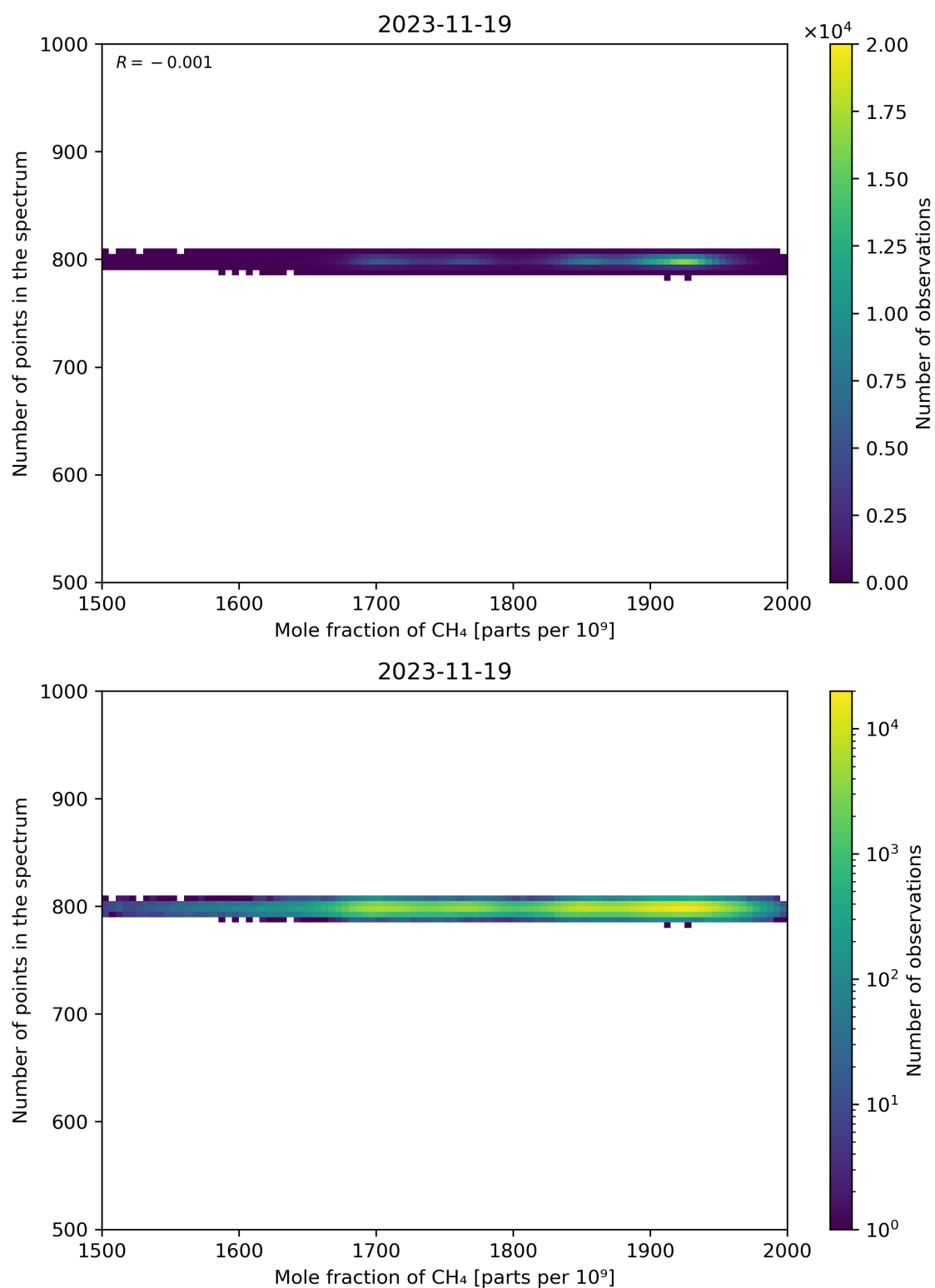
Figure 77: Scatter density plot of “Mole fraction of CH 4 ” against “Number of points in the spectrum” for 2023-11-18 to 2023-11-20.
