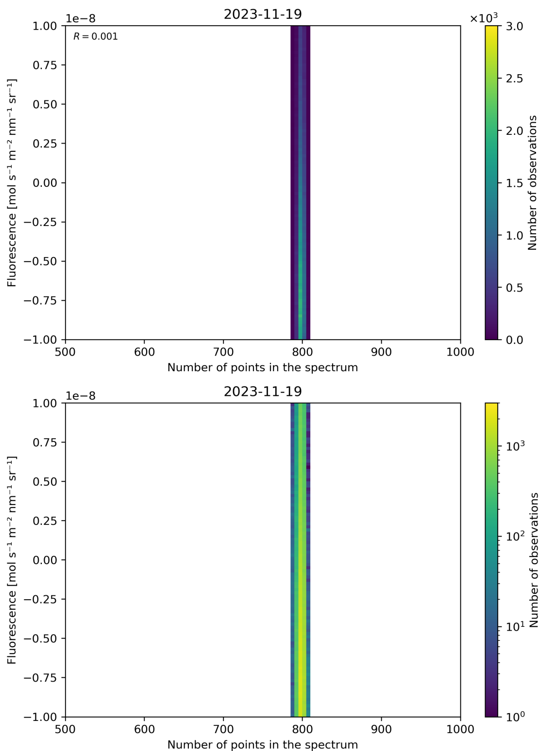
Figure 91: Scatter density plot of “Number of points in the spectrum” against “Fluorescence” for 2023-11-18 to 2023-11-20.
