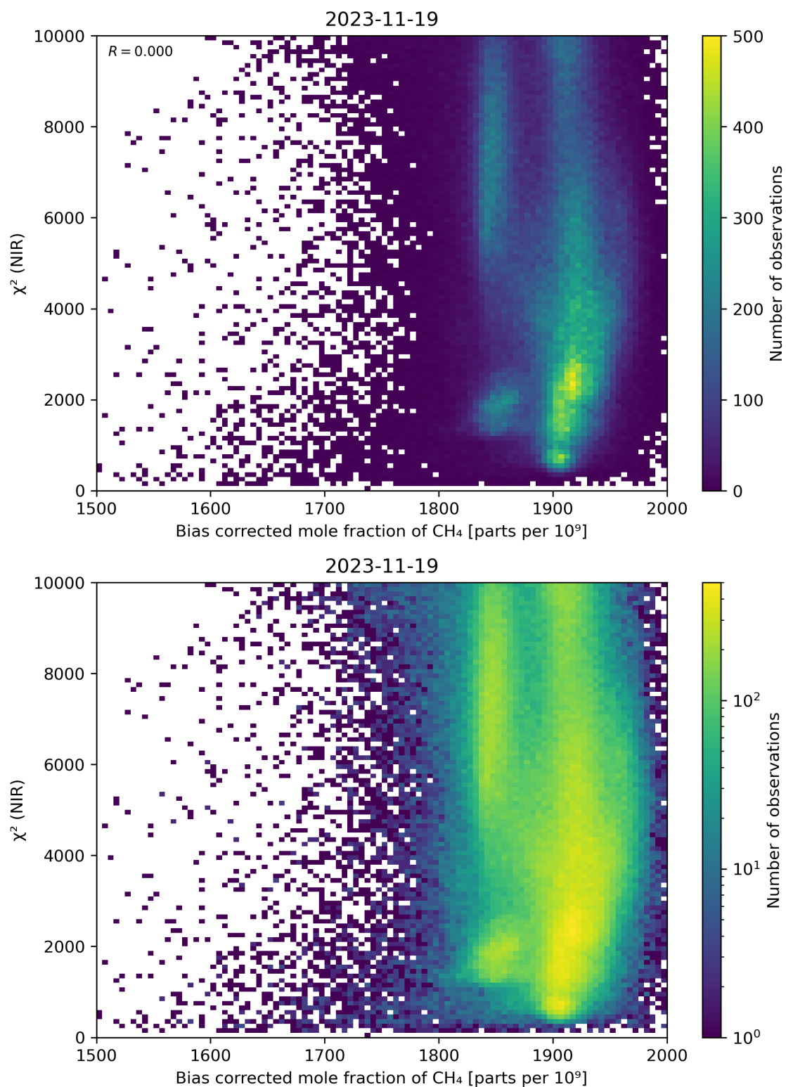
Figure 63: Scatter density plot of “Bias corrected mole fraction of CH 4 ” against “ \chi^2 (NIR)” for 2023-11-18 to 2023-11-20.
