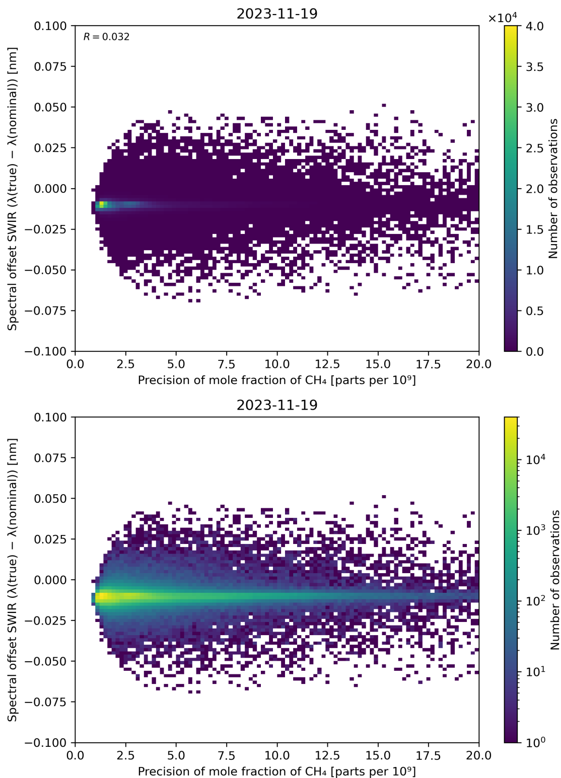
Figure 85: Scatter density plot of “Precision of mole fraction of \text{CH}_4 ” against “Spectral offset SWIR ( \lambda(\text{true}) - \lambda(\text{nominal}) )” for 2023-11-18 to 2023-11-20.
