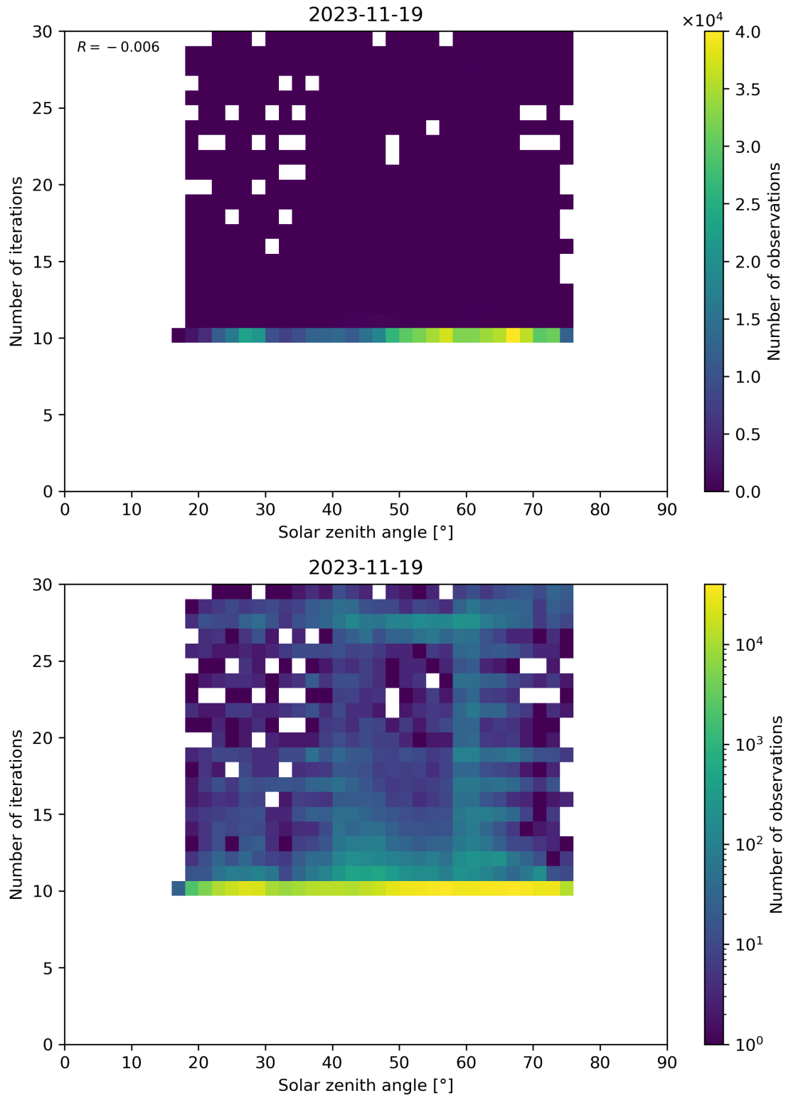
Figure 102: Scatter density plot of “Solar zenith angle” against “Number of iterations” for 2023-11-18 to 2023-11-20.
