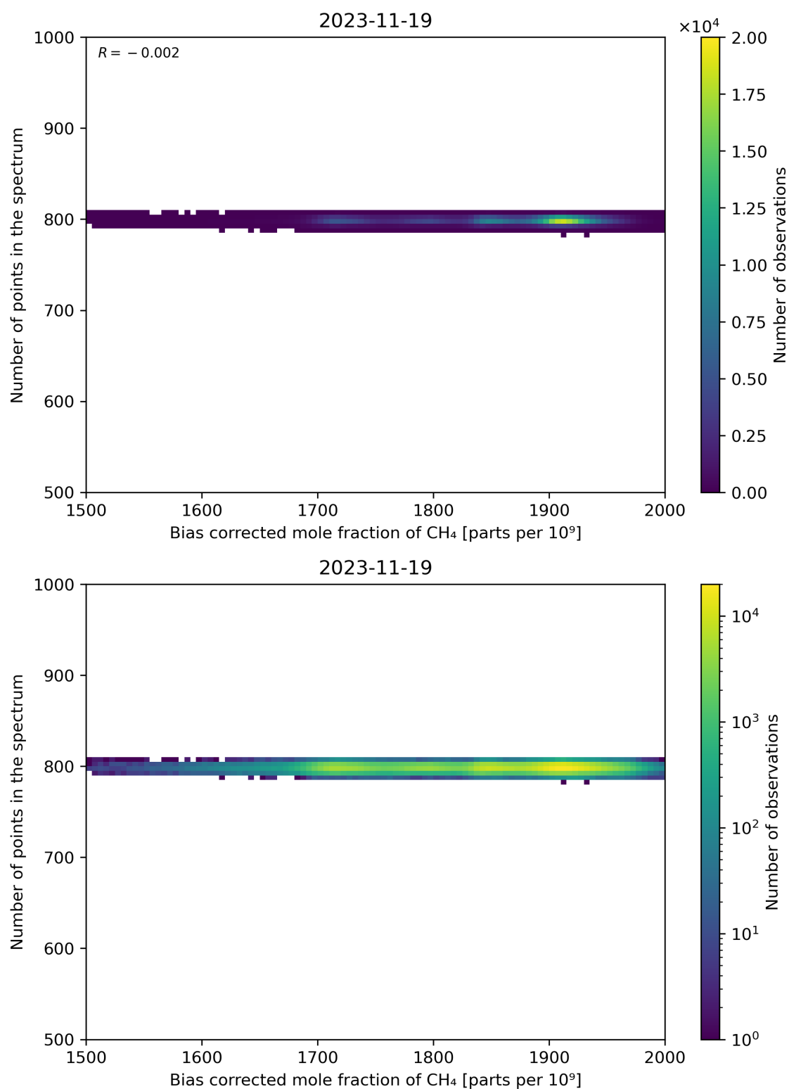
Figure 68: Scatter density plot of “Bias corrected mole fraction of CH 4 ” against “Number of points in the spectrum” for 2023-11-18 to 2023-11-20.
