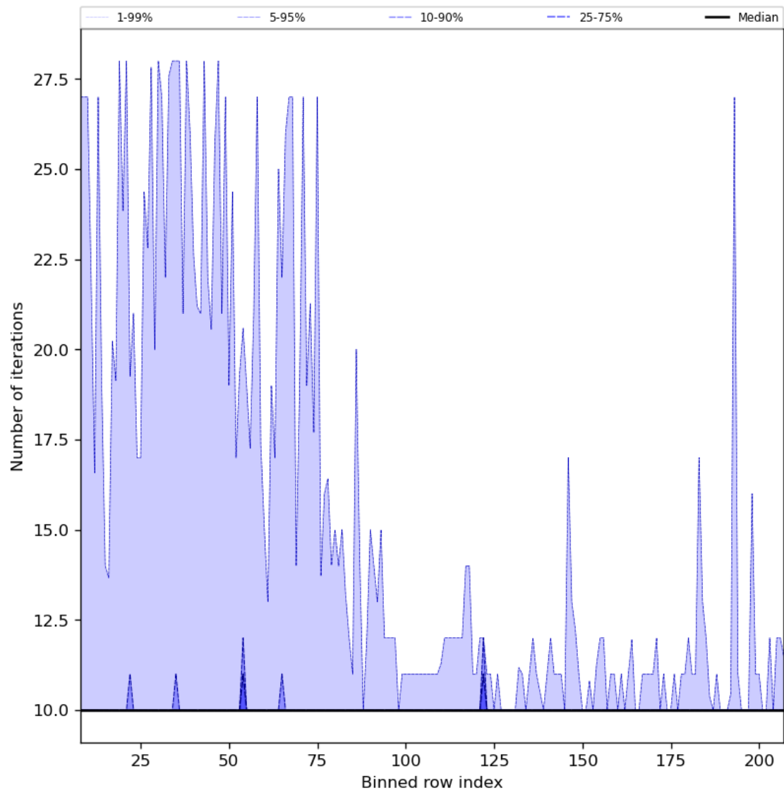
Figure 42: Along track statistics of “Number of iterations” for 2023-11-18 to 2023-11-20
