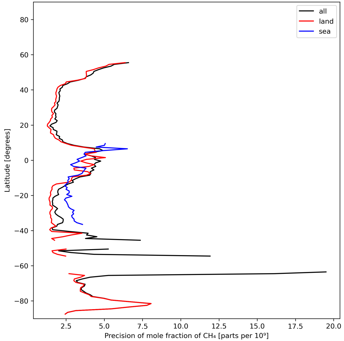
Figure 13: Zonal average of “Precision of mole fraction of CH 4 ” for 2023-11-18 to 2023-11-20.
