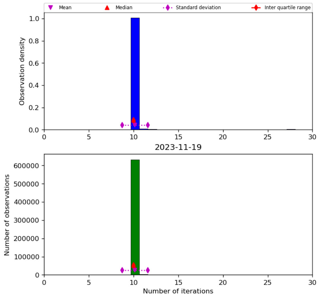
Figure 31: Histogram of “Number of iterations” for 2023-11-18 to 2023-11-20
