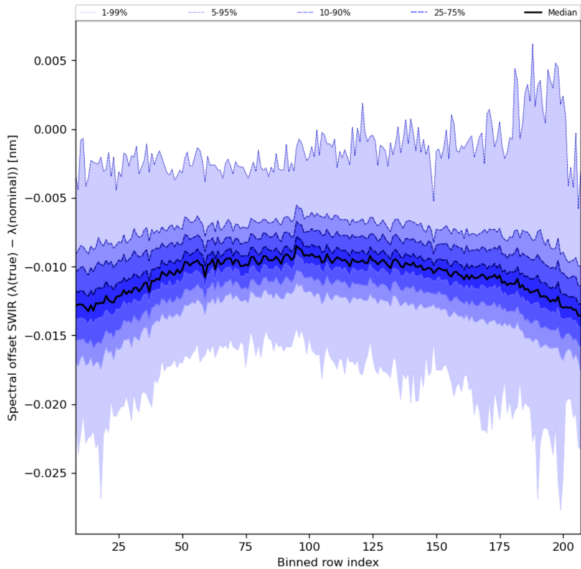
Figure 38: Along track statistics of “Spectral offset SWIR ( \lambda(\text{true}) - \lambda(\text{nominal}) )” for 2023-11-18 to 2023-11-20
