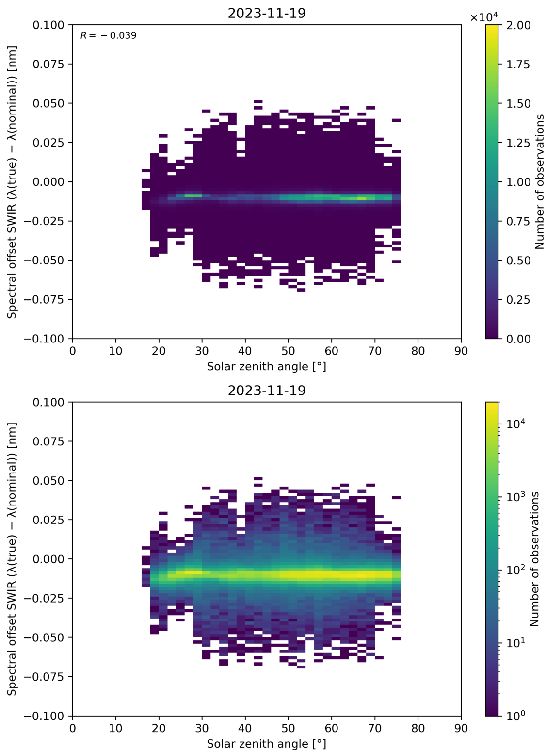
Figure 104: Scatter density plot of “Solar zenith angle” against “Spectral offset SWIR ( \lambda(\text{true}) - \lambda(\text{nominal}) )” for 2023-11-18 to 2023-11-20.
