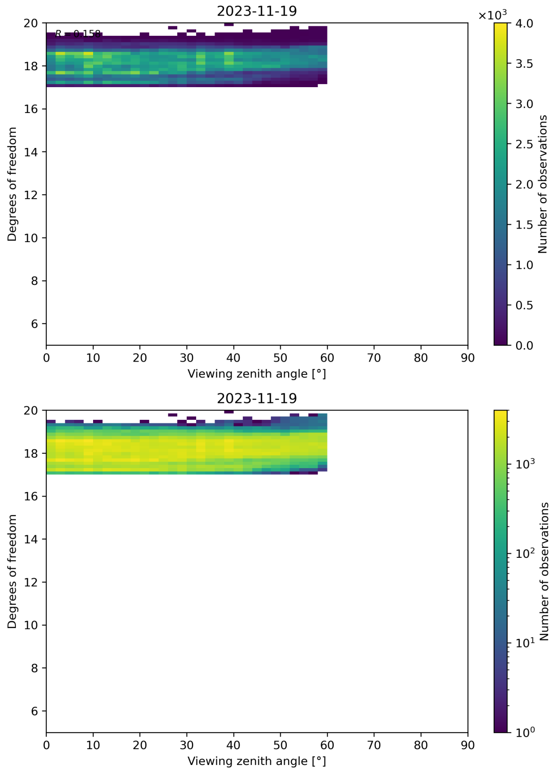
Figure 107: Scatter density plot of “Viewing zenith angle” against “Degrees of freedom” for 2023-11-18 to 2023-11-20.
