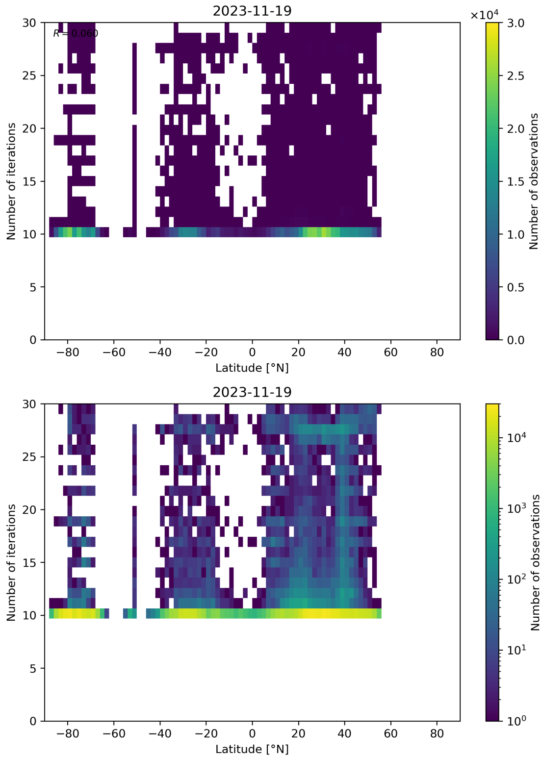
Figure 60: Scatter density plot of “Latitude” against “Number of iterations” for 2023-11-18 to 2023-11-20.
