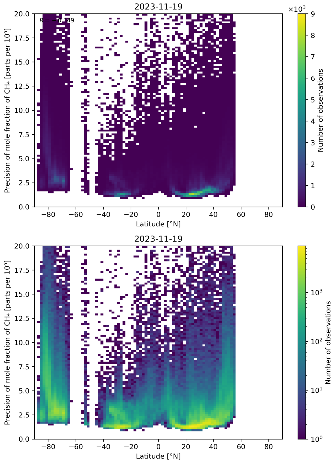
Figure 59: Scatter density plot of “Latitude” against “Precision of mole fraction of CH 4 ” for 2023-11-18 to 2023-11-20.
