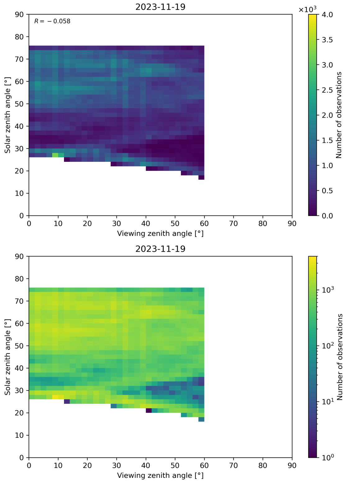
Figure 115: Scatter density plot of “Viewing zenith angle” against “Solar zenith angle” for 2023-11-18 to 2023-11-20.
