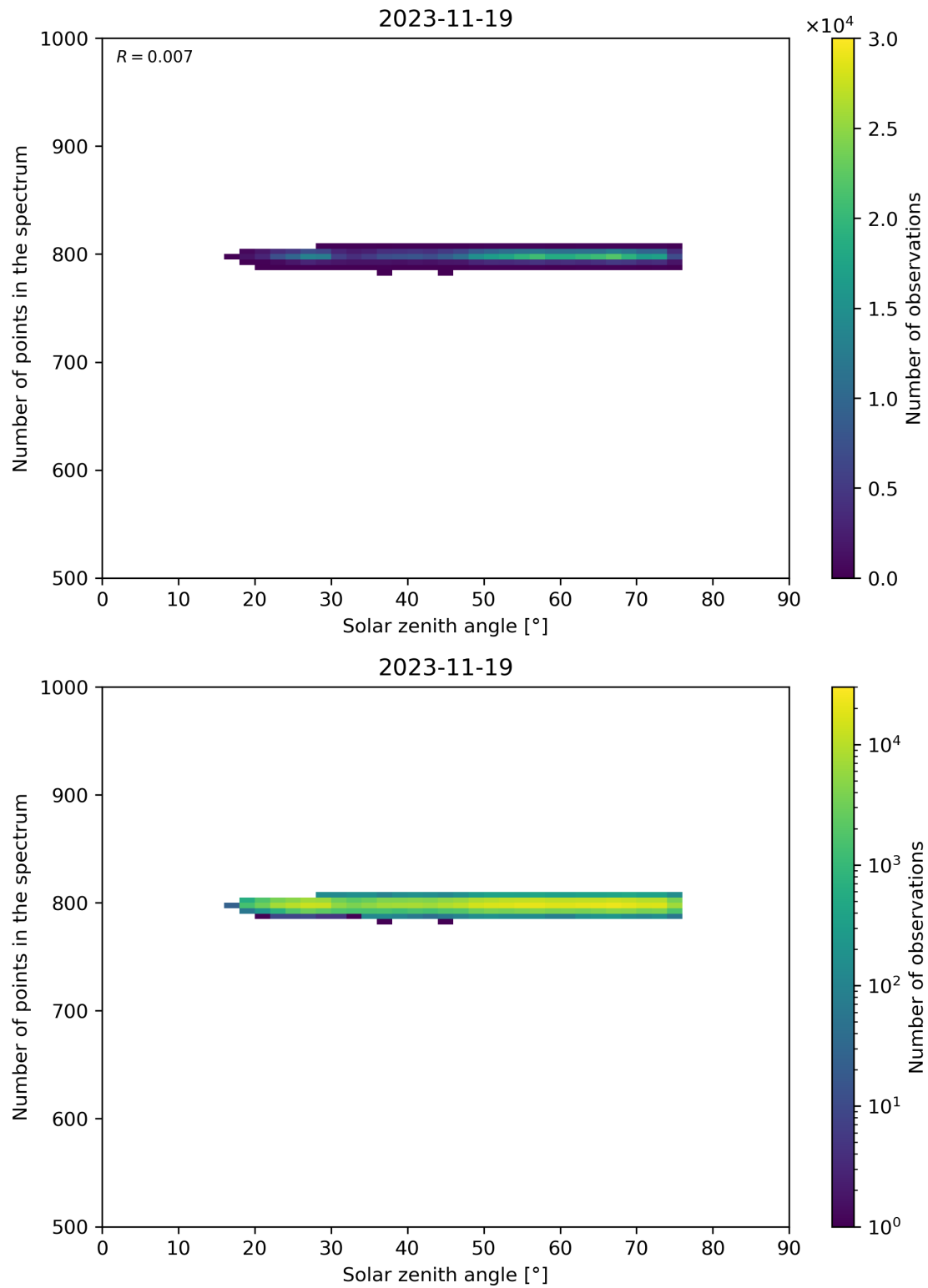
Figure 103: Scatter density plot of “Solar zenith angle” against “Number of points in the spectrum” for 2023-11-18 to 2023-11-20.
