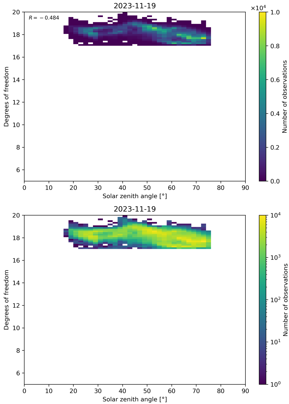
Figure 96: Scatter density plot of “Solar zenith angle” against “Degrees of freedom” for 2023-11-18 to 2023-11-20.
