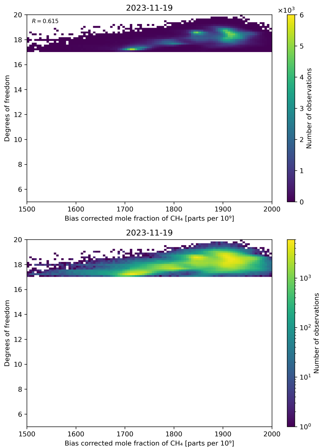
Figure 65: Scatter density plot of “Bias corrected mole fraction of CH 4 ” against “Degrees of freedom” for 2023-11-18 to 2023-11-20.
