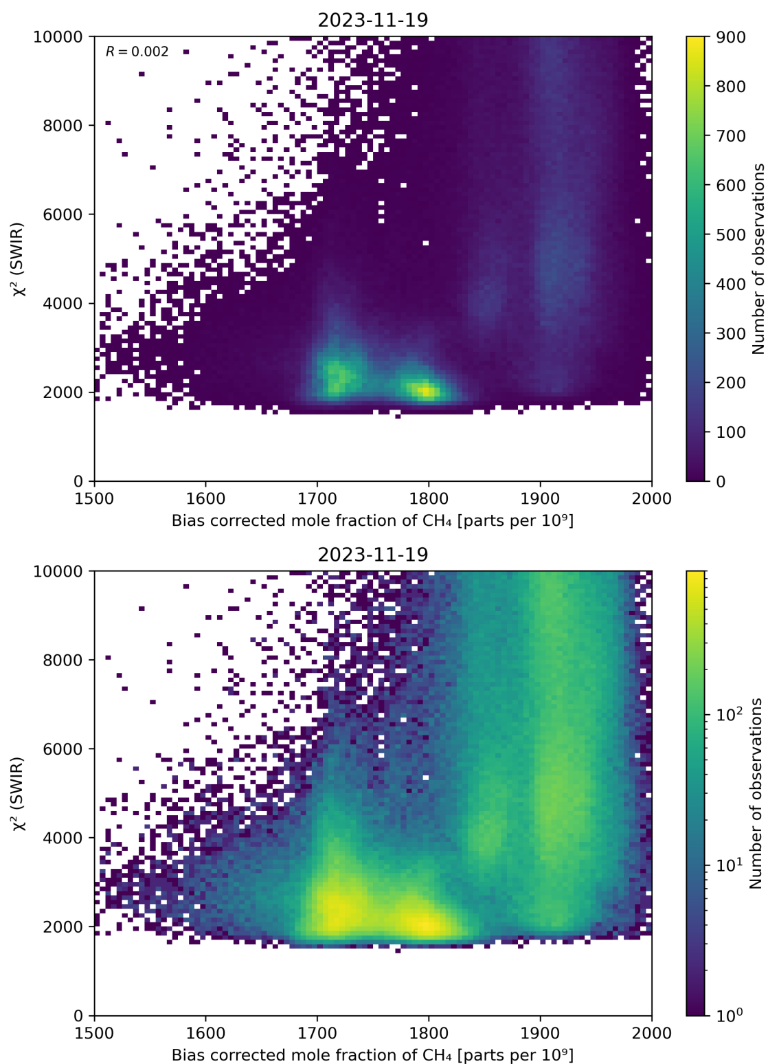
Figure 64: Scatter density plot of “Bias corrected mole fraction of CH 4 ” against “ \chi^2 (SWIR)” for 2023-11-18 to 2023-11-20.
