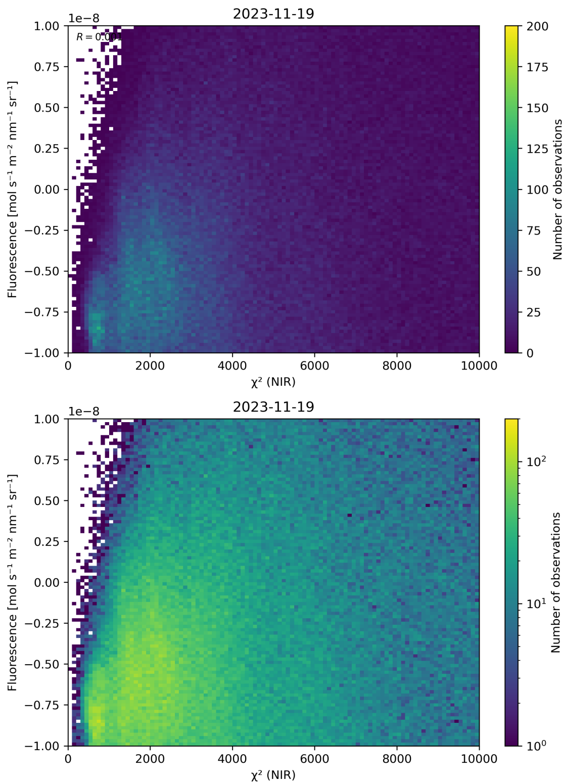
Figure 45: Scatter density plot of “ \chi^2 (NIR)” against “Fluorescence” for 2023-11-18 to 2023-11-20.
