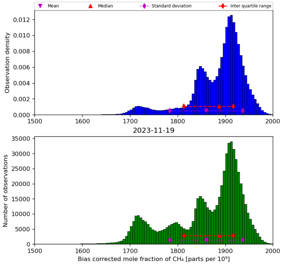
Figure 25: Histogram of “Bias corrected mole fraction of CH 4 ” for 2023-11-18 to 2023-11-20
