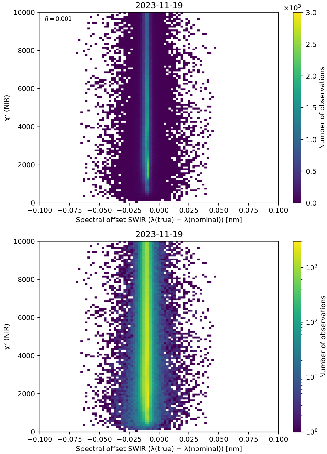
Figure 117: Scatter density plot of “Spectral offset SWIR ( \lambda(\text{true}) - \lambda(\text{nominal}) )” against “ \chi^2 (NIR)” for 2023-11-18 to 2023-11-20.
