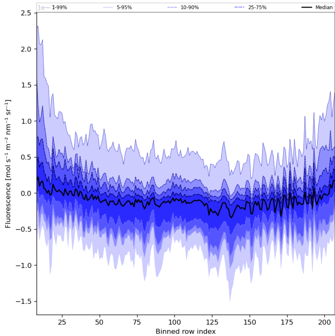
Figure 43: Along track statistics of “Fluorescence” for 2023-11-18 to 2023-11-20
