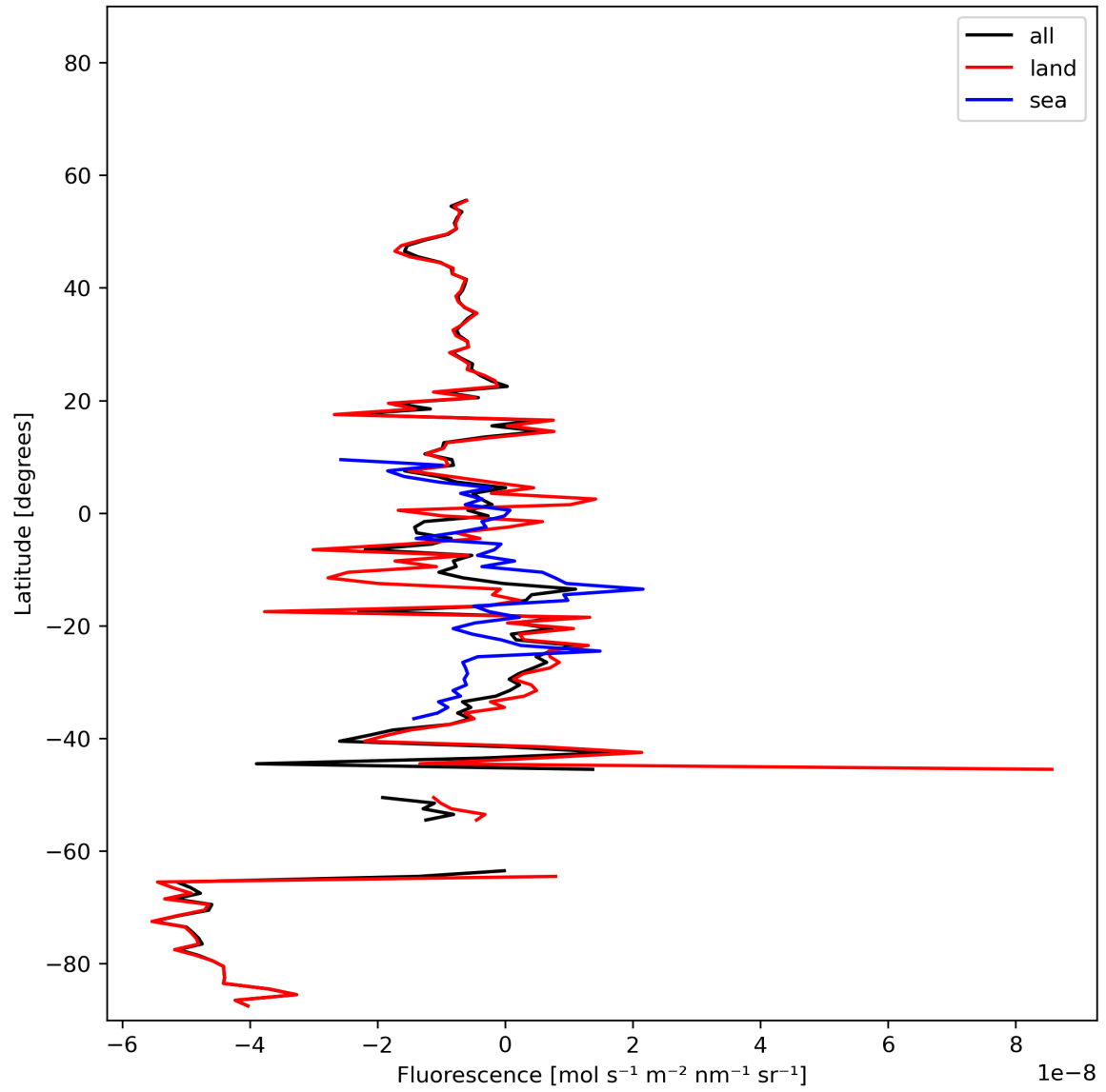
Figure 21: Zonal average of “Fluorescence” for 2023-11-18 to 2023-11-20.
