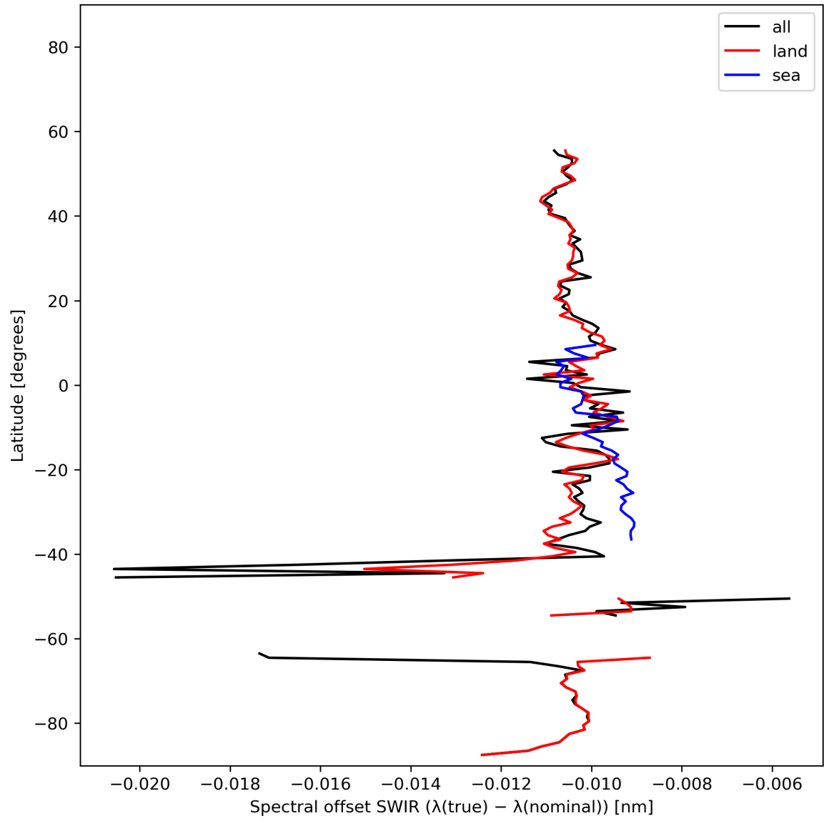
Figure 16: Zonal average of “Spectral offset SWIR ( \lambda(\text{true}) - \lambda(\text{nominal}) )” for 2023-11-18 to 2023-11-20.
