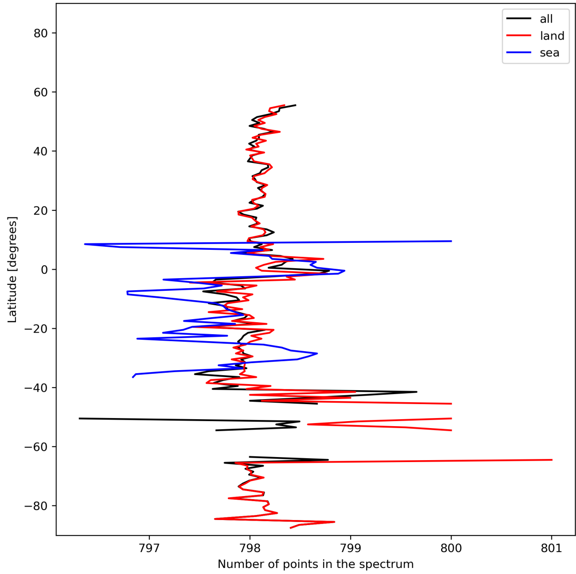
Figure 15: Zonal average of “Number of points in the spectrum” for 2023-11-18 to 2023-11-20.
