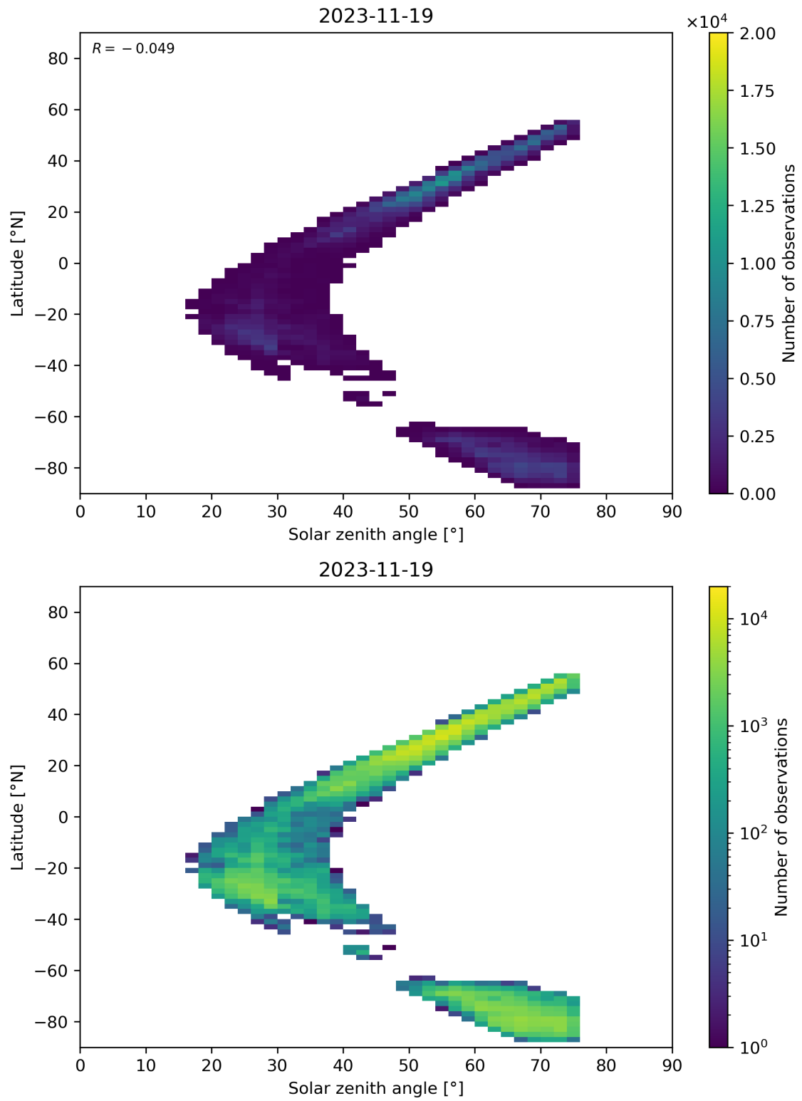
Figure 98: Scatter density plot of “Solar zenith angle” against “Latitude” for 2023-11-18 to 2023-11-20.
