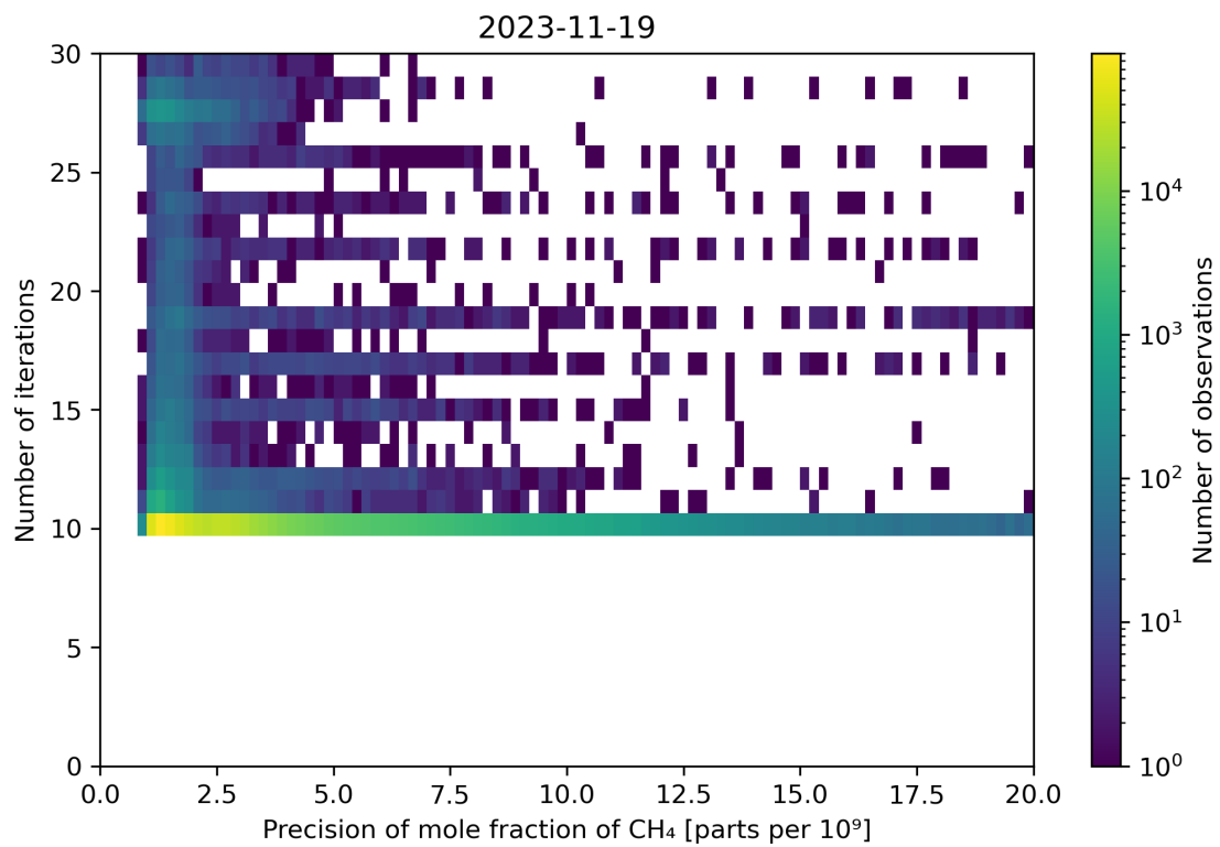
Figure 83: Scatter density plot of “Precision of mole fraction of CH 4 ” against “Number of iterations” for 2023-11-18 to 2023-11-20.
