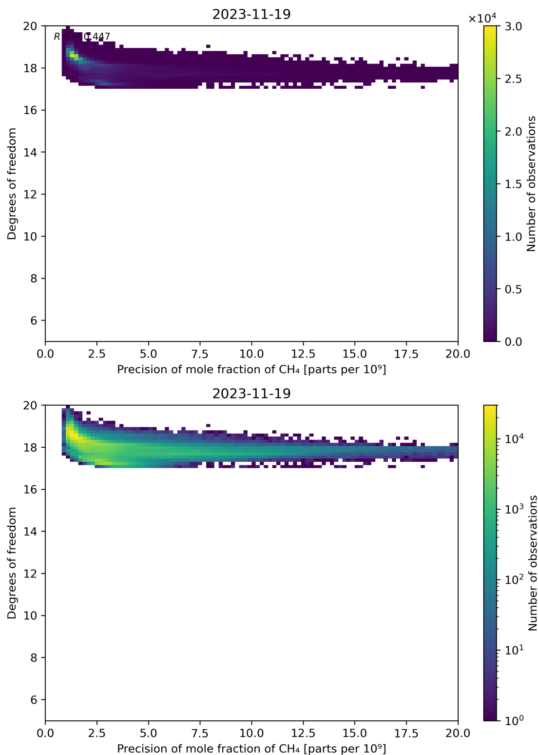
Figure 80: Scatter density plot of “Precision of mole fraction of CH 4 ” against “Degrees of freedom” for 2023-11-18 to 2023-11-20.
