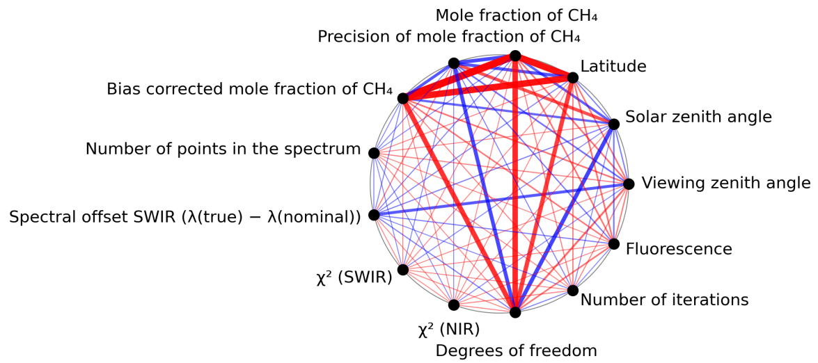
Figure 1: Map of correlation graph for 2023-11-18 to 2023-11-20.
