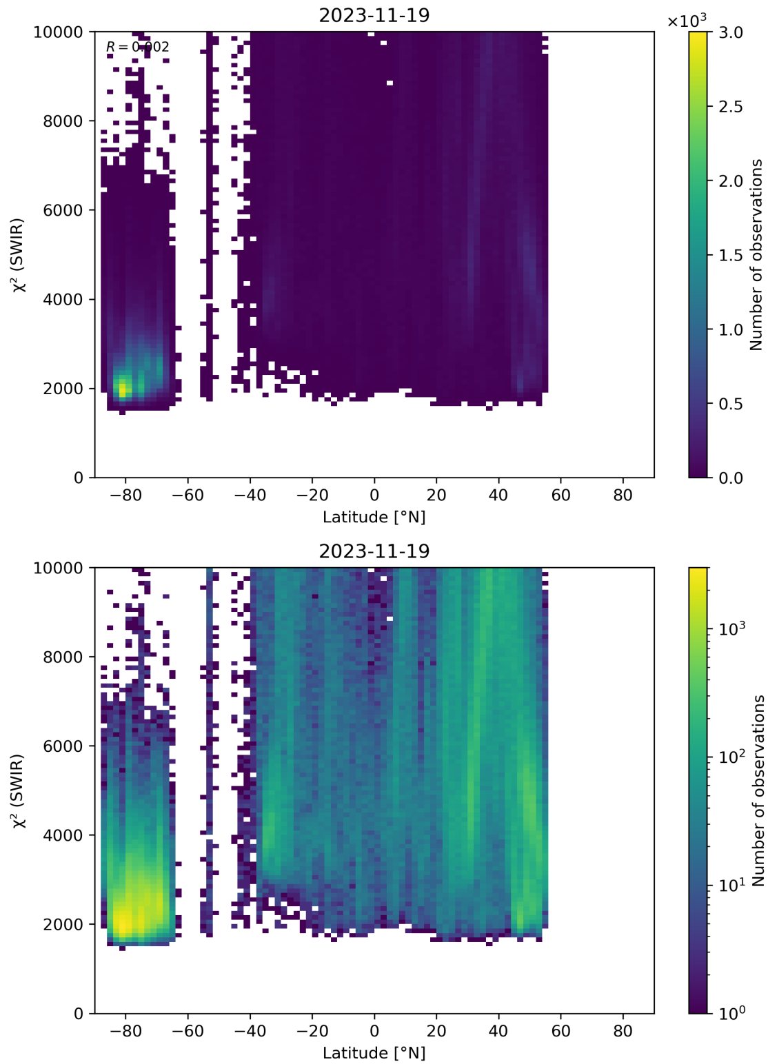
Figure 54: Scatter density plot of “Latitude” against “ \chi^2 (SWIR)” for 2023-11-18 to 2023-11-20.
