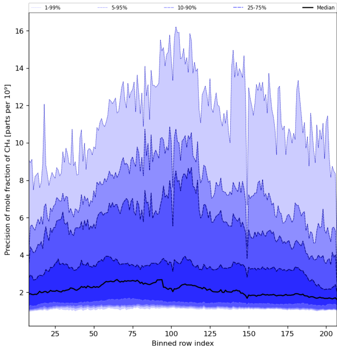
Figure 35: Along track statistics of “Precision of mole fraction of CH 4 ” for 2023-11-18 to 2023-11-20
