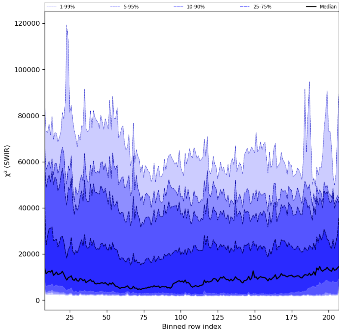
Figure 39: Along track statistics of “ \chi^2 (SWIR)” for 2023-11-18 to 2023-11-20
