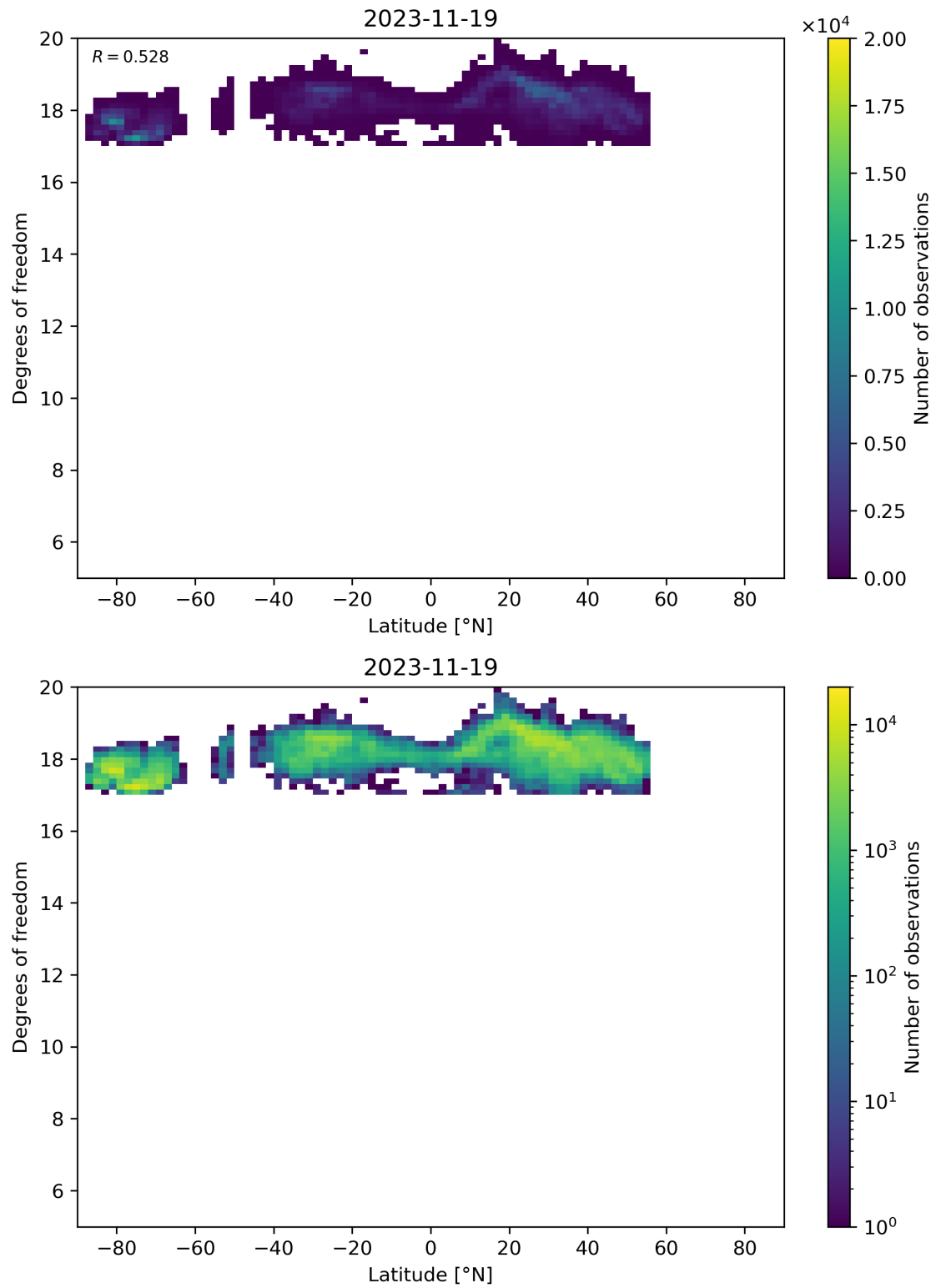
Figure 55: Scatter density plot of “Latitude” against “Degrees of freedom” for 2023-11-18 to 2023-11-20.
