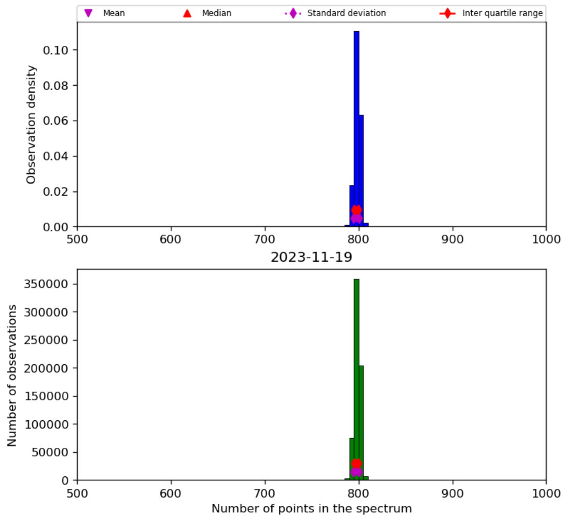
Figure 26: Histogram of “Number of points in the spectrum” for 2023-11-18 to 2023-11-20
