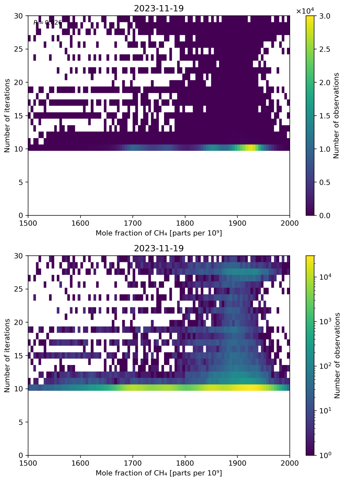
Figure 76: Scatter density plot of “Mole fraction of CH 4 ” against “Number of iterations” for 2023-11-18 to 2023-11-20.
