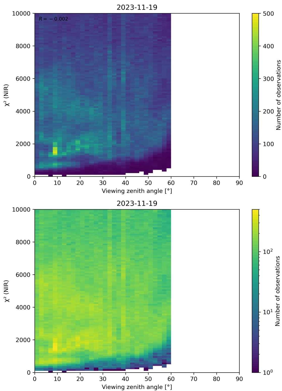
Figure 105: Scatter density plot of “Viewing zenith angle” against “ \chi^2 (NIR)” for 2023-11-18 to 2023-11-20.
