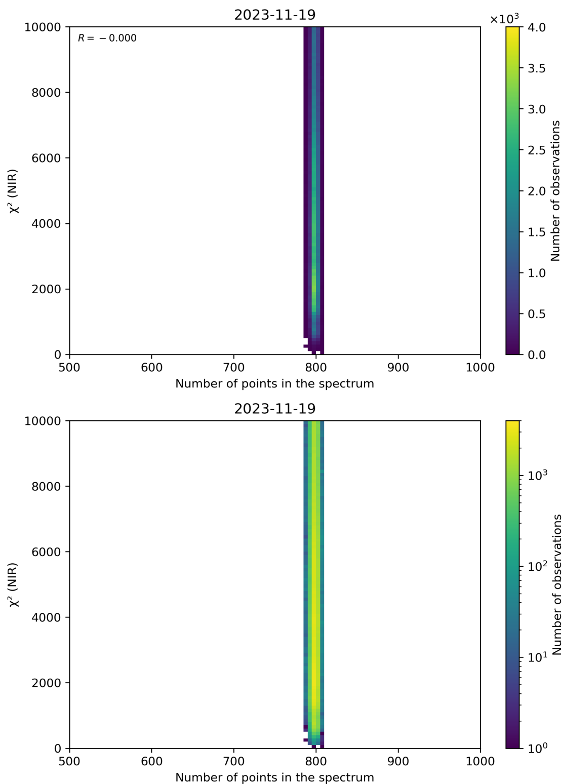
Figure 88: Scatter density plot of “Number of points in the spectrum” against “ \chi^2 (NIR)” for 2023-11-18 to 2023-11-20.
