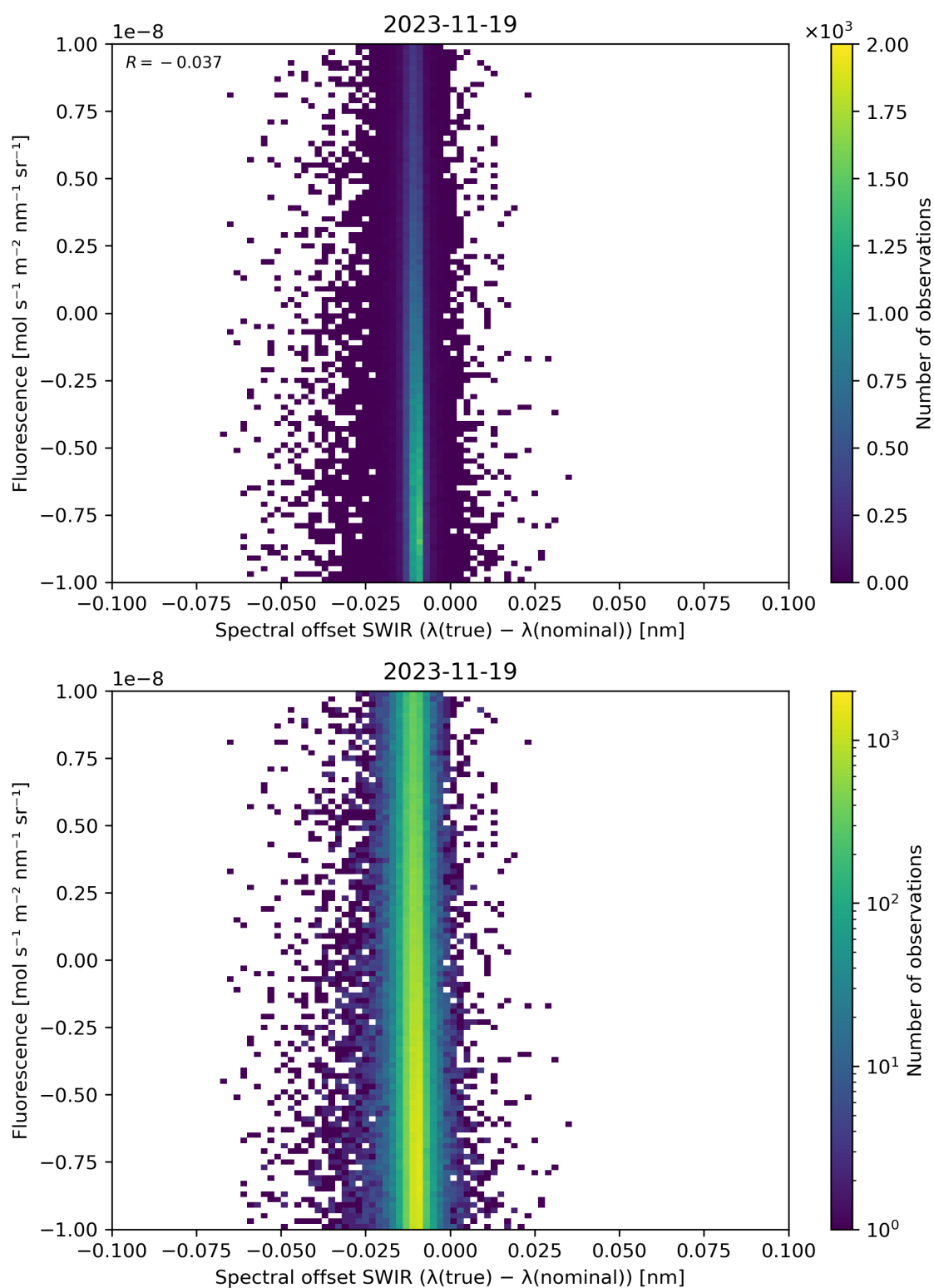
Figure 120: Scatter density plot of “Spectral offset SWIR ( \lambda(\text{true}) - \lambda(\text{nominal}) )” against “Fluorescence” for 2023-11-18 to 2023-11-20.
