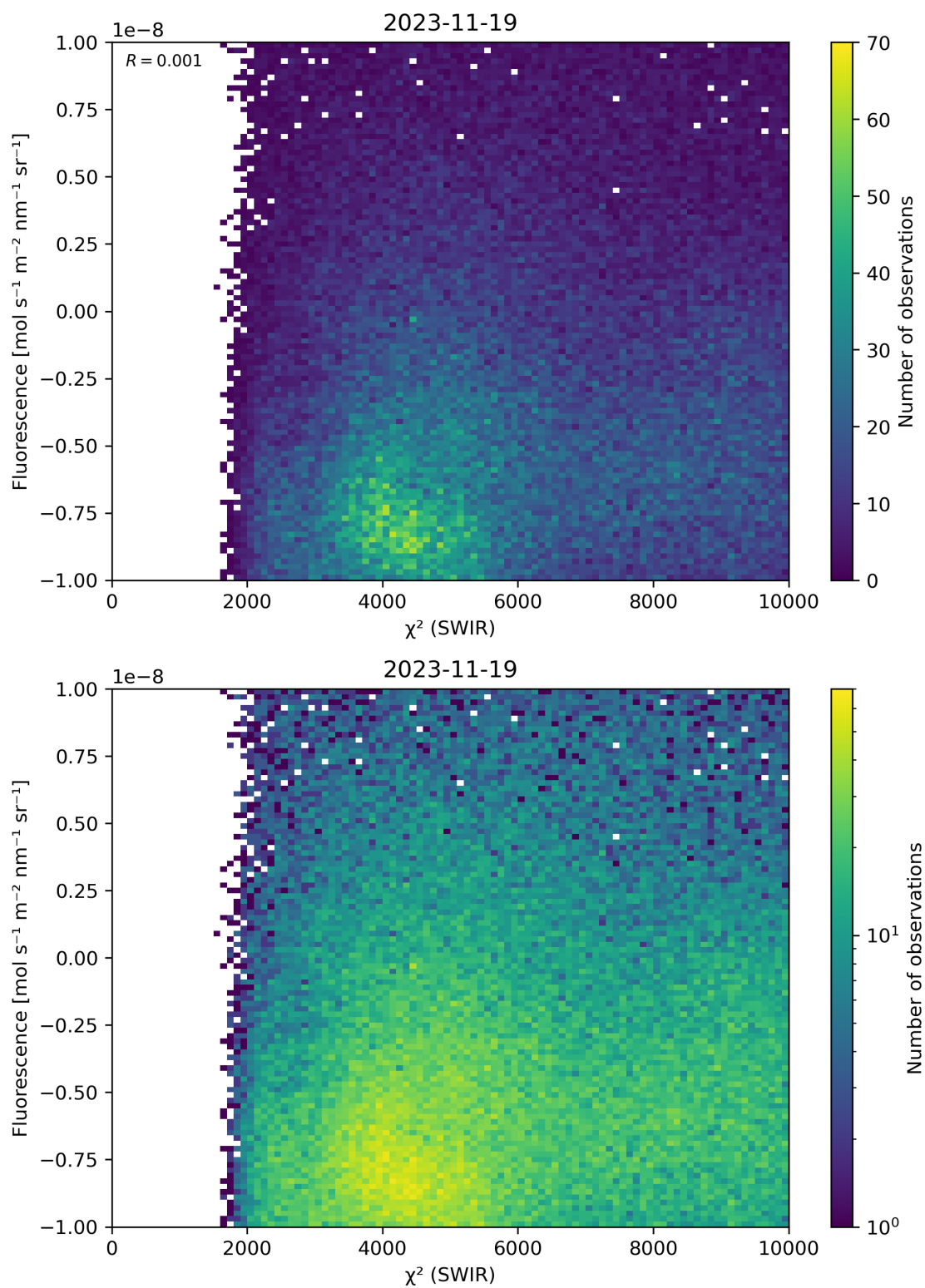
Figure 49: Scatter density plot of “ \chi^2 (SWIR)” against “Fluorescence” for 2023-11-18 to 2023-11-20.
