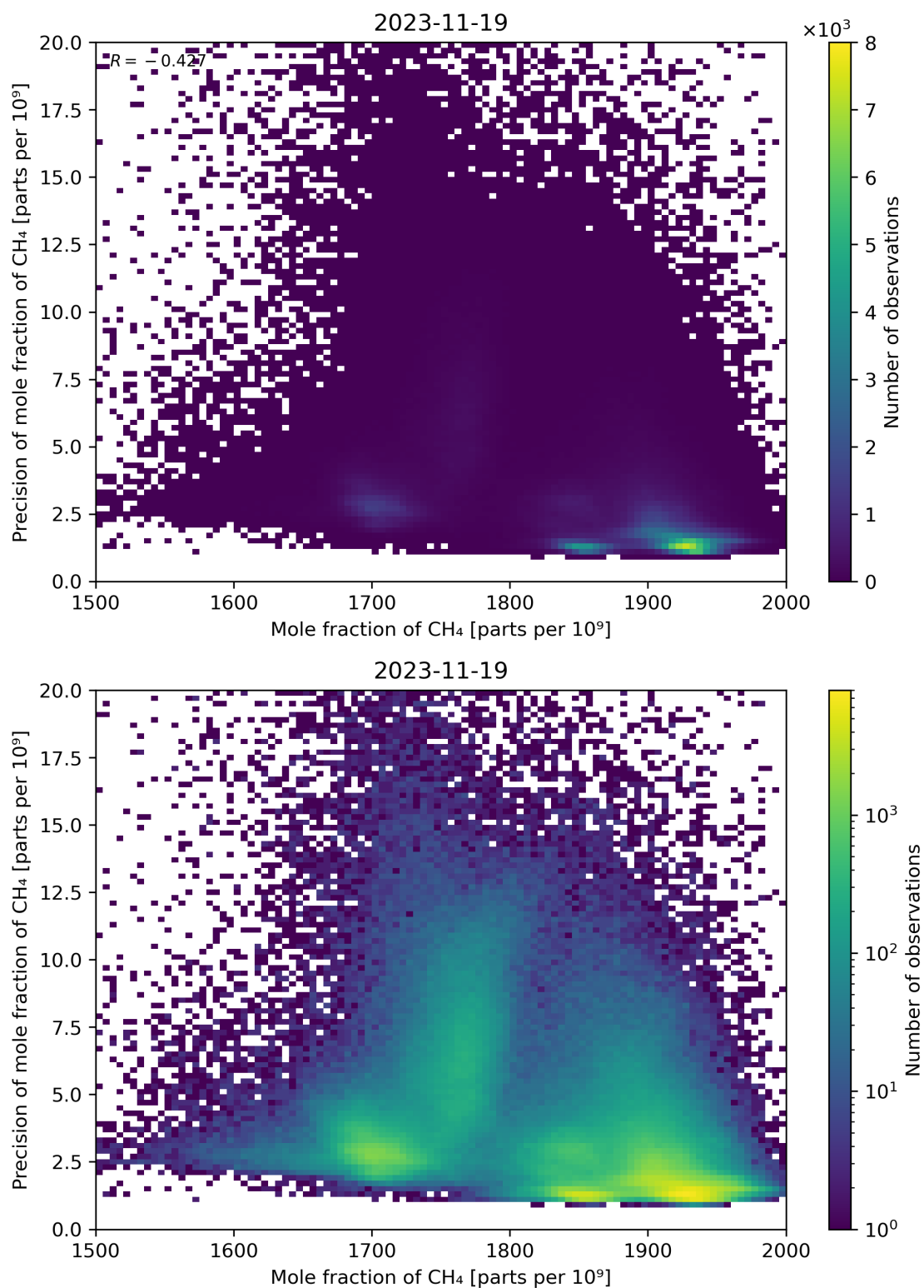
Figure 75: Scatter density plot of “Mole fraction of CH 4 ” against “Precision of mole fraction of CH 4 ” for 2023-11-18 to 2023-11-20.
