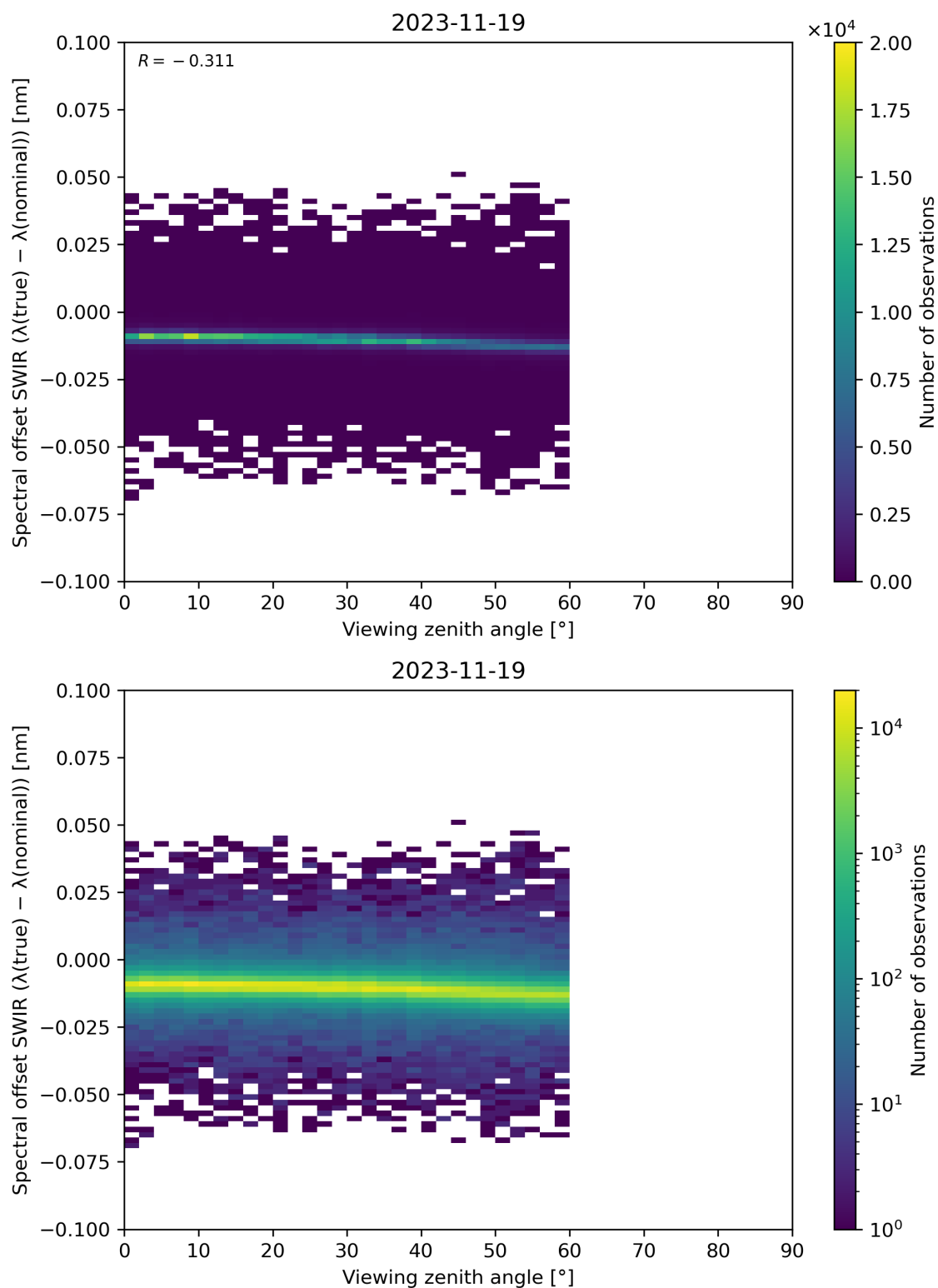
Figure 116: Scatter density plot of “Viewing zenith angle” against “Spectral offset SWIR ( \lambda(\text{true}) - \lambda(\text{nominal}) )” for 2023-11-18 to 2023-11-20.
