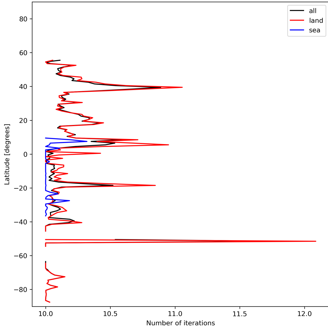
Figure 20: Zonal average of “Number of iterations” for 2023-11-18 to 2023-11-20.
