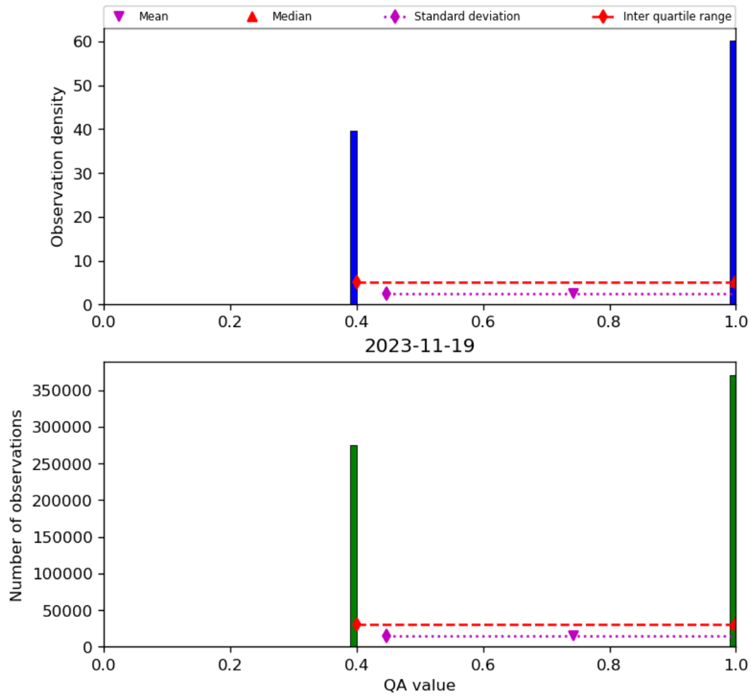
Figure 22: Histogram of “QA value” for 2023-11-18 to 2023-11-20
