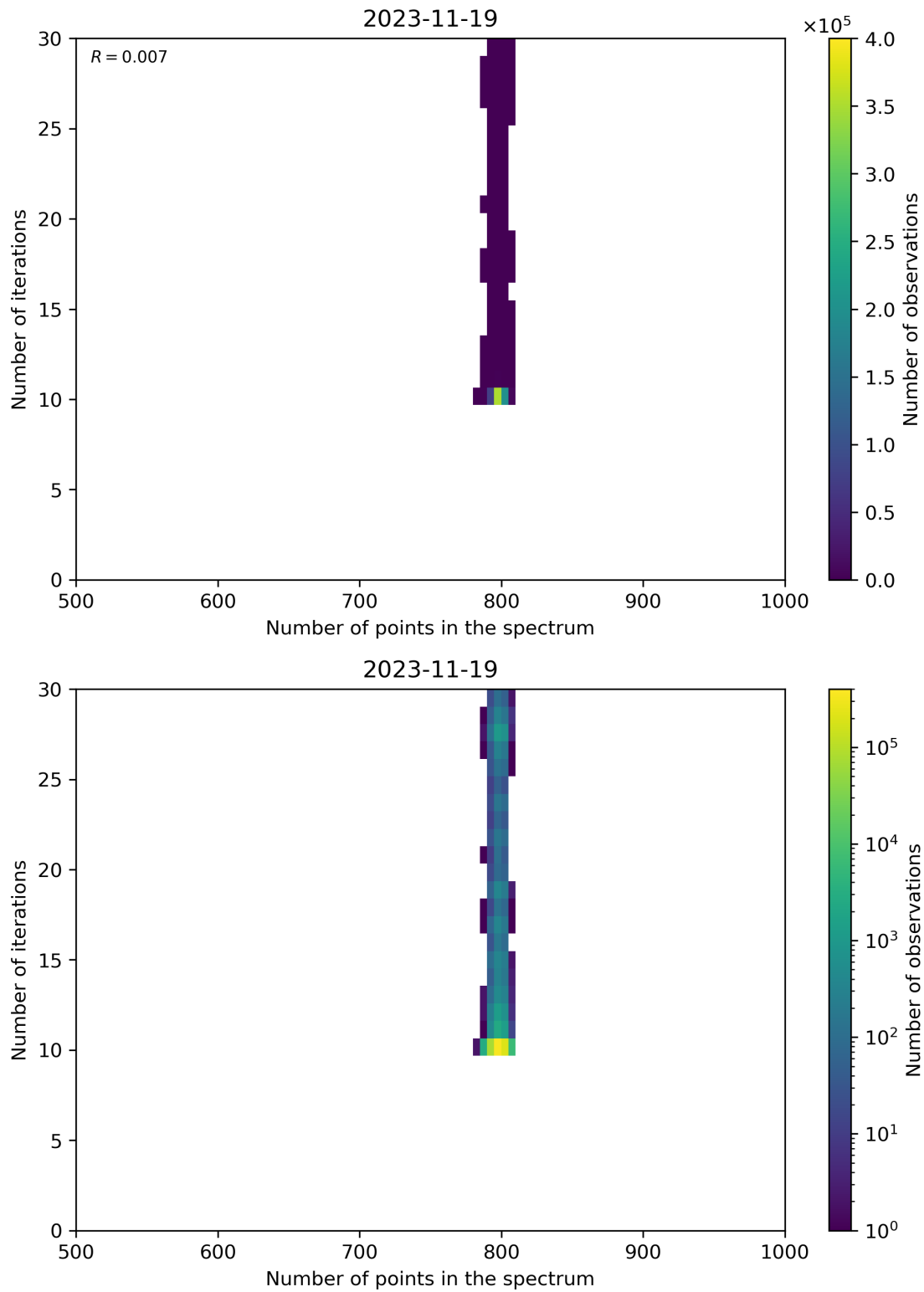
Figure 92: Scatter density plot of “Number of points in the spectrum” against “Number of iterations” for 2023-11-18 to 2023-11-20.
