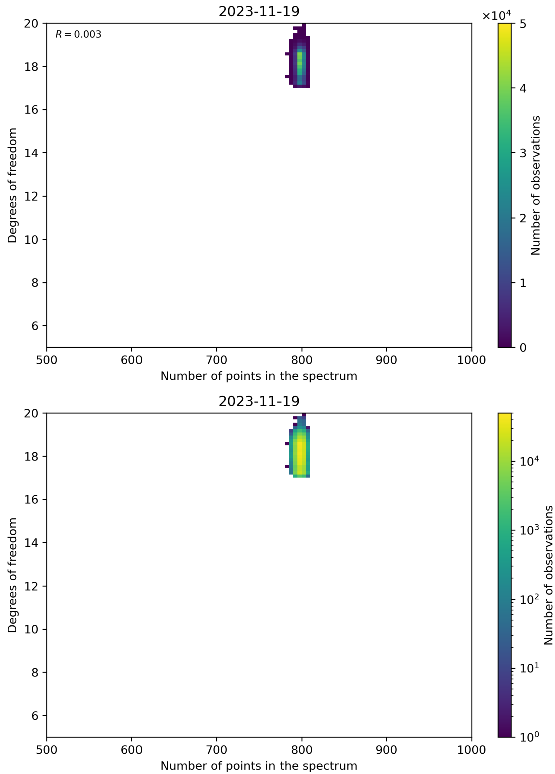
Figure 90: Scatter density plot of “Number of points in the spectrum” against “Degrees of freedom” for 2023-11-18 to 2023-11-20.
