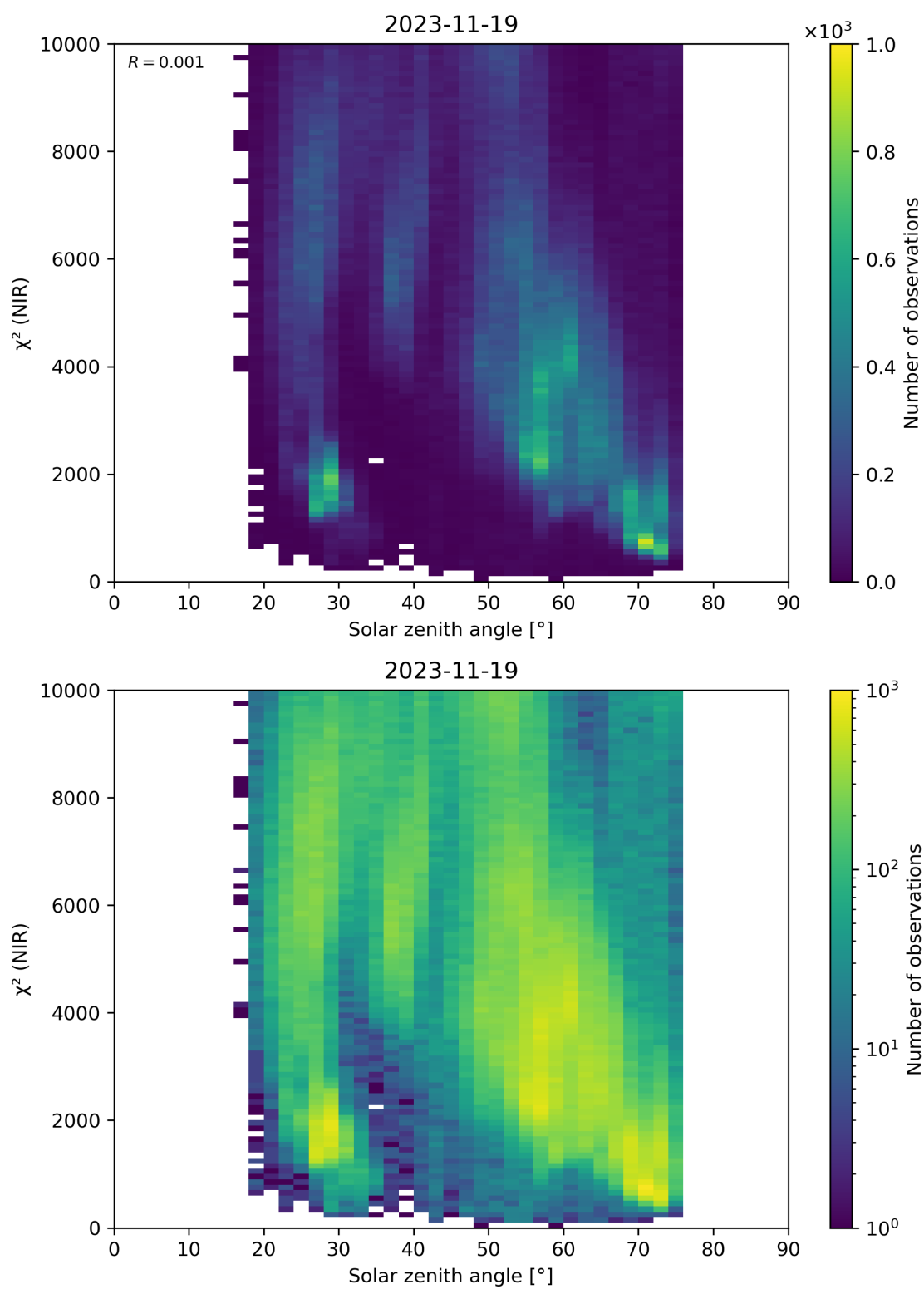
Figure 94: Scatter density plot of “Solar zenith angle” against “ \chi^2 (NIR)” for 2023-11-18 to 2023-11-20.
