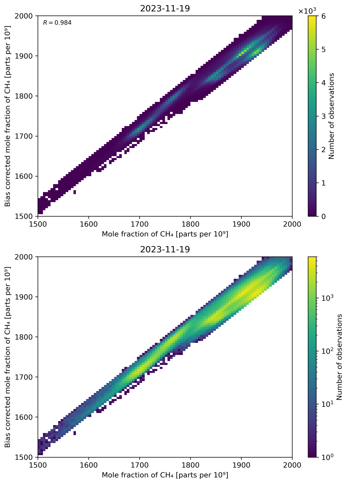
Figure 74: Scatter density plot of “Mole fraction of CH 4 ” against “Bias corrected mole fraction of CH 4 ” for 2023-11-18 to 2023-11-20.
