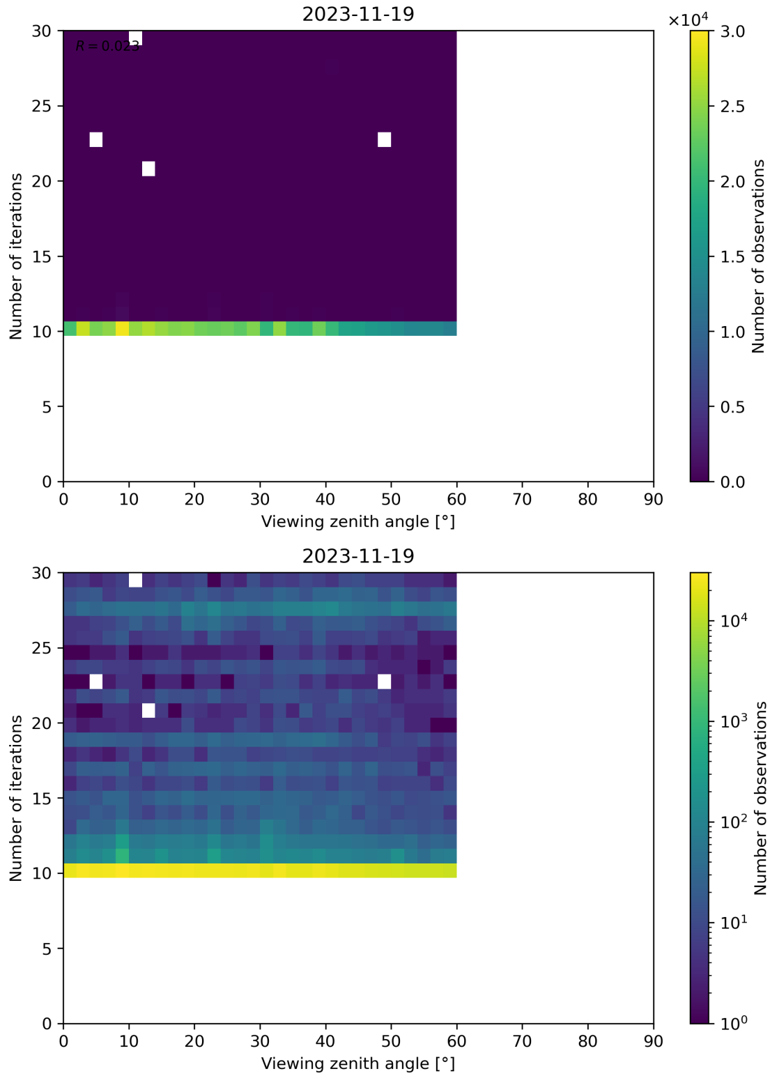
Figure 113: Scatter density plot of “Viewing zenith angle” against “Number of iterations” for 2023-11-18 to 2023-11-20.
