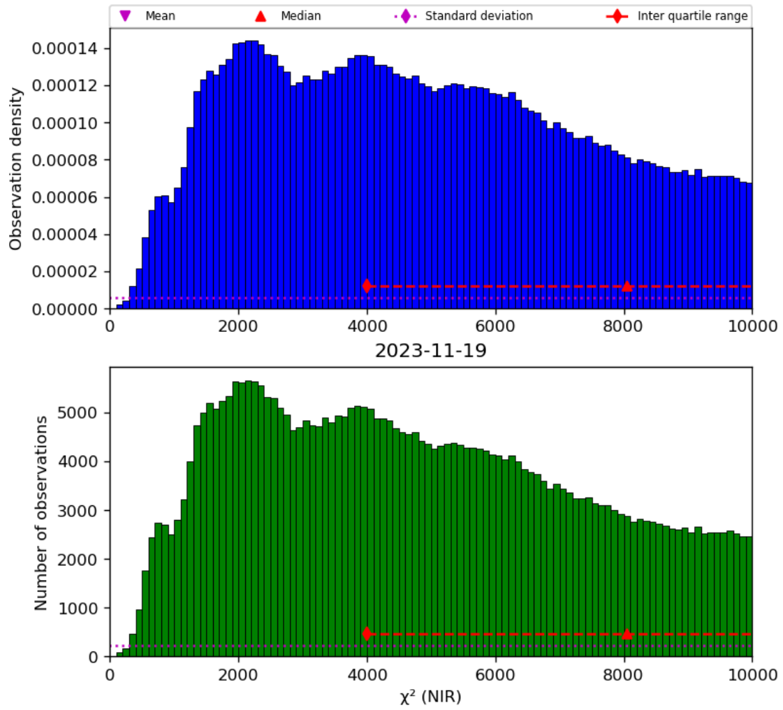
Figure 29: Histogram of “ \chi^2 (NIR)” for 2023-11-18 to 2023-11-20
