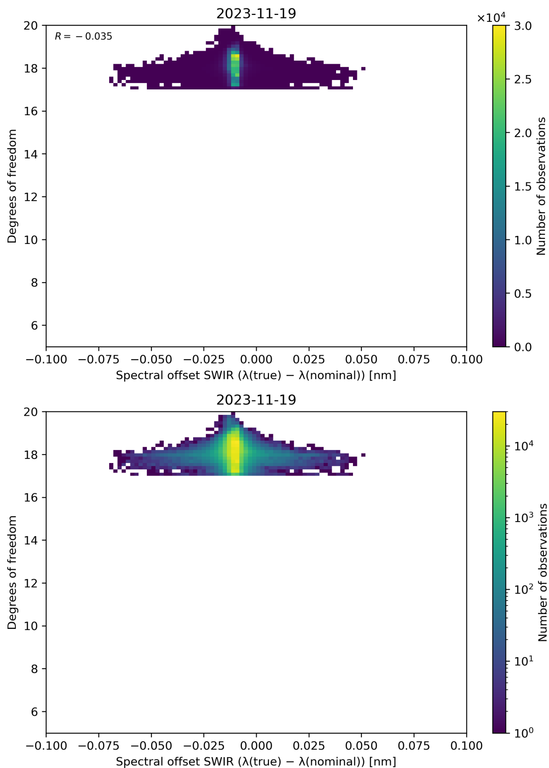
Figure 119: Scatter density plot of “Spectral offset SWIR ( \lambda(\text{true}) - \lambda(\text{nominal}) )” against “Degrees of freedom” for 2023-11-18 to 2023-11-20.
