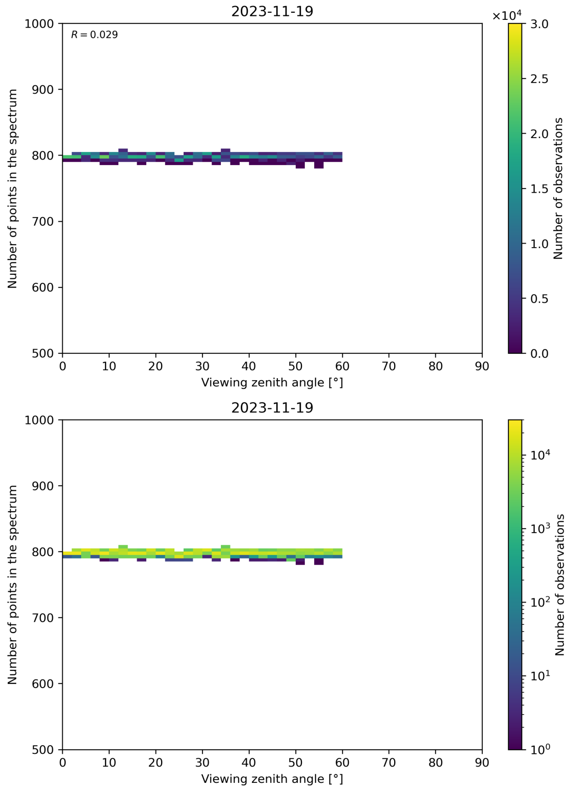
Figure 114: Scatter density plot of “Viewing zenith angle” against “Number of points in the spectrum” for 2023-11-18 to 2023-11-20.
