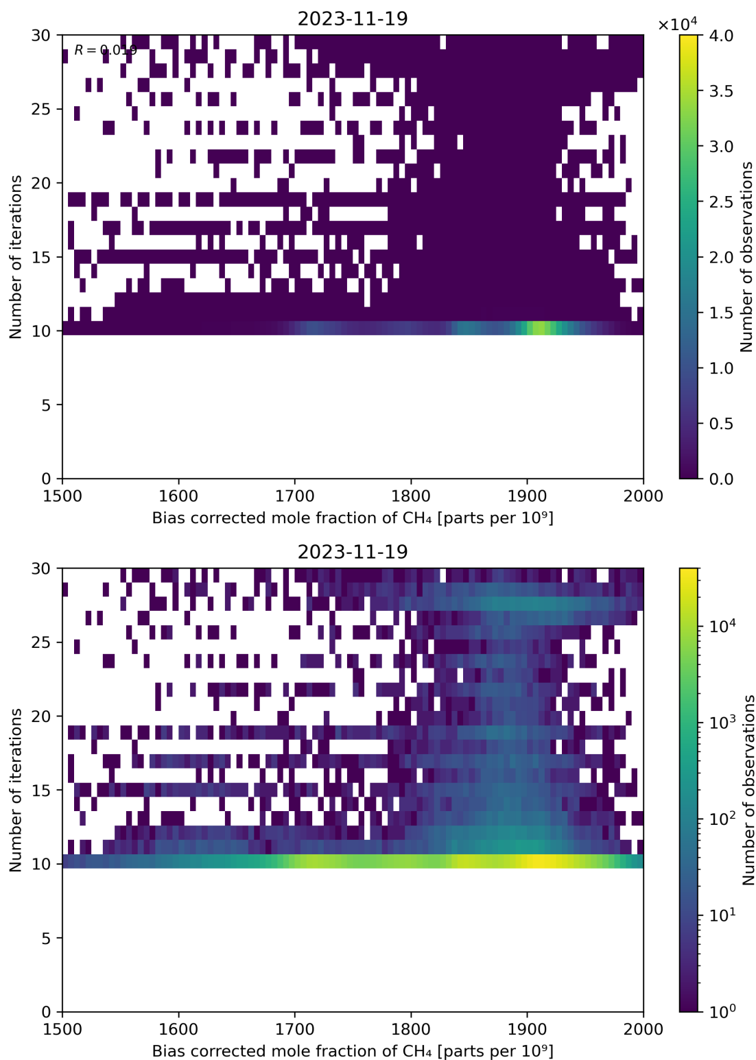
Figure 67: Scatter density plot of “Bias corrected mole fraction of \text{CH}_4 ” against “Number of iterations” for 2023-11-18 to 2023-11-20.
