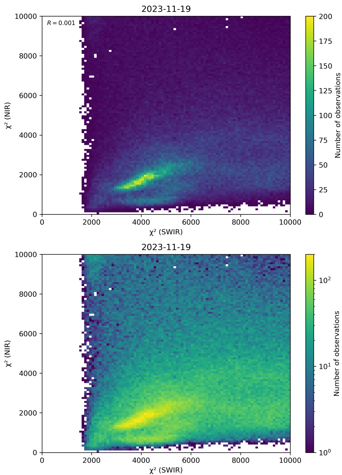
Figure 47: Scatter density plot of “ \chi^2 (SWIR)” against “ \chi^2 (NIR)” for 2023-11-18 to 2023-11-20.
