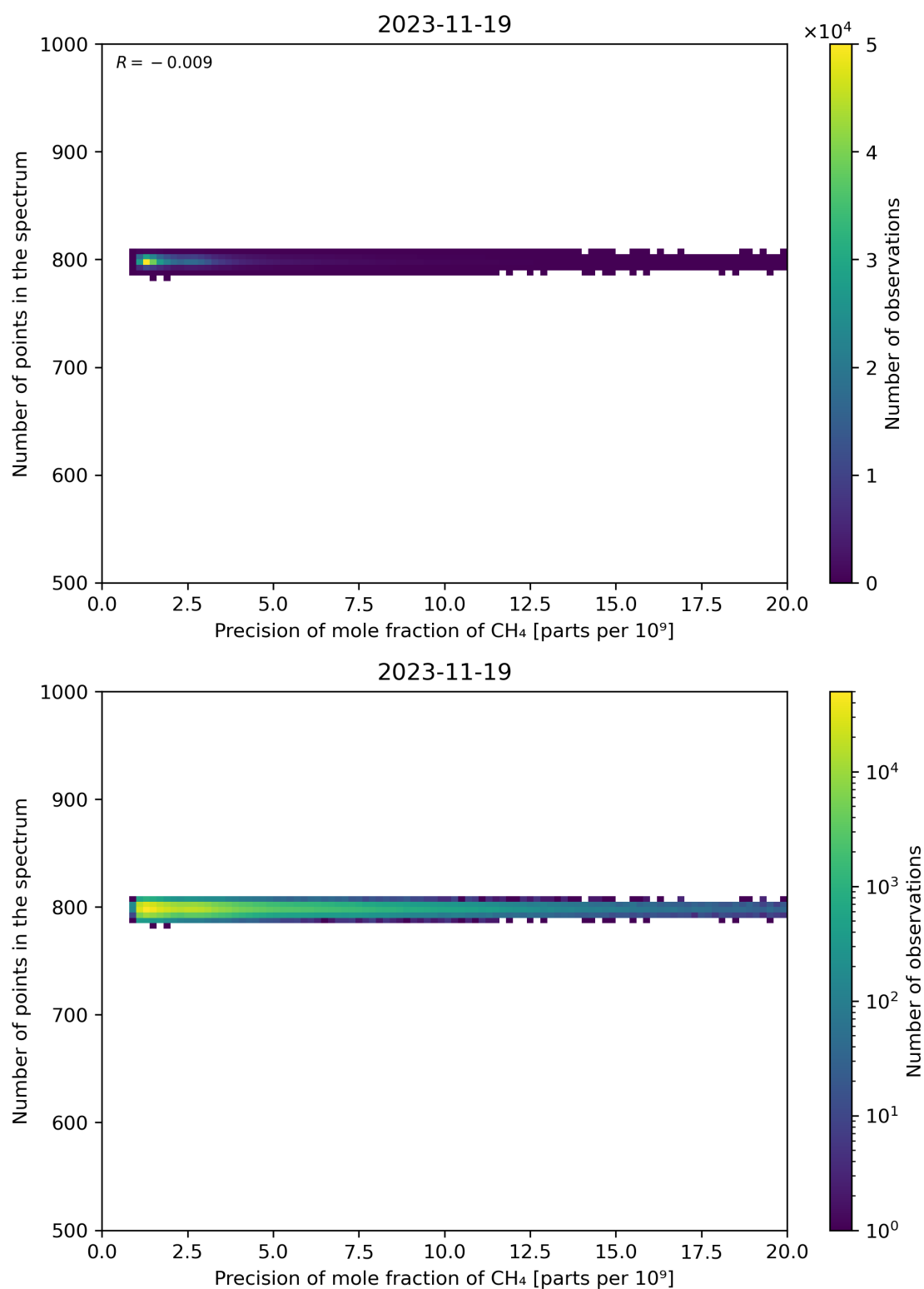
Figure 84: Scatter density plot of “Precision of mole fraction of CH 4 ” against “Number of points in the spectrum” for 2023-11-18 to 2023-11-20.
