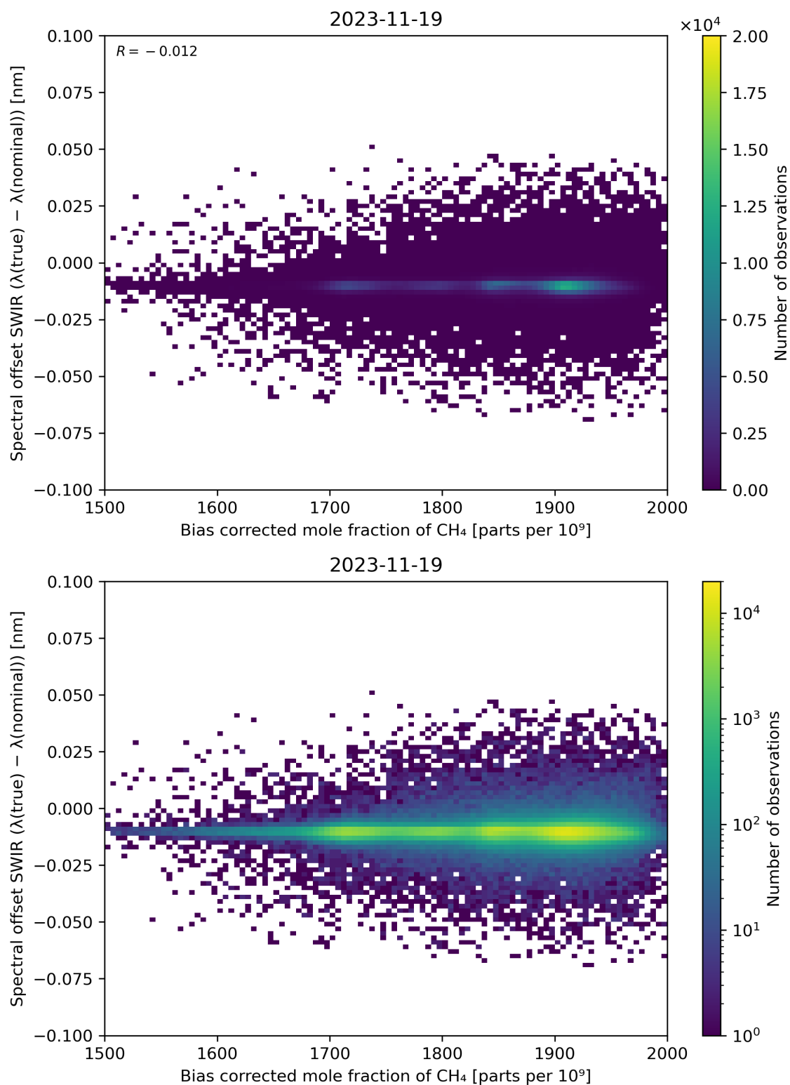
Figure 69: Scatter density plot of “Bias corrected mole fraction of \text{CH}_4 ” against “Spectral offset SWIR ( \lambda(\text{true}) - \lambda(\text{nominal}) )” for 2023-11-18 to 2023-11-20.
