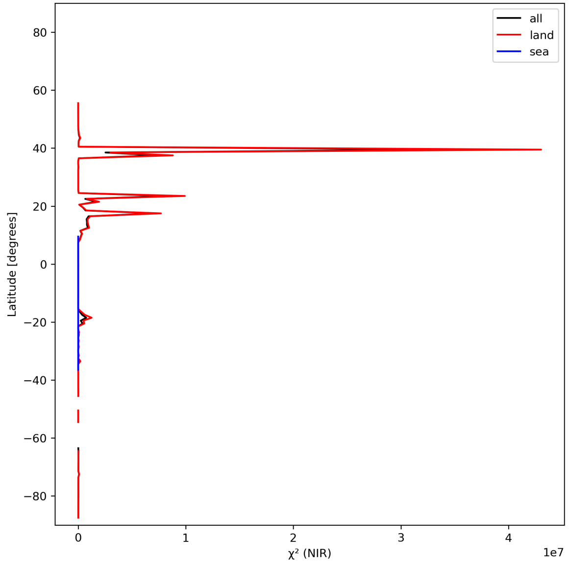
Figure 18: Zonal average of “ \chi^2 (NIR)” for 2023-11-18 to 2023-11-20.
