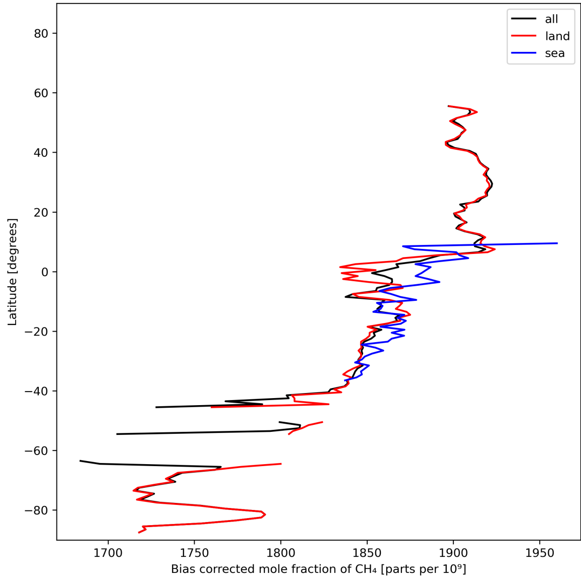
Figure 14: Zonal average of “Bias corrected mole fraction of CH 4 ” for 2023-11-18 to 2023-11-20.
