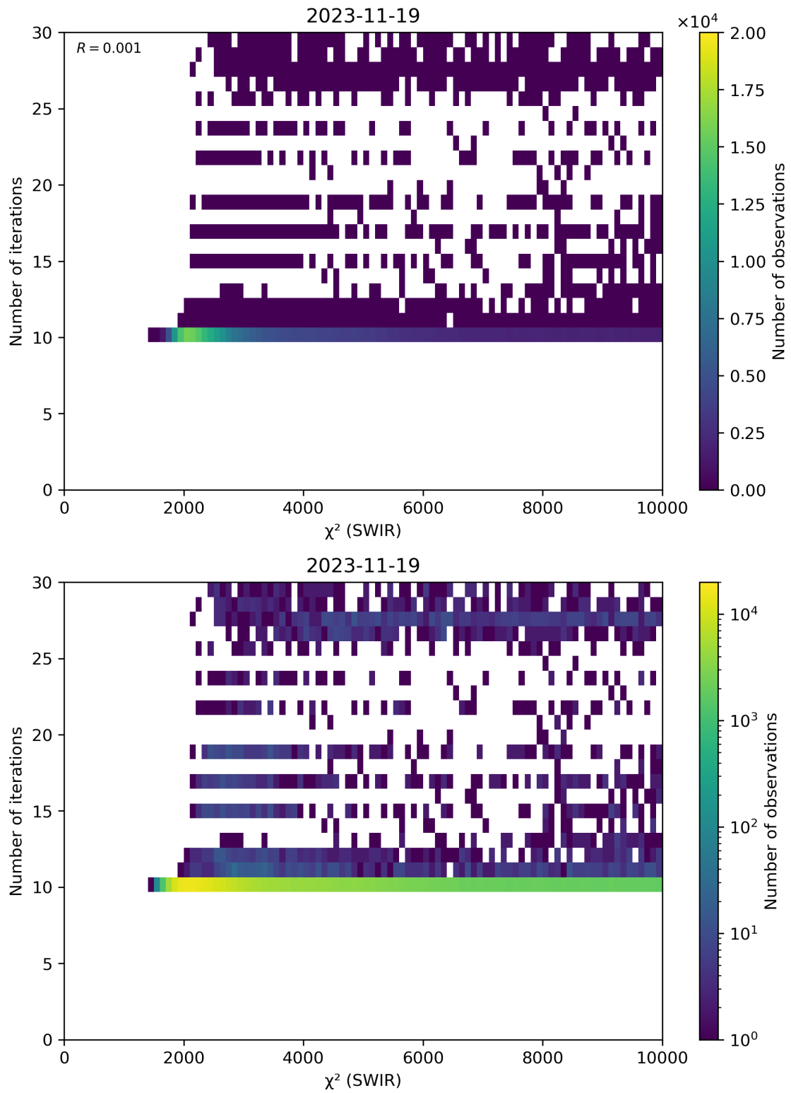
Figure 50: Scatter density plot of “ \chi^2 (SWIR)” against “Number of iterations” for 2023-11-18 to 2023-11-20.
