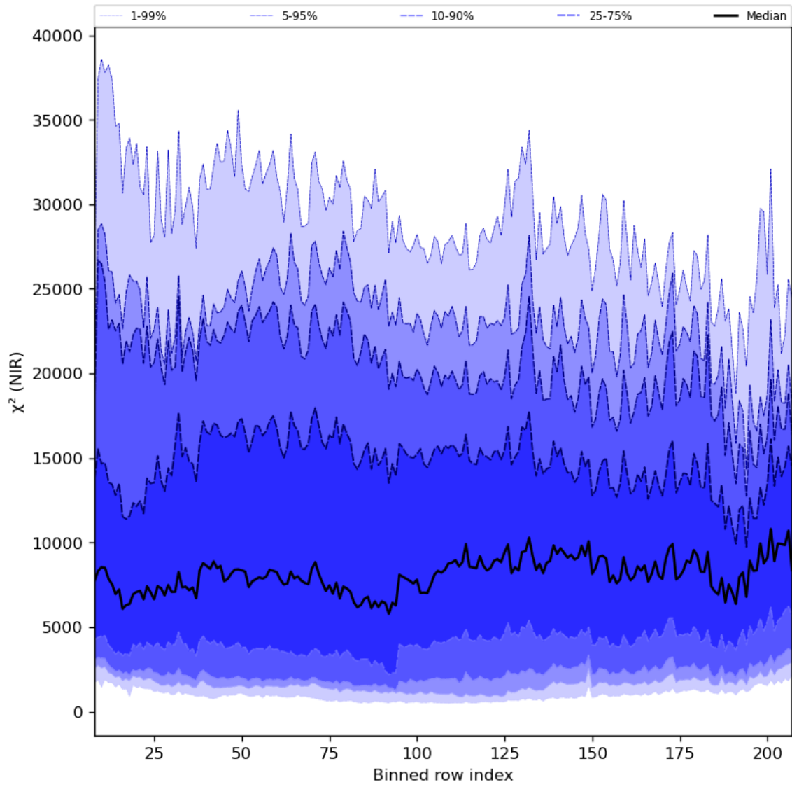
Figure 40: Along track statistics of “ \chi^2 (NIR)” for 2023-11-18 to 2023-11-20
