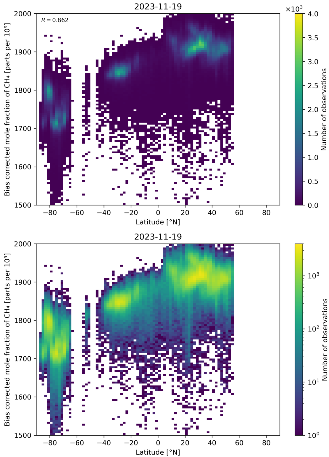
Figure 58: Scatter density plot of “Latitude” against “Bias corrected mole fraction of CH 4 ” for 2023-11-18 to 2023-11-20.
