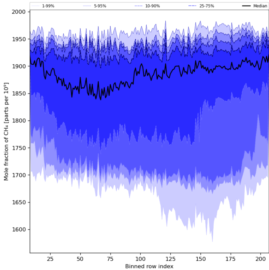
Figure 34: Along track statistics of “Mole fraction of CH 4 ” for 2023-11-18 to 2023-11-20
