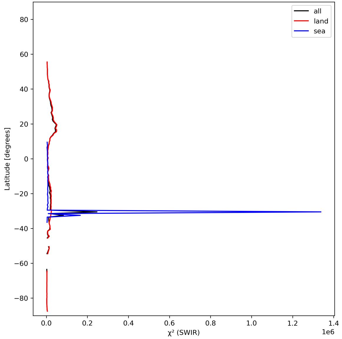
Figure 17: Zonal average of “ \chi^2 (SWIR)” for 2023-11-18 to 2023-11-20.
