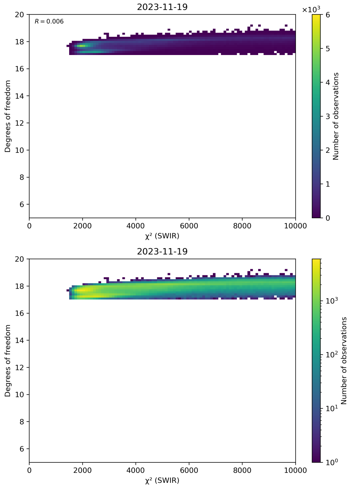
Figure 48: Scatter density plot of “ \chi^2 (SWIR)” against “Degrees of freedom” for 2023-11-18 to 2023-11-20.
