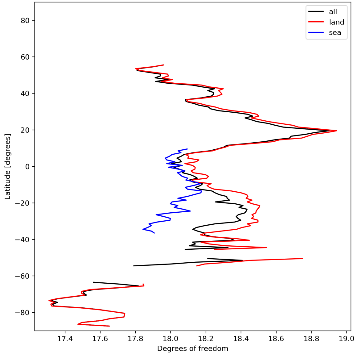
Figure 19: Zonal average of “Degrees of freedom” for 2023-11-18 to 2023-11-20.
