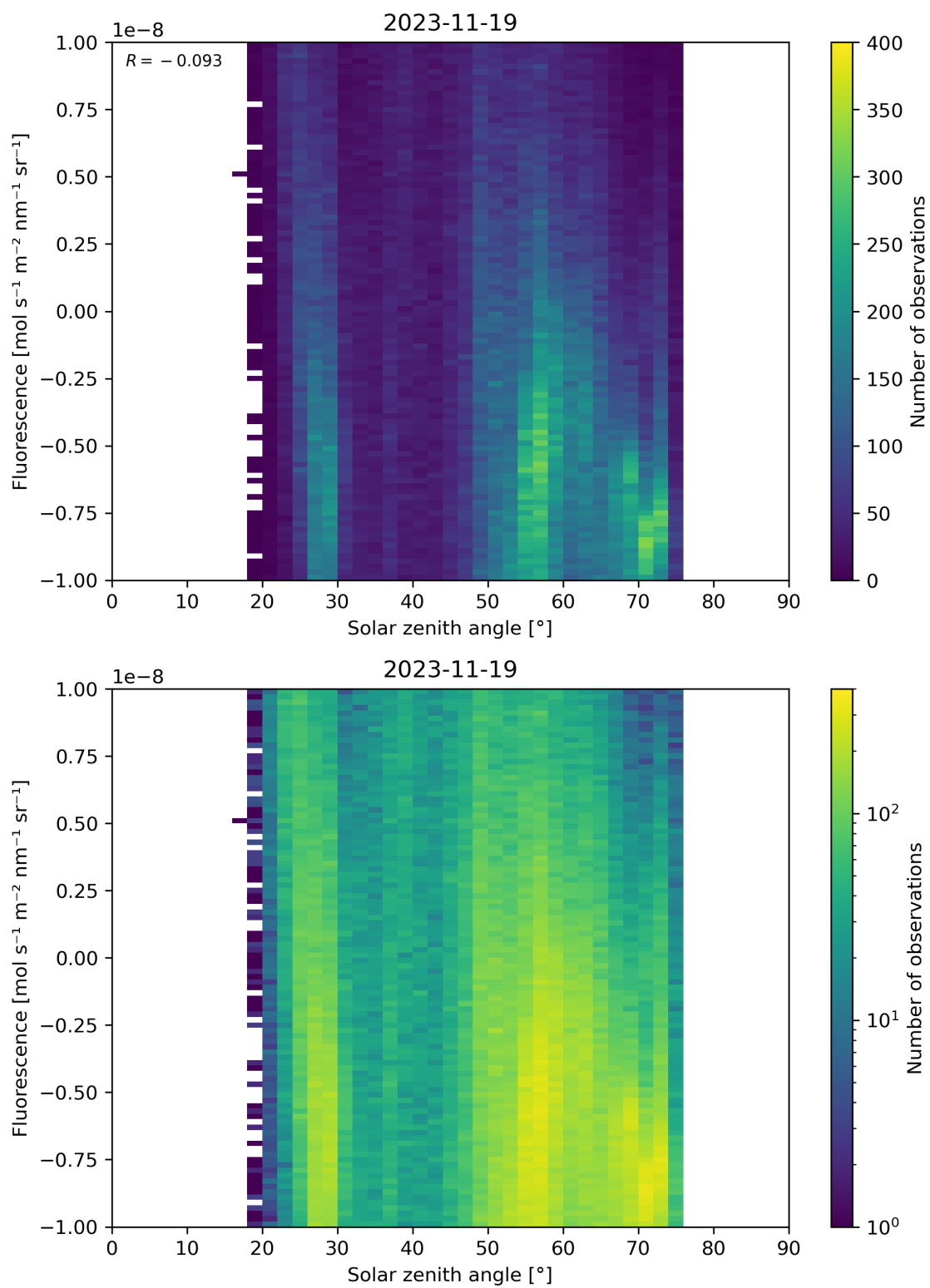
Figure 97: Scatter density plot of “Solar zenith angle” against “Fluorescence” for 2023-11-18 to 2023-11-20.
