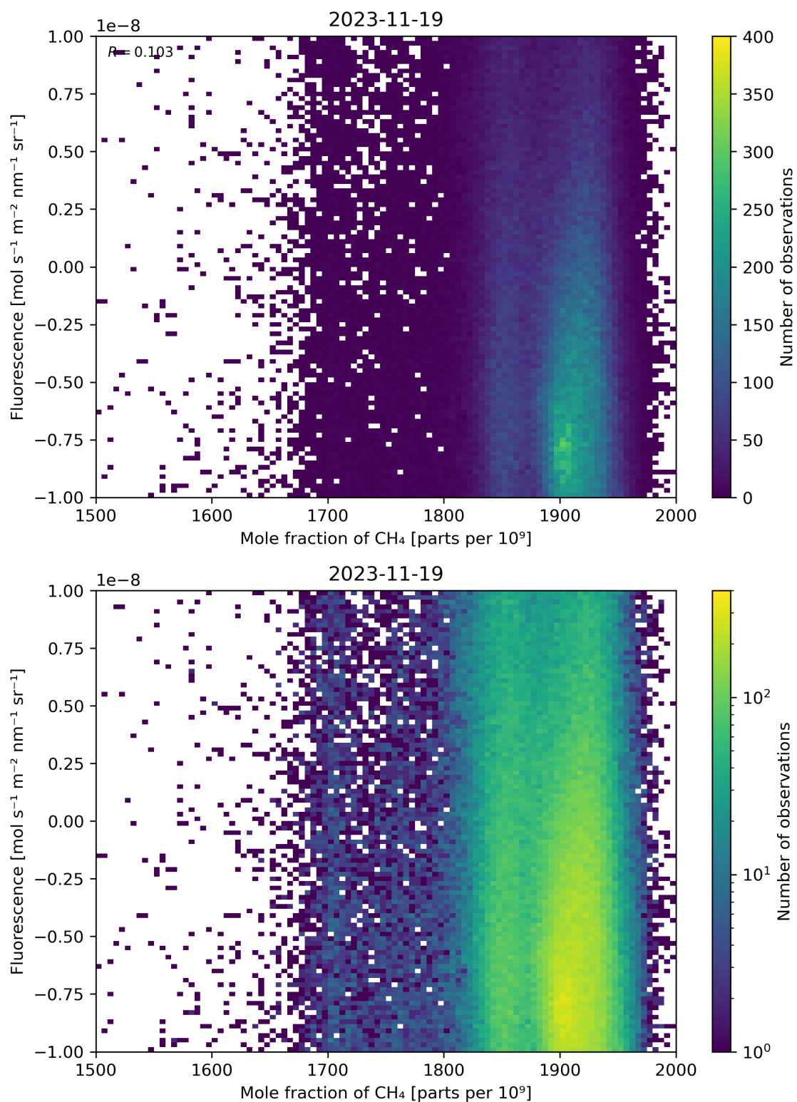
Figure 73: Scatter density plot of “Mole fraction of \text{CH}_4 ” against “Fluorescence” for 2023-11-18 to 2023-11-20.
