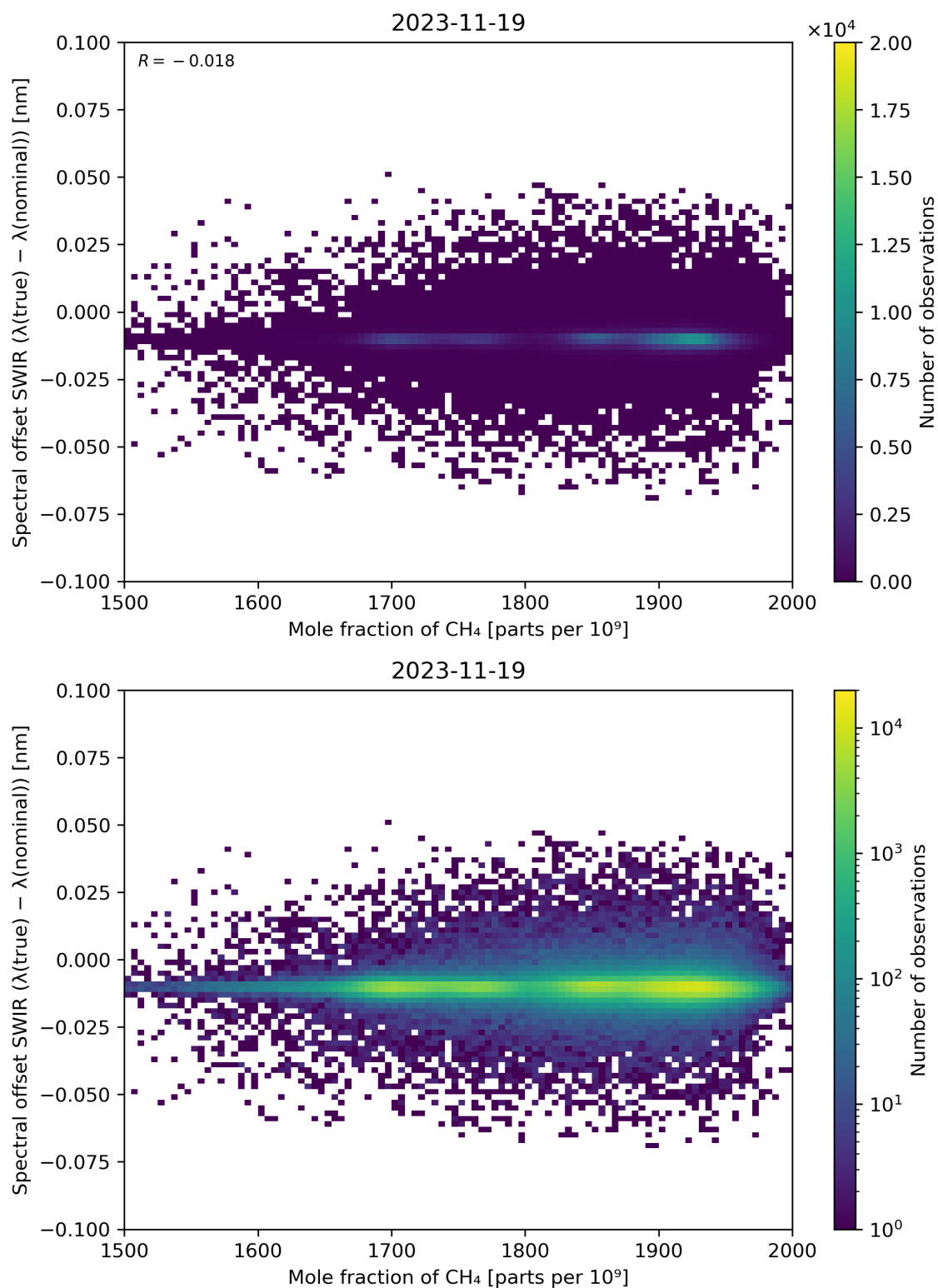
Figure 86: Scatter density plot of “Mole fraction of CH 4 ” against “Spectral offset SWIR ( \lambda(\text{true}) - \lambda(\text{nominal}) )” for 2023-11-18 to 2023-11-20.
