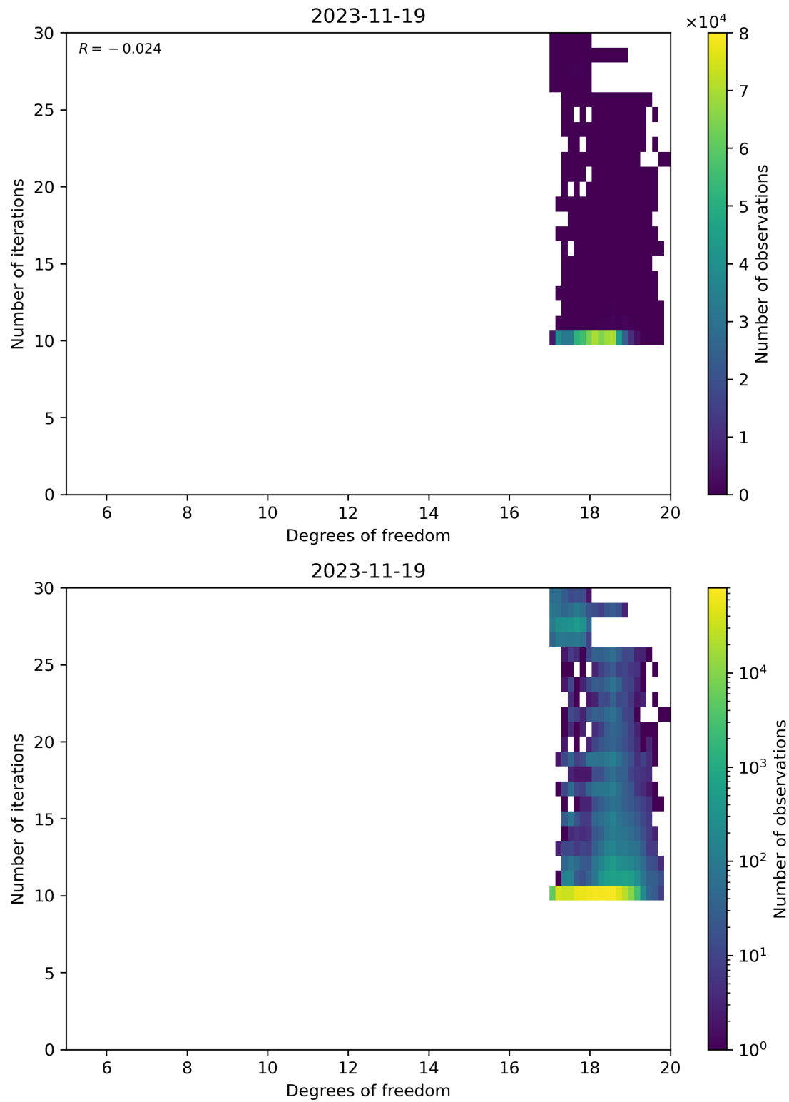
Figure 52: Scatter density plot of “Degrees of freedom” against “Number of iterations” for 2023-11-18 to 2023-11-20.
