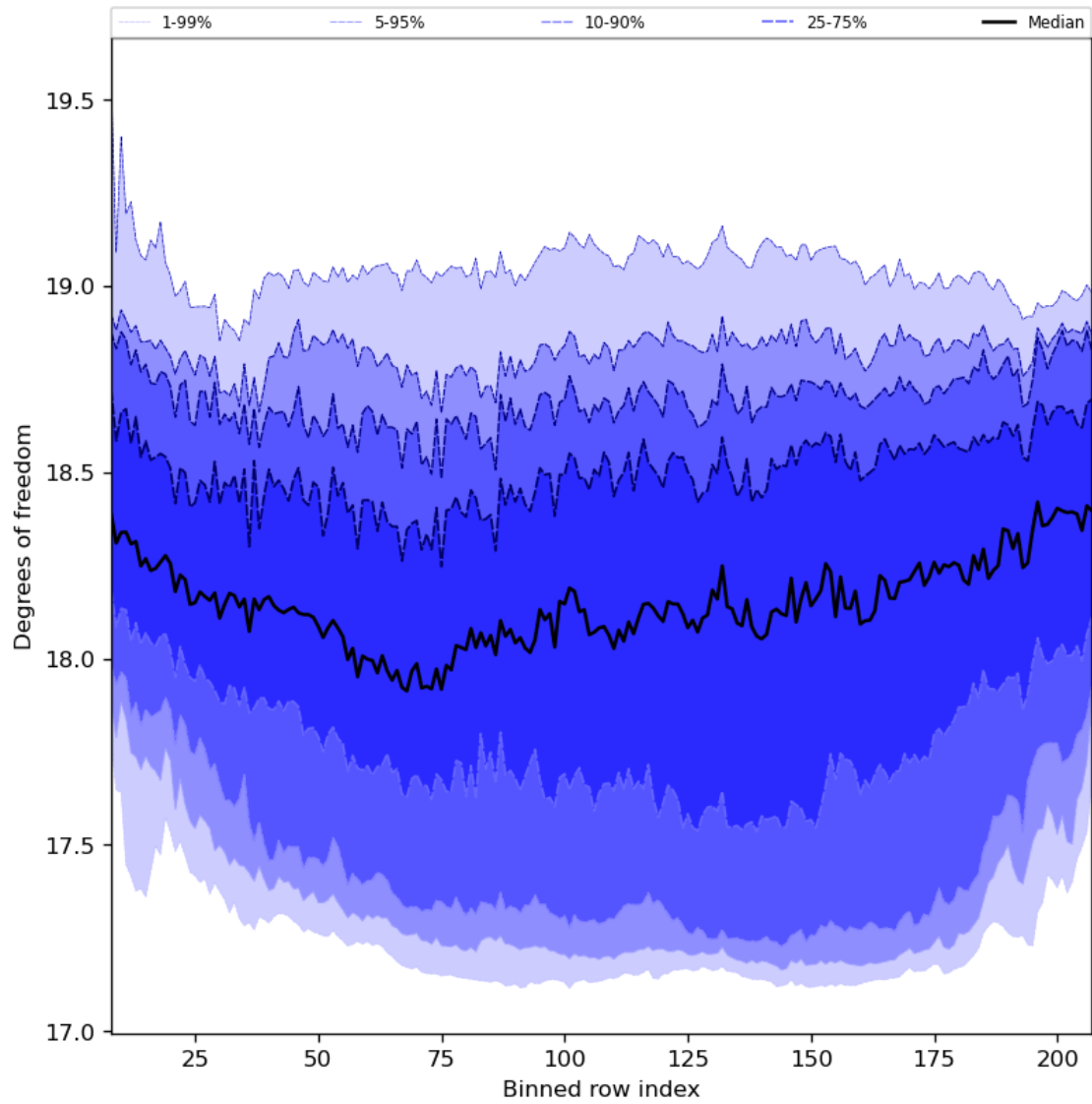
Figure 41: Along track statistics of “Degrees of freedom” for 2023-11-18 to 2023-11-20
