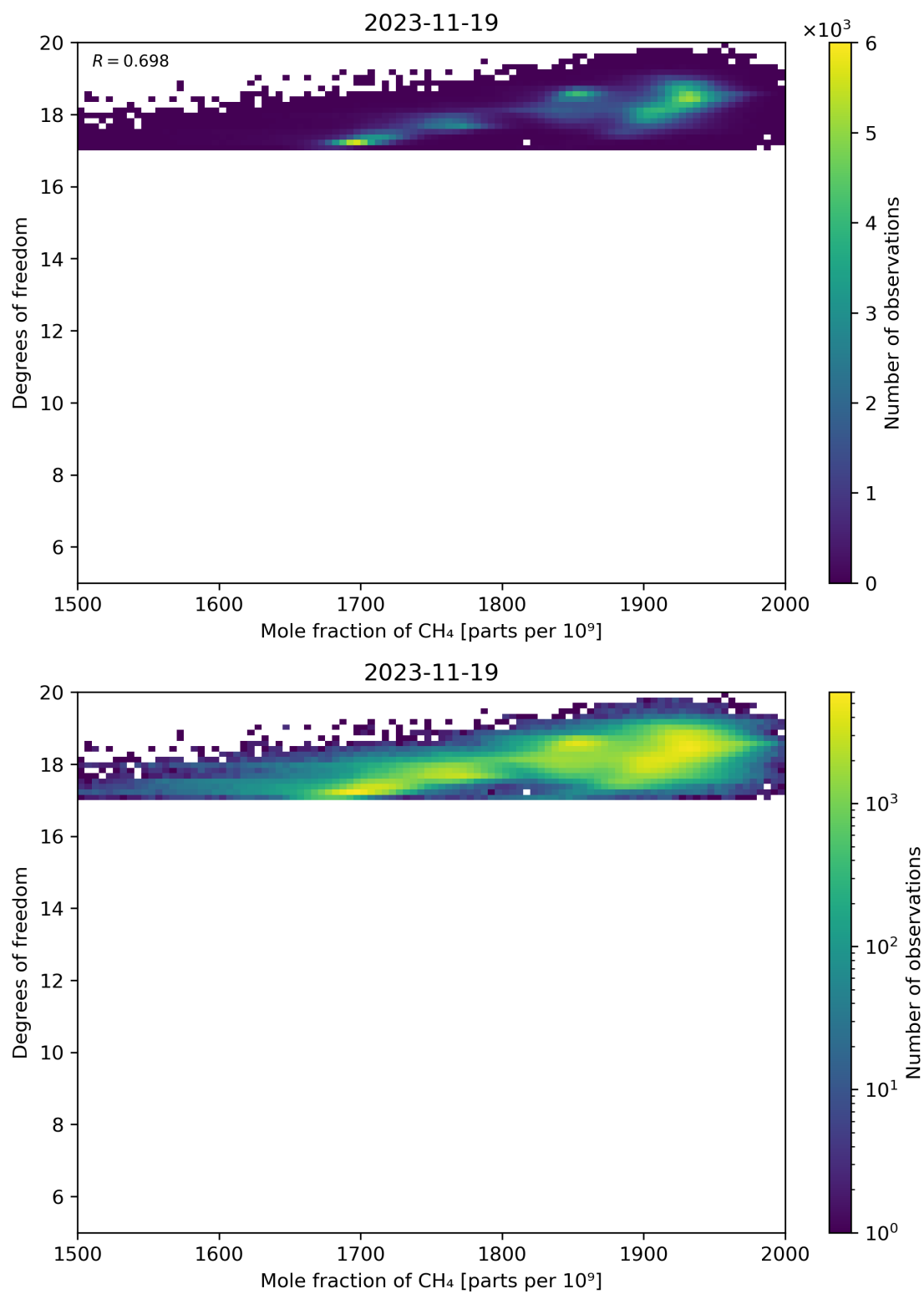
Figure 72: Scatter density plot of “Mole fraction of CH 4 ” against “Degrees of freedom” for 2023-11-18 to 2023-11-20.
