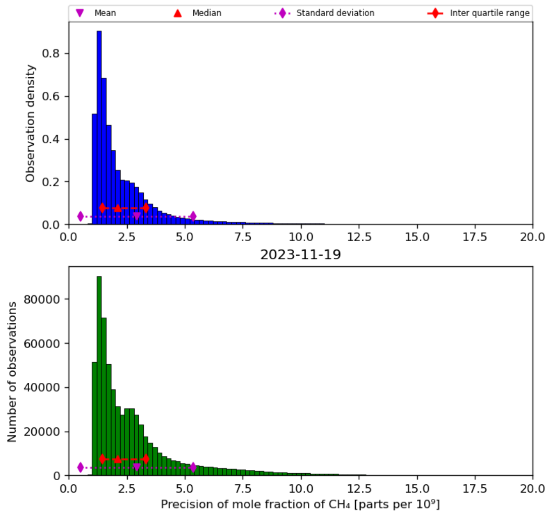
Figure 24: Histogram of “Precision of mole fraction of CH 4 ” for 2023-11-18 to 2023-11-20
