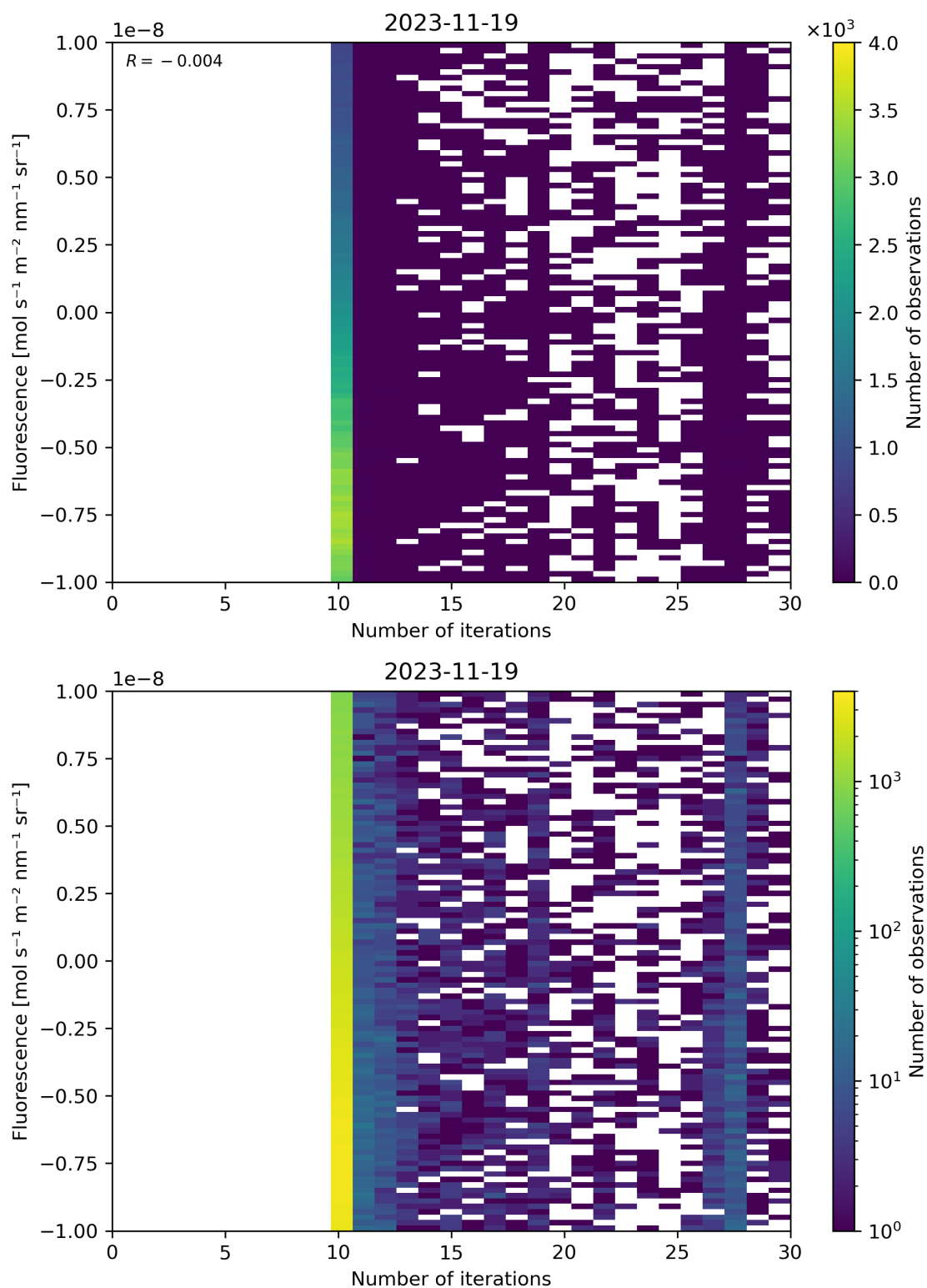
Figure 87: Scatter density plot of “Number of iterations” against “Fluorescence” for 2023-11-18 to 2023-11-20.
