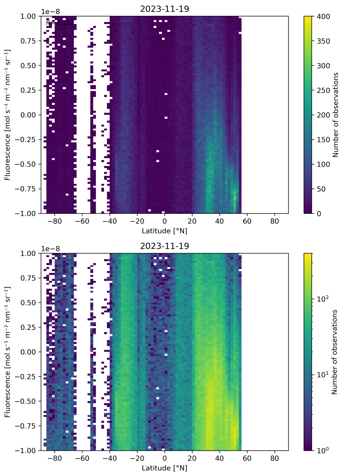
Figure 56: Scatter density plot of “Latitude” against “Fluorescence” for 2023-11-18 to 2023-11-20.
