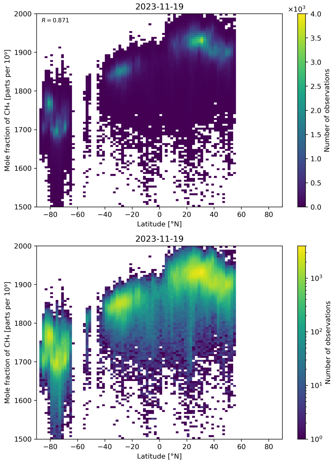
Figure 57: Scatter density plot of “Latitude” against “Mole fraction of \text{CH}_4 ” for 2023-11-18 to 2023-11-20.
