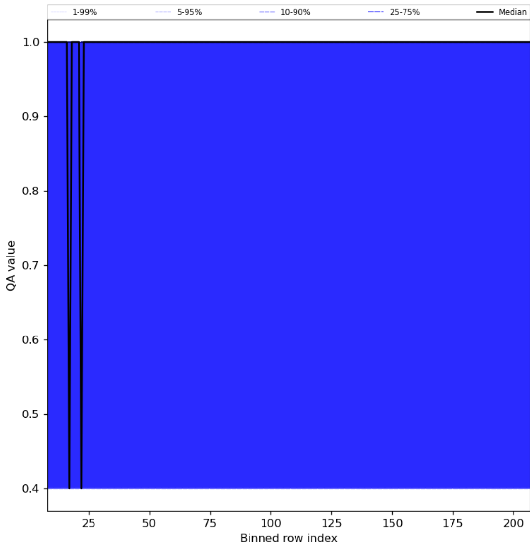
Figure 33: Along track statistics of “QA value” for 2023-11-18 to 2023-11-20
