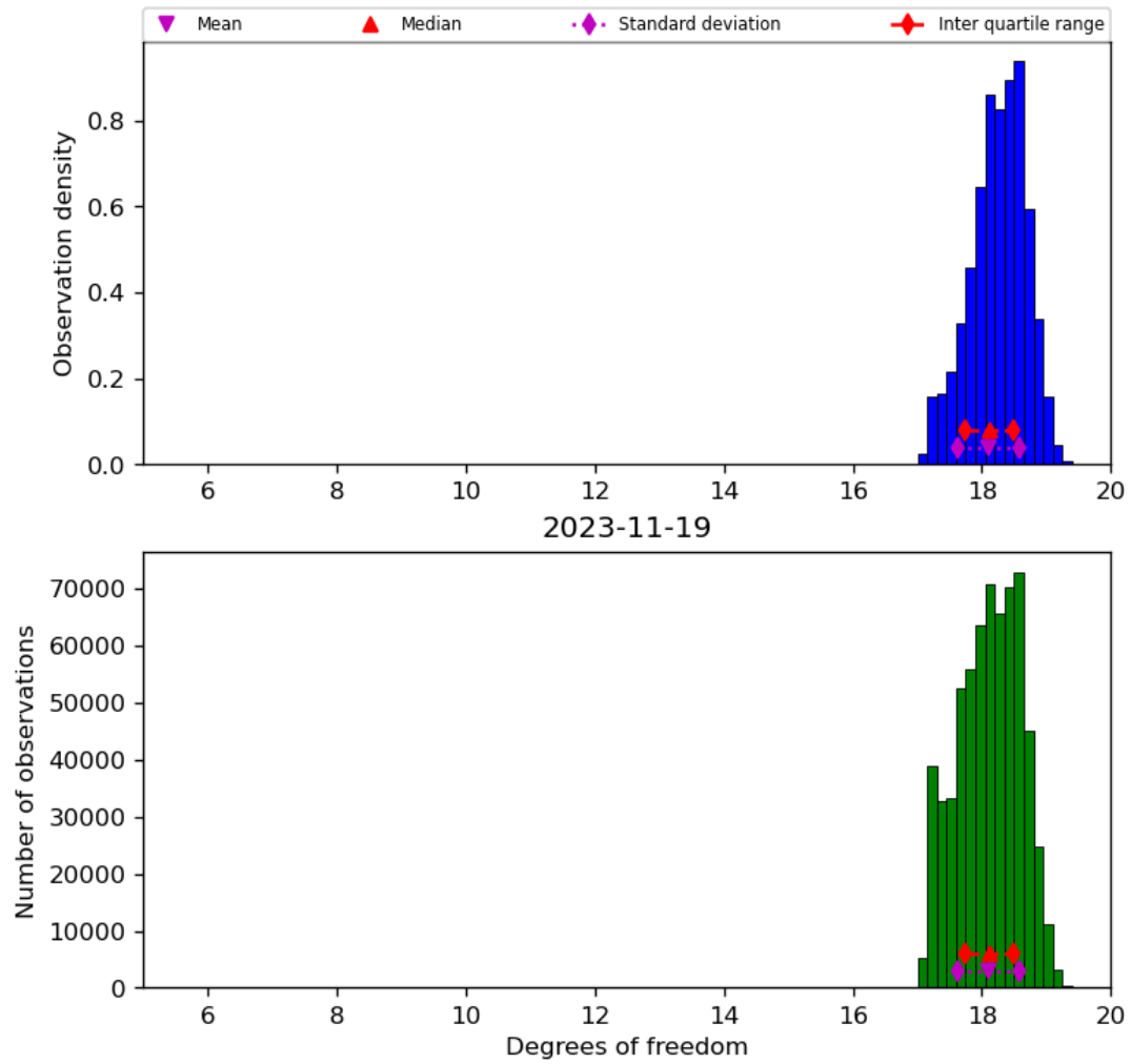
Figure 30: Histogram of “Degrees of freedom” for 2023-11-18 to 2023-11-20
