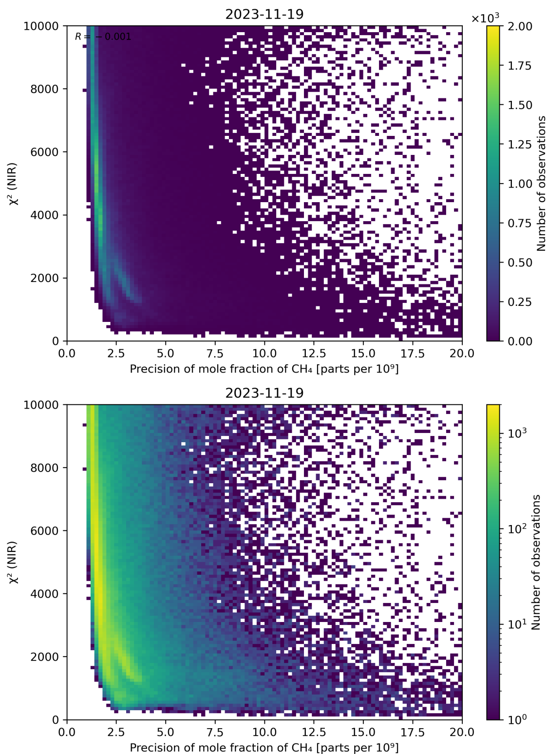
Figure 78: Scatter density plot of “Precision of mole fraction of \text{CH}_4 ” against “ \chi^2 (NIR)” for 2023-11-18 to 2023-11-20.
