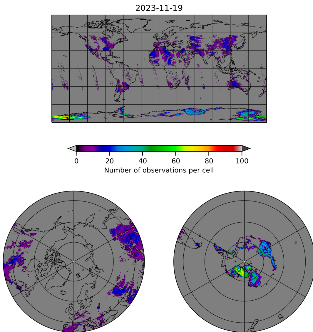
Figure 10: Map of the number of observations for 2023-11-18 to 2023-11-20
