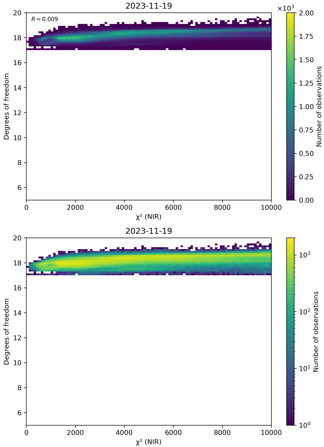
Figure 44: Scatter density plot of “ \chi^2 (NIR)” against “Degrees of freedom” for 2023-11-18 to 2023-11-20.
