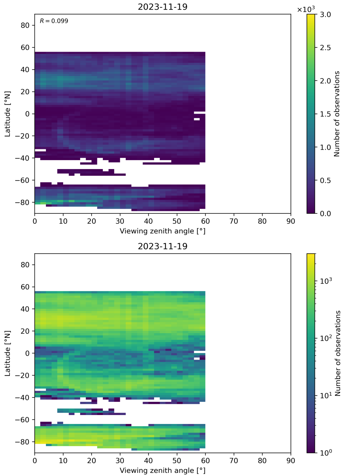
Figure 109: Scatter density plot of “Viewing zenith angle” against “Latitude” for 2023-11-18 to 2023-11-20.
