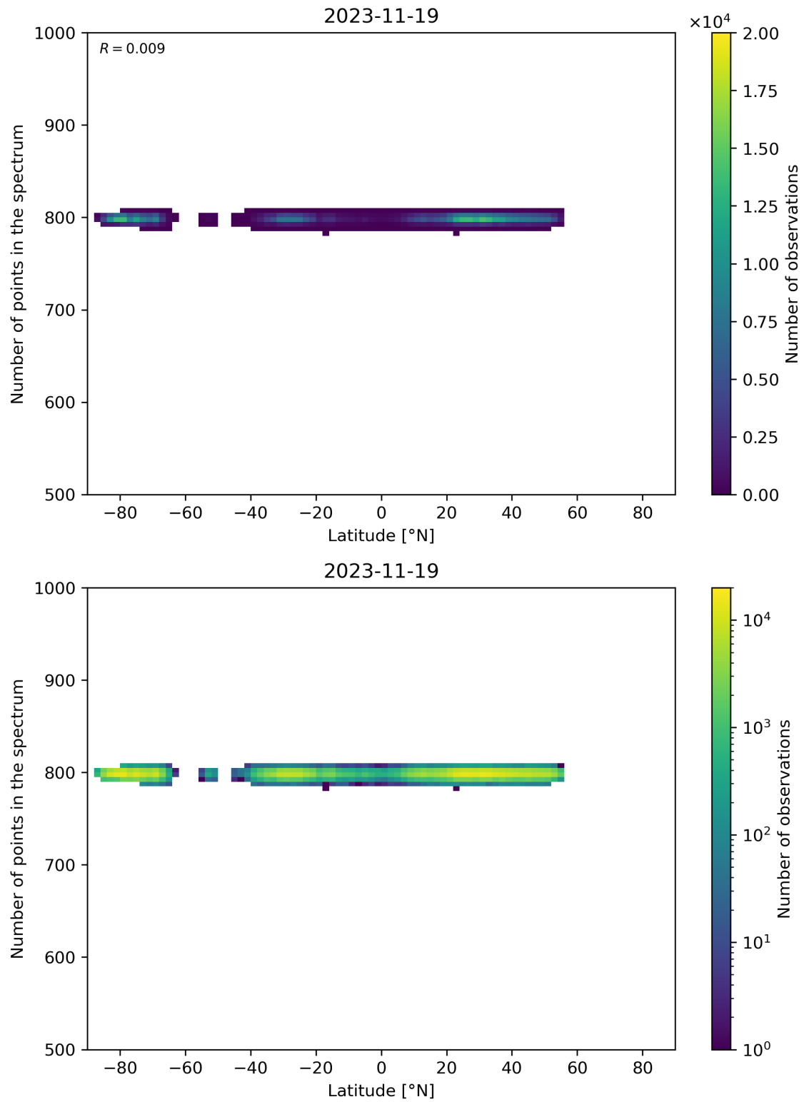
Figure 61: Scatter density plot of “Latitude” against “Number of points in the spectrum” for 2023-11-18 to 2023-11-20.
