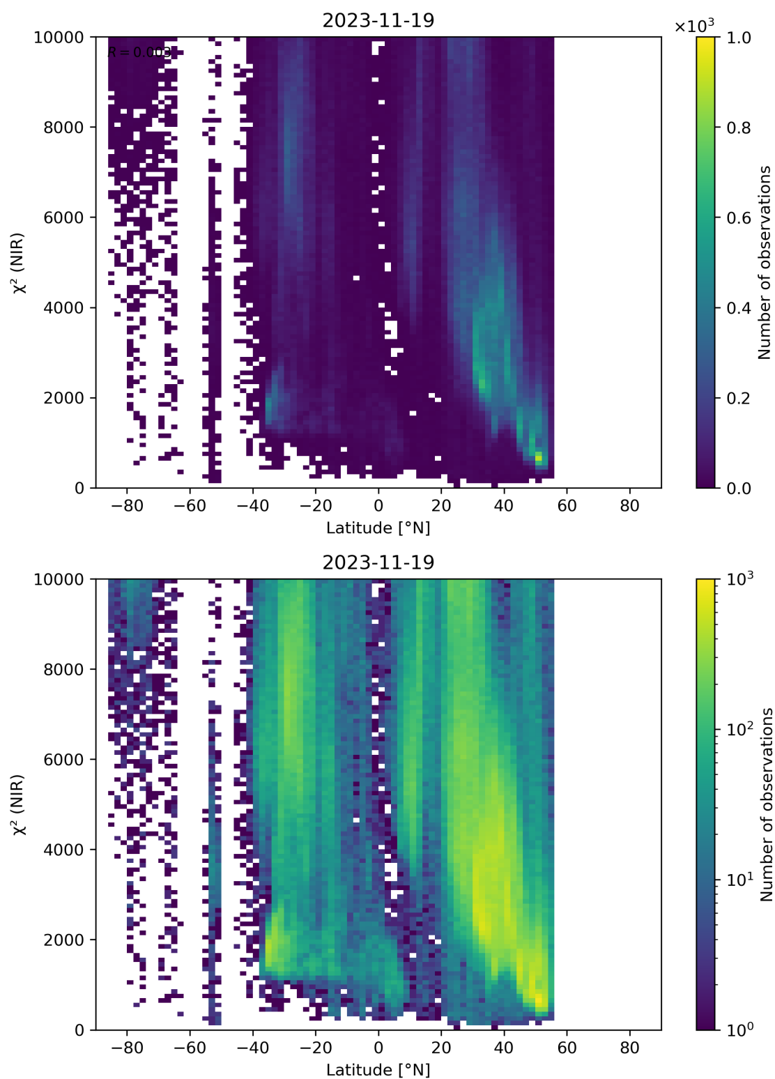
Figure 53: Scatter density plot of “Latitude” against “ \chi^2 (NIR)” for 2023-11-18 to 2023-11-20.
