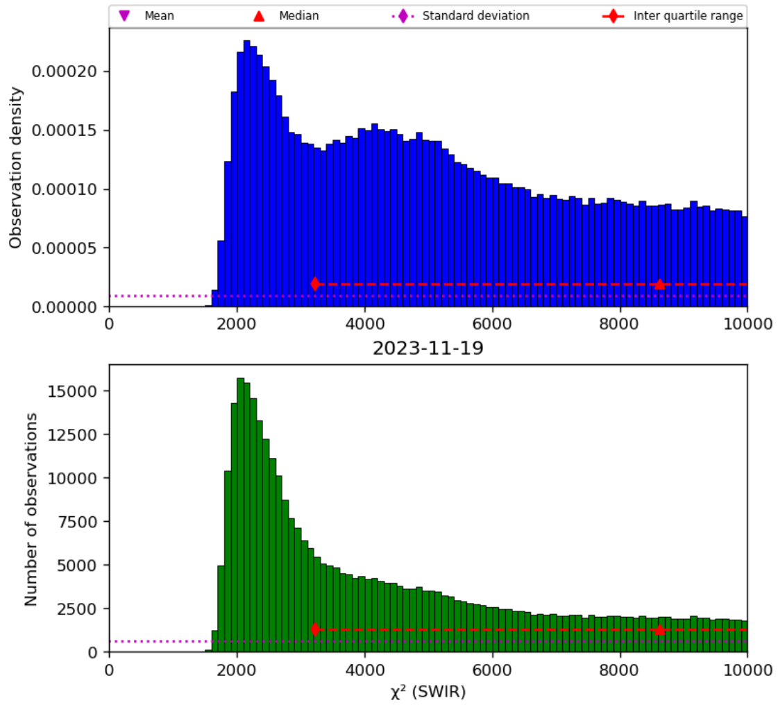
Figure 28: Histogram of “ \chi^2 (SWIR)” for 2023-11-18 to 2023-11-20
