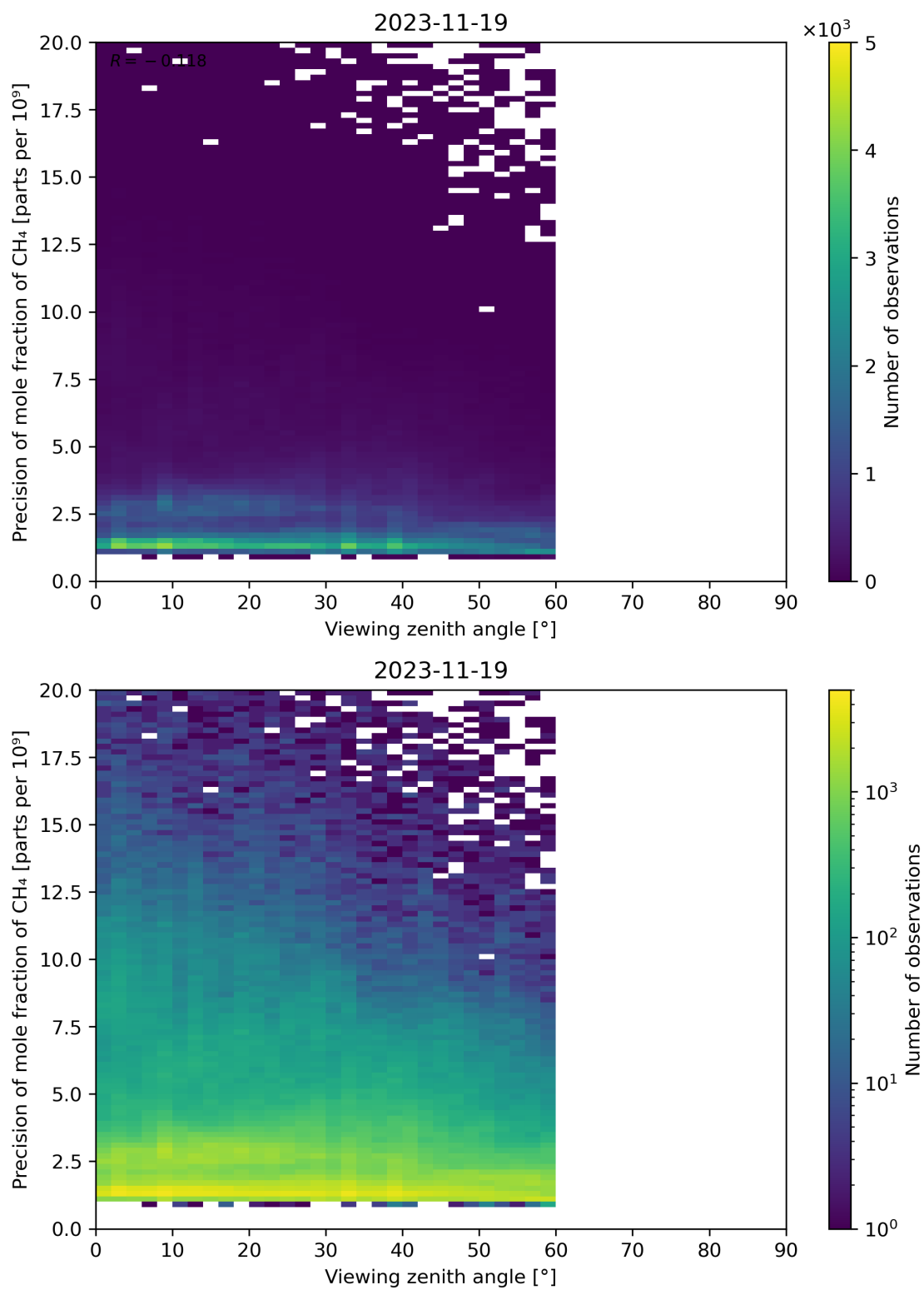
Figure 112: Scatter density plot of “Viewing zenith angle” against “Precision of mole fraction of CH 4 ” for 2023-11-18 to 2023-11-20.
