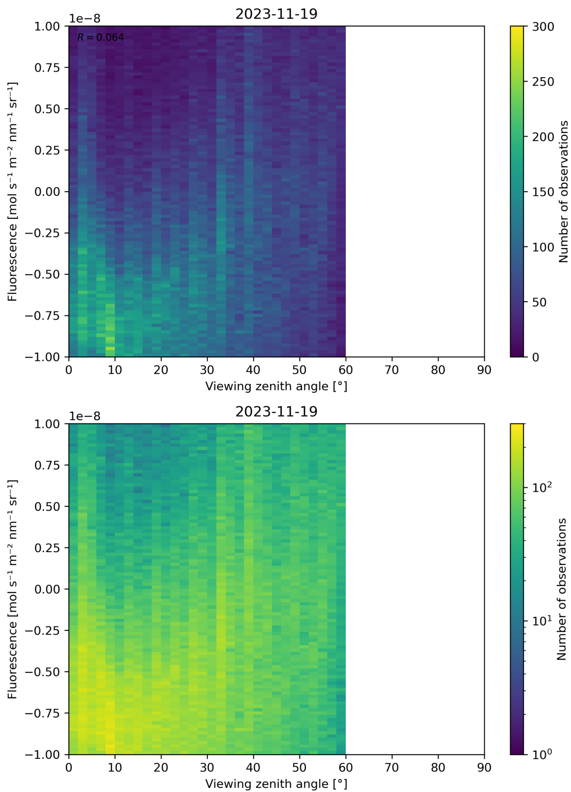
Figure 108: Scatter density plot of “Viewing zenith angle” against “Fluorescence” for 2023-11-18 to 2023-11-20.
