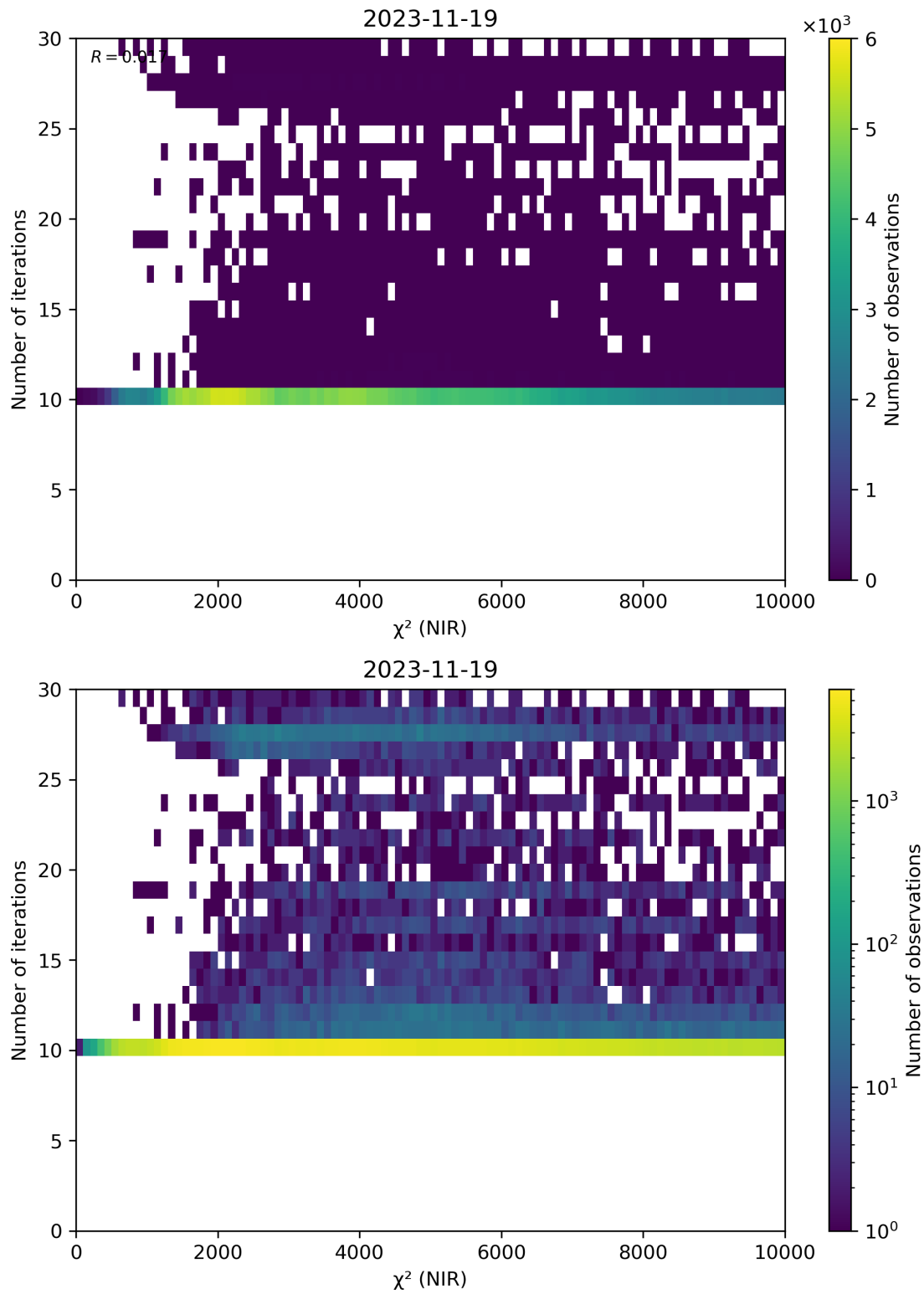
Figure 46: Scatter density plot of “ \chi^2 (NIR)” against “Number of iterations” for 2023-11-18 to 2023-11-20.
