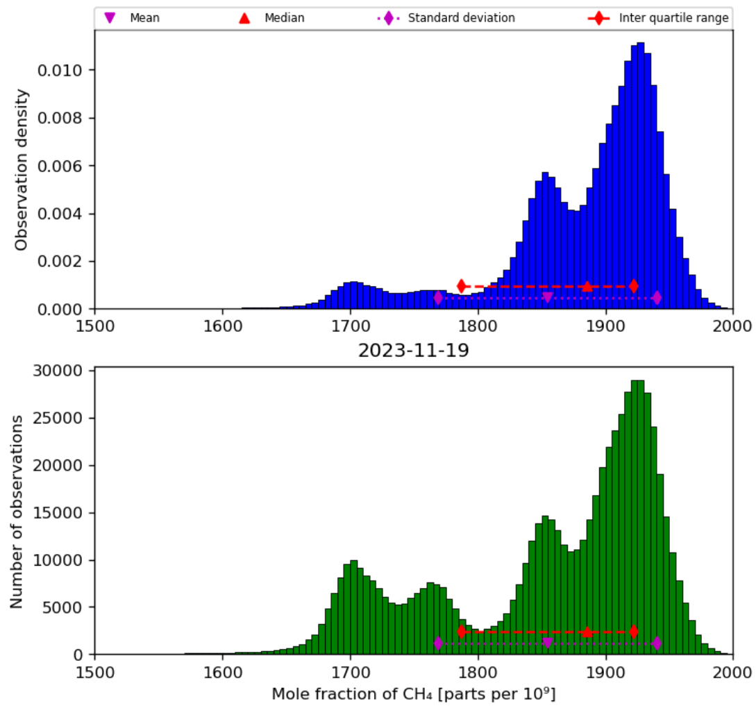
Figure 23: Histogram of “Mole fraction of CH 4 ” for 2023-11-18 to 2023-11-20
