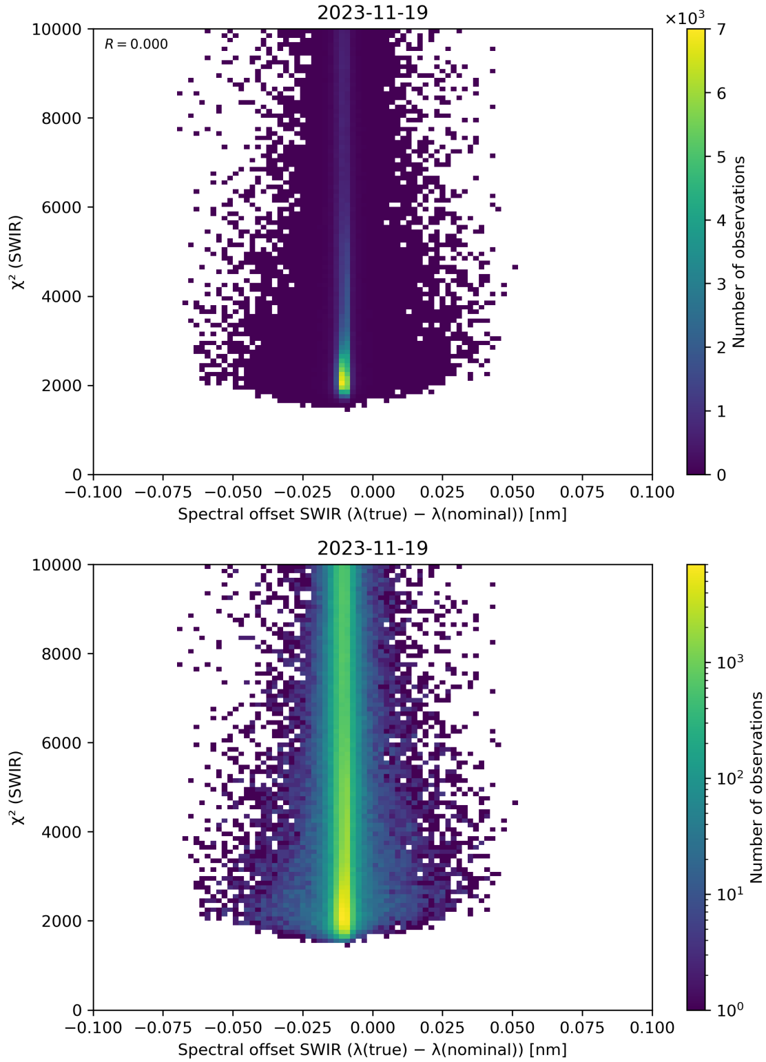
Figure 118: Scatter density plot of “Spectral offset SWIR ( \lambda(\text{true}) - \lambda(\text{nominal}) )” against “ \chi^2 (SWIR)” for 2023-11-18 to 2023-11-20.
