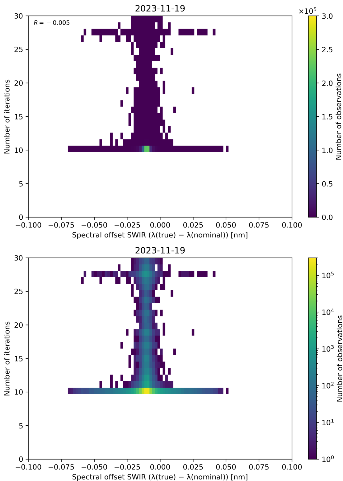
Figure 121: Scatter density plot of “Spectral offset SWIR ( \lambda(\text{true}) - \lambda(\text{nominal}) )” against “Number of iterations” for 2023-11-18 to 2023-11-20.
