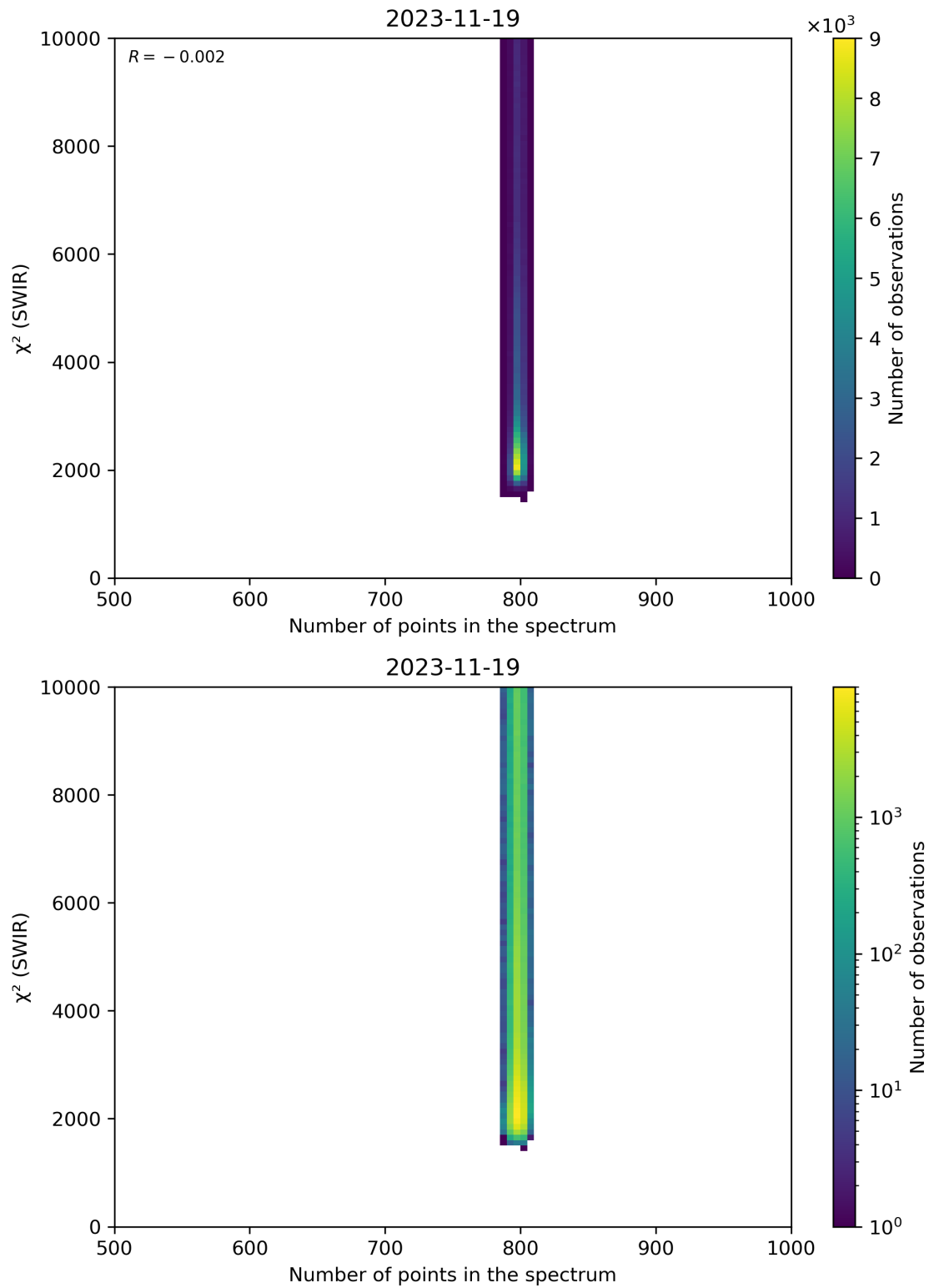
Figure 89: Scatter density plot of “Number of points in the spectrum” against “ \chi^2 (SWIR)” for 2023-11-18 to 2023-11-20.
