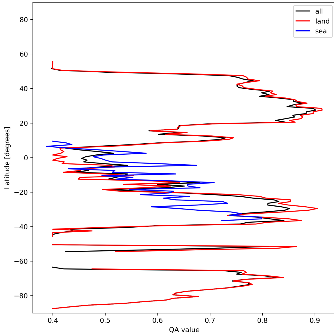
Figure 11: Zonal average of “QA value” for 2023-11-18 to 2023-11-20.
