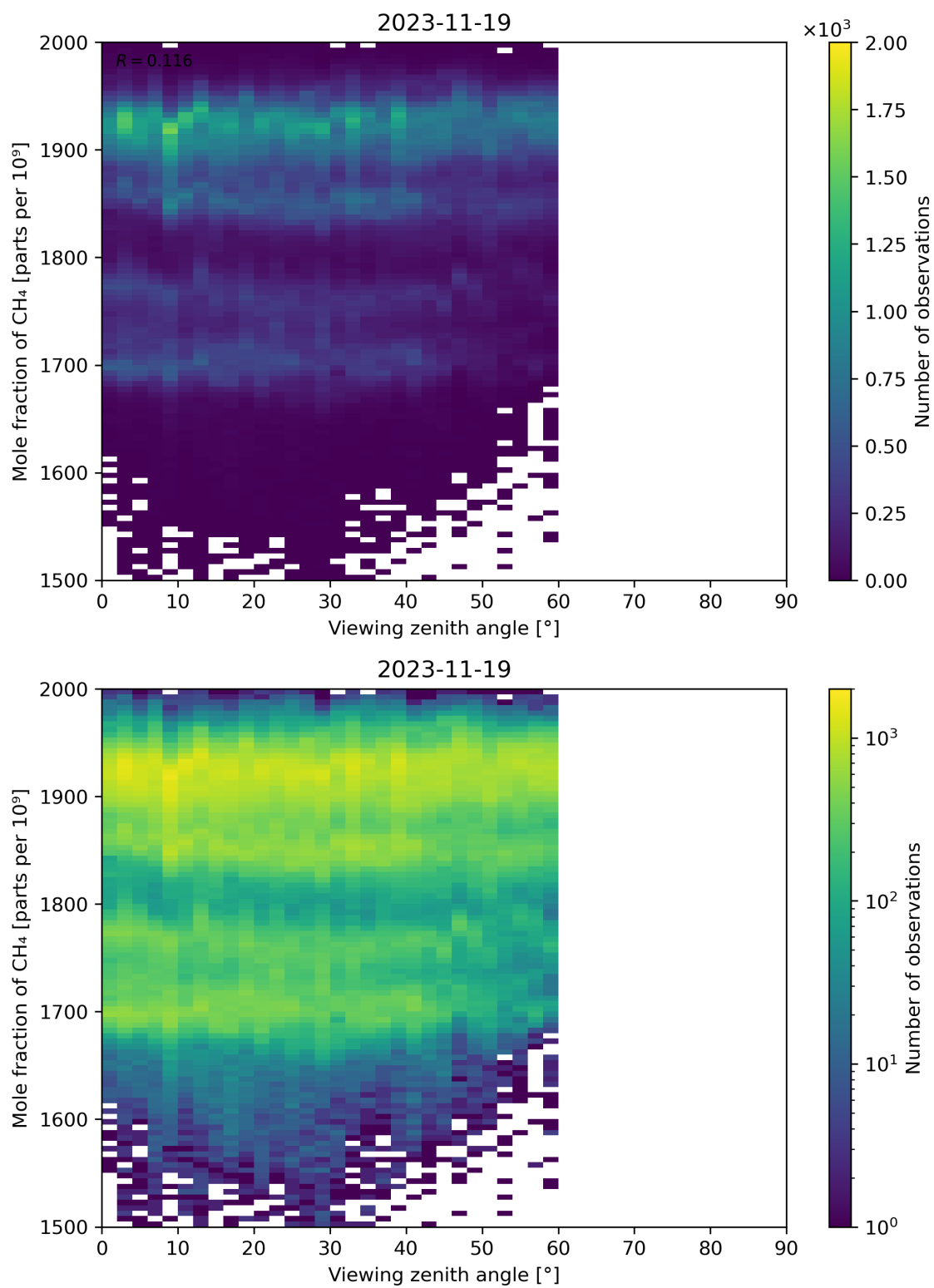
Figure 110: Scatter density plot of “Viewing zenith angle” against “Mole fraction of CH 4 ” for 2023-11-18 to 2023-11-20.
