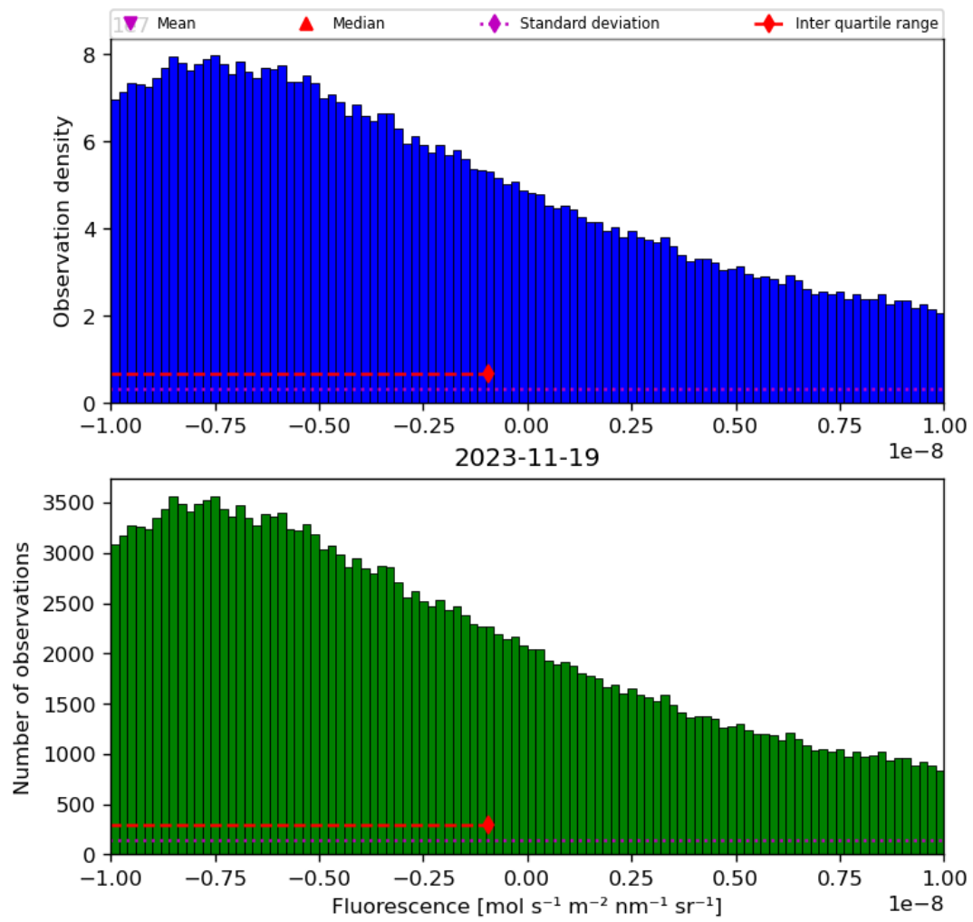
Figure 32: Histogram of “Fluorescence” for 2023-11-18 to 2023-11-20
