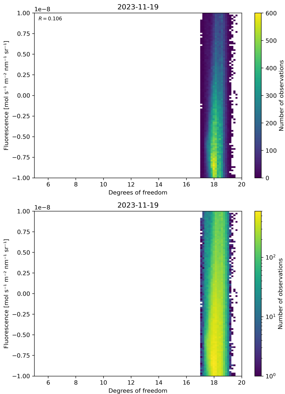
Figure 51: Scatter density plot of “Degrees of freedom” against “Fluorescence” for 2023-11-18 to 2023-11-20.
