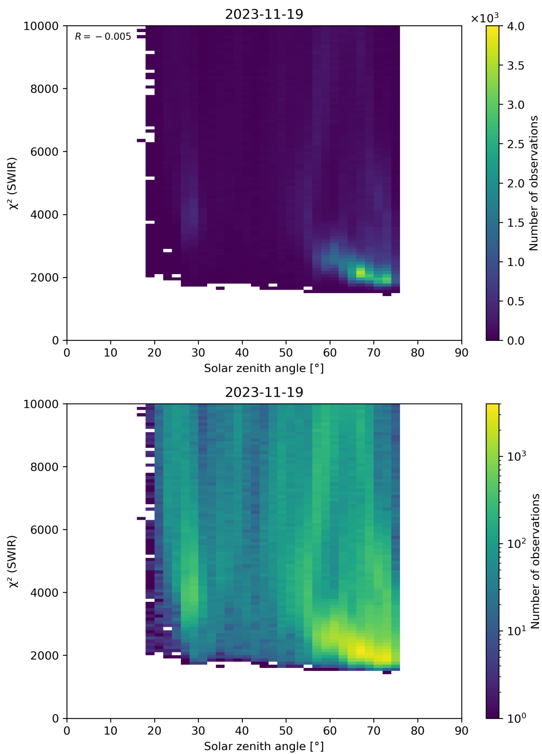
Figure 95: Scatter density plot of “Solar zenith angle” against “ \chi^2 (SWIR)” for 2023-11-18 to 2023-11-20.
