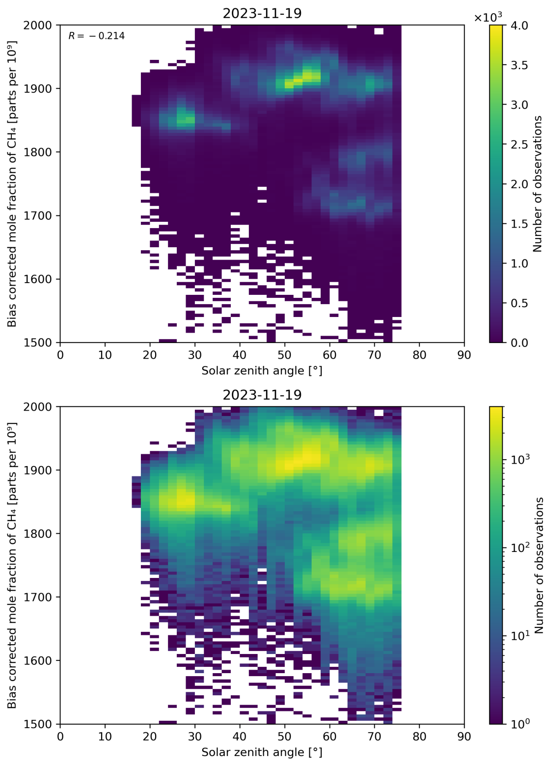
Figure 100: Scatter density plot of “Solar zenith angle” against “Bias corrected mole fraction of CH 4 ” for 2023-11-18 to 2023-11-20.
