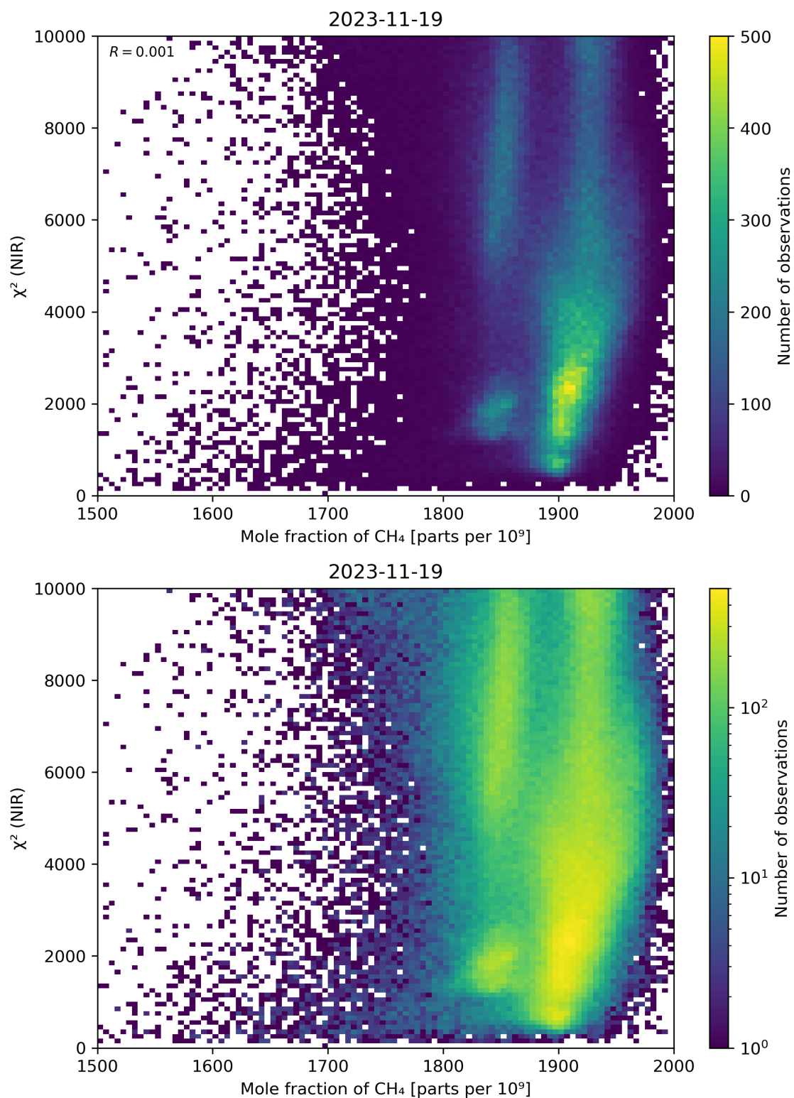
Figure 70: Scatter density plot of “Mole fraction of CH 4 ” against “ \chi^2 (NIR)” for 2023-11-18 to 2023-11-20.
