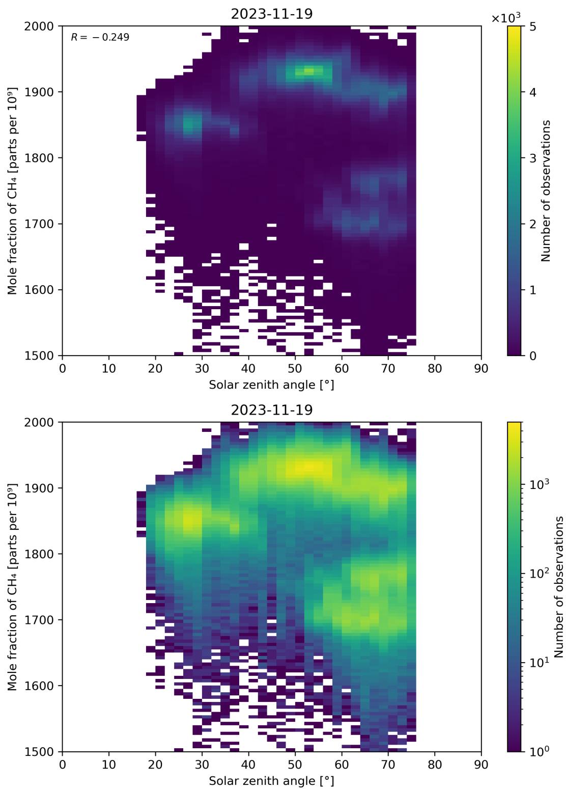
Figure 99: Scatter density plot of “Solar zenith angle” against “Mole fraction of CH 4 ” for 2023-11-18 to 2023-11-20.
