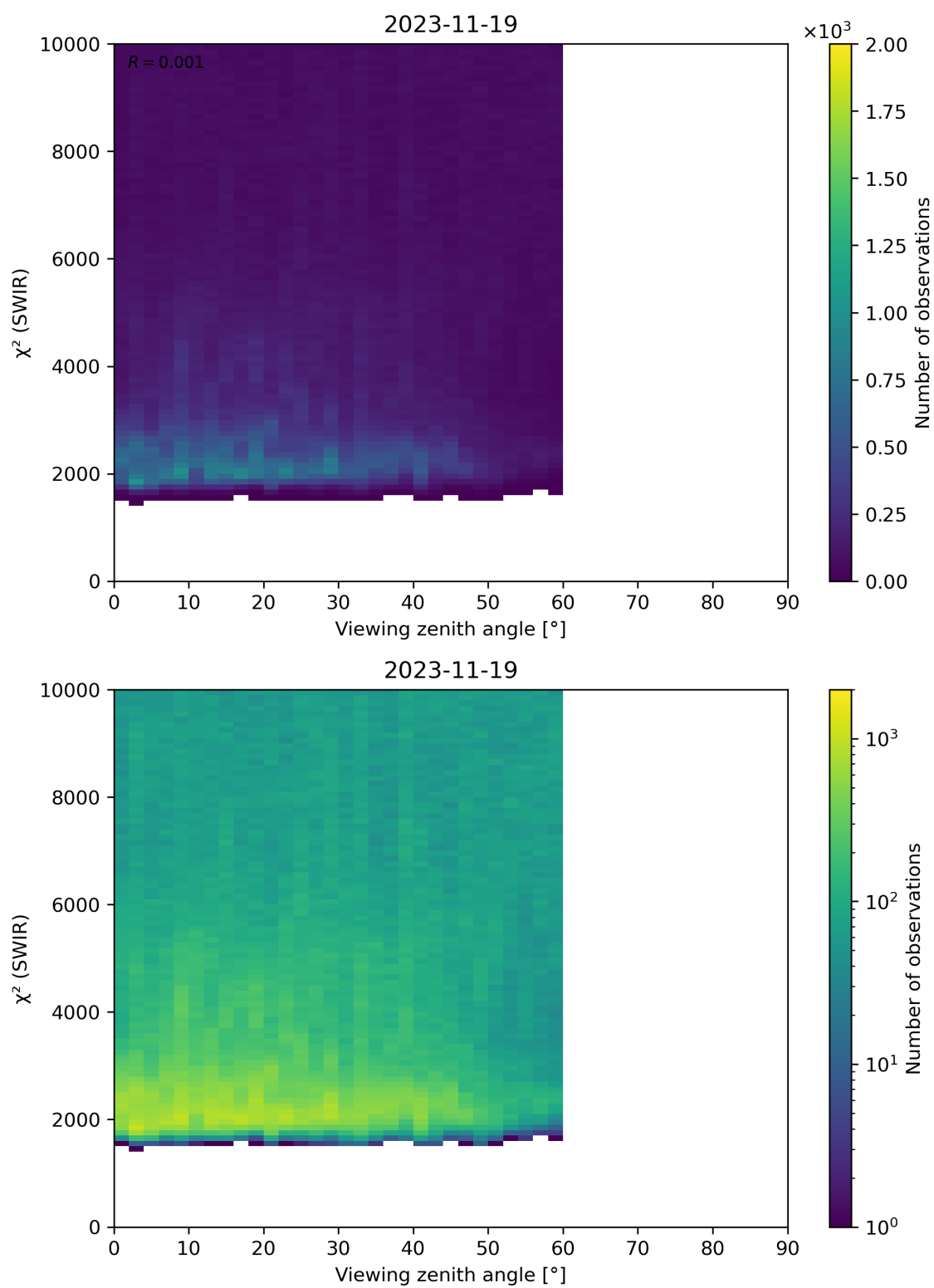
Figure 106: Scatter density plot of “Viewing zenith angle” against “ \chi^2 (SWIR)” for 2023-11-18 to 2023-11-20.
