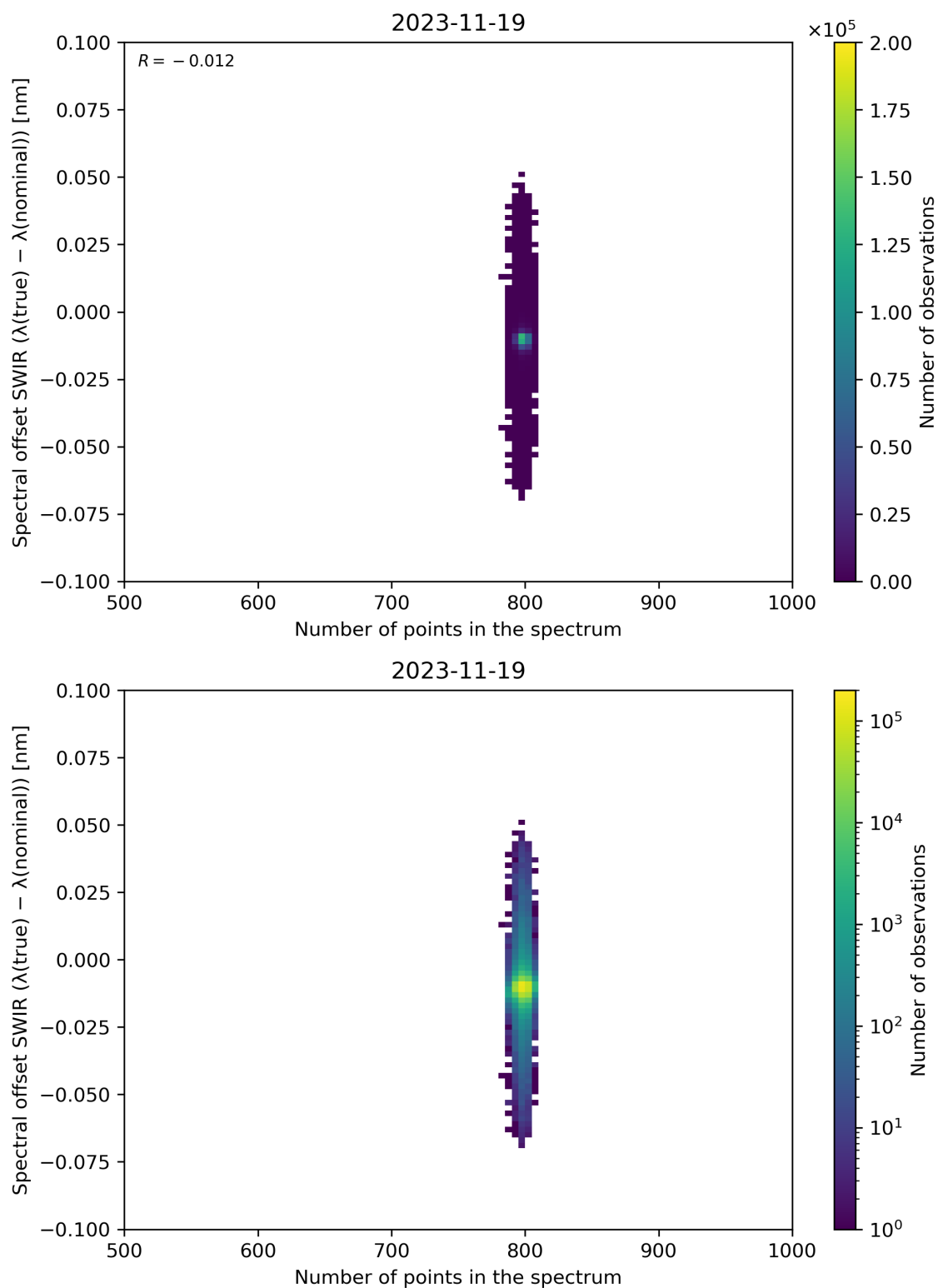
Figure 93: Scatter density plot of “Number of points in the spectrum” against “Spectral offset SWIR ( \lambda(\text{true}) - \lambda(\text{nominal}) )” for 2023-11-18 to 2023-11-20.
