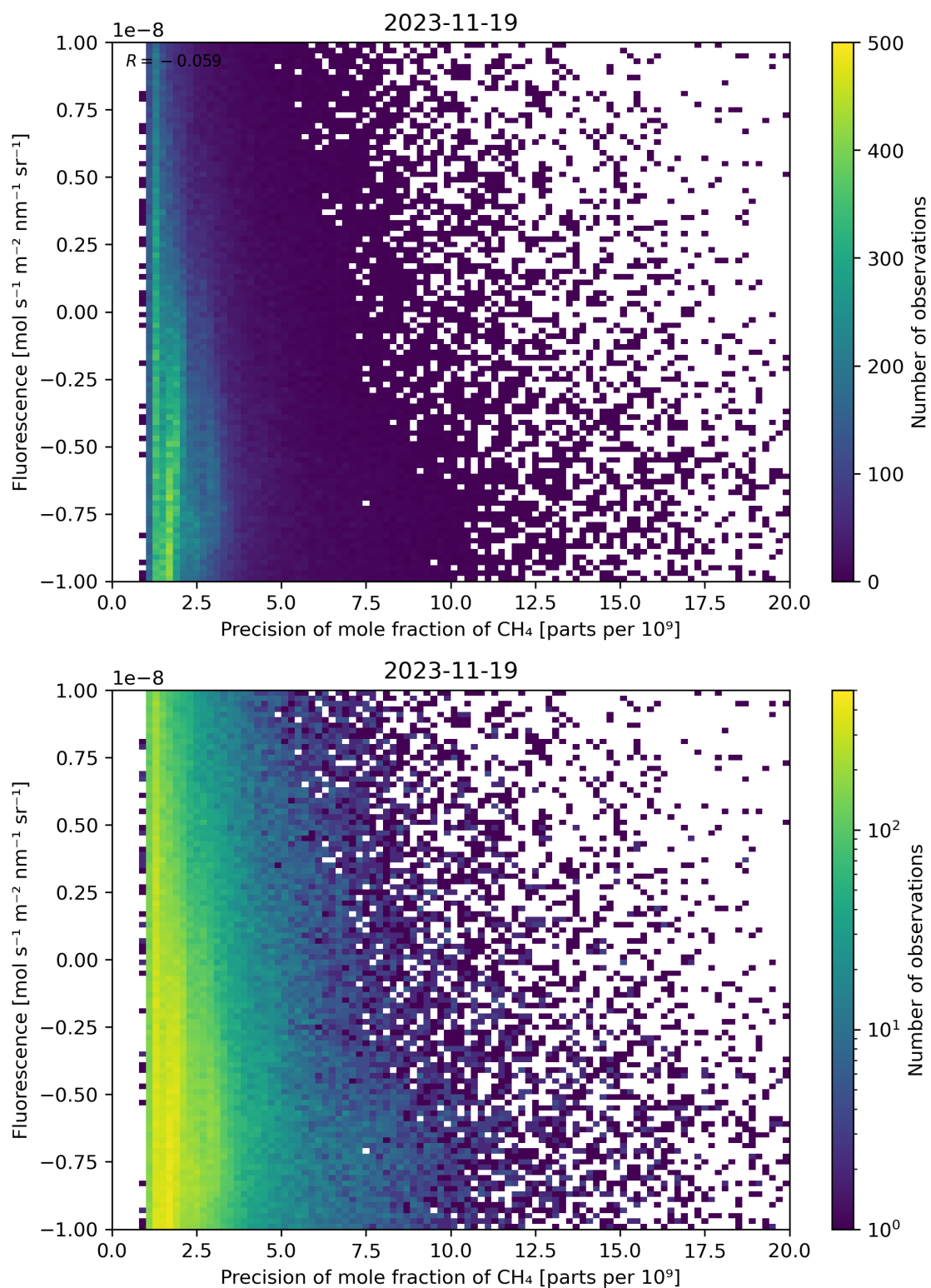
Figure 81: Scatter density plot of “Precision of mole fraction of CH 4 ” against “Fluorescence” for 2023-11-18 to 2023-11-20.
