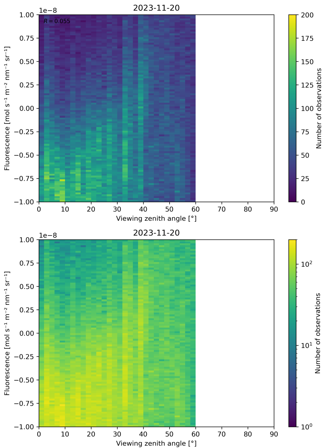
Figure 108: Scatter density plot of “Viewing zenith angle” against “Fluorescence” for 2023-11-19 to 2023-11-21.
