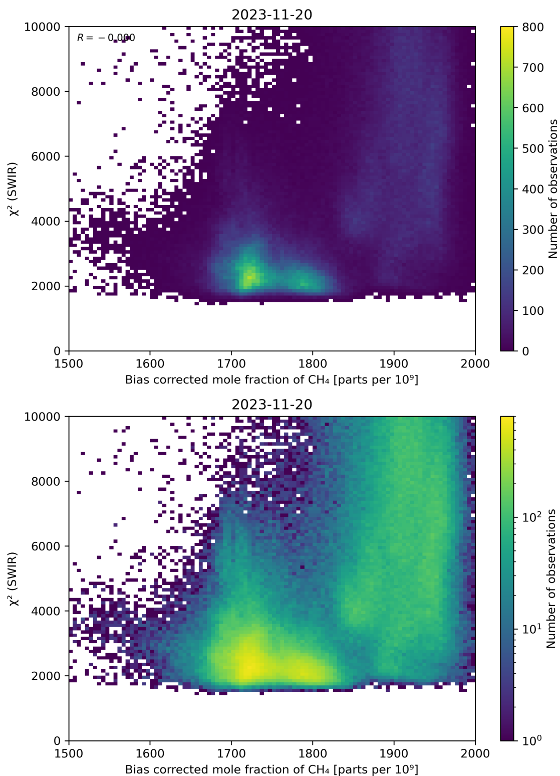
Figure 64: Scatter density plot of “Bias corrected mole fraction of CH 4 ” against “ \chi^2 (SWIR)” for 2023-11-19 to 2023-11-21.
