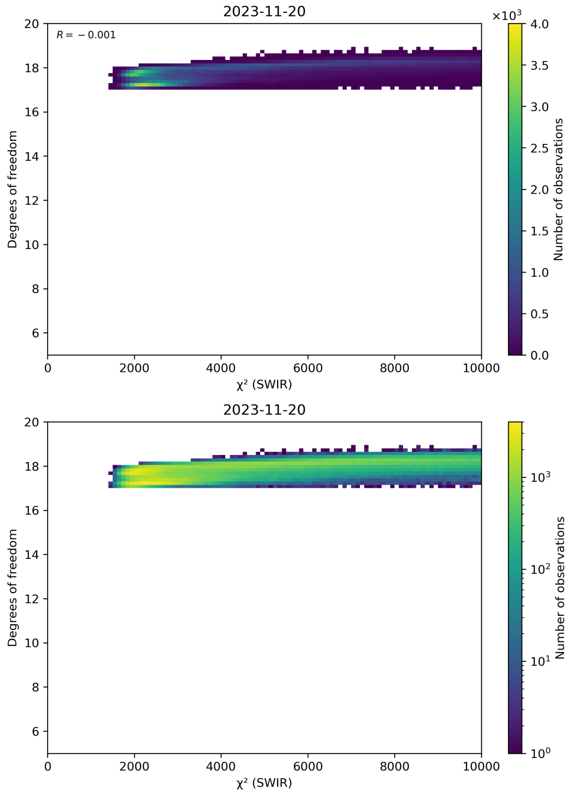
Figure 48: Scatter density plot of “ \chi^2 (SWIR)” against “Degrees of freedom” for 2023-11-19 to 2023-11-21.
