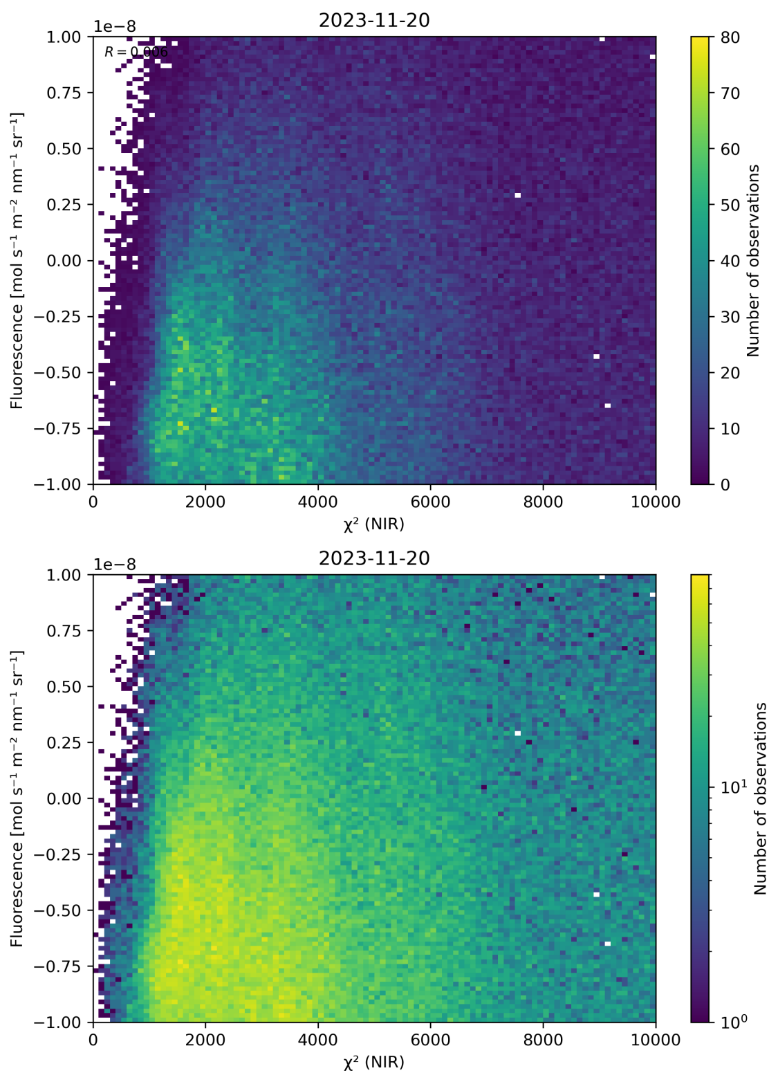
Figure 45: Scatter density plot of “ \chi^2 (NIR)” against “Fluorescence” for 2023-11-19 to 2023-11-21.
