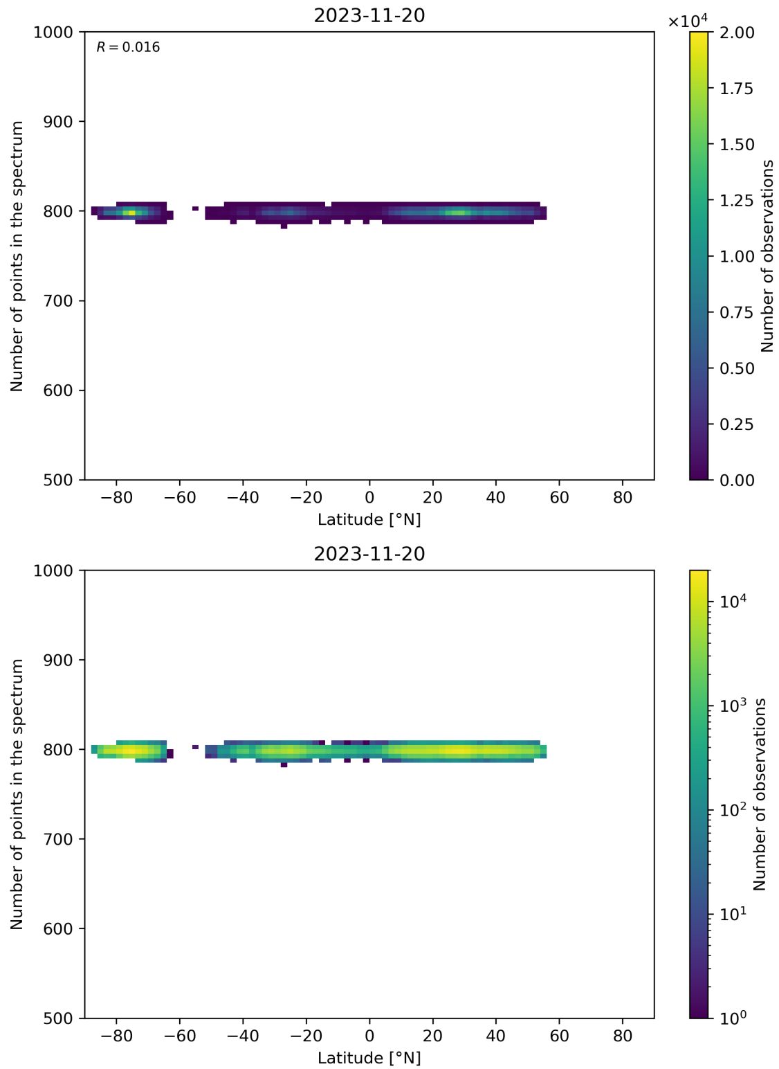
Figure 61: Scatter density plot of “Latitude” against “Number of points in the spectrum” for 2023-11-19 to 2023-11-21.
