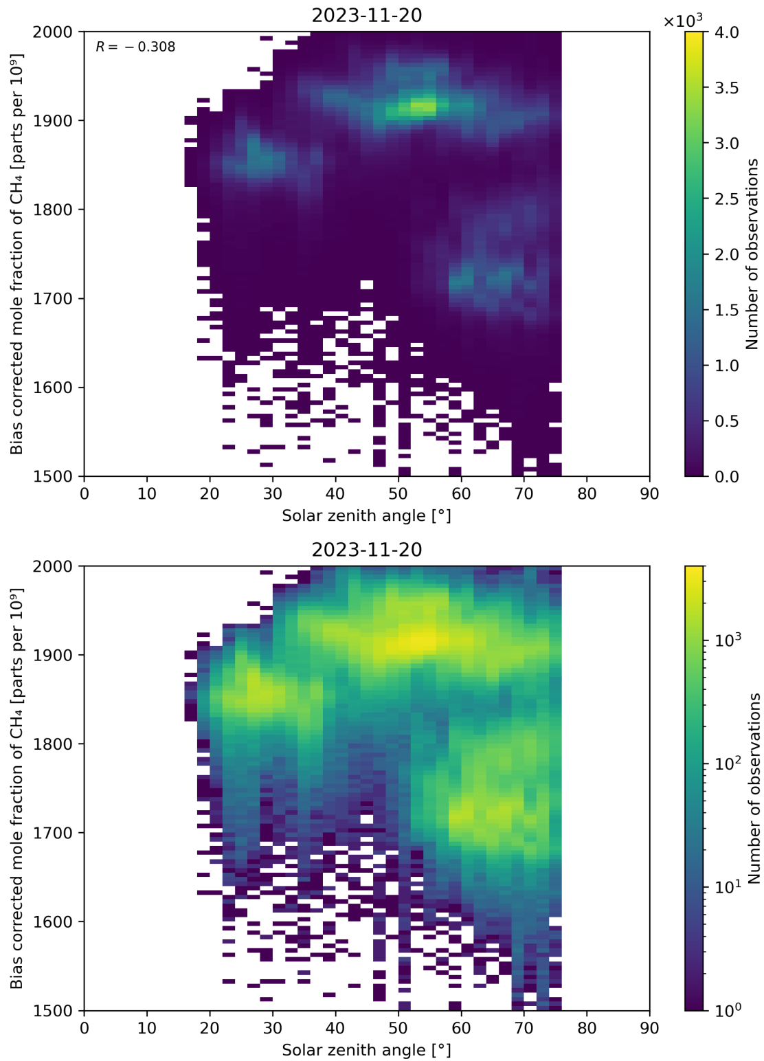
Figure 100: Scatter density plot of “Solar zenith angle” against “Bias corrected mole fraction of CH 4 ” for 2023-11-19 to 2023-11-21.
