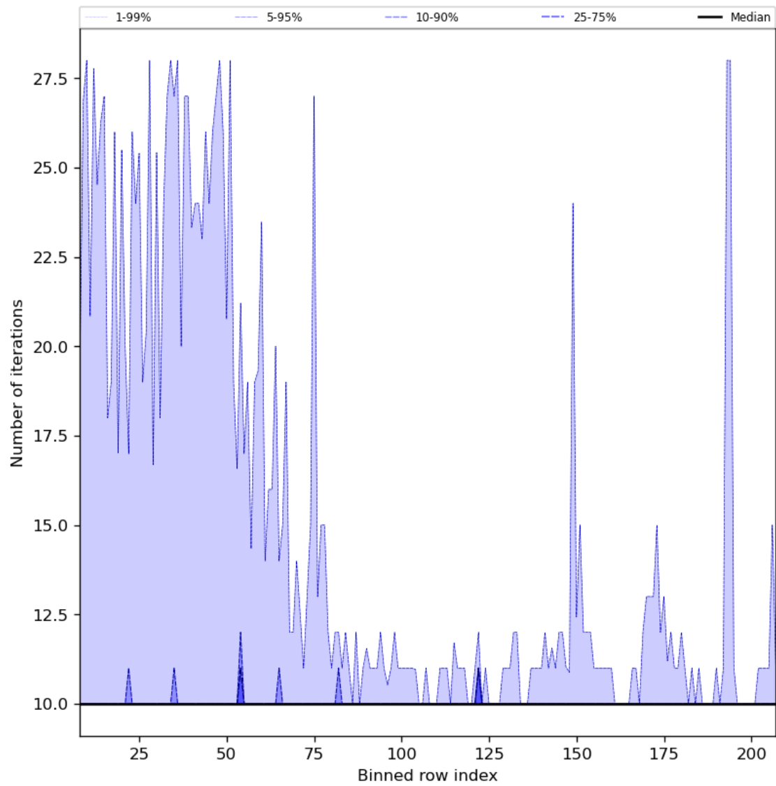
Figure 42: Along track statistics of “Number of iterations” for 2023-11-19 to 2023-11-21
