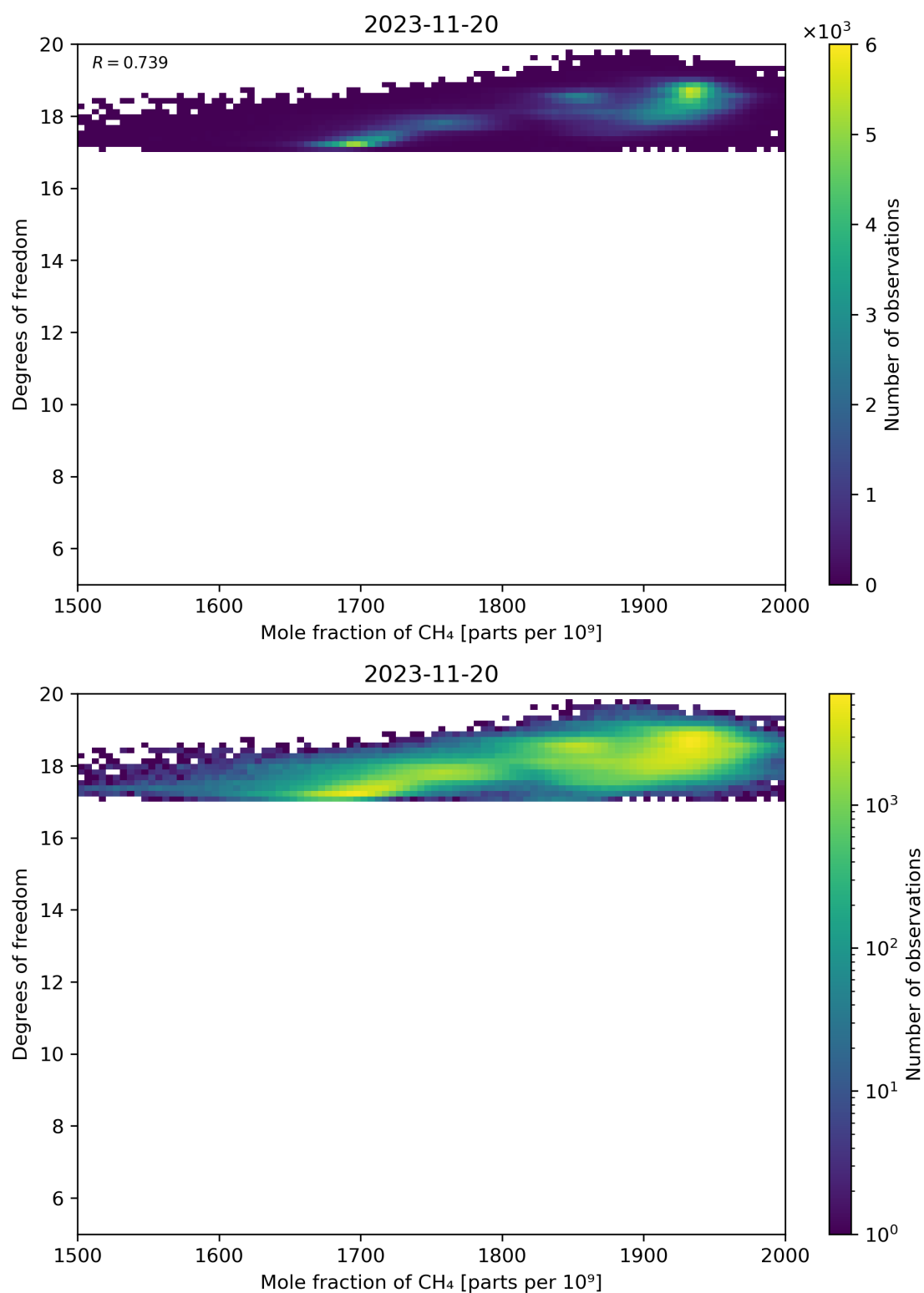
Figure 72: Scatter density plot of “Mole fraction of CH 4 ” against “Degrees of freedom” for 2023-11-19 to 2023-11-21.
