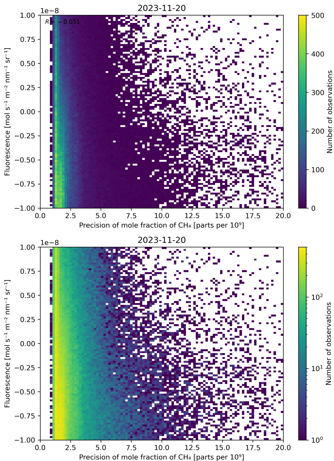
Figure 81: Scatter density plot of “Precision of mole fraction of \text{CH}_4 ” against “Fluorescence” for 2023-11-19 to 2023-11-21.
