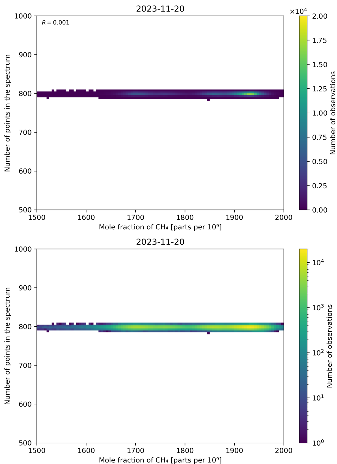
Figure 77: Scatter density plot of “Mole fraction of CH 4 ” against “Number of points in the spectrum” for 2023-11-19 to 2023-11-21.
