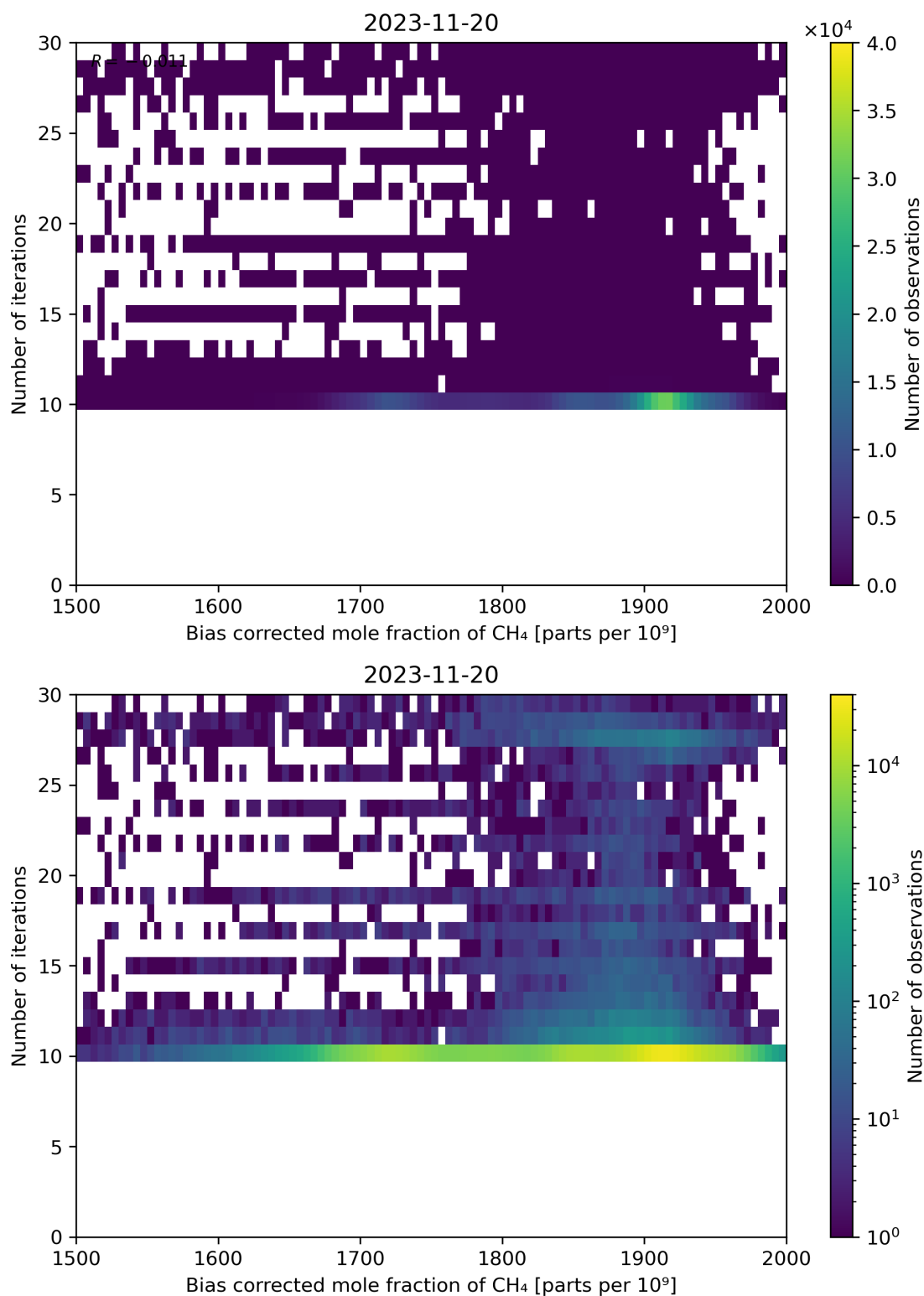
Figure 67: Scatter density plot of “Bias corrected mole fraction of \text{CH}_4 ” against “Number of iterations” for 2023-11-19 to 2023-11-21.
