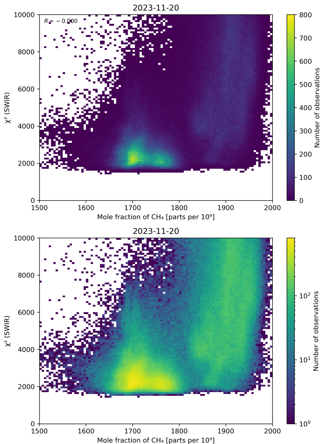
Figure 71: Scatter density plot of “Mole fraction of \text{CH}_4 ” against “ \chi^2 (SWIR)” for 2023-11-19 to 2023-11-21.
