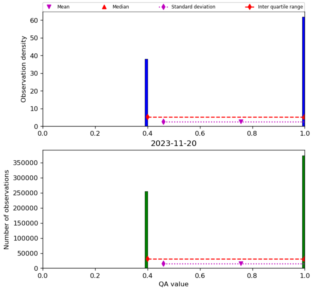
Figure 22: Histogram of “QA value” for 2023-11-19 to 2023-11-21
