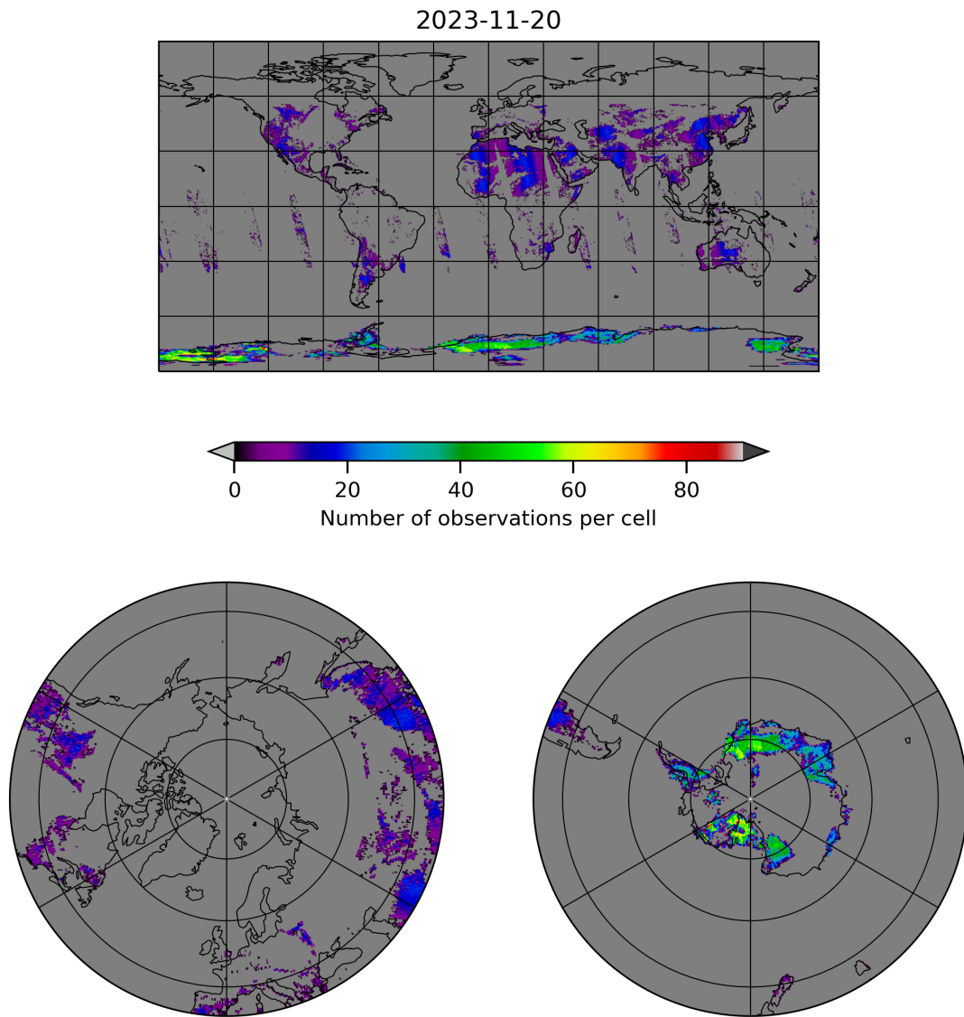
Figure 10: Map of the number of observations for 2023-11-19 to 2023-11-21
