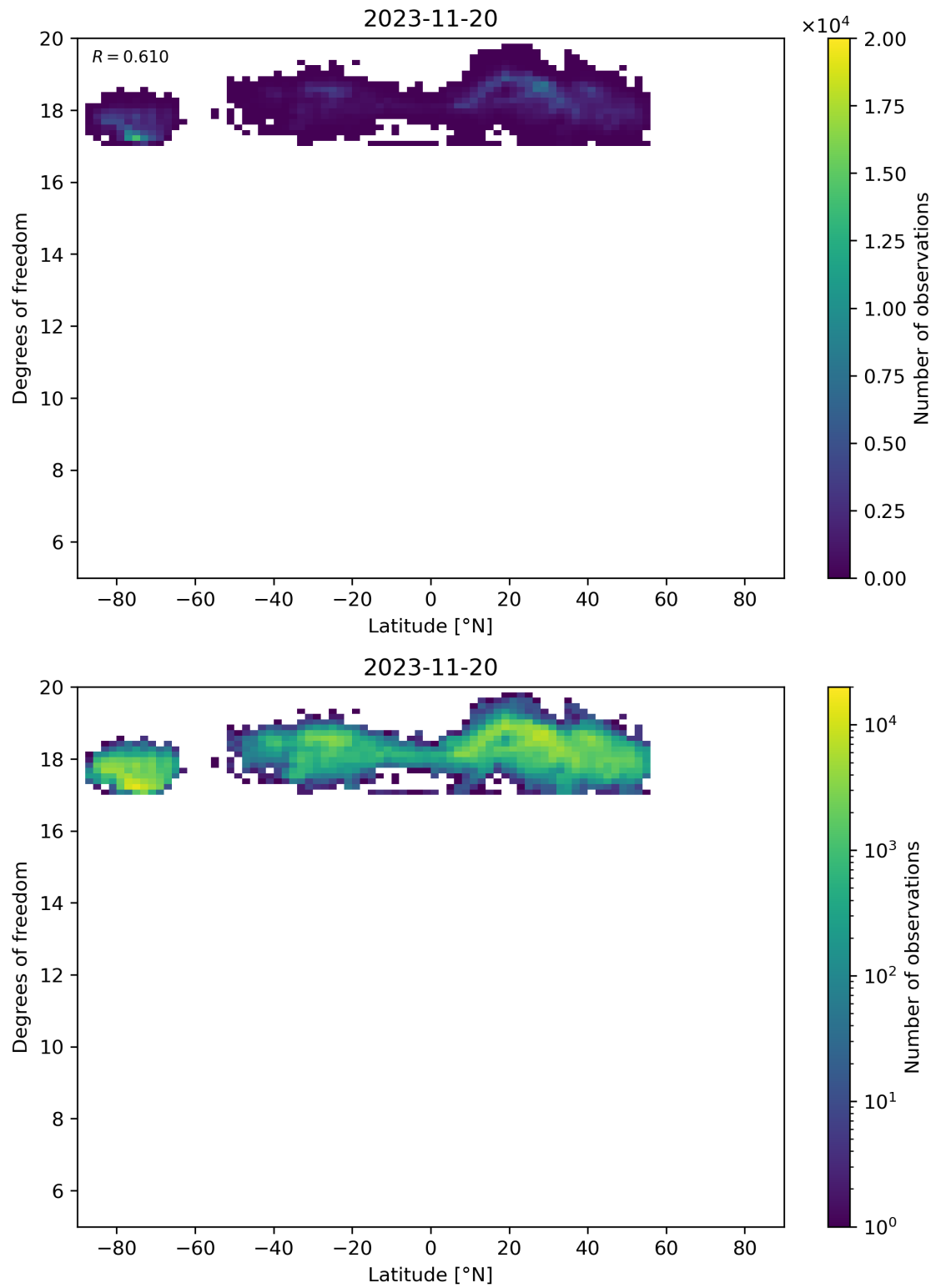
Figure 55: Scatter density plot of “Latitude” against “Degrees of freedom” for 2023-11-19 to 2023-11-21.
