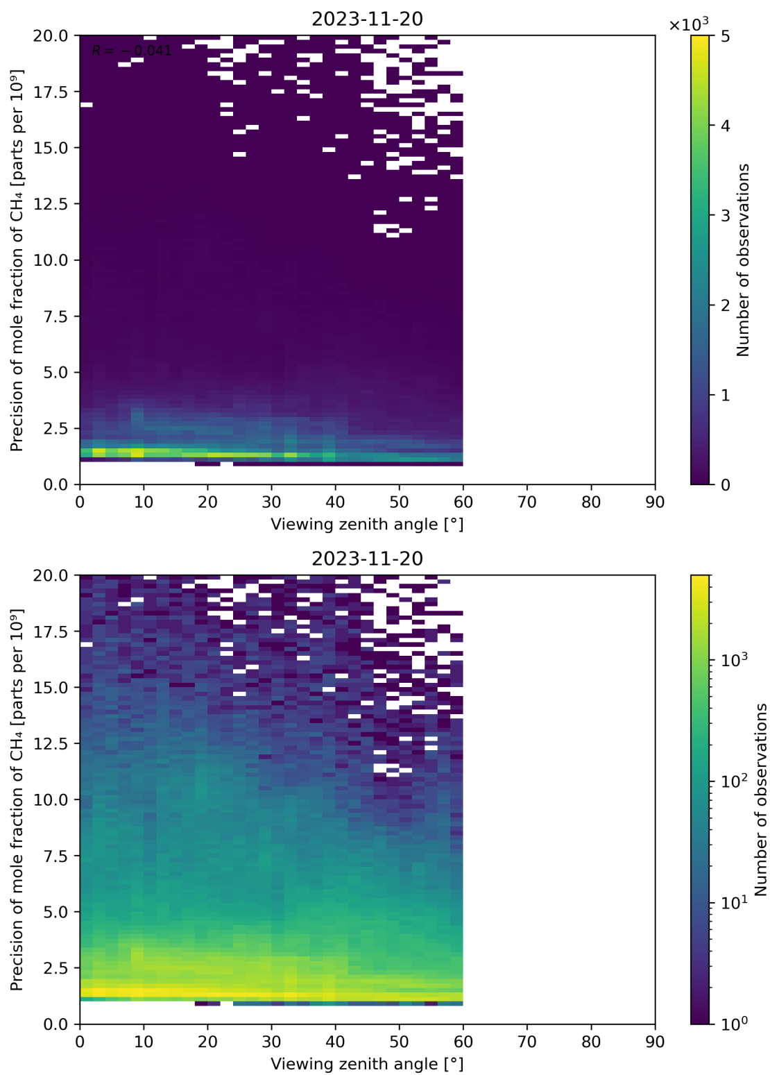
Figure 112: Scatter density plot of “Viewing zenith angle” against “Precision of mole fraction of CH 4 ” for 2023-11-19 to 2023-11-21.
