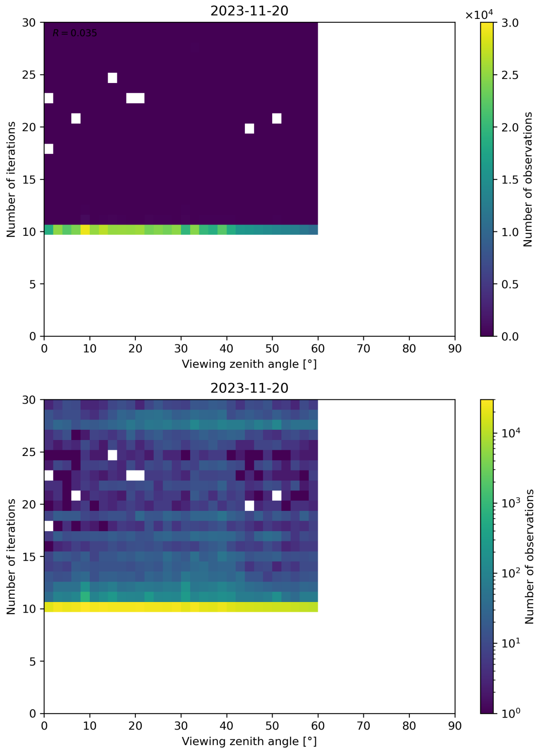
Figure 113: Scatter density plot of “Viewing zenith angle” against “Number of iterations” for 2023-11-19 to 2023-11-21.
