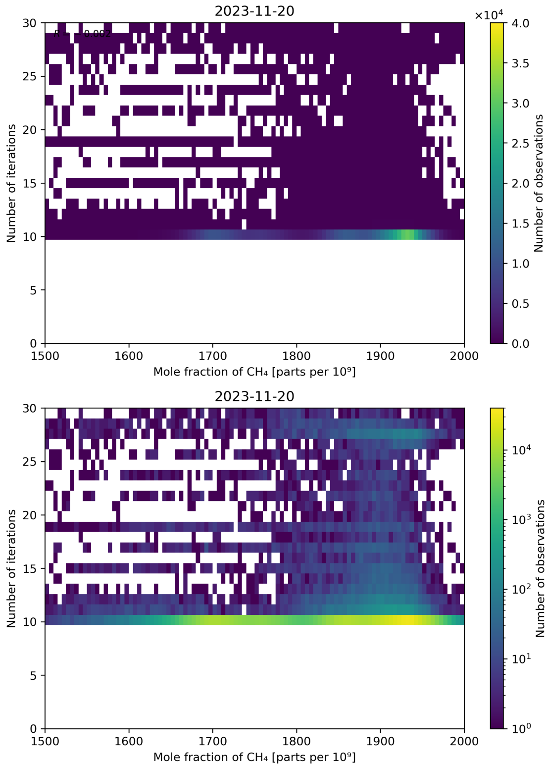
Figure 76: Scatter density plot of “Mole fraction of CH 4 ” against “Number of iterations” for 2023-11-19 to 2023-11-21.
