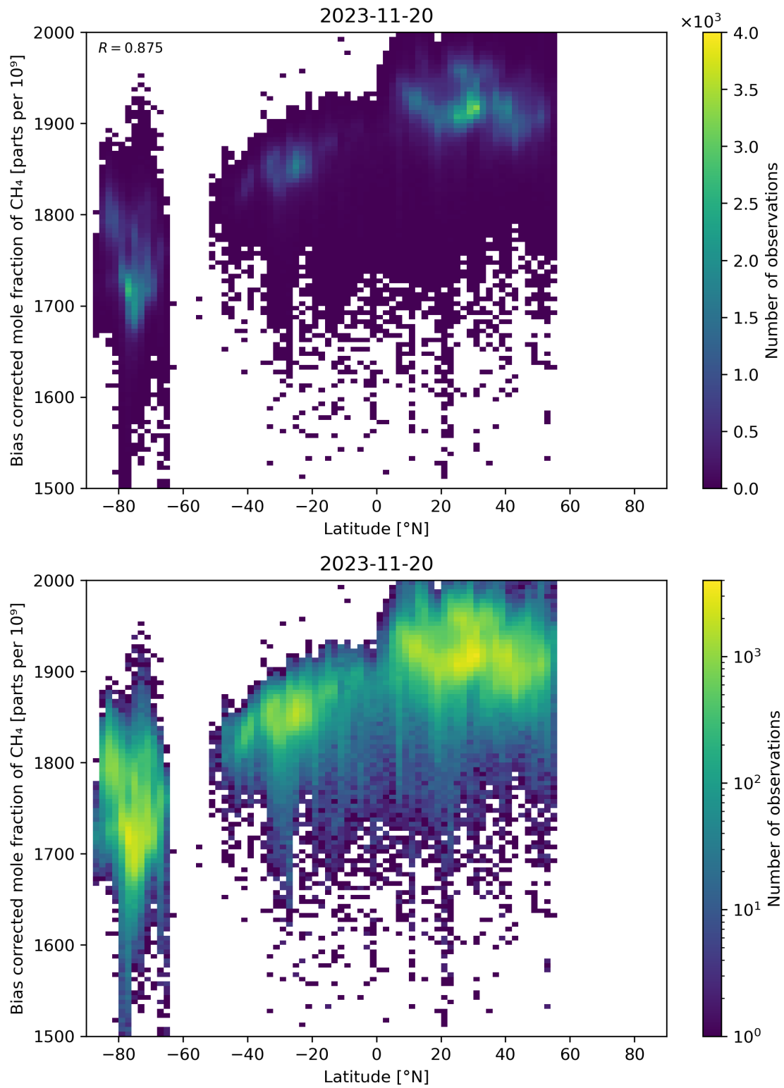
Figure 58: Scatter density plot of “Latitude” against “Bias corrected mole fraction of CH 4 ” for 2023-11-19 to 2023-11-21.
