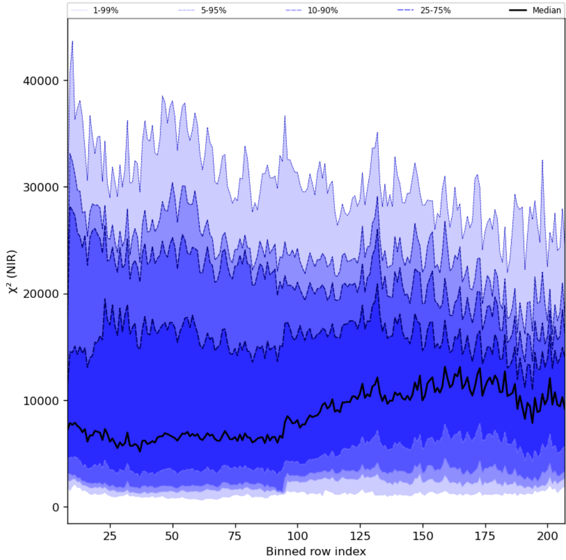
Figure 40: Along track statistics of " \chi^2 (NIR)" for 2023-11-19 to 2023-11-21
