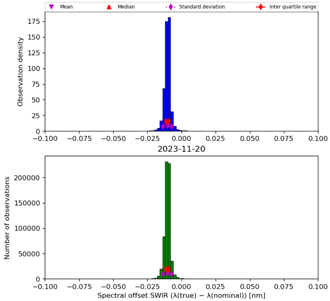
Figure 27: Histogram of “Spectral offset SWIR ( \lambda(\text{true}) - \lambda(\text{nominal}) )” for 2023-11-19 to 2023-11-21
