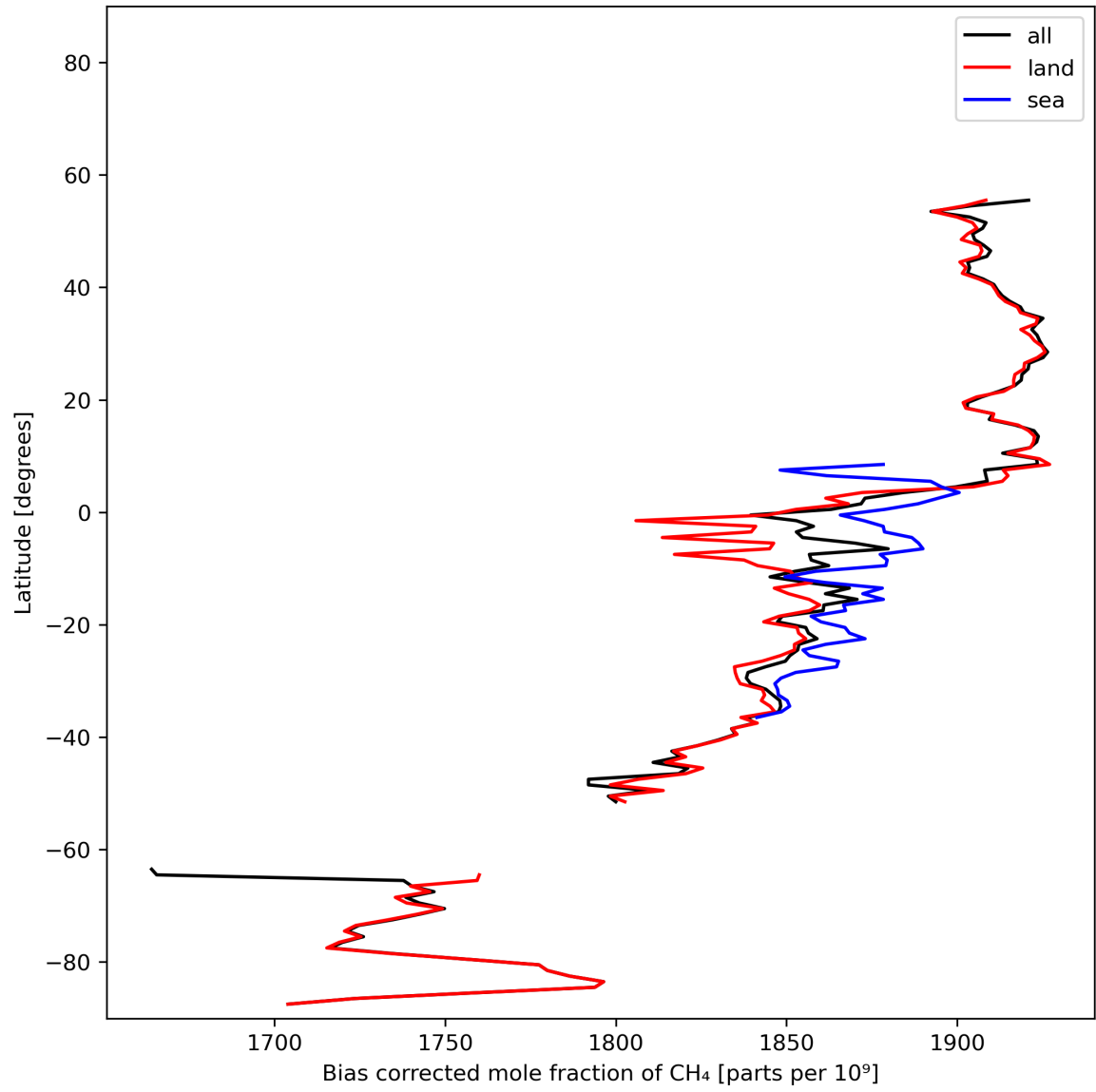
Figure 14: Zonal average of “Bias corrected mole fraction of CH 4 ” for 2023-11-19 to 2023-11-21.
