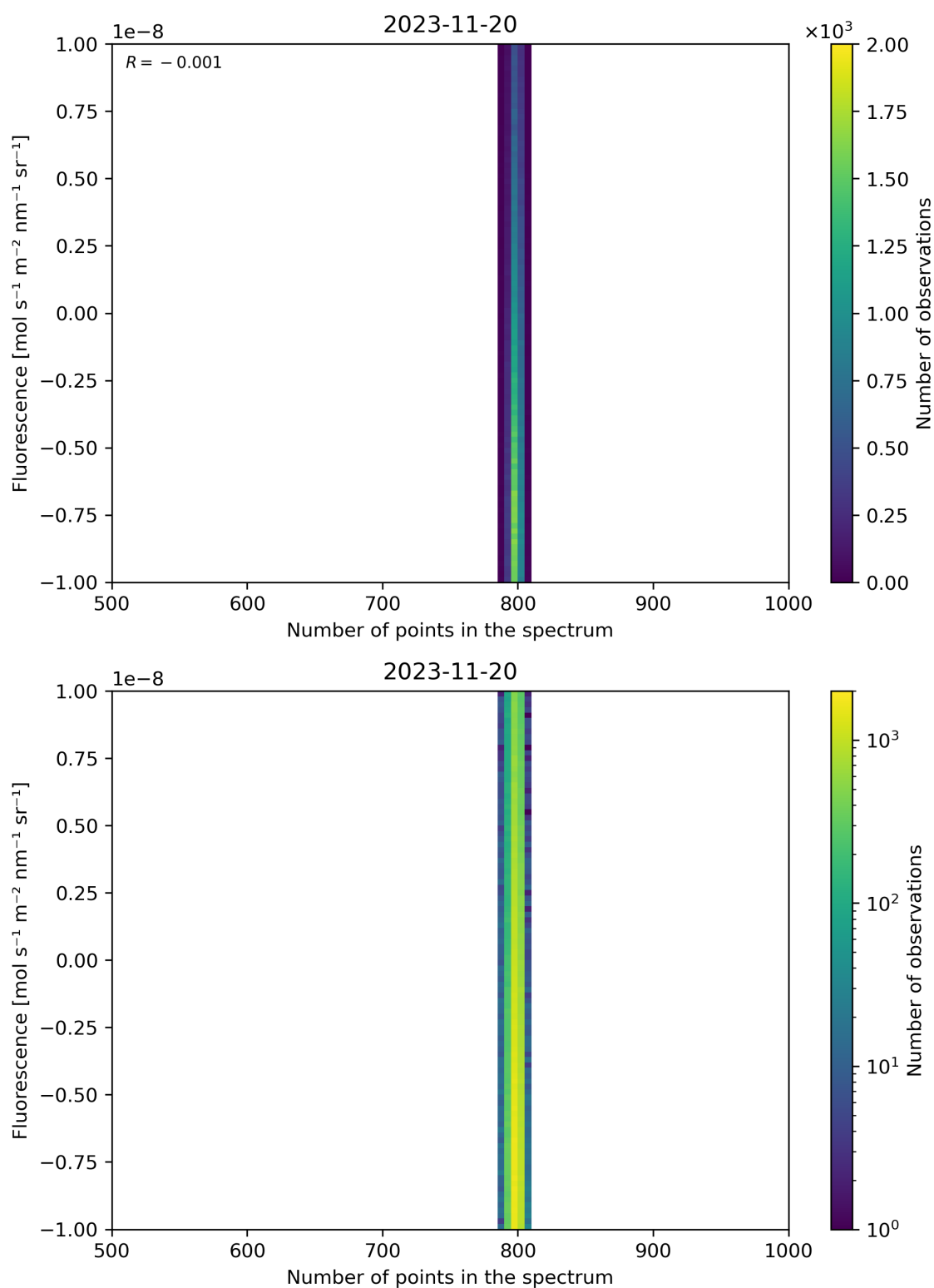
Figure 91: Scatter density plot of “Number of points in the spectrum” against “Fluorescence” for 2023-11-19 to 2023-11-21.
