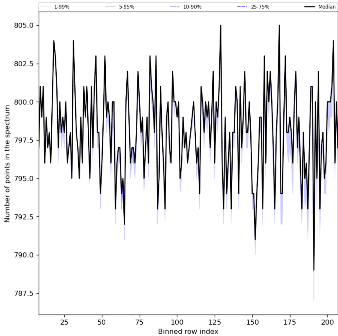
Figure 37: Along track statistics of “Number of points in the spectrum” for 2023-11-19 to 2023-11-21
