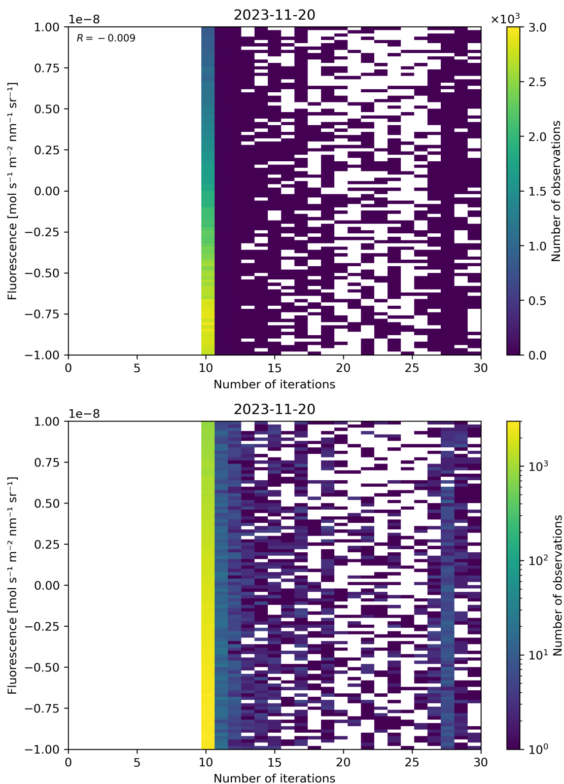
Figure 87: Scatter density plot of “Number of iterations” against “Fluorescence” for 2023-11-19 to 2023-11-21.
