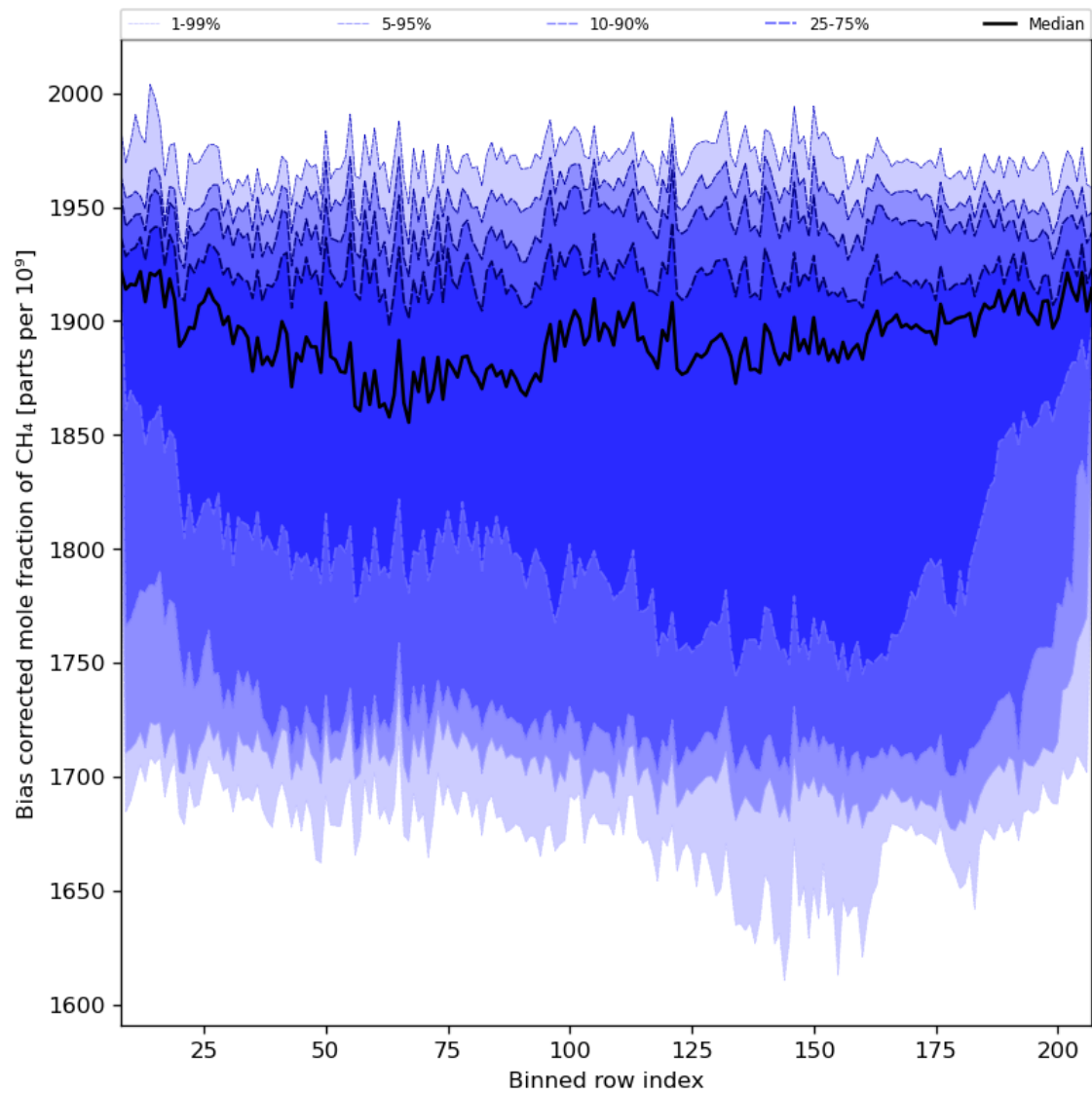
Figure 36: Along track statistics of “Bias corrected mole fraction of CH 4 ” for 2023-11-19 to 2023-11-21
