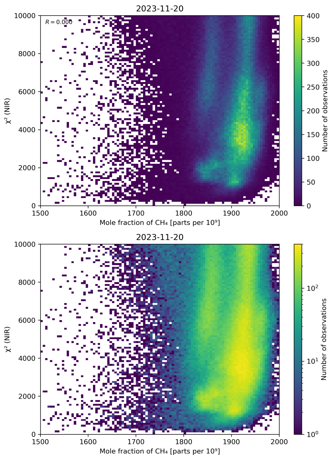
Figure 70: Scatter density plot of “Mole fraction of CH 4 ” against “ \chi^2 (NIR)” for 2023-11-19 to 2023-11-21.
