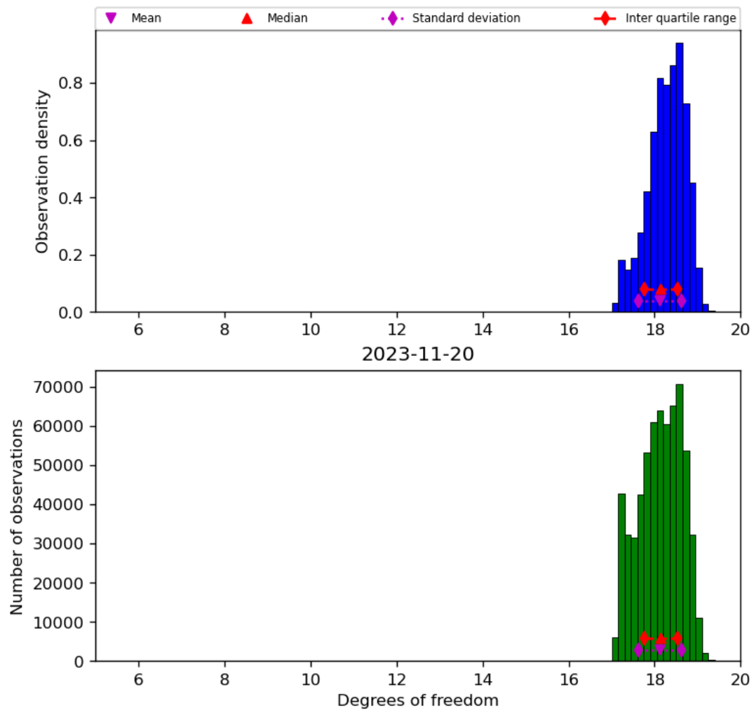
Figure 30: Histogram of “Degrees of freedom” for 2023-11-19 to 2023-11-21
