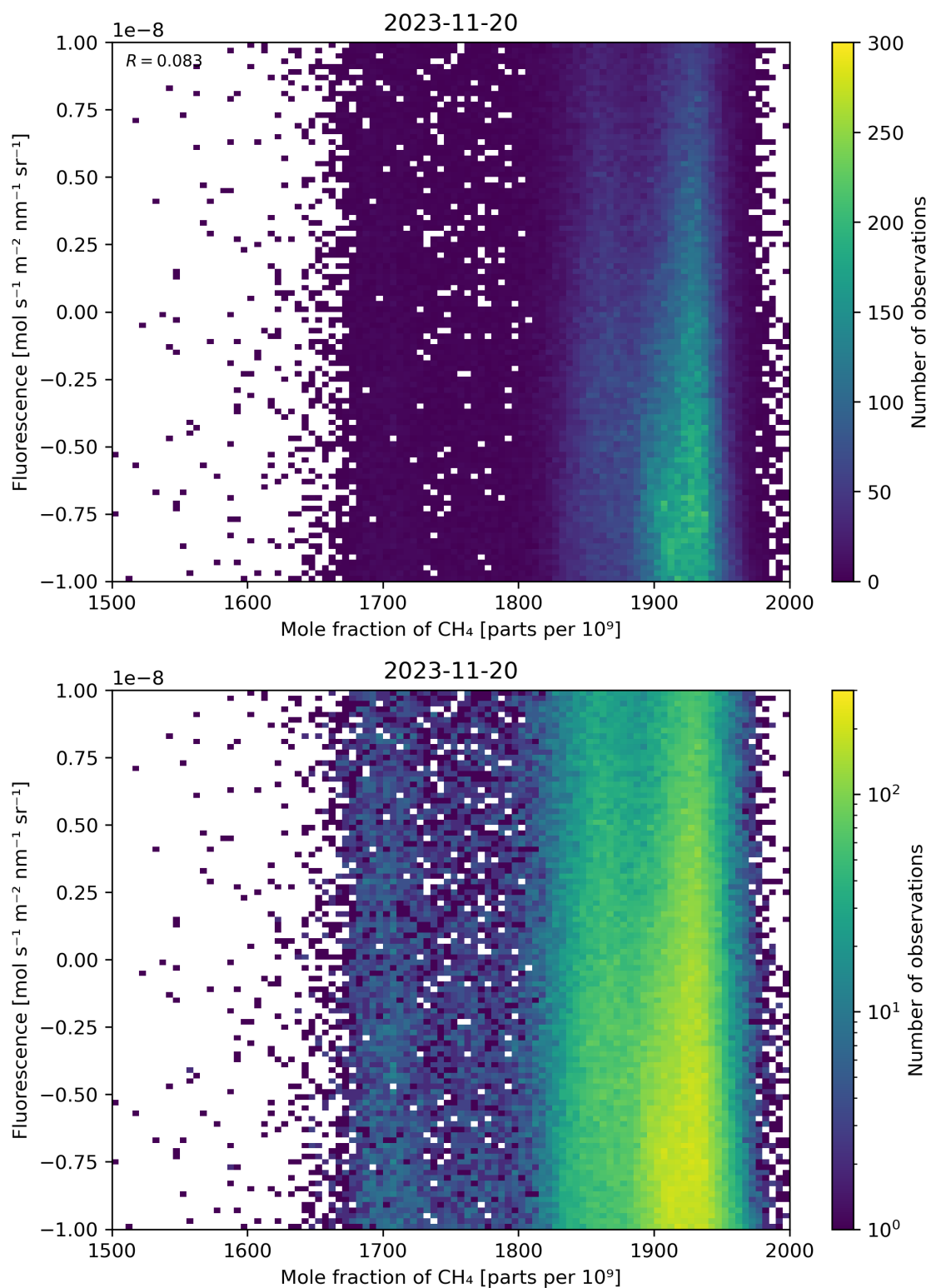
Figure 73: Scatter density plot of “Mole fraction of \text{CH}_4 ” against “Fluorescence” for 2023-11-19 to 2023-11-21.
