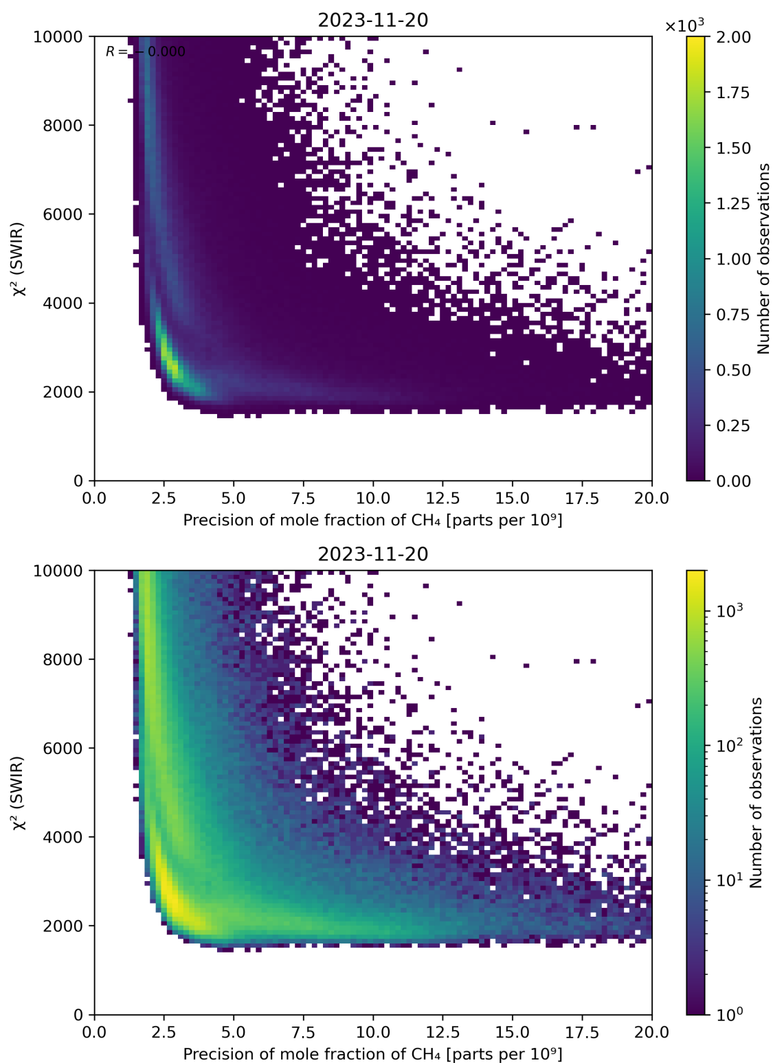
Figure 79: Scatter density plot of “Precision of mole fraction of CH 4 ” against “ \chi^2 (SWIR)” for 2023-11-19 to 2023-11-21.
