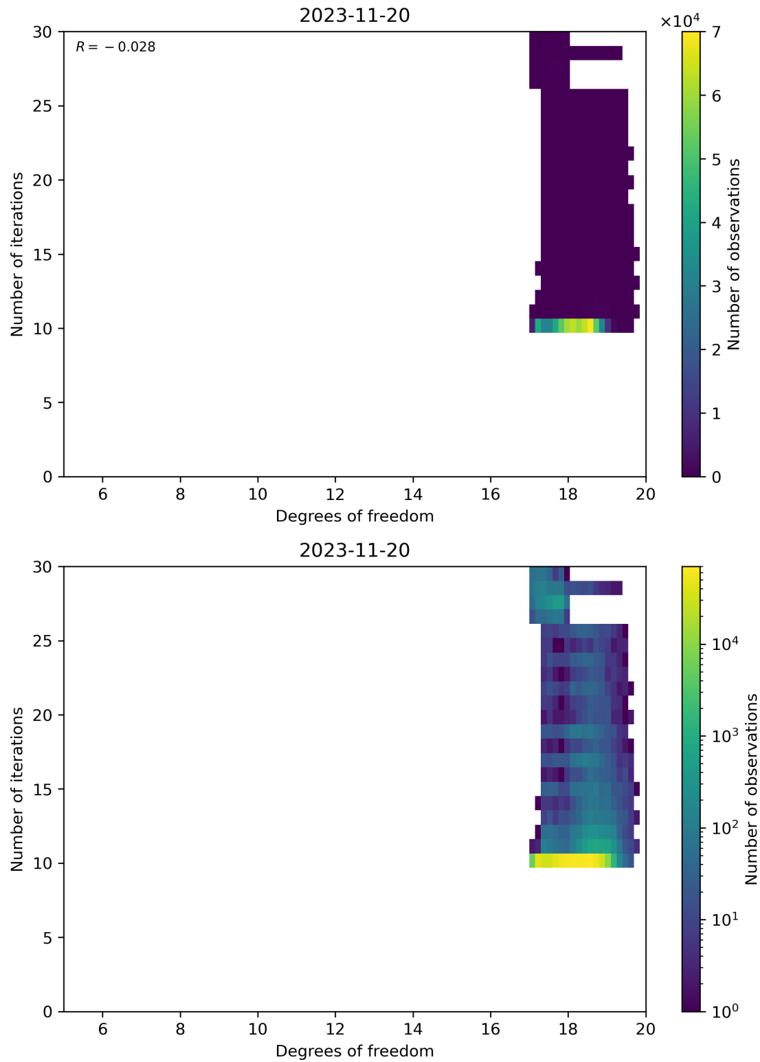
Figure 52: Scatter density plot of “Degrees of freedom” against “Number of iterations” for 2023-11-19 to 2023-11-21.
