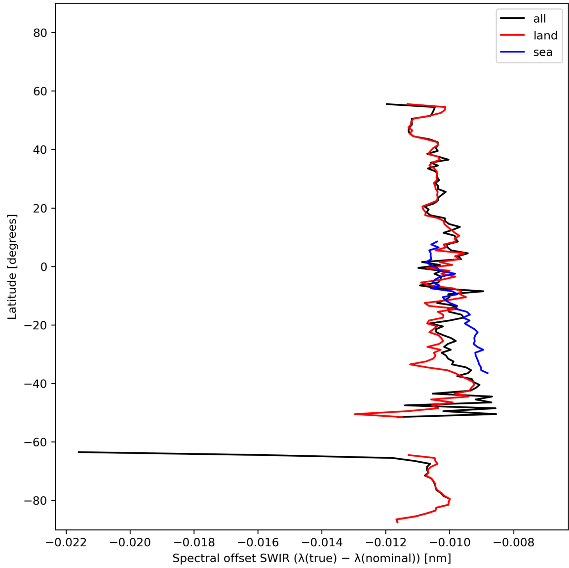
Figure 16: Zonal average of “Spectral offset SWIR ( \lambda(\text{true}) - \lambda(\text{nominal}) )” for 2023-11-19 to 2023-11-21.
