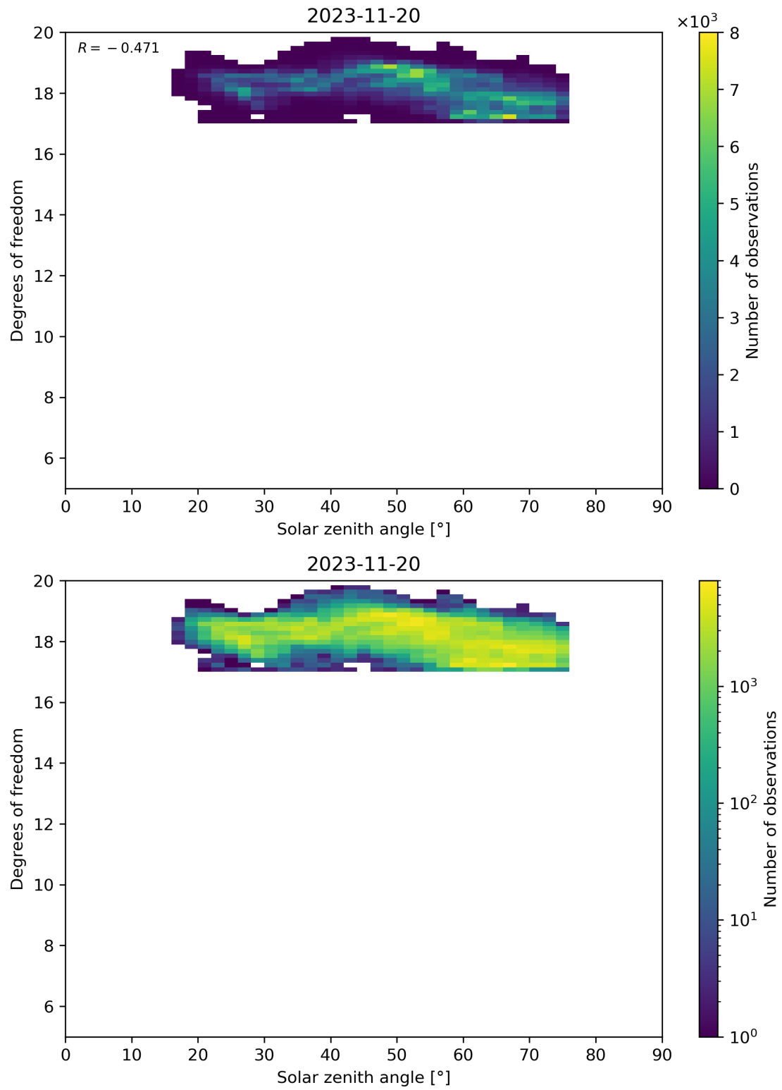
Figure 96: Scatter density plot of “Solar zenith angle” against “Degrees of freedom” for 2023-11-19 to 2023-11-21.
