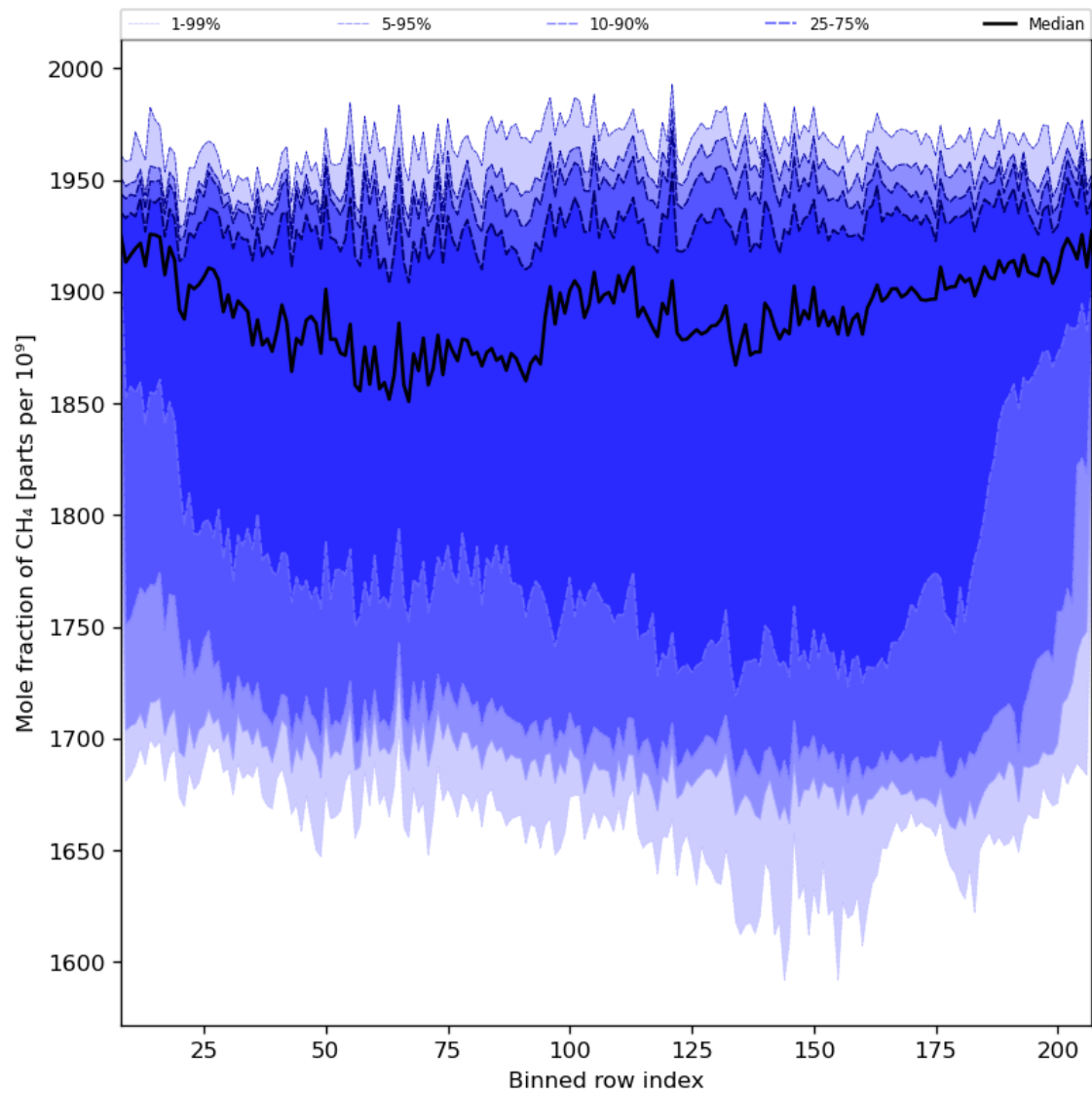
Figure 34: Along track statistics of “Mole fraction of CH 4 ” for 2023-11-19 to 2023-11-21
