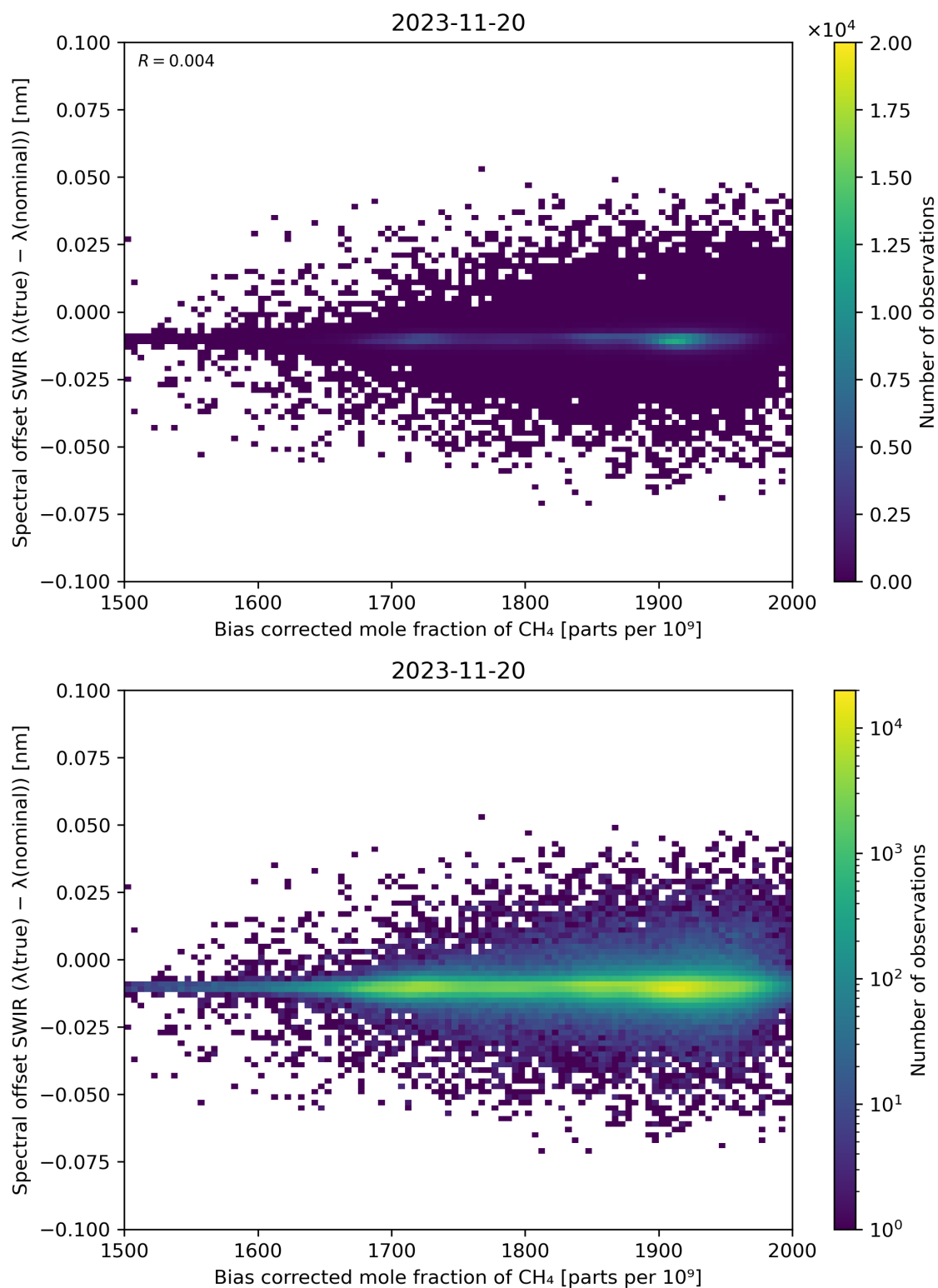
Figure 69: Scatter density plot of “Bias corrected mole fraction of \text{CH}_4 ” against “Spectral offset SWIR ( \lambda(\text{true}) - \lambda(\text{nominal}) )” for 2023-11-19 to 2023-11-21.
