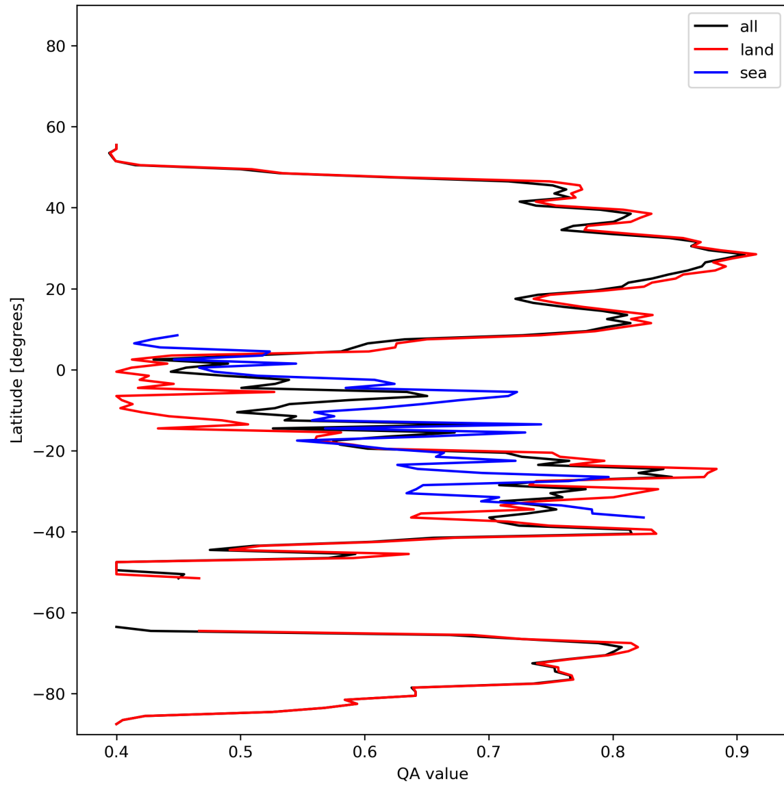
Figure 11: Zonal average of “QA value” for 2023-11-19 to 2023-11-21.
