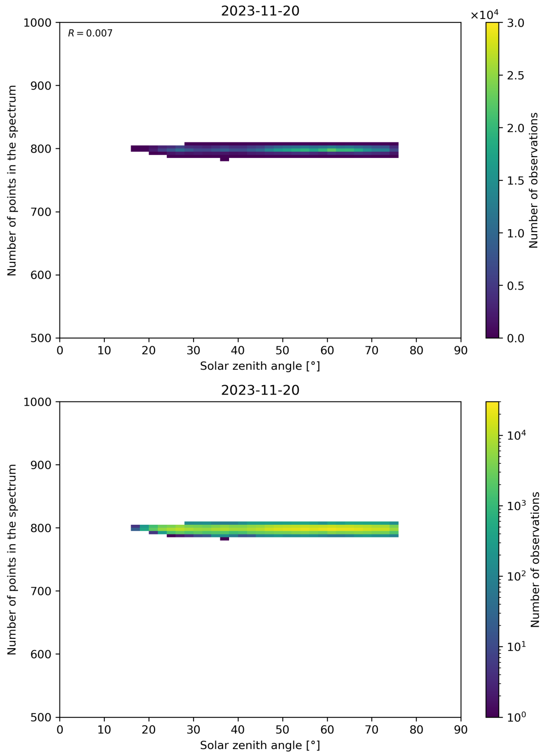
Figure 103: Scatter density plot of “Solar zenith angle” against “Number of points in the spectrum” for 2023-11-19 to 2023-11-21.
