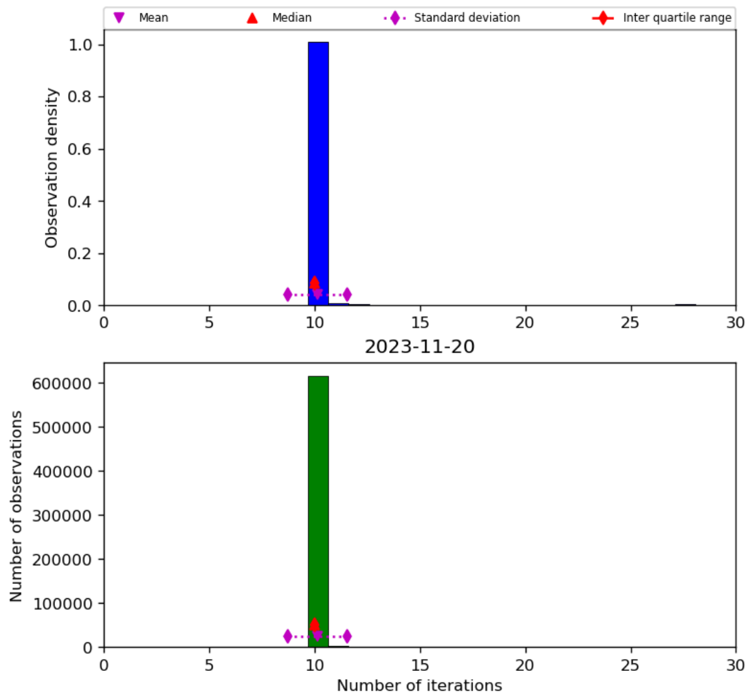
Figure 31: Histogram of “Number of iterations” for 2023-11-19 to 2023-11-21
