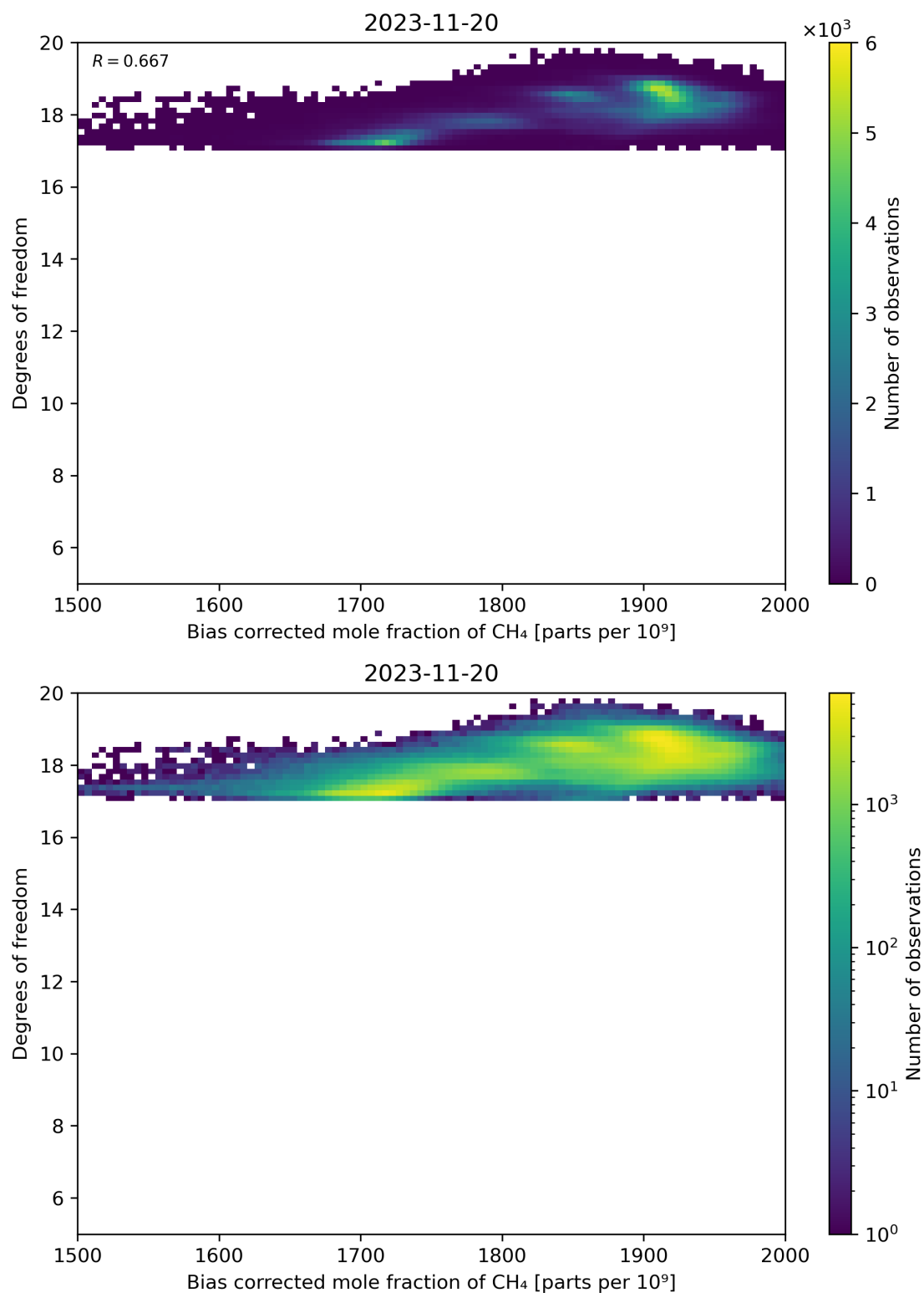
Figure 65: Scatter density plot of “Bias corrected mole fraction of CH 4 ” against “Degrees of freedom” for 2023-11-19 to 2023-11-21.
