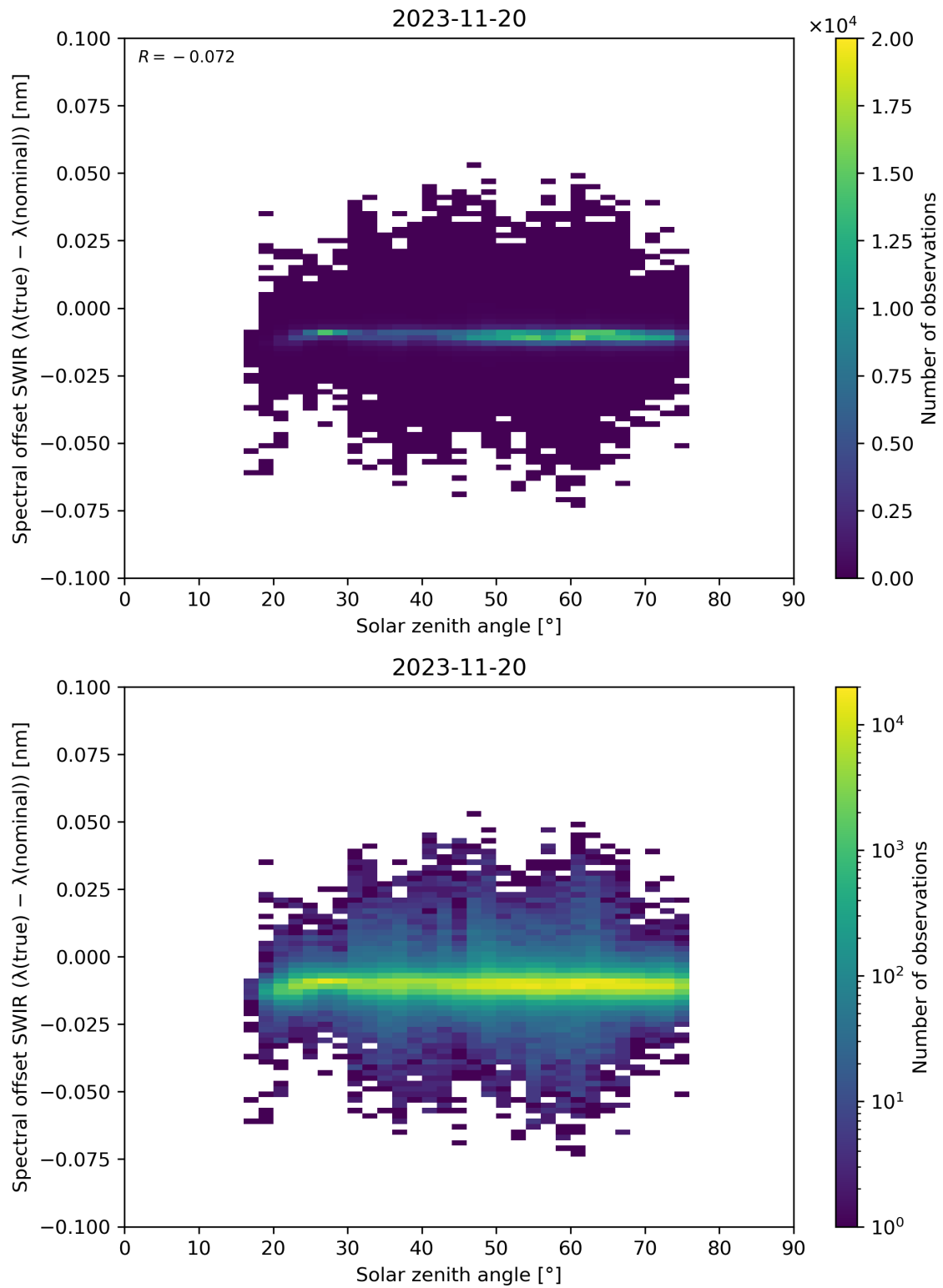
Figure 104: Scatter density plot of “Solar zenith angle” against “Spectral offset SWIR ( \lambda(\text{true}) - \lambda(\text{nominal}) )” for 2023-11-19 to 2023-11-21.
