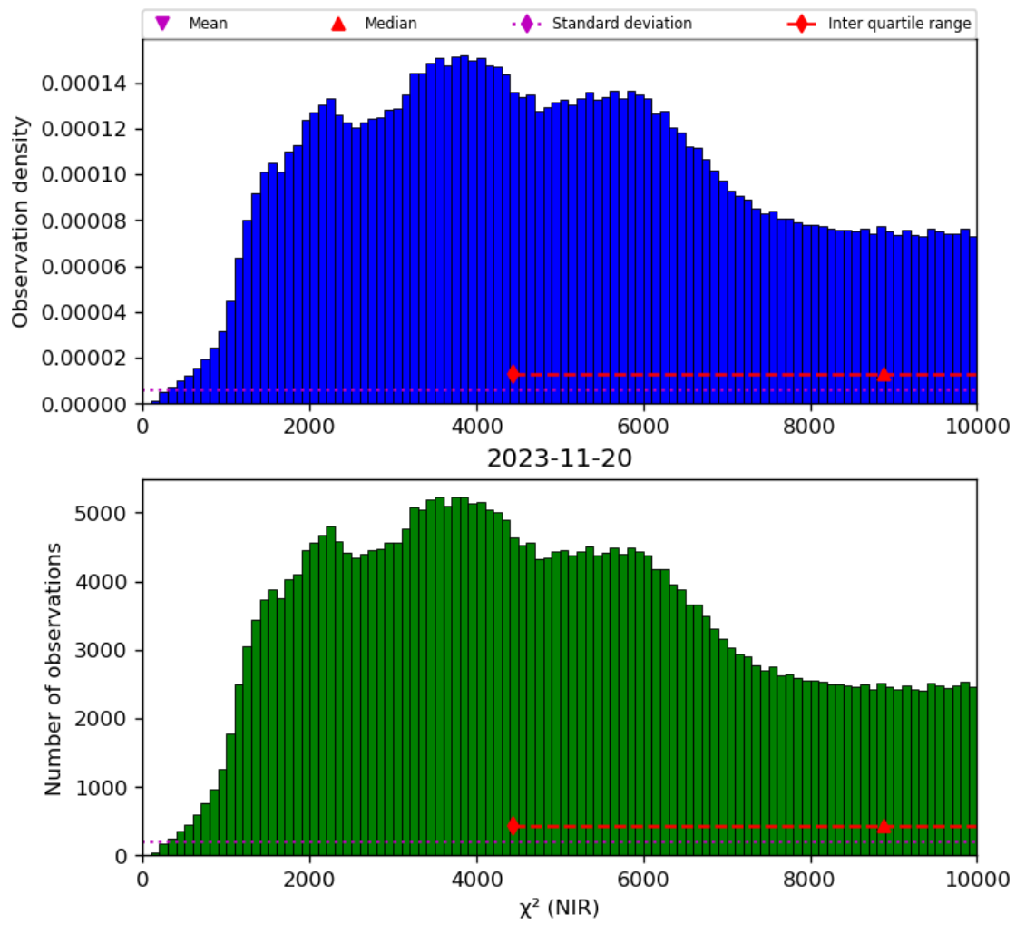
Figure 29: Histogram of “ \chi^2 (NIR)” for 2023-11-19 to 2023-11-21
