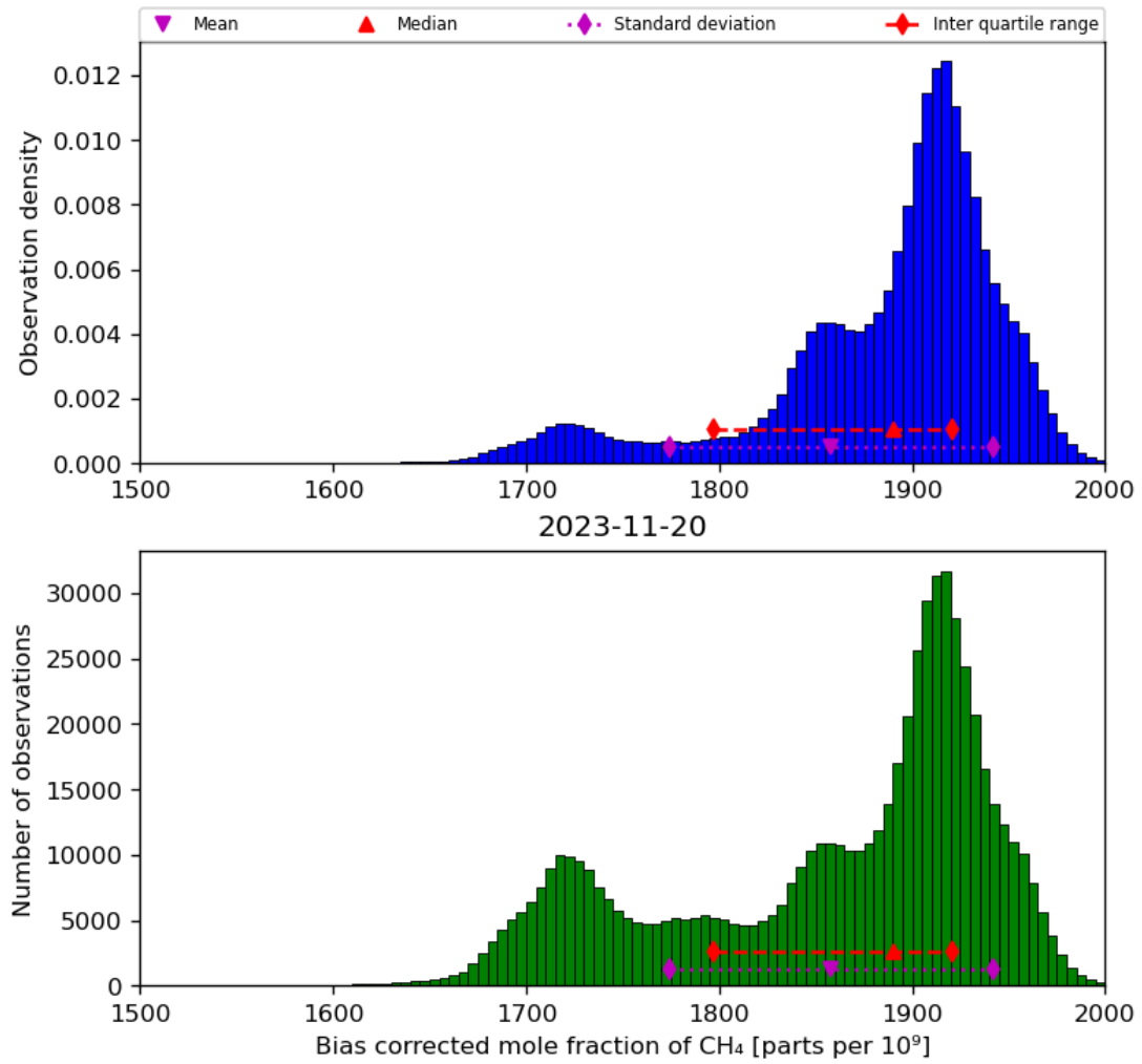
Figure 25: Histogram of “Bias corrected mole fraction of CH 4 ” for 2023-11-19 to 2023-11-21
