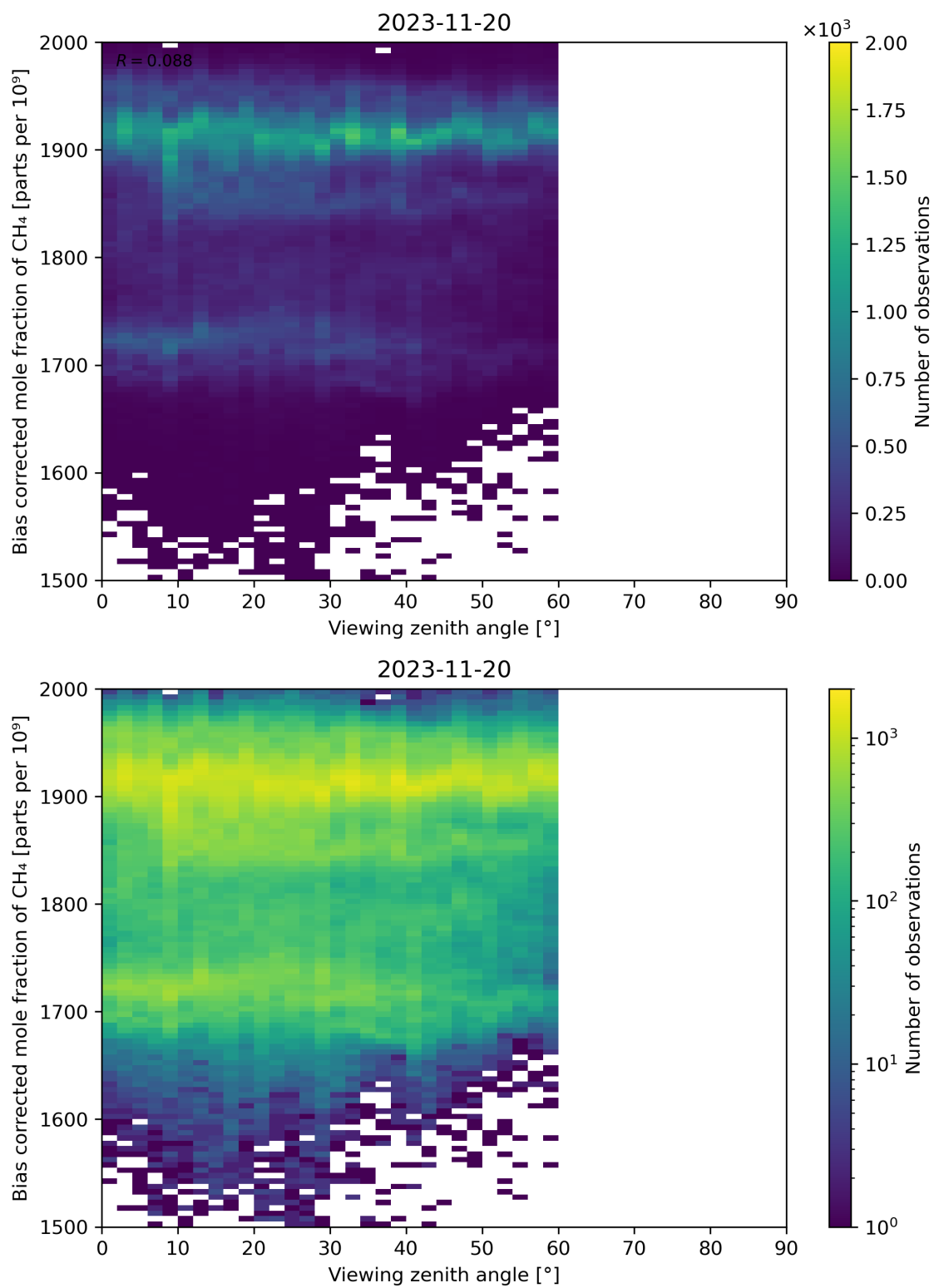
Figure 111: Scatter density plot of “Viewing zenith angle” against “Bias corrected mole fraction of CH 4 ” for 2023-11-19 to 2023-11-21.
