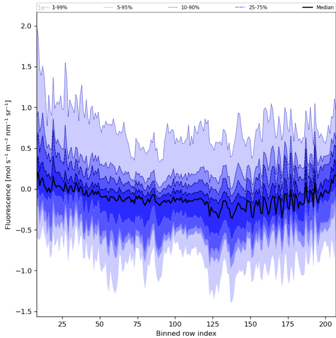
Figure 43: Along track statistics of “Fluorescence” for 2023-11-19 to 2023-11-21
