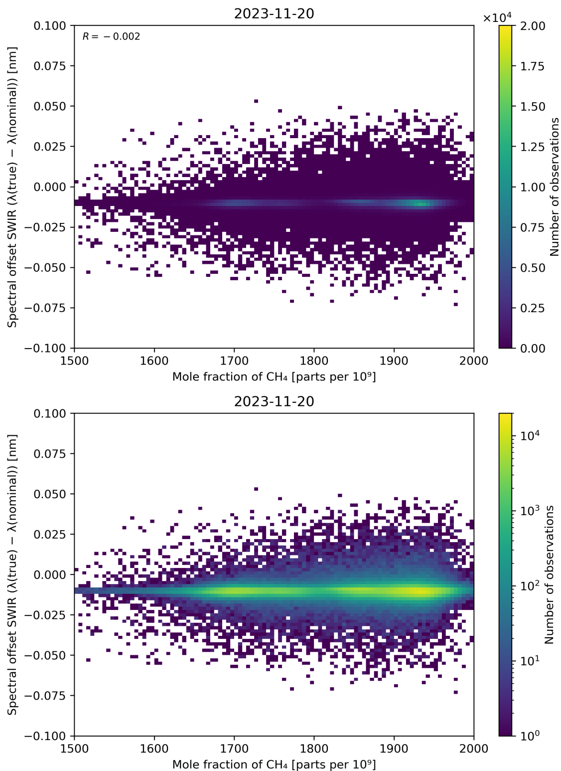
Figure 86: Scatter density plot of “Mole fraction of CH 4 ” against “Spectral offset SWIR ( \lambda(\text{true}) - \lambda(\text{nominal}) )” for 2023-11-19 to 2023-11-21.
