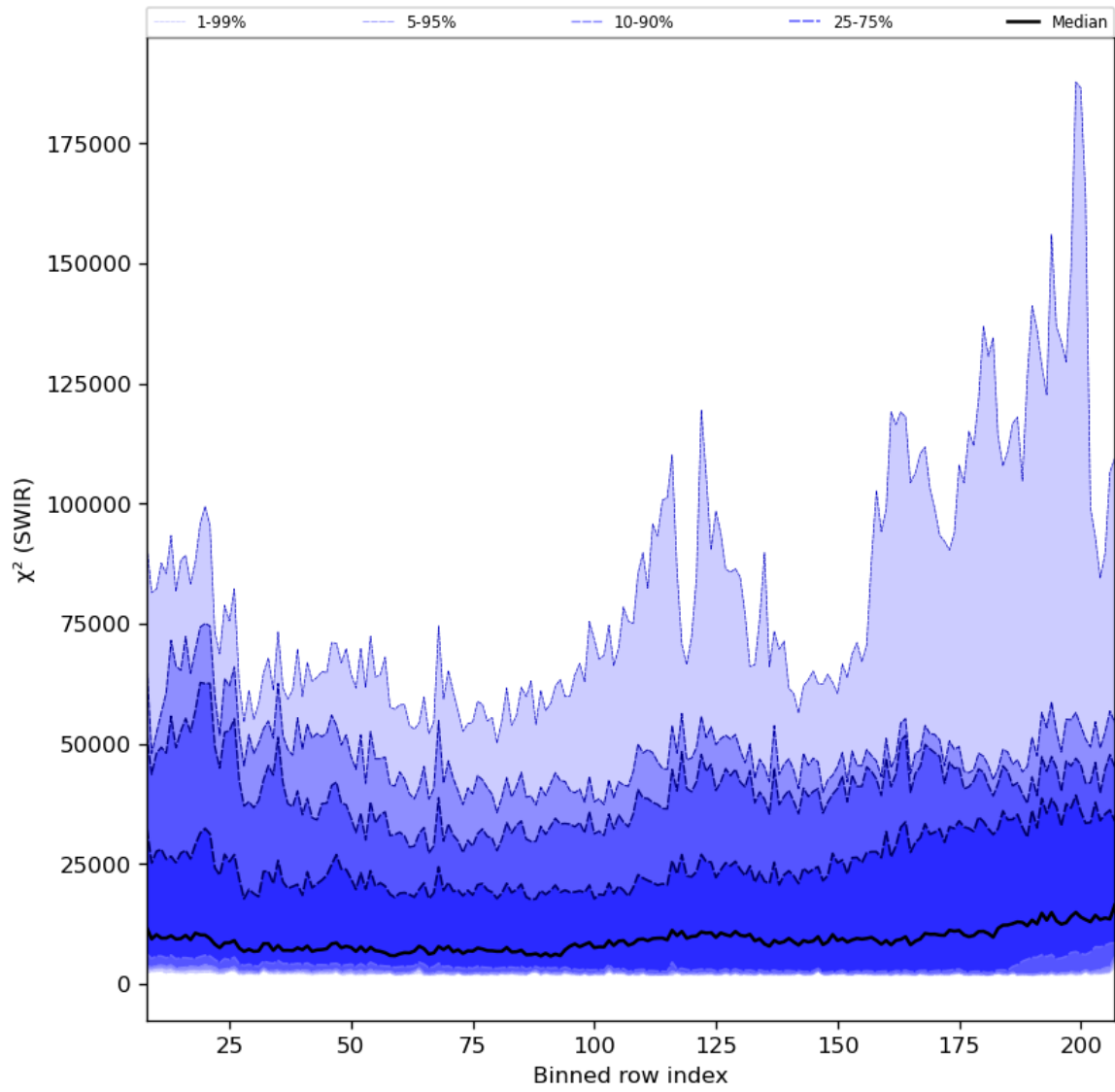
Figure 39: Along track statistics of “ \chi^2 (SWIR)” for 2023-11-19 to 2023-11-21
