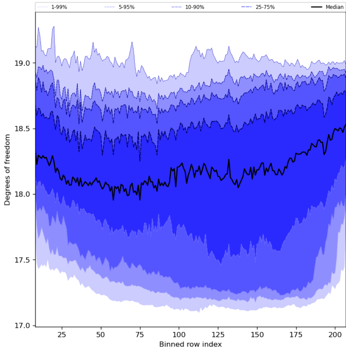
Figure 41: Along track statistics of “Degrees of freedom” for 2023-11-19 to 2023-11-21
