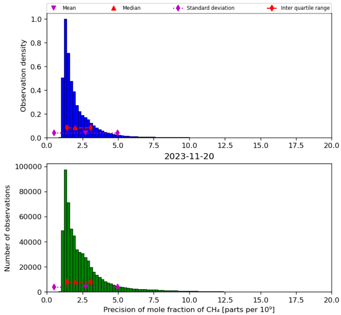
Figure 24: Histogram of “Precision of mole fraction of CH 4 ” for 2023-11-19 to 2023-11-21
