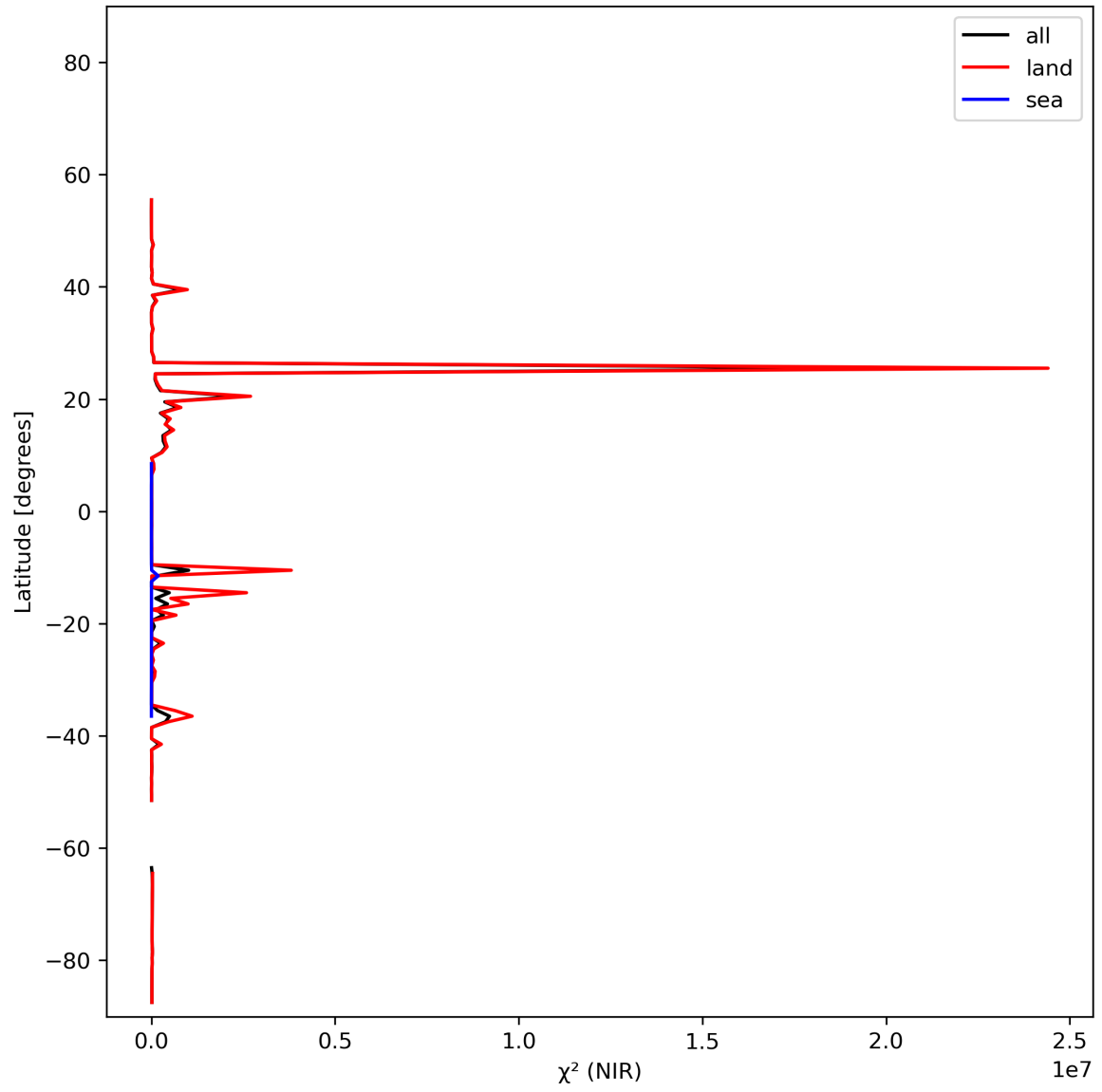
Figure 18: Zonal average of “ \chi^2 (NIR)” for 2023-11-19 to 2023-11-21.
