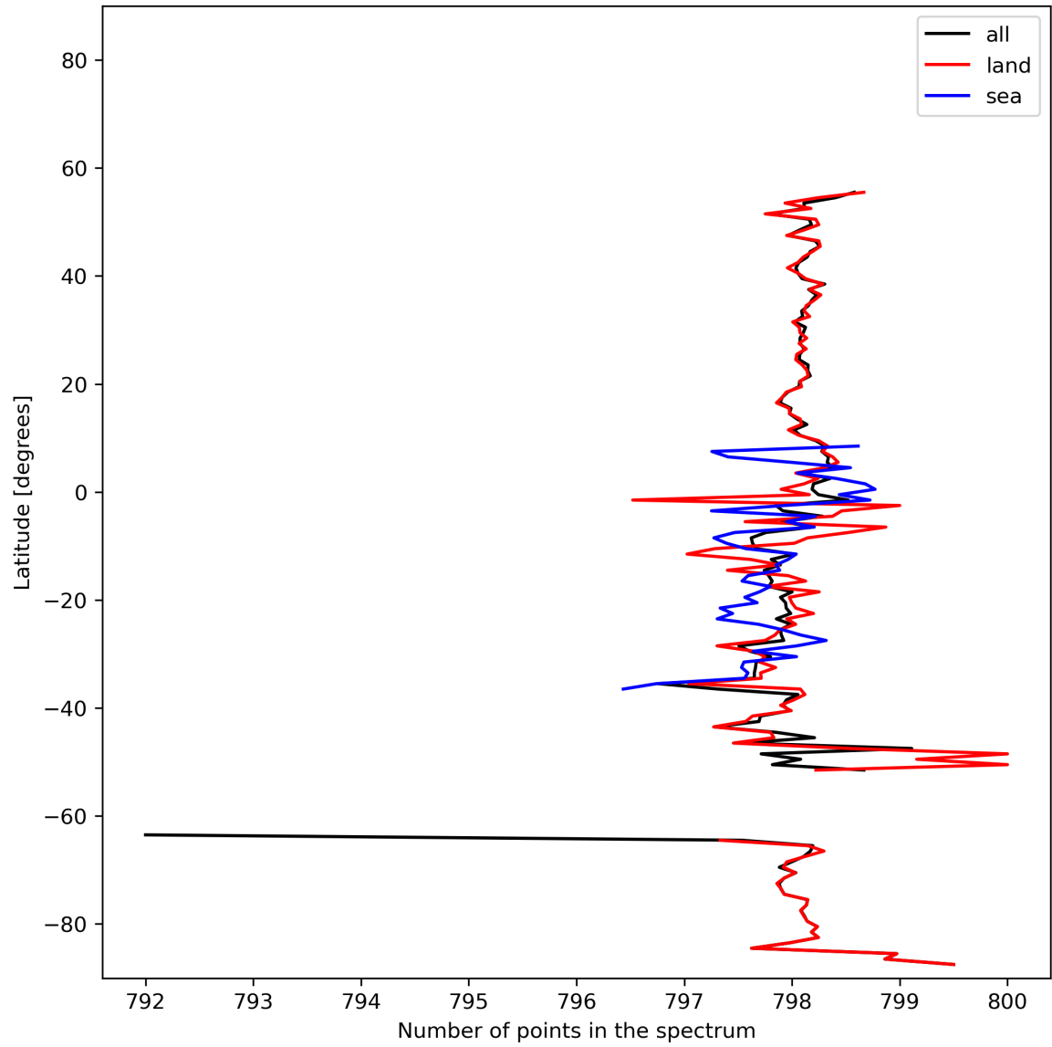
Figure 15: Zonal average of “Number of points in the spectrum” for 2023-11-19 to 2023-11-21.
