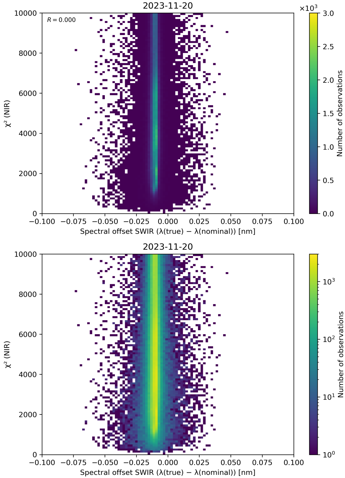
Figure 117: Scatter density plot of “Spectral offset SWIR ( \lambda(\text{true}) - \lambda(\text{nominal}) )” against “ \chi^2 (NIR)” for 2023-11-19 to 2023-11-21.
