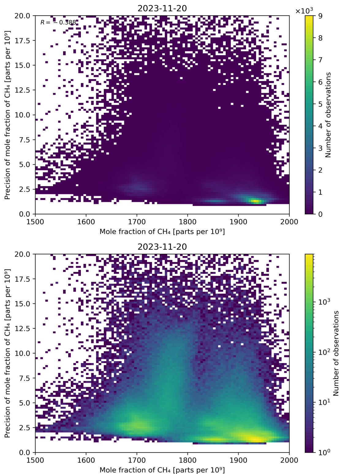
Figure 75: Scatter density plot of “Mole fraction of CH 4 ” against “Precision of mole fraction of CH 4 ” for 2023-11-19 to 2023-11-21.
