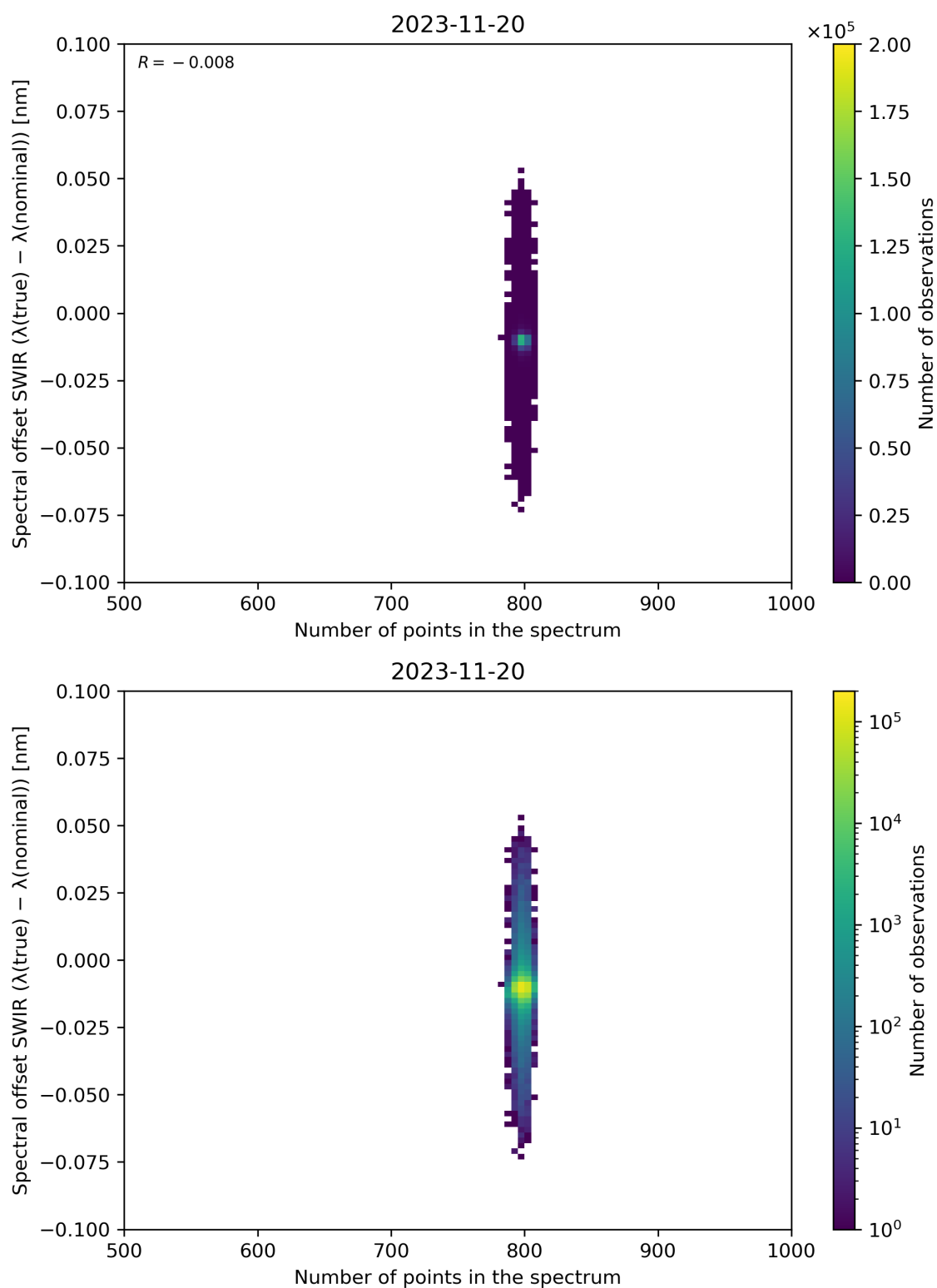
Figure 93: Scatter density plot of “Number of points in the spectrum” against “Spectral offset SWIR ( \lambda(\text{true}) - \lambda(\text{nominal}) )” for 2023-11-19 to 2023-11-21.
