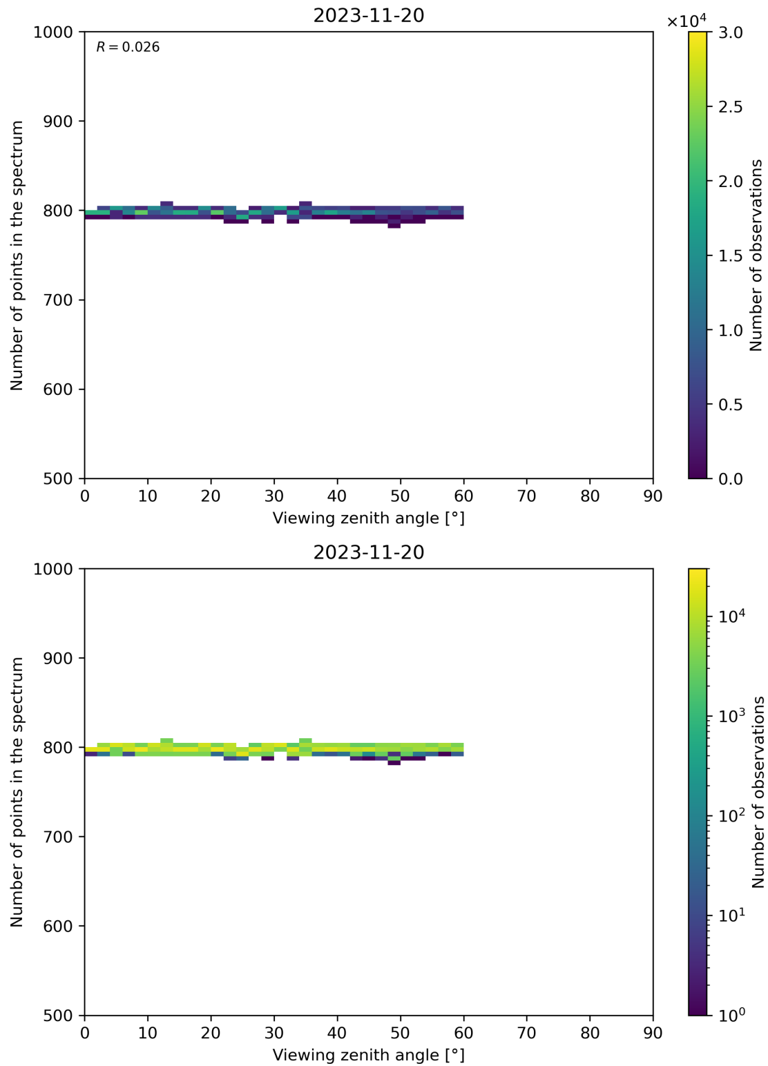
Figure 114: Scatter density plot of “Viewing zenith angle” against “Number of points in the spectrum” for 2023-11-19 to 2023-11-21.
