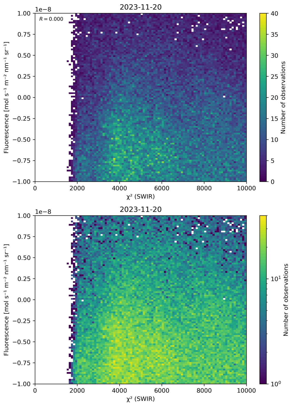
Figure 49: Scatter density plot of “ \chi^2 (SWIR)” against “Fluorescence” for 2023-11-19 to 2023-11-21.
