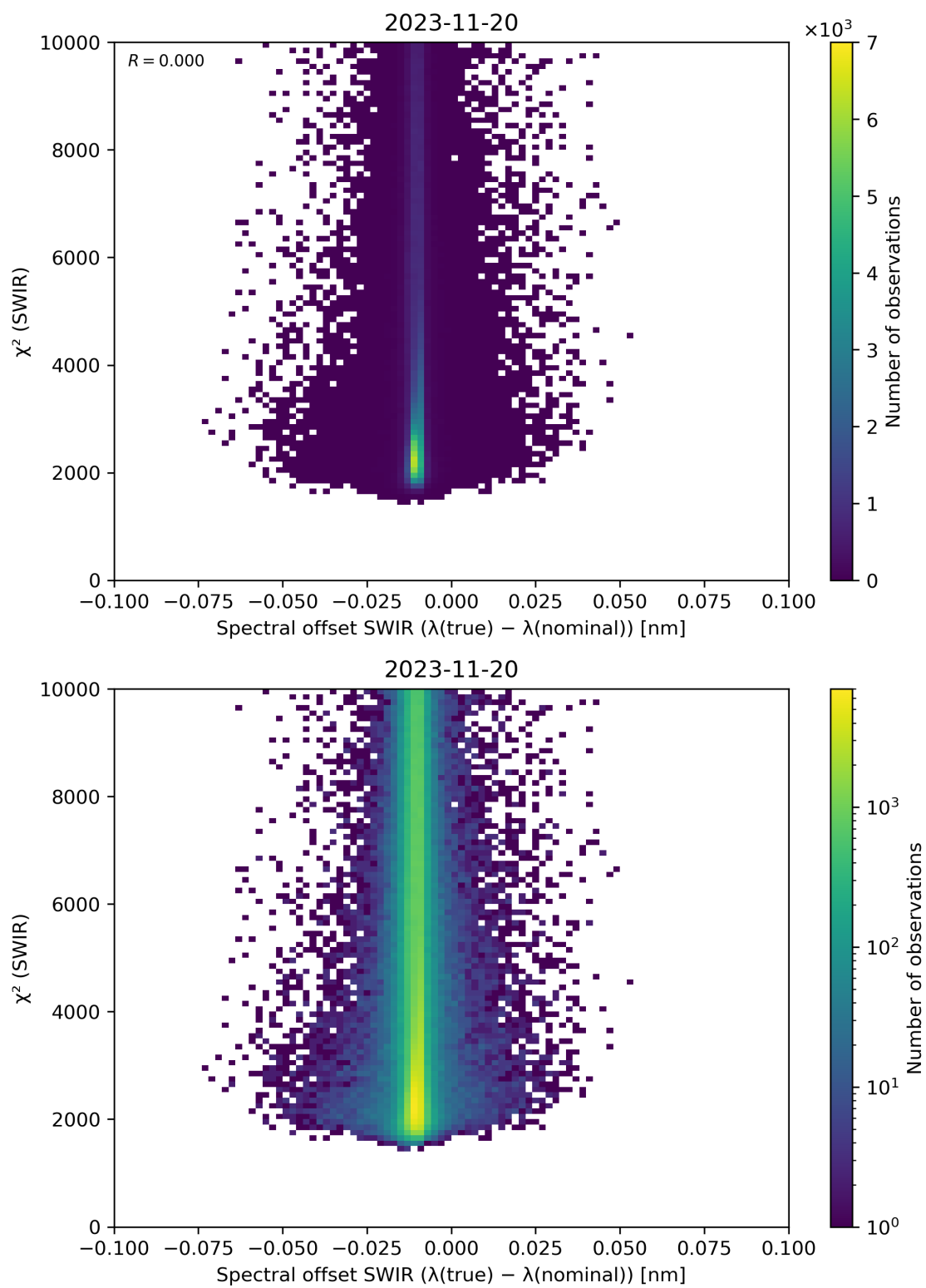
Figure 118: Scatter density plot of “Spectral offset SWIR ( \lambda(\text{true}) - \lambda(\text{nominal}) )” against “ \chi^2 (SWIR)” for 2023-11-19 to 2023-11-21.
