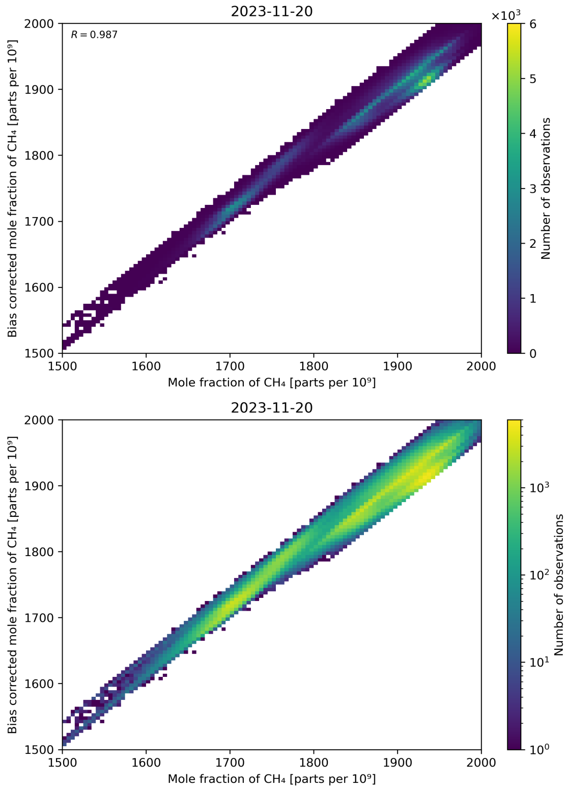
Figure 74: Scatter density plot of “Mole fraction of CH 4 ” against “Bias corrected mole fraction of CH 4 ” for 2023-11-19 to 2023-11-21.
