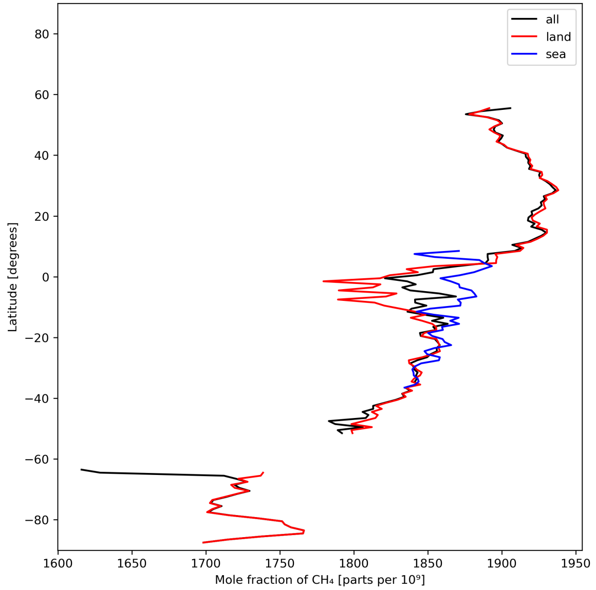
Figure 12: Zonal average of “Mole fraction of CH 4 ” for 2023-11-19 to 2023-11-21.
