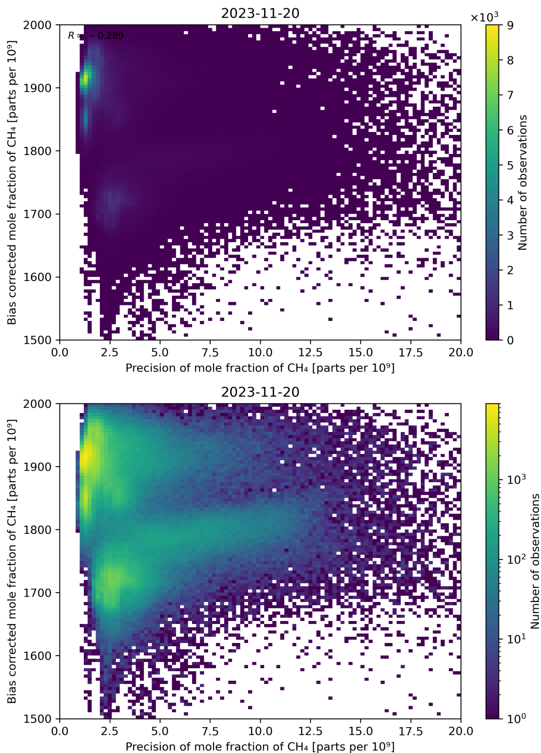
Figure 82: Scatter density plot of “Precision of mole fraction of CH 4 ” against “Bias corrected mole fraction of CH 4 ” for 2023-11-19 to 2023-11-21.
