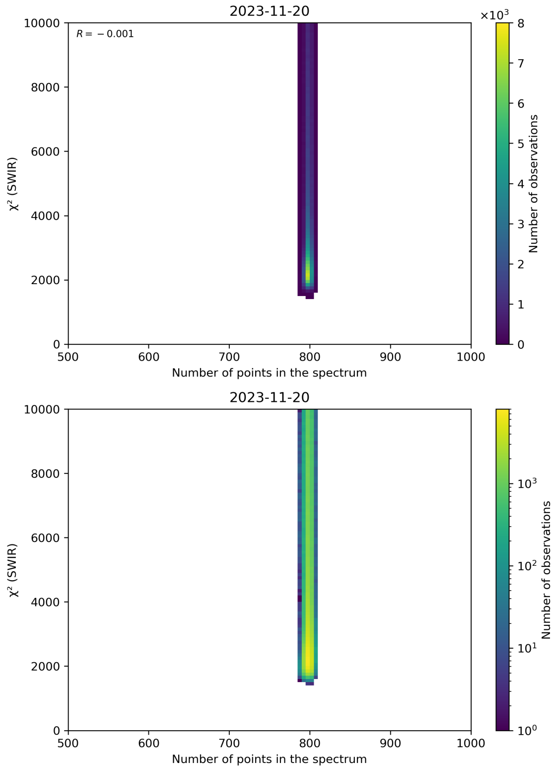
Figure 89: Scatter density plot of “Number of points in the spectrum” against “ \chi^2 (SWIR)” for 2023-11-19 to 2023-11-21.
