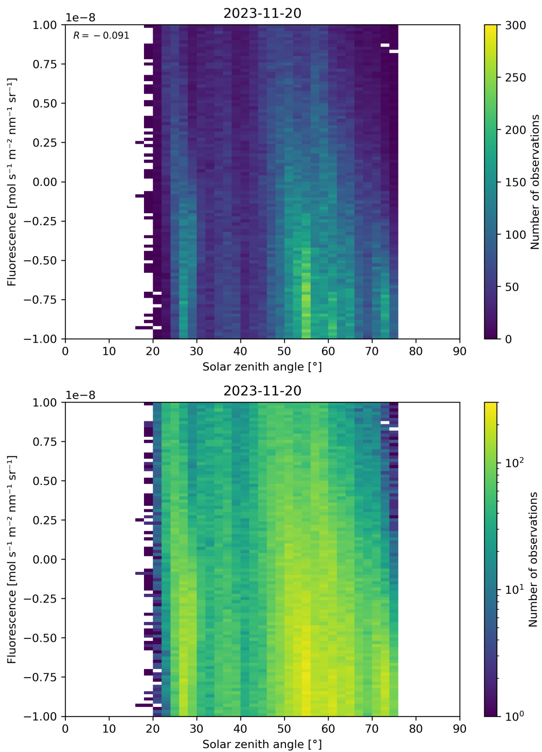
Figure 97: Scatter density plot of “Solar zenith angle” against “Fluorescence” for 2023-11-19 to 2023-11-21.
