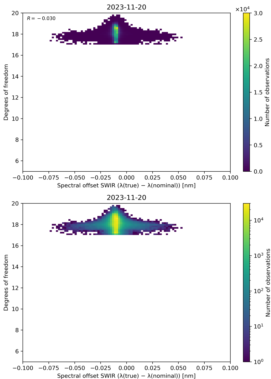
Figure 119: Scatter density plot of “Spectral offset SWIR ( \lambda(\text{true}) - \lambda(\text{nominal}) )” against “Degrees of freedom” for 2023-11-19 to 2023-11-21.
