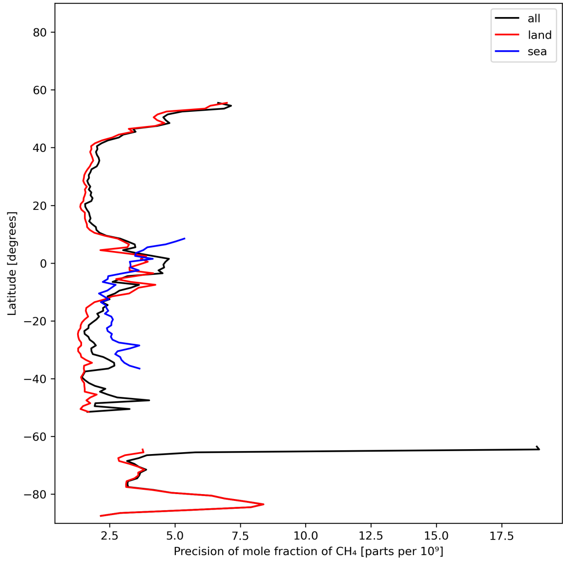
Figure 13: Zonal average of “Precision of mole fraction of CH 4 ” for 2023-11-19 to 2023-11-21.
