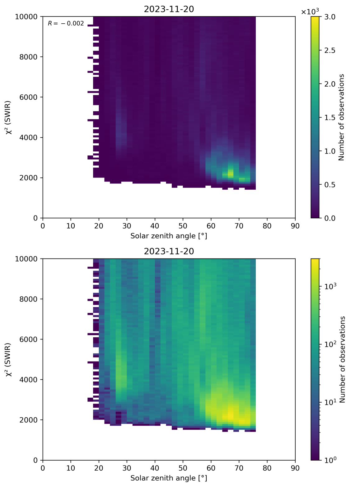
Figure 95: Scatter density plot of “Solar zenith angle” against “ \chi^2 (SWIR)” for 2023-11-19 to 2023-11-21.
