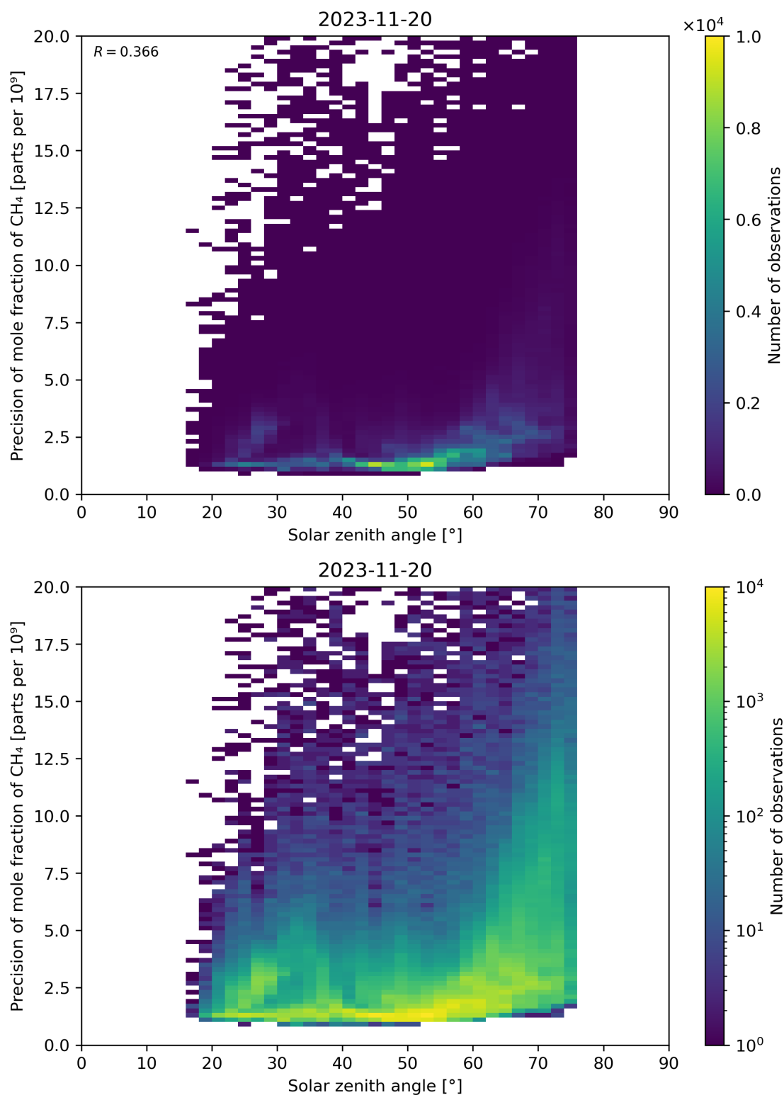
Figure 101: Scatter density plot of “Solar zenith angle” against “Precision of mole fraction of \text{CH}_4 ” for 2023-11-19 to 2023-11-21.
