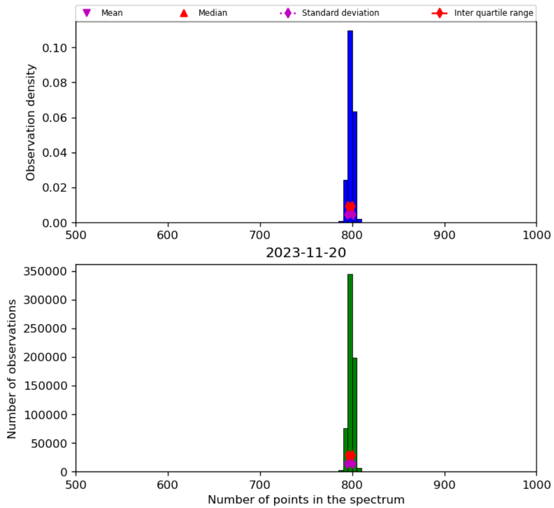
Figure 26: Histogram of “Number of points in the spectrum” for 2023-11-19 to 2023-11-21
