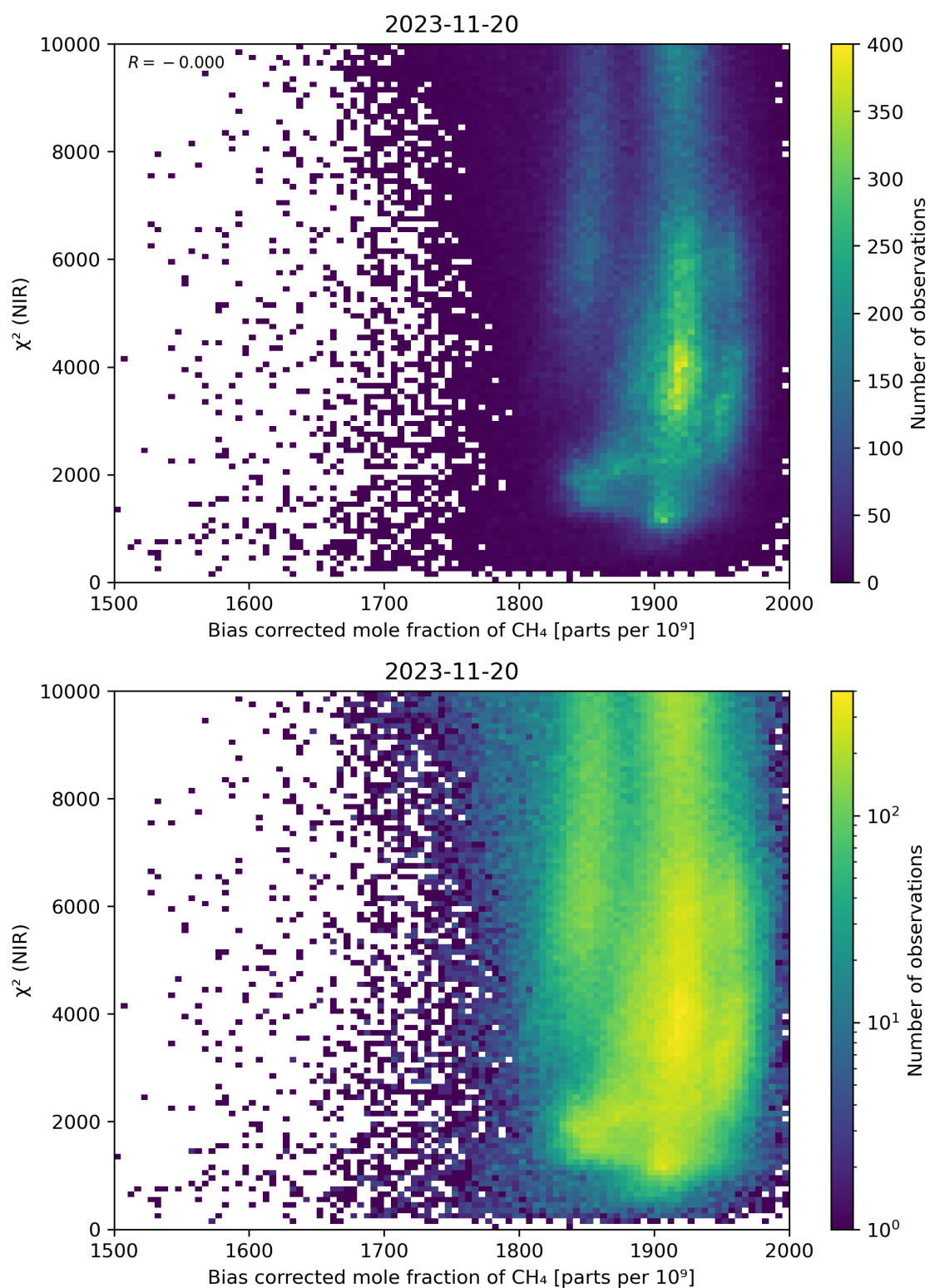
Figure 63: Scatter density plot of “Bias corrected mole fraction of CH 4 ” against “ \chi^2 (NIR)” for 2023-11-19 to 2023-11-21.
