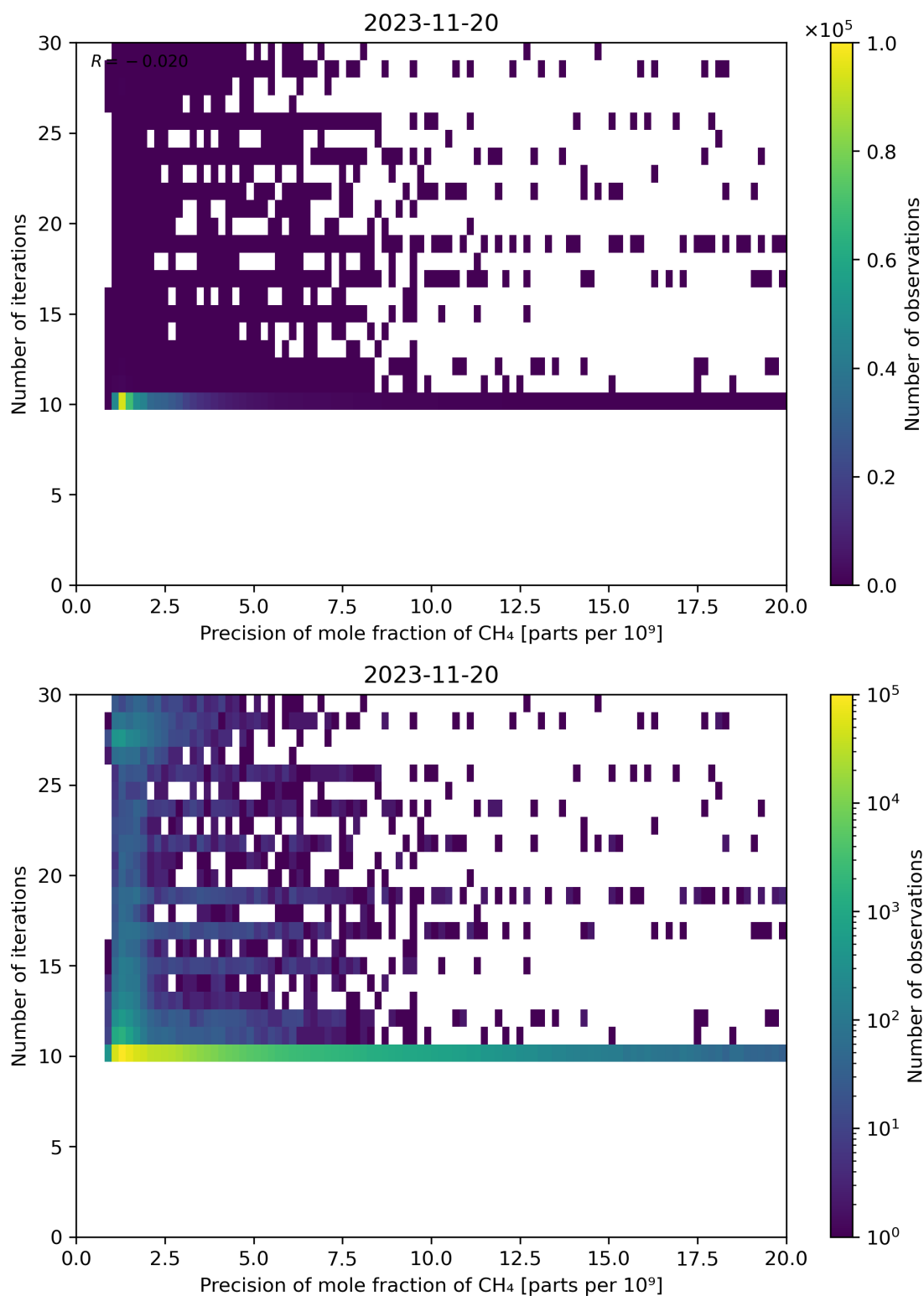
Figure 83: Scatter density plot of “Precision of mole fraction of CH 4 ” against “Number of iterations” for 2023-11-19 to 2023-11-21.
