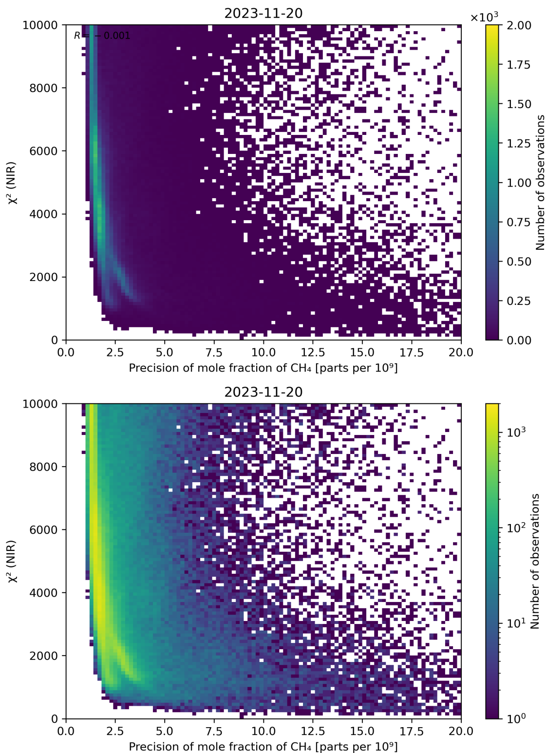
Figure 78: Scatter density plot of “Precision of mole fraction of CH 4 ” against “ \chi^2 (NIR)” for 2023-11-19 to 2023-11-21.
