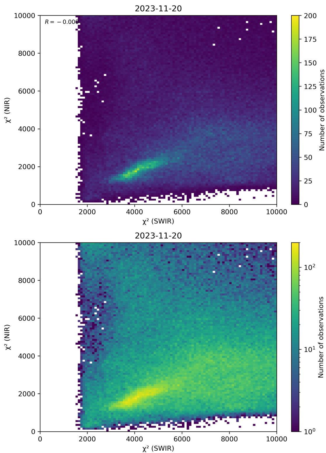
Figure 47: Scatter density plot of “ \chi^2 (SWIR)” against “ \chi^2 (NIR)” for 2023-11-19 to 2023-11-21.
