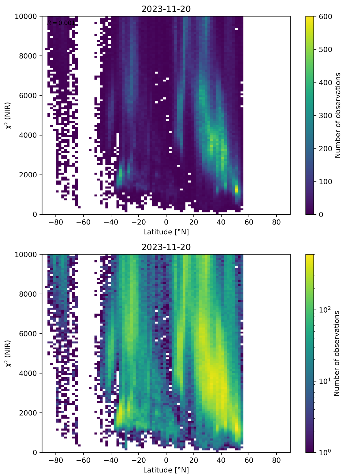
Figure 53: Scatter density plot of “Latitude” against “ \chi^2 (NIR)” for 2023-11-19 to 2023-11-21.
