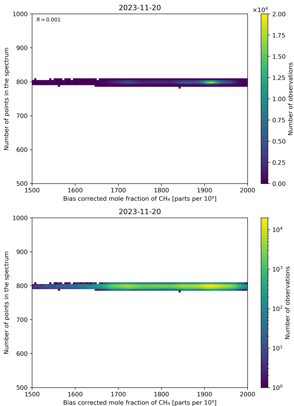
Figure 68: Scatter density plot of “Bias corrected mole fraction of CH 4 ” against “Number of points in the spectrum” for 2023-11-19 to 2023-11-21.
