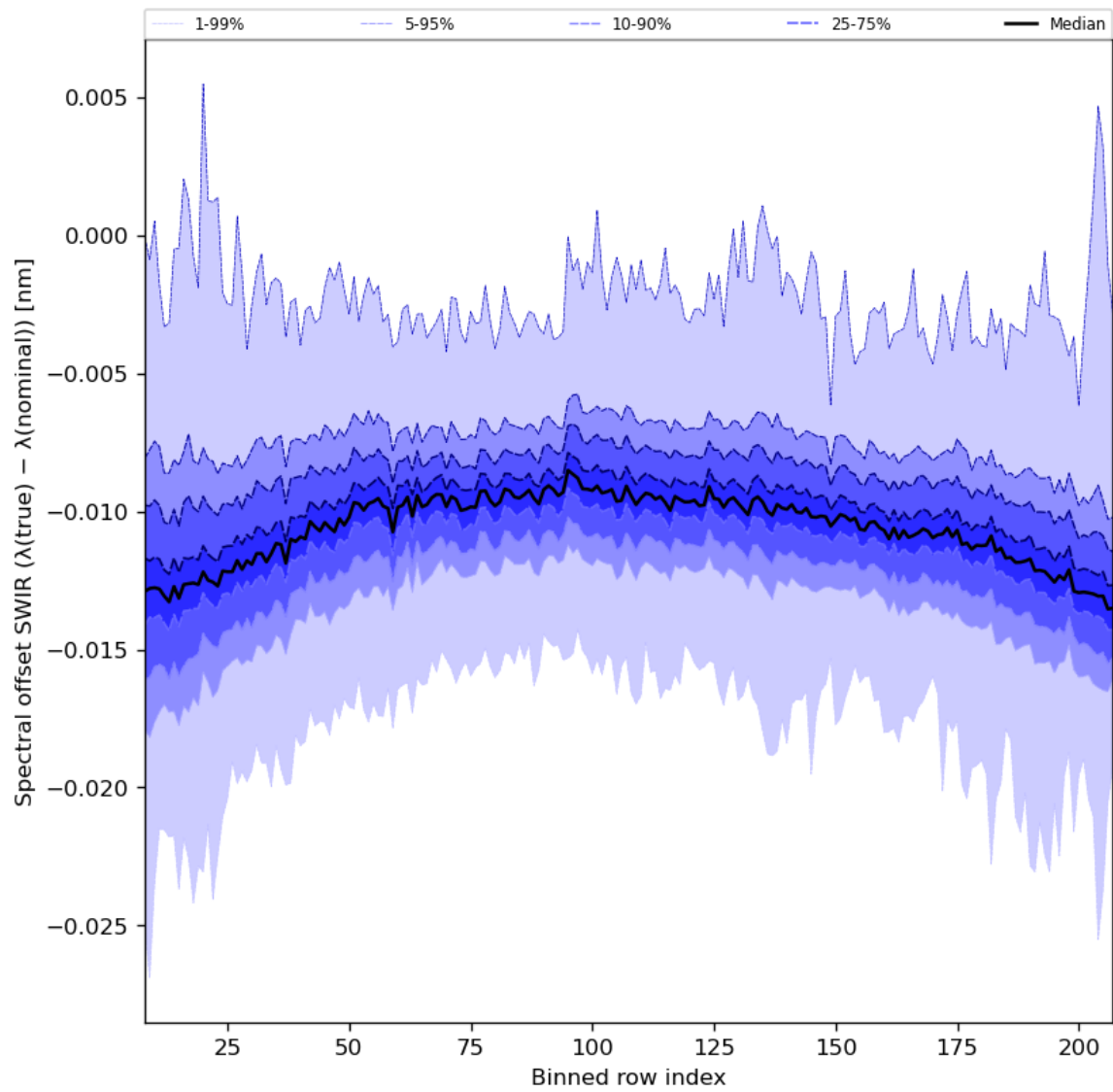
Figure 38: Along track statistics of “Spectral offset SWIR ( \lambda(\text{true}) - \lambda(\text{nominal}) )” for 2023-11-19 to 2023-11-21
