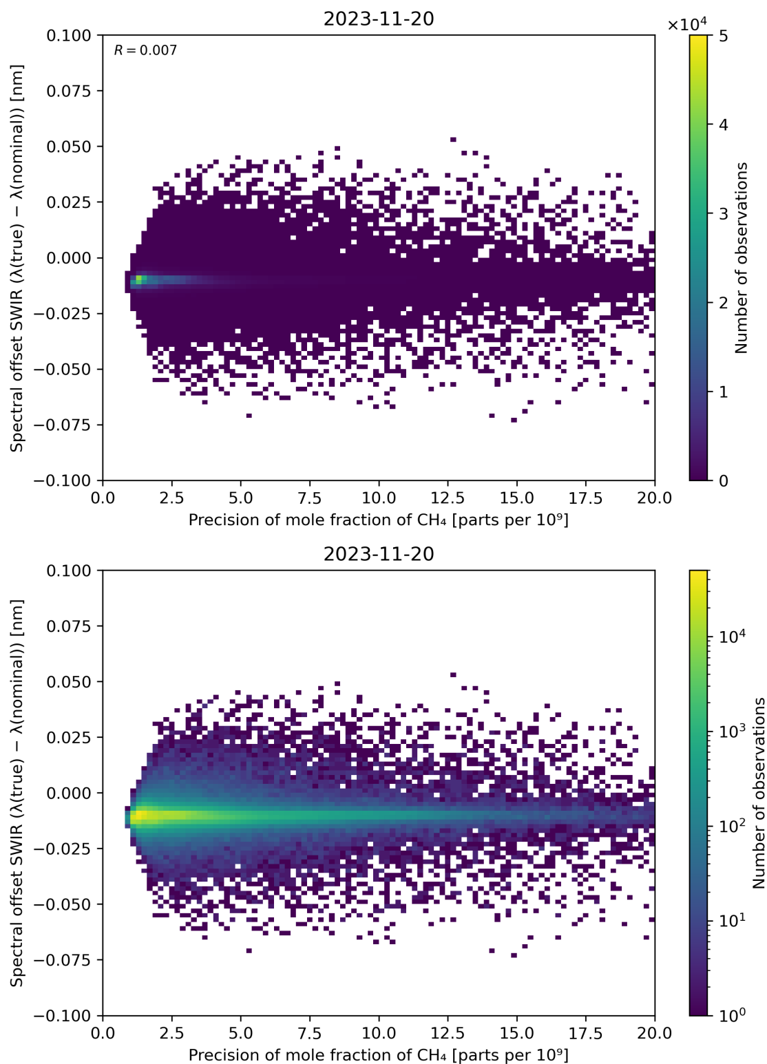
Figure 85: Scatter density plot of “Precision of mole fraction of CH 4 ” against “Spectral offset SWIR ( \lambda(\text{true}) - \lambda(\text{nominal}) )” for 2023-11-19 to 2023-11-21.
