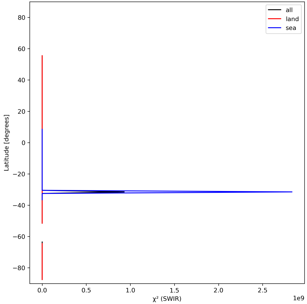
Figure 17: Zonal average of “ \chi^2 (SWIR)” for 2023-11-19 to 2023-11-21.
