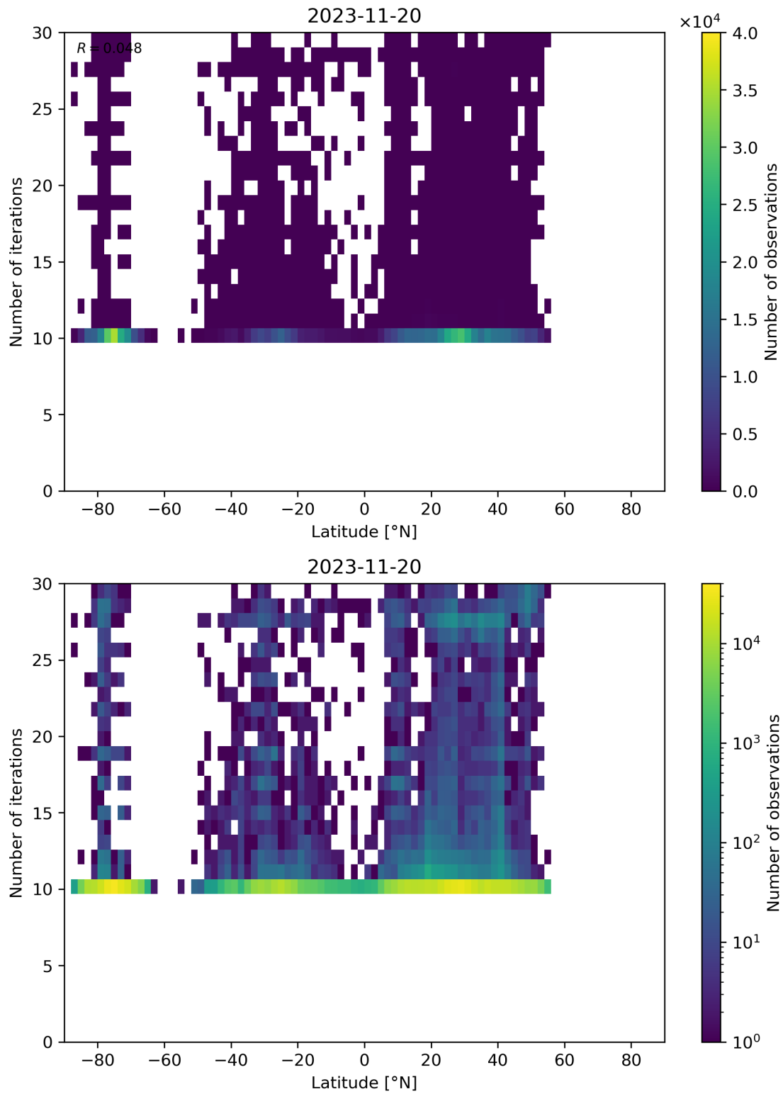
Figure 60: Scatter density plot of “Latitude” against “Number of iterations” for 2023-11-19 to 2023-11-21.
