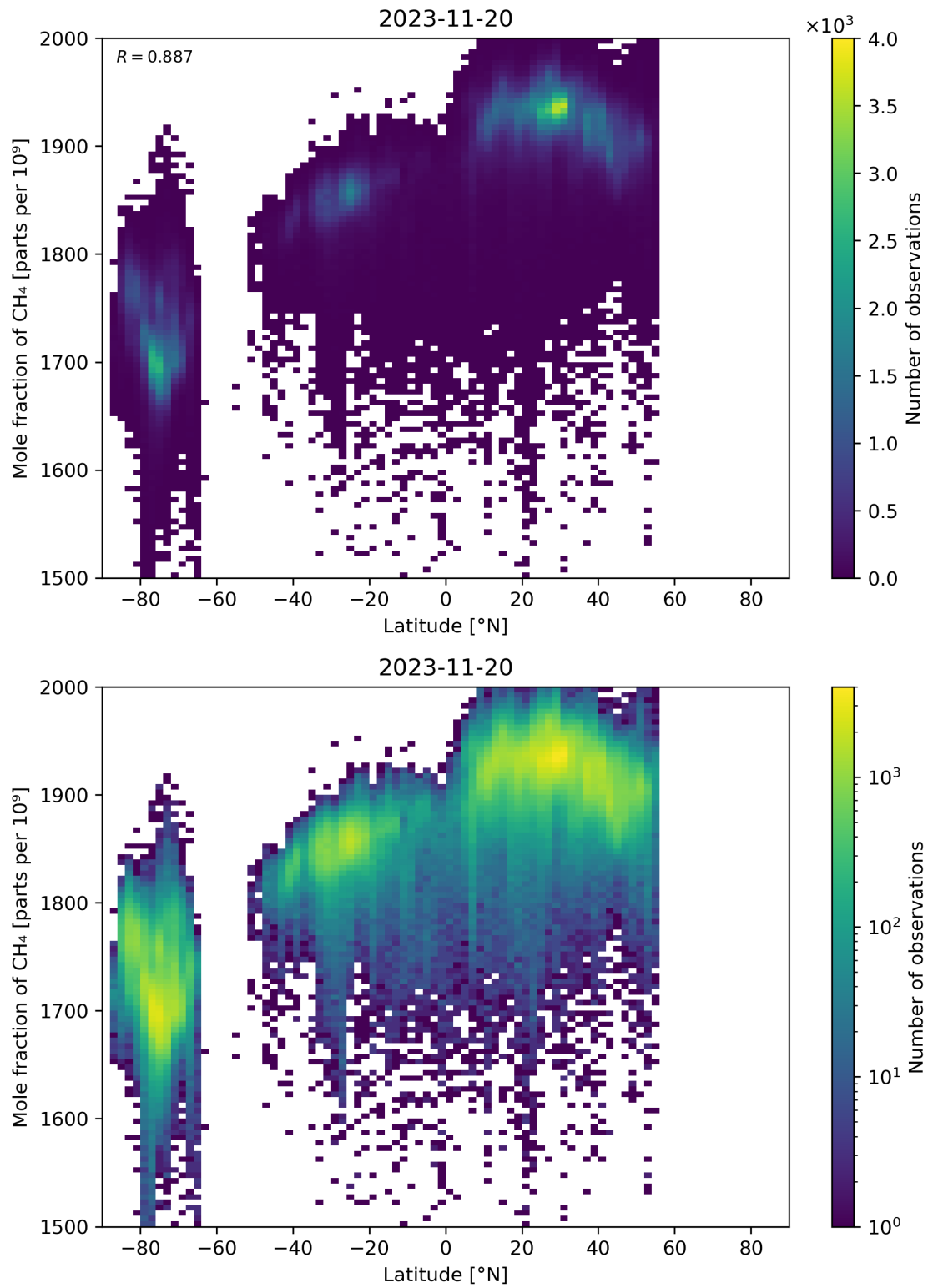
Figure 57: Scatter density plot of “Latitude” against “Mole fraction of CH 4 ” for 2023-11-19 to 2023-11-21.
