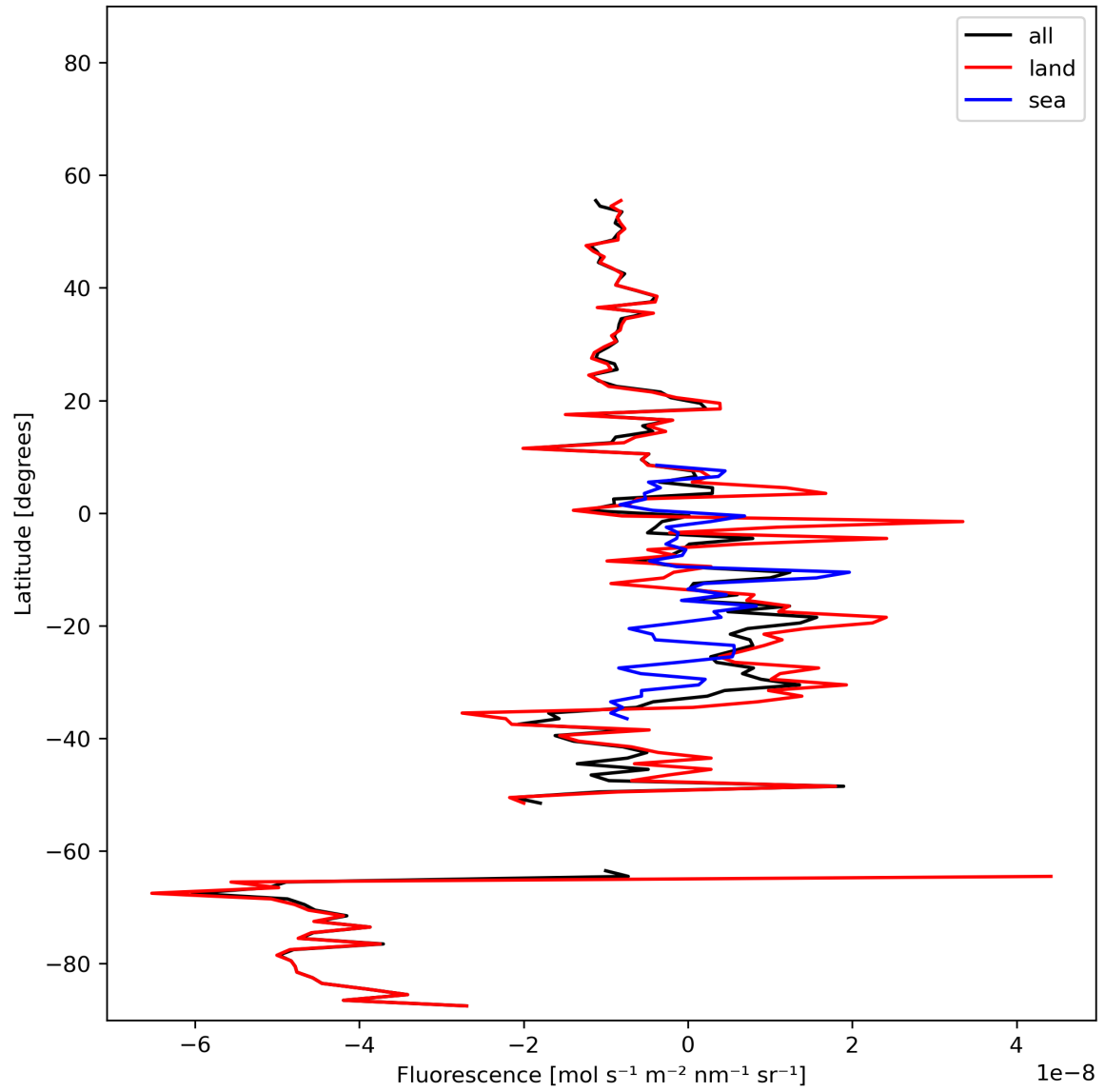
Figure 21: Zonal average of “Fluorescence” for 2023-11-19 to 2023-11-21.
