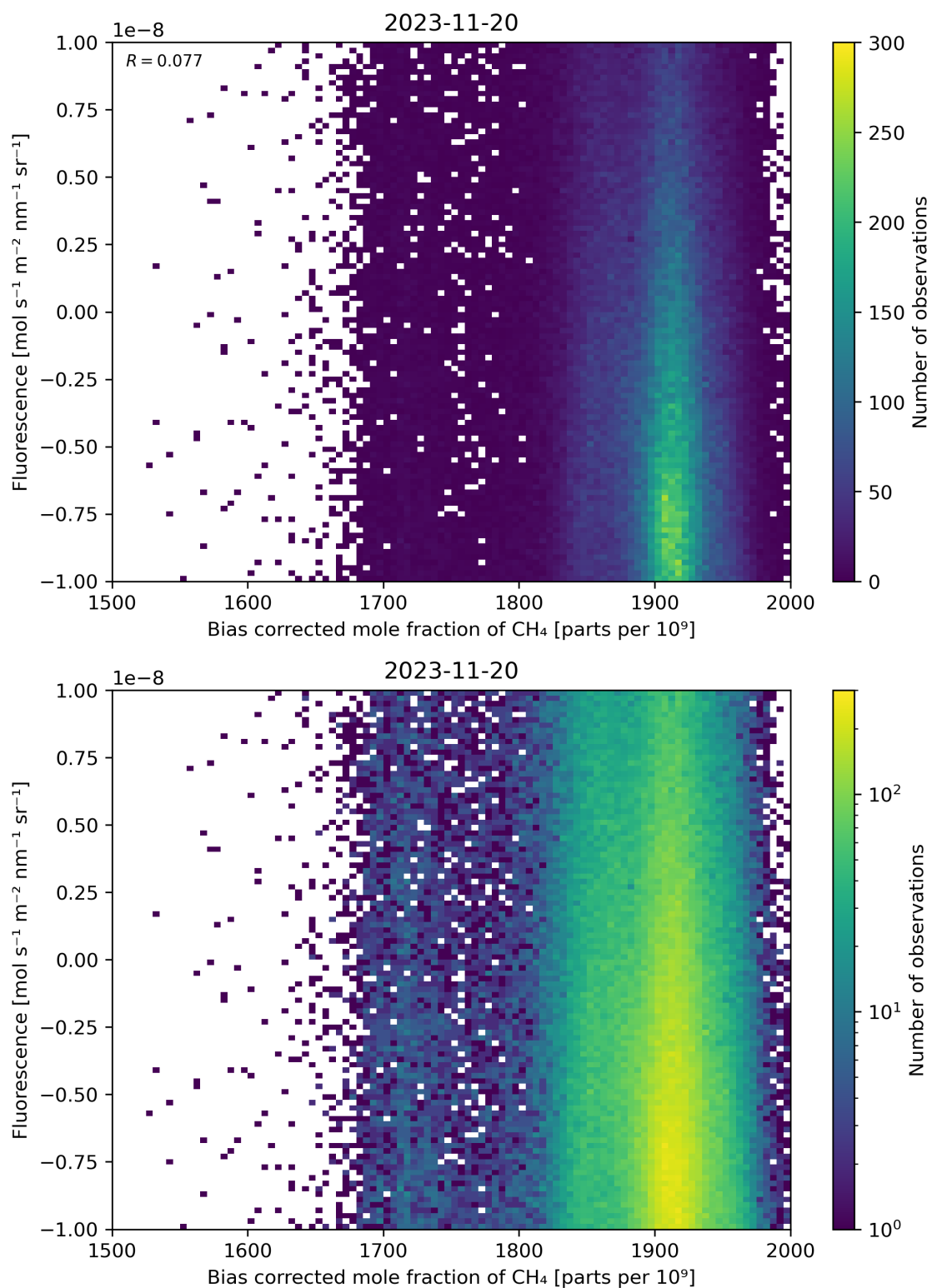
Figure 66: Scatter density plot of “Bias corrected mole fraction of \text{CH}_4 ” against “Fluorescence” for 2023-11-19 to 2023-11-21.
