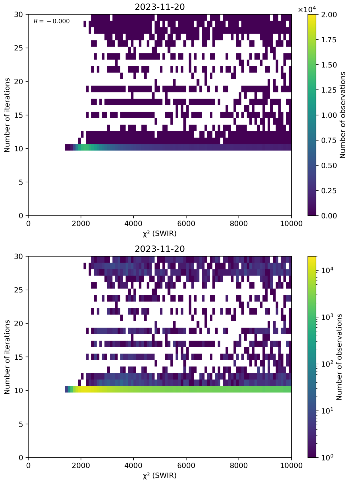
Figure 50: Scatter density plot of “ \chi^2 (SWIR)” against “Number of iterations” for 2023-11-19 to 2023-11-21.
