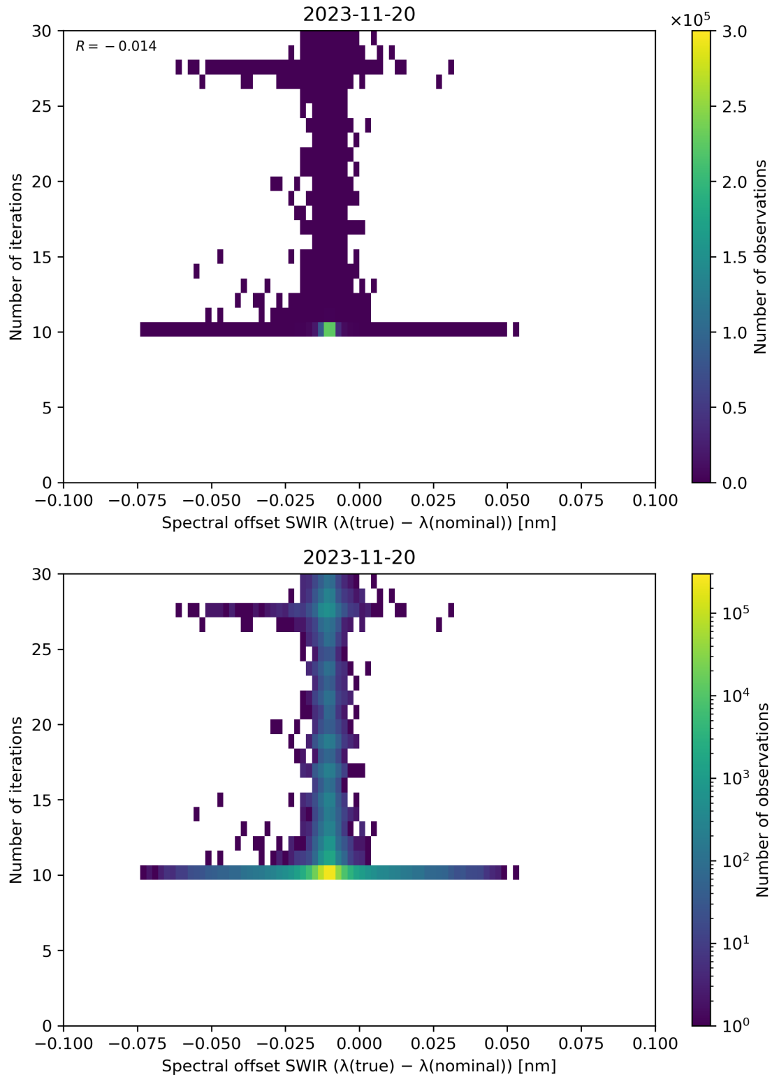
Figure 121: Scatter density plot of “Spectral offset SWIR ( \lambda(\text{true}) - \lambda(\text{nominal}) )” against “Number of iterations” for 2023-11-19 to 2023-11-21.
