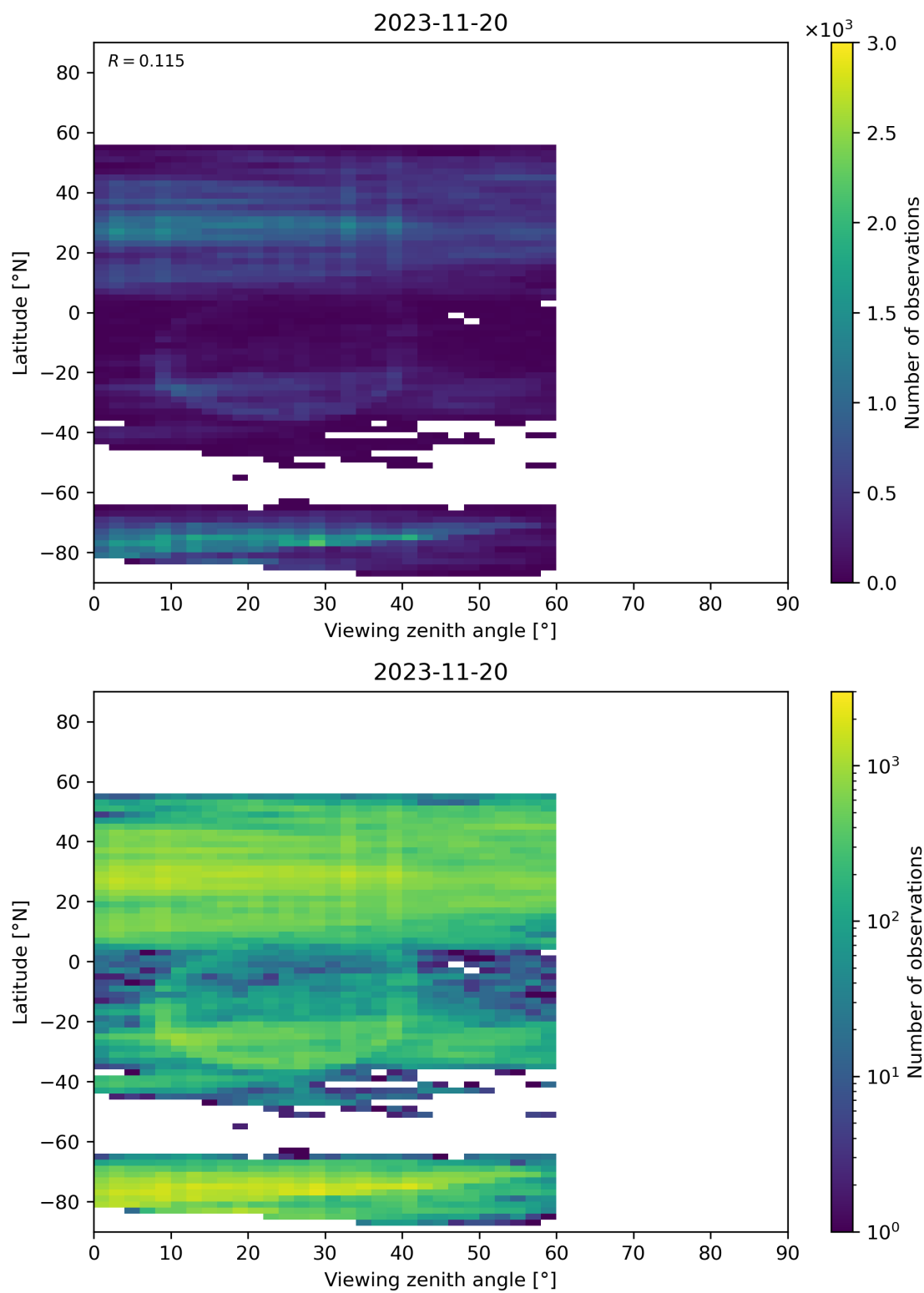
Figure 109: Scatter density plot of “Viewing zenith angle” against “Latitude” for 2023-11-19 to 2023-11-21.
