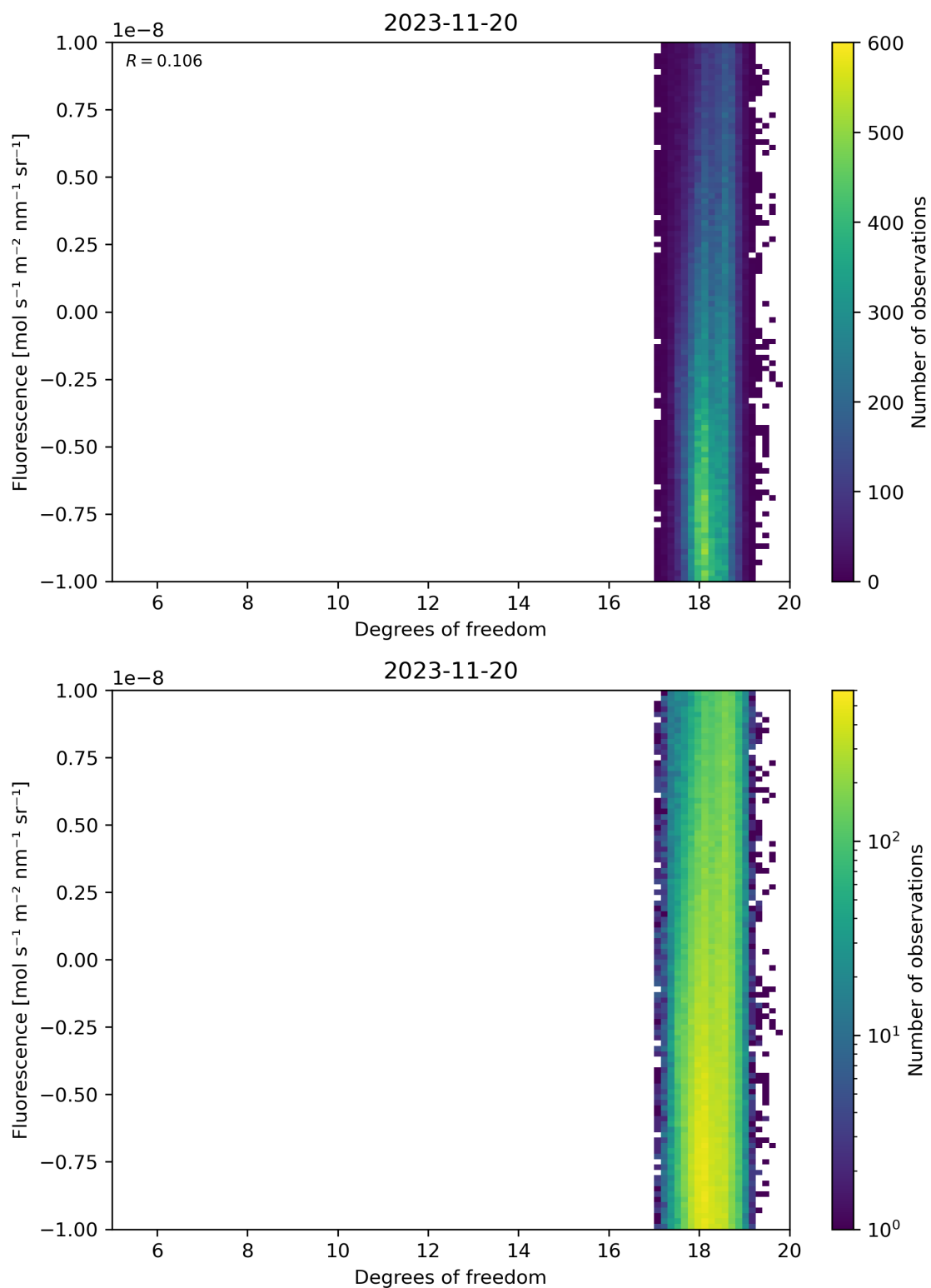
Figure 51: Scatter density plot of “Degrees of freedom” against “Fluorescence” for 2023-11-19 to 2023-11-21.
