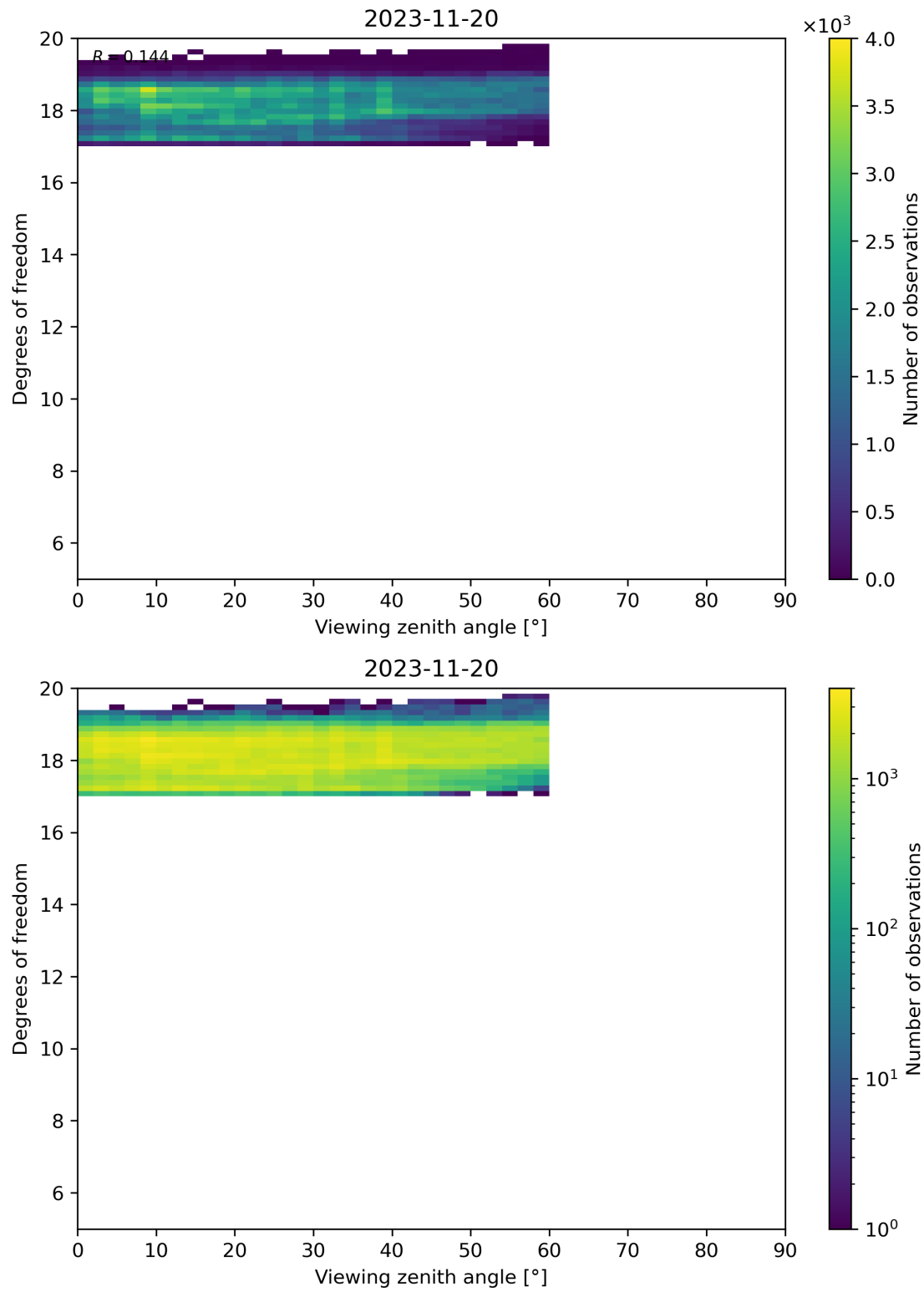
Figure 107: Scatter density plot of “Viewing zenith angle” against “Degrees of freedom” for 2023-11-19 to 2023-11-21.
