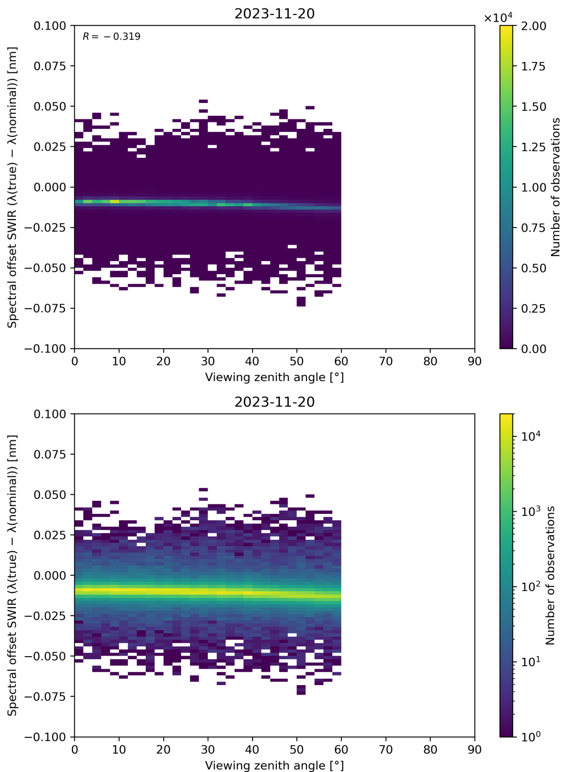
Figure 116: Scatter density plot of “Viewing zenith angle” against “Spectral offset SWIR ( \lambda(\text{true}) - \lambda(\text{nominal}) )” for 2023-11-19 to 2023-11-21.
