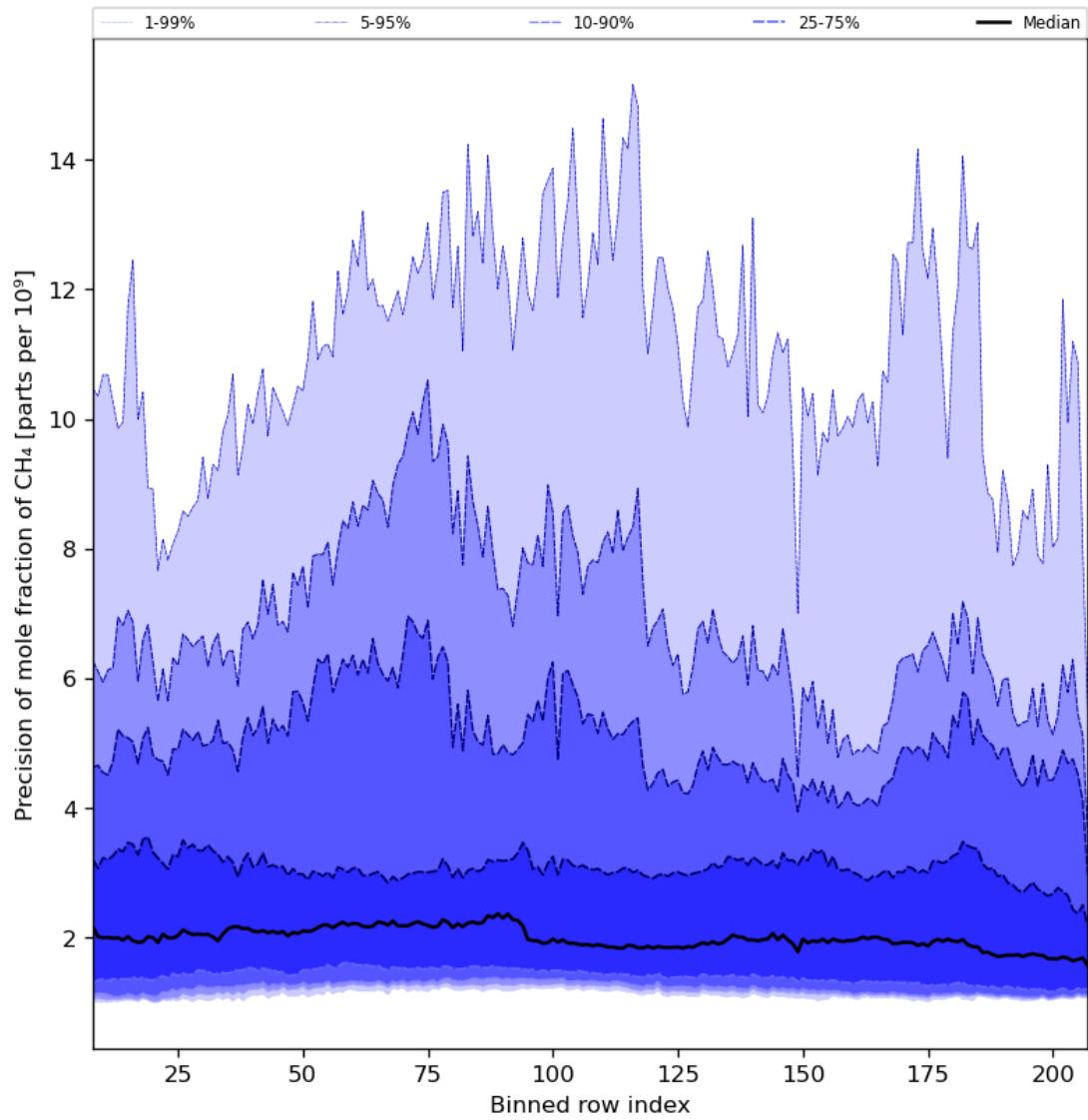
Figure 35: Along track statistics of “Precision of mole fraction of CH 4 ” for 2023-11-19 to 2023-11-21
