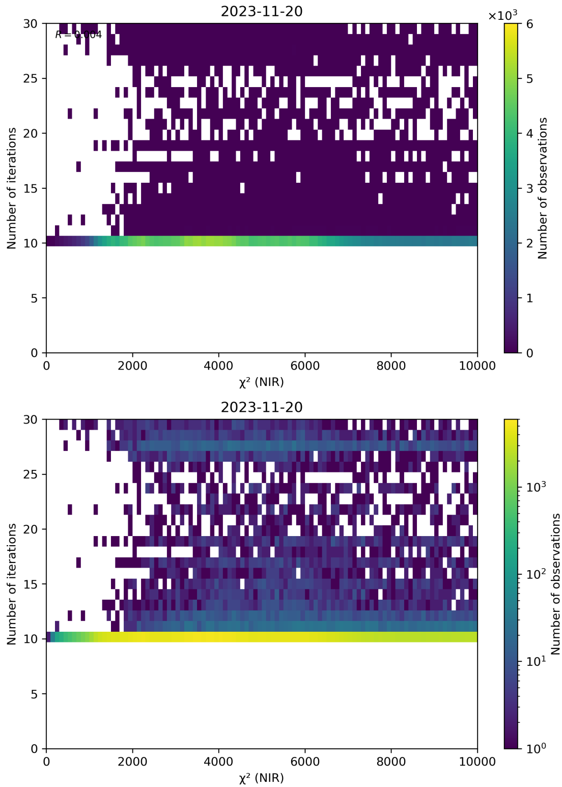
Figure 46: Scatter density plot of “ \chi^2 (NIR)” against “Number of iterations” for 2023-11-19 to 2023-11-21.
