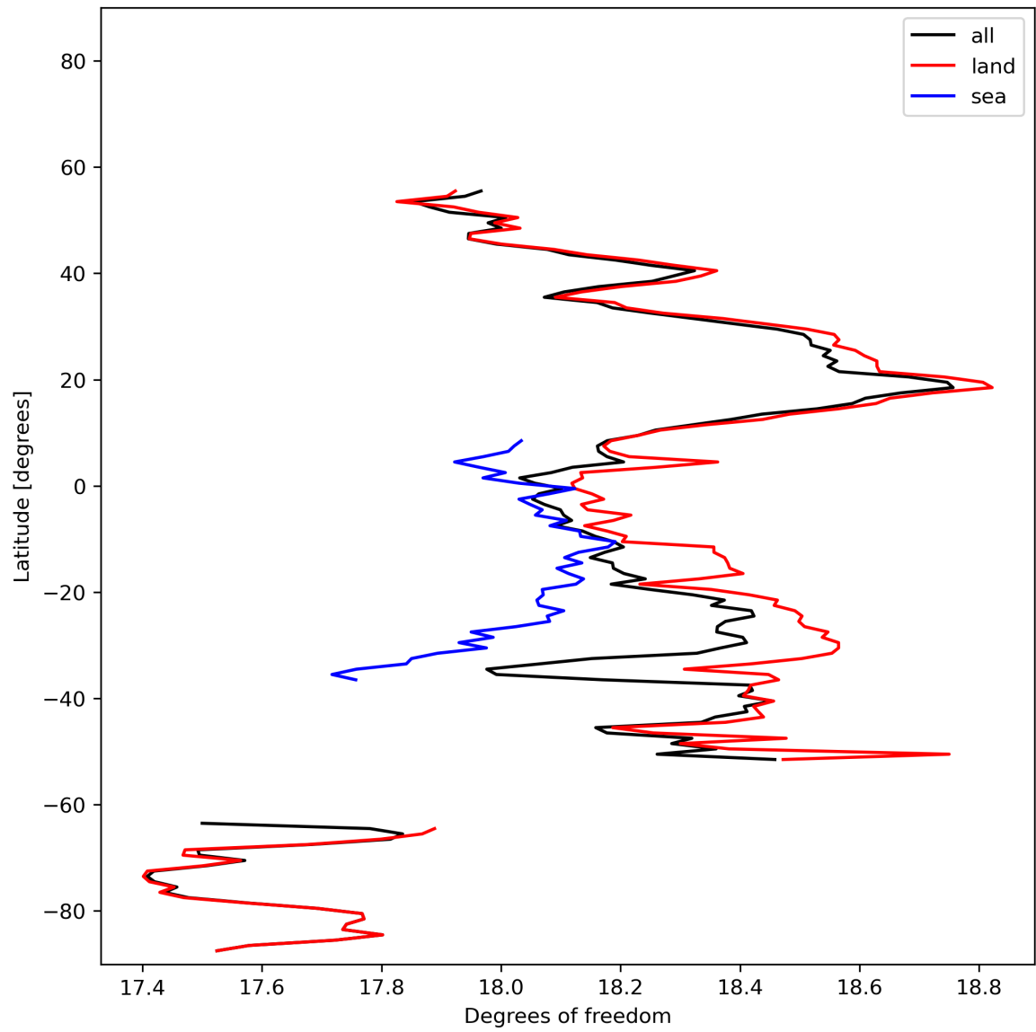
Figure 19: Zonal average of “Degrees of freedom” for 2023-11-19 to 2023-11-21.
