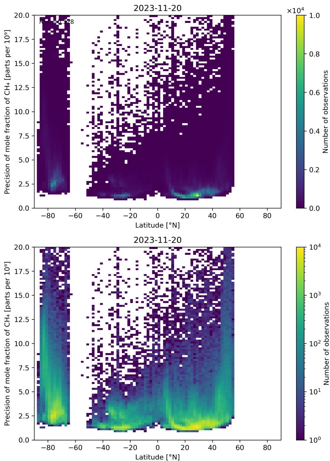
Figure 59: Scatter density plot of “Latitude” against “Precision of mole fraction of CH 4 ” for 2023-11-19 to 2023-11-21.
