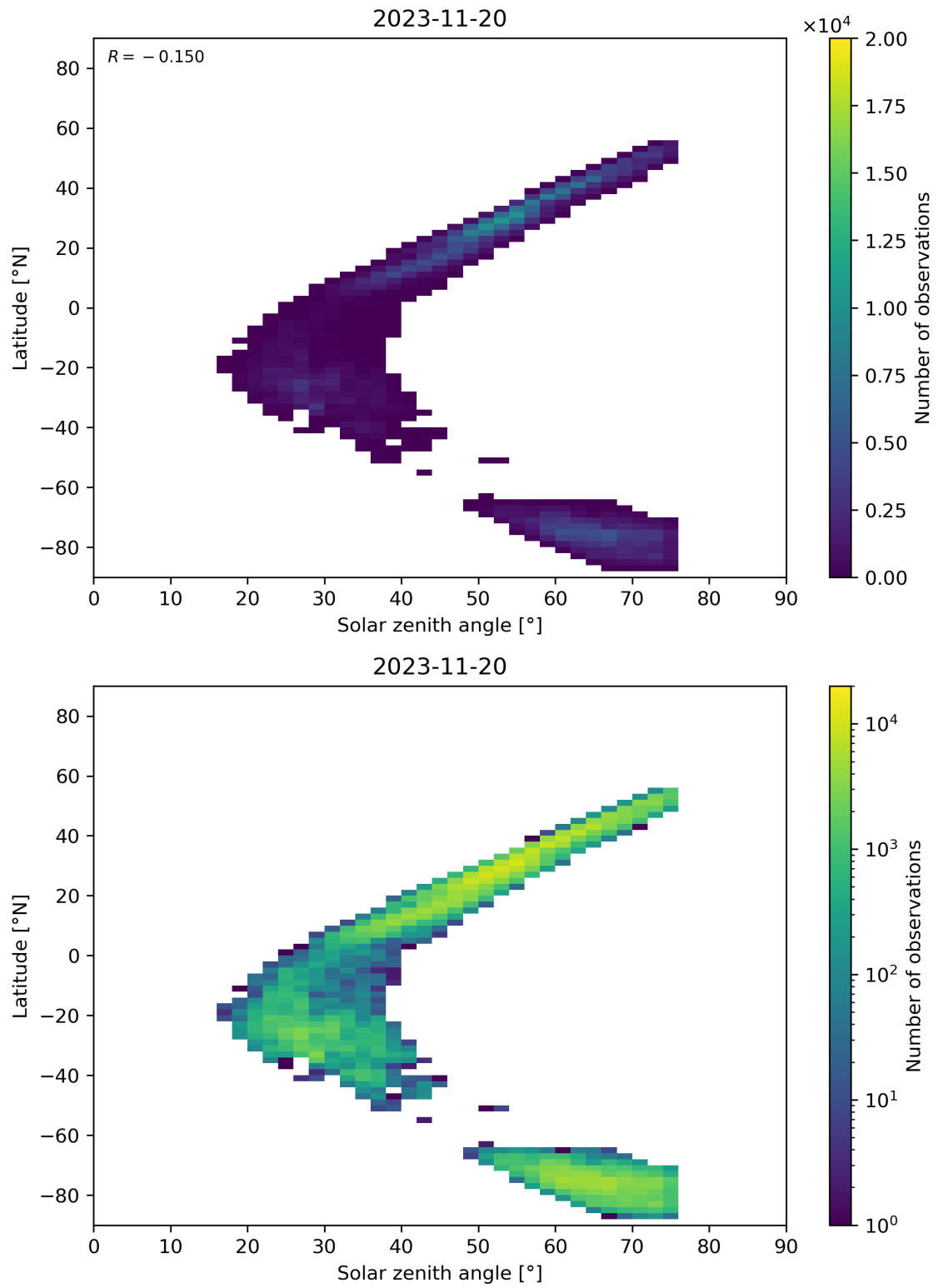
Figure 98: Scatter density plot of “Solar zenith angle” against “Latitude” for 2023-11-19 to 2023-11-21.
