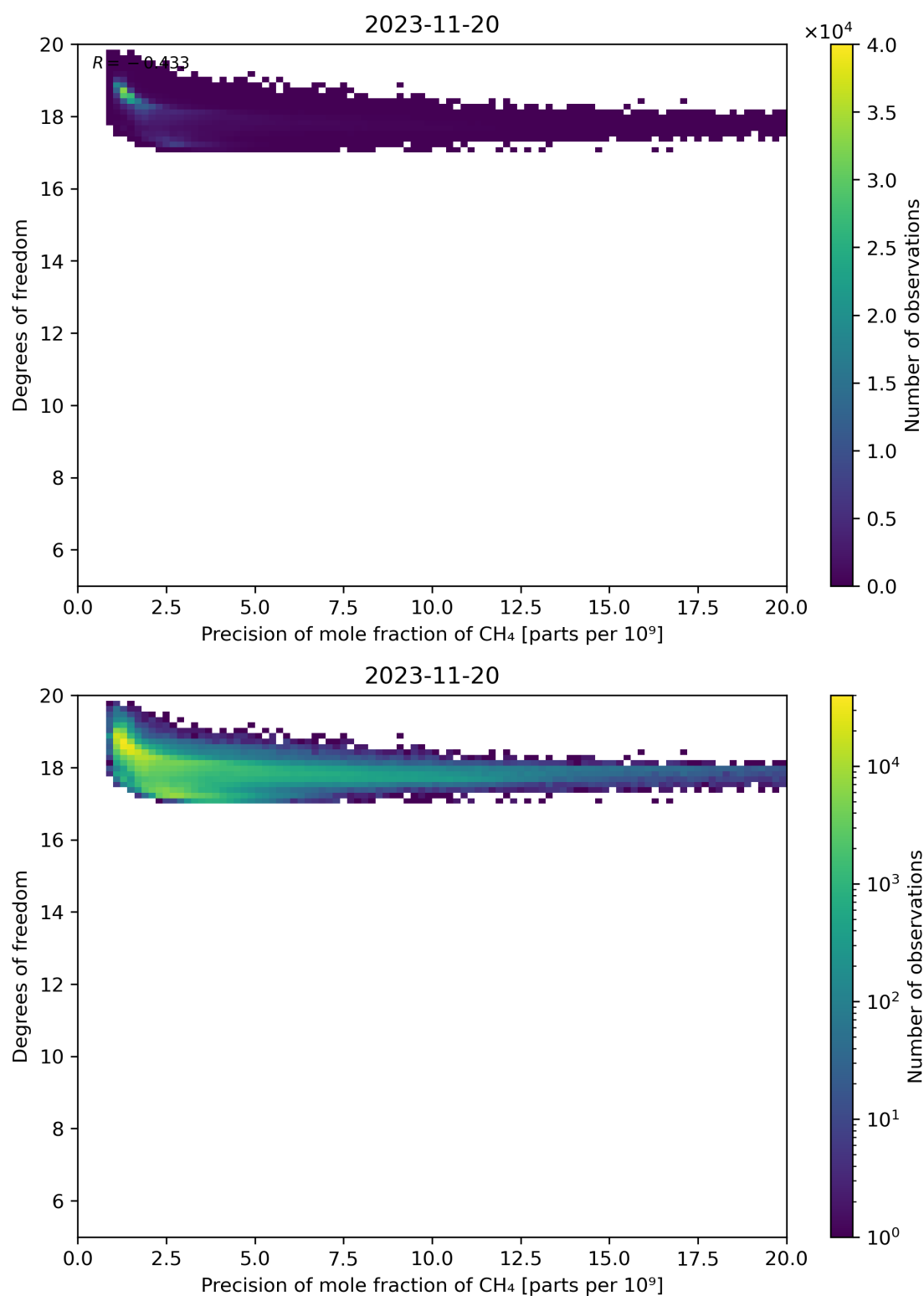
Figure 80: Scatter density plot of “Precision of mole fraction of CH 4 ” against “Degrees of freedom” for 2023-11-19 to 2023-11-21.
