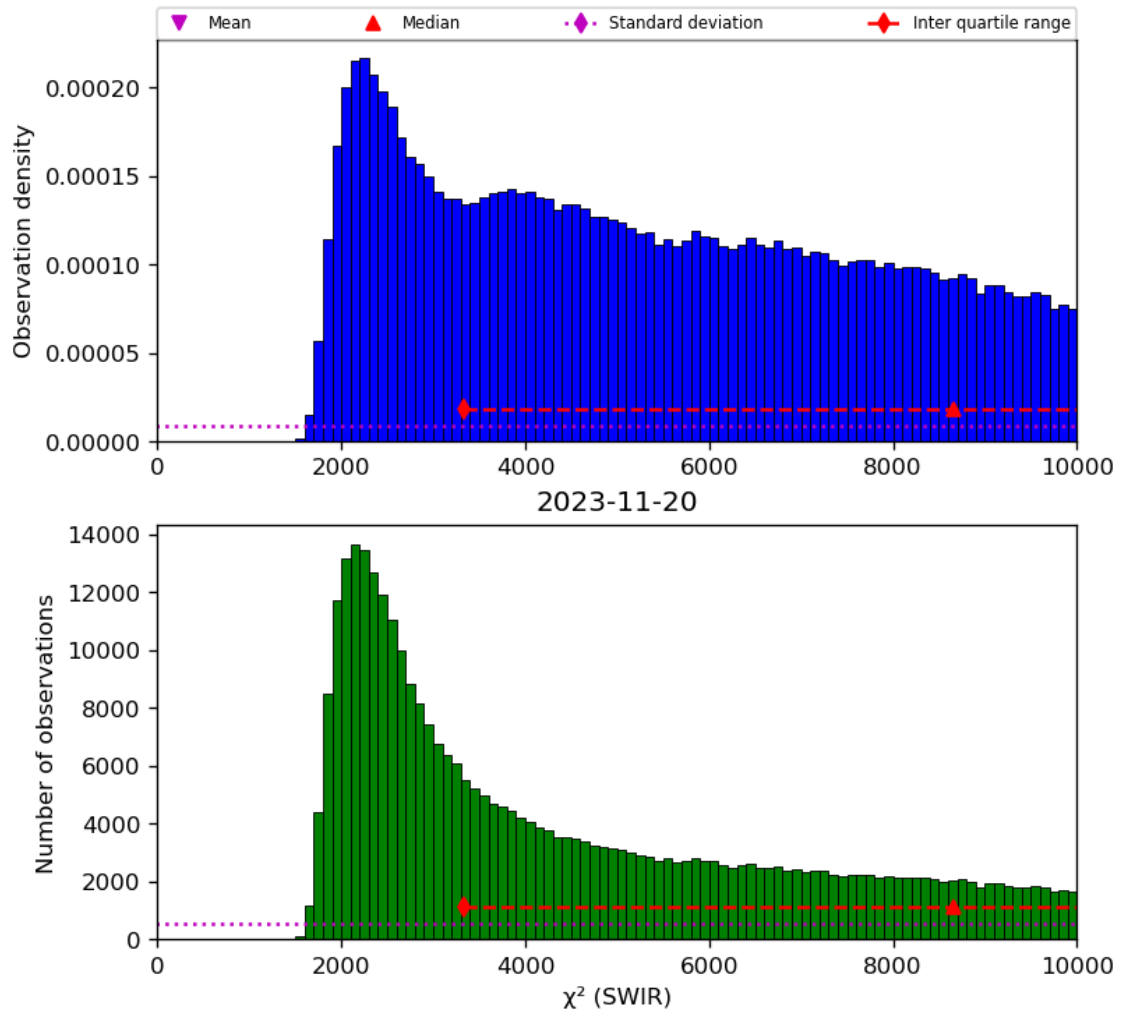
Figure 28: Histogram of “ \chi^2 (SWIR)” for 2023-11-19 to 2023-11-21
