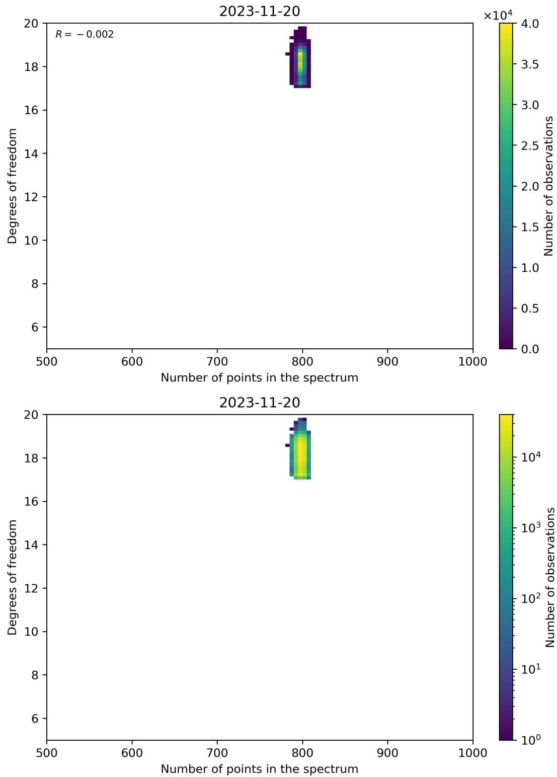
Figure 90: Scatter density plot of “Number of points in the spectrum” against “Degrees of freedom” for 2023-11-19 to 2023-11-21.
