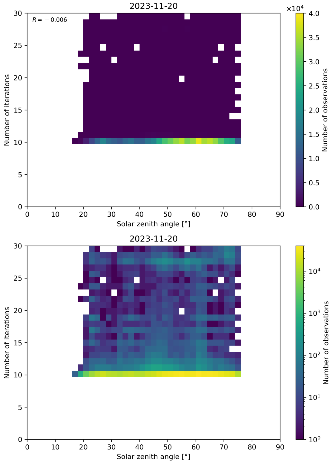
Figure 102: Scatter density plot of “Solar zenith angle” against “Number of iterations” for 2023-11-19 to 2023-11-21.
