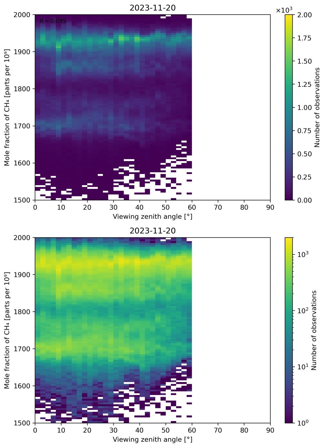
Figure 110: Scatter density plot of “Viewing zenith angle” against “Mole fraction of \text{CH}_4 ” for 2023-11-19 to 2023-11-21.
