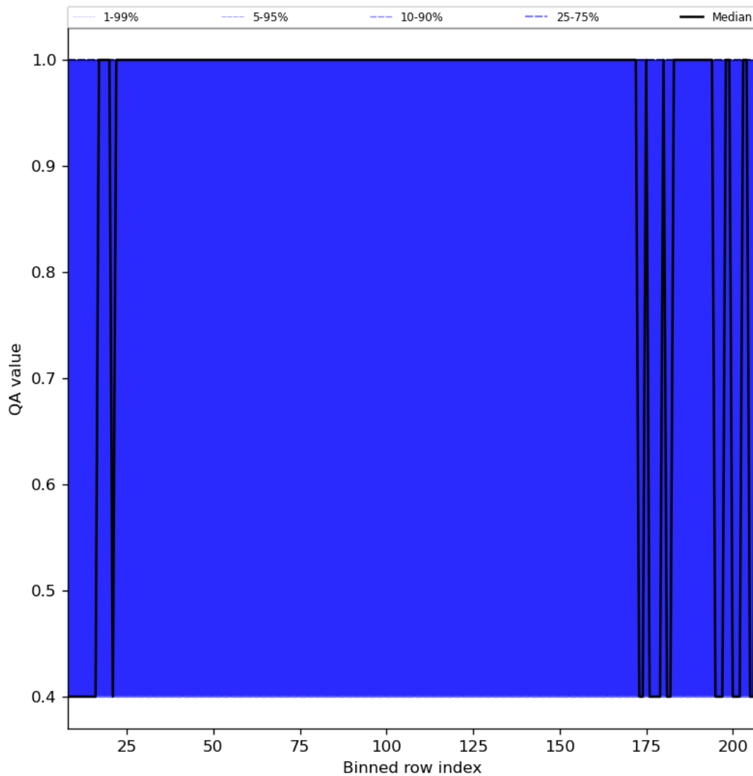
Figure 33: Along track statistics of “QA value” for 2023-11-19 to 2023-11-21
