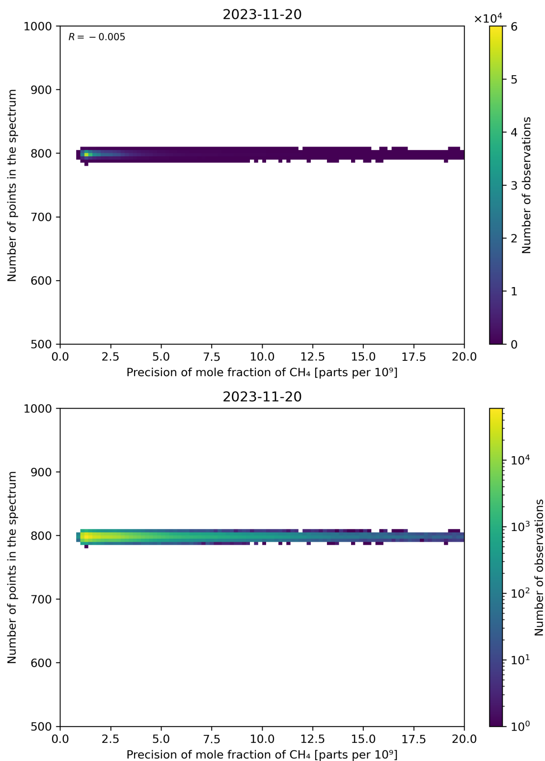
Figure 84: Scatter density plot of “Precision of mole fraction of CH 4 ” against “Number of points in the spectrum” for 2023-11-19 to 2023-11-21.
