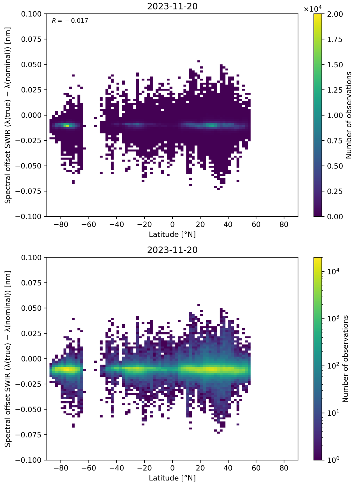
Figure 62: Scatter density plot of “Latitude” against “Spectral offset SWIR ( \lambda(\text{true}) - \lambda(\text{nominal}) )” for 2023-11-19 to 2023-11-21.
