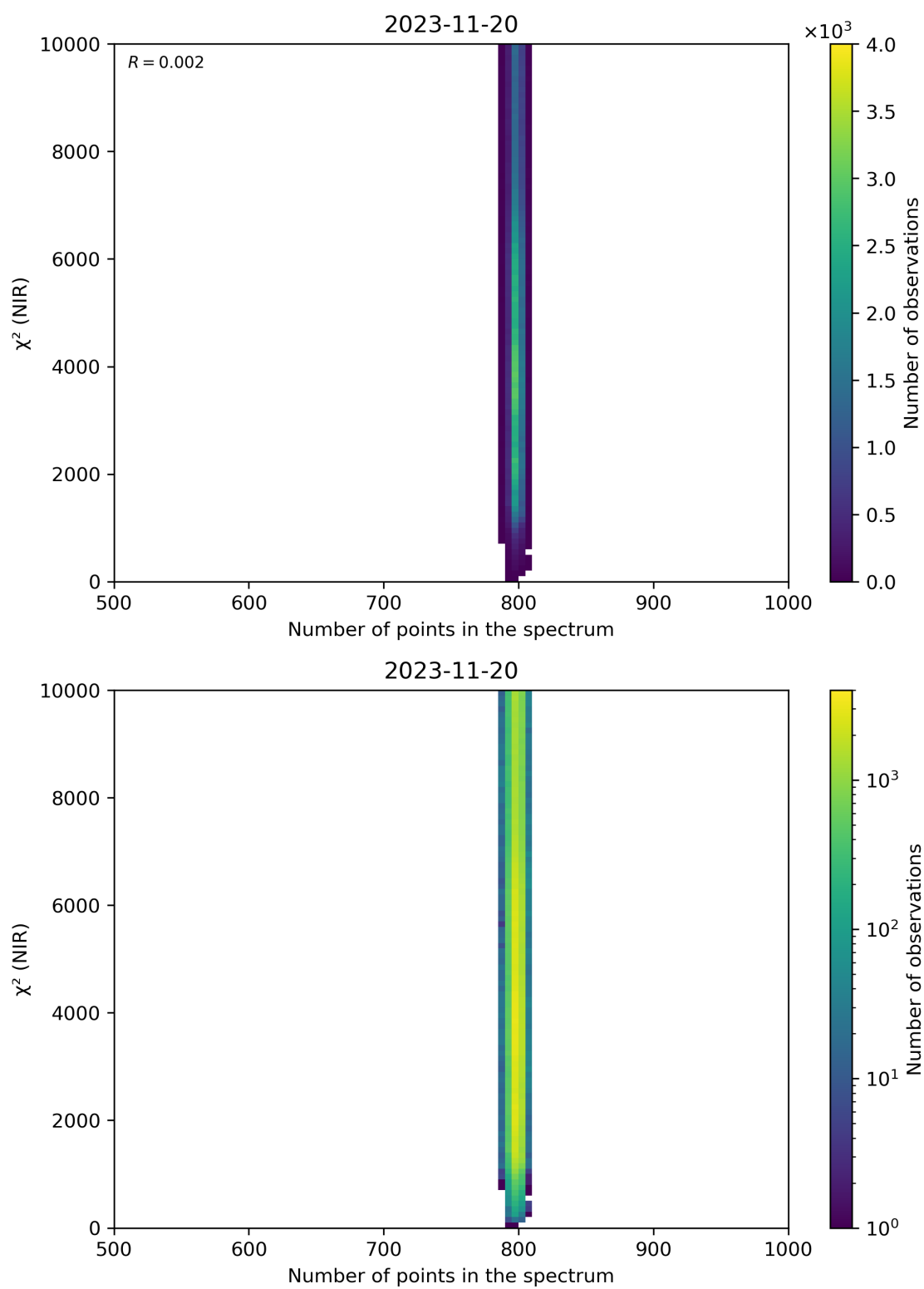
Figure 88: Scatter density plot of “Number of points in the spectrum” against “ \chi^2 (NIR)” for 2023-11-19 to 2023-11-21.
