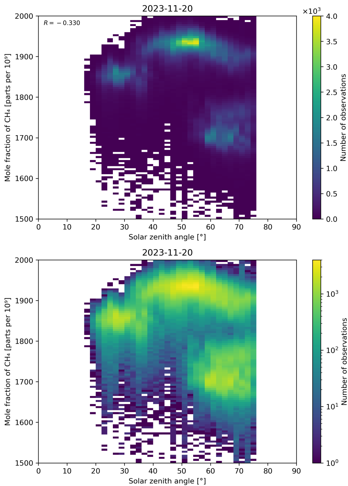
Figure 99: Scatter density plot of “Solar zenith angle” against “Mole fraction of CH 4 ” for 2023-11-19 to 2023-11-21.
