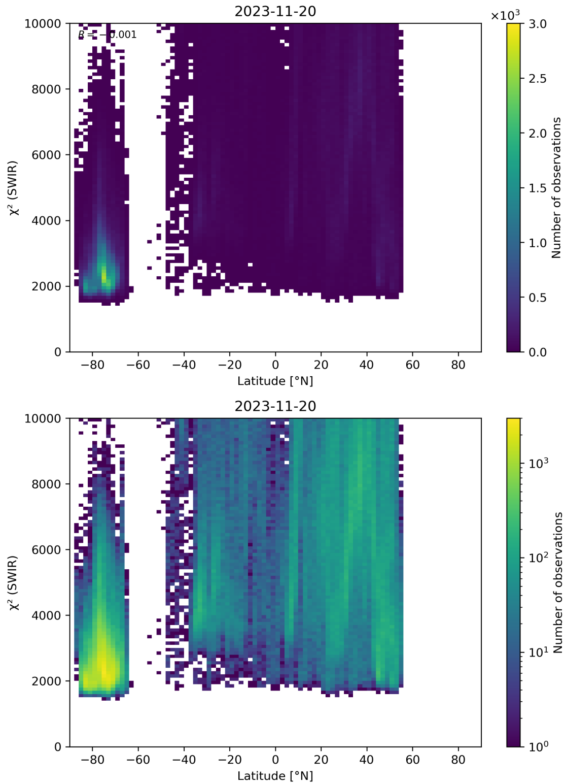
Figure 54: Scatter density plot of “Latitude” against “ \chi^2 (SWIR)” for 2023-11-19 to 2023-11-21.
