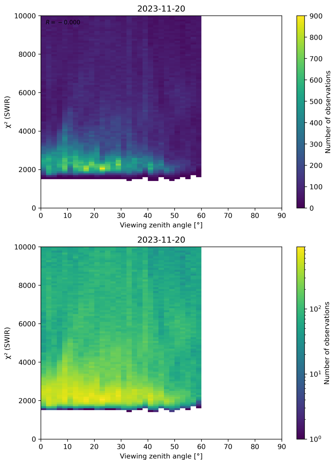
Figure 106: Scatter density plot of “Viewing zenith angle” against “ \chi^2 (SWIR)” for 2023-11-19 to 2023-11-21.
