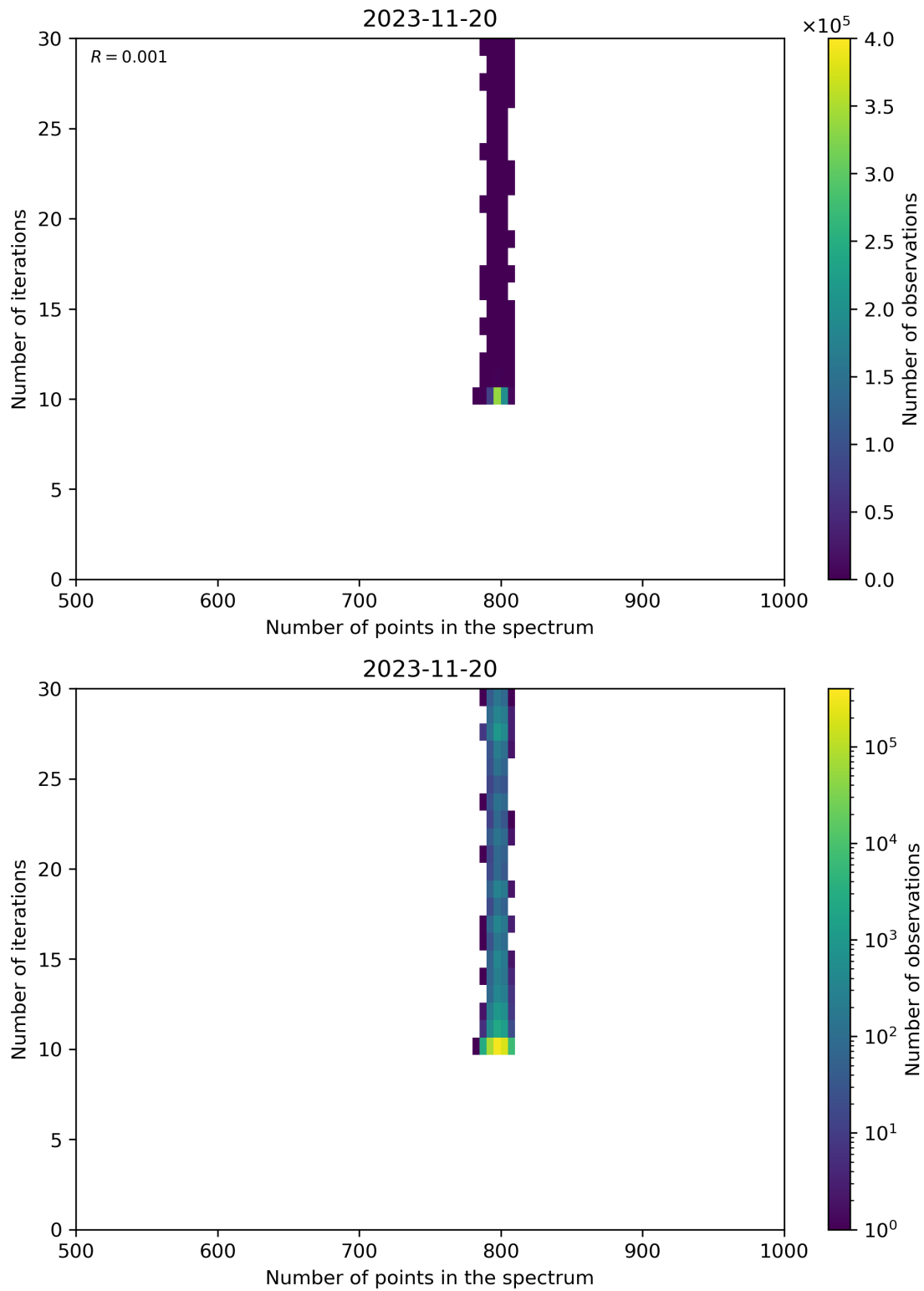
Figure 92: Scatter density plot of “Number of points in the spectrum” against “Number of iterations” for 2023-11-19 to 2023-11-21.
