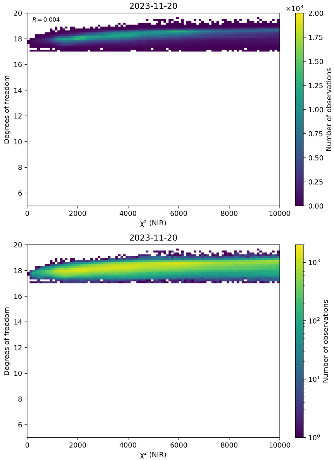
Figure 44: Scatter density plot of “ \chi^2 (NIR)” against “Degrees of freedom” for 2023-11-19 to 2023-11-21.
