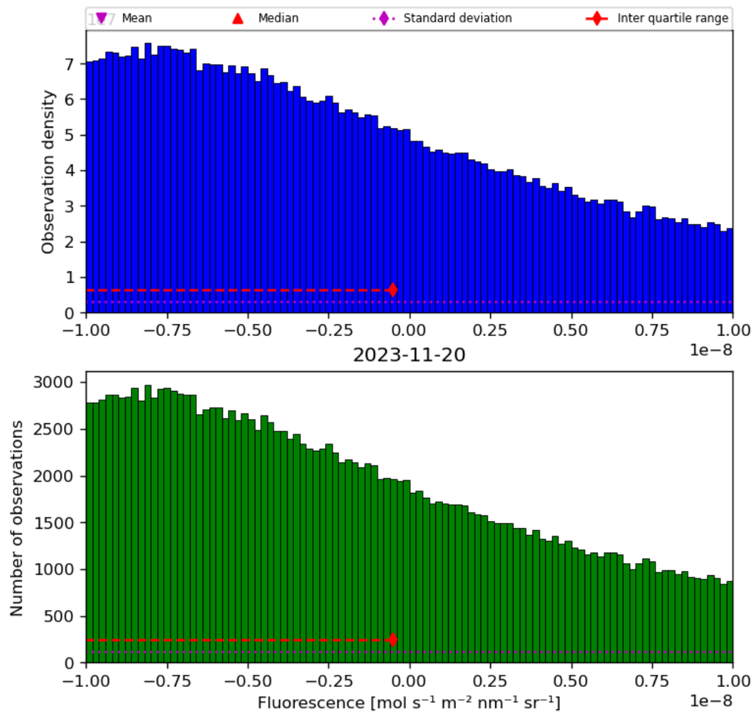
Figure 32: Histogram of “Fluorescence” for 2023-11-19 to 2023-11-21
