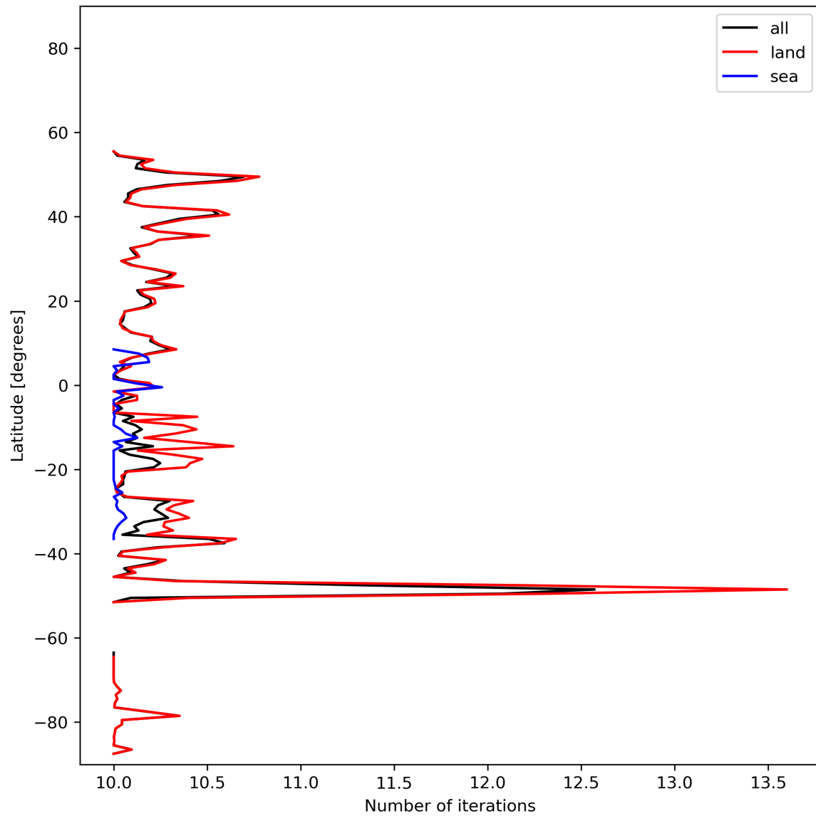
Figure 20: Zonal average of “Number of iterations” for 2023-11-19 to 2023-11-21.
