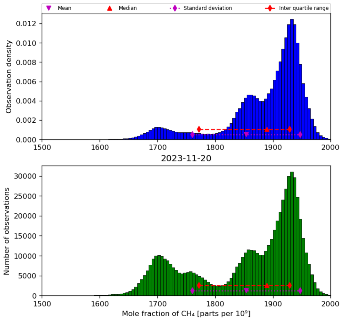
Figure 23: Histogram of “Mole fraction of CH 4 ” for 2023-11-19 to 2023-11-21
