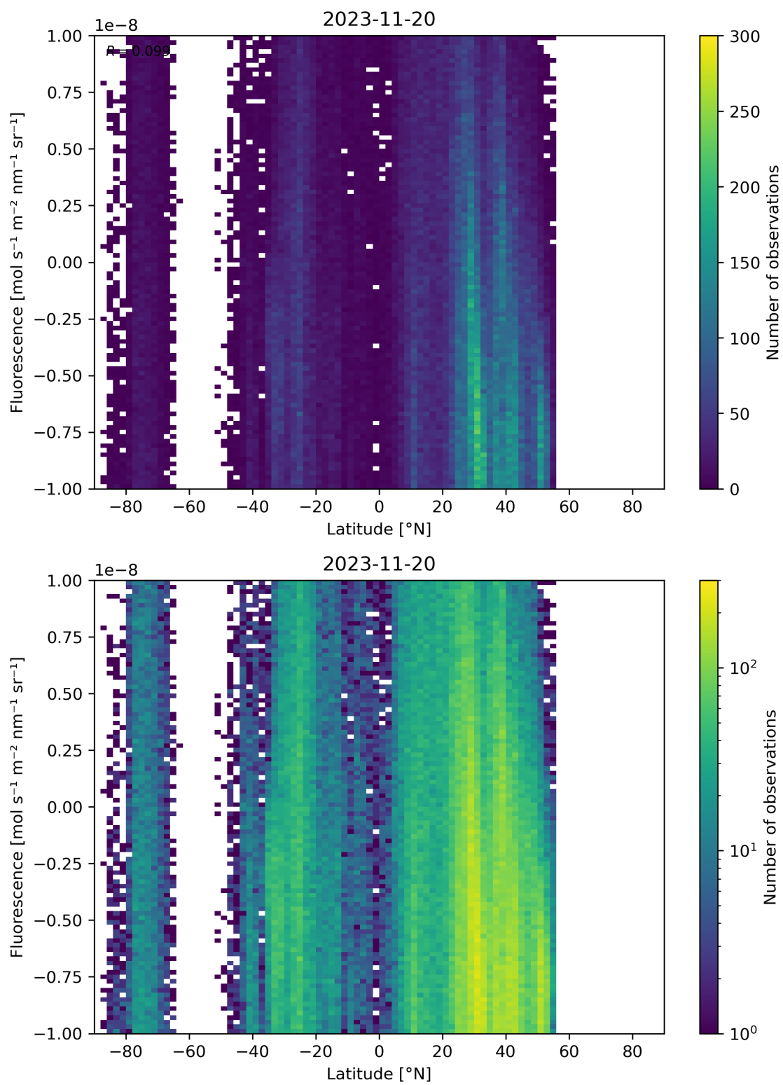
Figure 56: Scatter density plot of “Latitude” against “Fluorescence” for 2023-11-19 to 2023-11-21.
