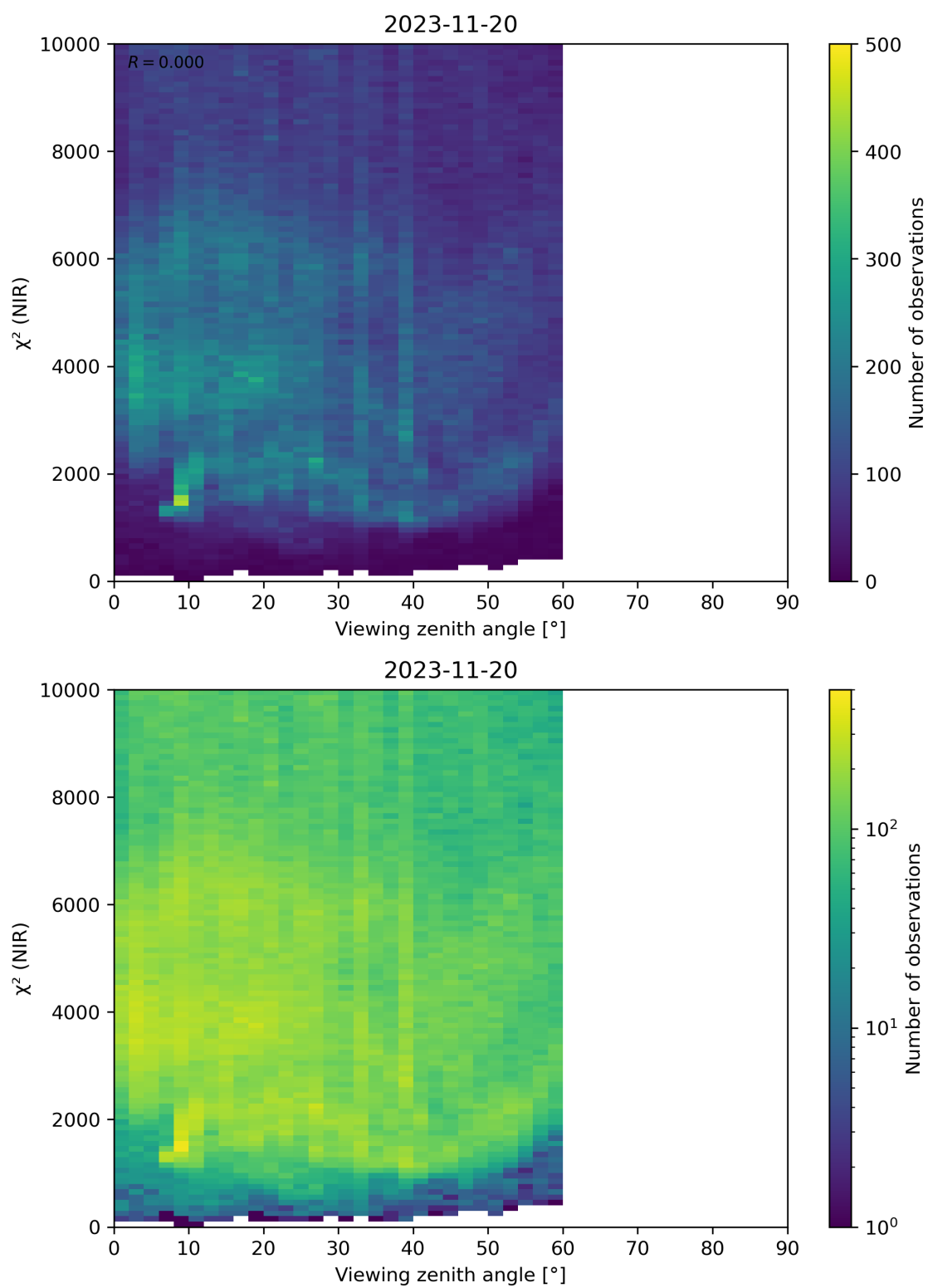
Figure 105: Scatter density plot of “Viewing zenith angle” against “ \chi^2 (NIR)” for 2023-11-19 to 2023-11-21.
