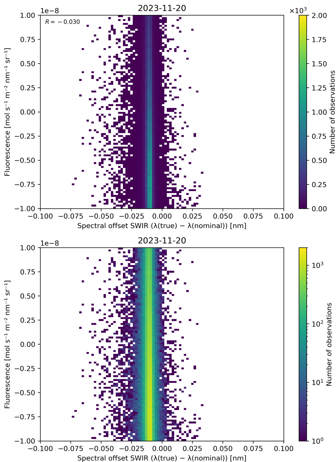
Figure 120: Scatter density plot of “Spectral offset SWIR ( \lambda(\text{true}) - \lambda(\text{nominal}) )” against “Fluorescence” for 2023-11-19 to 2023-11-21.
