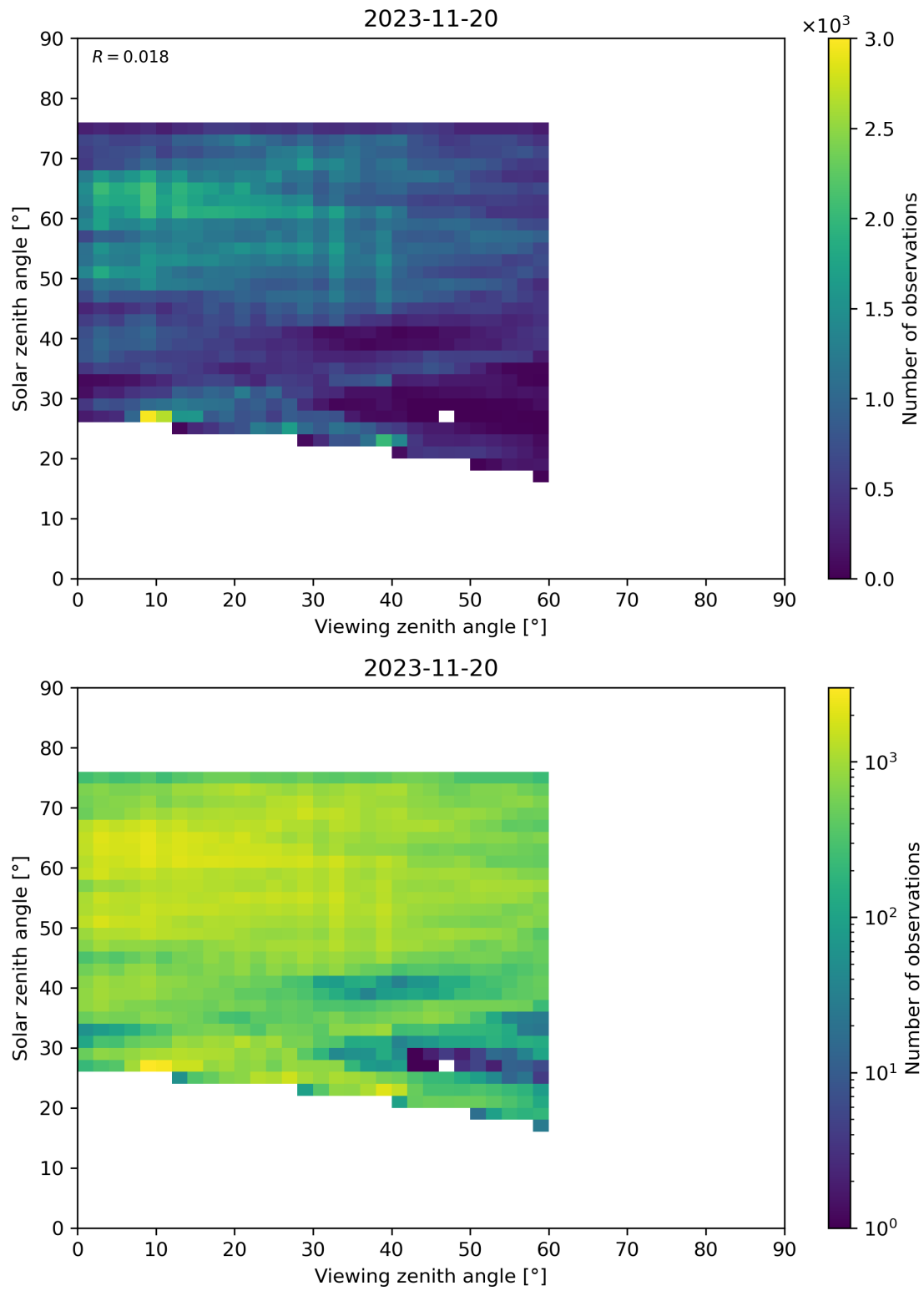
Figure 115: Scatter density plot of “Viewing zenith angle” against “Solar zenith angle” for 2023-11-19 to 2023-11-21.
