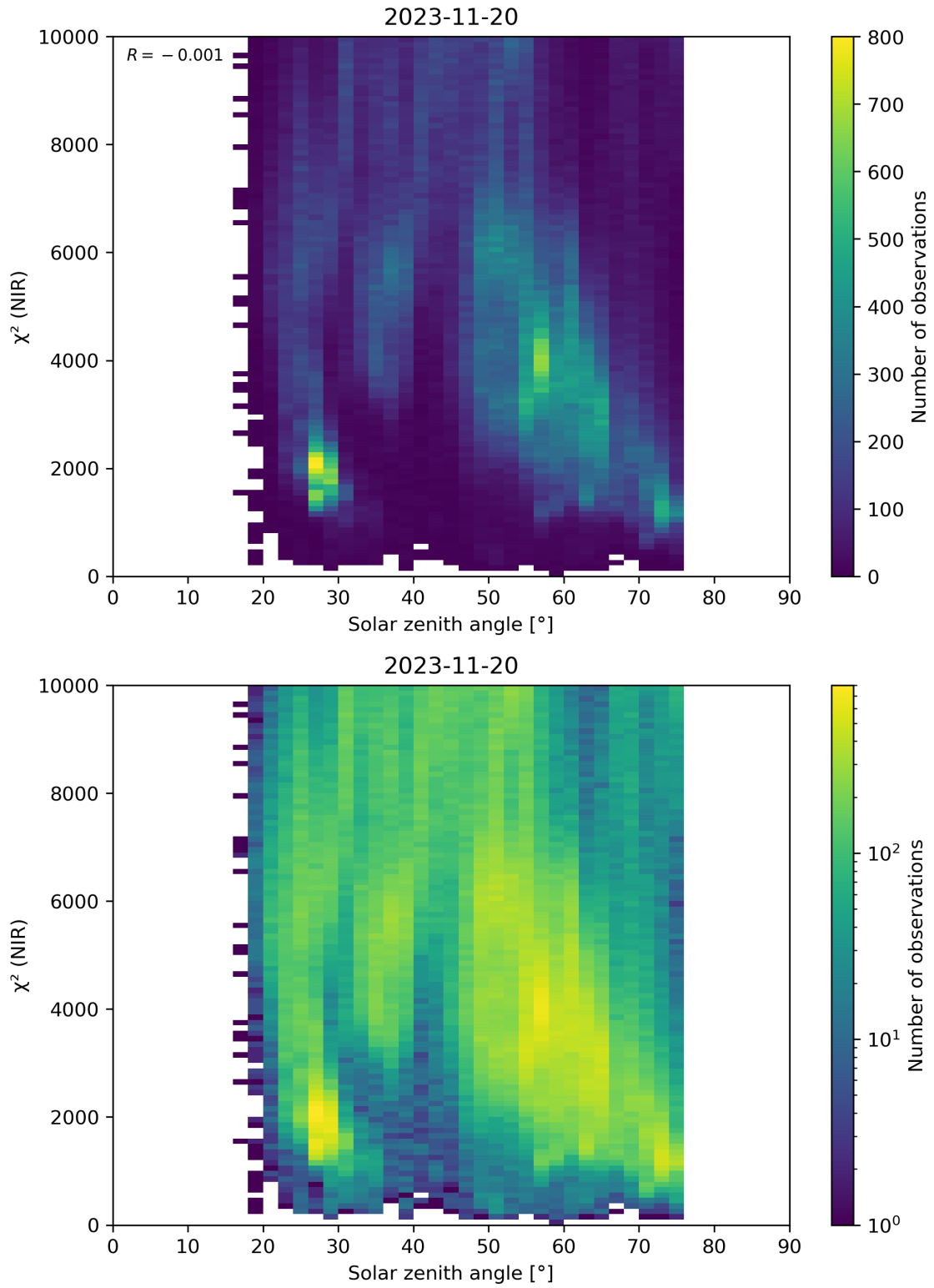
Figure 94: Scatter density plot of “Solar zenith angle” against “ \chi^2 (NIR)” for 2023-11-19 to 2023-11-21.
