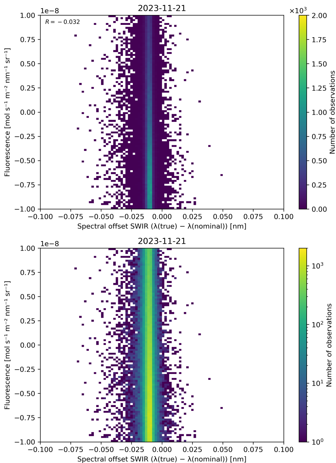
Figure 120: Scatter density plot of “Spectral offset SWIR ( \lambda(\text{true}) - \lambda(\text{nominal}) )” against “Fluorescence” for 2023-11-20 to 2023-11-22.
