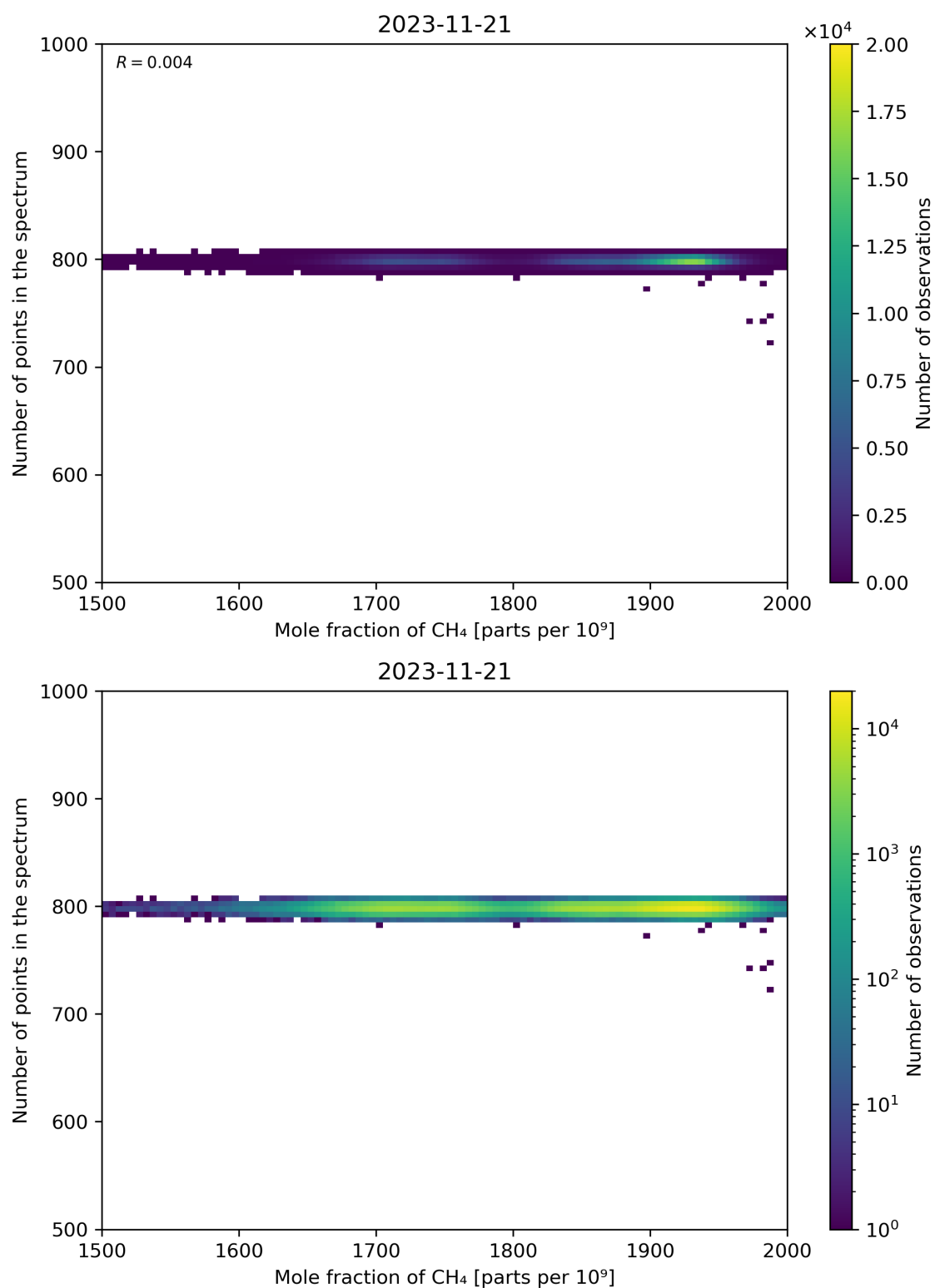
Figure 77: Scatter density plot of “Mole fraction of CH 4 ” against “Number of points in the spectrum” for 2023-11-20 to 2023-11-22.
