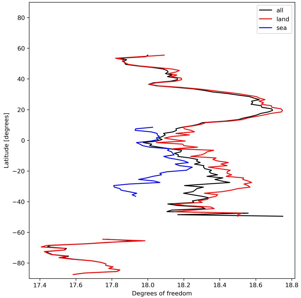
Figure 19: Zonal average of “Degrees of freedom” for 2023-11-20 to 2023-11-22.
