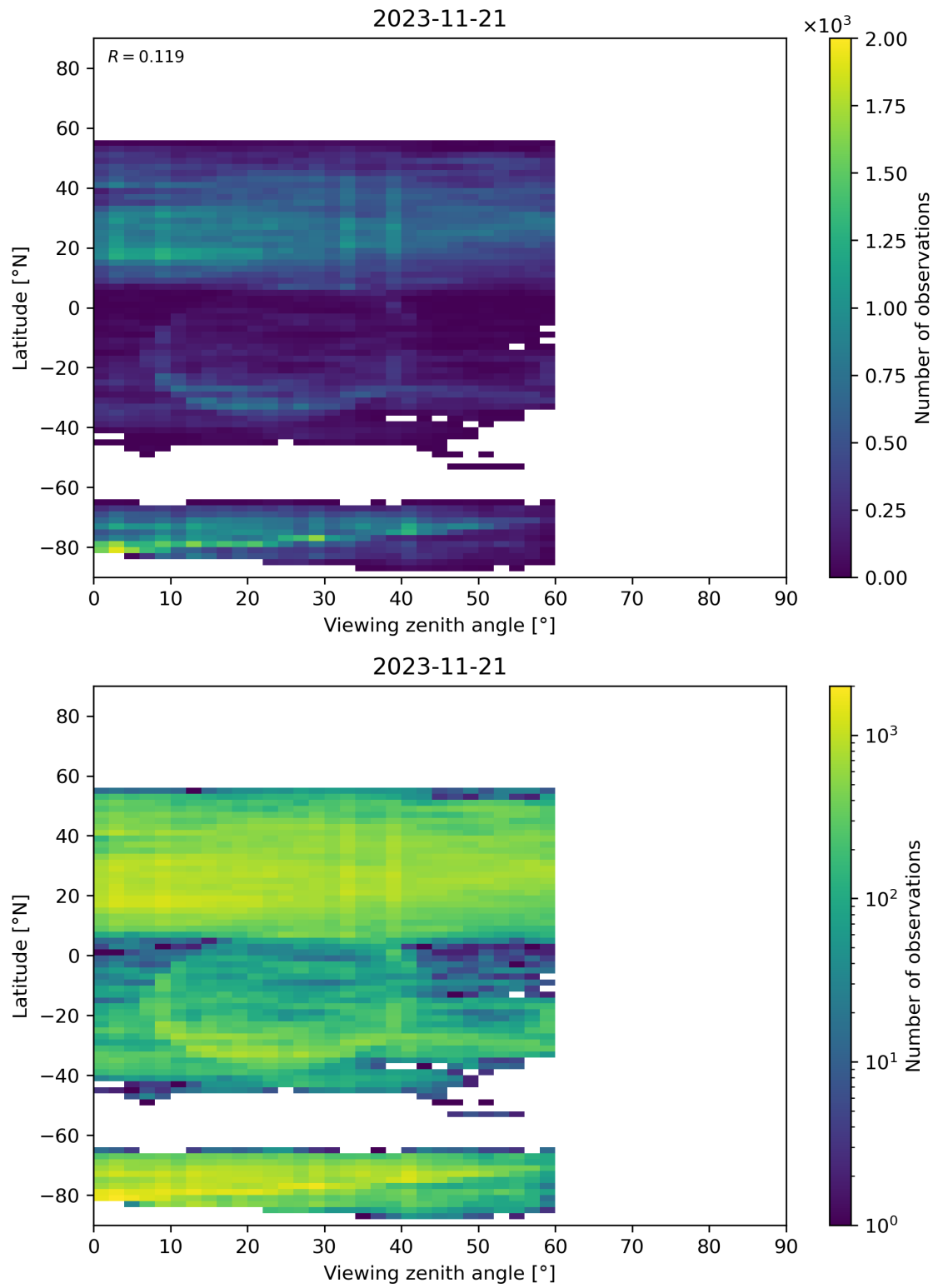
Figure 109: Scatter density plot of “Viewing zenith angle” against “Latitude” for 2023-11-20 to 2023-11-22.
