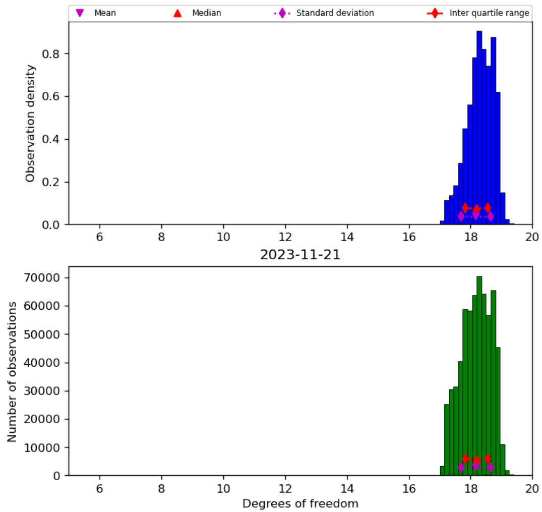
Figure 30: Histogram of “Degrees of freedom” for 2023-11-20 to 2023-11-22
