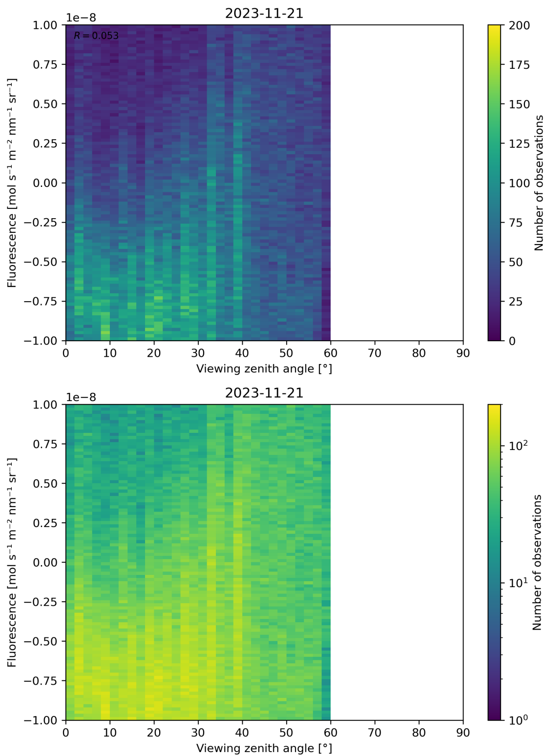
Figure 108: Scatter density plot of “Viewing zenith angle” against “Fluorescence” for 2023-11-20 to 2023-11-22.
