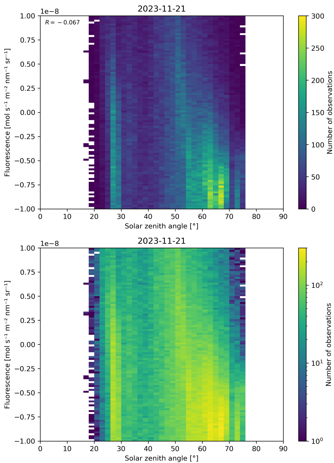
Figure 97: Scatter density plot of “Solar zenith angle” against “Fluorescence” for 2023-11-20 to 2023-11-22.
