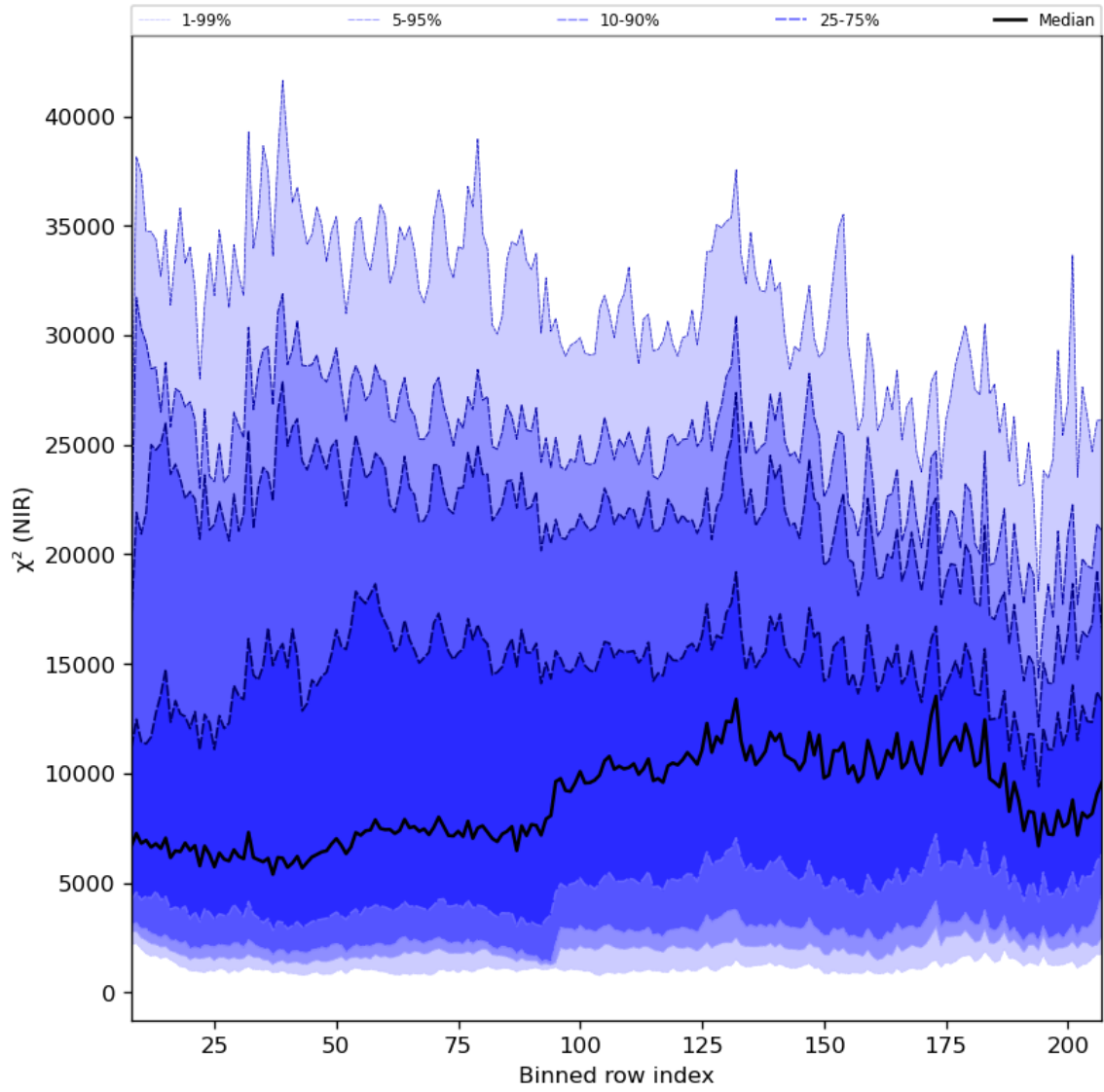
Figure 40: Along track statistics of “ \chi^2 (NIR)” for 2023-11-20 to 2023-11-22
