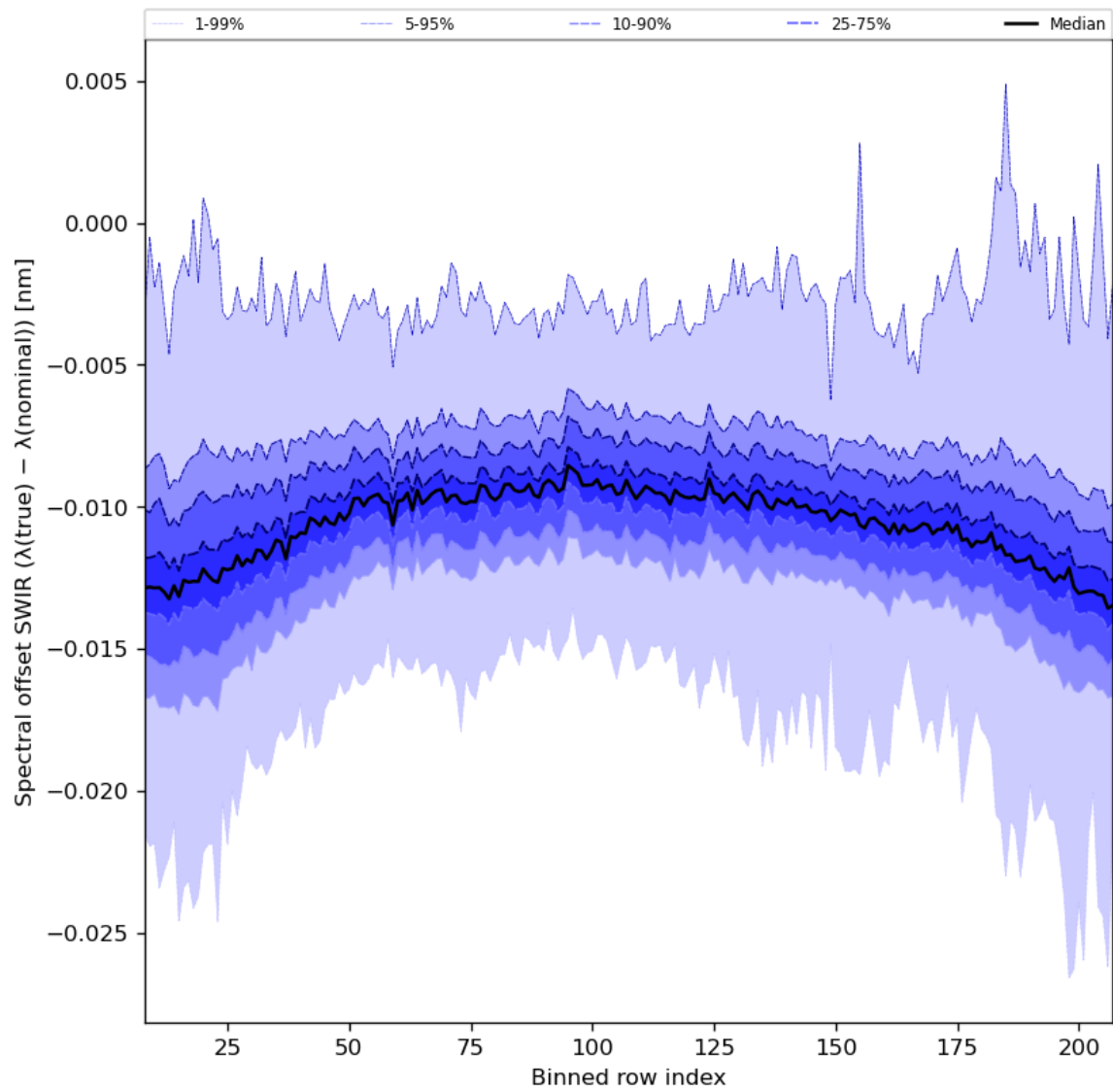
Figure 38: Along track statistics of “Spectral offset SWIR ( \lambda(\text{true}) - \lambda(\text{nominal}) )” for 2023-11-20 to 2023-11-22
