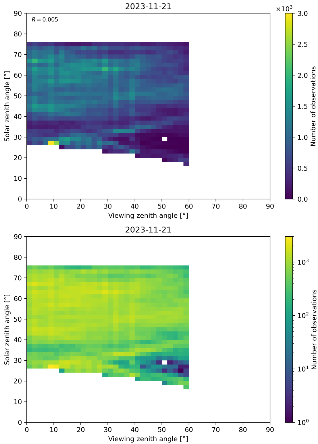
Figure 115: Scatter density plot of “Viewing zenith angle” against “Solar zenith angle” for 2023-11-20 to 2023-11-22.
