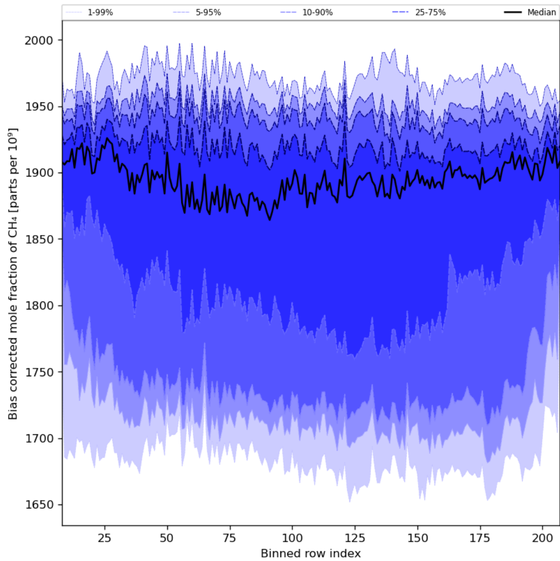
Figure 36: Along track statistics of “Bias corrected mole fraction of CH 4 ” for 2023-11-20 to 2023-11-22
