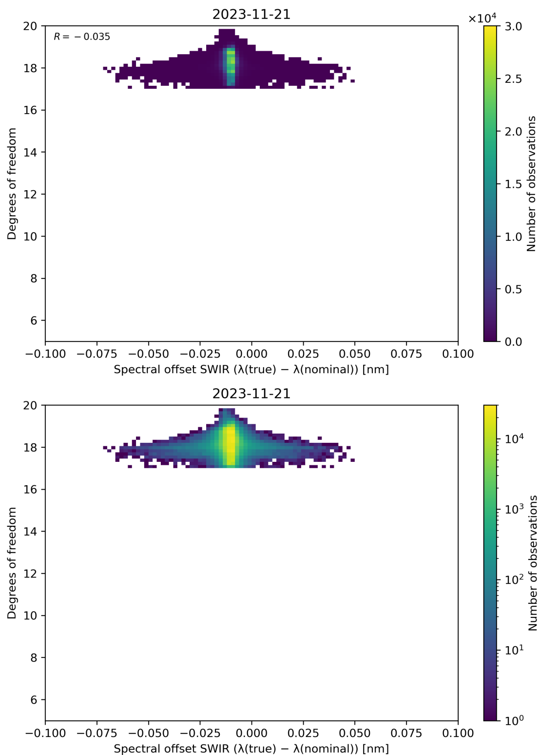
Figure 119: Scatter density plot of “Spectral offset SWIR ( \lambda(\text{true}) - \lambda(\text{nominal}) )” against “Degrees of freedom” for 2023-11-20 to 2023-11-22.
