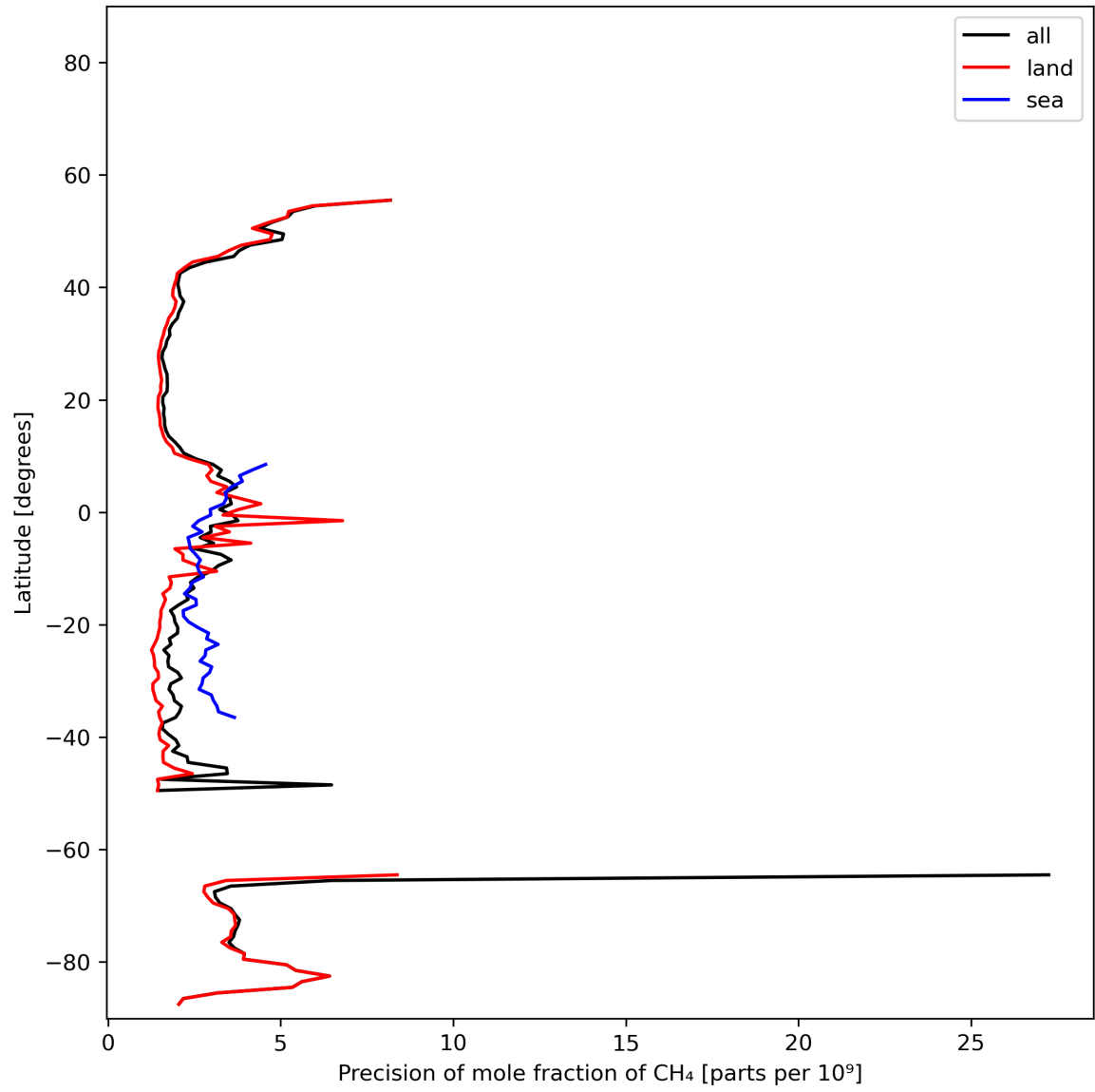
Figure 13: Zonal average of “Precision of mole fraction of CH 4 ” for 2023-11-20 to 2023-11-22.
