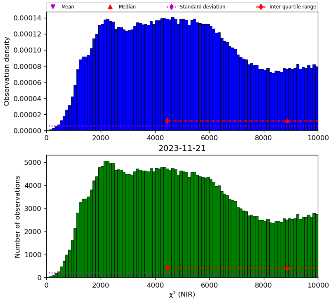
Figure 29: Histogram of “ \chi^2 (NIR)” for 2023-11-20 to 2023-11-22
