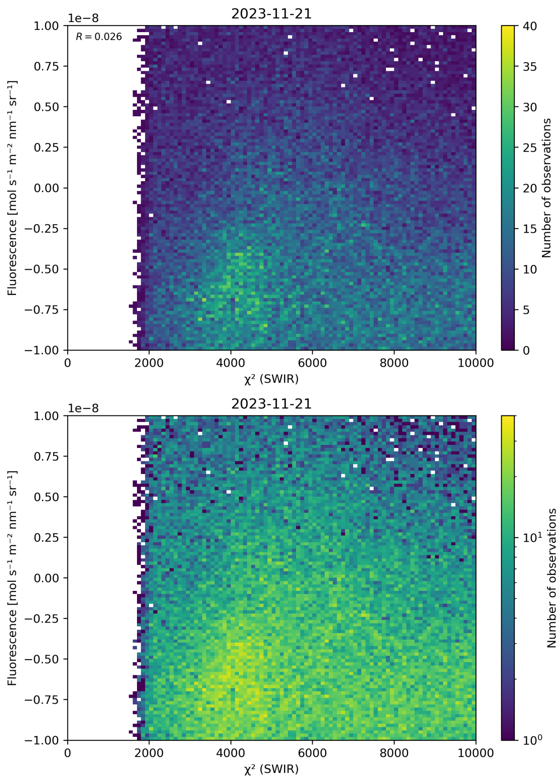
Figure 49: Scatter density plot of “ \chi^2 (SWIR)” against “Fluorescence” for 2023-11-20 to 2023-11-22.
