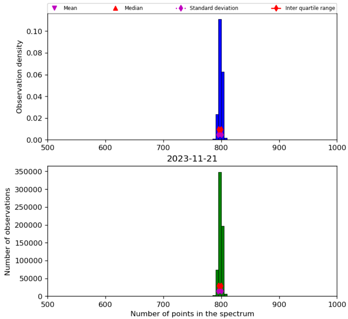
Figure 26: Histogram of “Number of points in the spectrum” for 2023-11-20 to 2023-11-22
