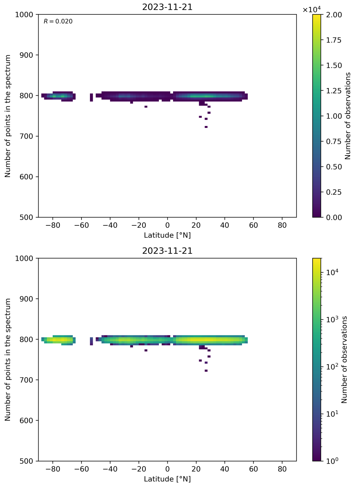
Figure 61: Scatter density plot of “Latitude” against “Number of points in the spectrum” for 2023-11-20 to 2023-11-22.
