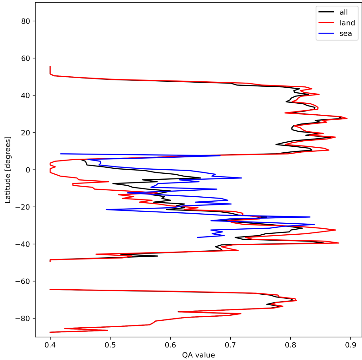
Figure 11: Zonal average of “QA value” for 2023-11-20 to 2023-11-22.
