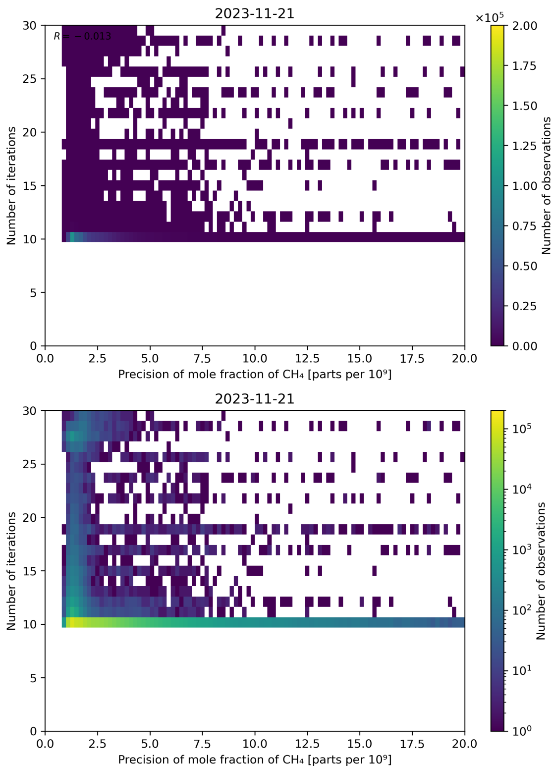
Figure 83: Scatter density plot of “Precision of mole fraction of CH 4 ” against “Number of iterations” for 2023-11-20 to 2023-11-22.
