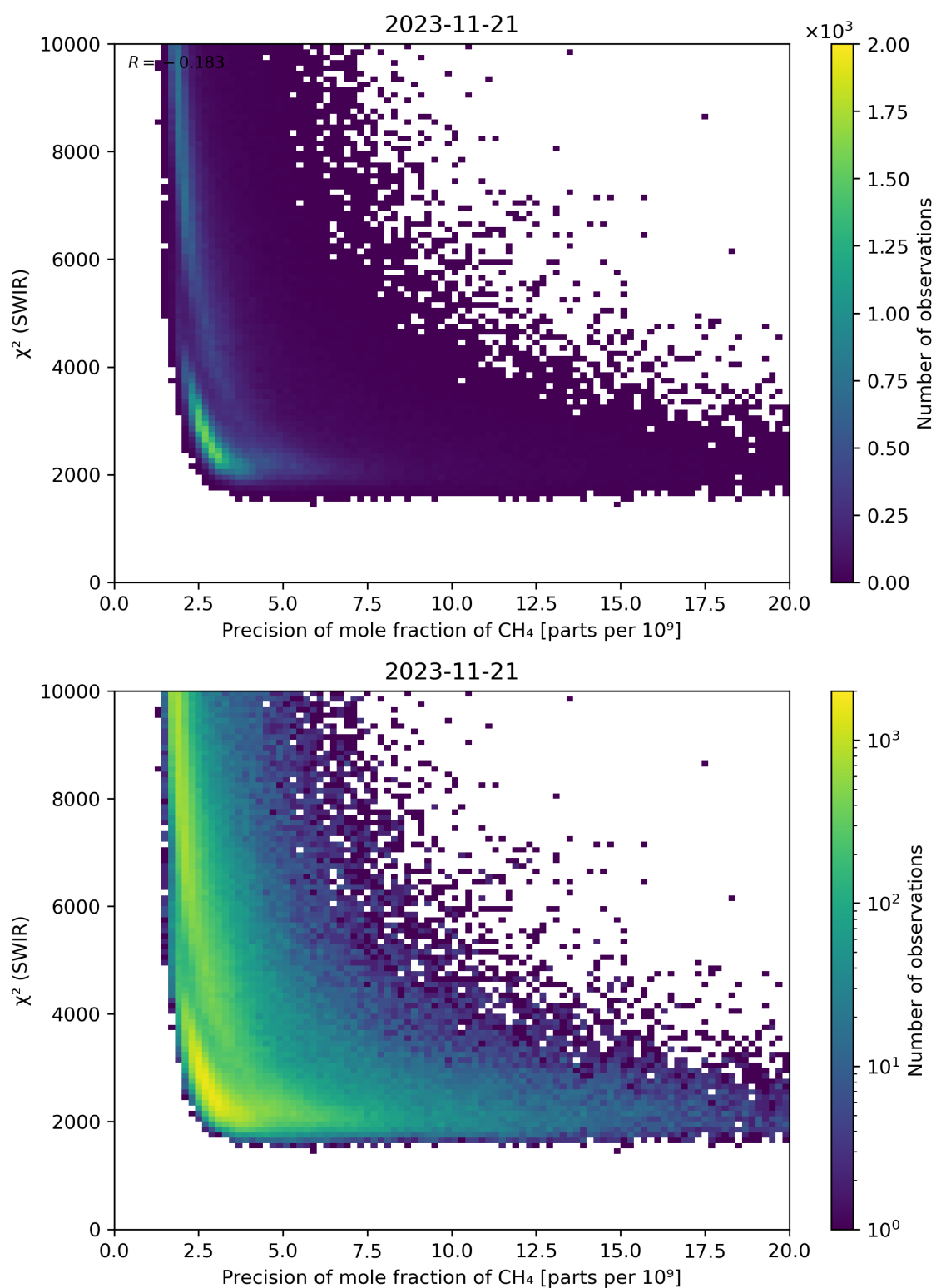
Figure 79: Scatter density plot of “Precision of mole fraction of \text{CH}_4 ” against “ \chi^2 (SWIR)” for 2023-11-20 to 2023-11-22.
