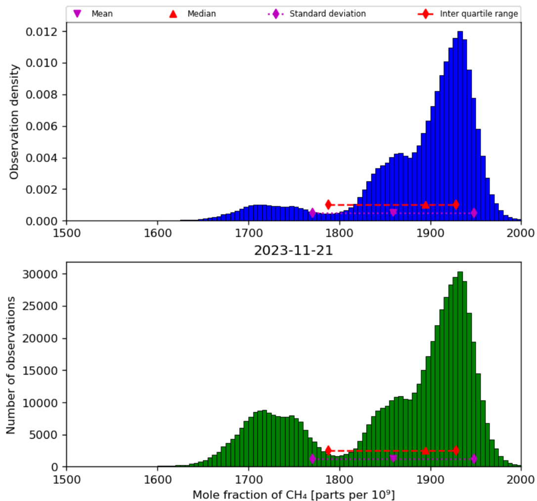
Figure 23: Histogram of “Mole fraction of CH 4 ” for 2023-11-20 to 2023-11-22
