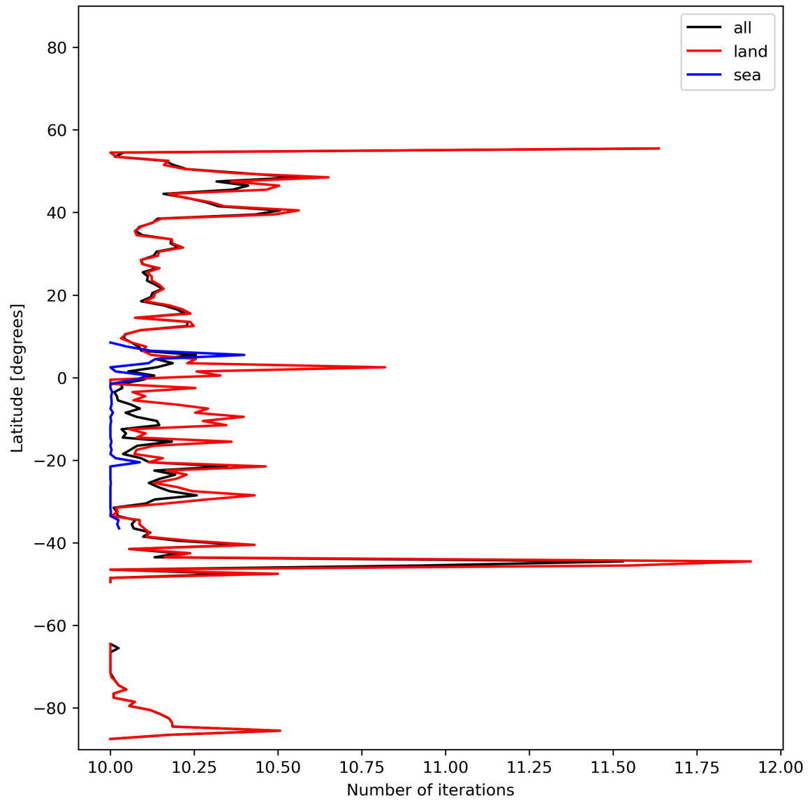
Figure 20: Zonal average of “Number of iterations” for 2023-11-20 to 2023-11-22.
