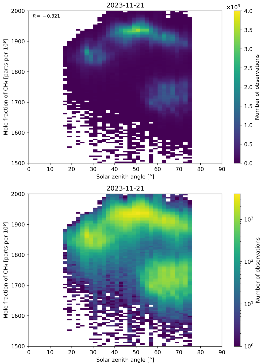
Figure 99: Scatter density plot of “Solar zenith angle” against “Mole fraction of CH 4 ” for 2023-11-20 to 2023-11-22.
