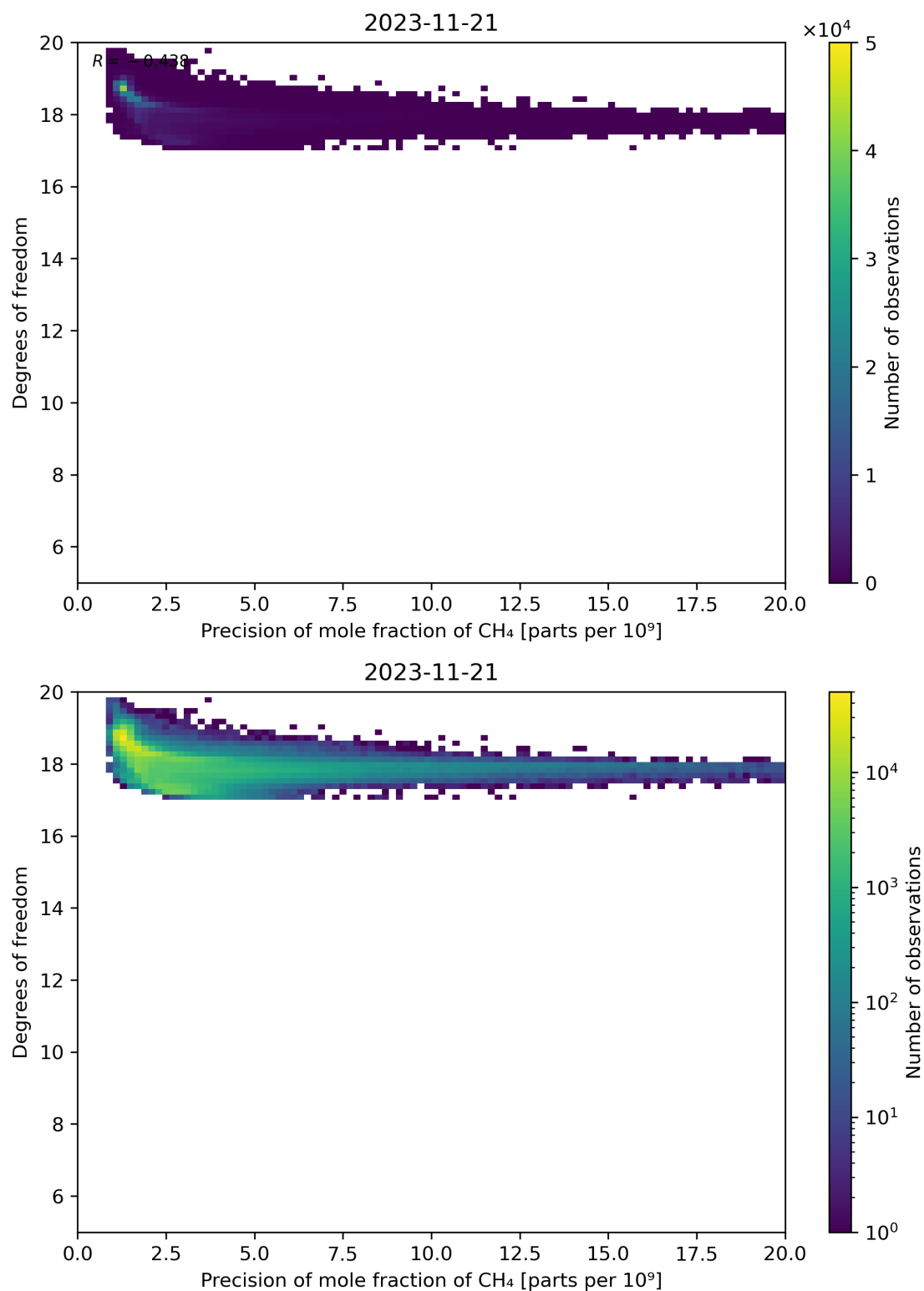
Figure 80: Scatter density plot of “Precision of mole fraction of \text{CH}_4 ” against “Degrees of freedom” for 2023-11-20 to 2023-11-22.
