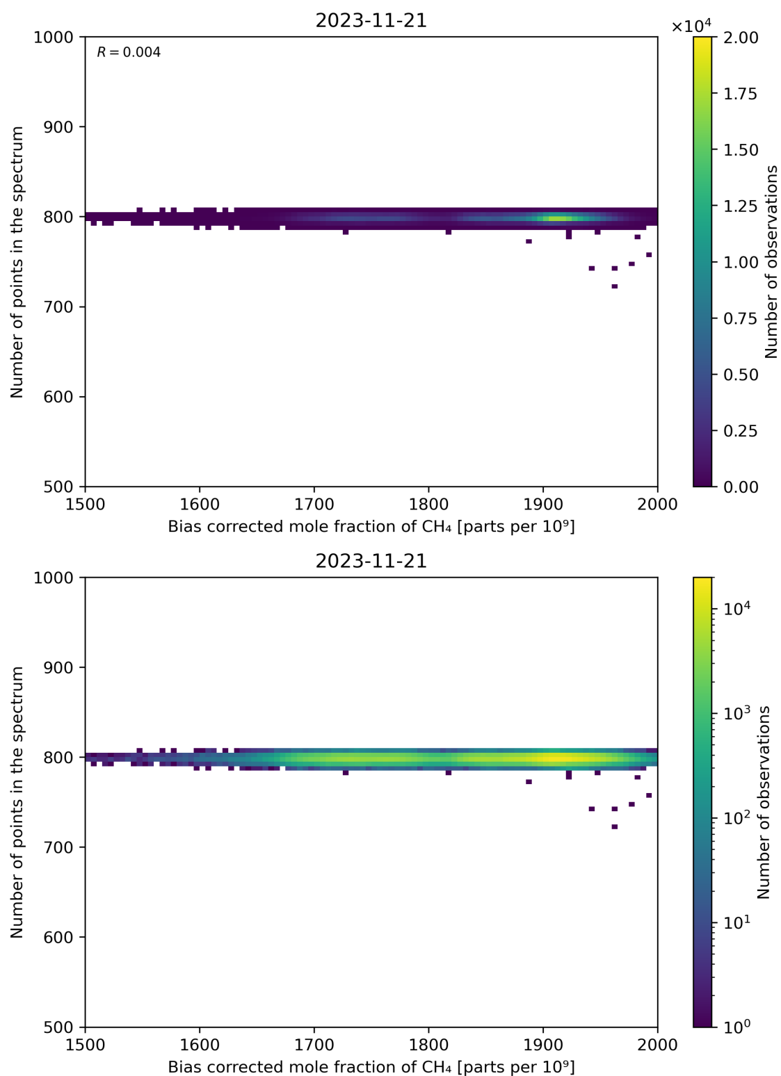
Figure 68: Scatter density plot of “Bias corrected mole fraction of CH 4 ” against “Number of points in the spectrum” for 2023-11-20 to 2023-11-22.
