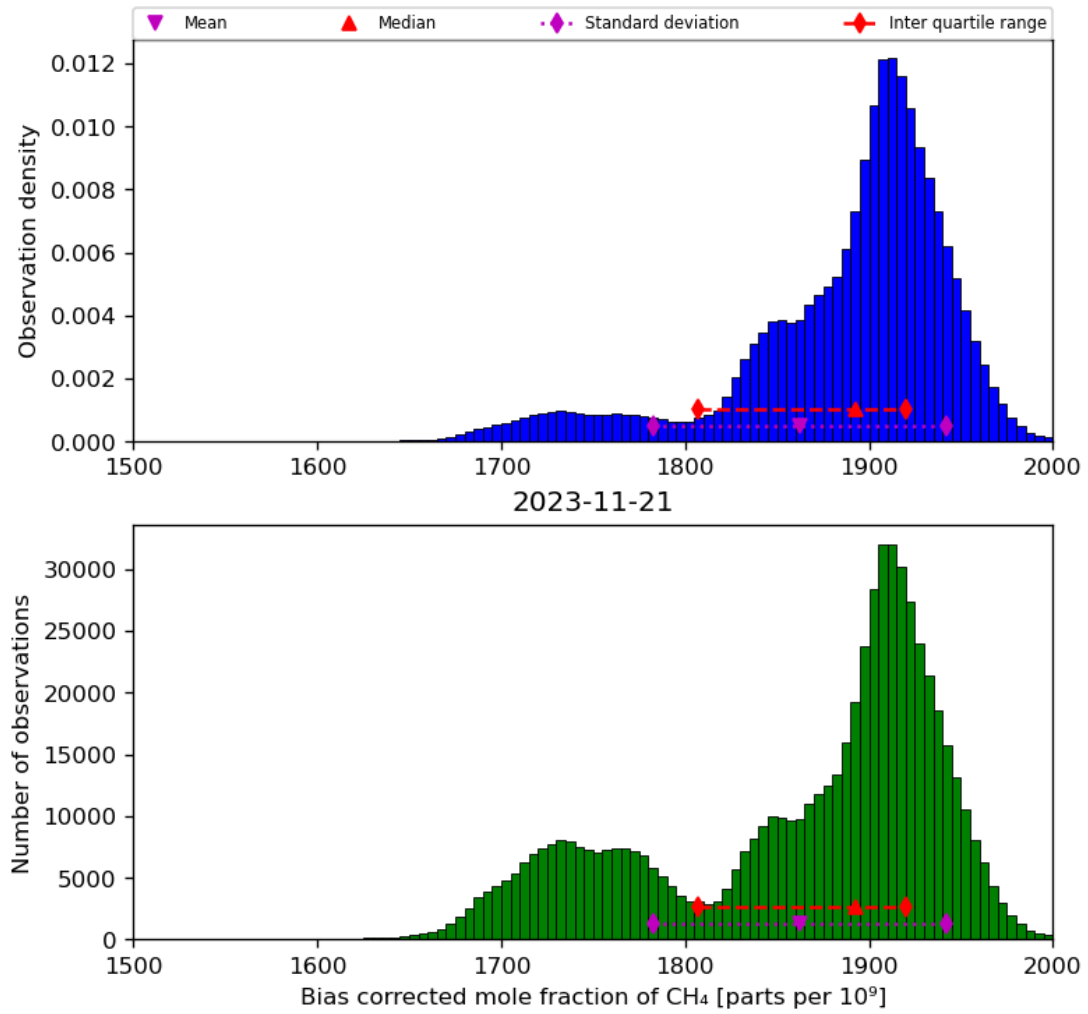
Figure 25: Histogram of “Bias corrected mole fraction of CH 4 ” for 2023-11-20 to 2023-11-22
