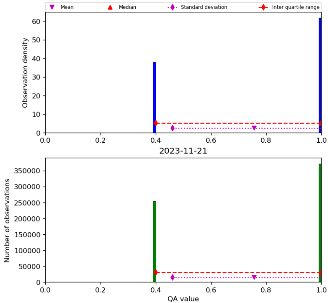
Figure 22: Histogram of “QA value” for 2023-11-20 to 2023-11-22
