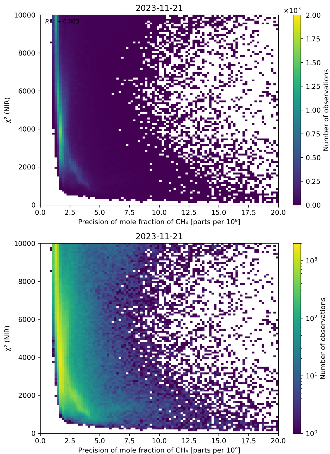
Figure 78: Scatter density plot of “Precision of mole fraction of \text{CH}_4 ” against “ \chi^2 (NIR)” for 2023-11-20 to 2023-11-22.
