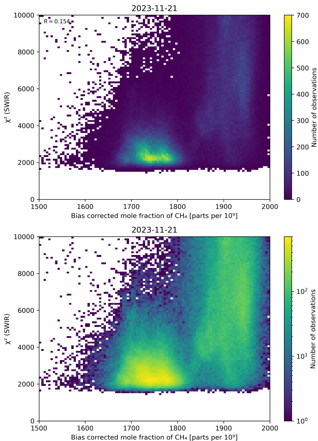
Figure 64: Scatter density plot of “Bias corrected mole fraction of \text{CH}_4 ” against “ \chi^2 (SWIR)” for 2023-11-20 to 2023-11-22.
