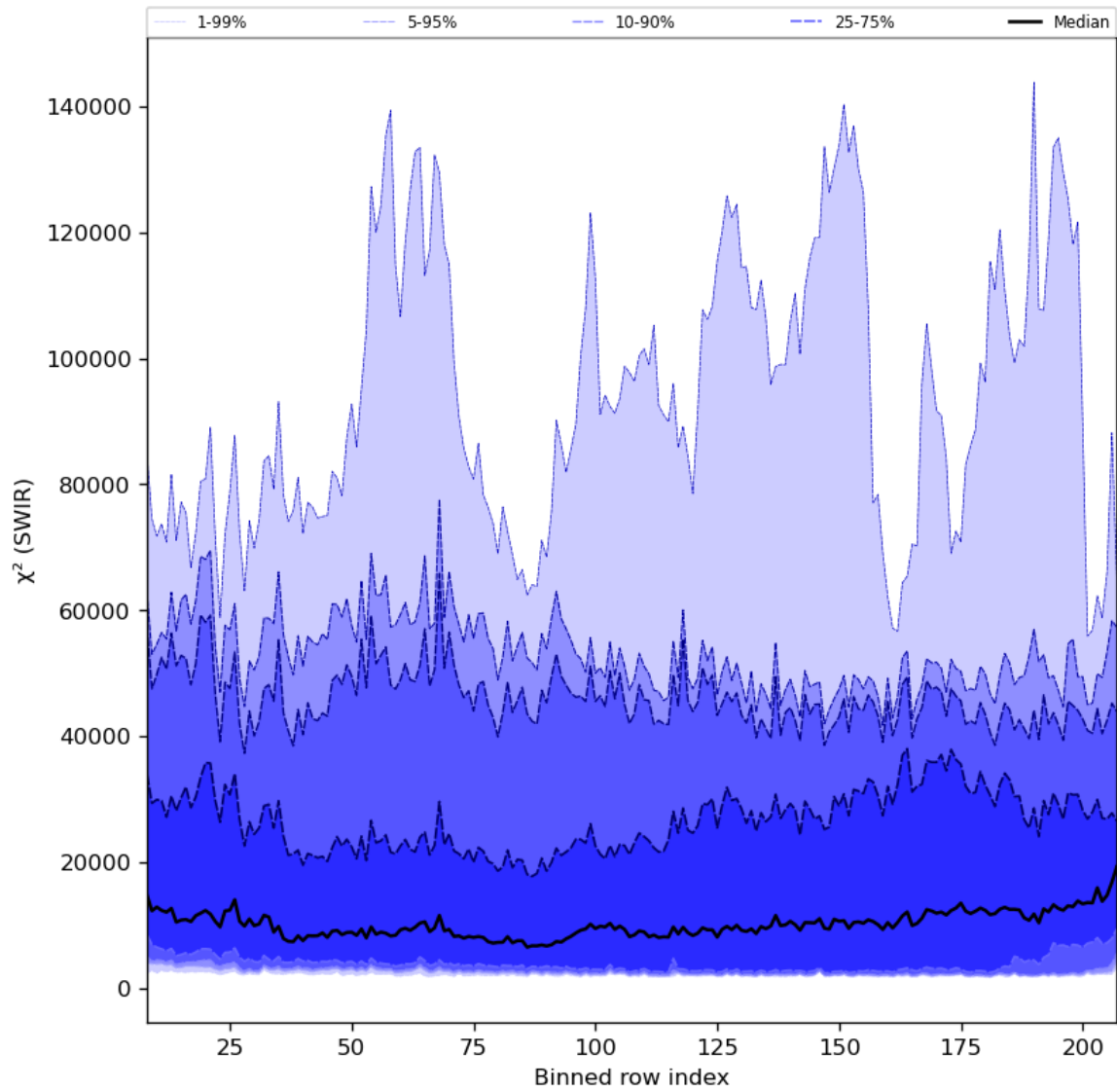
Figure 39: Along track statistics of “ \chi^2 (SWIR)” for 2023-11-20 to 2023-11-22
