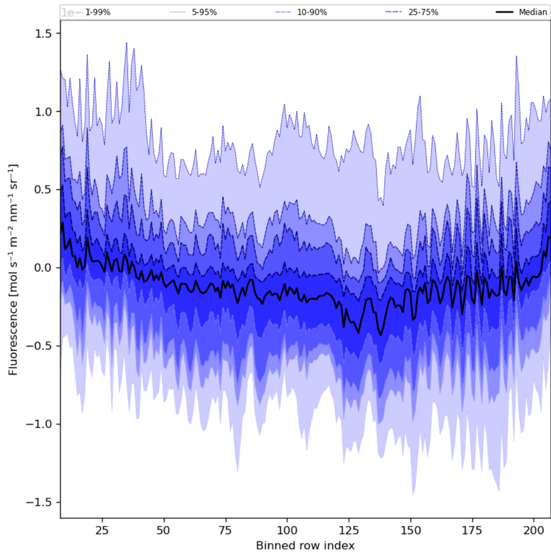
Figure 43: Along track statistics of “Fluorescence” for 2023-11-20 to 2023-11-22
