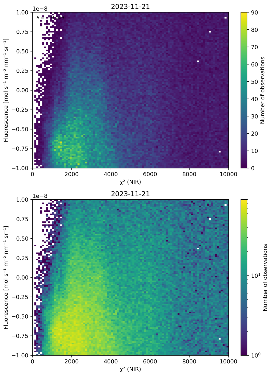
Figure 45: Scatter density plot of “ \chi^2 (NIR)” against “Fluorescence” for 2023-11-20 to 2023-11-22.
