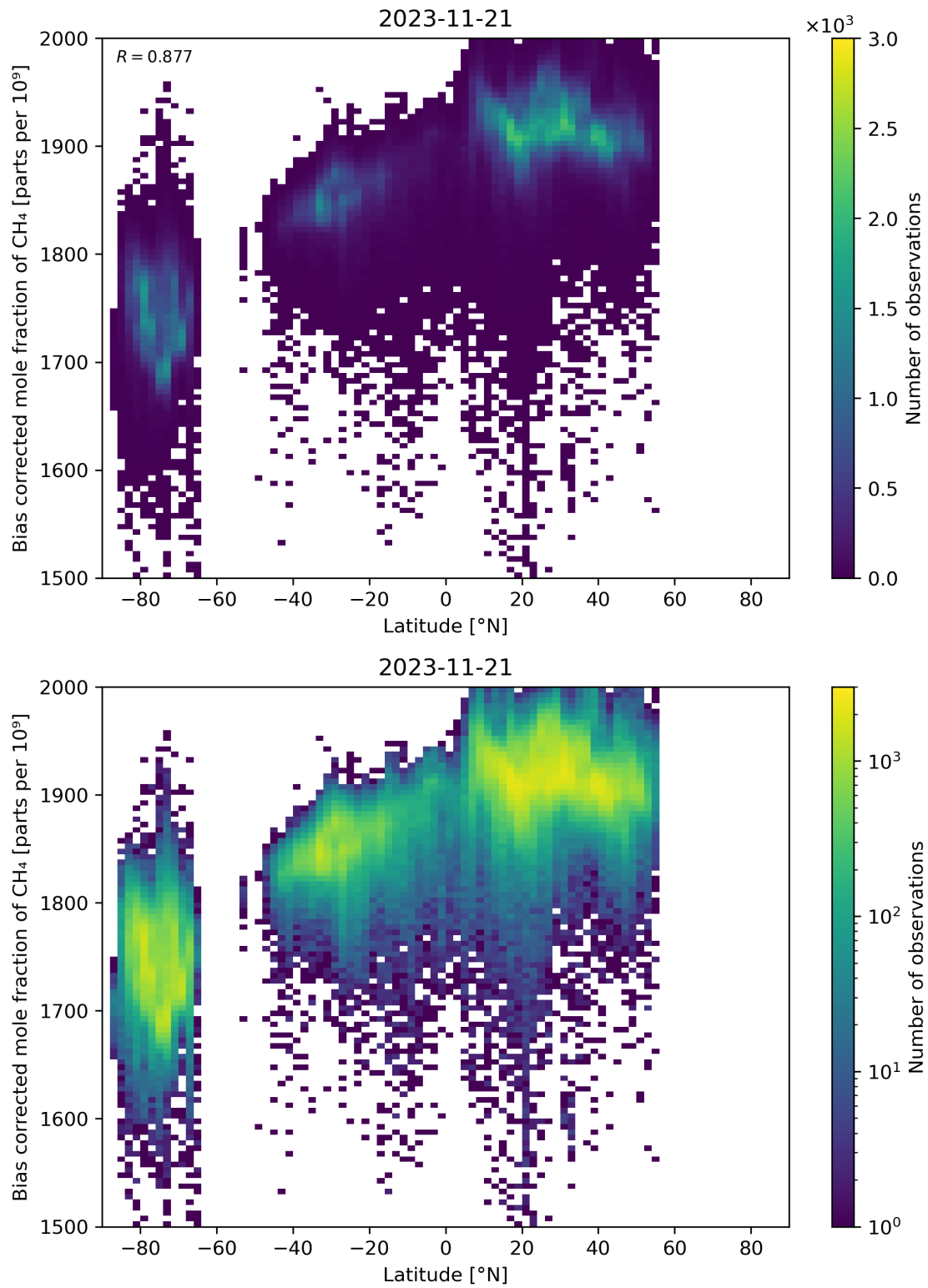
Figure 58: Scatter density plot of “Latitude” against “Bias corrected mole fraction of CH 4 ” for 2023-11-20 to 2023-11-22.
