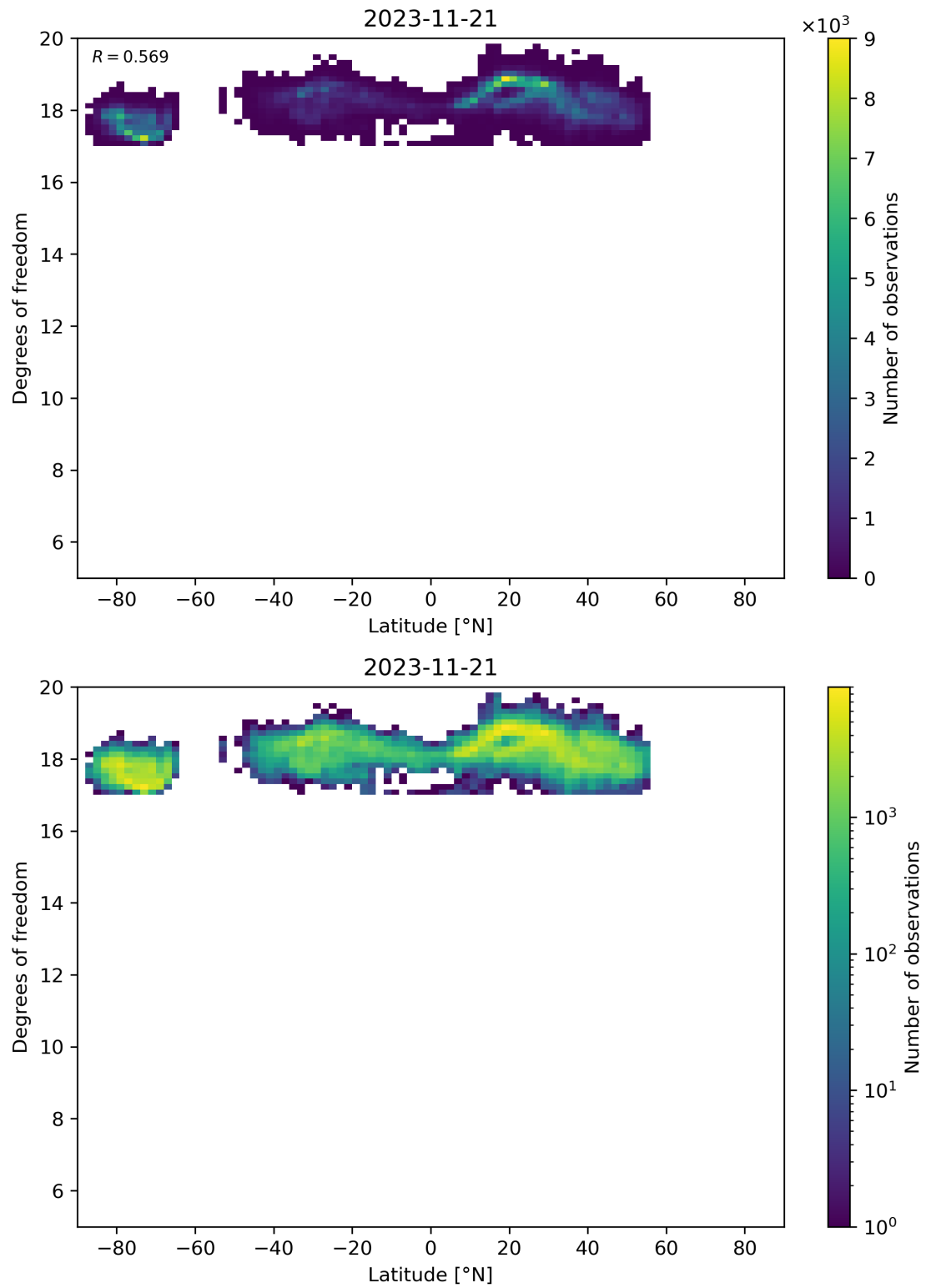
Figure 55: Scatter density plot of “Latitude” against “Degrees of freedom” for 2023-11-20 to 2023-11-22.
