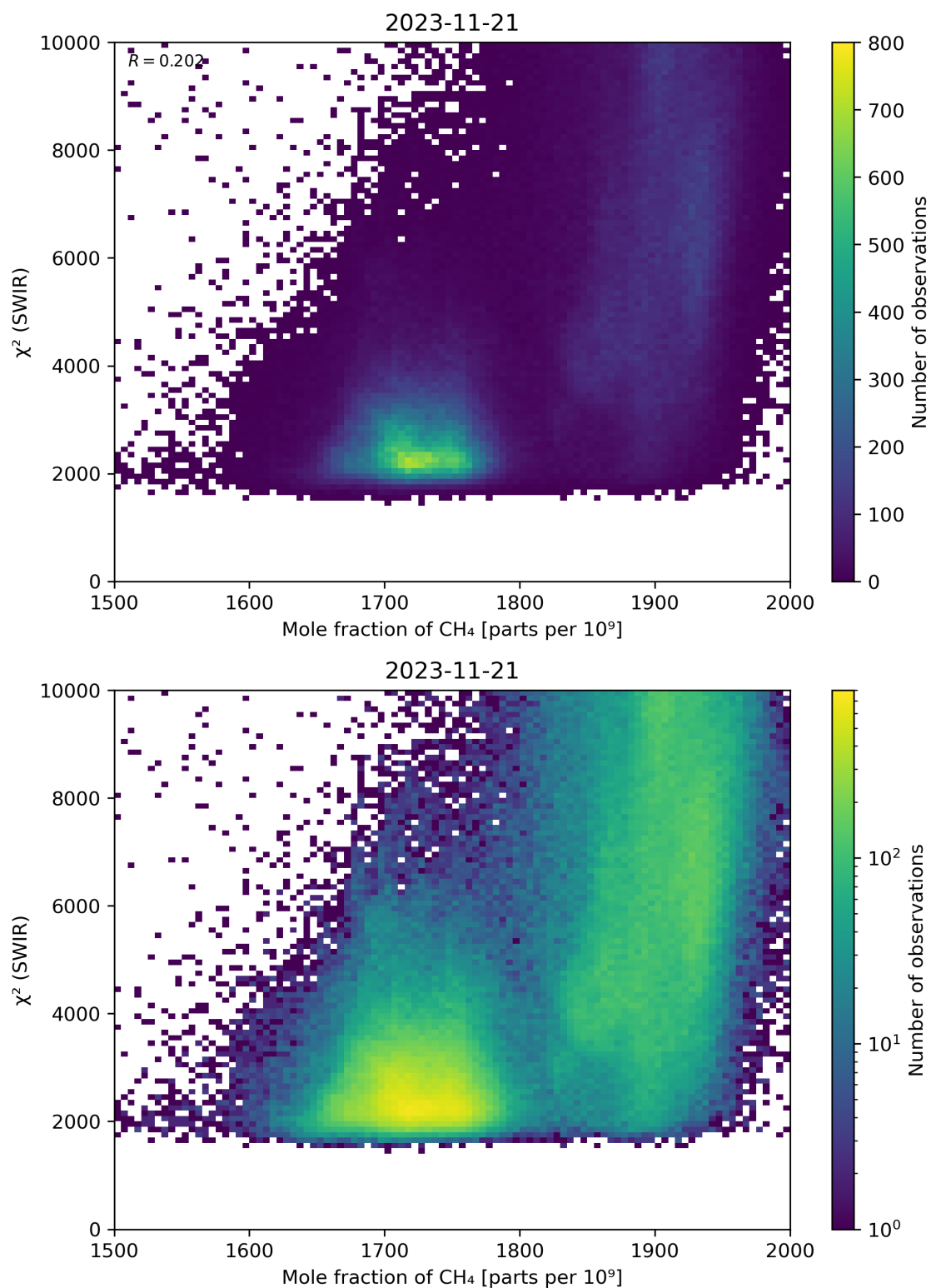
Figure 71: Scatter density plot of “Mole fraction of \text{CH}_4 ” against “ \chi^2 (SWIR)” for 2023-11-20 to 2023-11-22.
