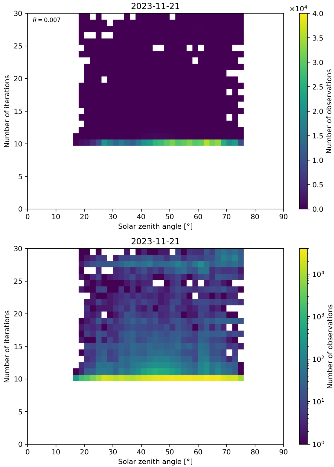
Figure 102: Scatter density plot of “Solar zenith angle” against “Number of iterations” for 2023-11-20 to 2023-11-22.
