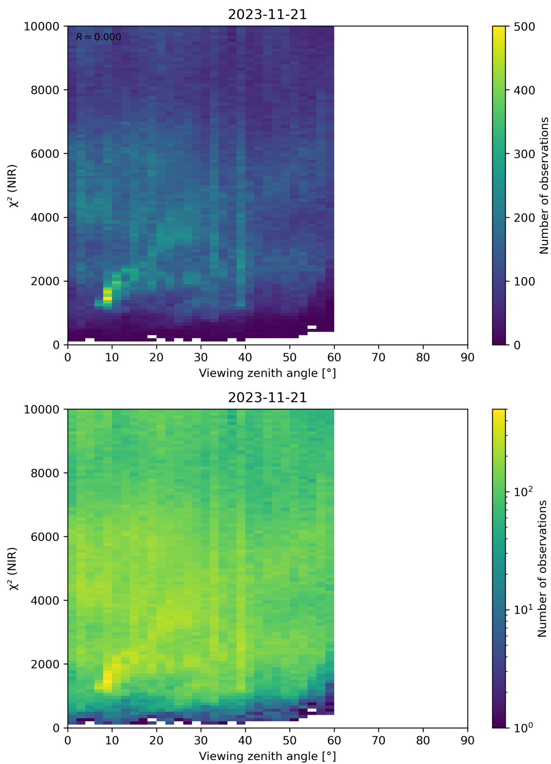
Figure 105: Scatter density plot of “Viewing zenith angle” against “ \chi^2 (NIR)” for 2023-11-20 to 2023-11-22.
