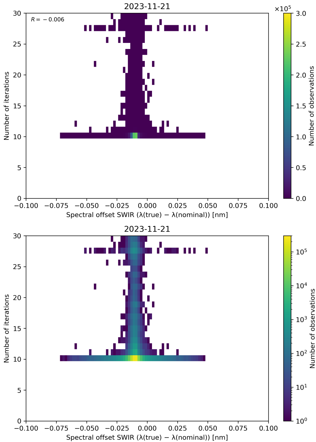
Figure 121: Scatter density plot of “Spectral offset SWIR ( \lambda(\text{true}) - \lambda(\text{nominal}) )” against “Number of iterations” for 2023-11-20 to 2023-11-22.
