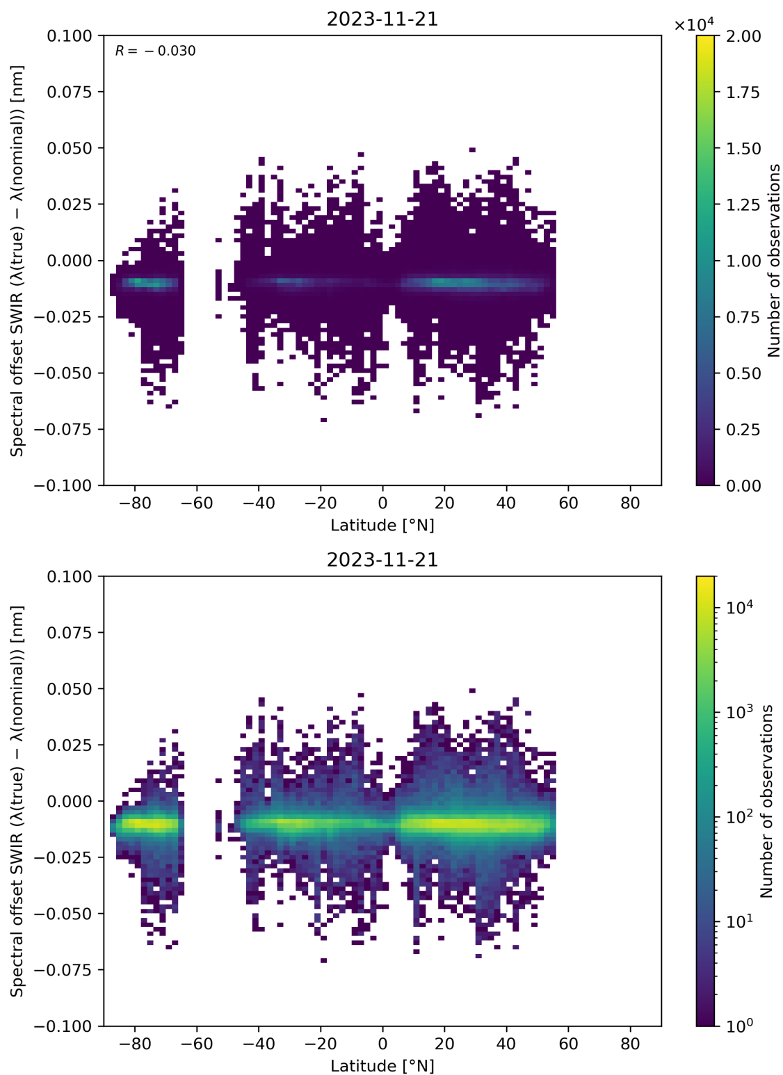
Figure 62: Scatter density plot of “Latitude” against “Spectral offset SWIR ( \lambda(\text{true}) - \lambda(\text{nominal}) )” for 2023-11-20 to 2023-11-22.
