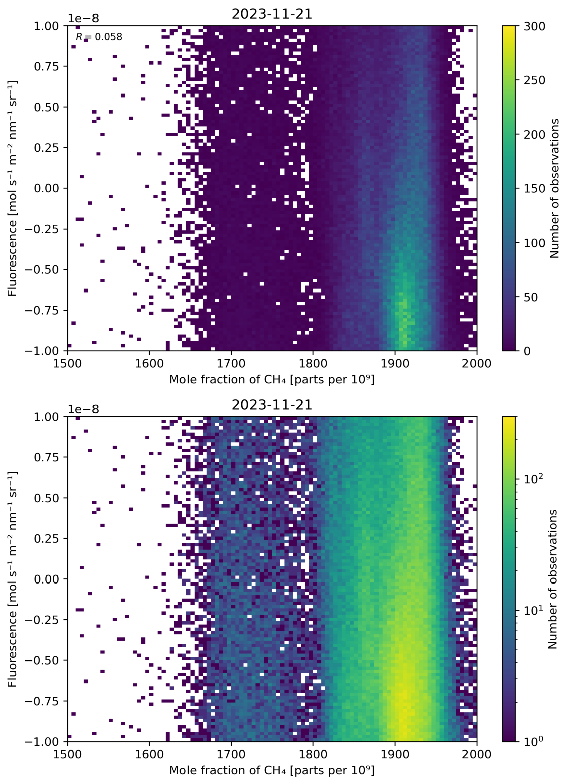
Figure 73: Scatter density plot of “Mole fraction of \text{CH}_4 ” against “Fluorescence” for 2023-11-20 to 2023-11-22.
