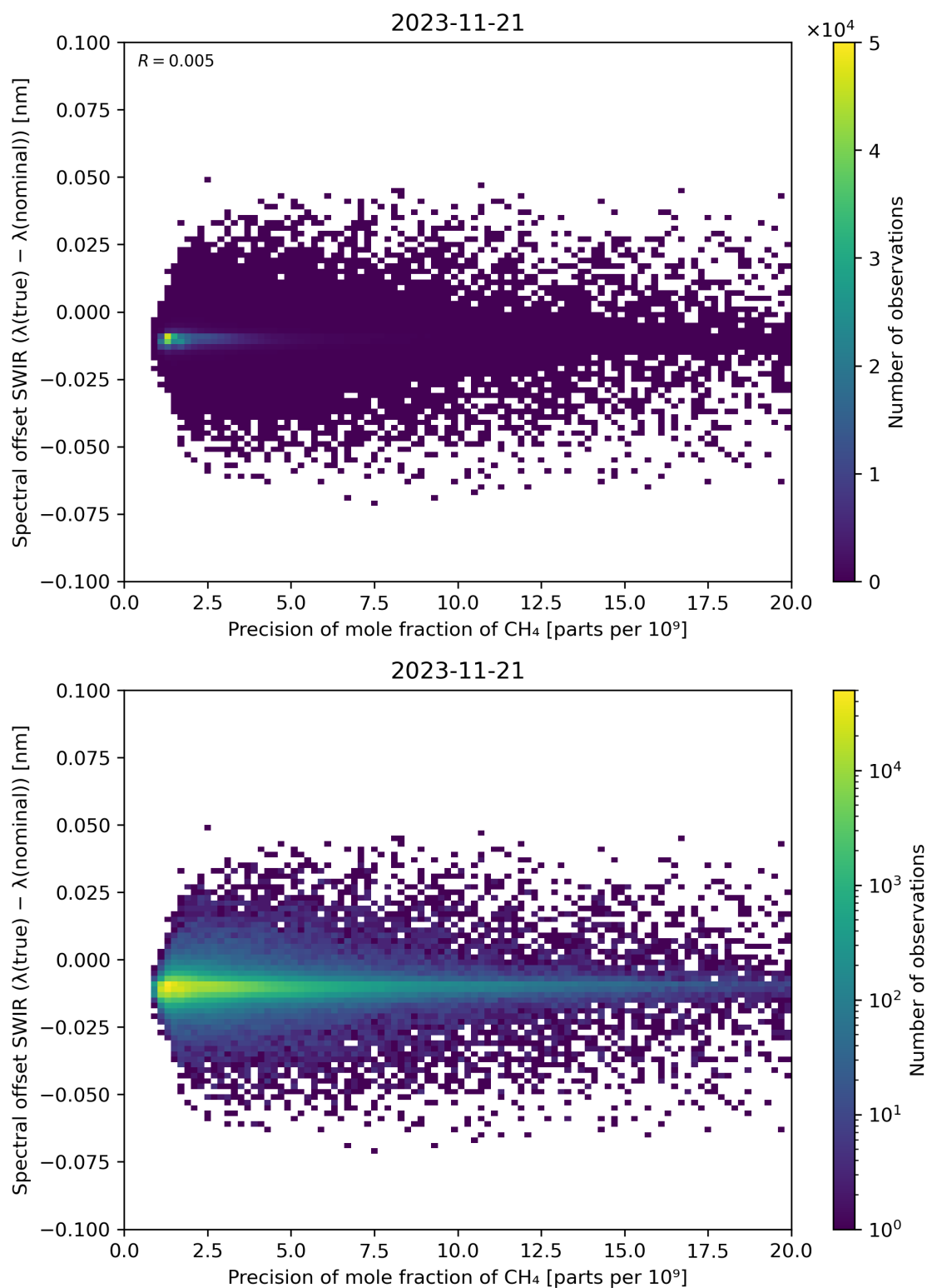
Figure 85: Scatter density plot of “Precision of mole fraction of \text{CH}_4 ” against “Spectral offset SWIR ( \lambda(\text{true}) - \lambda(\text{nominal}) )” for 2023-11-20 to 2023-11-22.
