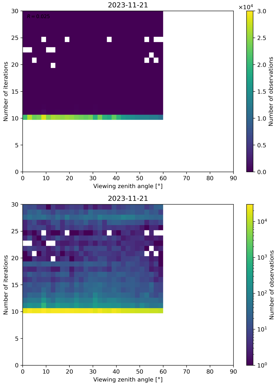
Figure 113: Scatter density plot of “Viewing zenith angle” against “Number of iterations” for 2023-11-20 to 2023-11-22.
