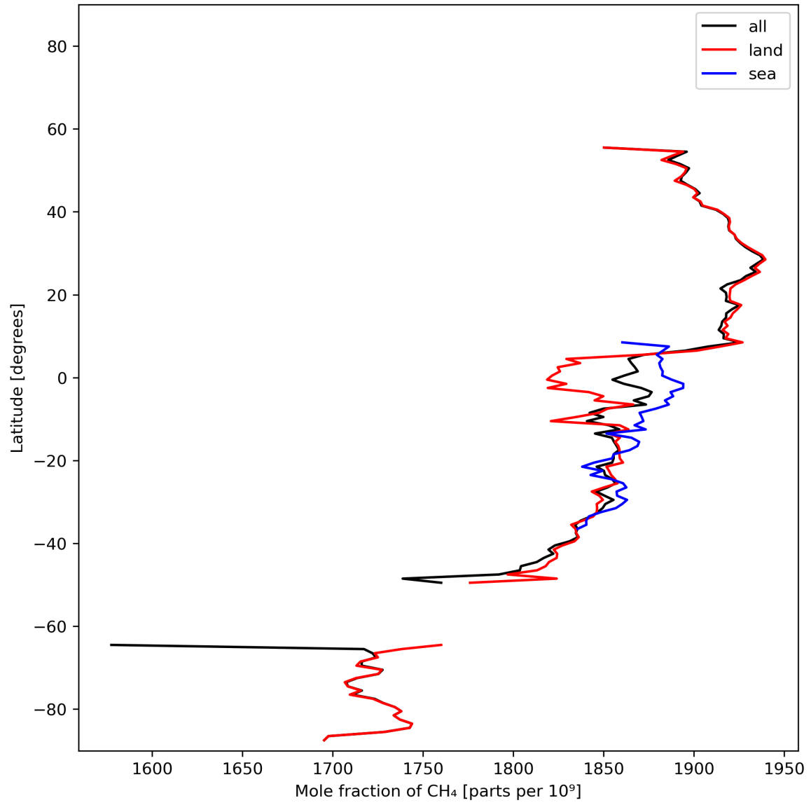
Figure 12: Zonal average of “Mole fraction of CH 4 ” for 2023-11-20 to 2023-11-22.
