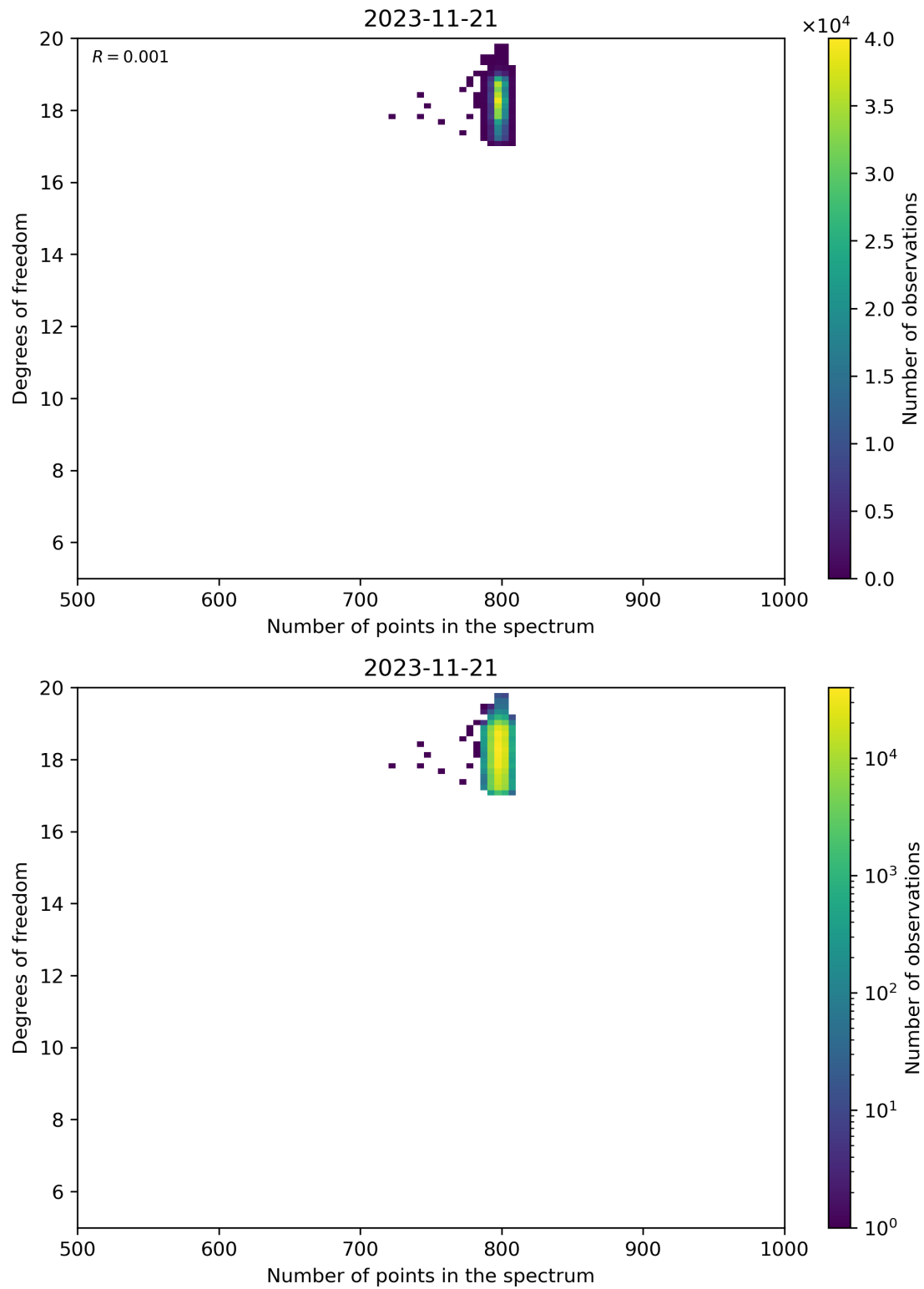
Figure 90: Scatter density plot of “Number of points in the spectrum” against “Degrees of freedom” for 2023-11-20 to 2023-11-22.
