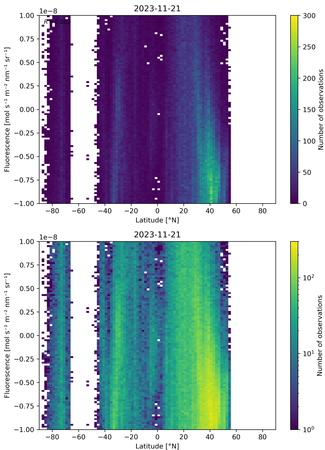
Figure 56: Scatter density plot of “Latitude” against “Fluorescence” for 2023-11-20 to 2023-11-22.
