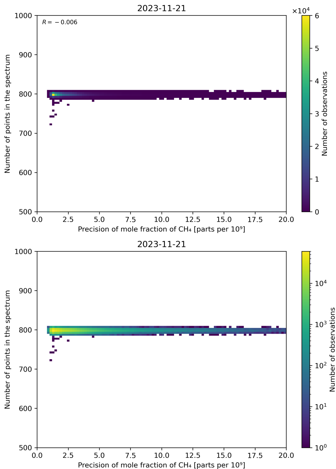
Figure 84: Scatter density plot of “Precision of mole fraction of CH 4 ” against “Number of points in the spectrum” for 2023-11-20 to 2023-11-22.
