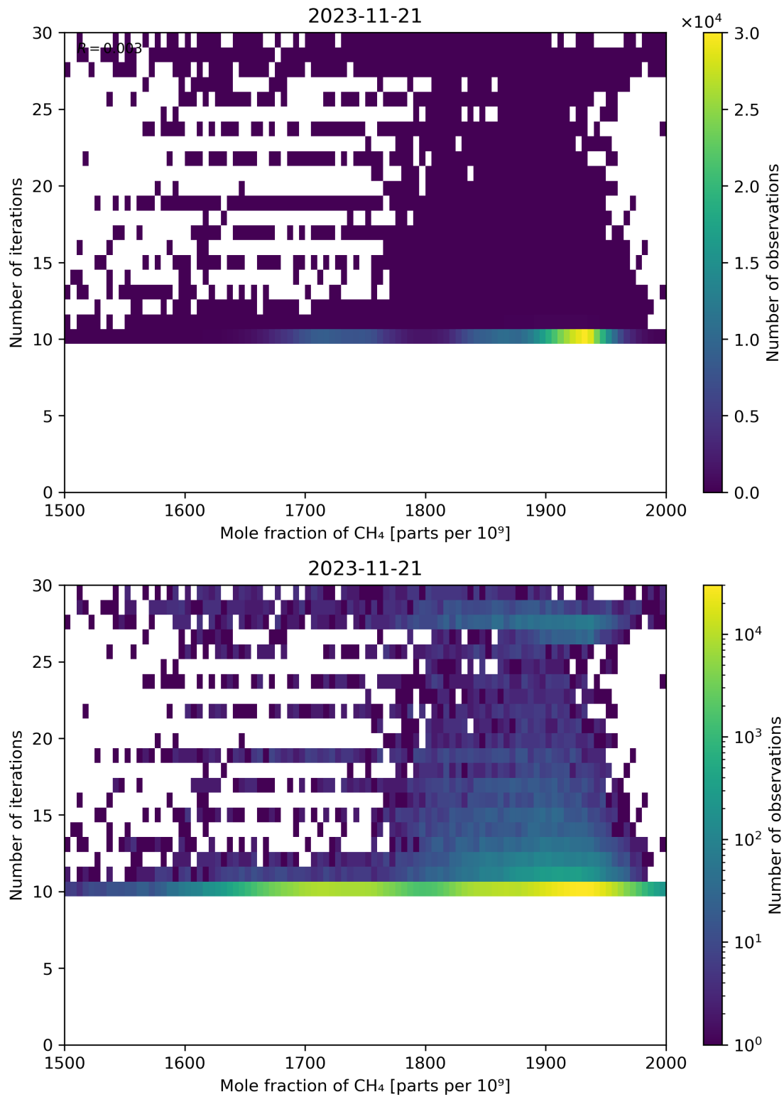
Figure 76: Scatter density plot of “Mole fraction of CH 4 ” against “Number of iterations” for 2023-11-20 to 2023-11-22.
