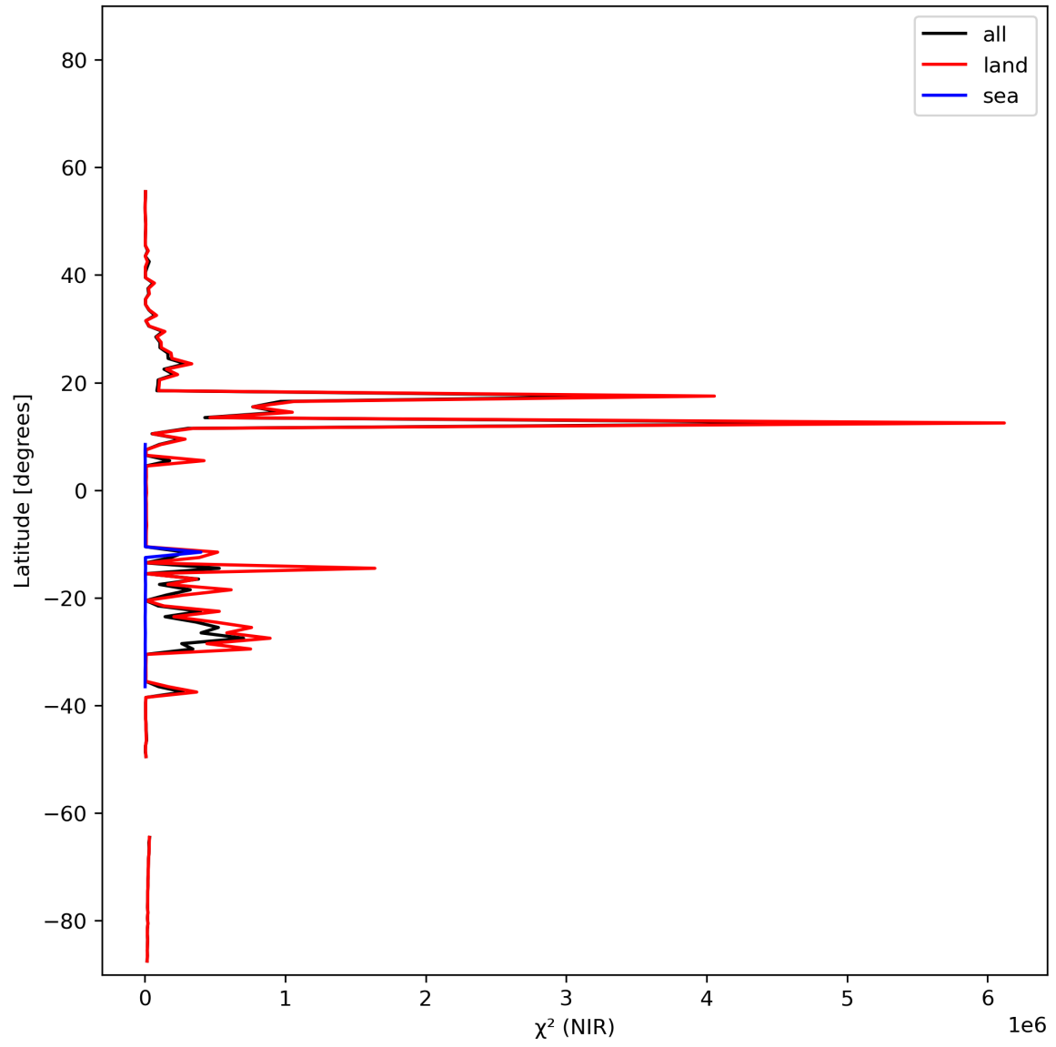
Figure 18: Zonal average of “ \chi^2 (NIR)” for 2023-11-20 to 2023-11-22.
