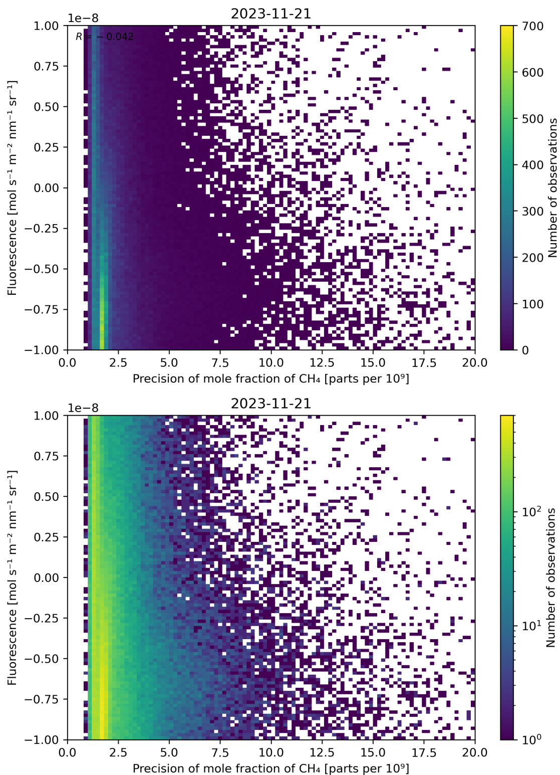
Figure 81: Scatter density plot of “Precision of mole fraction of \text{CH}_4 ” against “Fluorescence” for 2023-11-20 to 2023-11-22.
