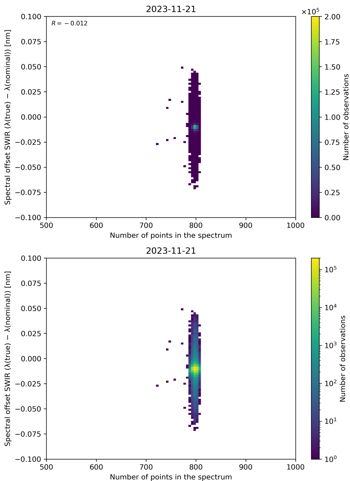
Figure 93: Scatter density plot of “Number of points in the spectrum” against “Spectral offset SWIR ( \lambda(\text{true}) - \lambda(\text{nominal}) )” for 2023-11-20 to 2023-11-22.
