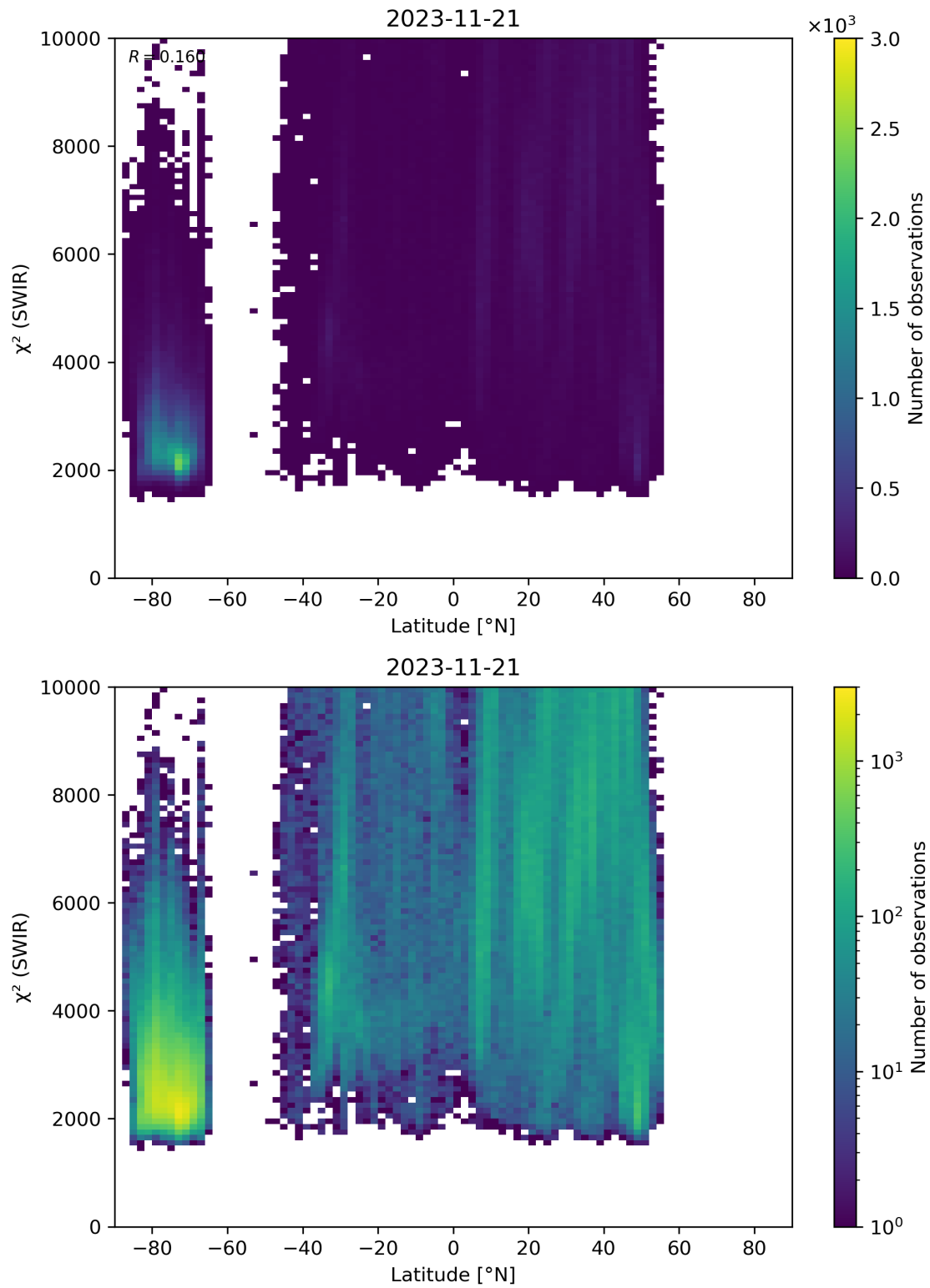
Figure 54: Scatter density plot of “Latitude” against “ \chi^2 (SWIR)” for 2023-11-20 to 2023-11-22.
