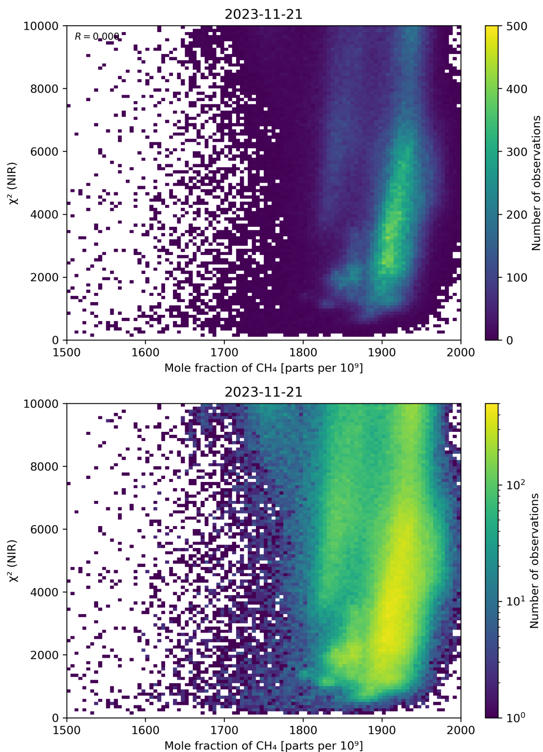
Figure 70: Scatter density plot of “Mole fraction of \text{CH}_4 ” against “ \chi^2 (NIR)” for 2023-11-20 to 2023-11-22.
