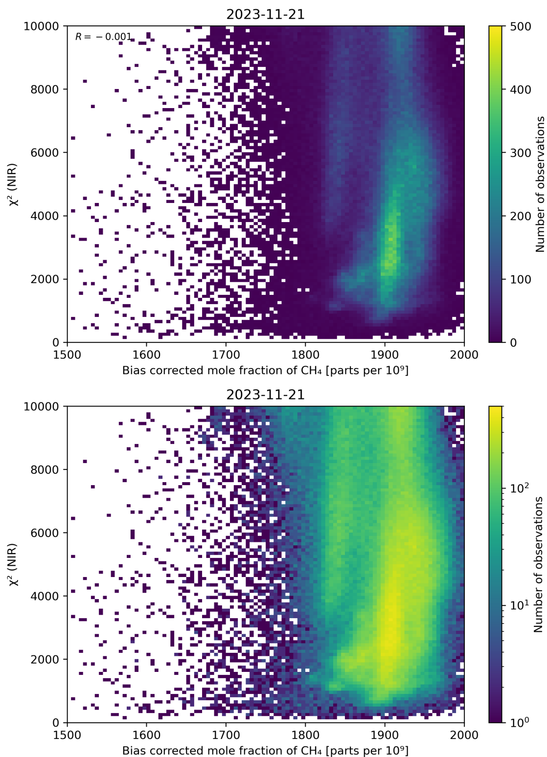
Figure 63: Scatter density plot of “Bias corrected mole fraction of CH 4 ” against “ \chi^2 (NIR)” for 2023-11-20 to 2023-11-22.
