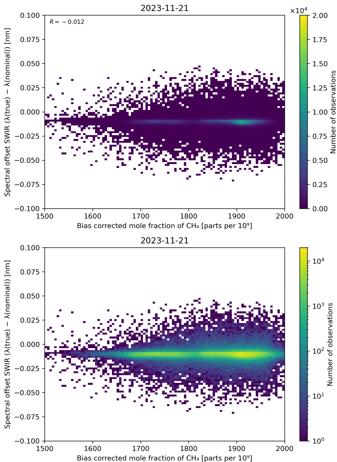
Figure 69: Scatter density plot of “Bias corrected mole fraction of \text{CH}_4 ” against “Spectral offset SWIR ( \lambda(\text{true}) - \lambda(\text{nominal}) )” for 2023-11-20 to 2023-11-22.
