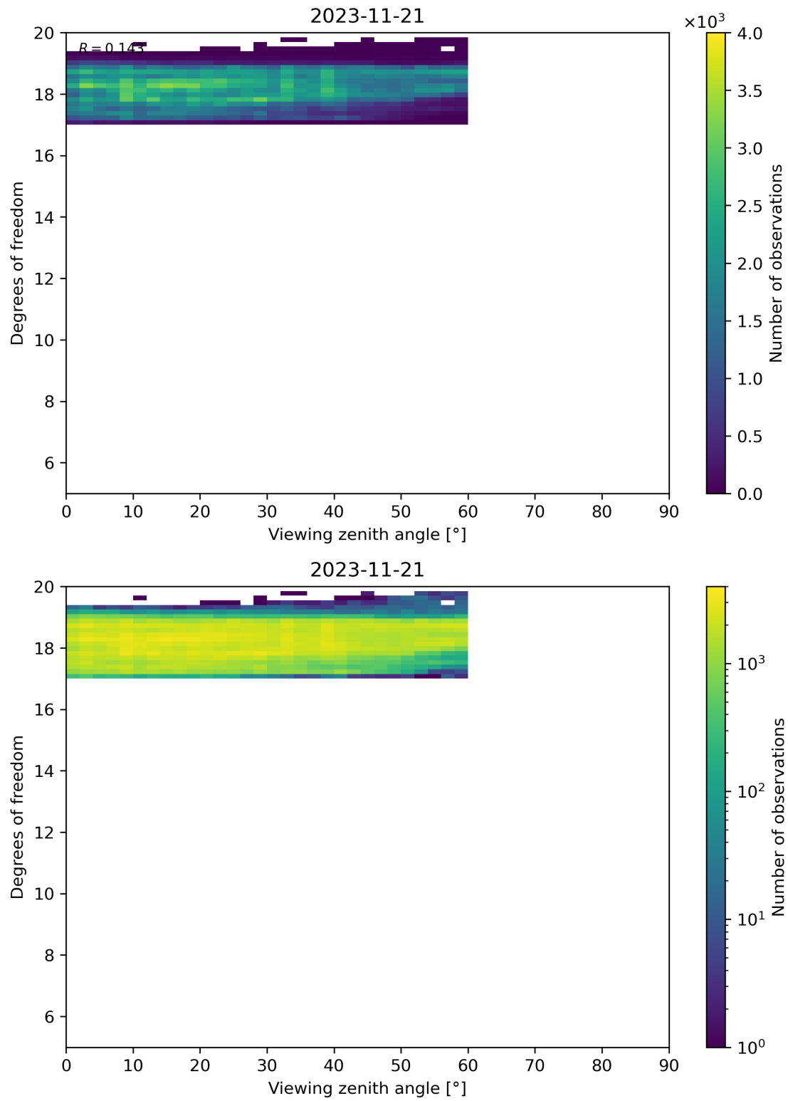
Figure 107: Scatter density plot of “Viewing zenith angle” against “Degrees of freedom” for 2023-11-20 to 2023-11-22.
