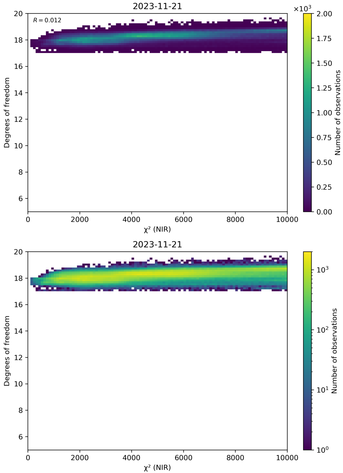
Figure 44: Scatter density plot of “ \chi^2 (NIR)” against “Degrees of freedom” for 2023-11-20 to 2023-11-22.
