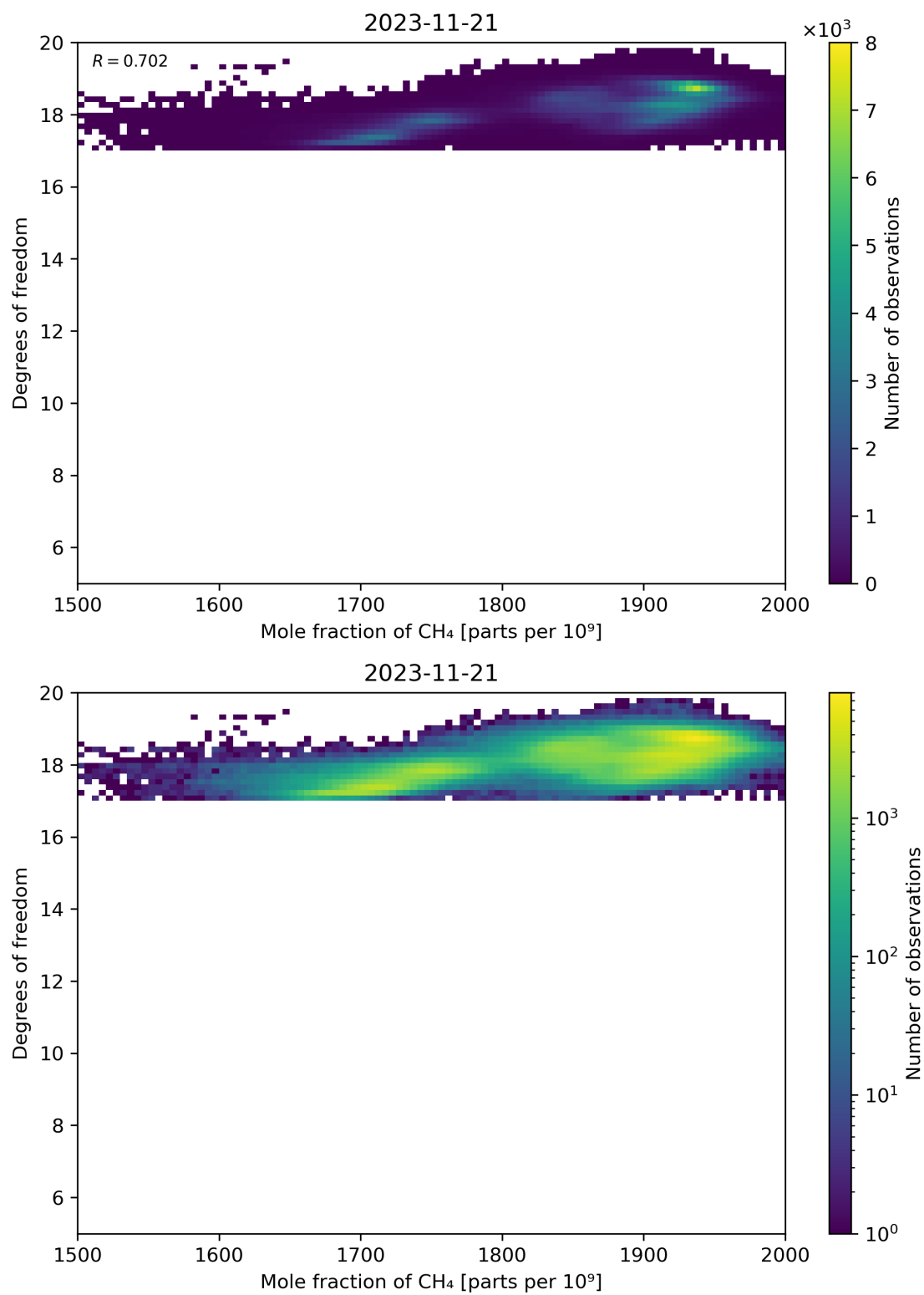
Figure 72: Scatter density plot of “Mole fraction of CH 4 ” against “Degrees of freedom” for 2023-11-20 to 2023-11-22.
