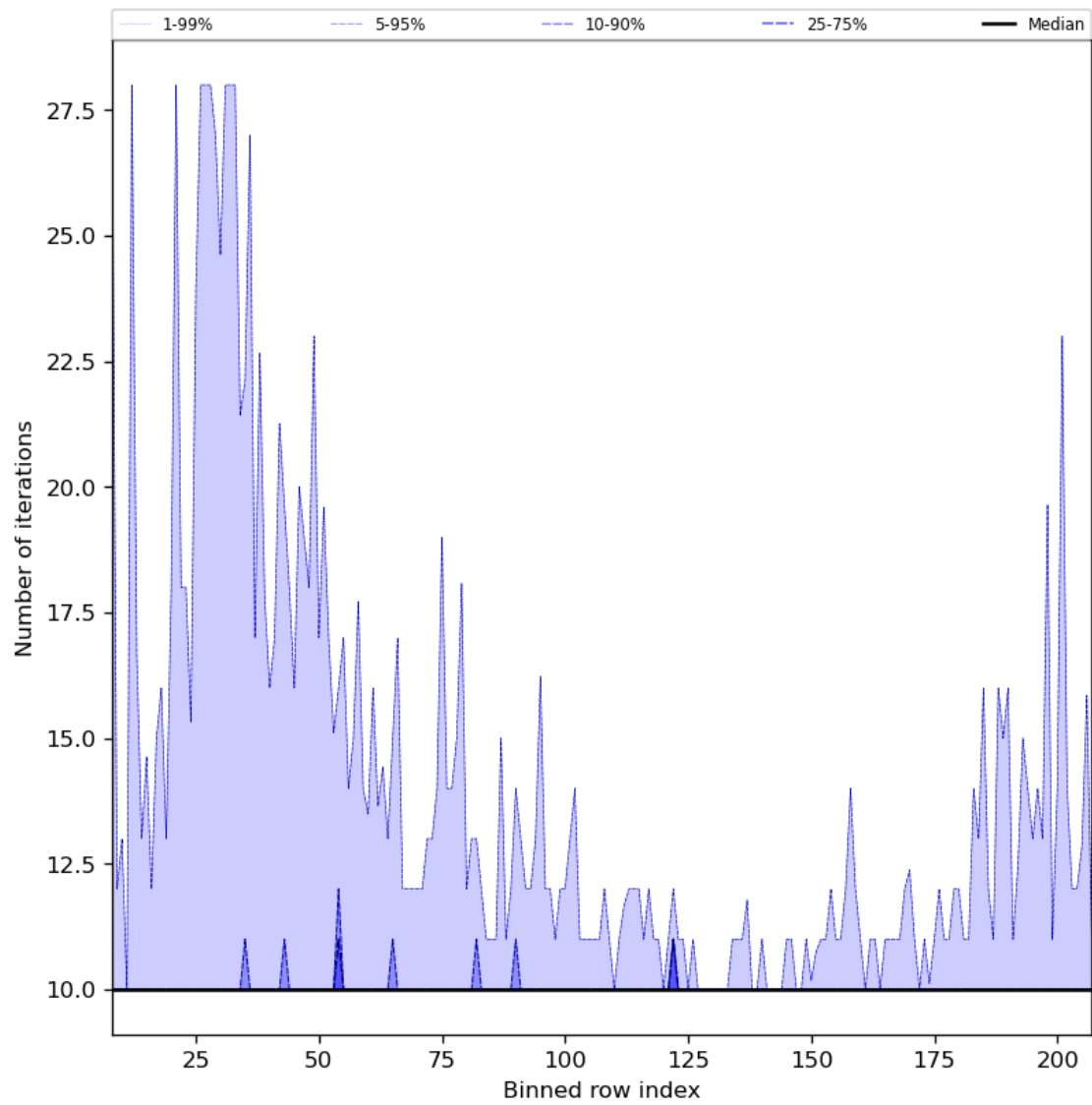
Figure 42: Along track statistics of “Number of iterations” for 2023-11-20 to 2023-11-22
