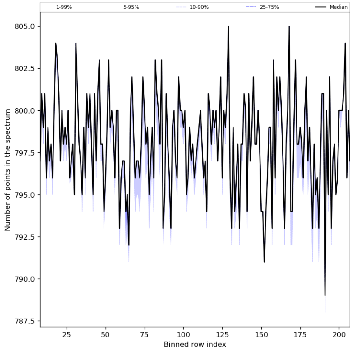
Figure 37: Along track statistics of “Number of points in the spectrum” for 2023-11-20 to 2023-11-22
