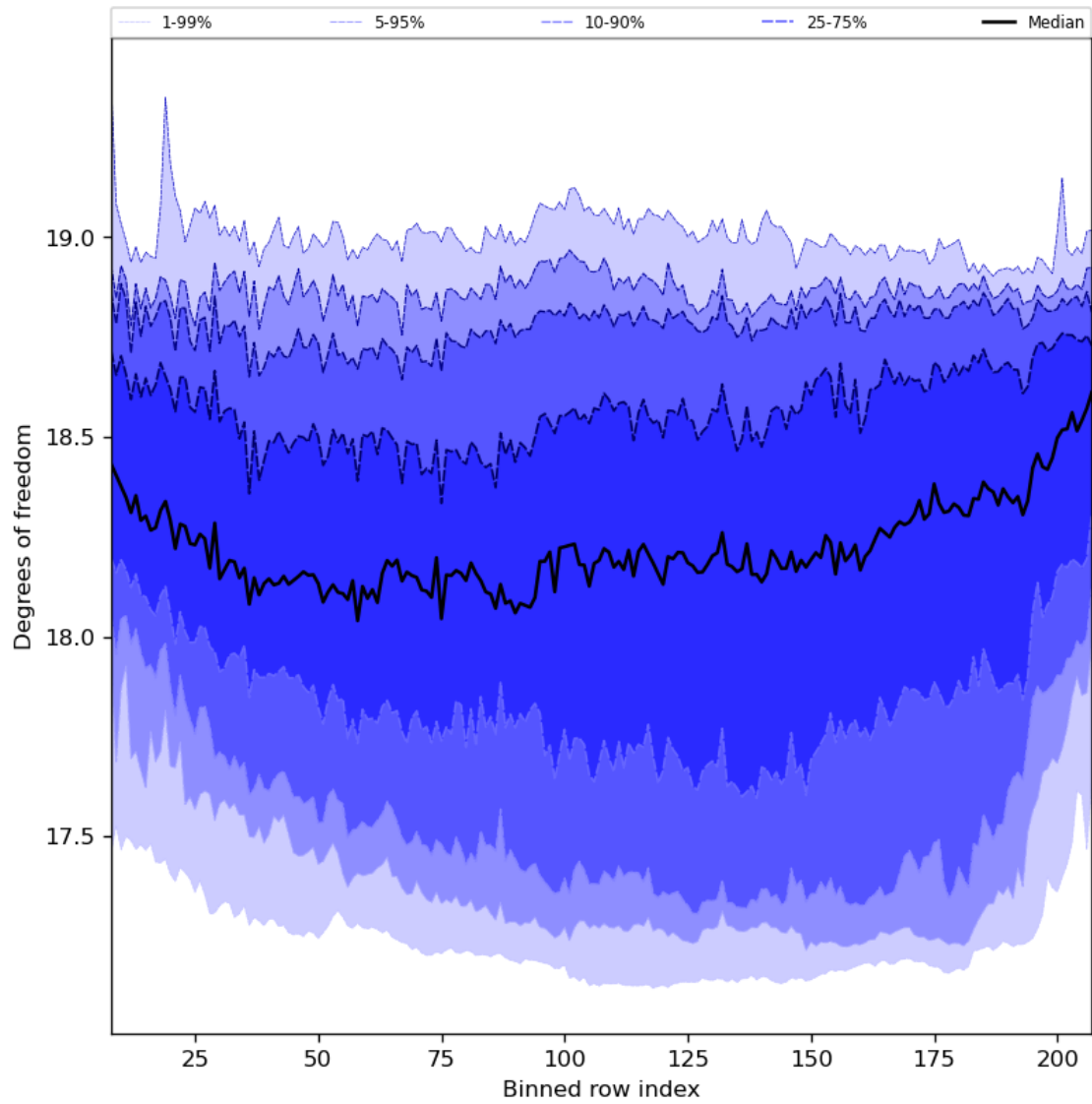
Figure 41: Along track statistics of “Degrees of freedom” for 2023-11-20 to 2023-11-22
