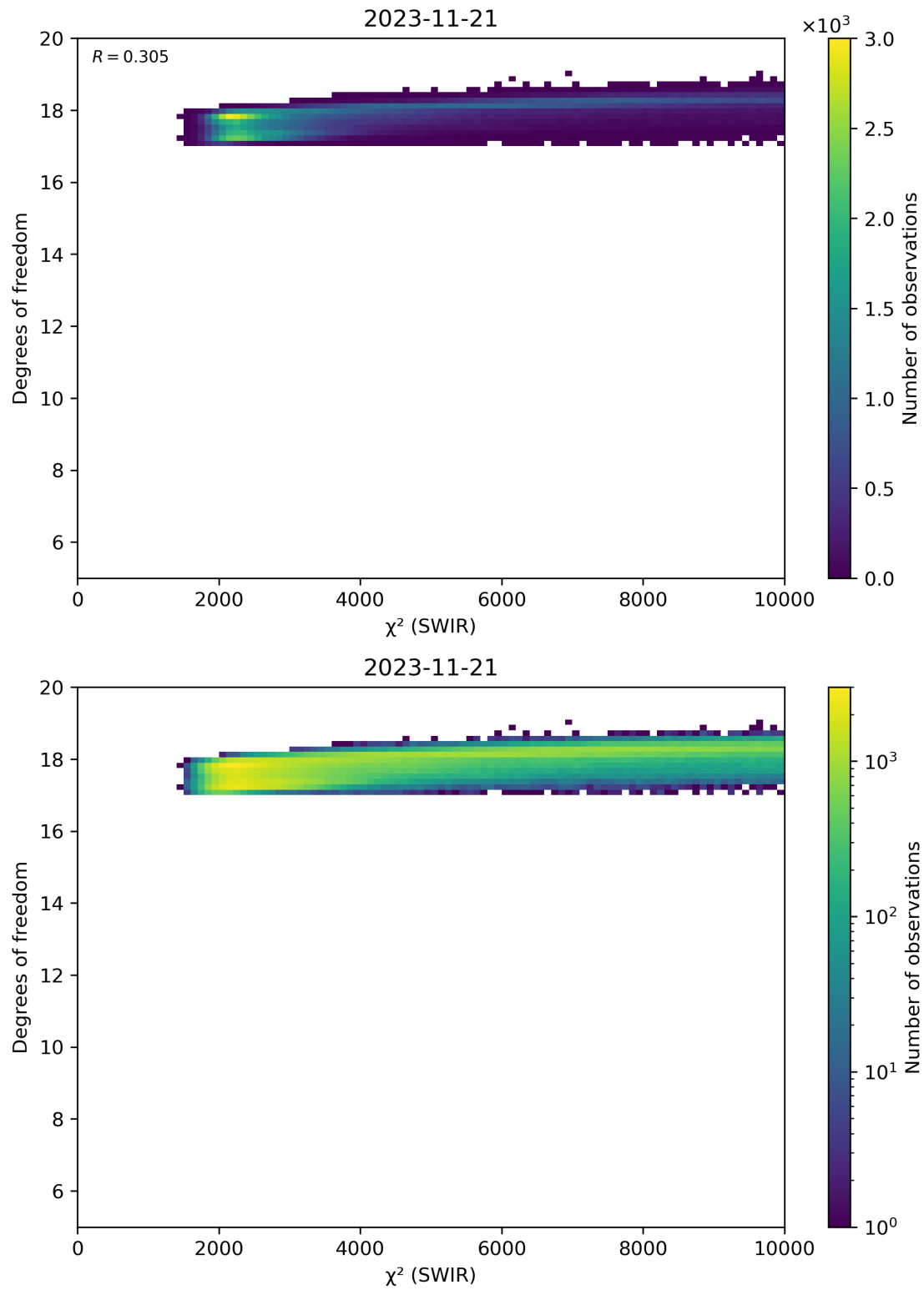
Figure 48: Scatter density plot of “ \chi^2 (SWIR)” against “Degrees of freedom” for 2023-11-20 to 2023-11-22.
