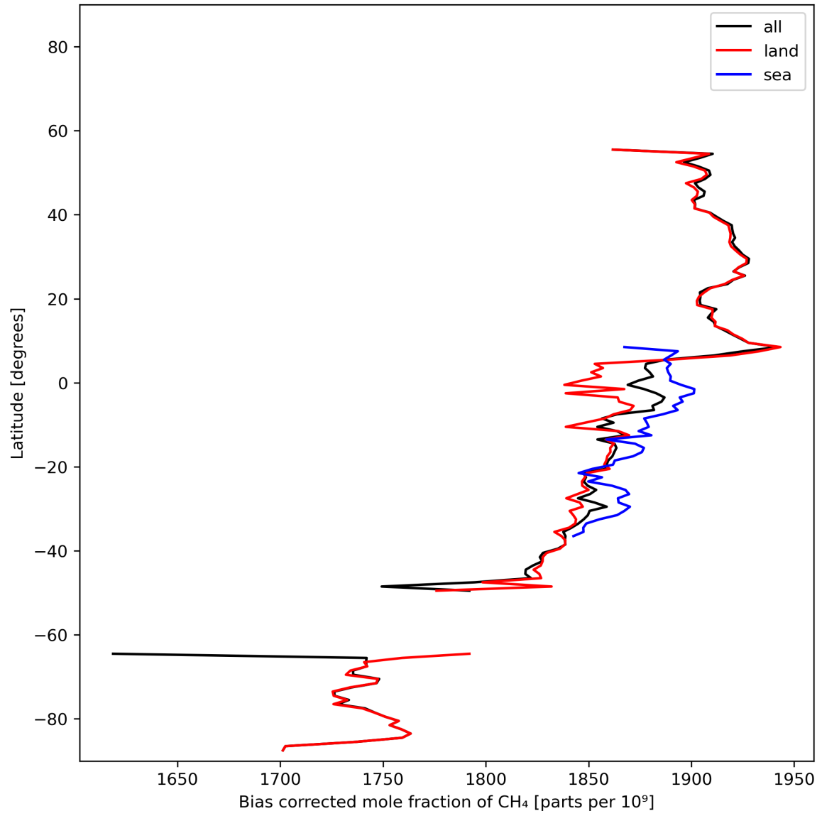
Figure 14: Zonal average of “Bias corrected mole fraction of CH 4 ” for 2023-11-20 to 2023-11-22.
