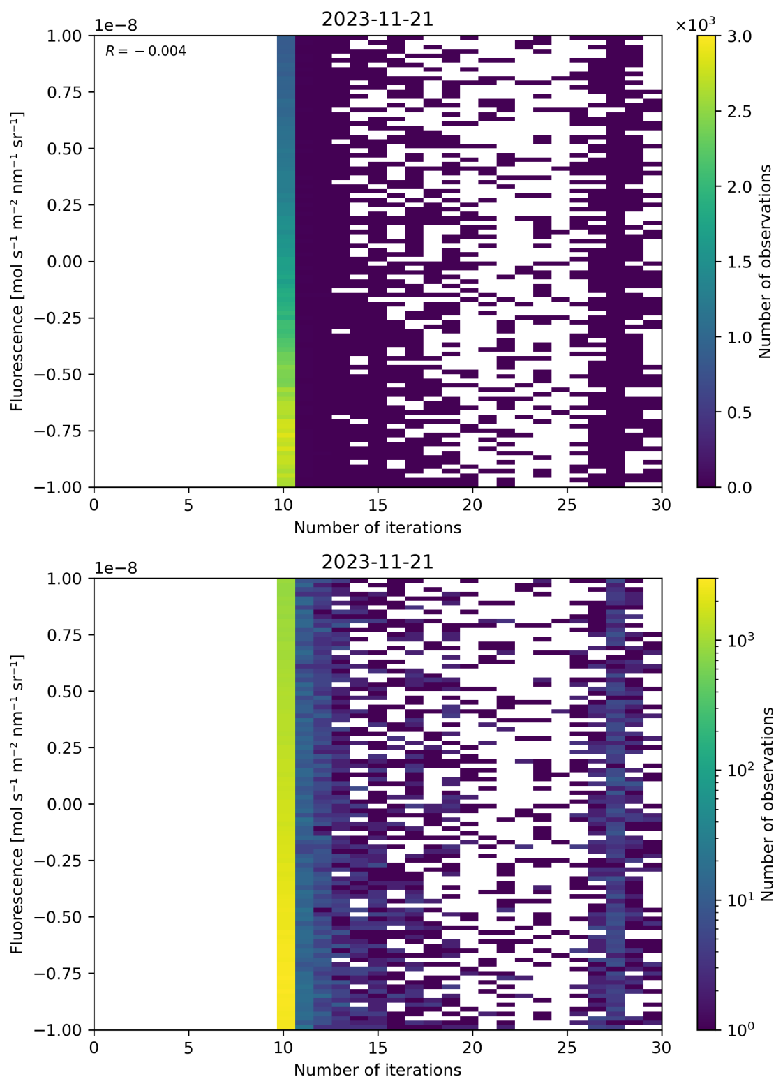
Figure 87: Scatter density plot of “Number of iterations” against “Fluorescence” for 2023-11-20 to 2023-11-22.
