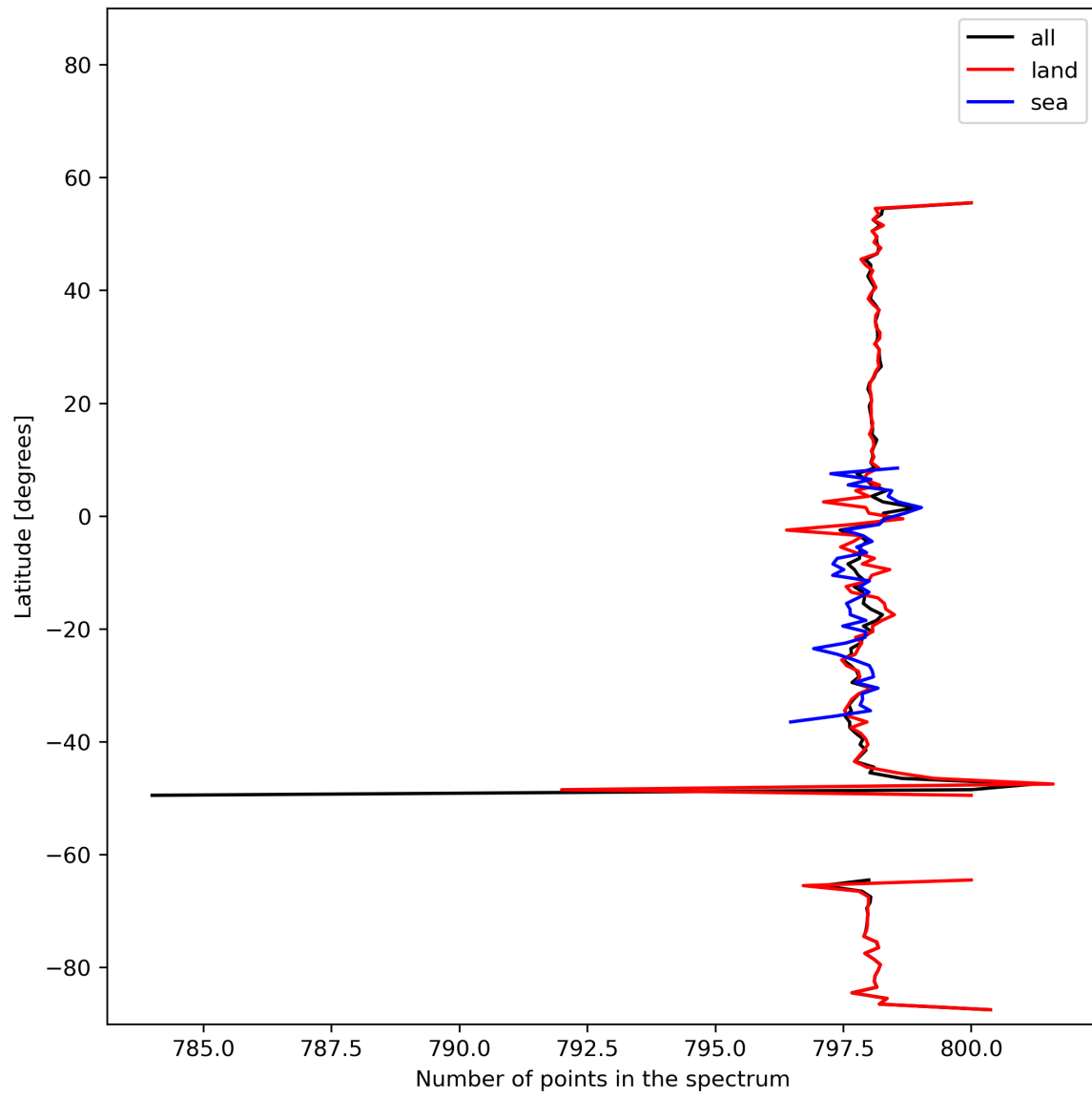
Figure 15: Zonal average of “Number of points in the spectrum” for 2023-11-20 to 2023-11-22.
