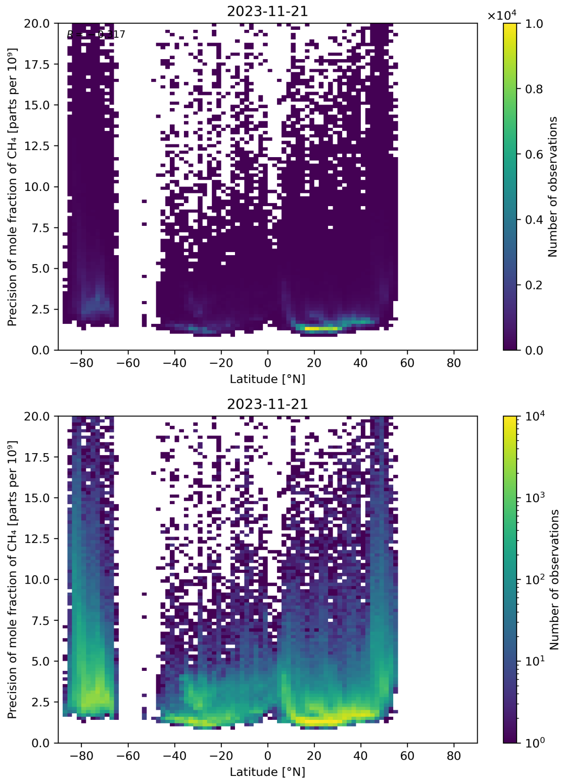
Figure 59: Scatter density plot of “Latitude” against “Precision of mole fraction of CH 4 ” for 2023-11-20 to 2023-11-22.
