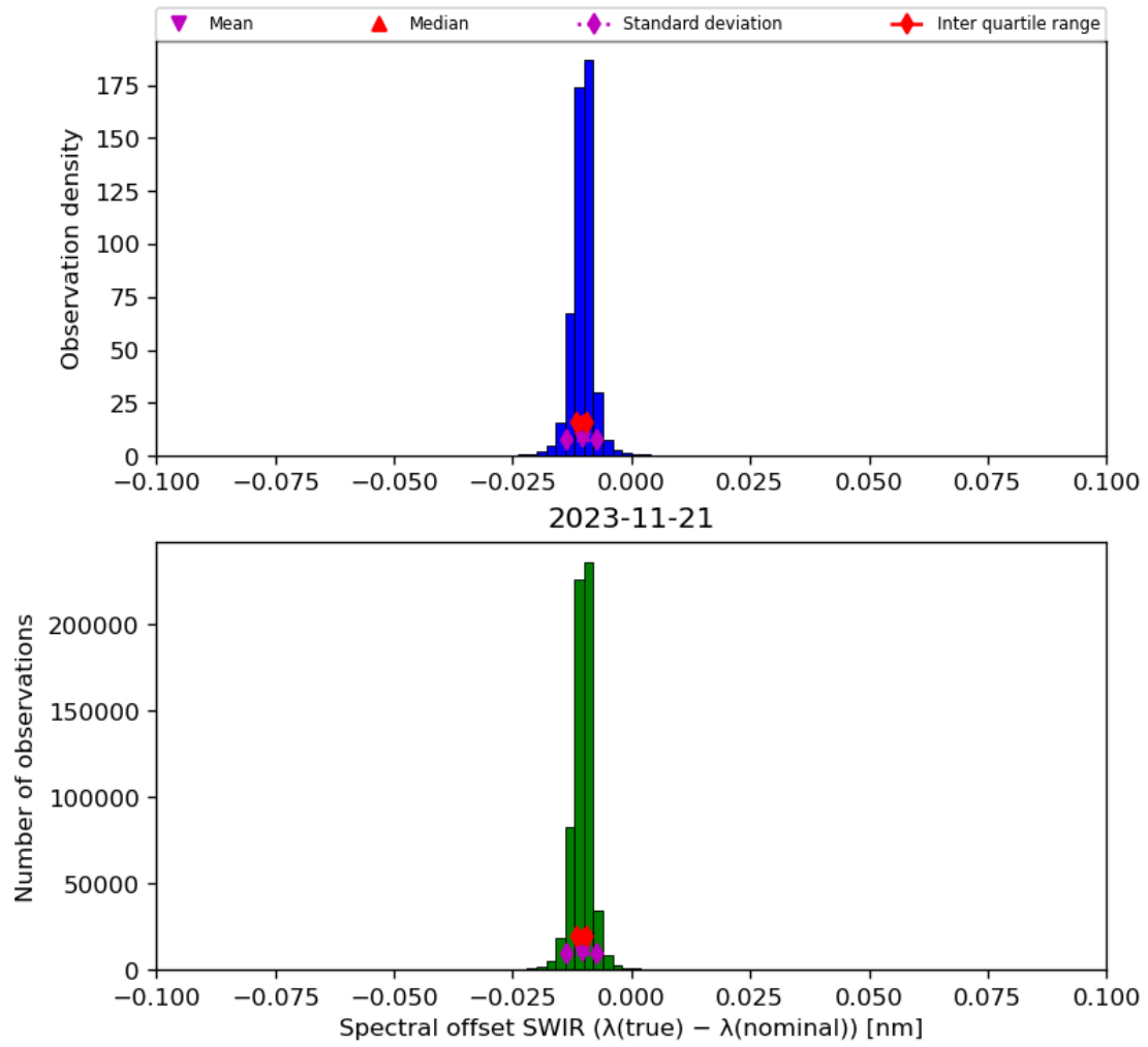
Figure 27: Histogram of “Spectral offset SWIR ( \lambda(\text{true}) - \lambda(\text{nominal}) )” for 2023-11-20 to 2023-11-22
