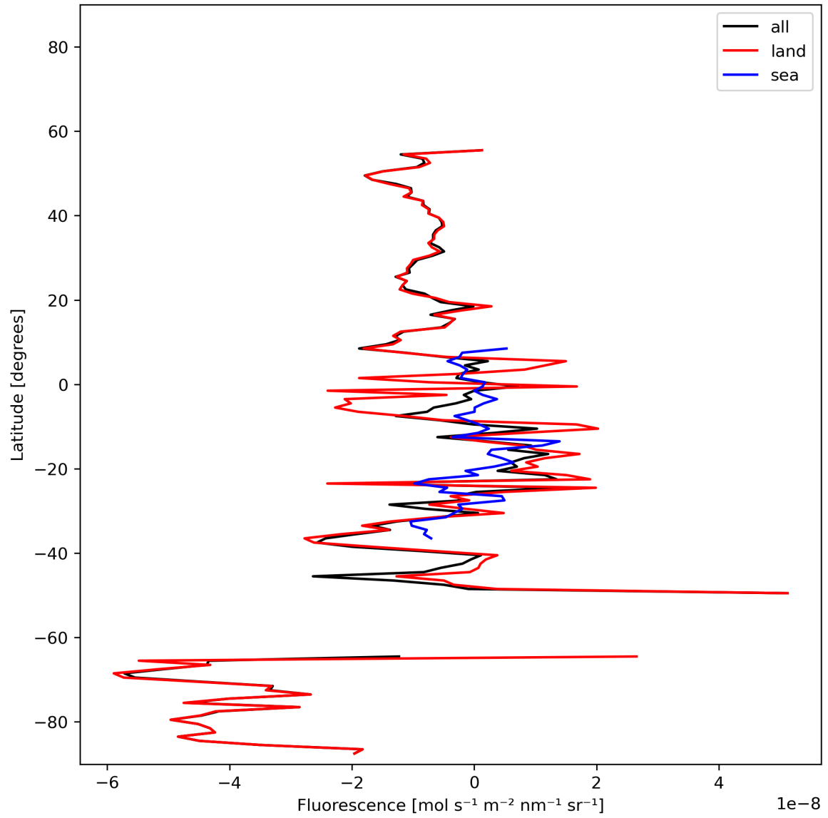
Figure 21: Zonal average of “Fluorescence” for 2023-11-20 to 2023-11-22.
