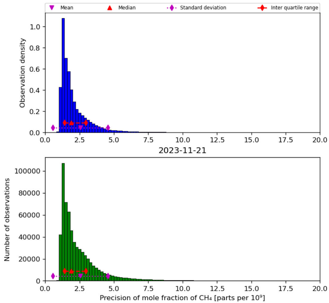
Figure 24: Histogram of “Precision of mole fraction of CH 4 ” for 2023-11-20 to 2023-11-22
