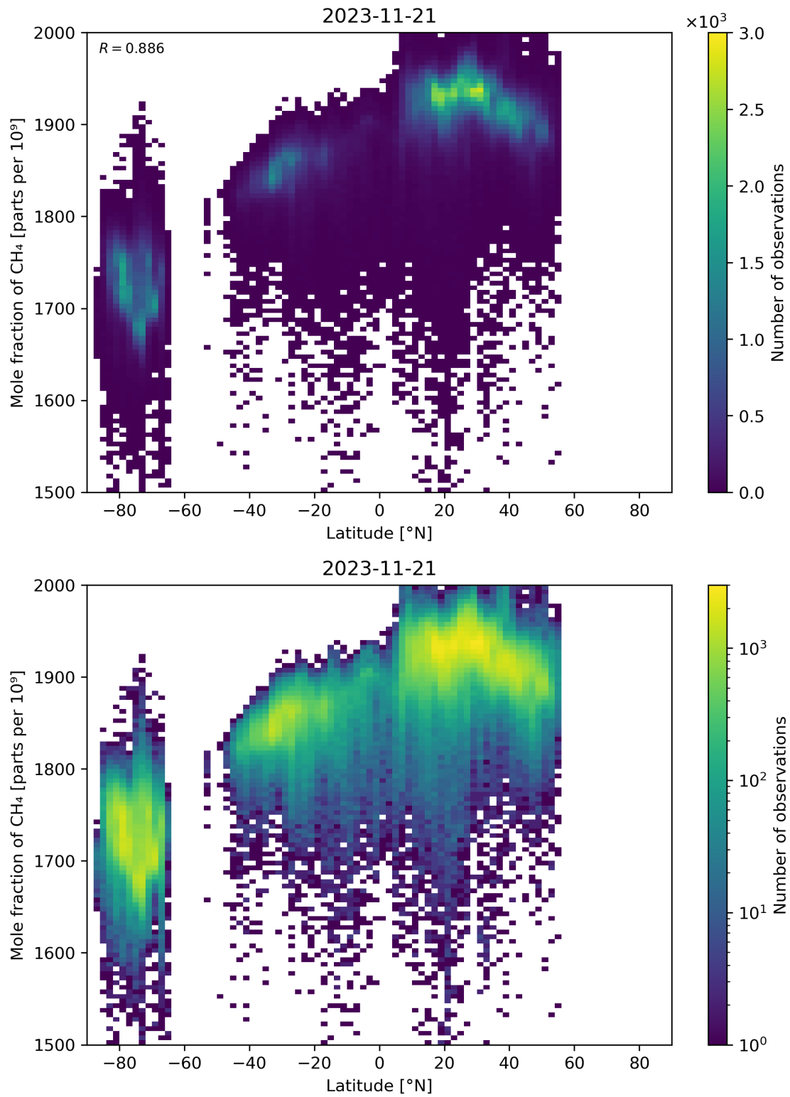
Figure 57: Scatter density plot of “Latitude” against “Mole fraction of CH 4 ” for 2023-11-20 to 2023-11-22.
