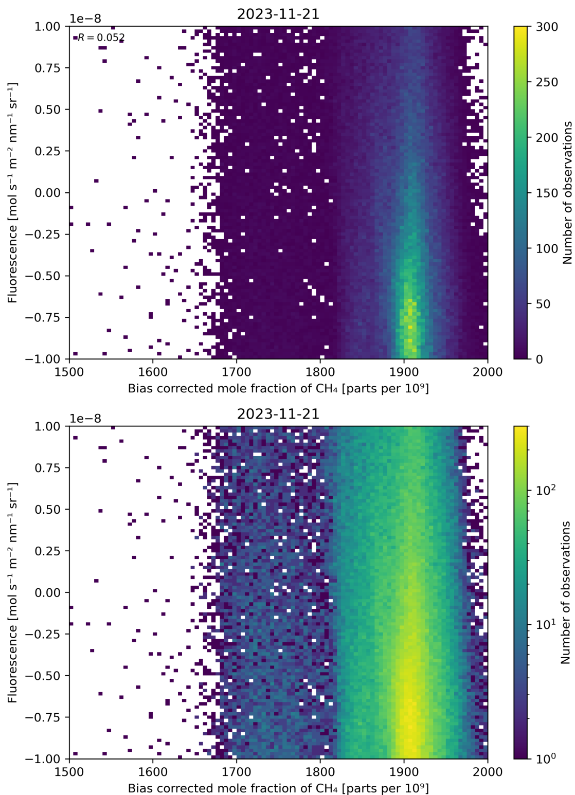
Figure 66: Scatter density plot of “Bias corrected mole fraction of \text{CH}_4 ” against “Fluorescence” for 2023-11-20 to 2023-11-22.
