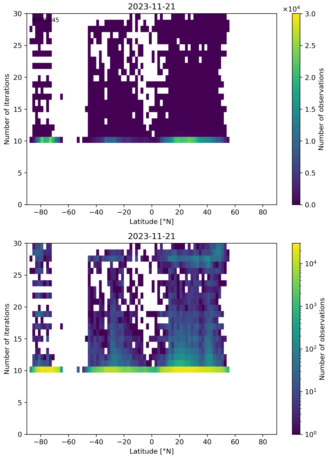
Figure 60: Scatter density plot of “Latitude” against “Number of iterations” for 2023-11-20 to 2023-11-22.
