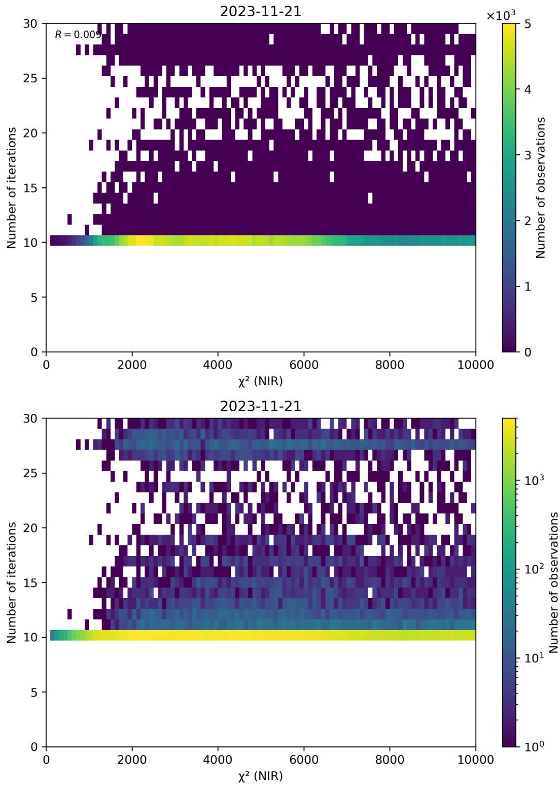
Figure 46: Scatter density plot of “ \chi^2 (NIR)” against “Number of iterations” for 2023-11-20 to 2023-11-22.
