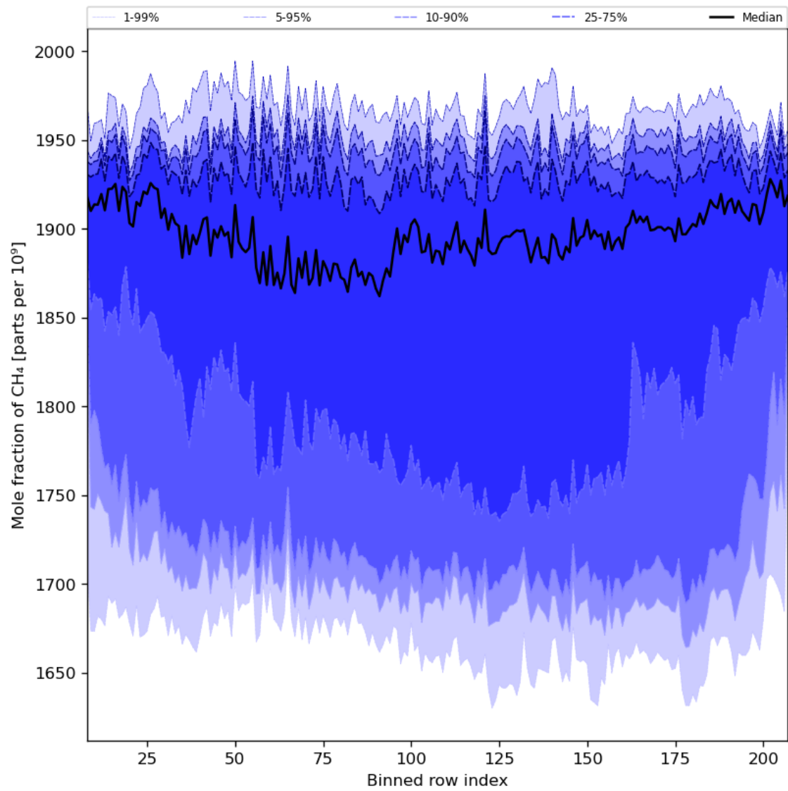
Figure 34: Along track statistics of “Mole fraction of CH 4 ” for 2023-11-20 to 2023-11-22
