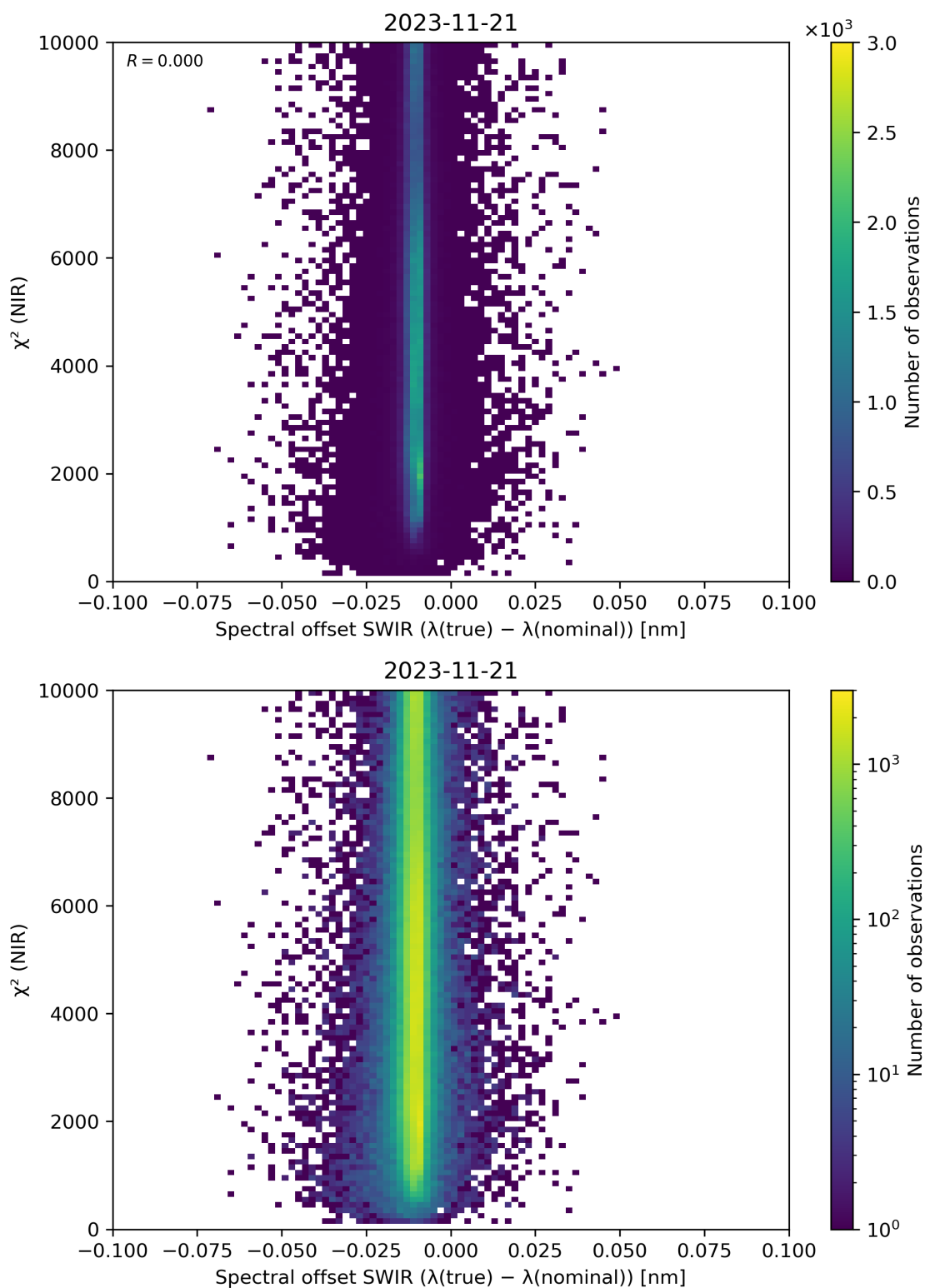
Figure 117: Scatter density plot of “Spectral offset SWIR ( \lambda(\text{true}) - \lambda(\text{nominal}) )” against “ \chi^2 (NIR)” for 2023-11-20 to 2023-11-22.
