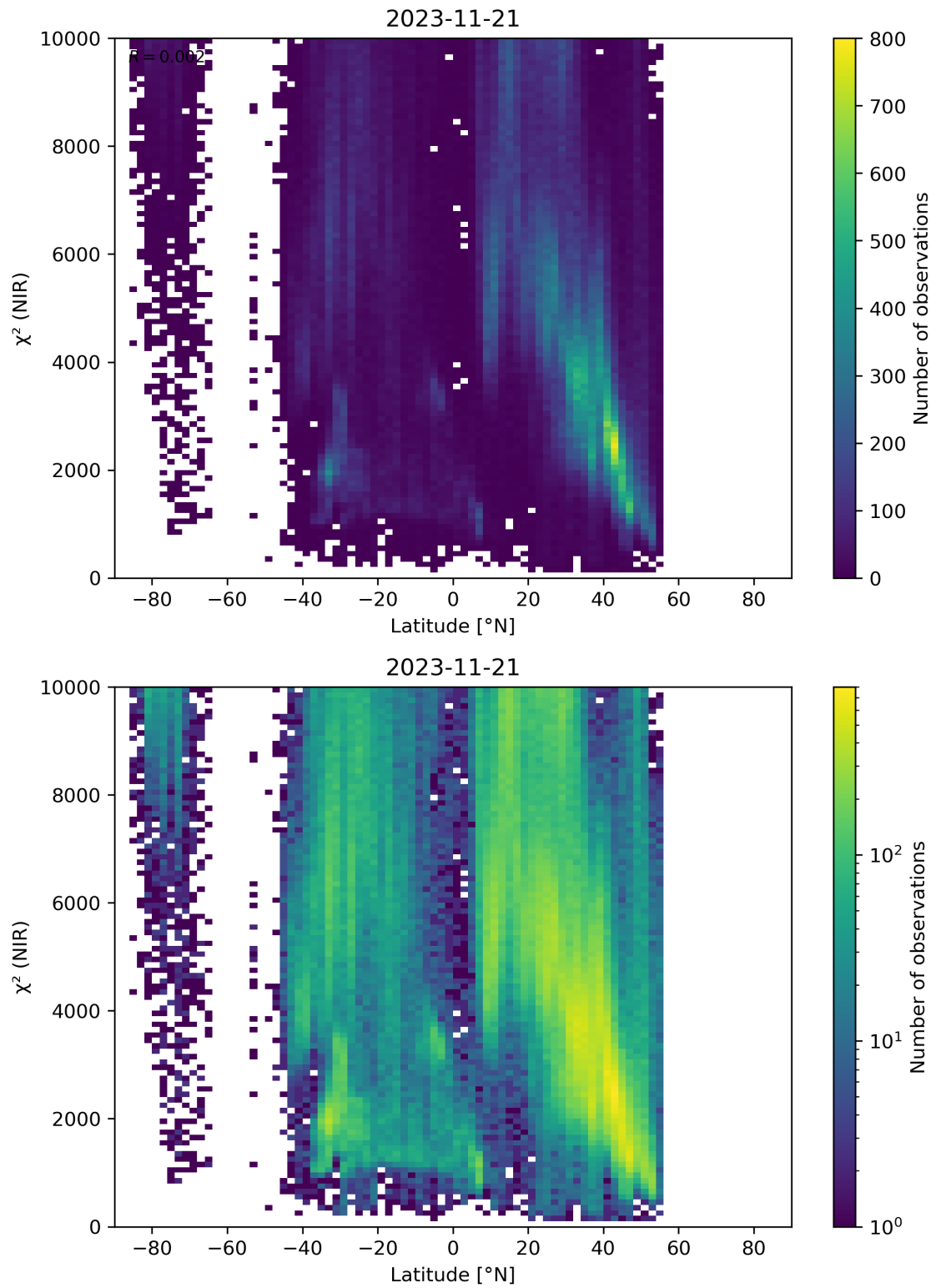
Figure 53: Scatter density plot of “Latitude” against “ \chi^2 (NIR)” for 2023-11-20 to 2023-11-22.
