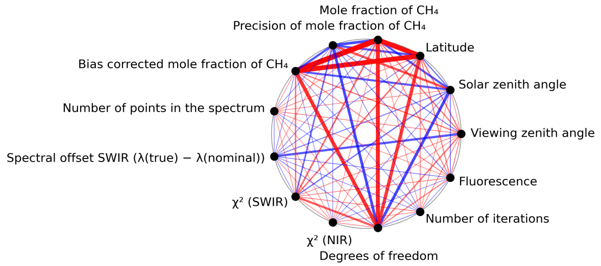
Figure 1: Map of correlation graph for 2023-11-20 to 2023-11-22.
