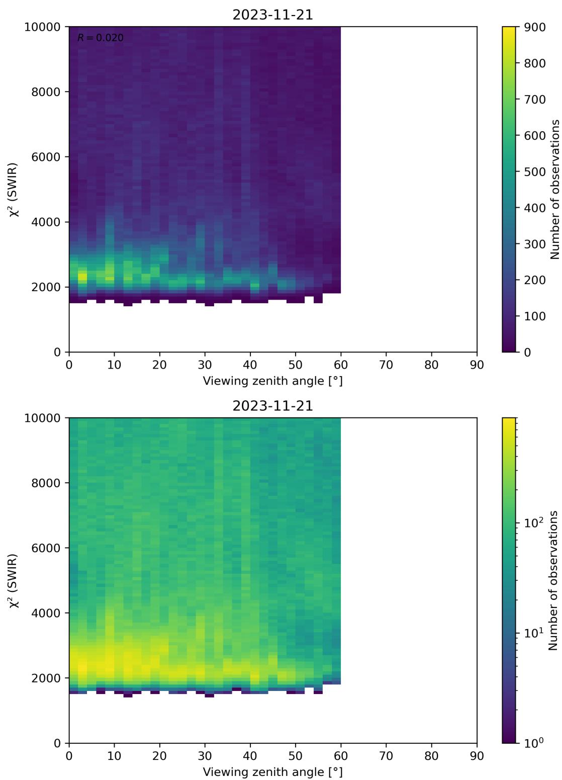
Figure 106: Scatter density plot of “Viewing zenith angle” against “ \chi^2 (SWIR)” for 2023-11-20 to 2023-11-22.
