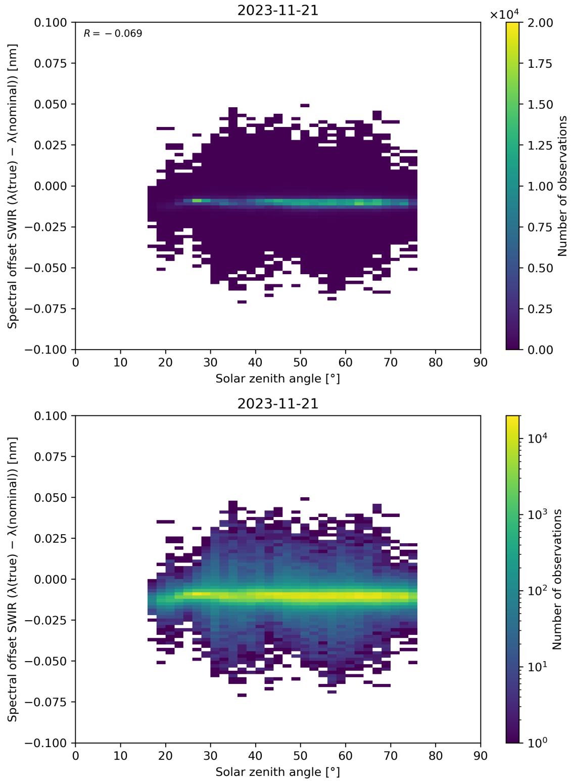
Figure 104: Scatter density plot of “Solar zenith angle” against “Spectral offset SWIR ( \lambda(\text{true}) - \lambda(\text{nominal}) )” for 2023-11-20 to 2023-11-22.
