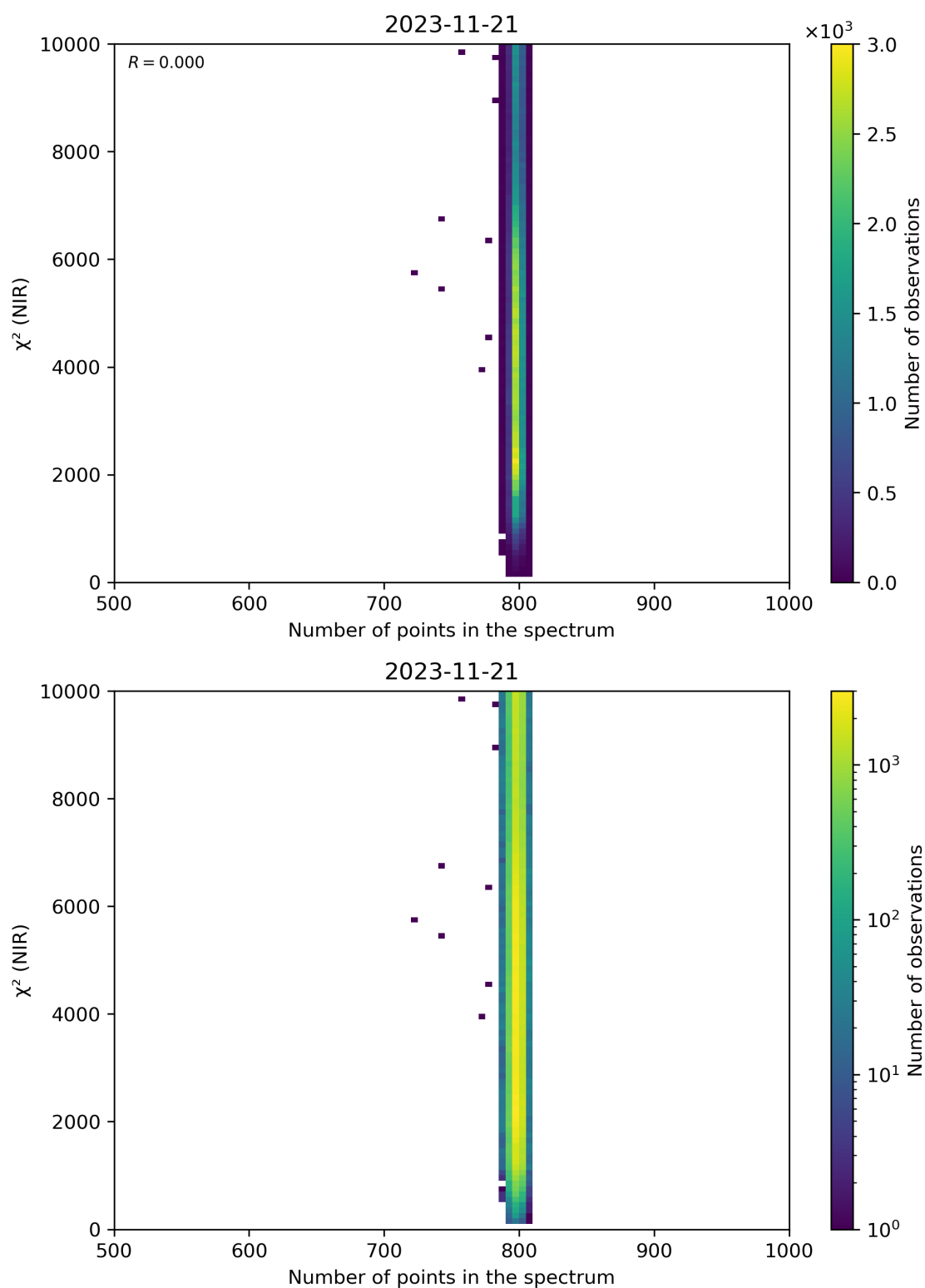
Figure 88: Scatter density plot of “Number of points in the spectrum” against “ \chi^2 (NIR)” for 2023-11-20 to 2023-11-22.
