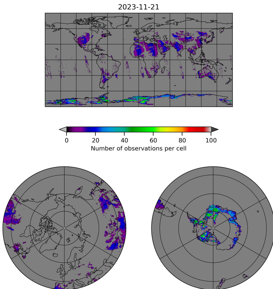
Figure 10: Map of the number of observations for 2023-11-20 to 2023-11-22
