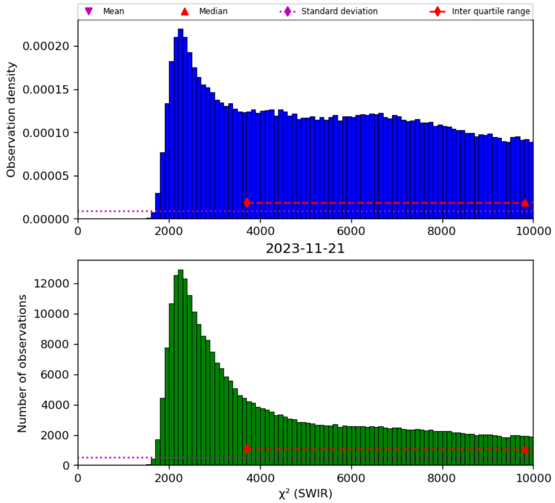
Figure 28: Histogram of “ \chi^2 (SWIR)” for 2023-11-20 to 2023-11-22
