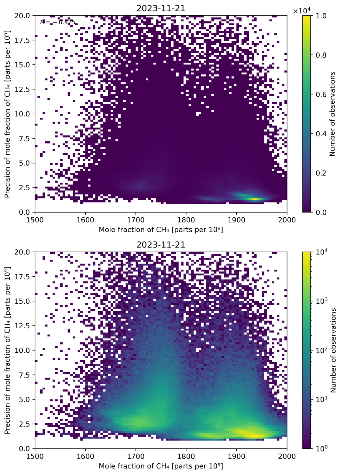
Figure 75: Scatter density plot of “Mole fraction of CH 4 ” against “Precision of mole fraction of CH 4 ” for 2023-11-20 to 2023-11-22.
