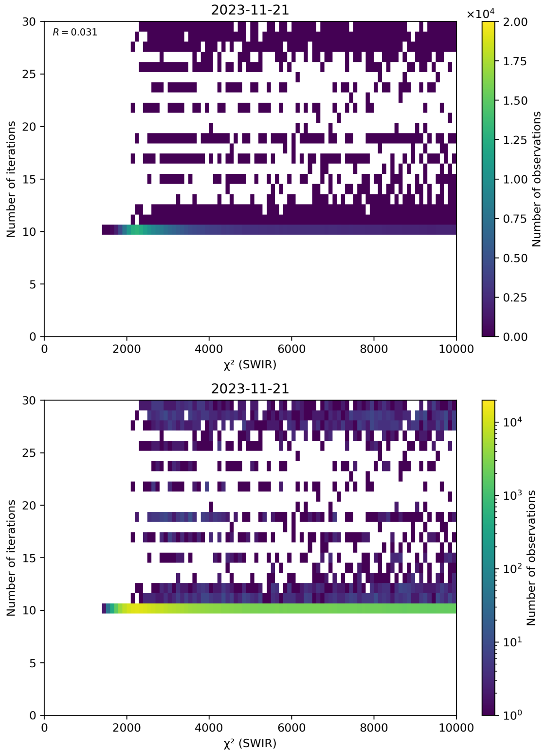
Figure 50: Scatter density plot of “ \chi^2 (SWIR)” against “Number of iterations” for 2023-11-20 to 2023-11-22.
