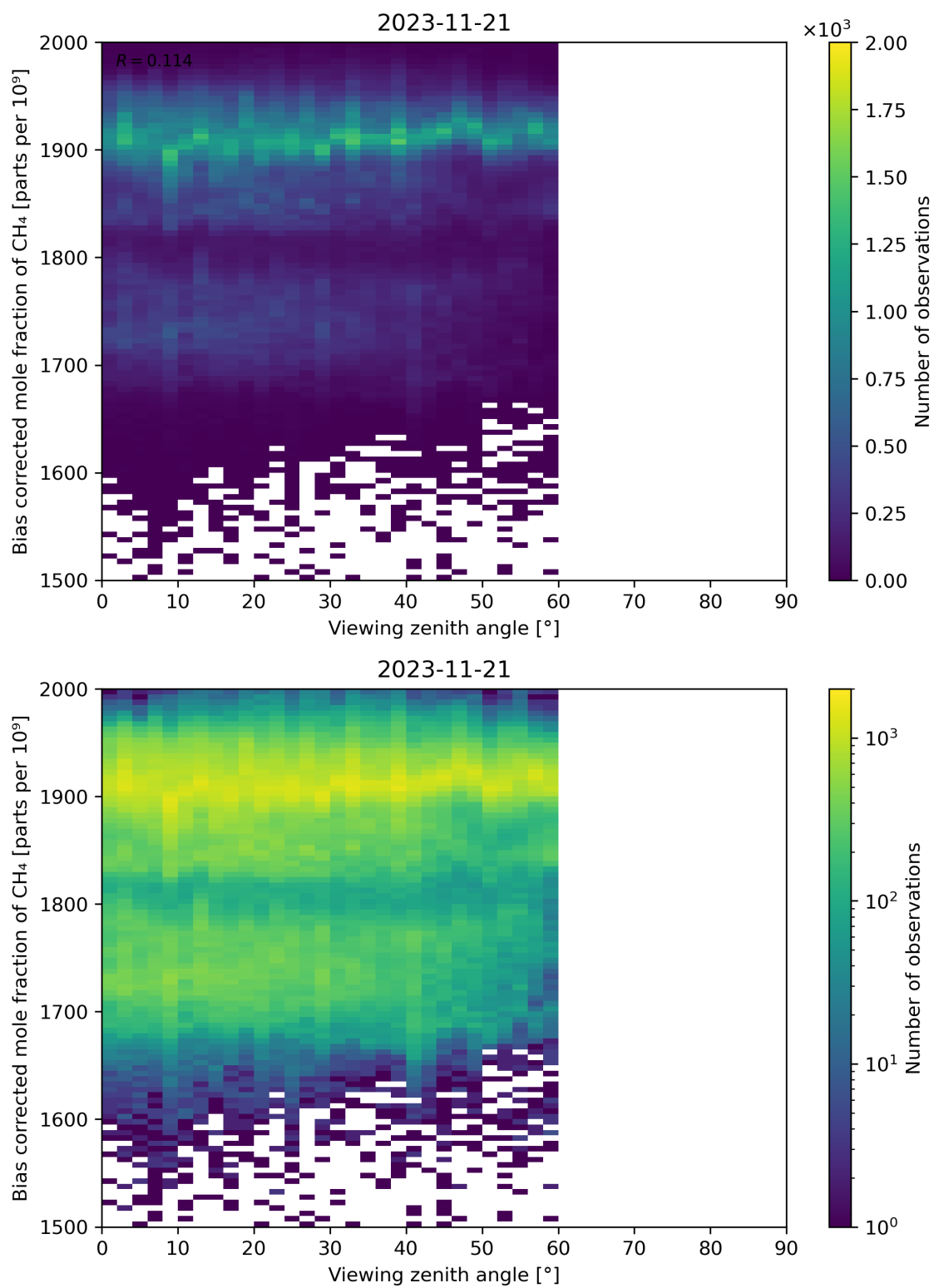
Figure 111: Scatter density plot of “Viewing zenith angle” against “Bias corrected mole fraction of CH 4 ” for 2023-11-20 to 2023-11-22.
