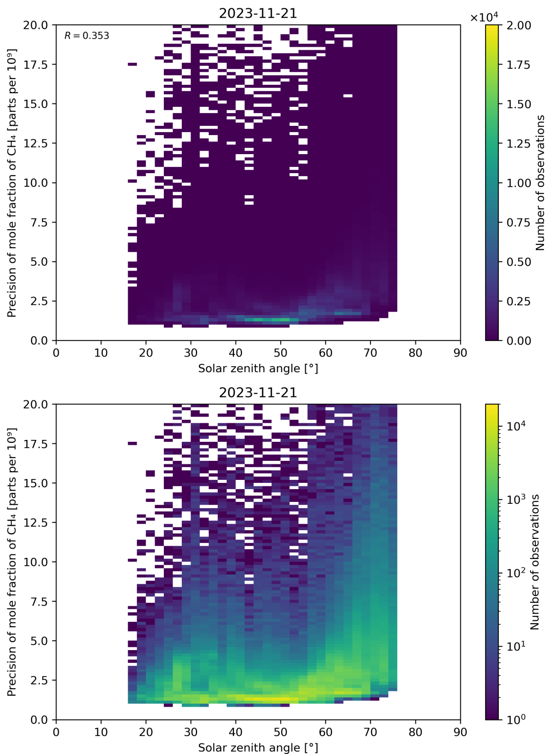
Figure 101: Scatter density plot of “Solar zenith angle” against “Precision of mole fraction of \text{CH}_4 ” for 2023-11-20 to 2023-11-22.
