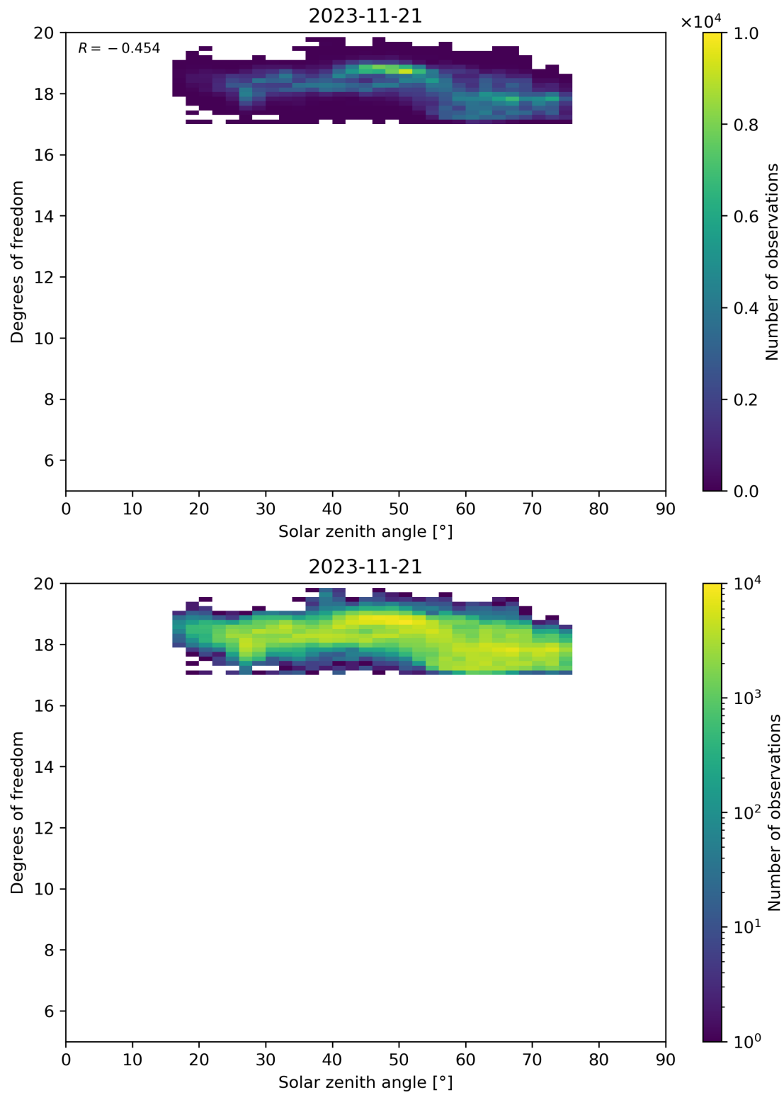
Figure 96: Scatter density plot of “Solar zenith angle” against “Degrees of freedom” for 2023-11-20 to 2023-11-22.
