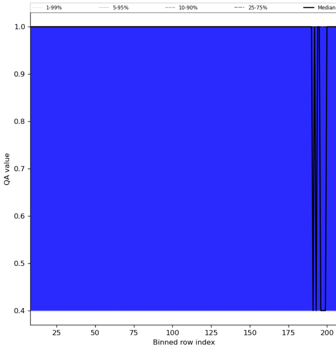
Figure 33: Along track statistics of “QA value” for 2023-11-20 to 2023-11-22
