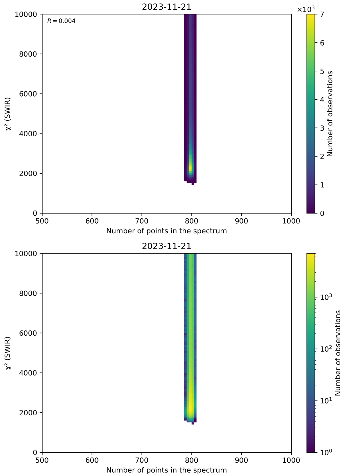
Figure 89: Scatter density plot of “Number of points in the spectrum” against “ \chi^2 (SWIR)” for 2023-11-20 to 2023-11-22.
