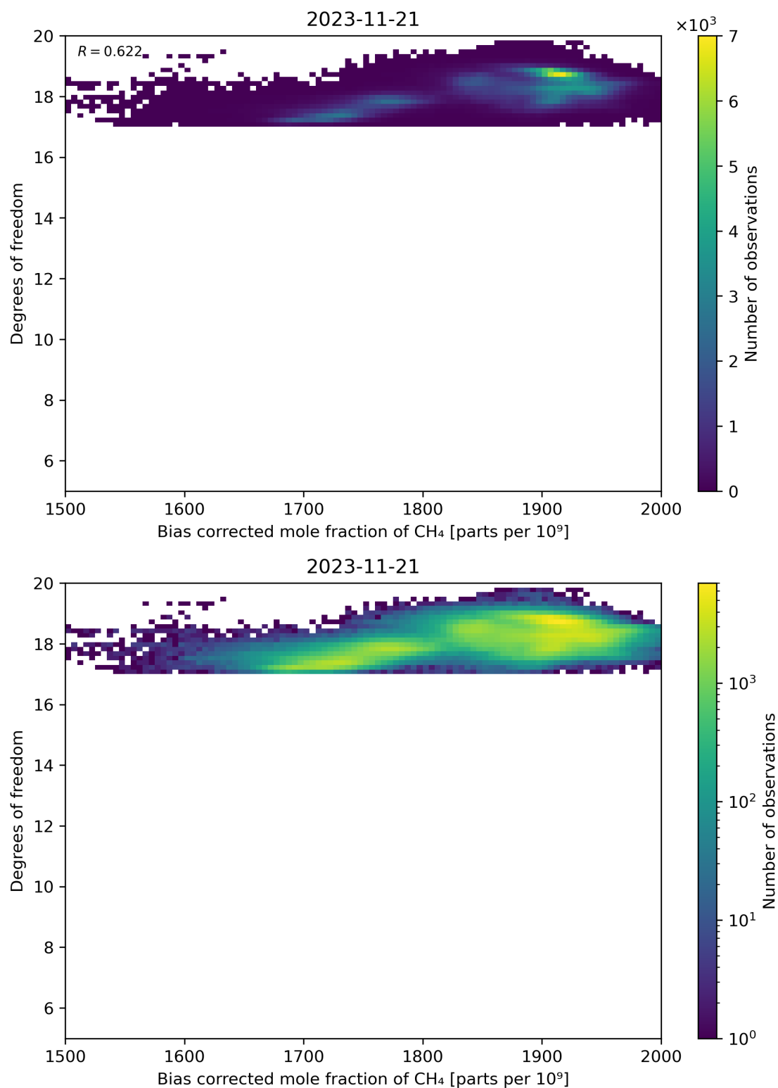
Figure 65: Scatter density plot of “Bias corrected mole fraction of CH 4 ” against “Degrees of freedom” for 2023-11-20 to 2023-11-22.
