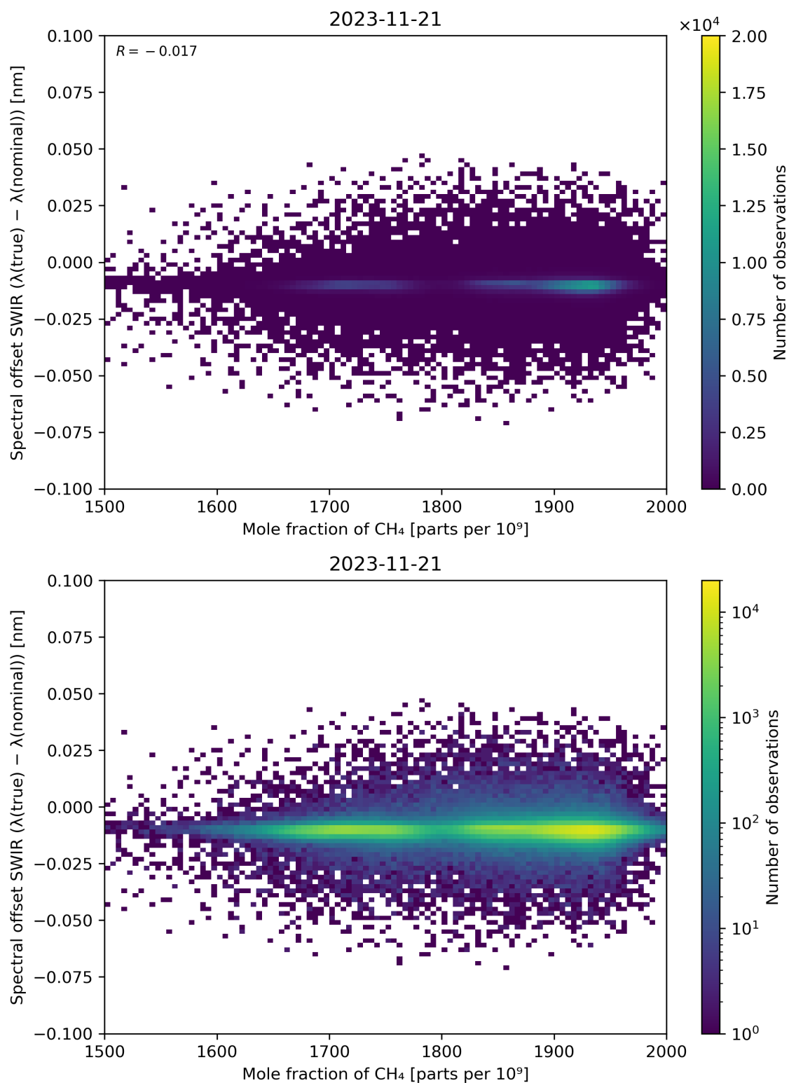
Figure 86: Scatter density plot of “Mole fraction of CH 4 ” against “Spectral offset SWIR ( \lambda(\text{true}) - \lambda(\text{nominal}) )” for 2023-11-20 to 2023-11-22.
