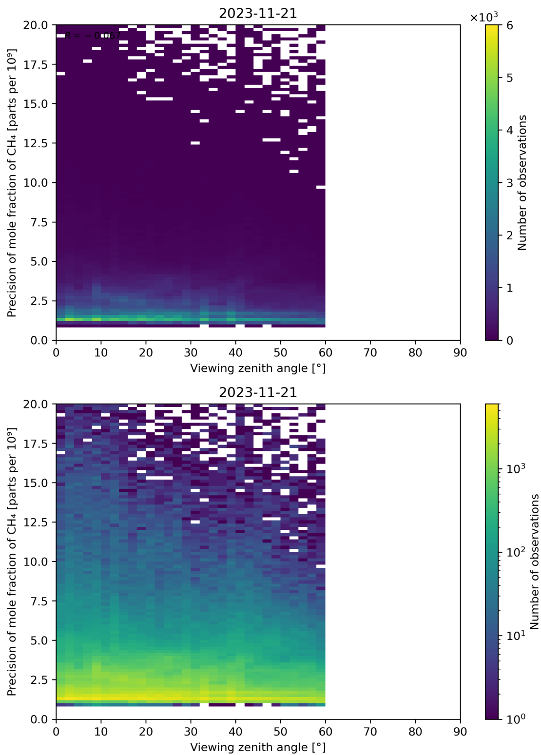
Figure 112: Scatter density plot of “Viewing zenith angle” against “Precision of mole fraction of CH 4 ” for 2023-11-20 to 2023-11-22.
