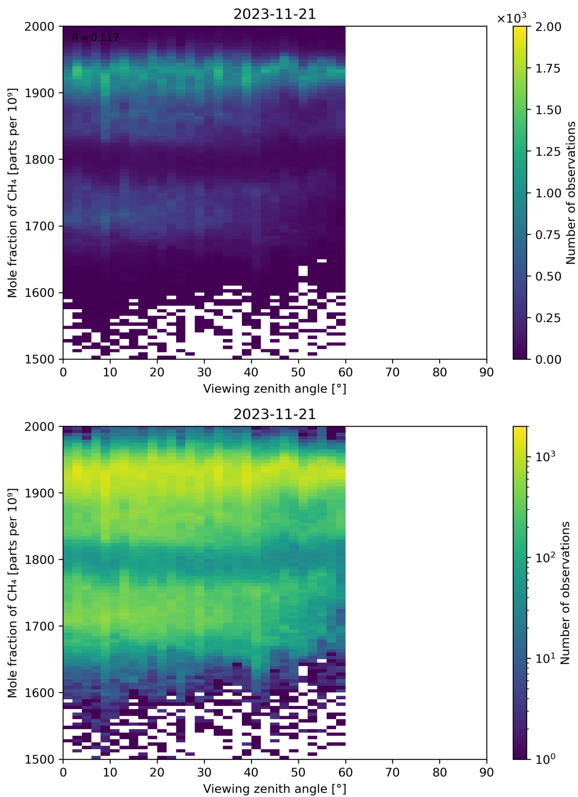
Figure 110: Scatter density plot of “Viewing zenith angle” against “Mole fraction of \text{CH}_4 ” for 2023-11-20 to 2023-11-22.
