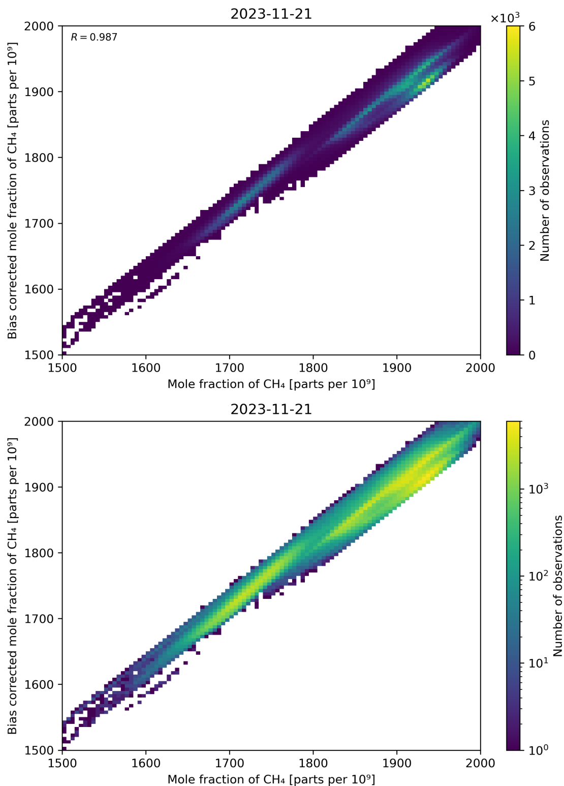
Figure 74: Scatter density plot of “Mole fraction of CH 4 ” against “Bias corrected mole fraction of CH 4 ” for 2023-11-20 to 2023-11-22.
