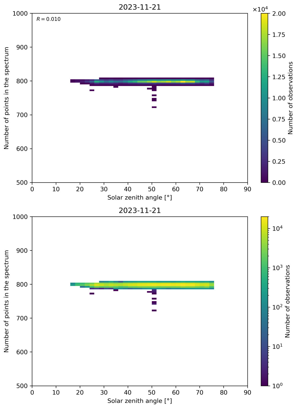
Figure 103: Scatter density plot of “Solar zenith angle” against “Number of points in the spectrum” for 2023-11-20 to 2023-11-22.
