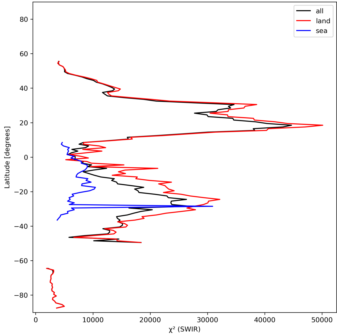
Figure 17: Zonal average of “ \chi^2 (SWIR)” for 2023-11-20 to 2023-11-22.
