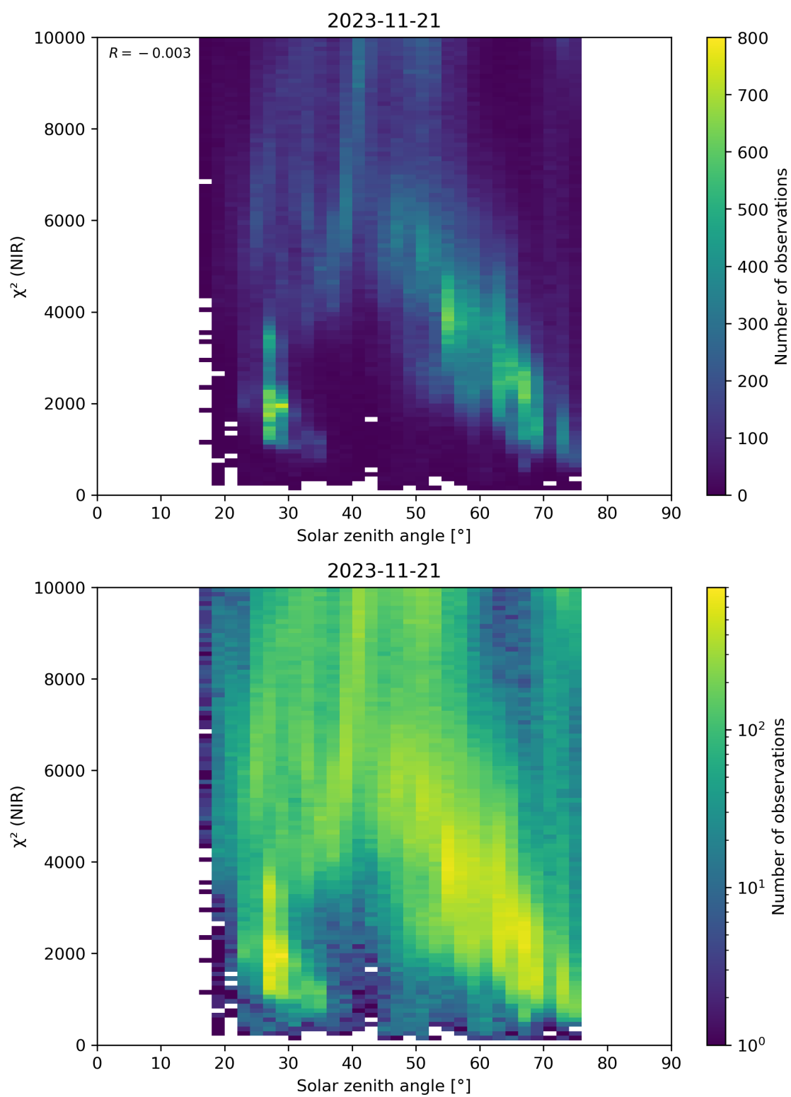
Figure 94: Scatter density plot of “Solar zenith angle” against “ \chi^2 (NIR)” for 2023-11-20 to 2023-11-22.
