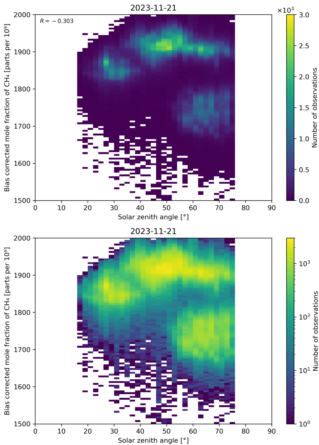
Figure 100: Scatter density plot of “Solar zenith angle” against “Bias corrected mole fraction of \text{CH}_4 ” for 2023-11-20 to 2023-11-22.
