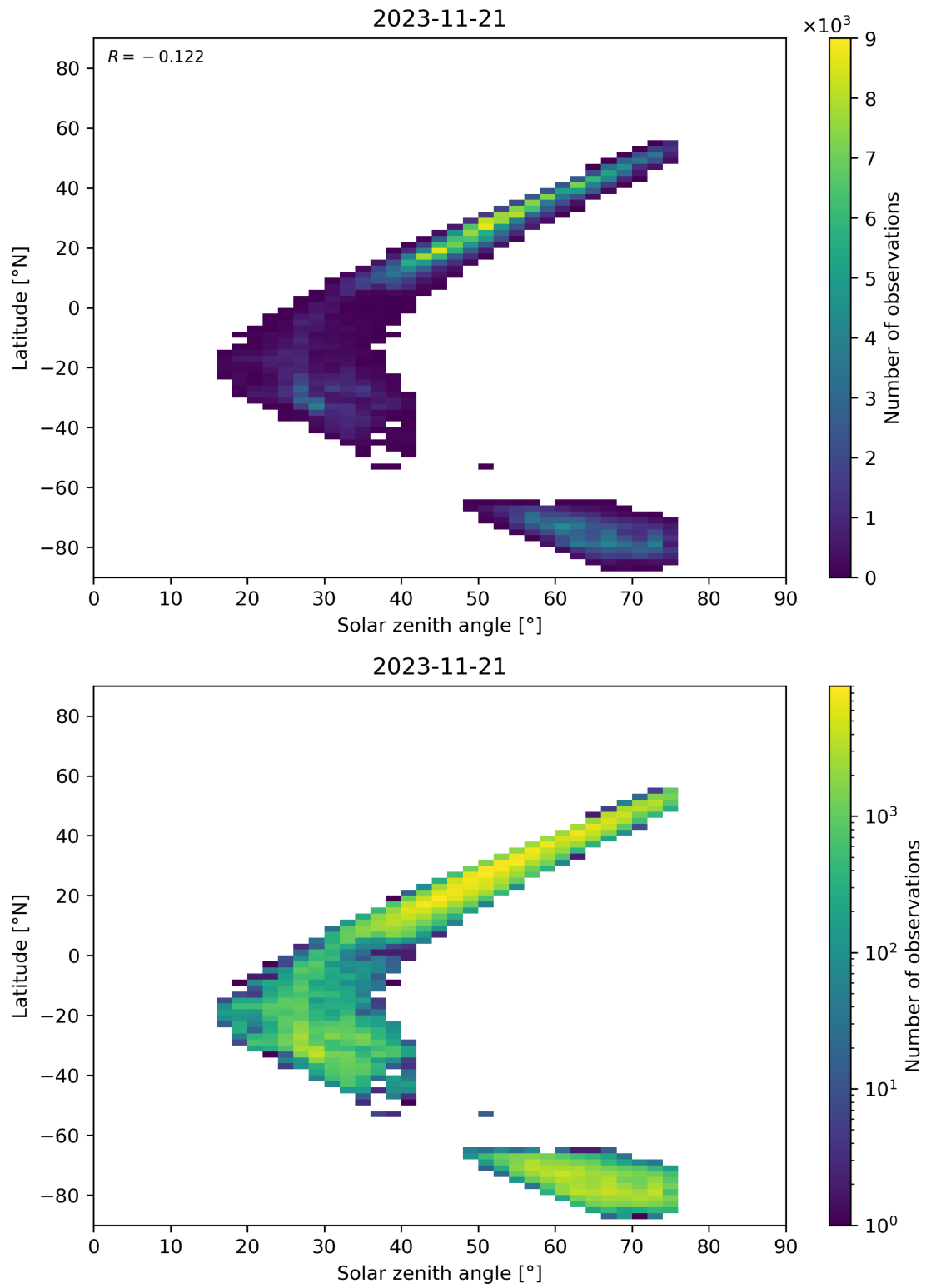
Figure 98: Scatter density plot of “Solar zenith angle” against “Latitude” for 2023-11-20 to 2023-11-22.
