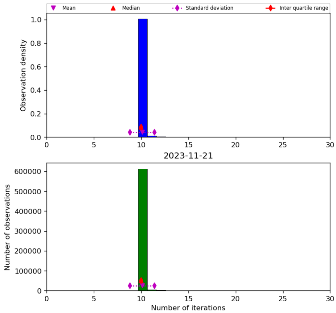
Figure 31: Histogram of “Number of iterations” for 2023-11-20 to 2023-11-22
