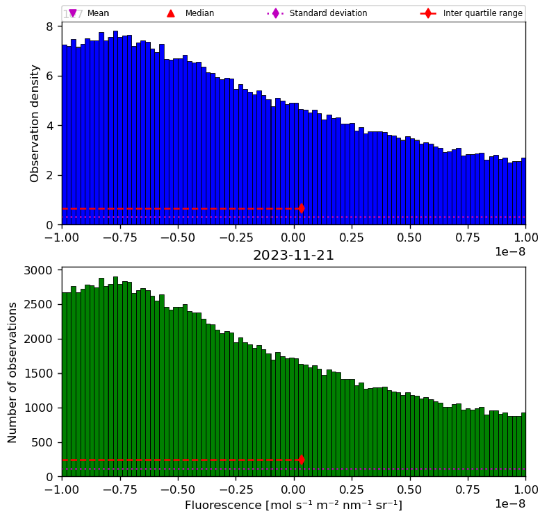
Figure 32: Histogram of “Fluorescence” for 2023-11-20 to 2023-11-22
