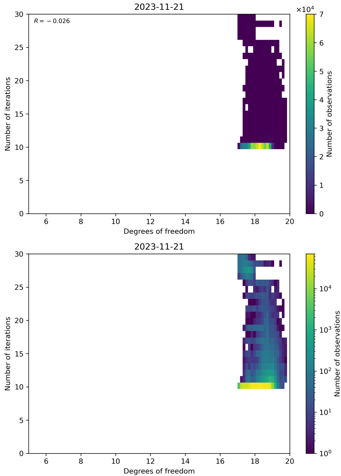
Figure 52: Scatter density plot of “Degrees of freedom” against “Number of iterations” for 2023-11-20 to 2023-11-22.
