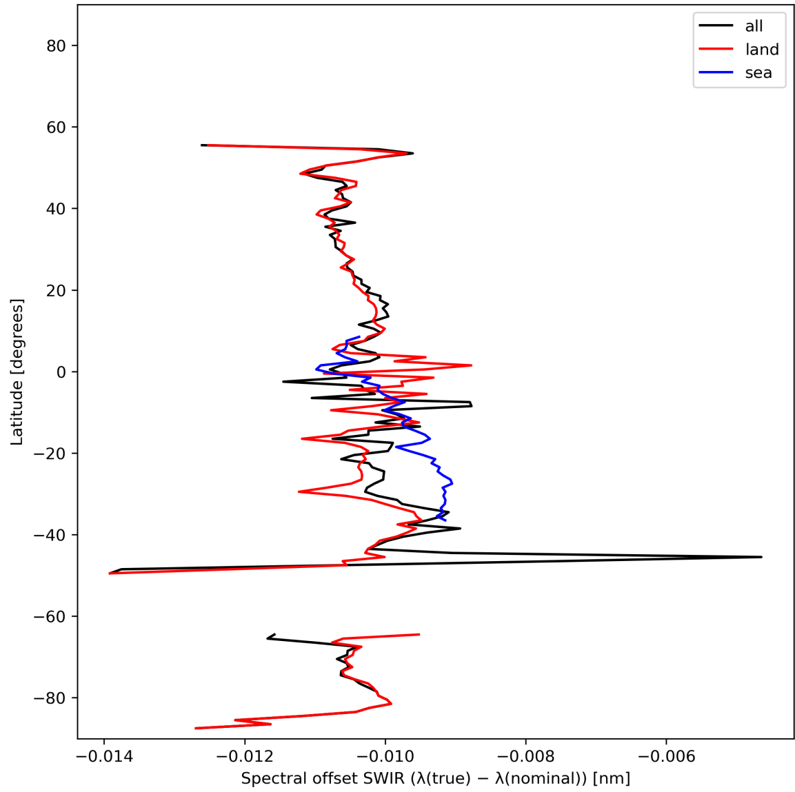
Figure 16: Zonal average of “Spectral offset SWIR ( \lambda(\text{true}) - \lambda(\text{nominal}) )” for 2023-11-20 to 2023-11-22.
