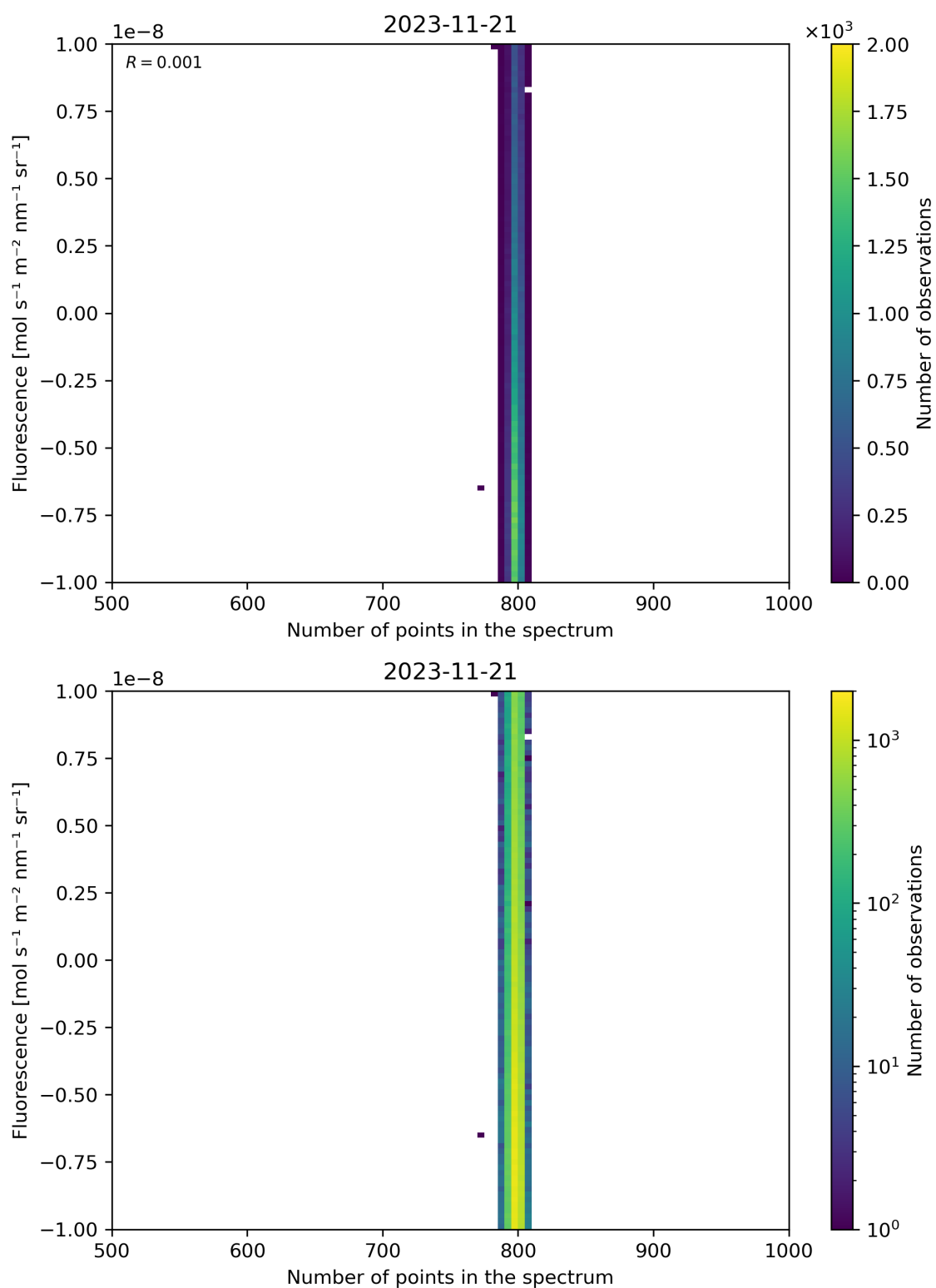
Figure 91: Scatter density plot of “Number of points in the spectrum” against “Fluorescence” for 2023-11-20 to 2023-11-22.
