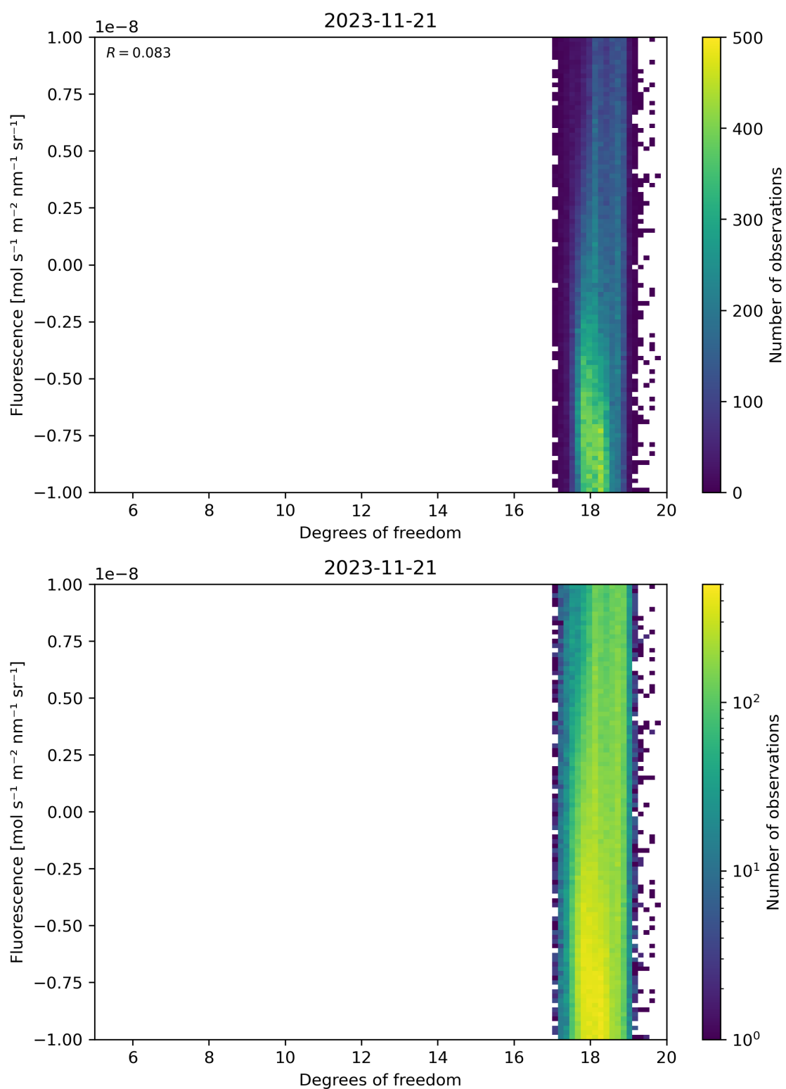
Figure 51: Scatter density plot of “Degrees of freedom” against “Fluorescence” for 2023-11-20 to 2023-11-22.
