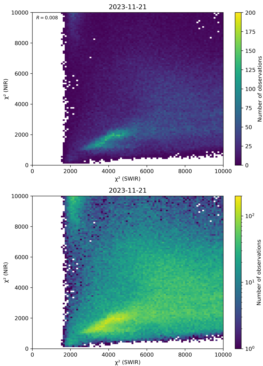
Figure 47: Scatter density plot of “ \chi^2 (SWIR)” against “ \chi^2 (NIR)” for 2023-11-20 to 2023-11-22.
