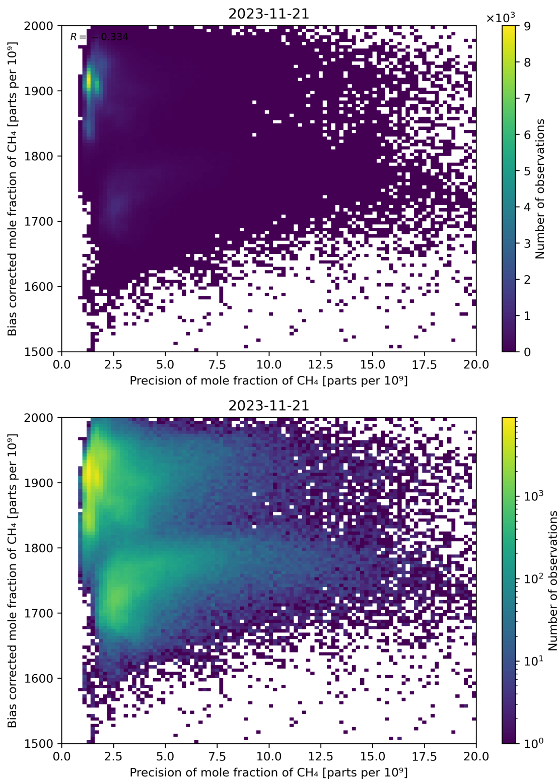
Figure 82: Scatter density plot of “Precision of mole fraction of CH 4 ” against “Bias corrected mole fraction of CH 4 ” for 2023-11-20 to 2023-11-22.
