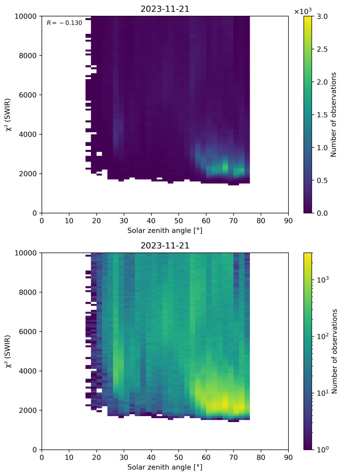
Figure 95: Scatter density plot of “Solar zenith angle” against “ \chi^2 (SWIR)” for 2023-11-20 to 2023-11-22.
