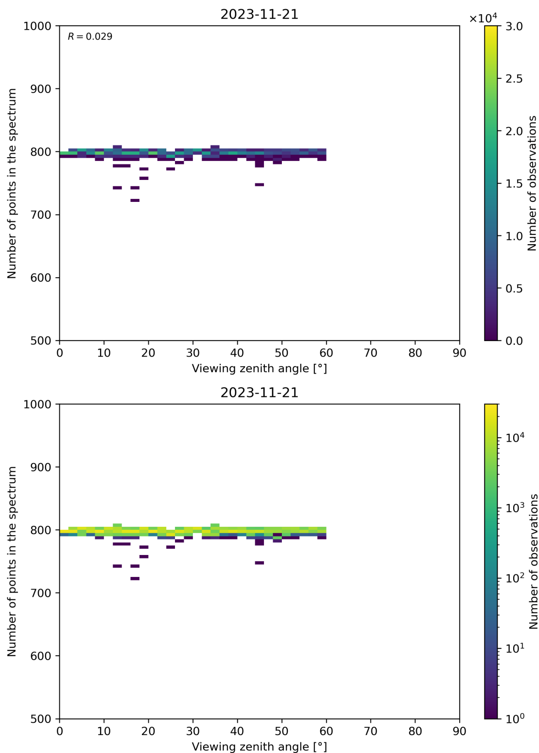
Figure 114: Scatter density plot of “Viewing zenith angle” against “Number of points in the spectrum” for 2023-11-20 to 2023-11-22.
