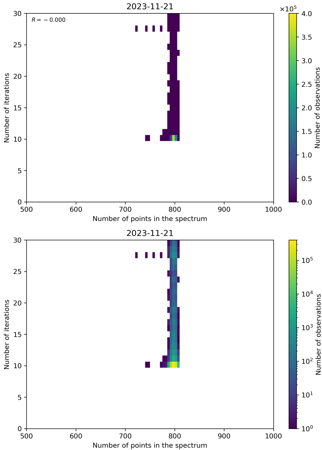
Figure 92: Scatter density plot of “Number of points in the spectrum” against “Number of iterations” for 2023-11-20 to 2023-11-22.
