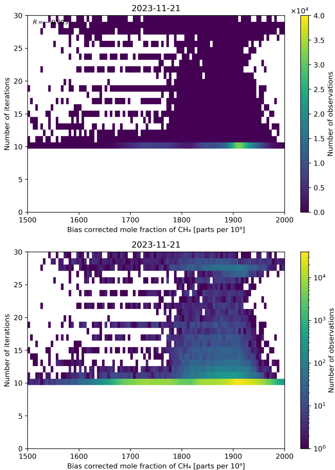
Figure 67: Scatter density plot of “Bias corrected mole fraction of \text{CH}_4 ” against “Number of iterations” for 2023-11-20 to 2023-11-22.
