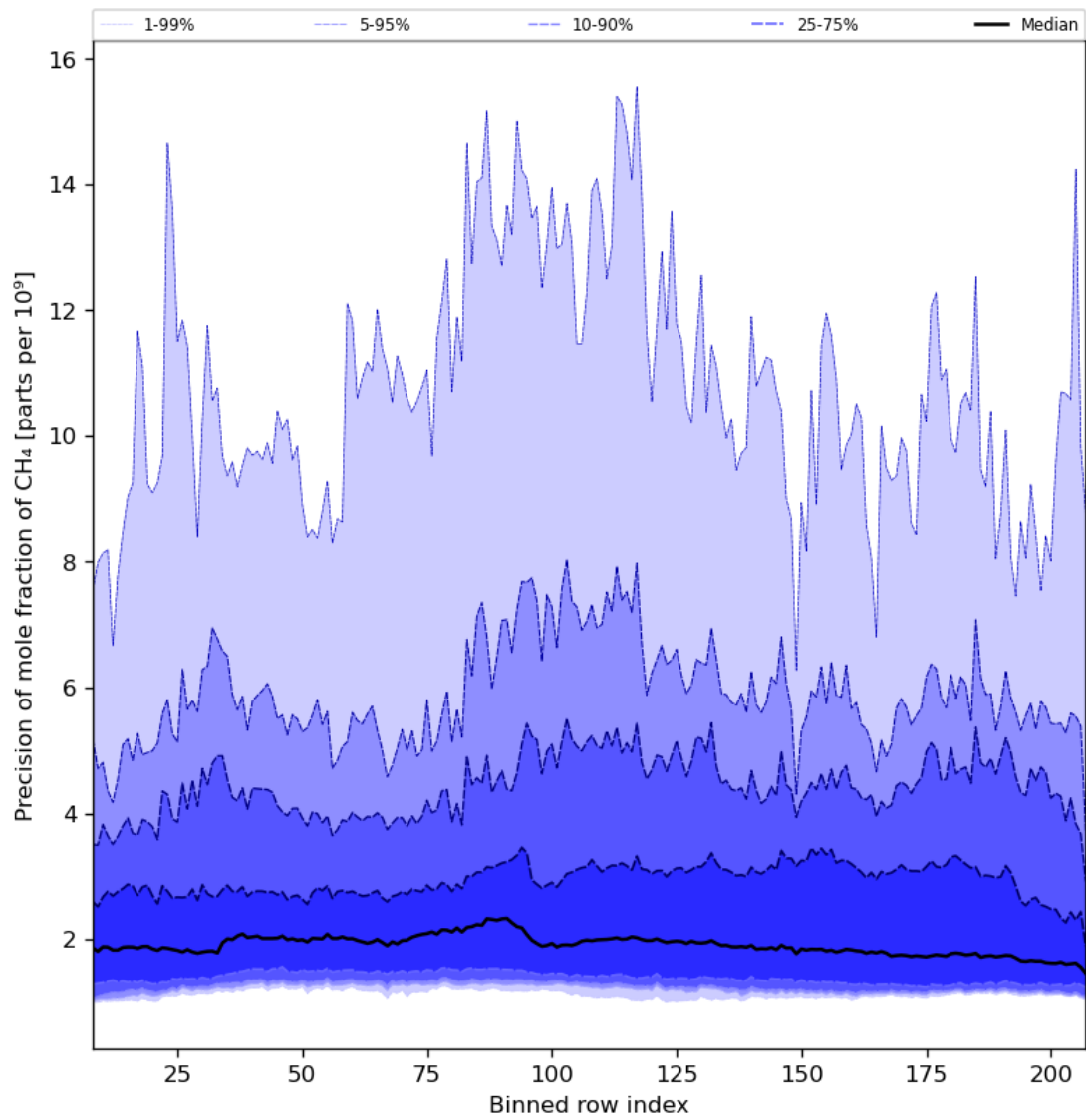
Figure 35: Along track statistics of “Precision of mole fraction of CH 4 ” for 2023-11-20 to 2023-11-22
