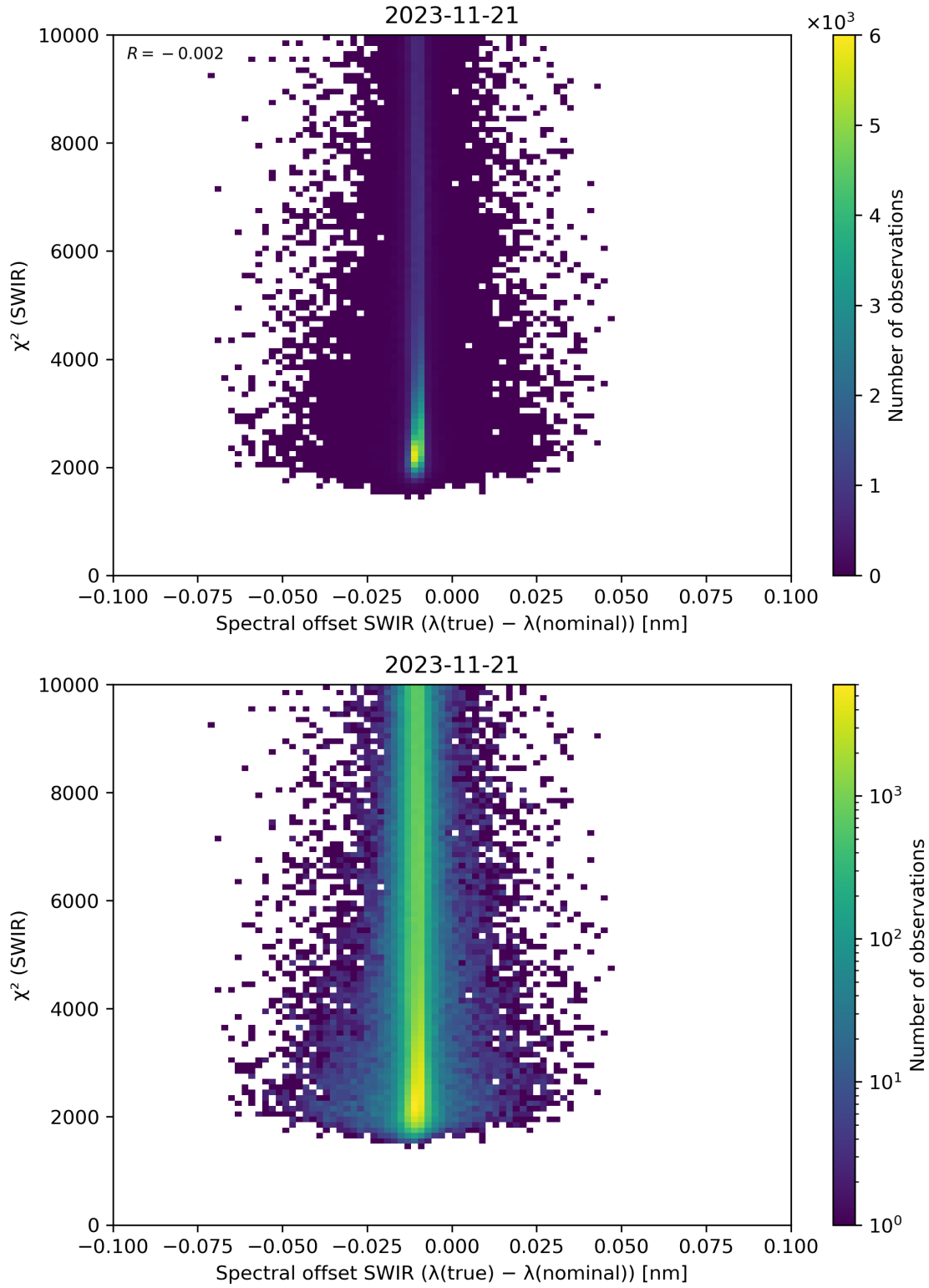
Figure 118: Scatter density plot of “Spectral offset SWIR ( \lambda(\text{true}) - \lambda(\text{nominal}) )” against “ \chi^2 (SWIR)” for 2023-11-20 to 2023-11-22.
