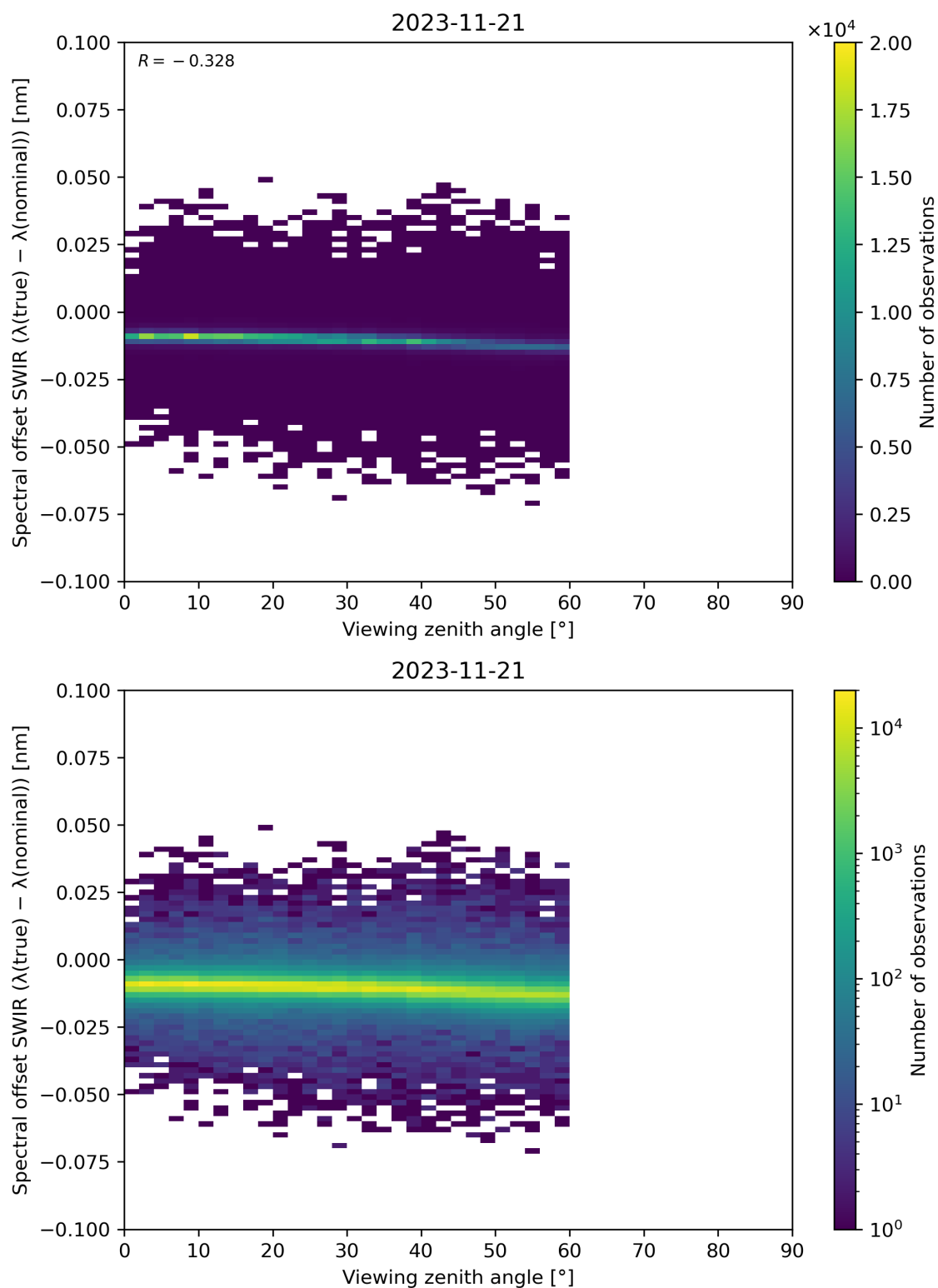
Figure 116: Scatter density plot of “Viewing zenith angle” against “Spectral offset SWIR ( \lambda(\text{true}) - \lambda(\text{nominal}) )” for 2023-11-20 to 2023-11-22.
