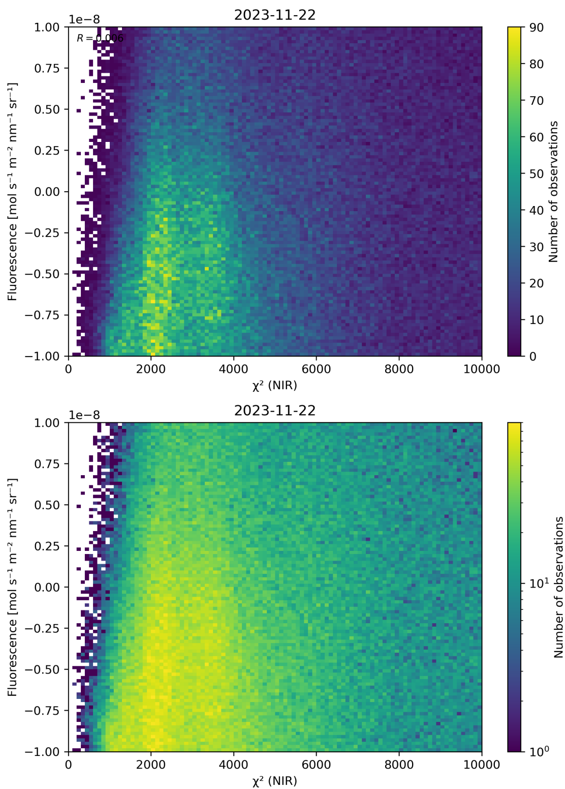
Figure 45: Scatter density plot of “ \chi^2 (NIR)” against “Fluorescence” for 2023-11-21 to 2023-11-23.
