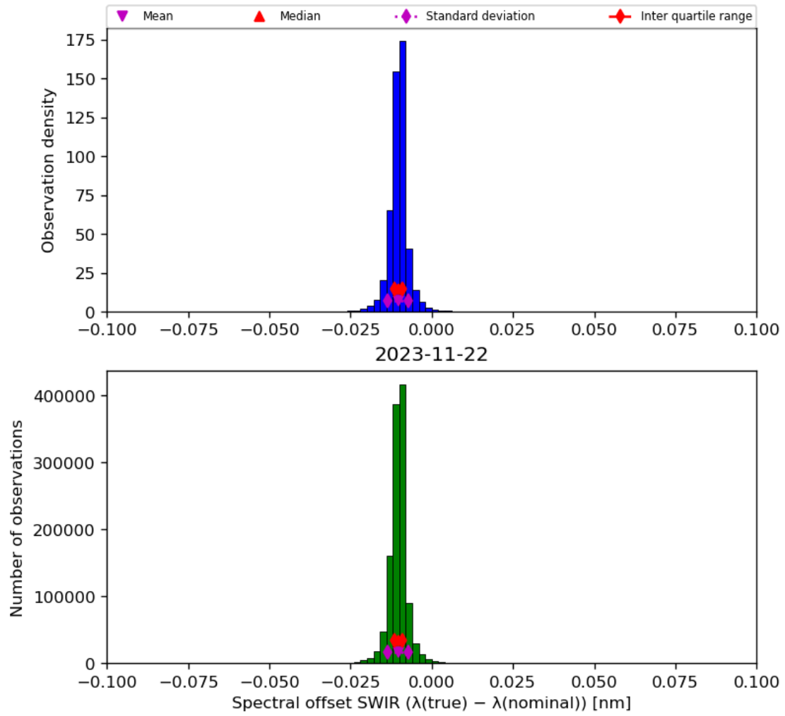
Figure 27: Histogram of “Spectral offset SWIR ( \lambda(\text{true}) - \lambda(\text{nominal}) )” for 2023-11-21 to 2023-11-23
