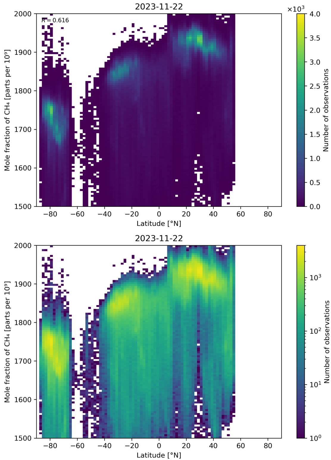
Figure 57: Scatter density plot of “Latitude” against “Mole fraction of CH 4 ” for 2023-11-21 to 2023-11-23.
