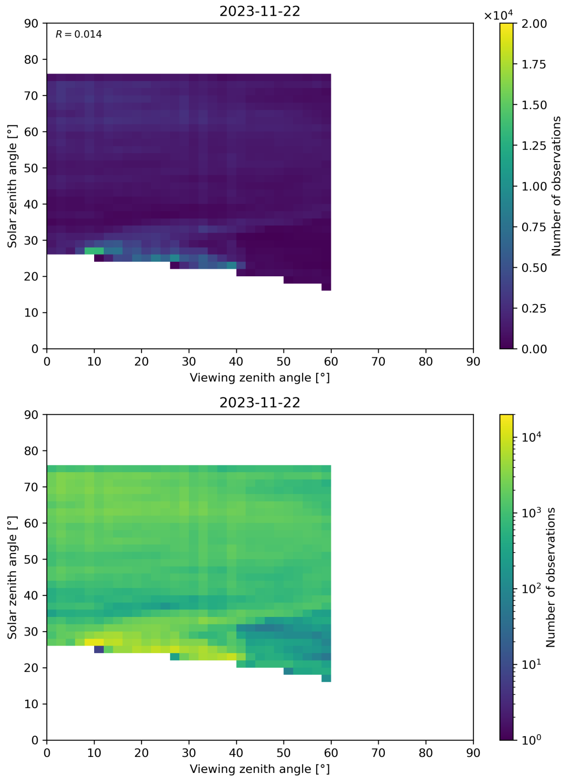
Figure 115: Scatter density plot of “Viewing zenith angle” against “Solar zenith angle” for 2023-11-21 to 2023-11-23.
