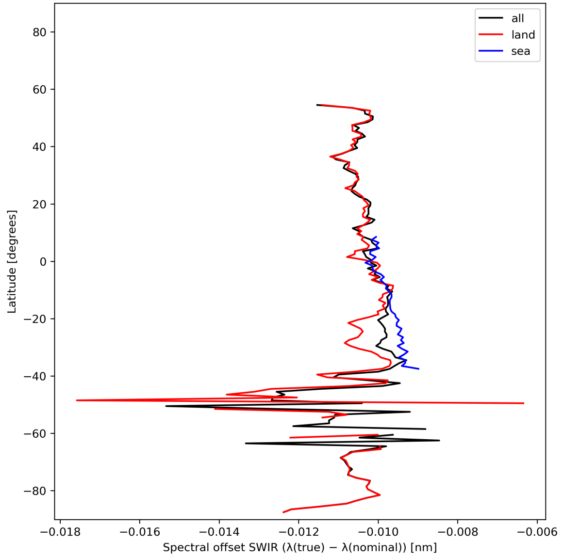
Figure 16: Zonal average of “Spectral offset SWIR ( \lambda(\text{true}) - \lambda(\text{nominal}) )” for 2023-11-21 to 2023-11-23.
