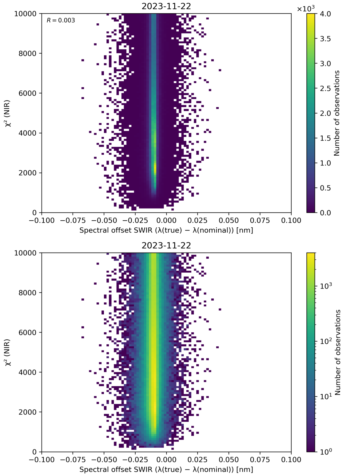
Figure 117: Scatter density plot of “Spectral offset SWIR ( \lambda(\text{true}) - \lambda(\text{nominal}) )” against “ \chi^2 (NIR)” for 2023-11-21 to 2023-11-23.
