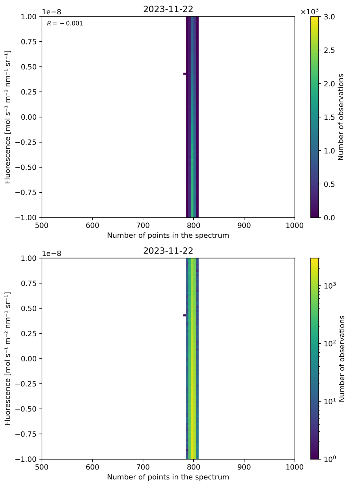
Figure 91: Scatter density plot of “Number of points in the spectrum” against “Fluorescence” for 2023-11-21 to 2023-11-23.
