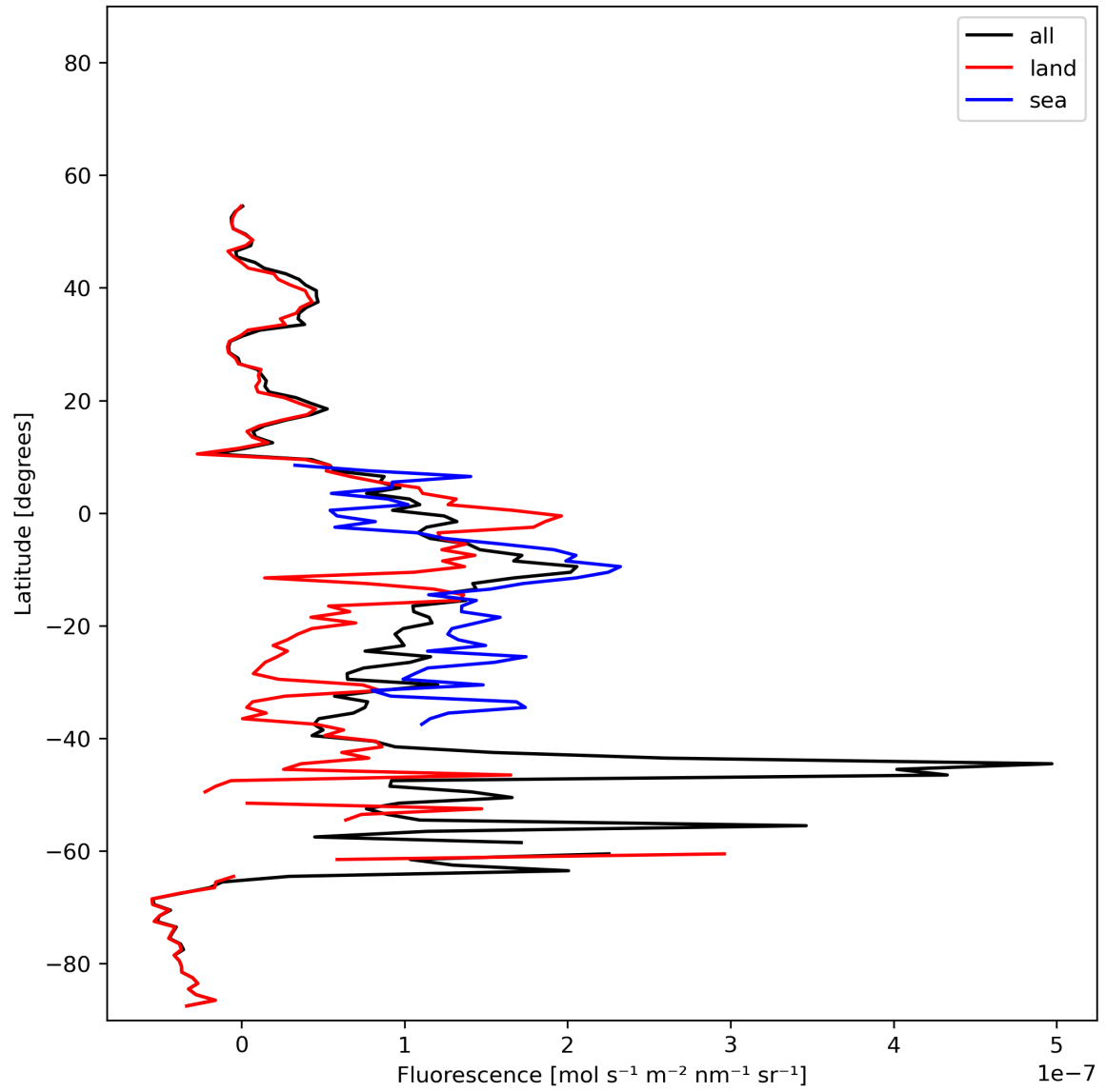
Figure 21: Zonal average of “Fluorescence” for 2023-11-21 to 2023-11-23.
