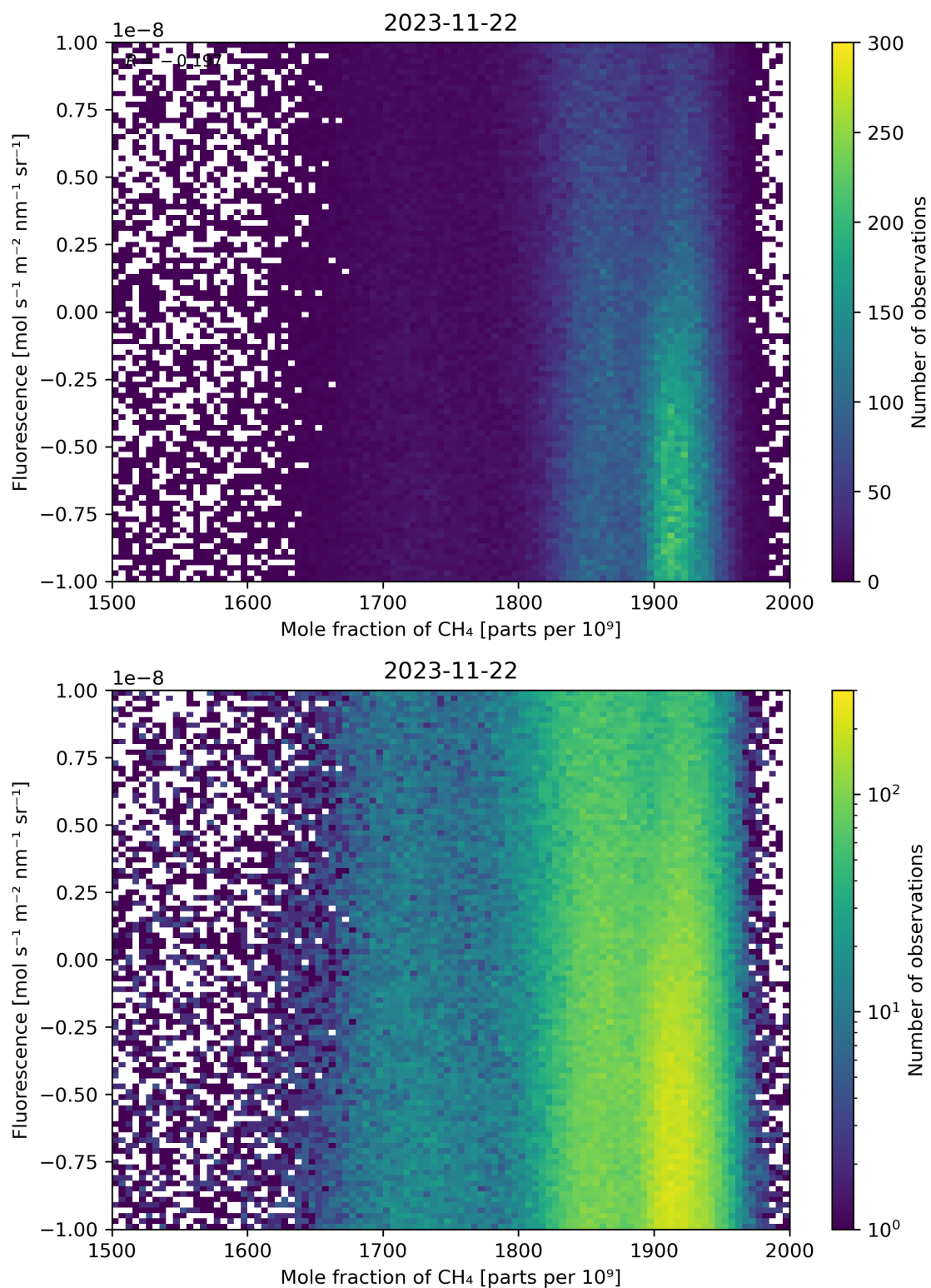
Figure 73: Scatter density plot of “Mole fraction of \text{CH}_4 ” against “Fluorescence” for 2023-11-21 to 2023-11-23.
