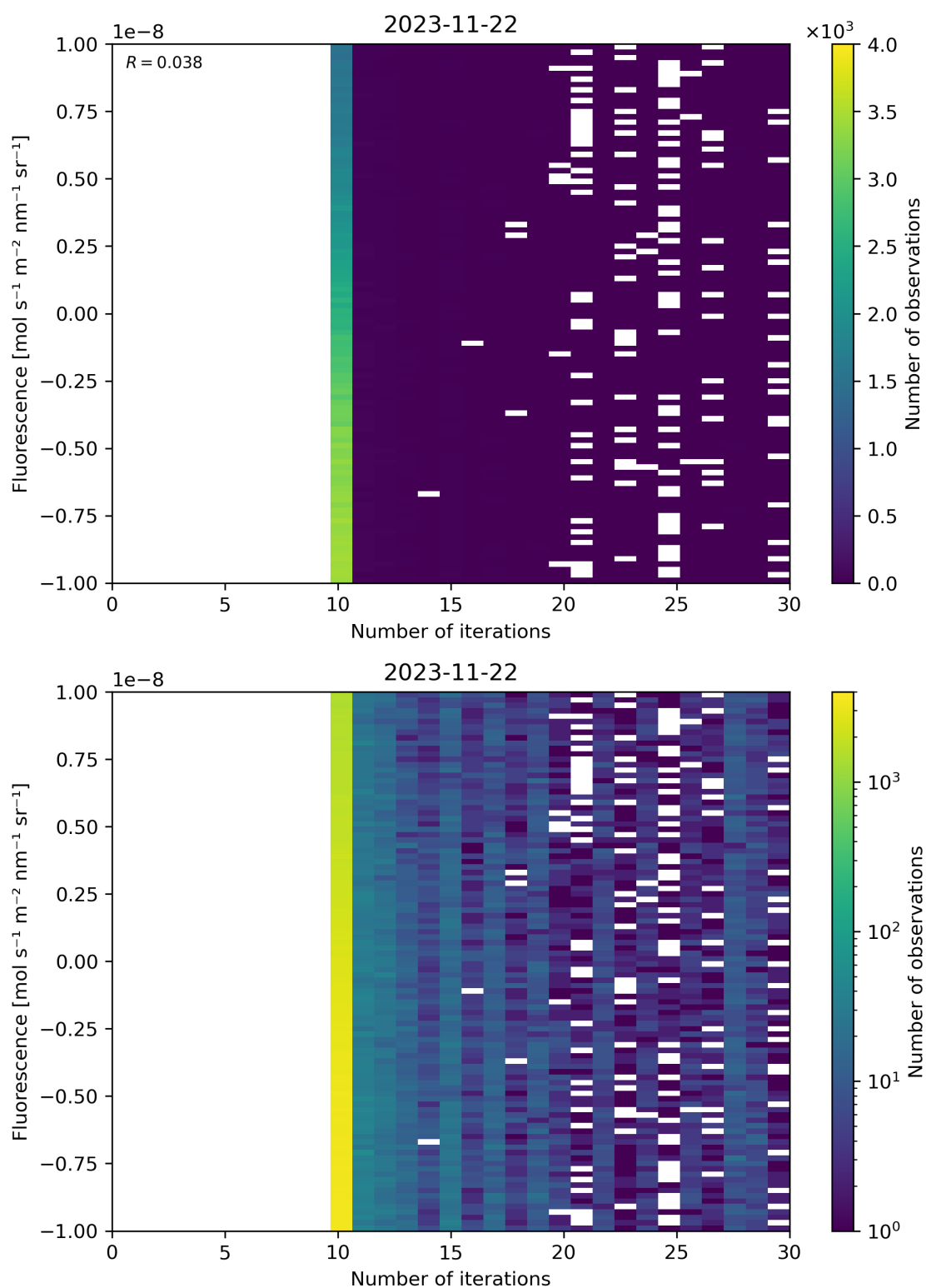
Figure 87: Scatter density plot of “Number of iterations” against “Fluorescence” for 2023-11-21 to 2023-11-23.
