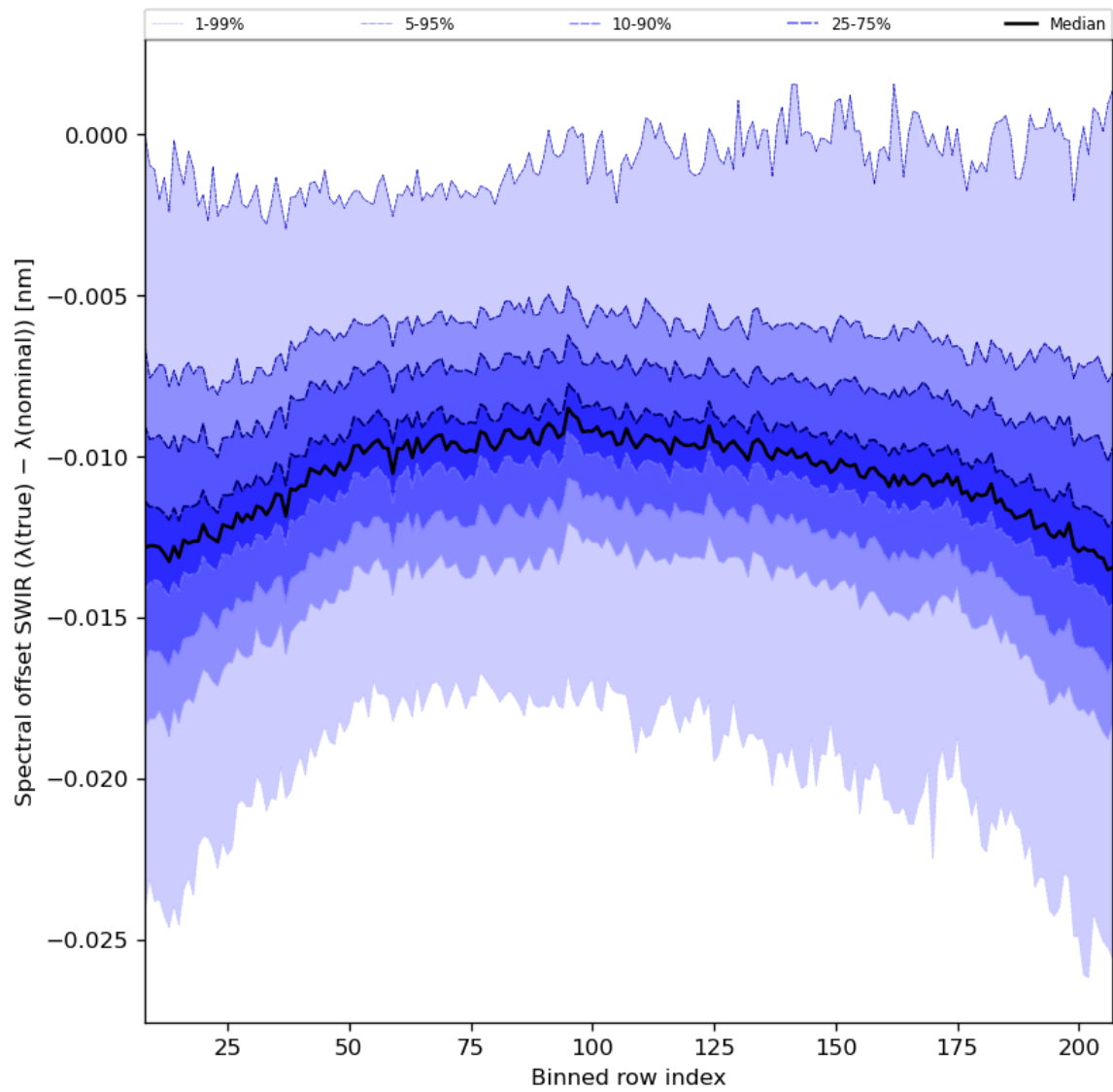
Figure 38: Along track statistics of “Spectral offset SWIR ( \lambda(\text{true}) - \lambda(\text{nominal}) )” for 2023-11-21 to 2023-11-23
