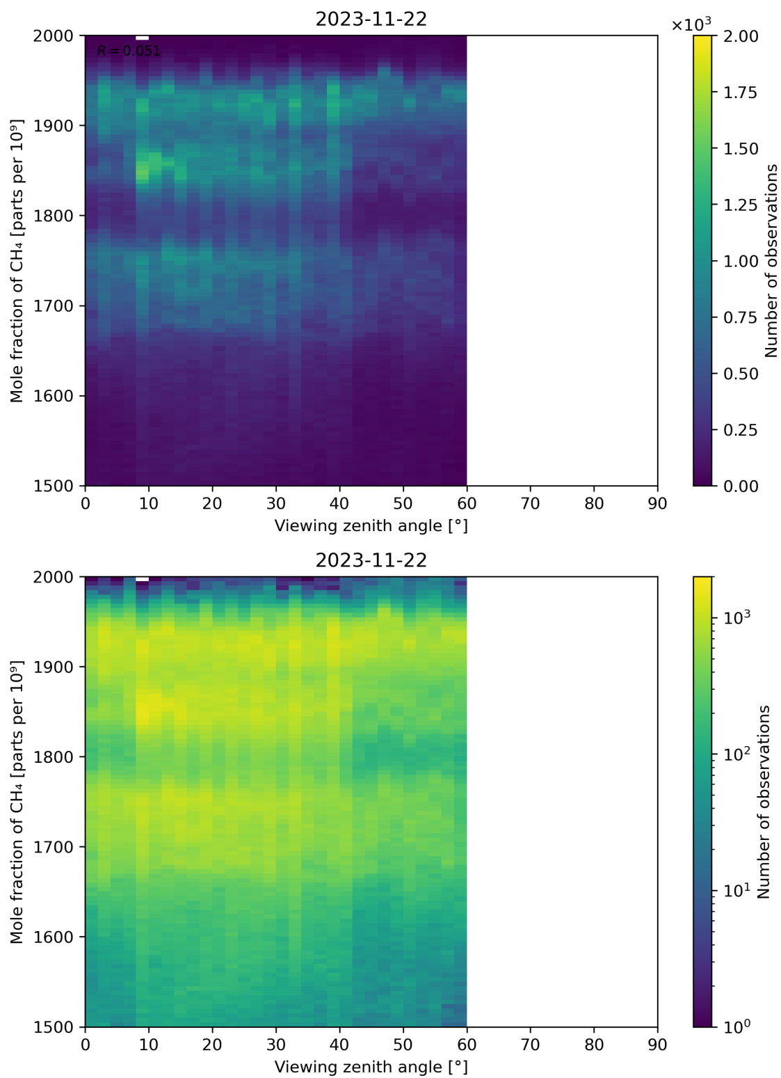
Figure 110: Scatter density plot of “Viewing zenith angle” against “Mole fraction of CH 4 ” for 2023-11-21 to 2023-11-23.
