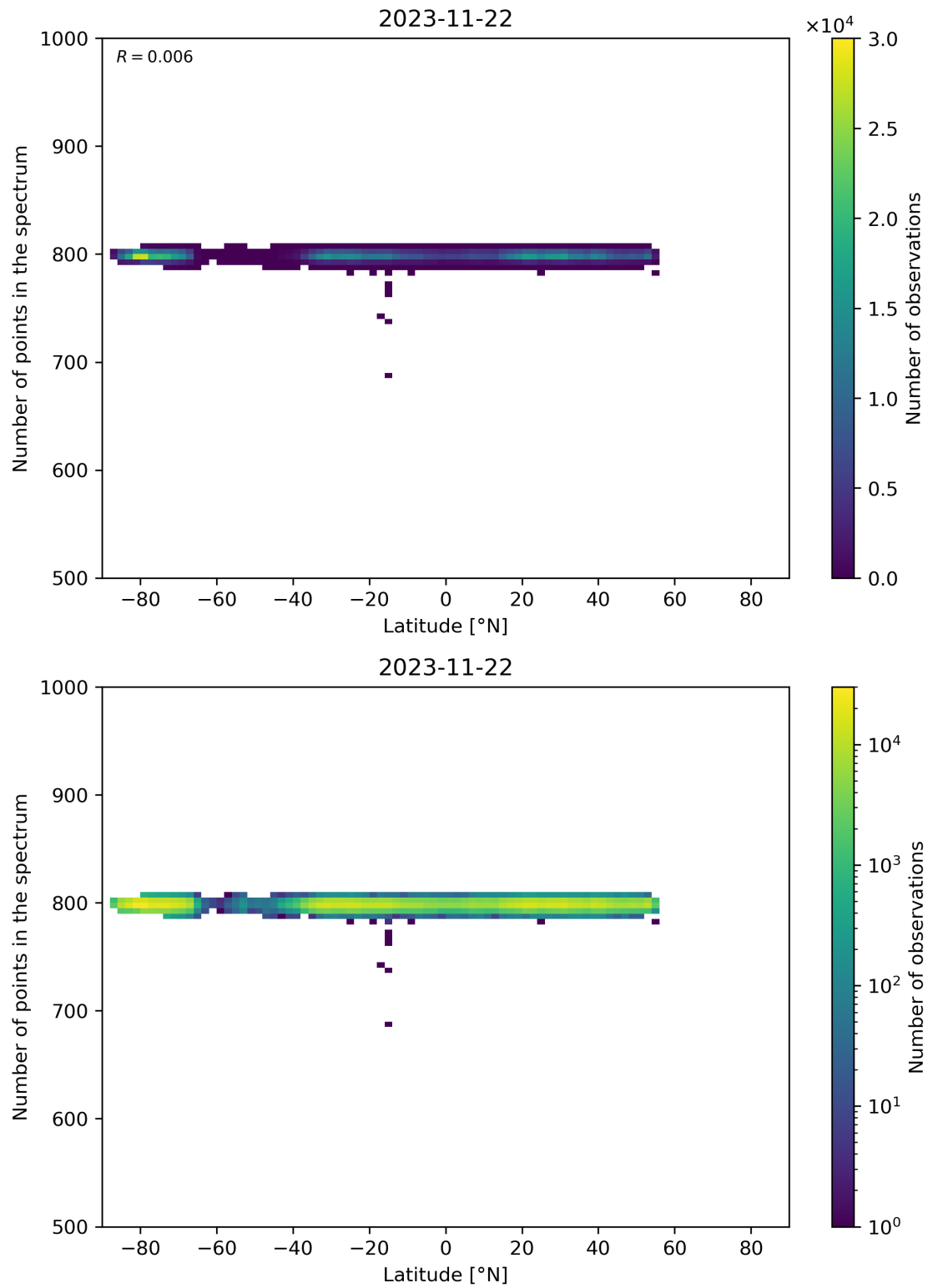
Figure 61: Scatter density plot of “Latitude” against “Number of points in the spectrum” for 2023-11-21 to 2023-11-23.
