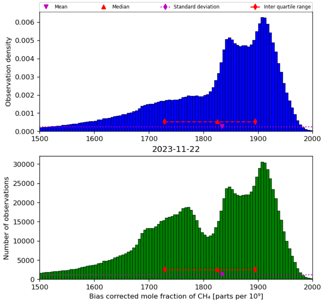
Figure 25: Histogram of “Bias corrected mole fraction of CH 4 ” for 2023-11-21 to 2023-11-23
