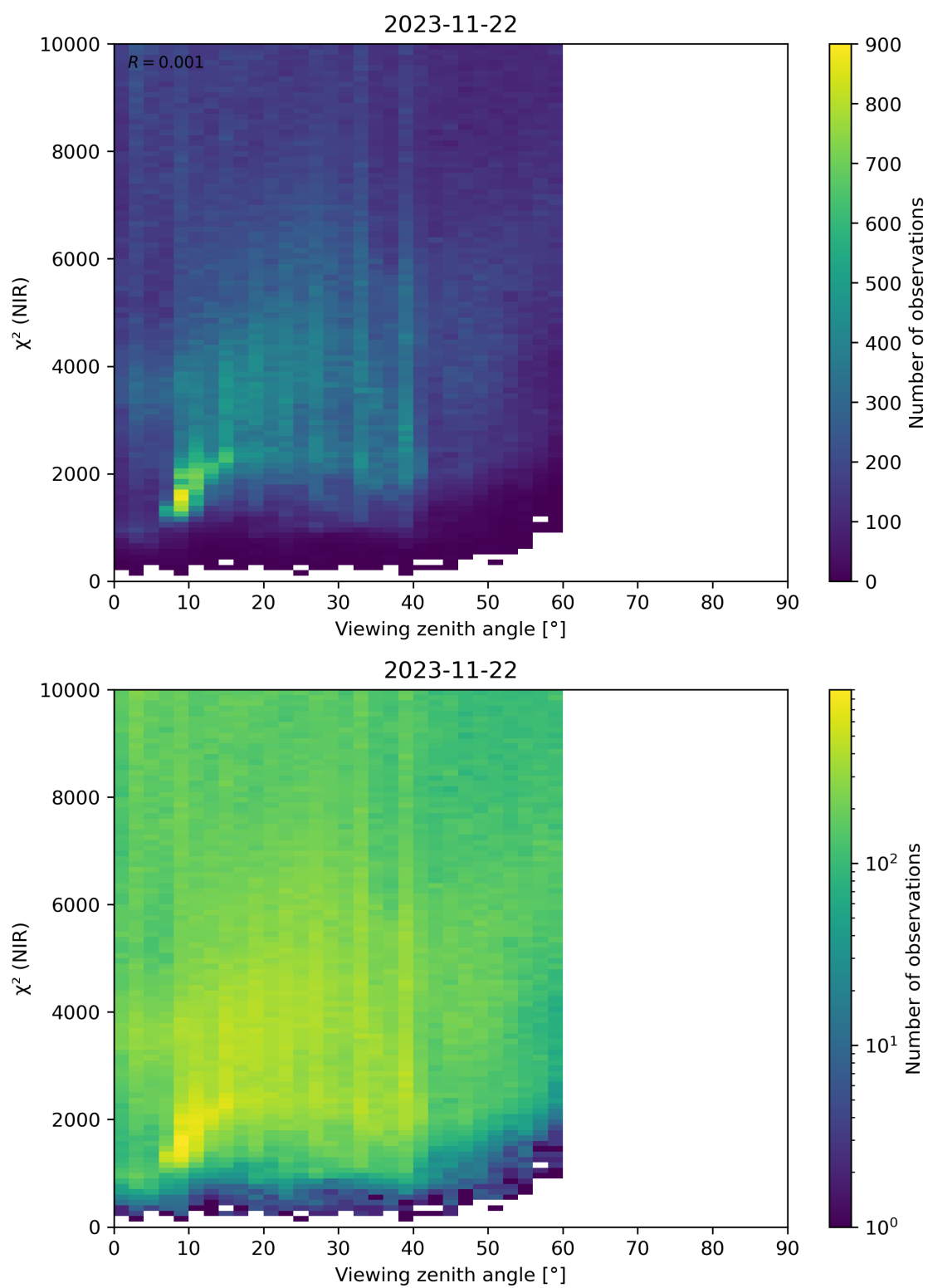
Figure 105: Scatter density plot of “Viewing zenith angle” against “ \chi^2 (NIR)” for 2023-11-21 to 2023-11-23.
