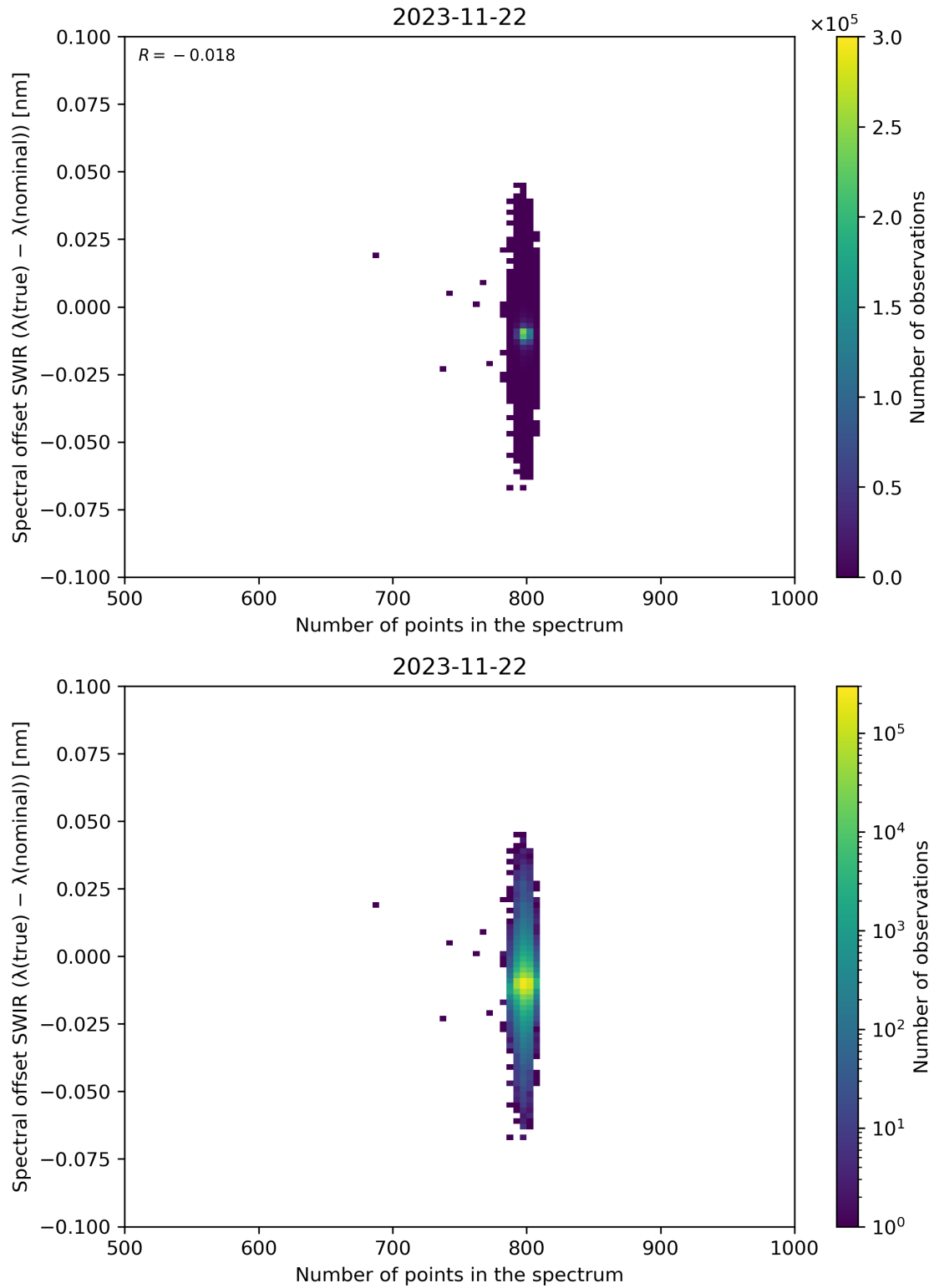
Figure 93: Scatter density plot of “Number of points in the spectrum” against “Spectral offset SWIR ( \lambda(\text{true}) - \lambda(\text{nominal}) )” for 2023-11-21 to 2023-11-23.
