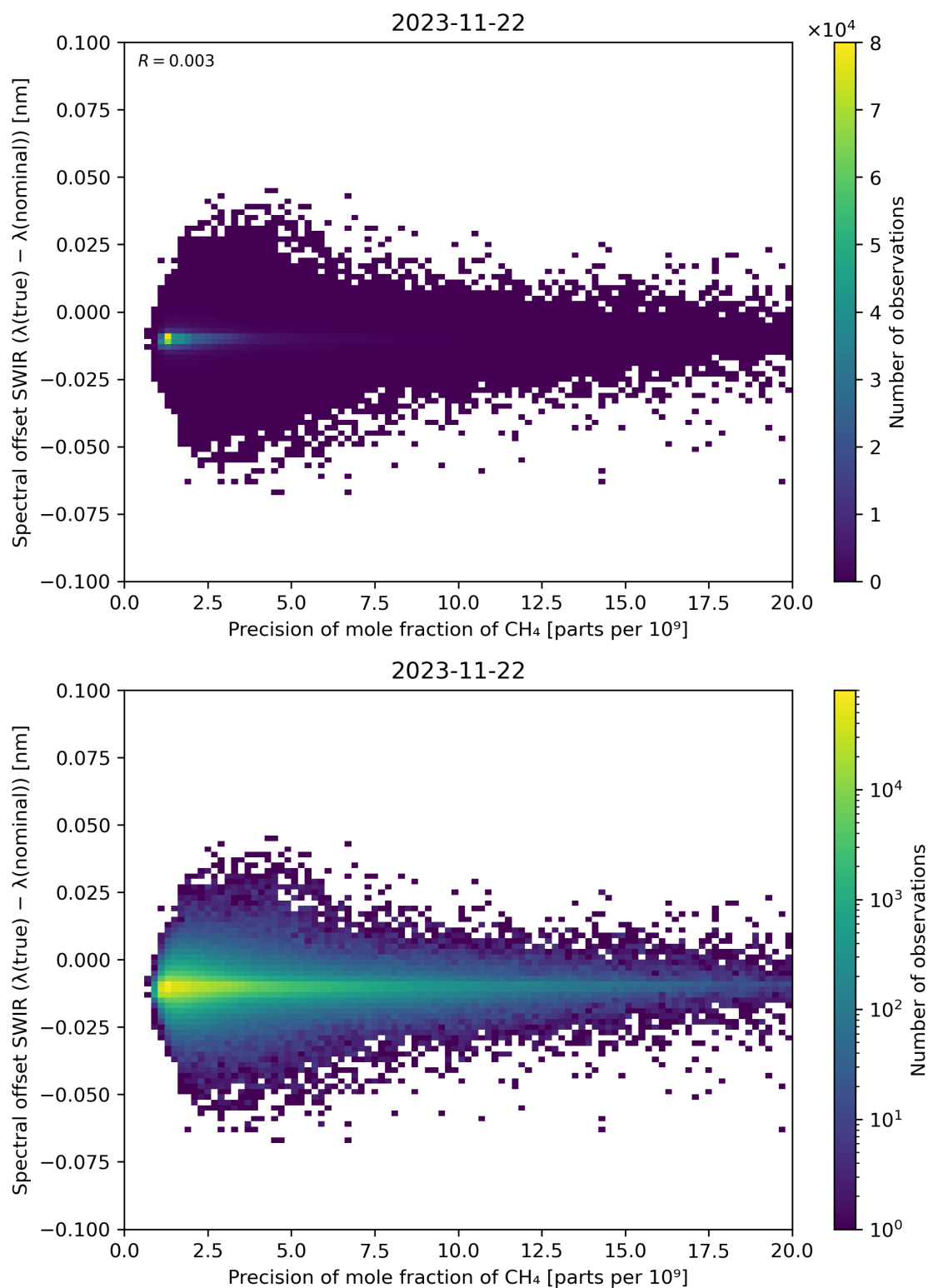
Figure 85: Scatter density plot of “Precision of mole fraction of CH 4 ” against “Spectral offset SWIR ( \lambda(\text{true}) - \lambda(\text{nominal}) )” for 2023-11-21 to 2023-11-23.
