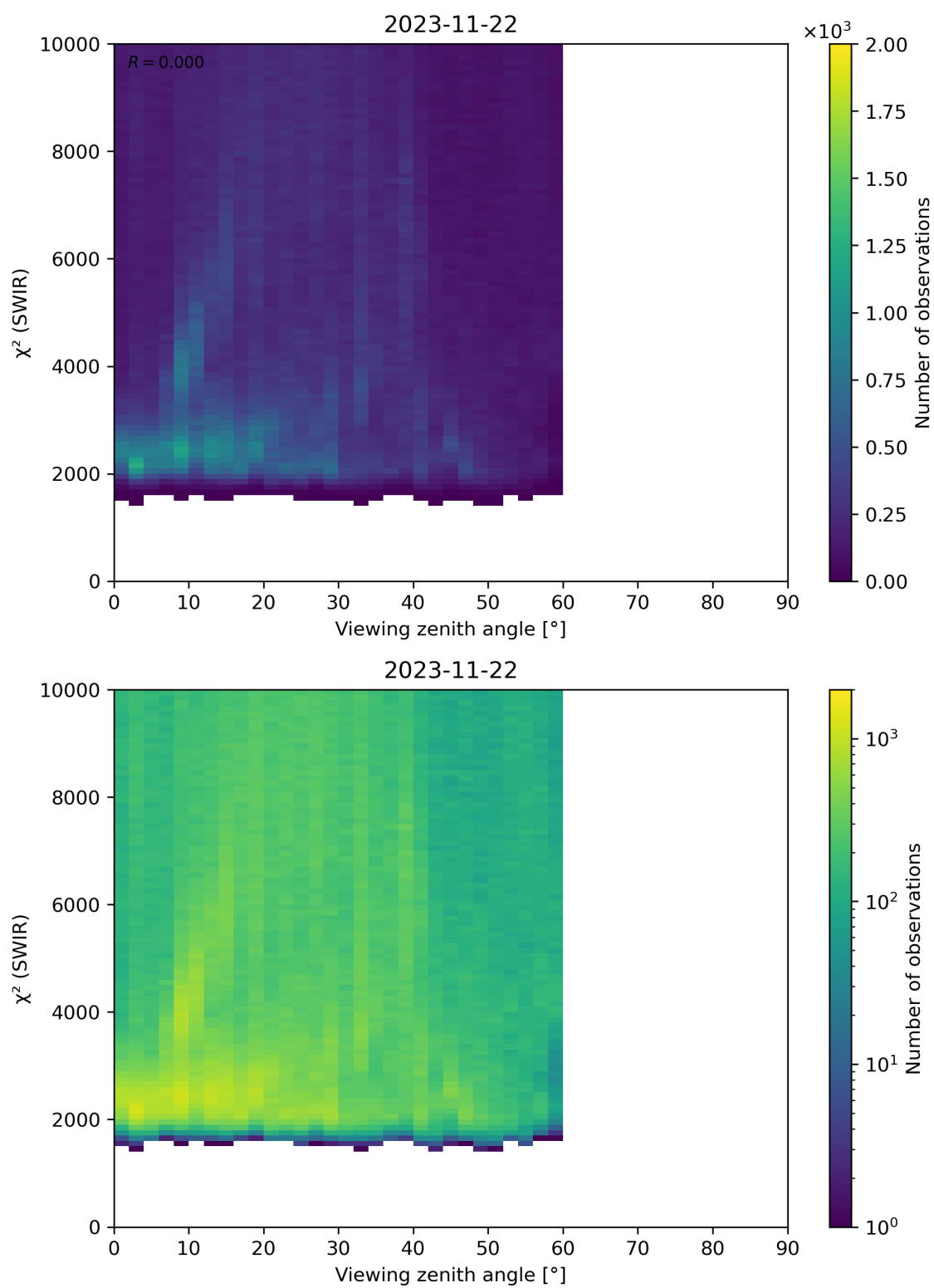
Figure 106: Scatter density plot of “Viewing zenith angle” against “ \chi^2 (SWIR)” for 2023-11-21 to 2023-11-23.
