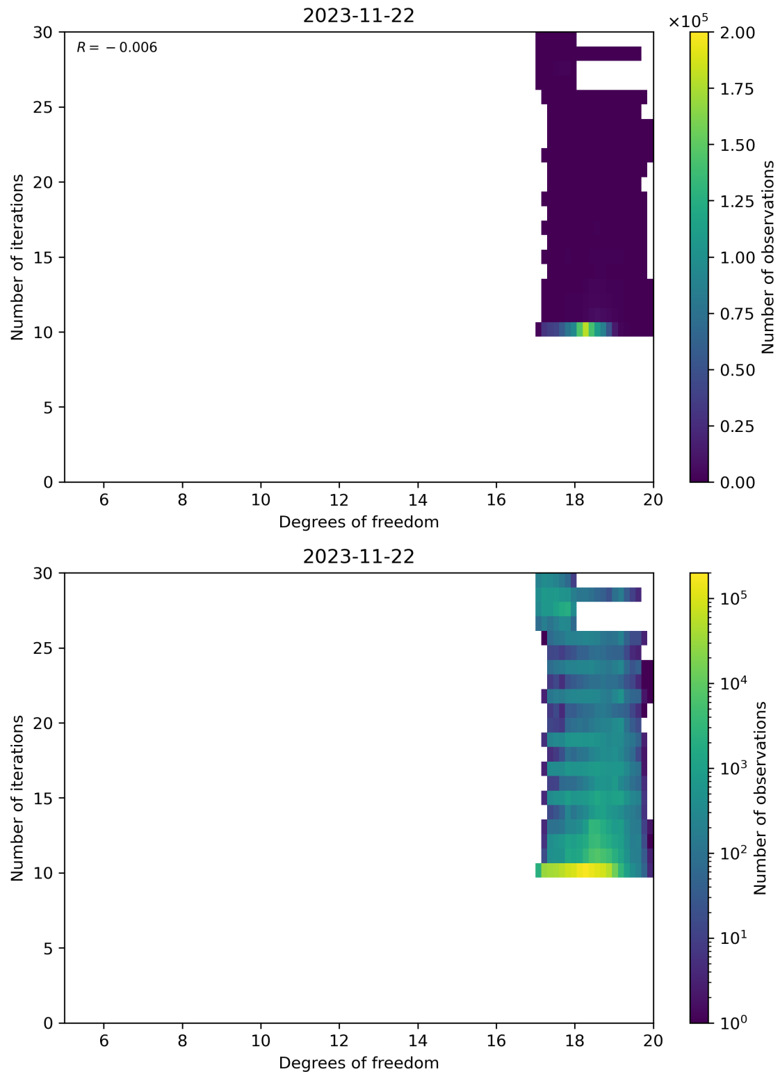
Figure 52: Scatter density plot of “Degrees of freedom” against “Number of iterations” for 2023-11-21 to 2023-11-23.
