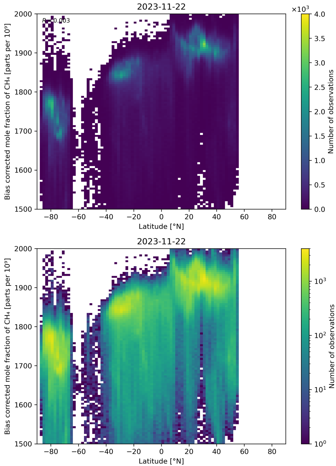
Figure 58: Scatter density plot of “Latitude” against “Bias corrected mole fraction of CH 4 ” for 2023-11-21 to 2023-11-23.
