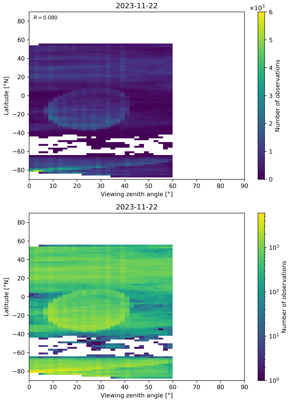
Figure 109: Scatter density plot of “Viewing zenith angle” against “Latitude” for 2023-11-21 to 2023-11-23.
