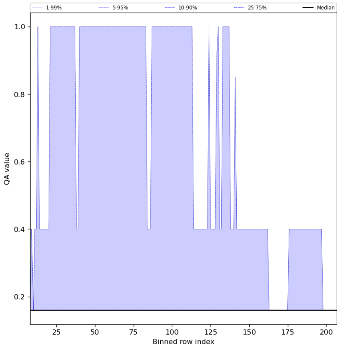
Figure 33: Along track statistics of “QA value” for 2023-11-21 to 2023-11-23
