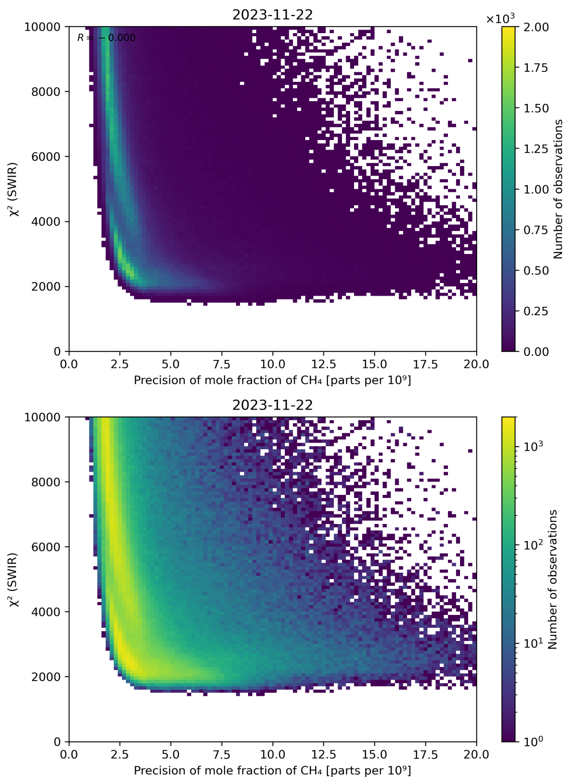
Figure 79: Scatter density plot of “Precision of mole fraction of \text{CH}_4 ” against “ \chi^2 (SWIR)” for 2023-11-21 to 2023-11-23.
