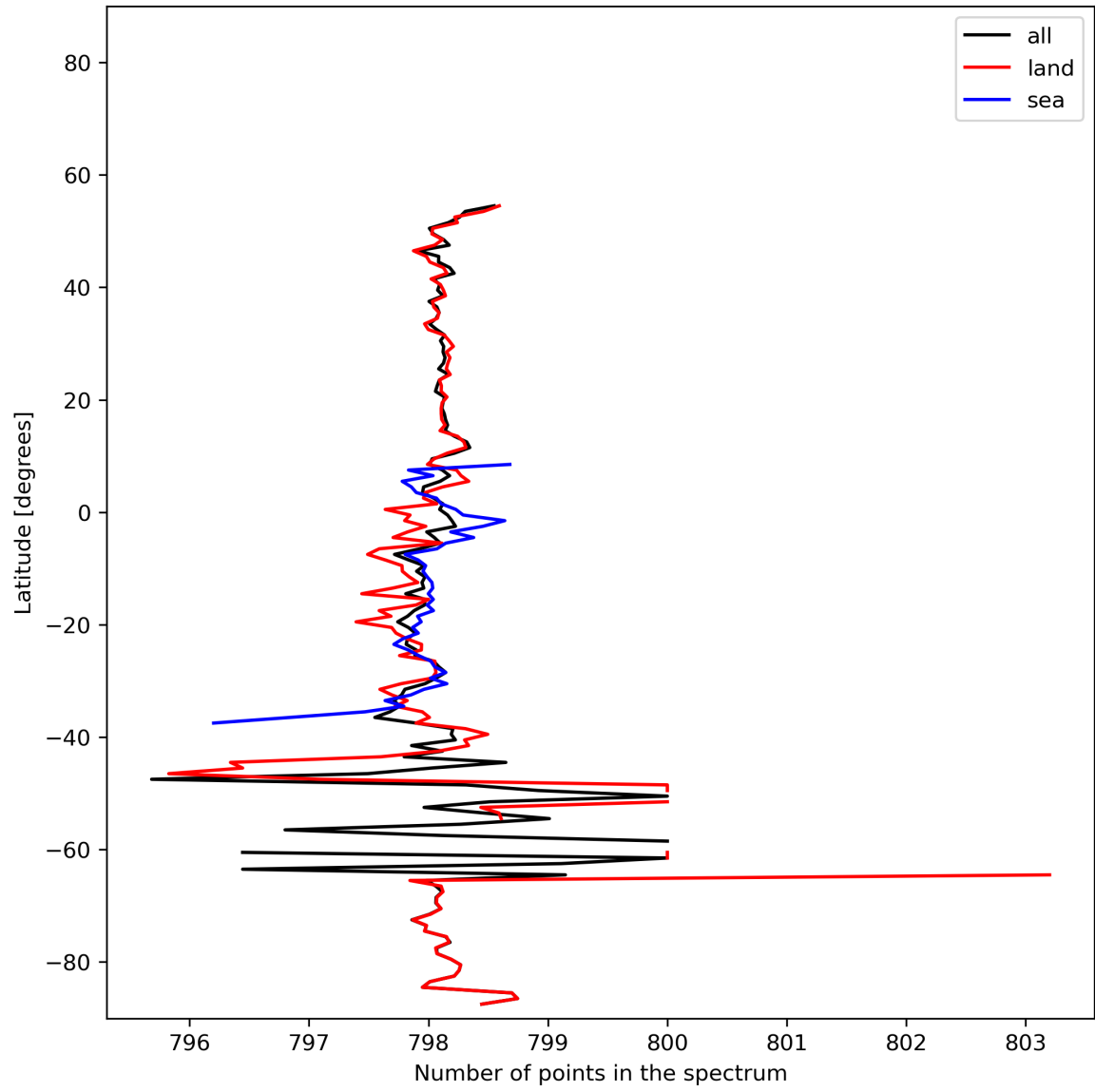
Figure 15: Zonal average of “Number of points in the spectrum” for 2023-11-21 to 2023-11-23.
