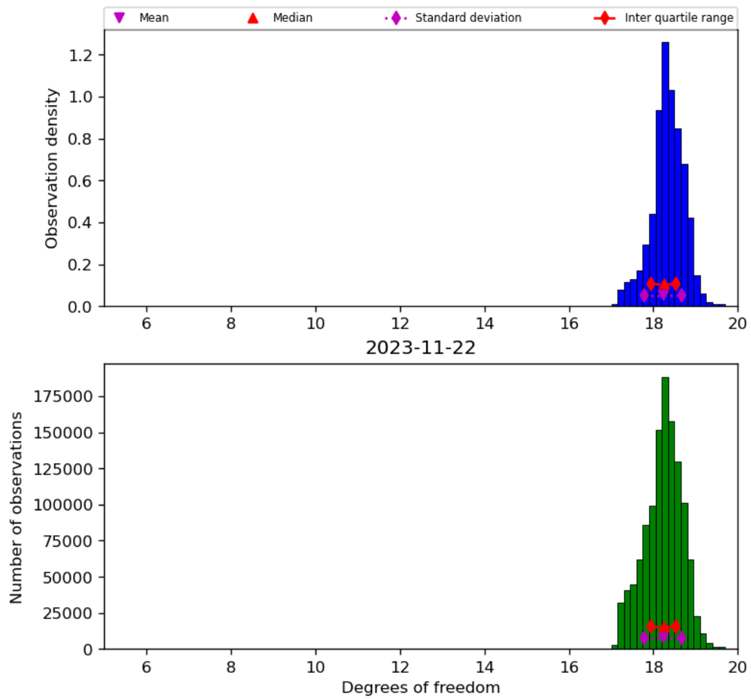
Figure 30: Histogram of “Degrees of freedom” for 2023-11-21 to 2023-11-23
