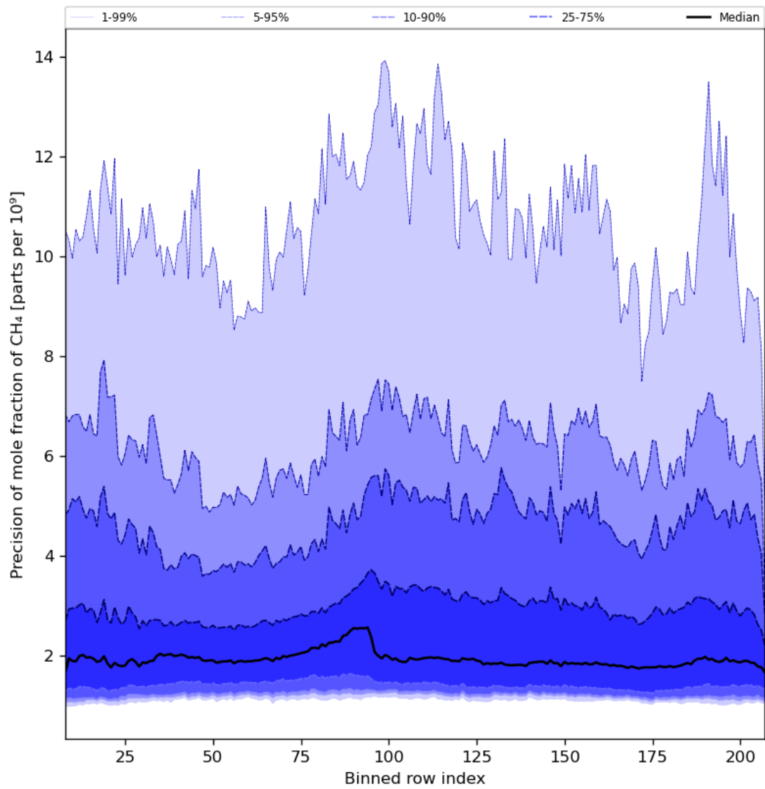
Figure 35: Along track statistics of “Precision of mole fraction of CH 4 ” for 2023-11-21 to 2023-11-23
