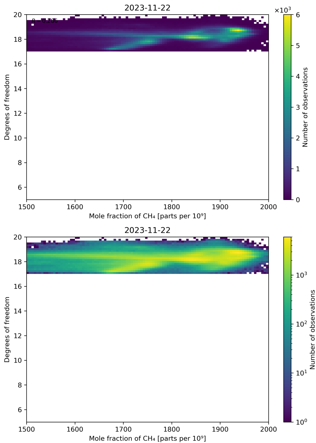
Figure 72: Scatter density plot of “Mole fraction of CH 4 ” against “Degrees of freedom” for 2023-11-21 to 2023-11-23.
