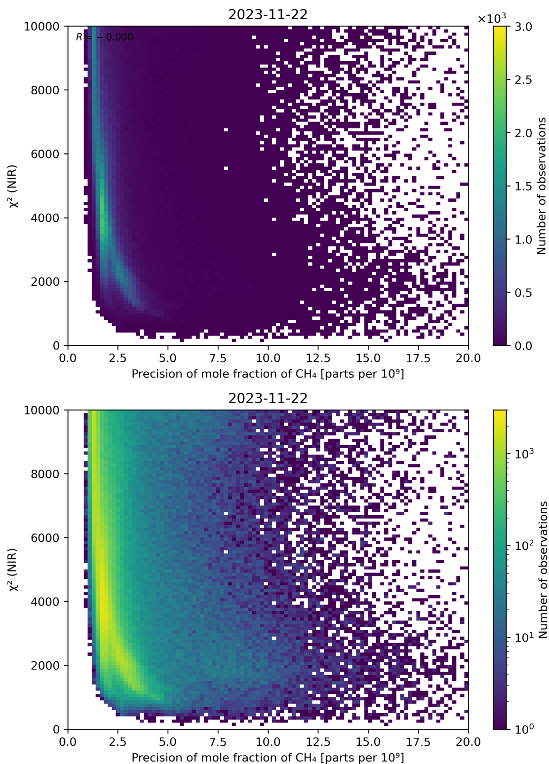
Figure 78: Scatter density plot of “Precision of mole fraction of CH 4 ” against “ \chi^2 (NIR)” for 2023-11-21 to 2023-11-23.
