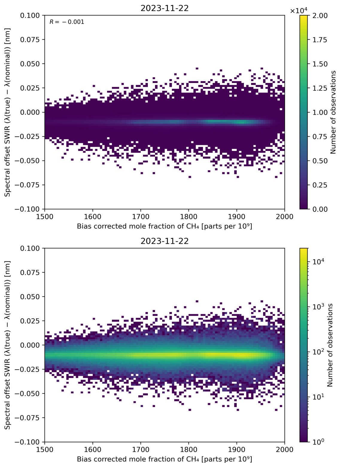
Figure 69: Scatter density plot of “Bias corrected mole fraction of \text{CH}_4 ” against “Spectral offset SWIR ( \lambda(\text{true}) - \lambda(\text{nominal}) )” for 2023-11-21 to 2023-11-23.
