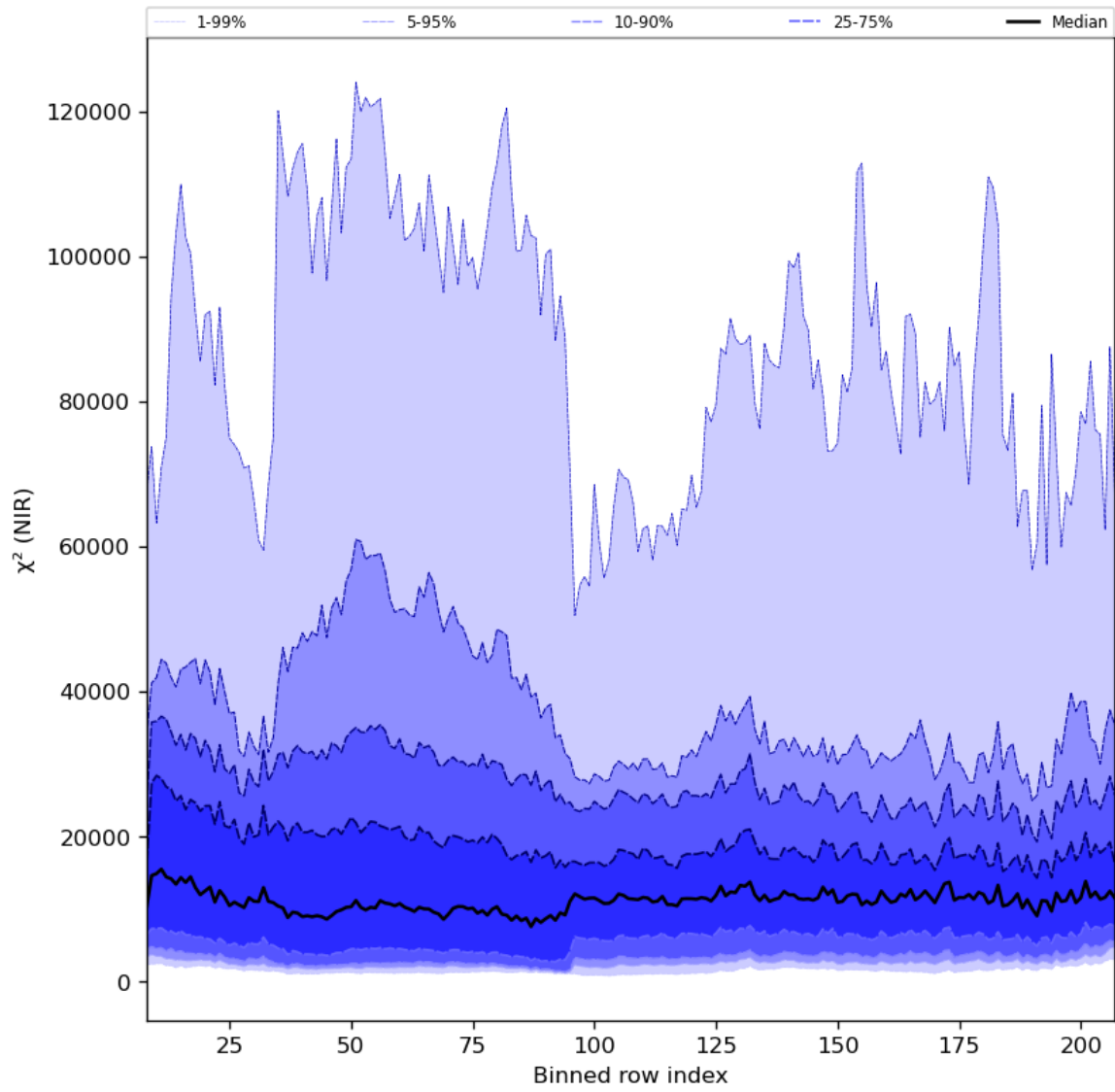
Figure 40: Along track statistics of “ \chi^2 (NIR)” for 2023-11-21 to 2023-11-23
