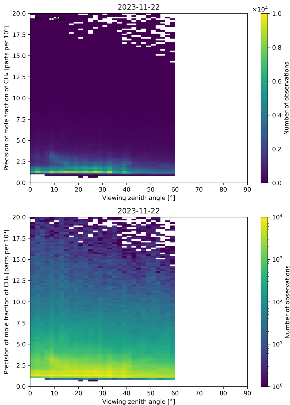
Figure 112: Scatter density plot of “Viewing zenith angle” against “Precision of mole fraction of CH 4 ” for 2023-11-21 to 2023-11-23.
