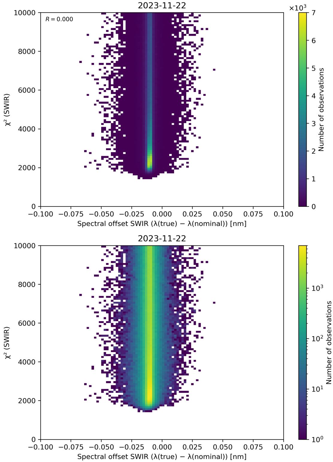
Figure 118: Scatter density plot of “Spectral offset SWIR ( \lambda(\text{true}) - \lambda(\text{nominal}) )” against “ \chi^2 (SWIR)” for 2023-11-21 to 2023-11-23.
