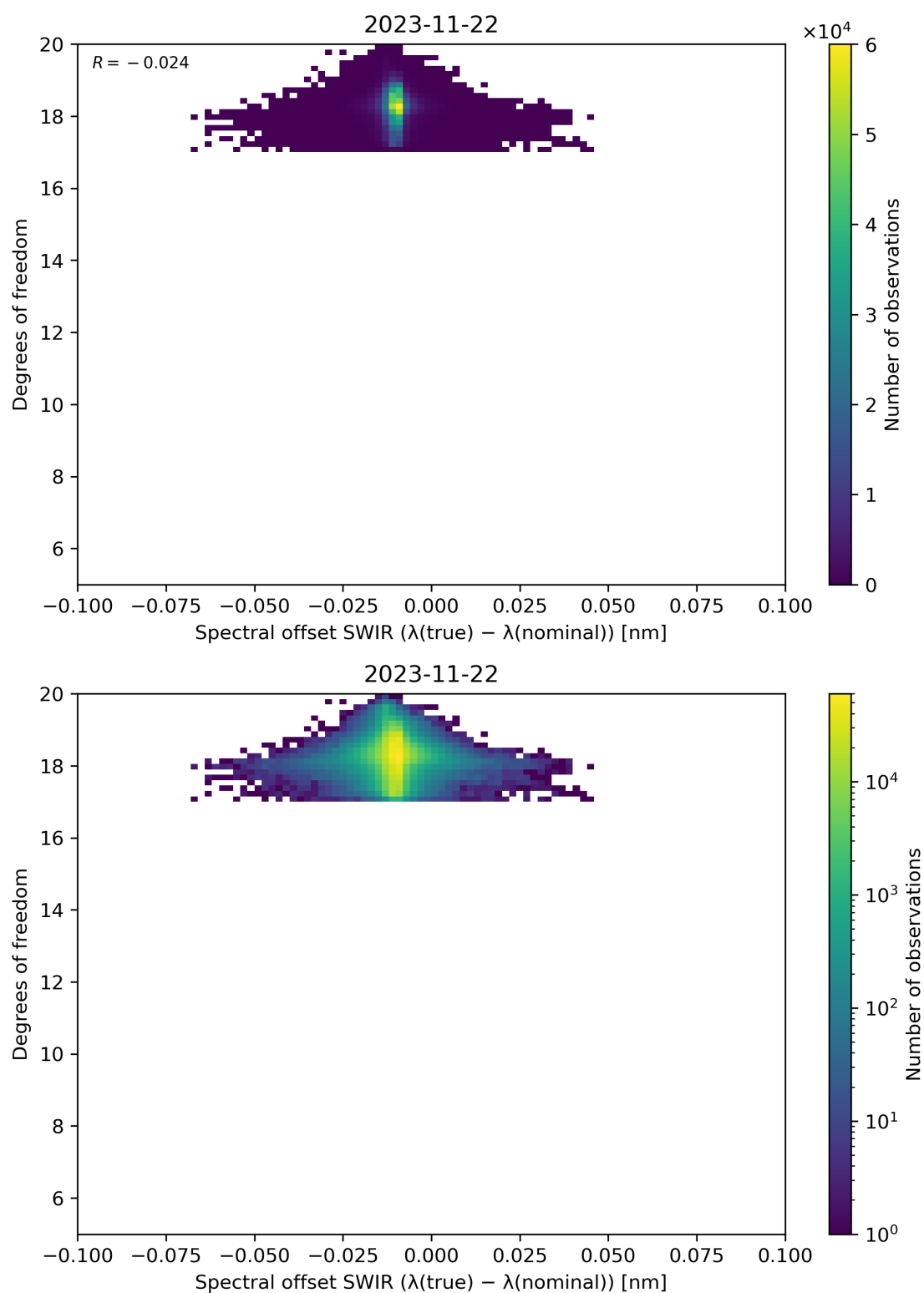
Figure 119: Scatter density plot of “Spectral offset SWIR ( \lambda(\text{true}) - \lambda(\text{nominal}) )” against “Degrees of freedom” for 2023-11-21 to 2023-11-23.
