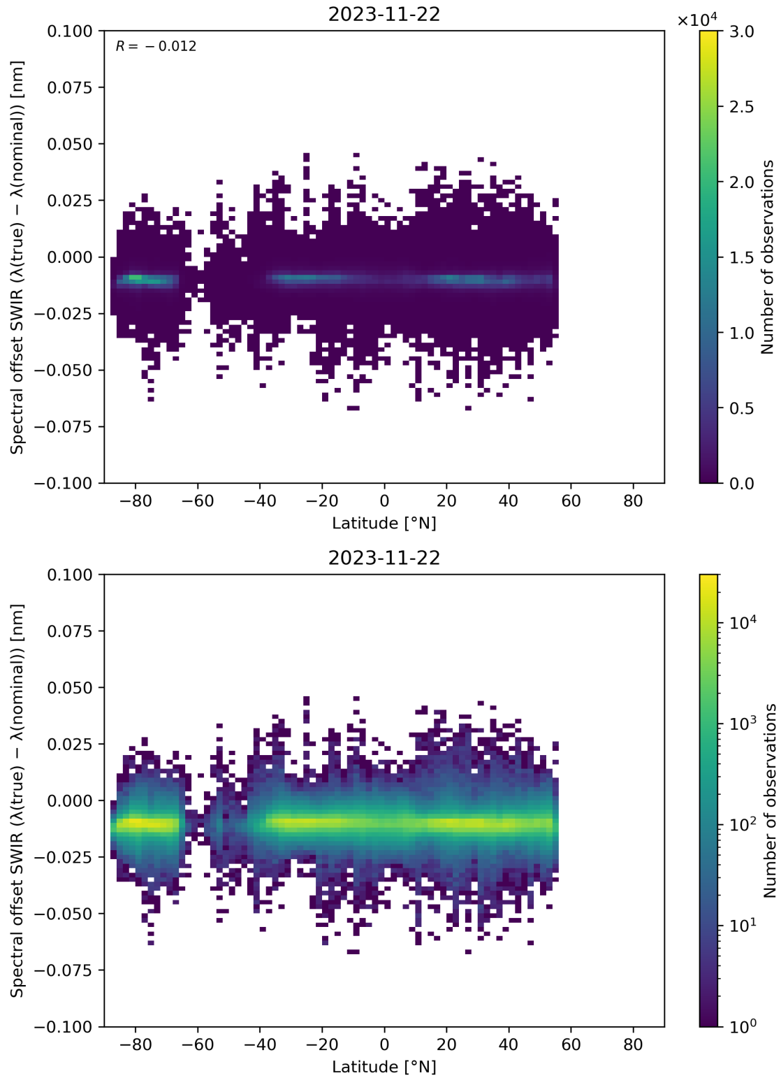
Figure 62: Scatter density plot of “Latitude” against “Spectral offset SWIR ( \lambda(\text{true}) - \lambda(\text{nominal}) )” for 2023-11-21 to 2023-11-23.
