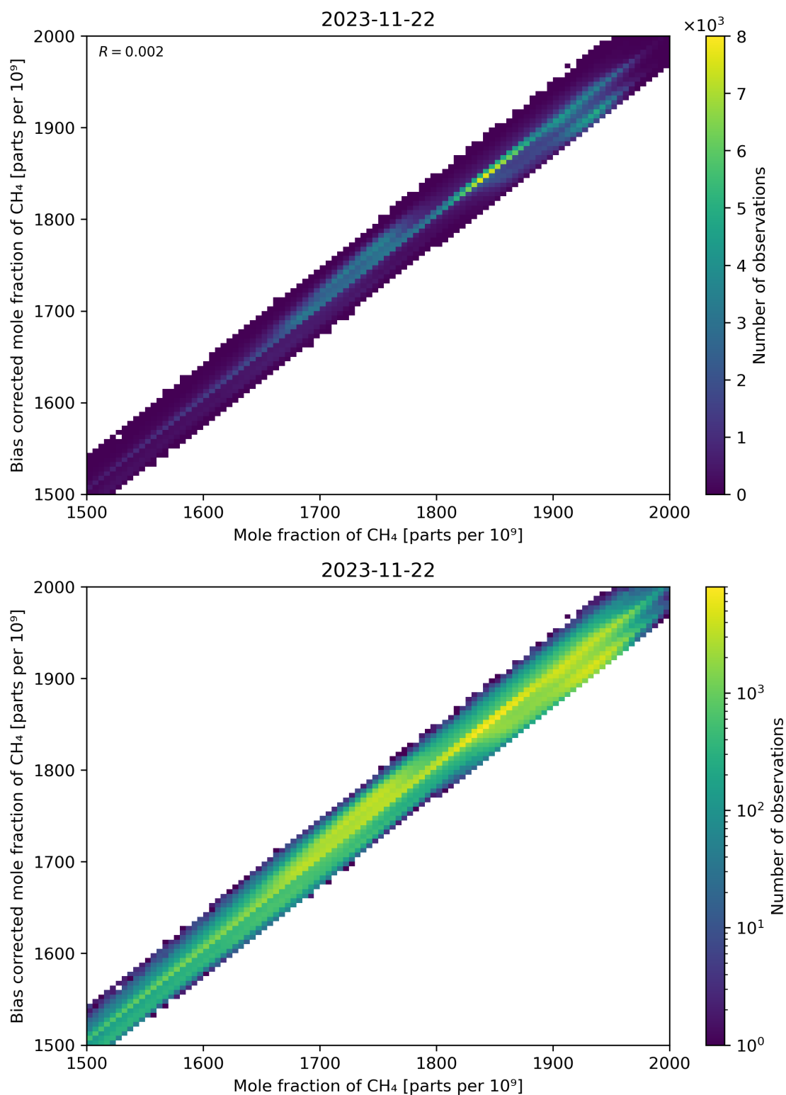
Figure 74: Scatter density plot of “Mole fraction of CH 4 ” against “Bias corrected mole fraction of CH 4 ” for 2023-11-21 to 2023-11-23.
