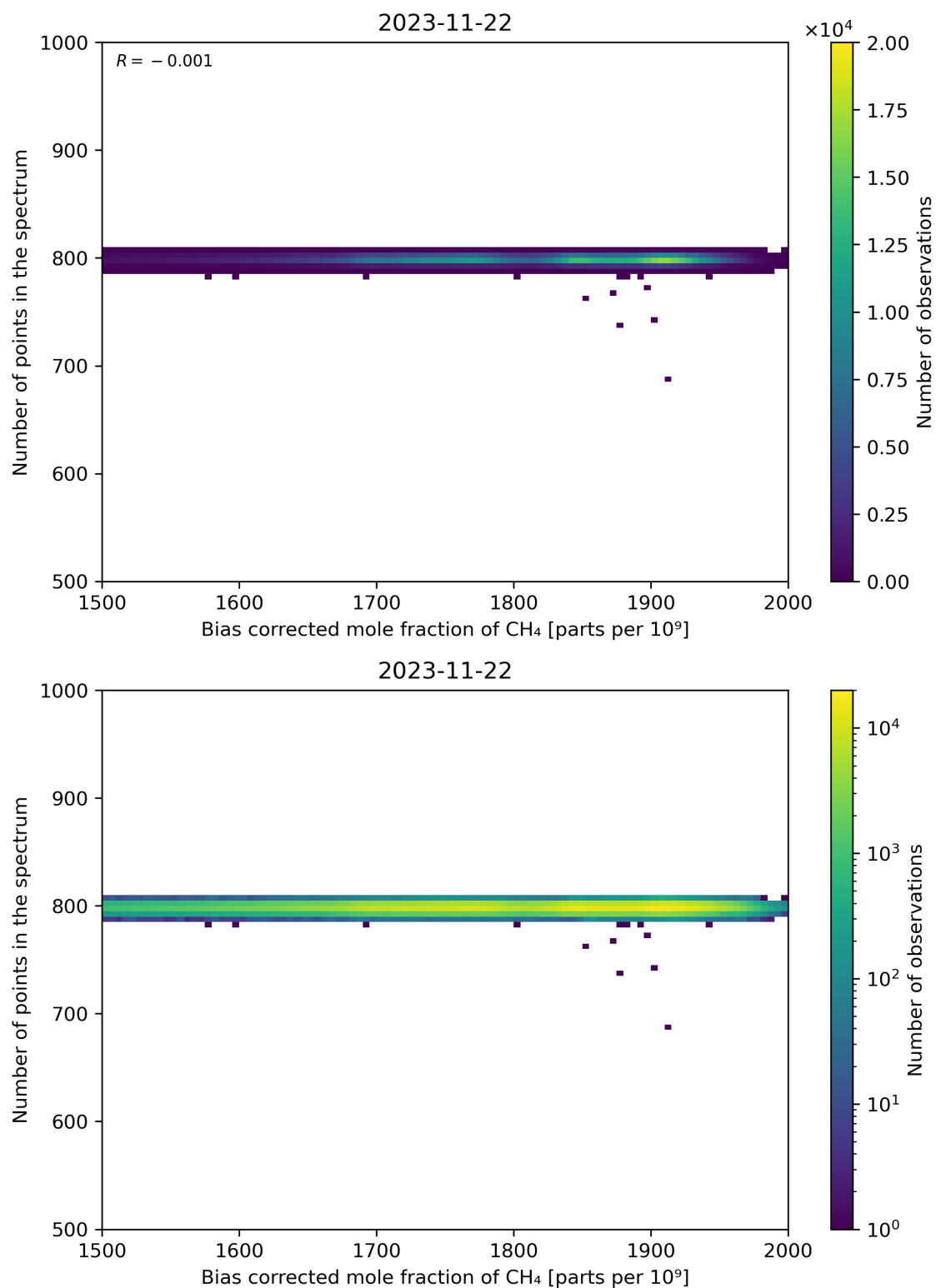
Figure 68: Scatter density plot of “Bias corrected mole fraction of CH 4 ” against “Number of points in the spectrum” for 2023-11-21 to 2023-11-23.
