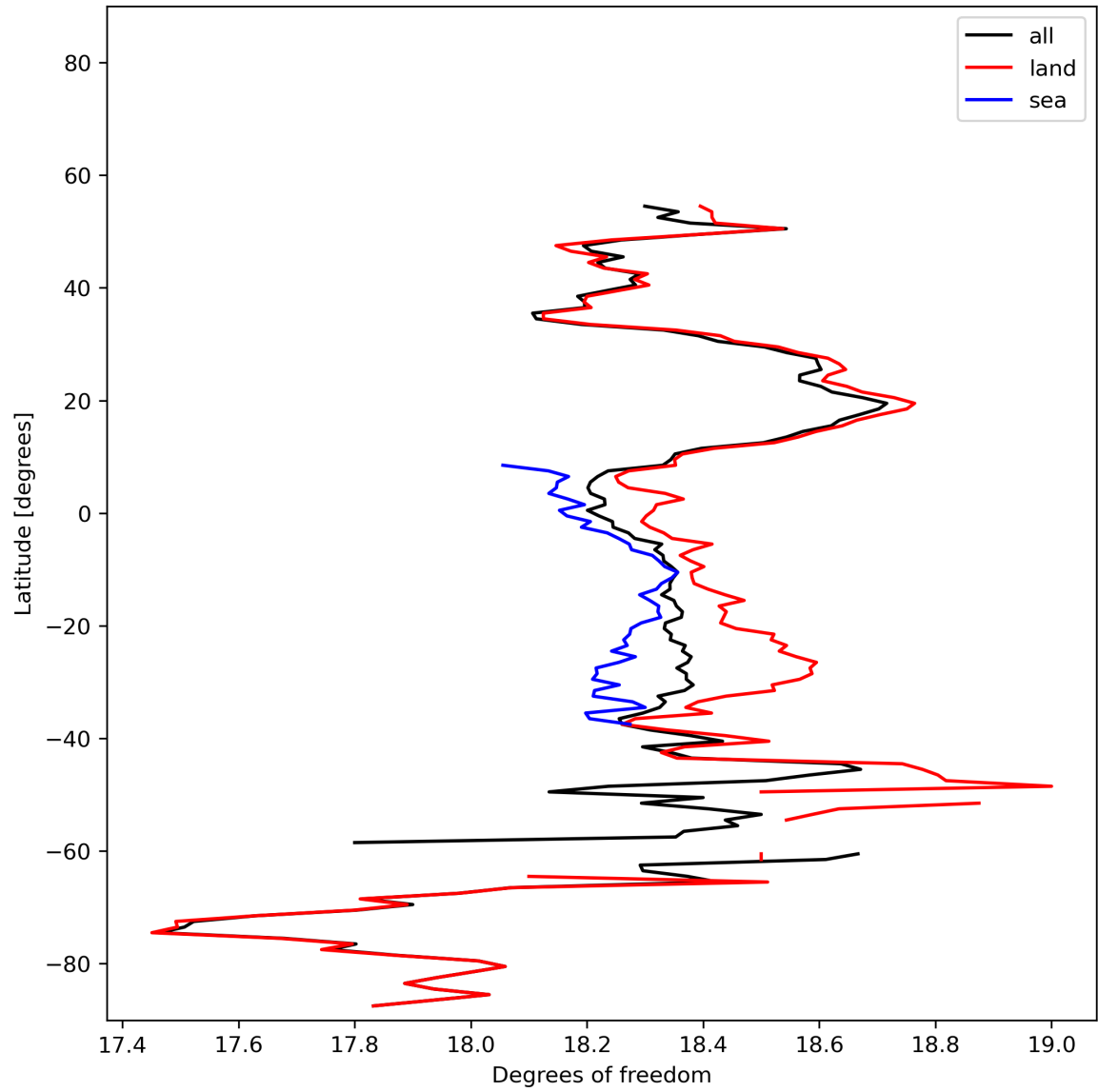
Figure 19: Zonal average of “Degrees of freedom” for 2023-11-21 to 2023-11-23.
