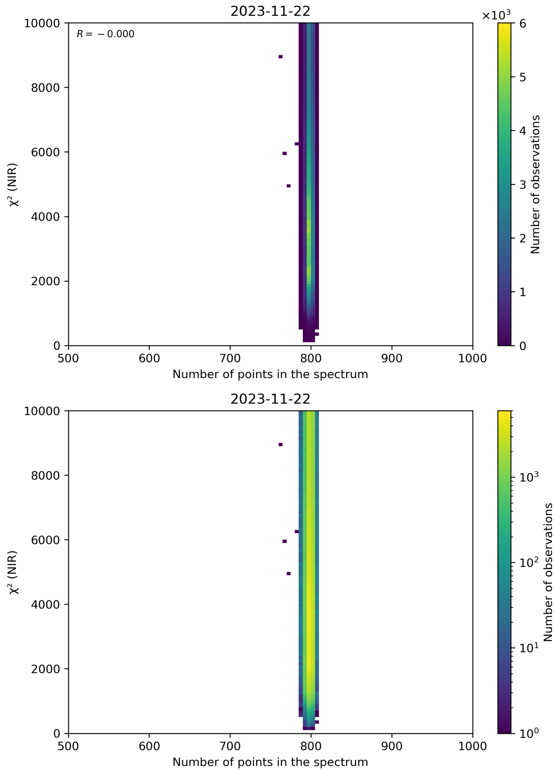
Figure 88: Scatter density plot of “Number of points in the spectrum” against “ \chi^2 (NIR)” for 2023-11-21 to 2023-11-23.
