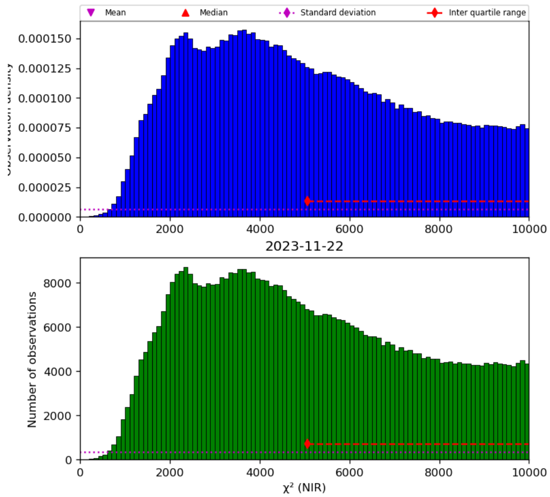
Figure 29: Histogram of “ \chi^2 (NIR)” for 2023-11-21 to 2023-11-23
