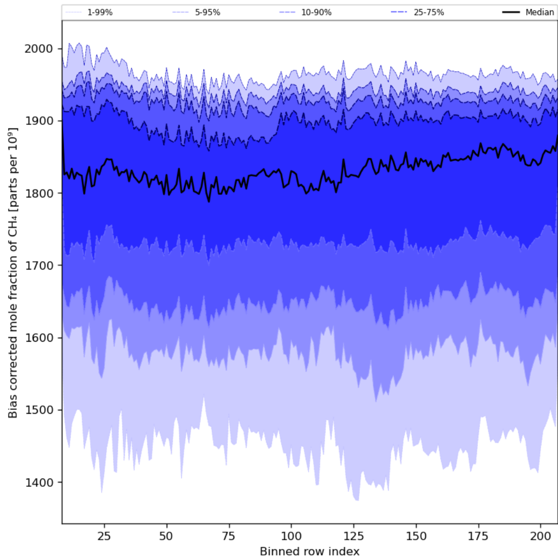
Figure 36: Along track statistics of “Bias corrected mole fraction of CH 4 ” for 2023-11-21 to 2023-11-23
