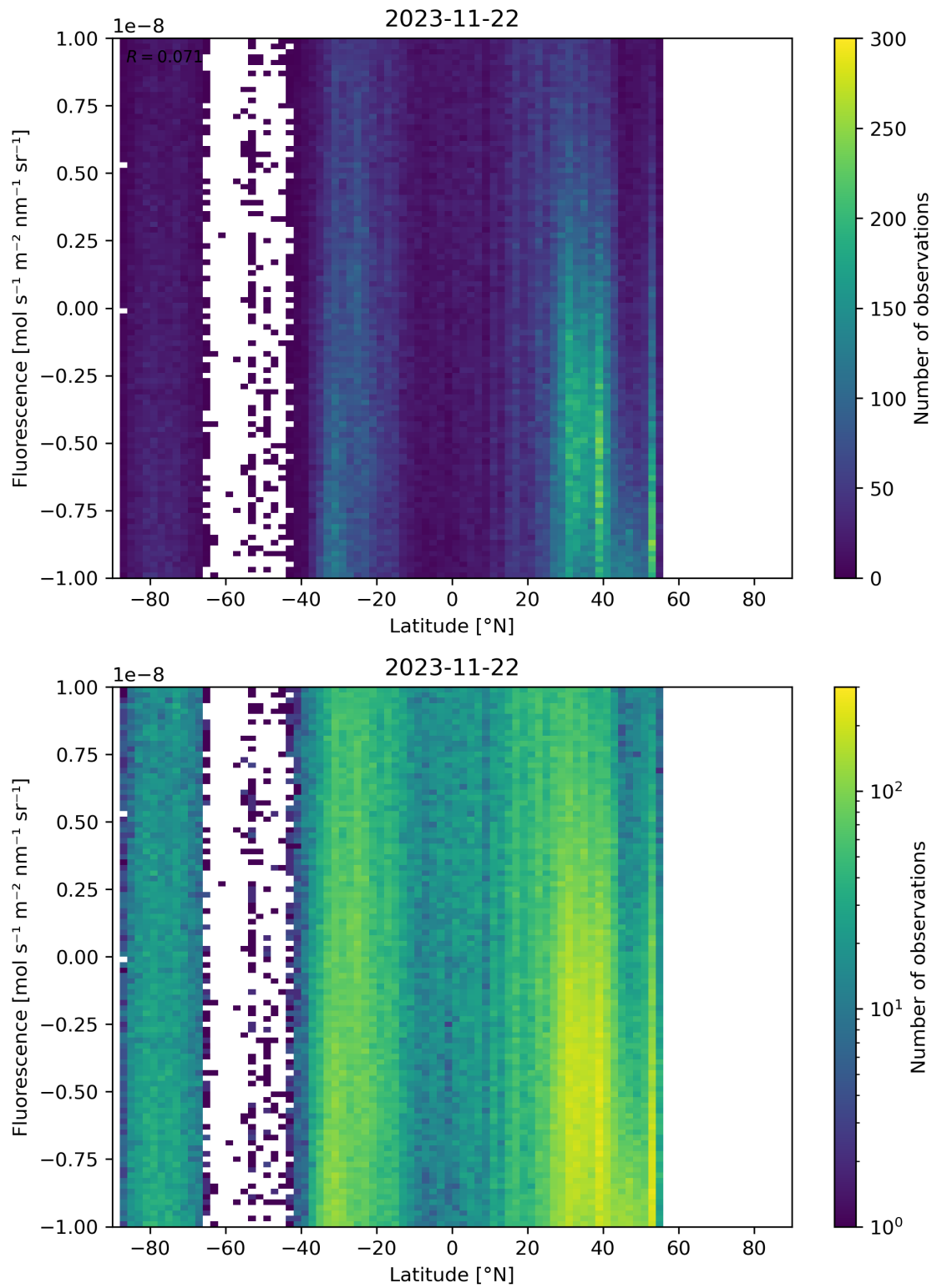
Figure 56: Scatter density plot of “Latitude” against “Fluorescence” for 2023-11-21 to 2023-11-23.
