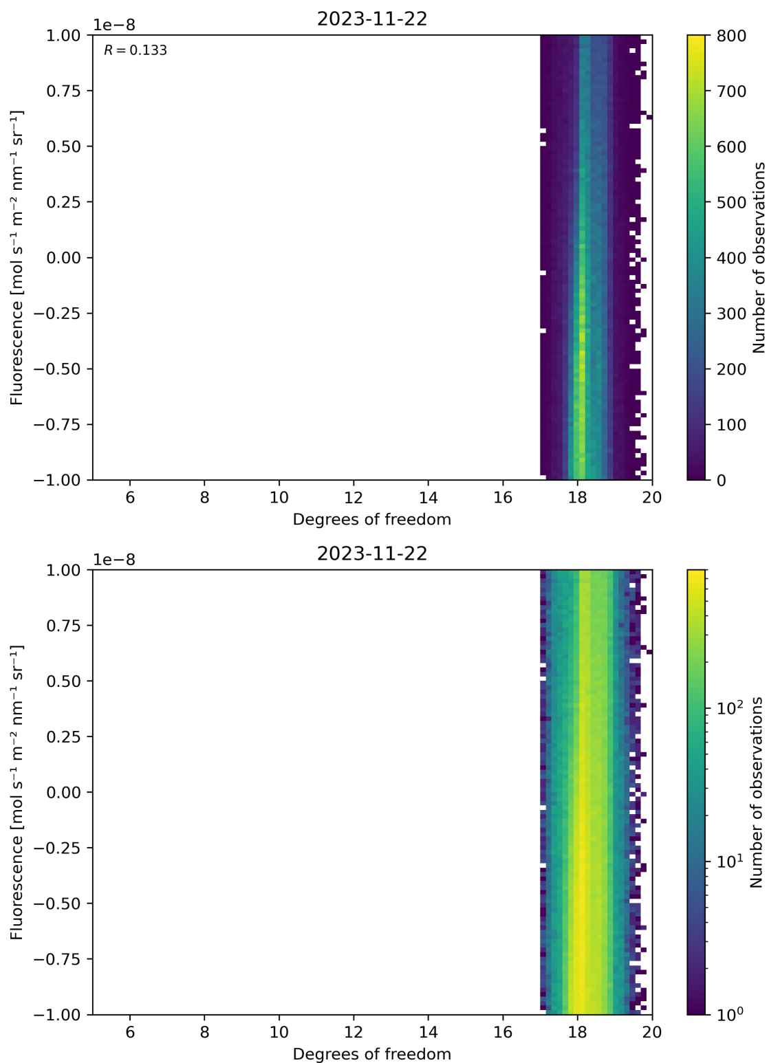
Figure 51: Scatter density plot of “Degrees of freedom” against “Fluorescence” for 2023-11-21 to 2023-11-23.
