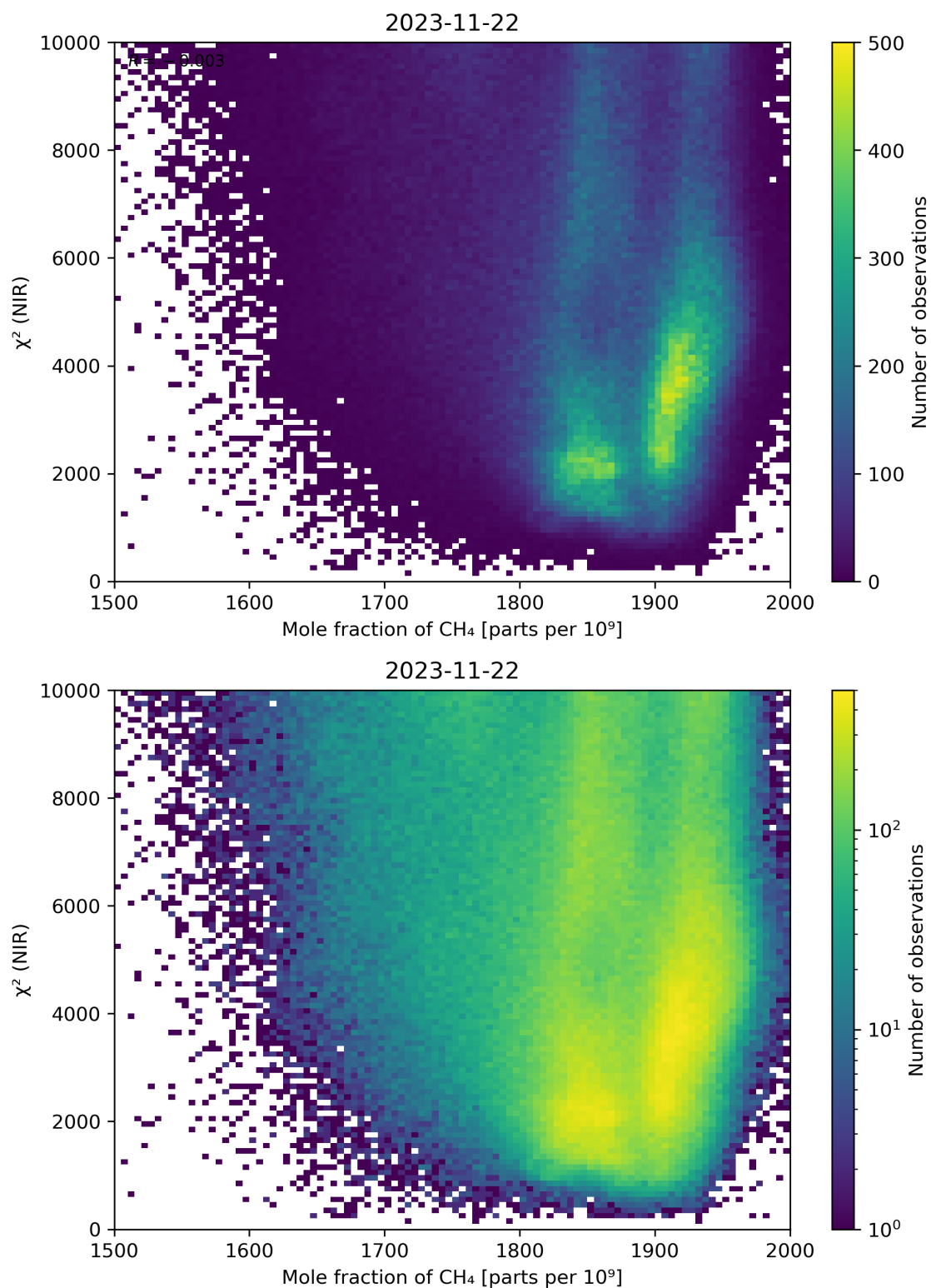
Figure 70: Scatter density plot of “Mole fraction of CH 4 ” against “ \chi^2 (NIR)” for 2023-11-21 to 2023-11-23.
