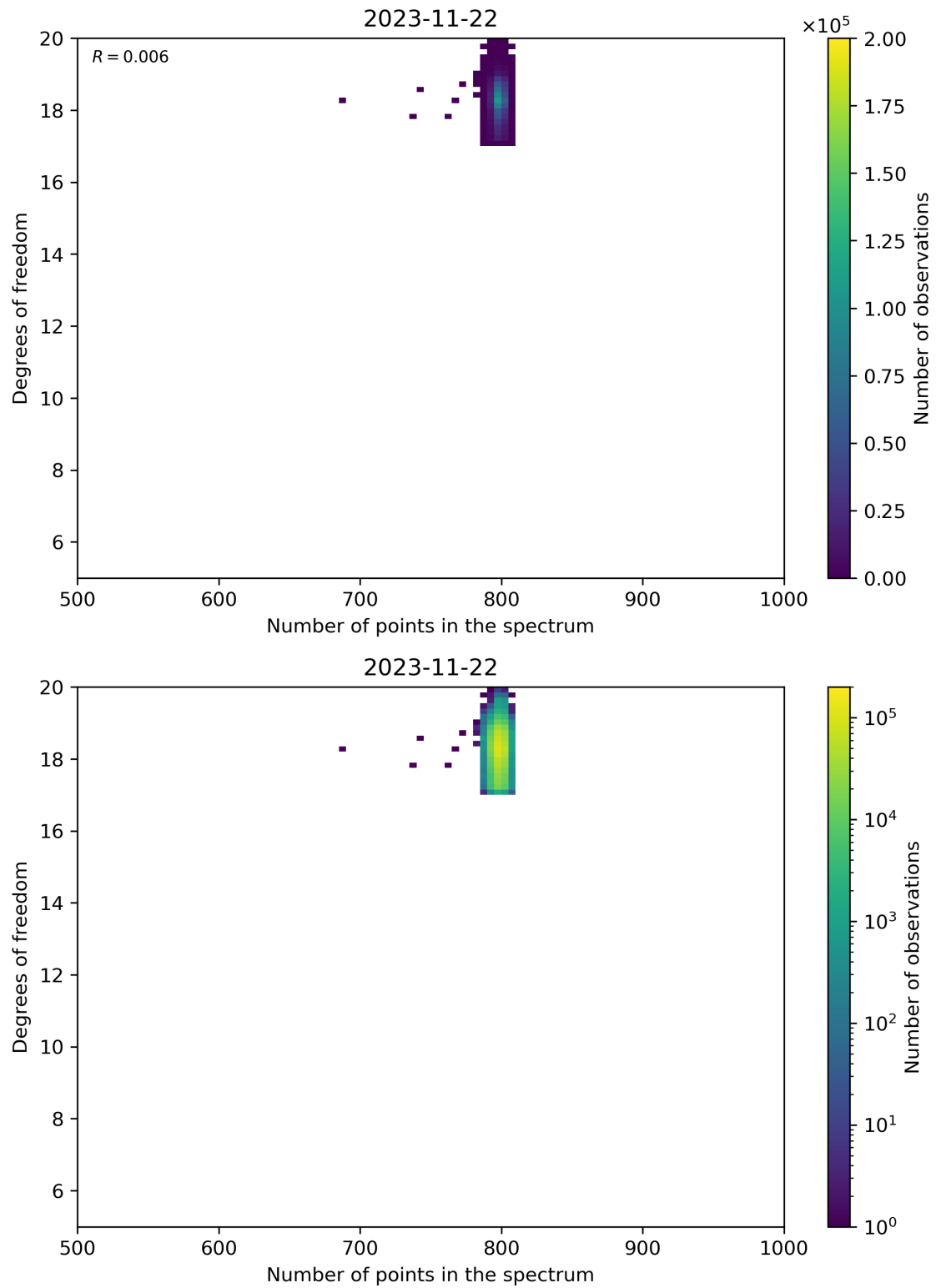
Figure 90: Scatter density plot of “Number of points in the spectrum” against “Degrees of freedom” for 2023-11-21 to 2023-11-23.
