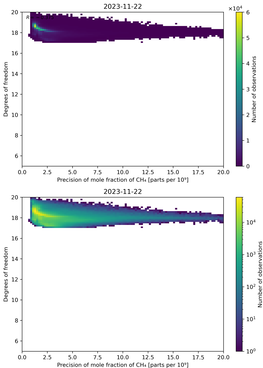
Figure 80: Scatter density plot of “Precision of mole fraction of CH 4 ” against “Degrees of freedom” for 2023-11-21 to 2023-11-23.
