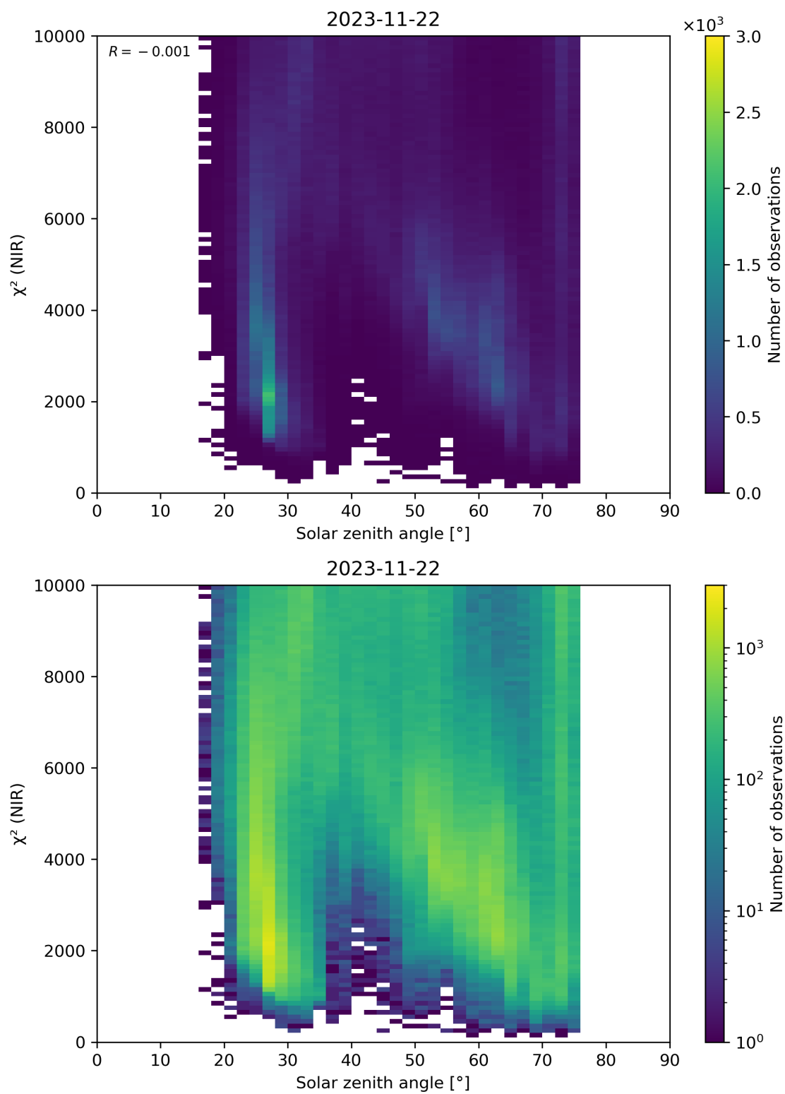
Figure 94: Scatter density plot of “Solar zenith angle” against “ \chi^2 (NIR)” for 2023-11-21 to 2023-11-23.
