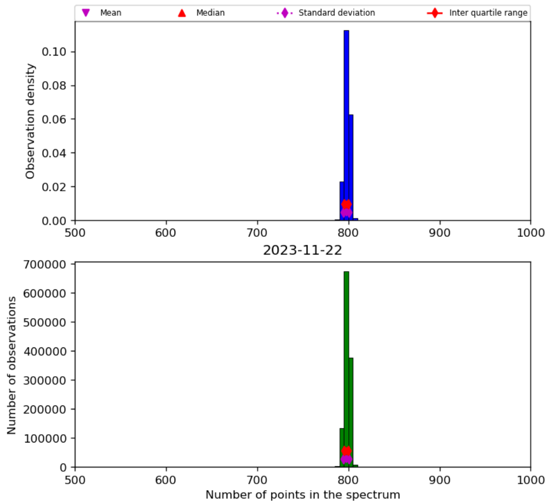
Figure 26: Histogram of “Number of points in the spectrum” for 2023-11-21 to 2023-11-23
