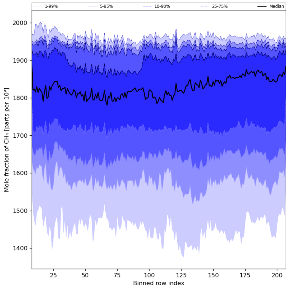
Figure 34: Along track statistics of “Mole fraction of CH 4 ” for 2023-11-21 to 2023-11-23
