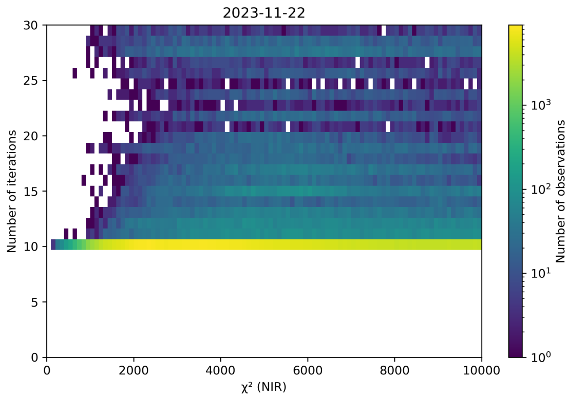
Figure 46: Scatter density plot of “ \chi^2 (NIR)” against “Number of iterations” for 2023-11-21 to 2023-11-23.
