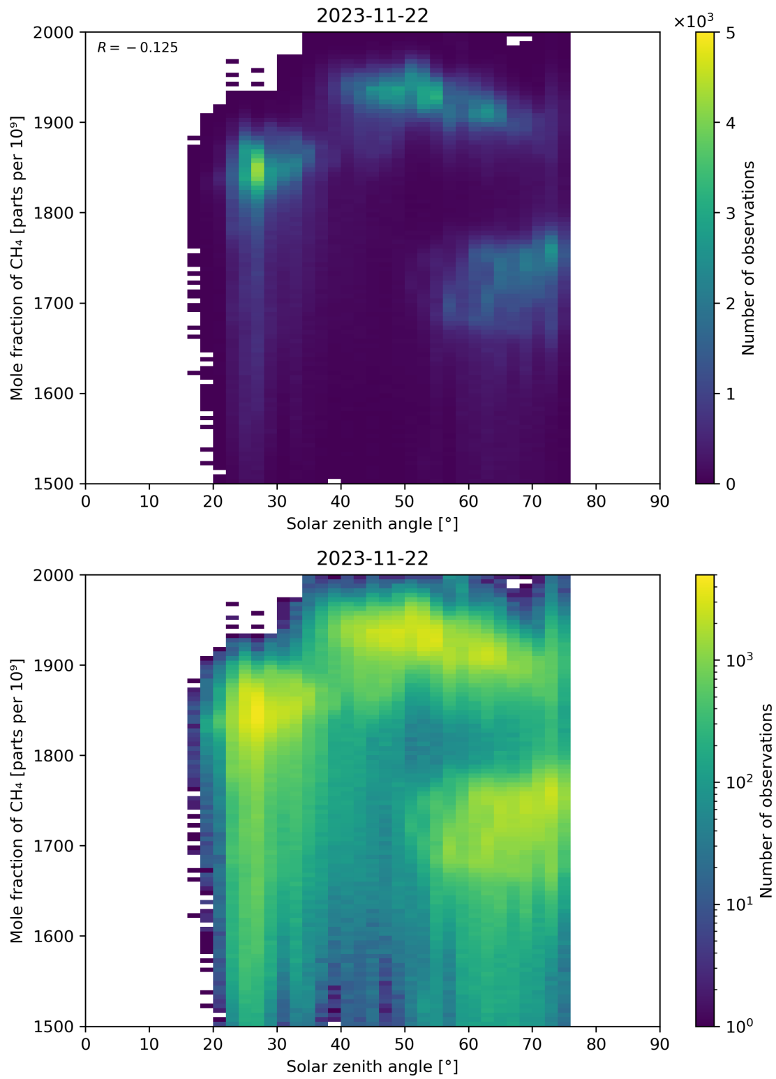
Figure 99: Scatter density plot of “Solar zenith angle” against “Mole fraction of \text{CH}_4 ” for 2023-11-21 to 2023-11-23.
