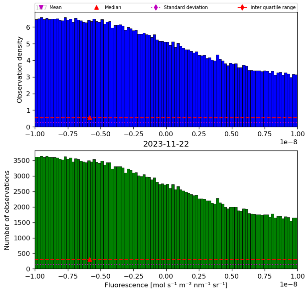
Figure 32: Histogram of “Fluorescence” for 2023-11-21 to 2023-11-23
