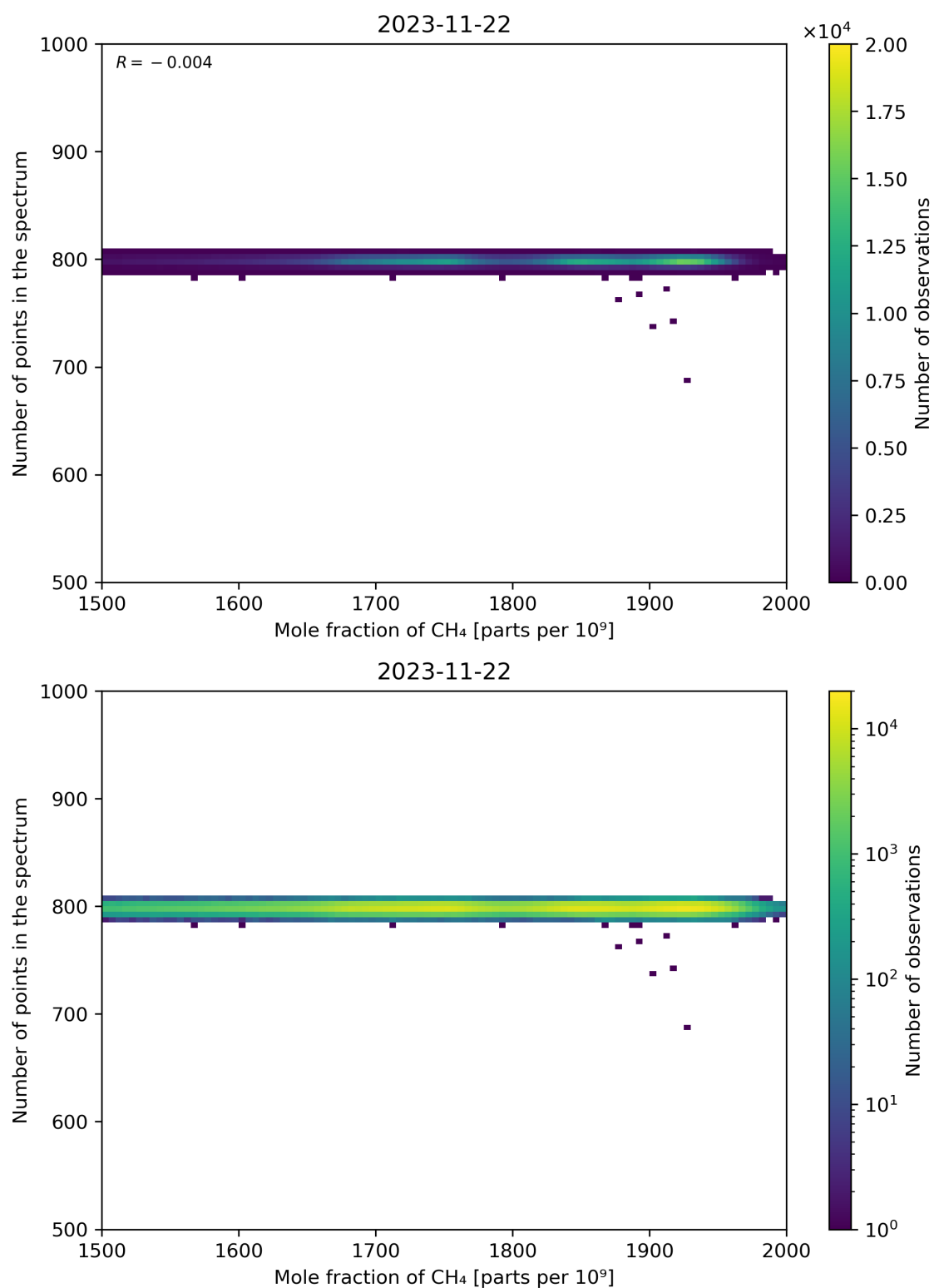
Figure 77: Scatter density plot of “Mole fraction of CH 4 ” against “Number of points in the spectrum” for 2023-11-21 to 2023-11-23.
