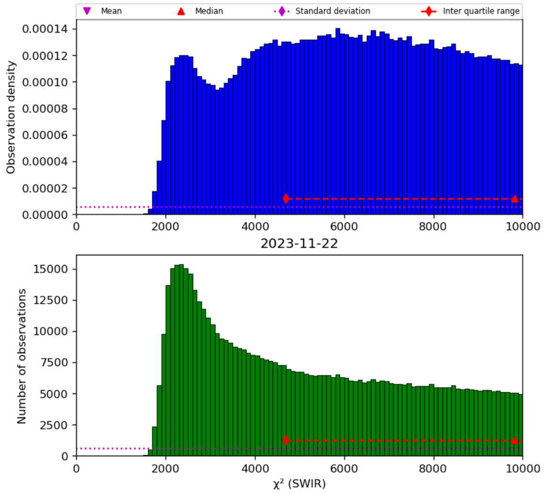
Figure 28: Histogram of “ \chi^2 (SWIR)” for 2023-11-21 to 2023-11-23
