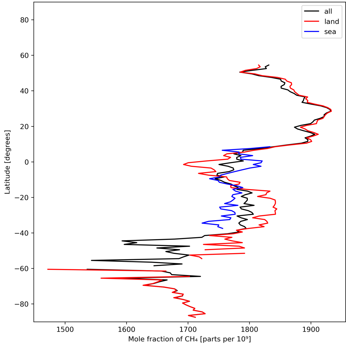
Figure 12: Zonal average of “Mole fraction of \text{CH}_4 ” for 2023-11-21 to 2023-11-23.
