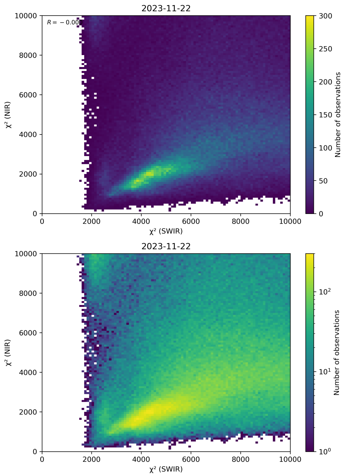
Figure 47: Scatter density plot of “ \chi^2 (SWIR)” against “ \chi^2 (NIR)” for 2023-11-21 to 2023-11-23.
