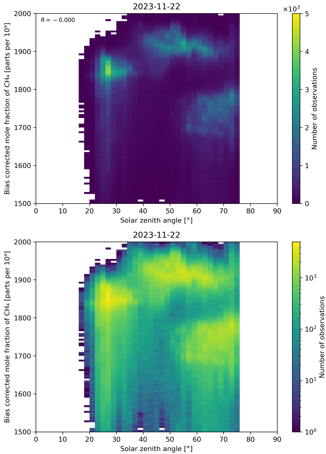
Figure 100: Scatter density plot of “Solar zenith angle” against “Bias corrected mole fraction of CH 4 ” for 2023-11-21 to 2023-11-23.
