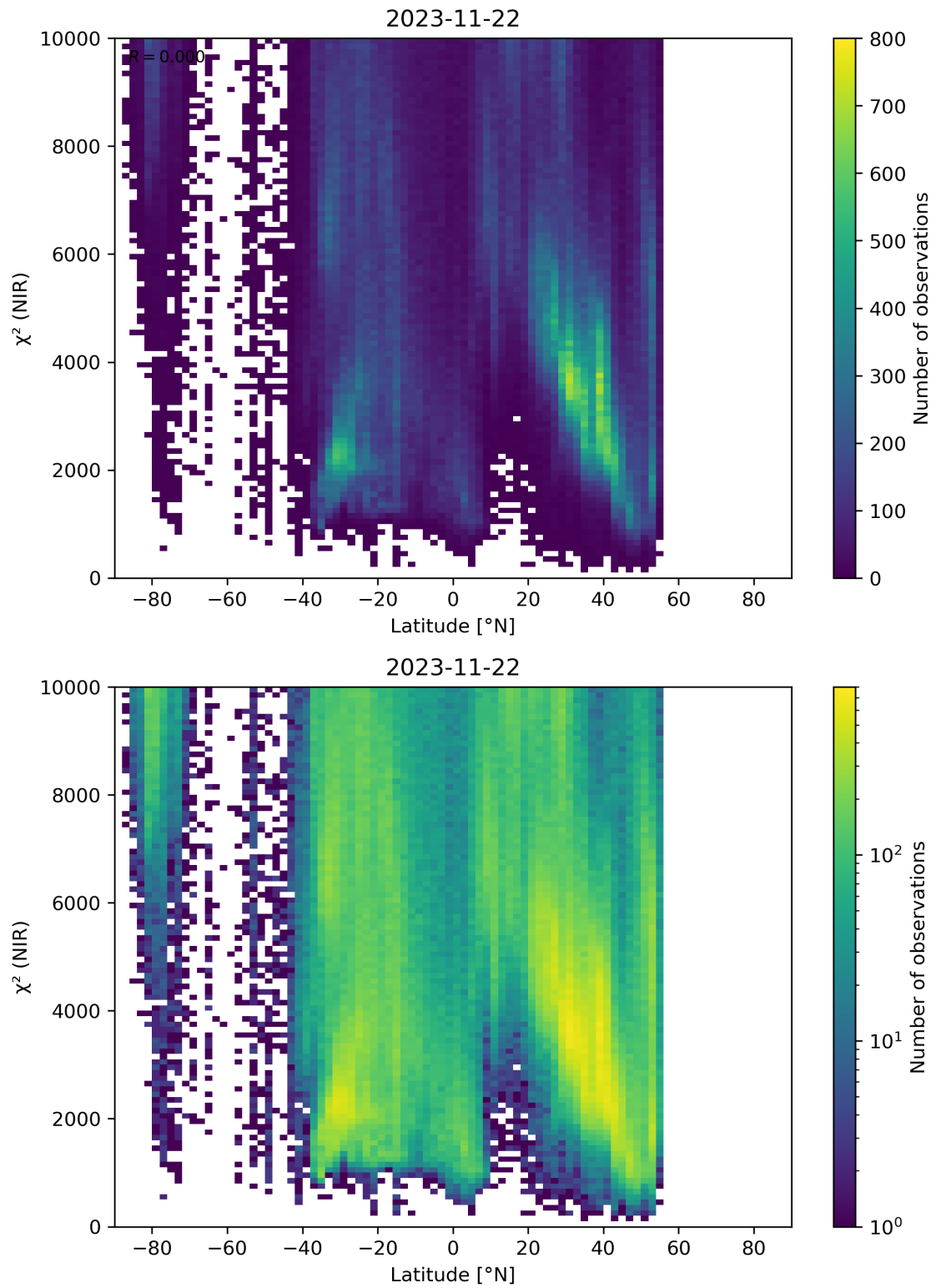
Figure 53: Scatter density plot of “Latitude” against “ \chi^2 (NIR)” for 2023-11-21 to 2023-11-23.
