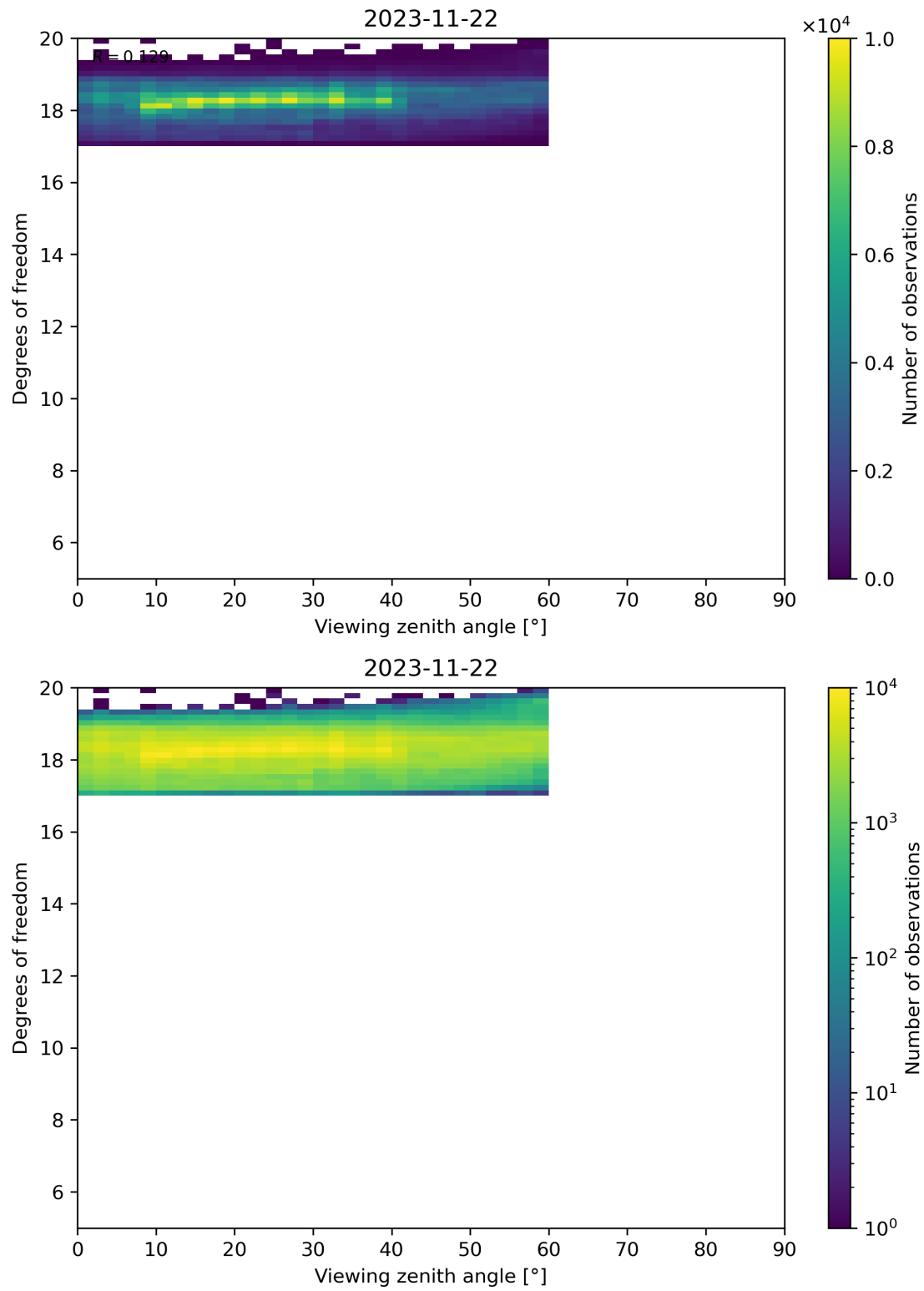
Figure 107: Scatter density plot of “Viewing zenith angle” against “Degrees of freedom” for 2023-11-21 to 2023-11-23.
