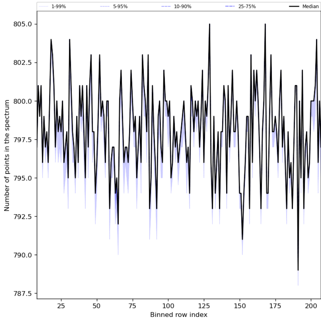
Figure 37: Along track statistics of “Number of points in the spectrum” for 2023-11-21 to 2023-11-23
