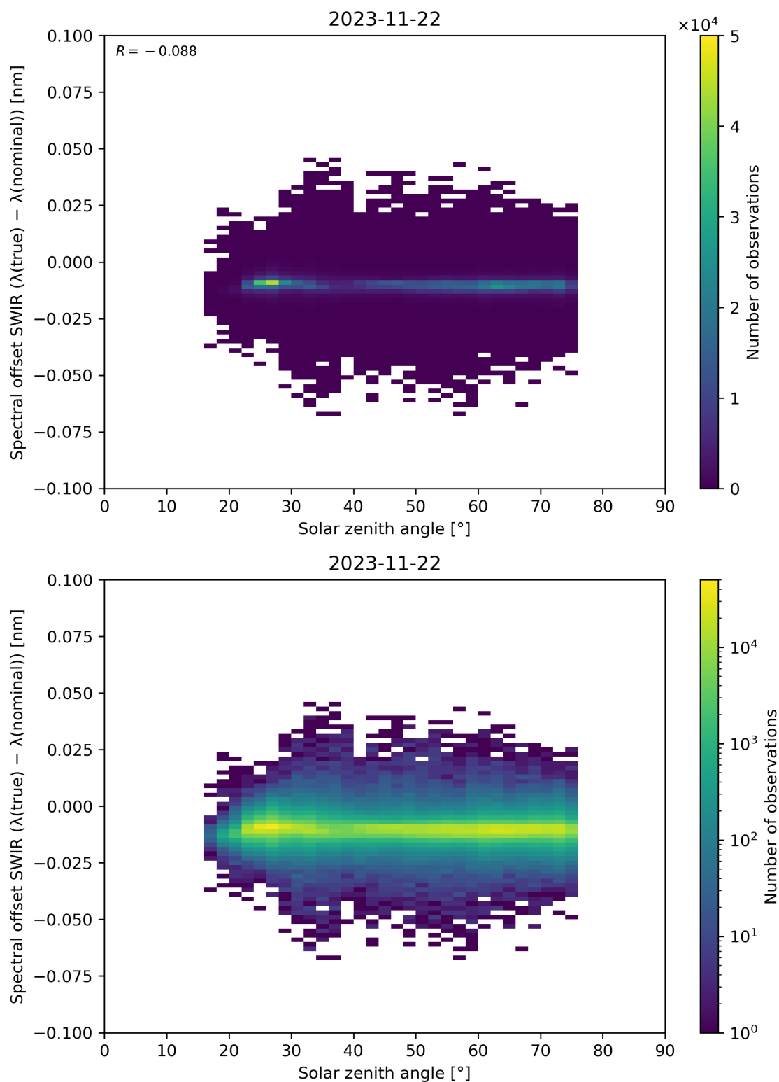
Figure 104: Scatter density plot of “Solar zenith angle” against “Spectral offset SWIR ( \lambda(\text{true}) - \lambda(\text{nominal}) )” for 2023-11-21 to 2023-11-23.
