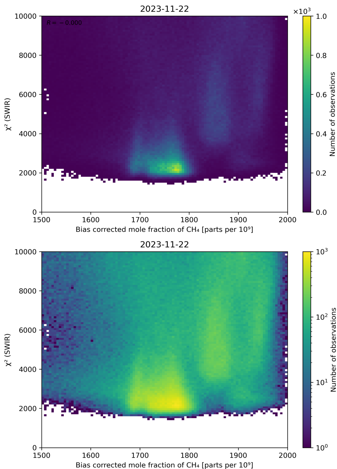
Figure 64: Scatter density plot of “Bias corrected mole fraction of CH 4 ” against “ \chi^2 (SWIR)” for 2023-11-21 to 2023-11-23.
