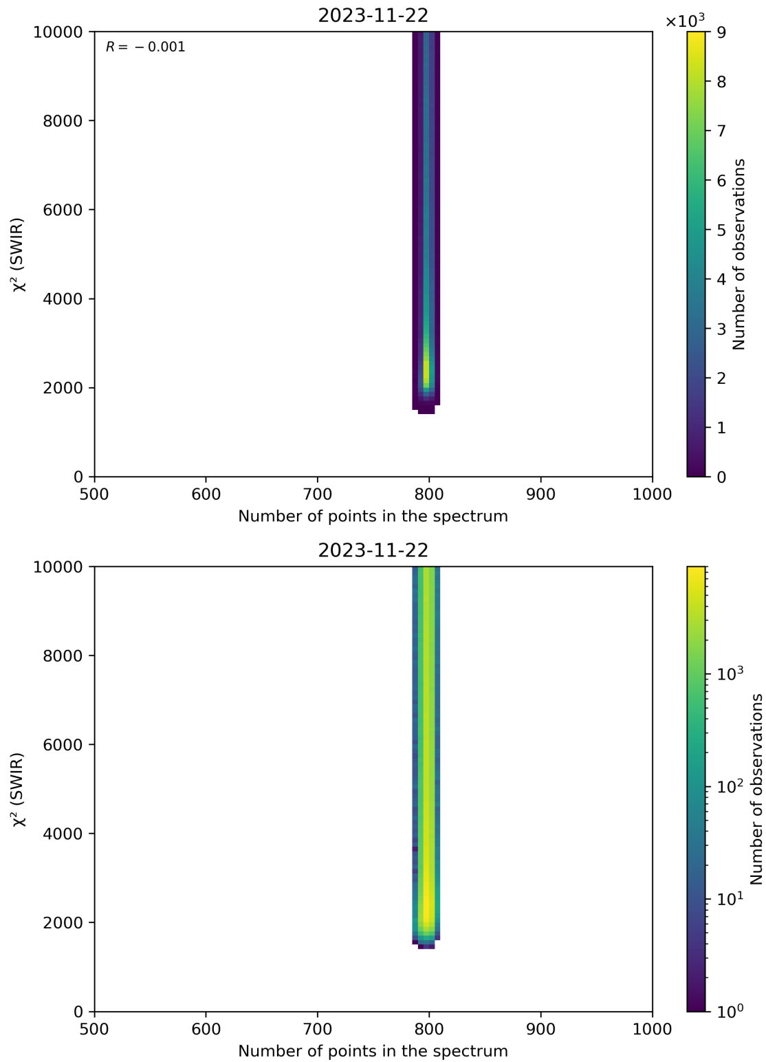
Figure 89: Scatter density plot of “Number of points in the spectrum” against “ \chi^2 (SWIR)” for 2023-11-21 to 2023-11-23.
