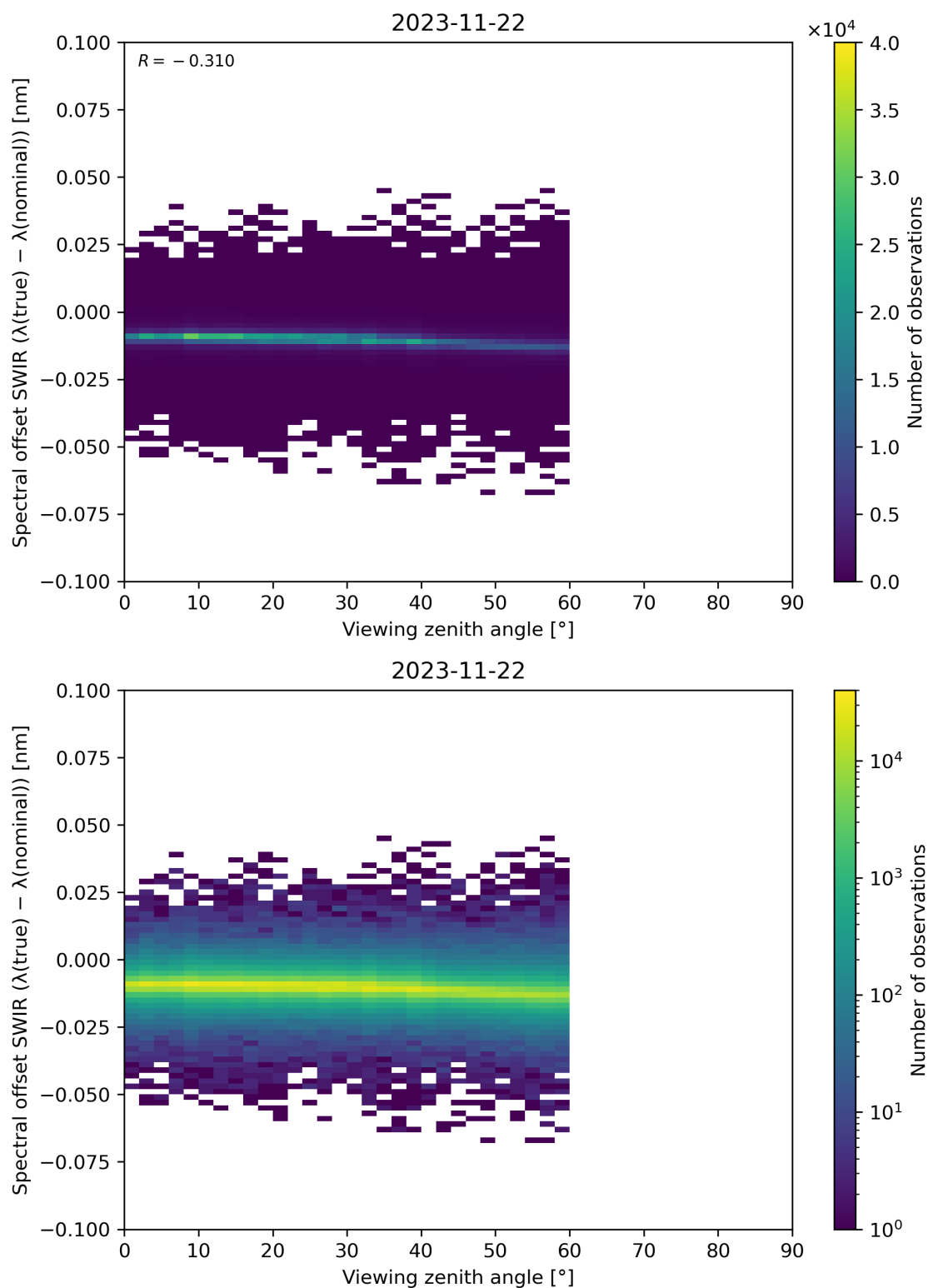
Figure 116: Scatter density plot of “Viewing zenith angle” against “Spectral offset SWIR ( \lambda(\text{true}) - \lambda(\text{nominal}) )” for 2023-11-21 to 2023-11-23.
