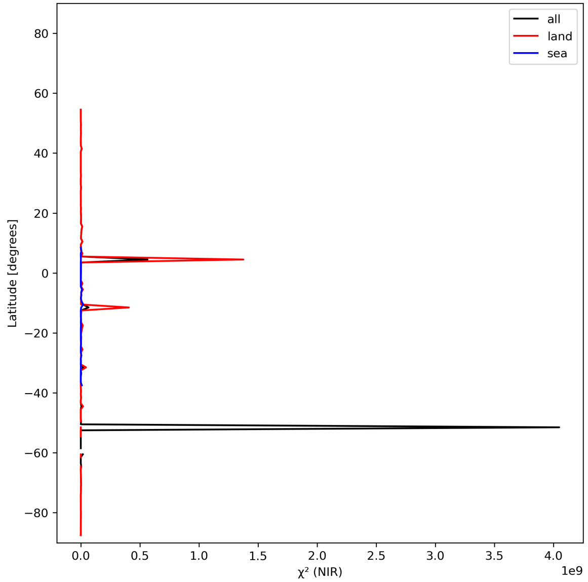
Figure 18: Zonal average of “ \chi^2 (NIR)” for 2023-11-21 to 2023-11-23.
