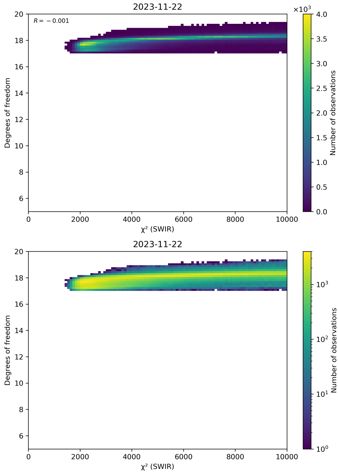
Figure 48: Scatter density plot of “ \chi^2 (SWIR)” against “Degrees of freedom” for 2023-11-21 to 2023-11-23.
