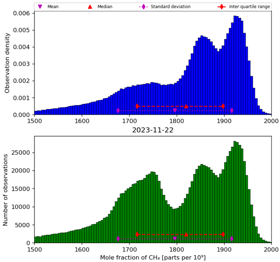
Figure 23: Histogram of “Mole fraction of CH 4 ” for 2023-11-21 to 2023-11-23
