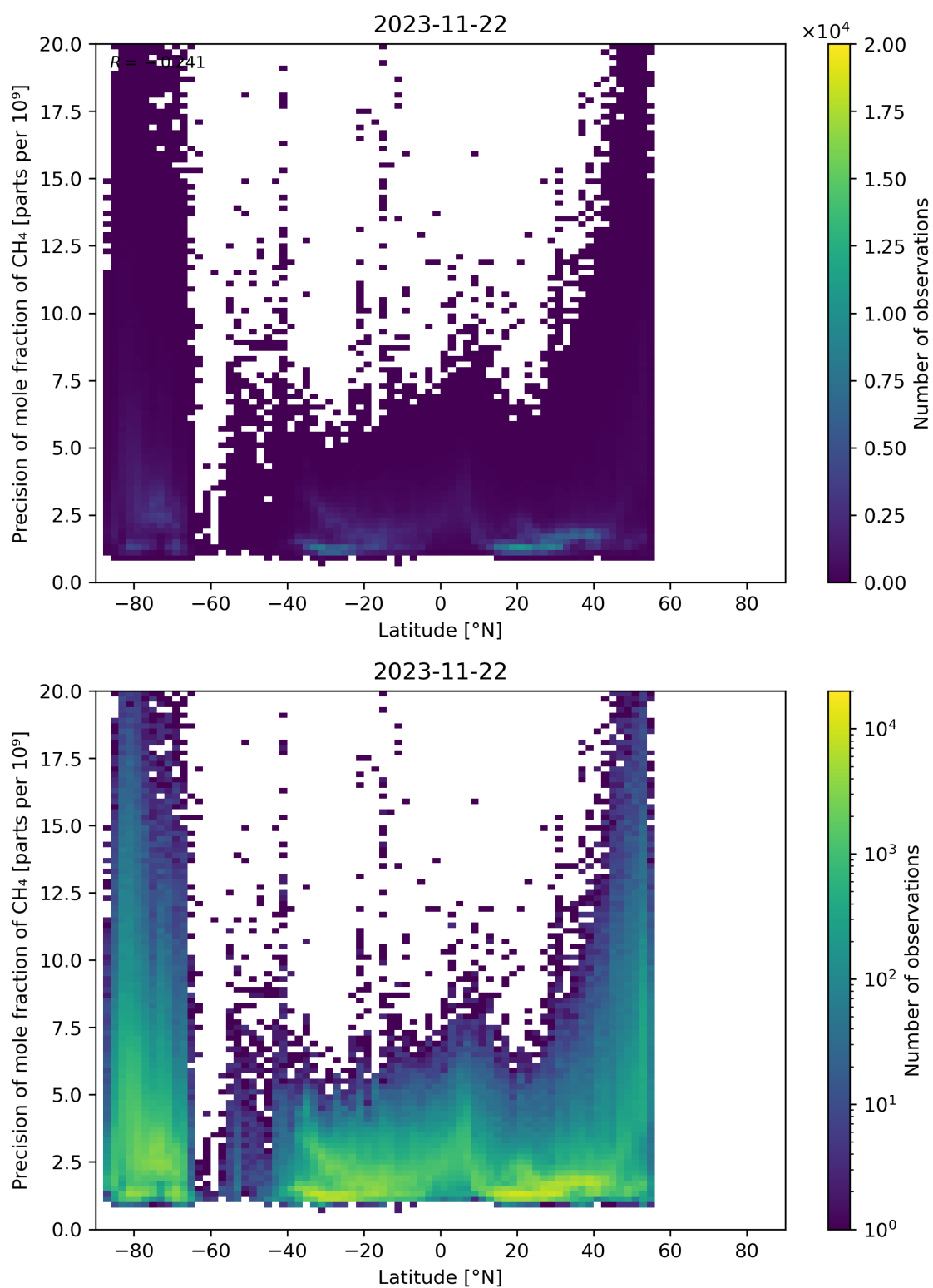
Figure 59: Scatter density plot of “Latitude” against “Precision of mole fraction of CH 4 ” for 2023-11-21 to 2023-11-23.
