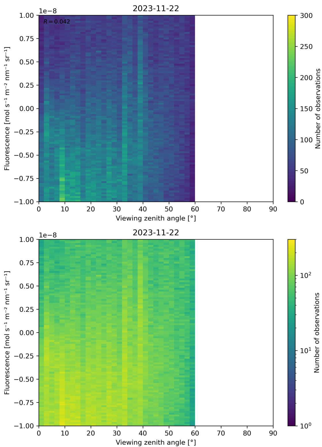
Figure 108: Scatter density plot of “Viewing zenith angle” against “Fluorescence” for 2023-11-21 to 2023-11-23.
