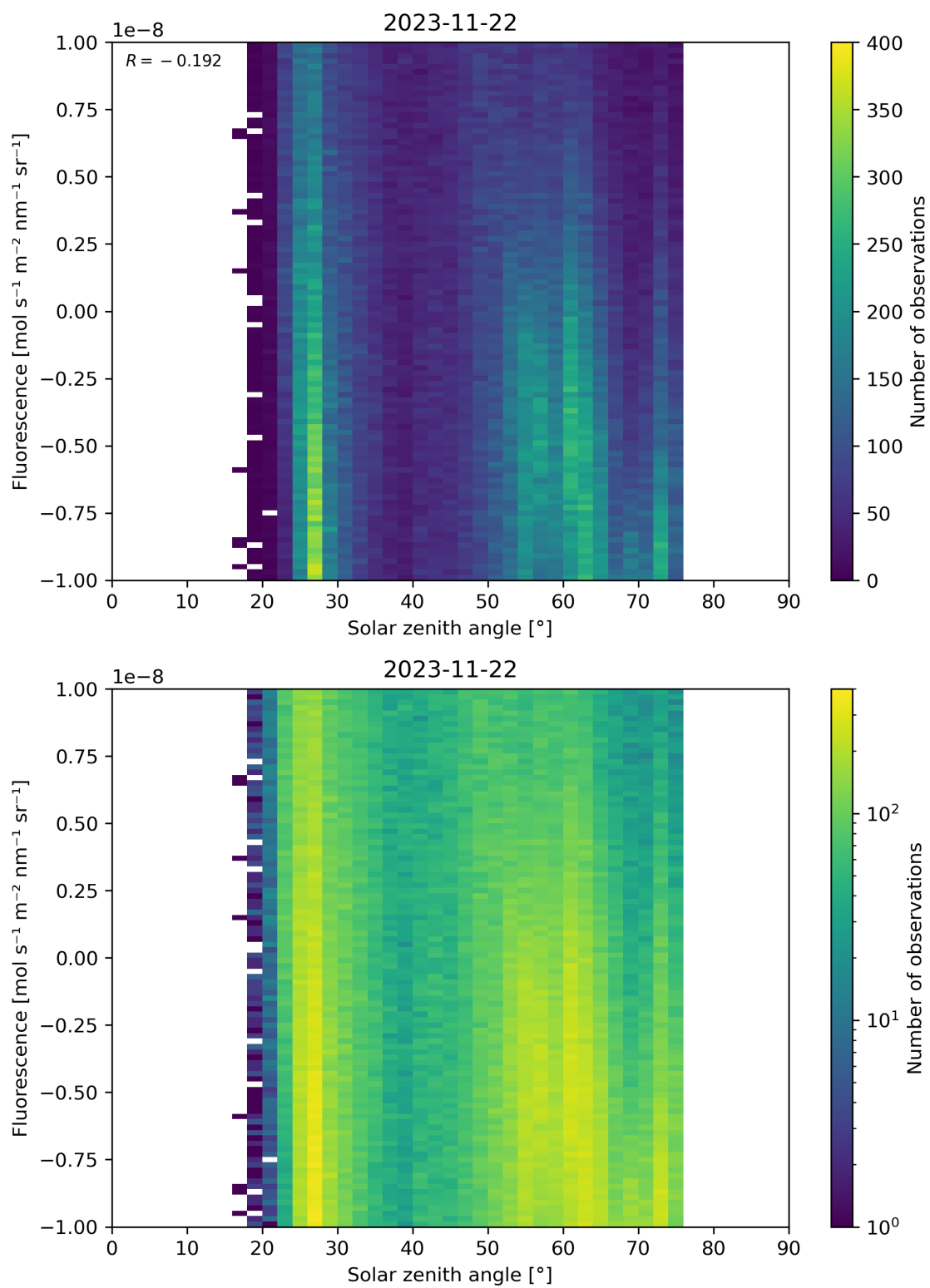
Figure 97: Scatter density plot of “Solar zenith angle” against “Fluorescence” for 2023-11-21 to 2023-11-23.
