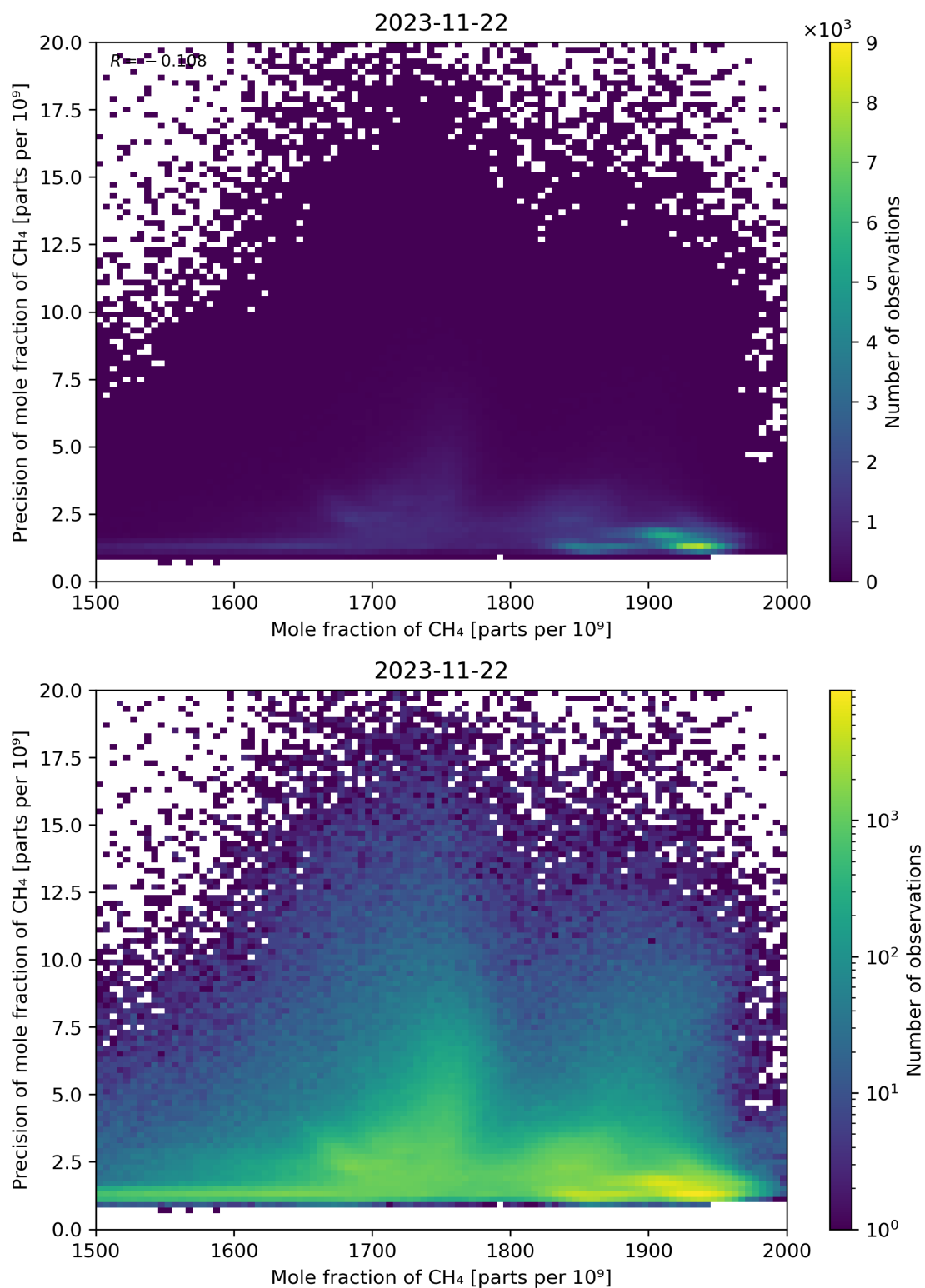
Figure 75: Scatter density plot of “Mole fraction of CH 4 ” against “Precision of mole fraction of CH 4 ” for 2023-11-21 to 2023-11-23.
