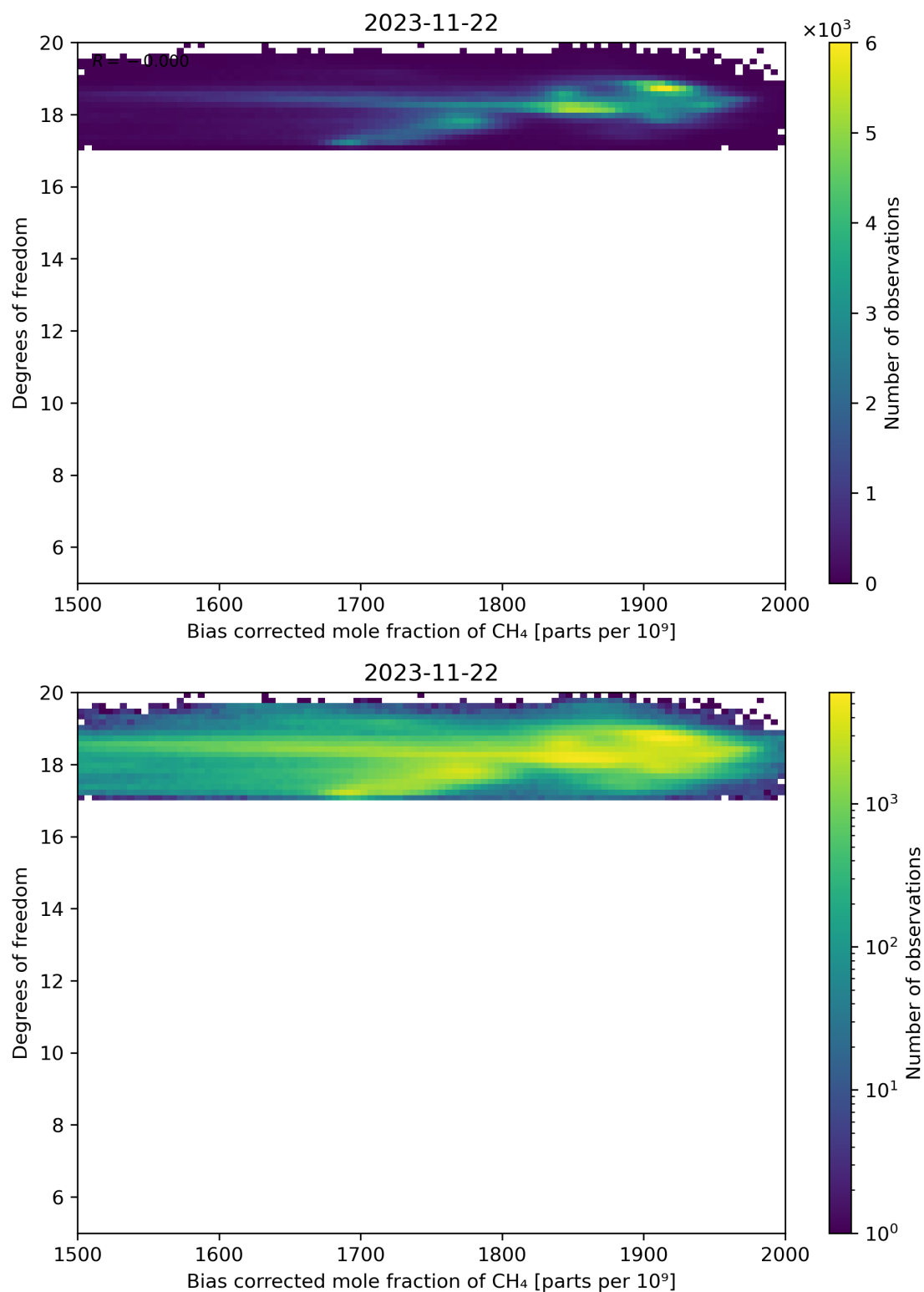
Figure 65: Scatter density plot of “Bias corrected mole fraction of CH 4 ” against “Degrees of freedom” for 2023-11-21 to 2023-11-23.
