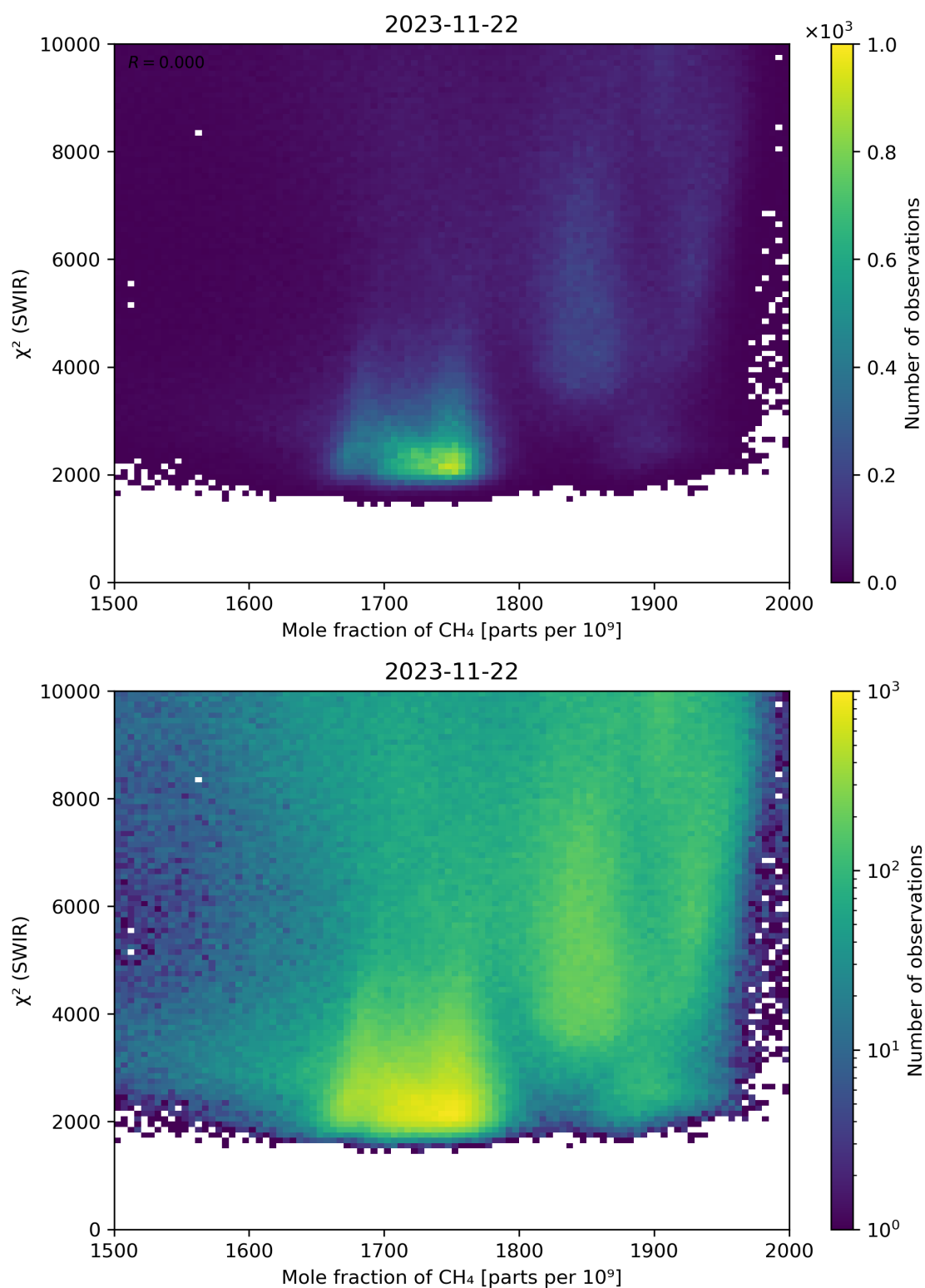
Figure 71: Scatter density plot of “Mole fraction of \text{CH}_4 ” against “ \chi^2 (SWIR)” for 2023-11-21 to 2023-11-23.
