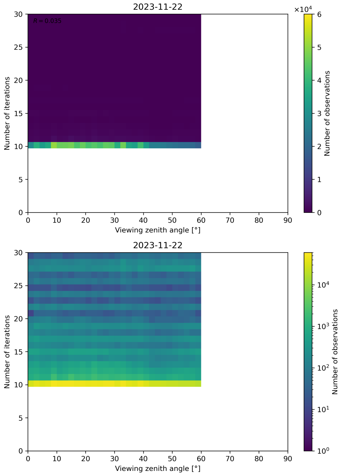
Figure 113: Scatter density plot of “Viewing zenith angle” against “Number of iterations” for 2023-11-21 to 2023-11-23.
