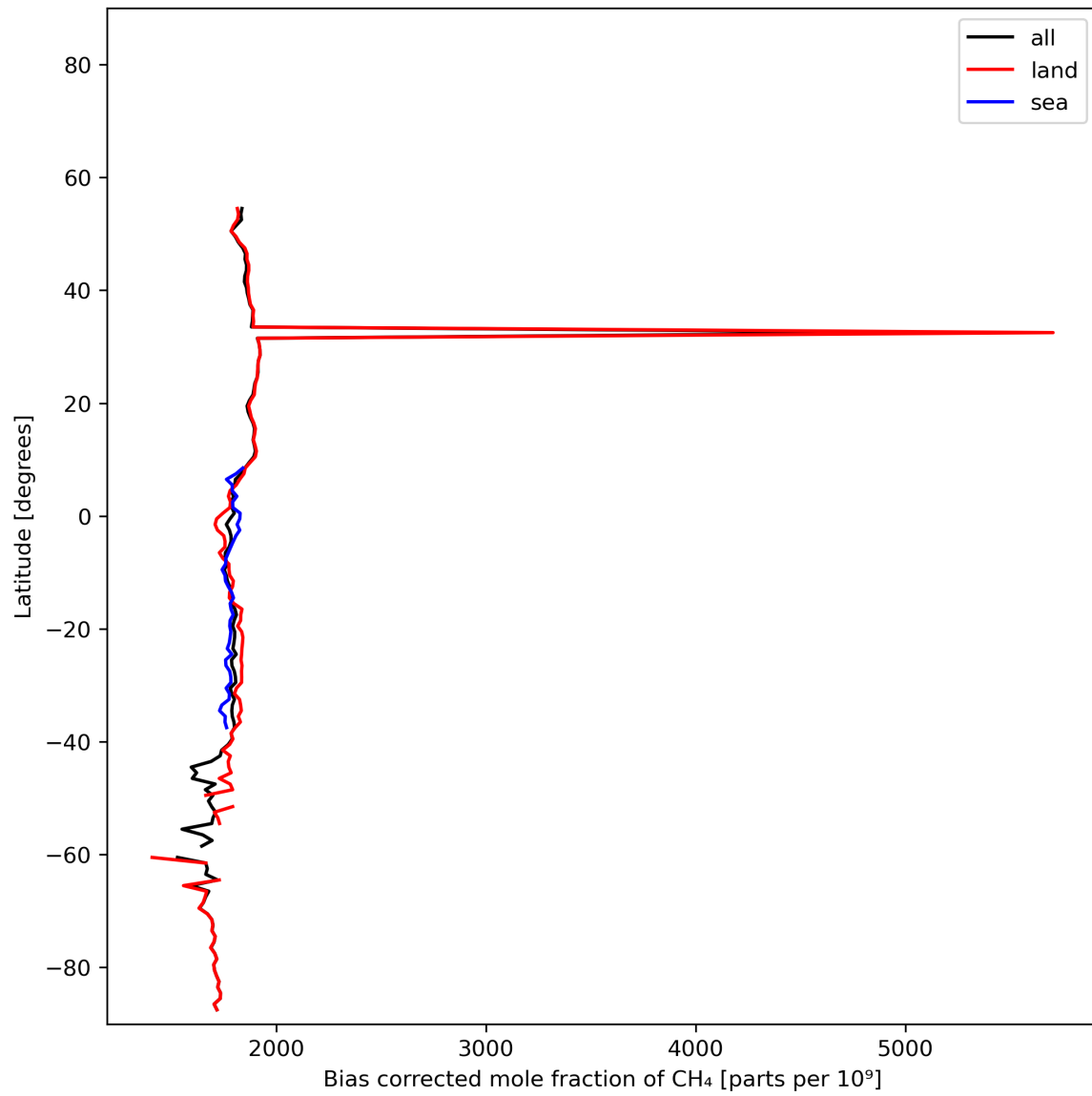
Figure 14: Zonal average of “Bias corrected mole fraction of CH 4 ” for 2023-11-21 to 2023-11-23.
