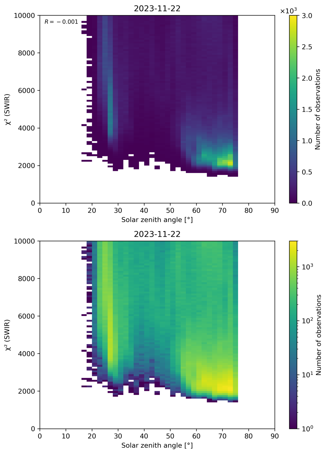
Figure 95: Scatter density plot of “Solar zenith angle” against “ \chi^2 (SWIR)” for 2023-11-21 to 2023-11-23.
