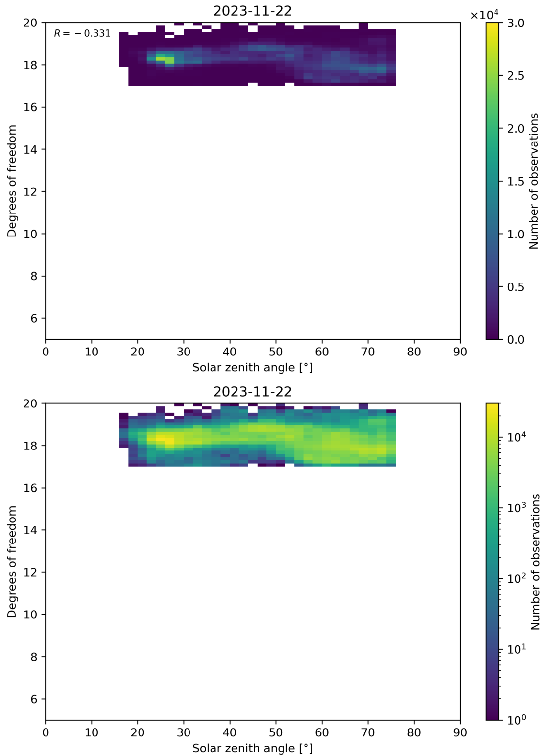
Figure 96: Scatter density plot of “Solar zenith angle” against “Degrees of freedom” for 2023-11-21 to 2023-11-23.
