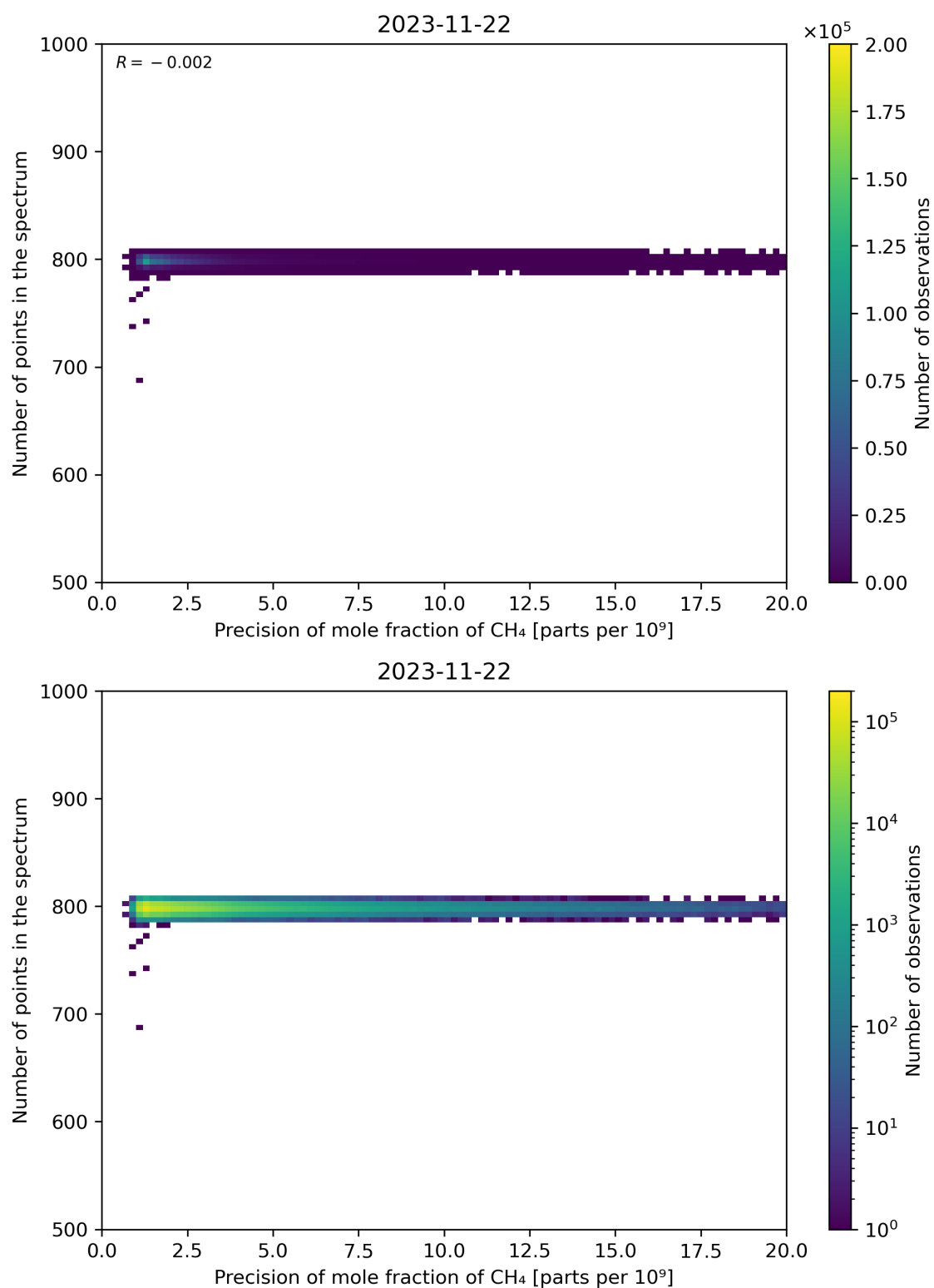
Figure 84: Scatter density plot of “Precision of mole fraction of CH 4 ” against “Number of points in the spectrum” for 2023-11-21 to 2023-11-23.
