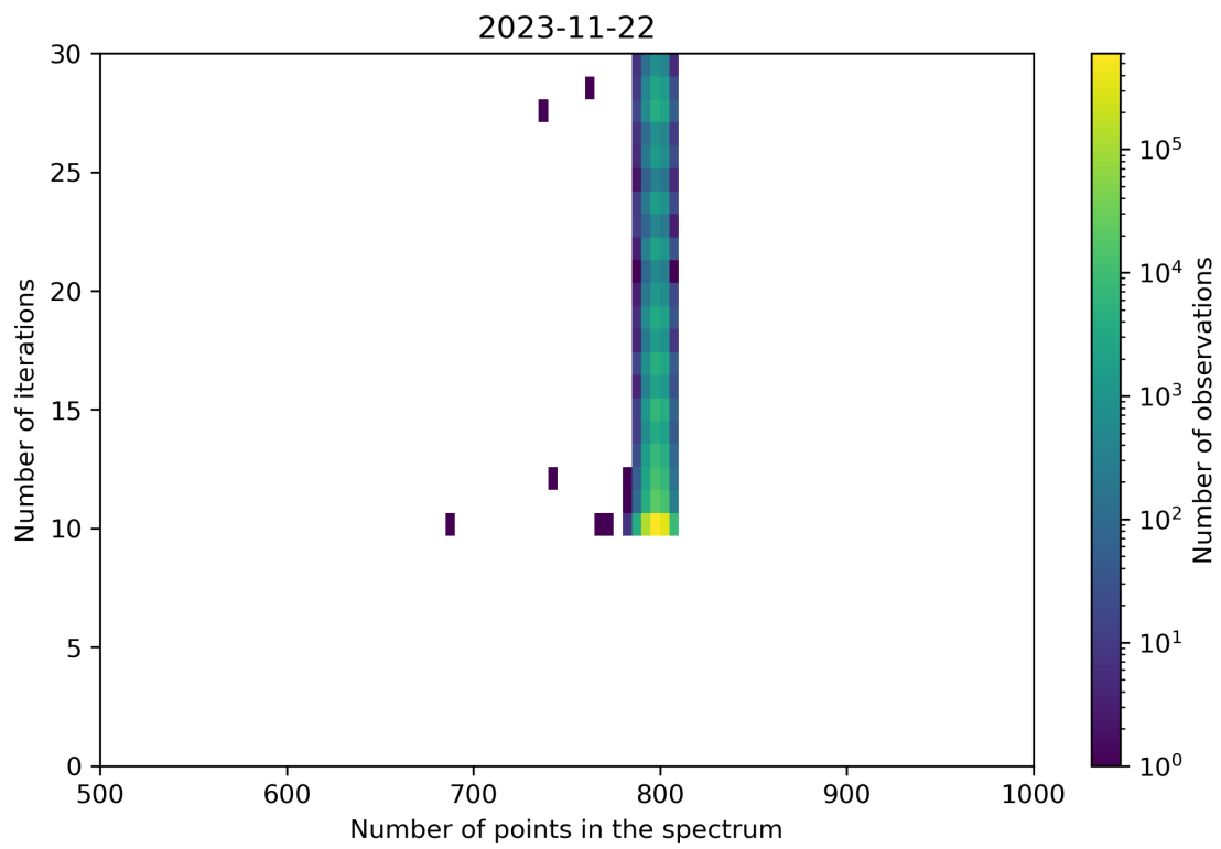
Figure 92: Scatter density plot of “Number of points in the spectrum” against “Number of iterations” for 2023-11-21 to 2023-11-23.
