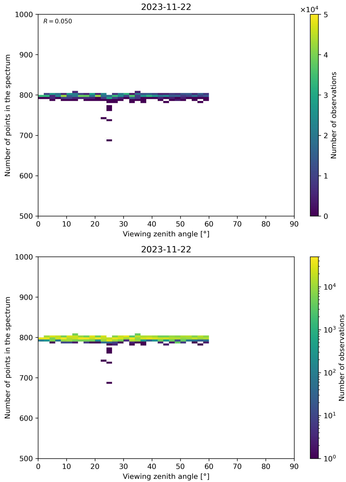
Figure 114: Scatter density plot of “Viewing zenith angle” against “Number of points in the spectrum” for 2023-11-21 to 2023-11-23.
