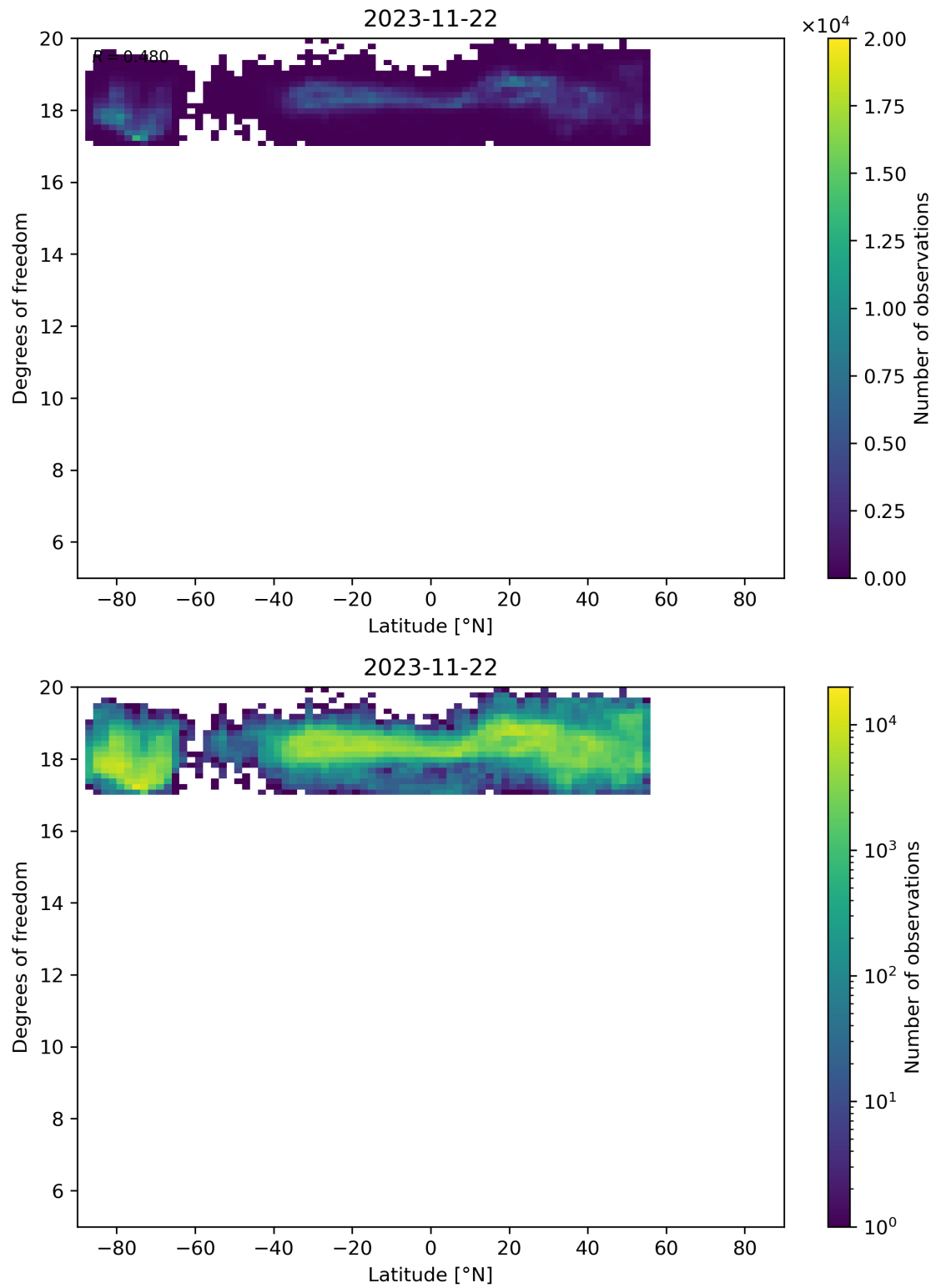
Figure 55: Scatter density plot of “Latitude” against “Degrees of freedom” for 2023-11-21 to 2023-11-23.
