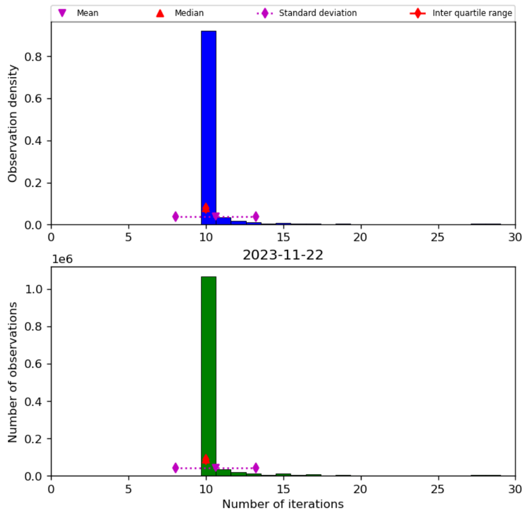
Figure 31: Histogram of “Number of iterations” for 2023-11-21 to 2023-11-23
