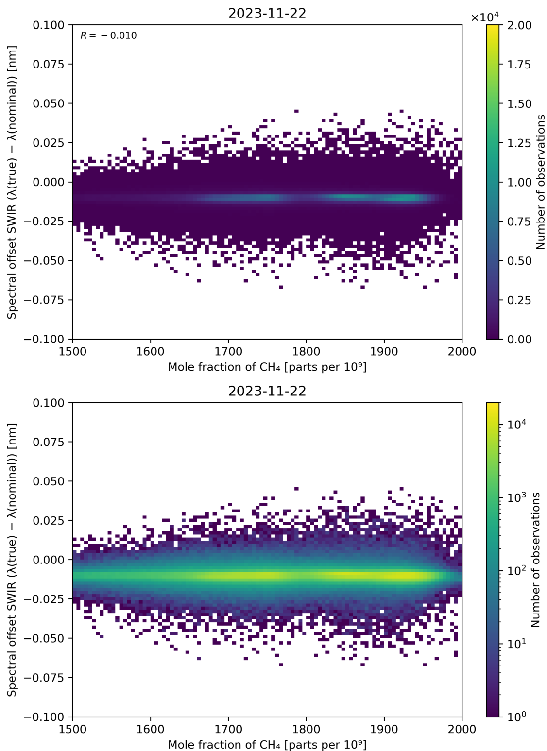
Figure 86: Scatter density plot of “Mole fraction of CH 4 ” against “Spectral offset SWIR ( \lambda(\text{true}) - \lambda(\text{nominal}) )” for 2023-11-21 to 2023-11-23.
