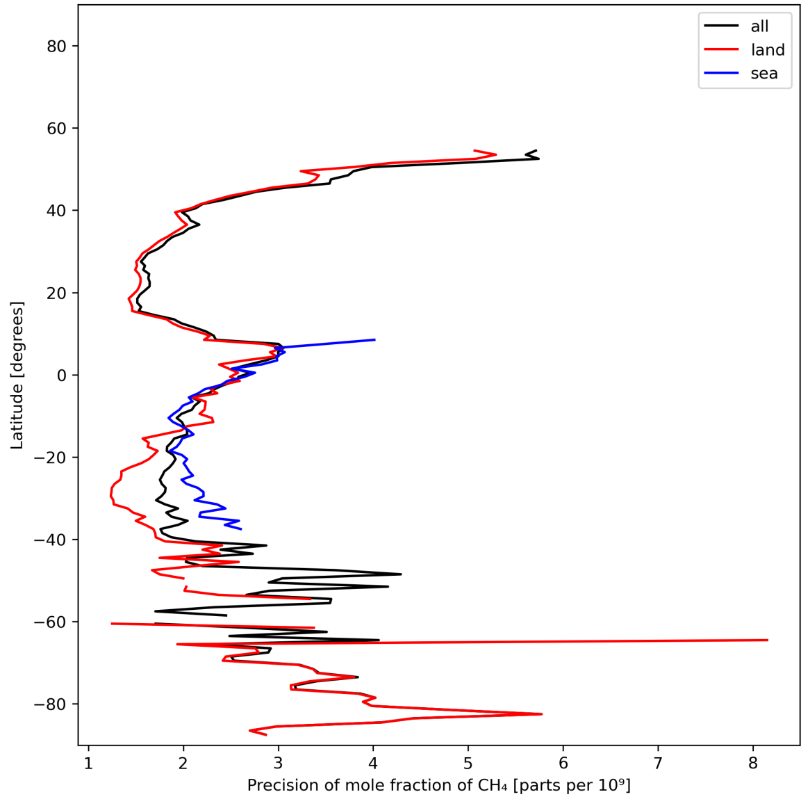
Figure 13: Zonal average of “Precision of mole fraction of CH 4 ” for 2023-11-21 to 2023-11-23.
