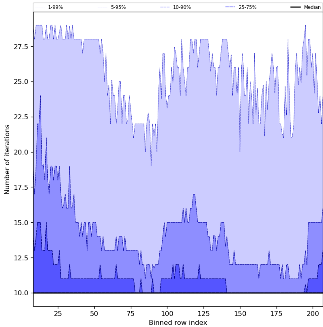
Figure 42: Along track statistics of “Number of iterations” for 2023-11-21 to 2023-11-23
