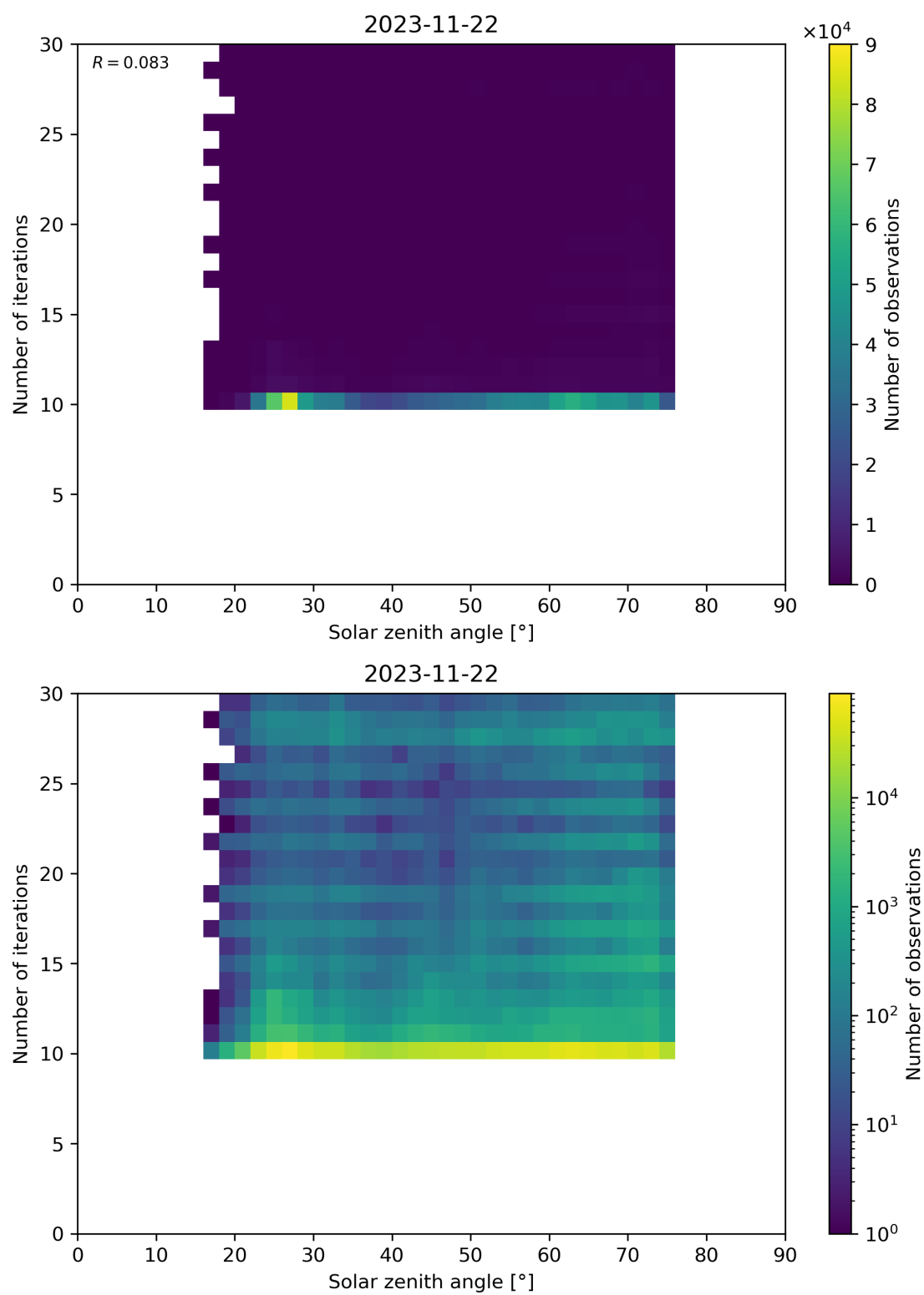
Figure 102: Scatter density plot of “Solar zenith angle” against “Number of iterations” for 2023-11-21 to 2023-11-23.
