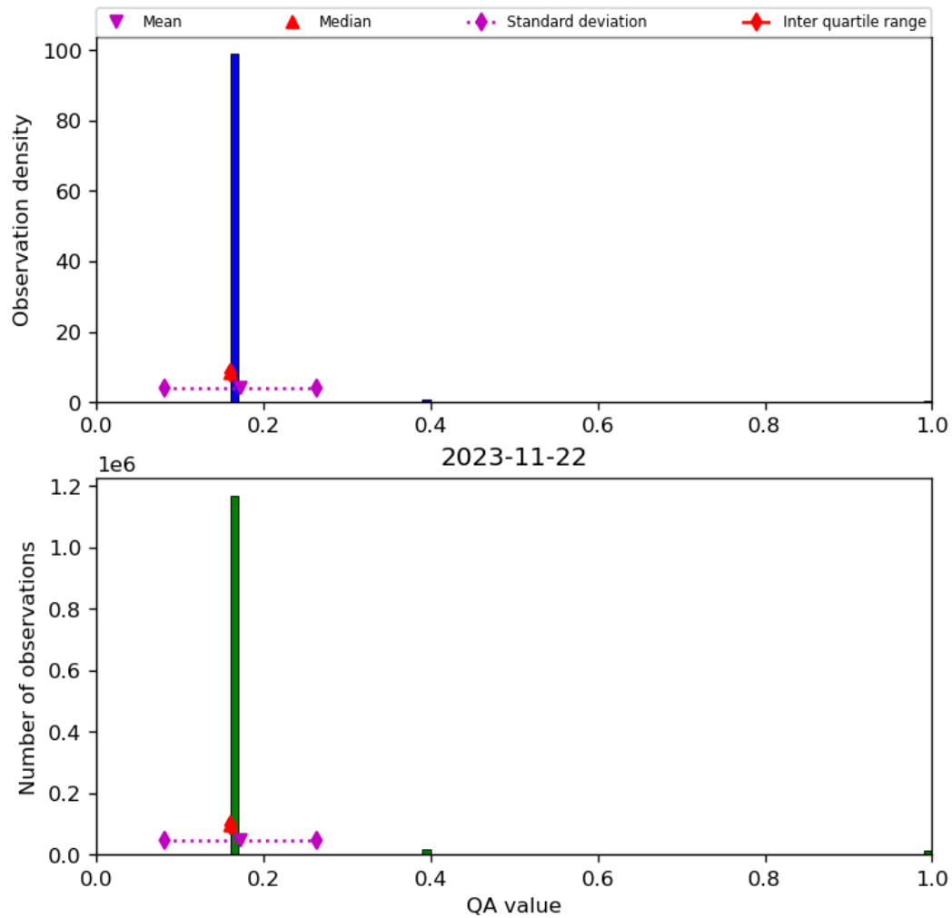
Figure 22: Histogram of “QA value” for 2023-11-21 to 2023-11-23
