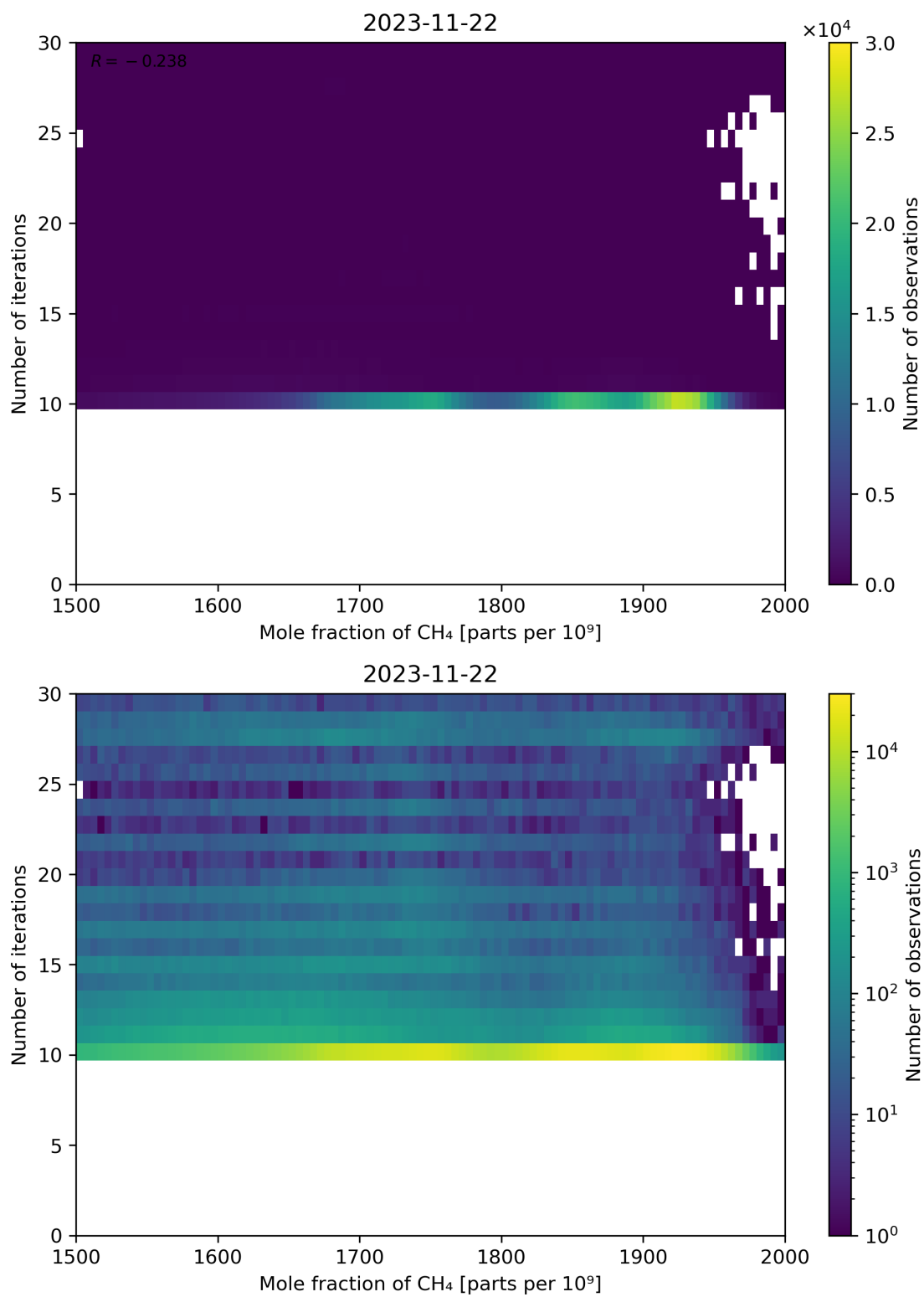
Figure 76: Scatter density plot of “Mole fraction of CH 4 ” against “Number of iterations” for 2023-11-21 to 2023-11-23.
