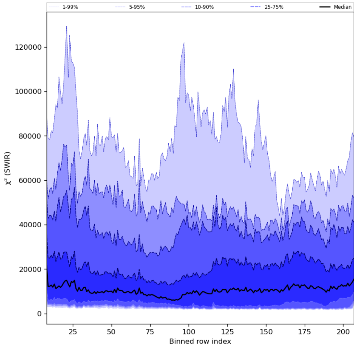
Figure 39: Along track statistics of “ \chi^2 (SWIR)” for 2023-11-21 to 2023-11-23
