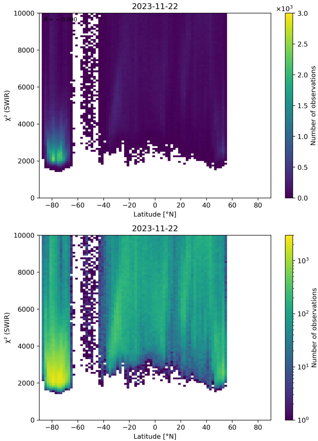
Figure 54: Scatter density plot of “Latitude” against “ \chi^2 (SWIR)” for 2023-11-21 to 2023-11-23.
