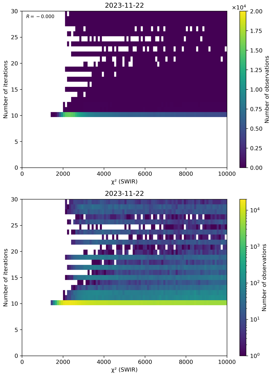
Figure 50: Scatter density plot of “ \chi^2 (SWIR)” against “Number of iterations” for 2023-11-21 to 2023-11-23.
