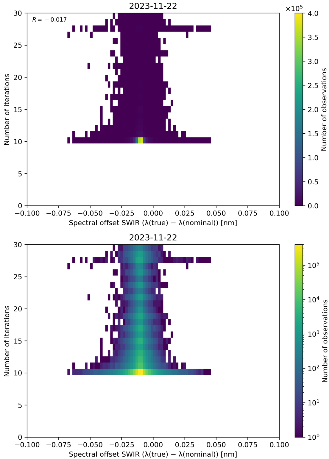
Figure 121: Scatter density plot of “Spectral offset SWIR ( \lambda(\text{true}) - \lambda(\text{nominal}) )” against “Number of iterations” for 2023-11-21 to 2023-11-23.
