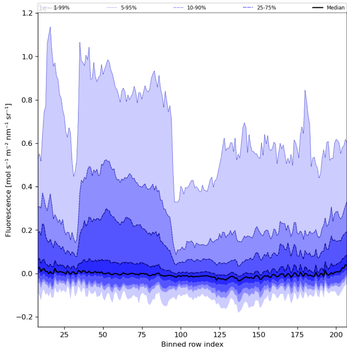
Figure 43: Along track statistics of “Fluorescence” for 2023-11-21 to 2023-11-23
