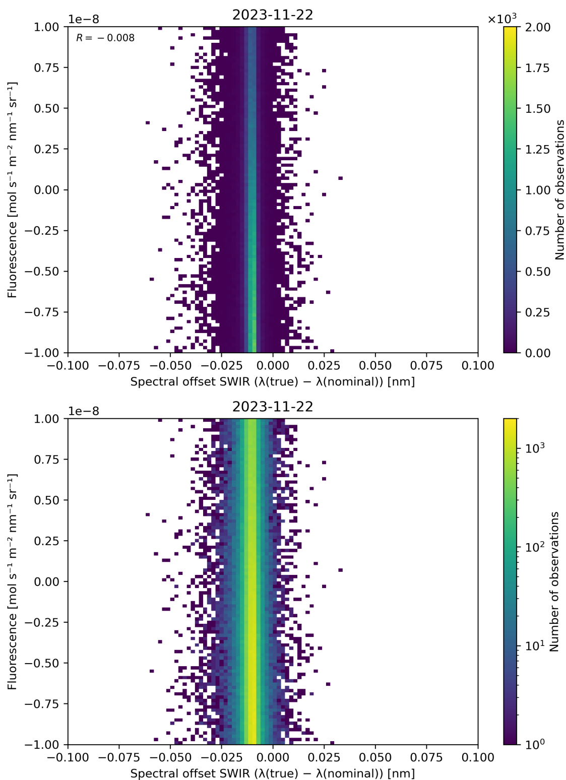
Figure 120: Scatter density plot of “Spectral offset SWIR ( \lambda(\text{true}) - \lambda(\text{nominal}) )” against “Fluorescence” for 2023-11-21 to 2023-11-23.
