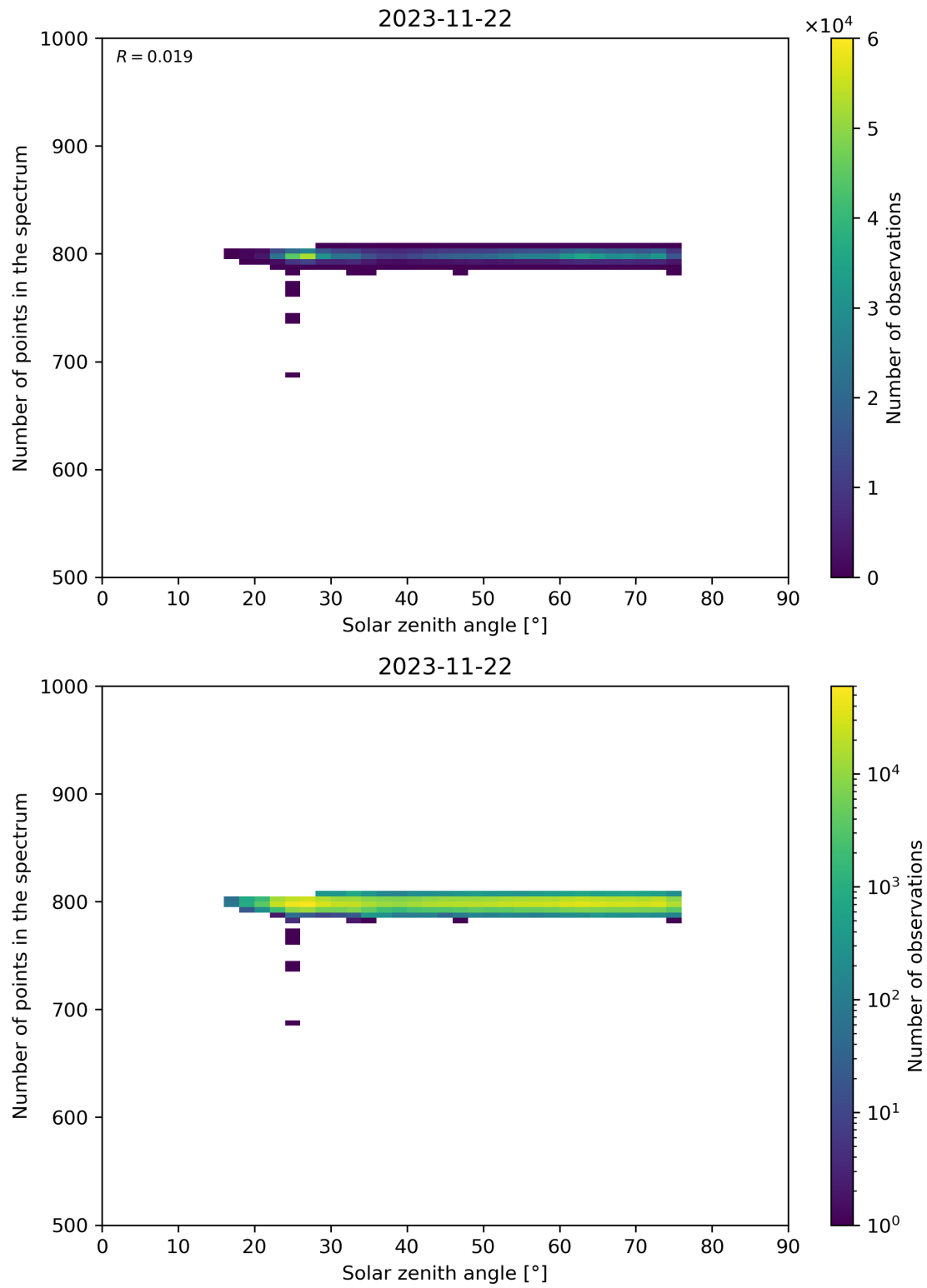
Figure 103: Scatter density plot of “Solar zenith angle” against “Number of points in the spectrum” for 2023-11-21 to 2023-11-23.
