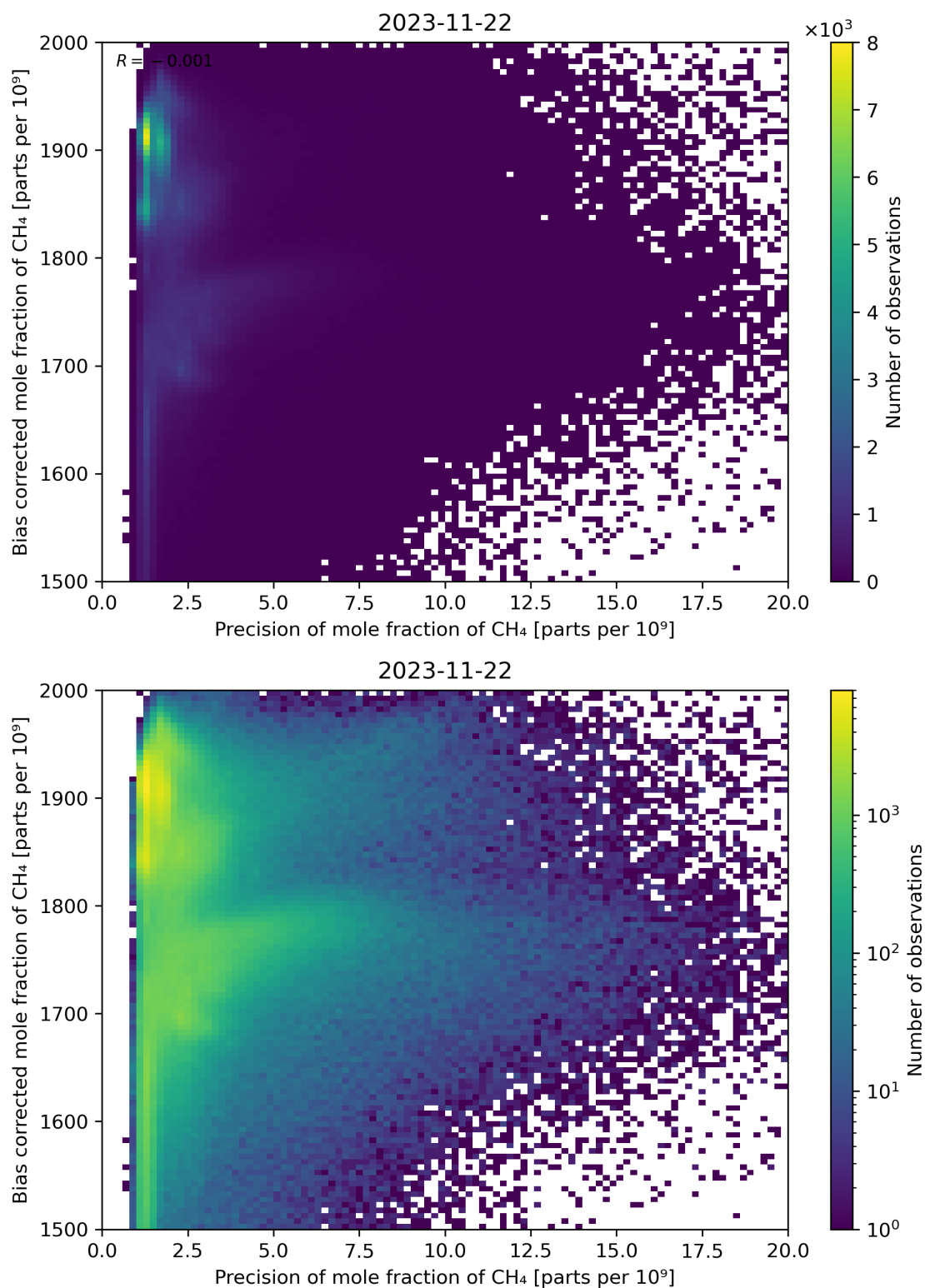
Figure 82: Scatter density plot of “Precision of mole fraction of CH 4 ” against “Bias corrected mole fraction of CH 4 ” for 2023-11-21 to 2023-11-23.
