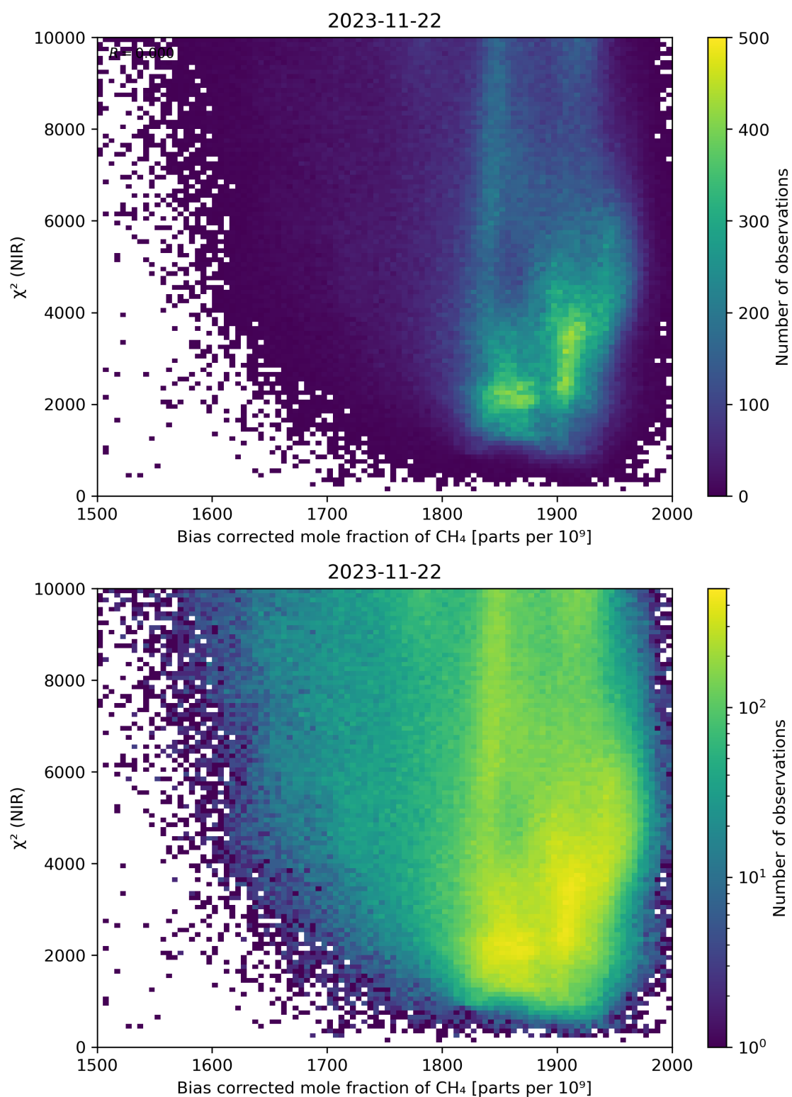
Figure 63: Scatter density plot of “Bias corrected mole fraction of CH 4 ” against “ \chi^2 (NIR)” for 2023-11-21 to 2023-11-23.
