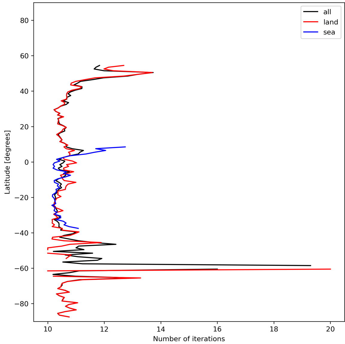
Figure 20: Zonal average of “Number of iterations” for 2023-11-21 to 2023-11-23.
