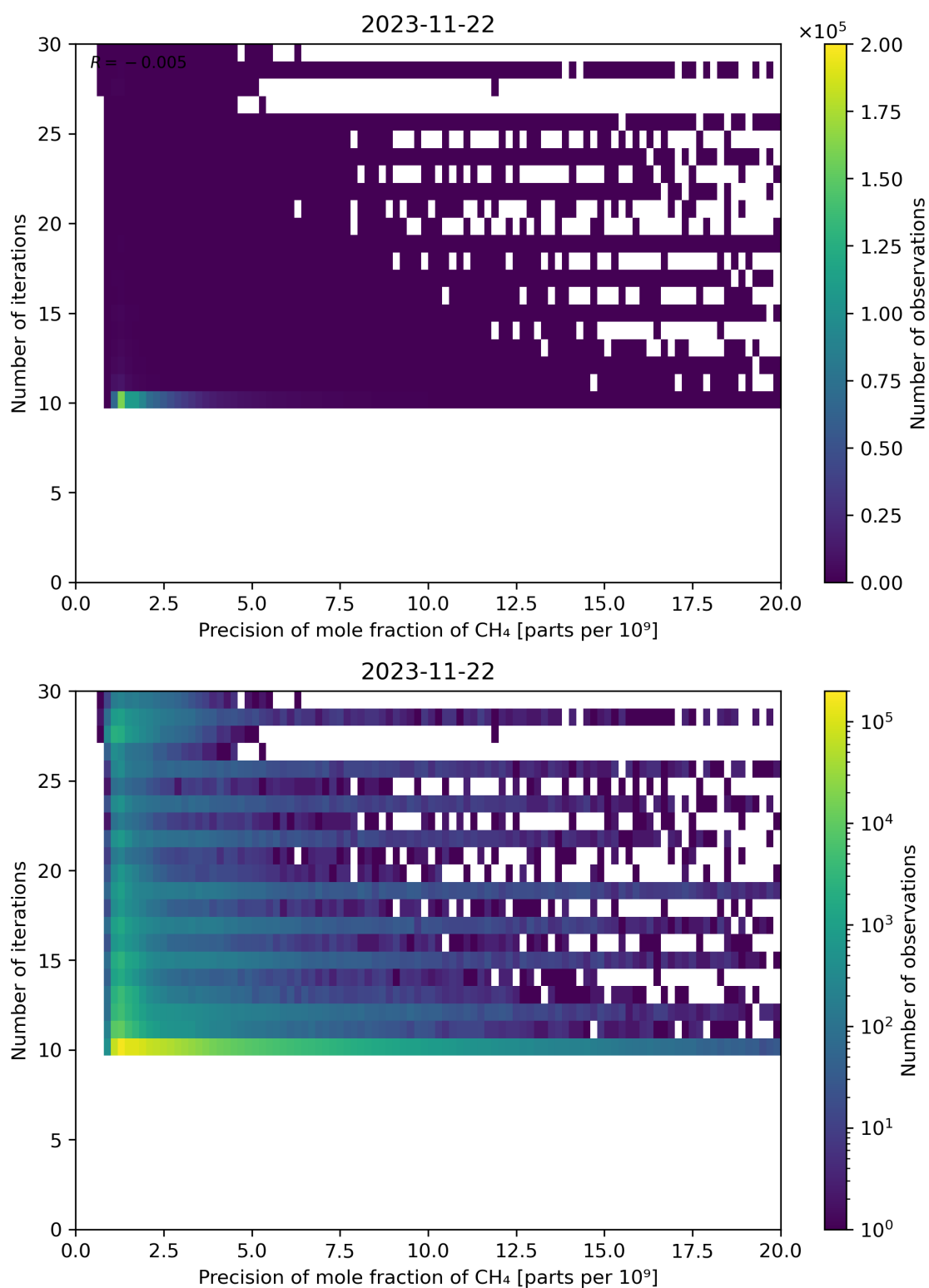
Figure 83: Scatter density plot of “Precision of mole fraction of CH 4 ” against “Number of iterations” for 2023-11-21 to 2023-11-23.
