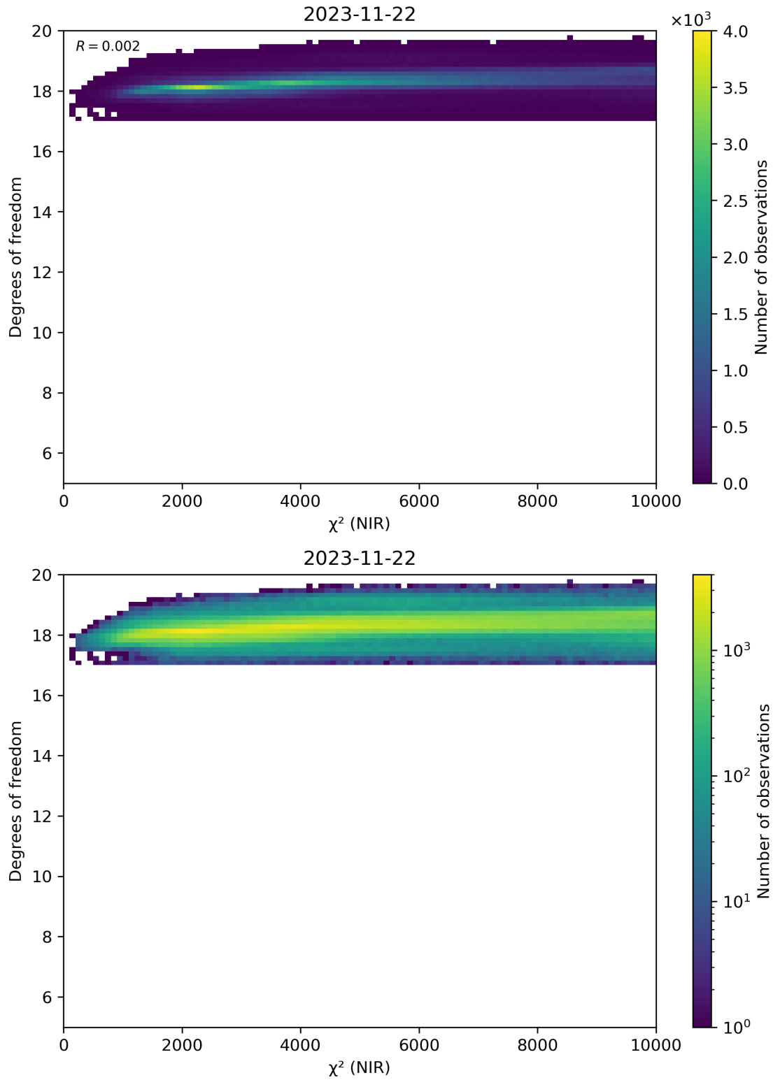
Figure 44: Scatter density plot of “ \chi^2 (NIR)” against “Degrees of freedom” for 2023-11-21 to 2023-11-23.
