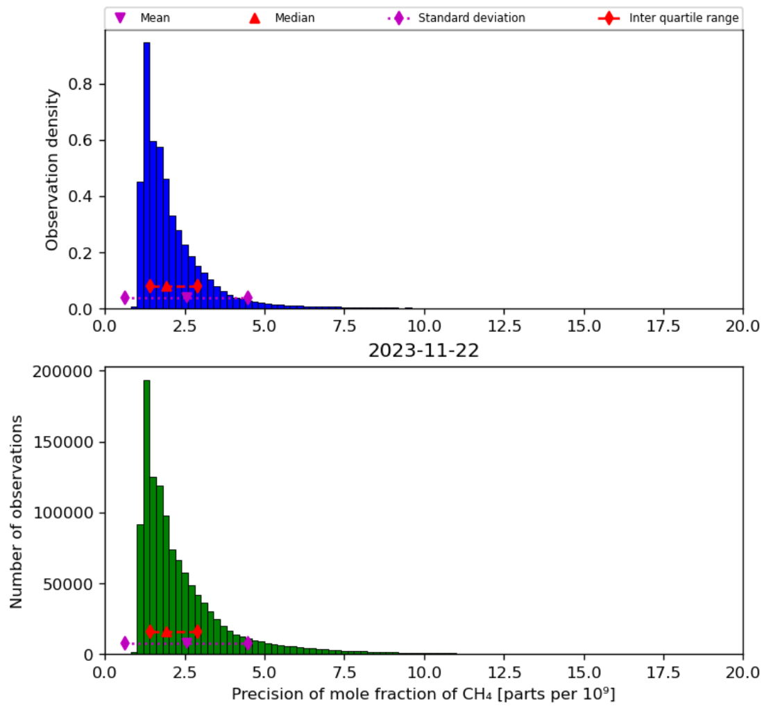
Figure 24: Histogram of “Precision of mole fraction of CH 4 ” for 2023-11-21 to 2023-11-23
