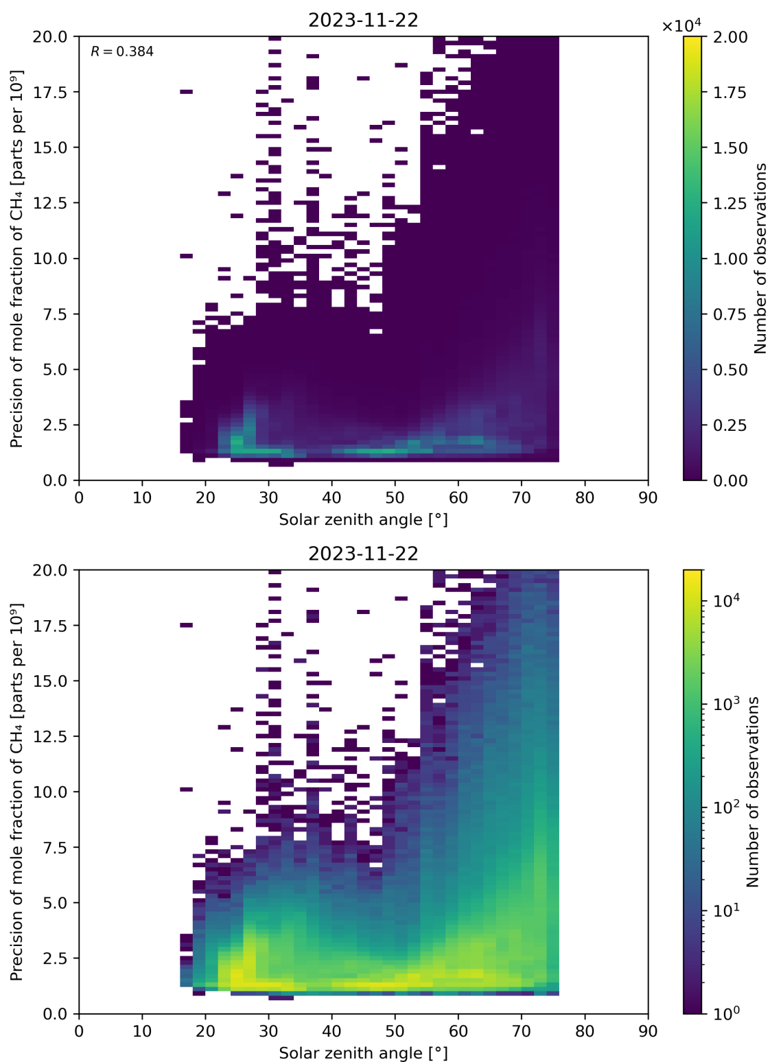
Figure 101: Scatter density plot of “Solar zenith angle” against “Precision of mole fraction of CH 4 ” for 2023-11-21 to 2023-11-23.
