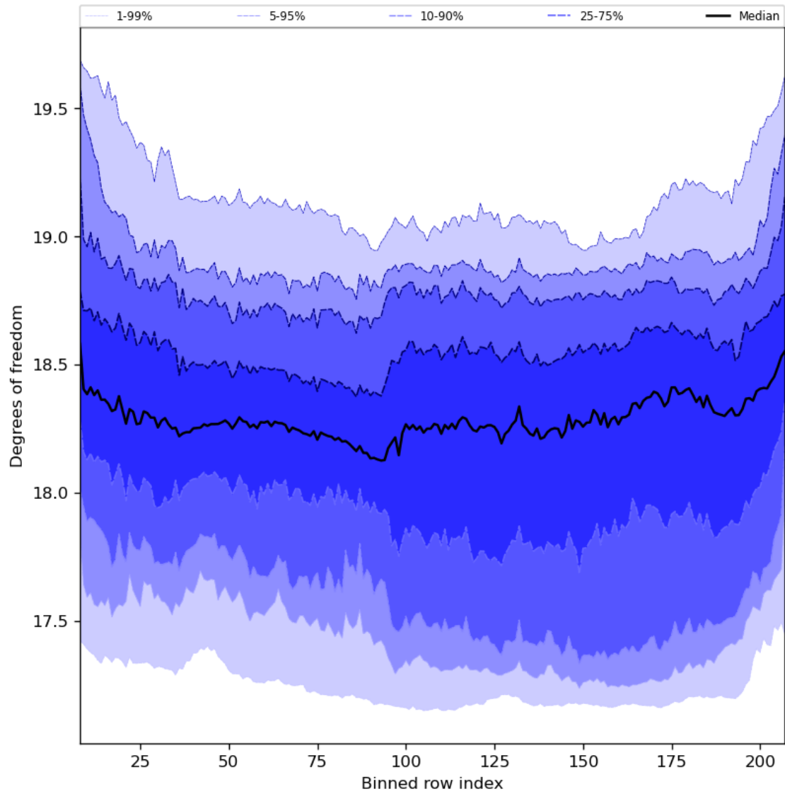
Figure 41: Along track statistics of “Degrees of freedom” for 2023-11-21 to 2023-11-23
