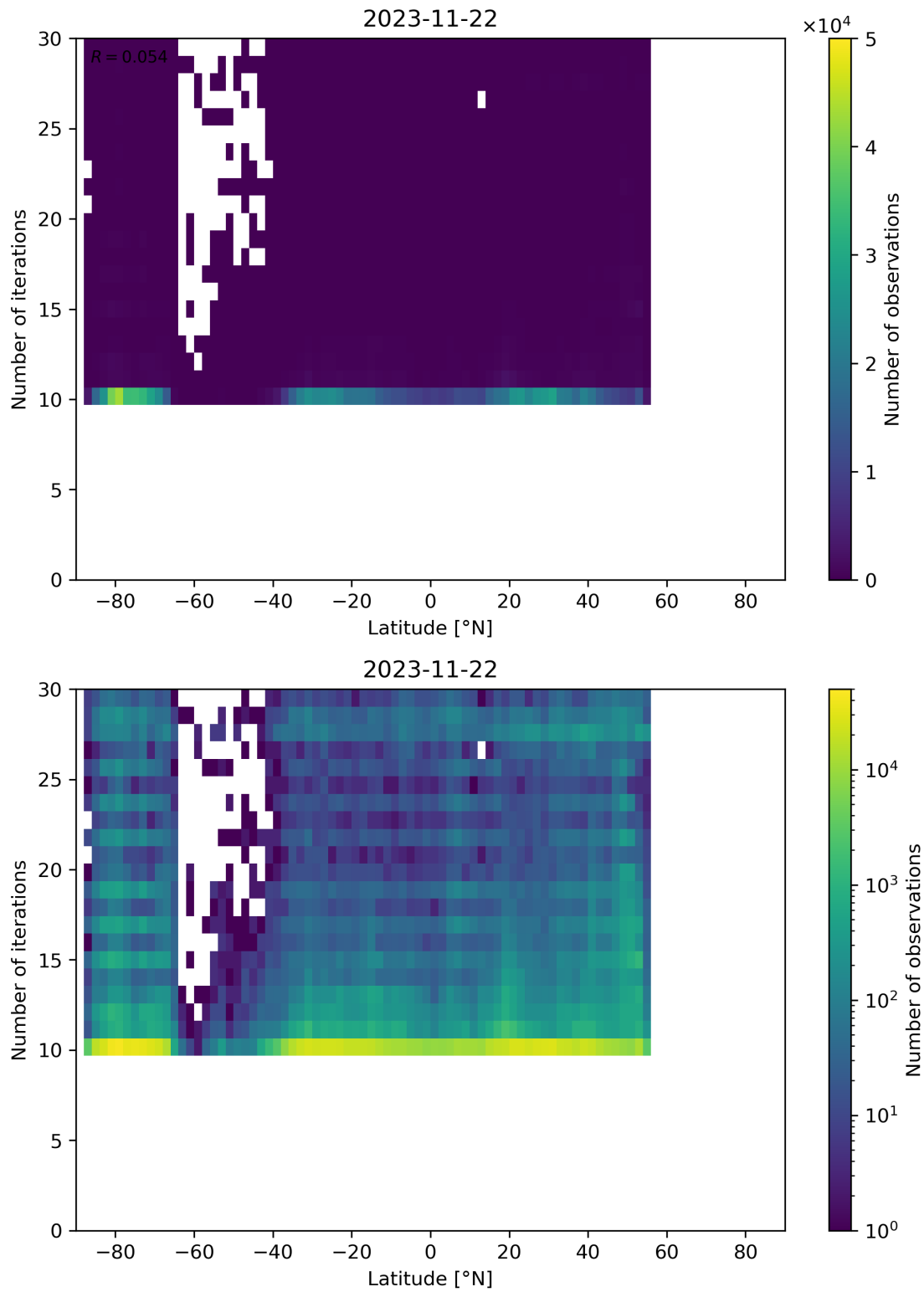
Figure 60: Scatter density plot of “Latitude” against “Number of iterations” for 2023-11-21 to 2023-11-23.
