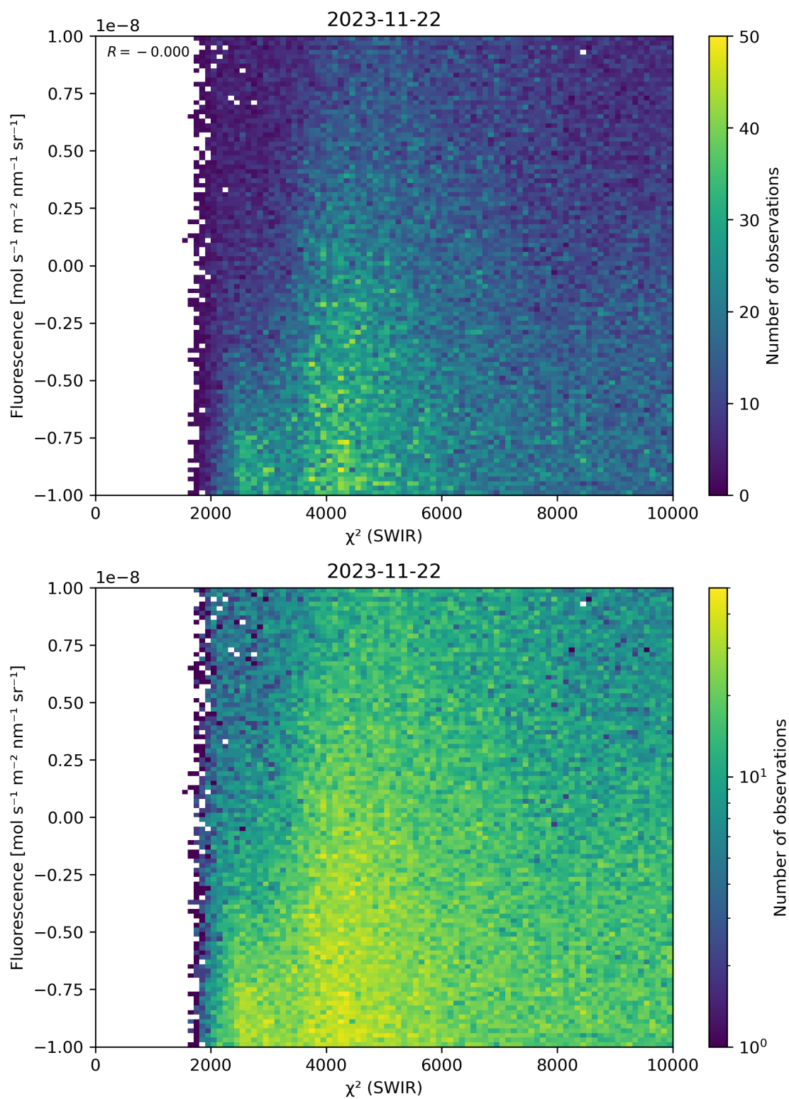
Figure 49: Scatter density plot of “ \chi^2 (SWIR)” against “Fluorescence” for 2023-11-21 to 2023-11-23.
