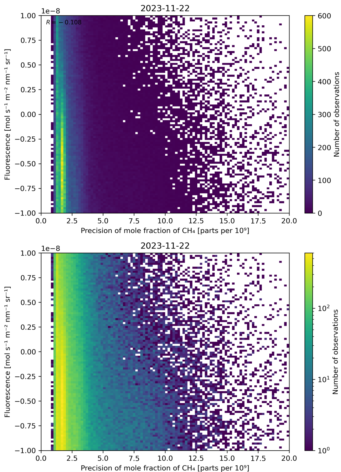
Figure 81: Scatter density plot of “Precision of mole fraction of \text{CH}_4 ” against “Fluorescence” for 2023-11-21 to 2023-11-23.
