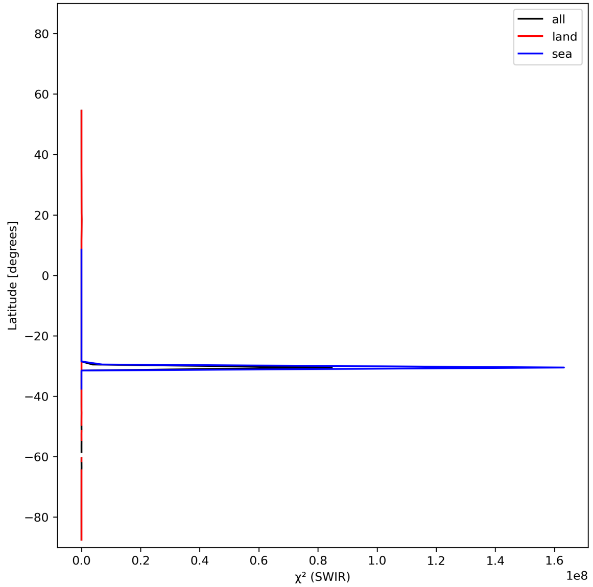
Figure 17: Zonal average of “ \chi^2 (SWIR)” for 2023-11-21 to 2023-11-23.
