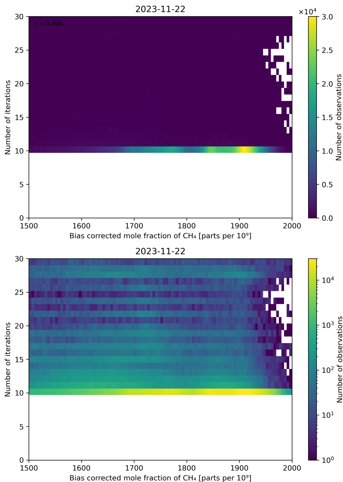
Figure 67: Scatter density plot of “Bias corrected mole fraction of \text{CH}_4 ” against “Number of iterations” for 2023-11-21 to 2023-11-23.
