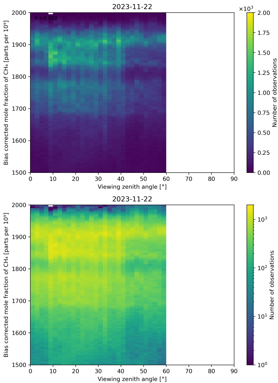
Figure 111: Scatter density plot of “Viewing zenith angle” against “Bias corrected mole fraction of CH 4 ” for 2023-11-21 to 2023-11-23.
