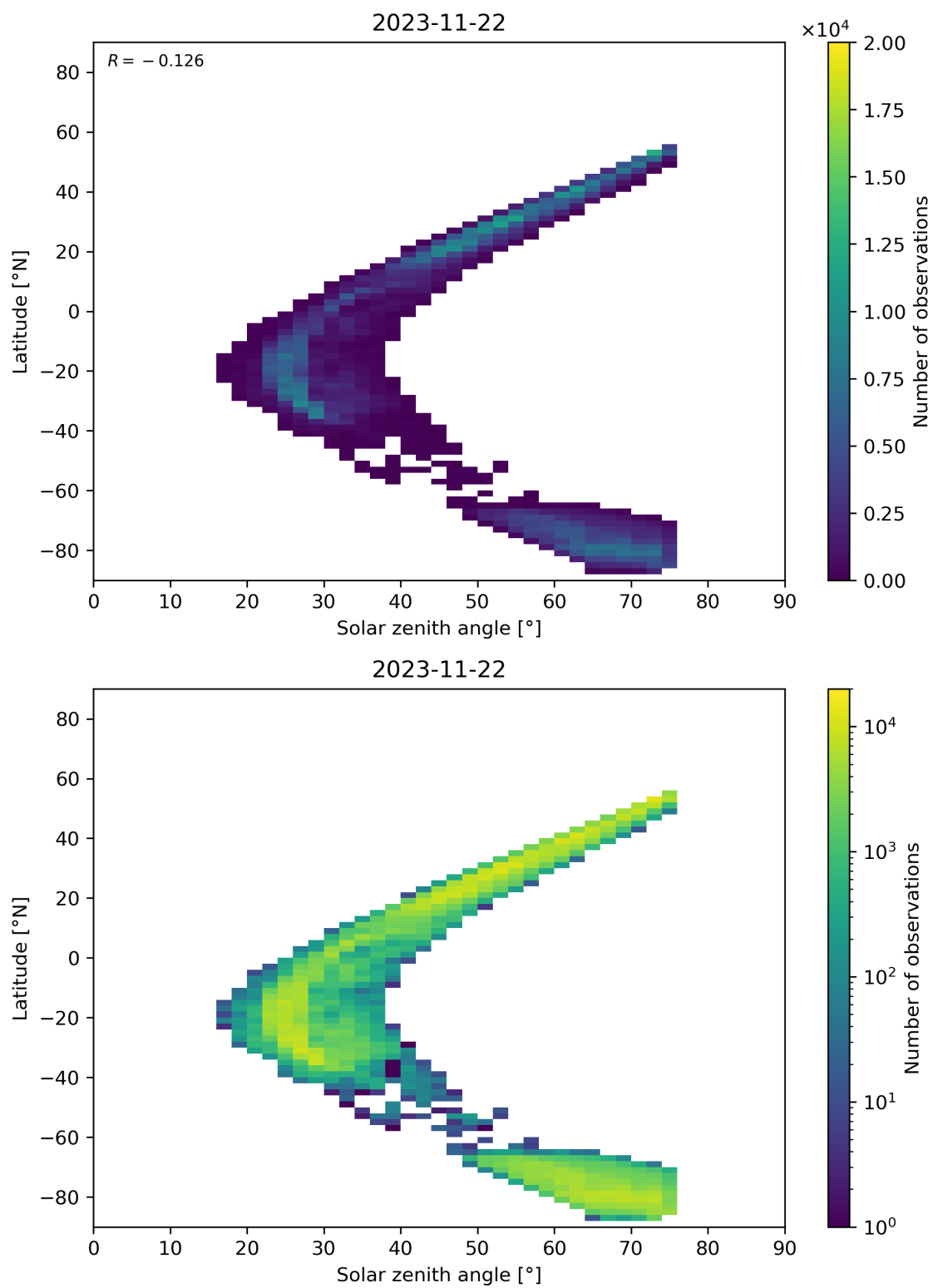
Figure 98: Scatter density plot of “Solar zenith angle” against “Latitude” for 2023-11-21 to 2023-11-23.
