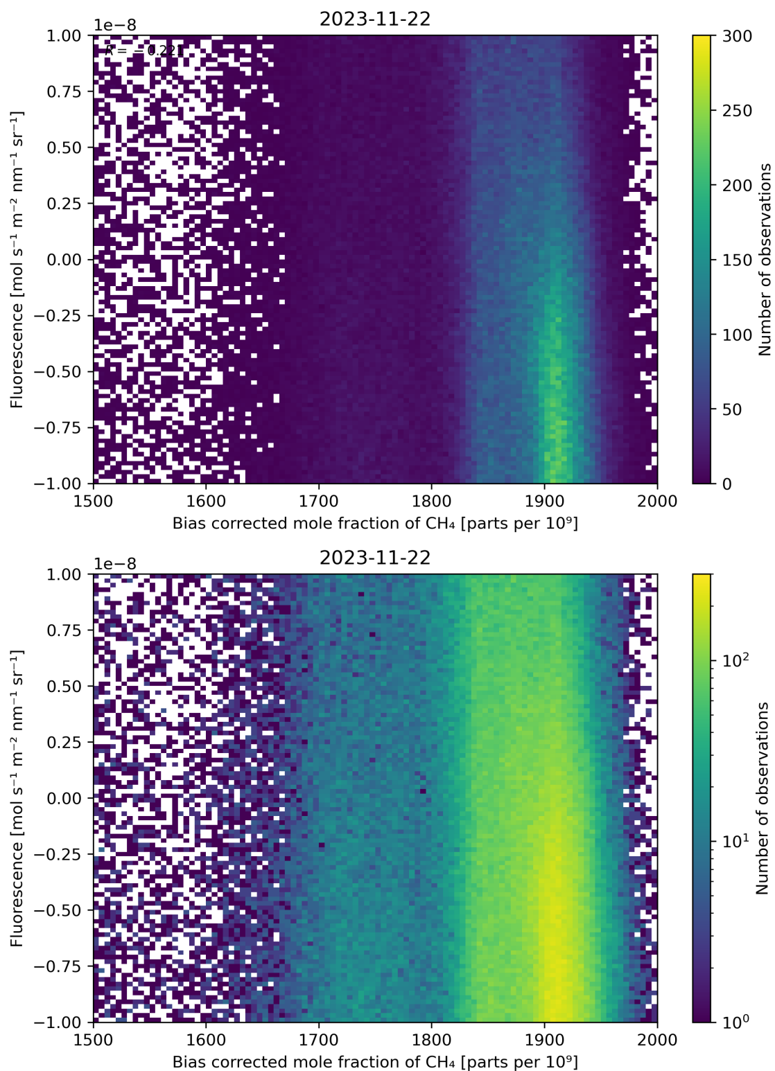
Figure 66: Scatter density plot of “Bias corrected mole fraction of \text{CH}_4 ” against “Fluorescence” for 2023-11-21 to 2023-11-23.
