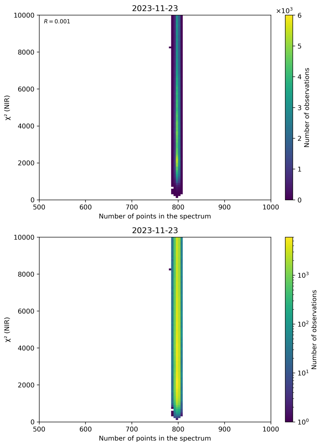
Figure 88: Scatter density plot of “Number of points in the spectrum” against “ \chi^2 (NIR)” for 2023-11-23 to 2023-11-24.
