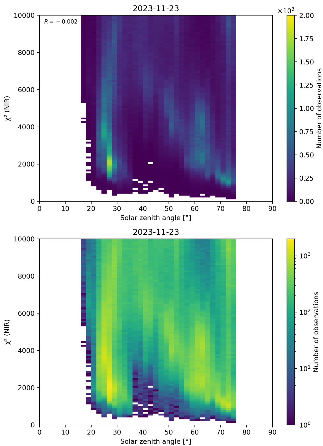
Figure 94: Scatter density plot of “Solar zenith angle” against “ \chi^2 (NIR)” for 2023-11-23 to 2023-11-24.
