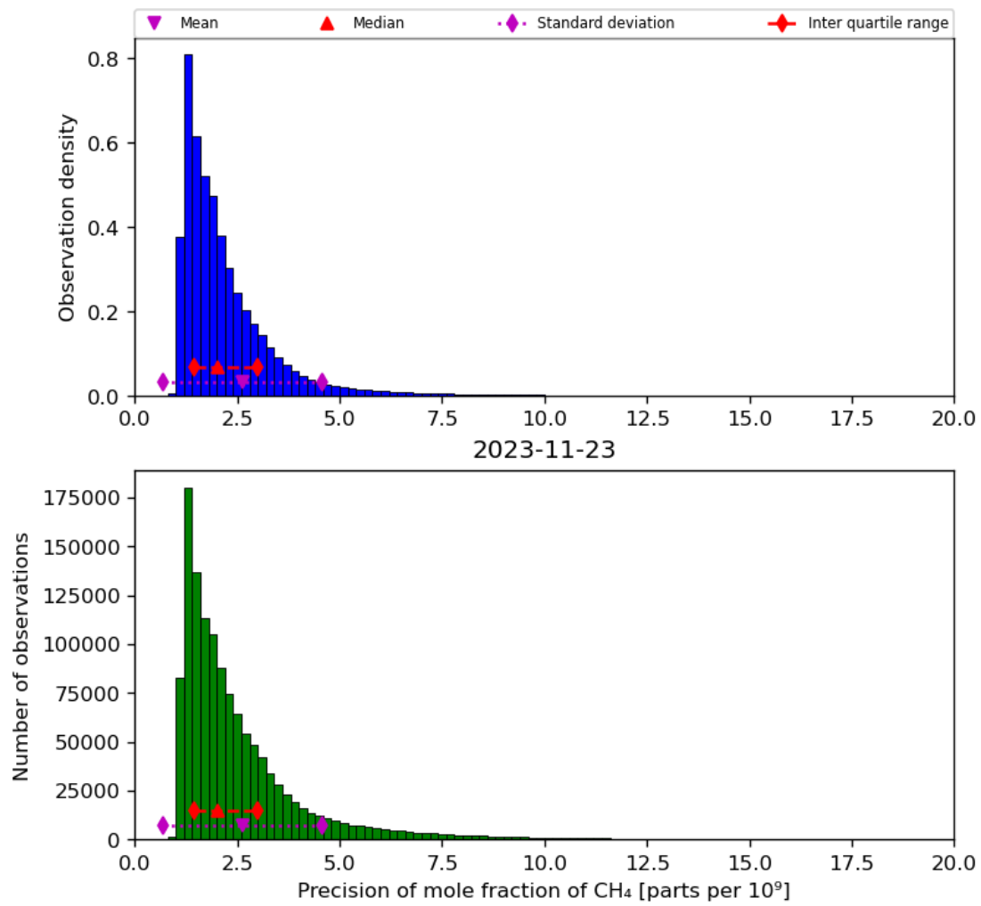
Figure 24: Histogram of “Precision of mole fraction of CH 4 ” for 2023-11-23 to 2023-11-24
