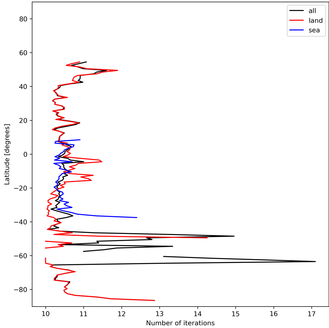
Figure 20: Zonal average of “Number of iterations” for 2023-11-23 to 2023-11-24.
