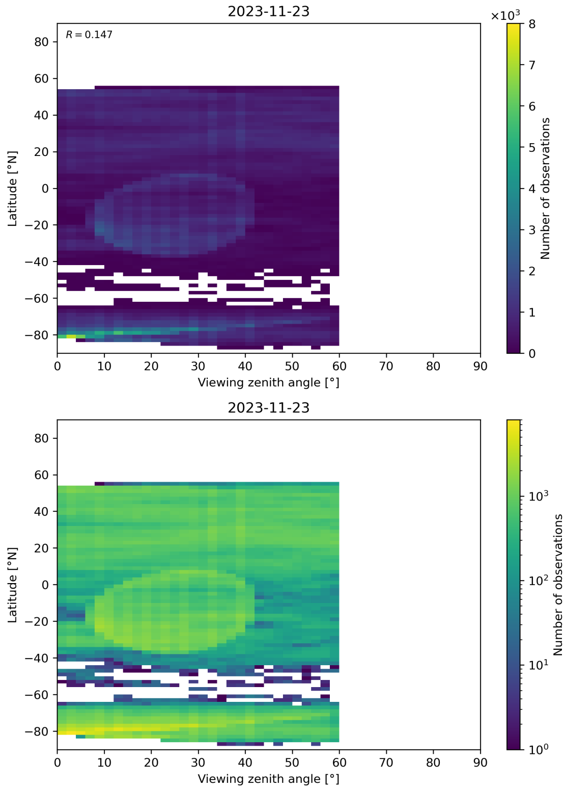
Figure 109: Scatter density plot of “Viewing zenith angle” against “Latitude” for 2023-11-23 to 2023-11-24.
