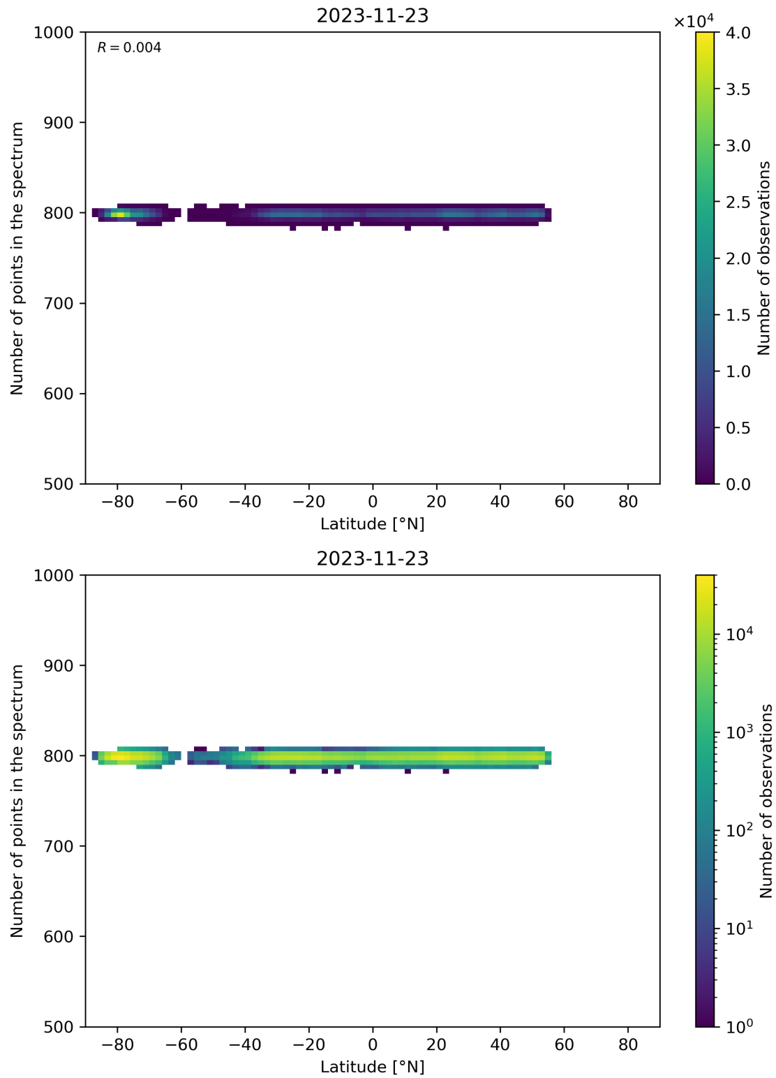
Figure 61: Scatter density plot of “Latitude” against “Number of points in the spectrum” for 2023-11-23 to 2023-11-24.
