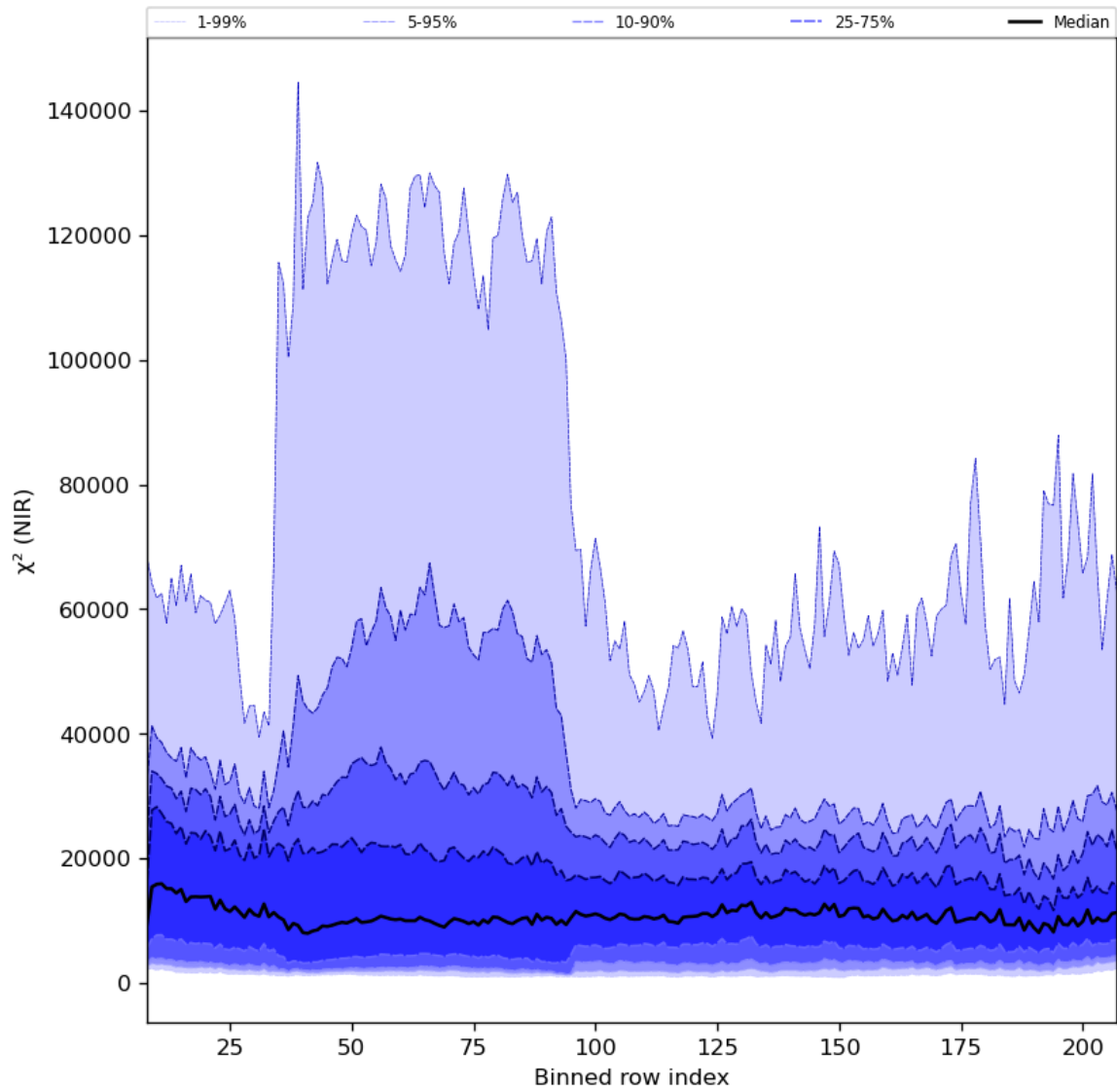
Figure 40: Along track statistics of “ \chi^2 (NIR)” for 2023-11-23 to 2023-11-24
