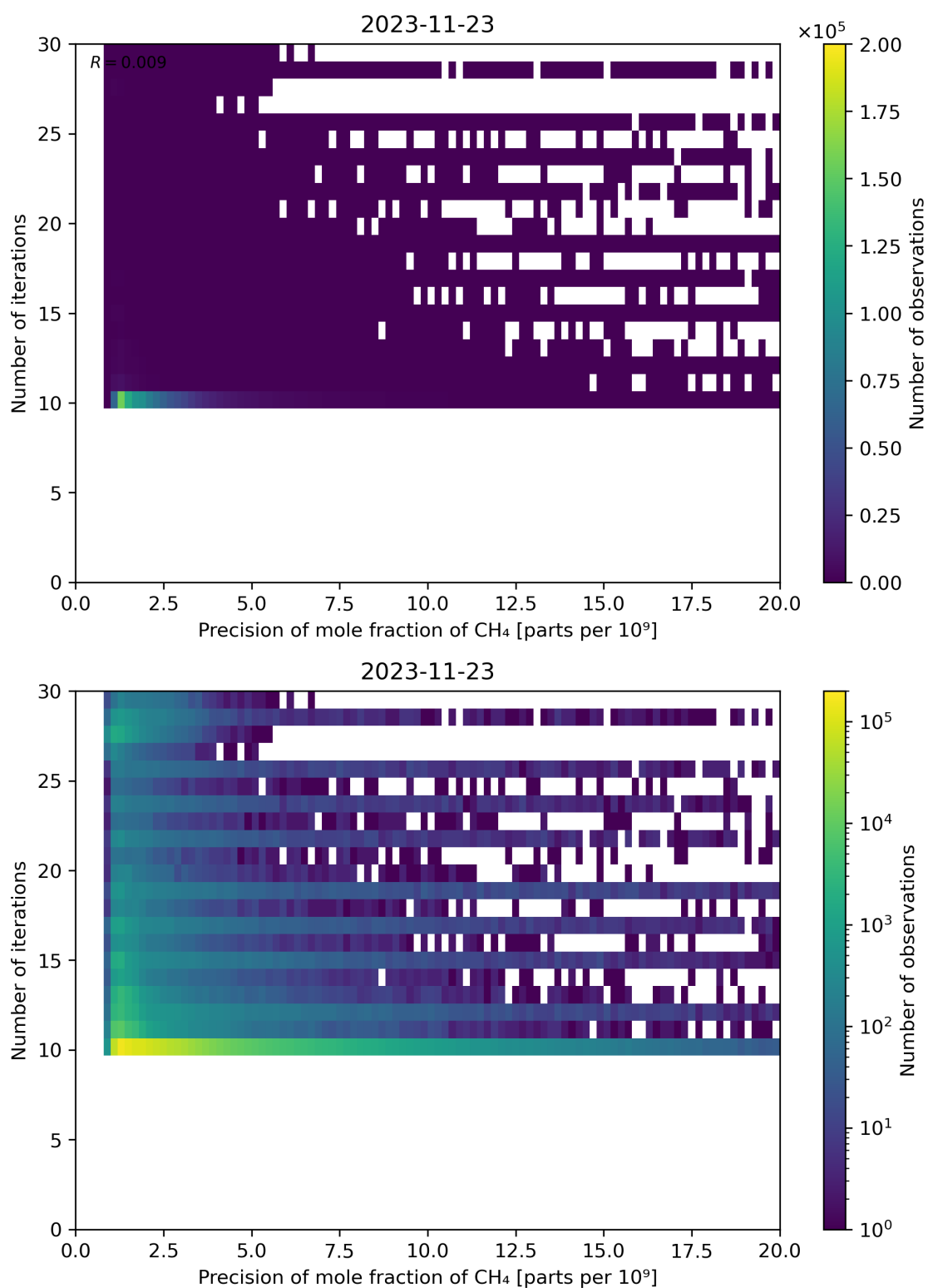
Figure 83: Scatter density plot of “Precision of mole fraction of CH 4 ” against “Number of iterations” for 2023-11-23 to 2023-11-24.
