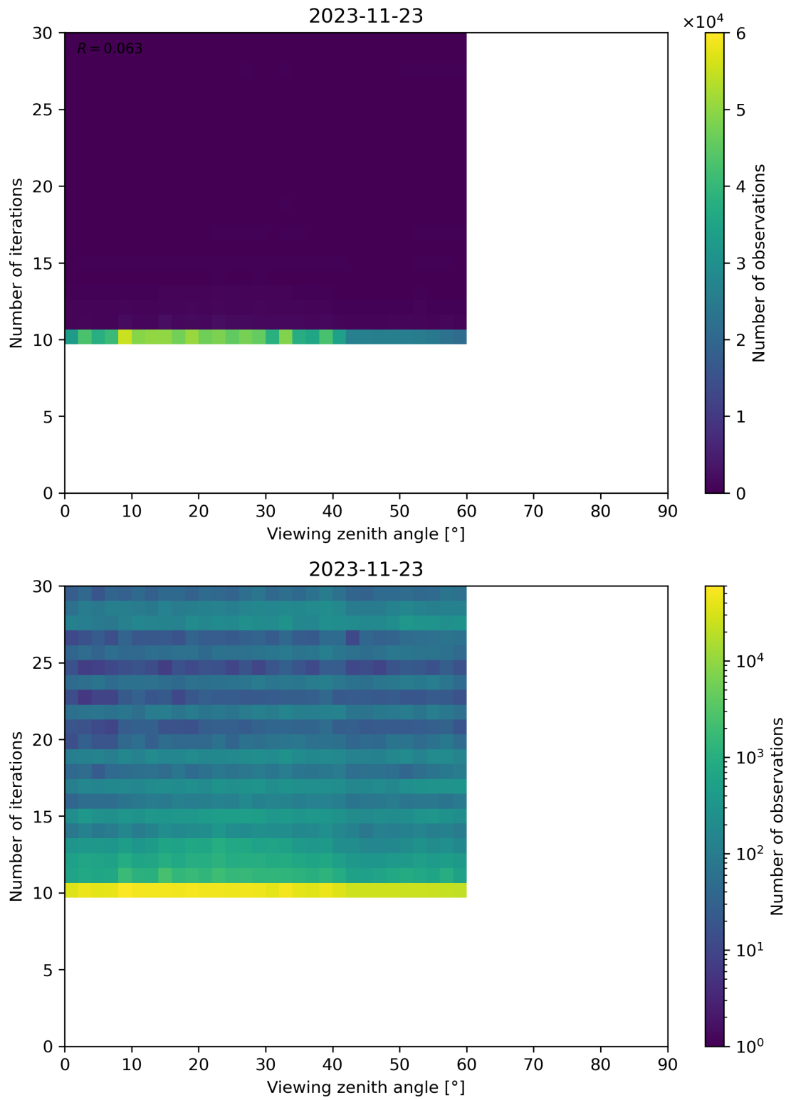
Figure 113: Scatter density plot of “Viewing zenith angle” against “Number of iterations” for 2023-11-23 to 2023-11-24.
