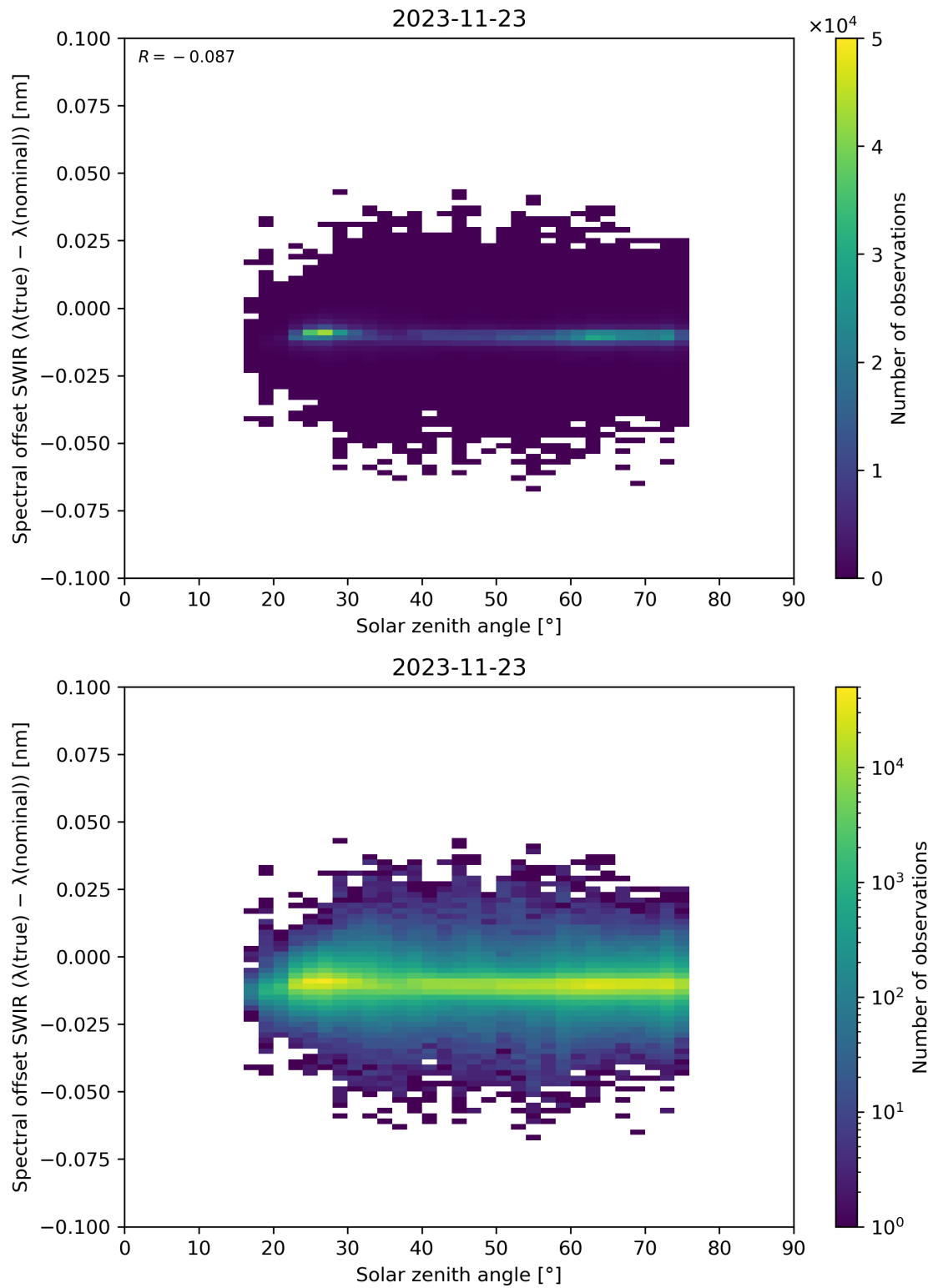
Figure 104: Scatter density plot of “Solar zenith angle” against “Spectral offset SWIR ( \lambda(\text{true}) - \lambda(\text{nominal}) )” for 2023-11-23 to 2023-11-24.
