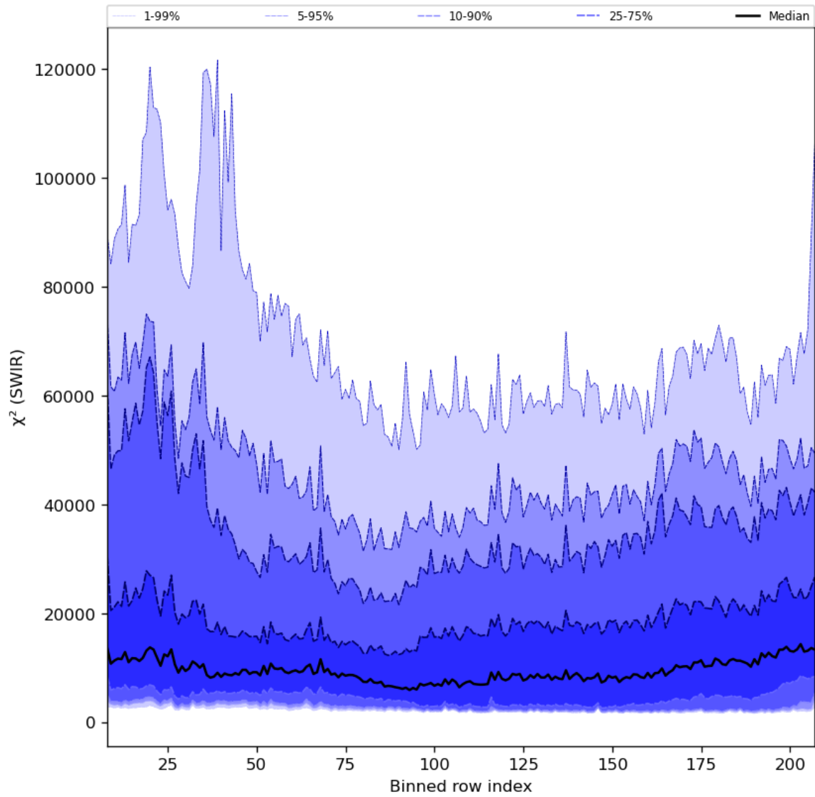
Figure 39: Along track statistics of “ \chi^2 (SWIR)” for 2023-11-23 to 2023-11-24
