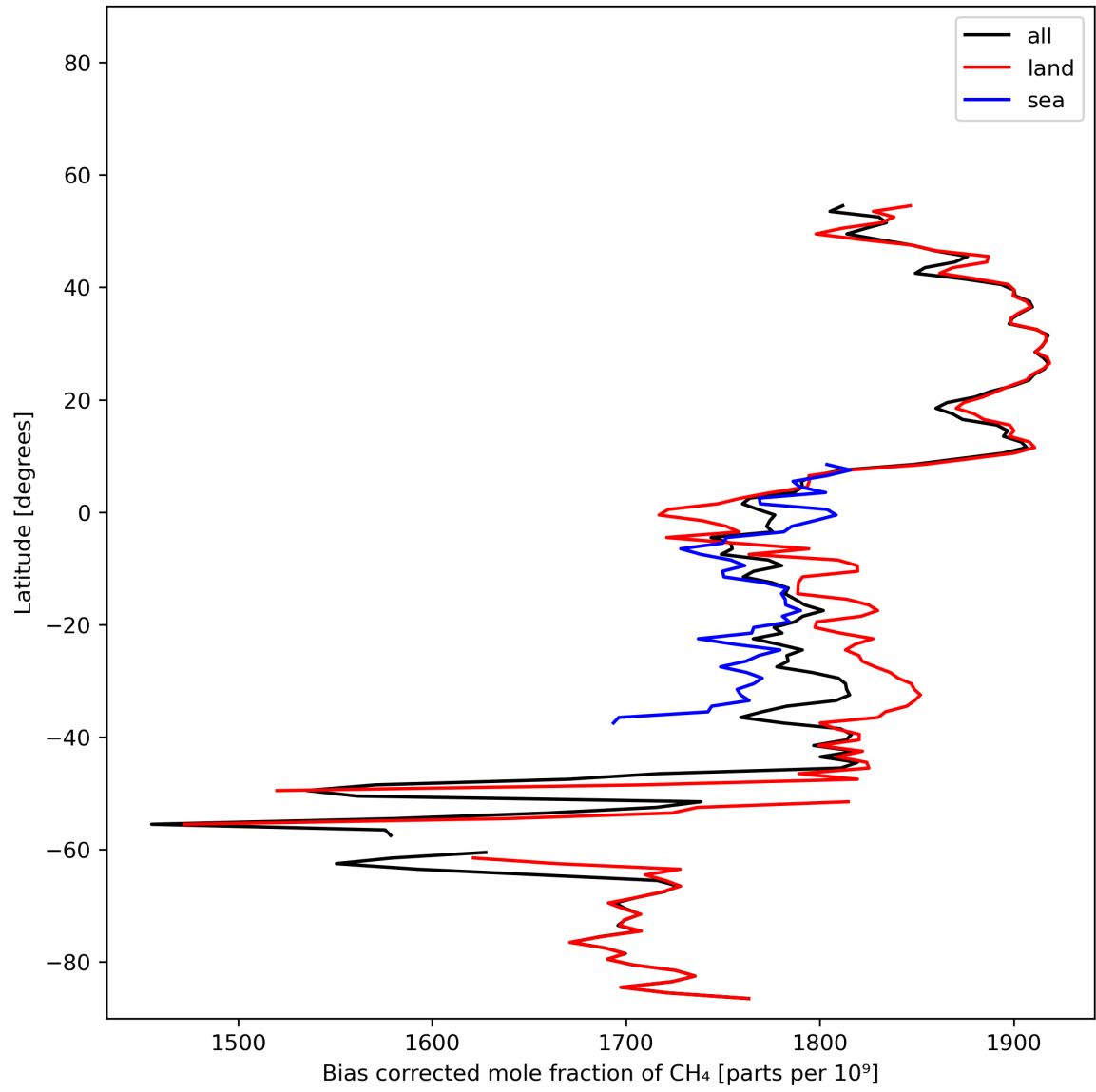
Figure 14: Zonal average of “Bias corrected mole fraction of CH 4 ” for 2023-11-23 to 2023-11-24.
