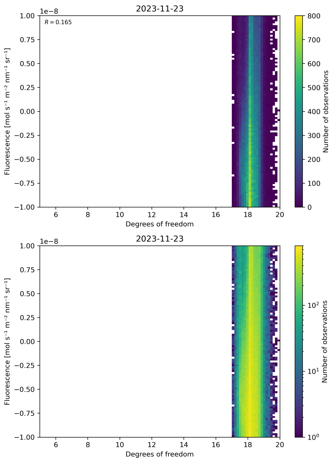
Figure 51: Scatter density plot of “Degrees of freedom” against “Fluorescence” for 2023-11-23 to 2023-11-24.
