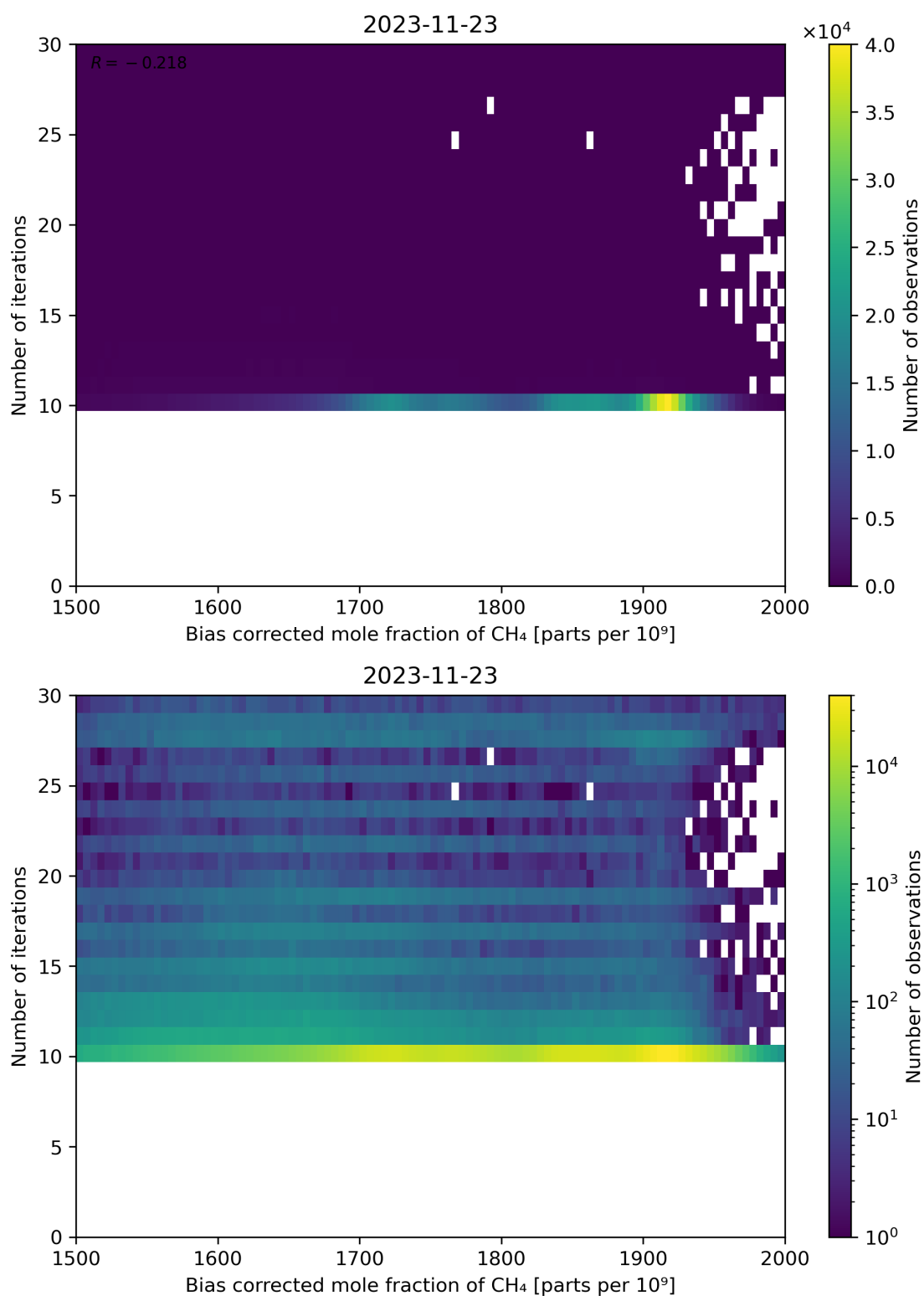
Figure 67: Scatter density plot of “Bias corrected mole fraction of CH 4 ” against “Number of iterations” for 2023-11-23 to 2023-11-24.
