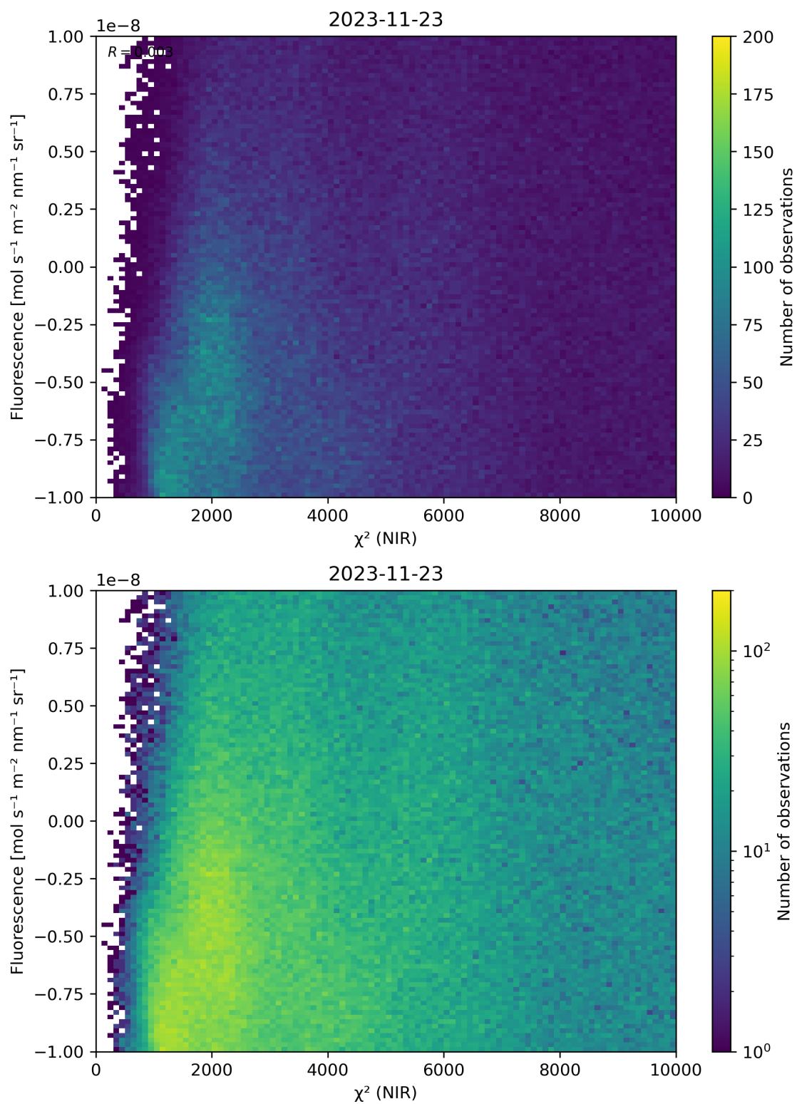
Figure 45: Scatter density plot of “ \chi^2 (NIR)” against “Fluorescence” for 2023-11-23 to 2023-11-24.
