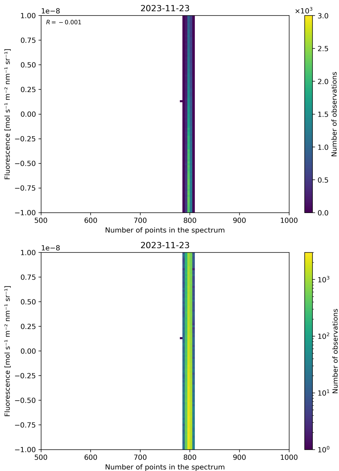
Figure 91: Scatter density plot of “Number of points in the spectrum” against “Fluorescence” for 2023-11-23 to 2023-11-24.
