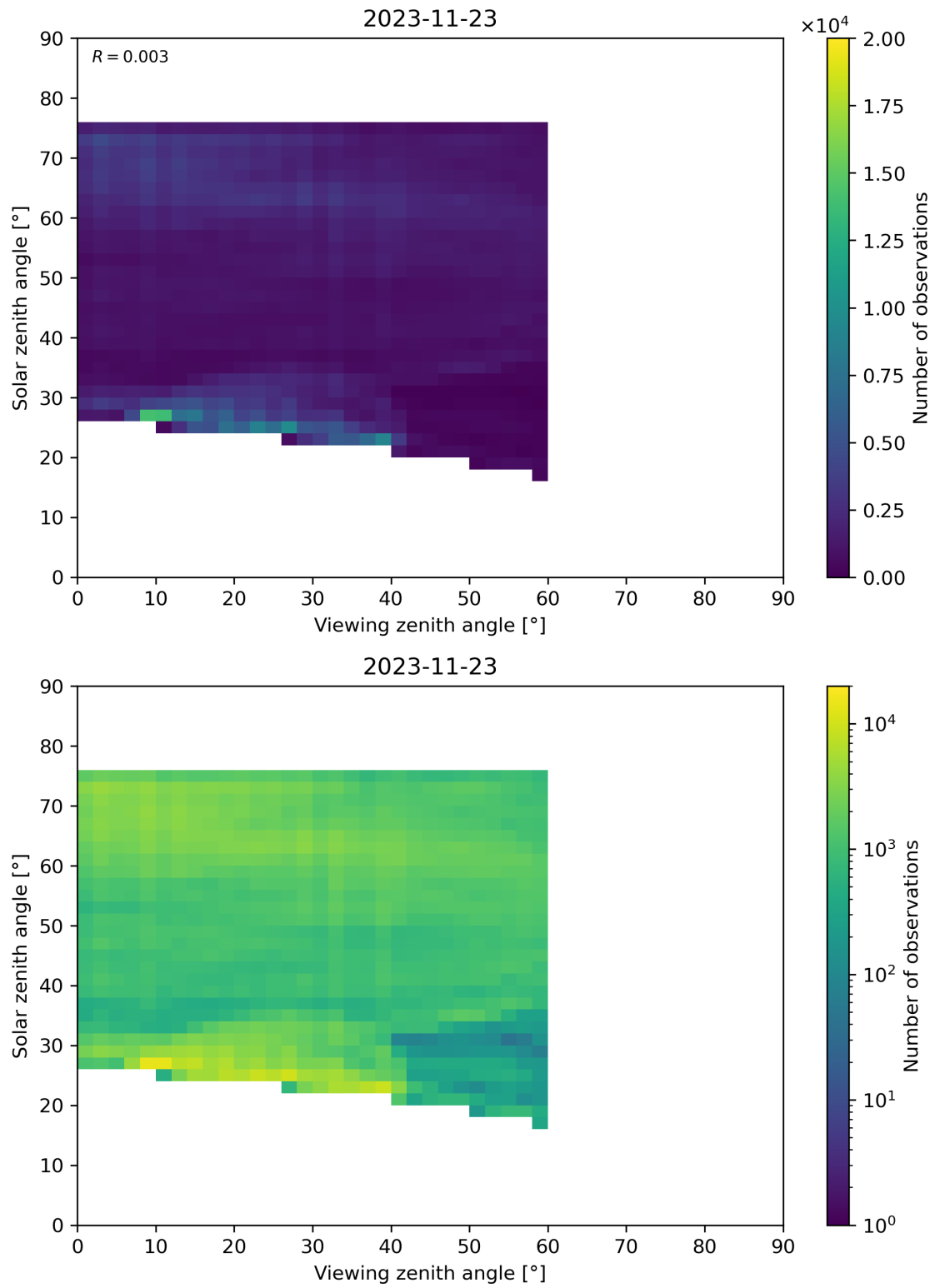
Figure 115: Scatter density plot of “Viewing zenith angle” against “Solar zenith angle” for 2023-11-23 to 2023-11-24.
