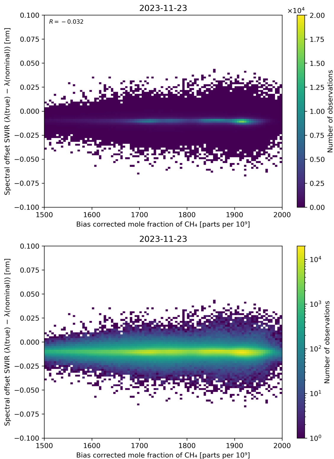
Figure 69: Scatter density plot of “Bias corrected mole fraction of \text{CH}_4 ” against “Spectral offset SWIR ( \lambda(\text{true}) - \lambda(\text{nominal}) )” for 2023-11-23 to 2023-11-24.
