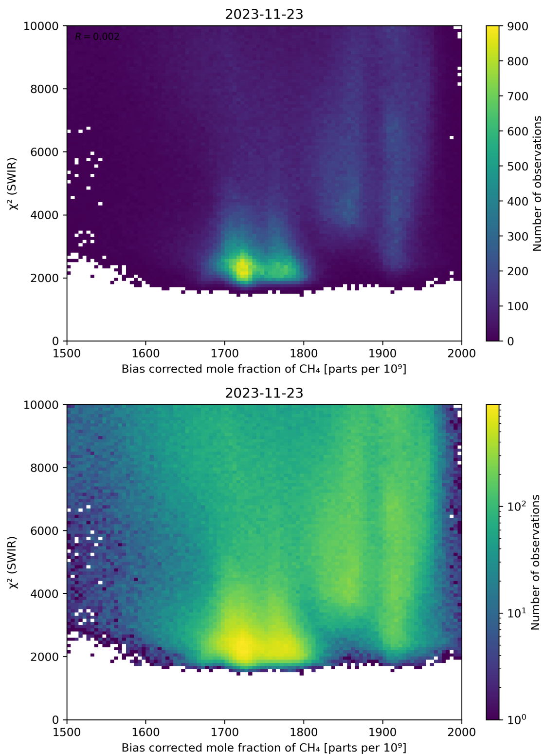
Figure 64: Scatter density plot of “Bias corrected mole fraction of CH 4 ” against “ \chi^2 (SWIR)” for 2023-11-23 to 2023-11-24.
