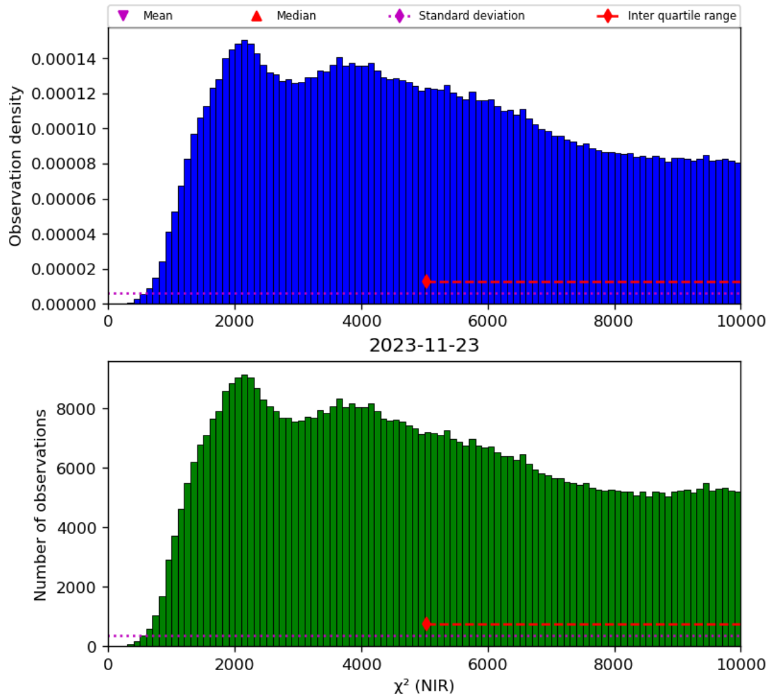
Figure 29: Histogram of “ \chi^2 (NIR)” for 2023-11-23 to 2023-11-24
