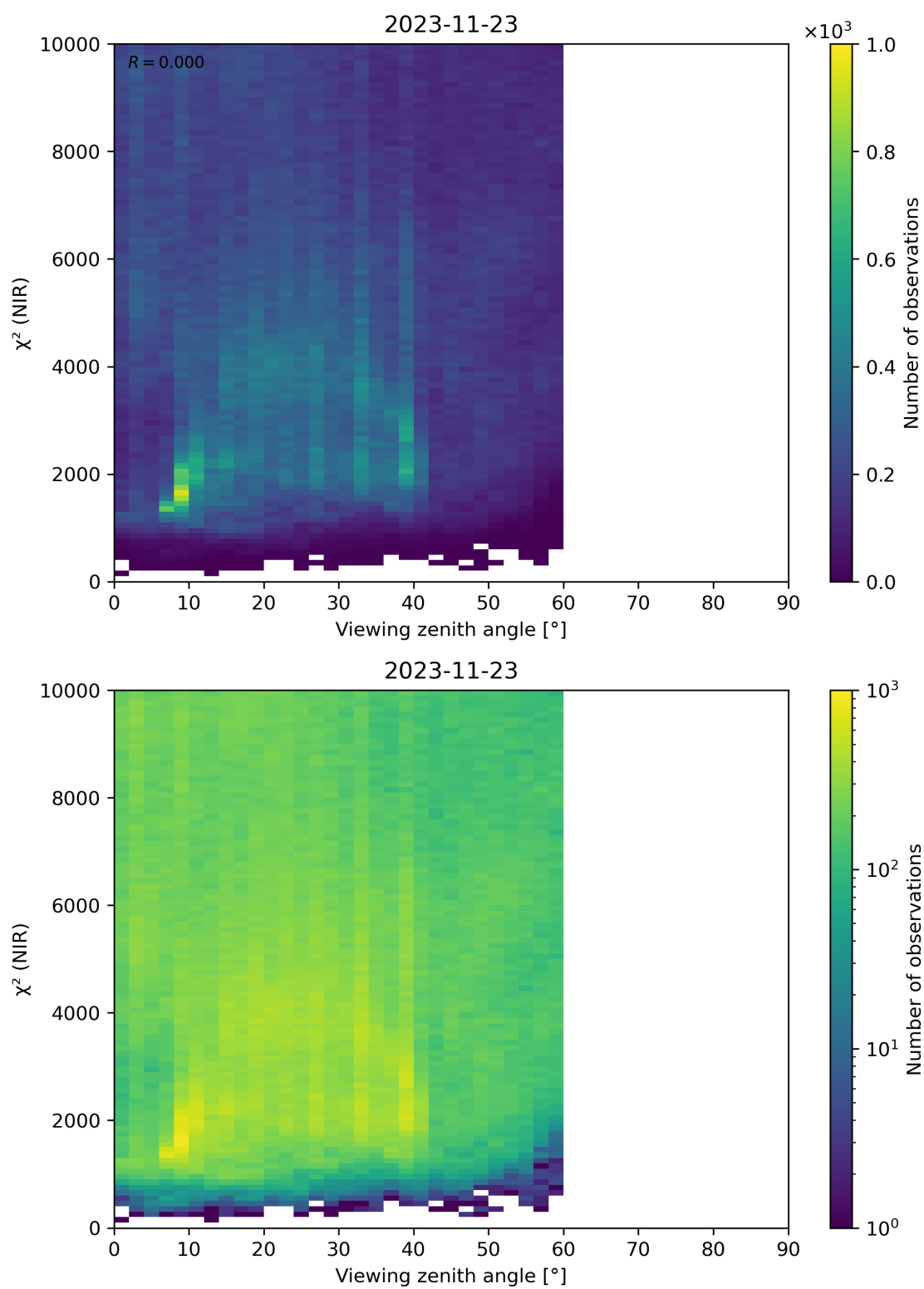
Figure 105: Scatter density plot of “Viewing zenith angle” against “ \chi^2 (NIR)” for 2023-11-23 to 2023-11-24.
