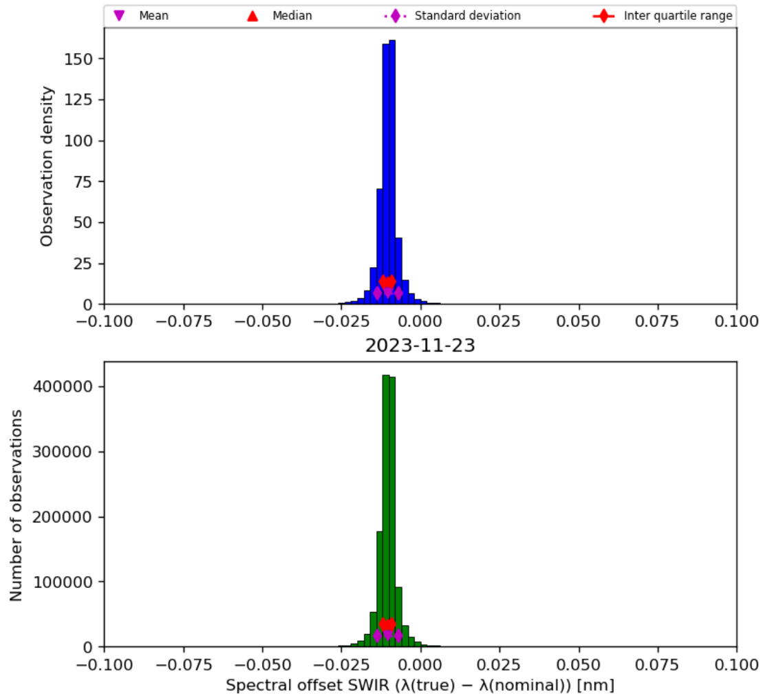
Figure 27: Histogram of “Spectral offset SWIR ( \lambda(\text{true}) - \lambda(\text{nominal}) )” for 2023-11-23 to 2023-11-24
