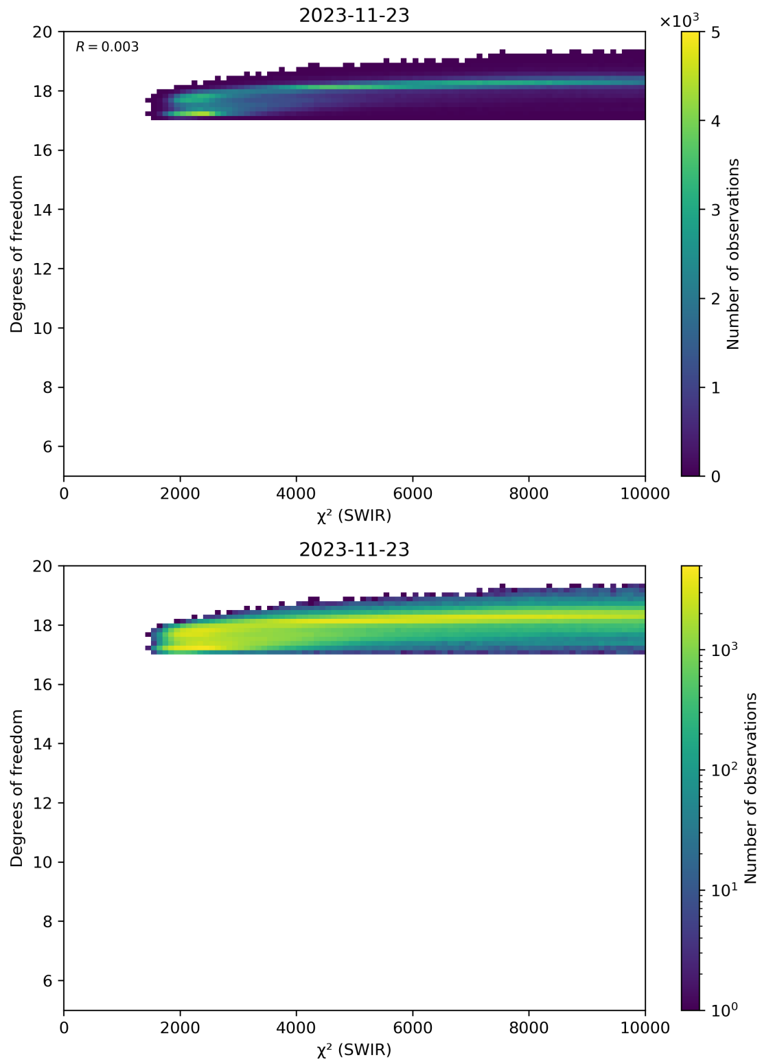
Figure 48: Scatter density plot of “ \chi^2 (SWIR)” against “Degrees of freedom” for 2023-11-23 to 2023-11-24.
