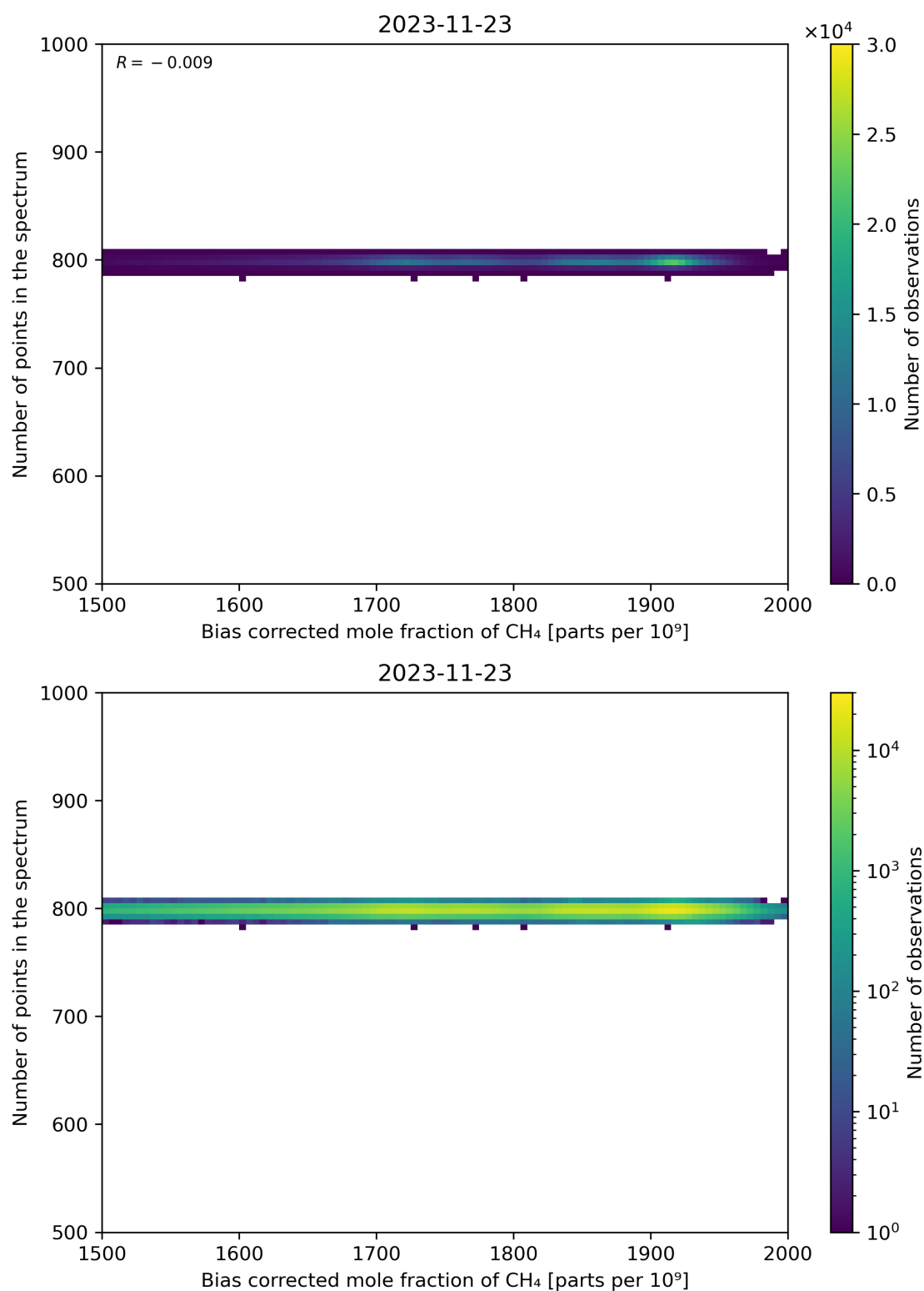
Figure 68: Scatter density plot of “Bias corrected mole fraction of CH 4 ” against “Number of points in the spectrum” for 2023-11-23 to 2023-11-24.
