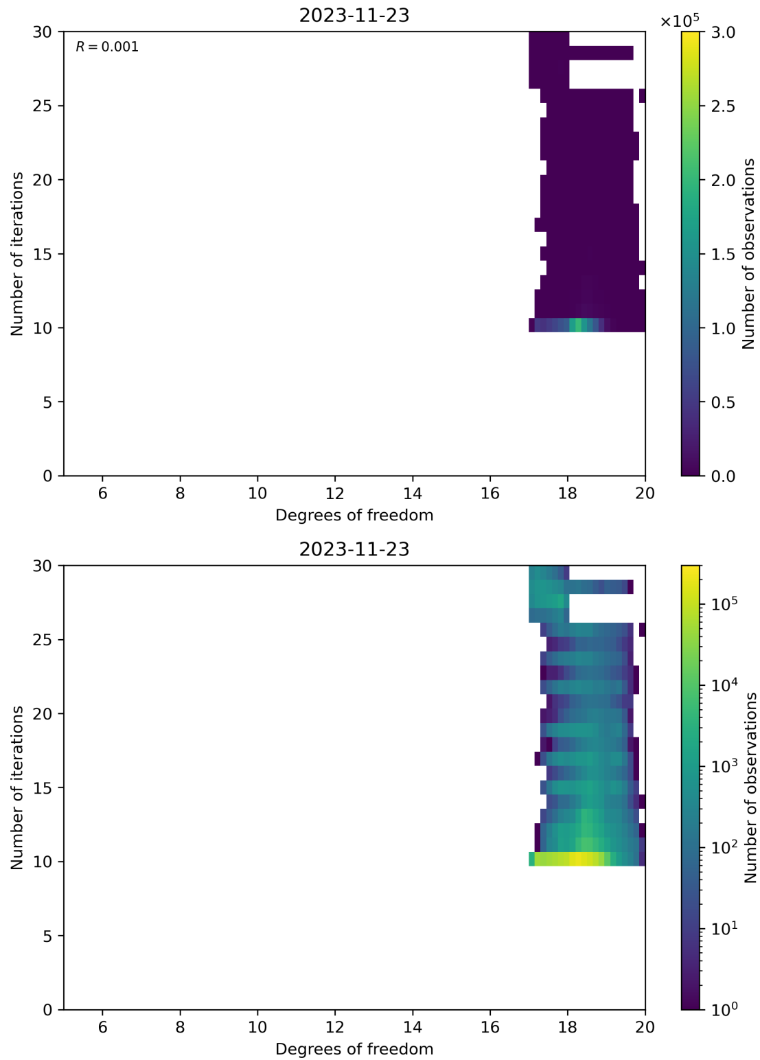
Figure 52: Scatter density plot of “Degrees of freedom” against “Number of iterations” for 2023-11-23 to 2023-11-24.
