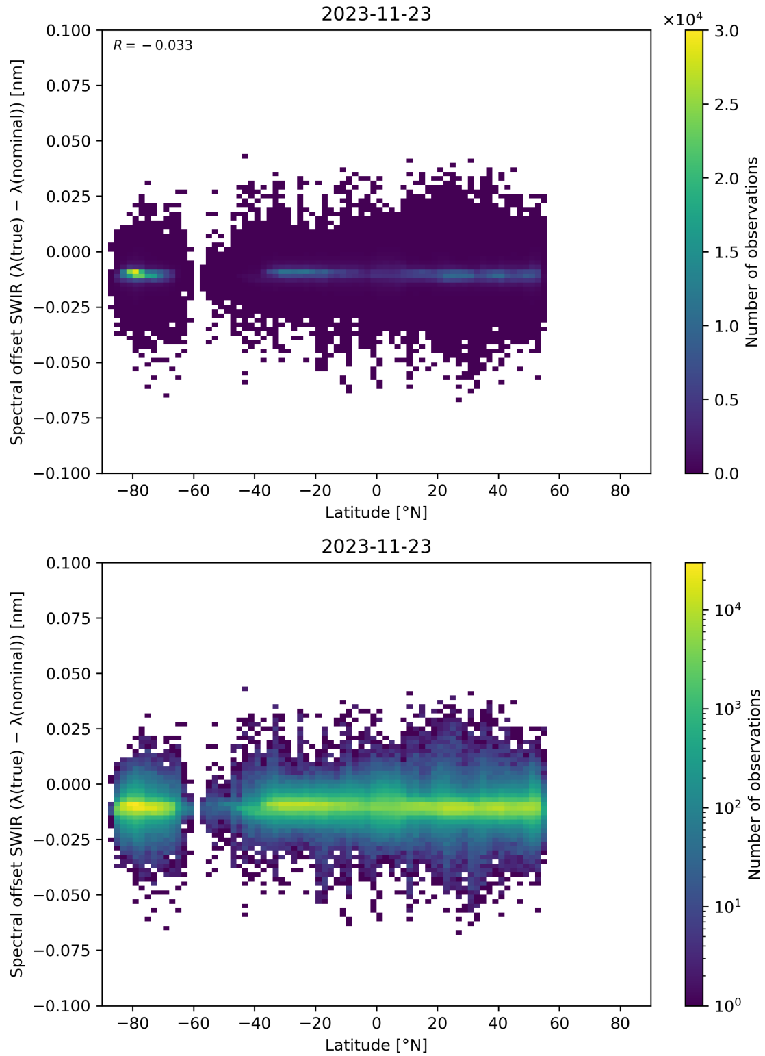
Figure 62: Scatter density plot of “Latitude” against “Spectral offset SWIR ( \lambda(\text{true}) - \lambda(\text{nominal}) )” for 2023-11-23 to 2023-11-24.
