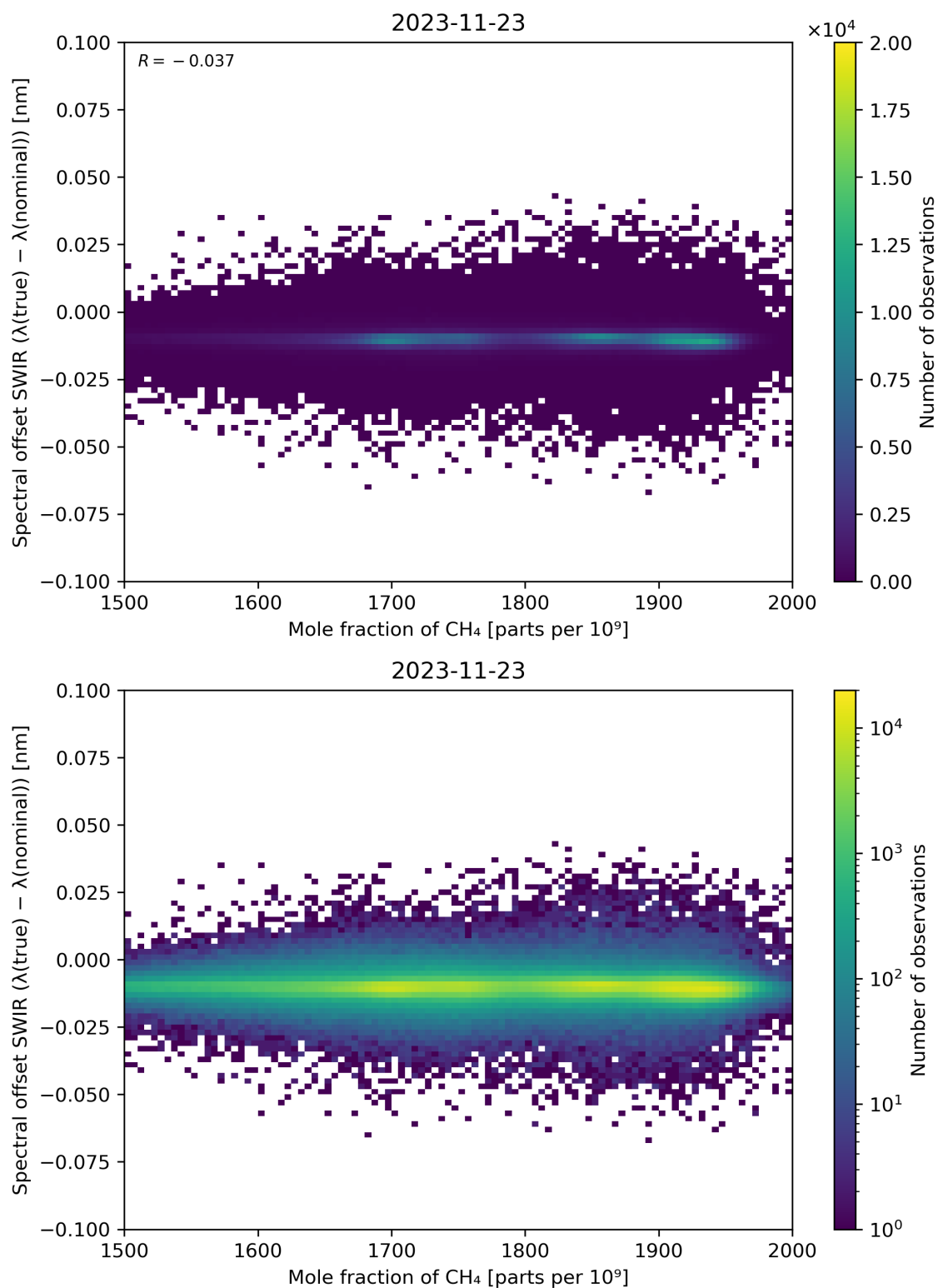
Figure 86: Scatter density plot of “Mole fraction of CH 4 ” against “Spectral offset SWIR ( \lambda(\text{true}) - \lambda(\text{nominal}) )” for 2023-11-23 to 2023-11-24.
