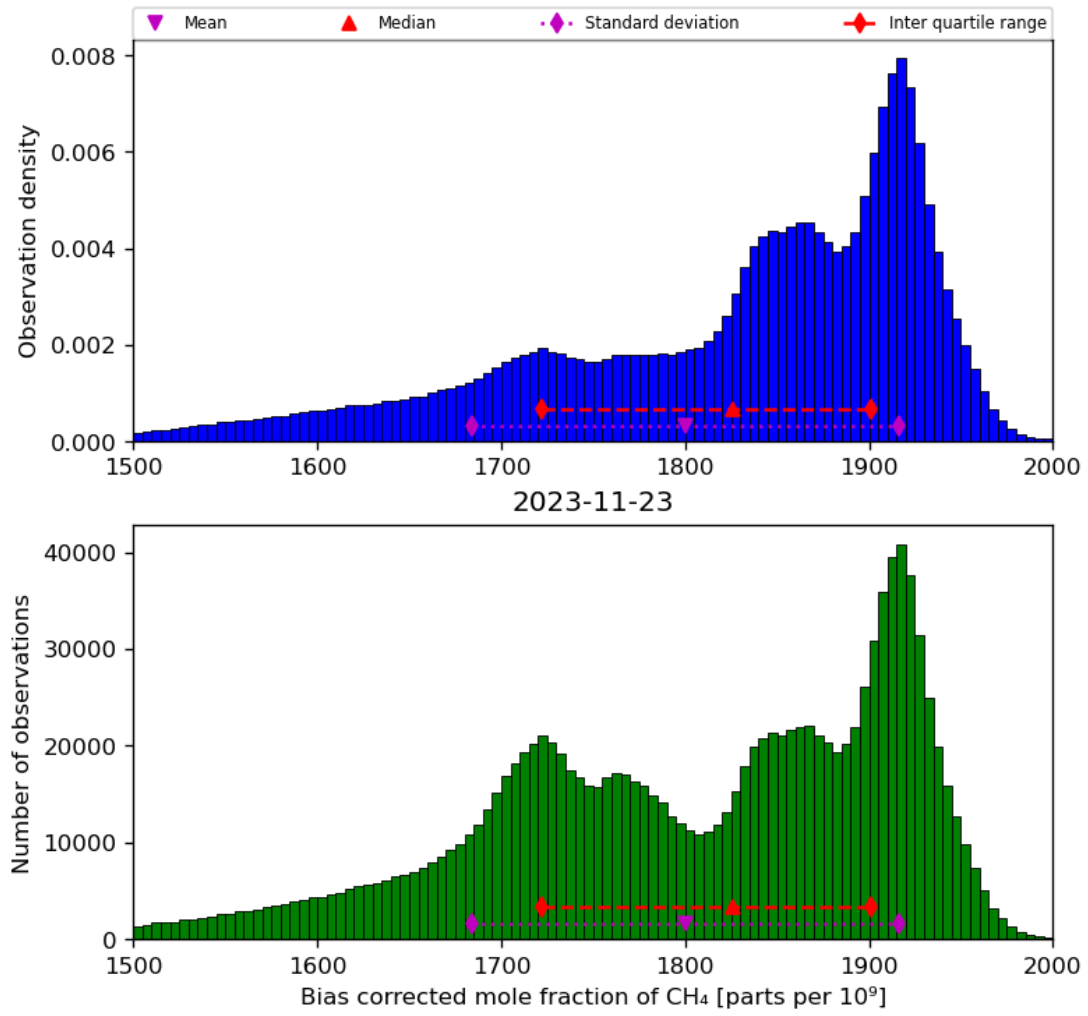
Figure 25: Histogram of “Bias corrected mole fraction of CH 4 ” for 2023-11-23 to 2023-11-24
