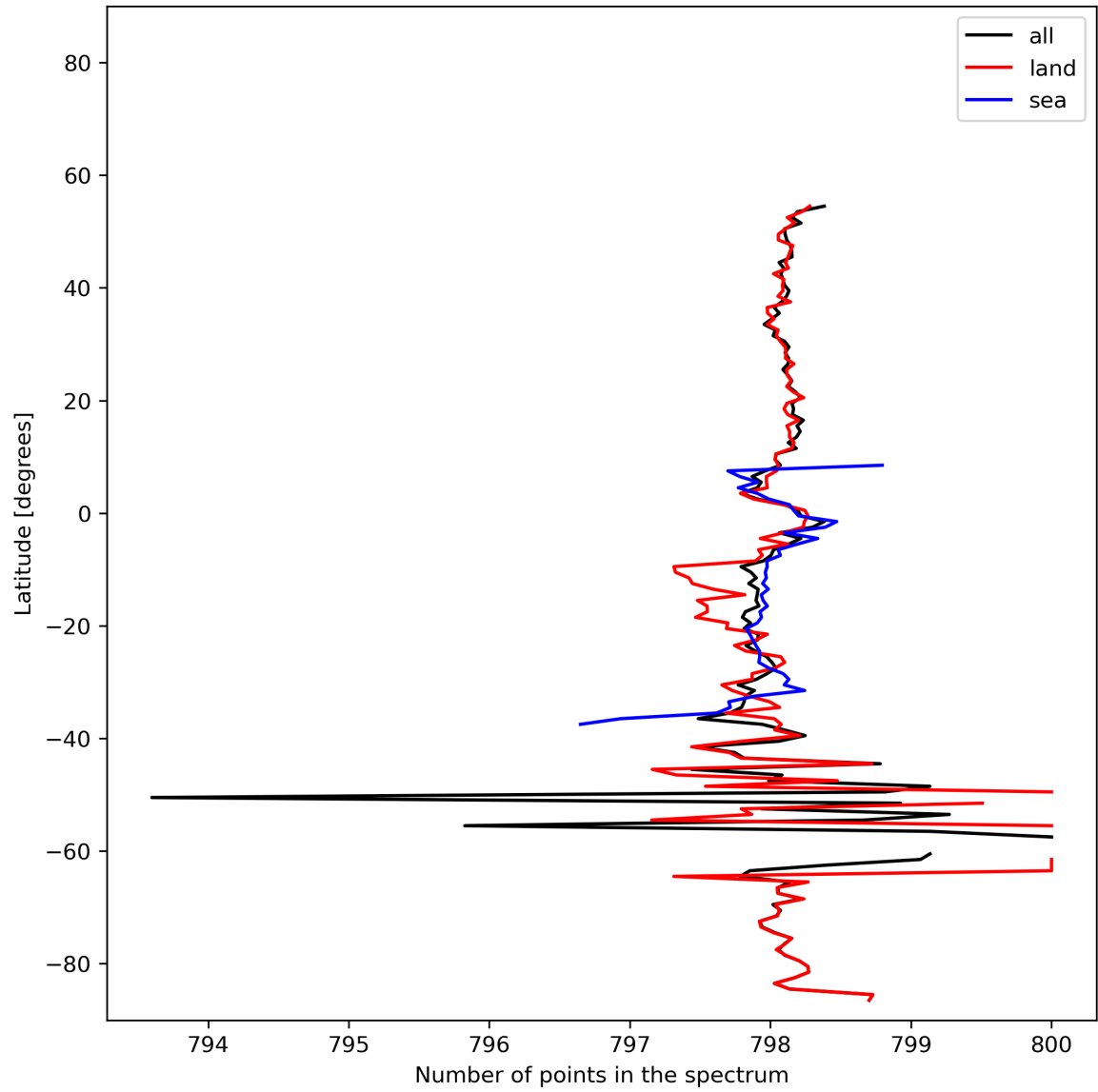
Figure 15: Zonal average of “Number of points in the spectrum” for 2023-11-23 to 2023-11-24.
