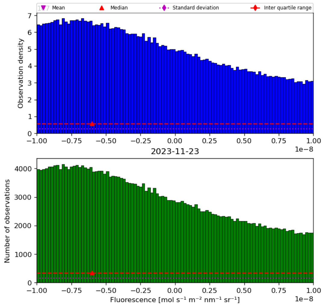
Figure 32: Histogram of “Fluorescence” for 2023-11-23 to 2023-11-24
