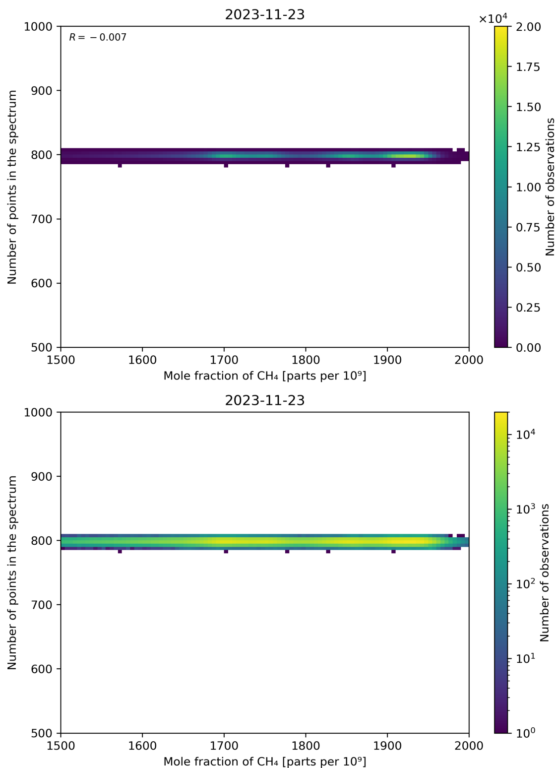
Figure 77: Scatter density plot of “Mole fraction of CH 4 ” against “Number of points in the spectrum” for 2023-11-23 to 2023-11-24.
