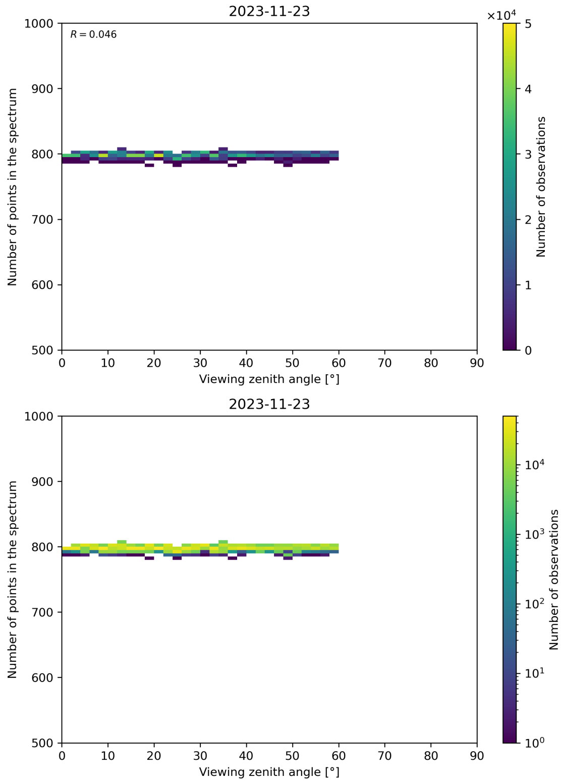
Figure 114: Scatter density plot of “Viewing zenith angle” against “Number of points in the spectrum” for 2023-11-23 to 2023-11-24.
