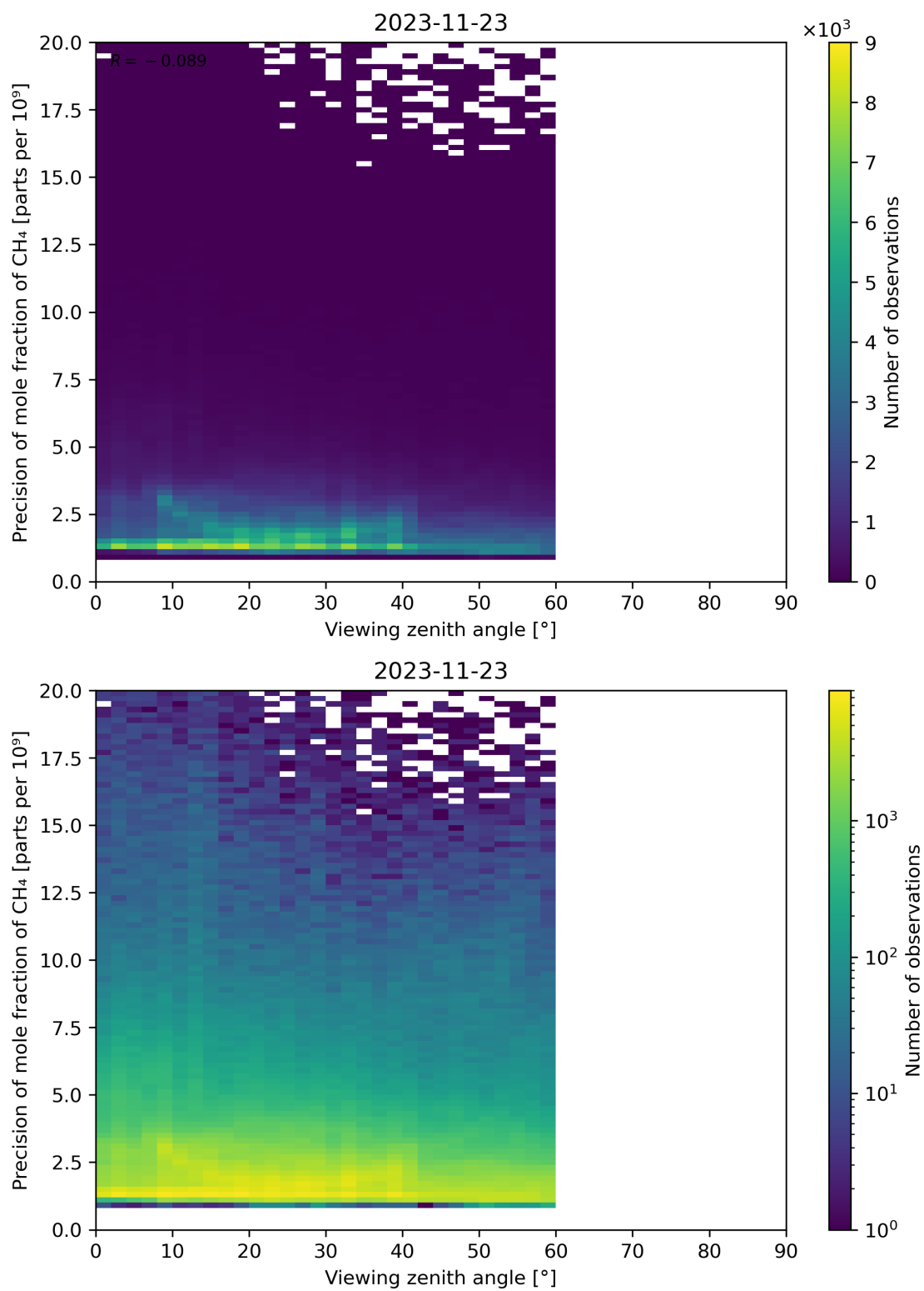
Figure 112: Scatter density plot of “Viewing zenith angle” against “Precision of mole fraction of CH 4 ” for 2023-11-23 to 2023-11-24.
