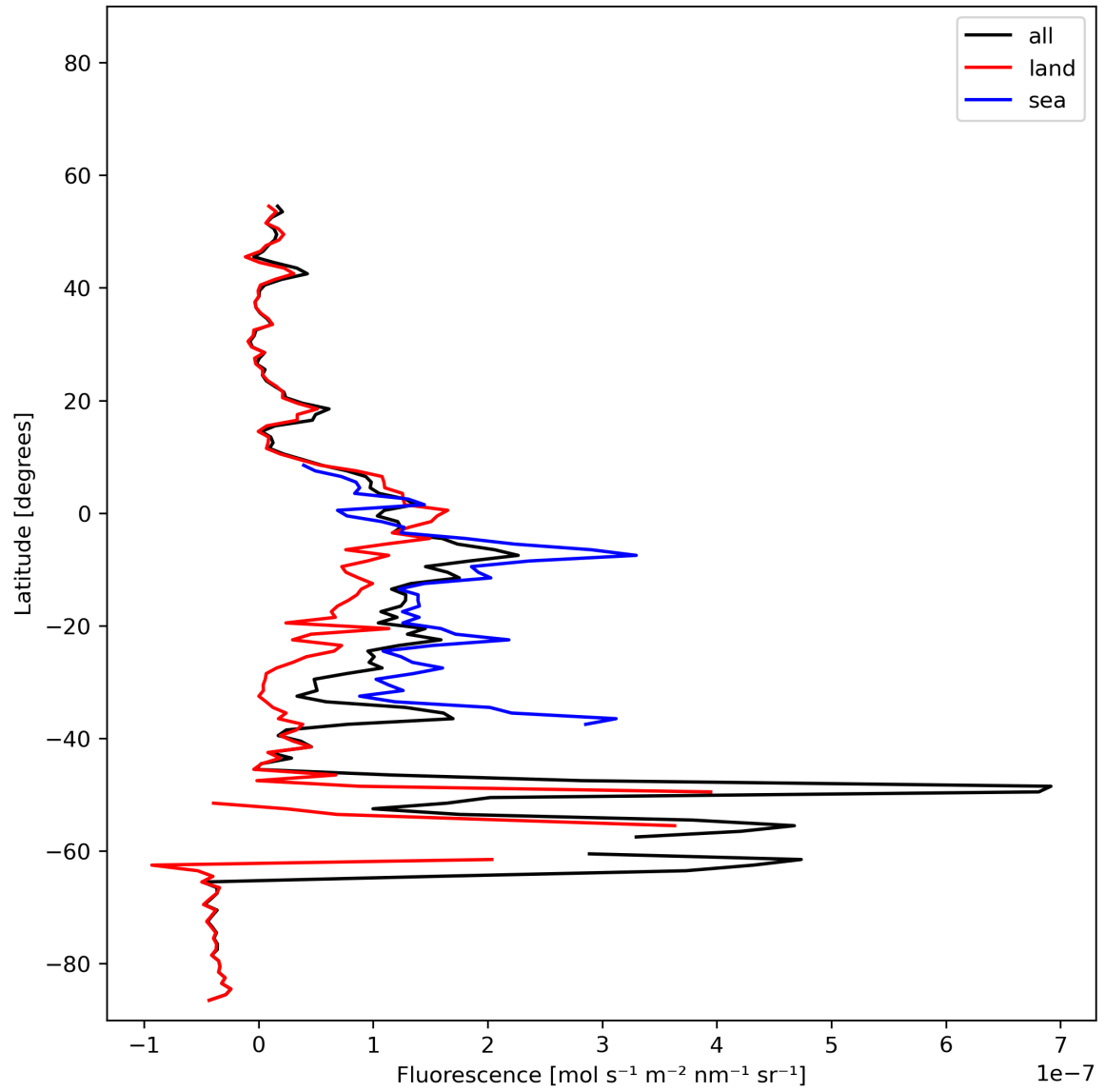
Figure 21: Zonal average of “Fluorescence” for 2023-11-23 to 2023-11-24.
