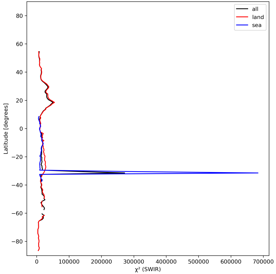
Figure 17: Zonal average of “ \chi^2 (SWIR)” for 2023-11-23 to 2023-11-24.
