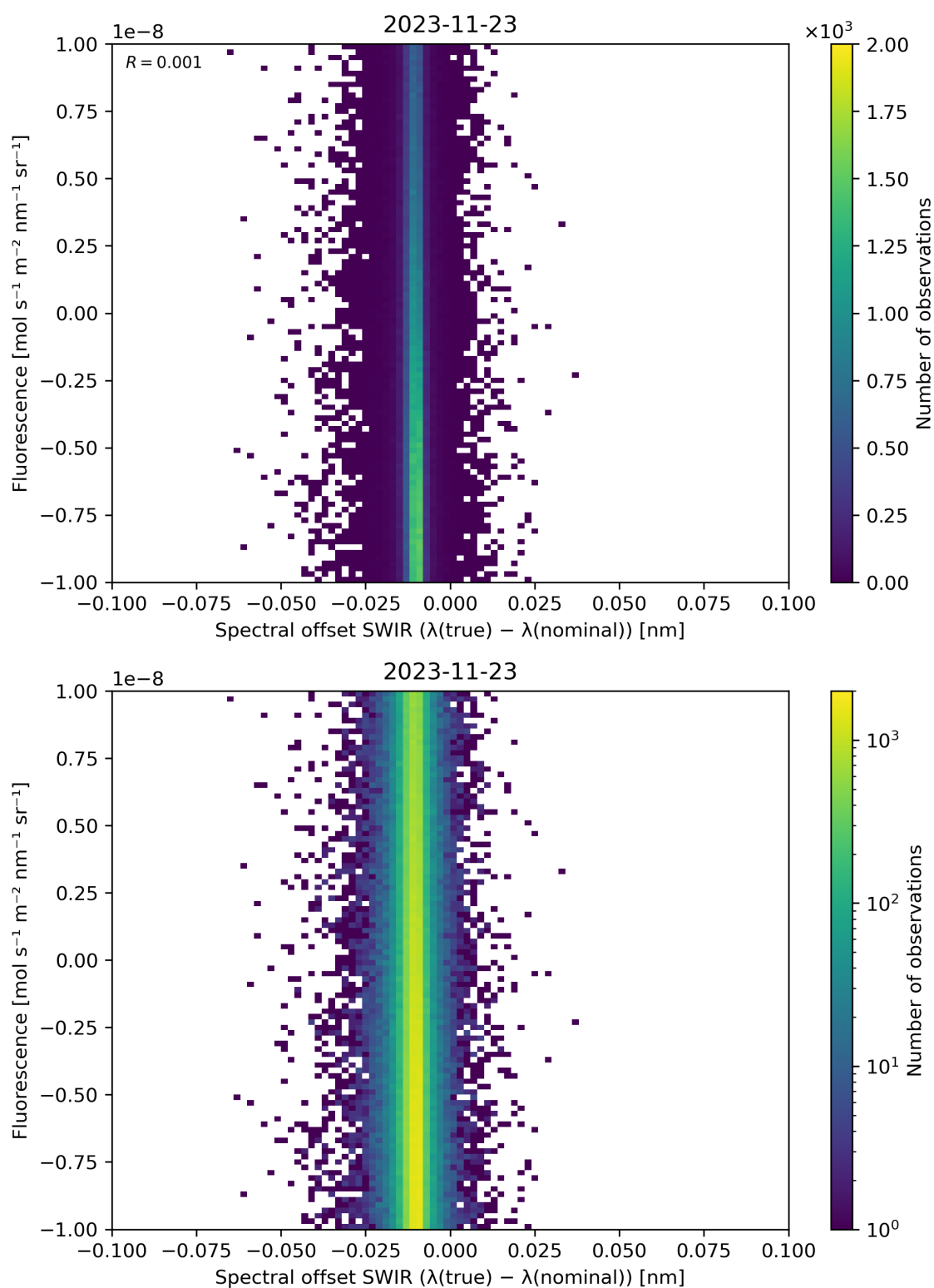
Figure 120: Scatter density plot of “Spectral offset SWIR ( \lambda(\text{true}) - \lambda(\text{nominal}) )” against “Fluorescence” for 2023-11-23 to 2023-11-24.
