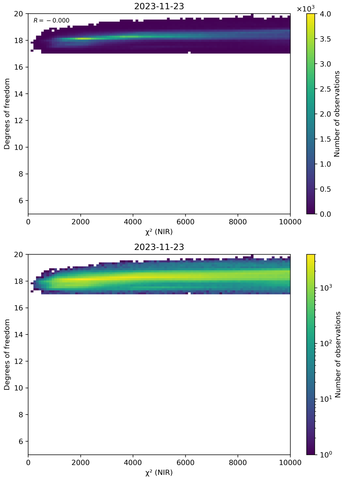
Figure 44: Scatter density plot of “ \chi^2 (NIR)” against “Degrees of freedom” for 2023-11-23 to 2023-11-24.
