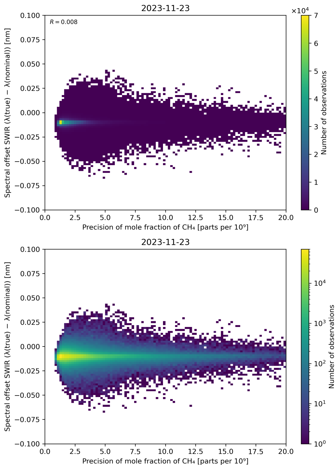
Figure 85: Scatter density plot of “Precision of mole fraction of CH 4 ” against “Spectral offset SWIR ( \lambda(\text{true}) - \lambda(\text{nominal}) )” for 2023-11-23 to 2023-11-24.
