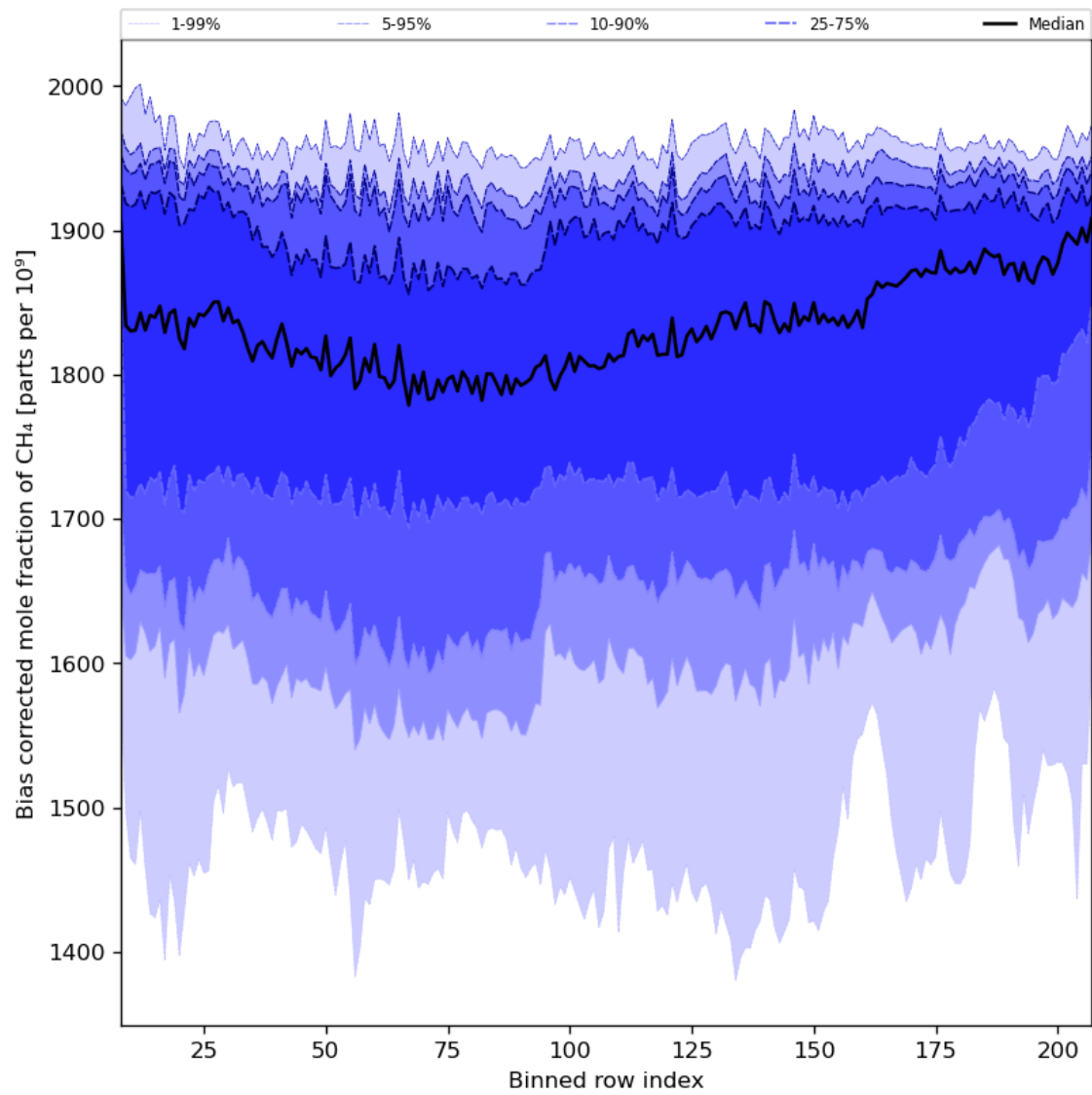
Figure 36: Along track statistics of “Bias corrected mole fraction of CH 4 ” for 2023-11-23 to 2023-11-24
