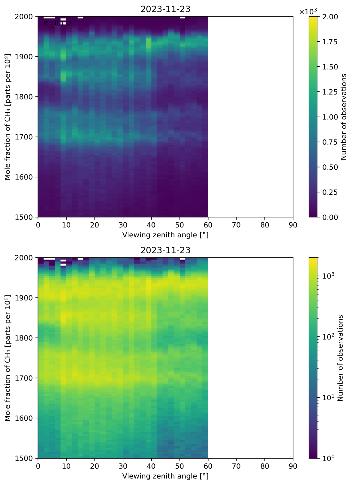
Figure 110: Scatter density plot of “Viewing zenith angle” against “Mole fraction of CH 4 ” for 2023-11-23 to 2023-11-24.
