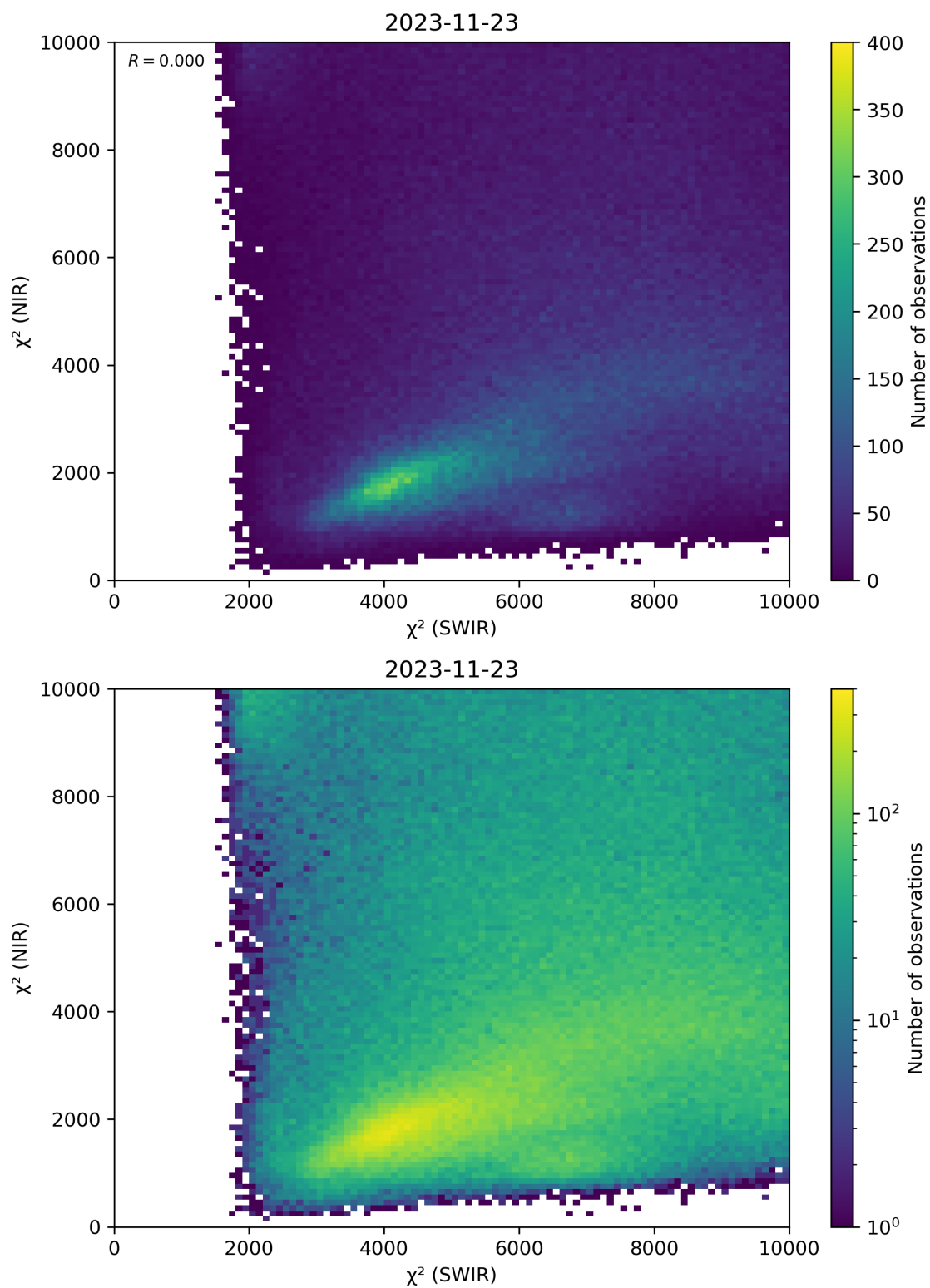
Figure 47: Scatter density plot of “ \chi^2 (SWIR)” against “ \chi^2 (NIR)” for 2023-11-23 to 2023-11-24.
