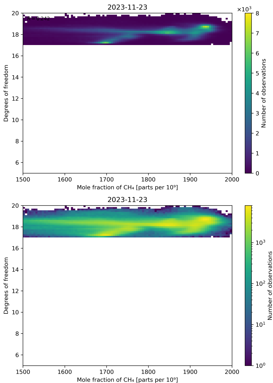
Figure 72: Scatter density plot of “Mole fraction of CH 4 ” against “Degrees of freedom” for 2023-11-23 to 2023-11-24.
