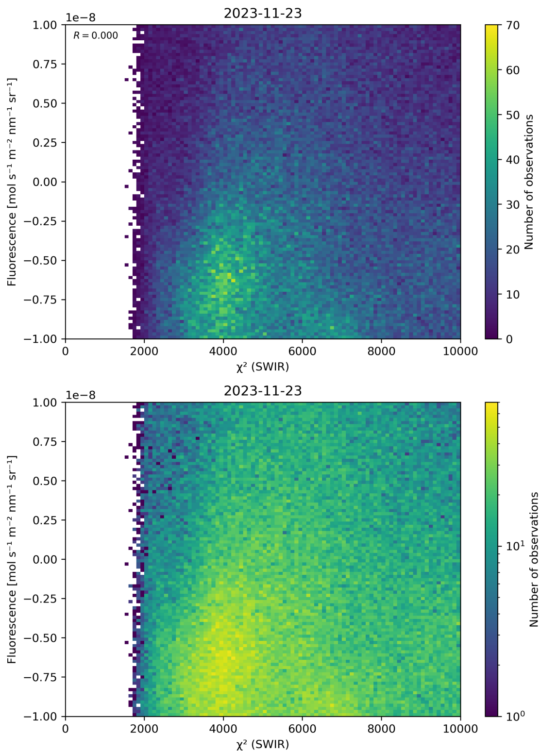
Figure 49: Scatter density plot of “ \chi^2 (SWIR)” against “Fluorescence” for 2023-11-23 to 2023-11-24.
